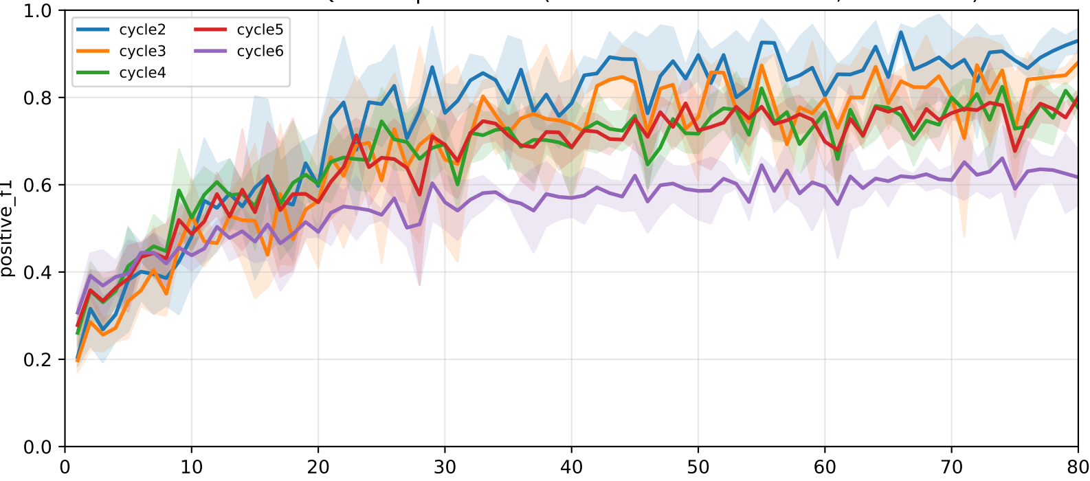
Pooled APPLE-QOracle positive F1 (after-local selected model, rounds=80)
