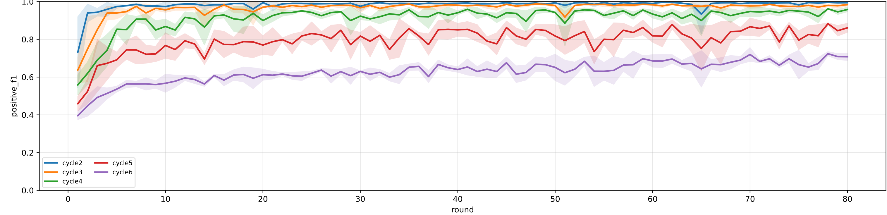
FedAvg pooled positive F1 (post-aggregation)
