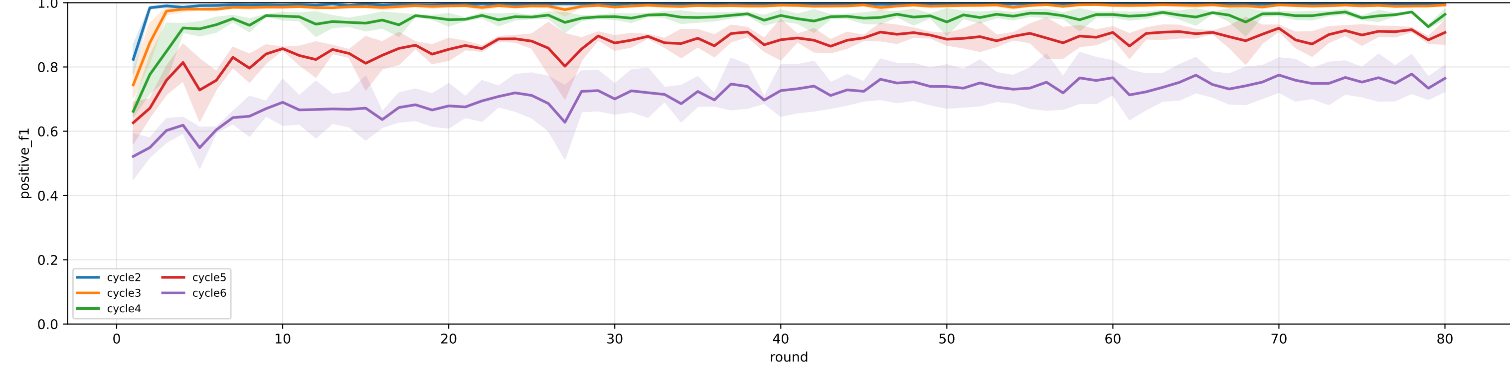
FedProx pooled positive F1 (post-aggregation)
