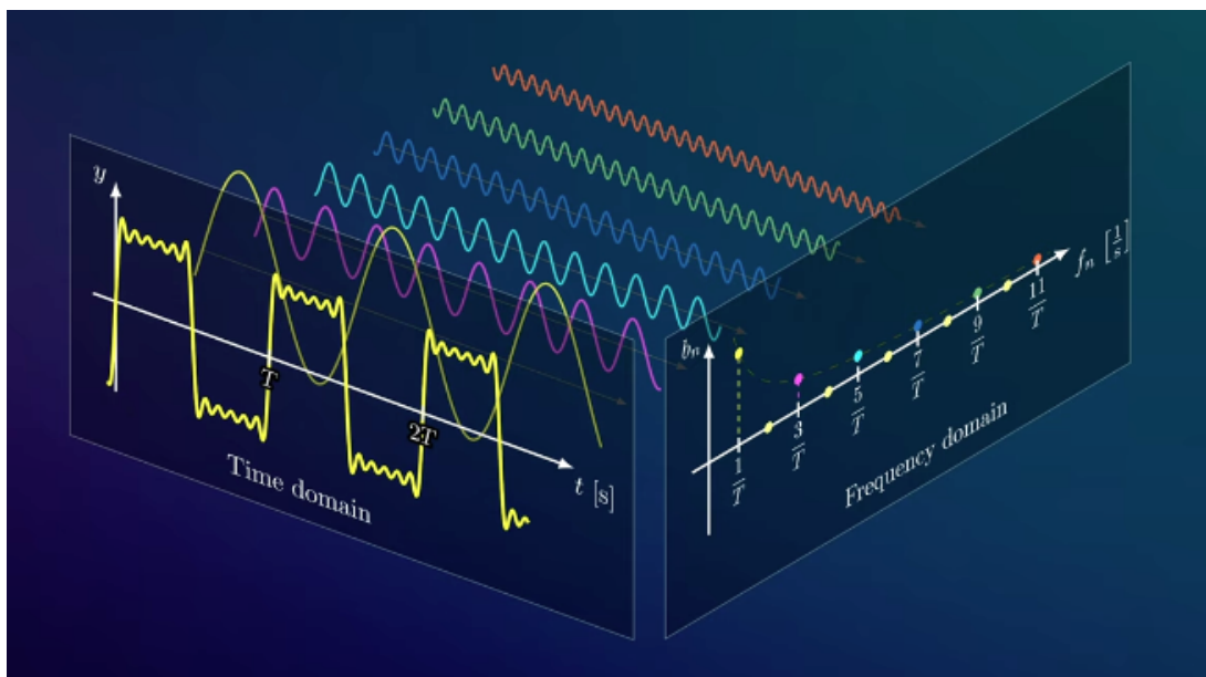
Figure 1: Fourier Transform of a rectangular signal.
