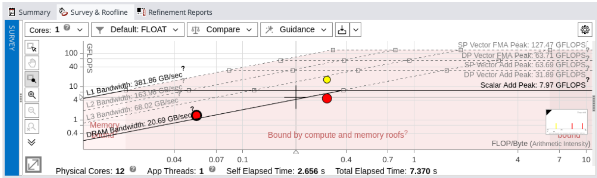
Figure 2: Roofline Analysis - baseline compilation.
