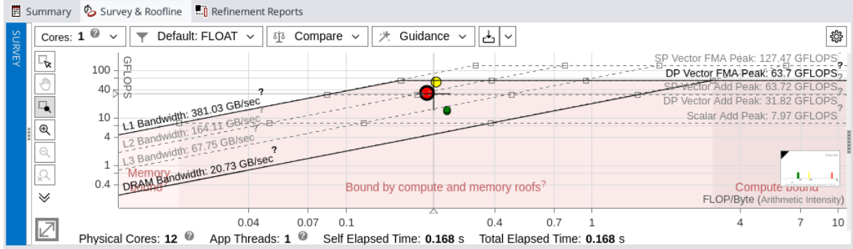
Figure 4: Roofline Analysis - best-optimized compilation.
