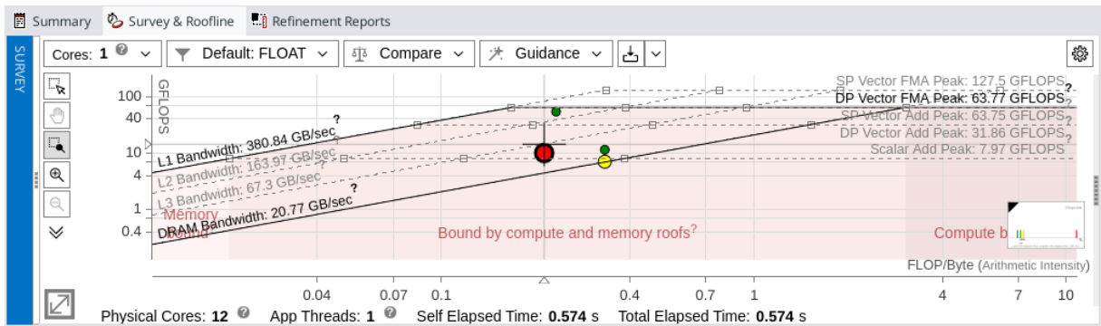
Figure 3: Roofline Analysis - basic optimization.
