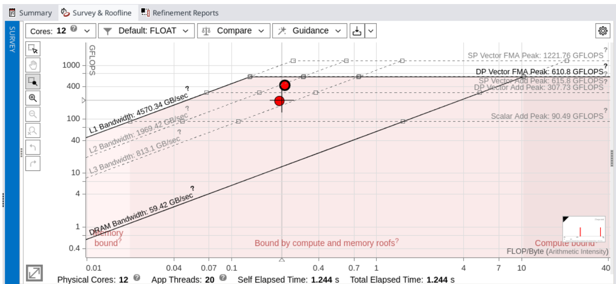
Figure 5: Roofline Analysis - parallelized and optimized code.
