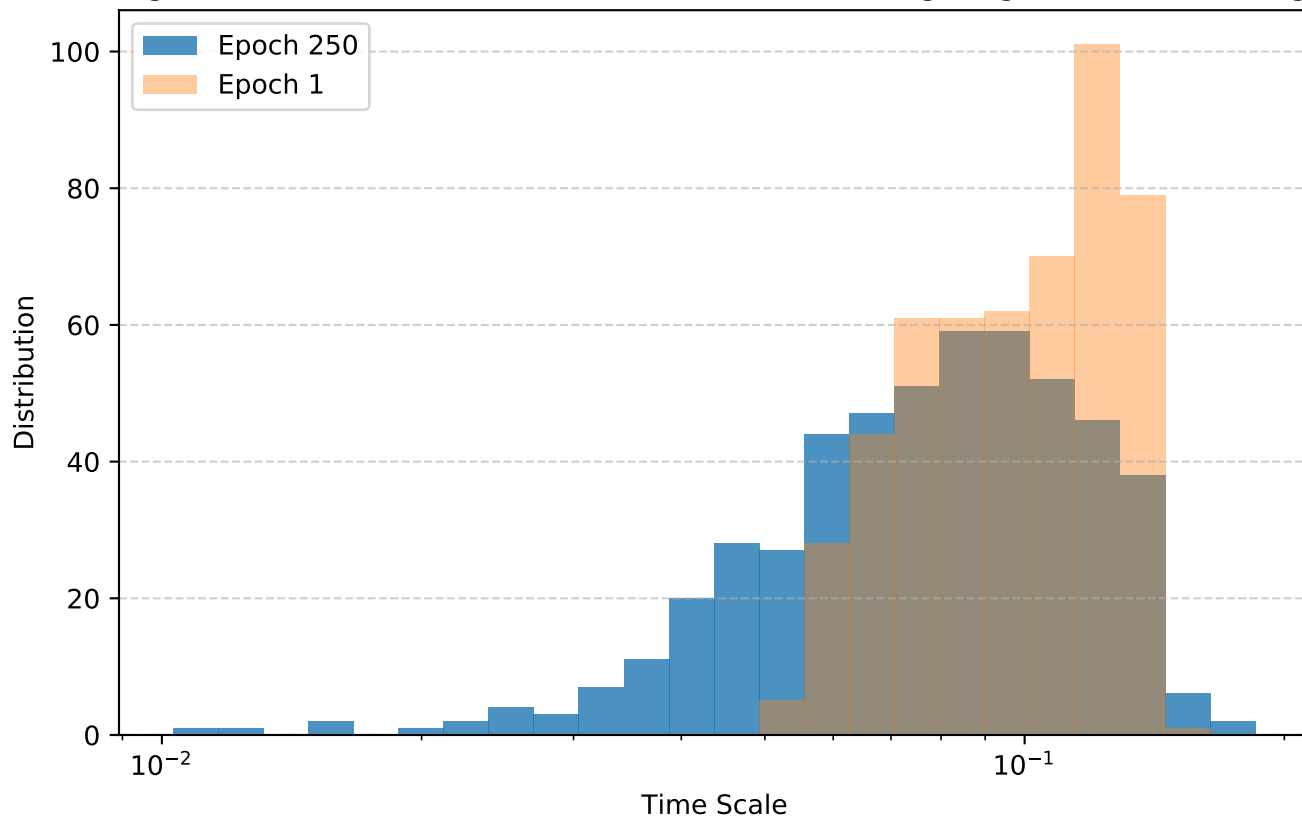
Log Distributions of Characteristic Time Scales (begining vs end of training)
