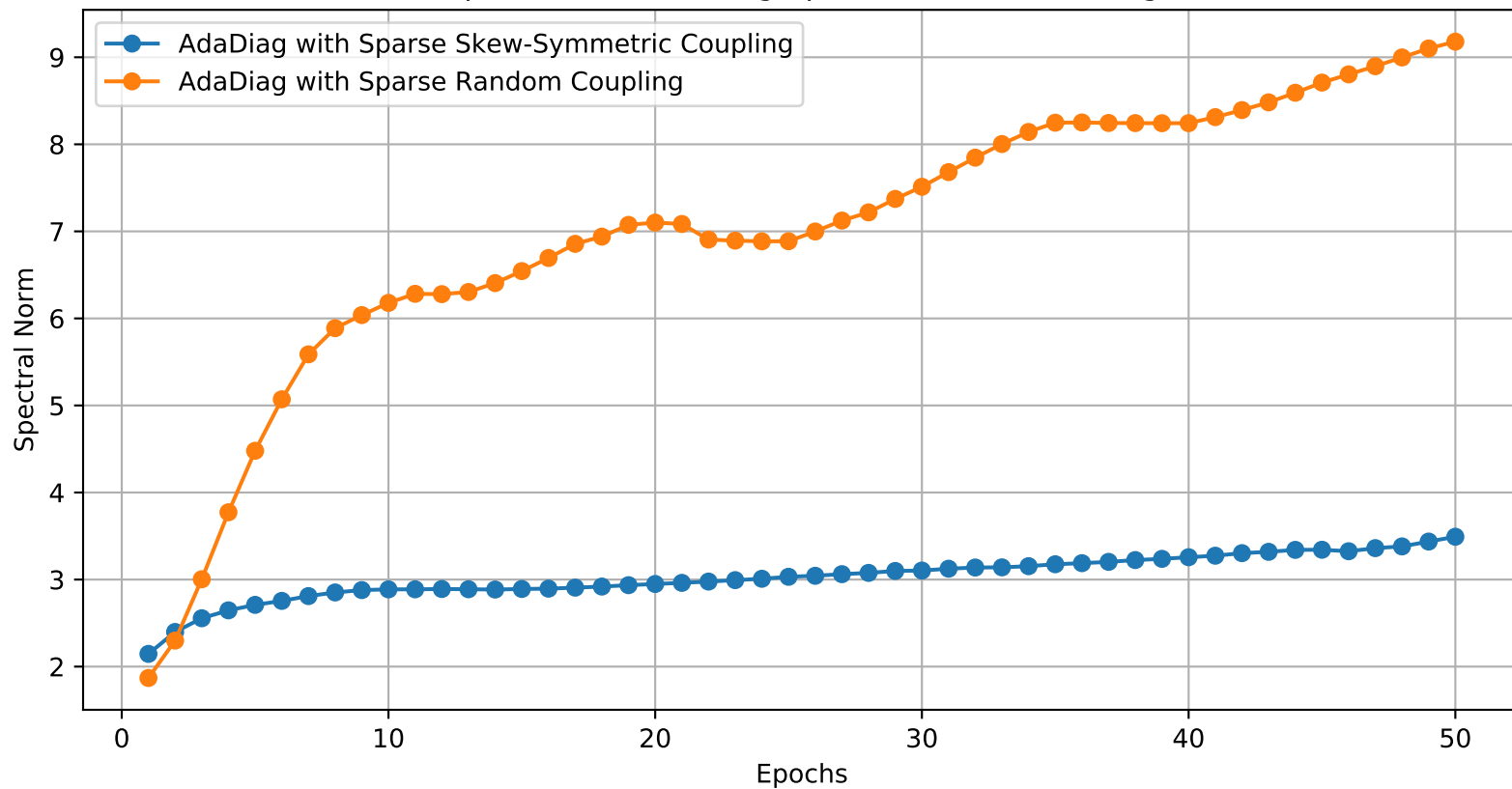
Spectral Norm during epochs of Adiac training
