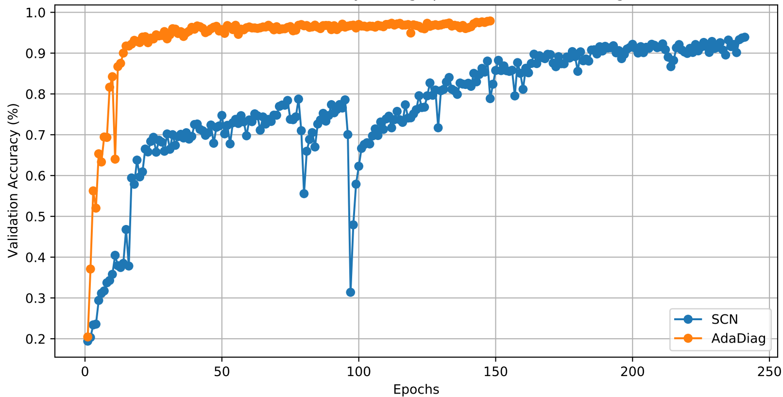
Validation Accuracy during epochs of sMNIST training
