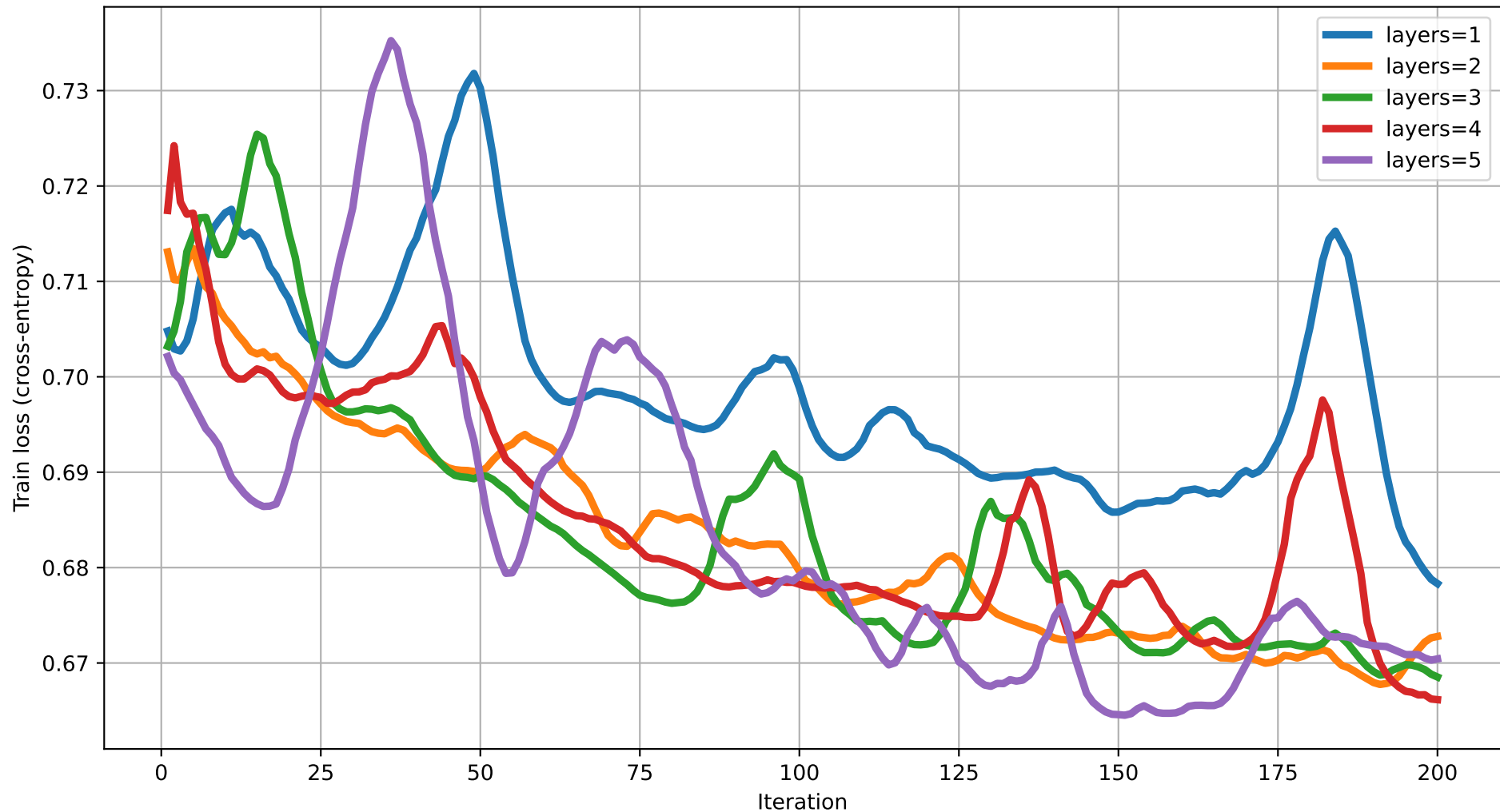
Train loss vs Iteration (dim=14) rot=RY, ent=ring, gate=CZ
