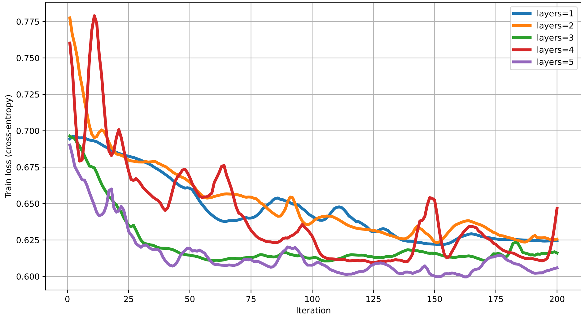
Train loss vs Iteration (dim=17) rot=Rot, ent=chain, gate=IsingXX
