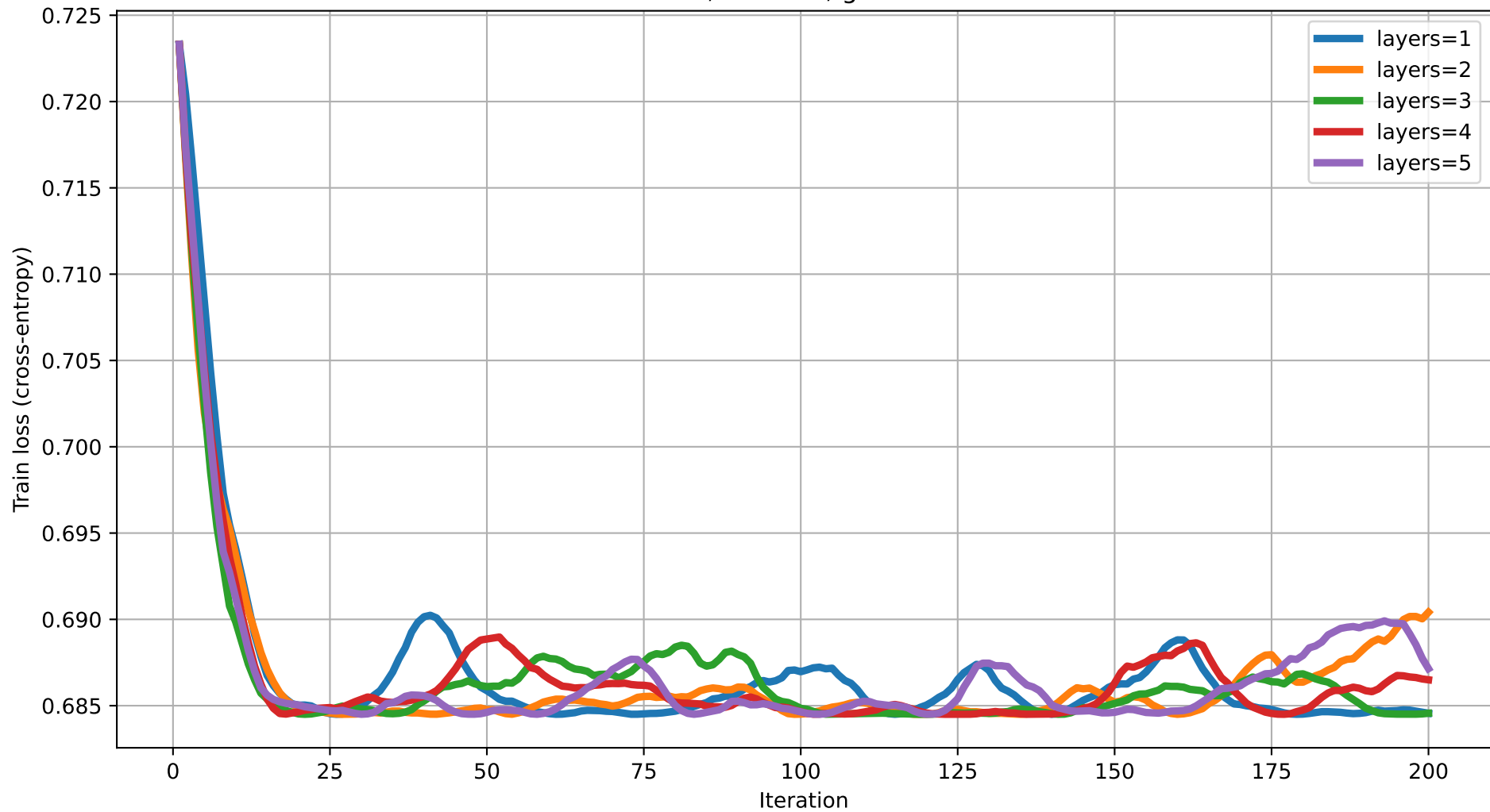
Train loss vs Iteration (degree=3) rot=RZ, ent=full, gate=CNOT
