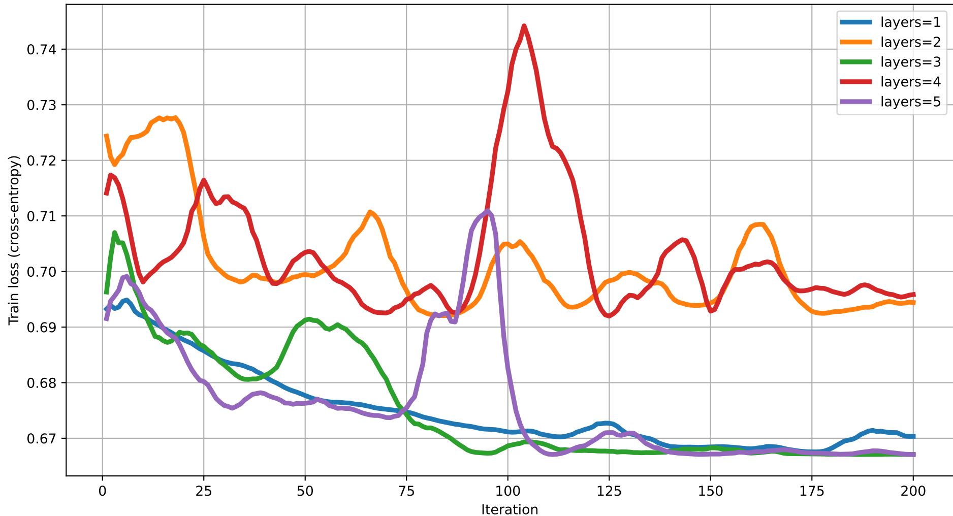
Train loss vs Iteration (dim=6) rot=RX, ent=chain, gate=IsingXX
