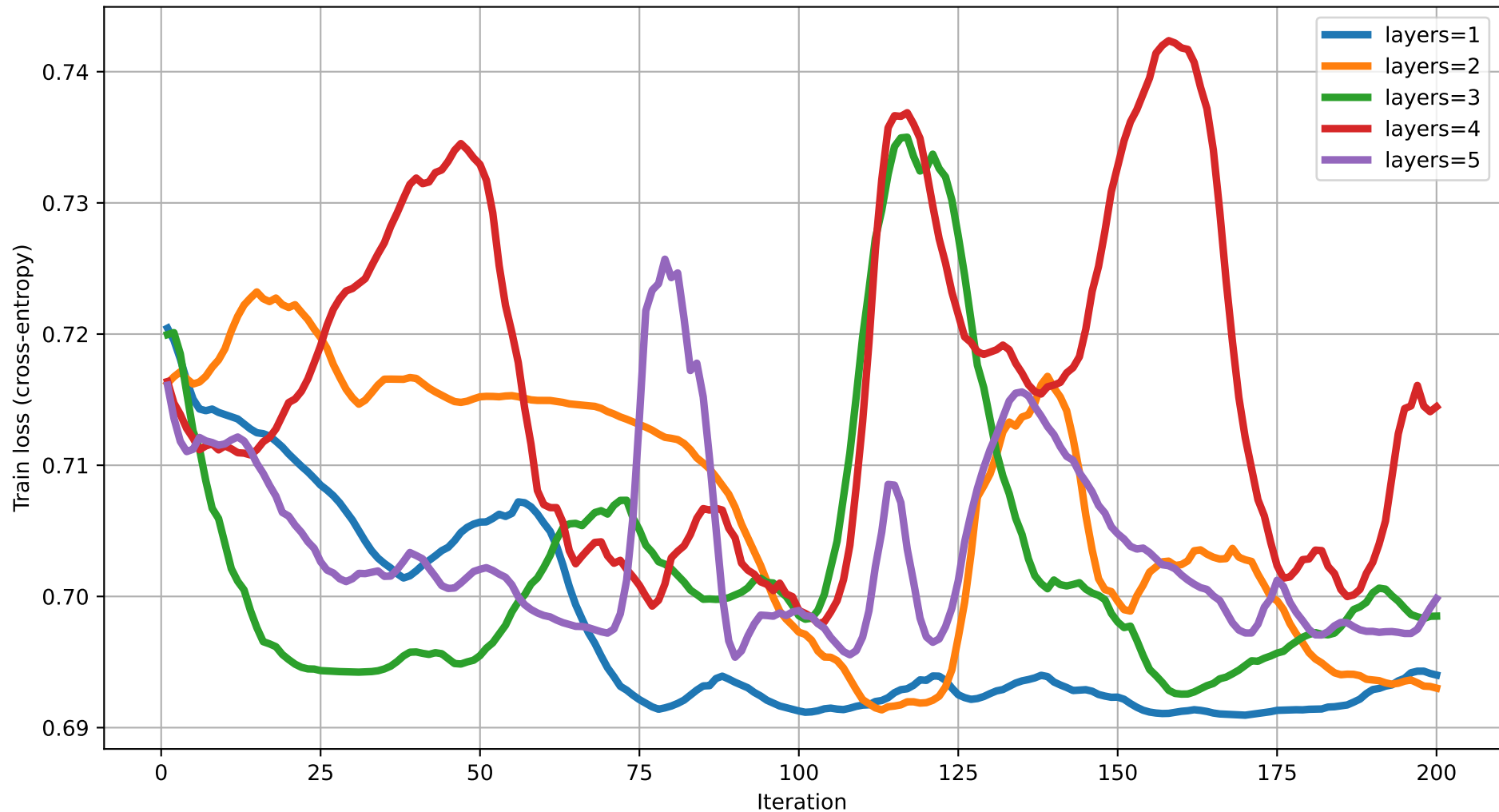
Train loss vs Iteration (dim=3) rot=RX, ent=full, gate=CNOT
