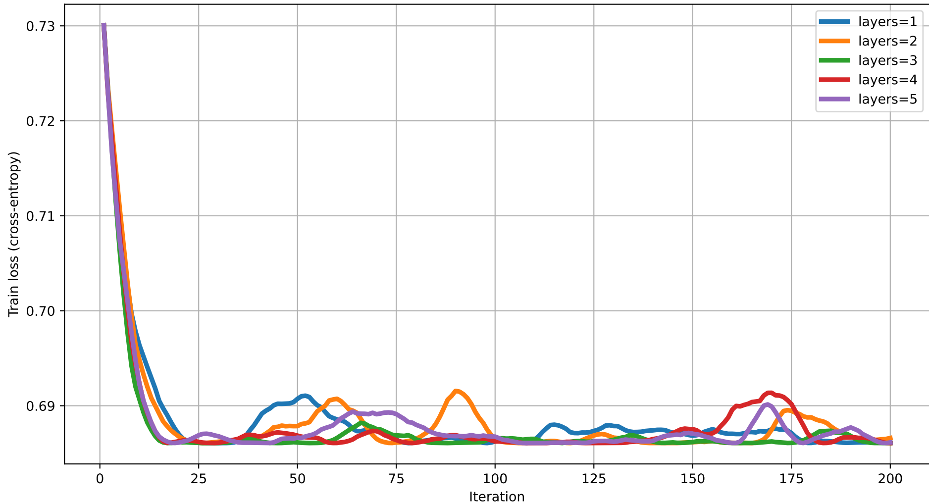
Train loss vs Iteration (degree=2) rot=RZ, ent=ring, gate=CZ
