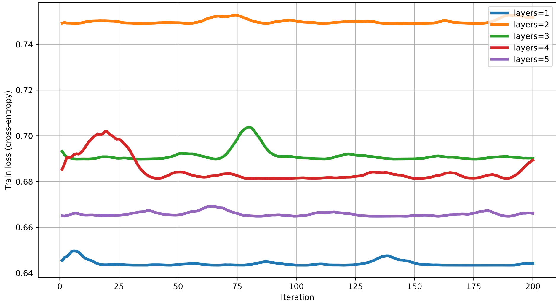
Train loss vs Iteration (degree=3) rot=RZ, ent=ring, gate=CNOT
