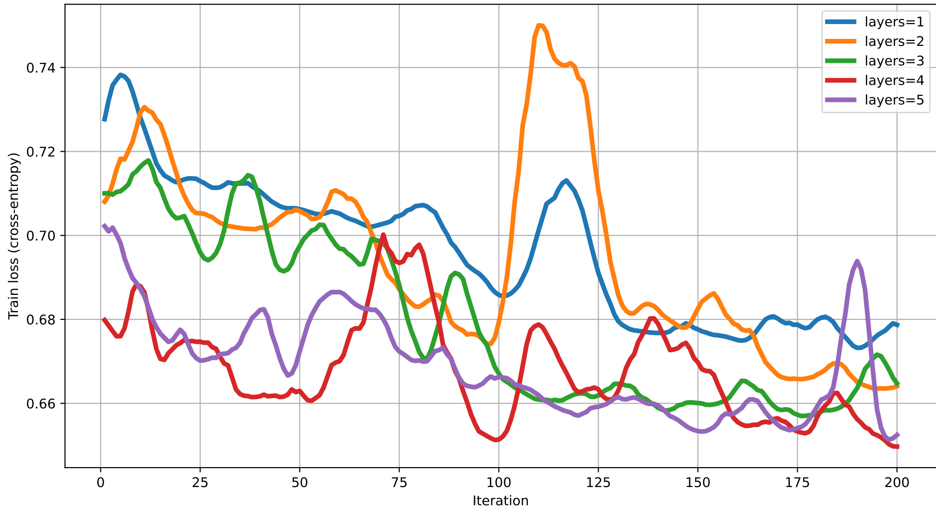
Train loss vs Iteration (dim=7) rot=RYZ, ent=ring, gate=CNOT
