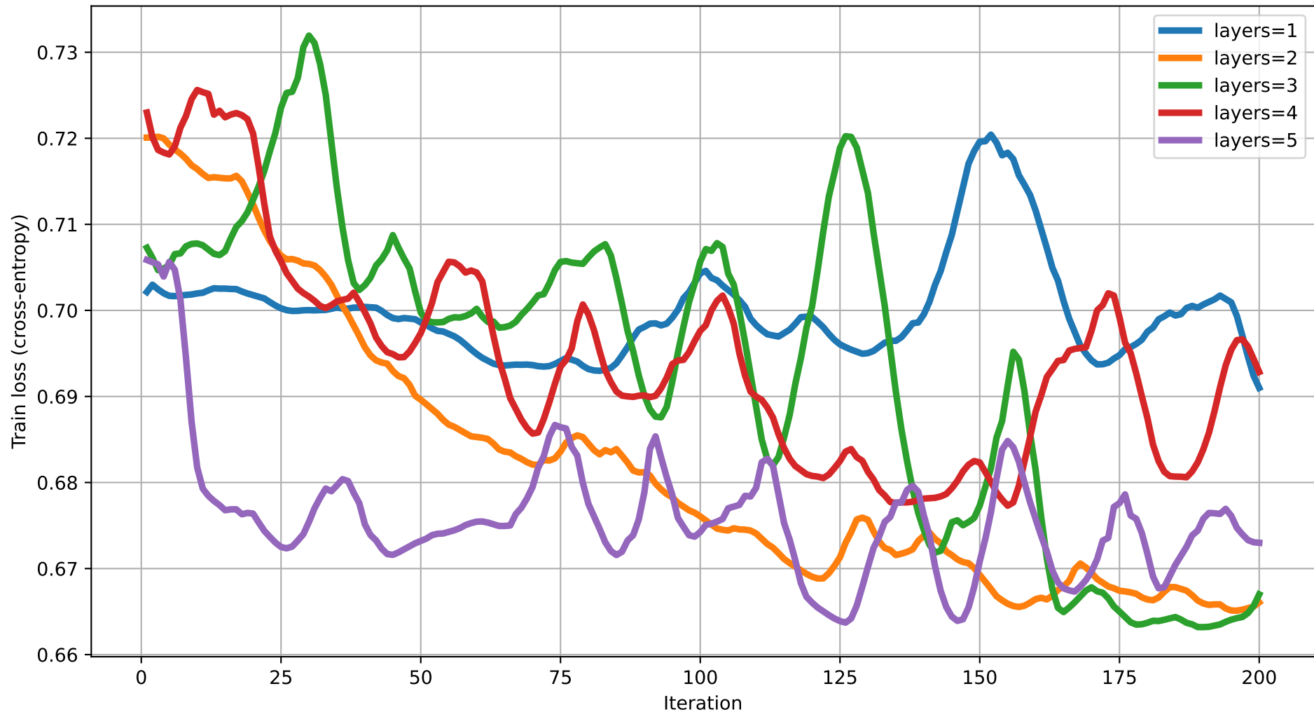
Train loss vs Iteration (dim=15) rot=RY, ent=ring, gate=CNOT
