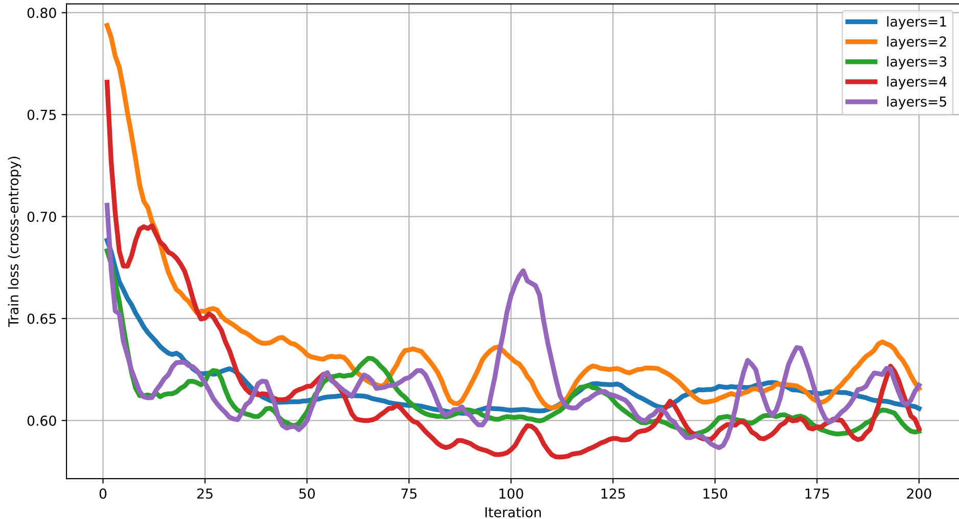
Train loss vs Iteration (dim=4) rot=Rot, ent=ring, gate=IsingXX
