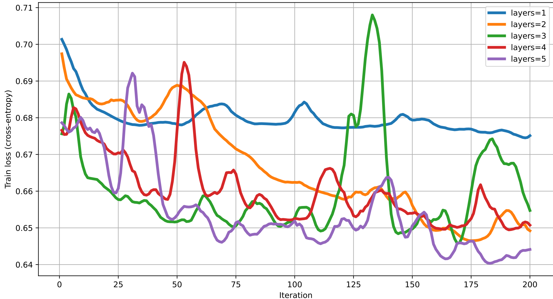
Train loss vs Iteration (dim=9) rot=RYZ, ent=ring, gate=CNOT
