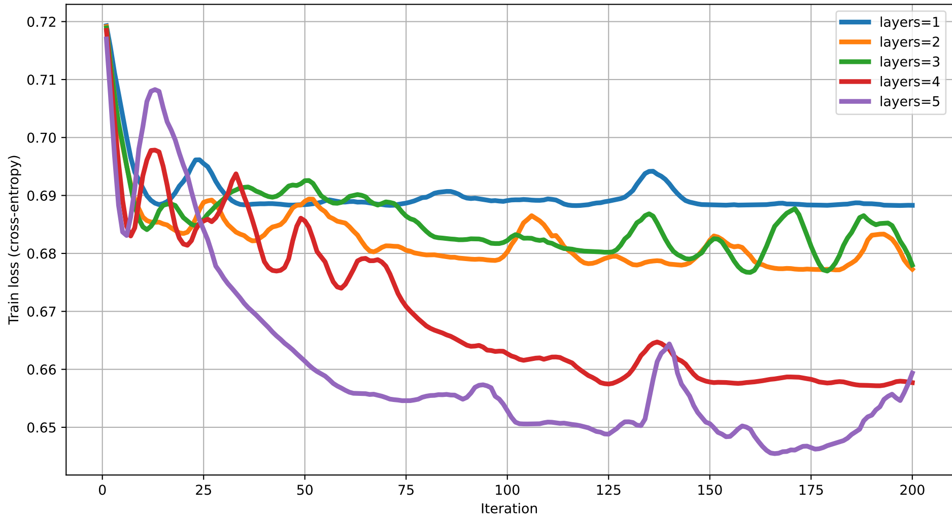
Train loss vs Iteration (degree=4) rot=RX, ent=chain, gate=CZ
