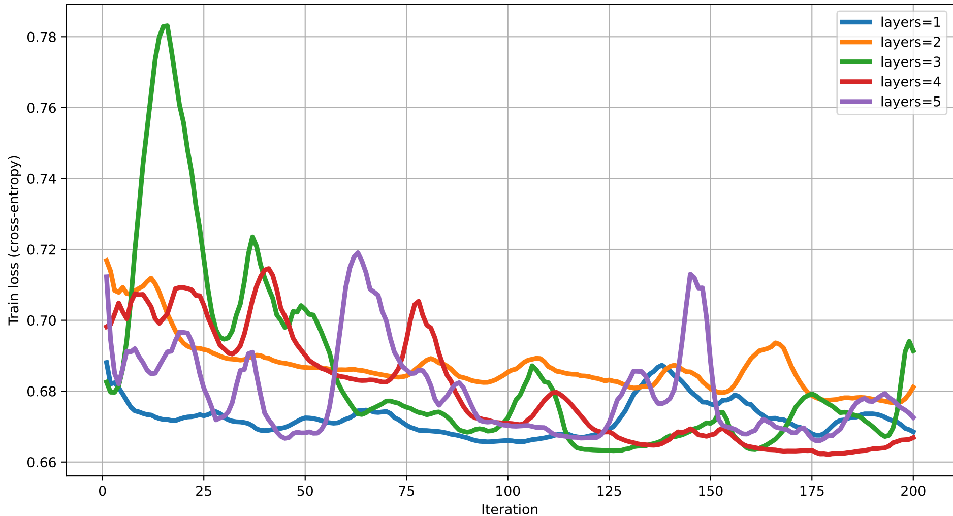
Train loss vs Iteration (dim=12) rot=RYZ, ent=ring, gate=IsingXX
