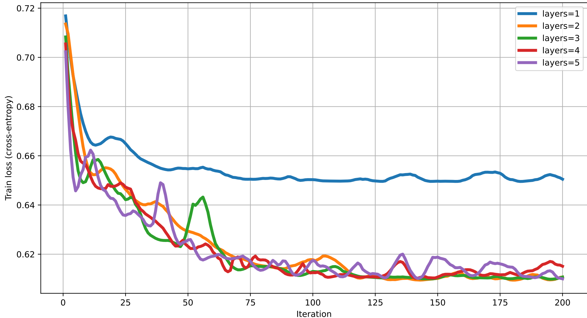
Train loss vs Iteration (degree=4) rot=Rot, ent=pairwise, gate=CZ
