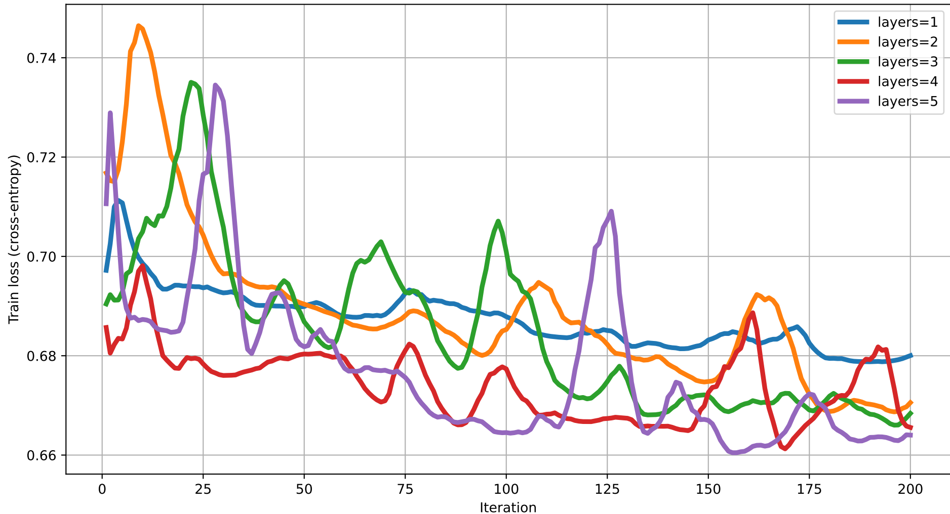
Train loss vs Iteration (dim=13) rot=RYZ, ent=chain, gate=IsingXX
