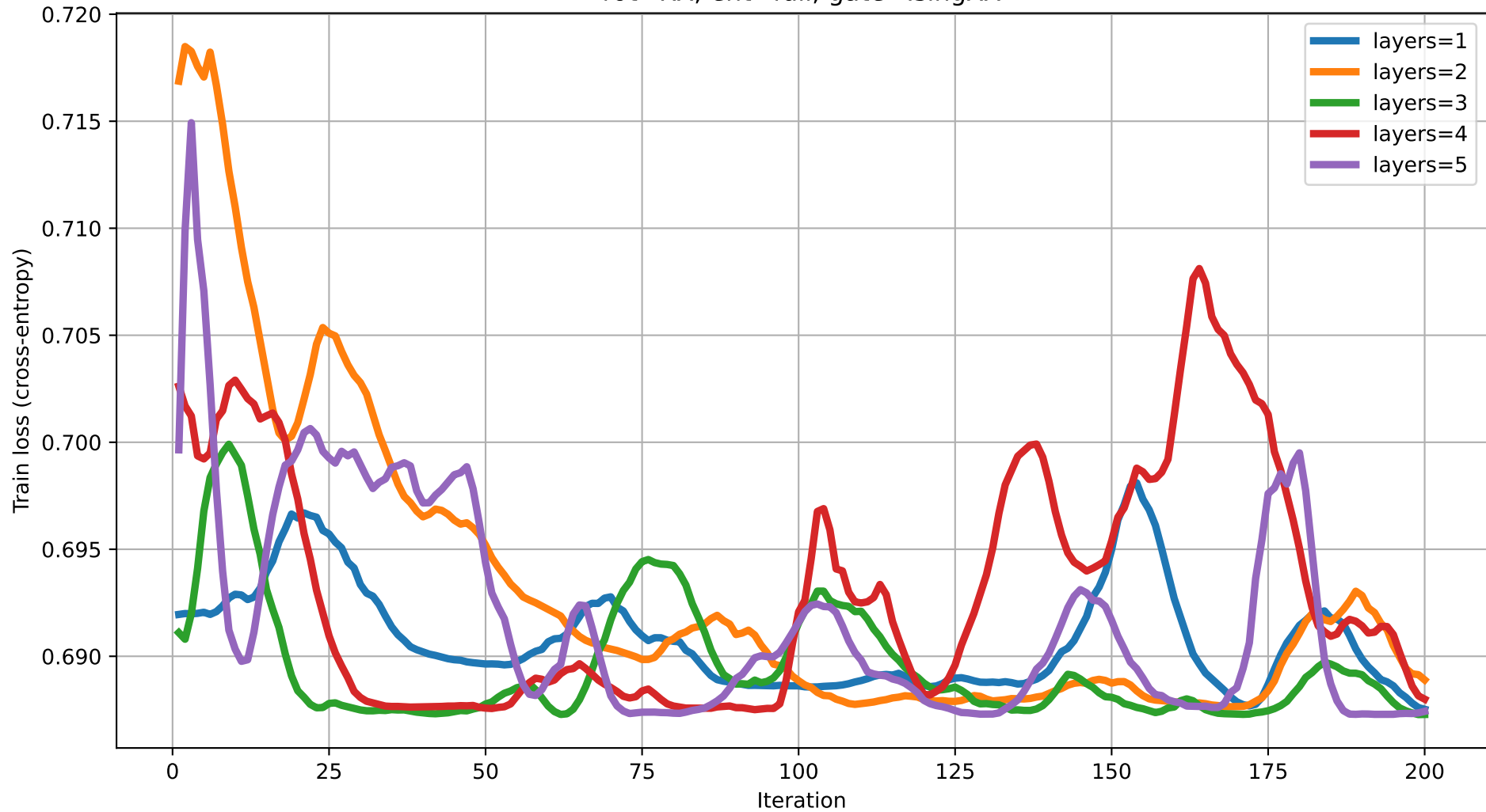
Train loss vs Iteration (dim=13) rot=RX, ent=full, gate=IsingXX
