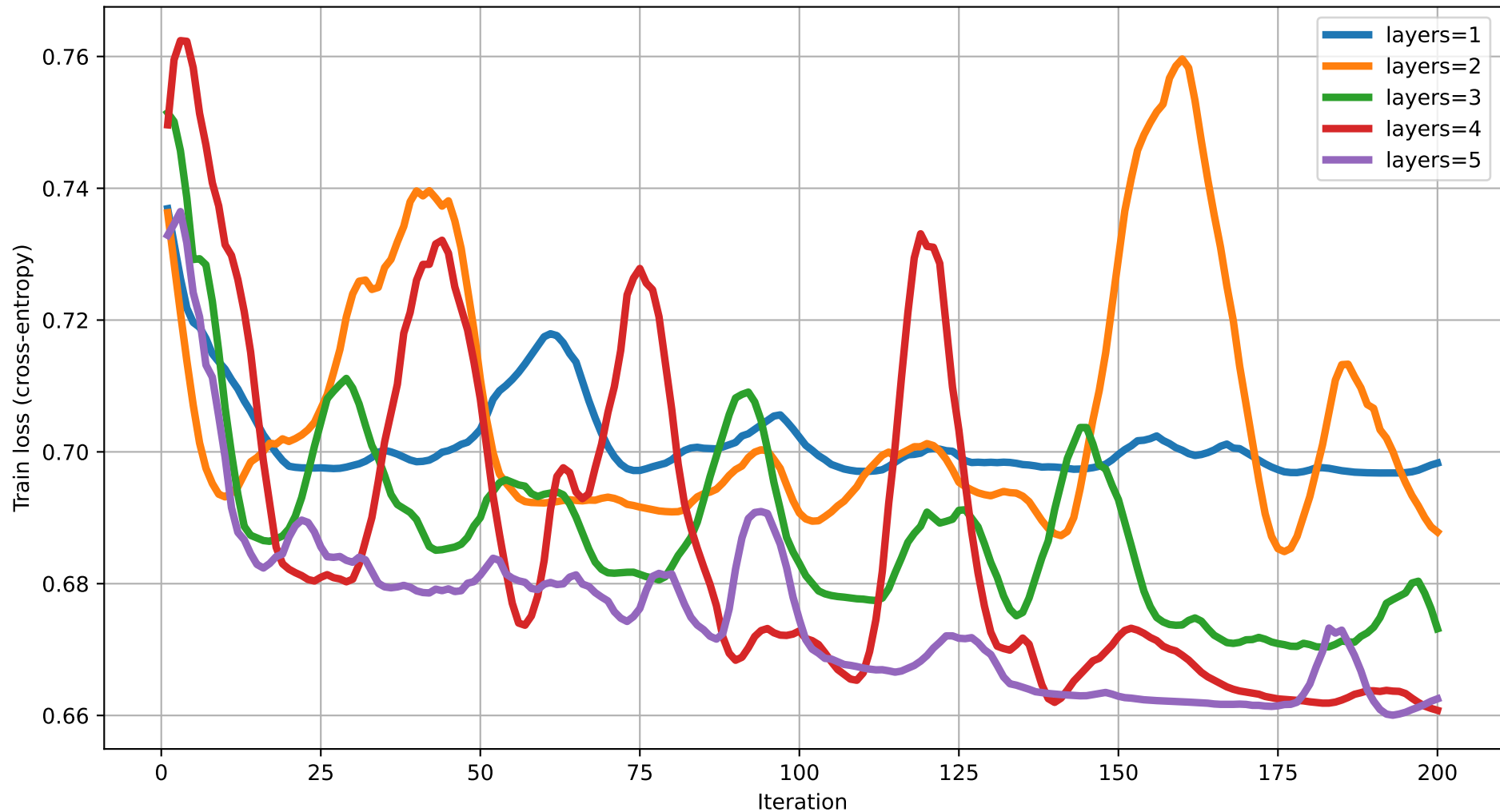
Train loss vs Iteration (dim=18) rot=RX, ent=chain, gate=CNOT
