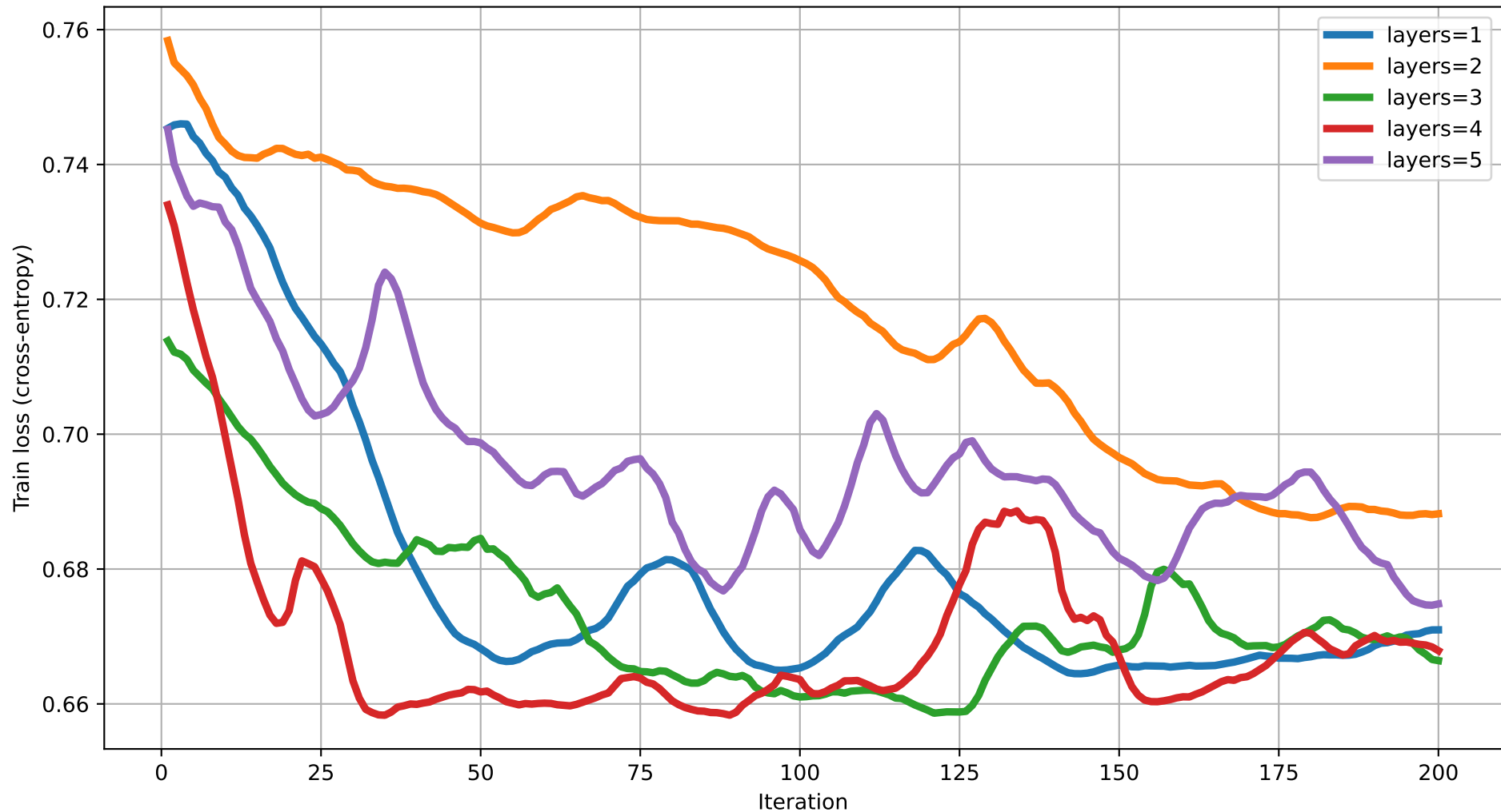
Train loss vs Iteration (dim=3) rot=RYZ, ent=ring, gate=CNOT
