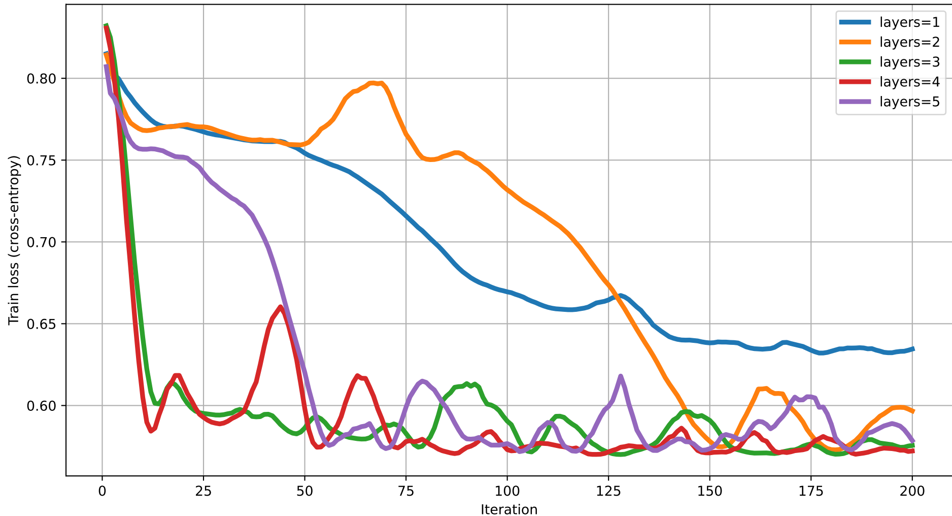
Train loss vs Iteration (dim=2) rot=RY, ent=chain, gate=CNOT
