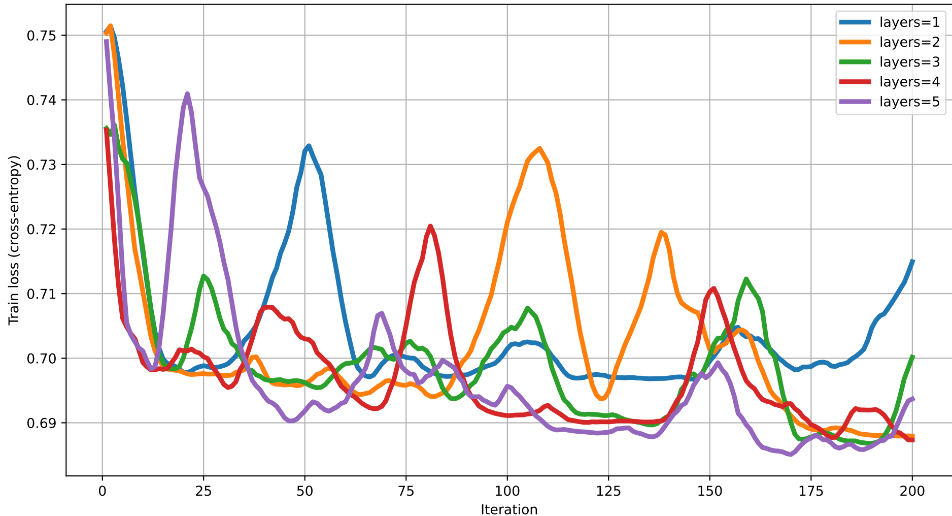
Train loss vs Iteration (dim=19) rot=RX, ent=chain, gate=CZ
