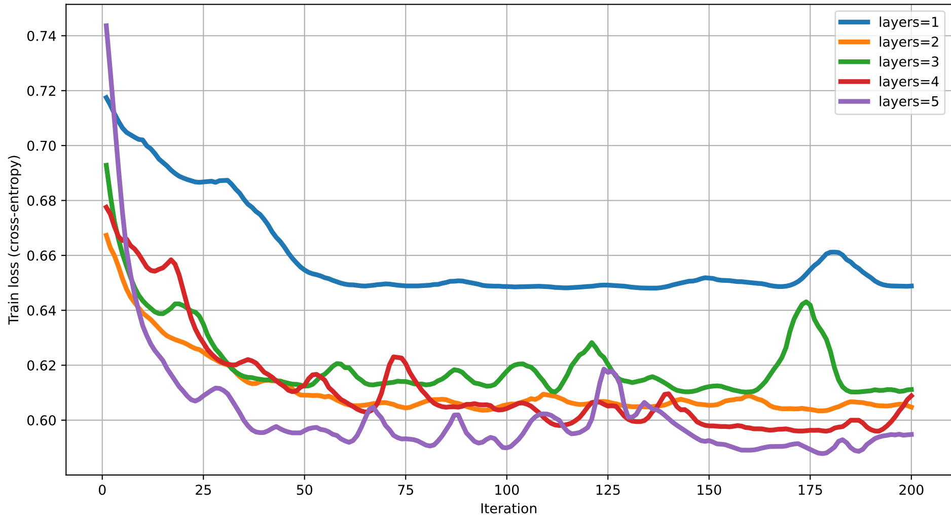
Train loss vs Iteration (degree=2) rot=RYZ, ent=ring, gate=CNOT
