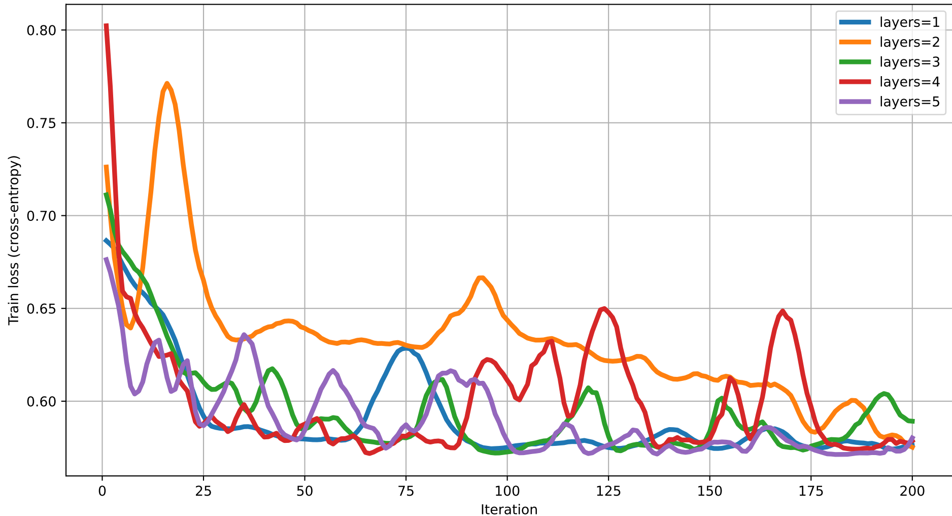
Train loss vs Iteration (dim=2) rot=Rot, ent=chain, gate=IsingXX
