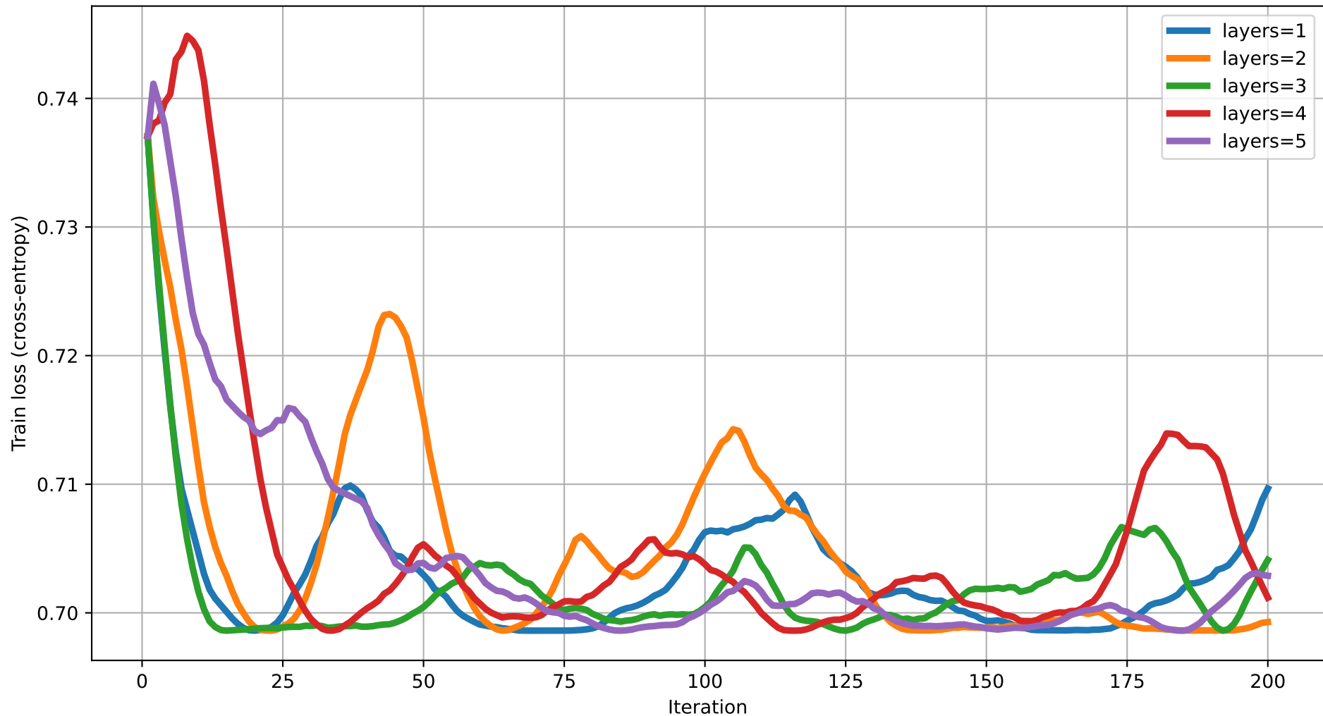
Train loss vs Iteration (dim=18) rot=RZ, ent=chain, gate=CZ
