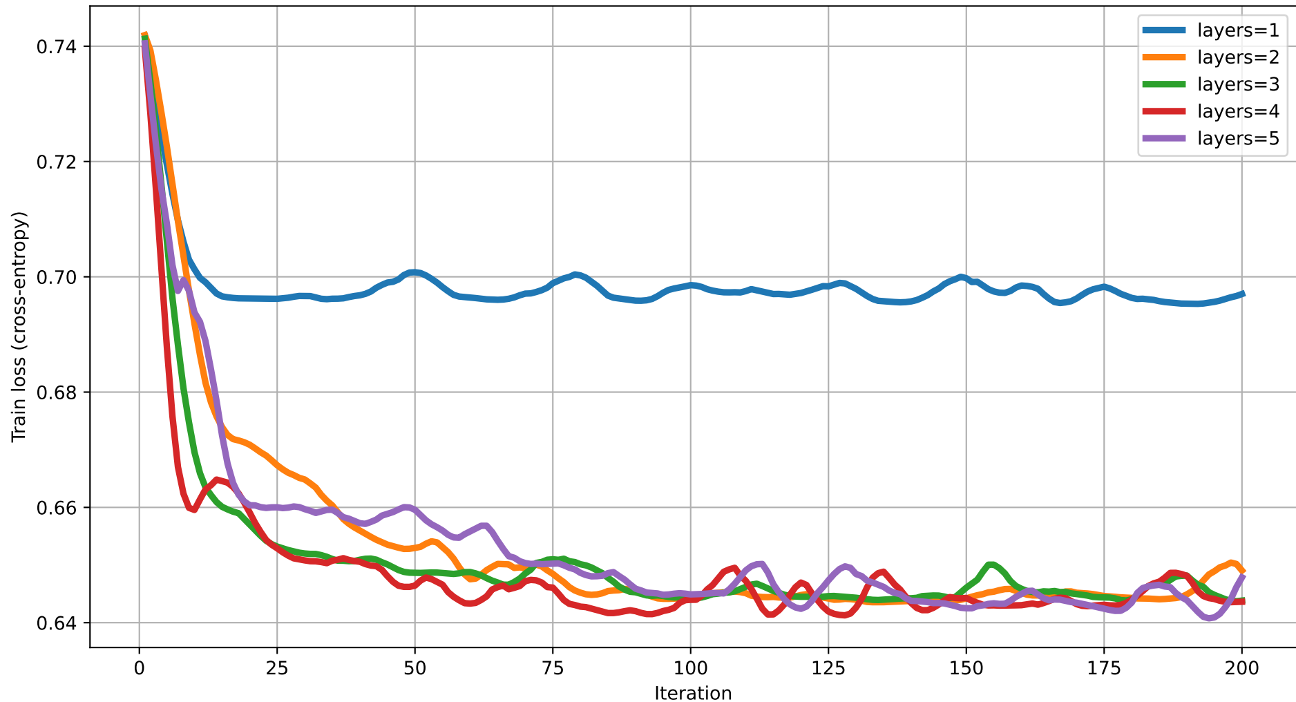
Train loss vs Iteration (degree=5) rot=RX, ent=chain, gate=CZ
