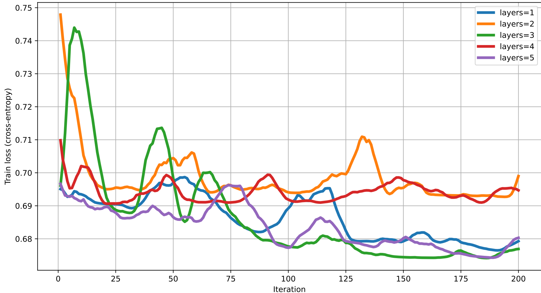
Train loss vs Iteration (dim=20) rot=RX, ent=pairwise, gate=IsingXX
