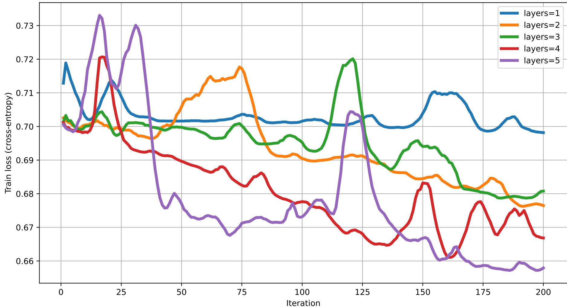
Train loss vs Iteration (dim=12) rot=RYZ, ent=full, gate=CNOT
