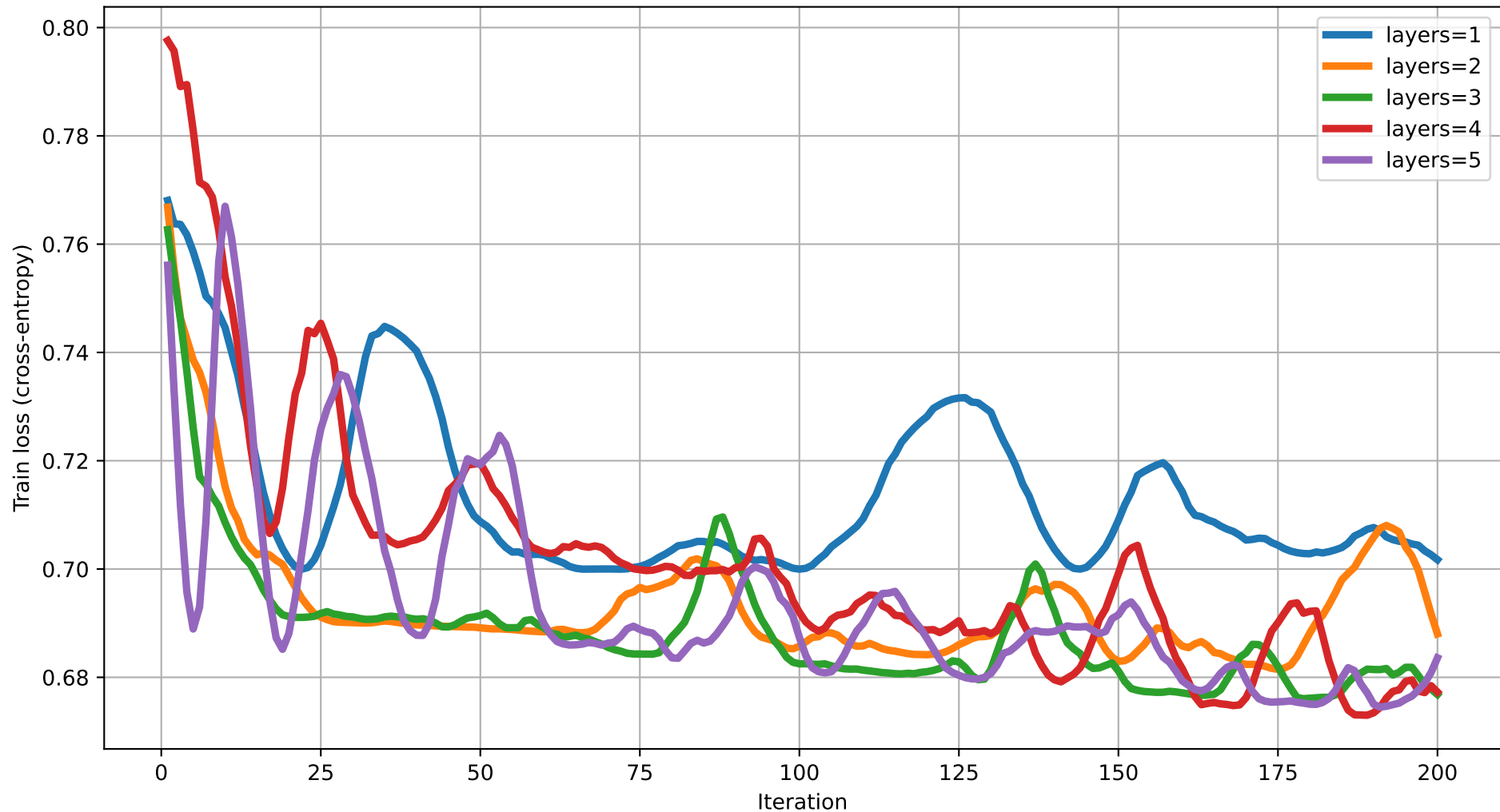
Train loss vs Iteration (dim=17) rot=RYZ, ent=pairwise, gate=CZ
