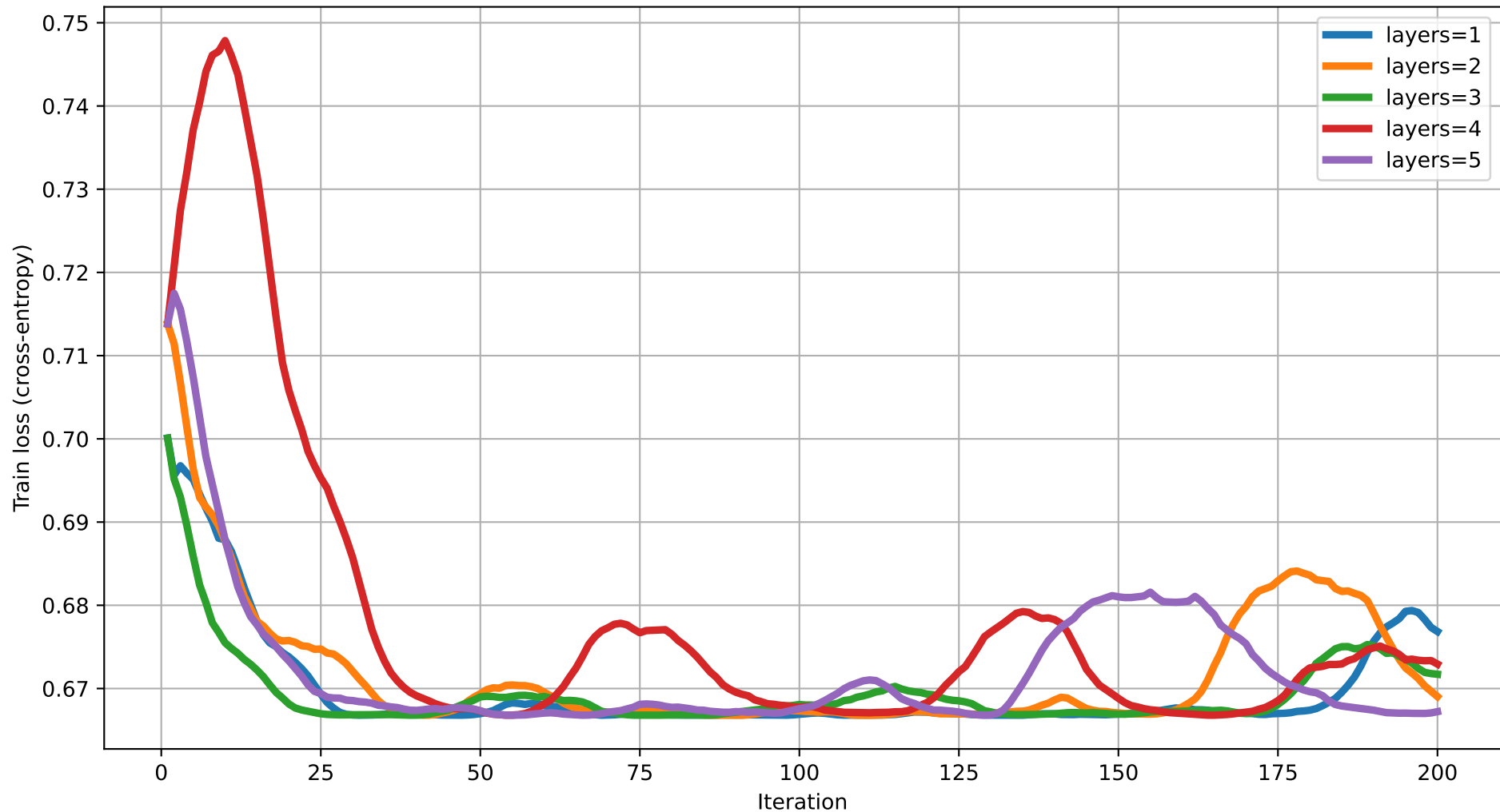
Train loss vs Iteration (dim=10) rot=RZ, ent=chain, gate=CZ
