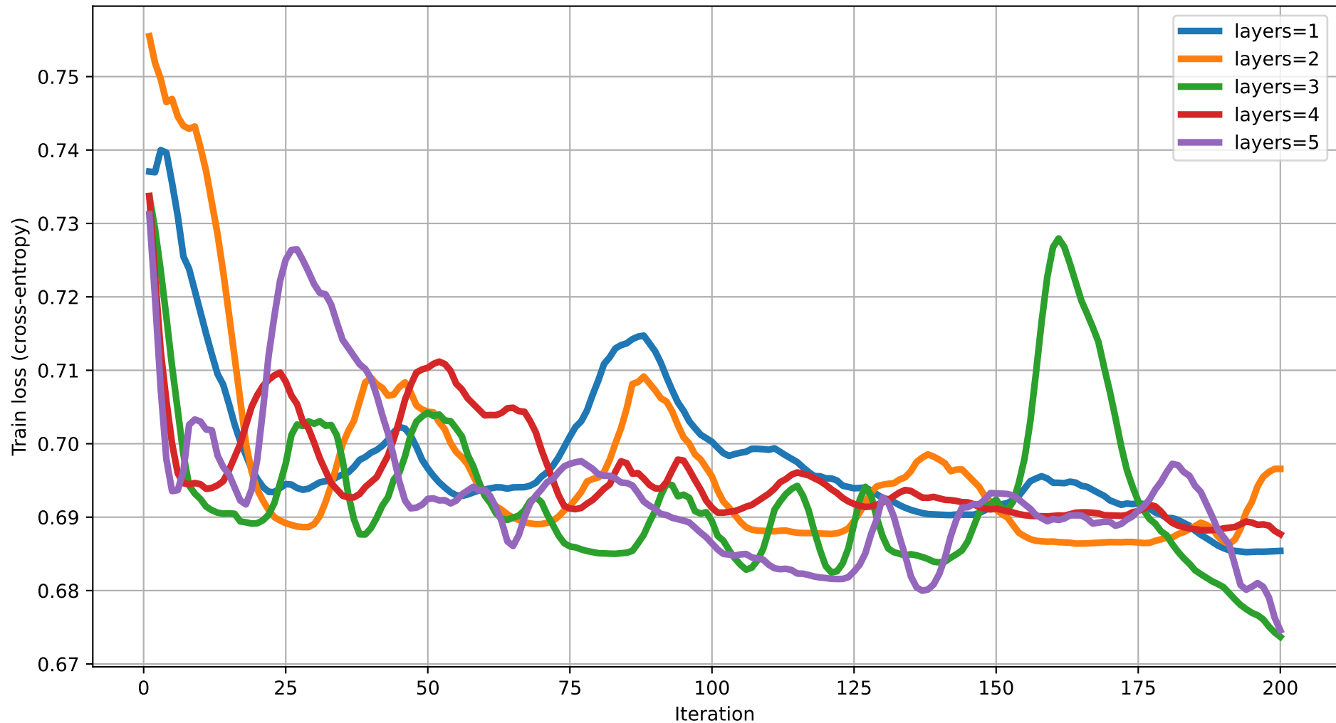
Train loss vs Iteration (dim=16) rot=RY, ent=full, gate=CZ
