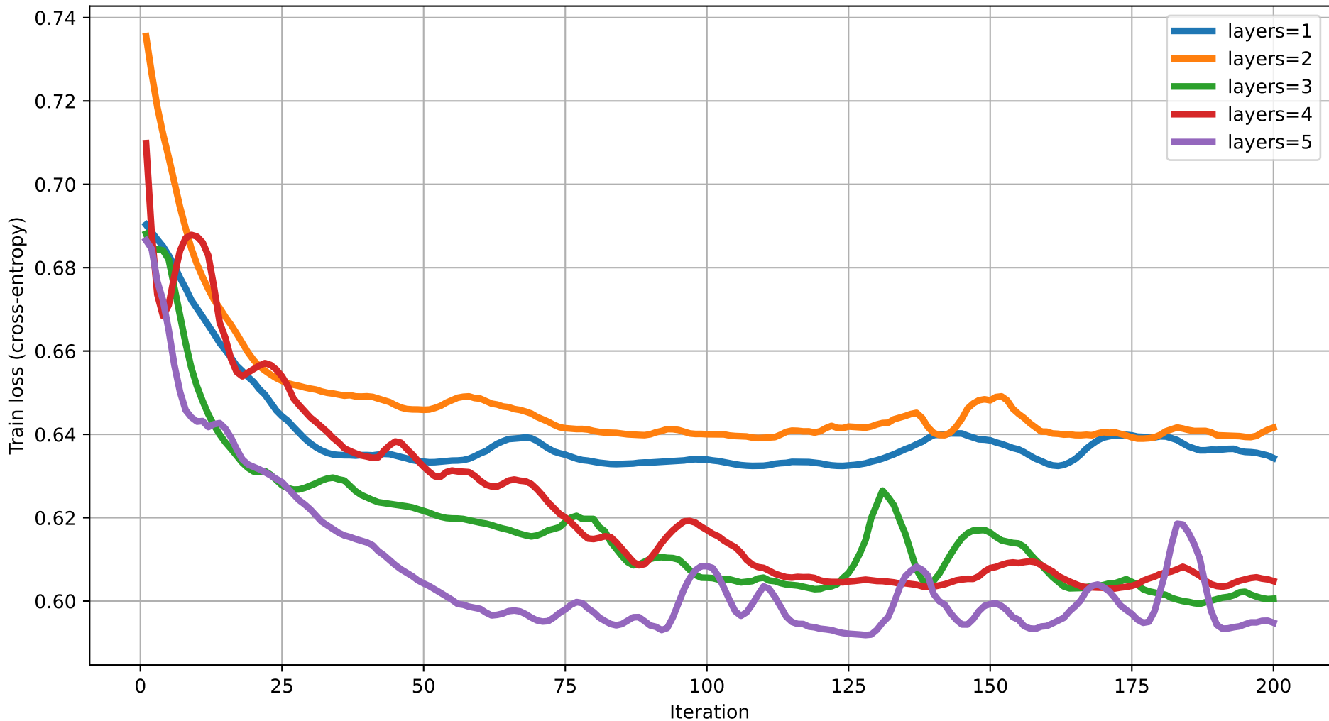
Train loss vs Iteration (degree=2) rot=RYZ, ent=chain, gate=IsingXX
