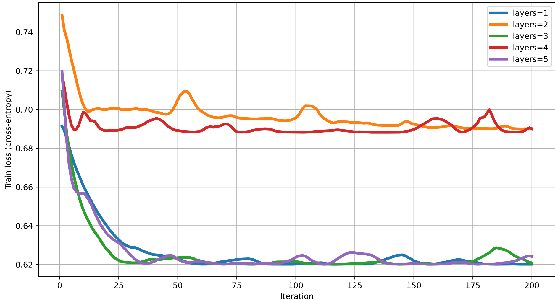
Train loss vs Iteration (degree=4) rot=RX, ent=chain, gate=IsingXX
