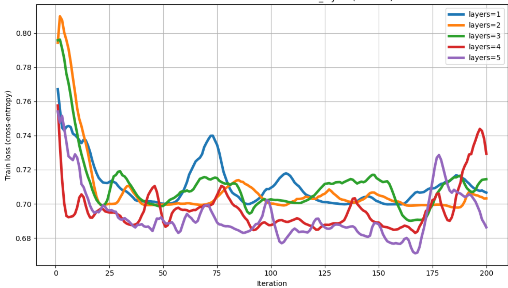
Train loss vs Iteration for different num_layers (dim=17)
