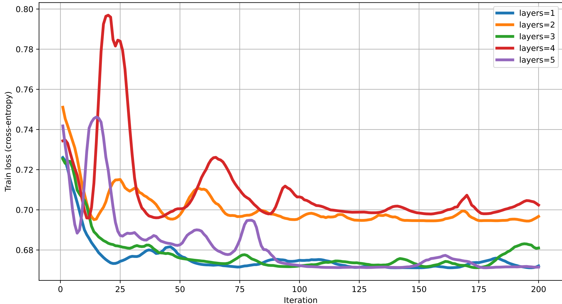
Train loss vs Iteration (dim=18) rot=RX, ent=ring, gate=IsingXX
