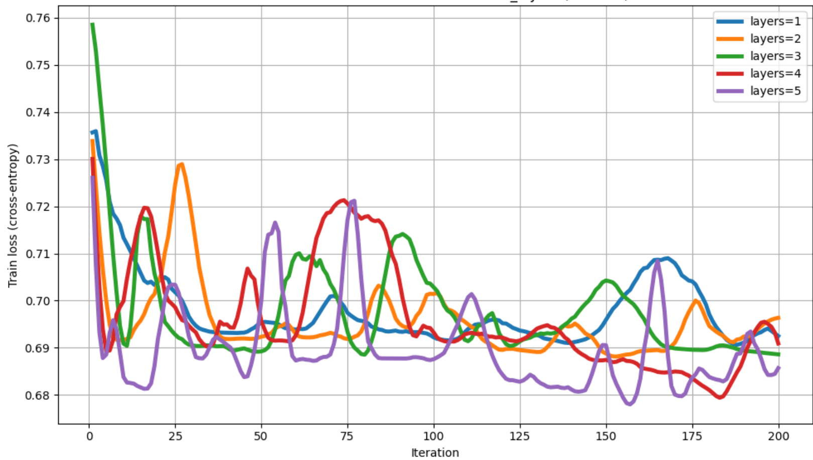
Train loss vs Iteration for different num_layers (dim=16)
