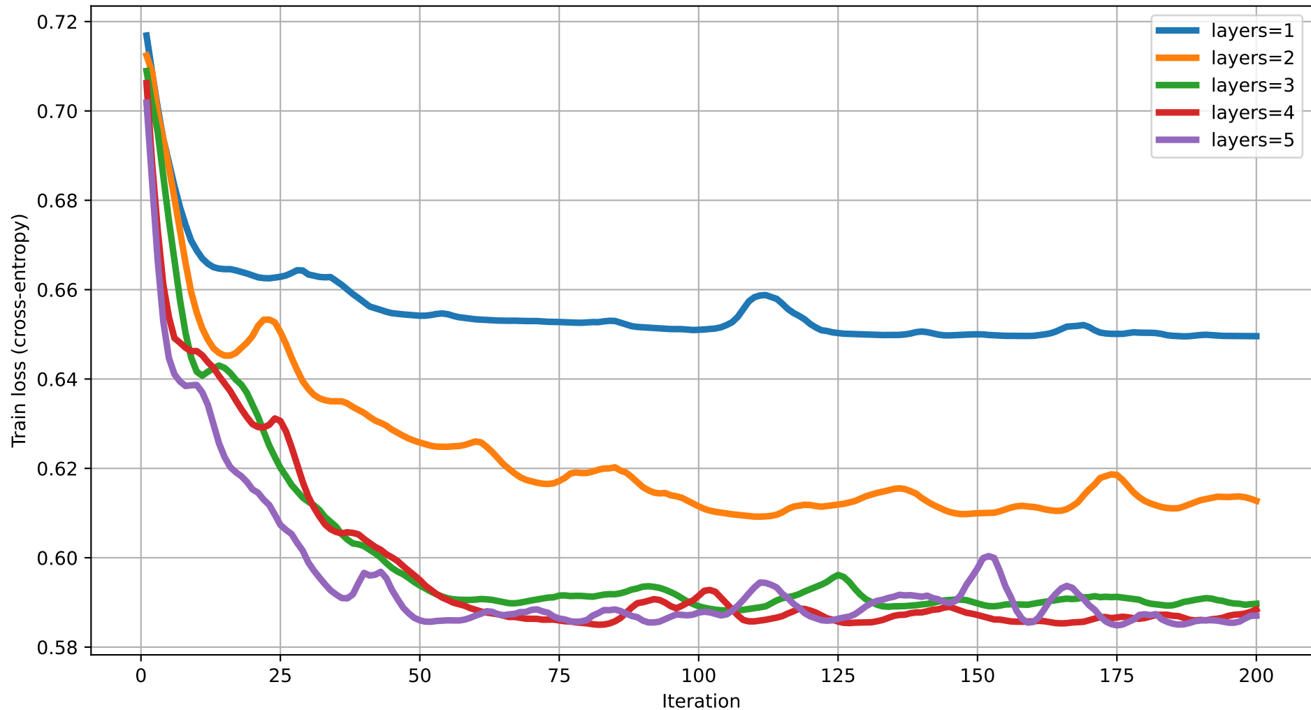
Train loss vs Iteration (degree=4) rot=RY, ent=chain, gate=CZ
