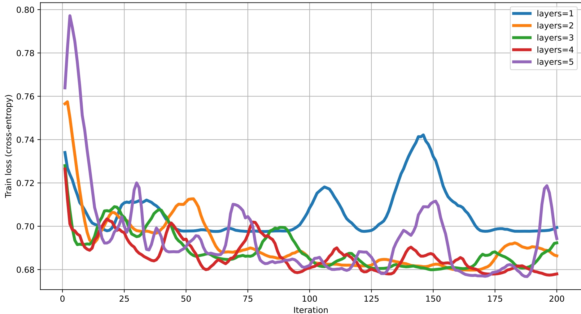
Train loss vs Iteration (dim=19) rot=Rot, ent=pairwise, gate=CZ
