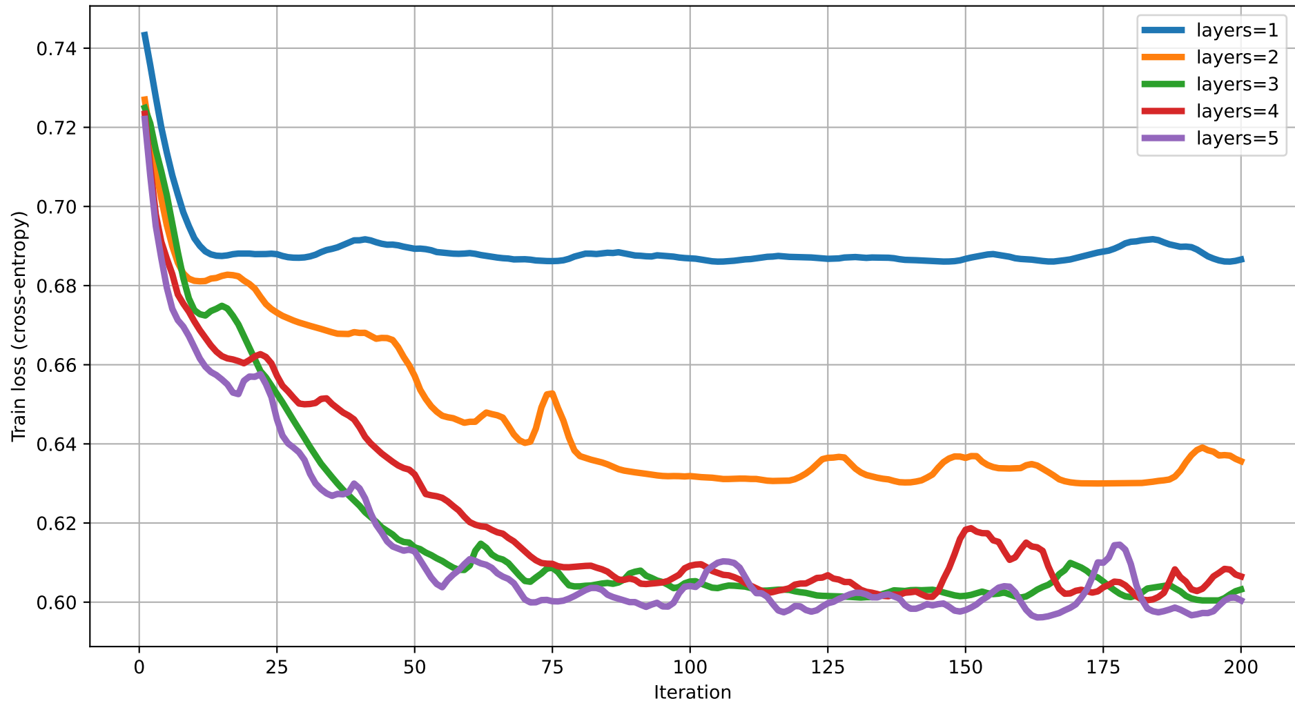
Train loss vs Iteration (degree=2) rot=Rot, ent=ring, gate=CZ
