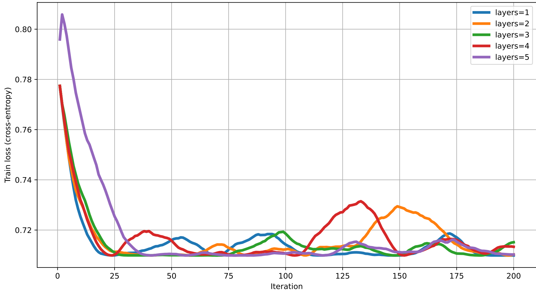
Train loss vs Iteration (dim=4) rot=RZ, ent=chain, gate=CZ
