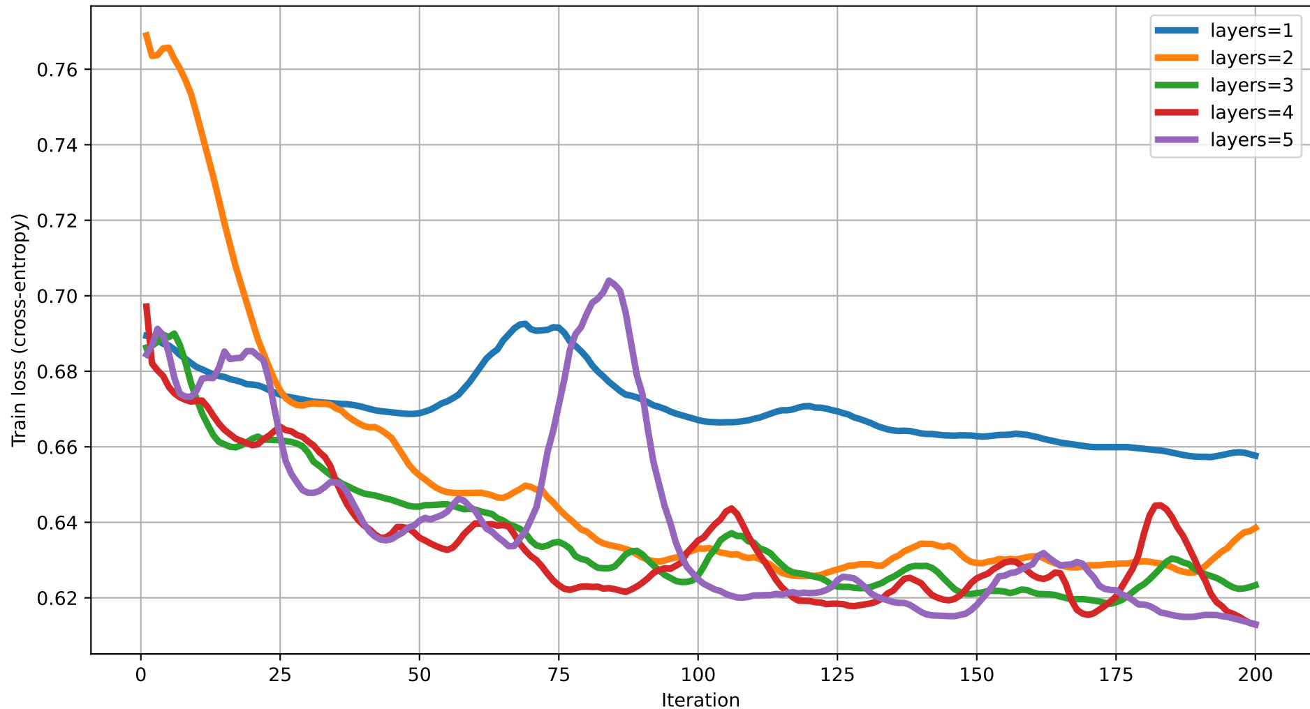
Train loss vs Iteration (dim=10) rot=RZ, ent=full, gate=IsingXX
