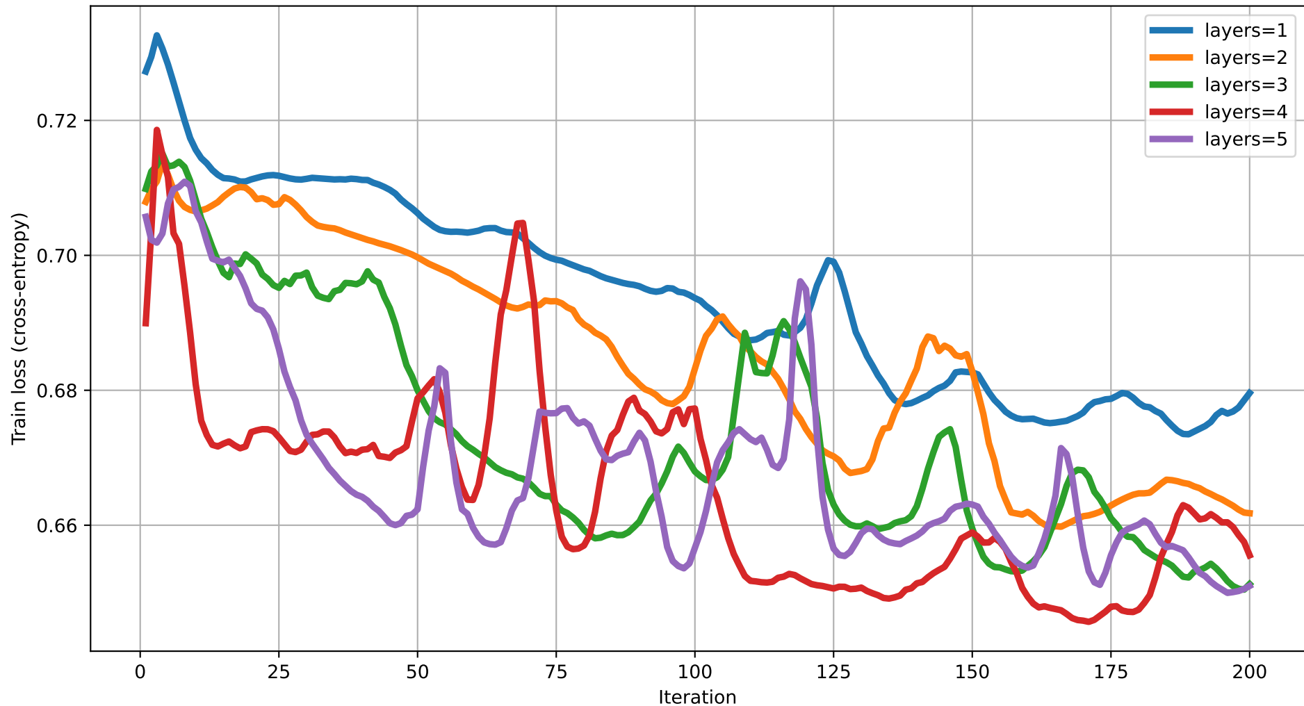
Train loss vs Iteration (dim=7) rot=Rot, ent=ring, gate=CNOT
