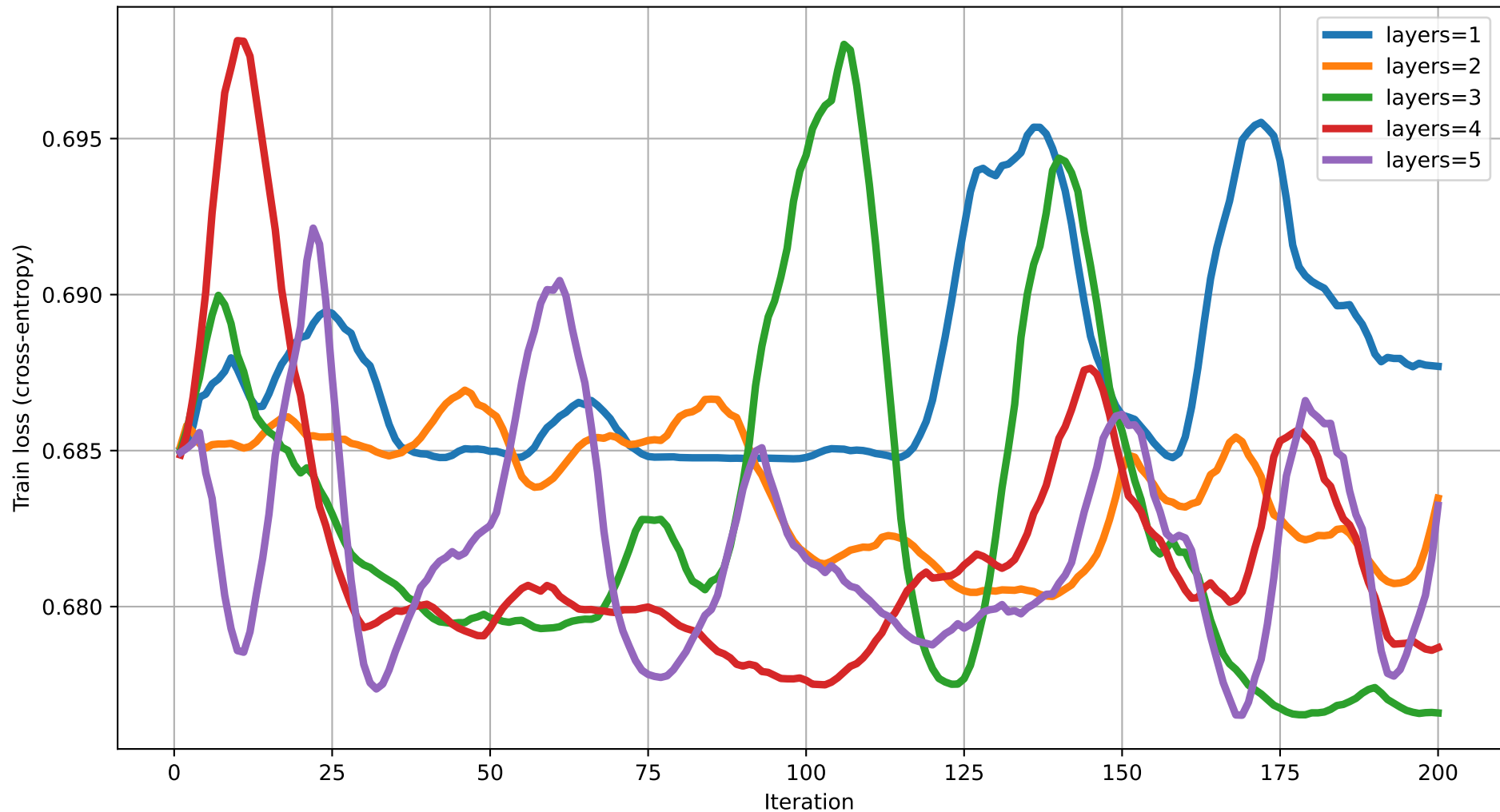
Train loss vs Iteration (dim=15) rot=RX, ent=chain, gate=CZ
