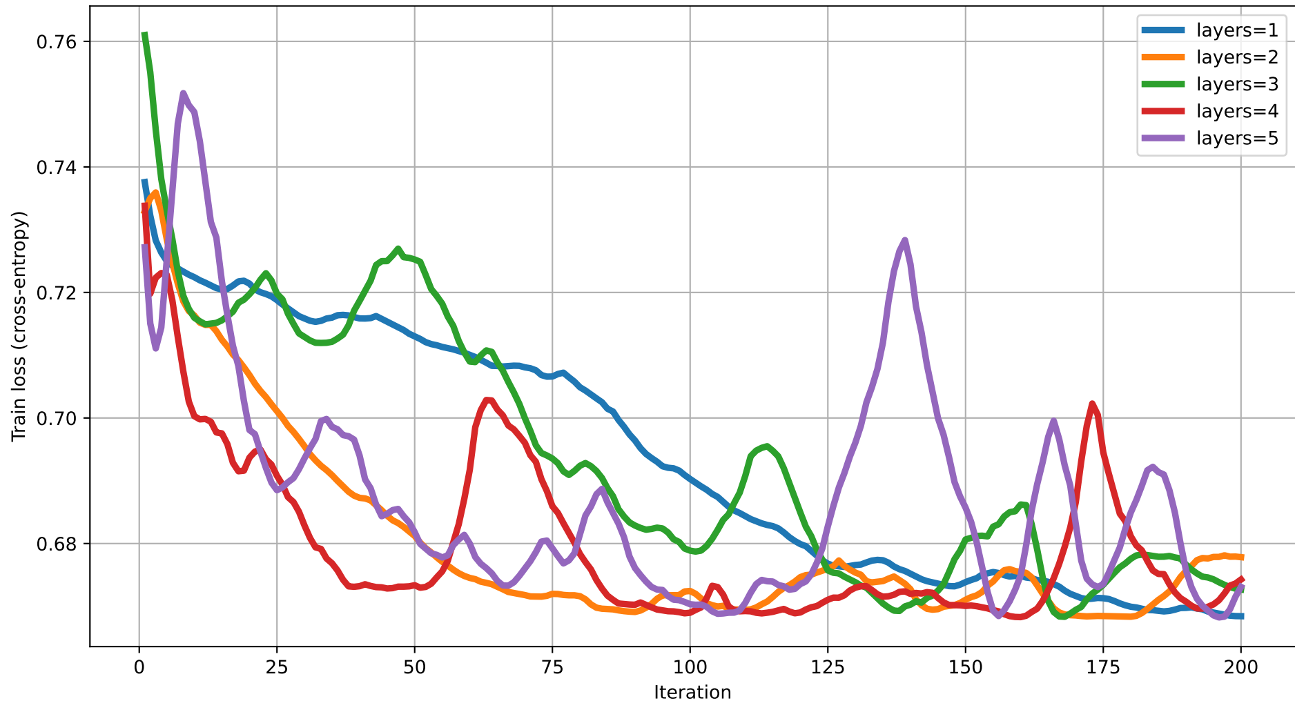
Train loss vs Iteration (dim=3) rot=RYZ, ent=ring, gate=CZ
