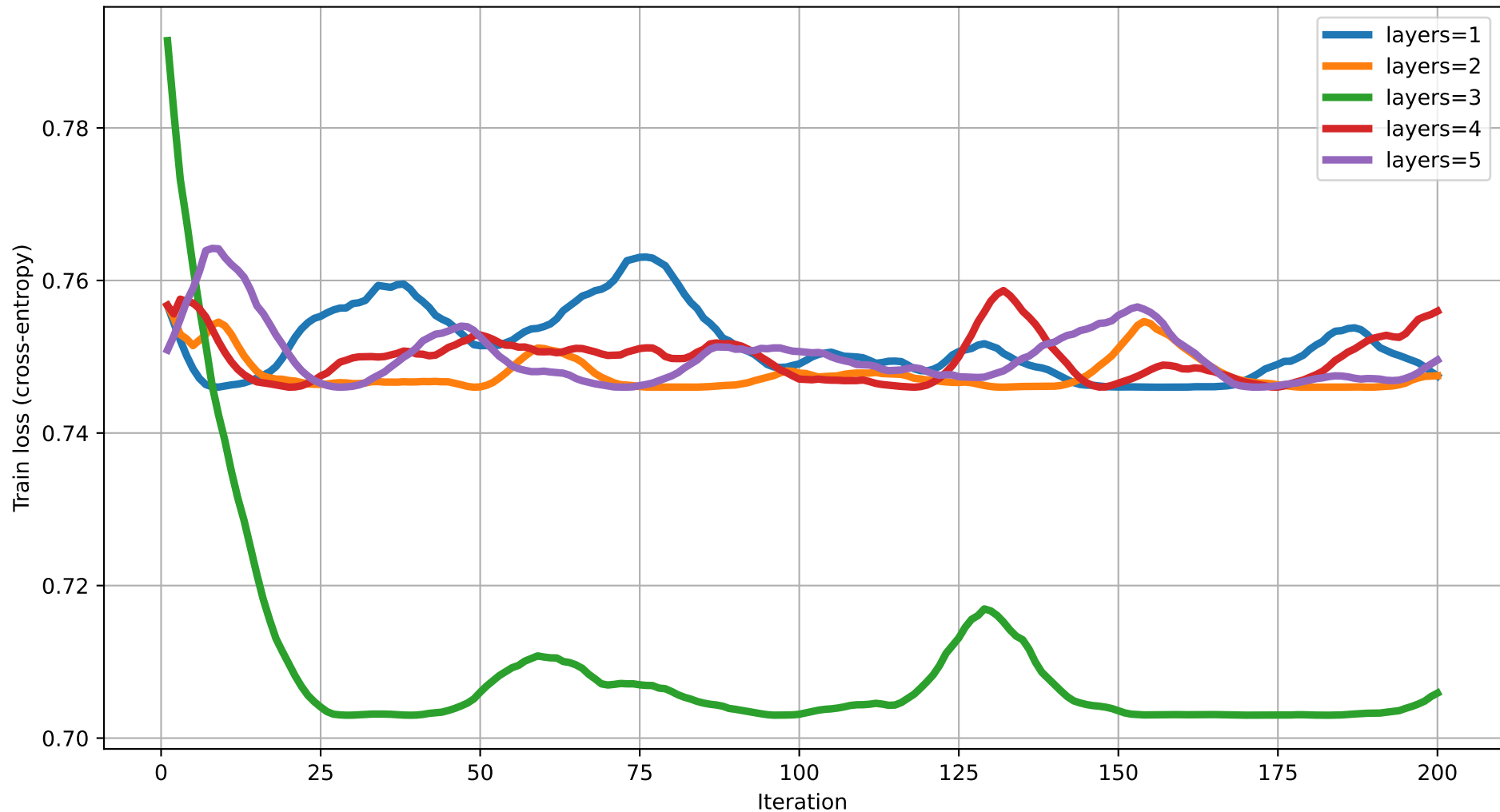
Train loss vs Iteration (dim=2) rot=RZ, ent=ring, gate=CNOT
