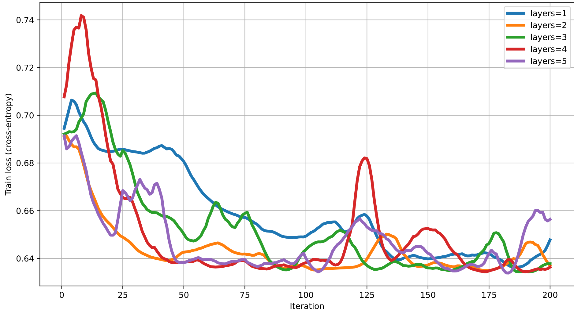
Train loss vs Iteration (dim=7) rot=RYZ, ent=pairwise, gate=IsingXX
