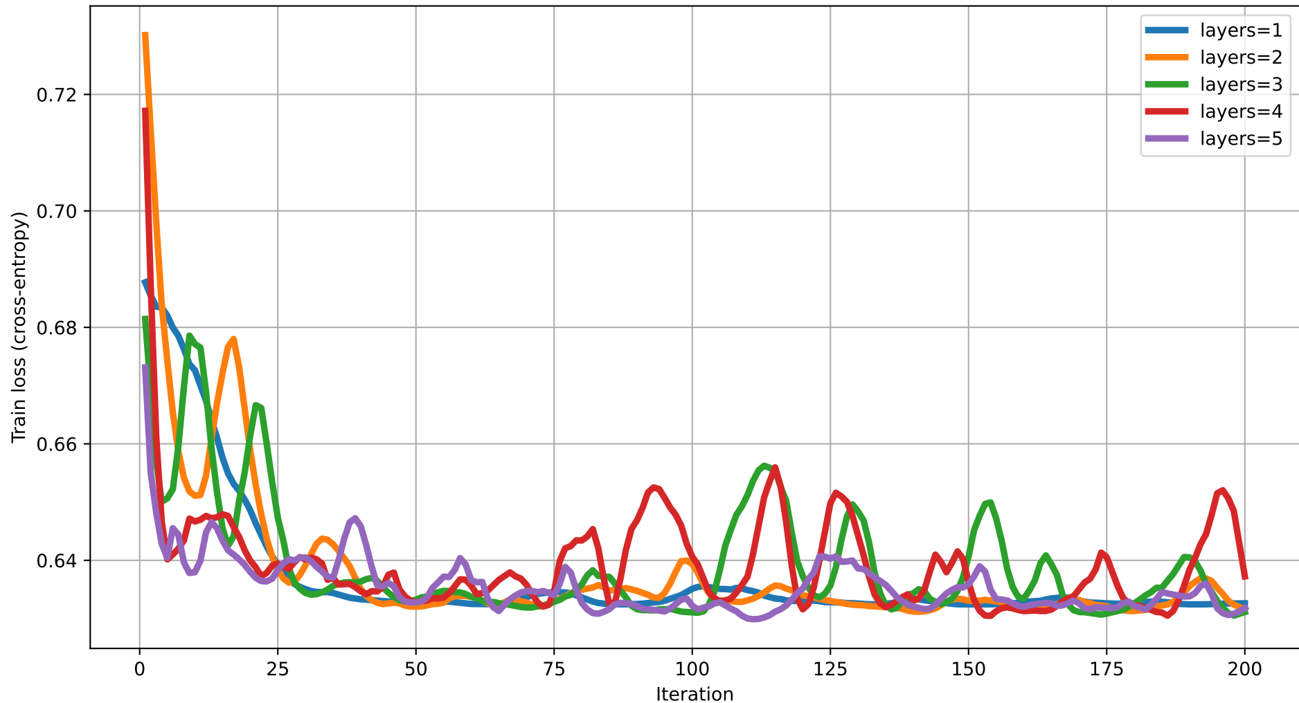
Train loss vs Iteration (degree=2) rot=Rot, ent=pairwise, gate=IsingXX
