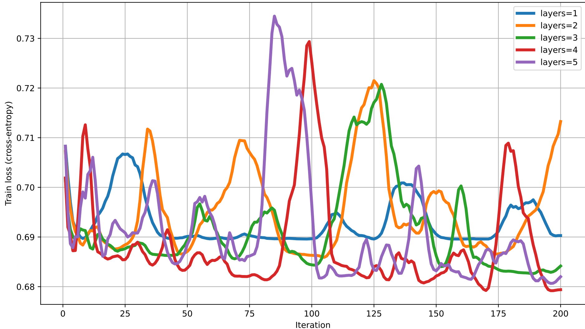
Train loss vs Iteration for different num_layers (dim=20)
