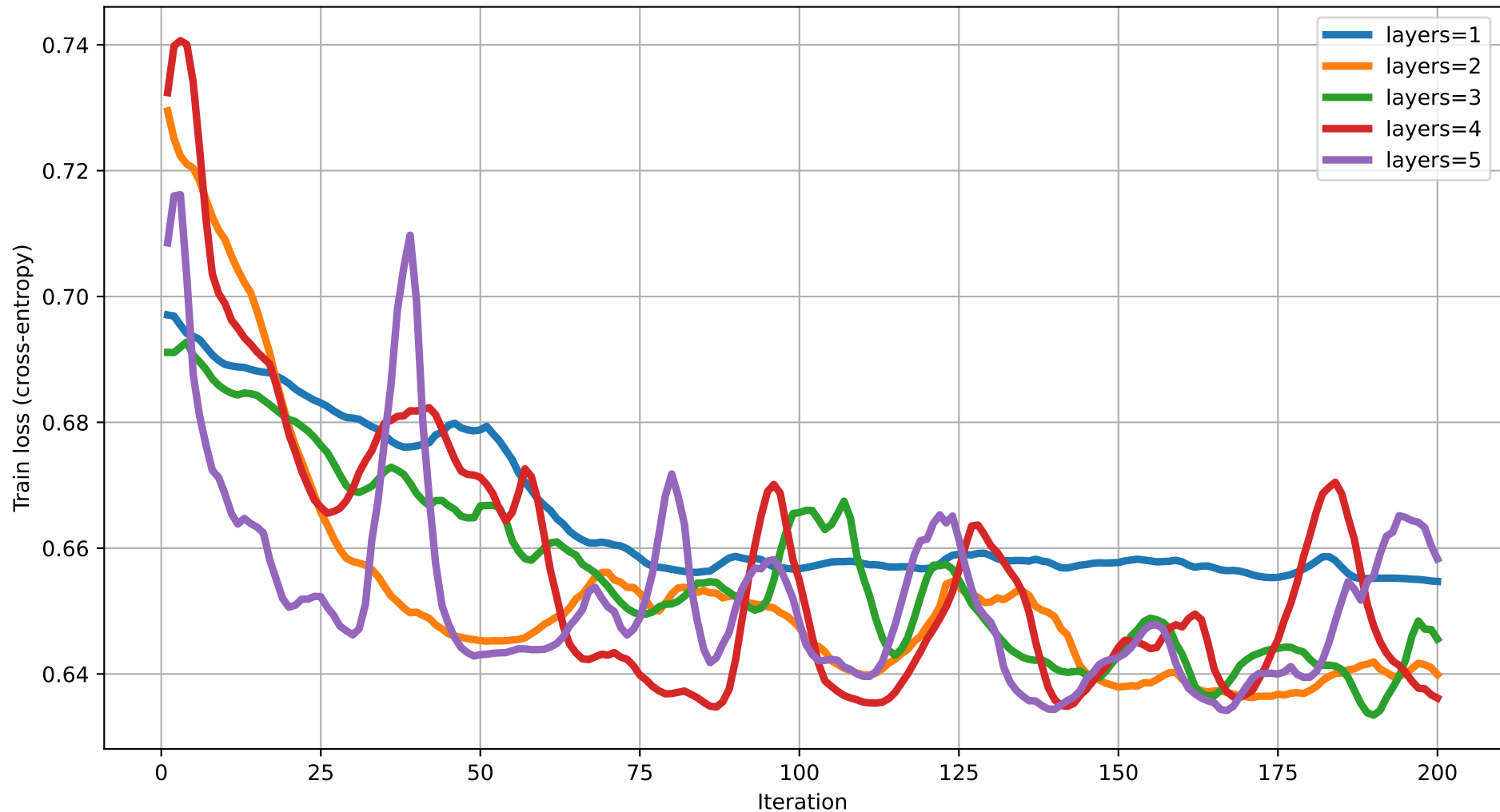
Train loss vs Iteration (dim=3) rot=RYZ, ent=full, gate=IsingXX
