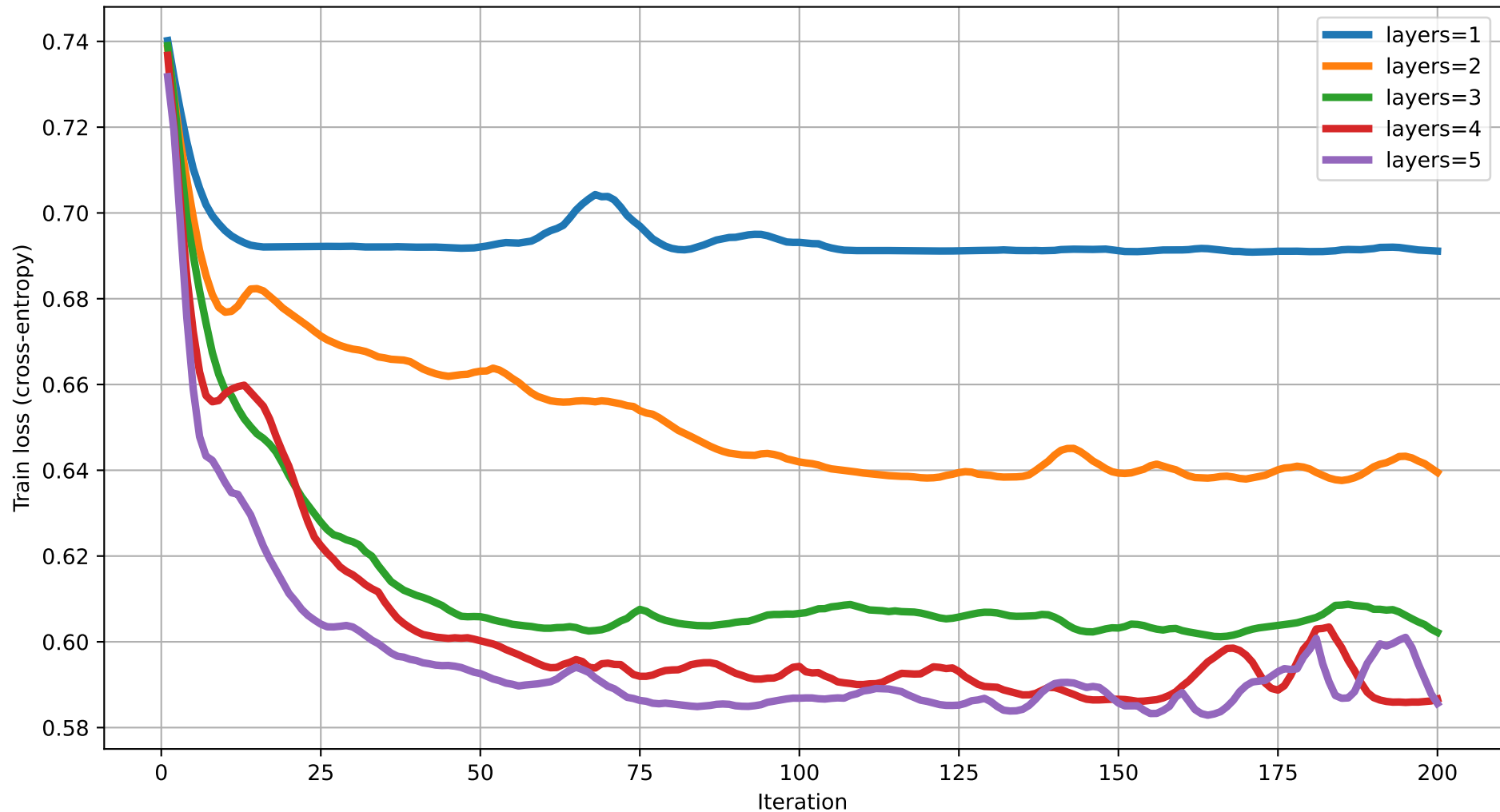
Train loss vs Iteration (degree=5) rot=RYZ, ent=full, gate=CNOT
