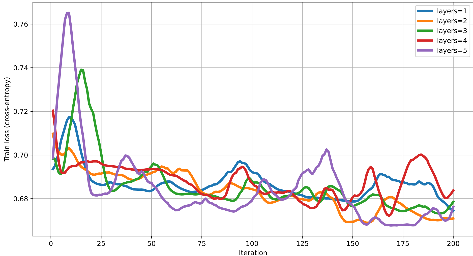
Train loss vs Iteration (dim=12) rot=RZ, ent=full, gate=IsingXX
