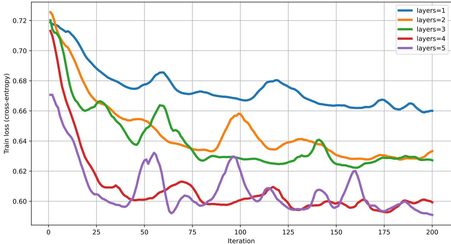
Train loss vs Iteration (dim=8) rot=RY, ent=ring, gate=CNOT
