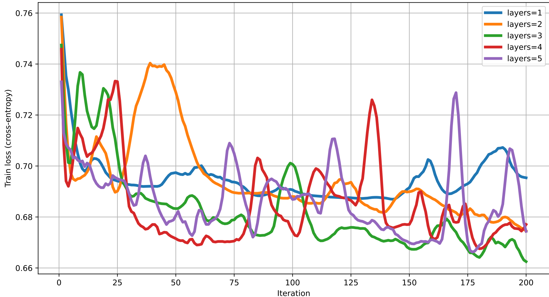
Train loss vs Iteration (dim=17) rot=Rot, ent=full, gate=IsingXX
