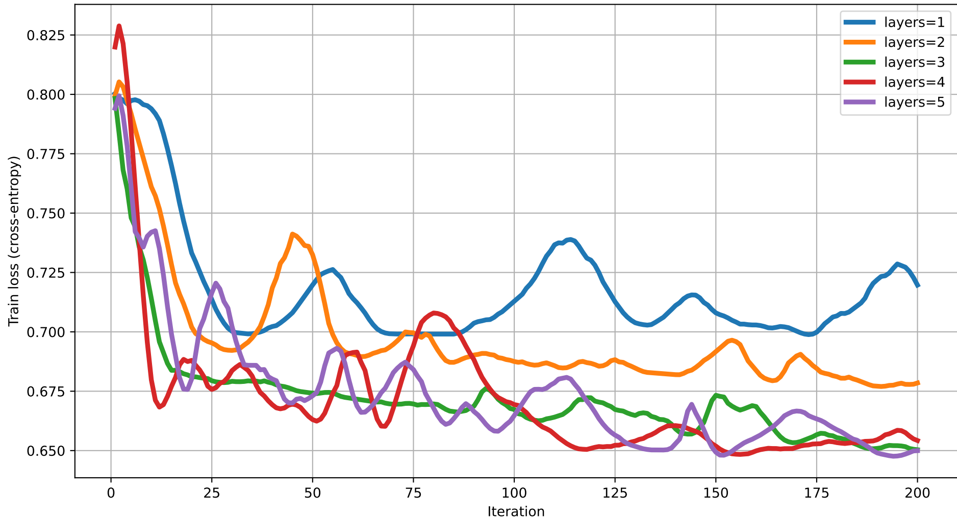
Train loss vs Iteration (dim=8) rot=RX, ent=full, gate=CNOT
