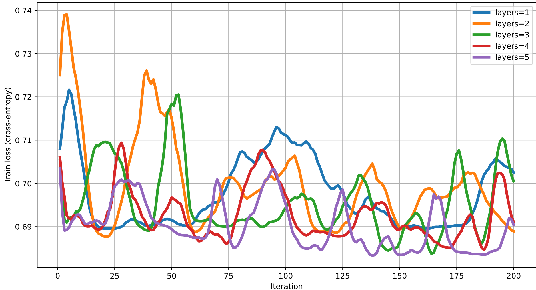
Train loss vs Iteration (dim=20) rot=Rot, ent=ring, gate=CZ
