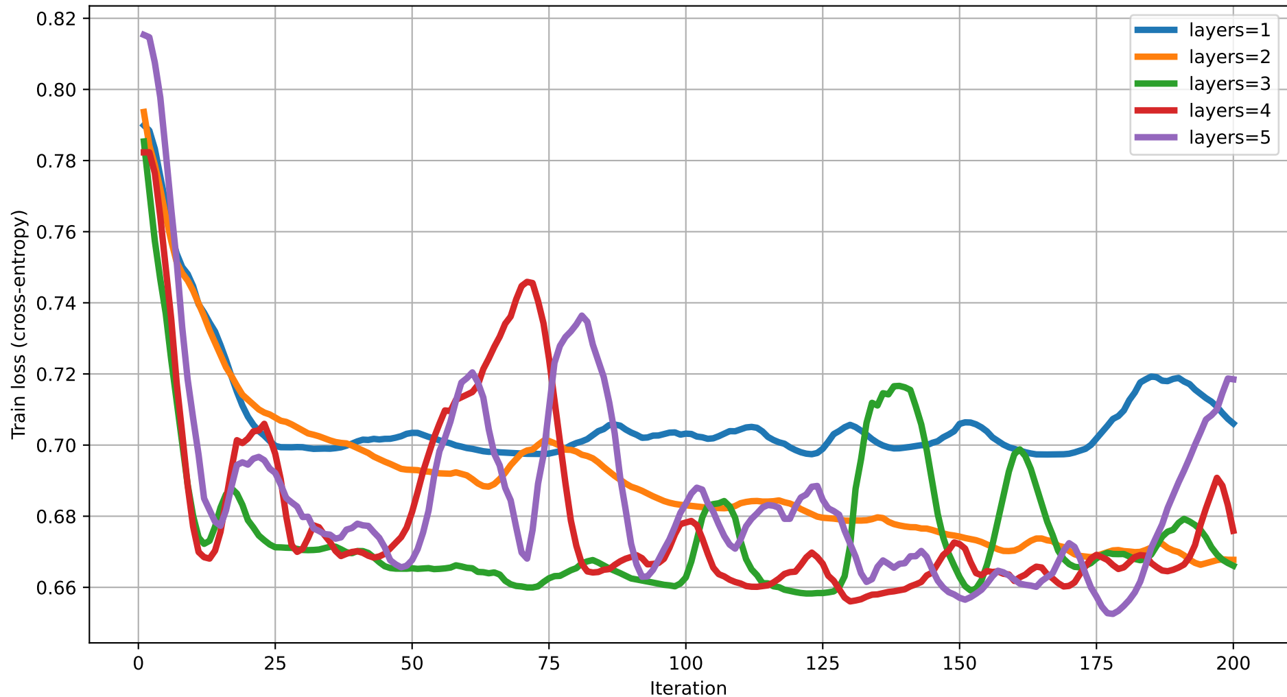
Train loss vs Iteration (dim=2) rot=Rot, ent=full, gate=CNOT
