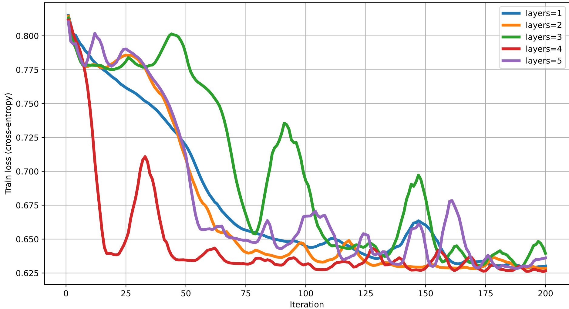
Train loss vs Iteration (dim=2) rot=RY, ent=ring, gate=CZ
