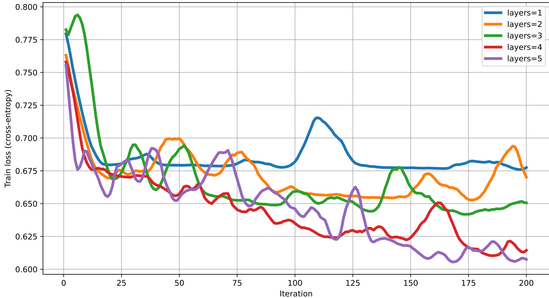
Train loss vs Iteration (dim=8) rot=Rot, ent=ring, gate=CZ
