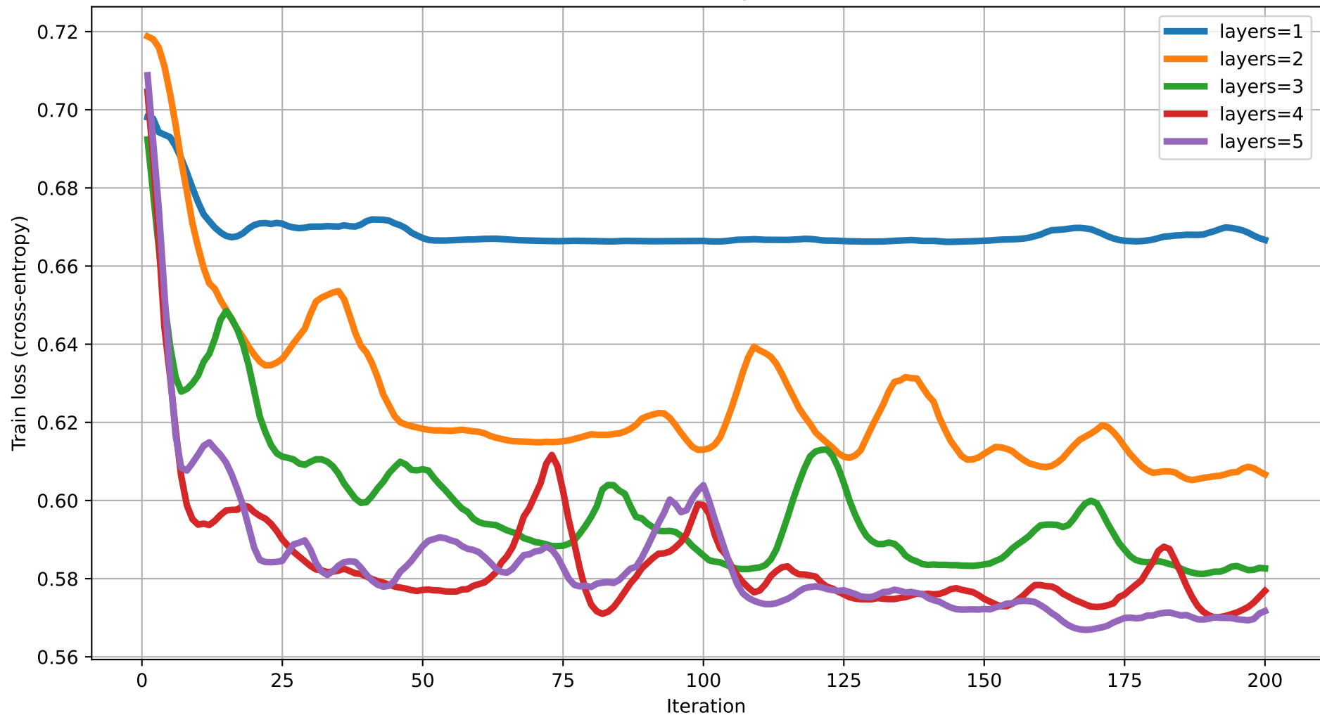
Train loss vs Iteration (dim=10) rot=RY, ent=full, gate=CNOT
