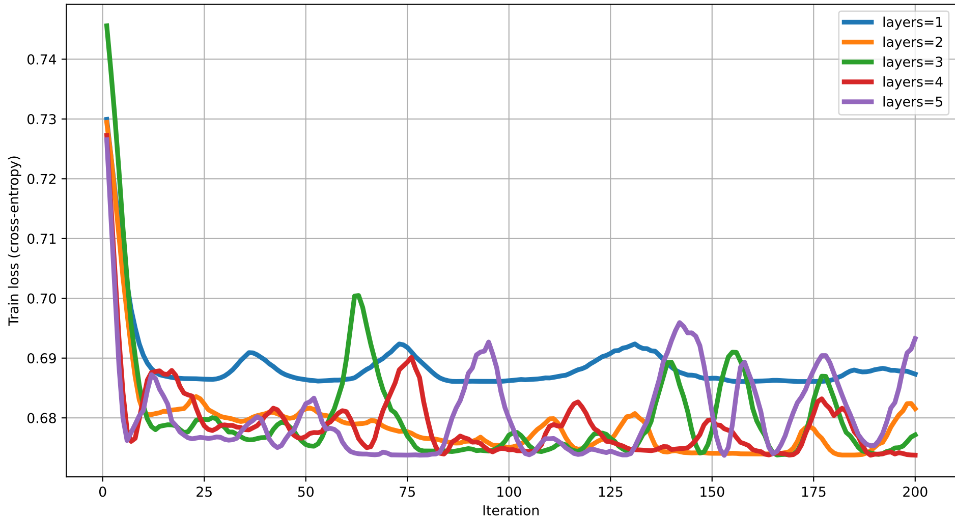
Train loss vs Iteration (degree=2) rot=RX, ent=pairwise, gate=CNOT
