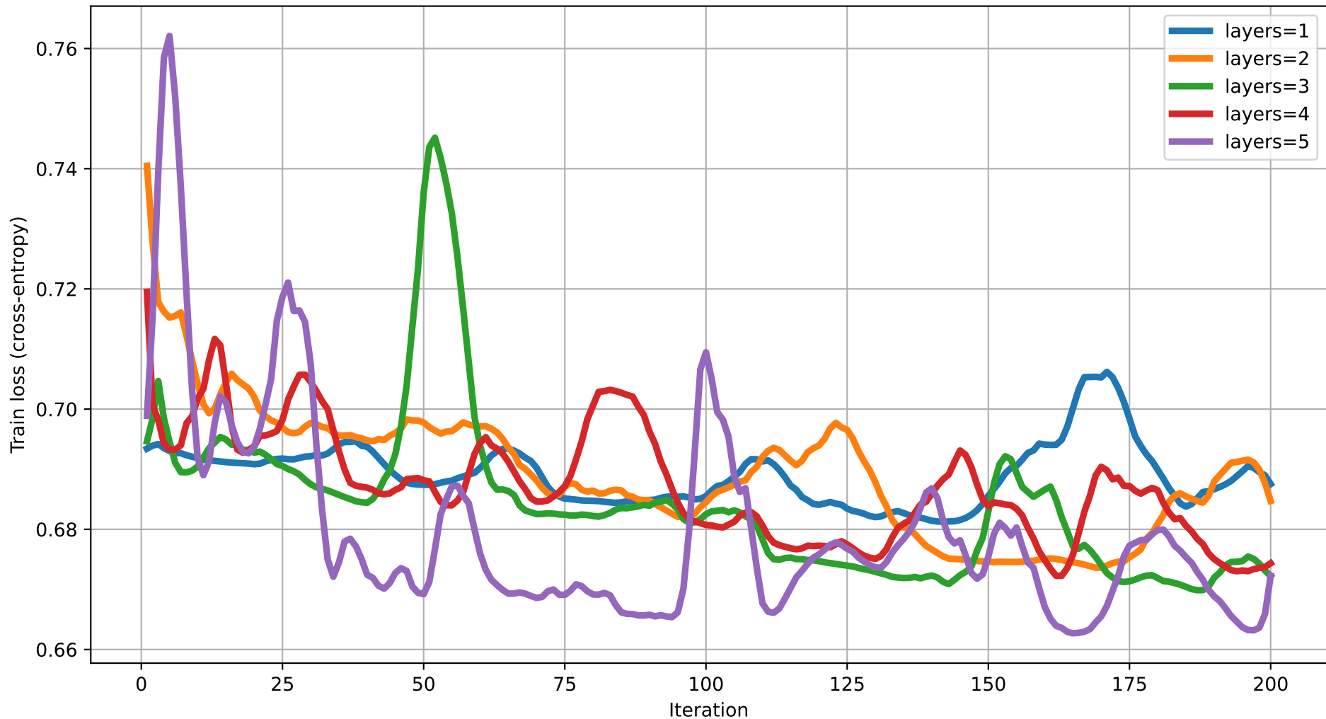
Train loss vs Iteration (dim=19) rot=RYZ, ent=chain, gate=IsingXX
