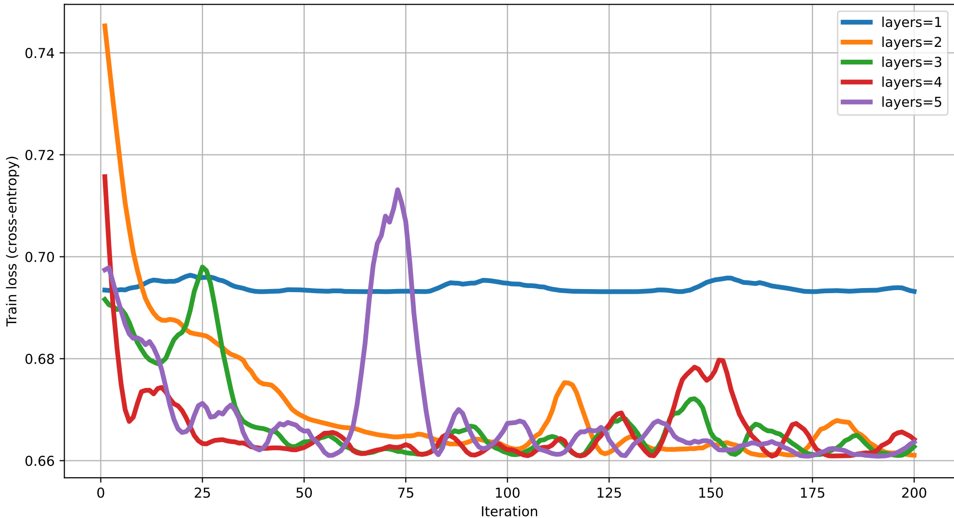
Train loss vs Iteration (degree=3) rot=RY, ent=pairwise, gate=IsingXX
