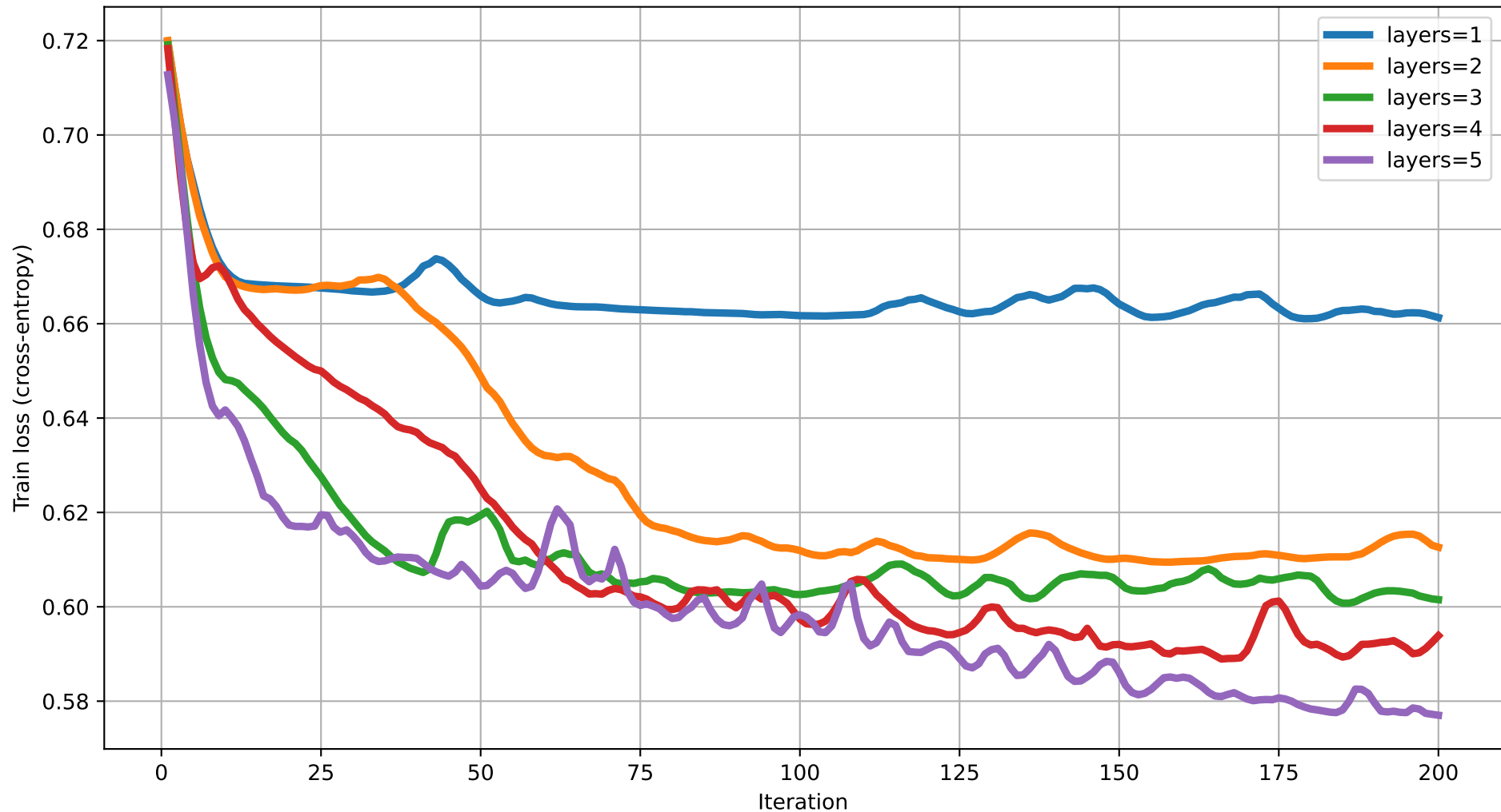
Train loss vs Iteration (degree=3) rot=Rot, ent=full, gate=CZ
