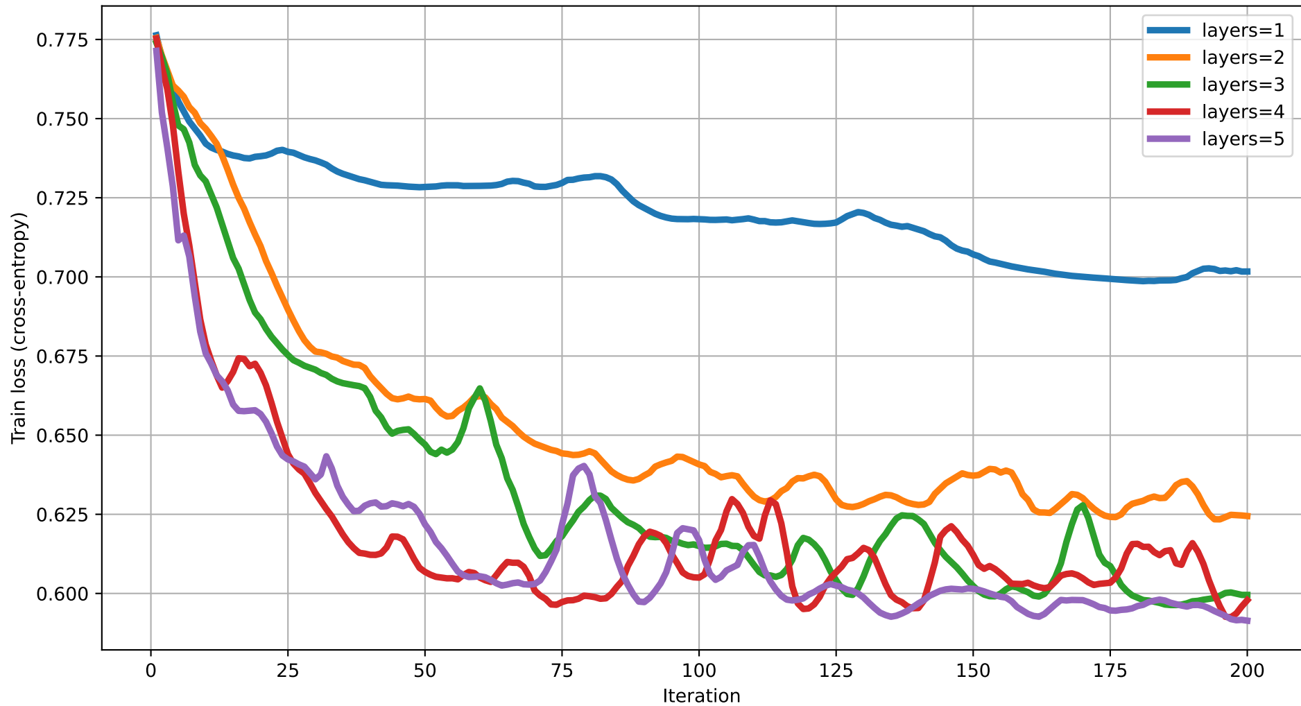
Train loss vs Iteration (dim=9) rot=Rot, ent=full, gate=CNOT
