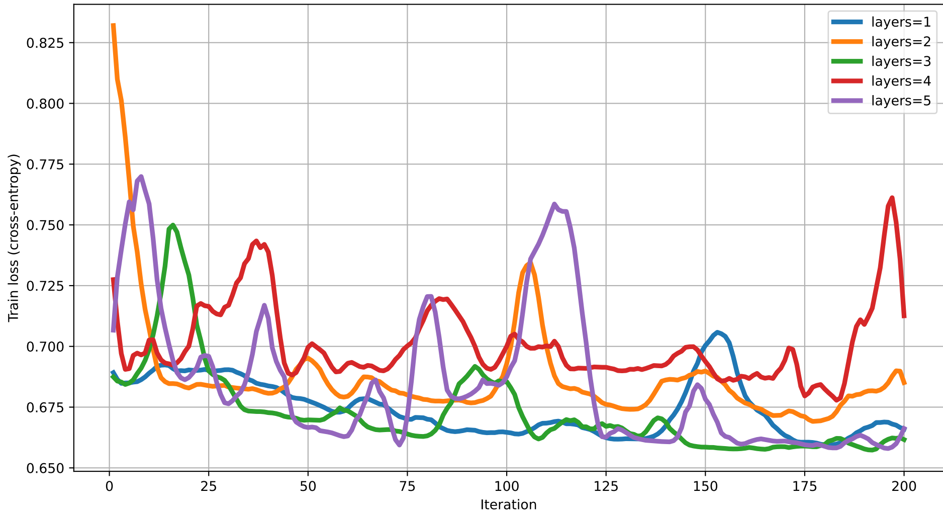
Train loss vs Iteration (dim=16) rot=RYZ, ent=pairwise, gate=IsingXX
