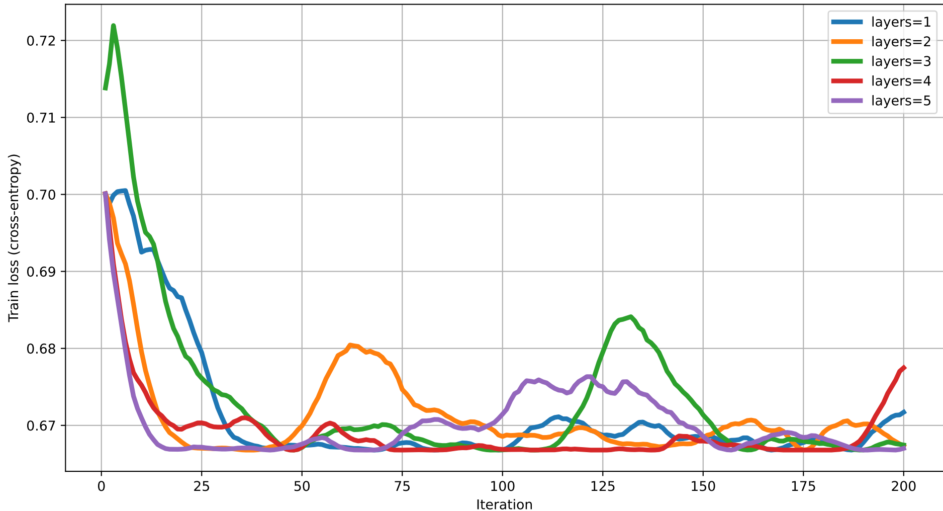
Train loss vs Iteration (dim=10) rot=RZ, ent=ring, gate=CZ
