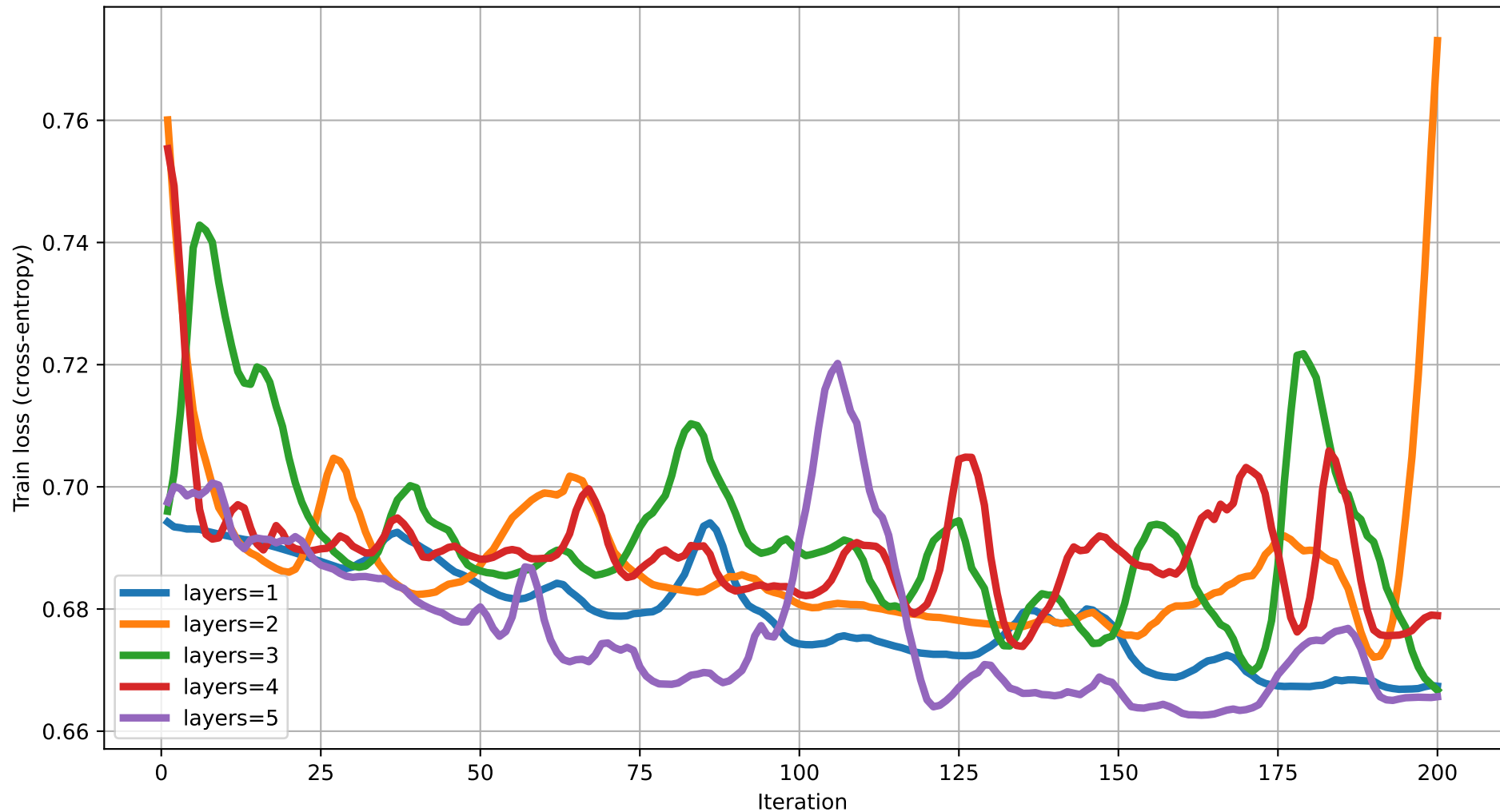
Train loss vs Iteration (dim=17) rot=RYZ, ent=chain, gate=IsingXX
