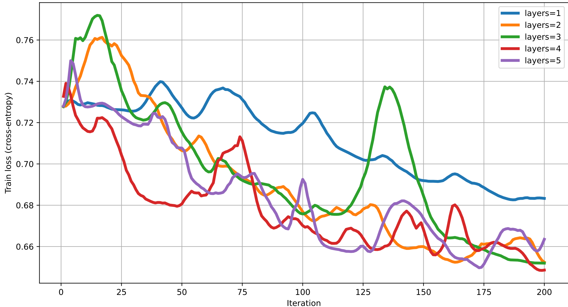
Train loss vs Iteration (dim=7) rot=RYZ, ent=pairwise, gate=CZ
