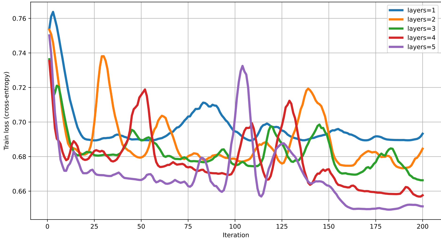
Train loss vs Iteration (dim=16) rot=RX, ent=chain, gate=CNOT
