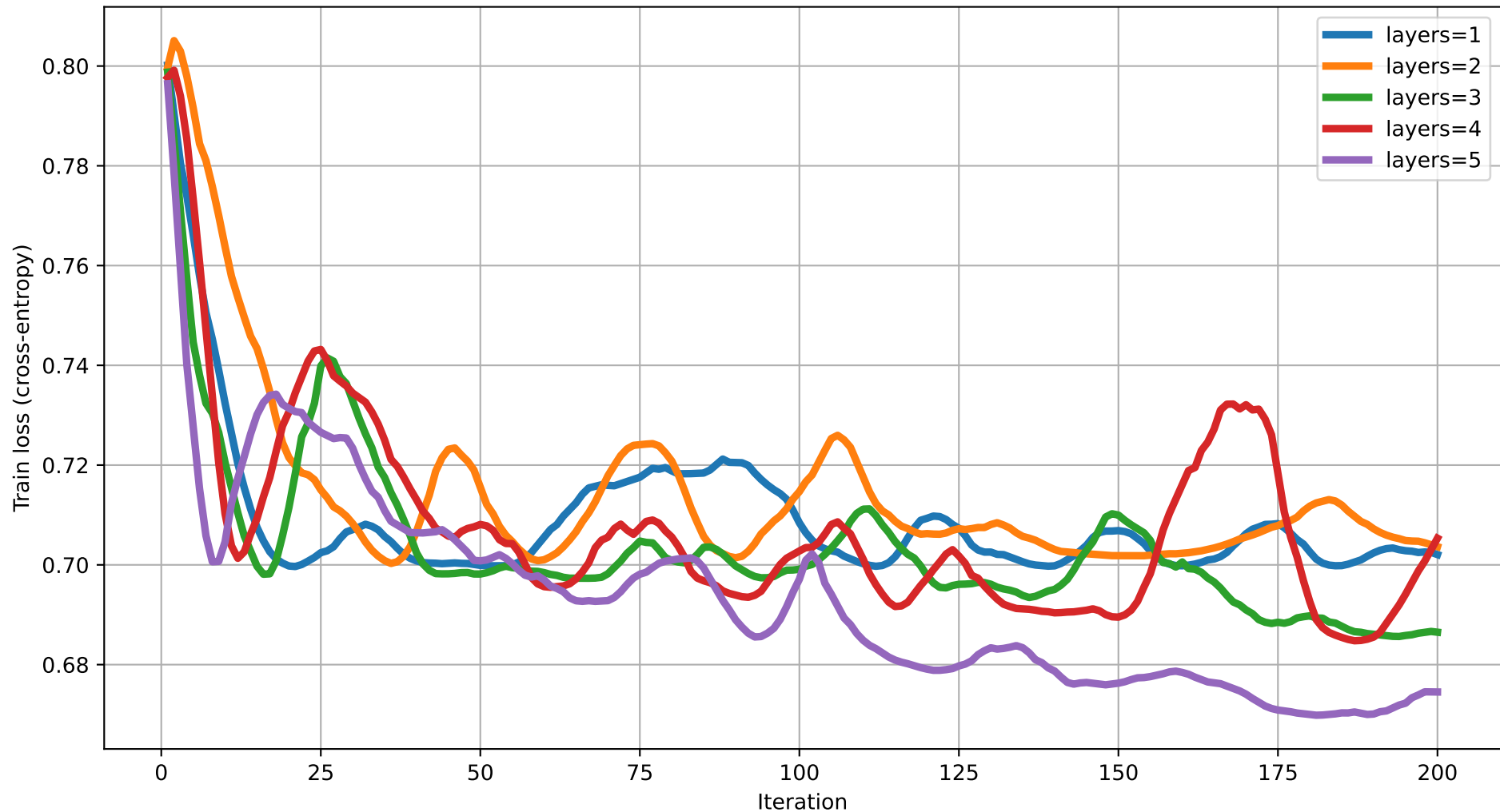
Train loss vs Iteration (dim=8) rot=RX, ent=full, gate=CZ
