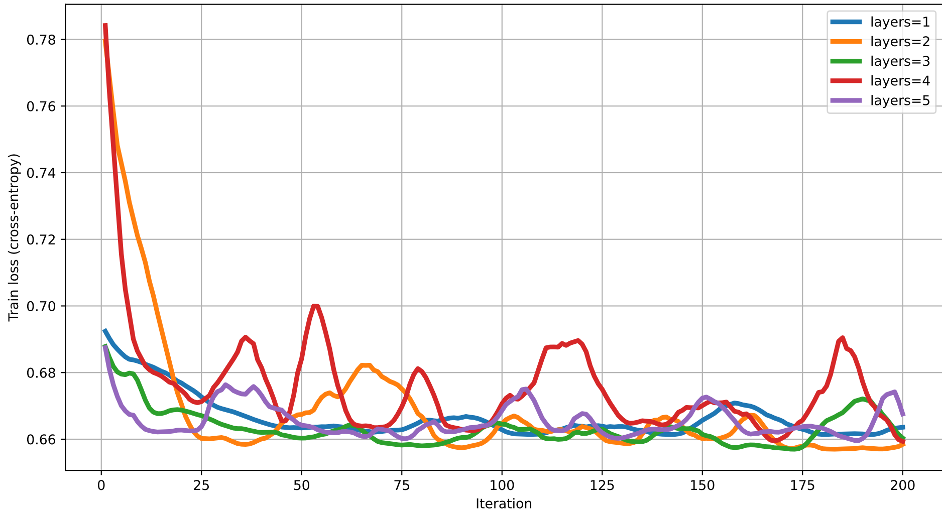
Train loss vs Iteration (dim=4) rot=RZ, ent=pairwise, gate=IsingXX
