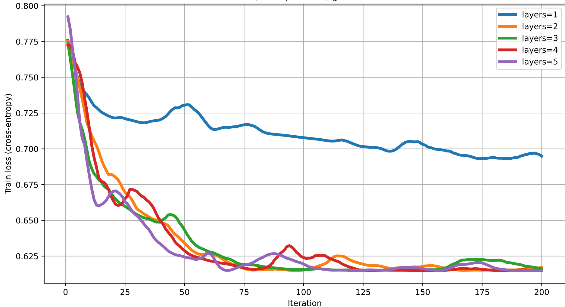
Train loss vs Iteration (dim=9) rot=RX, ent=pairwise, gate=CNOT
