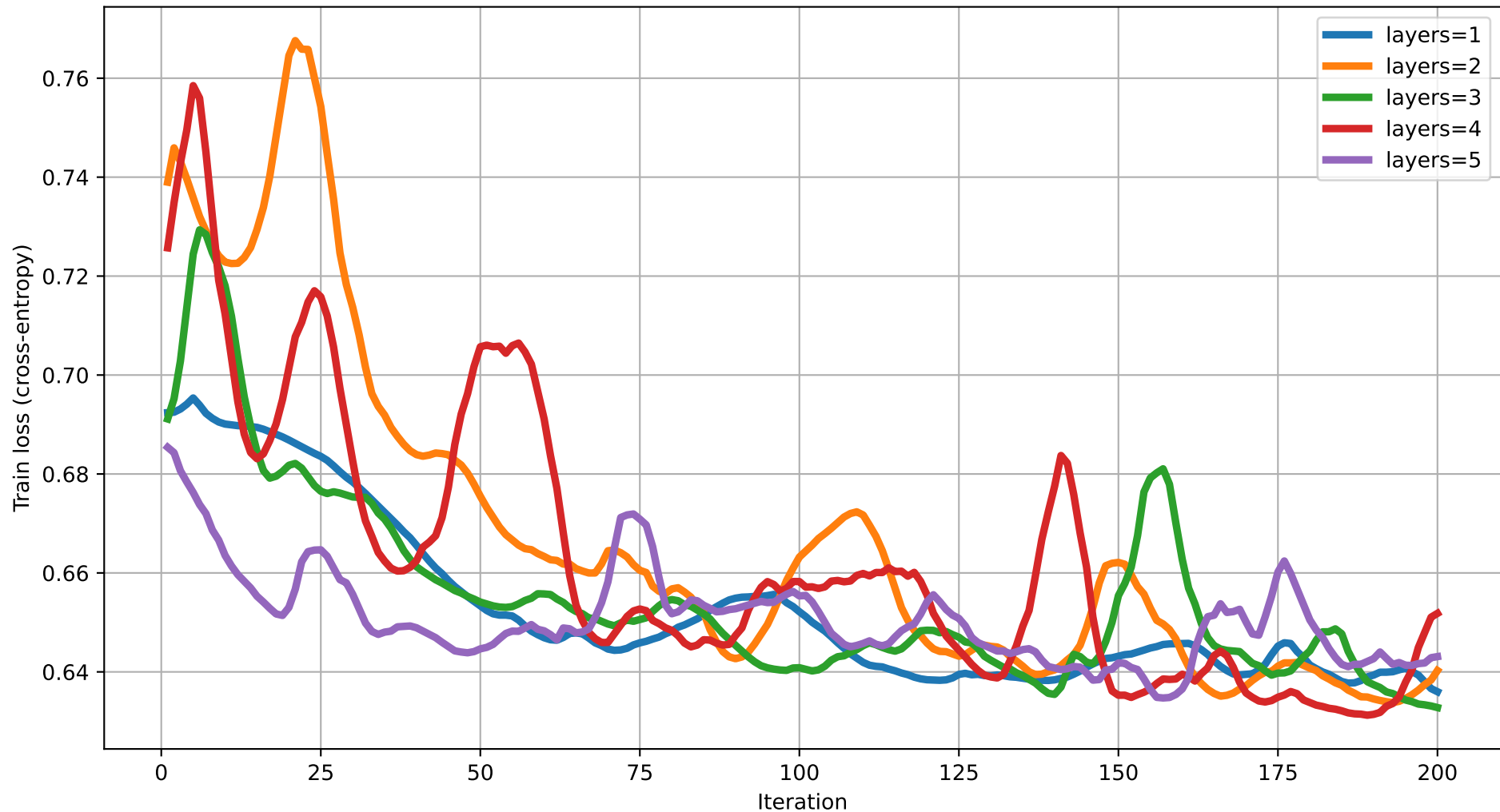
Train loss vs Iteration (dim=3) rot=RYZ, ent=chain, gate=IsingXX
