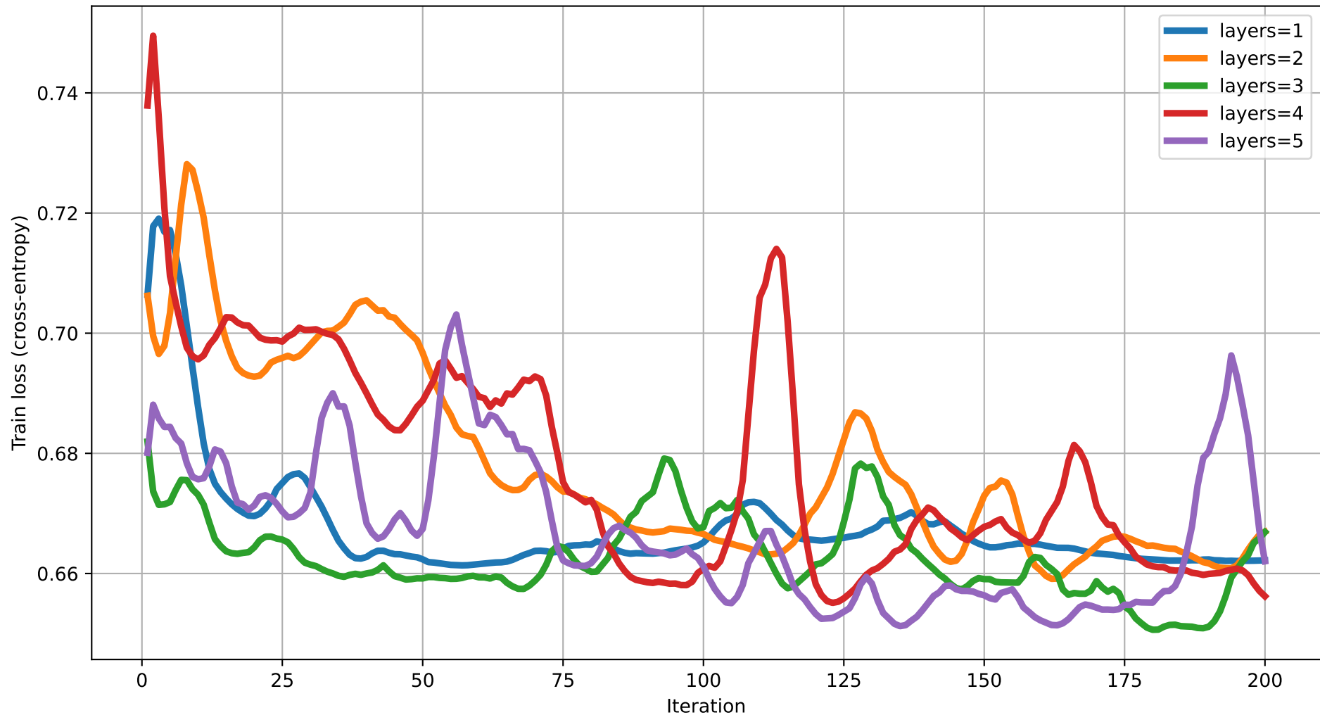
Train loss vs Iteration (dim=11) rot=RYZ, ent=ring, gate=IsingXX
