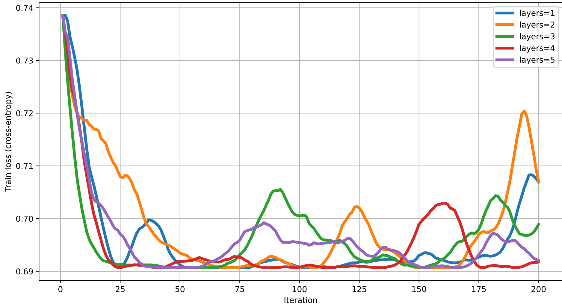
Train loss vs Iteration (dim=16) rot=RZ, ent=full, gate=CNOT
