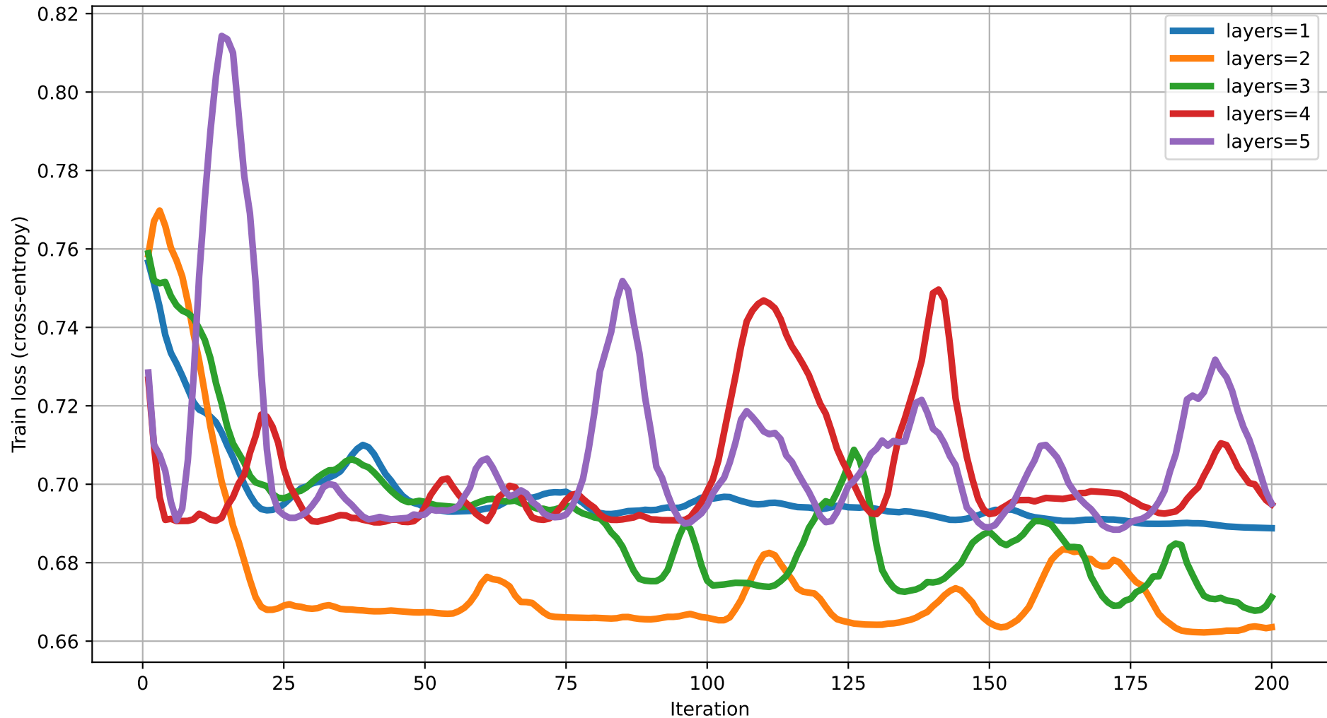
Train loss vs Iteration (dim=16) rot=RY, ent=pairwise, gate=CNOT
