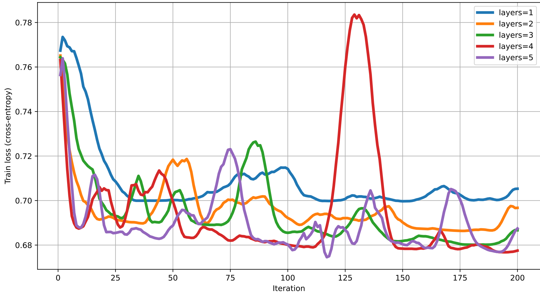
Train loss vs Iteration (dim=17) rot=Rot, ent=chain, gate=CZ
