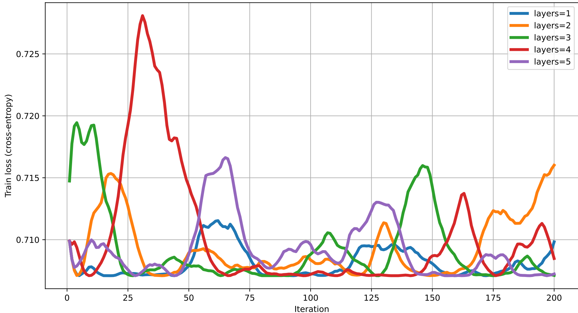
Train loss vs Iteration (dim=6) rot=RZ, ent=full, gate=CNOT
