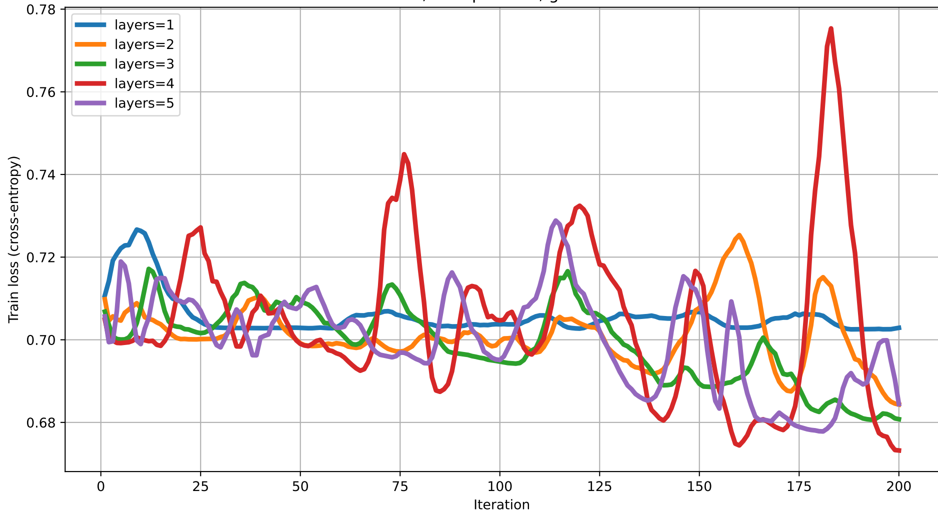
Train loss vs Iteration (dim=11) rot=Rot, ent=pairwise, gate=CNOT
