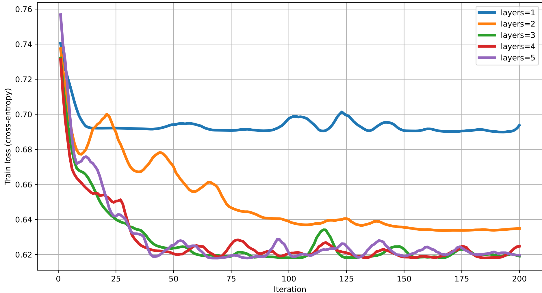
Train loss vs Iteration (degree=5) rot=RY, ent=pairwise, gate=CNOT
