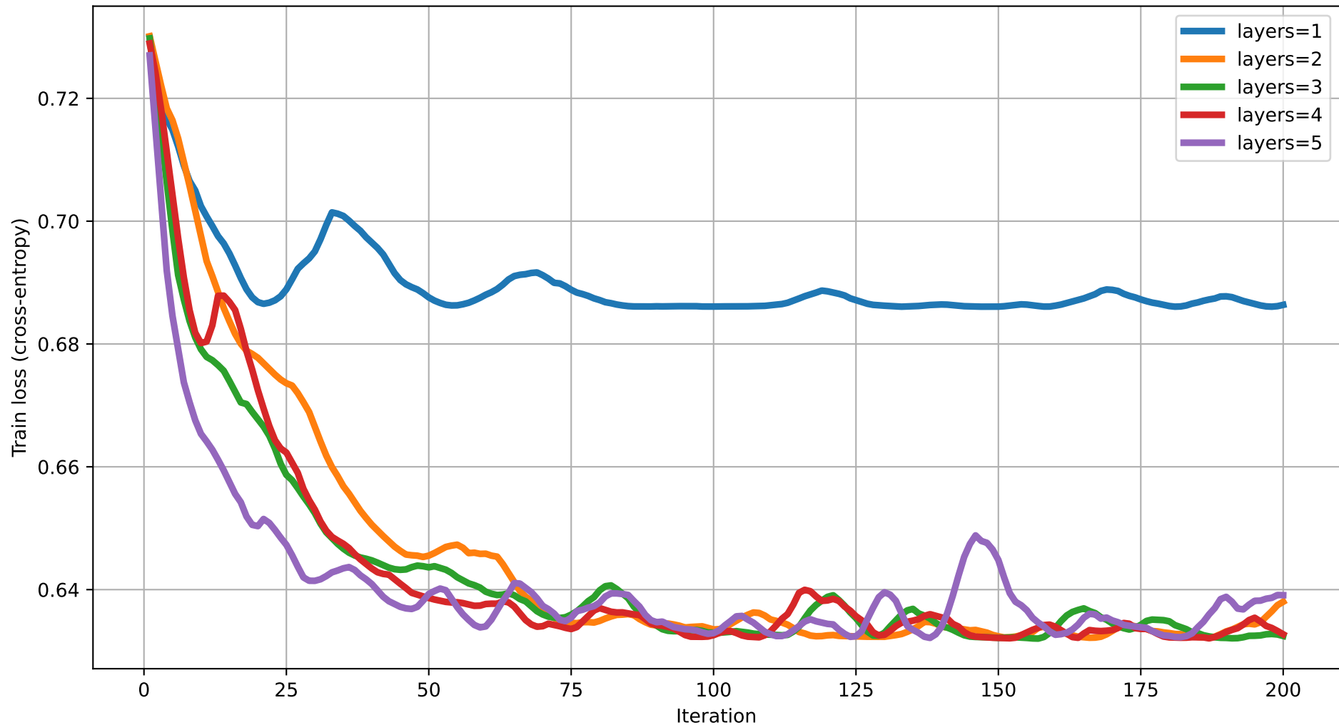
Train loss vs Iteration (degree=2) rot=RX, ent=pairwise, gate=CZ
