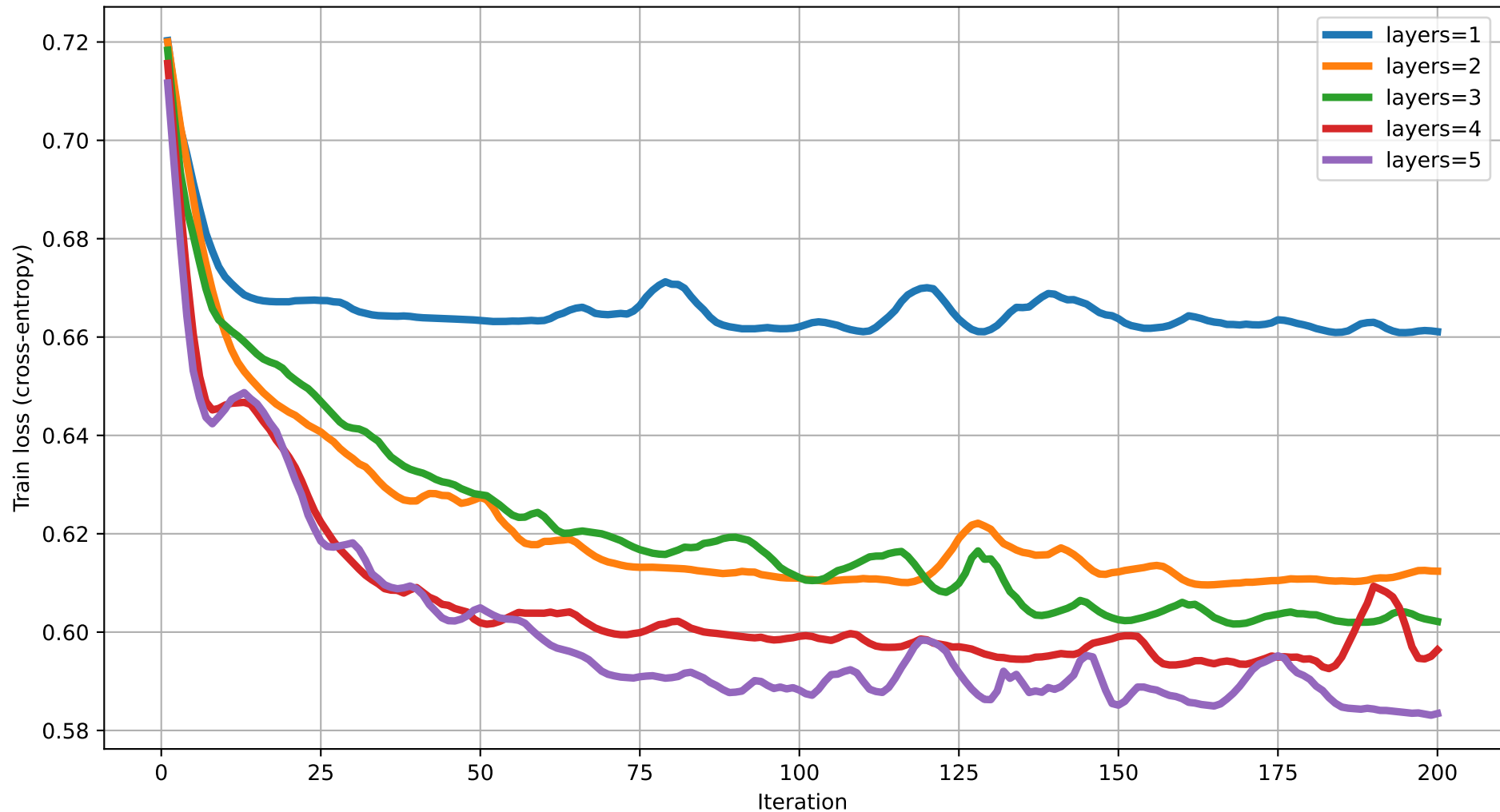
Train loss vs Iteration (degree=3) rot=RYZ, ent=full, gate=CZ
