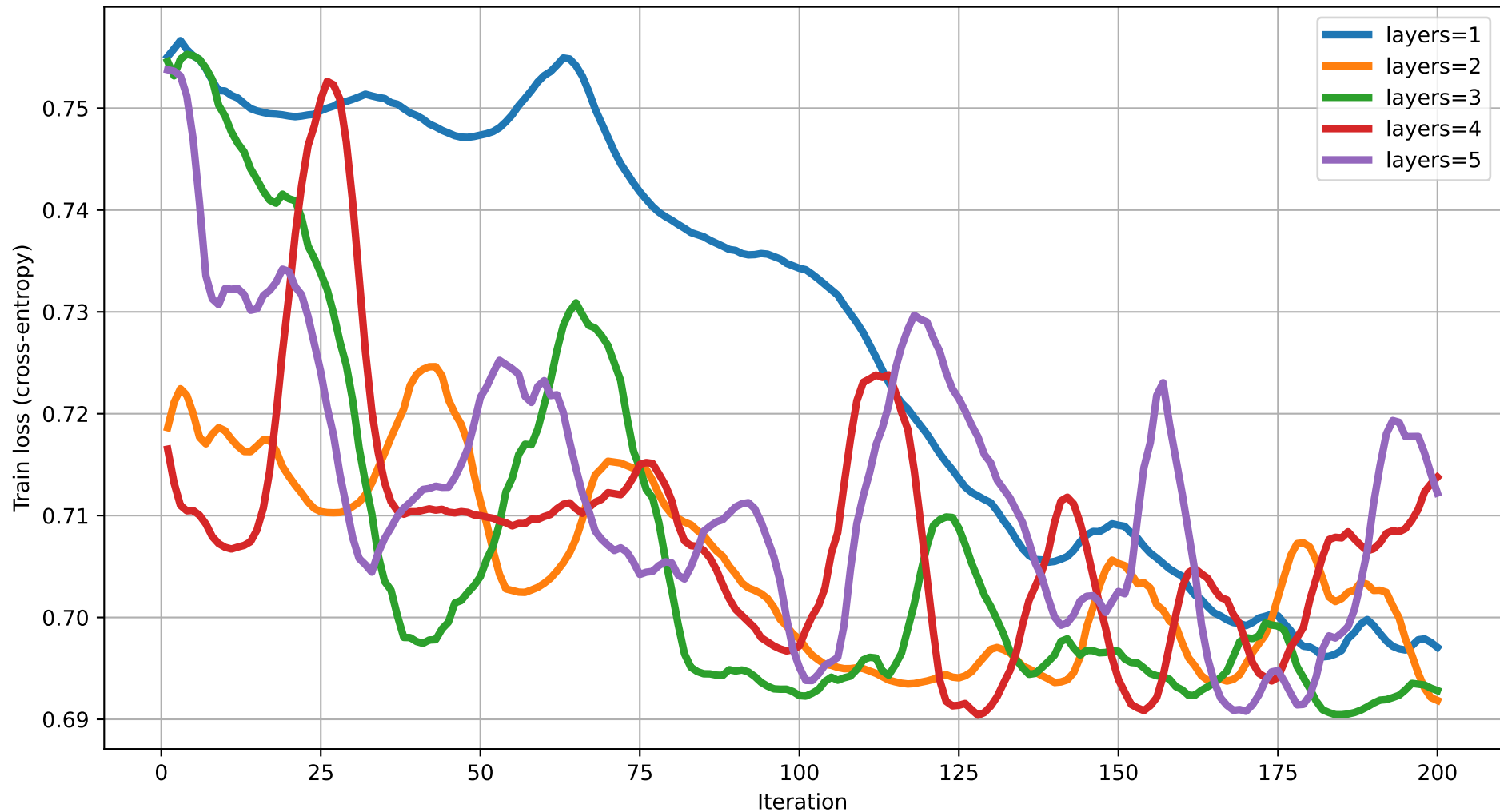
Train loss vs Iteration (dim=3) rot=Rot, ent=ring, gate=IsingXX
