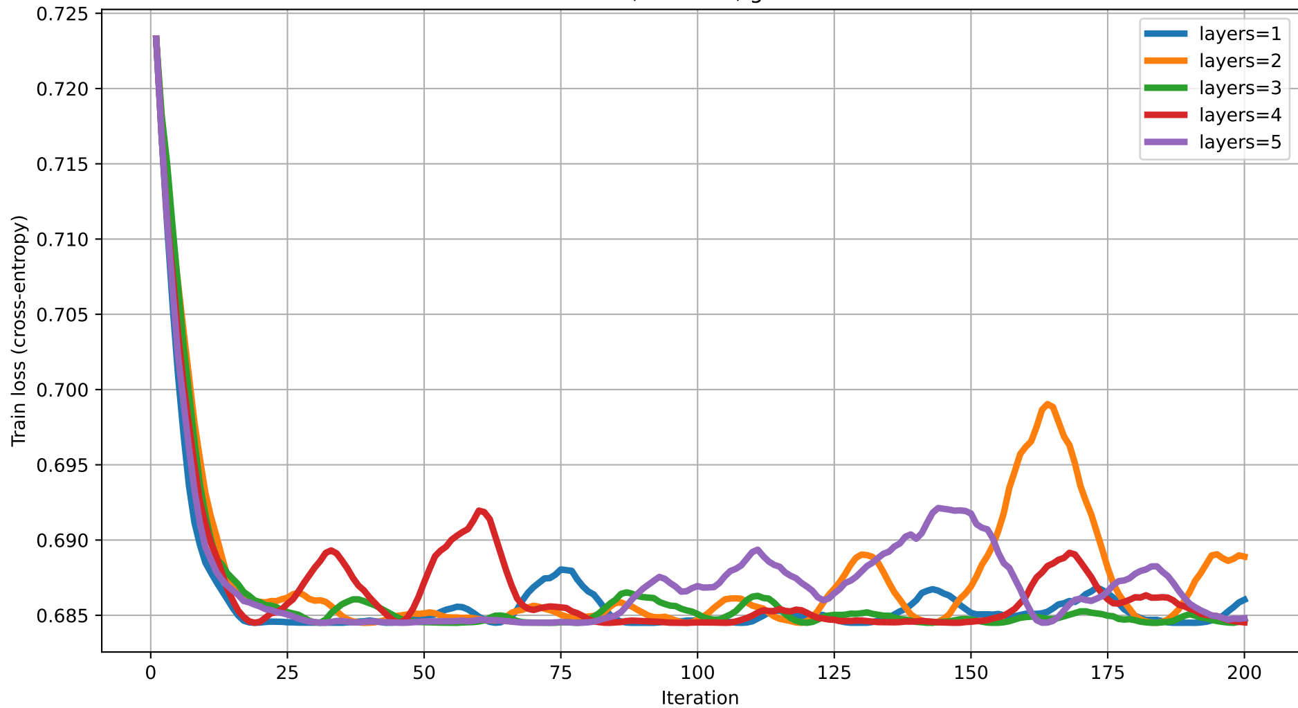
Train loss vs Iteration (degree=3) rot=RZ, ent=full, gate=CZ
