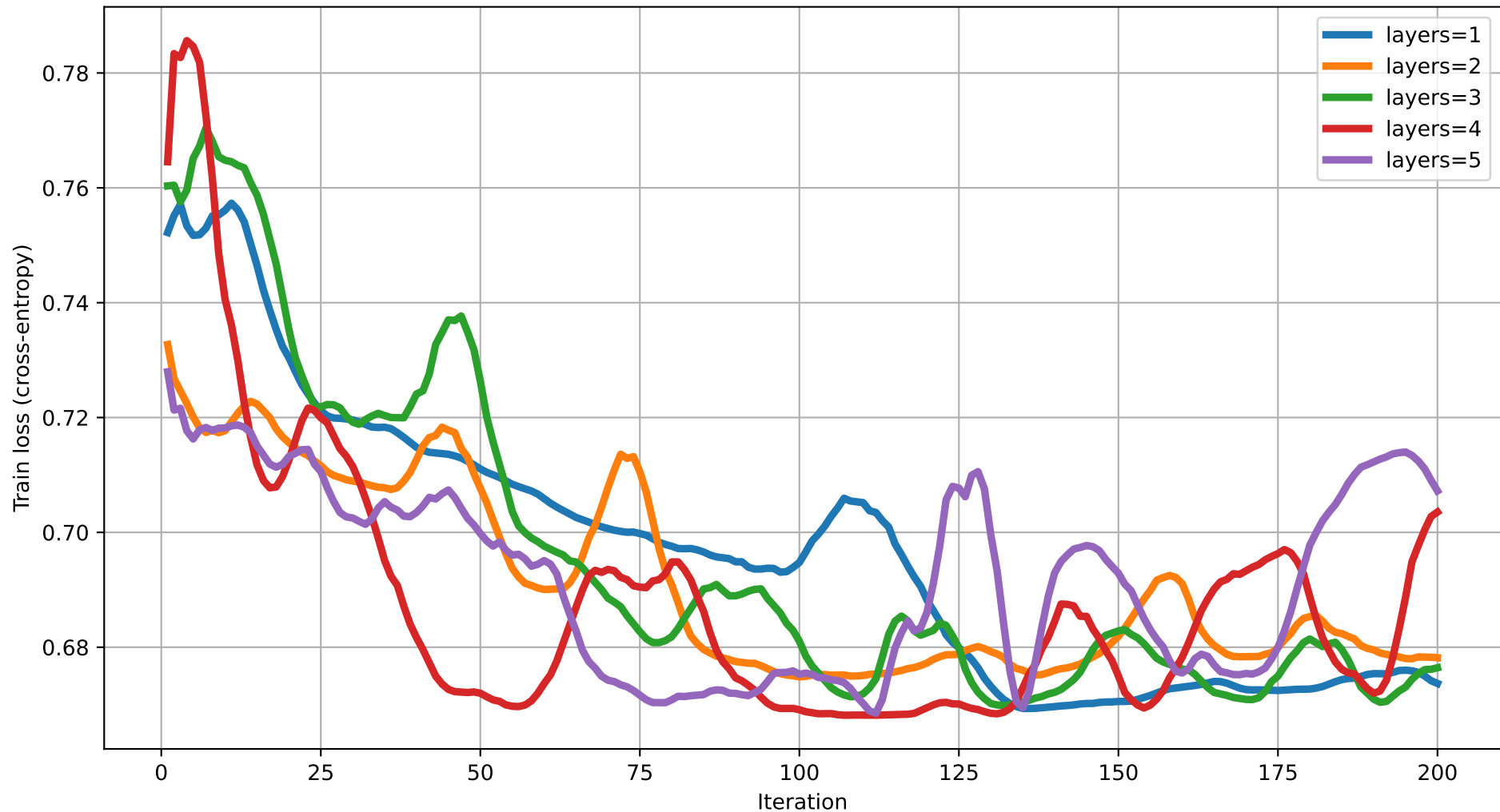
Train loss vs Iteration (dim=3) rot=RY, ent=ring, gate=CZ
