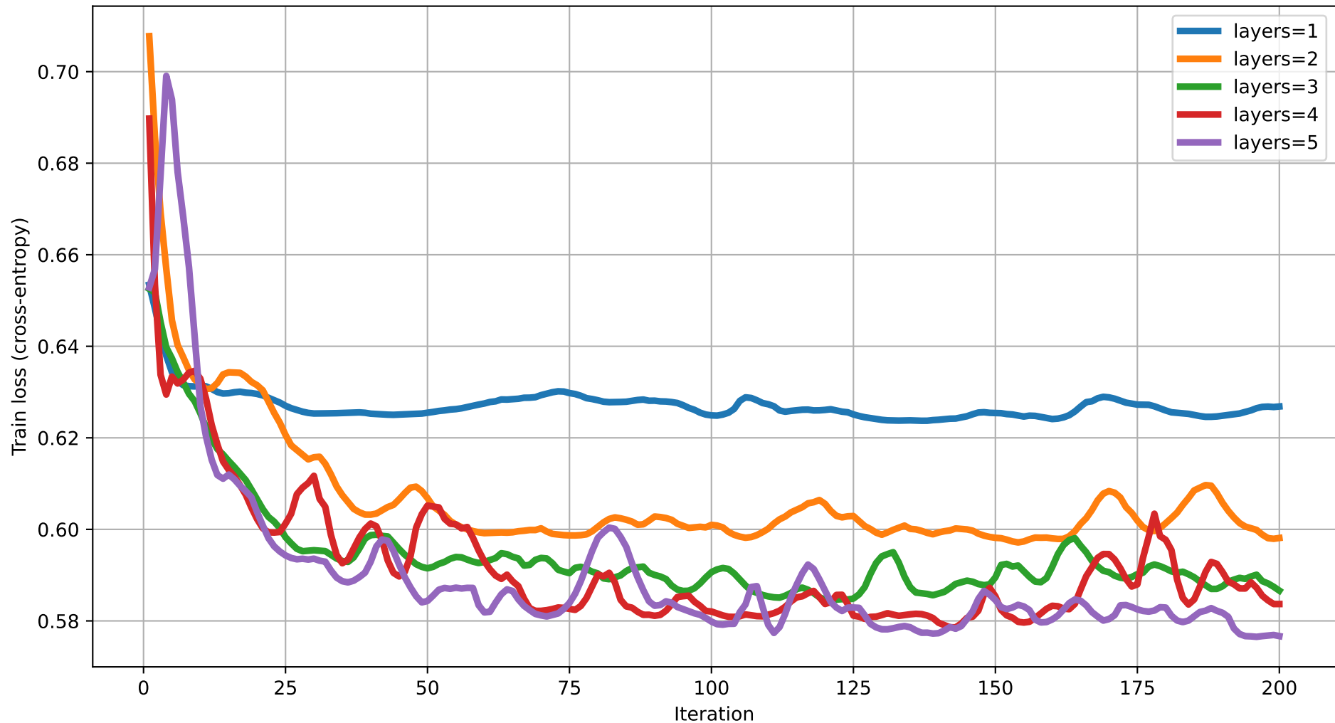
Train loss vs Iteration (degree=3) rot=Rot, ent=ring, gate=IsingXX
