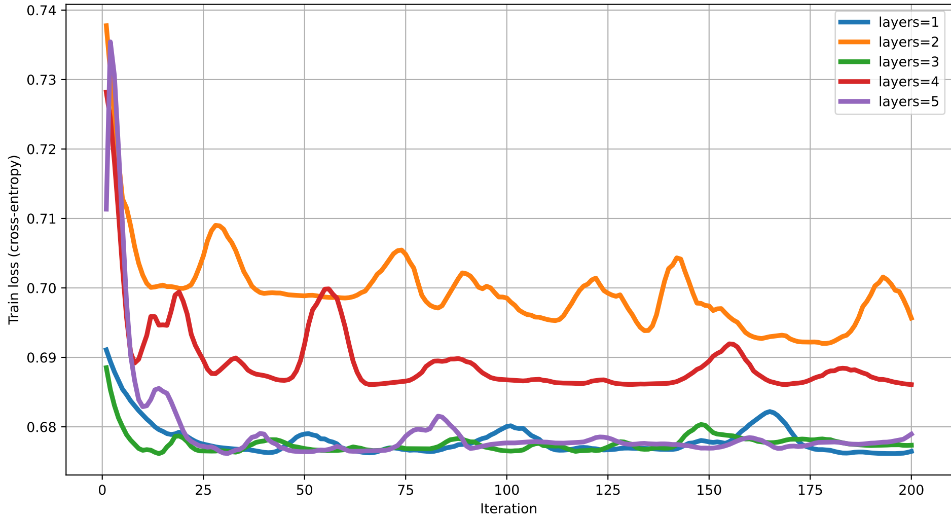
Train loss vs Iteration (degree=2) rot=RX, ent=pairwise, gate=IsingXX
