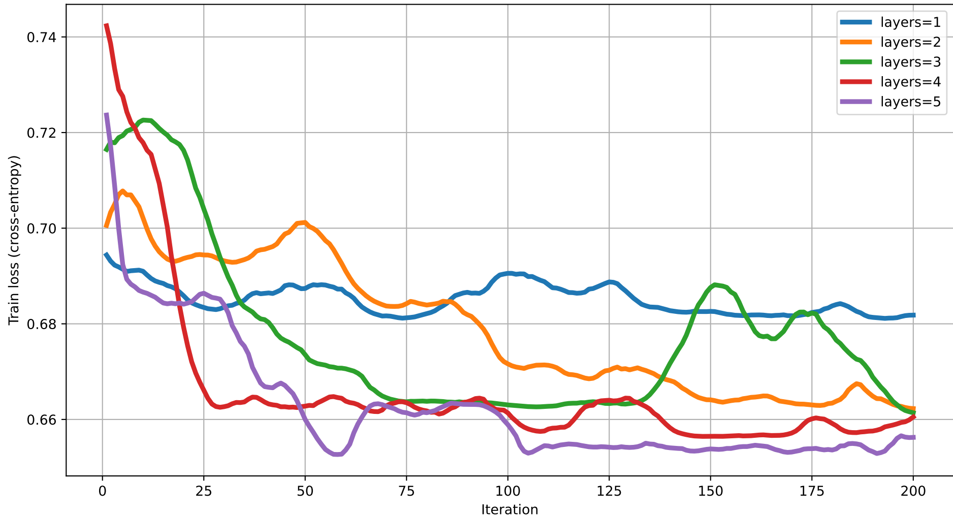
Train loss vs Iteration (dim=9) rot=RX, ent=ring, gate=CNOT
