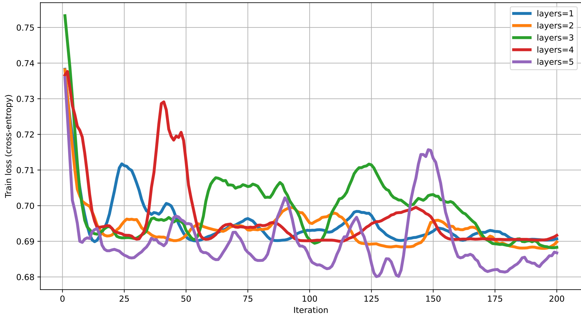
Train loss vs Iteration (dim=16) rot=RX, ent=full, gate=CZ
