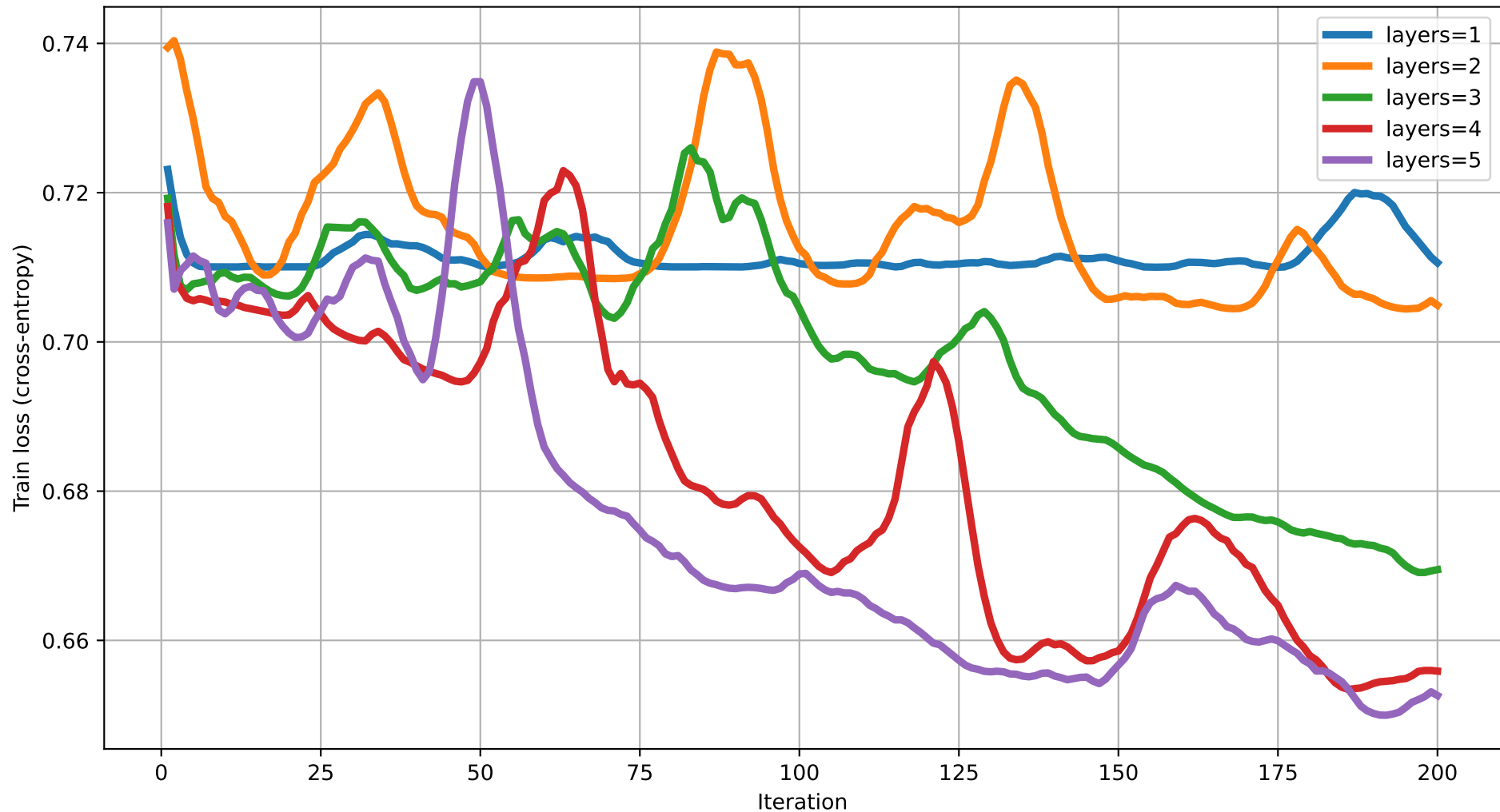
Train loss vs Iteration (dim=10) rot=RY, ent=chain, gate=CNOT
