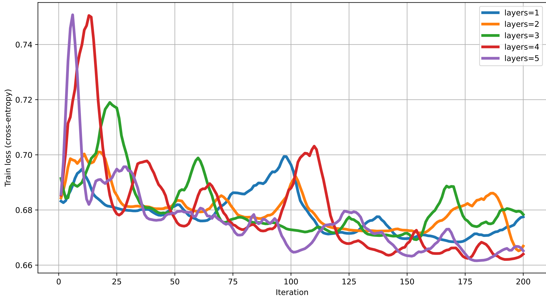
Train loss vs Iteration (dim=15) rot=RYZ, ent=chain, gate=CNOT
