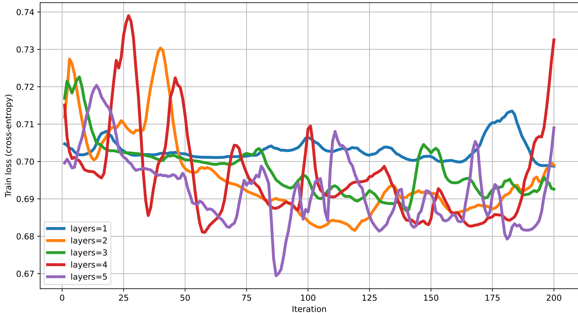
Train loss vs Iteration (dim=12) rot=Rot, ent=full, gate=CNOT
