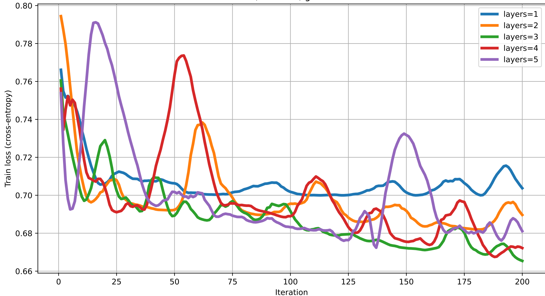
Train loss vs Iteration (dim=17) rot=RY, ent=full, gate=CNOT
