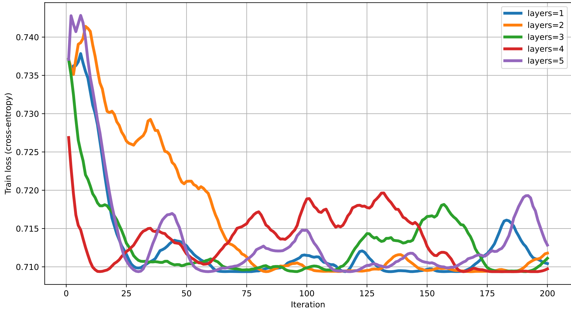
Train loss vs Iteration (dim=5) rot=RZ, ent=chain, gate=CNOT
