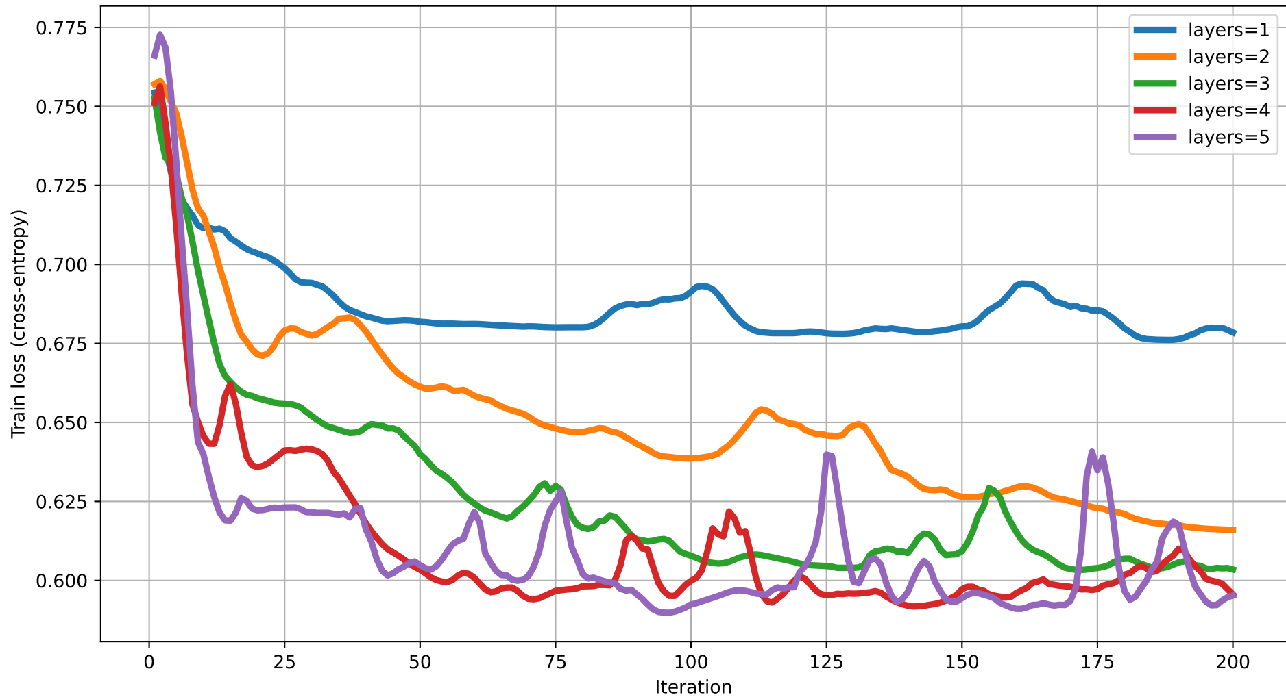
Train loss vs Iteration (dim=19) rot=Rot, ent=chain, gate=CNOT
