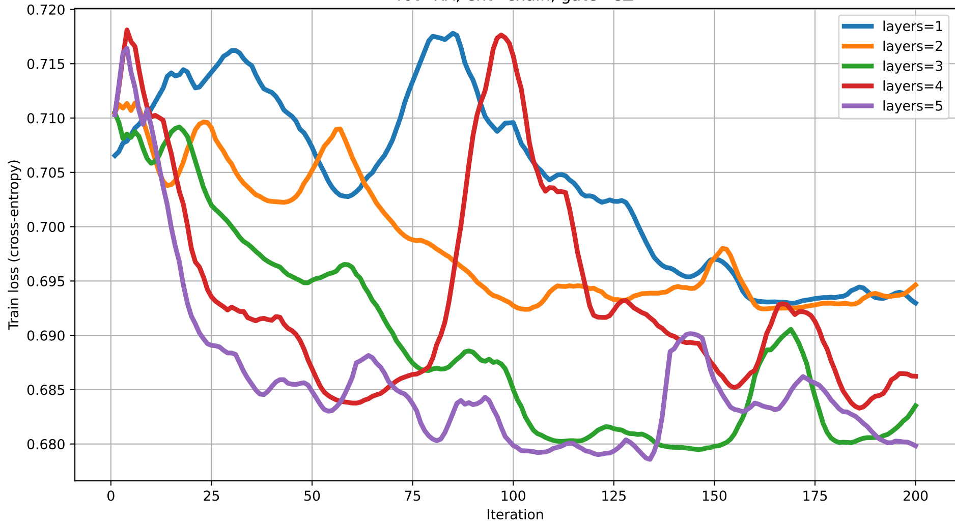
Train loss vs Iteration (dim=14) rot=RX, ent=chain, gate=CZ
