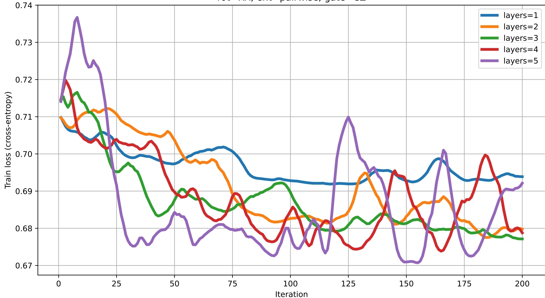
Train loss vs Iteration (dim=6) rot=RX, ent=pairwise, gate=CZ
