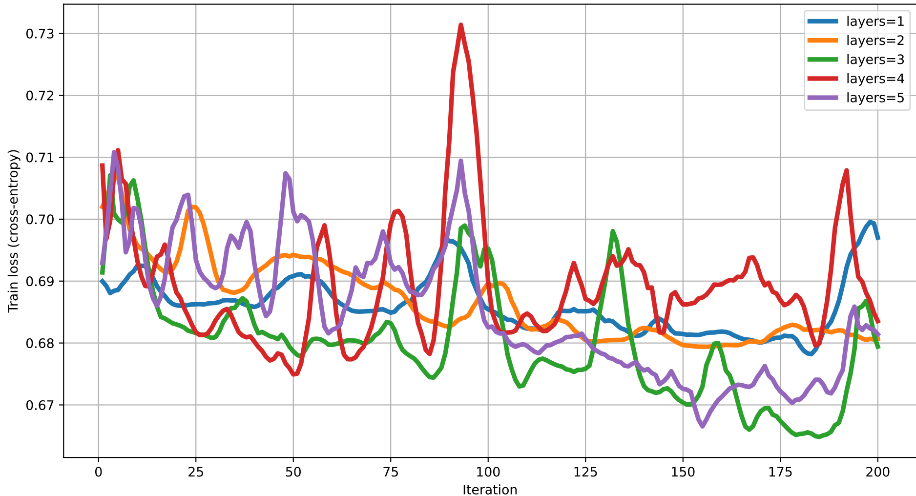
Train loss vs Iteration (dim=14) rot=Rot, ent=ring, gate=IsingXX
