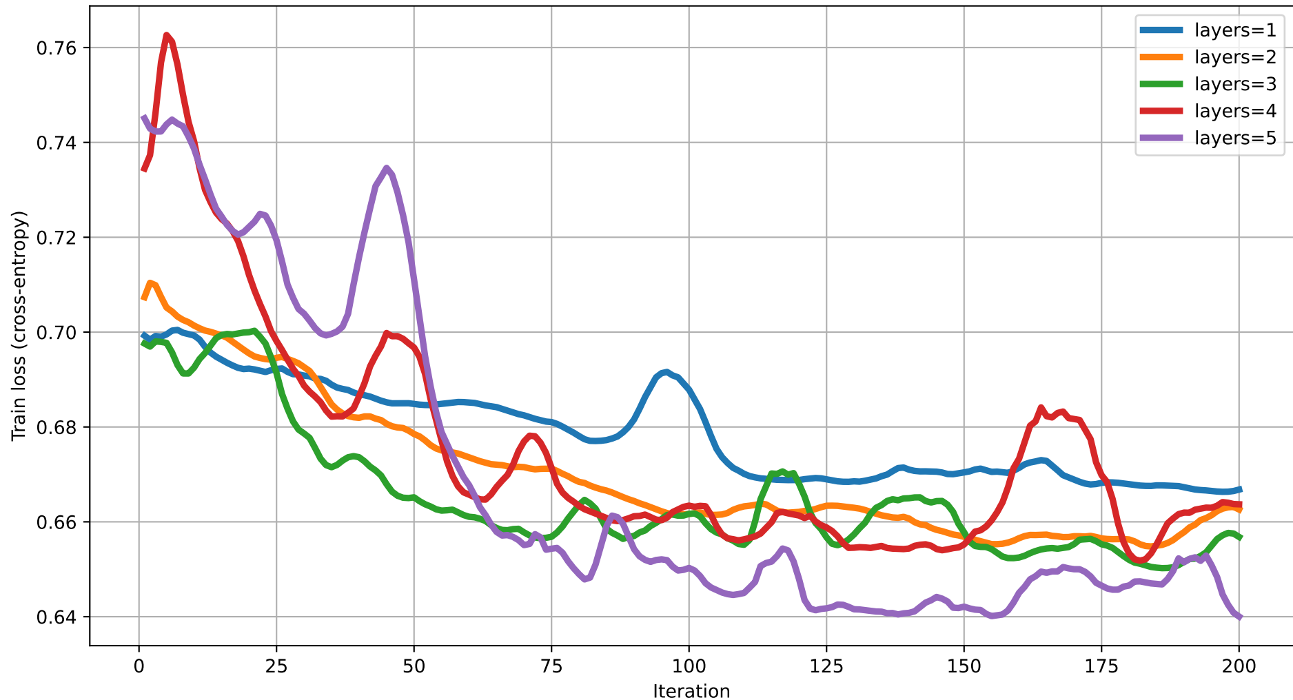
Train loss vs Iteration (dim=6) rot=RY, ent=ring, gate=CNOT
