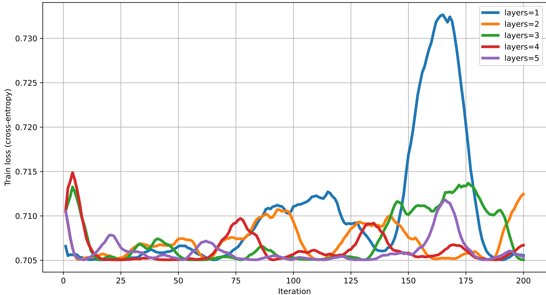
Train loss vs Iteration (dim=14) rot=RZ, ent=chain, gate=CNOT
