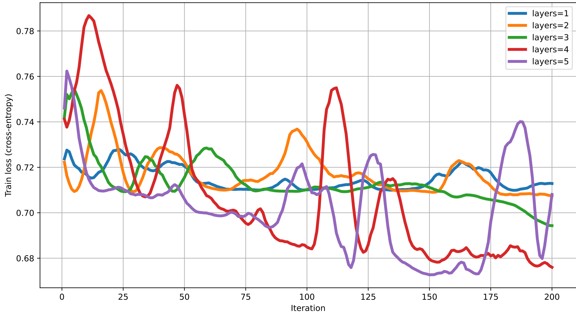
Train loss vs Iteration (dim=10) rot=RYZ, ent=pairwise, gate=CZ
