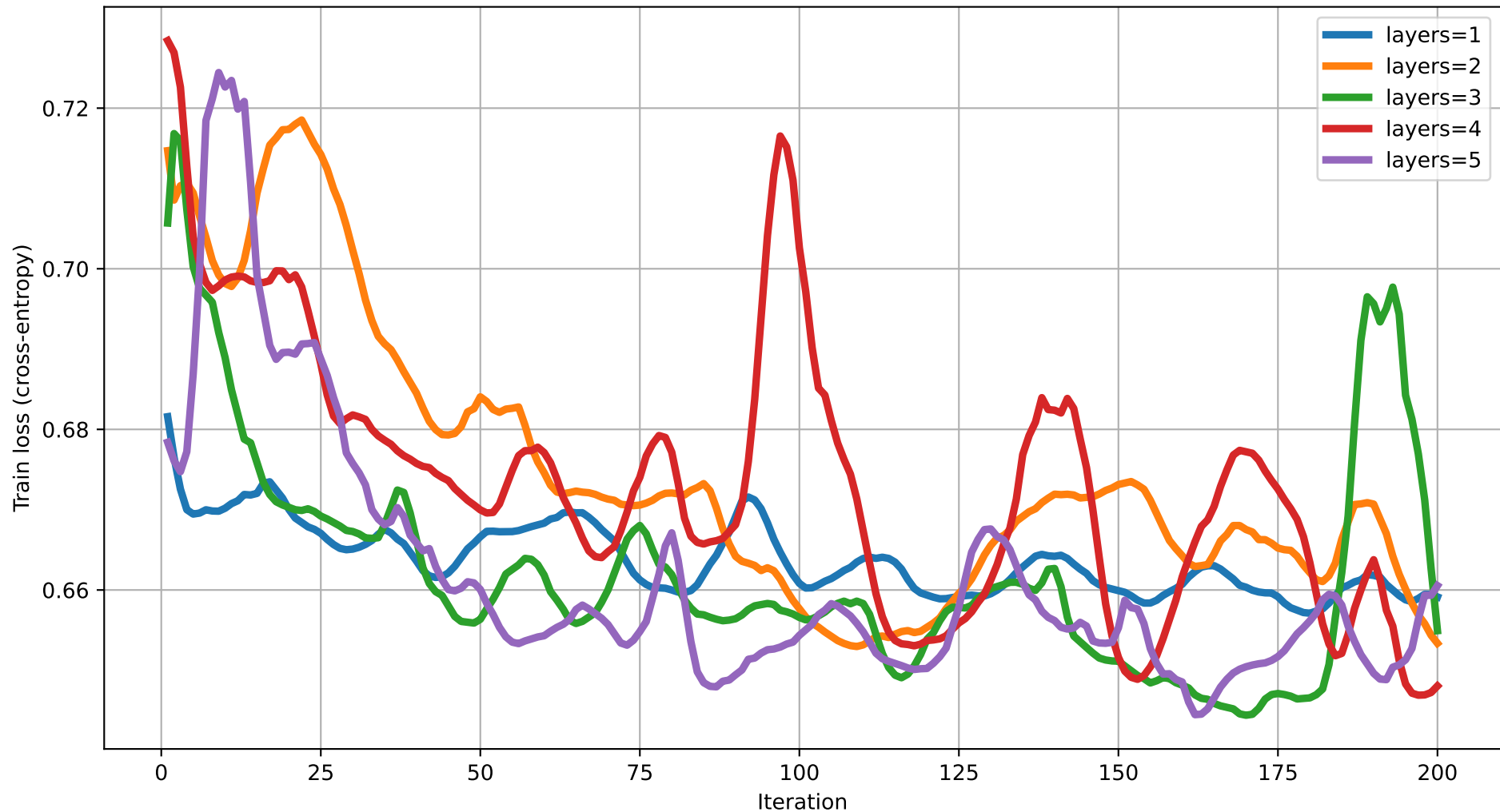
Train loss vs Iteration (dim=6) rot=RYZ, ent=full, gate=IsingXX
