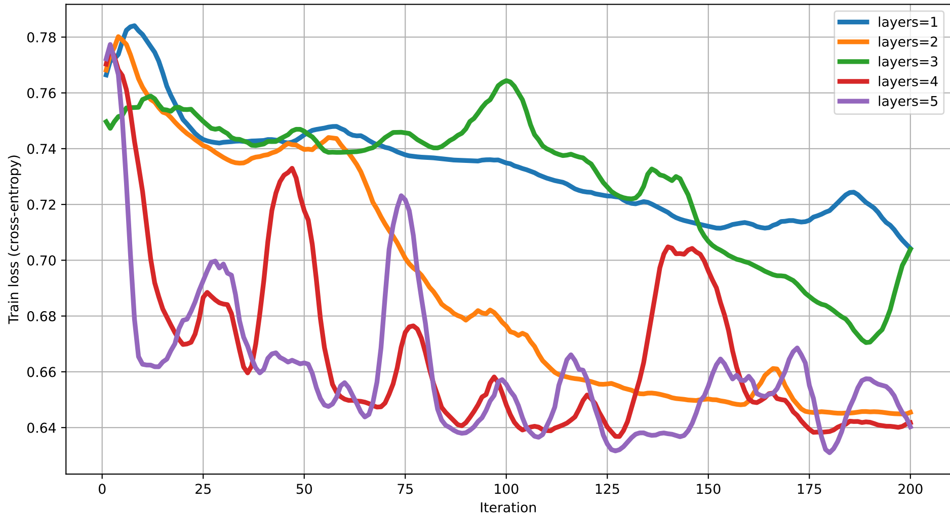
Train loss vs Iteration (dim=5) rot=RYZ, ent=chain, gate=CNOT
