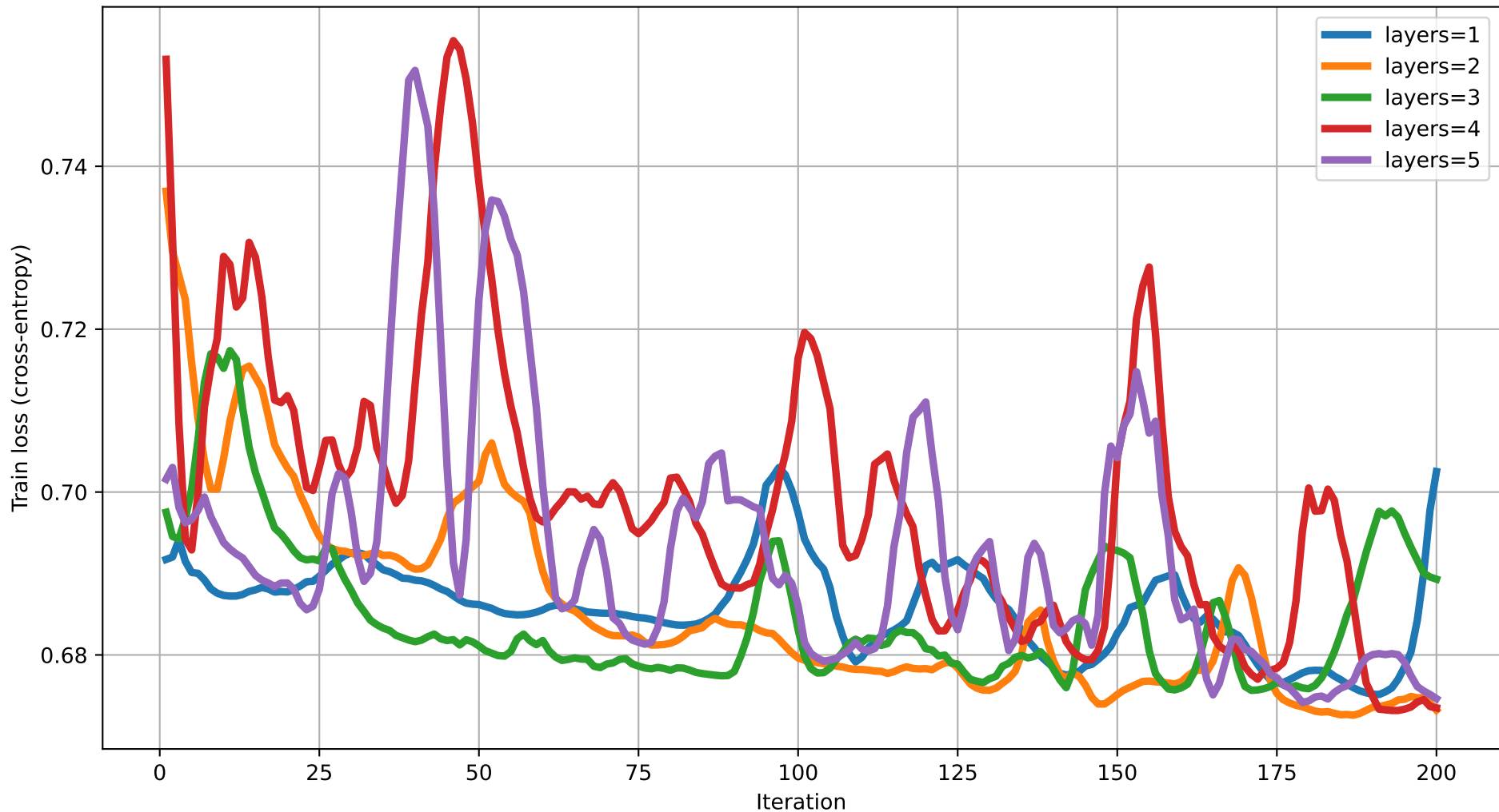
Train loss vs Iteration (dim=19) rot=Rot, ent=pairwise, gate=IsingXX
