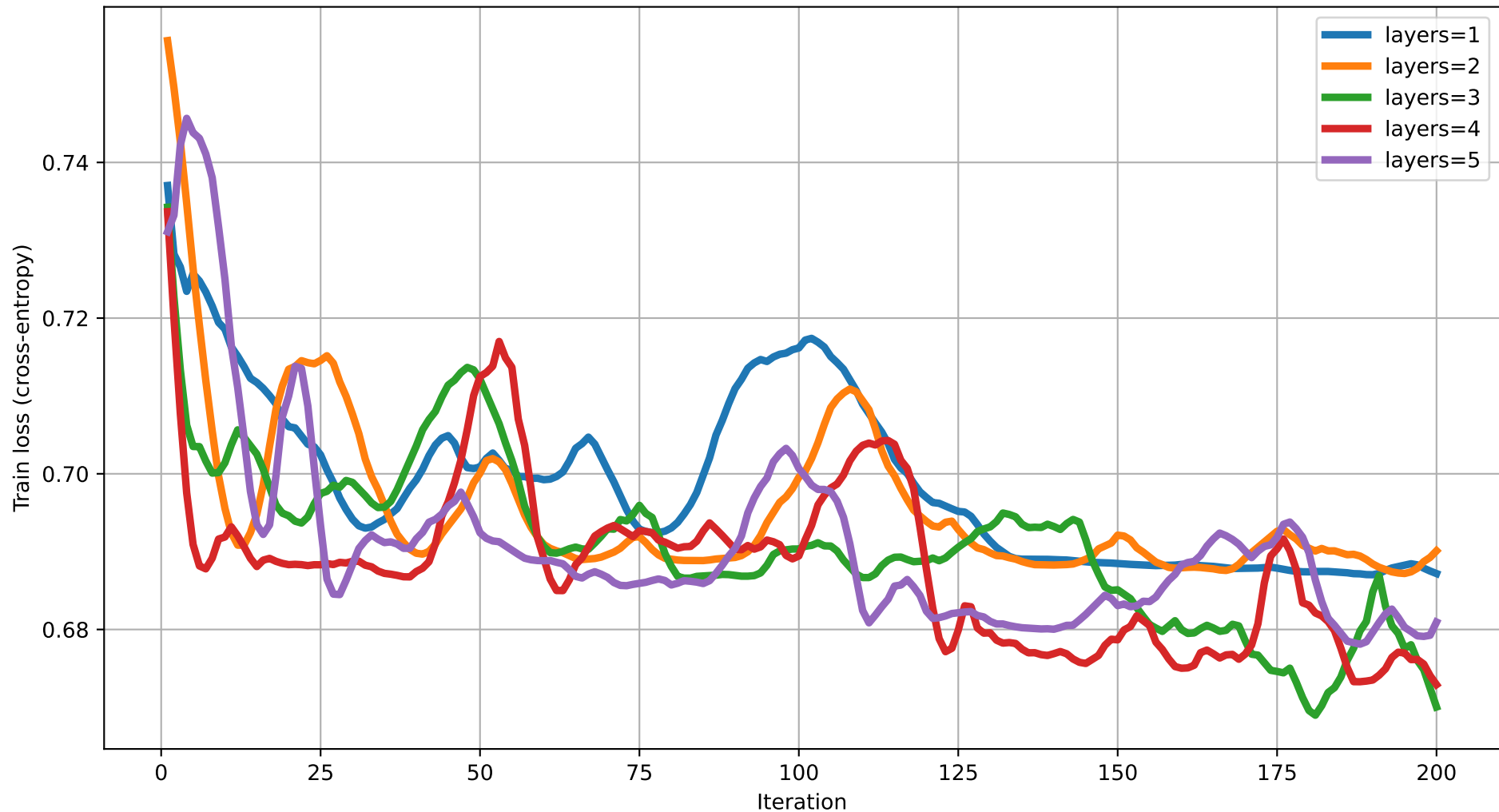
Train loss vs Iteration (dim=16) rot=RYZ, ent=full, gate=CZ
