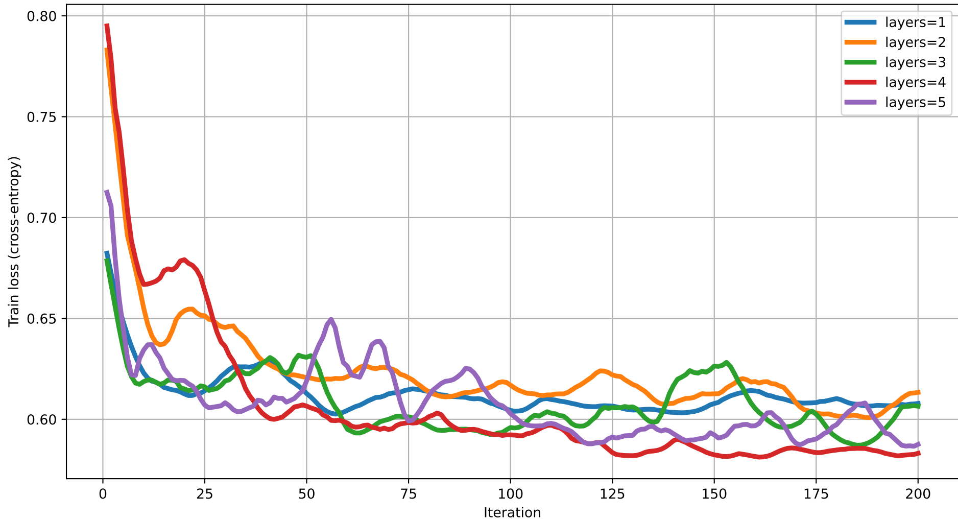
Train loss vs Iteration (dim=4) rot=RYZ, ent=full, gate=IsingXX
