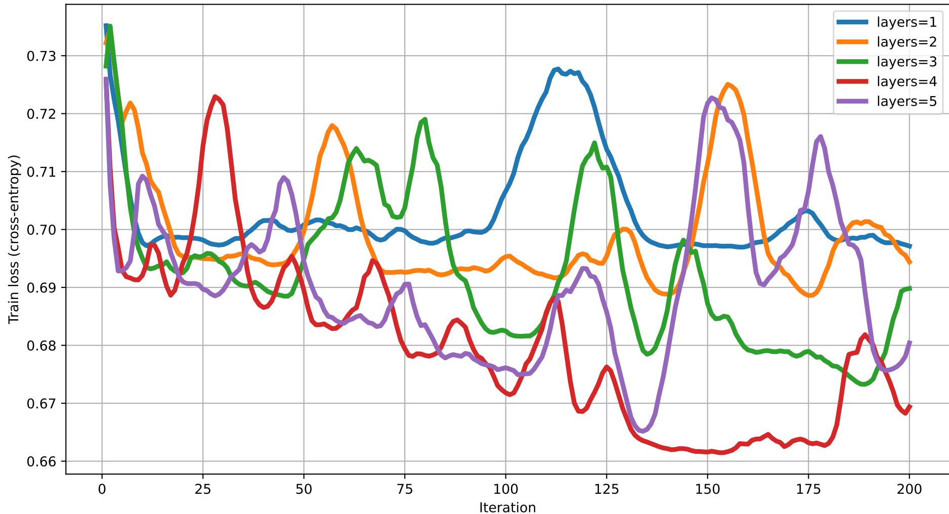
Train loss vs Iteration (dim=18) rot=RY, ent=full, gate=CNOT
