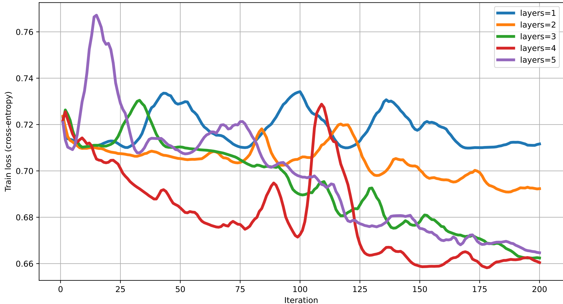
Train loss vs Iteration (dim=10) rot=RYZ, ent=ring, gate=CZ
