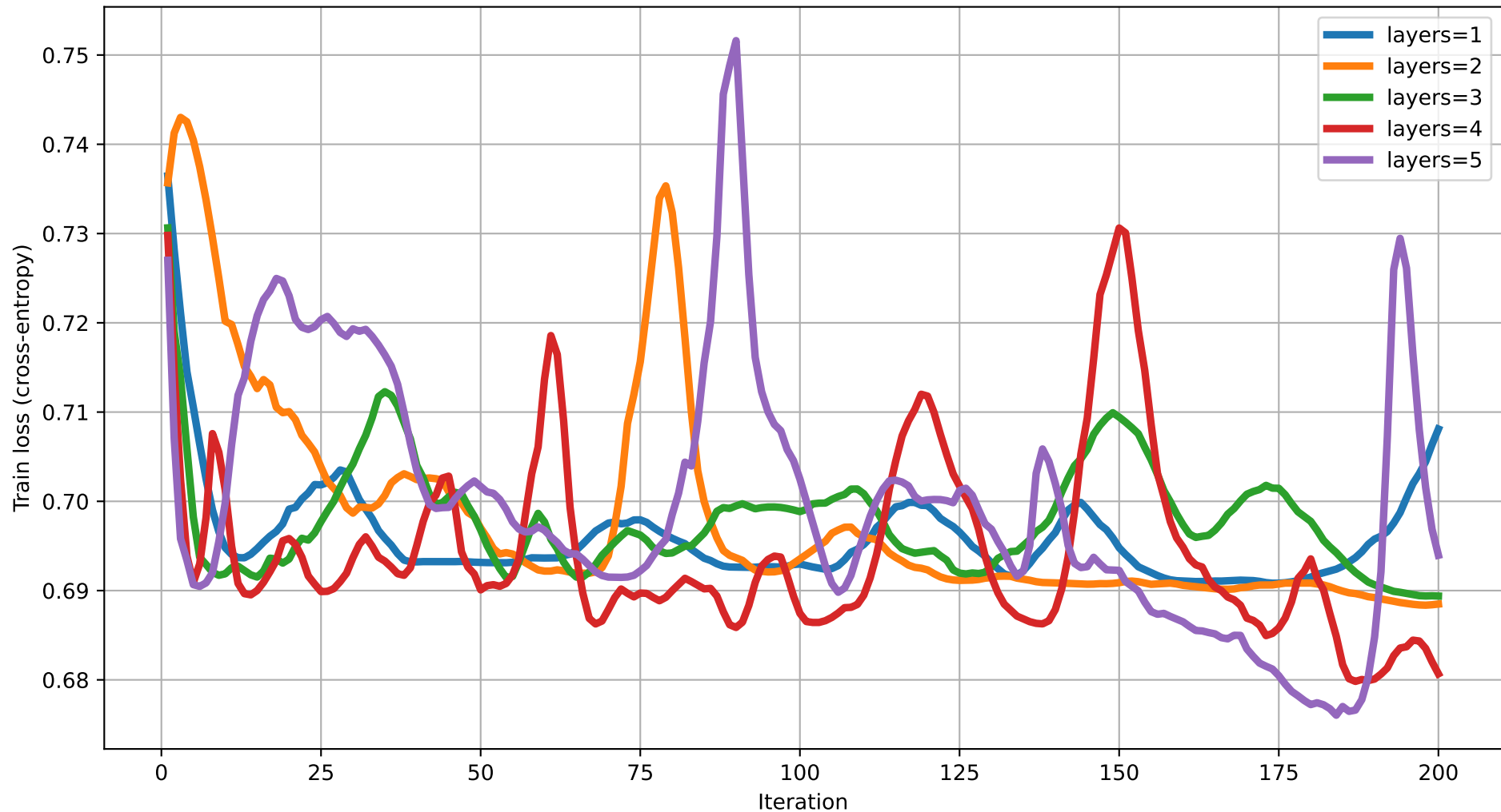
Train loss vs Iteration (dim=16) rot=Rot, ent=pairwise, gate=CNOT
