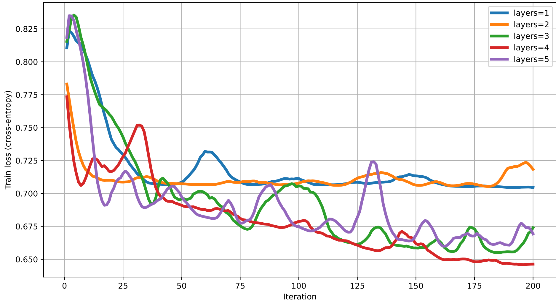
Train loss vs Iteration (dim=9) rot=RY, ent=full, gate=CZ
