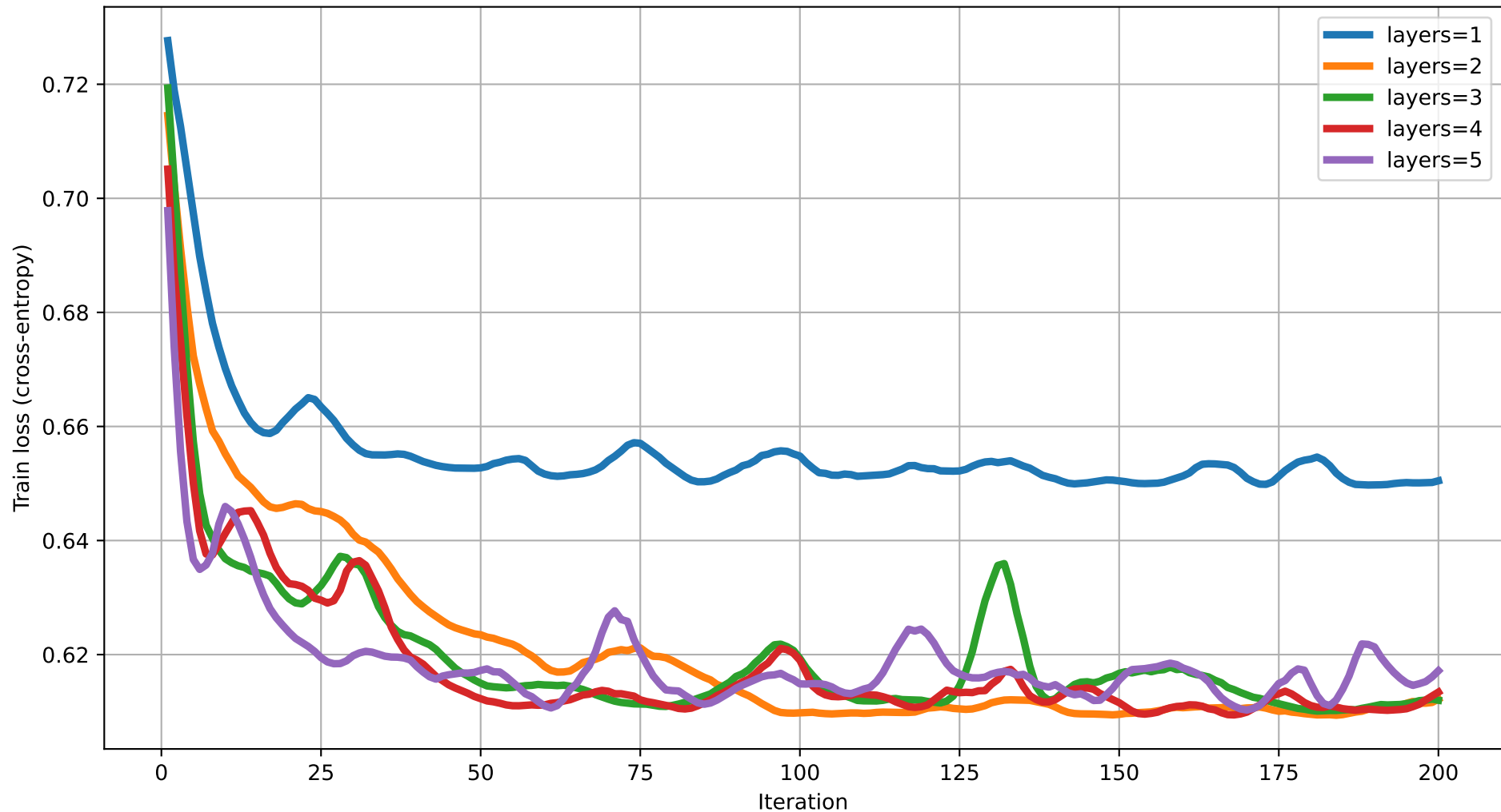
Train loss vs Iteration (degree=4) rot=RYZ, ent=pairwise, gate=CNOT
