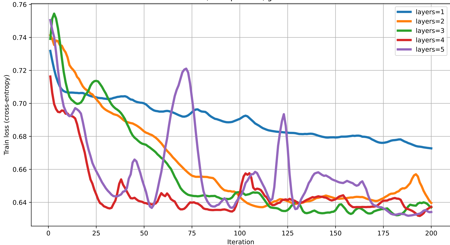
Train loss vs Iteration (dim=6) rot=RY, ent=pairwise, gate=CZ
