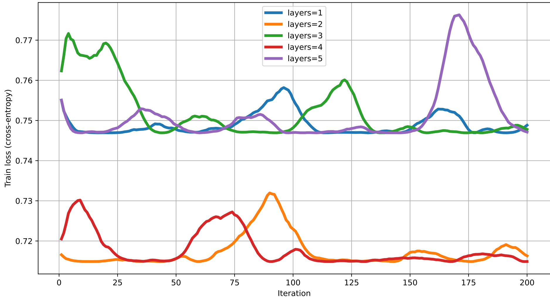
Train loss vs Iteration (dim=3) rot=RZ, ent=ring, gate=IsingXX
