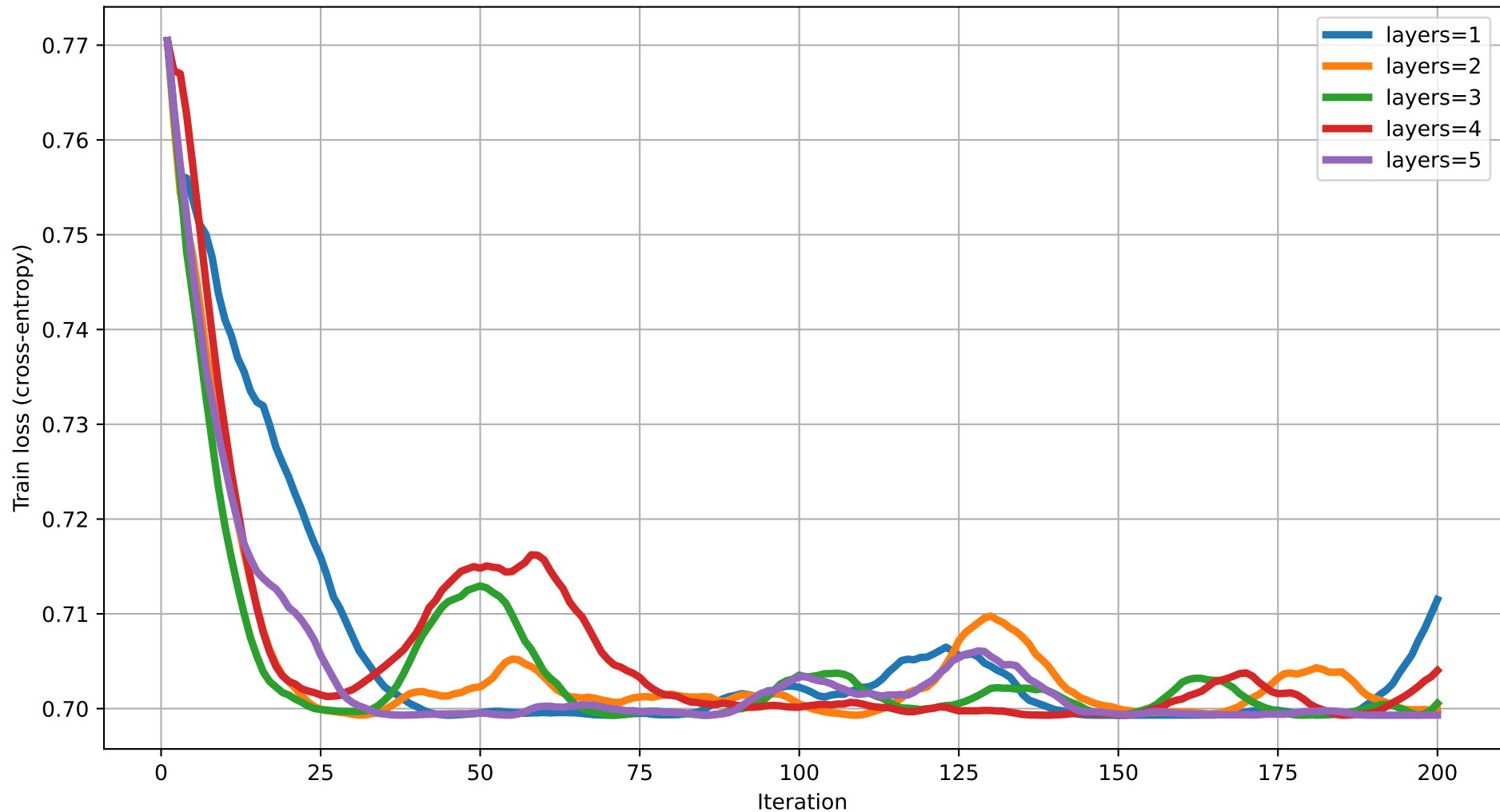
Train loss vs Iteration (dim=17) rot=RZ, ent=pairwise, gate=CZ
