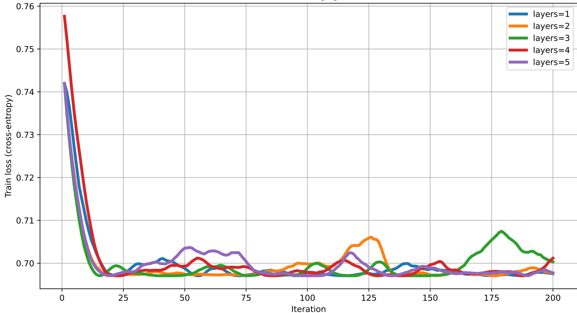
Train loss vs Iteration (degree=5) rot=RZ, ent=ring, gate=CZ
