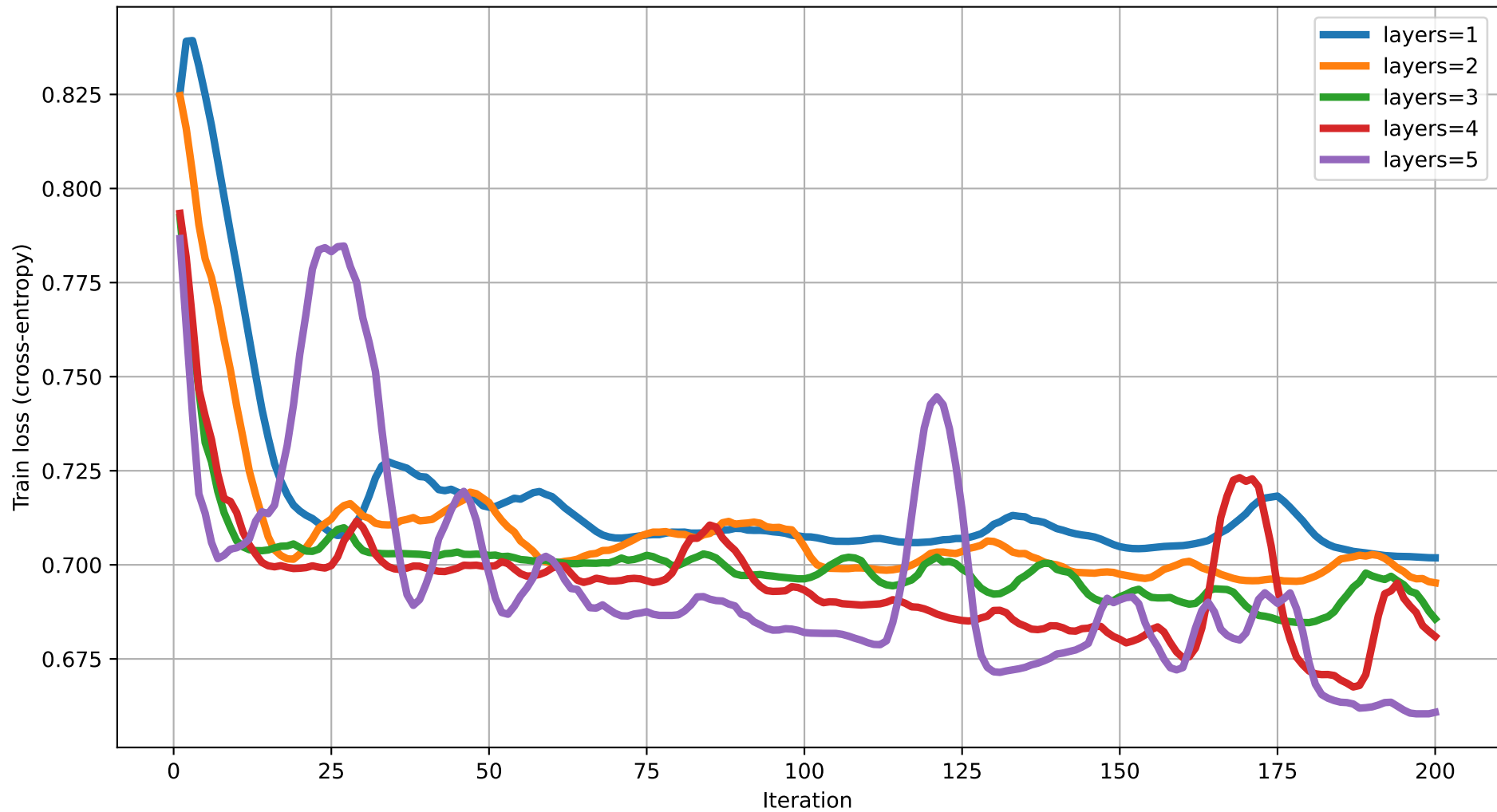
Train loss vs Iteration (dim=8) rot=RYZ, ent=pairwise, gate=CZ
