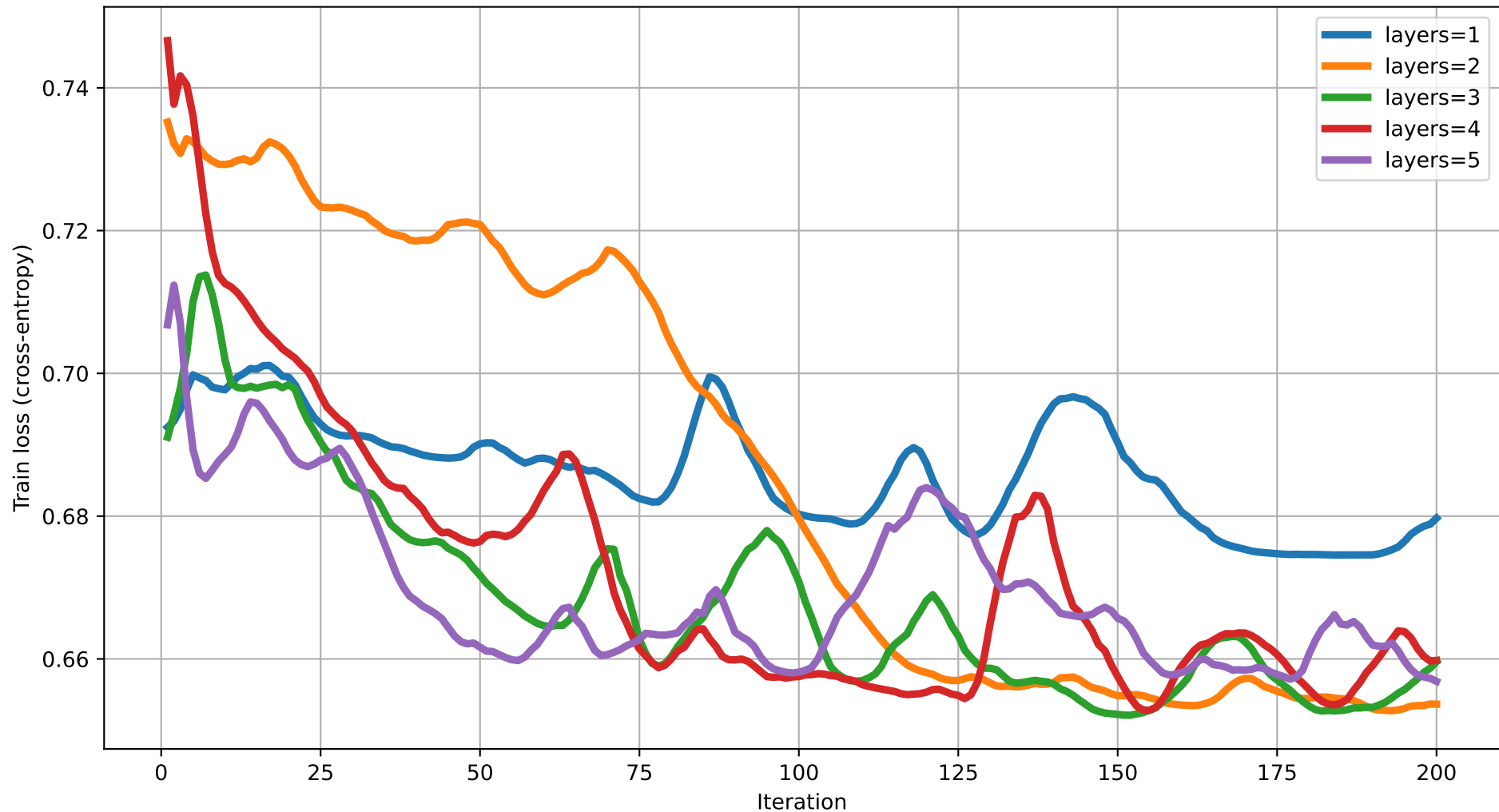
Train loss vs Iteration (dim=3) rot=RZ, ent=pairwise, gate=IsingXX
