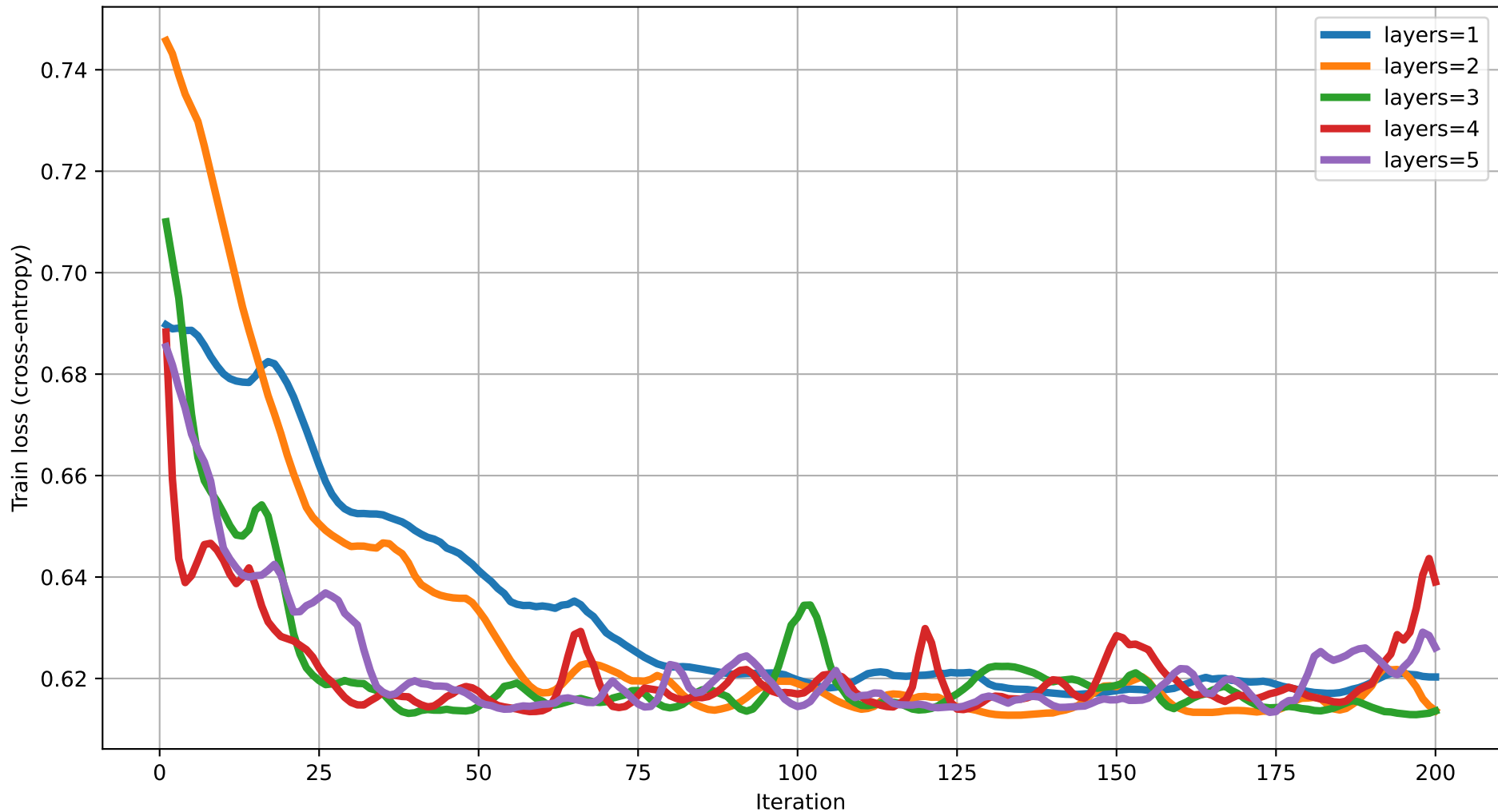
Train loss vs Iteration (degree=3) rot=Rot, ent=pairwise, gate=IsingXX
