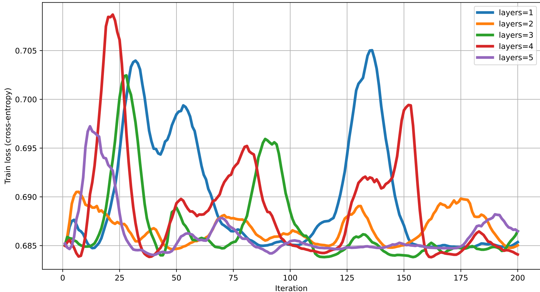
Train loss vs Iteration (dim=15) rot=RX, ent=pairwise, gate=CNOT
