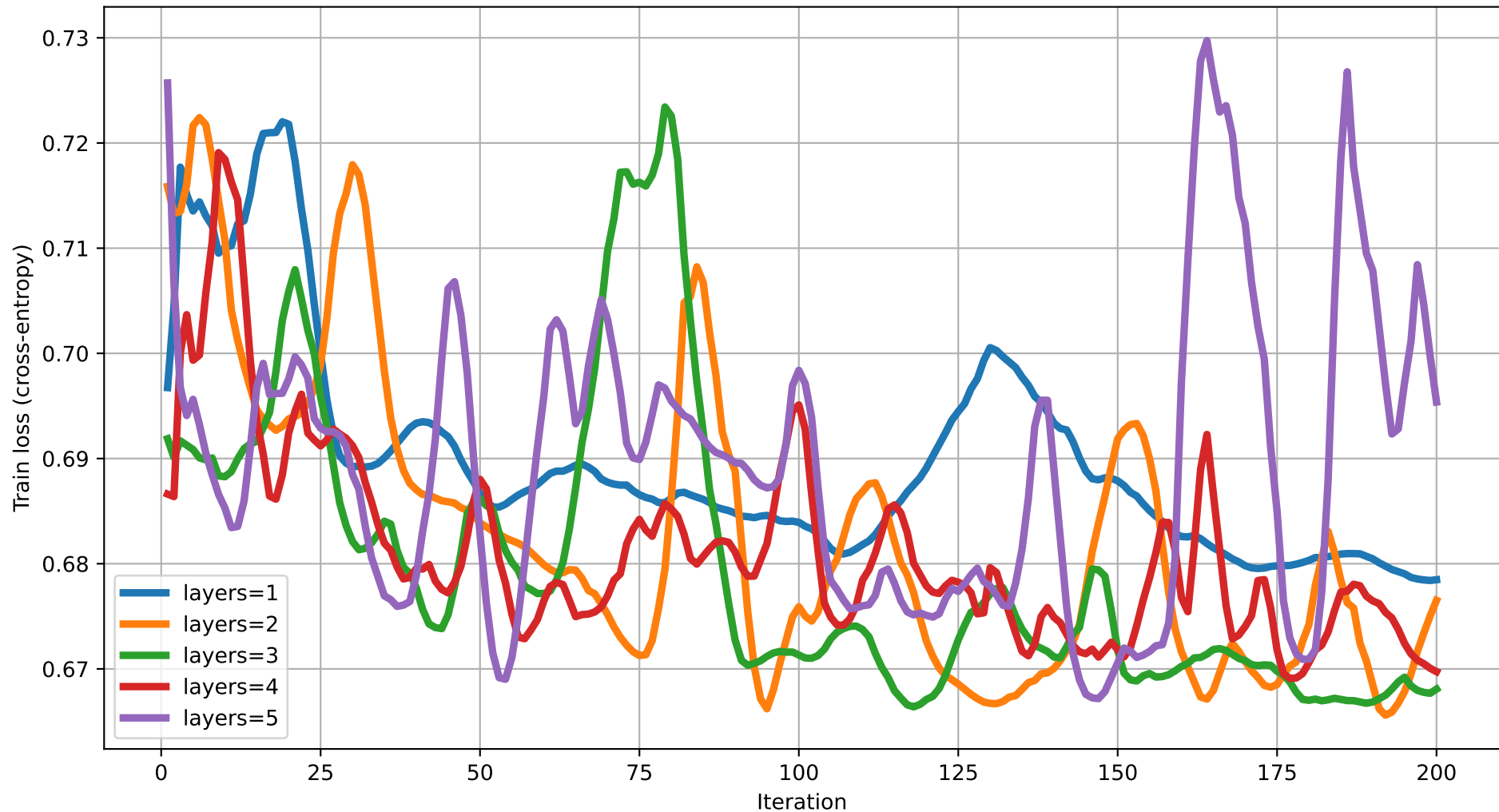
Train loss vs Iteration (dim=13) rot=Rot, ent=full, gate=IsingXX
