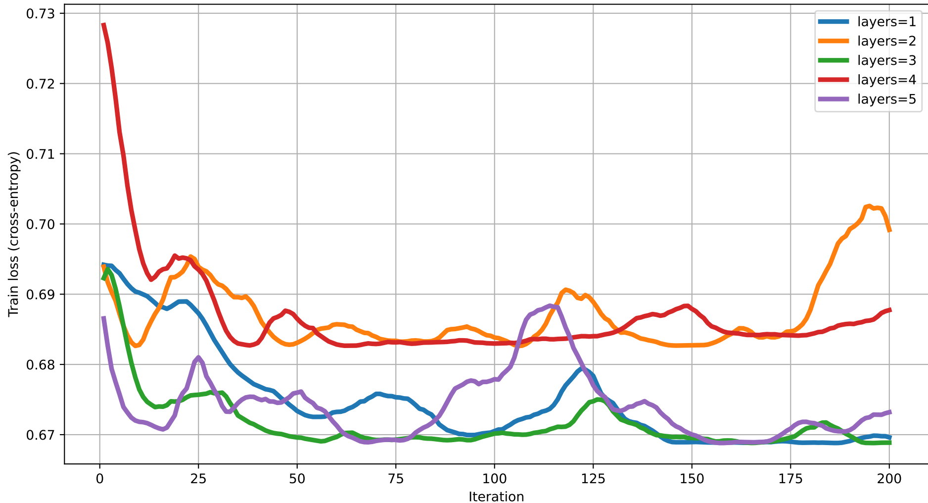
Train loss vs Iteration (dim=7) rot=RX, ent=pairwise, gate=IsingXX
