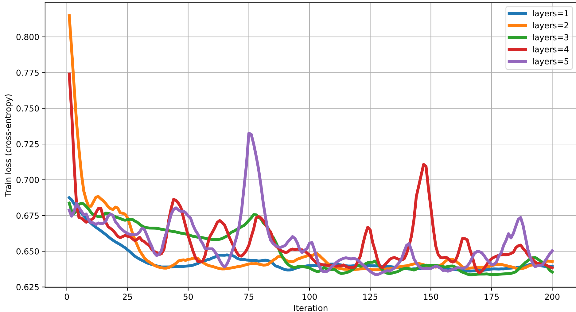
Train loss vs Iteration (dim=8) rot=Rot, ent=pairwise, gate=IsingXX
