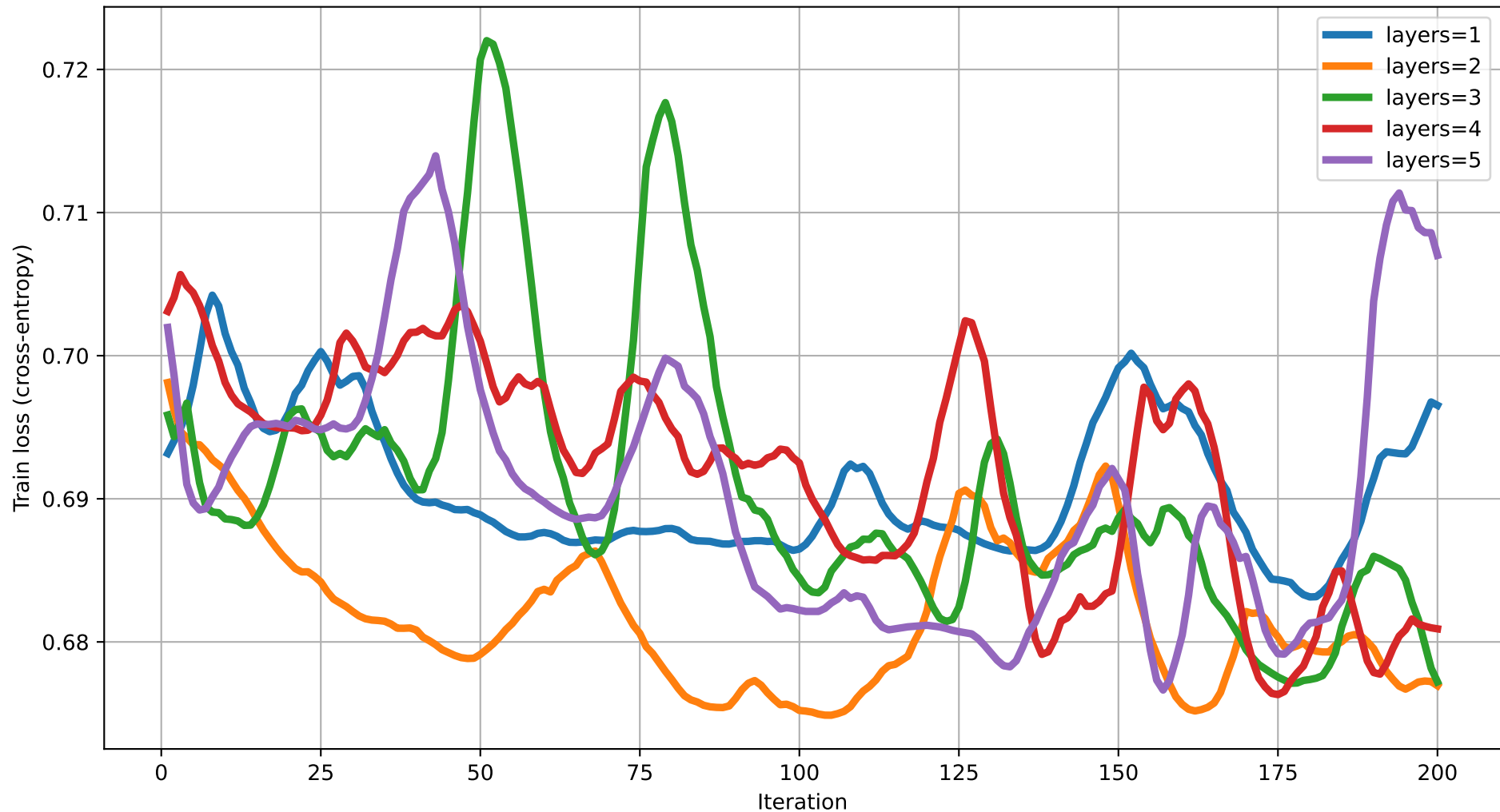
Train loss vs Iteration (dim=14) rot=RZ, ent=full, gate=IsingXX
