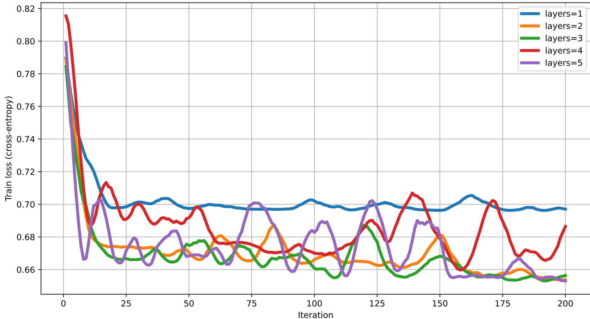
Train loss vs Iteration (dim=2) rot=RYZ, ent=chain, gate=CNOT
