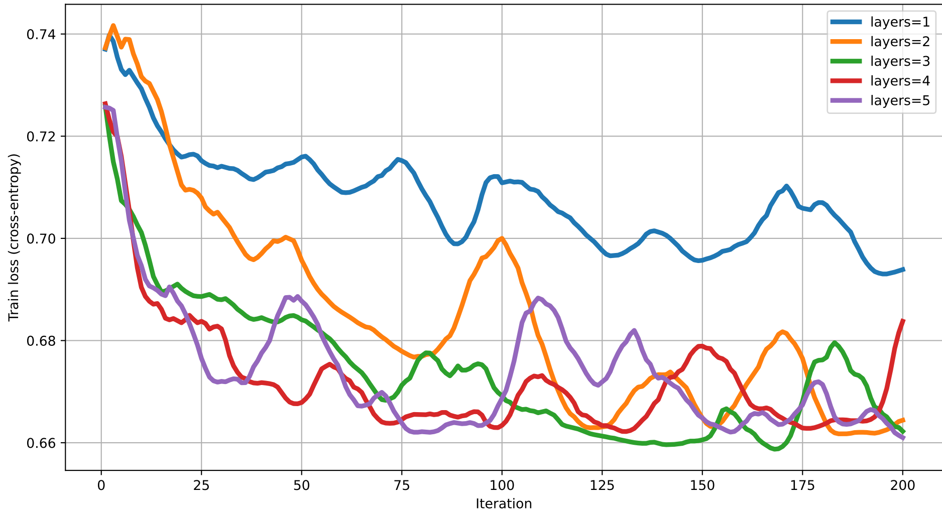
Train loss vs Iteration (dim=5) rot=RX, ent=ring, gate=CZ
