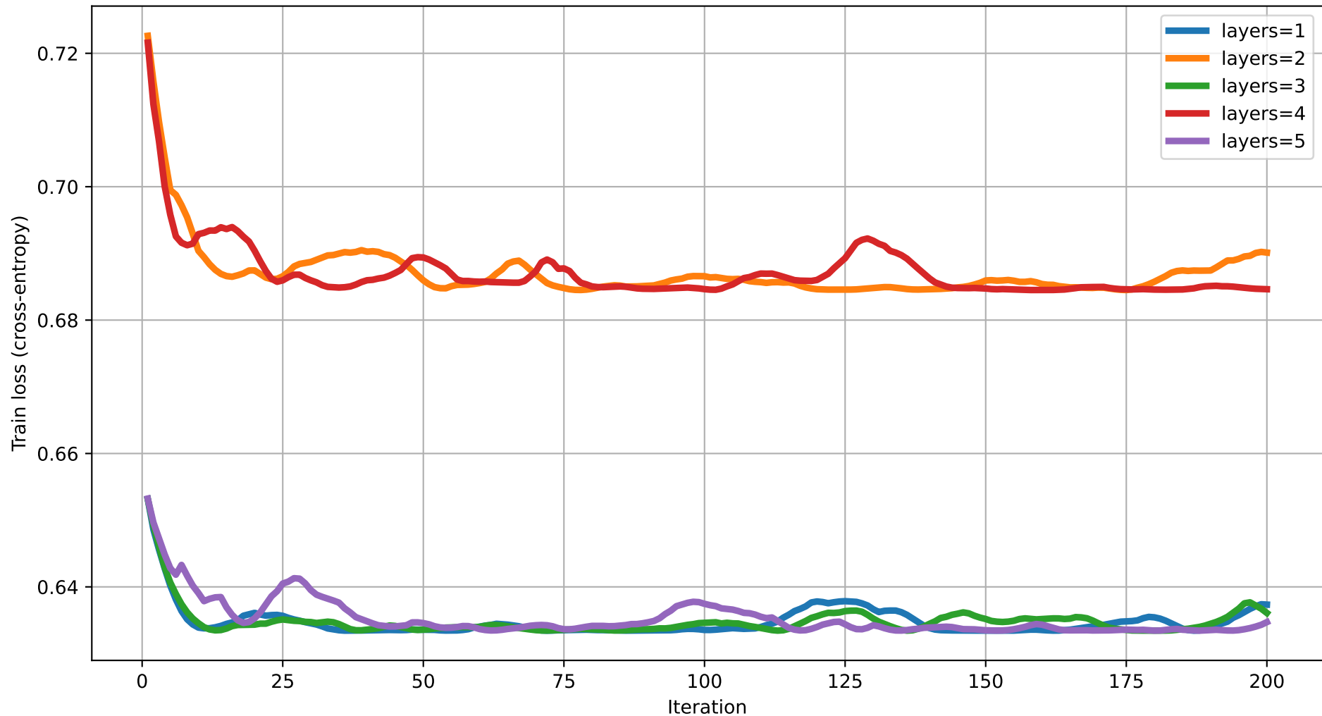
Train loss vs Iteration (degree=3) rot=RX, ent=ring, gate=IsingXX
