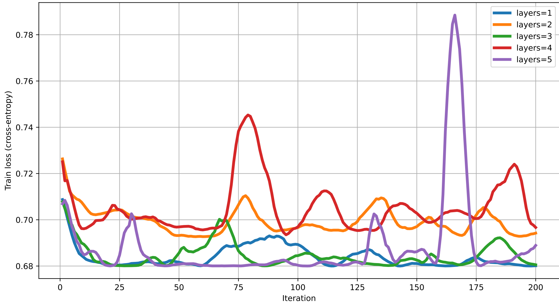
Train loss vs Iteration (dim=5) rot=RX, ent=ring, gate=IsingXX
