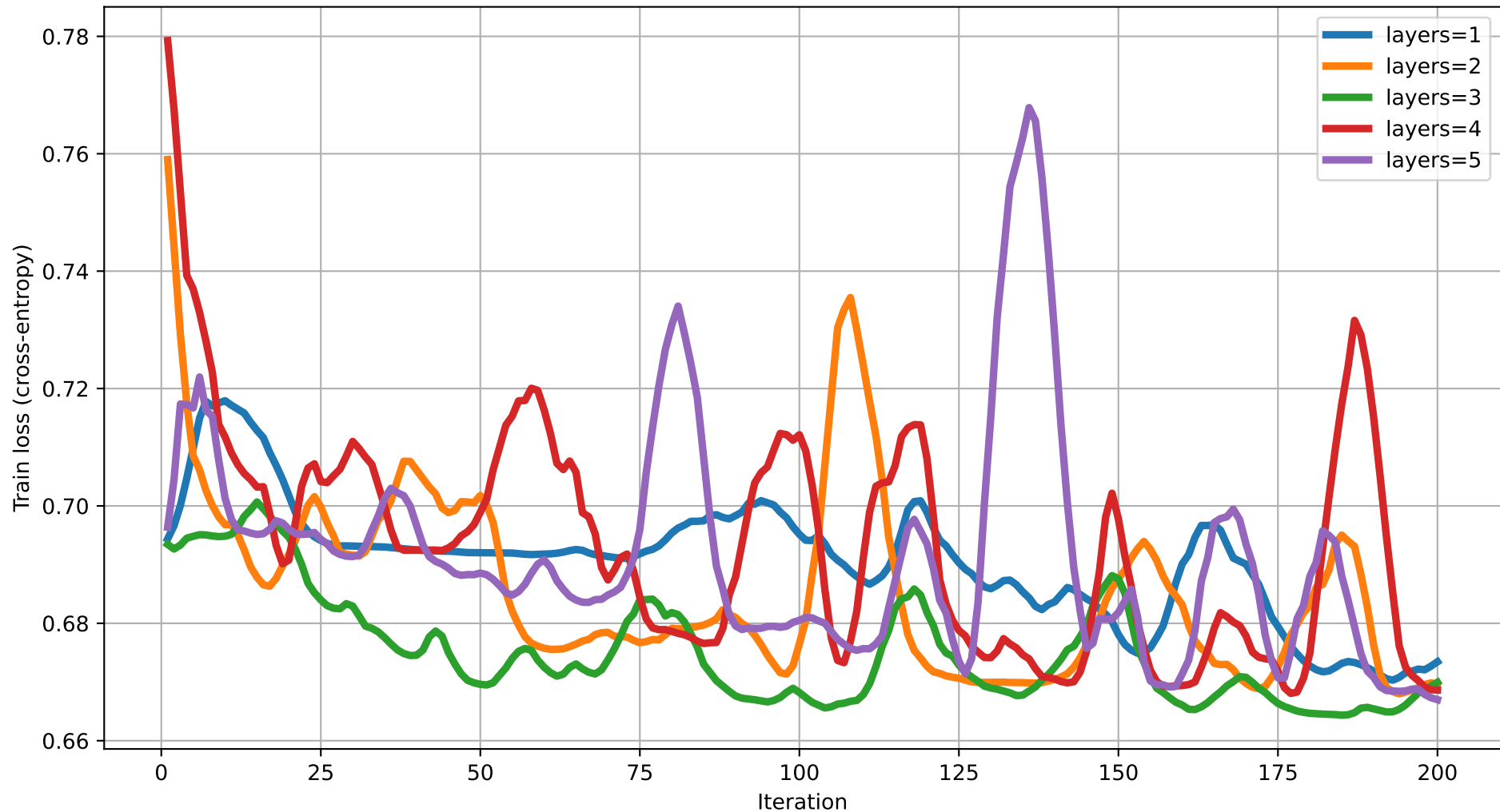
Train loss vs Iteration (dim=17) rot=RYZ, ent=pairwise, gate=IsingXX
