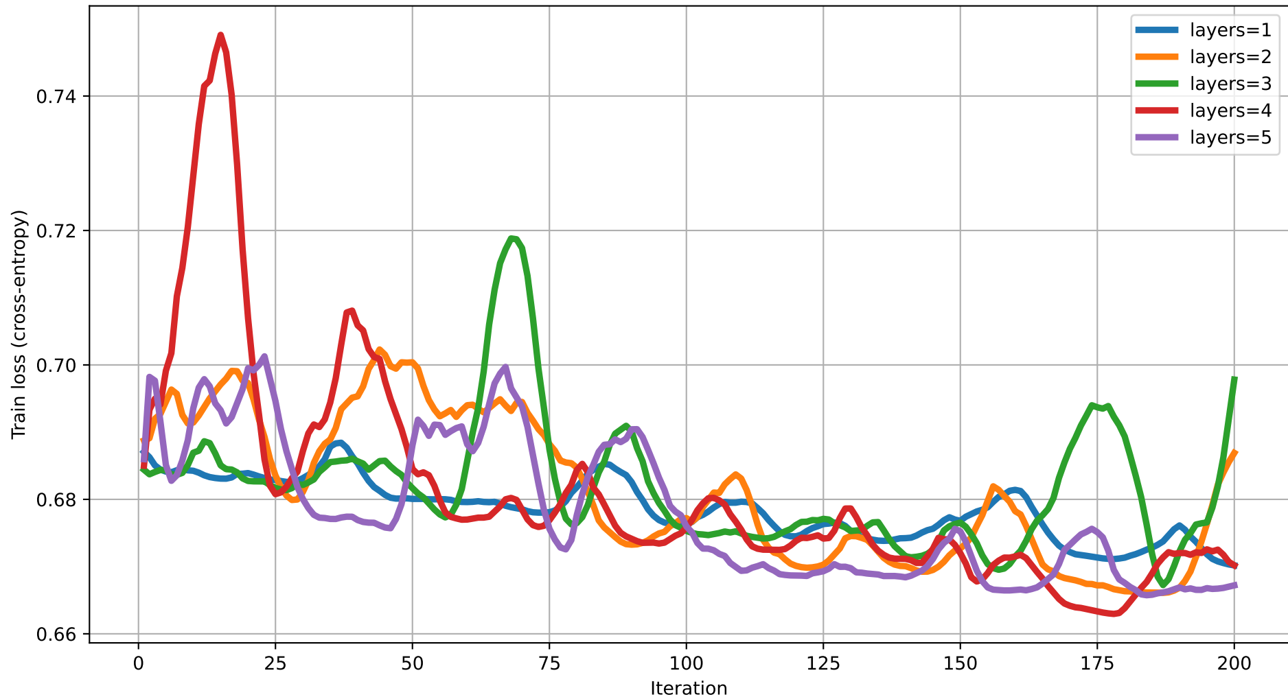
Train loss vs Iteration (dim=15) rot=RY, ent=pairwise, gate=CNOT
