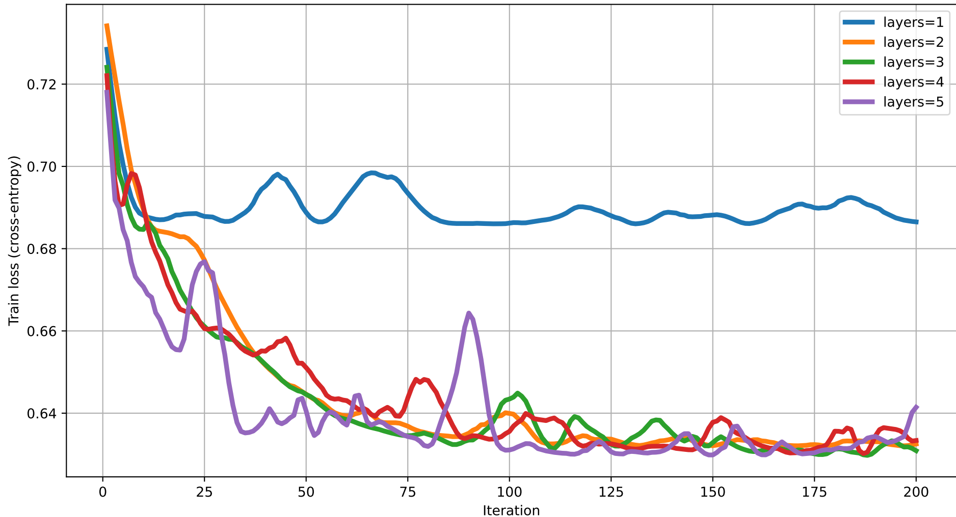
Train loss vs Iteration (degree=2) rot=Rot, ent=pairwise, gate=CNOT
