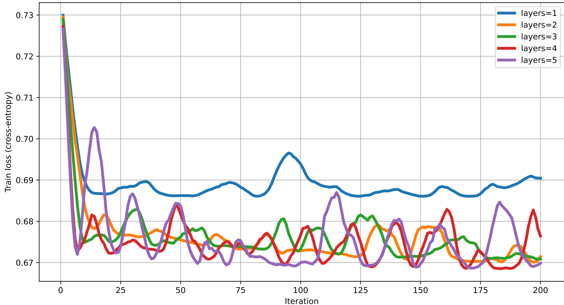
Train loss vs Iteration (degree=2) rot=RX, ent=full, gate=CNOT
