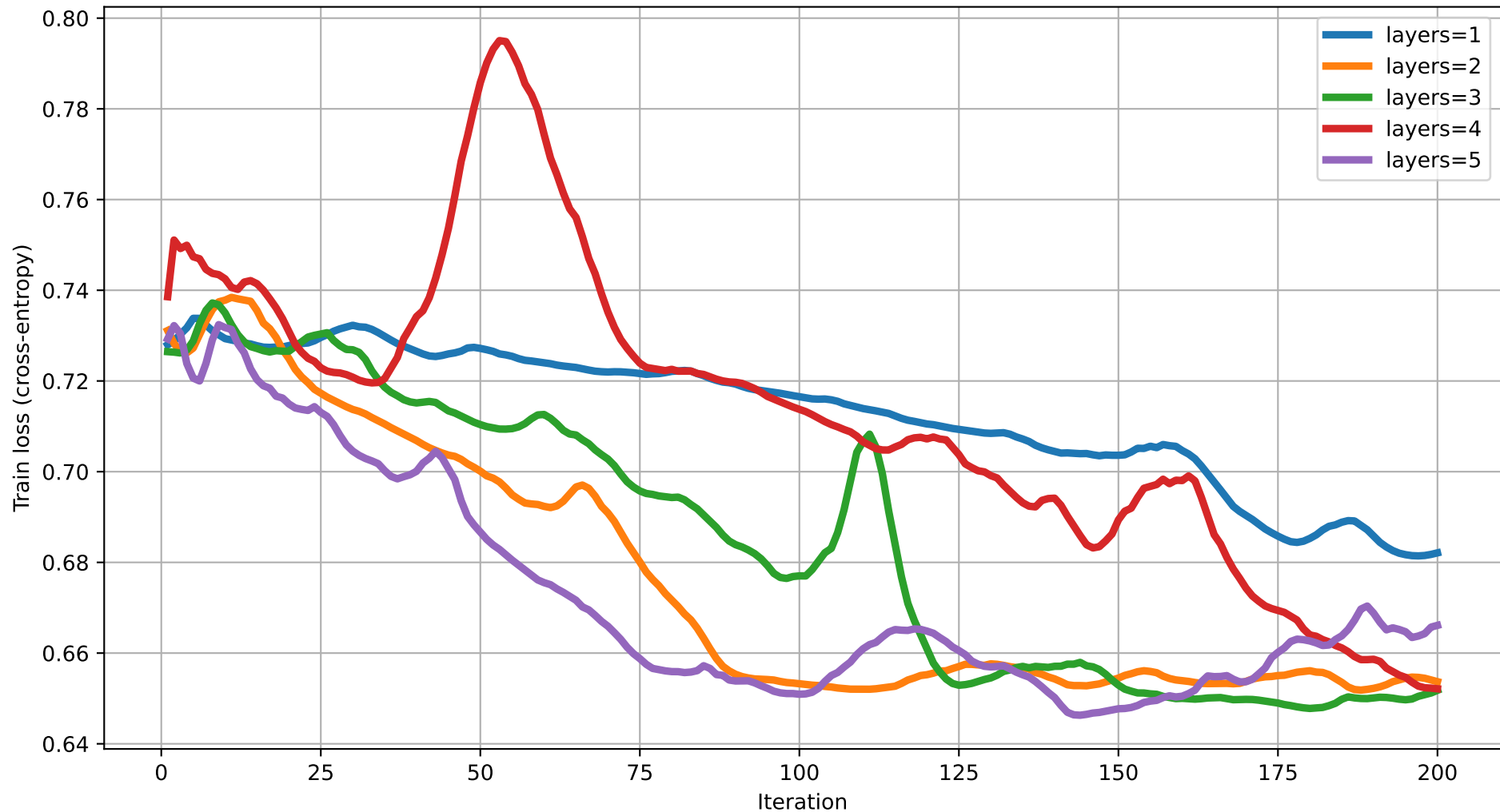
Train loss vs Iteration (dim=7) rot=RY, ent=pairwise, gate=CNOT
