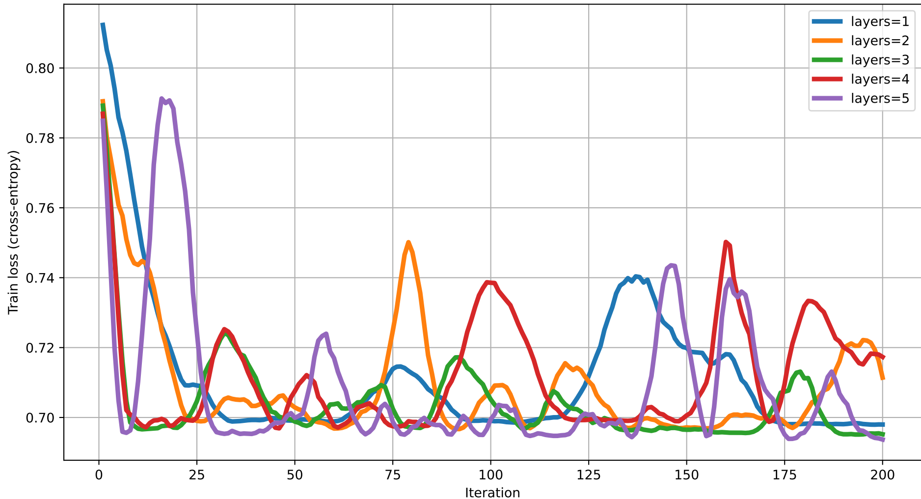
Train loss vs Iteration (dim=2) rot=RX, ent=ring, gate=CZ
