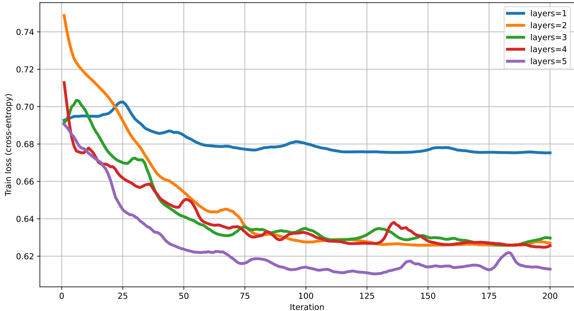
Train loss vs Iteration (degree=4) rot=RZ, ent=chain, gate=IsingXX
