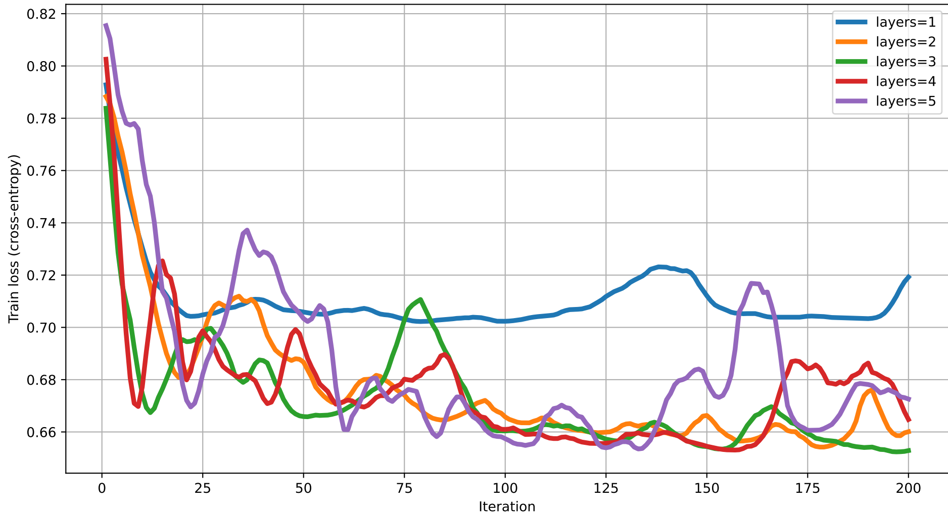
Train loss vs Iteration (dim=2) rot=Rot, ent=pairwise, gate=CNOT
