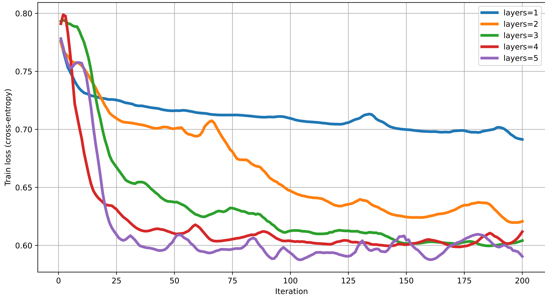
Train loss vs Iteration (dim=9) rot=RY, ent=full, gate=CNOT
