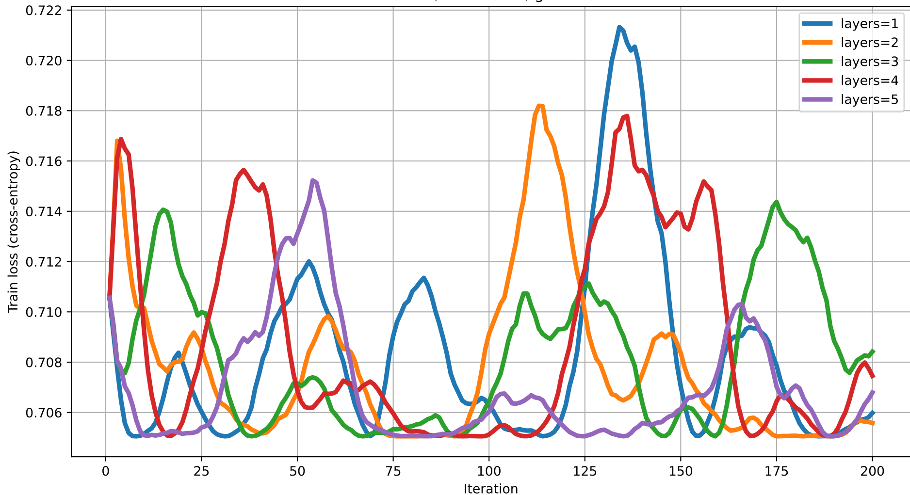
Train loss vs Iteration (dim=14) rot=RZ, ent=chain, gate=CZ
