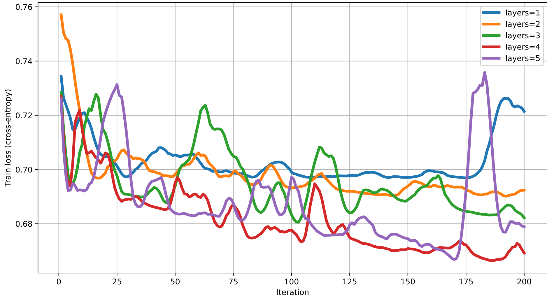
Train loss vs Iteration (dim=18) rot=RYZ, ent=full, gate=CNOT
