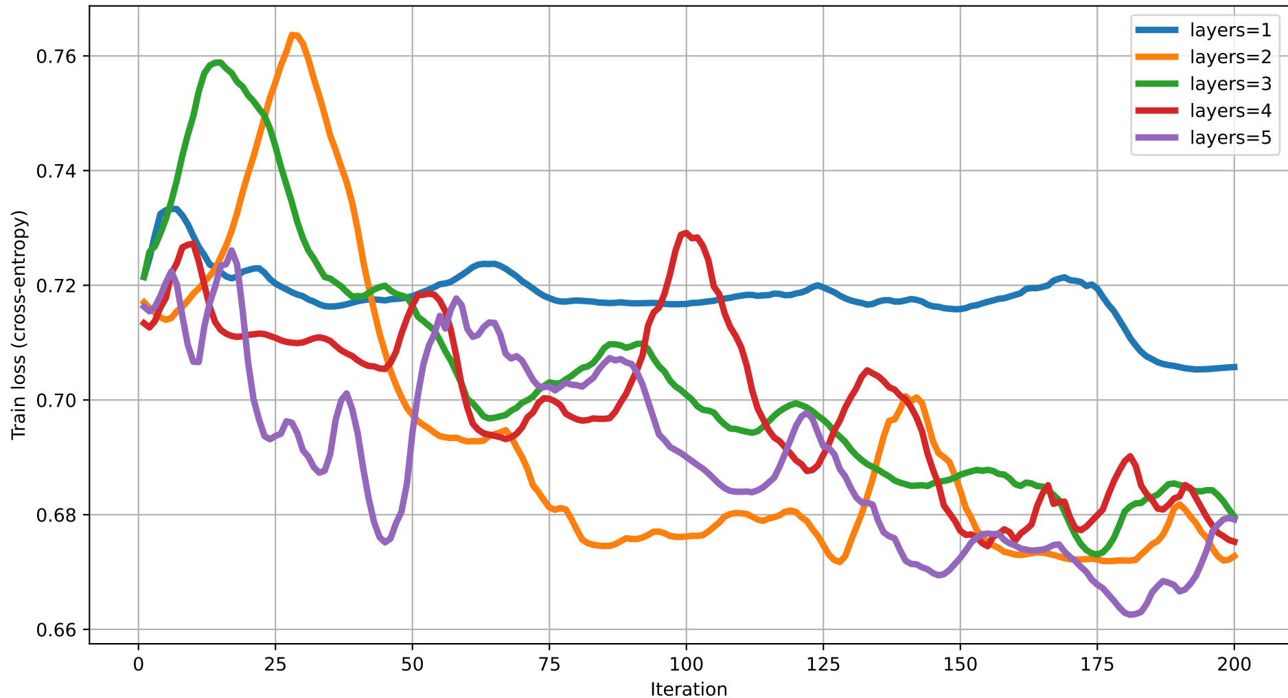
Train loss vs Iteration (dim=3) rot=Rot, ent=chain, gate=CNOT
