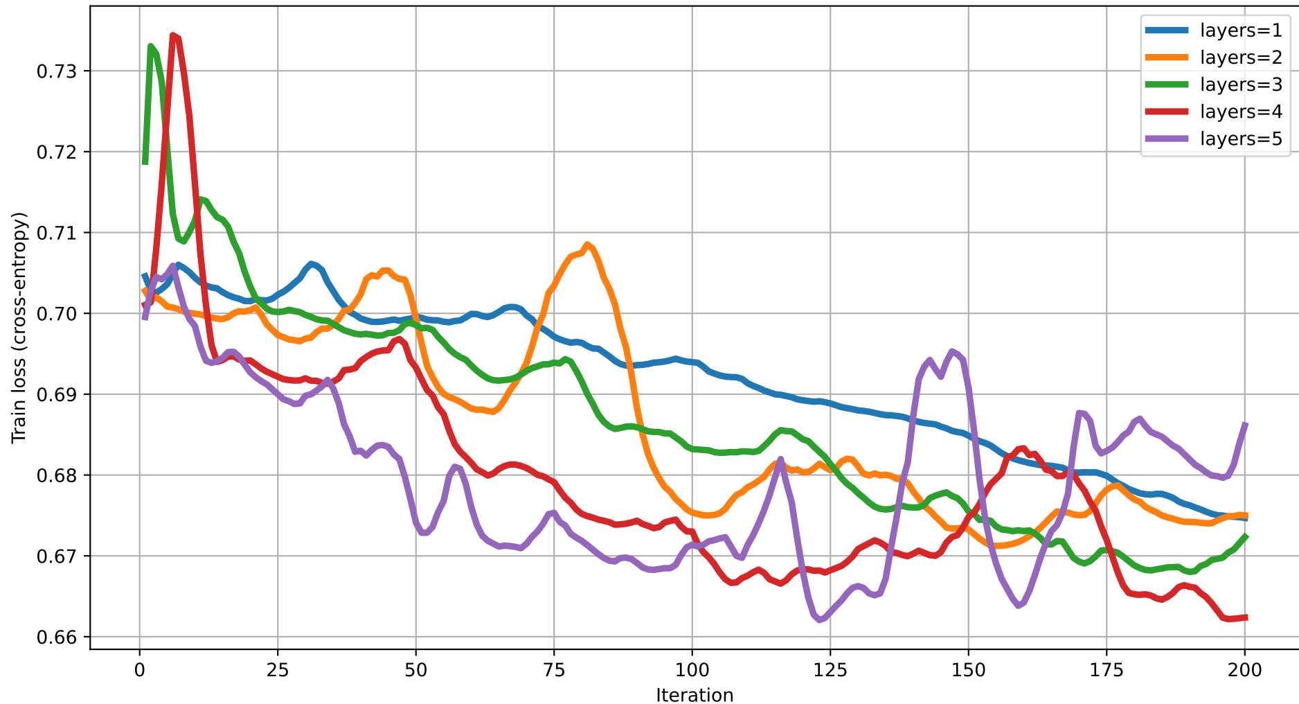
Train loss vs Iteration (dim=14) rot=RYZ, ent=full, gate=CNOT
