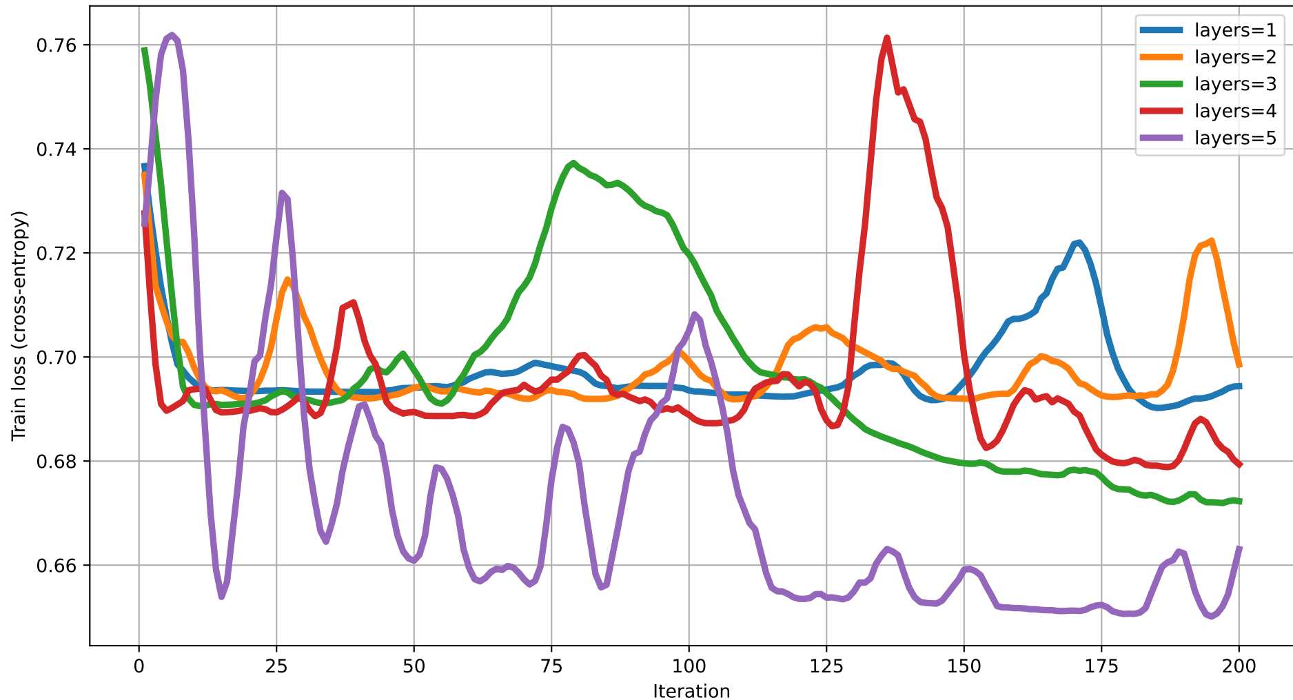
Train loss vs Iteration (dim=16) rot=RY, ent=chain, gate=CNOT
