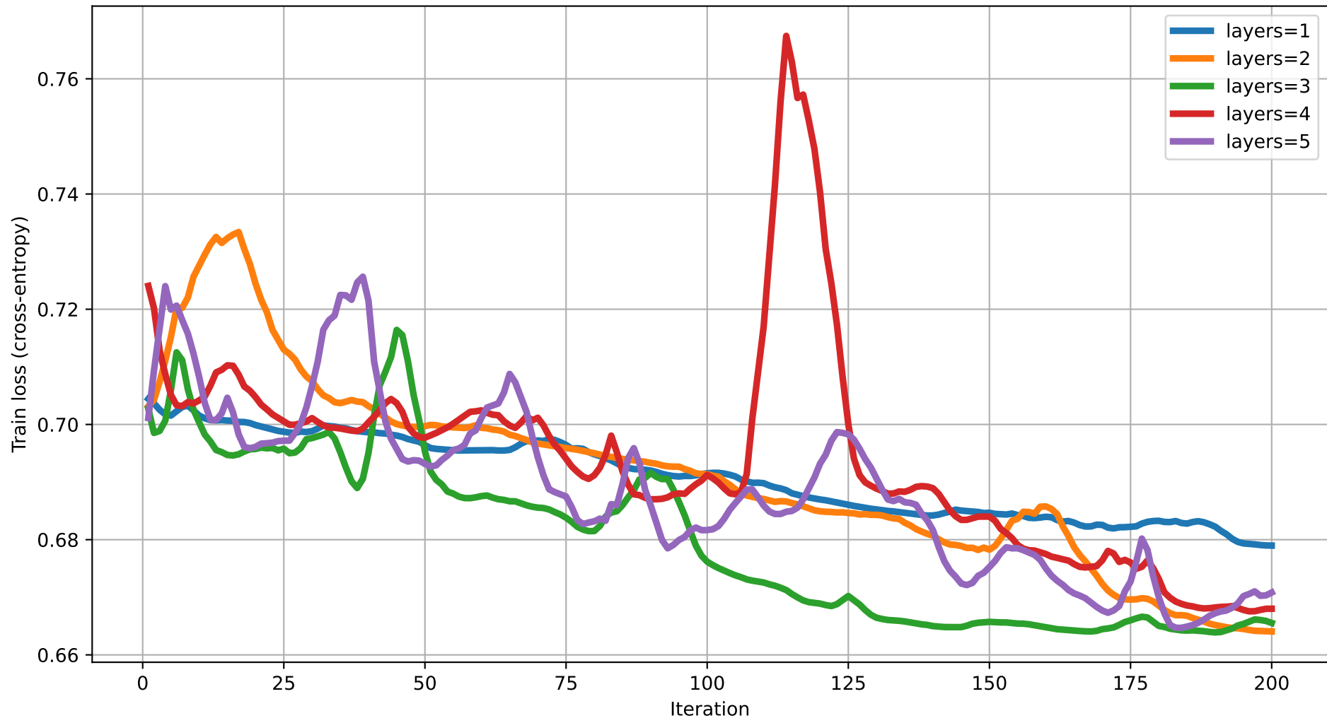
Train loss vs Iteration (dim=14) rot=Rot, ent=pairwise, gate=CNOT
