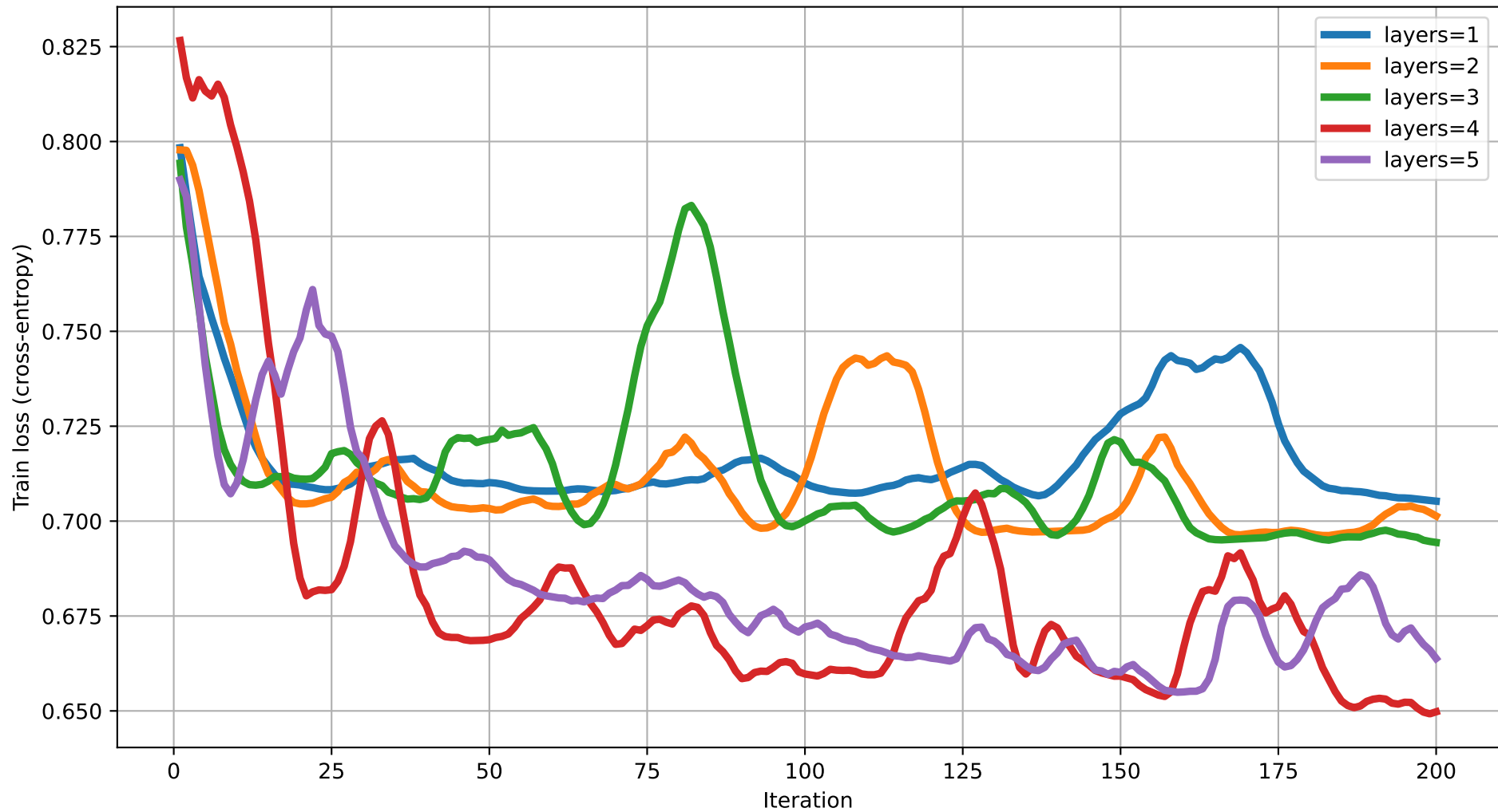
Train loss vs Iteration (dim=8) rot=RYZ, ent=ring, gate=CZ
