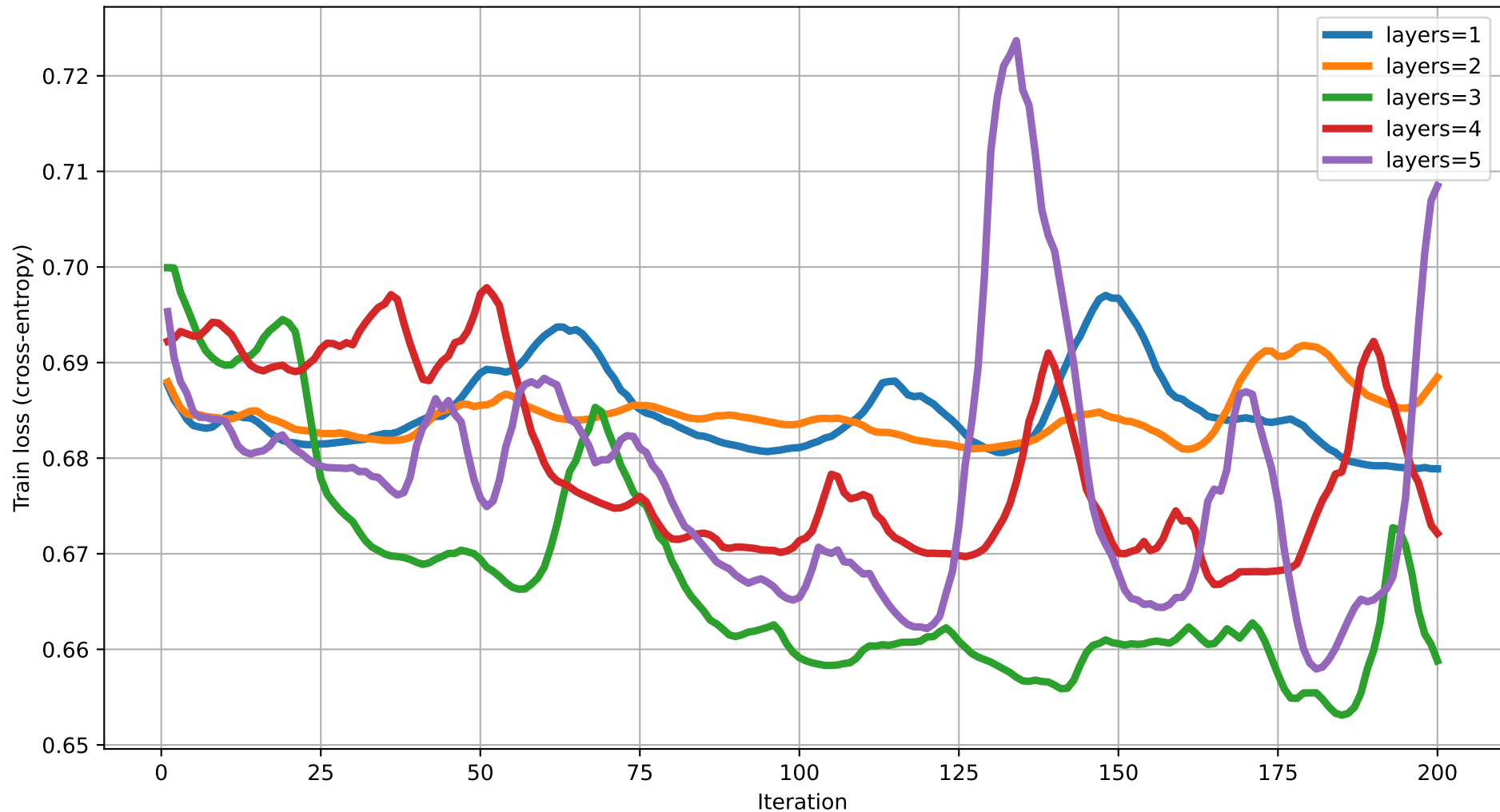
Train loss vs Iteration (dim=16) rot=RYZ, ent=ring, gate=CNOT
