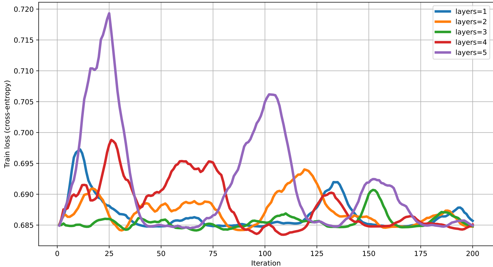
Train loss vs Iteration (dim=15) rot=RX, ent=full, gate=CNOT
