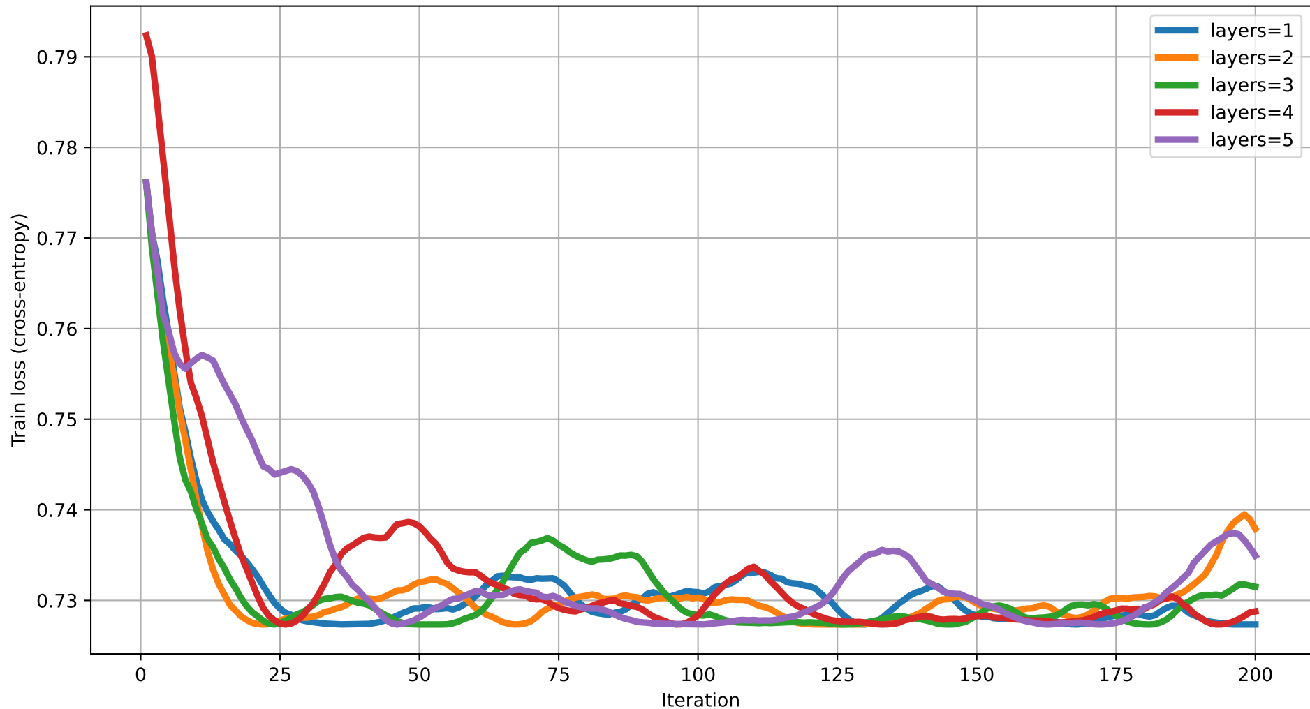
Train loss vs Iteration (dim=9) rot=RZ, ent=pairwise, gate=CZ
