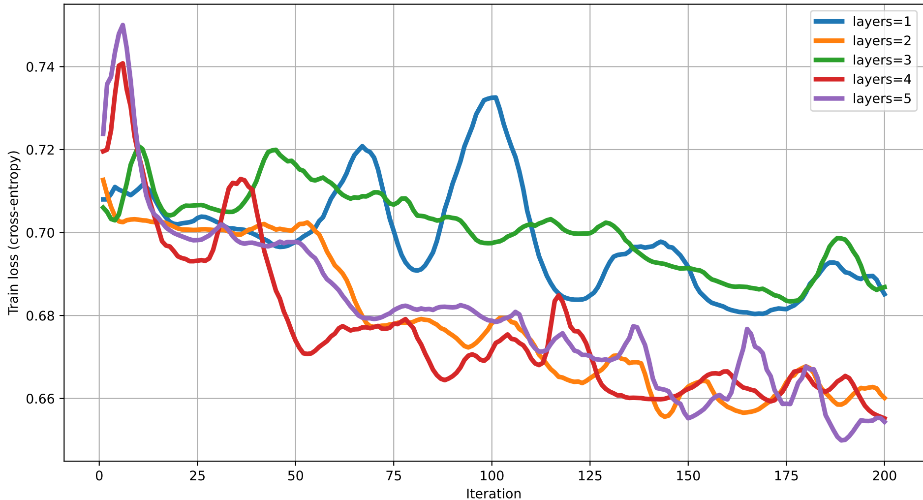
Train loss vs Iteration (dim=6) rot=RYZ, ent=full, gate=CZ
