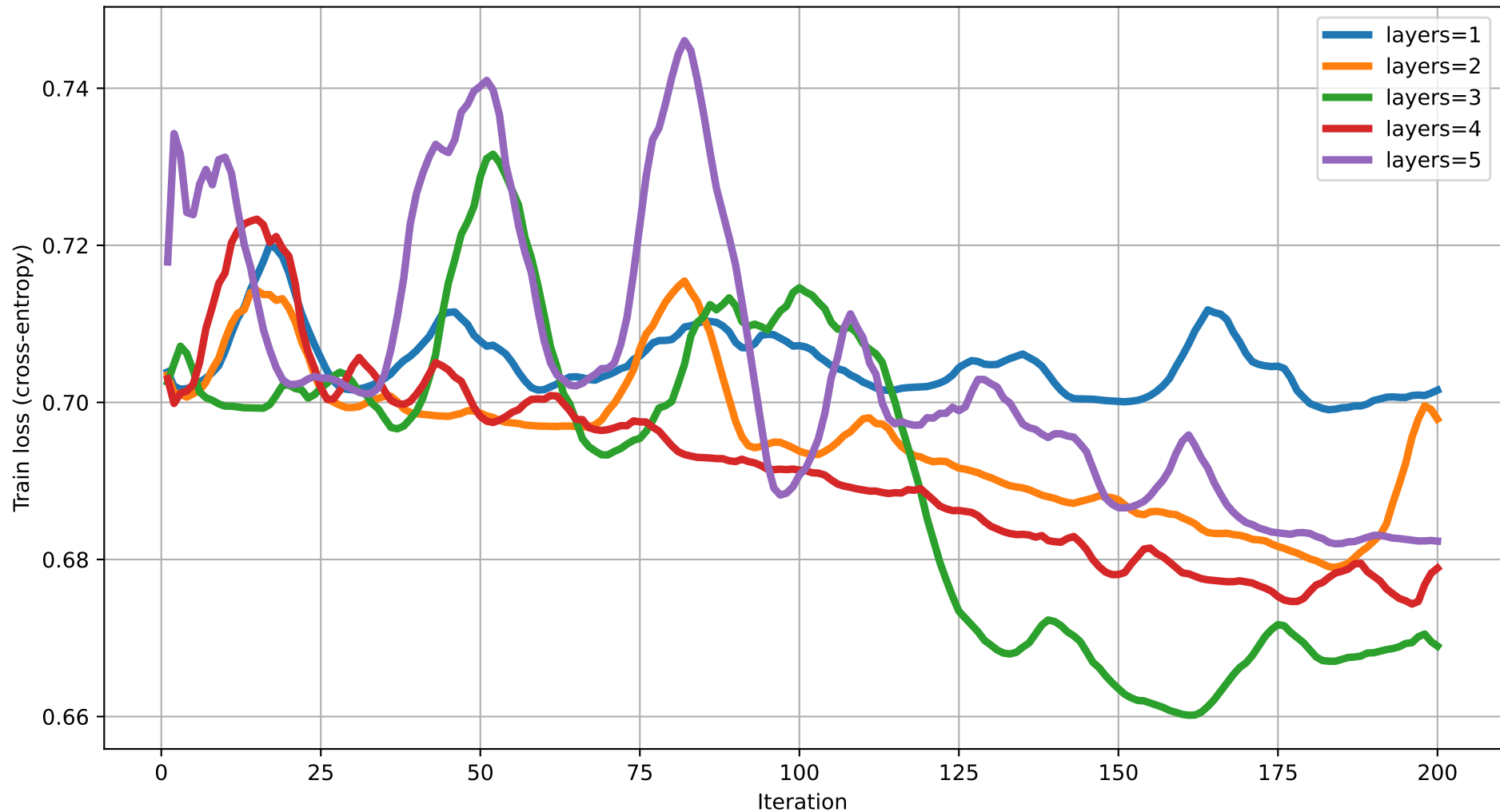
Train loss vs Iteration (dim=12) rot=RY, ent=chain, gate=CNOT
