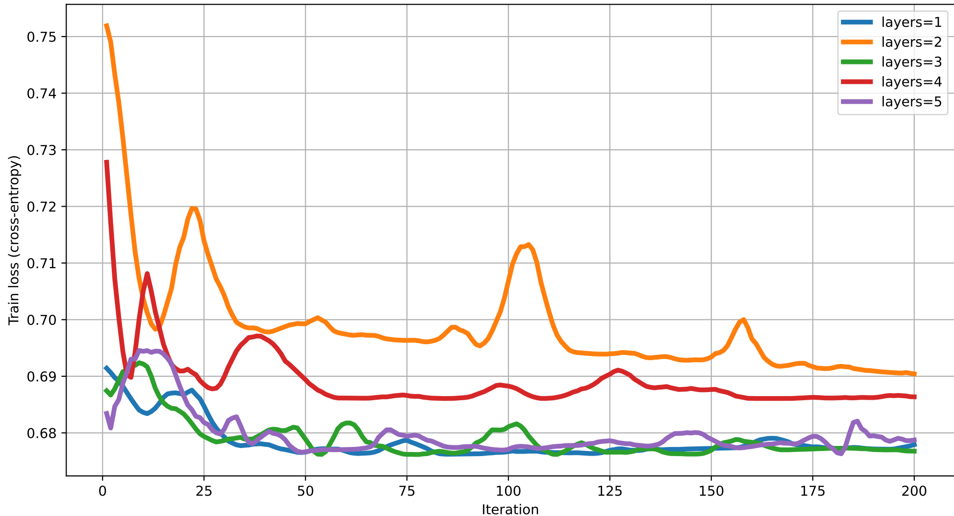
Train loss vs Iteration (degree=2) rot=RX, ent=chain, gate=IsingXX
