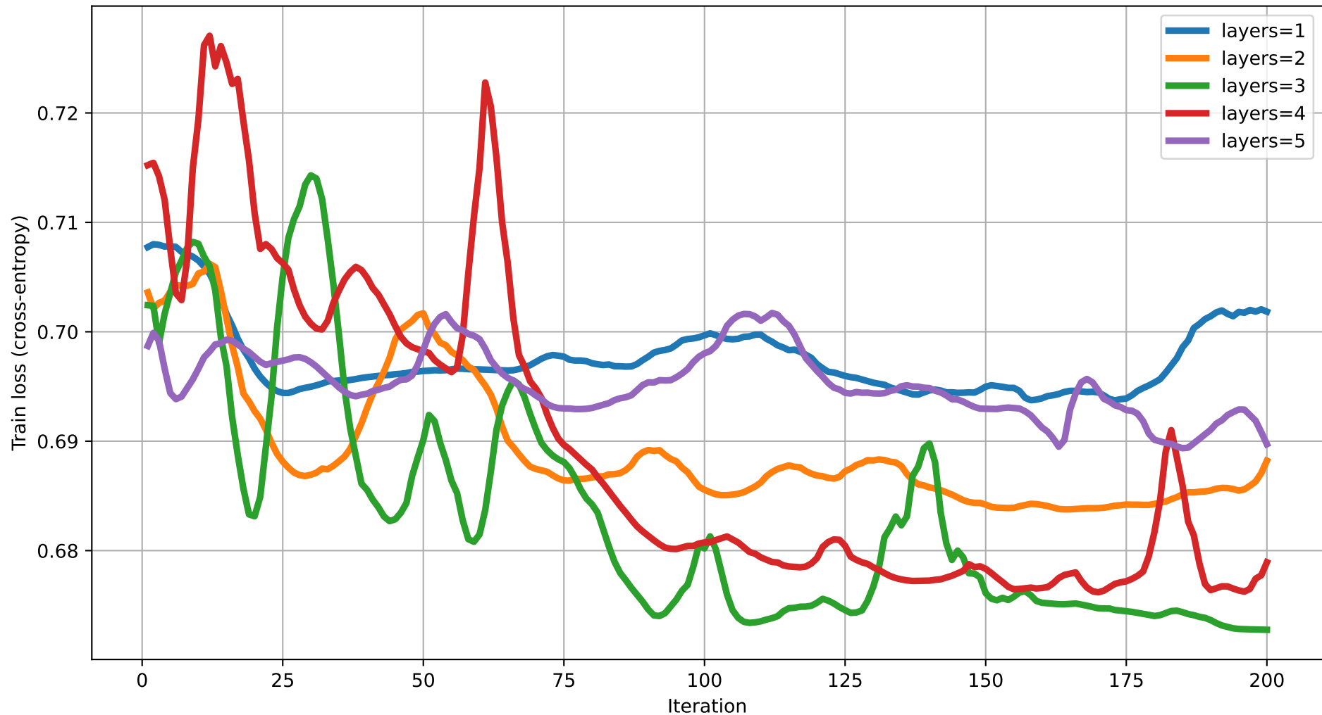
Train loss vs Iteration (dim=12) rot=RX, ent=ring, gate=CNOT
