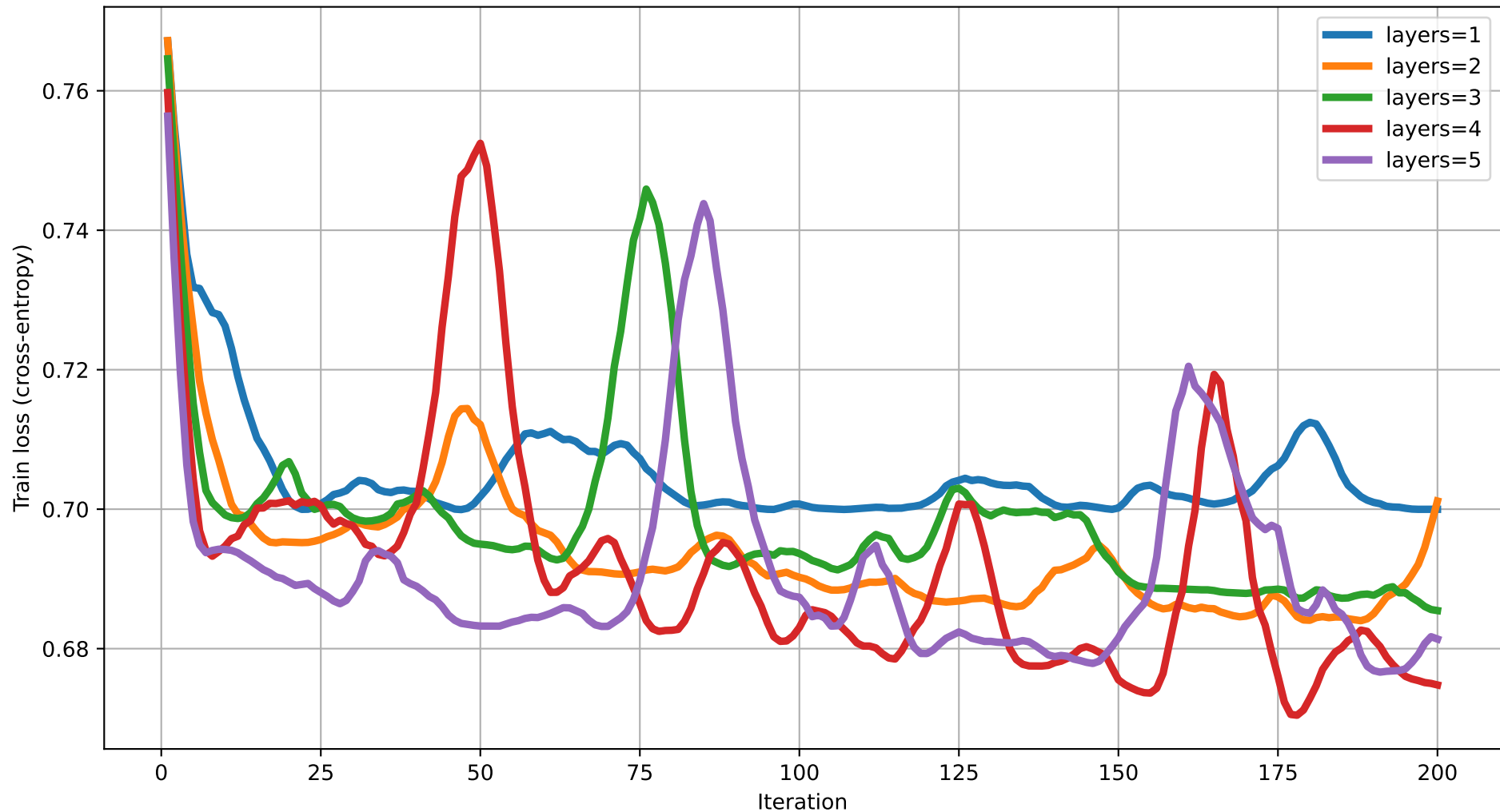
Train loss vs Iteration (dim=17) rot=RYZ, ent=ring, gate=CZ
