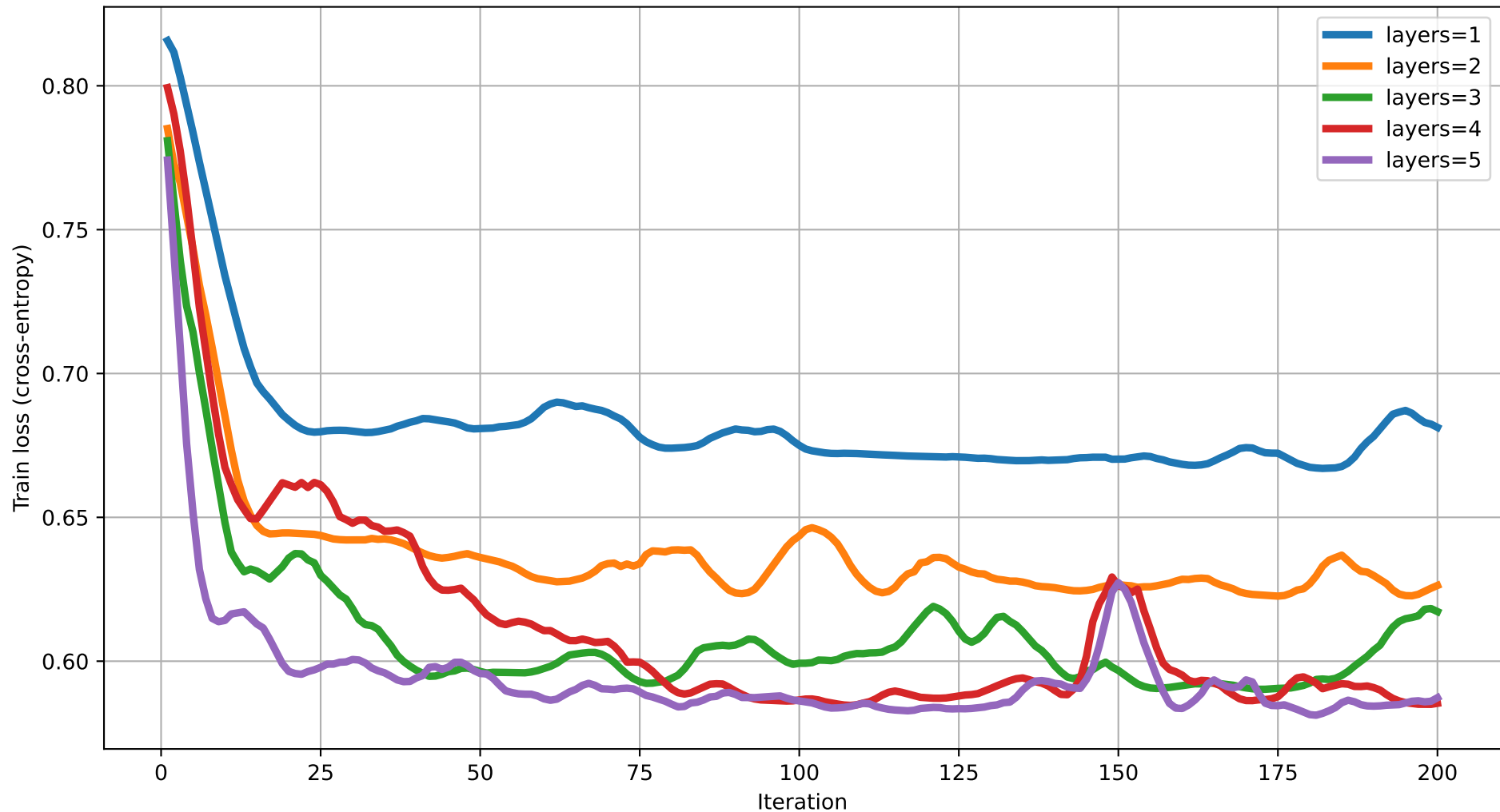
Train loss vs Iteration (dim=4) rot=Rot, ent=chain, gate=CNOT
