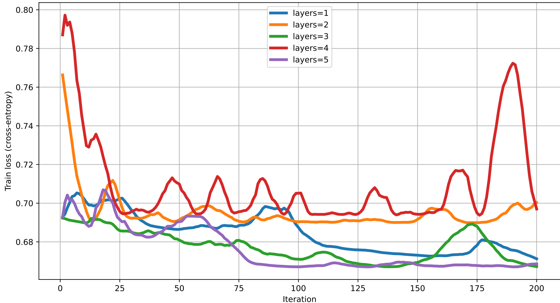
Train loss vs Iteration (dim=17) rot=RX, ent=chain, gate=IsingXX
