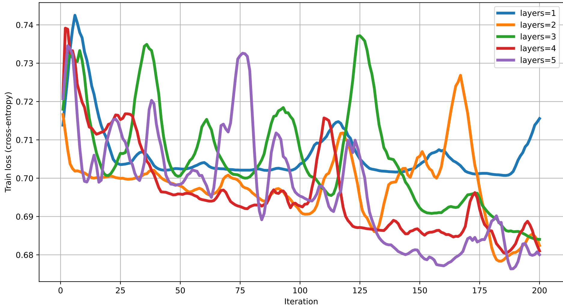
Train loss vs Iteration (dim=12) rot=Rot, ent=pairwise, gate=CZ
