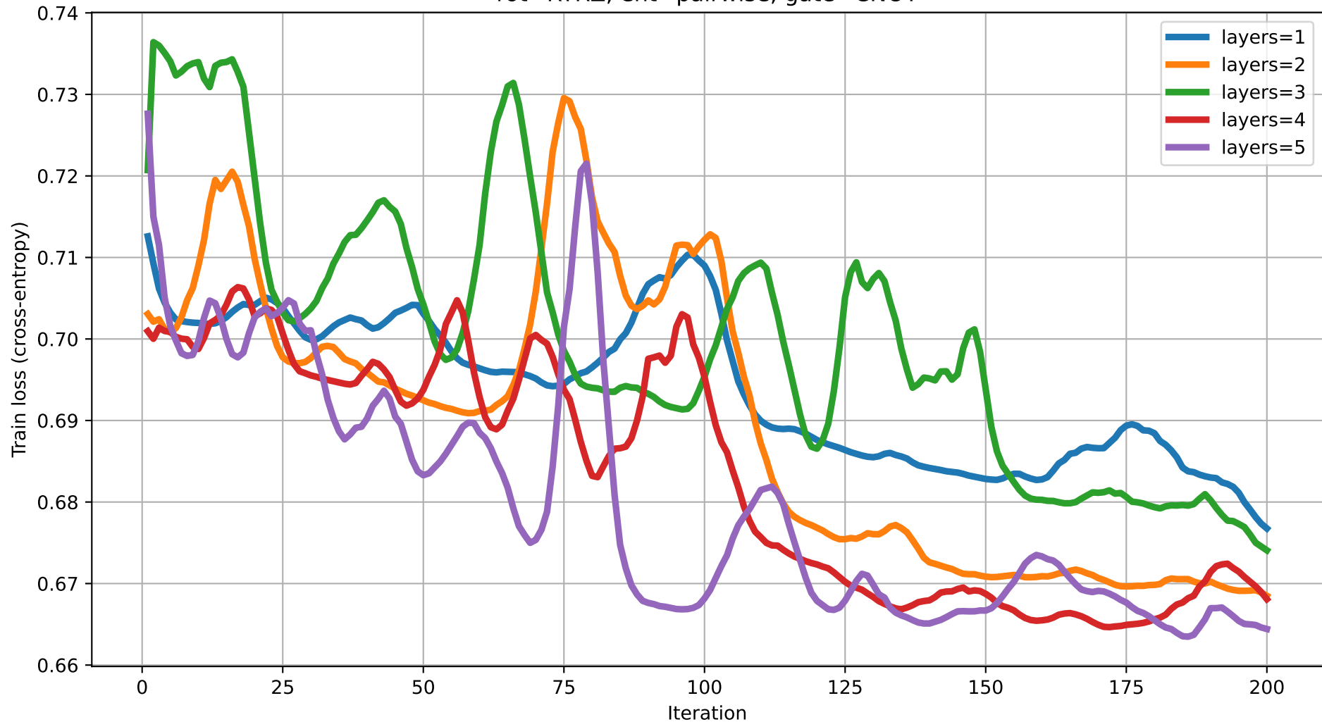
Train loss vs Iteration (dim=14) rot=RYZ, ent=pairwise, gate=CNOT
