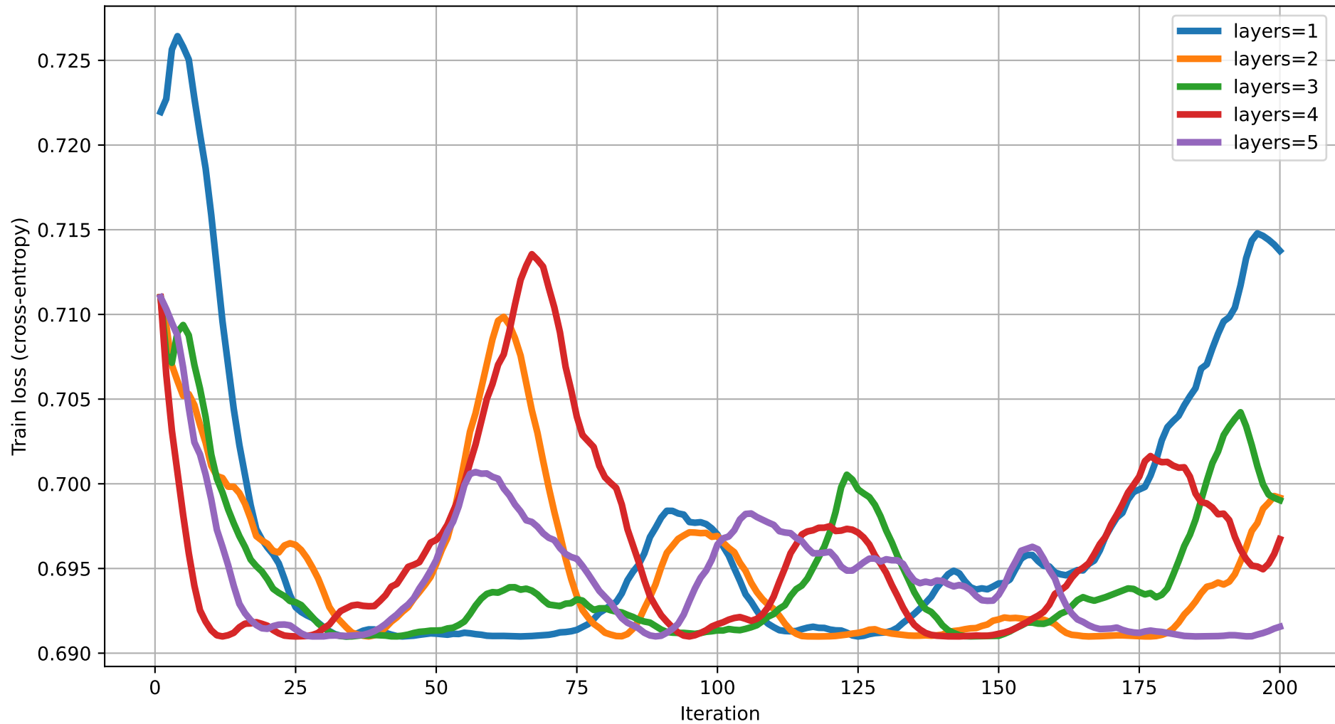
Train loss vs Iteration (dim=20) rot=RZ, ent=full, gate=CNOT
