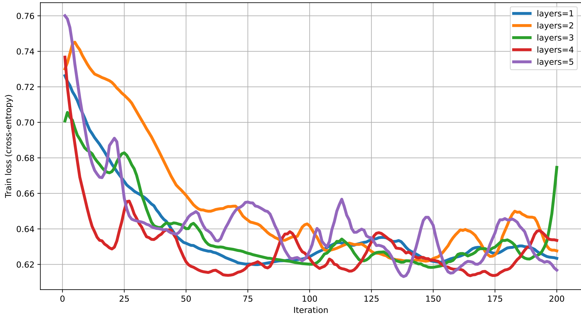
Train loss vs Iteration (dim=6) rot=RYZ, ent=ring, gate=CNOT
