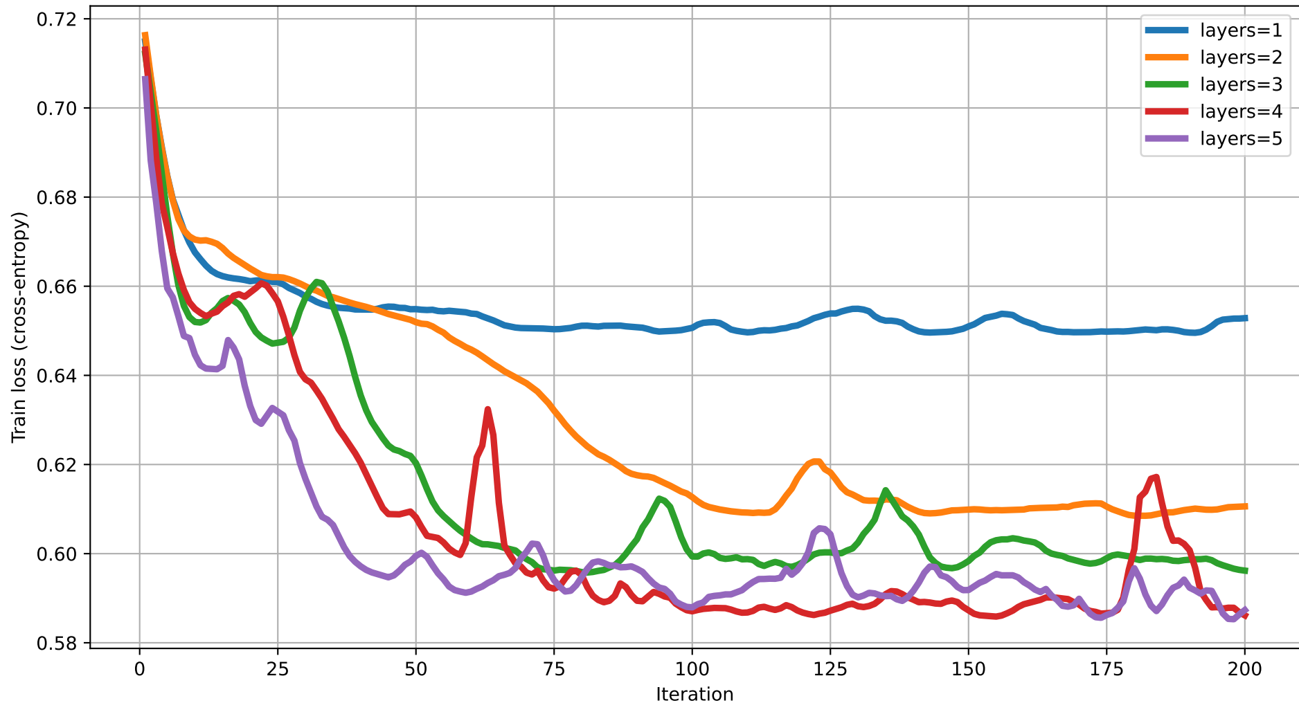
Train loss vs Iteration (degree=4) rot=Rot, ent=ring, gate=CZ
