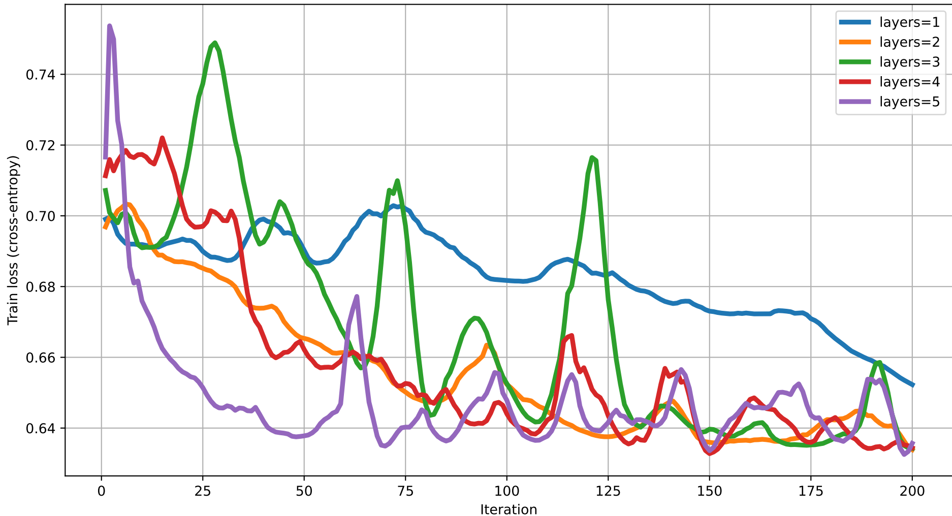
Train loss vs Iteration (dim=6) rot=Rot, ent=pairwise, gate=IsingXX
