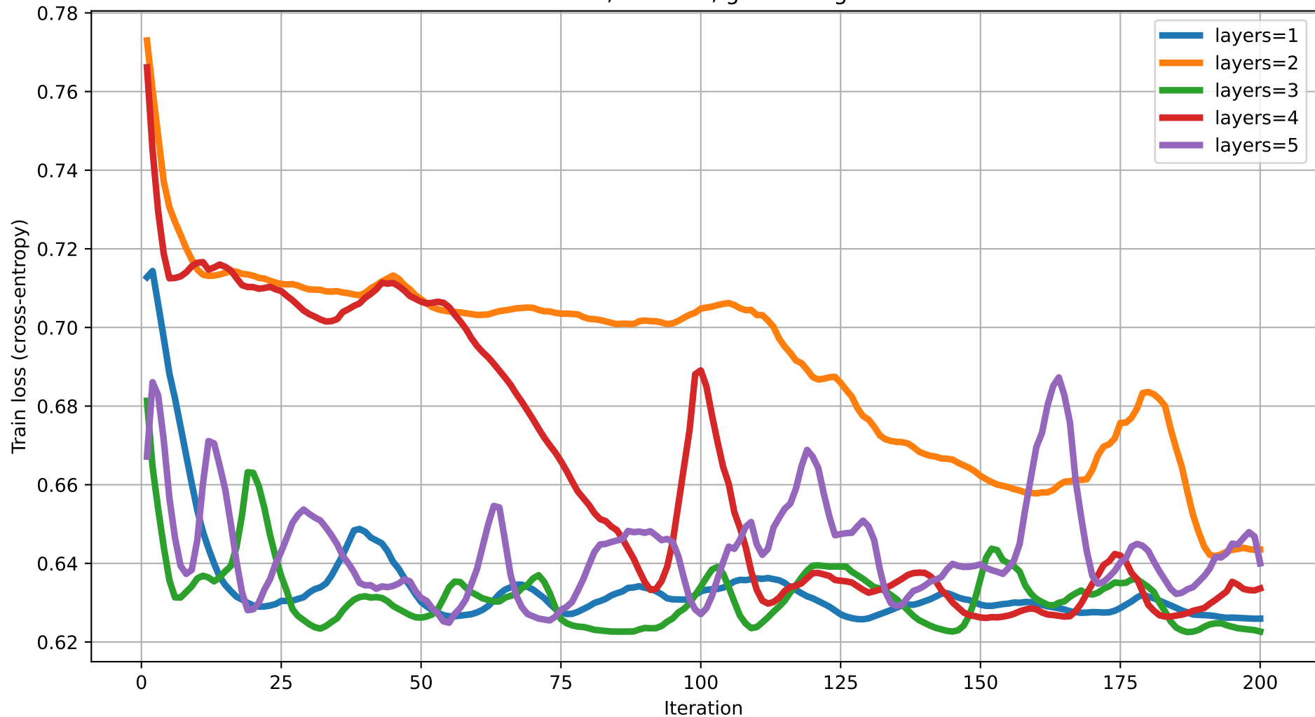
Train loss vs Iteration (dim=4) rot=RY, ent=full, gate=IsingXX
