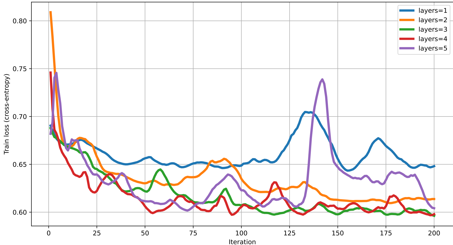
Train loss vs Iteration (dim=8) rot=Rot, ent=full, gate=IsingXX
