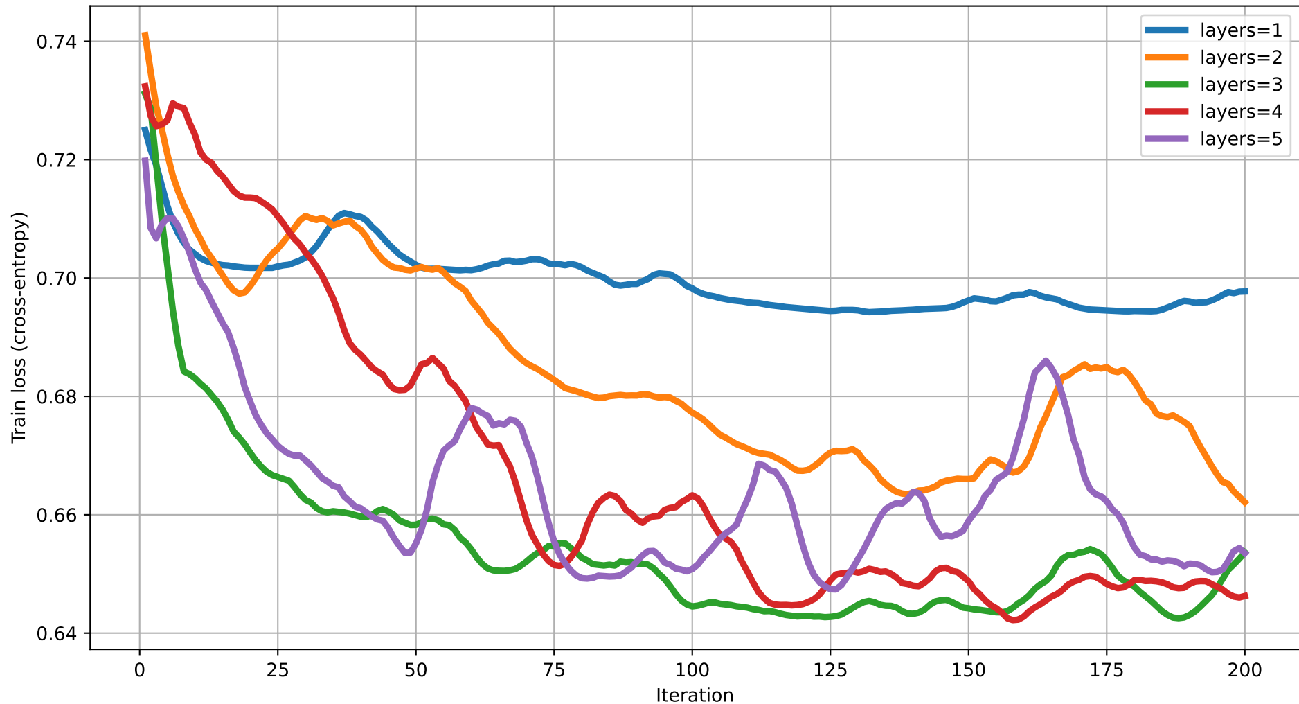
Train loss vs Iteration (dim=5) rot=RY, ent=ring, gate=CZ
