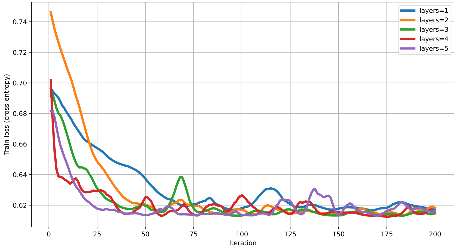
Train loss vs Iteration (degree=3) rot=RYZ, ent=pairwise, gate=IsingXX
