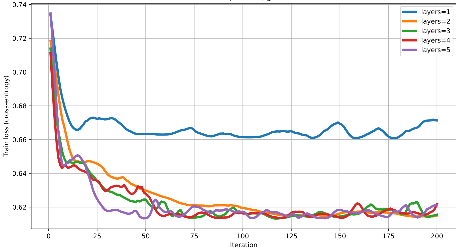
Train loss vs Iteration (degree=3) rot=Rot, ent=pairwise, gate=CNOT
