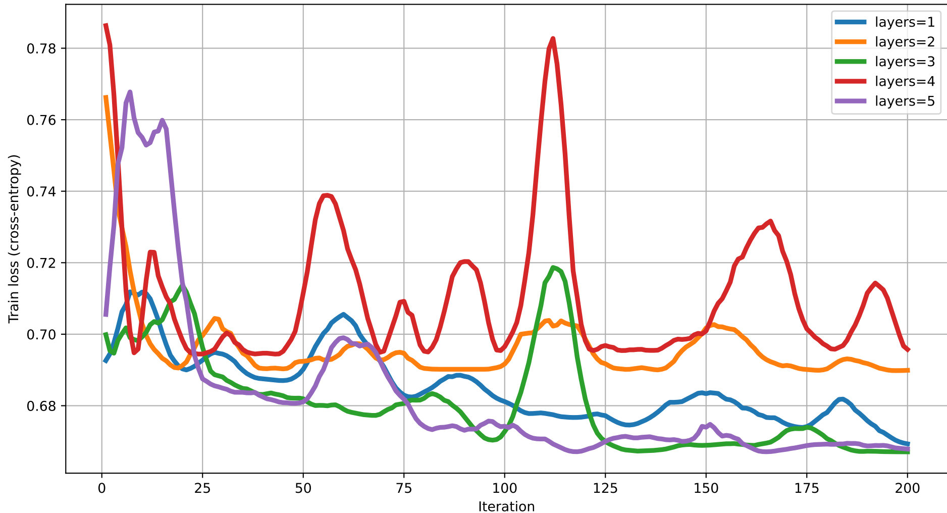
Train loss vs Iteration (dim=17) rot=RX, ent=pairwise, gate=IsingXX
