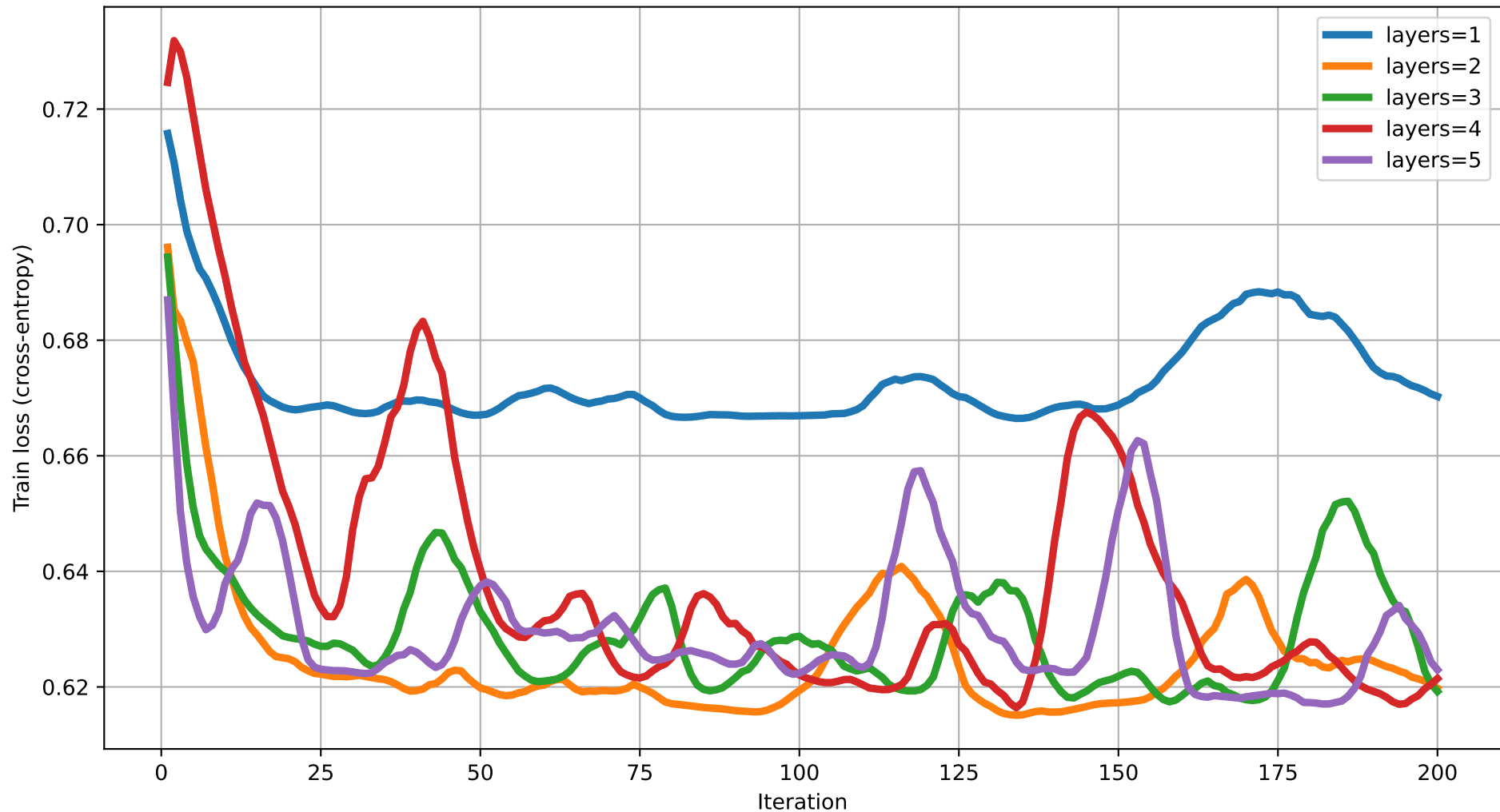
Train loss vs Iteration (dim=10) rot=RY, ent=pairwise, gate=CNOT
