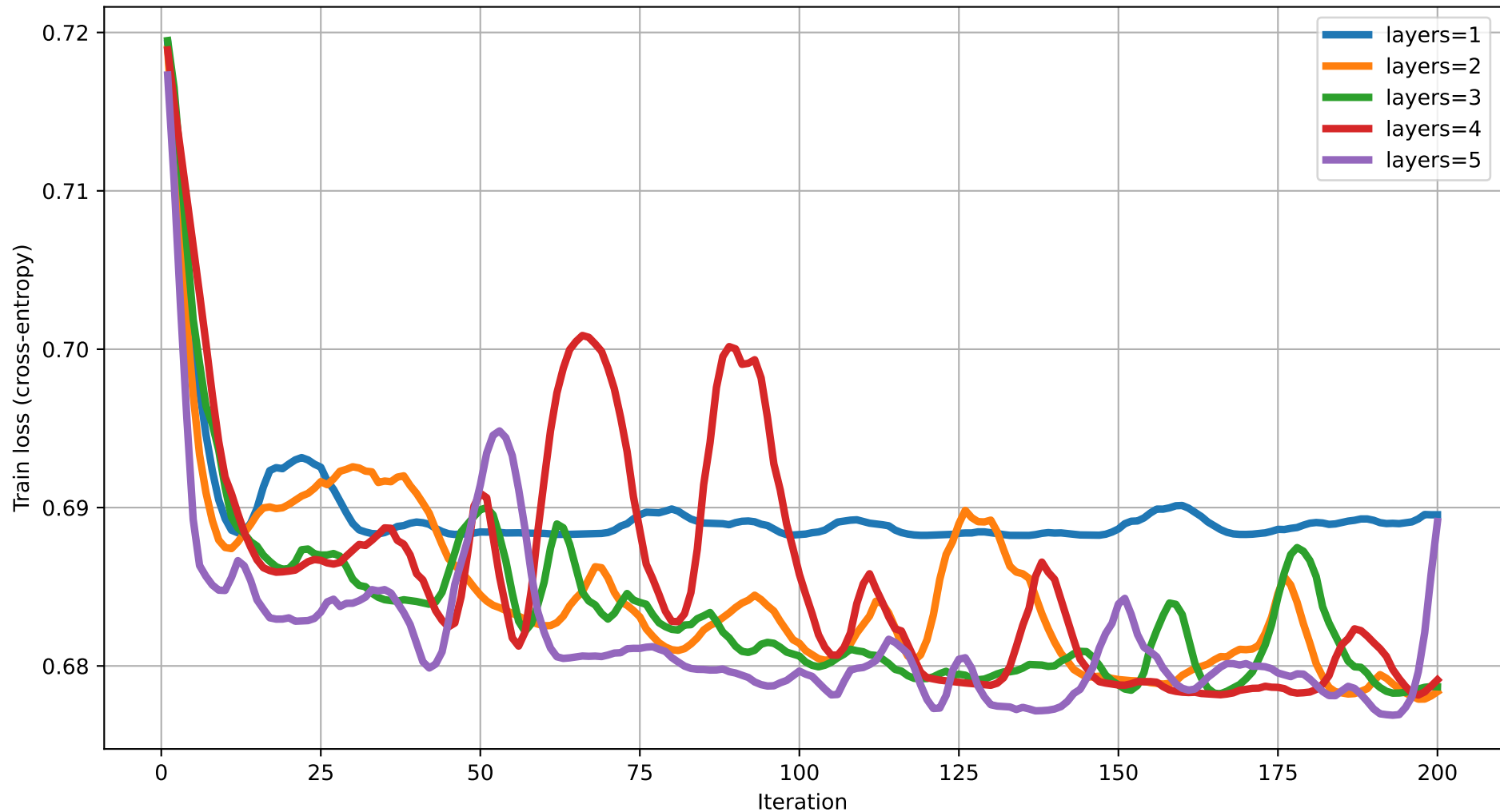
Train loss vs Iteration (degree=4) rot=RX, ent=pairwise, gate=CZ
