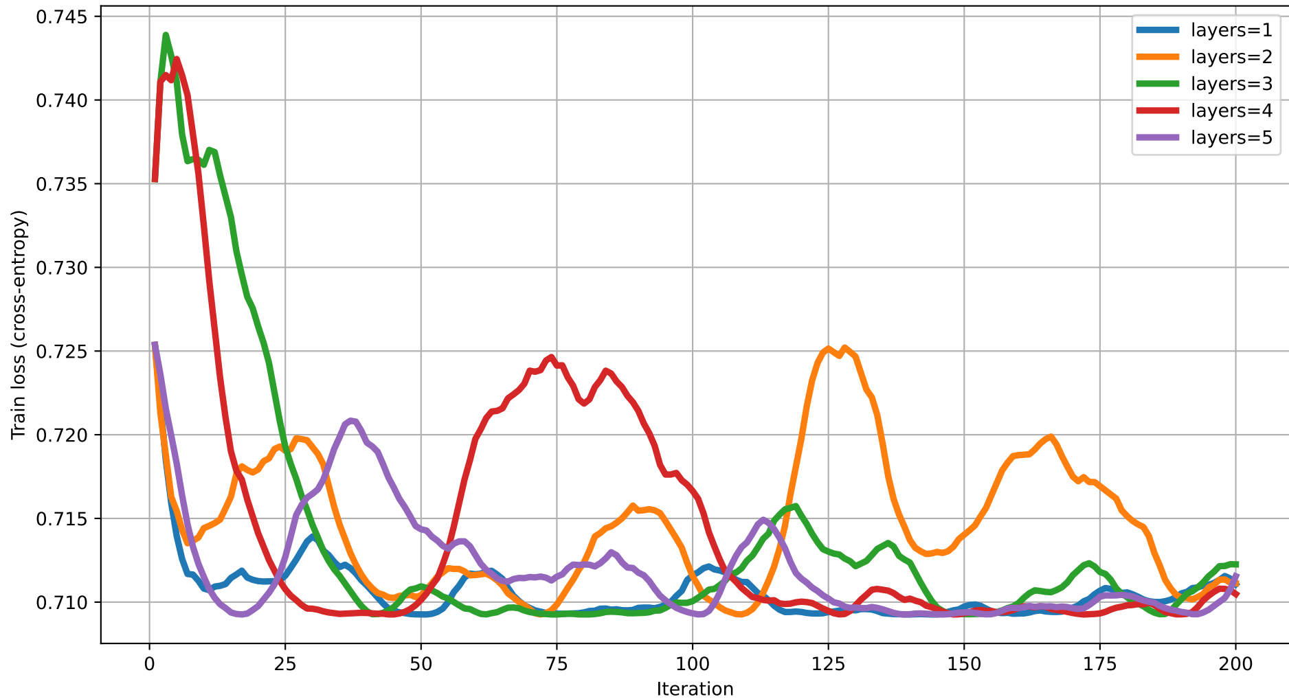
Train loss vs Iteration (dim=10) rot=RZ, ent=full, gate=CZ
