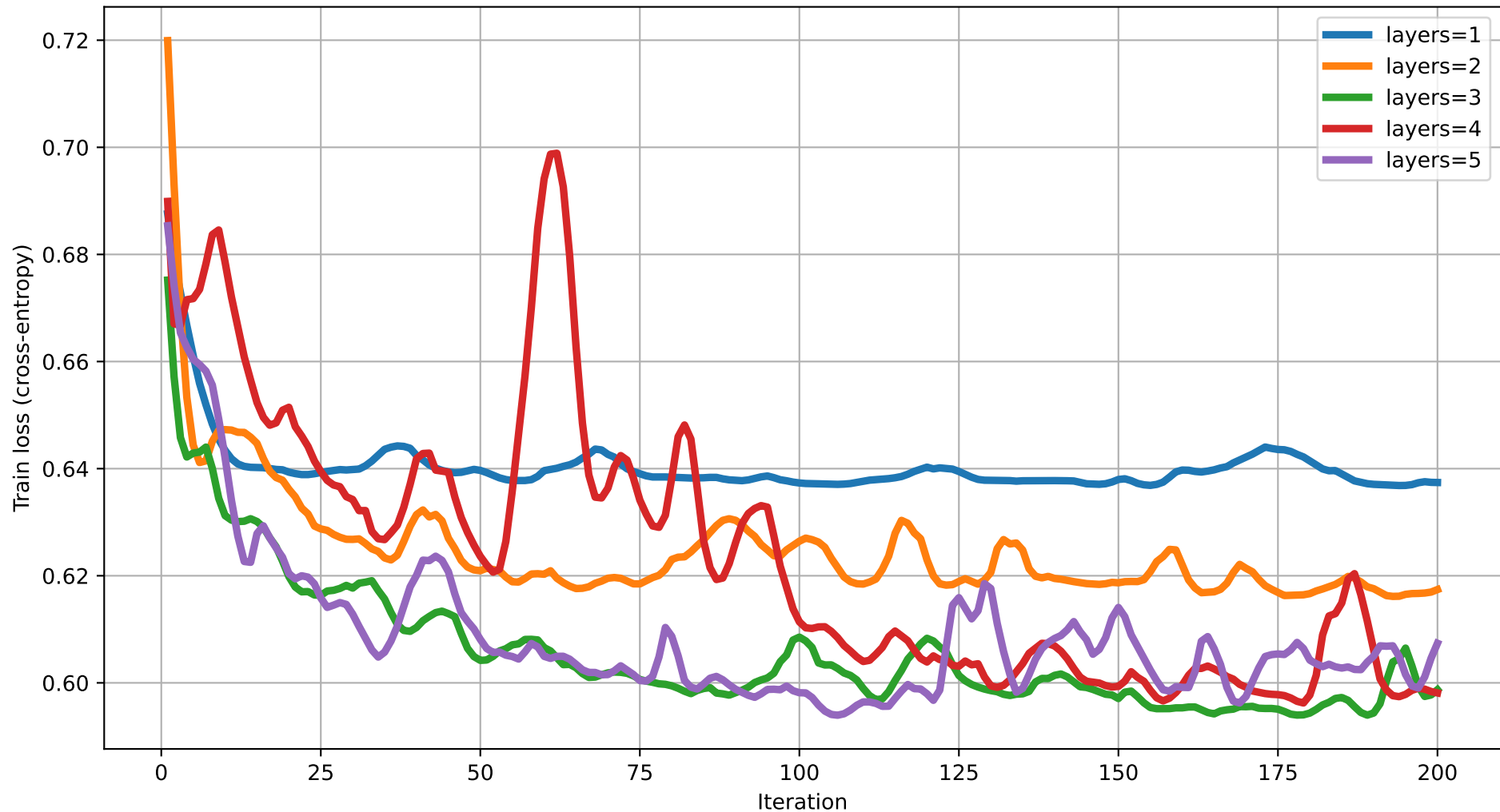
Train loss vs Iteration (degree=2) rot=Rot, ent=full, gate=IsingXX
