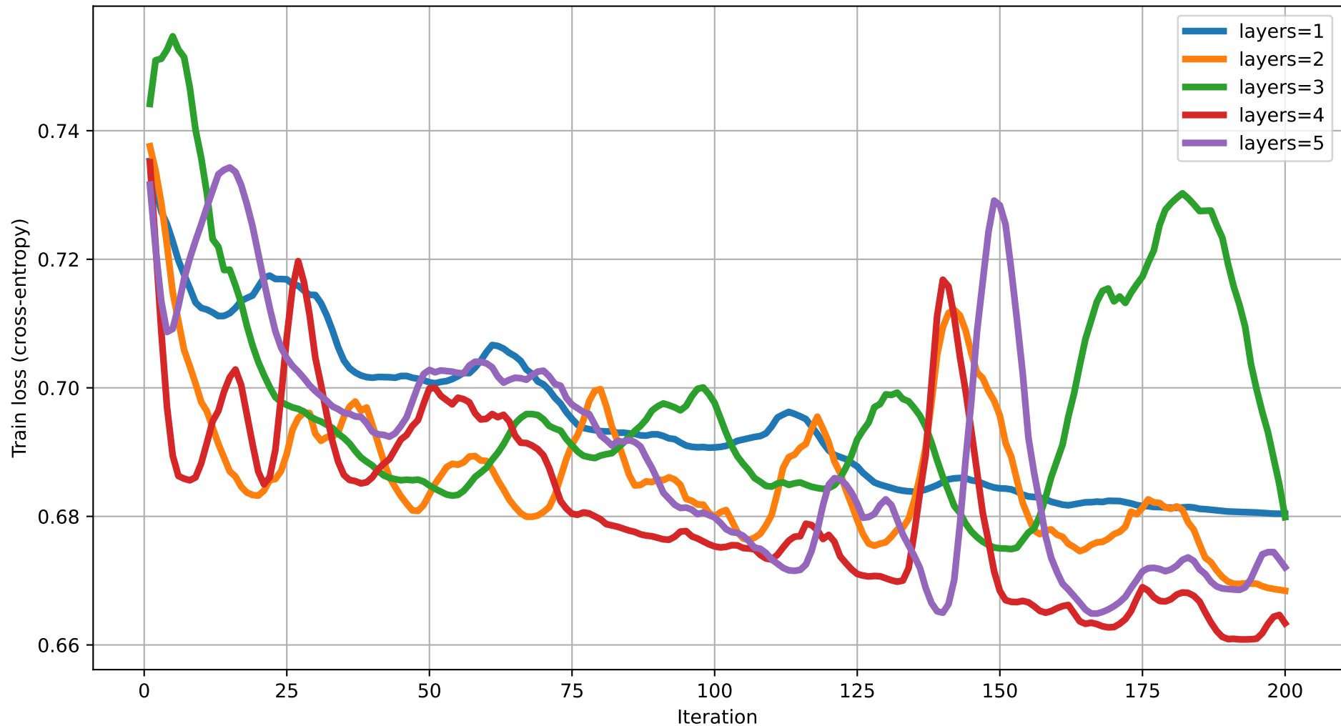
Train loss vs Iteration (dim=16) rot=RZ, ent=full, gate=IsingXX
