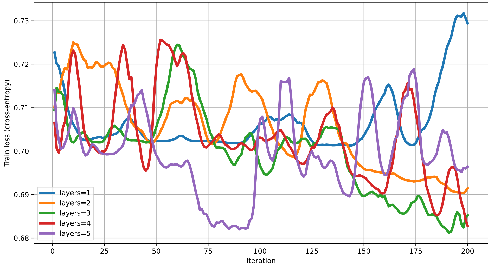
Train loss vs Iteration (dim=11) rot=Rot, ent=chain, gate=CZ
