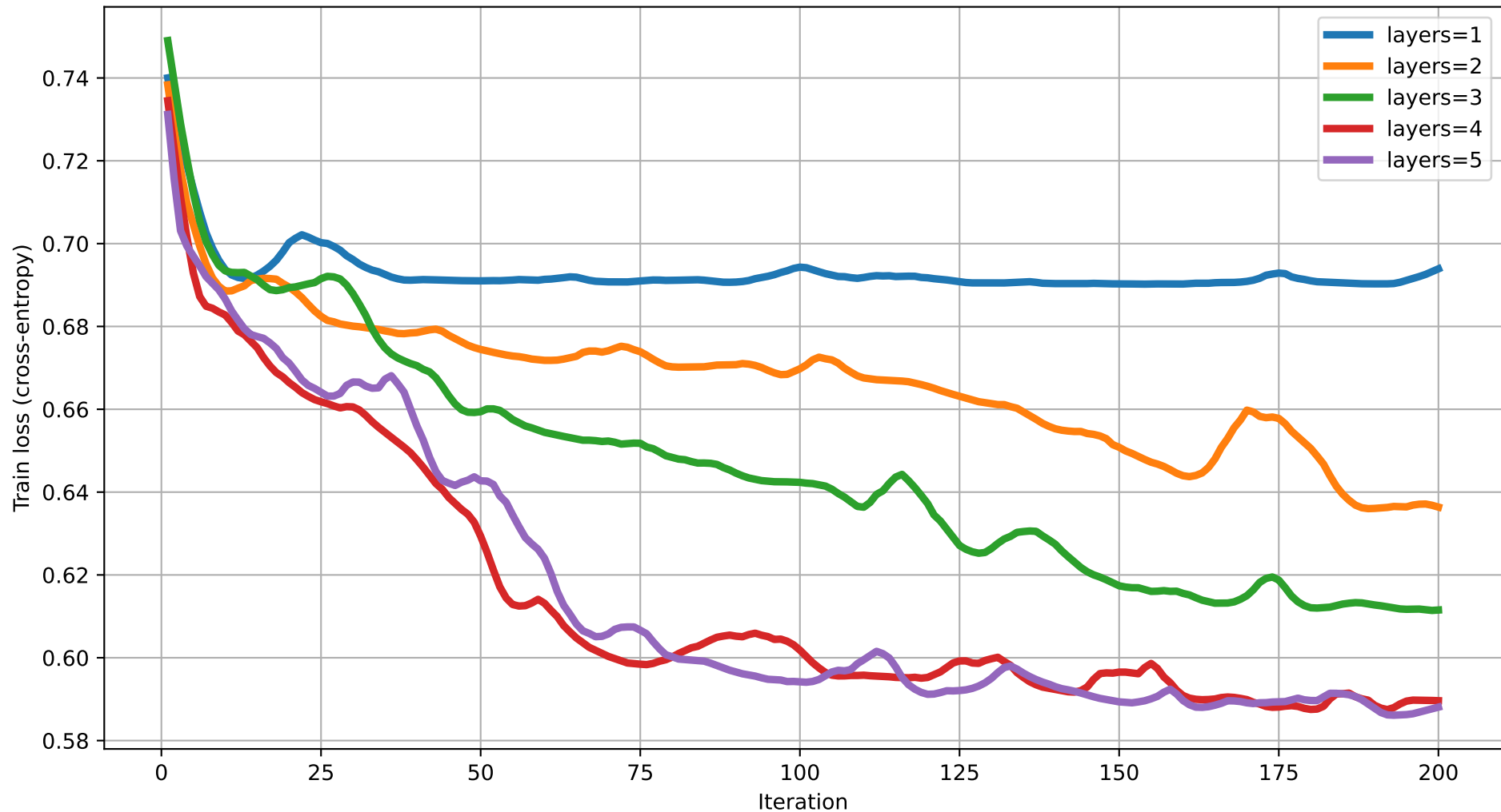
Train loss vs Iteration (degree=5) rot=RYZ, ent=chain, gate=CZ
