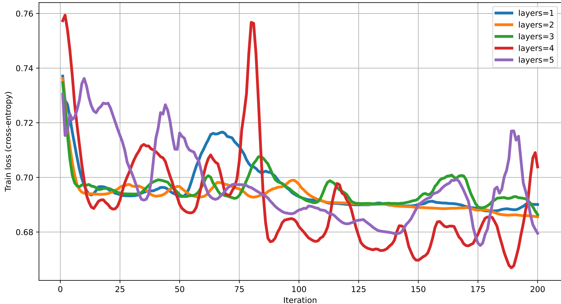
Train loss vs Iteration (dim=16) rot=RY, ent=ring, gate=CZ
