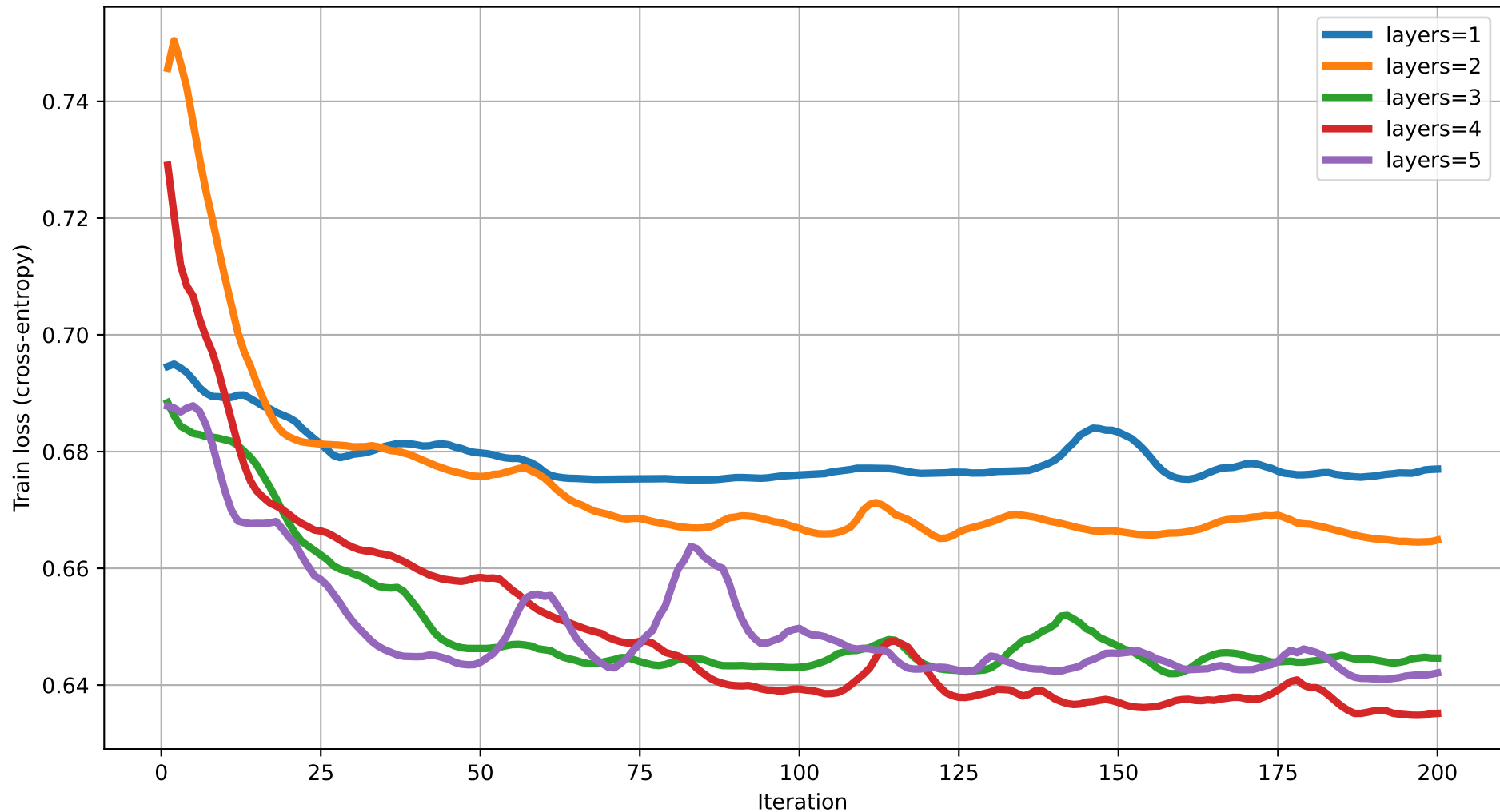
Train loss vs Iteration (degree=2) rot=RZ, ent=ring, gate=IsingXX
