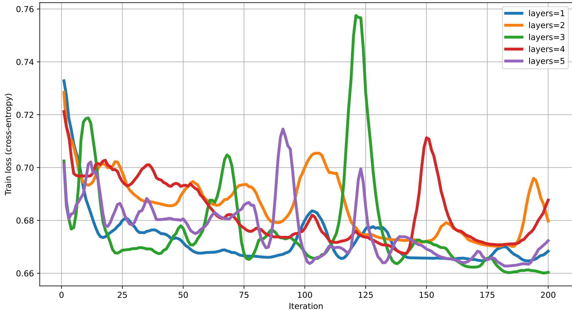
Train loss vs Iteration (dim=19) rot=RYZ, ent=ring, gate=IsingXX
