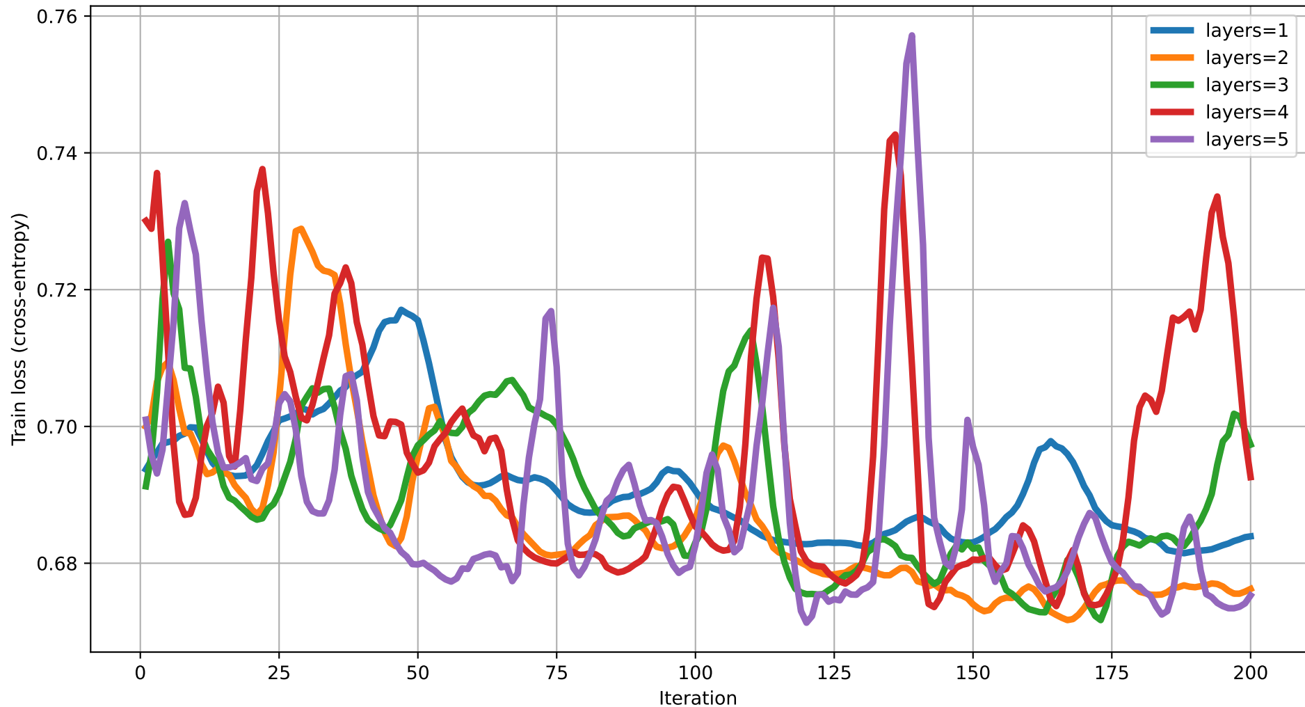
Train loss vs Iteration (dim=14) rot=Rot, ent=full, gate=IsingXX
