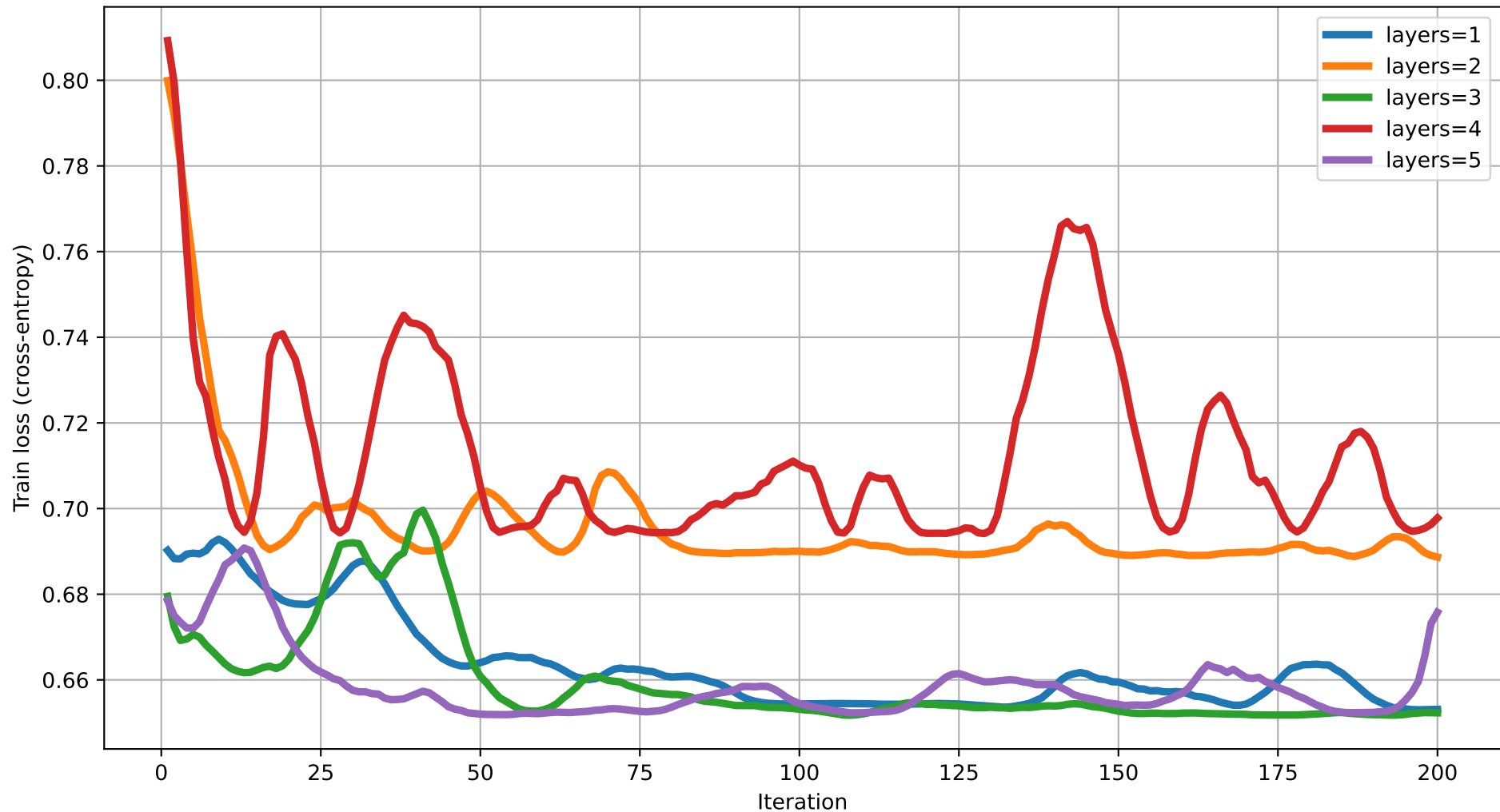
Train loss vs Iteration (dim=4) rot=RX, ent=pairwise, gate=IsingXX
