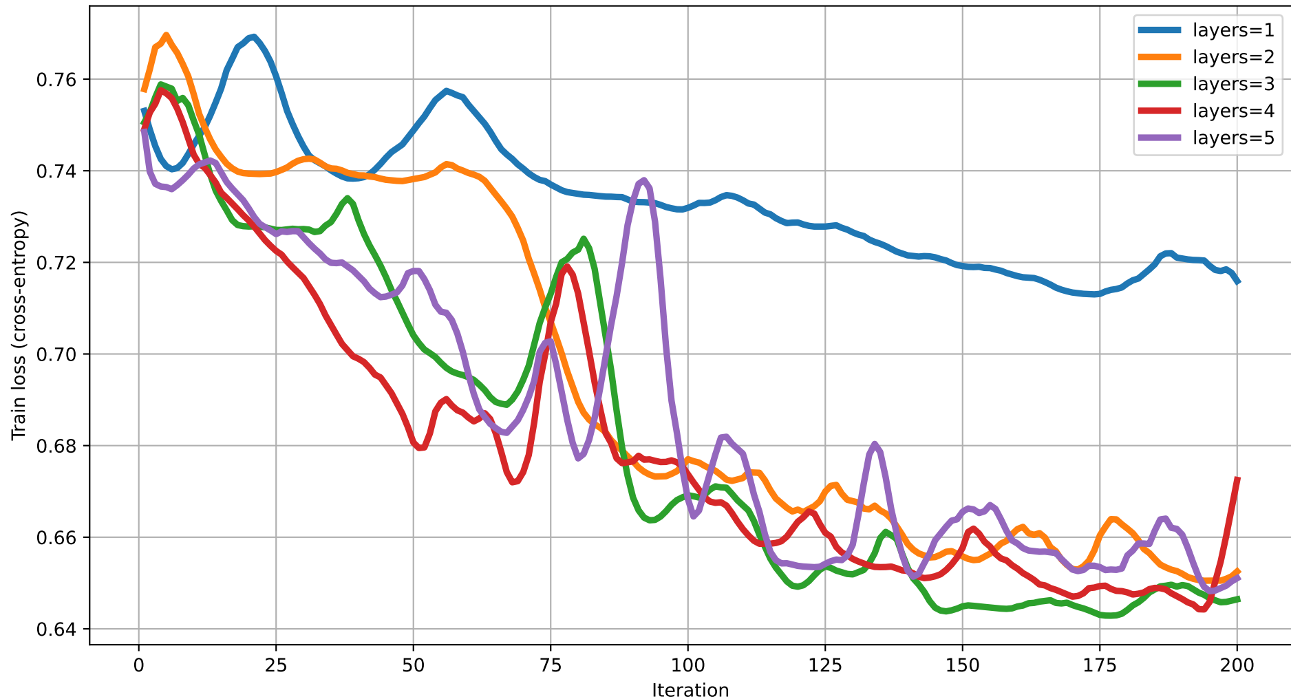
Train loss vs Iteration (dim=5) rot=RY, ent=chain, gate=CZ
