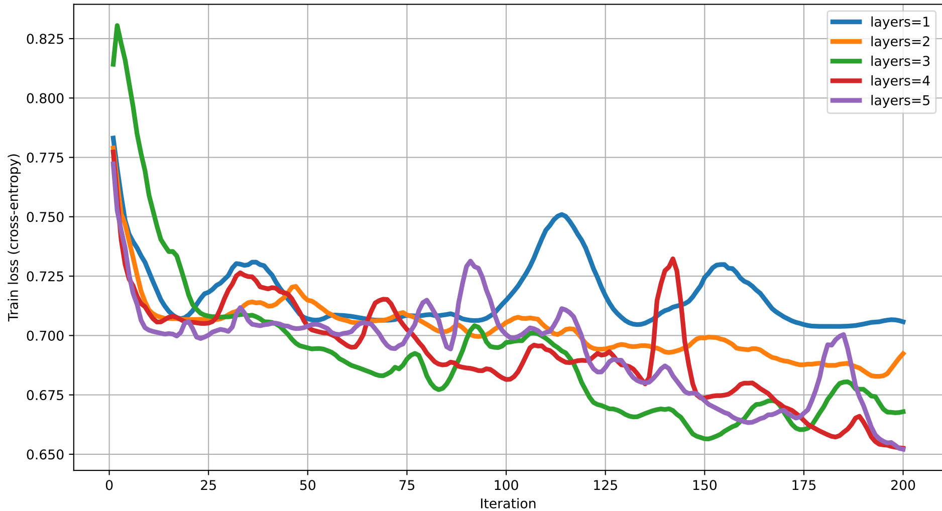
Train loss vs Iteration (dim=9) rot=Rot, ent=ring, gate=CZ
