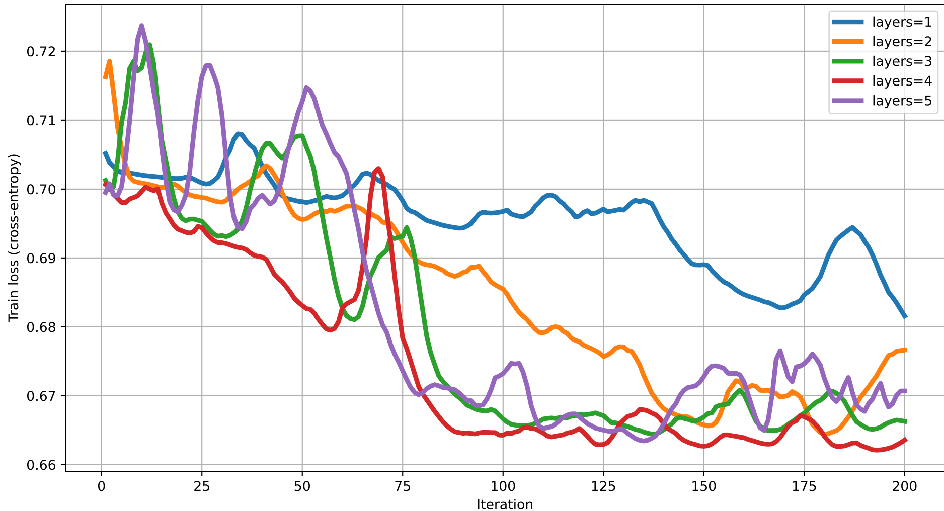
Train loss vs Iteration (dim=14) rot=RY, ent=pairwise, gate=CNOT
