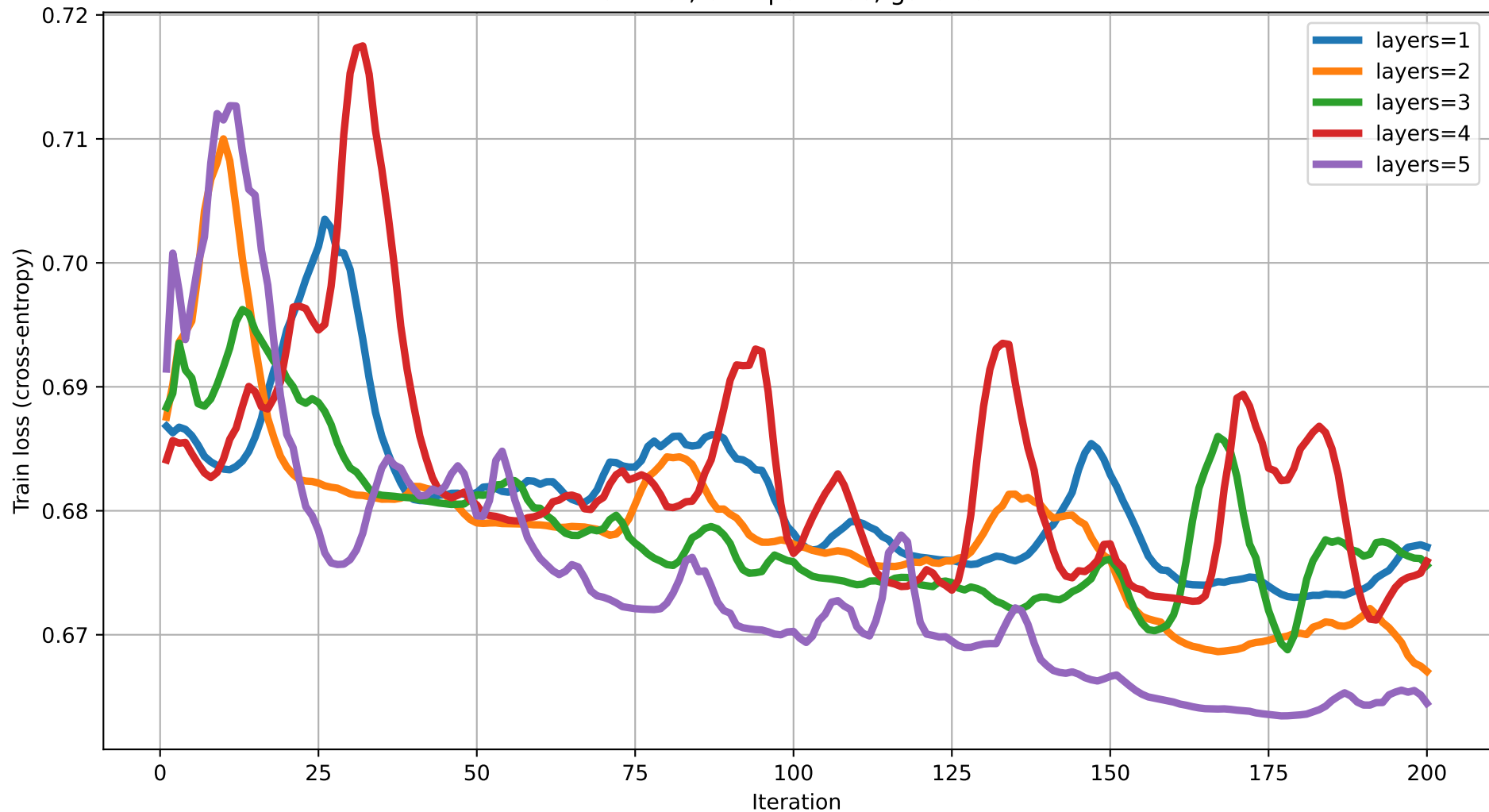
Train loss vs Iteration (dim=15) rot=Rot, ent=pairwise, gate=CZ
