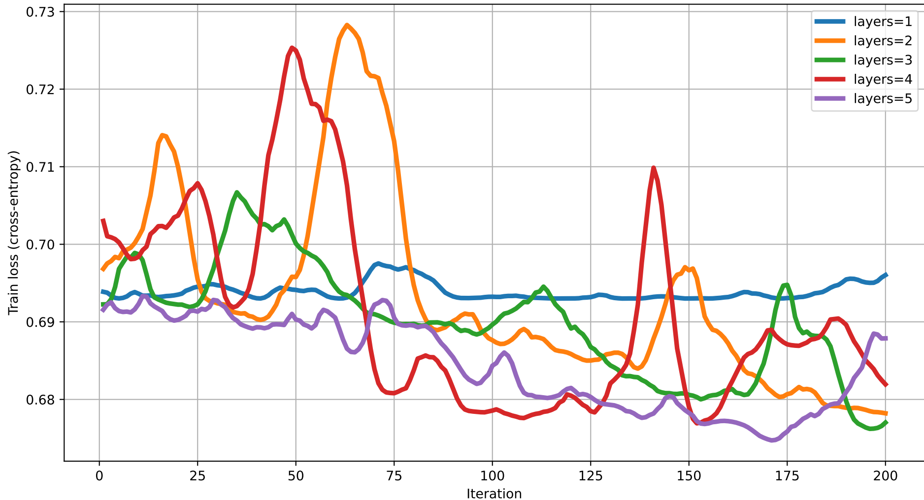
Train loss vs Iteration (dim=14) rot=RY, ent=full, gate=IsingXX
