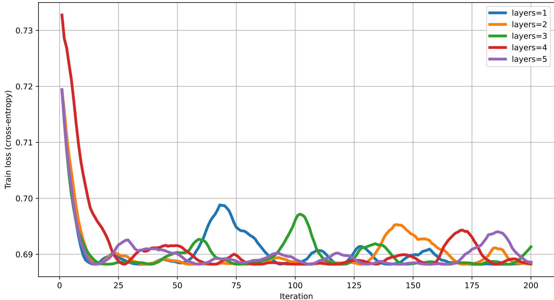
Train loss vs Iteration (degree=4) rot=RZ, ent=ring, gate=CZ
