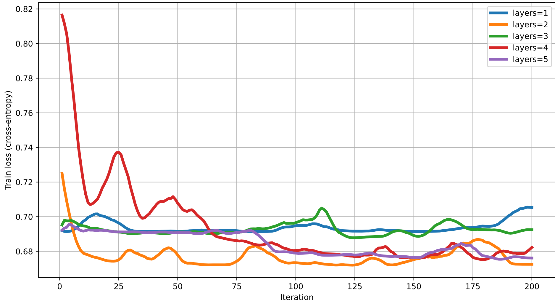
Train loss vs Iteration (dim=9) rot=RY, ent=chain, gate=IsingXX
