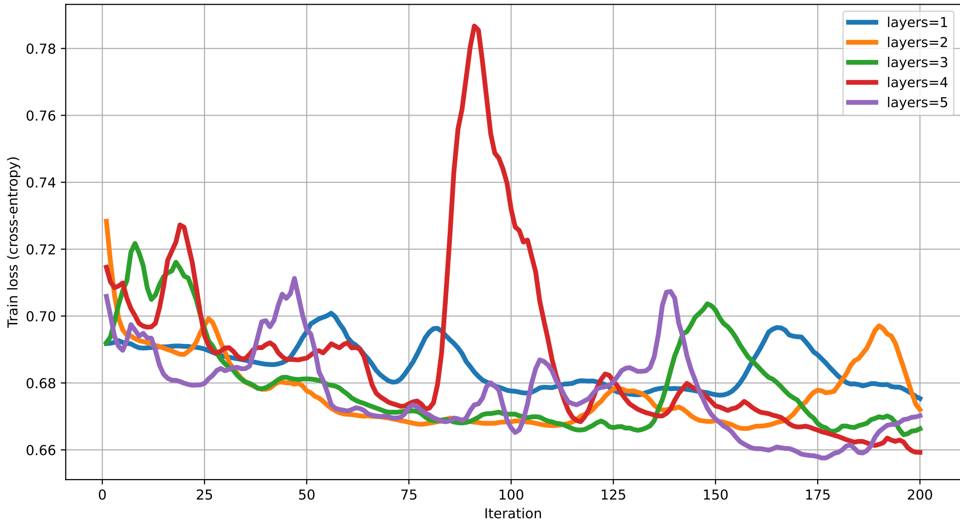
Train loss vs Iteration (dim=10) rot=RYZ, ent=chain, gate=IsingXX
