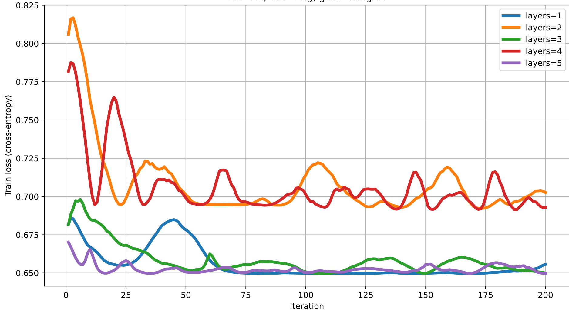
Train loss vs Iteration (dim=9) rot=RX, ent=ring, gate=IsingXX
