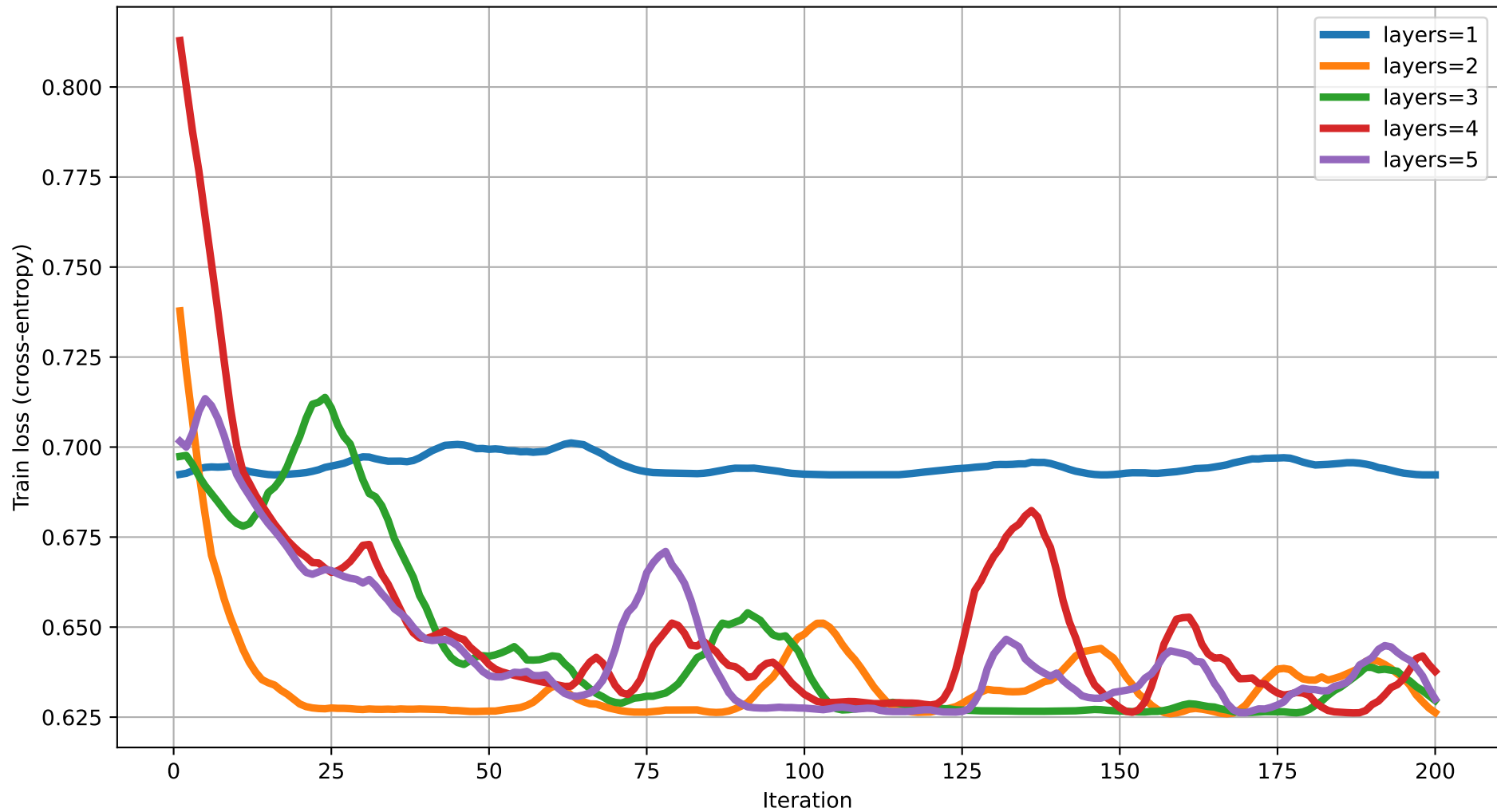
Train loss vs Iteration (dim=2) rot=RY, ent=chain, gate=IsingXX
