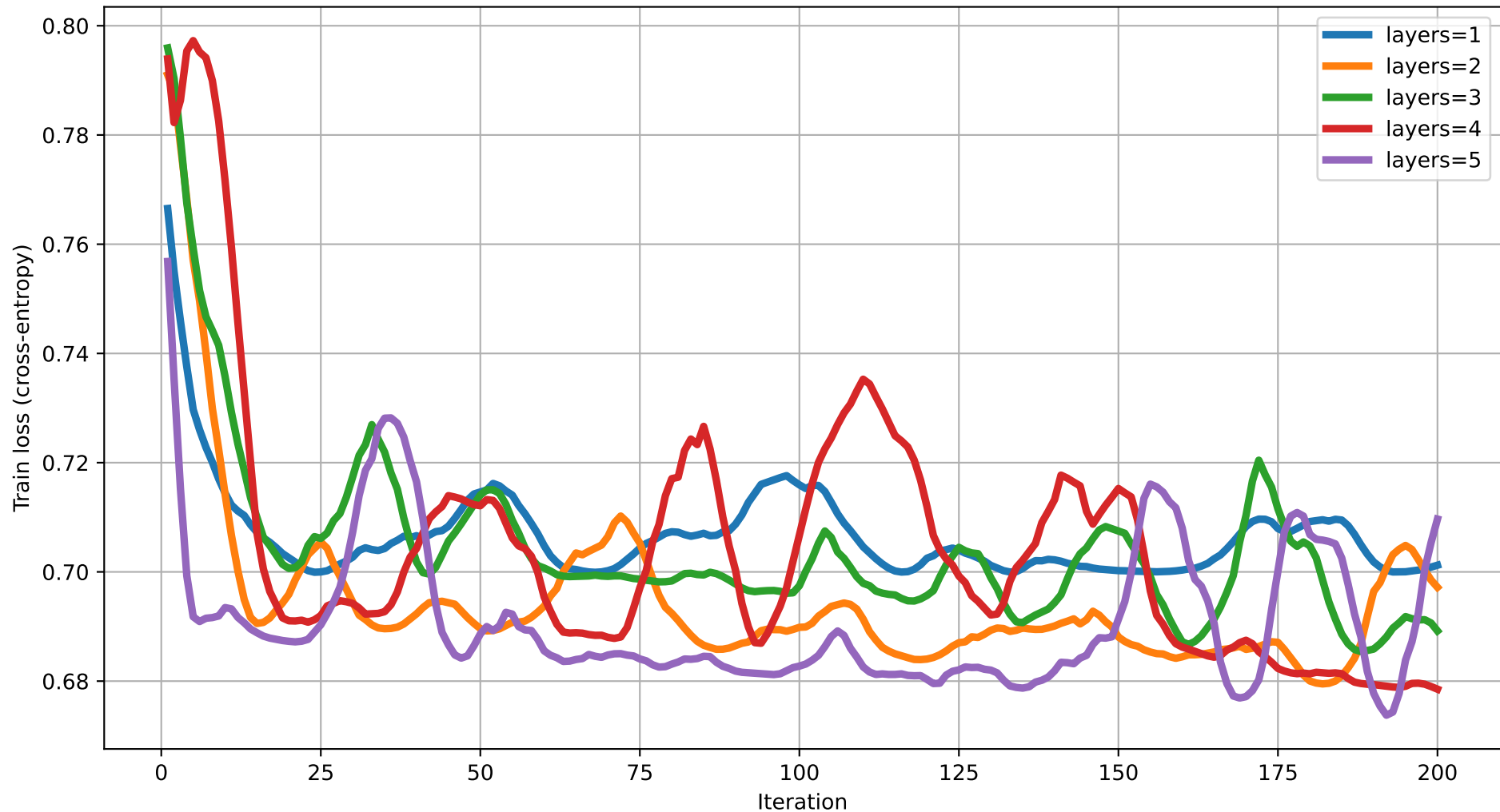
Train loss vs Iteration (dim=17) rot=RY, ent=pairwise, gate=CZ
