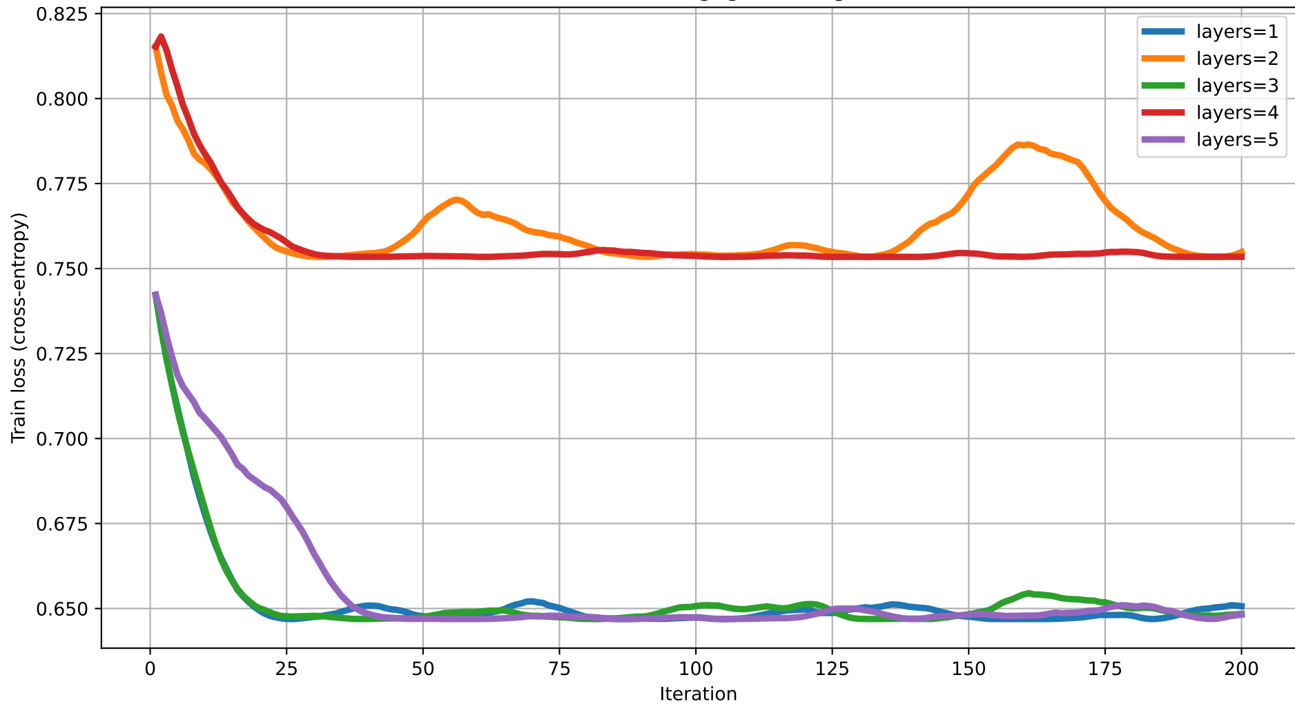
Train loss vs Iteration (dim=2) rot=RZ, ent=ring, gate=IsingXX
