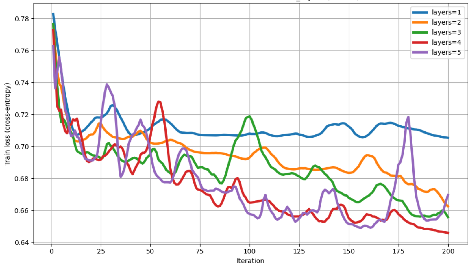
Train loss vs Iteration for different num_layers (dim=9)
