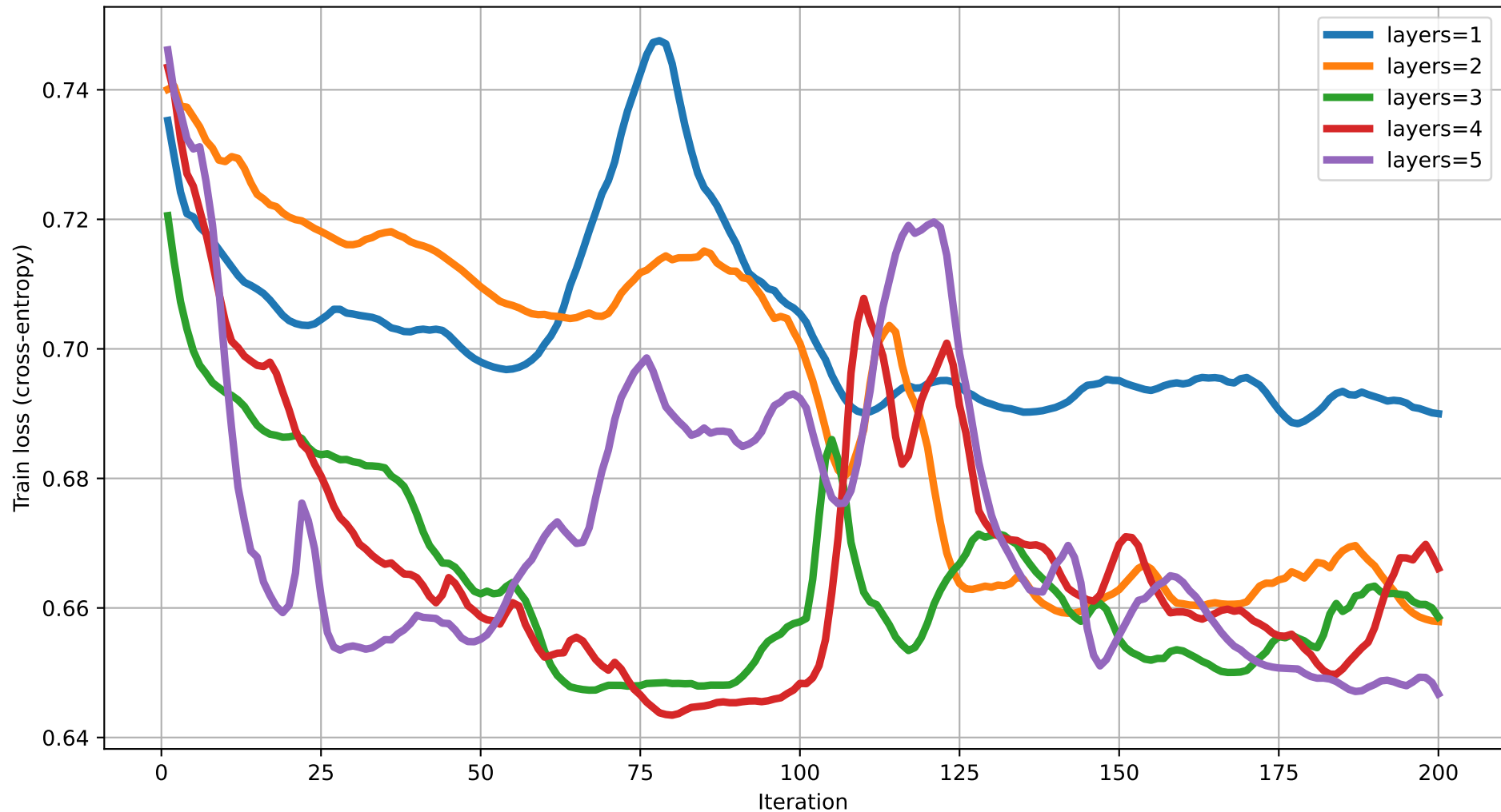
Train loss vs Iteration (dim=5) rot=Rot, ent=full, gate=CZ
