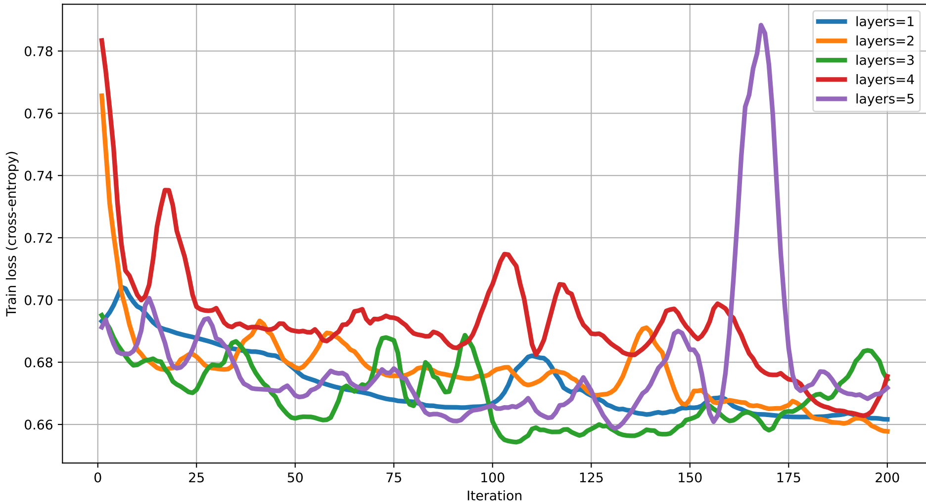
Train loss vs Iteration (dim=8) rot=RYZ, ent=chain, gate=IsingXX
