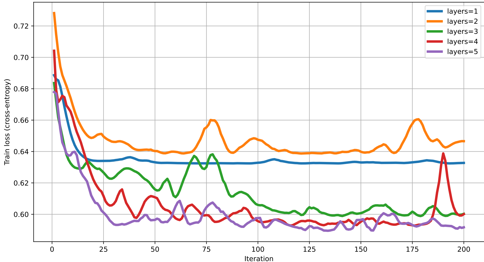
Train loss vs Iteration (degree=2) rot=Rot, ent=chain, gate=IsingXX
