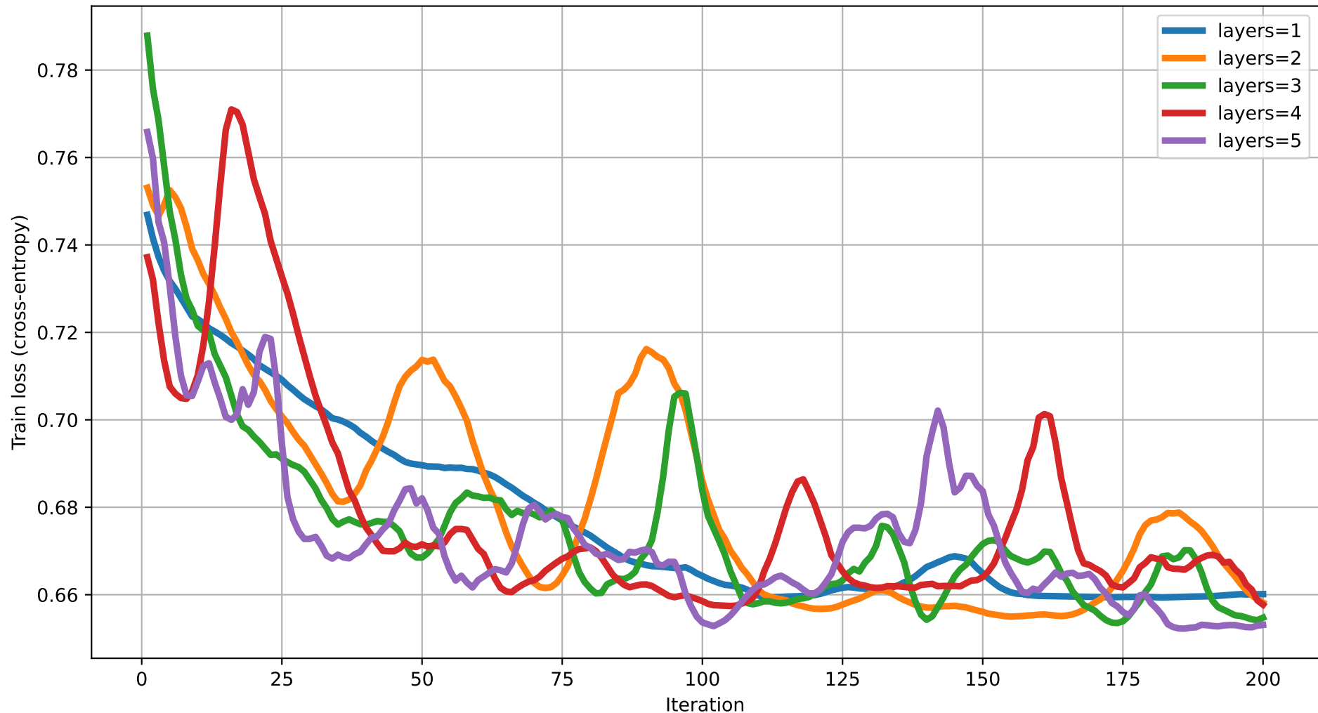
Train loss vs Iteration (dim=2) rot=Rot, ent=ring, gate=CNOT
