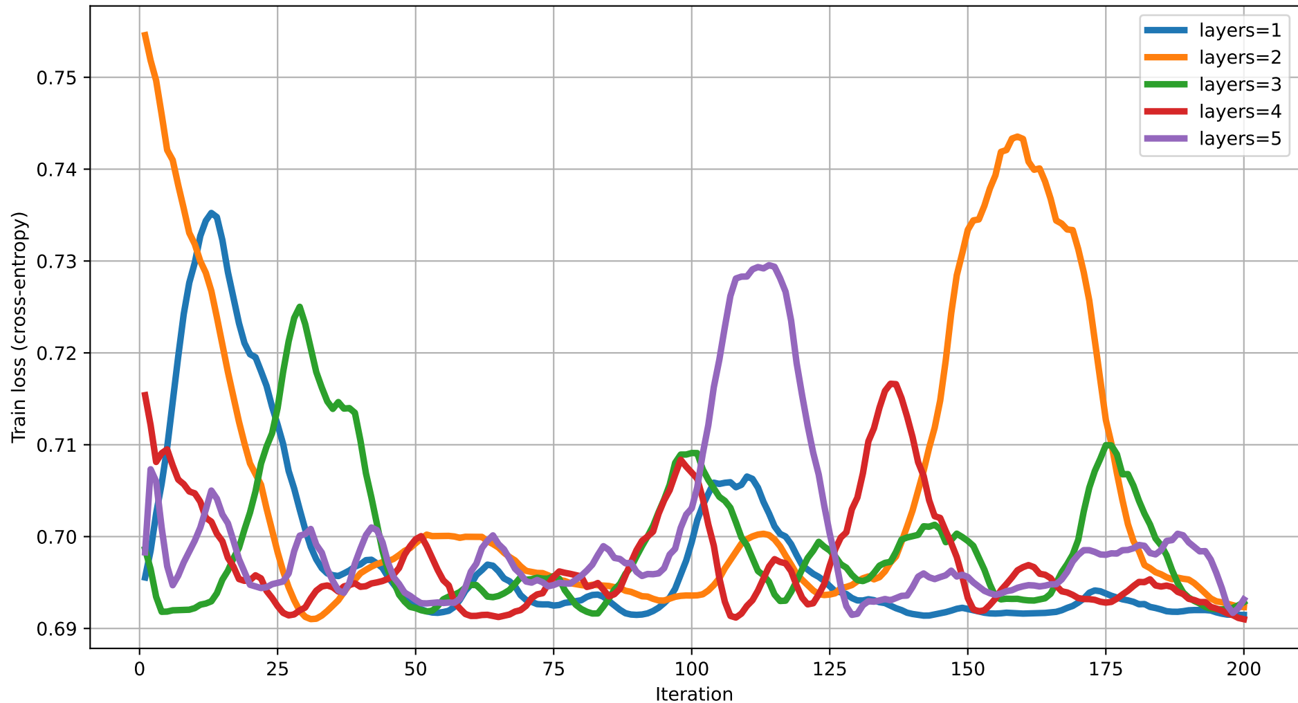
Train loss vs Iteration (dim=3) rot=RX, ent=pairwise, gate=IsingXX
