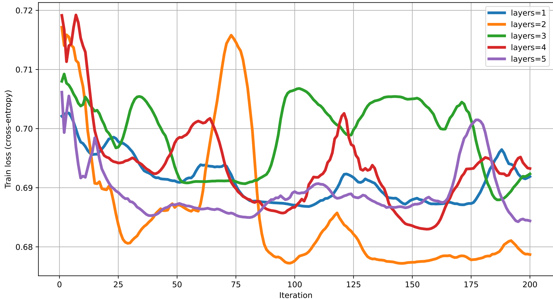
Train loss vs Iteration (dim=15) rot=RX, ent=ring, gate=CNOT
