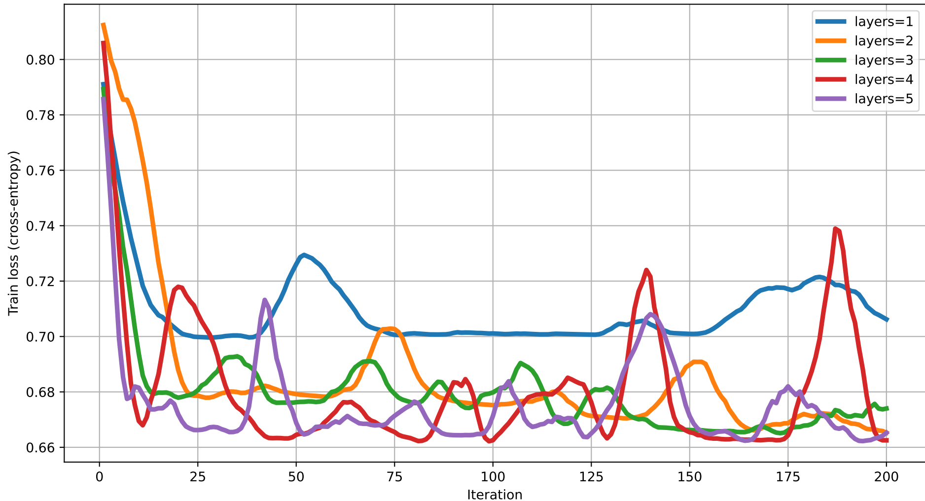
Train loss vs Iteration (dim=2) rot=RX, ent=chain, gate=CNOT
