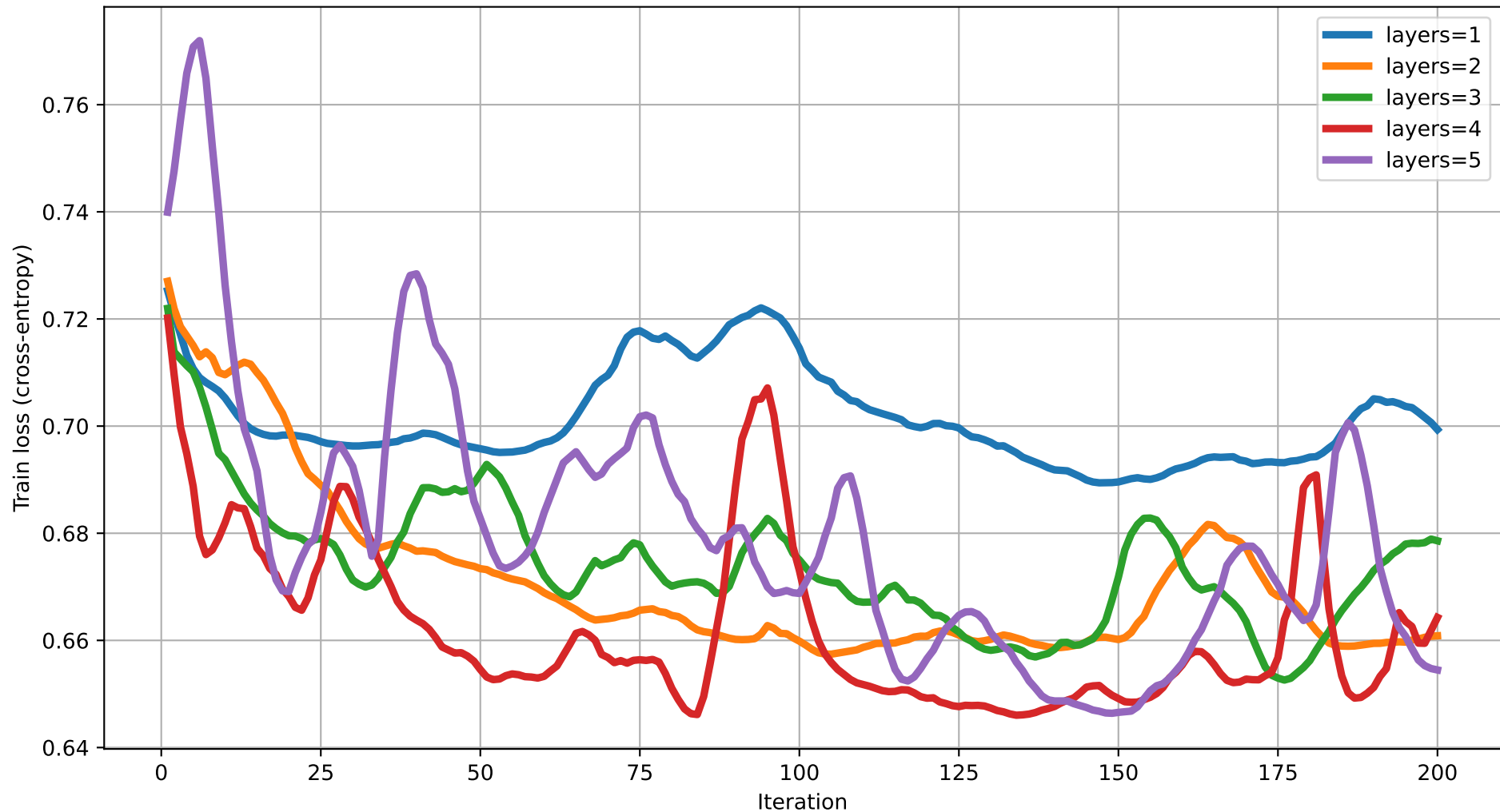
Train loss vs Iteration (dim=5) rot=Rot, ent=chain, gate=CNOT
