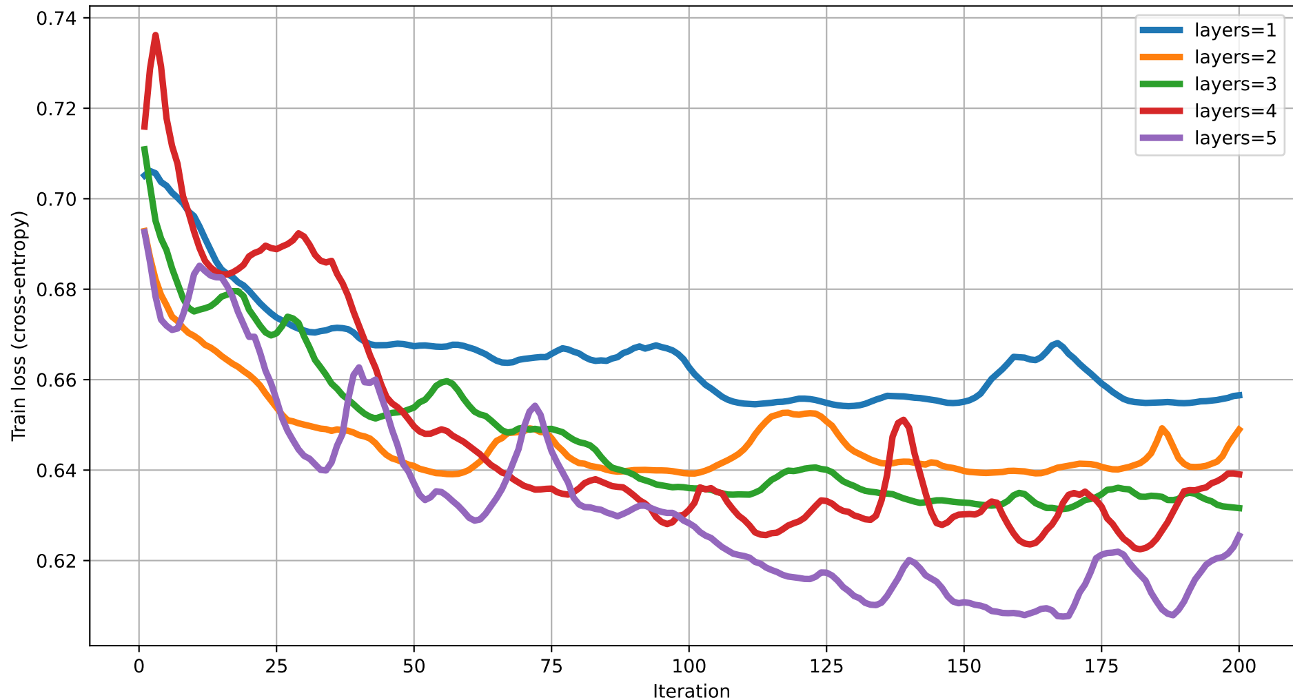
Train loss vs Iteration (dim=14) rot=Rot, ent=chain, gate=CNOT
