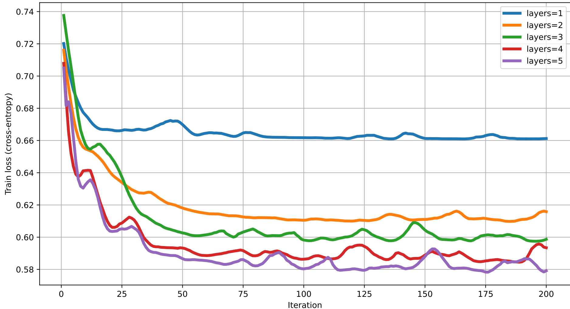
Train loss vs Iteration (degree=3) rot=RY, ent=full, gate=CNOT
