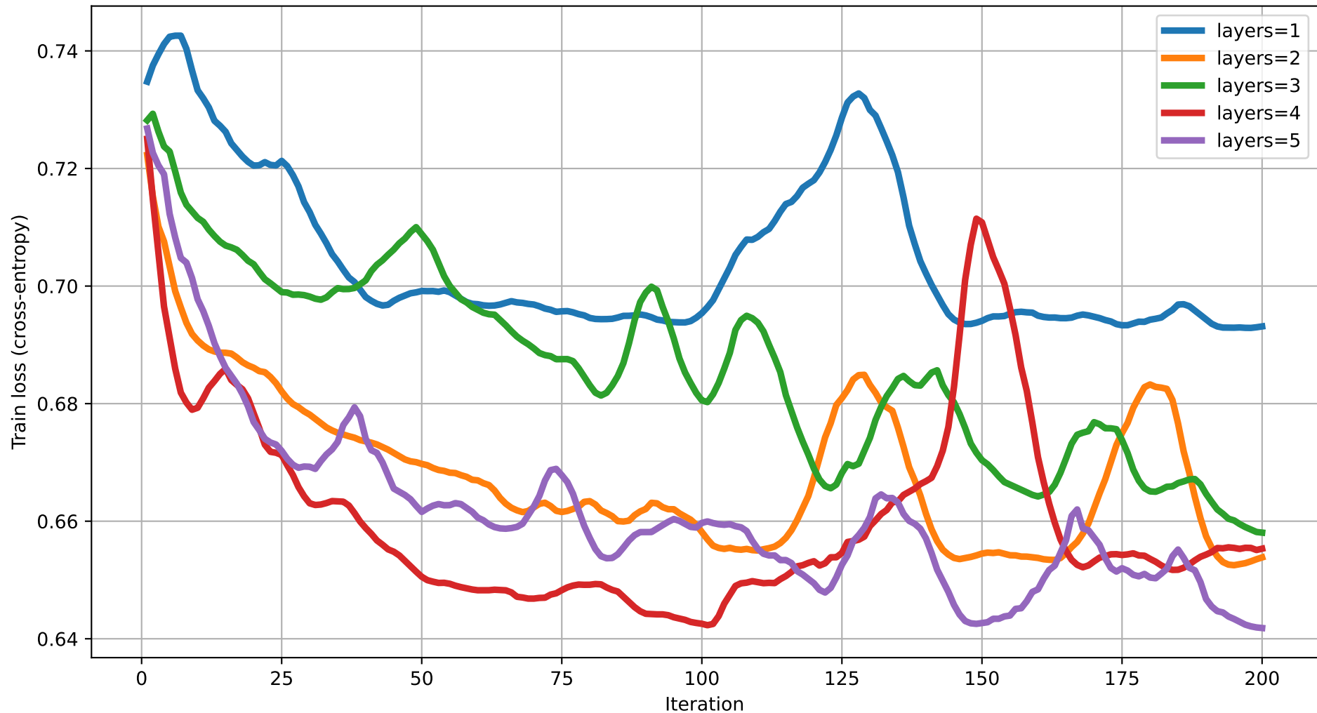
Train loss vs Iteration (dim=5) rot=RYZ, ent=full, gate=CNOT
