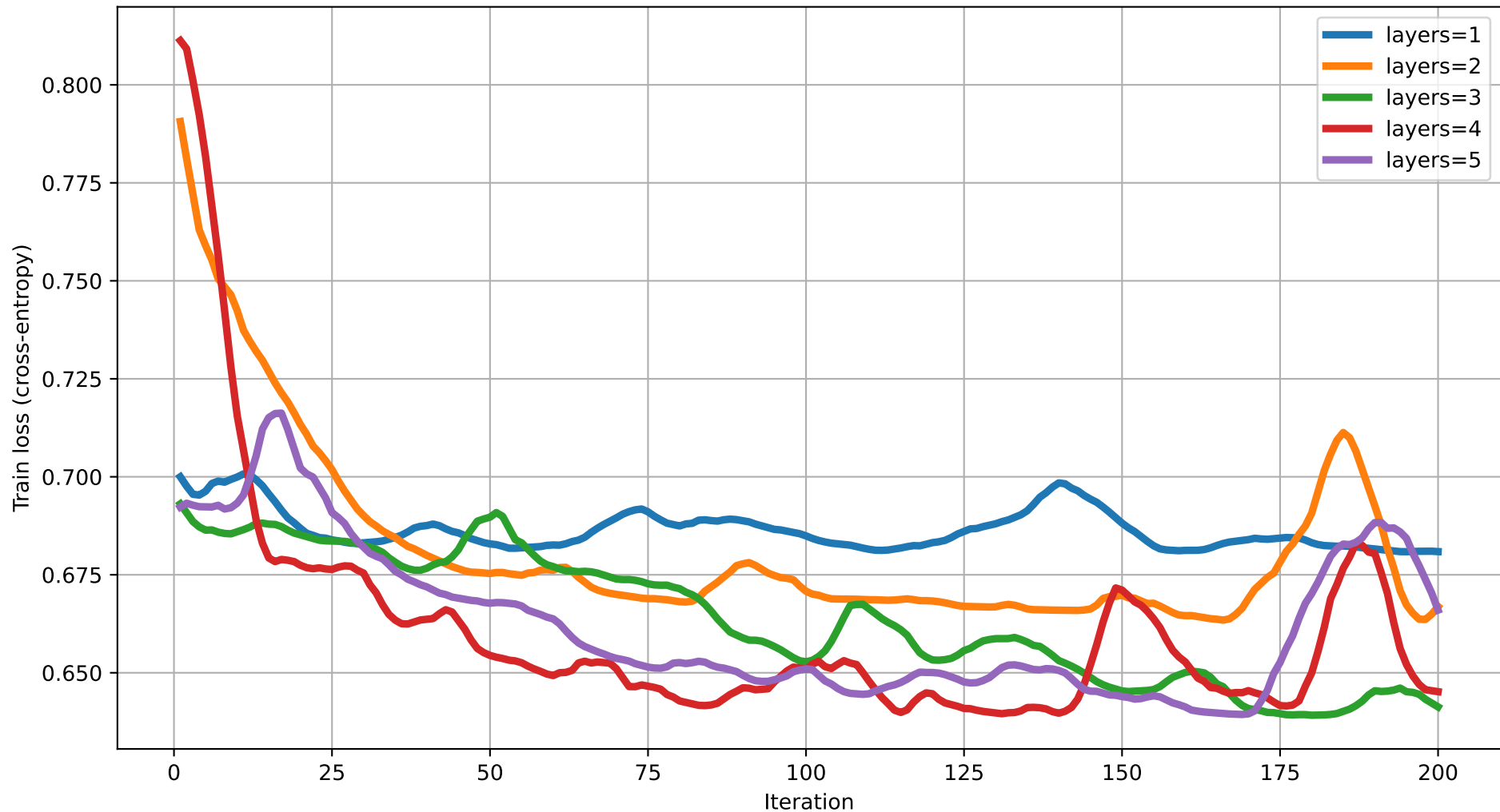
Train loss vs Iteration (dim=4) rot=RZ, ent=ring, gate=IsingXX
