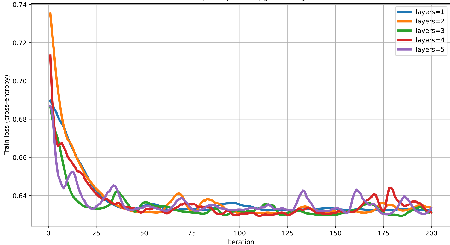
Train loss vs Iteration (degree=2) rot=RYZ, ent=pairwise, gate=IsingXX
