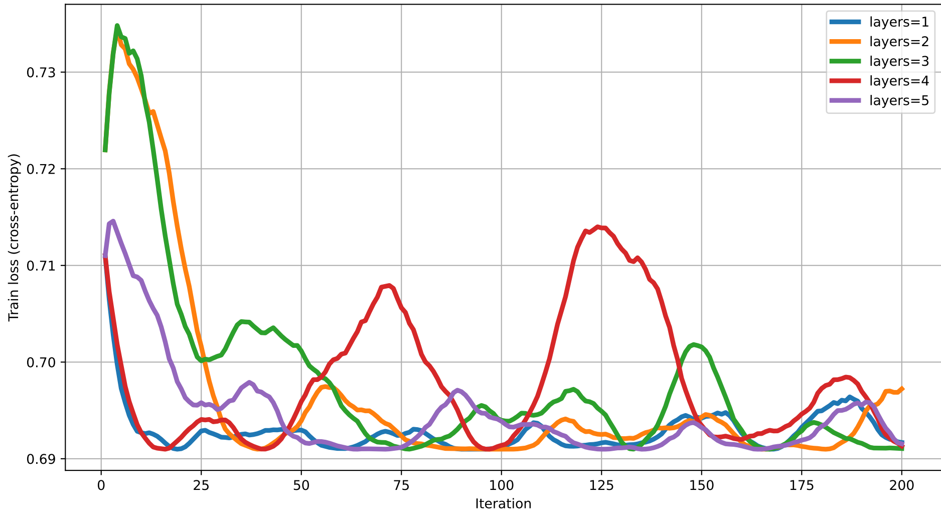
Train loss vs Iteration (dim=20) rot=RZ, ent=pairwise, gate=CZ
