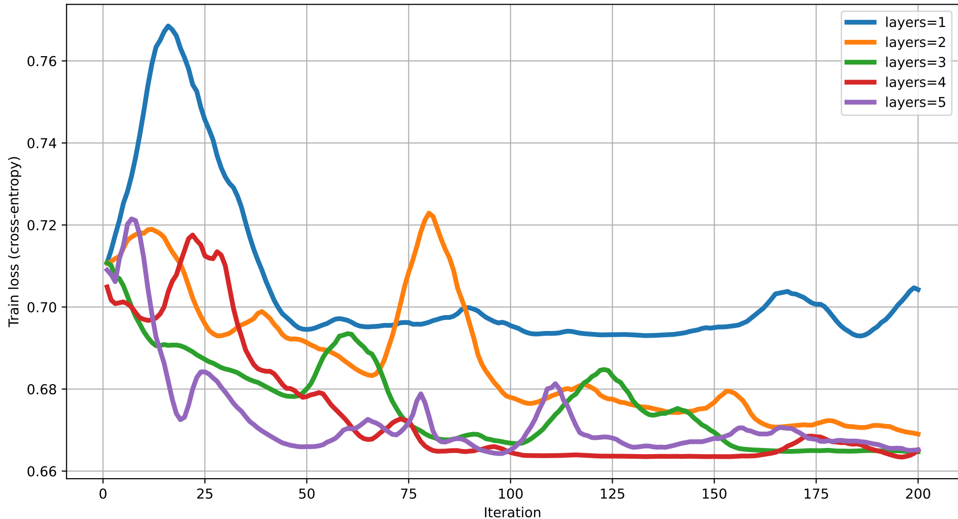
Train loss vs Iteration (dim=12) rot=RX, ent=chain, gate=CNOT
