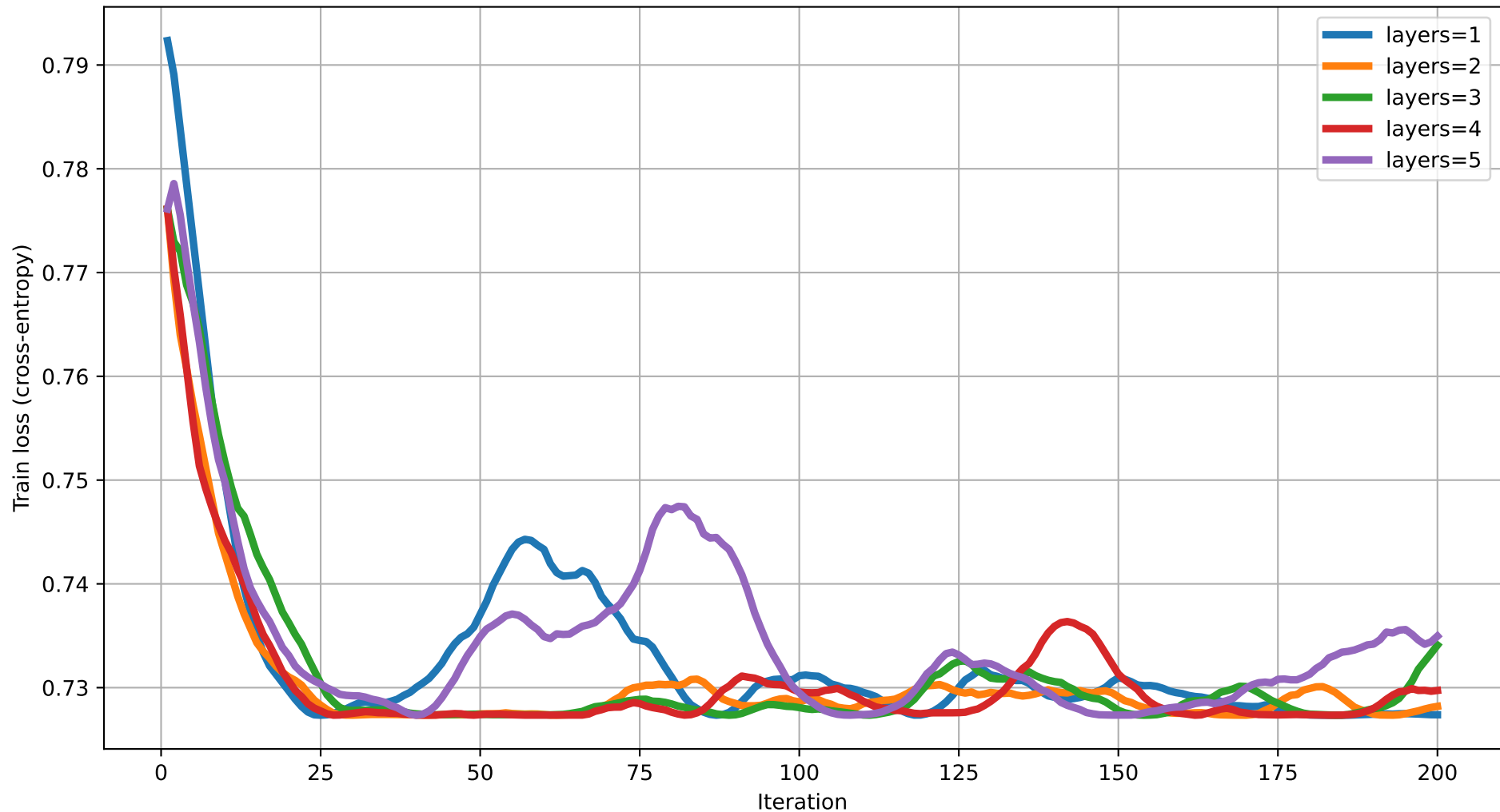
Train loss vs Iteration (dim=9) rot=RZ, ent=pairwise, gate=CNOT
