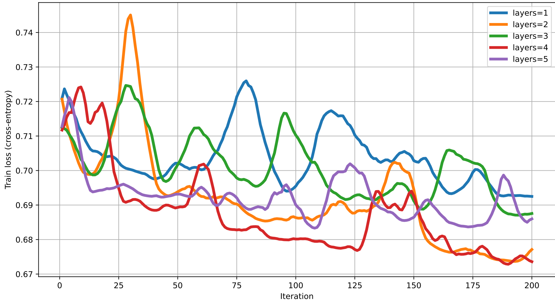
Train loss vs Iteration (dim=11) rot=RX, ent=chain, gate=CZ
