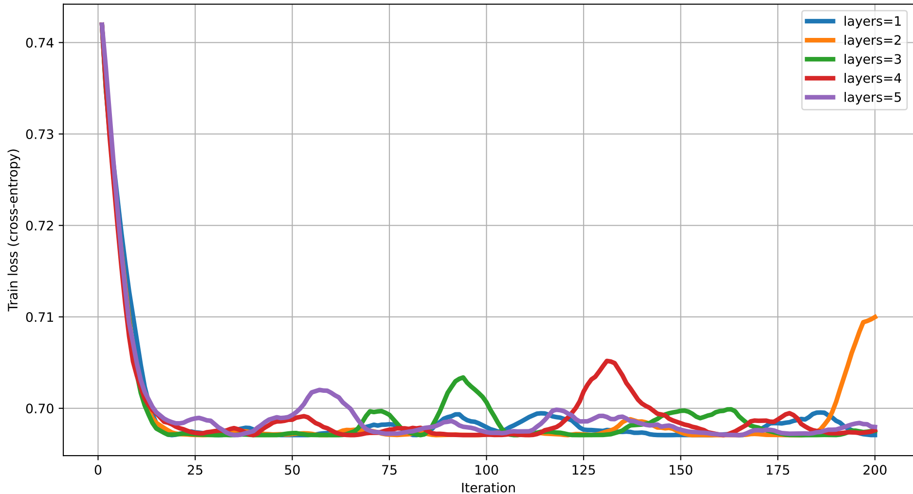
Train loss vs Iteration (degree=5) rot=RZ, ent=chain, gate=CNOT
