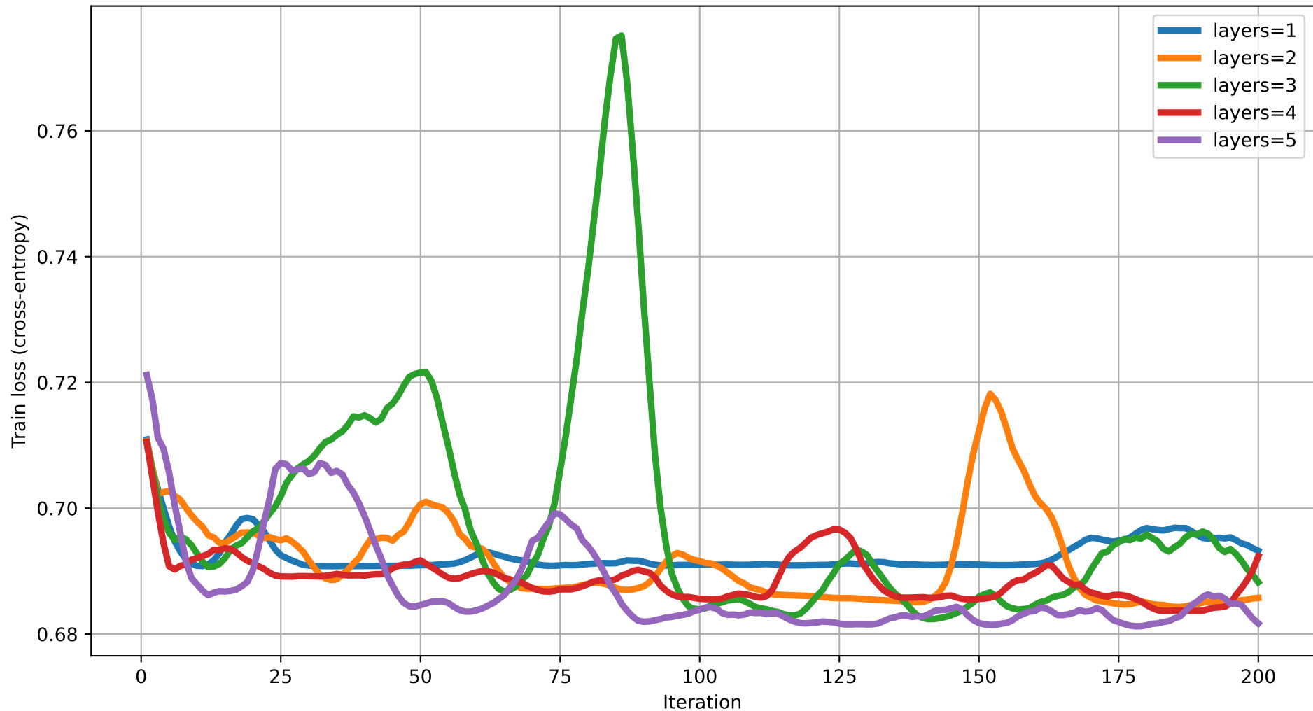
Train loss vs Iteration (dim=20) rot=RX, ent=chain, gate=CZ
