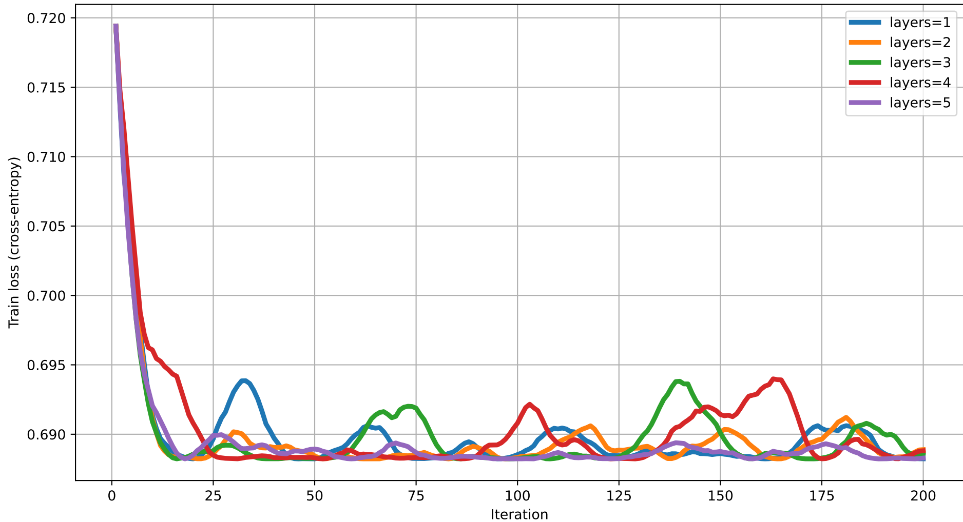
Train loss vs Iteration (degree=4) rot=RZ, ent=chain, gate=CNOT
