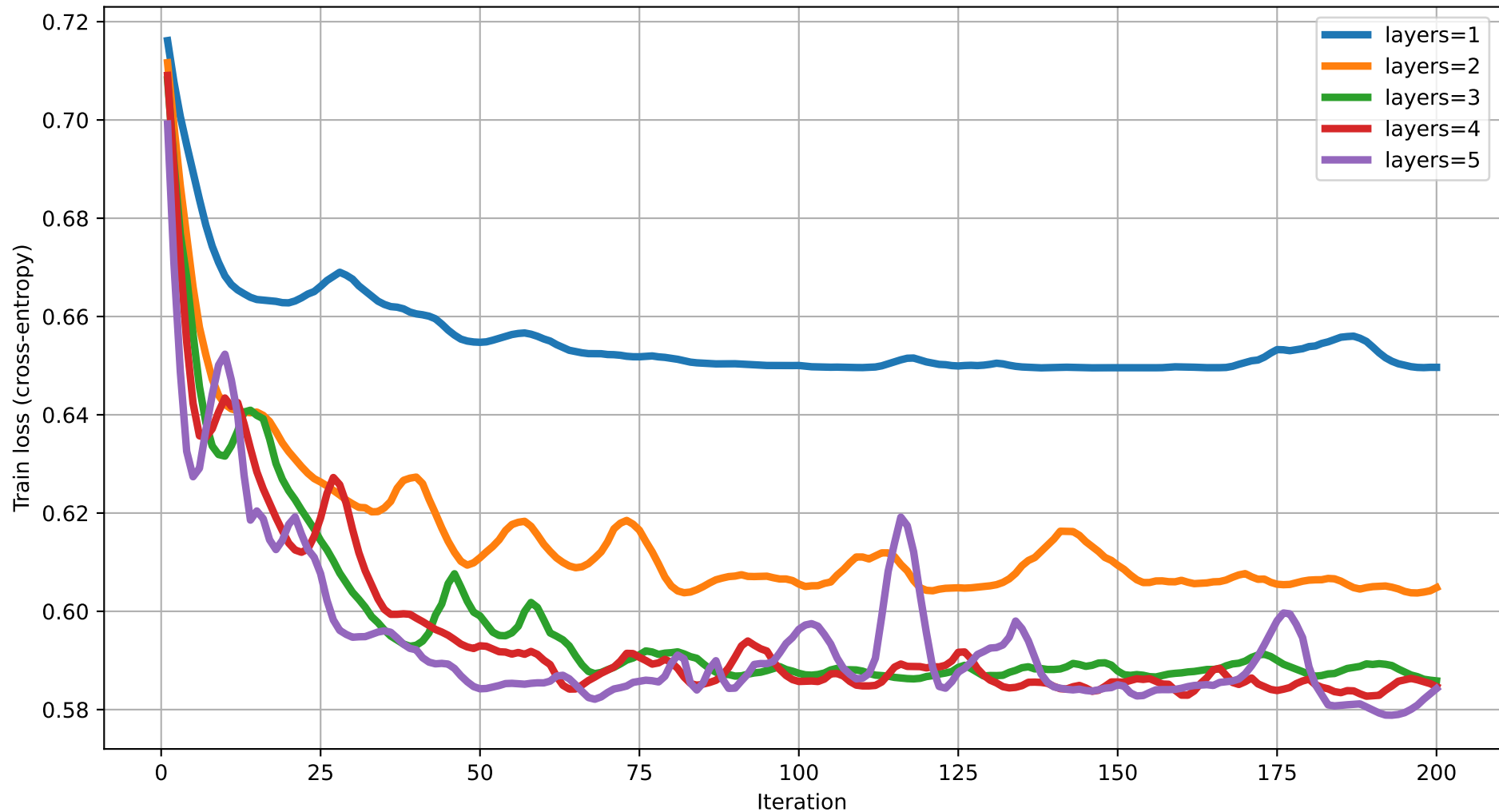
Train loss vs Iteration (degree=4) rot=Rot, ent=full, gate=CNOT
