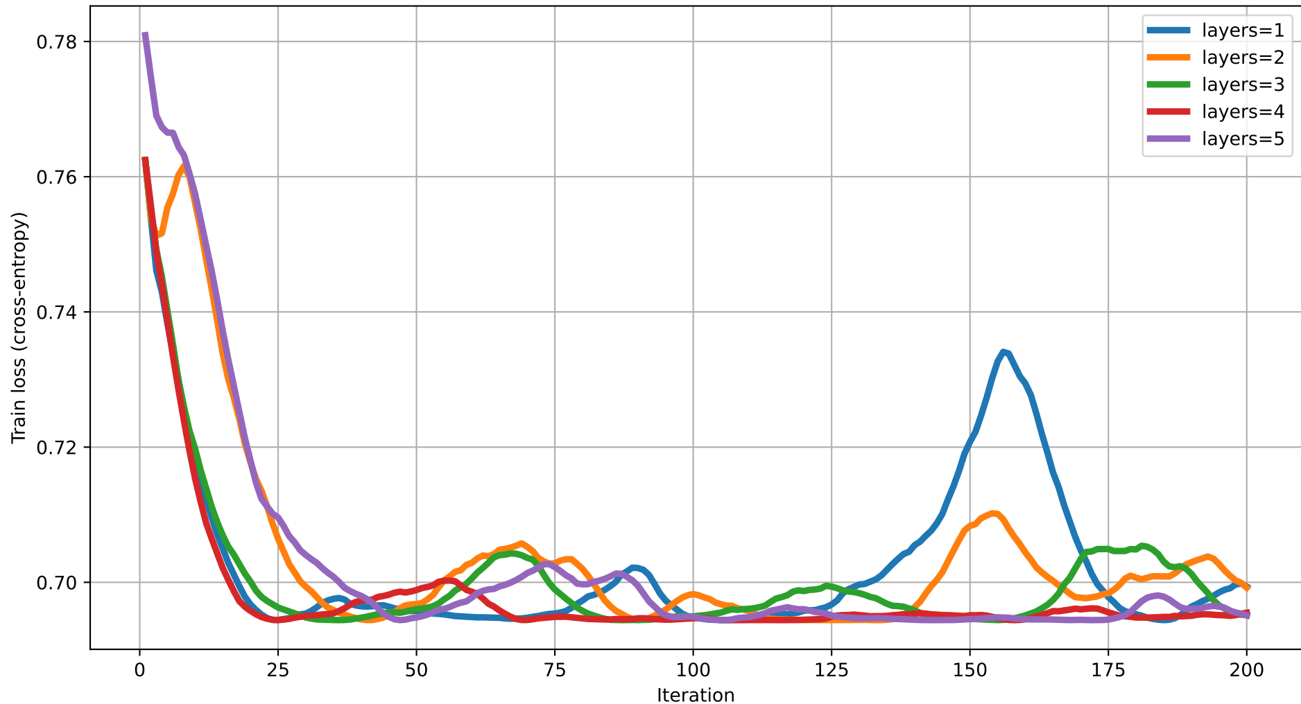
Train loss vs Iteration (dim=8) rot=RZ, ent=ring, gate=CZ
