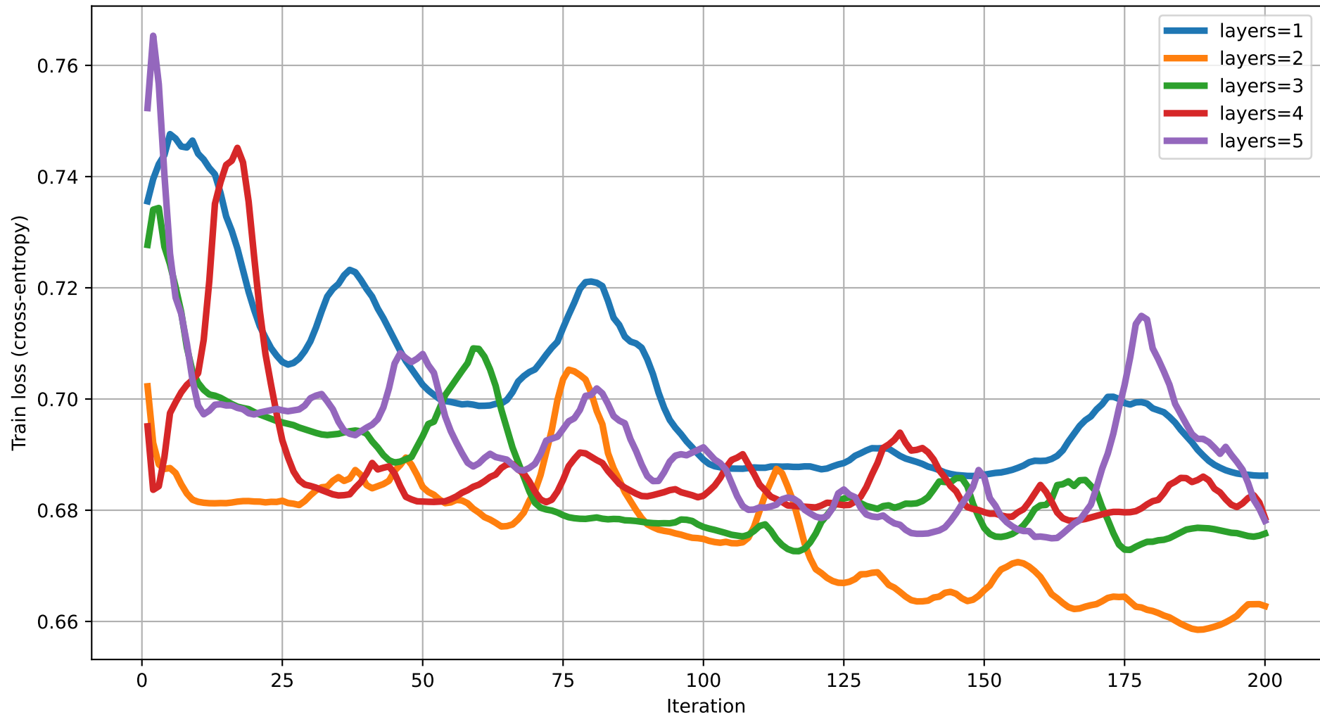
Train loss vs Iteration (dim=20) rot=RY, ent=full, gate=IsingXX
