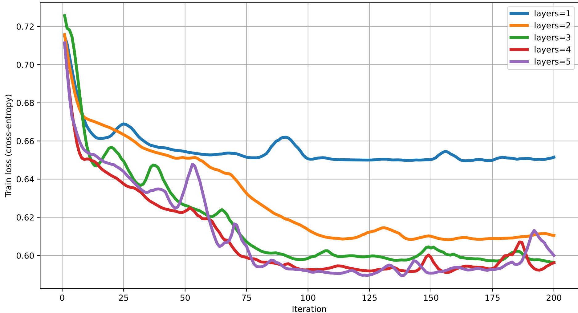
Train loss vs Iteration (degree=4) rot=RY, ent=ring, gate=CZ
