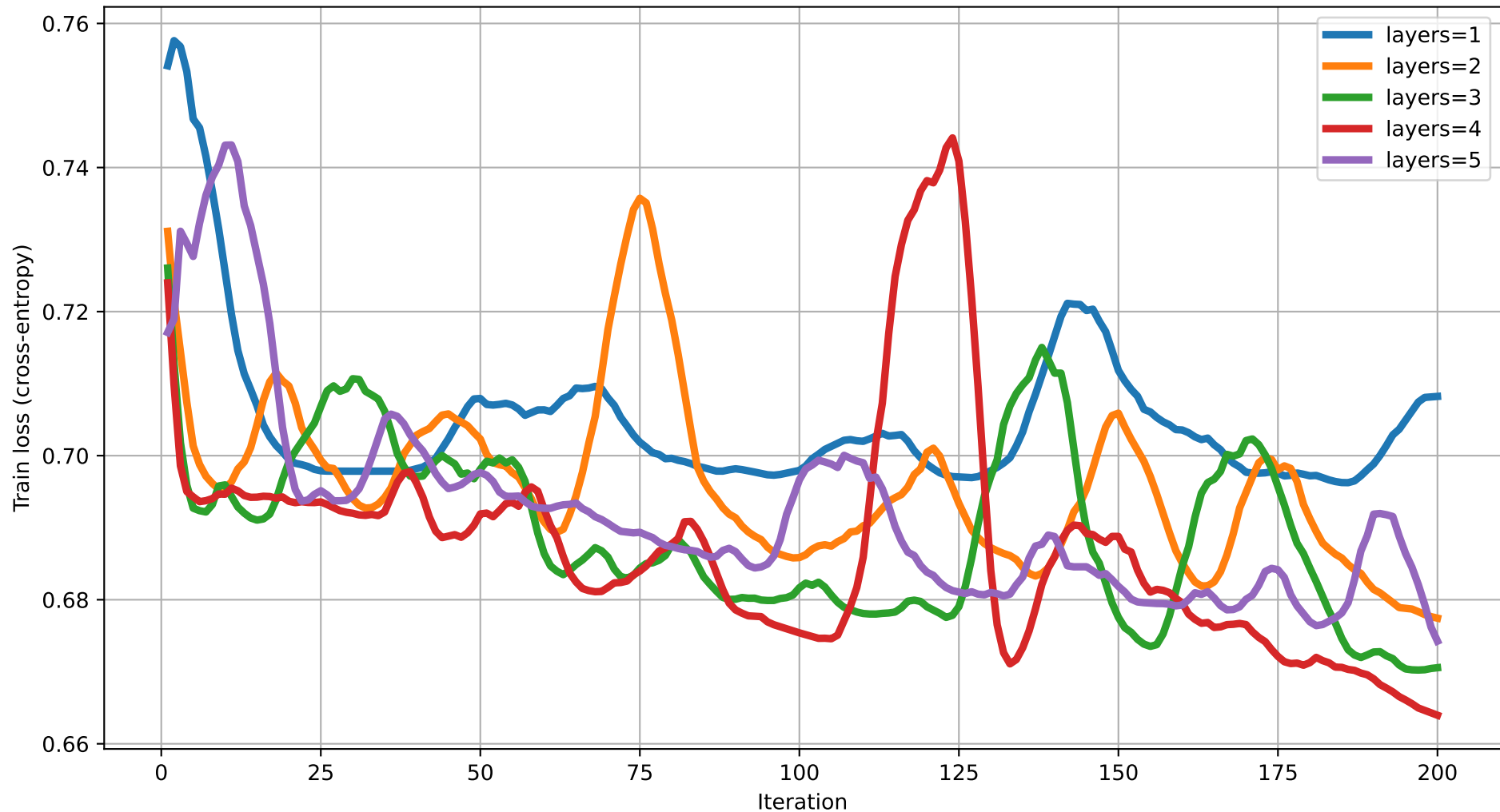
Train loss vs Iteration (dim=19) rot=RYZ, ent=chain, gate=CNOT
