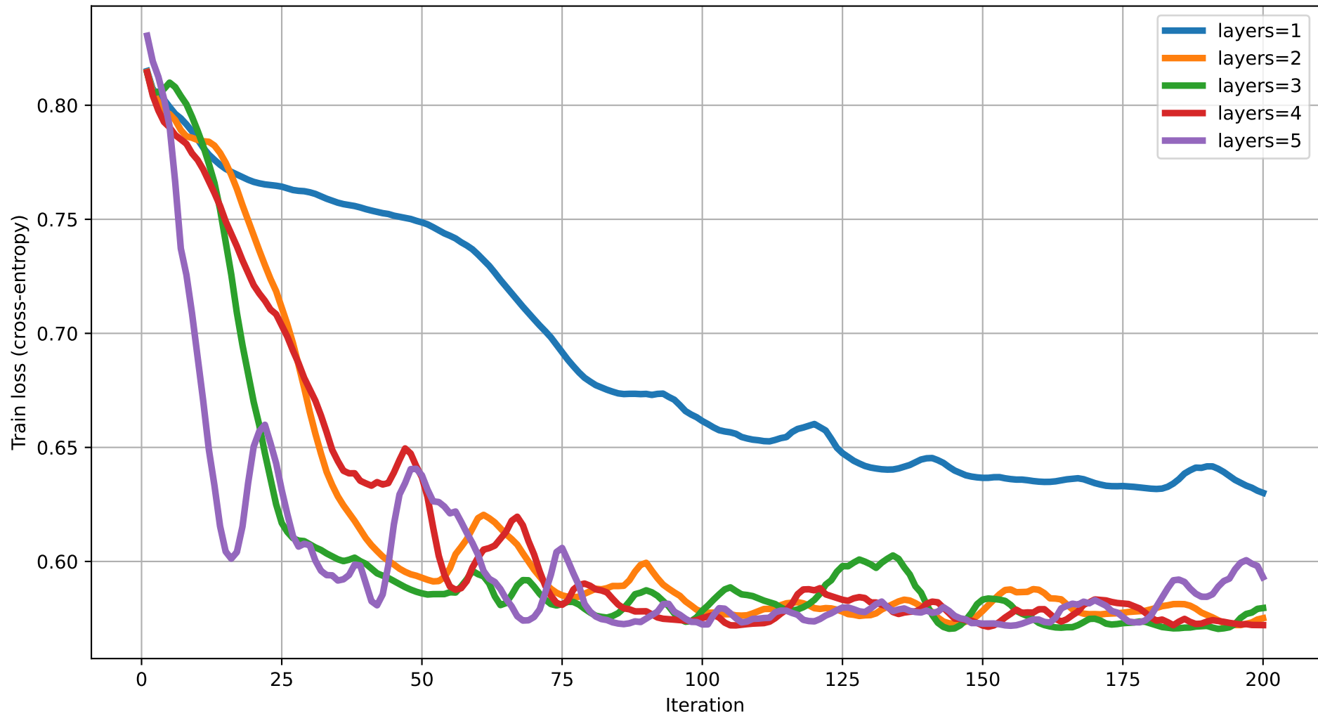
Train loss vs Iteration (dim=2) rot=Rot, ent=pairwise, gate=CZ
