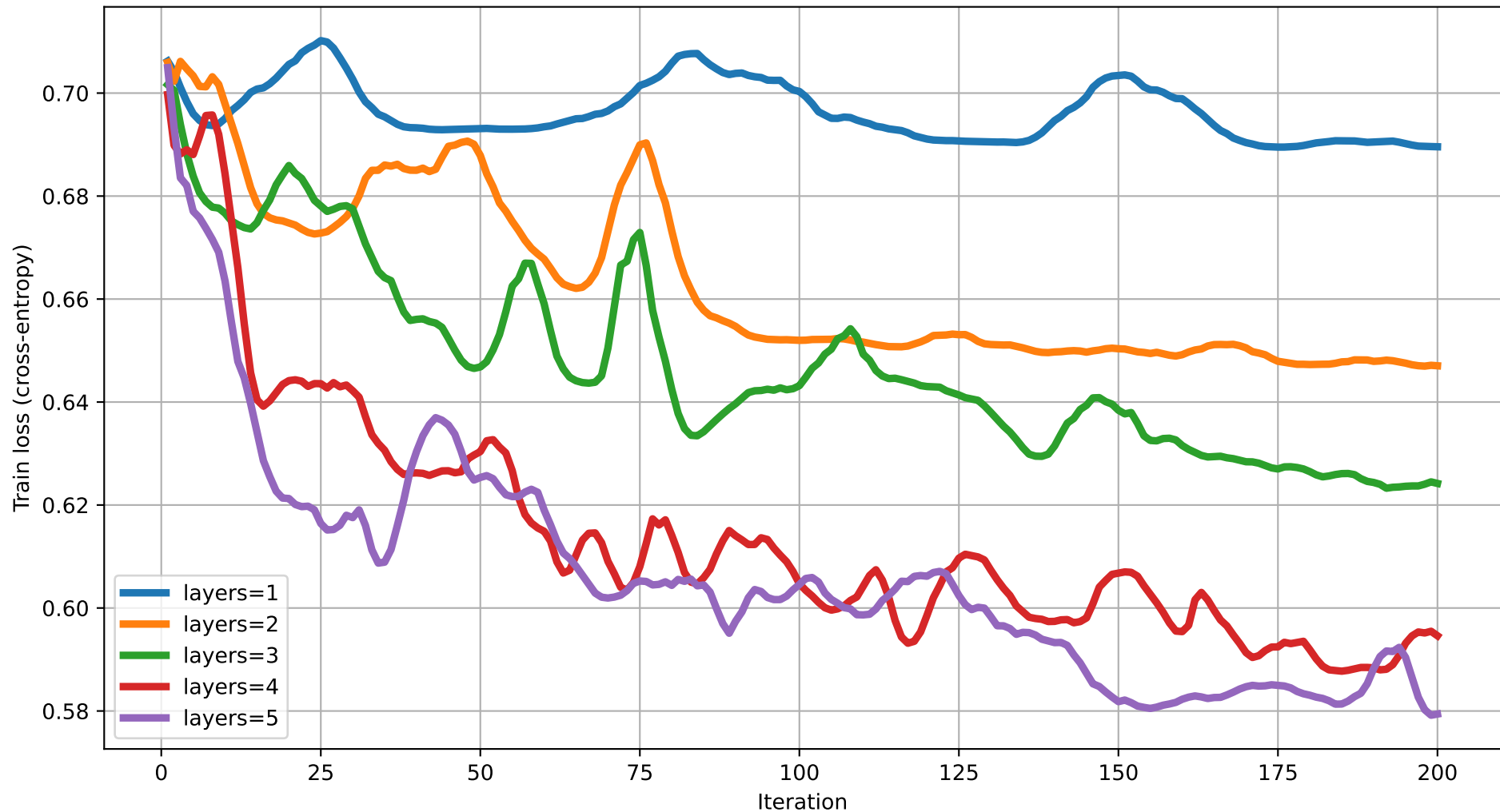
Train loss vs Iteration (dim=11) rot=Rot, ent=chain, gate=CNOT
