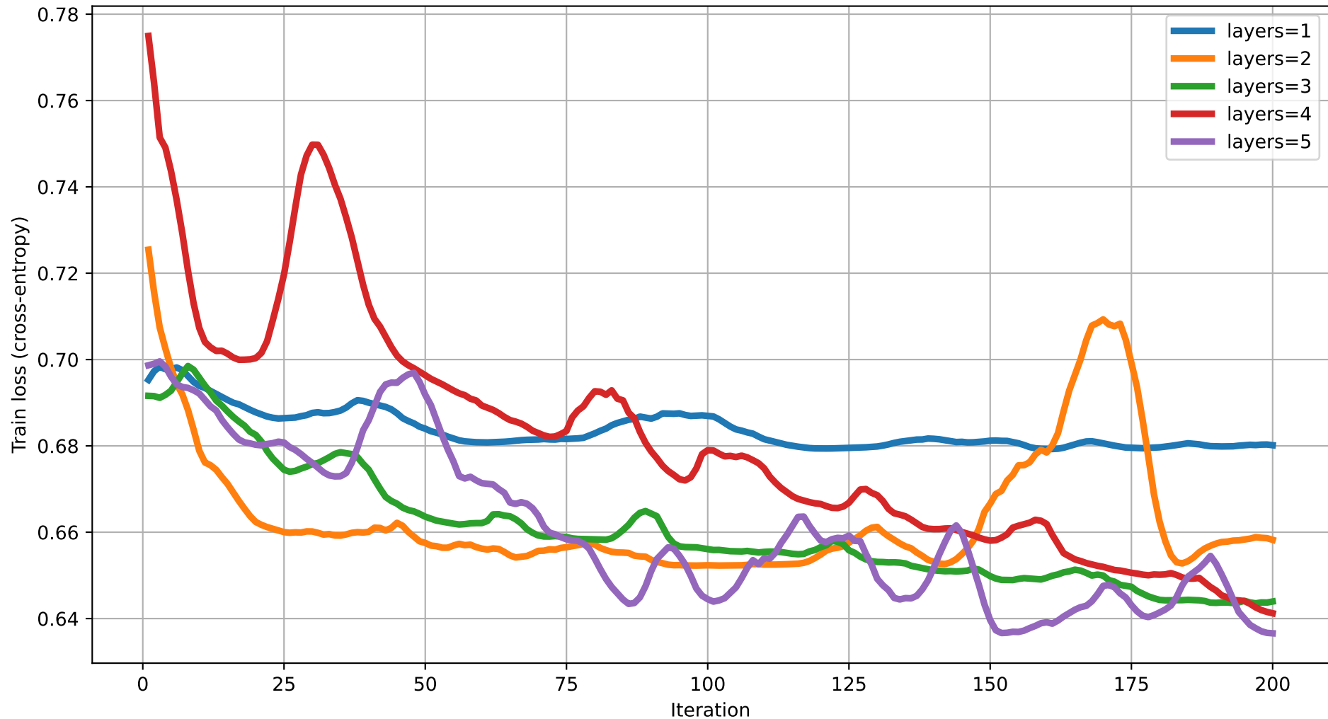
Train loss vs Iteration (dim=9) rot=RZ, ent=chain, gate=IsingXX
