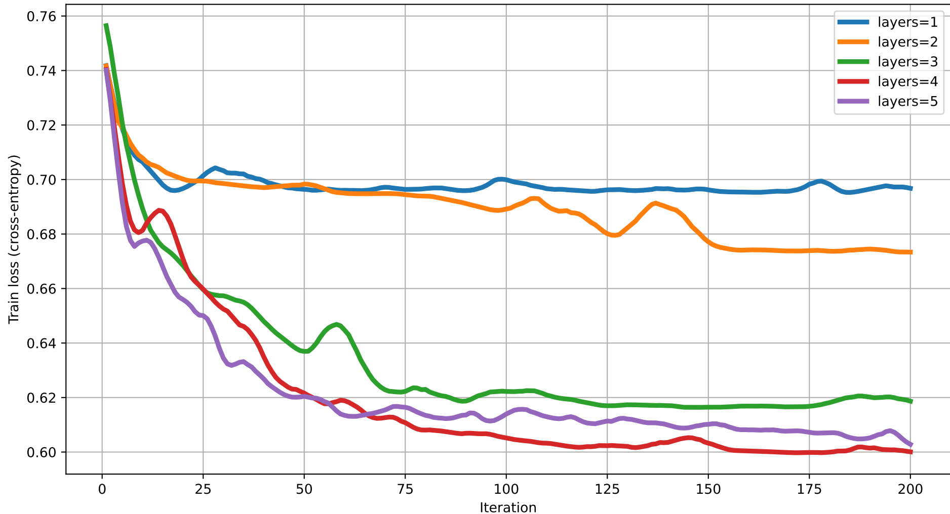
Train loss vs Iteration (degree=5) rot=RX, ent=ring, gate=CZ
