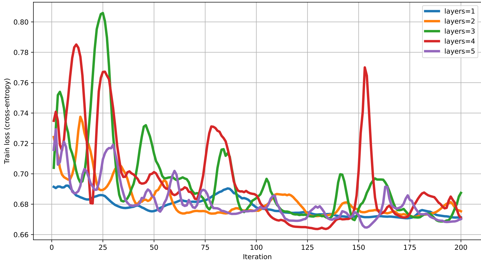
Train loss vs Iteration (dim=12) rot=Rot, ent=pairwise, gate=IsingXX
