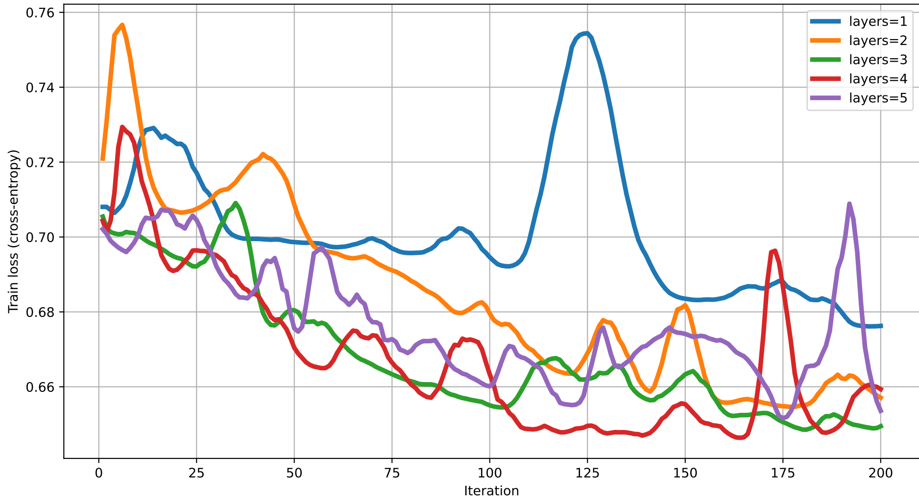
Train loss vs Iteration (dim=6) rot=RYZ, ent=chain, gate=CNOT
