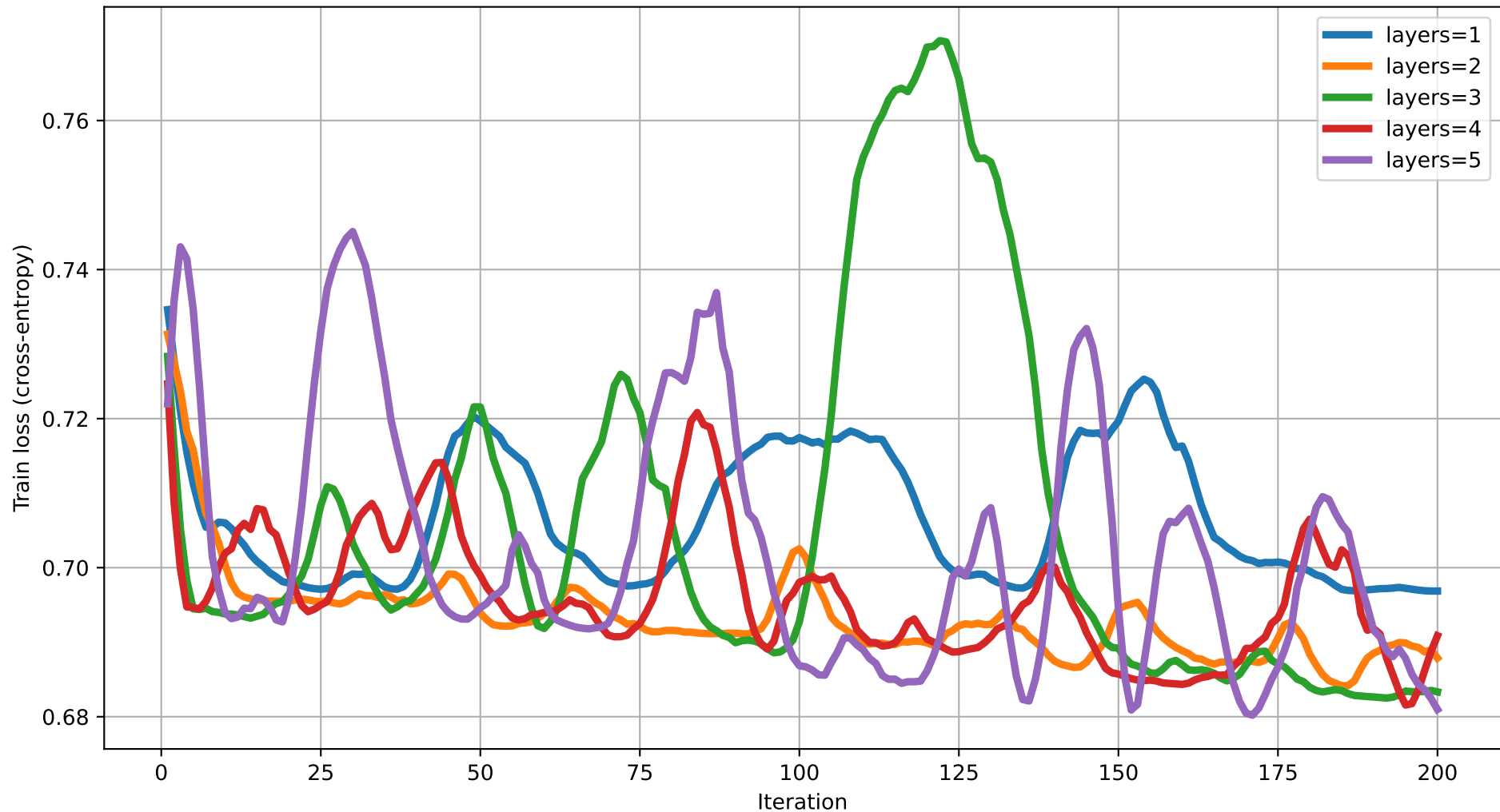
Train loss vs Iteration (dim=18) rot=RY, ent=pairwise, gate=CNOT
