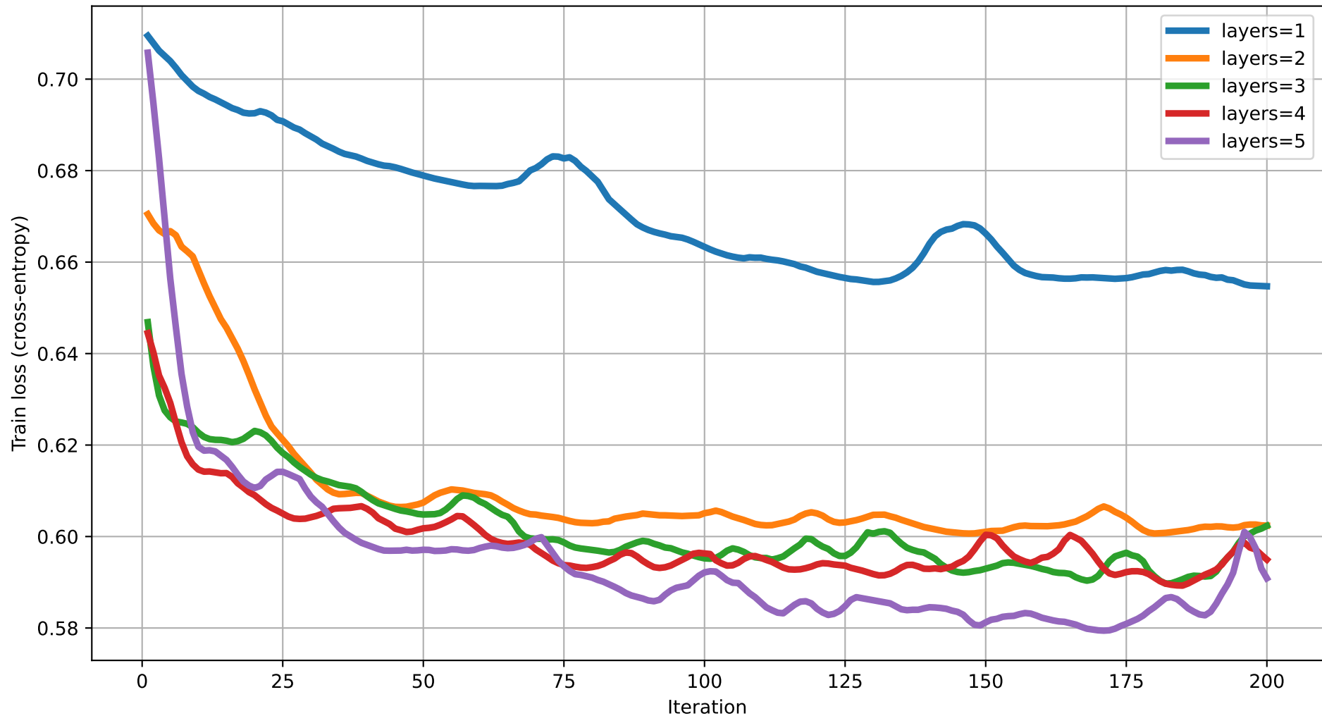
Train loss vs Iteration (degree=5) rot=RYZ, ent=ring, gate=CNOT
