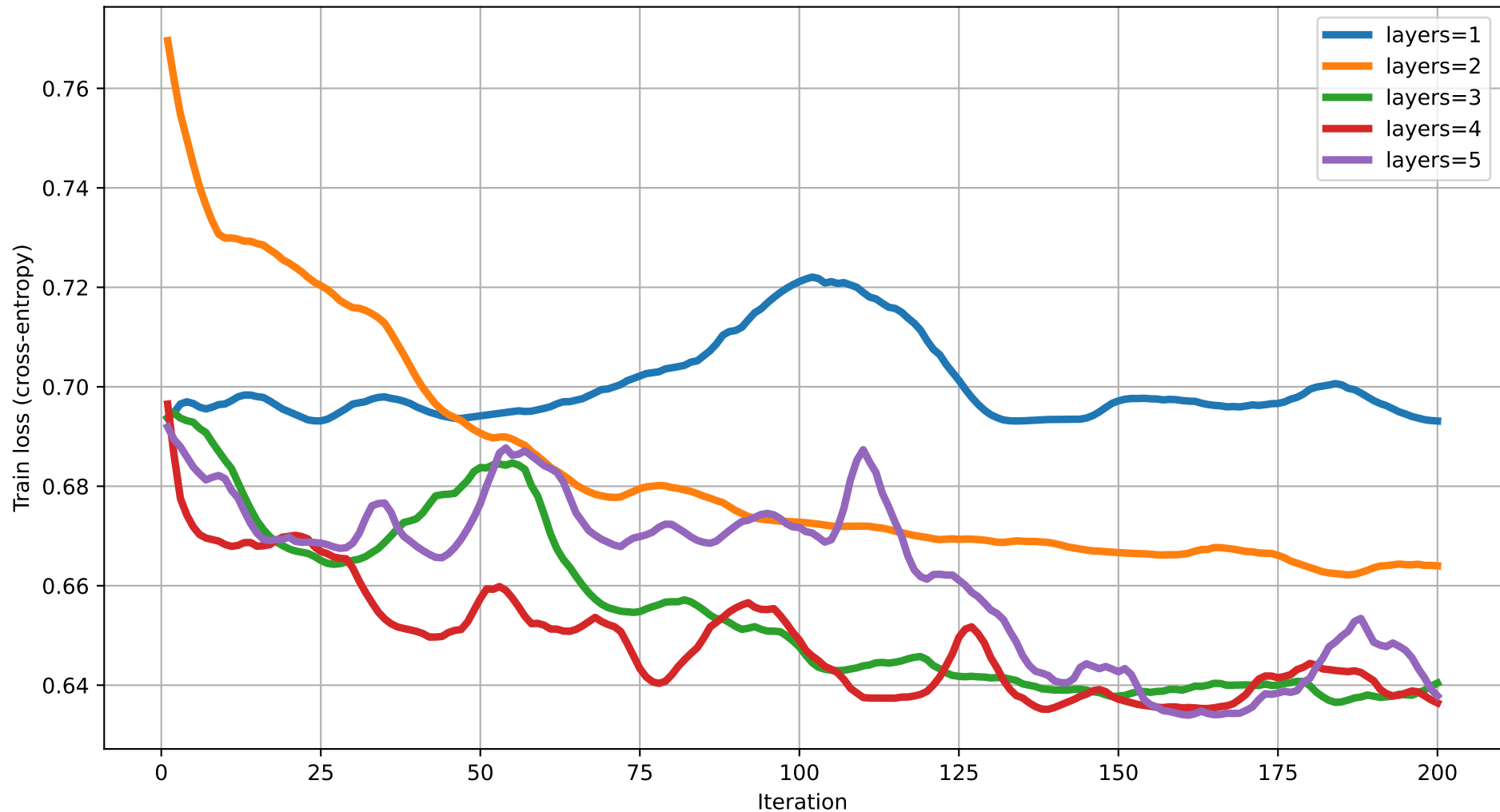
Train loss vs Iteration (dim=10) rot=RY, ent=full, gate=IsingXX
