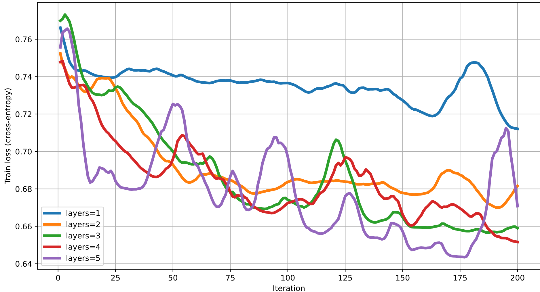
Train loss vs Iteration (dim=5) rot=RYZ, ent=ring, gate=CZ
