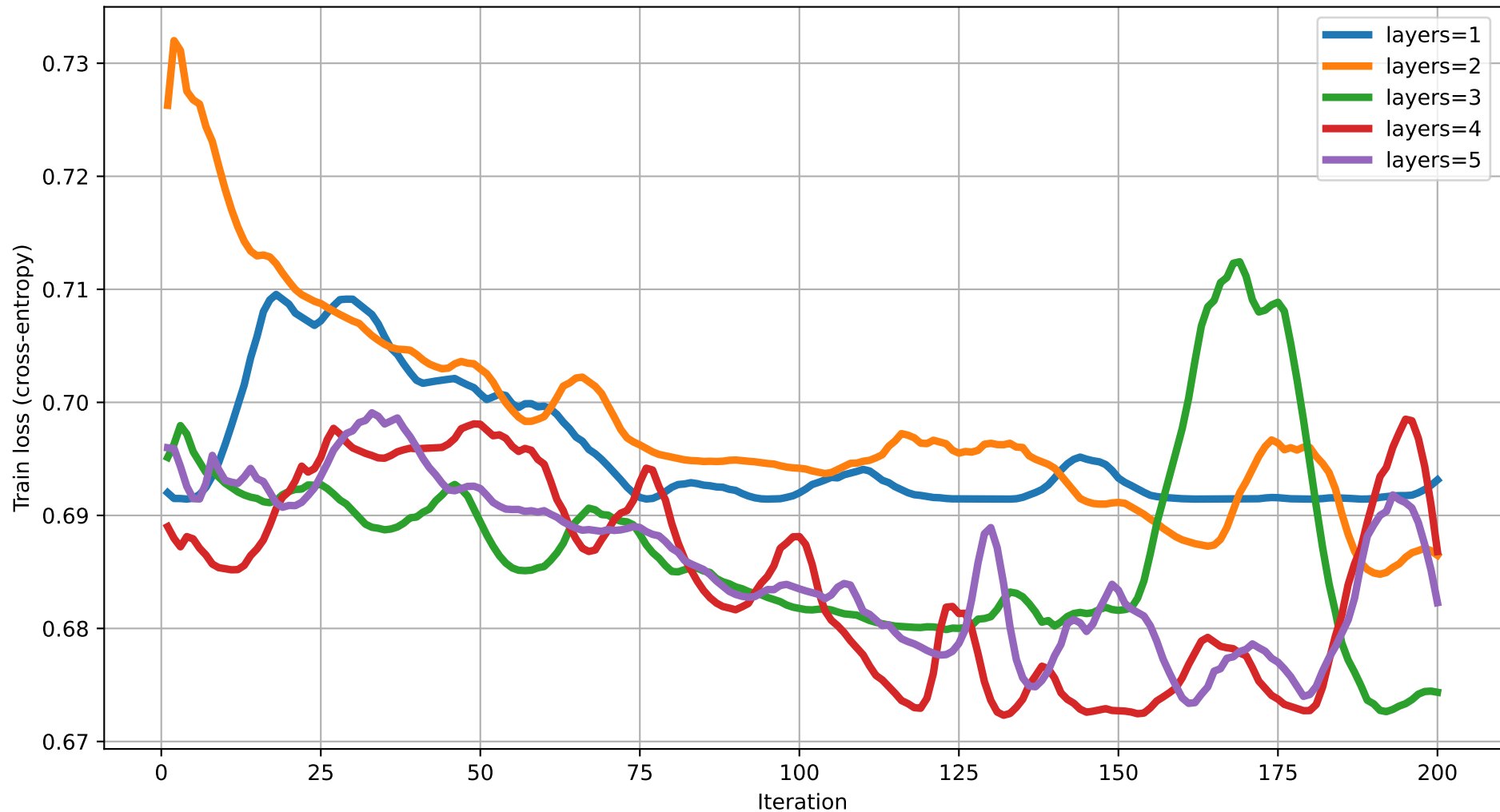
Train loss vs Iteration (dim=15) rot=RY, ent=chain, gate=IsingXX
