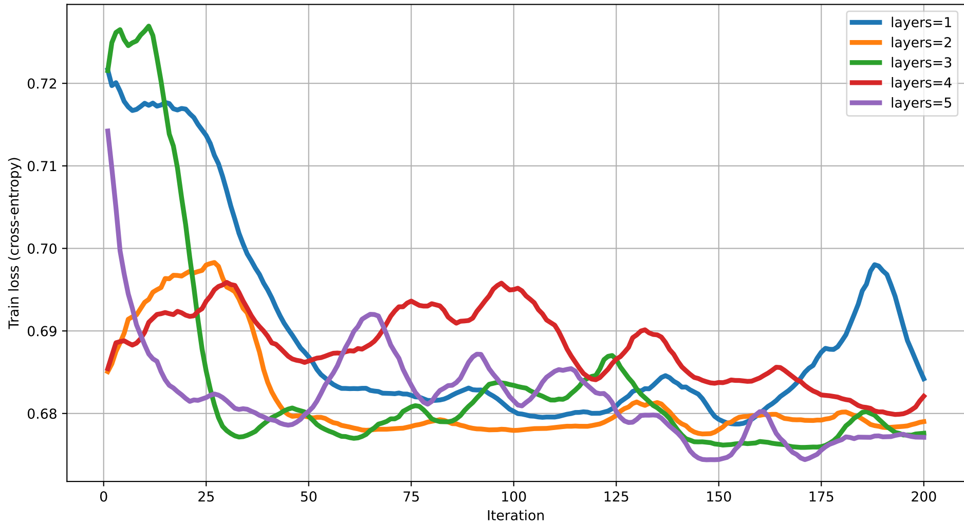
Train loss vs Iteration (dim=15) rot=RZ, ent=ring, gate=IsingXX
