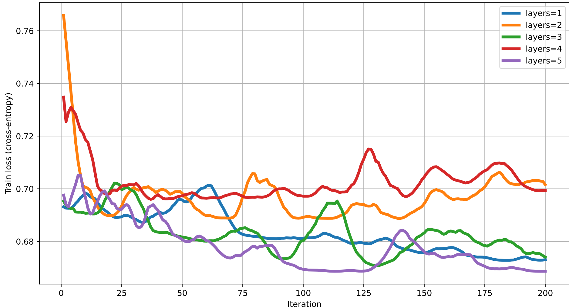
Train loss vs Iteration (dim=18) rot=RX, ent=chain, gate=IsingXX
