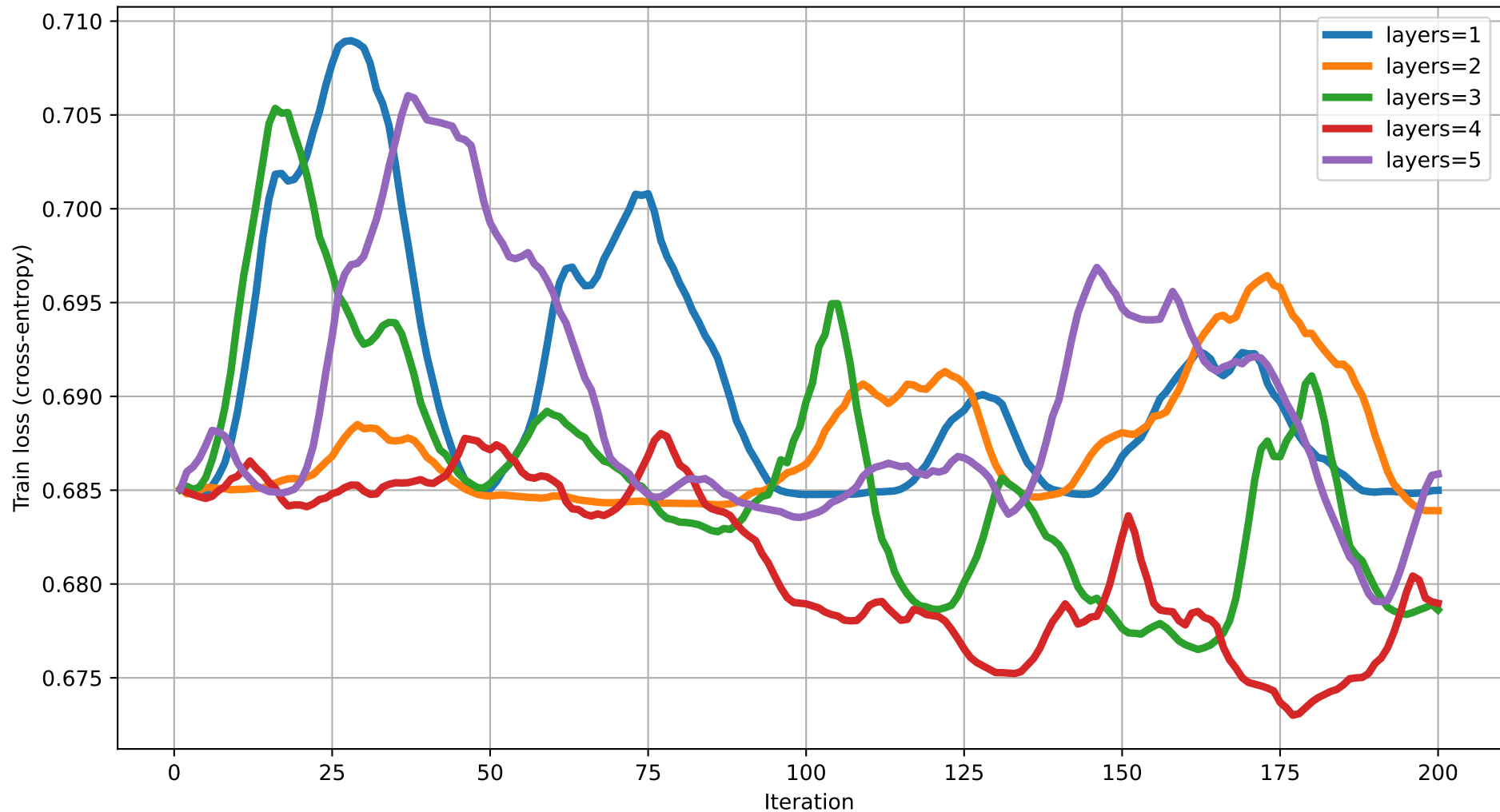
Train loss vs Iteration (dim=15) rot=RX, ent=full, gate=CZ
