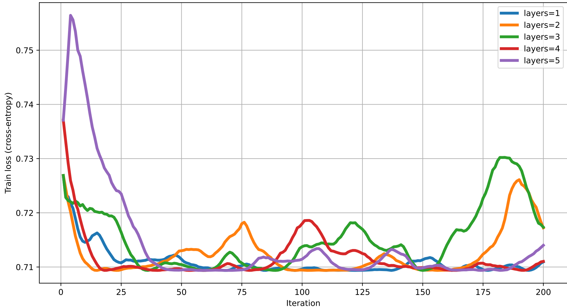
Train loss vs Iteration (dim=5) rot=RZ, ent=full, gate=CNOT
