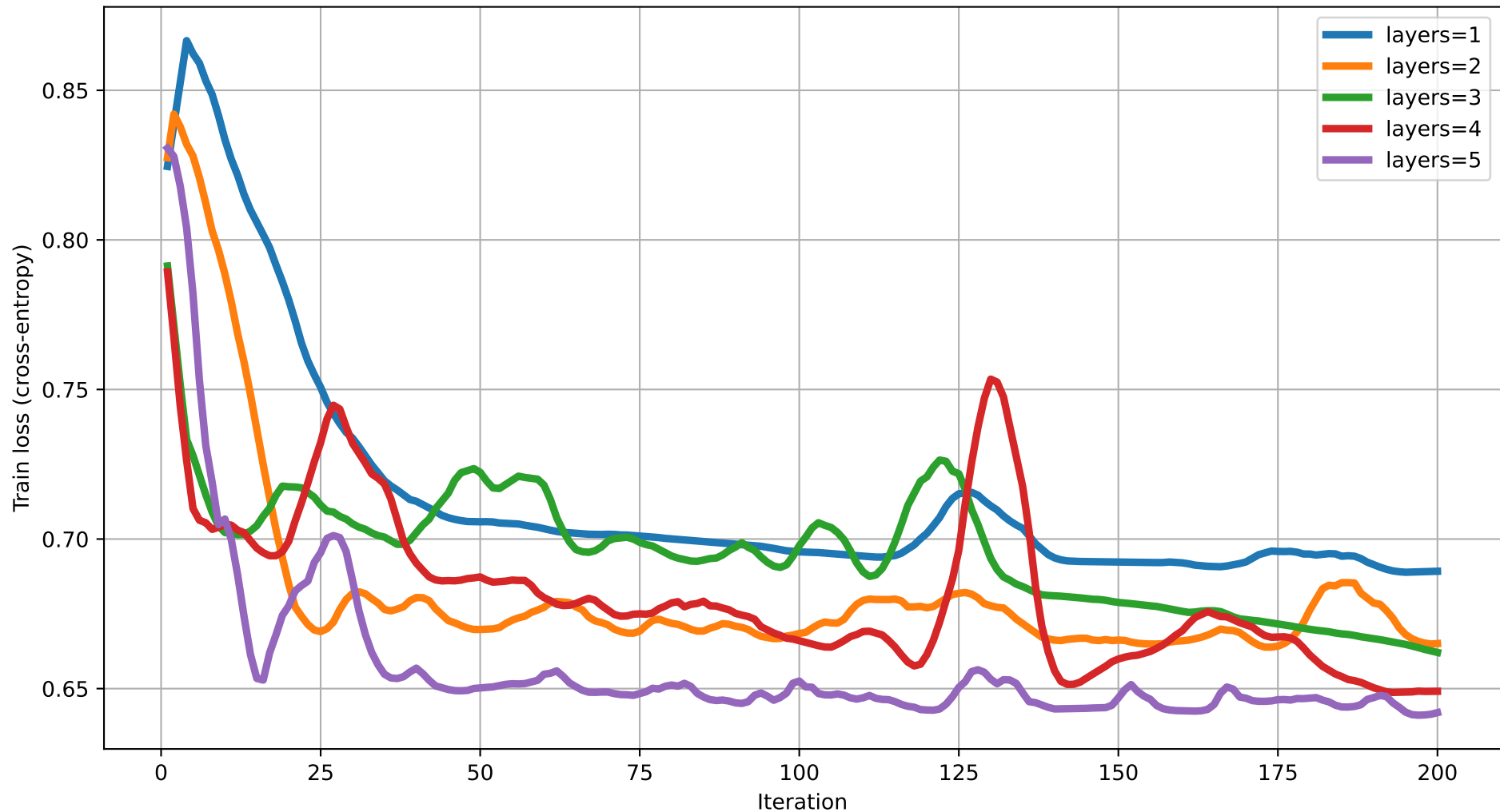
Train loss vs Iteration (dim=8) rot=RY, ent=chain, gate=CNOT
