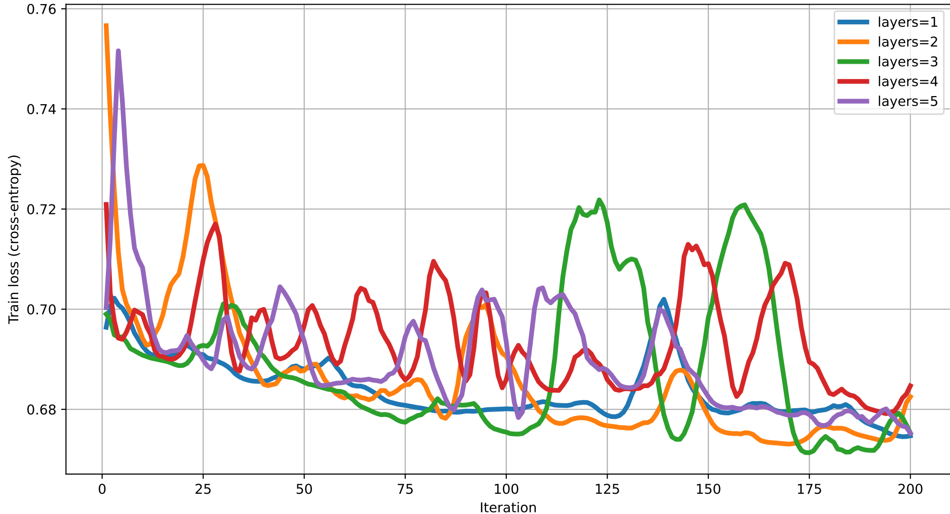
Train loss vs Iteration (dim=18) rot=RYZ, ent=pairwise, gate=IsingXX
