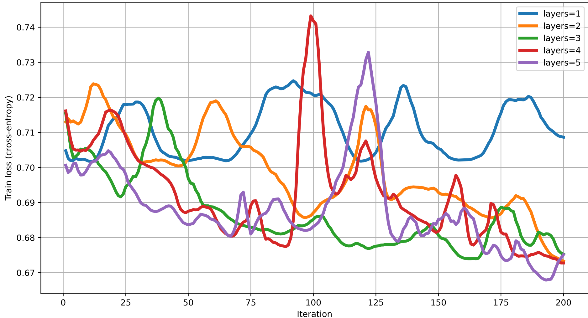
Train loss vs Iteration (dim=12) rot=Rot, ent=ring, gate=CZ
