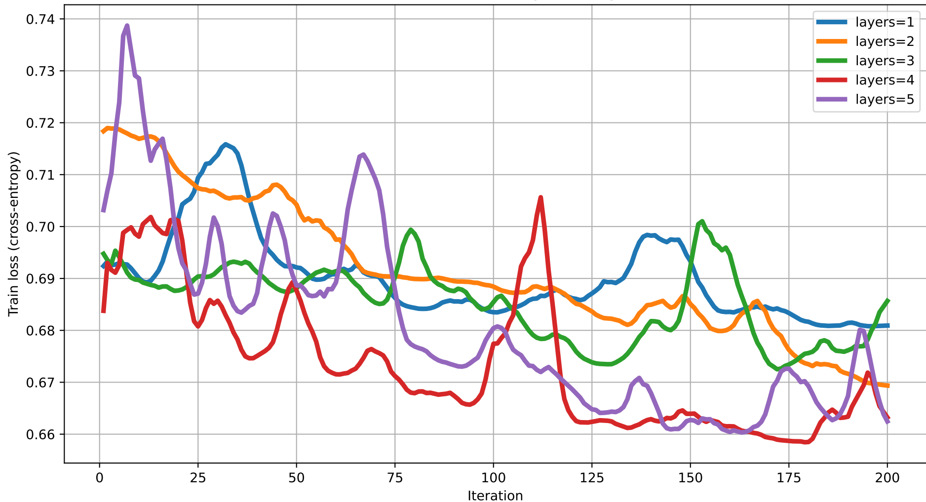
Train loss vs Iteration (dim=15) rot=RYZ, ent=chain, gate=IsingXX
