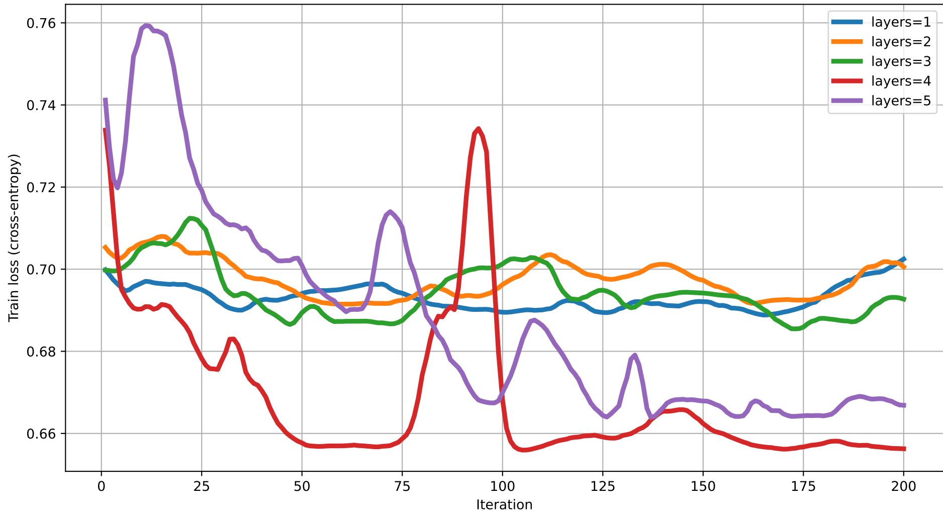
Train loss vs Iteration (dim=6) rot=RX, ent=ring, gate=CNOT
