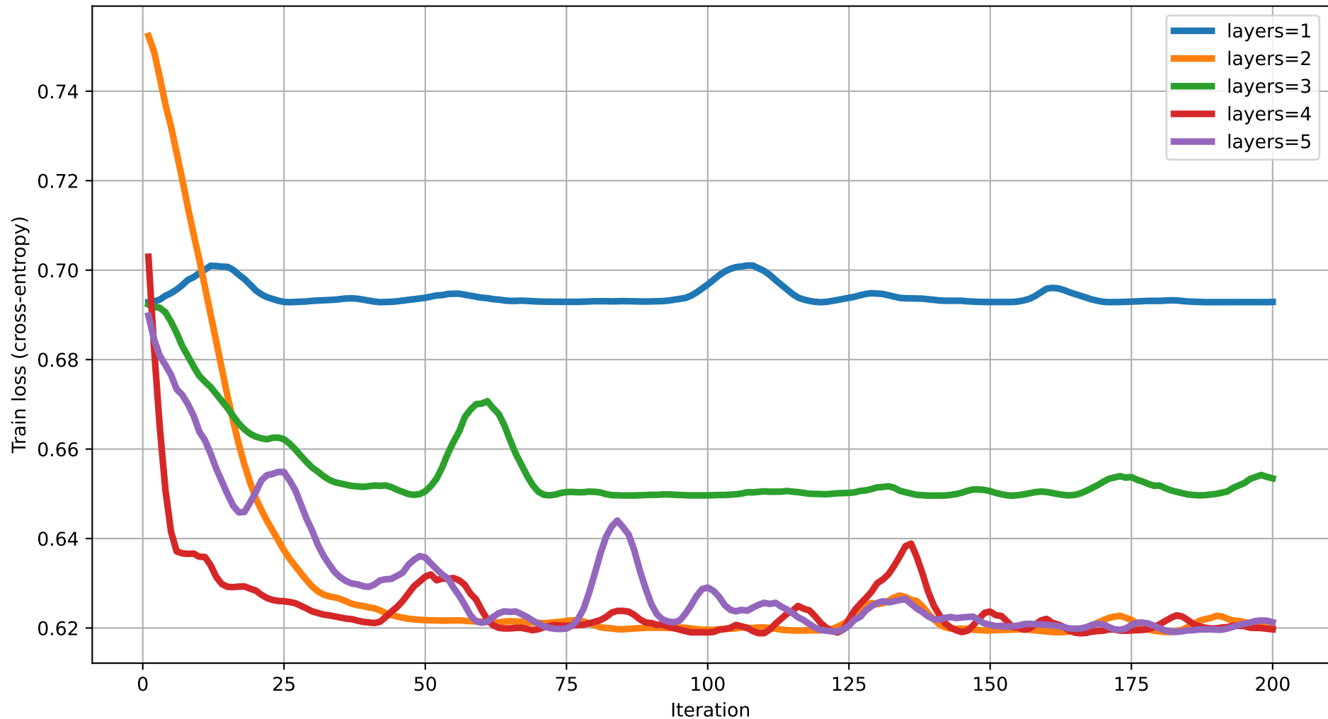
Train loss vs Iteration (degree=4) rot=RY, ent=chain, gate=IsingXX
