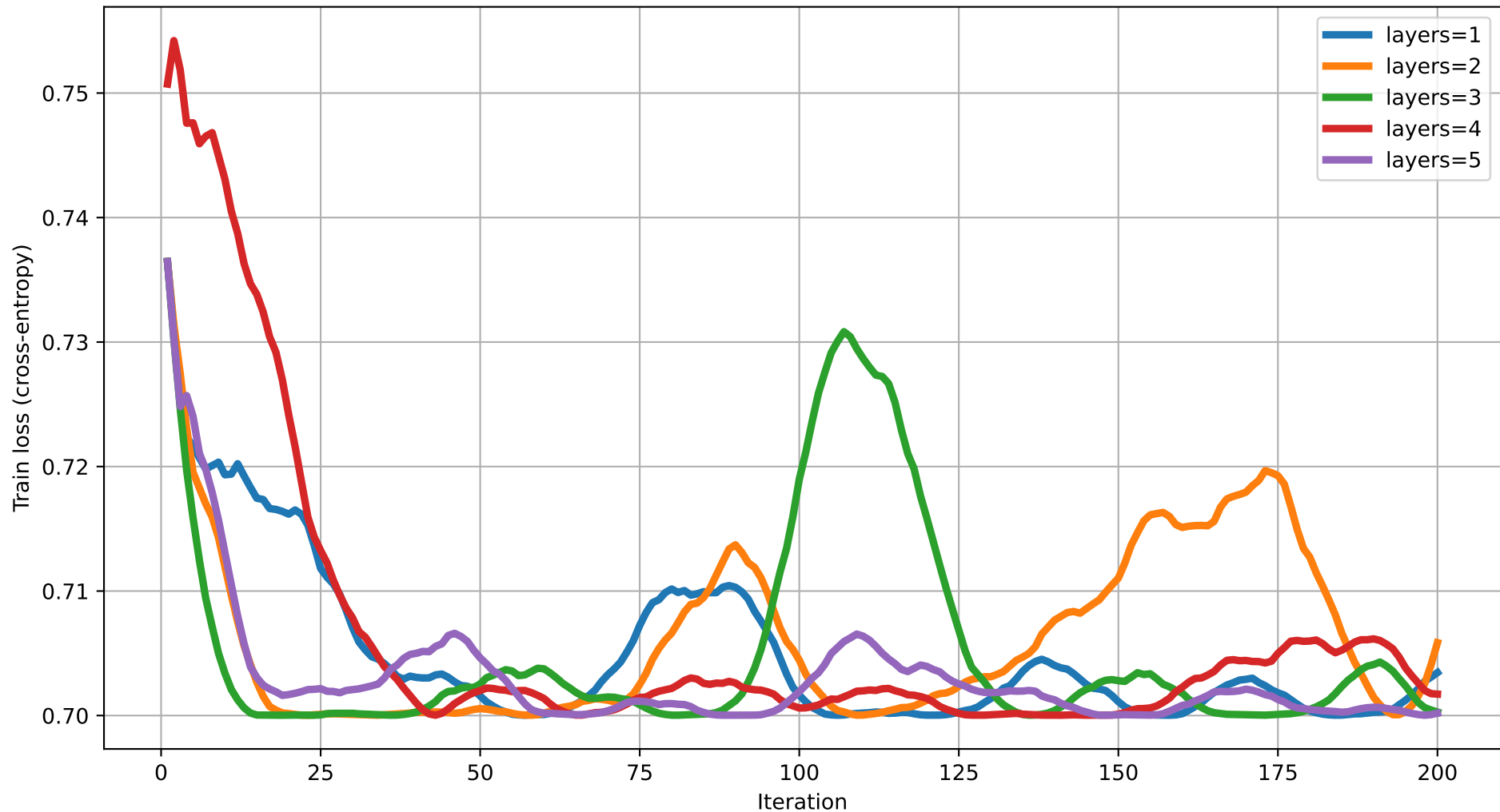
Train loss vs Iteration (dim=19) rot=RZ, ent=pairwise, gate=CZ
