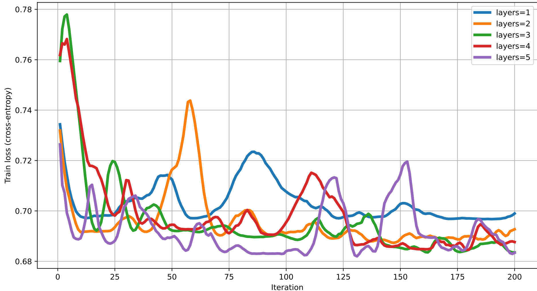
Train loss vs Iteration (dim=18) rot=RYZ, ent=pairwise, gate=CZ
