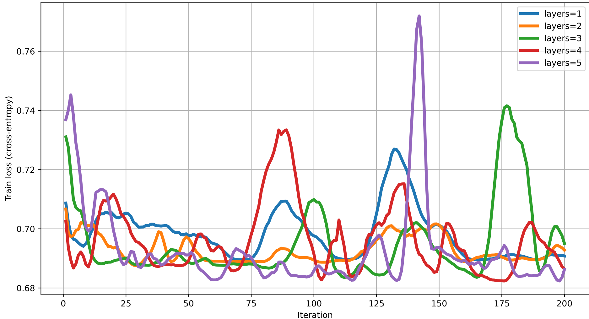
Train loss vs Iteration (dim=20) rot=Rot, ent=pairwise, gate=CNOT
