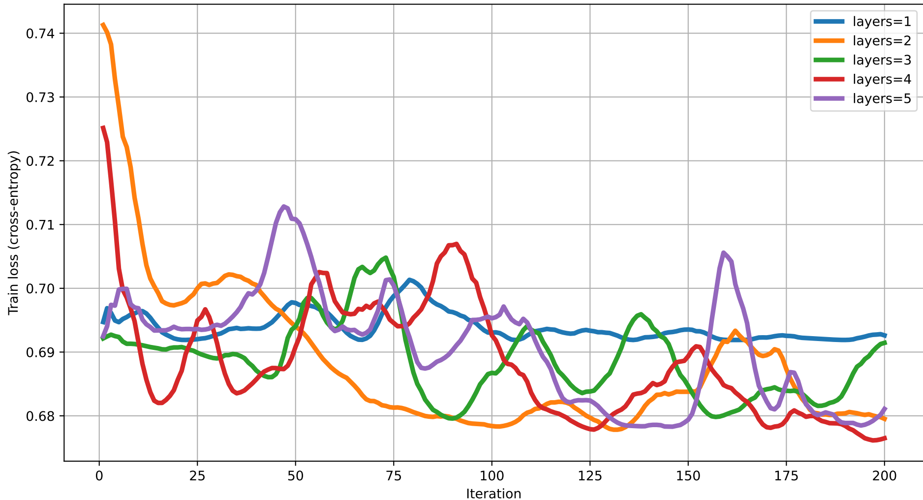
Train loss vs Iteration (dim=11) rot=RY, ent=full, gate=IsingXX
