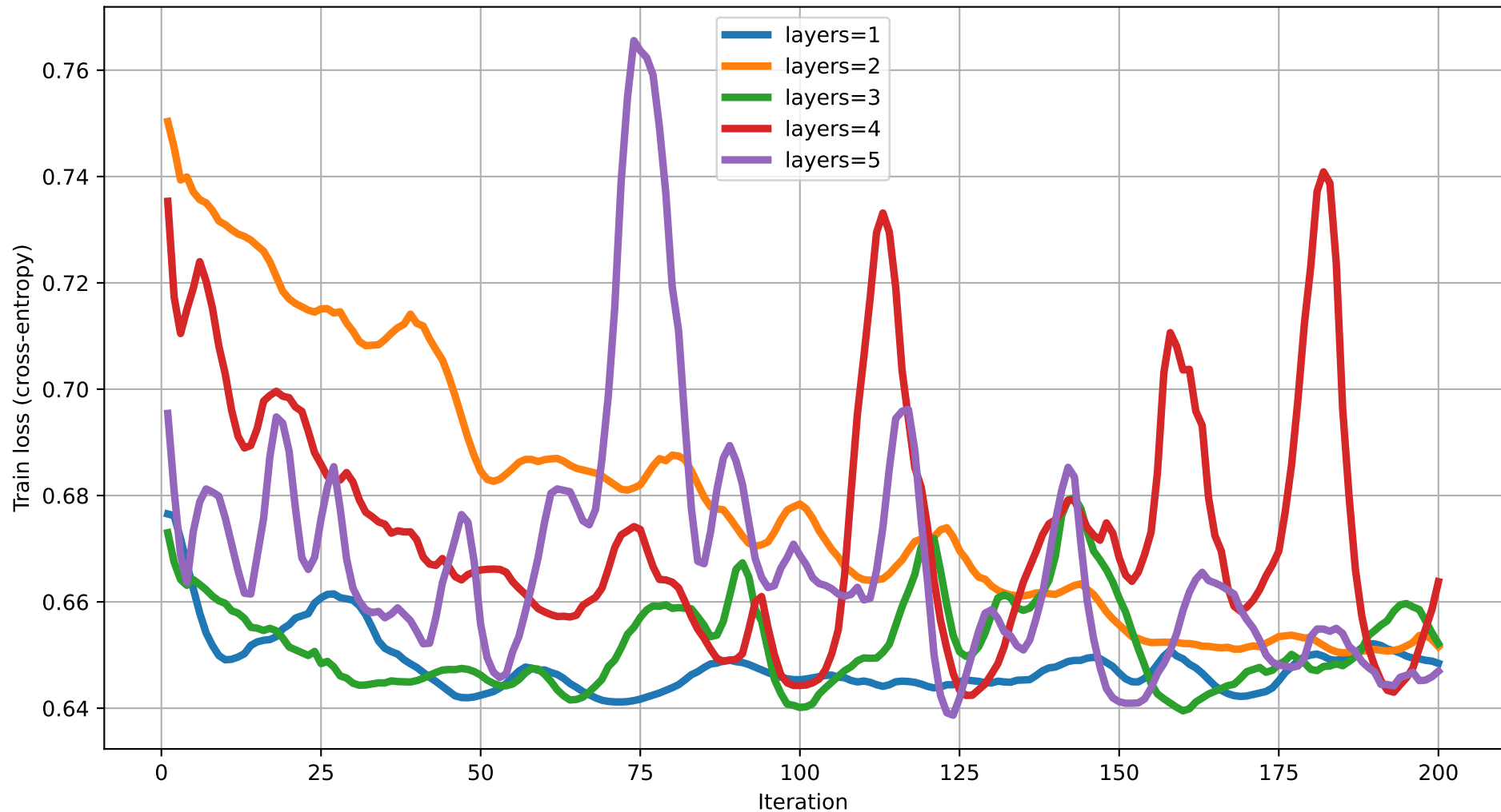
Train loss vs Iteration (dim=5) rot=Rot, ent=ring, gate=IsingXX
