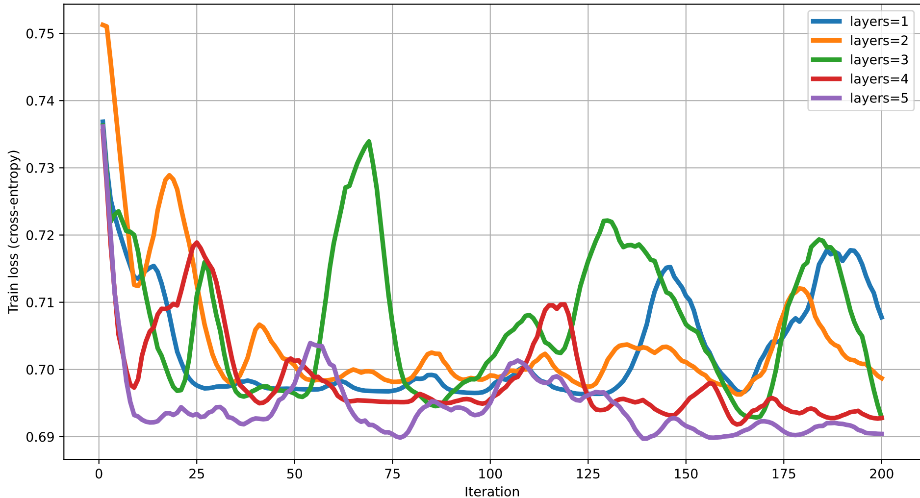
Train loss vs Iteration (dim=18) rot=RX, ent=chain, gate=CZ
