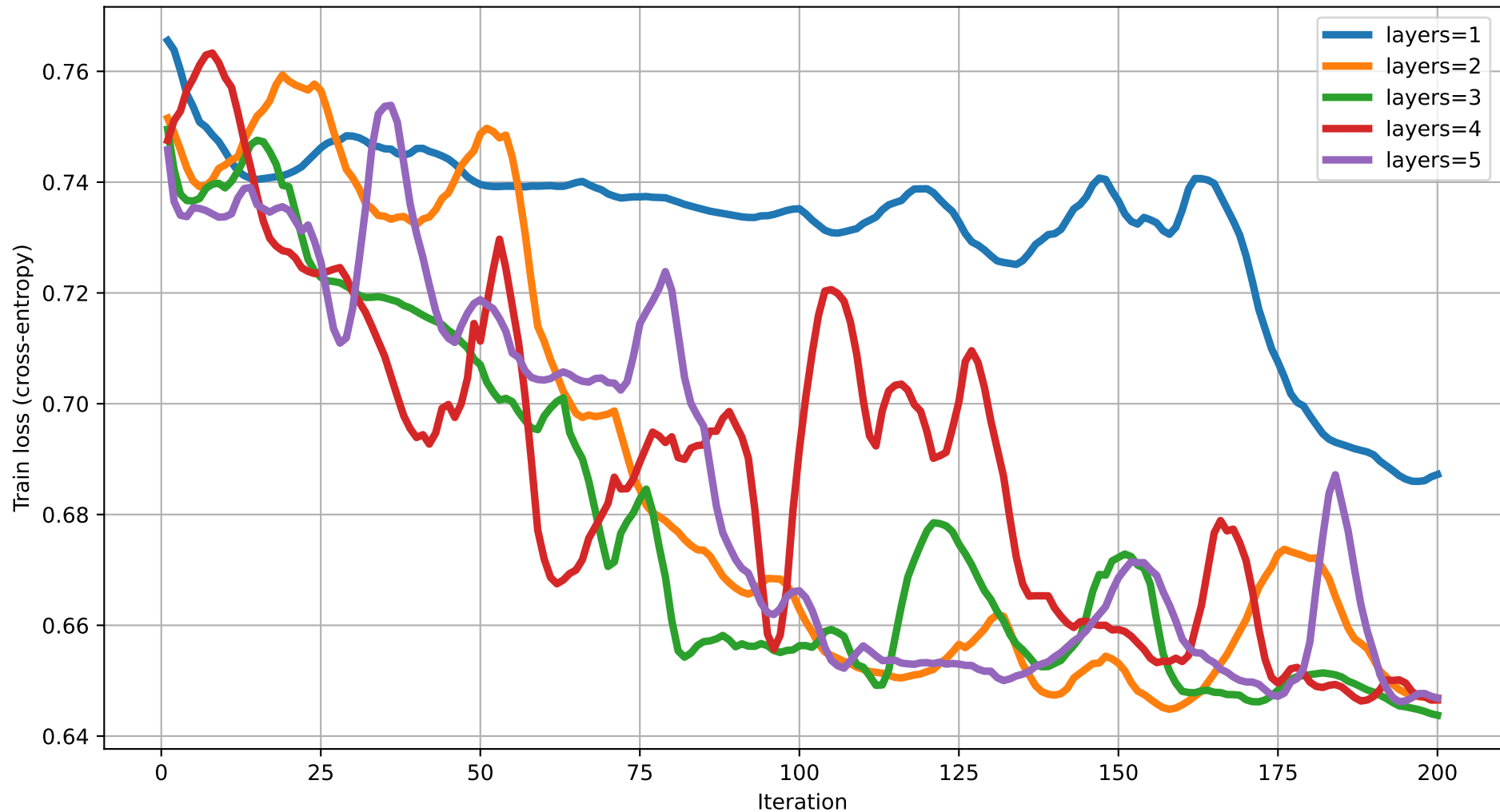
Train loss vs Iteration (dim=5) rot=Rot, ent=pairwise, gate=CNOT
