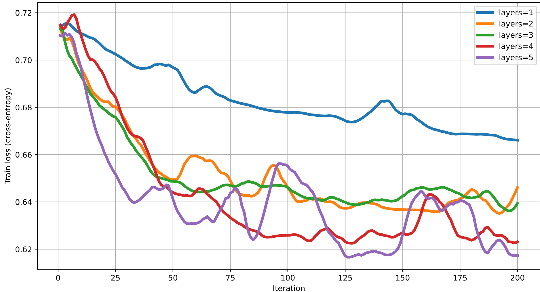
Train loss vs Iteration (dim=7) rot=RY, ent=chain, gate=CNOT
