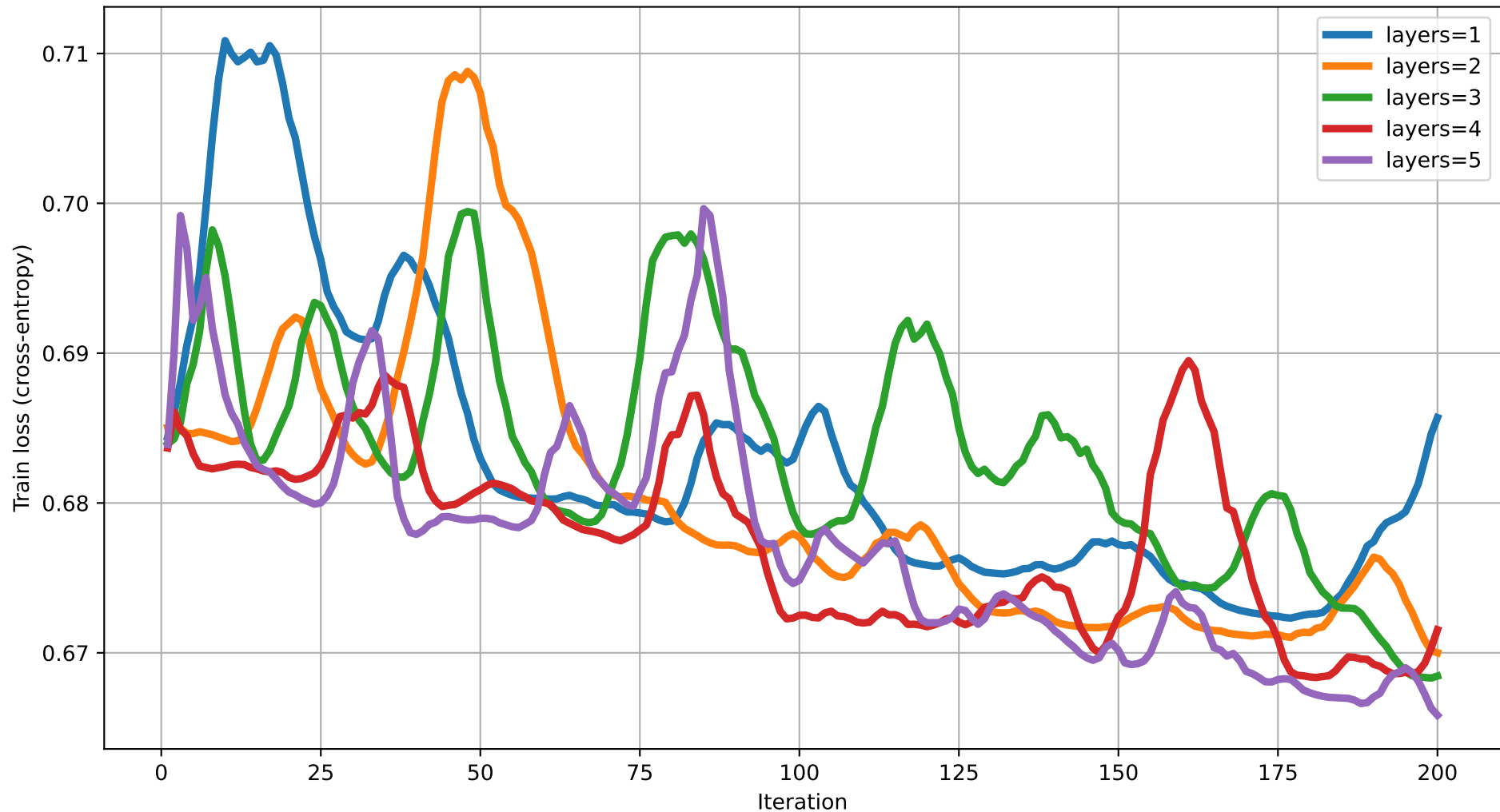
Train loss vs Iteration (dim=15) rot=Rot, ent=full, gate=CZ
