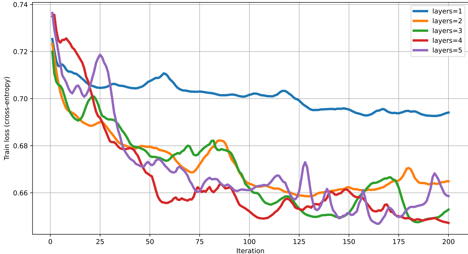
Train loss vs Iteration (dim=5) rot=Rot, ent=pairwise, gate=CZ
