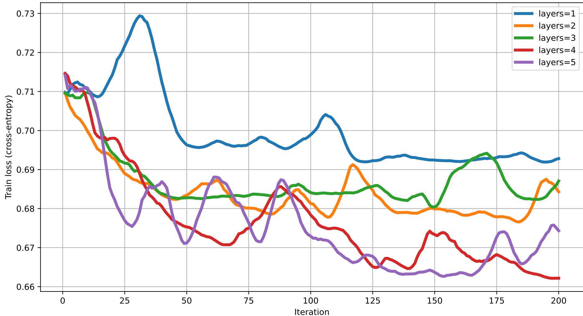
Train loss vs Iteration (dim=6) rot=RX, ent=chain, gate=CZ
