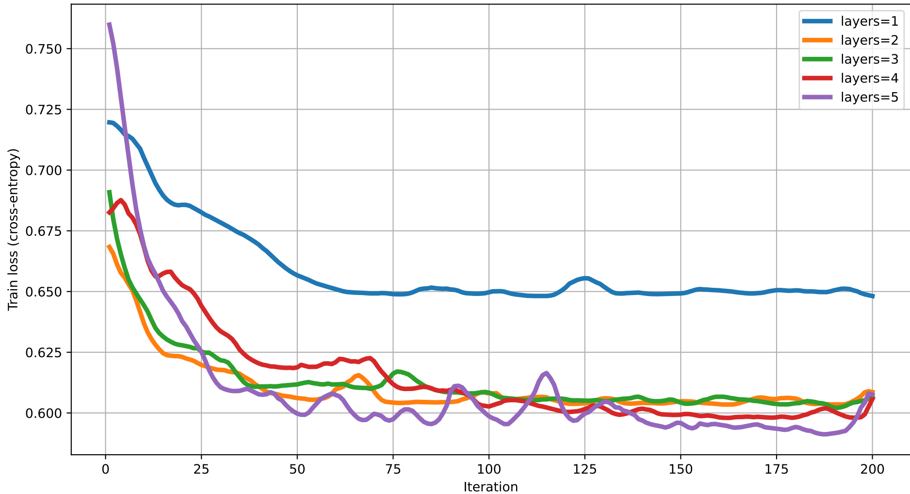
Train loss vs Iteration (degree=2) rot=RY, ent=ring, gate=CNOT
