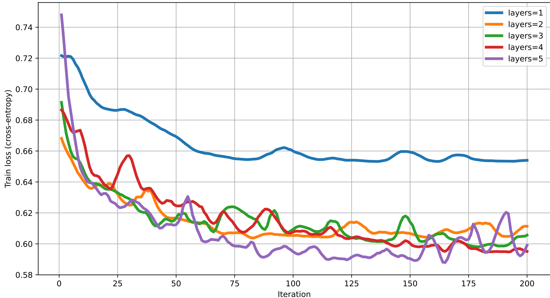
Train loss vs Iteration (degree=2) rot=Rot, ent=ring, gate=CNOT
