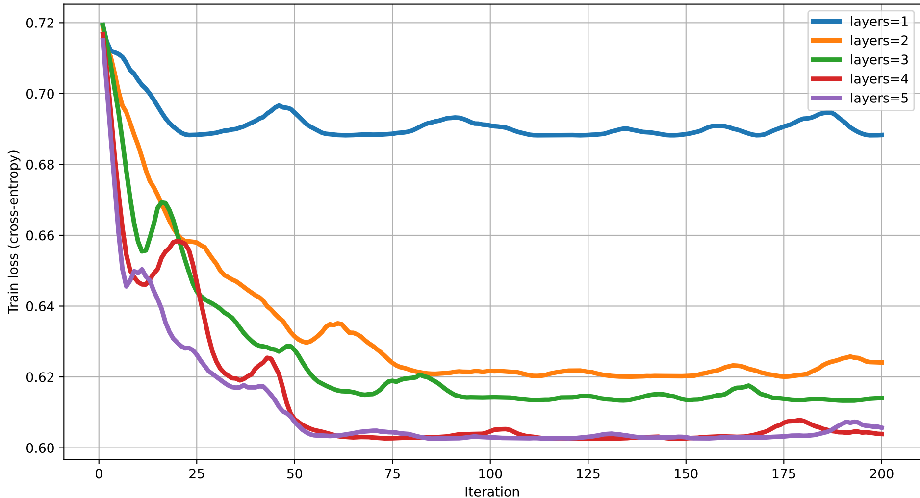
Train loss vs Iteration (degree=4) rot=RX, ent=chain, gate=CNOT
