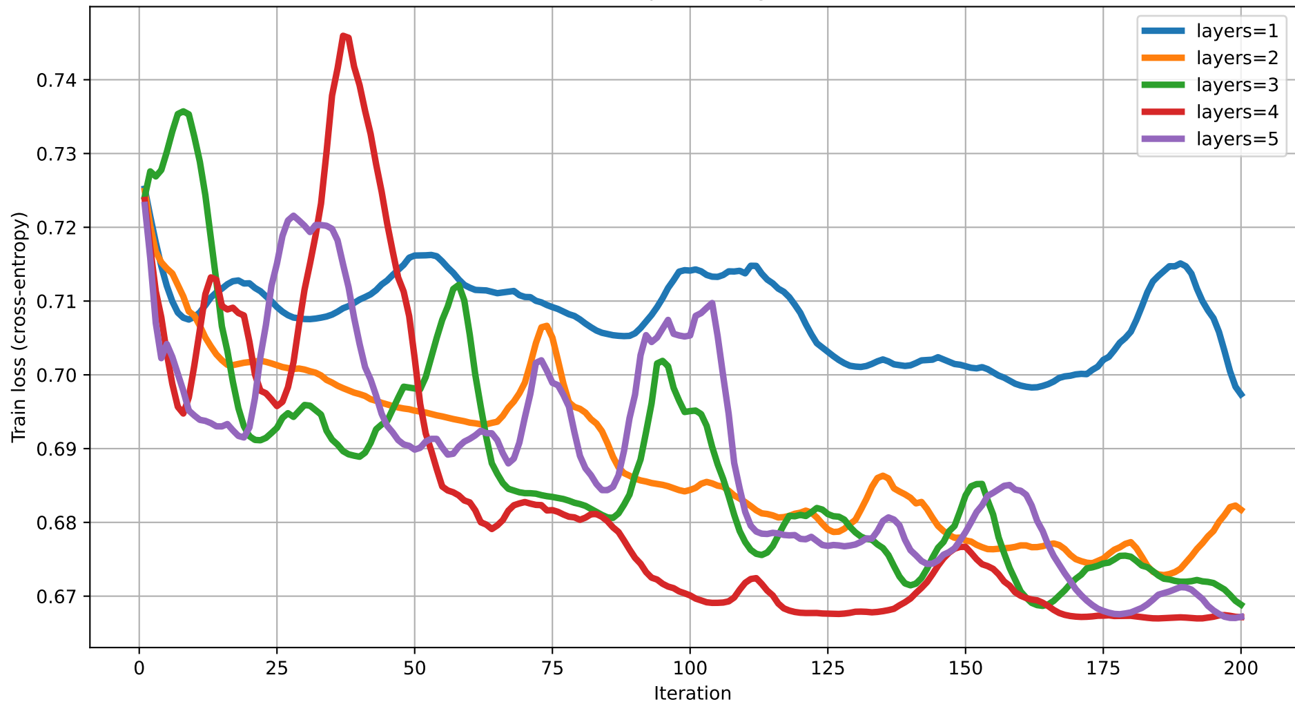
Train loss vs Iteration (dim=10) rot=RX, ent=pairwise, gate=CNOT
