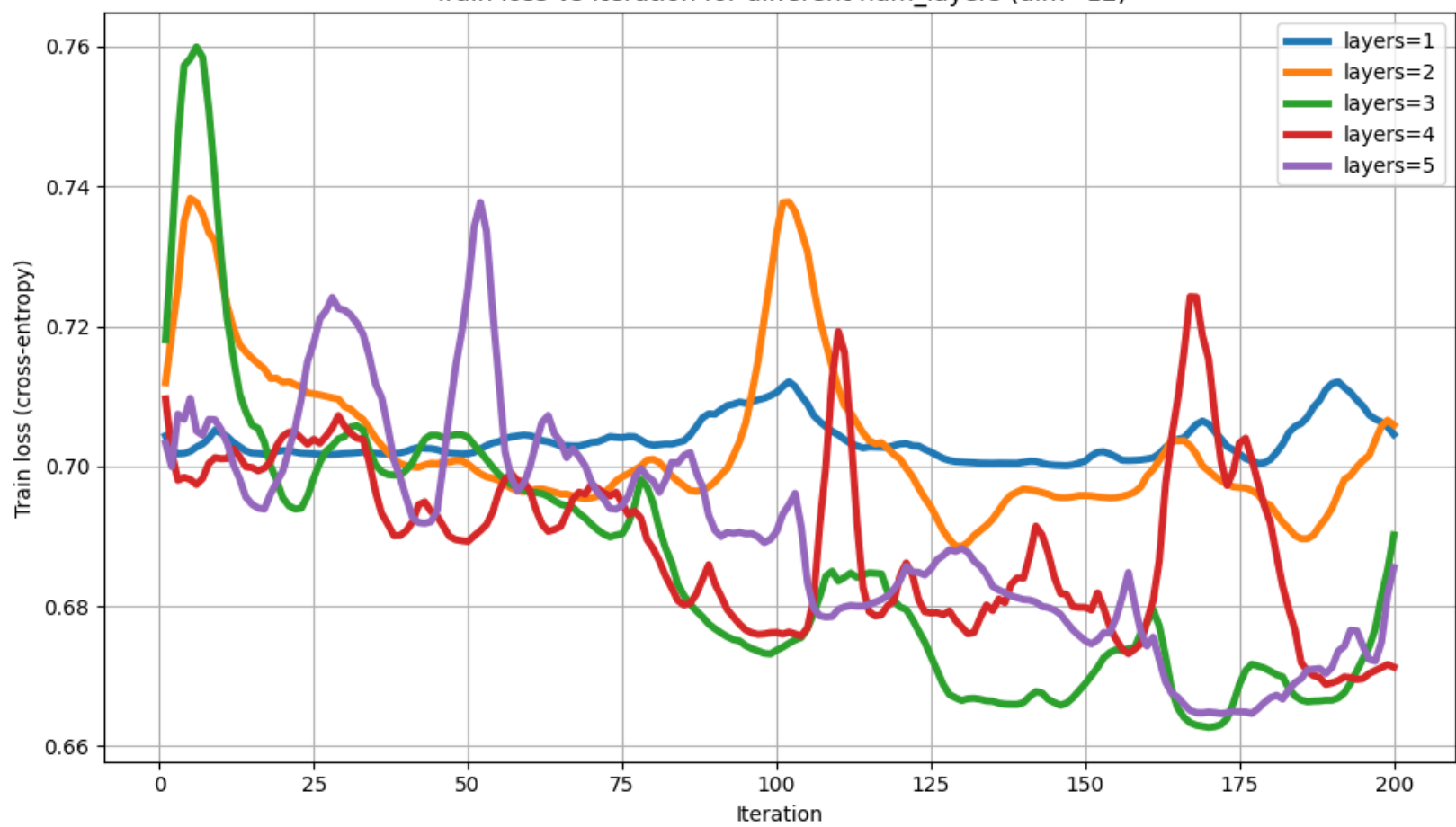
Train loss vs Iteration for different num_layers (dim=12)
