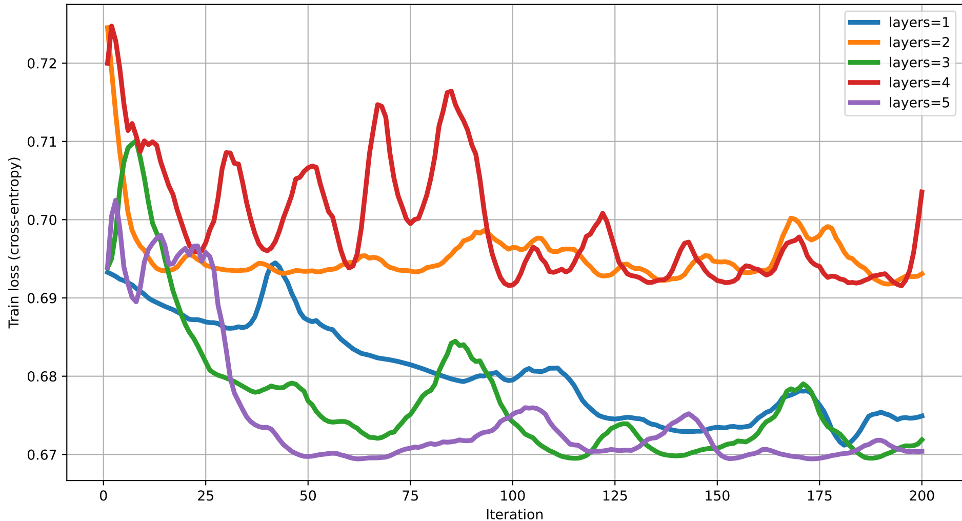
Train loss vs Iteration (dim=11) rot=RX, ent=pairwise, gate=IsingXX
