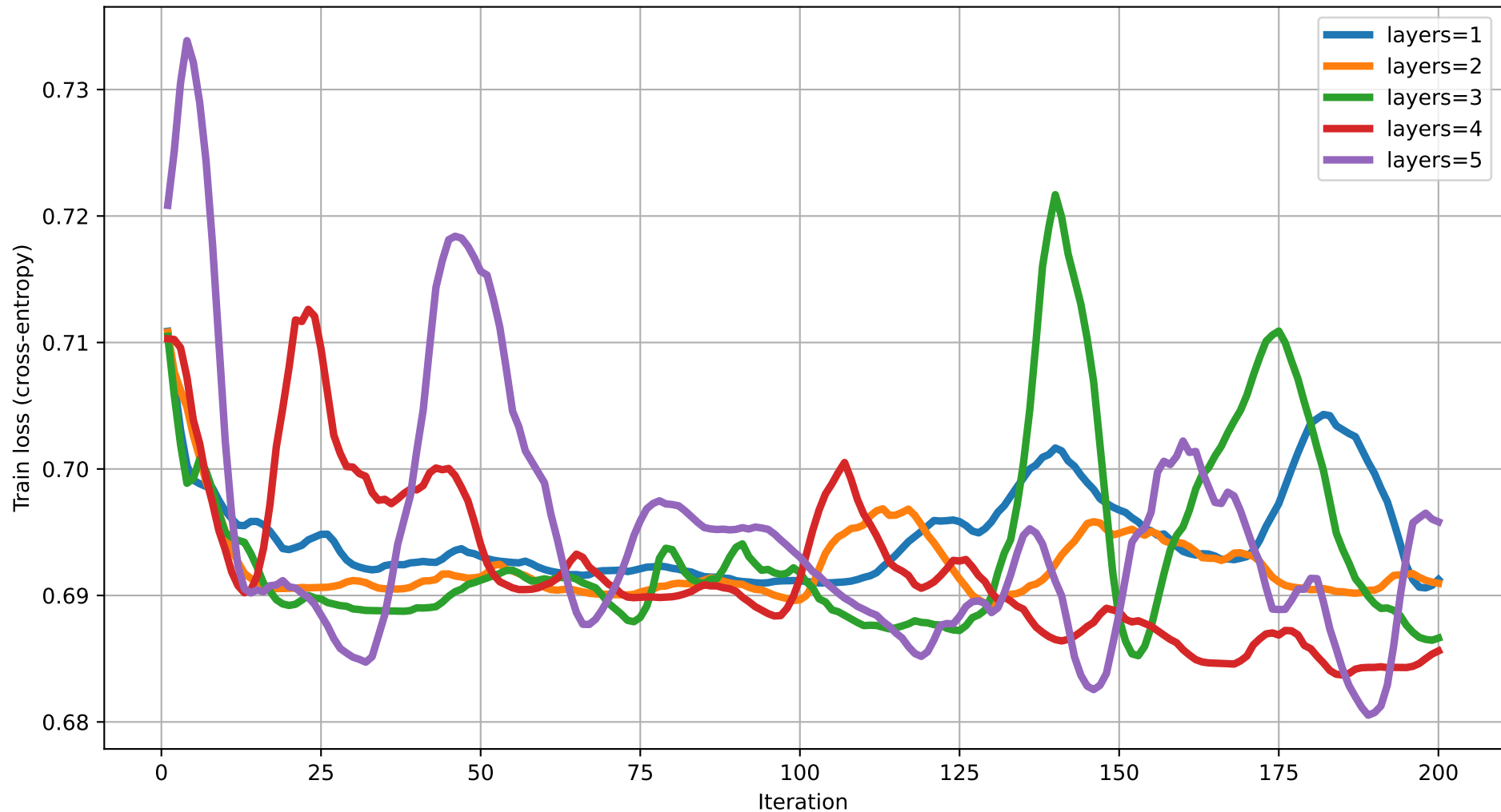
Train loss vs Iteration (dim=20) rot=RX, ent=ring, gate=CZ
