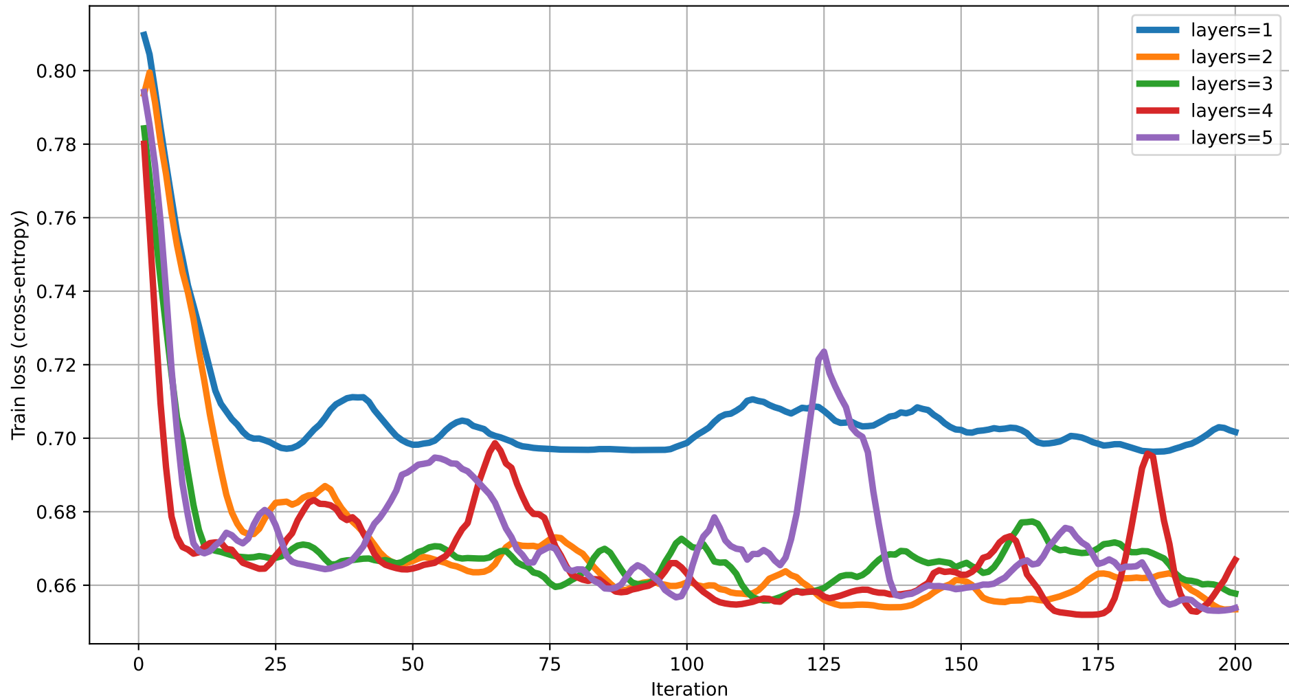
Train loss vs Iteration (dim=2) rot=RY, ent=full, gate=CNOT
