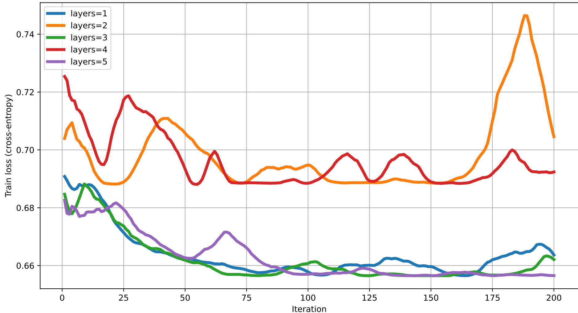
Train loss vs Iteration (dim=6) rot=RX, ent=pairwise, gate=IsingXX
