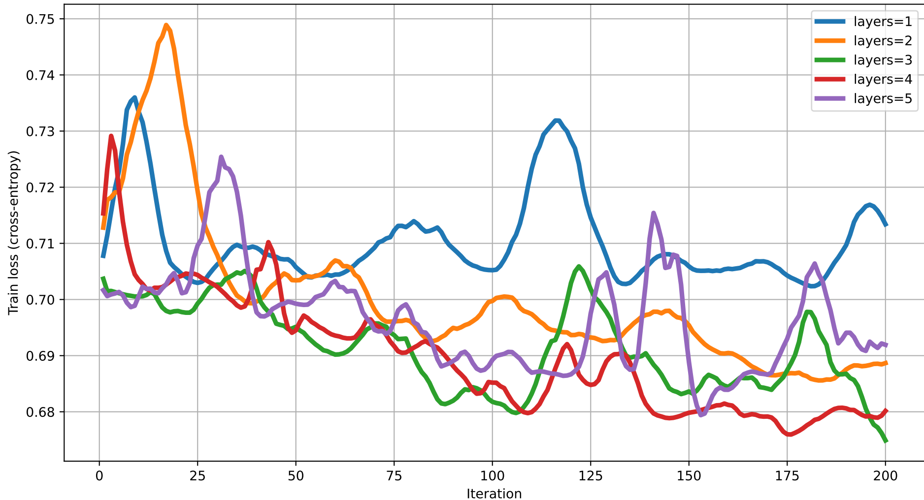
Train loss vs Iteration (dim=12) rot=Rot, ent=full, gate=CZ
