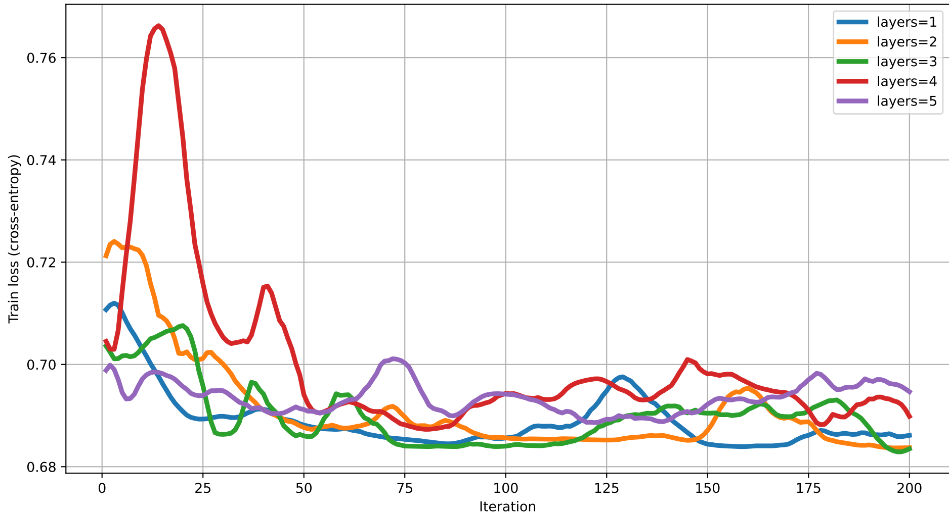
Train loss vs Iteration (dim=14) rot=RX, ent=ring, gate=CNOT
