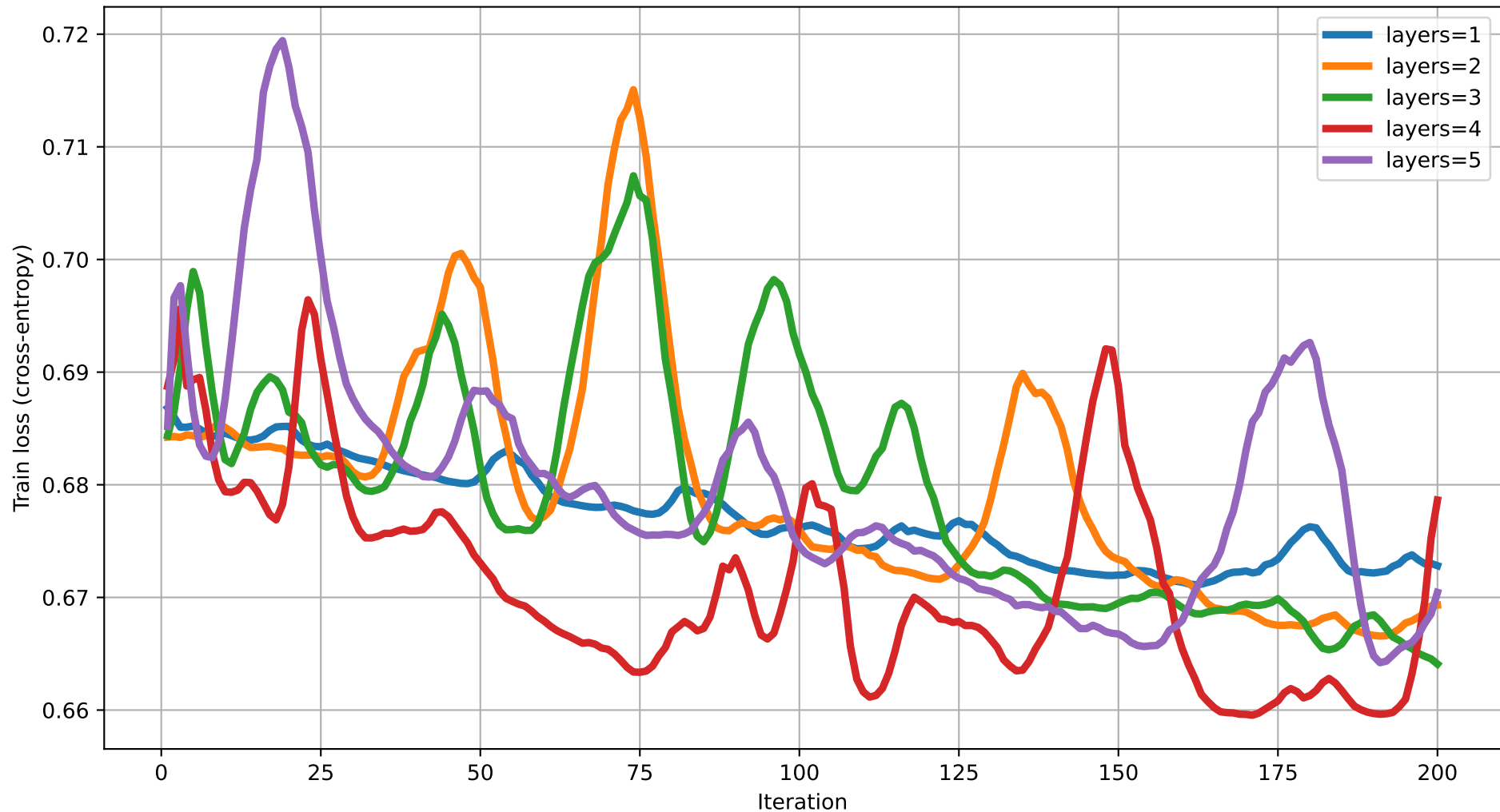
Train loss vs Iteration (dim=15) rot=RY, ent=full, gate=CNOT
