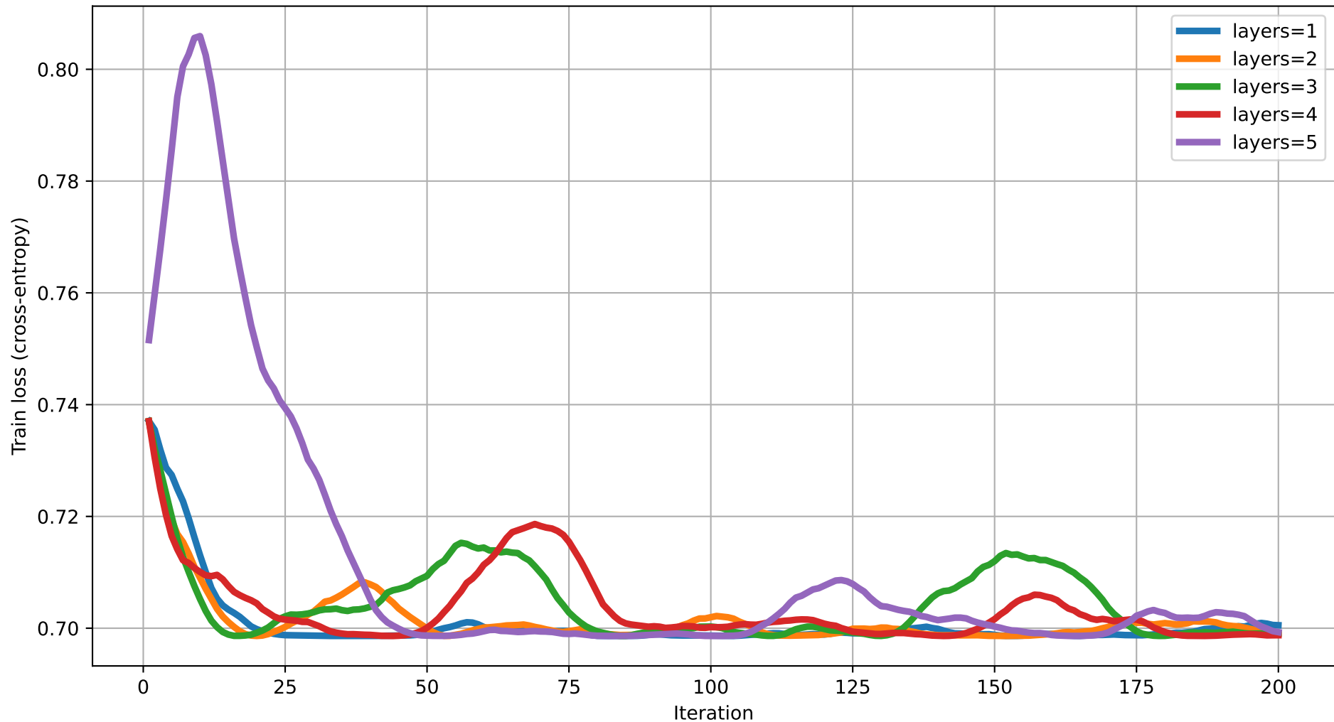
Train loss vs Iteration (dim=18) rot=RZ, ent=pairwise, gate=CNOT
