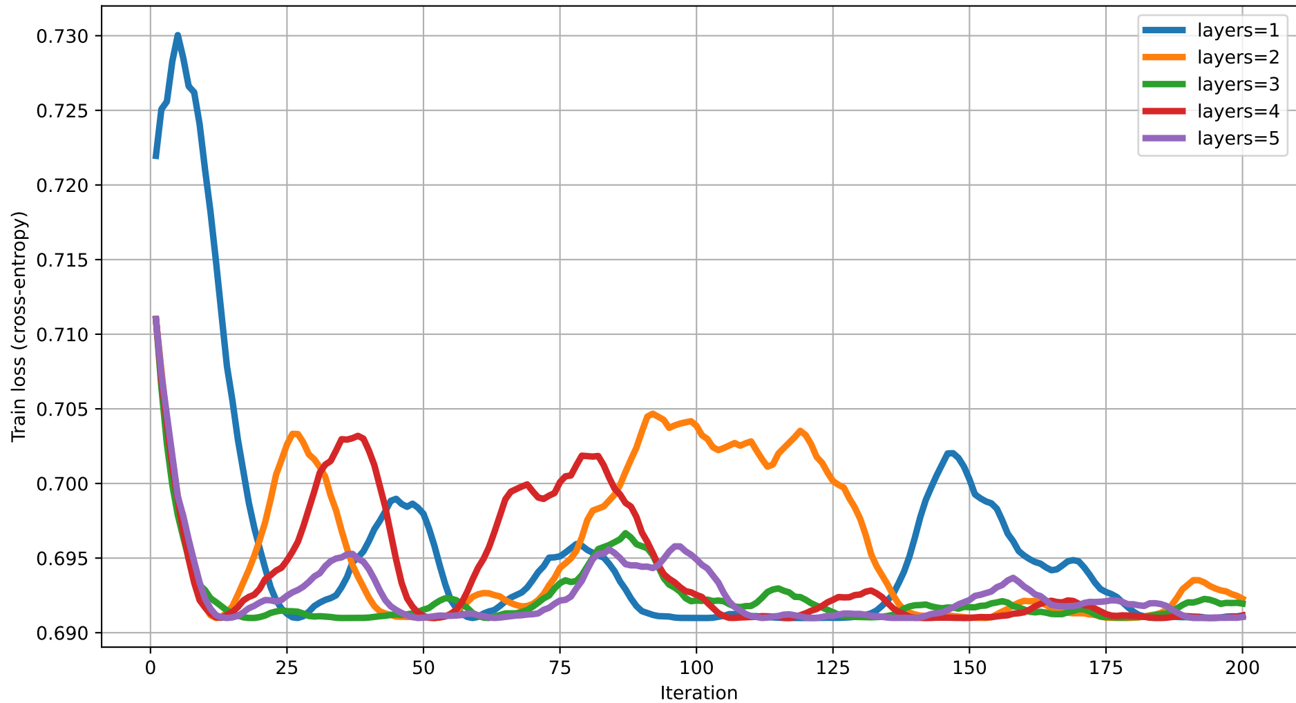
Train loss vs Iteration (dim=20) rot=RZ, ent=chain, gate=CZ
