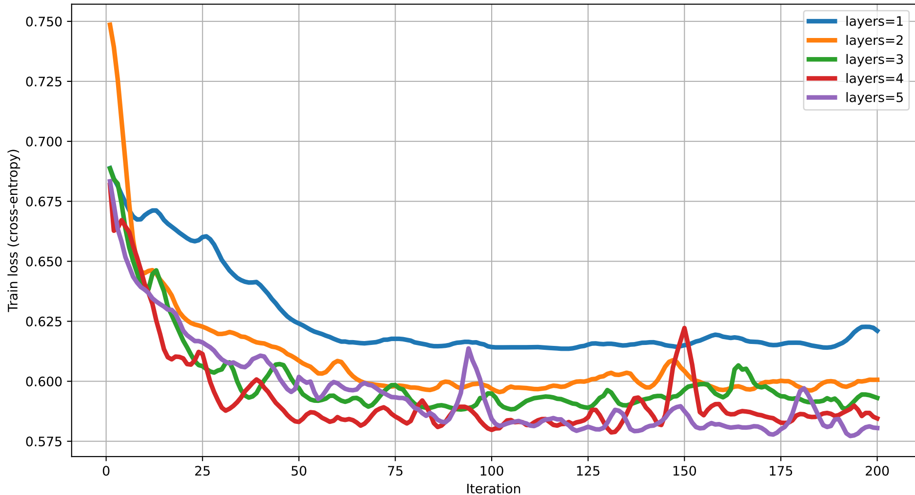
Train loss vs Iteration (degree=3) rot=Rot, ent=full, gate=IsingXX
