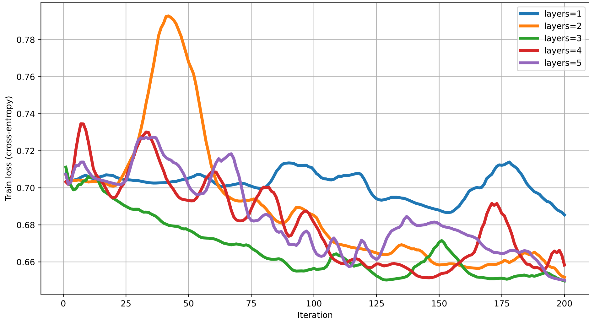
Train loss vs Iteration (dim=6) rot=RYZ, ent=pairwise, gate=CNOT
