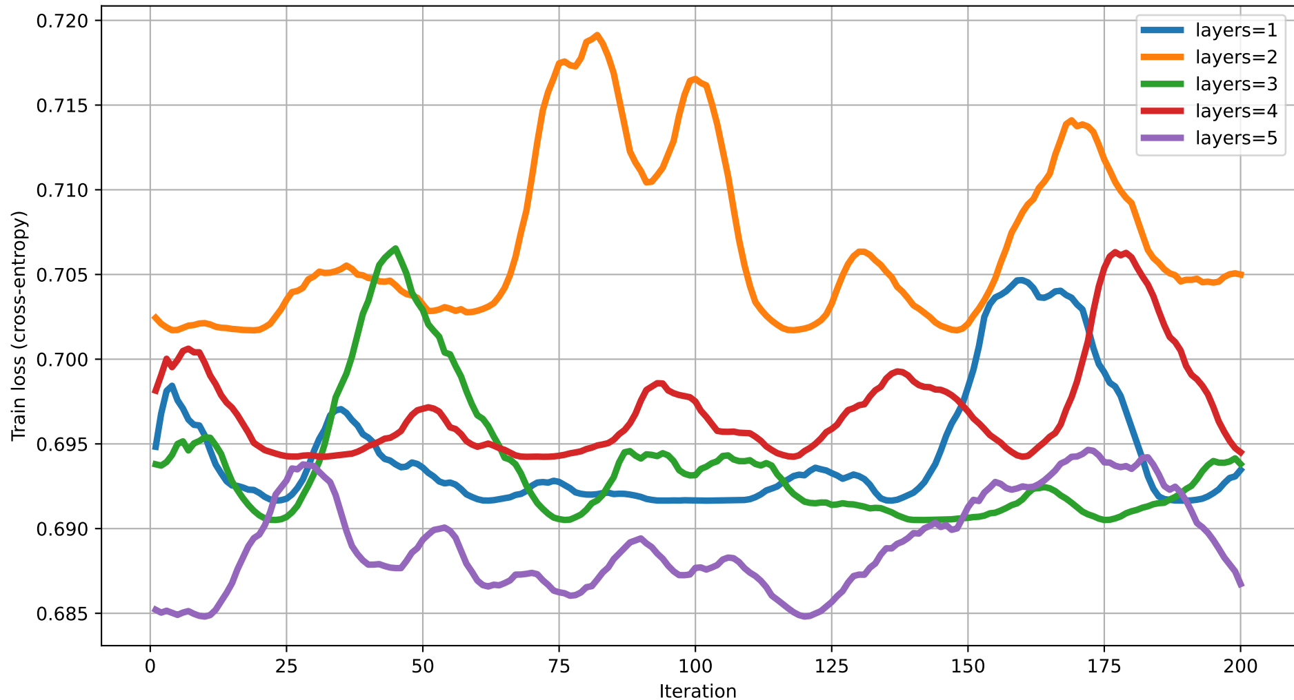
Train loss vs Iteration (dim=18) rot=RZ, ent=ring, gate=CNOT
