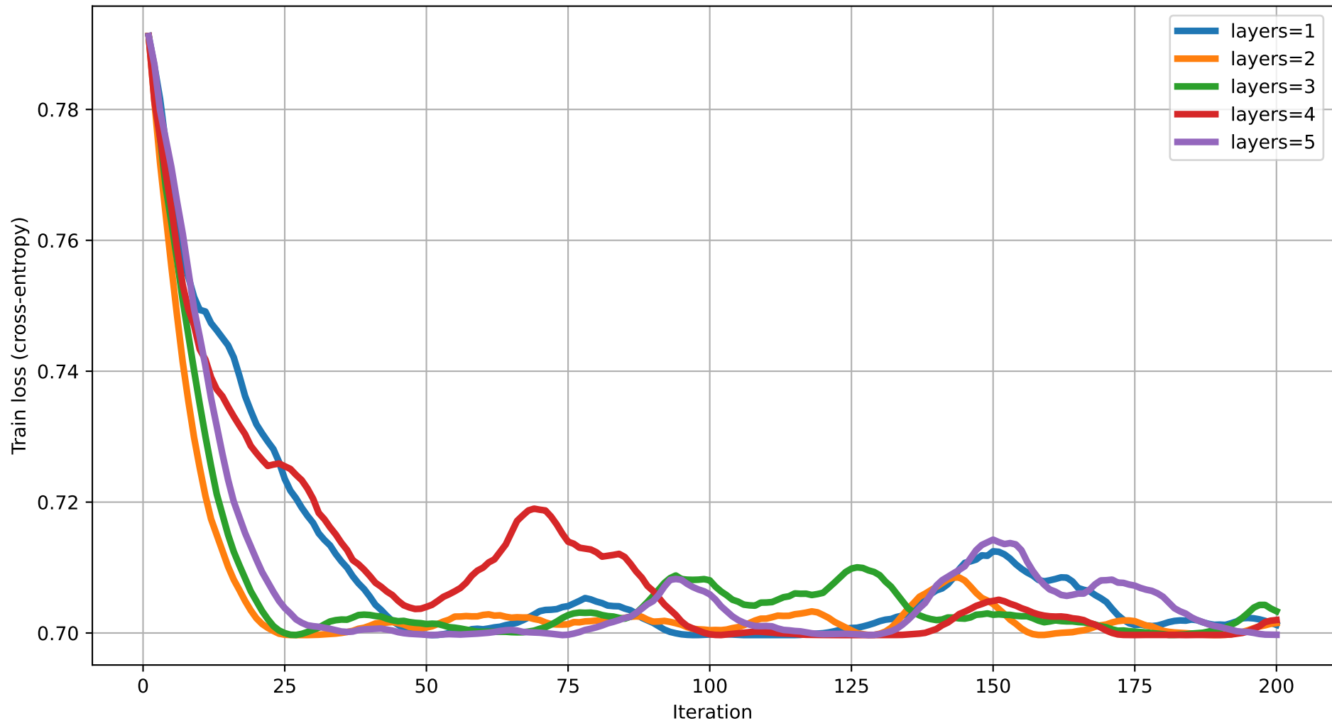
Train loss vs Iteration (dim=4) rot=RZ, ent=full, gate=CZ
