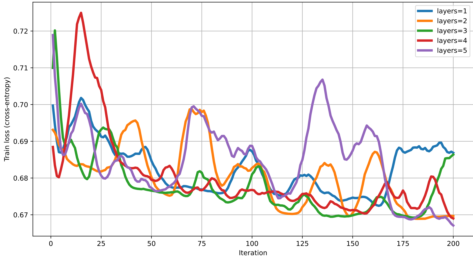
Train loss vs Iteration (dim=13) rot=RYZ, ent=ring, gate=CZ
