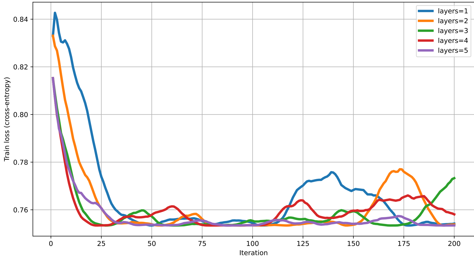
Train loss vs Iteration (dim=2) rot=RZ, ent=full, gate=CNOT
