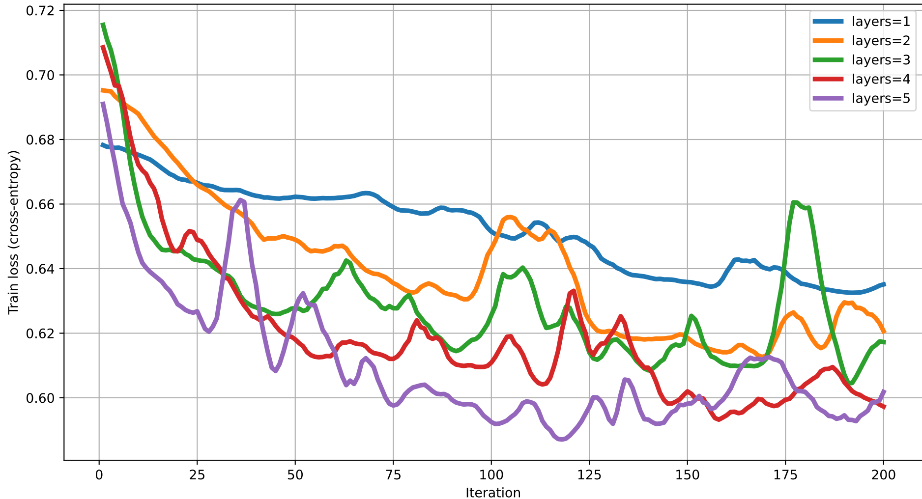
Train loss vs Iteration (dim=17) rot=Rot, ent=ring, gate=CNOT
