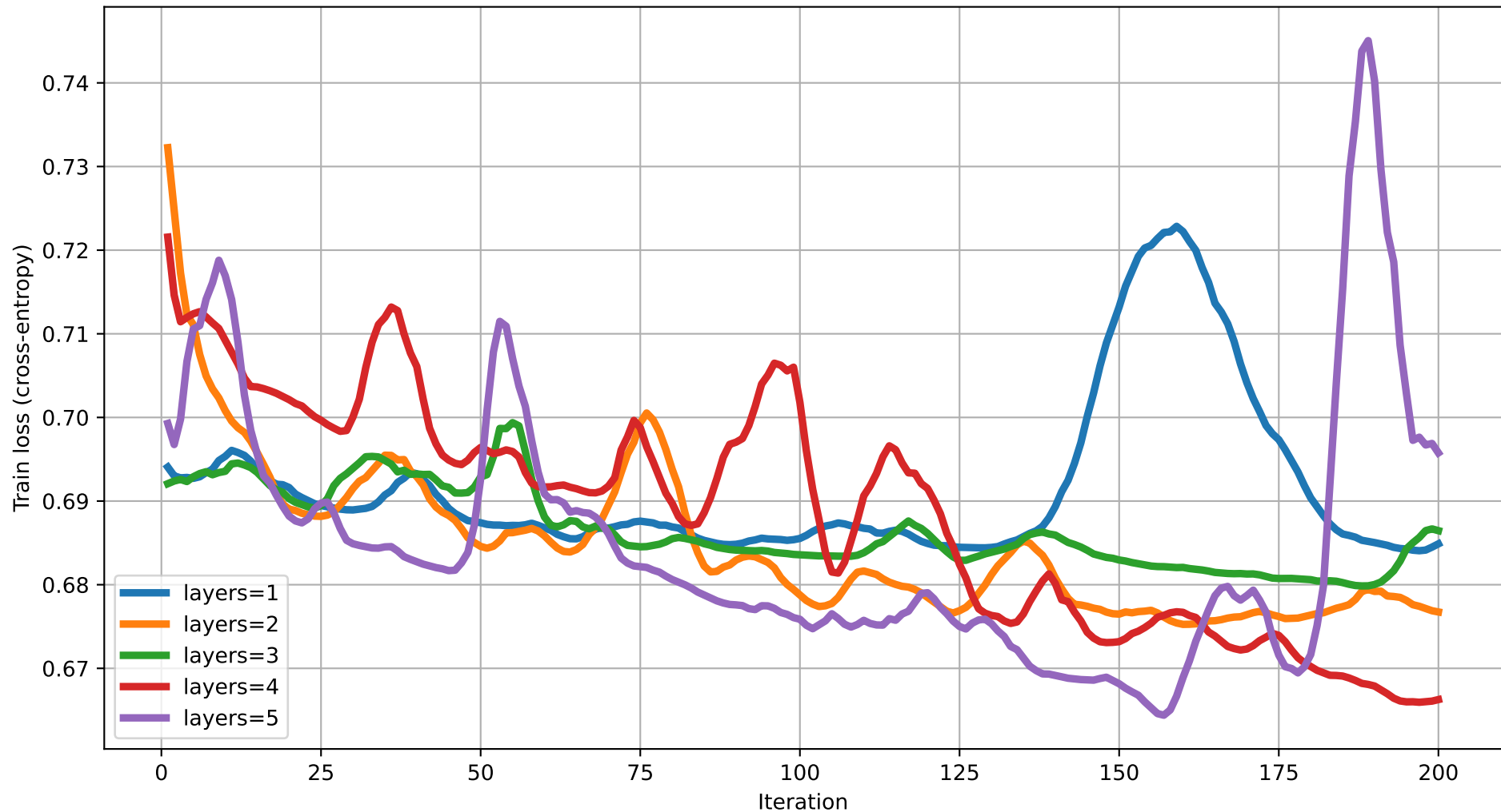
Train loss vs Iteration (dim=10) rot=RZ, ent=chain, gate=IsingXX
