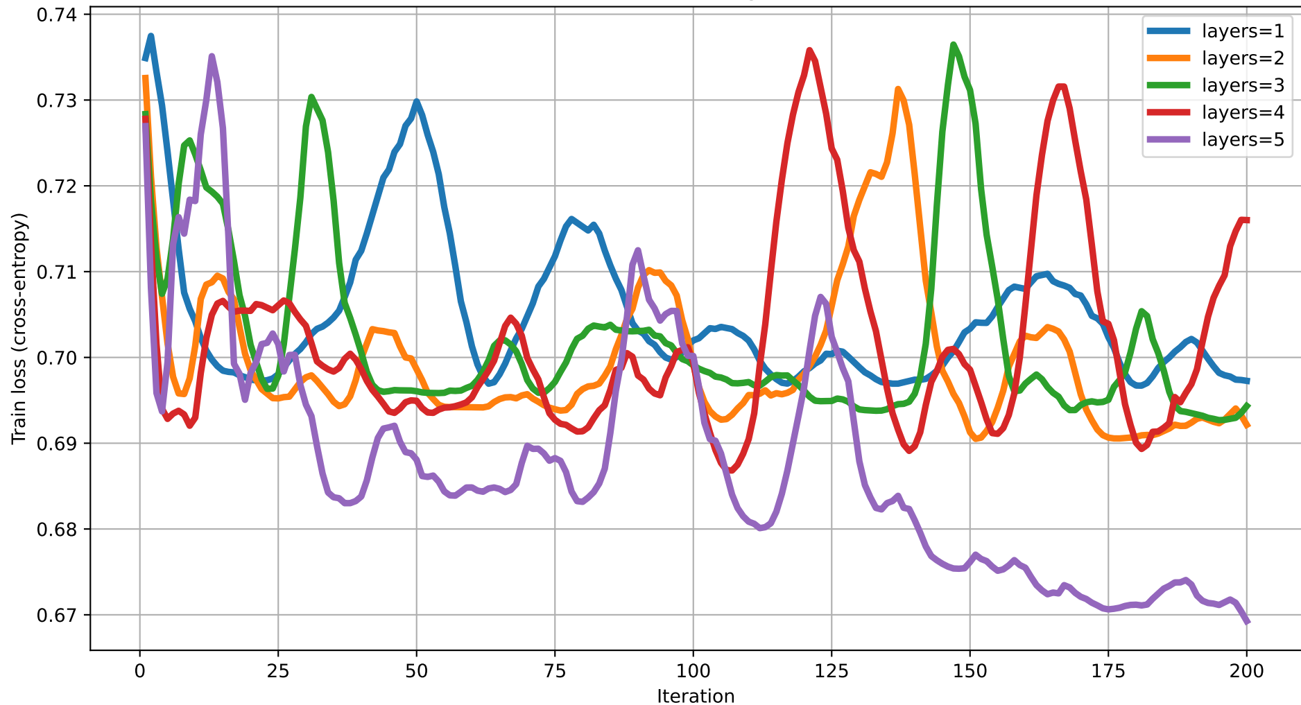
Train loss vs Iteration (dim=18) rot=Rot, ent=chain, gate=CNOT
