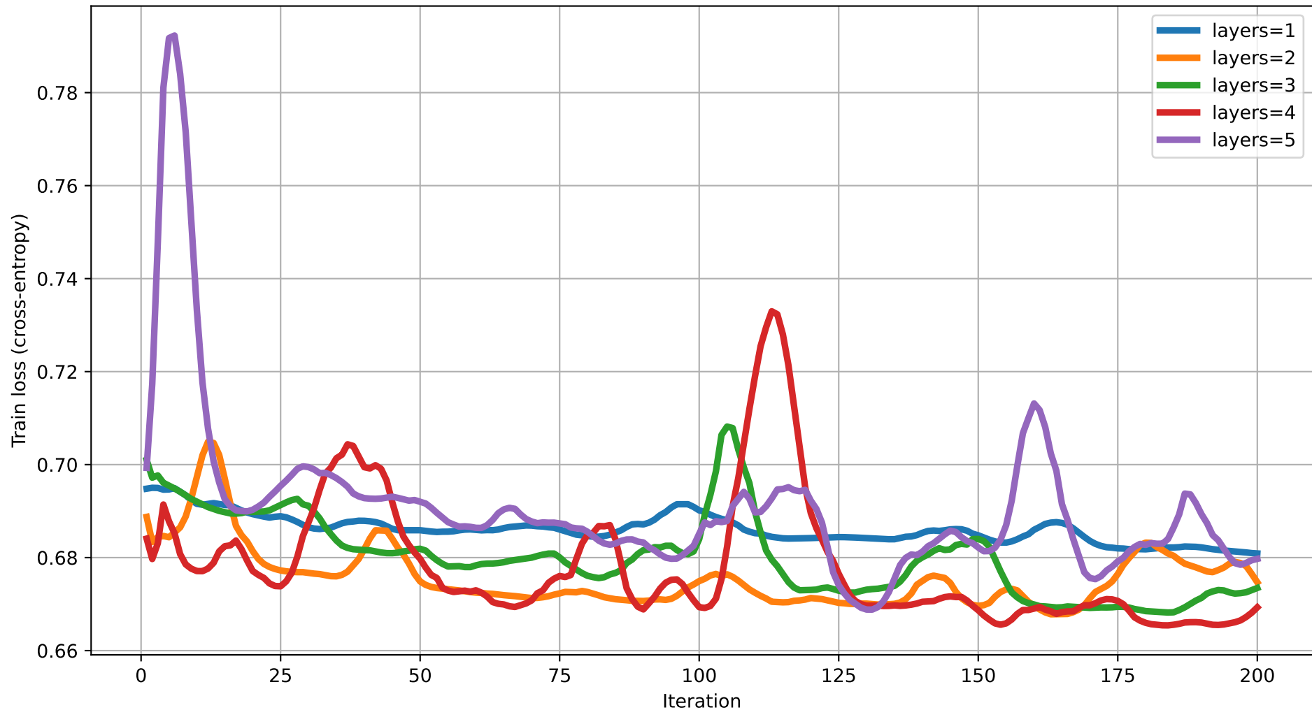
Train loss vs Iteration (dim=13) rot=RY, ent=ring, gate=IsingXX
