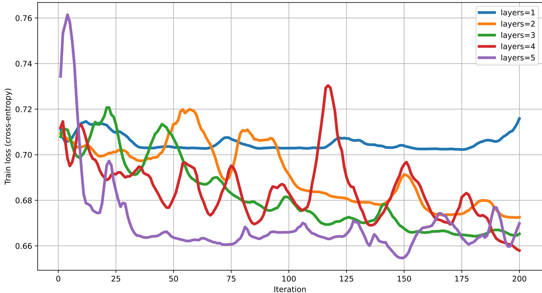
Train loss vs Iteration (dim=11) rot=RYZ, ent=full, gate=CNOT
