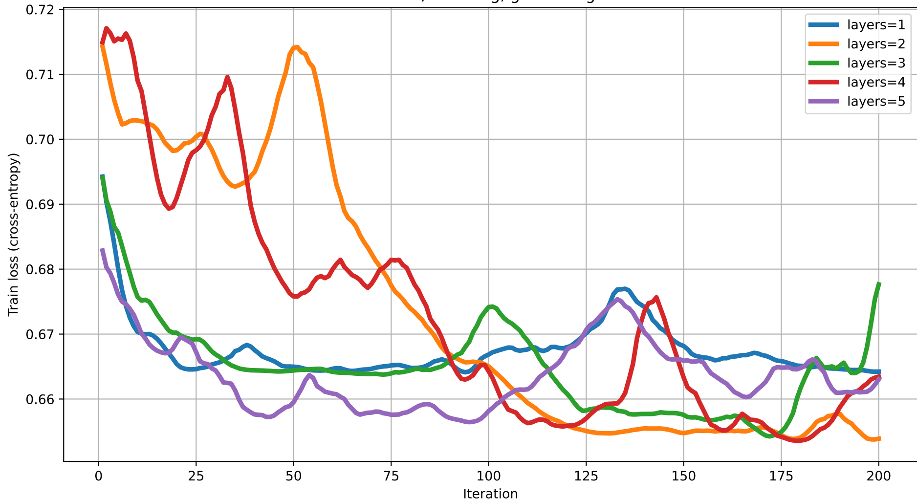
Train loss vs Iteration (dim=6) rot=RZ, ent=ring, gate=IsingXX
