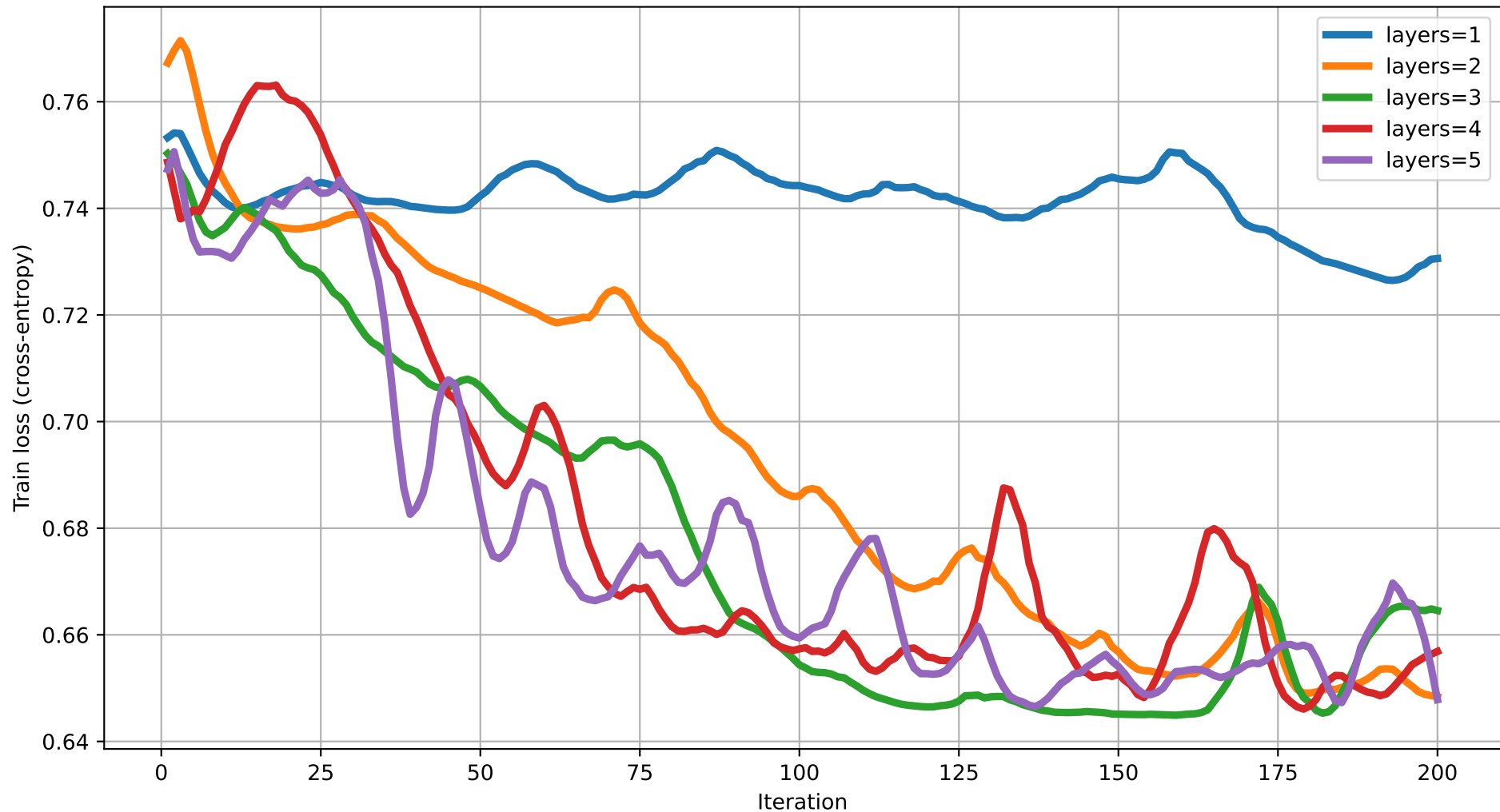
Train loss vs Iteration (dim=5) rot=RY, ent=pairwise, gate=CZ
