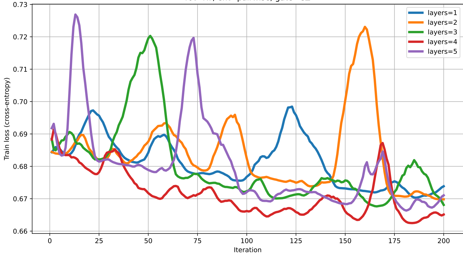
Train loss vs Iteration (dim=15) rot=RY, ent=pairwise, gate=CZ
