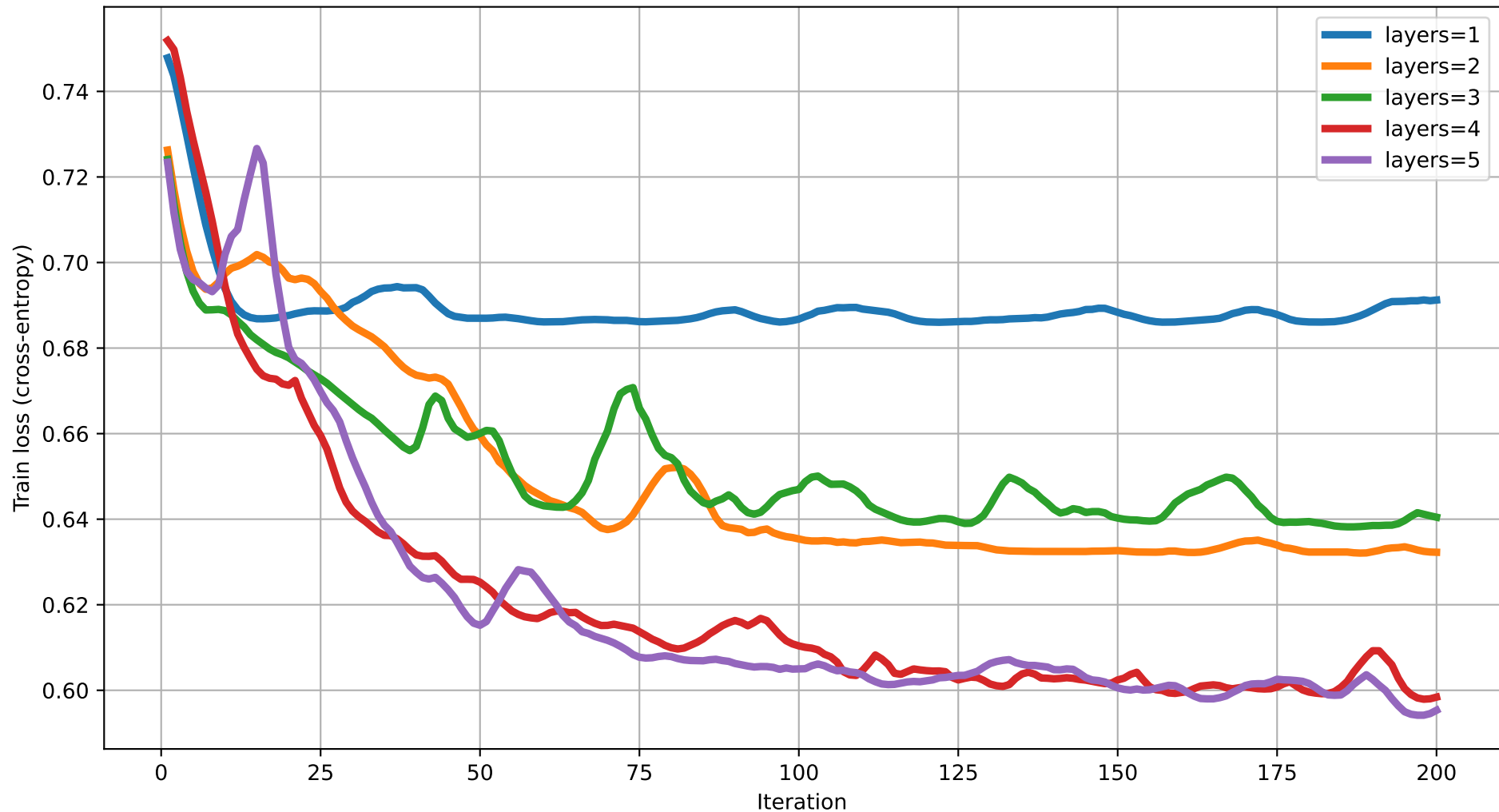
Train loss vs Iteration (degree=2) rot=Rot, ent=chain, gate=CZ
