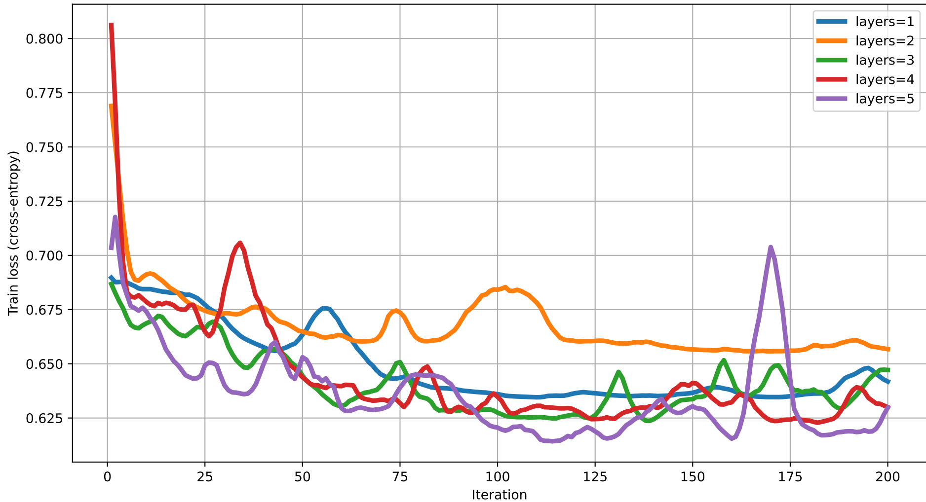
Train loss vs Iteration (dim=16) rot=Rot, ent=chain, gate=IsingXX
