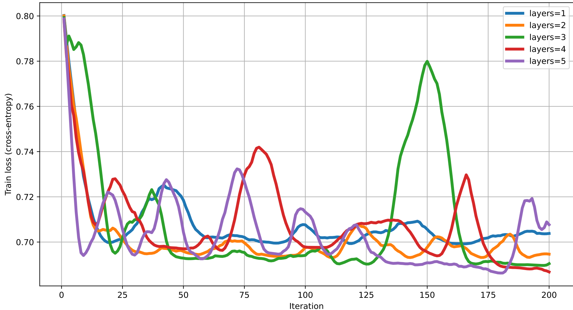
Train loss vs Iteration (dim=8) rot=RX, ent=pairwise, gate=CZ
