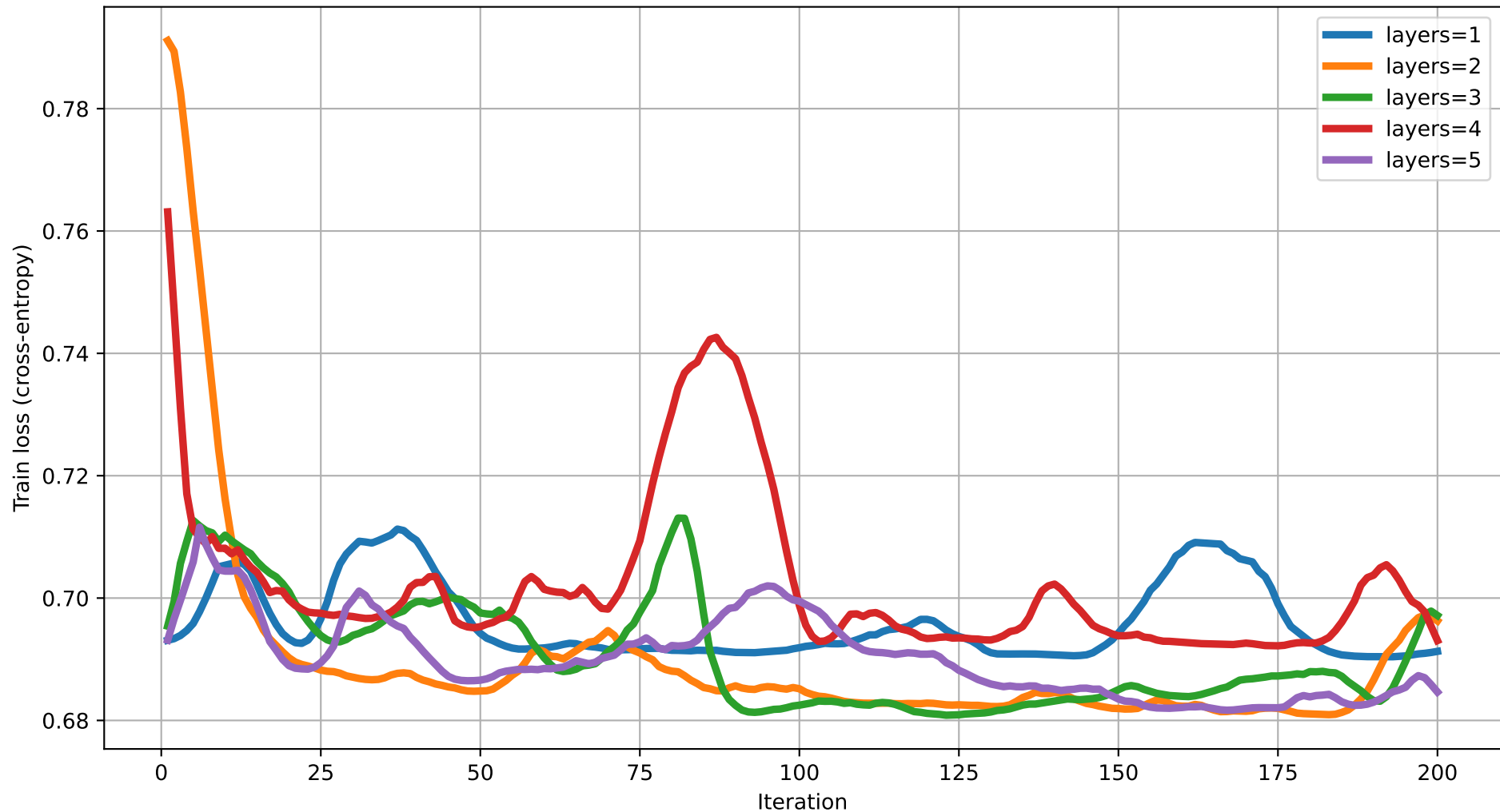
Train loss vs Iteration (dim=17) rot=RZ, ent=chain, gate=IsingXX
