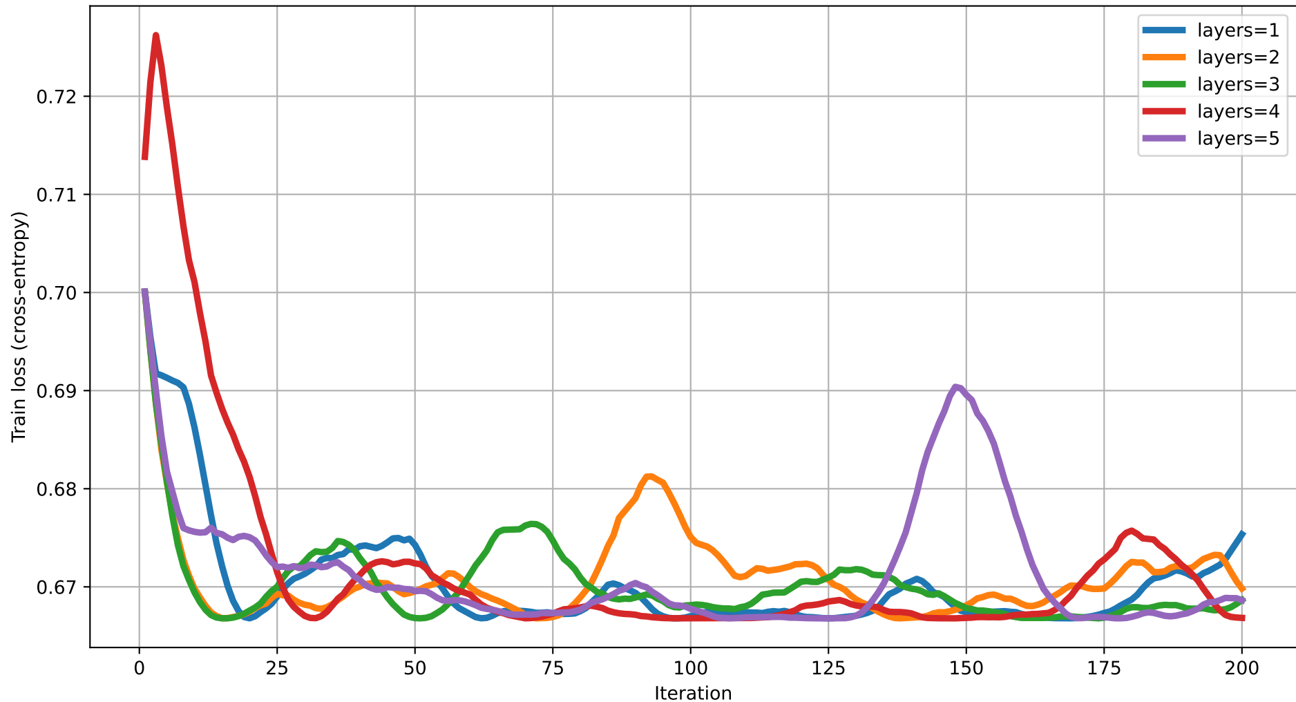
Train loss vs Iteration (dim=10) rot=RZ, ent=full, gate=CNOT
