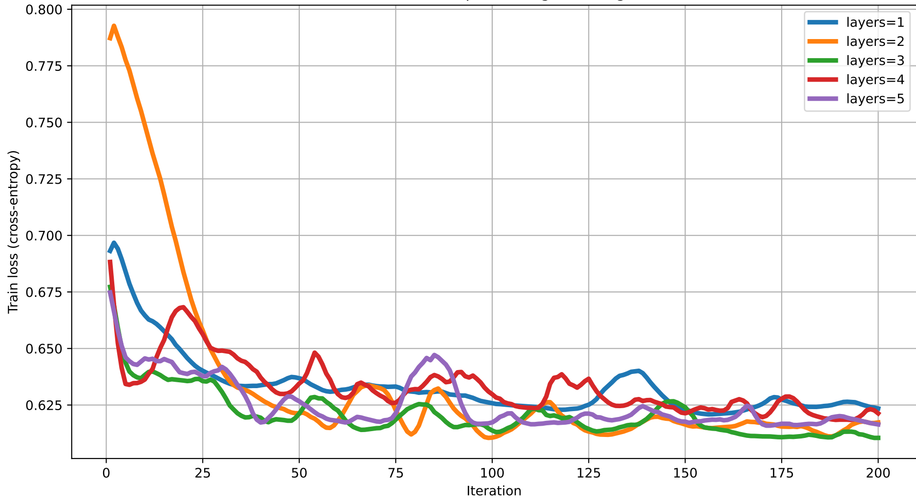
Train loss vs Iteration (dim=10) rot=RYZ, ent=pairwise, gate=IsingXX
