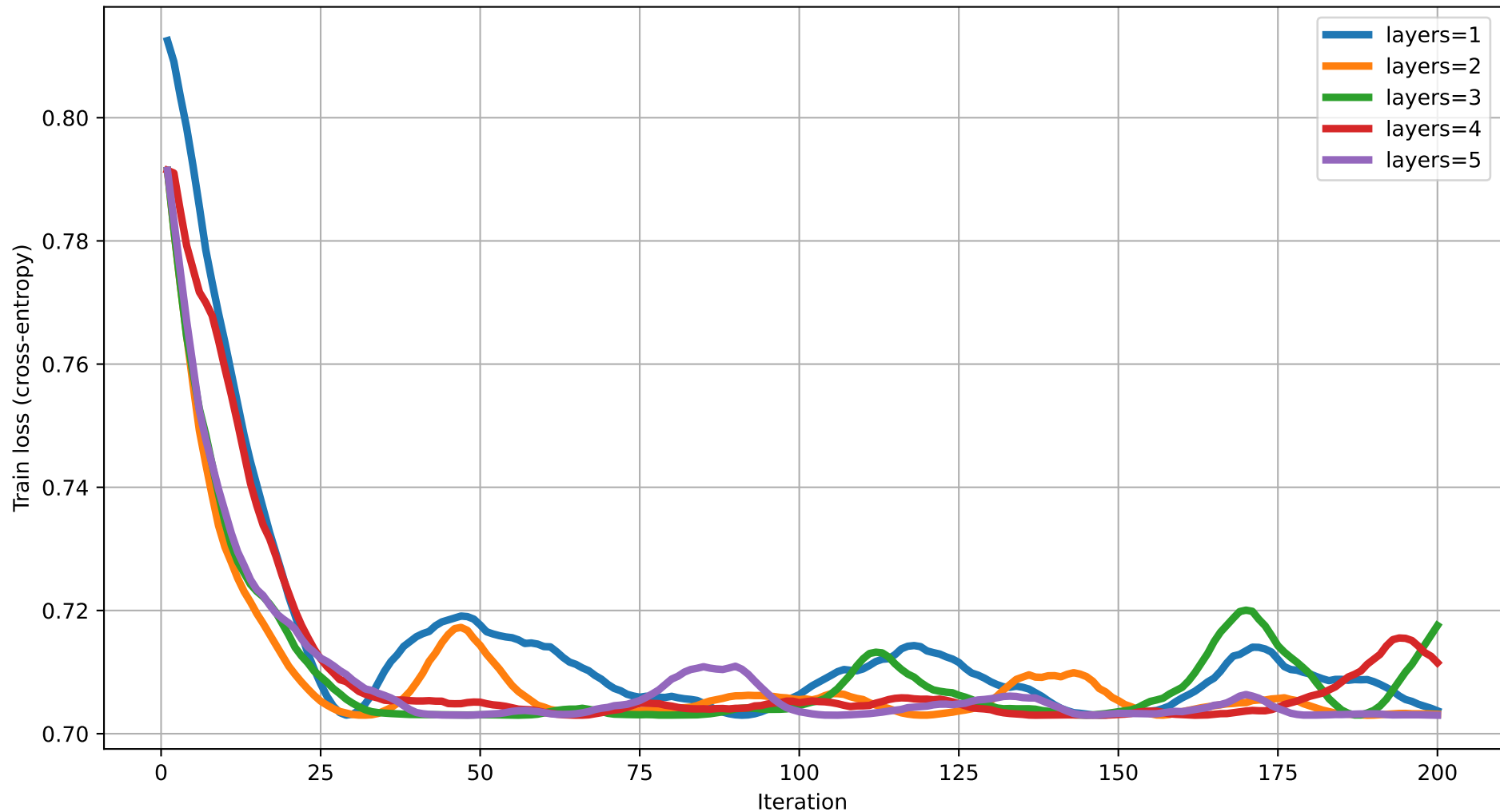
Train loss vs Iteration (dim=2) rot=RZ, ent=chain, gate=CZ
