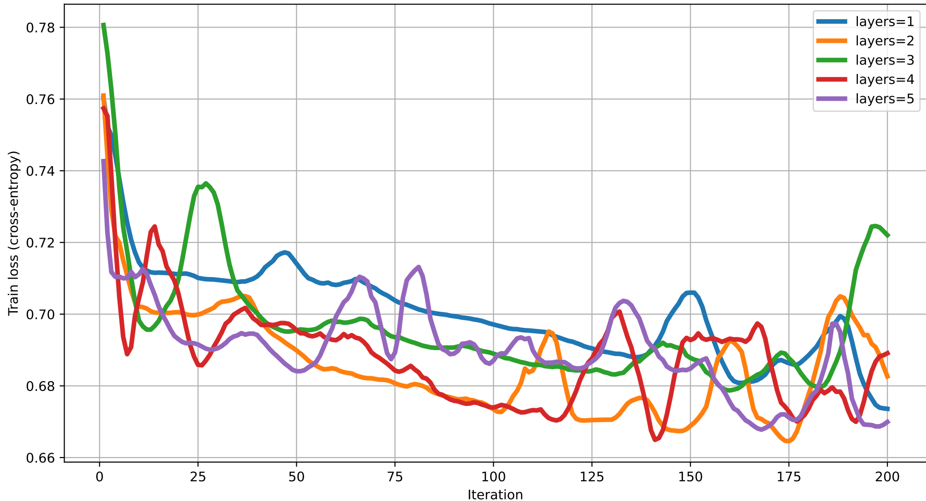
Train loss vs Iteration (dim=17) rot=RY, ent=full, gate=IsingXX
