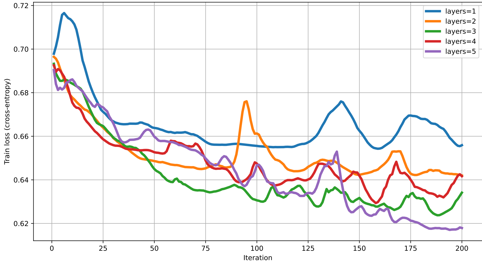
Train loss vs Iteration (dim=14) rot=Rot, ent=chain, gate=CZ
