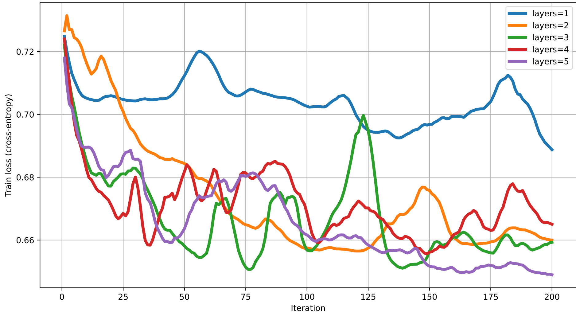
Train loss vs Iteration (dim=5) rot=Rot, ent=chain, gate=CZ
