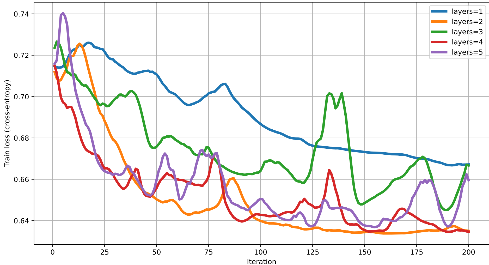
Train loss vs Iteration (dim=7) rot=Rot, ent=pairwise, gate=CNOT
