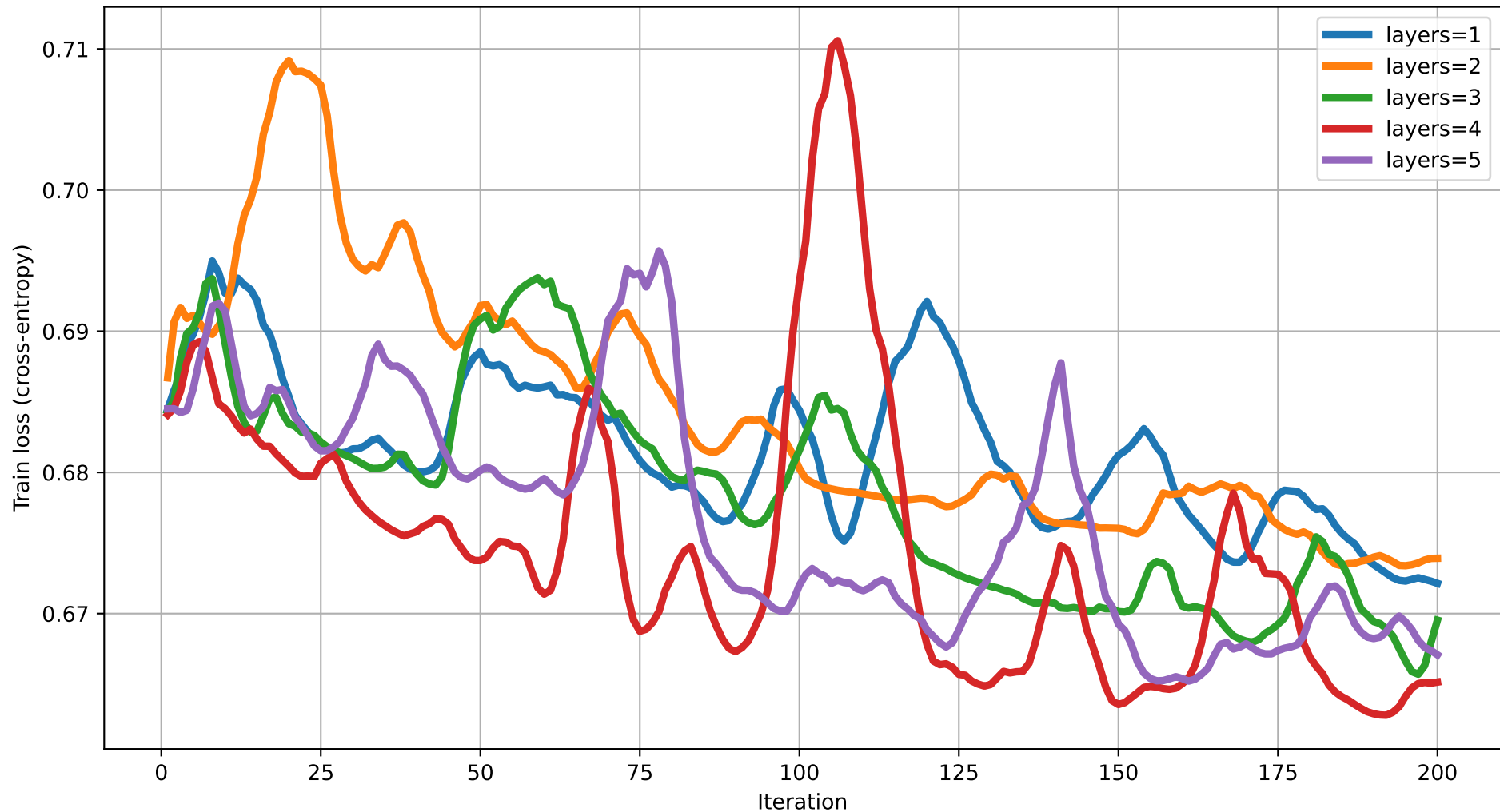
Train loss vs Iteration (dim=15) rot=RYZ, ent=pairwise, gate=CZ
