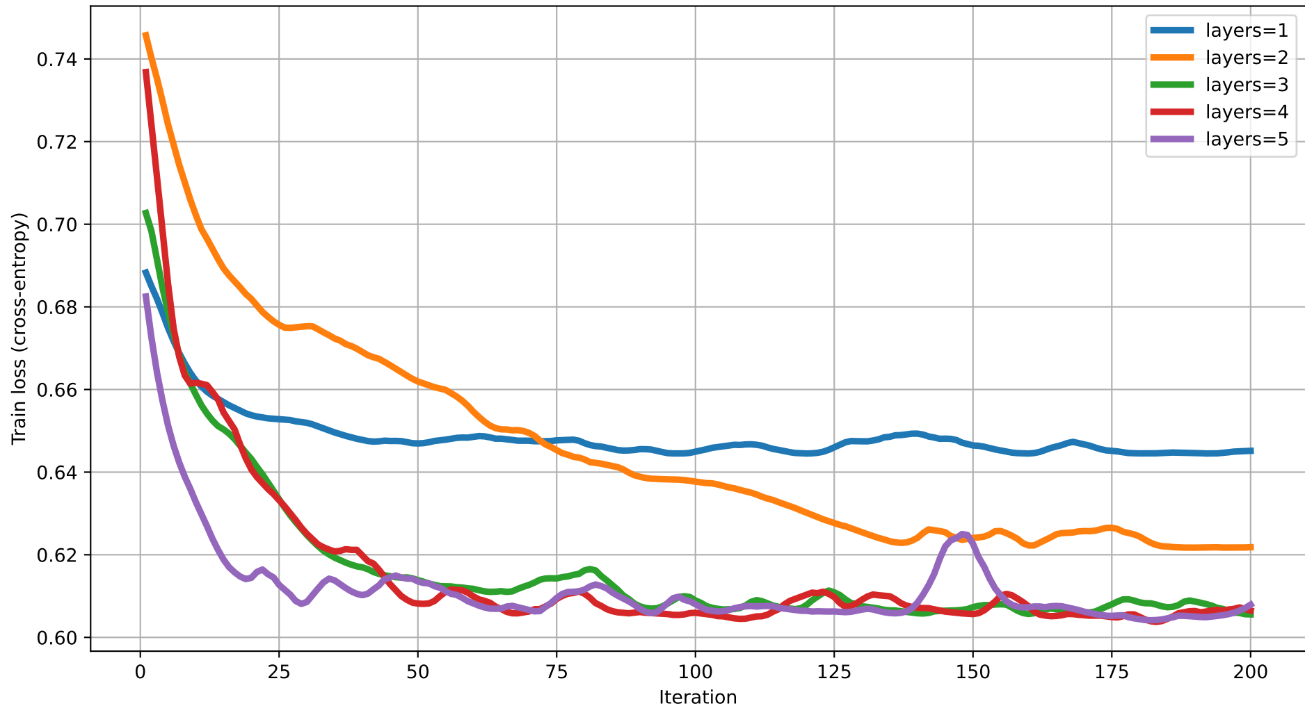
Train loss vs Iteration (degree=5) rot=RZ, ent=chain, gate=IsingXX
