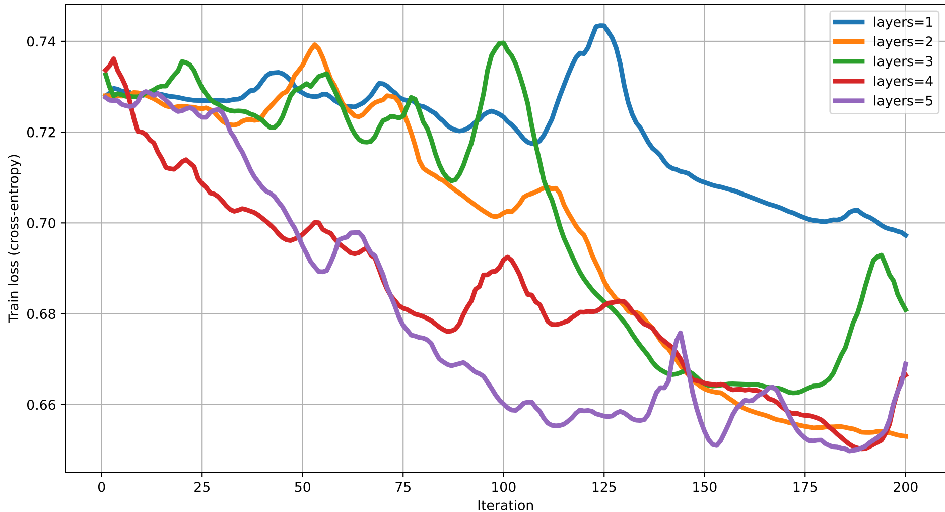
Train loss vs Iteration (dim=7) rot=RY, ent=pairwise, gate=CZ
