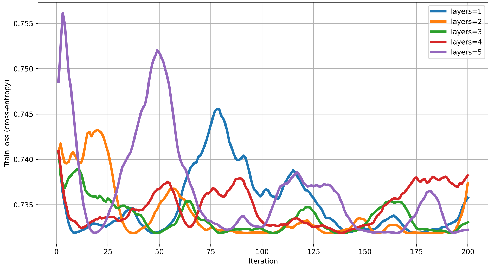
Train loss vs Iteration (dim=3) rot=RZ, ent=chain, gate=CZ
