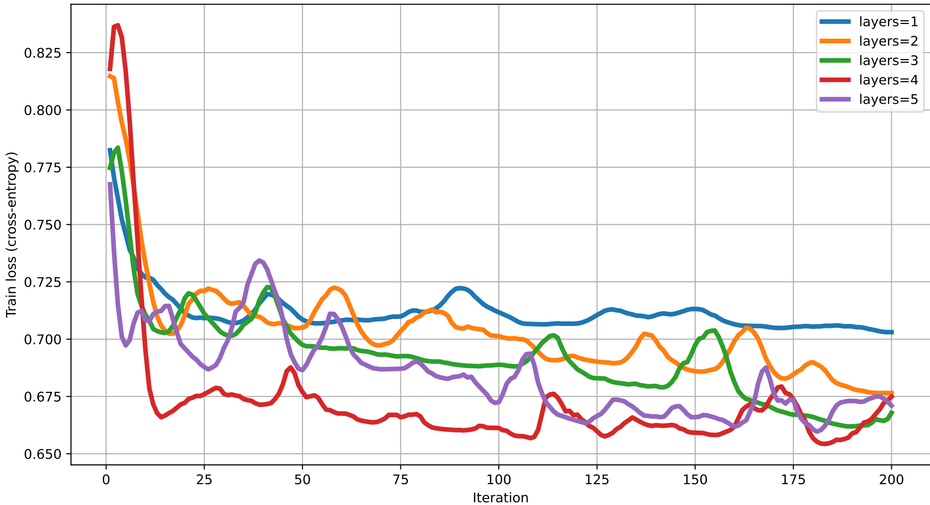
Train loss vs Iteration (dim=9) rot=RYZ, ent=pairwise, gate=CNOT
