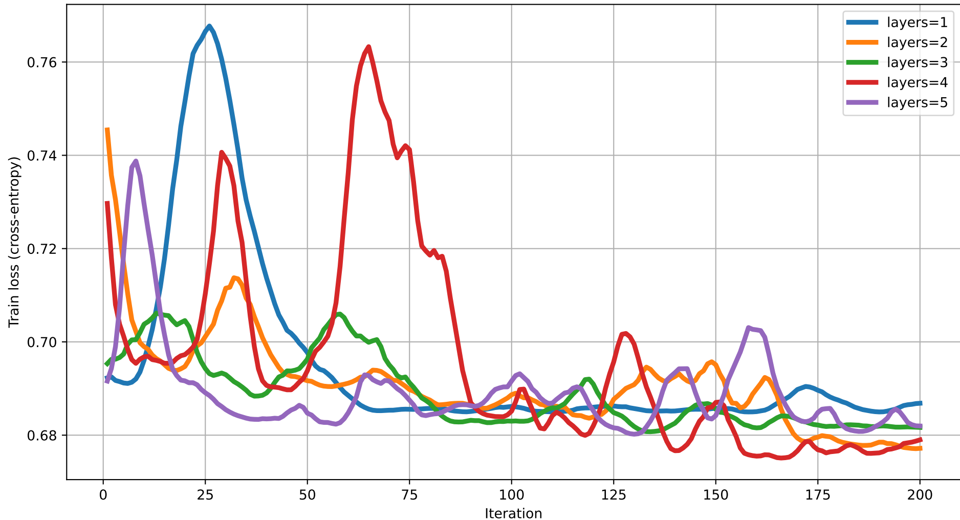
Train loss vs Iteration (dim=19) rot=RZ, ent=chain, gate=IsingXX
