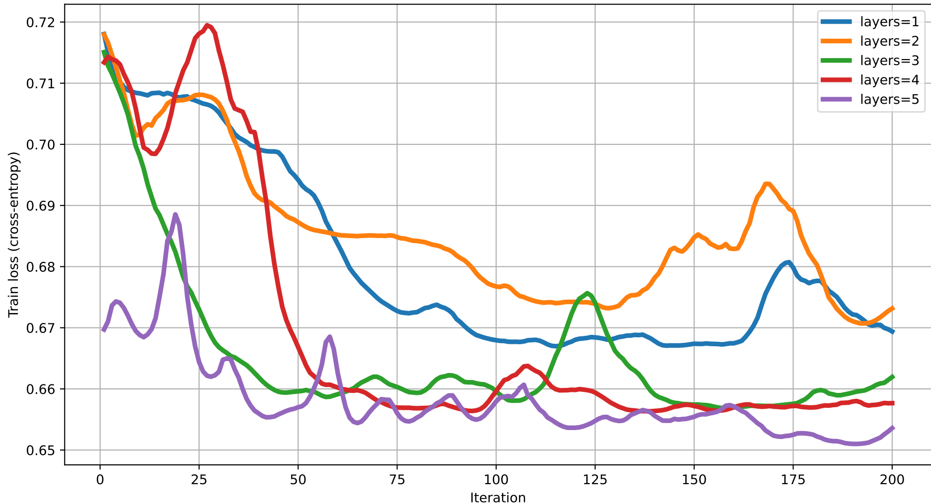
Train loss vs Iteration (dim=8) rot=RX, ent=ring, gate=CNOT
