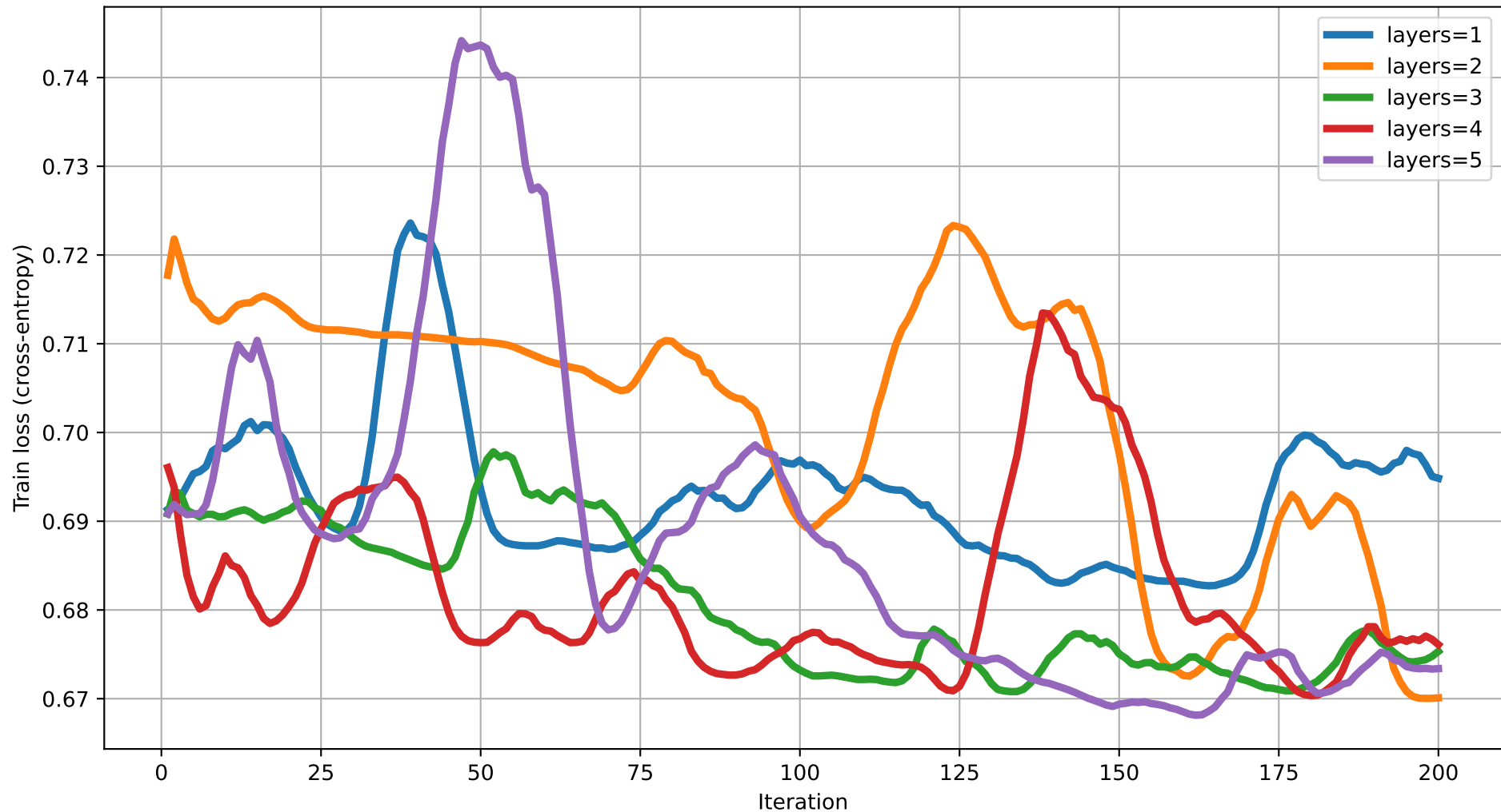
Train loss vs Iteration (dim=13) rot=RZ, ent=chain, gate=IsingXX
