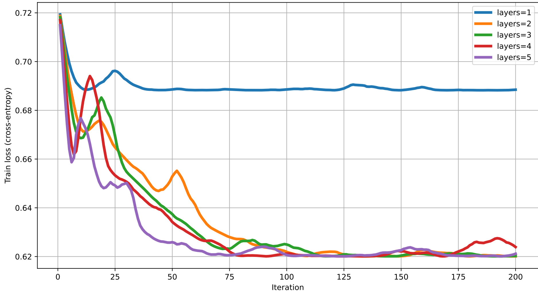
Train loss vs Iteration (degree=4) rot=RX, ent=pairwise, gate=CNOT
