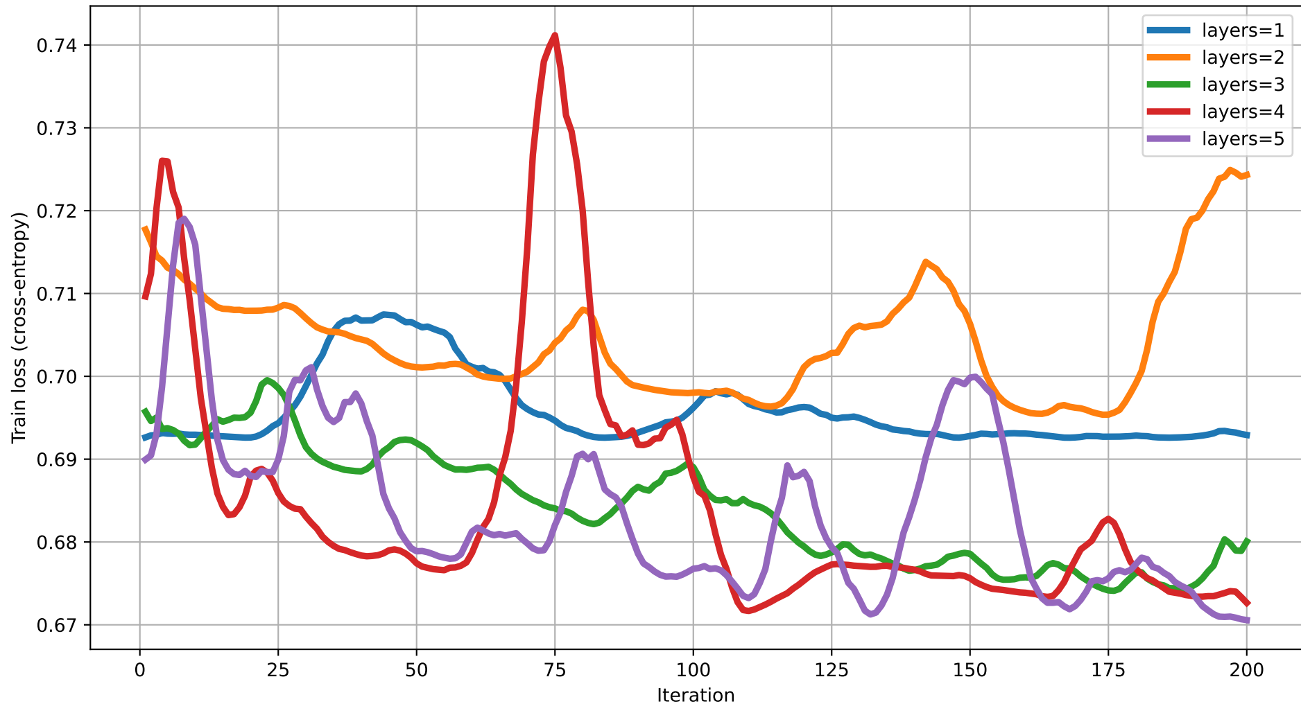
Train loss vs Iteration (dim=13) rot=RY, ent=full, gate=IsingXX
