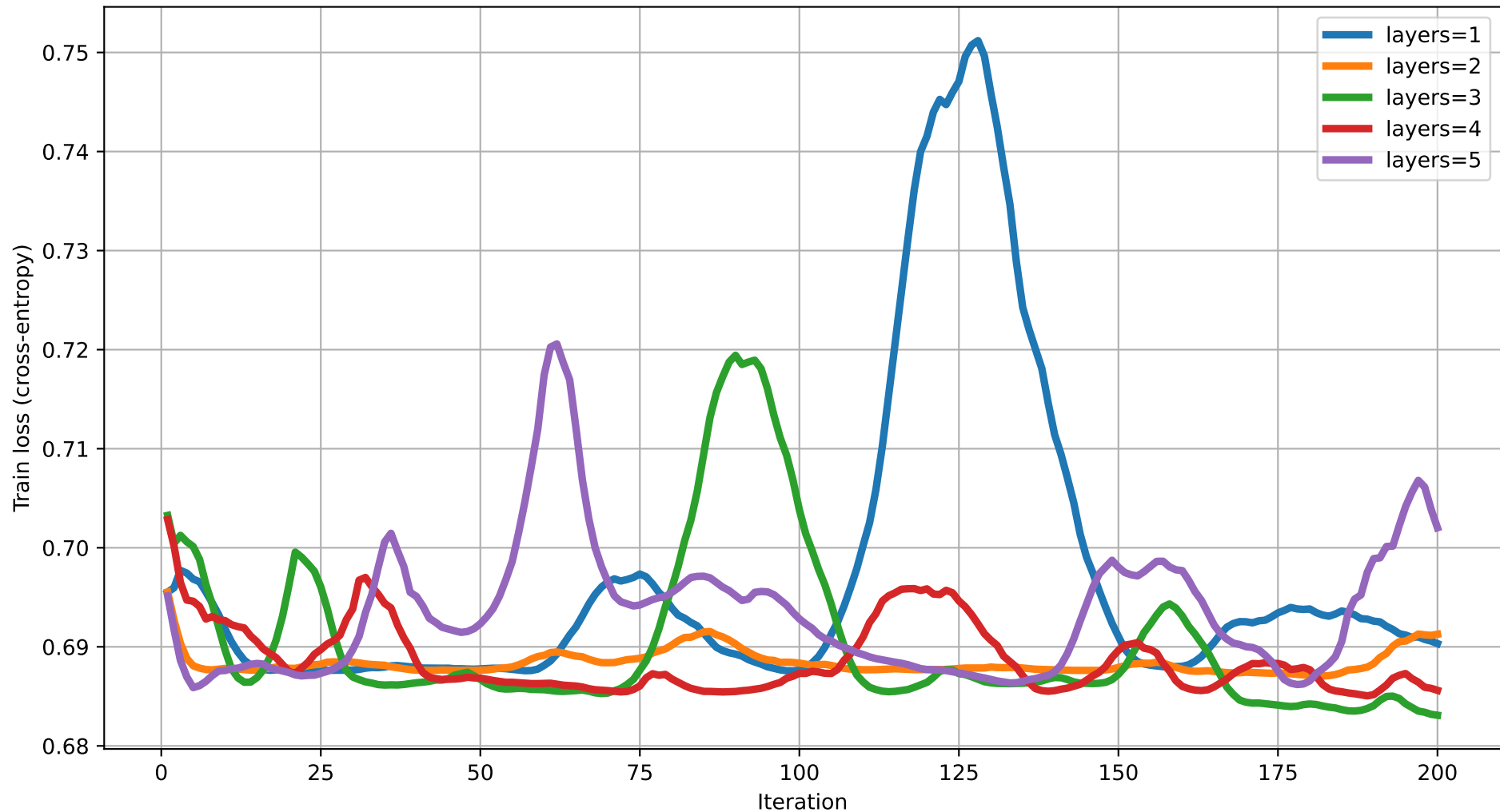
Train loss vs Iteration (dim=13) rot=RX, ent=pairwise, gate=CZ
