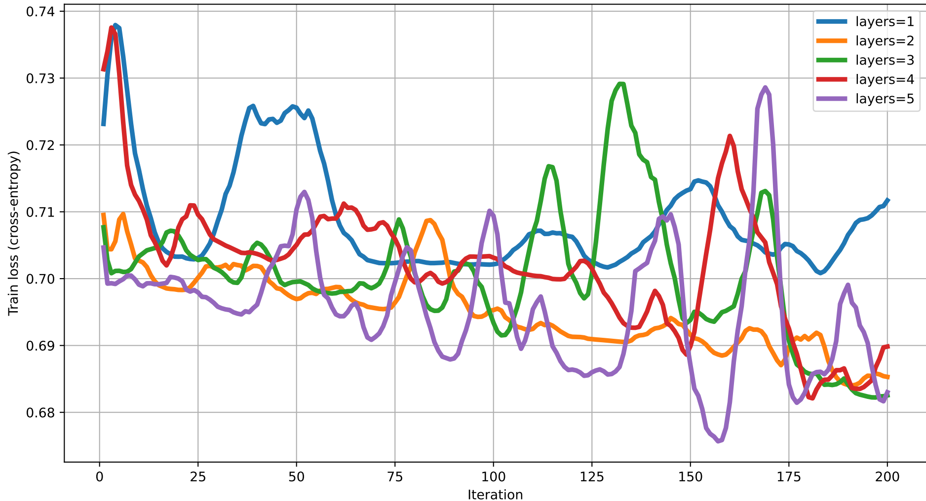
Train loss vs Iteration (dim=11) rot=Rot, ent=pairwise, gate=CZ
