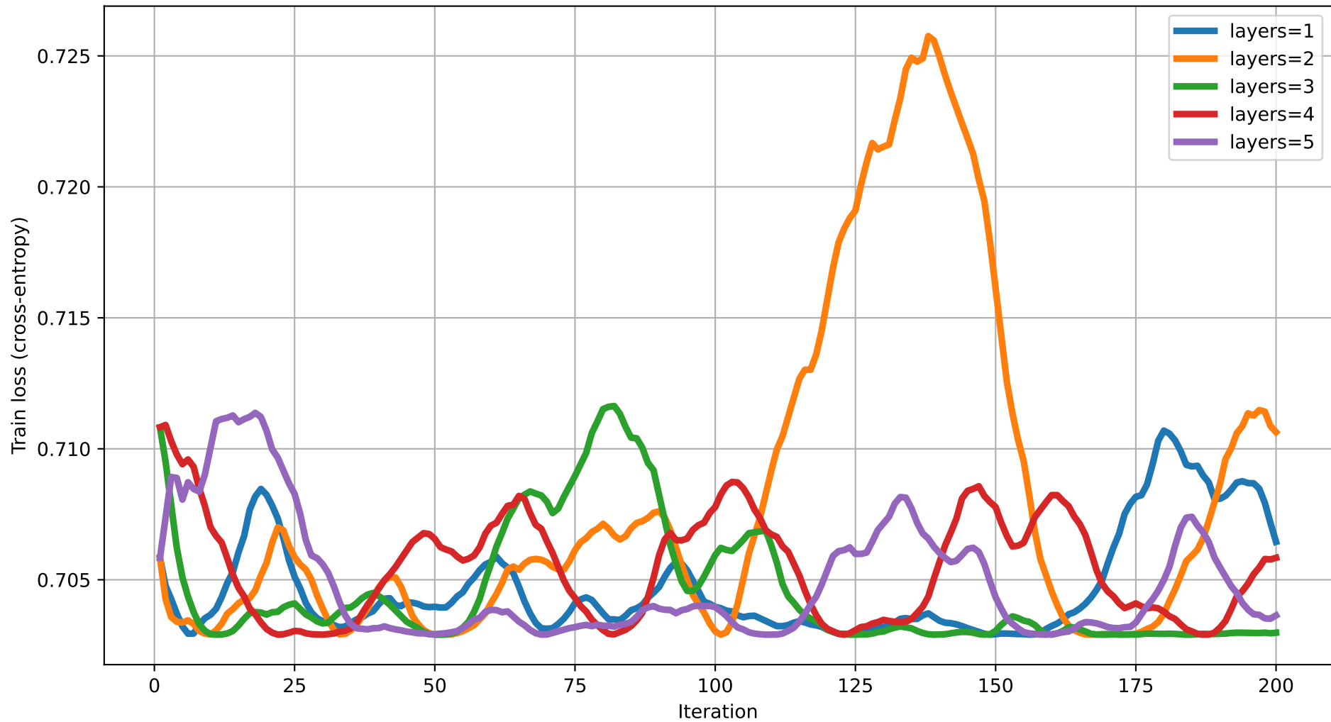
Train loss vs Iteration (dim=12) rot=RZ, ent=pairwise, gate=CNOT
