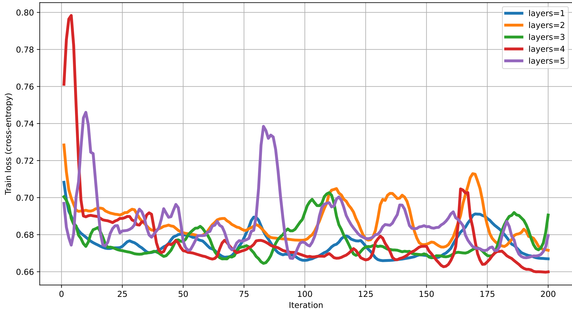
Train loss vs Iteration (dim=19) rot=Rot, ent=ring, gate=IsingXX
