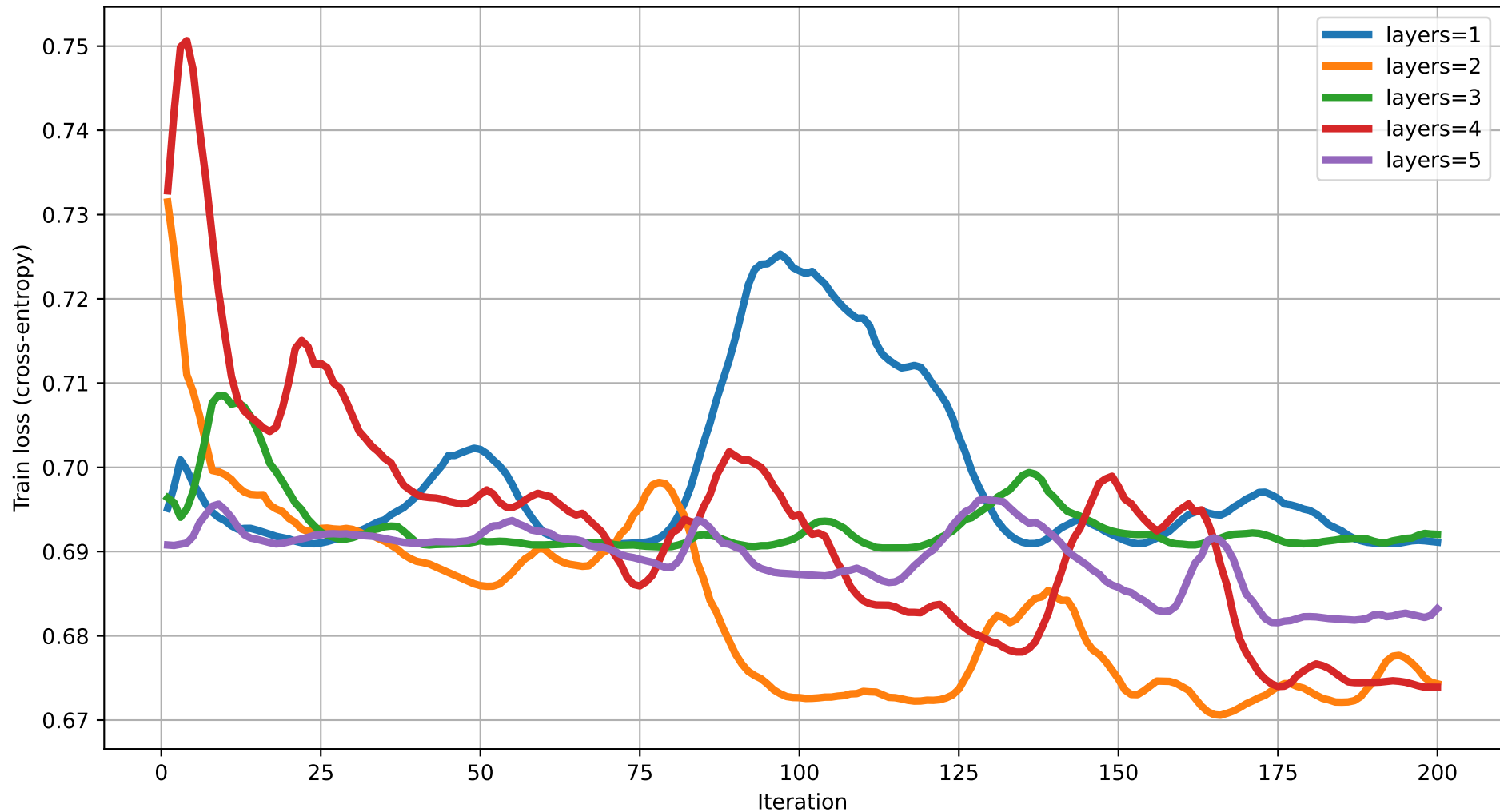
Train loss vs Iteration (dim=10) rot=RY, ent=chain, gate=IsingXX
