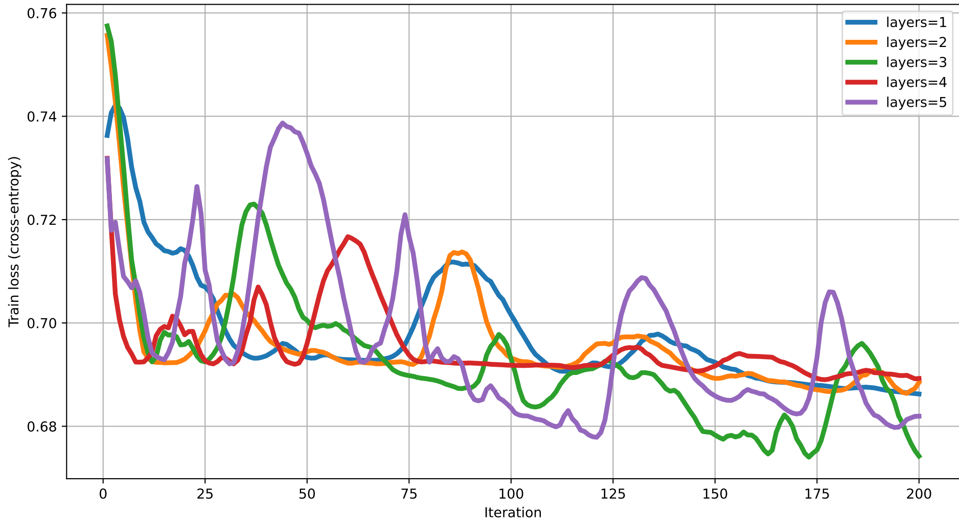
Train loss vs Iteration (dim=16) rot=RYZ, ent=pairwise, gate=CZ
