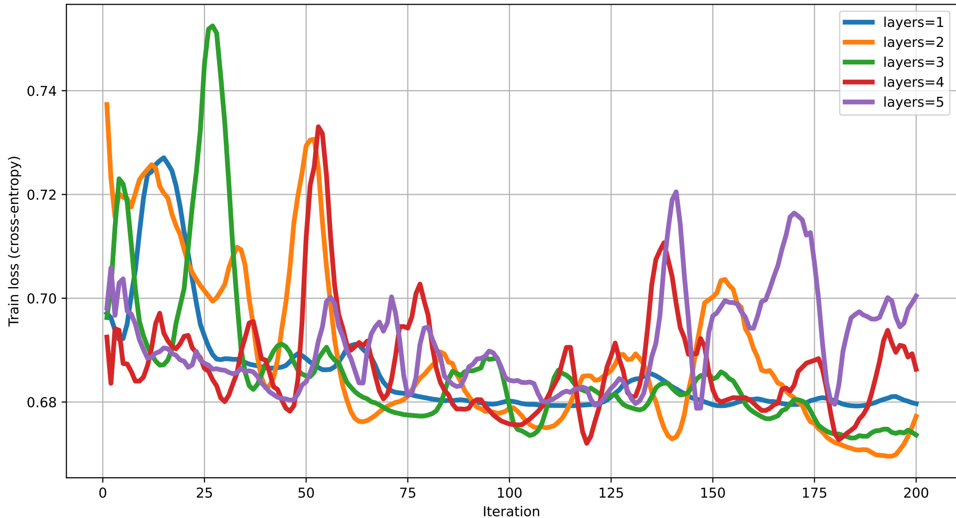
Train loss vs Iteration (dim=20) rot=Rot, ent=chain, gate=IsingXX
