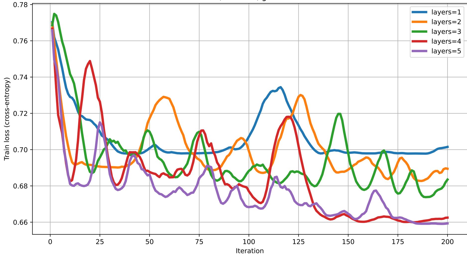
Train loss vs Iteration (dim=17) rot=RX, ent=full, gate=CNOT
