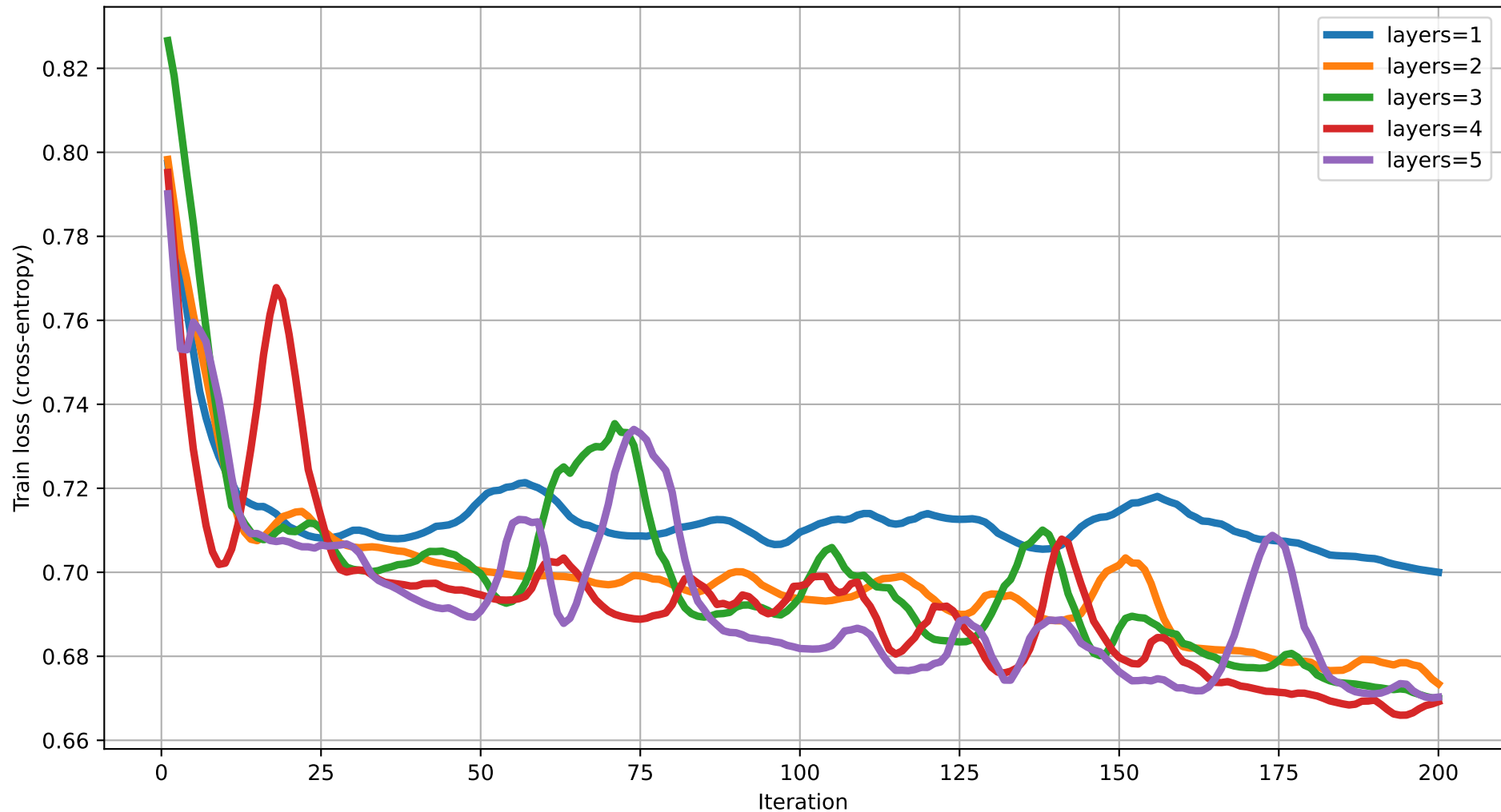
Train loss vs Iteration (dim=8) rot=RYZ, ent=full, gate=CZ
