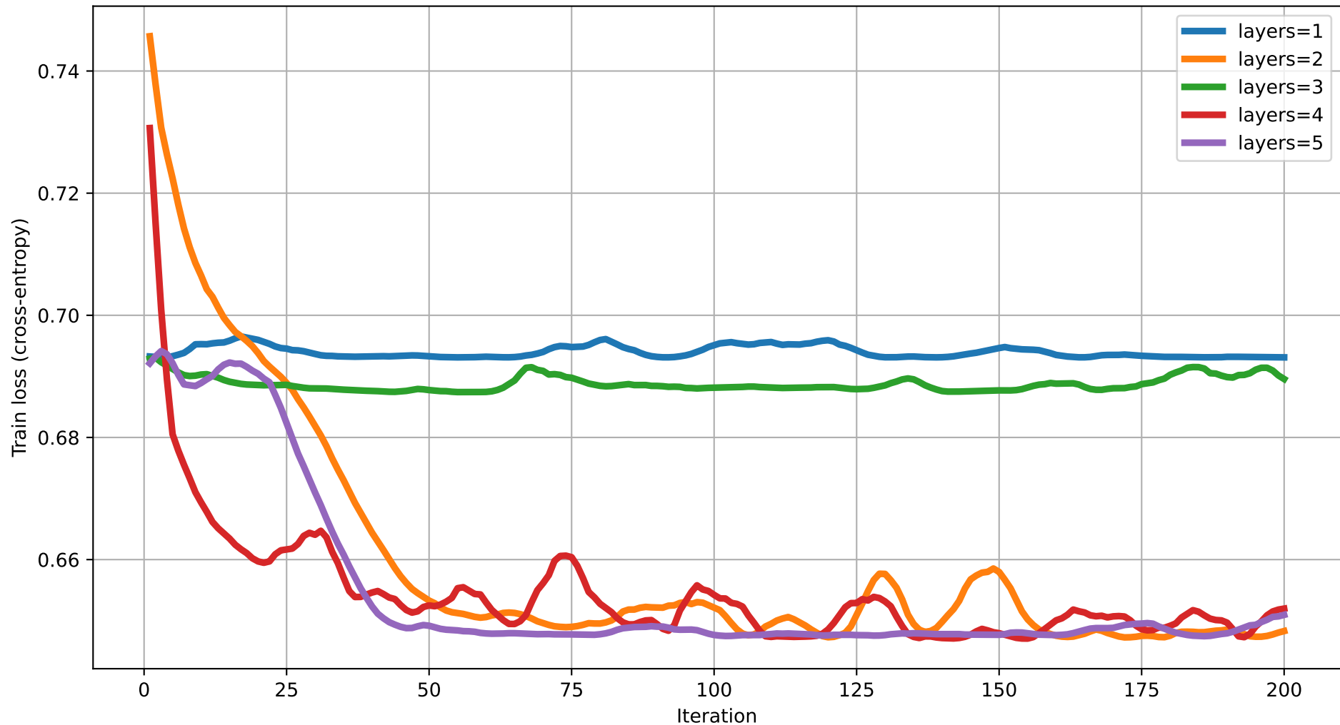
Train loss vs Iteration (degree=5) rot=RY, ent=chain, gate=IsingXX
