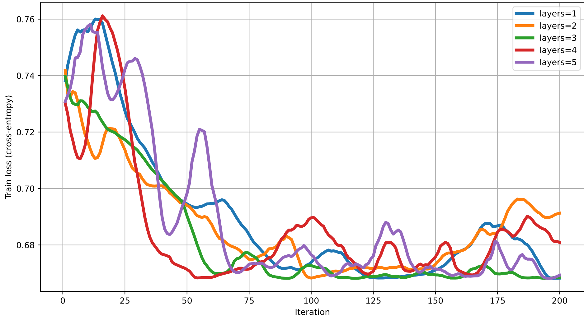
Train loss vs Iteration (dim=3) rot=RY, ent=ring, gate=IsingXX
