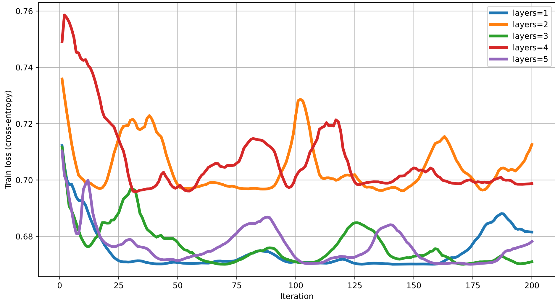
Train loss vs Iteration (dim=19) rot=RX, ent=ring, gate=IsingXX
