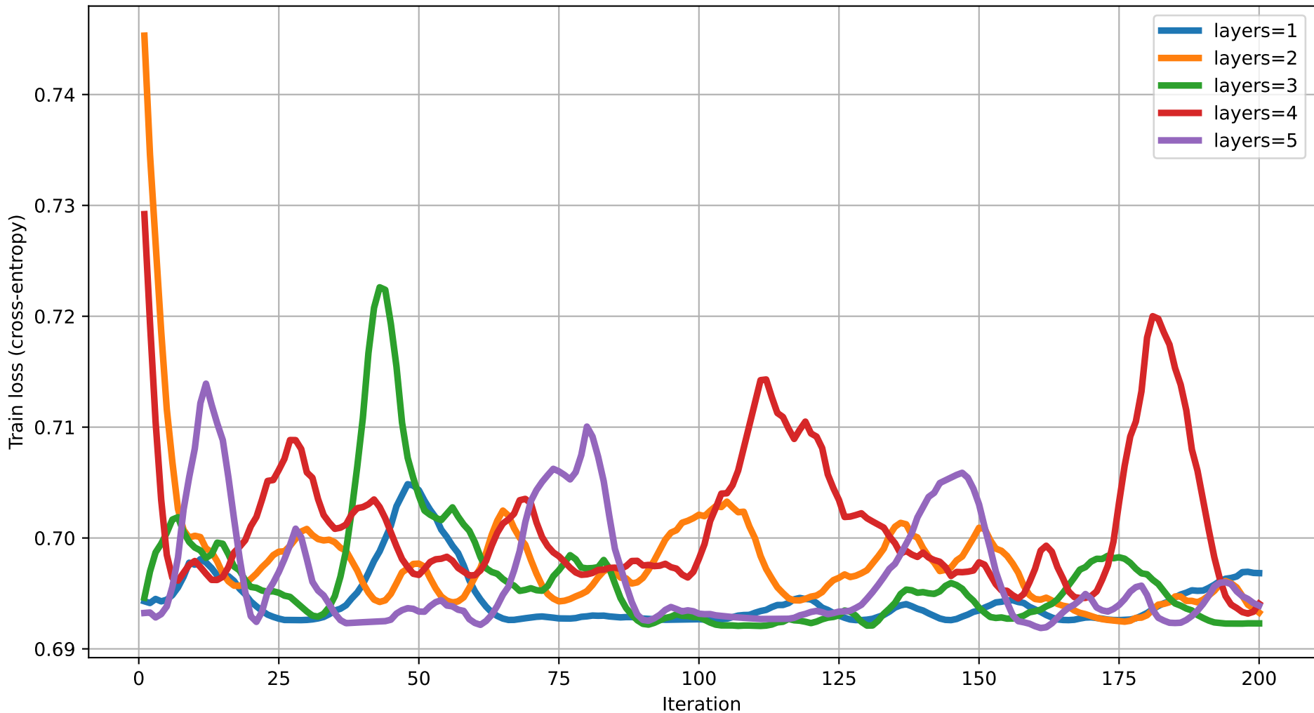
Train loss vs Iteration (dim=19) rot=RY, ent=pairwise, gate=IsingXX
