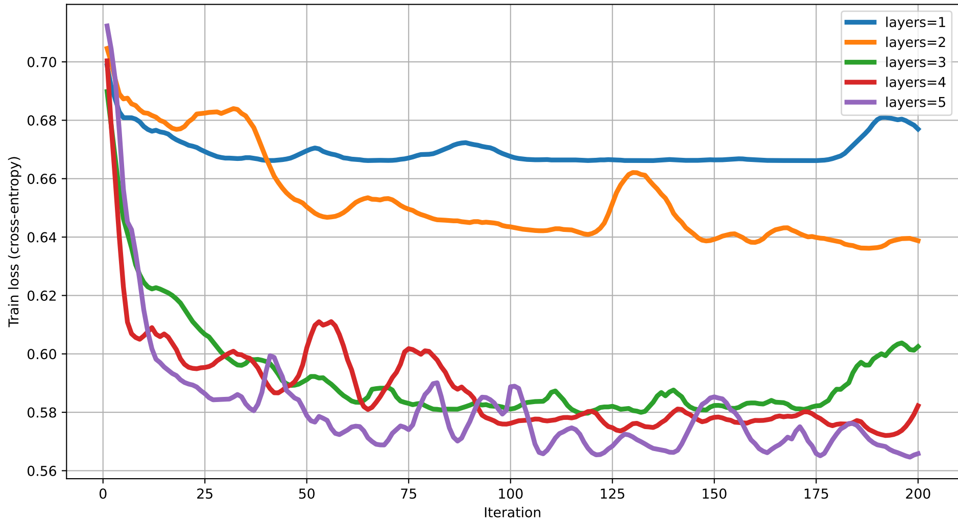
Train loss vs Iteration (dim=10) rot=RYZ, ent=full, gate=CNOT
