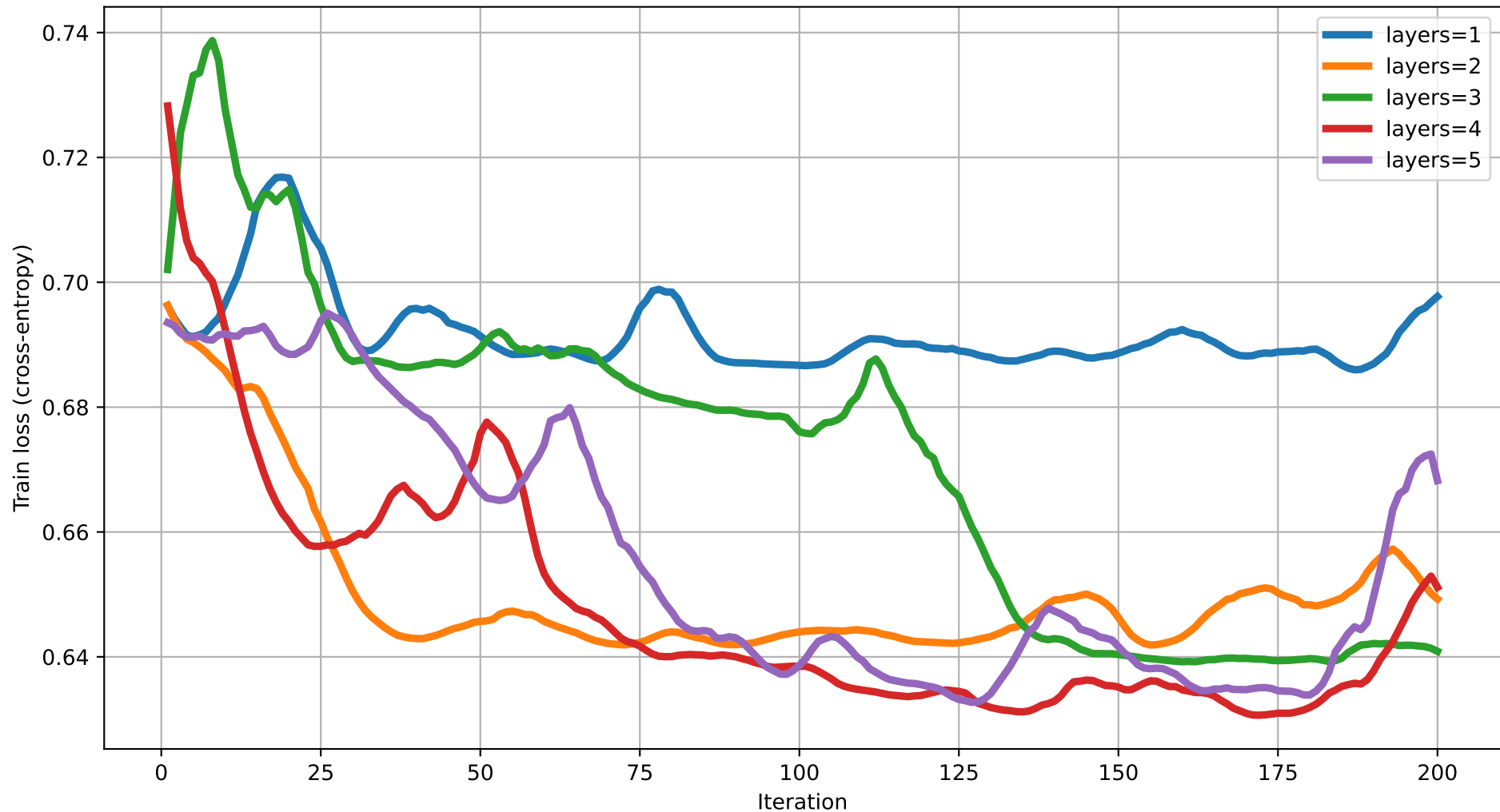
Train loss vs Iteration (dim=6) rot=RZ, ent=chain, gate=IsingXX
