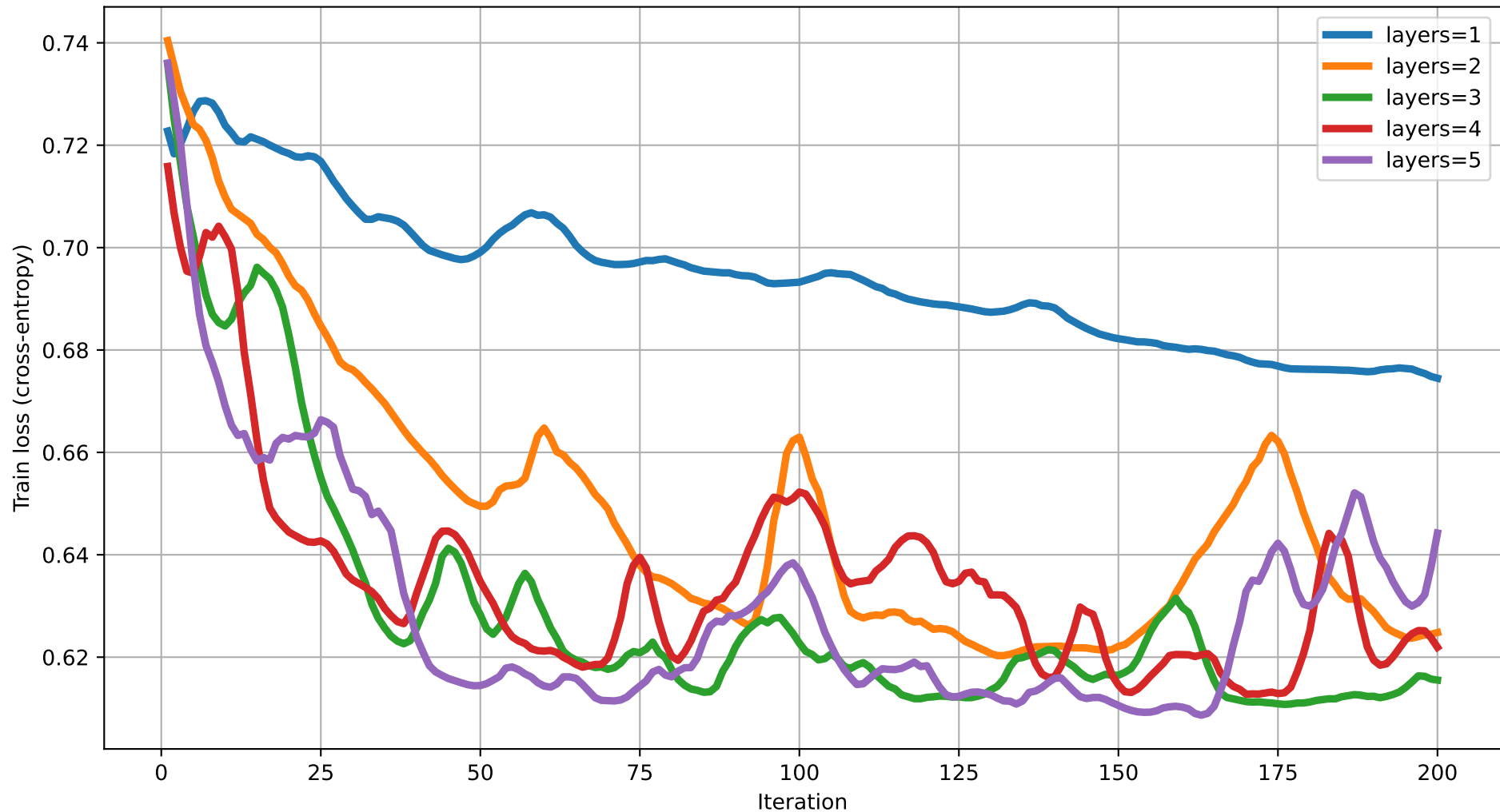
Train loss vs Iteration (dim=6) rot=Rot, ent=full, gate=CNOT
