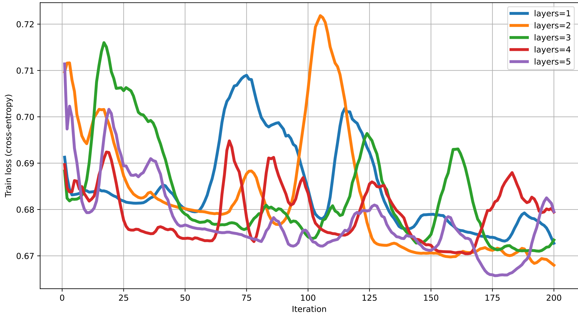
Train loss vs Iteration (dim=13) rot=RYZ, ent=pairwise, gate=CZ
