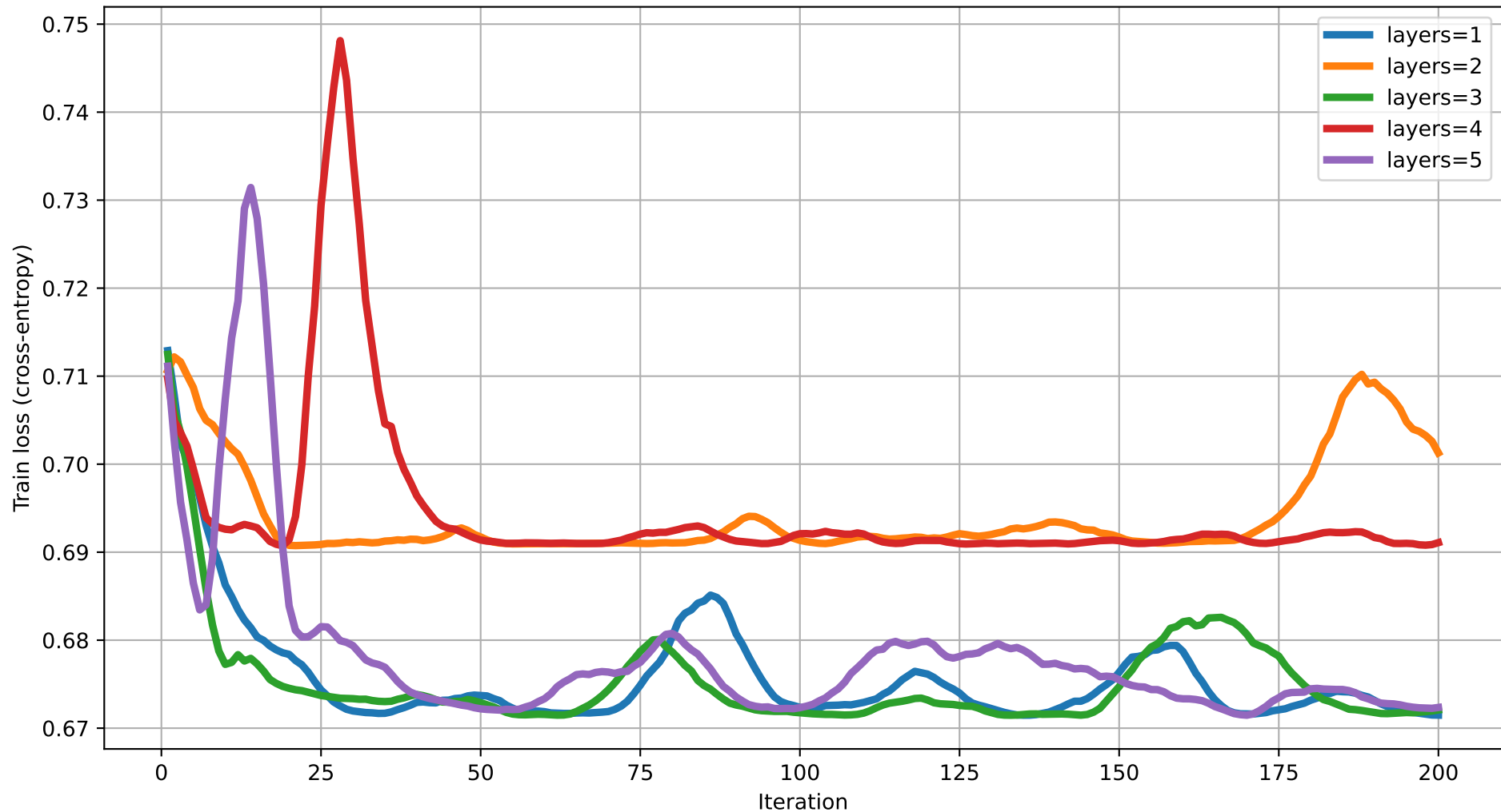
Train loss vs Iteration (dim=20) rot=RX, ent=ring, gate=IsingXX
