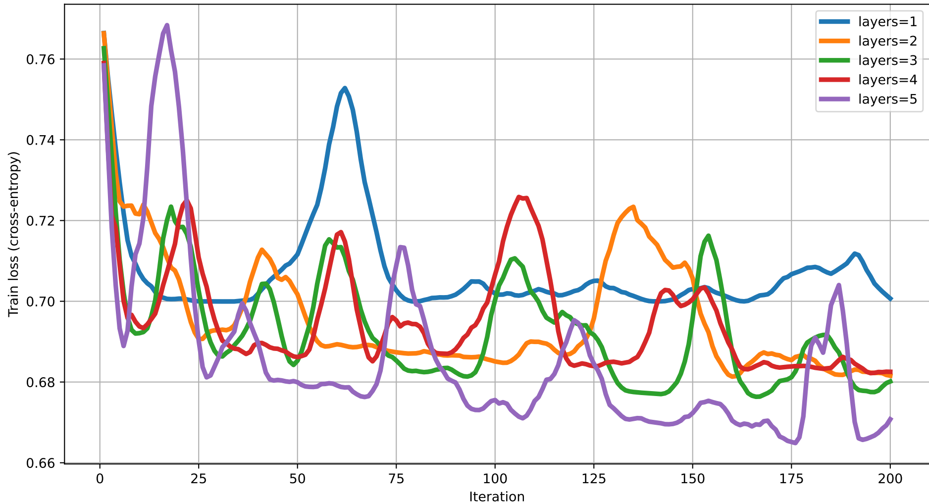
Train loss vs Iteration (dim=17) rot=RYZ, ent=chain, gate=CZ
