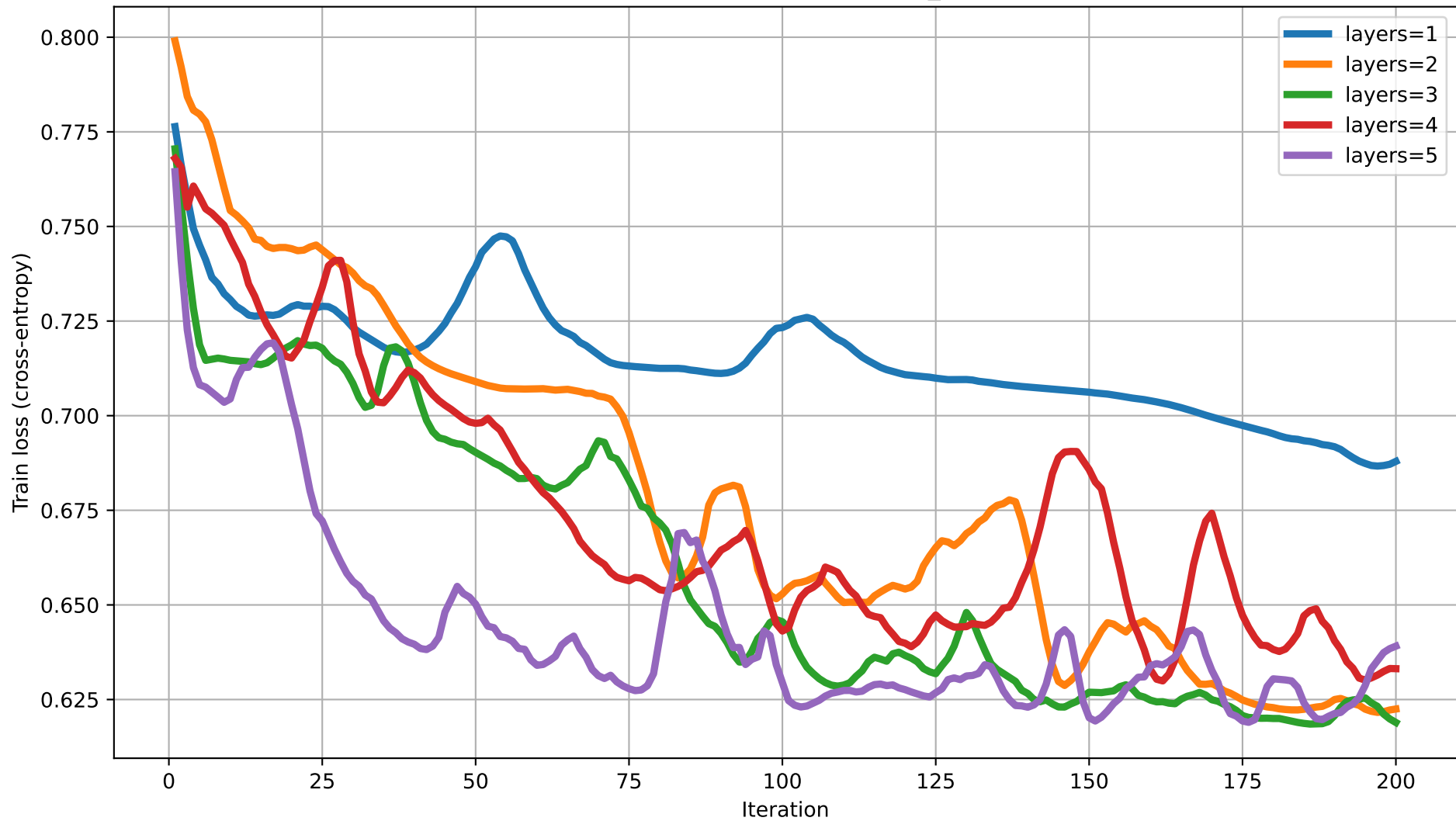
Train loss vs Iteration for different num_layers (dim=4)
