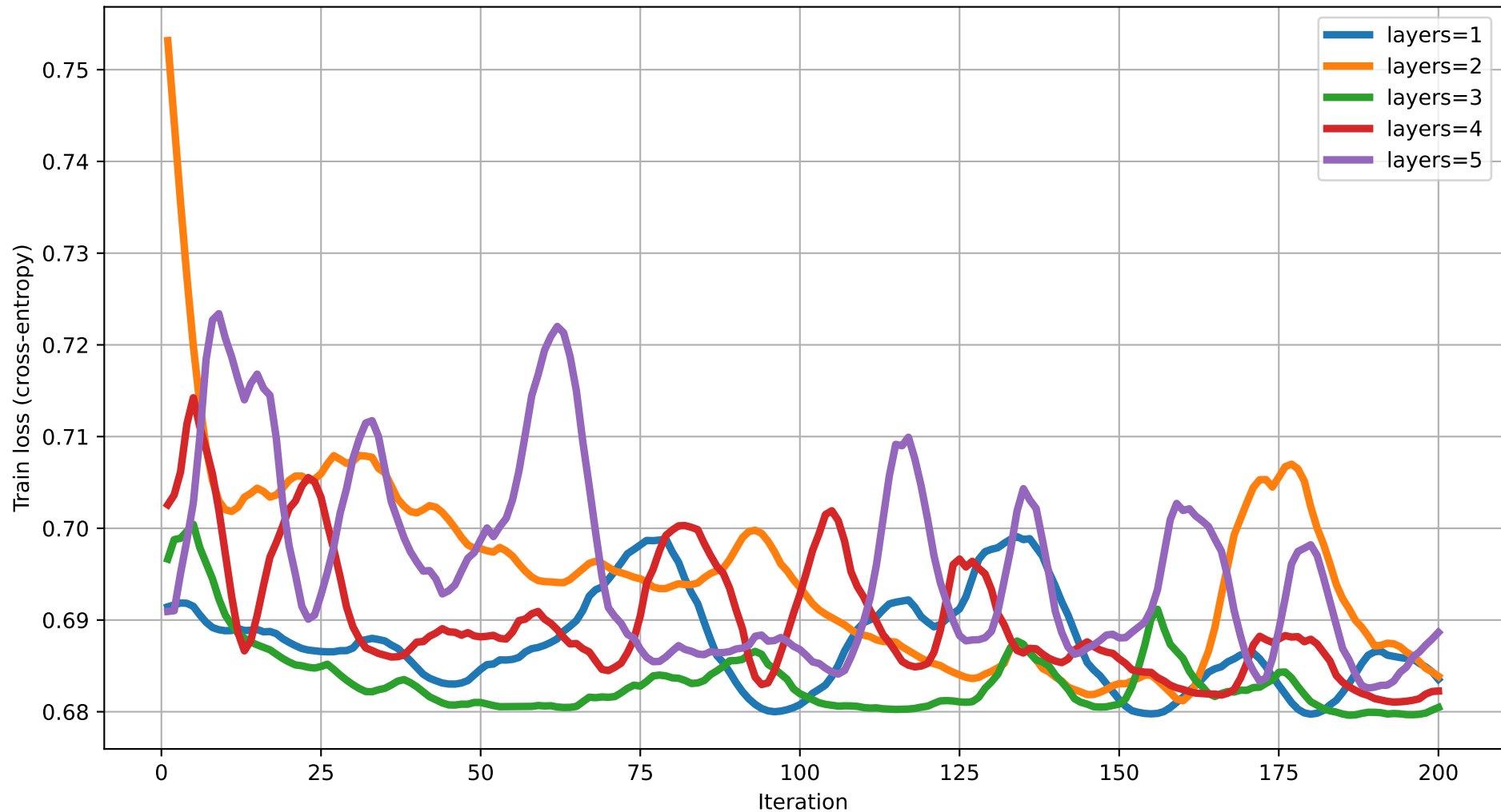
Train loss vs Iteration (dim=20) rot=RZ, ent=pairwise, gate=IsingXX
