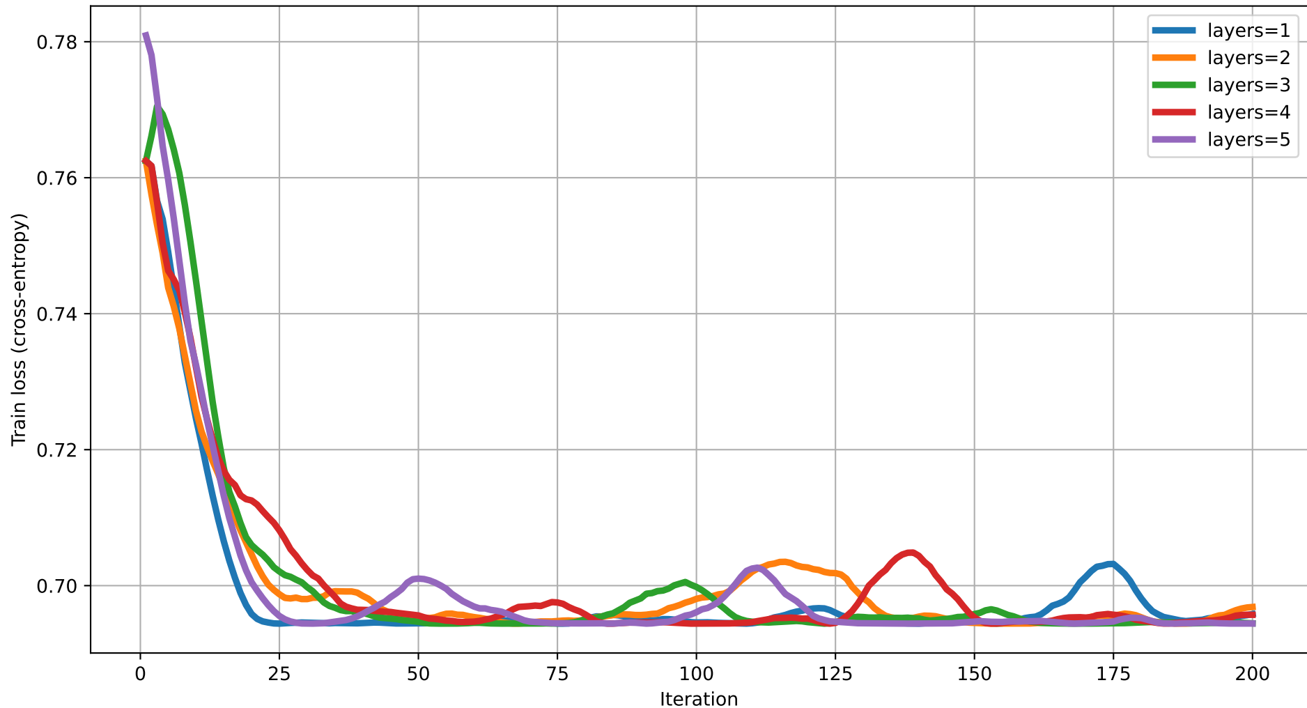
Train loss vs Iteration (dim=8) rot=RZ, ent=pairwise, gate=CZ
