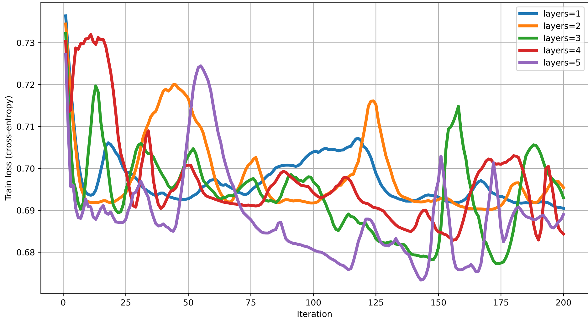
Train loss vs Iteration (dim=16) rot=Rot, ent=chain, gate=CNOT
