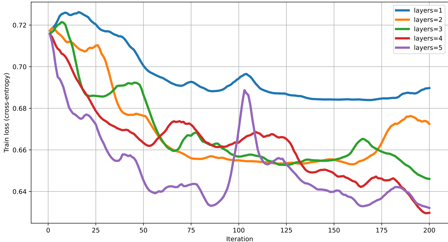
Train loss vs Iteration (dim=7) rot=RX, ent=ring, gate=CZ
