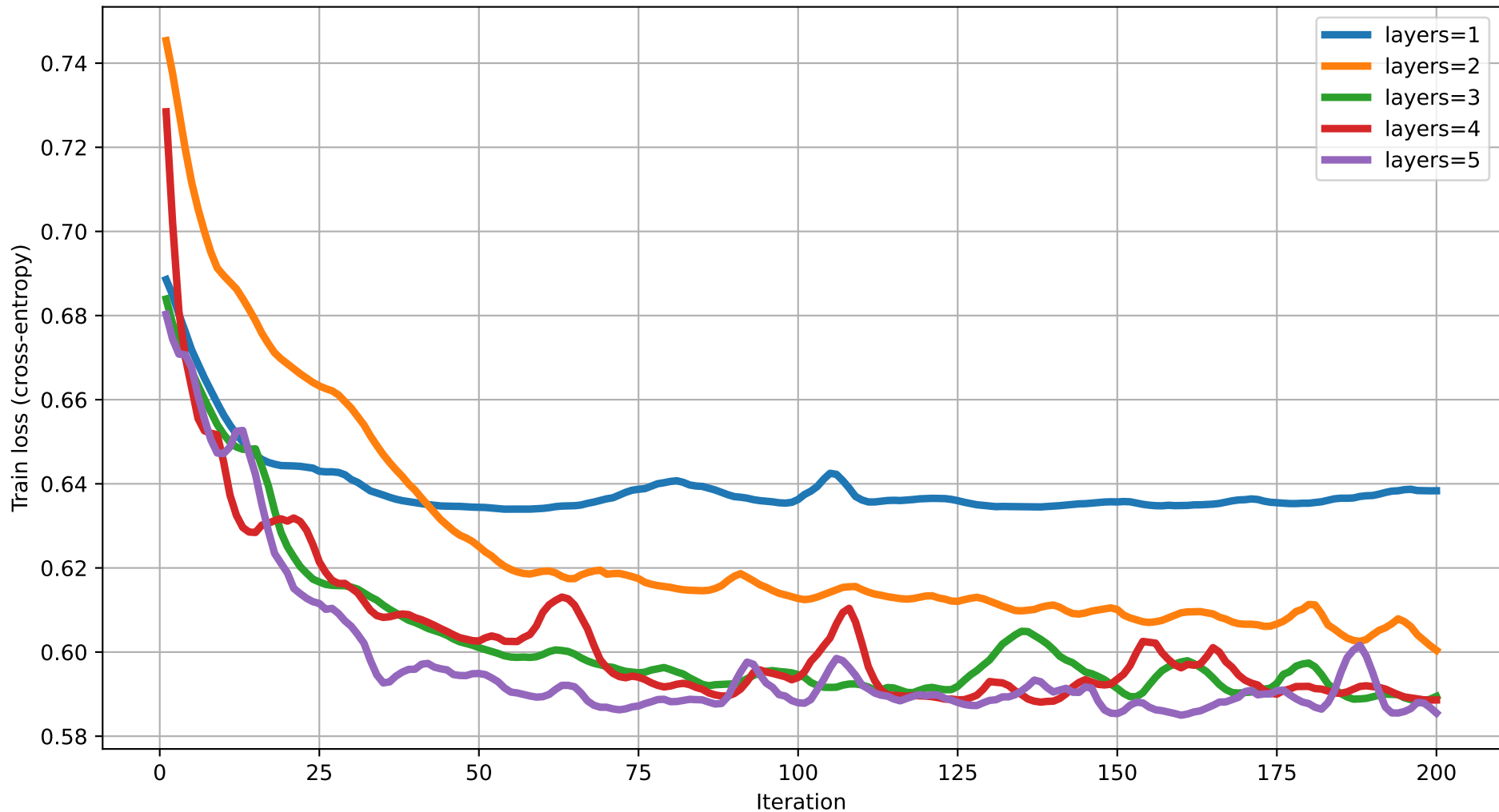
Train loss vs Iteration (degree=5) rot=RYZ, ent=full, gate=IsingXX
