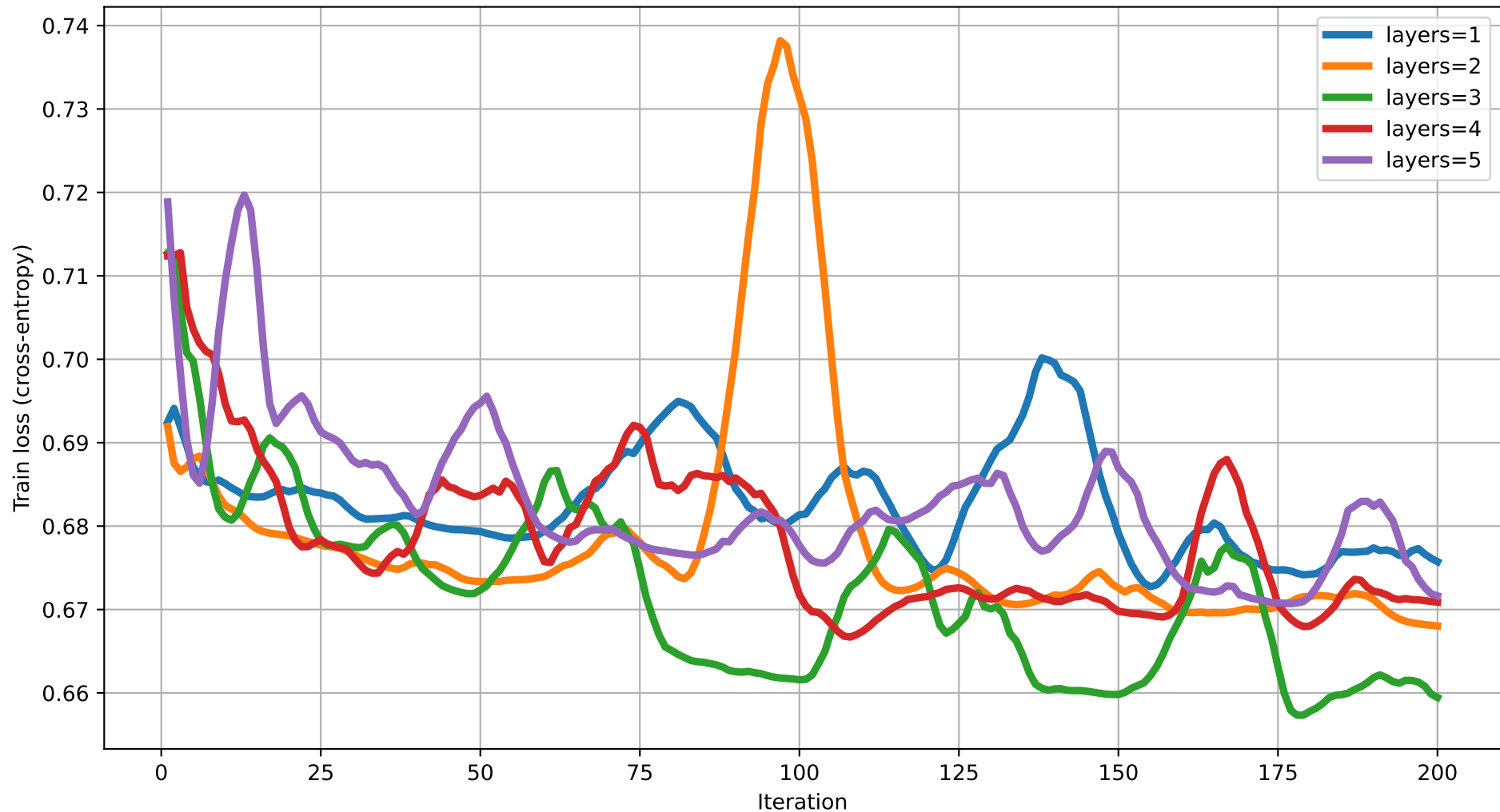
Train loss vs Iteration (dim=13) rot=RY, ent=full, gate=CZ
