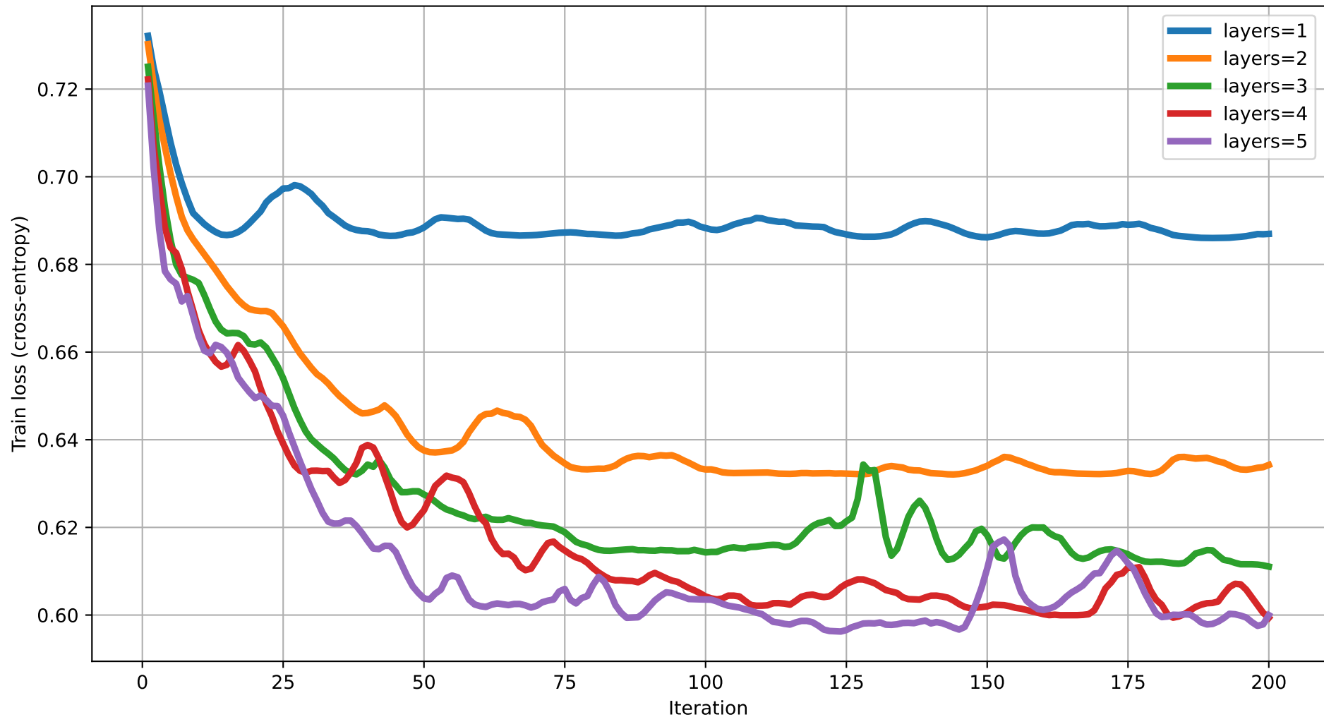
Train loss vs Iteration (degree=2) rot=Rot, ent=chain, gate=CNOT
