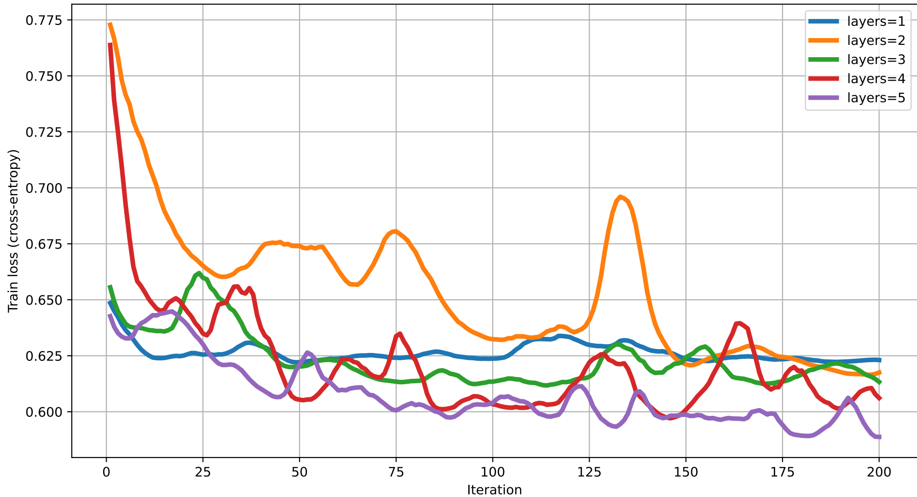
Train loss vs Iteration (dim=9) rot=RYZ, ent=ring, gate=IsingXX
