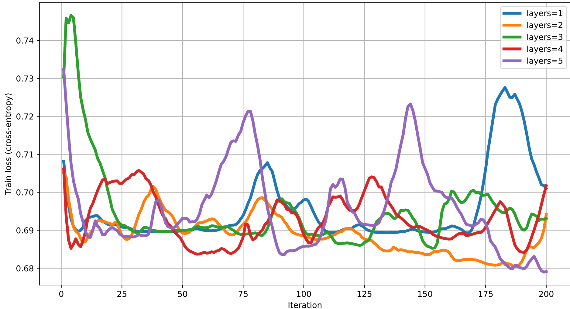
Train loss vs Iteration (dim=20) rot=Rot, ent=full, gate=CNOT
