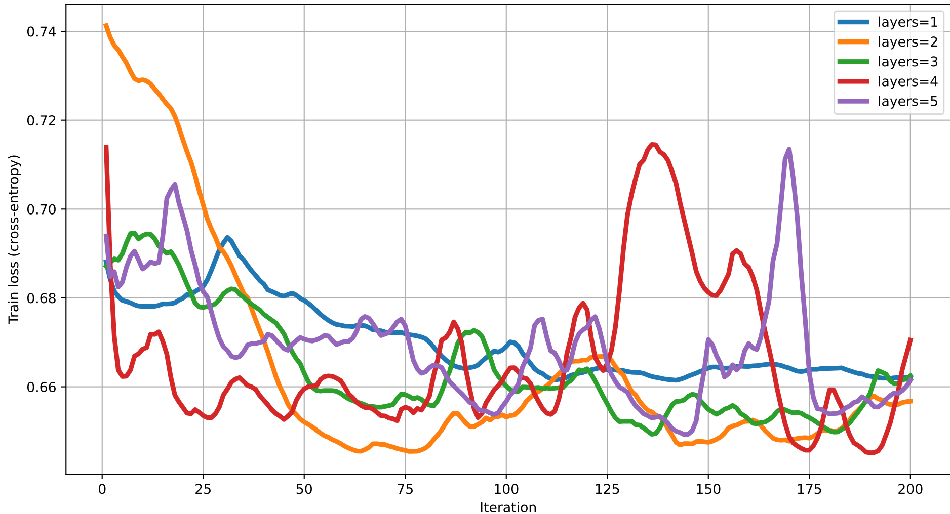
Train loss vs Iteration (dim=5) rot=Rot, ent=pairwise, gate=IsingXX
