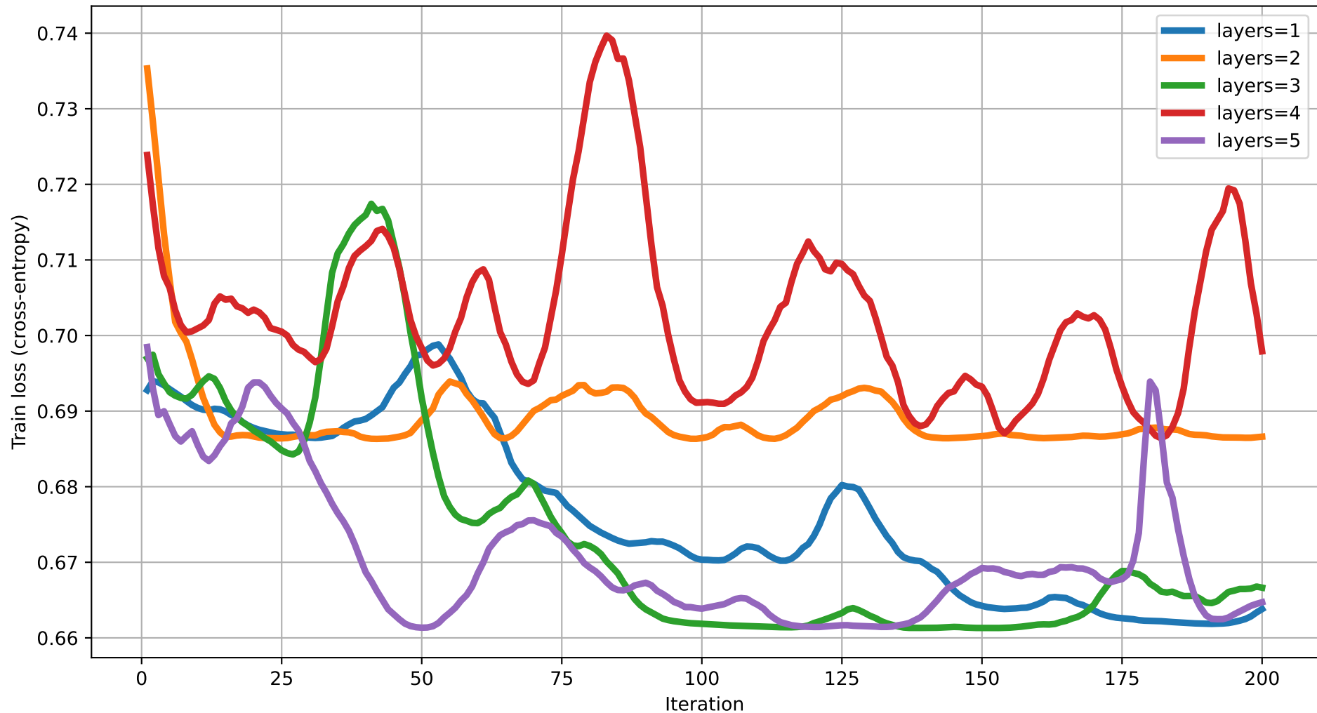
Train loss vs Iteration (dim=10) rot=RX, ent=full, gate=IsingXX
