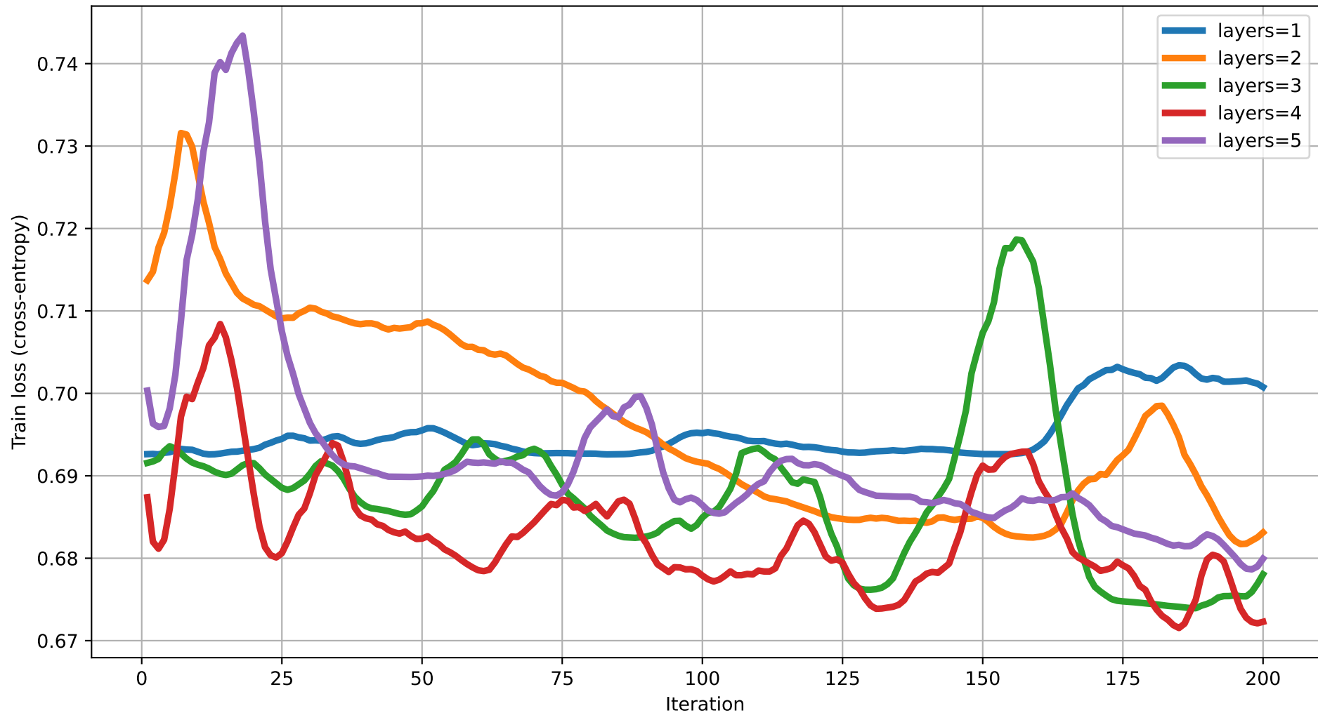
Train loss vs Iteration (dim=13) rot=RY, ent=chain, gate=IsingXX
