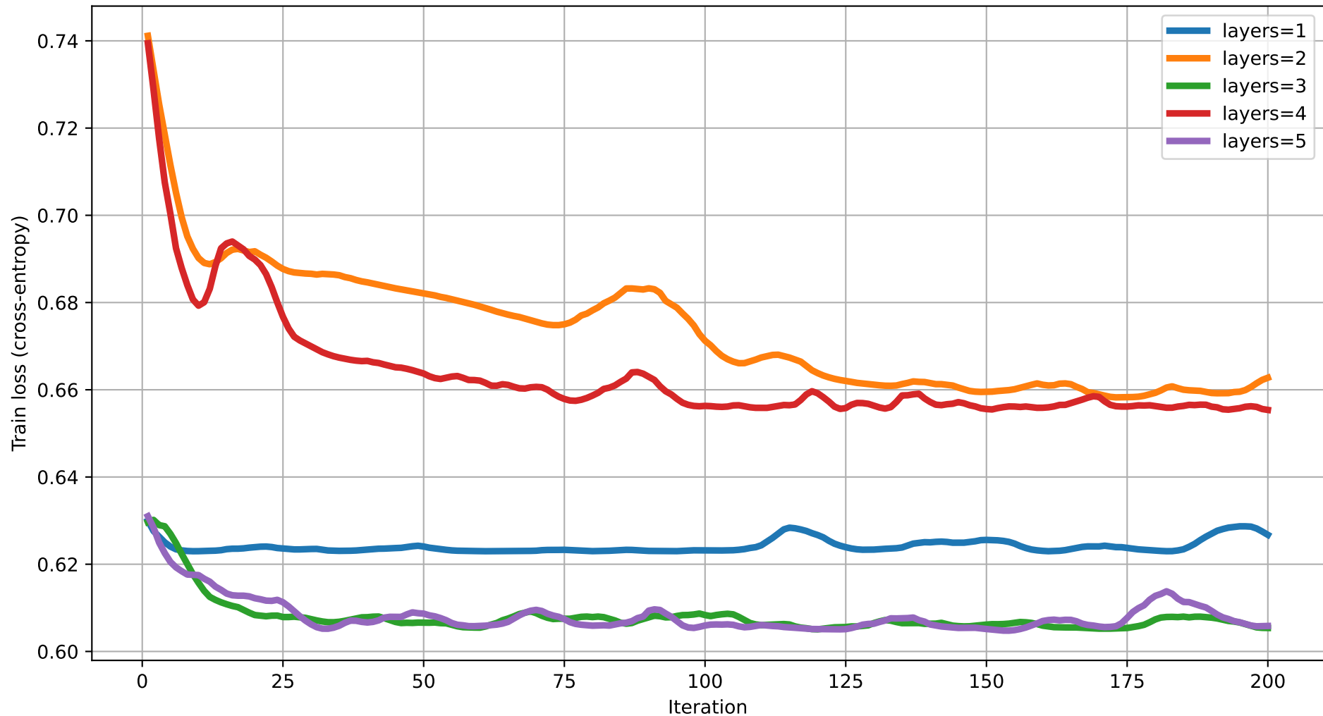
Train loss vs Iteration (degree=5) rot=RZ, ent=ring, gate=IsingXX
