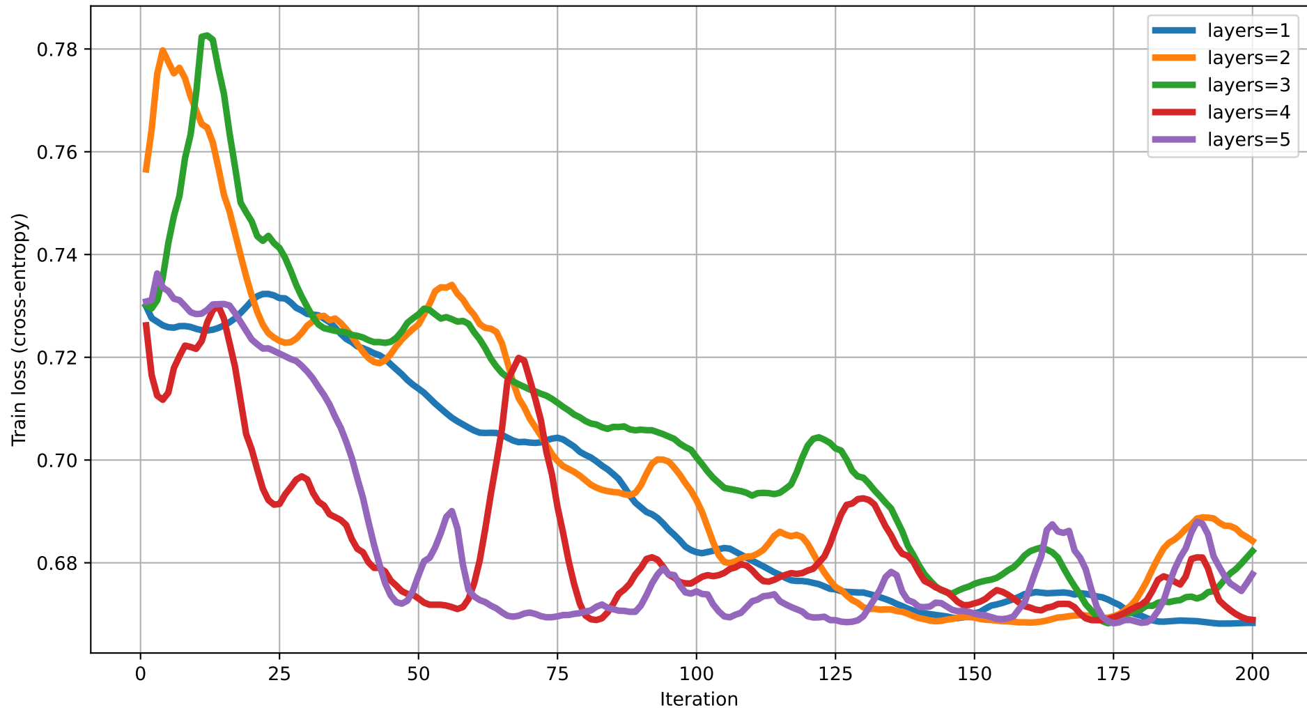
Train loss vs Iteration (dim=3) rot=RYZ, ent=ring, gate=IsingXX
