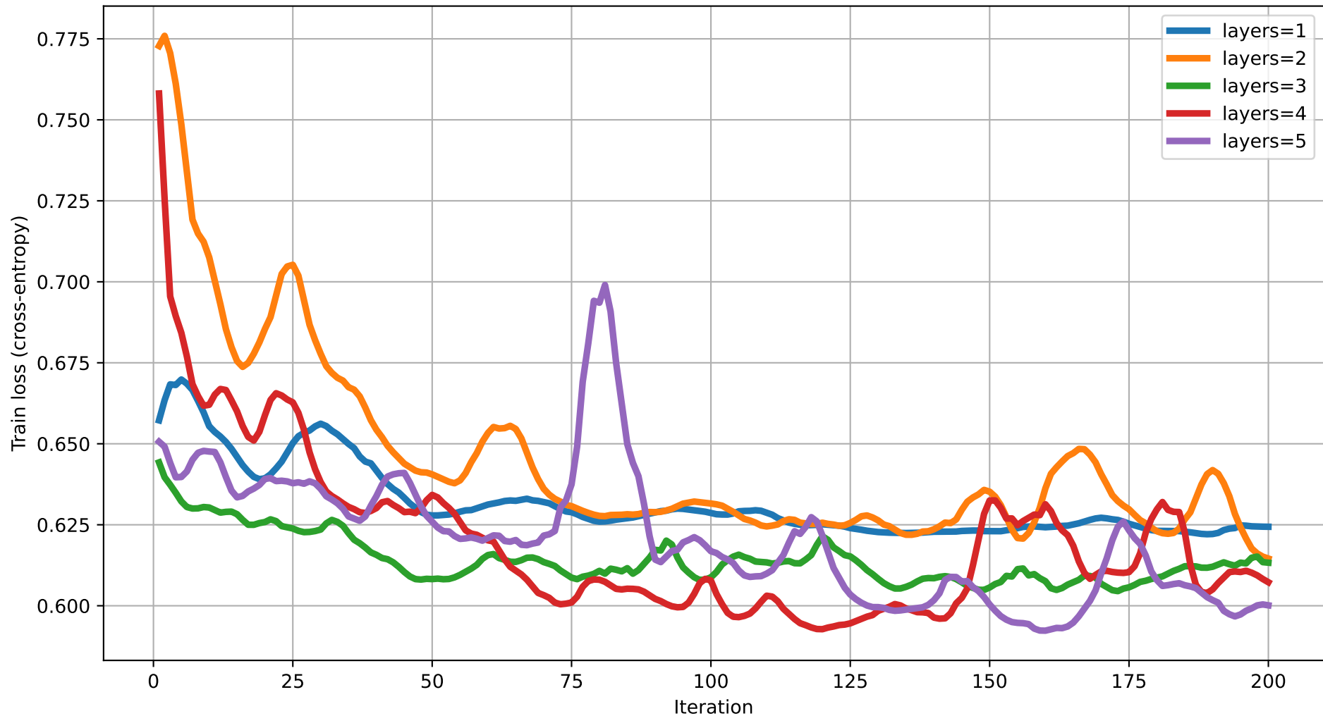
Train loss vs Iteration (dim=9) rot=Rot, ent=ring, gate=IsingXX
