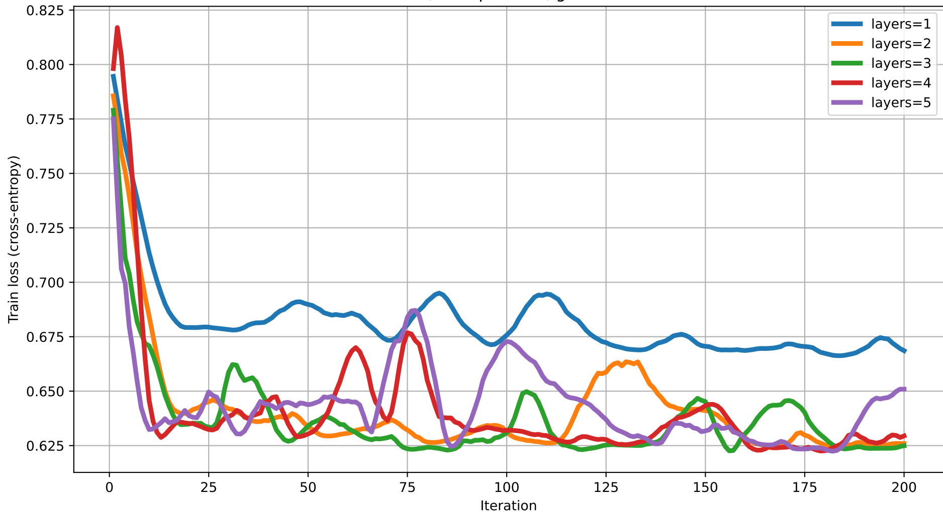
Train loss vs Iteration (dim=4) rot=Rot, ent=pairwise, gate=CNOT
