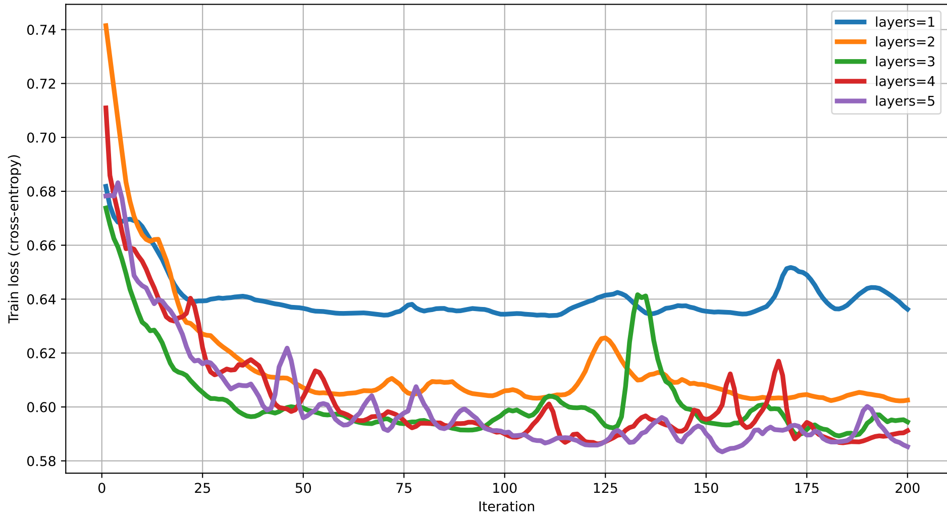
Train loss vs Iteration (degree=5) rot=Rot, ent=full, gate=IsingXX
