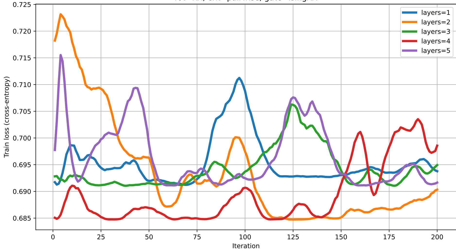
Train loss vs Iteration (dim=15) rot=RX, ent=pairwise, gate=IsingXX
