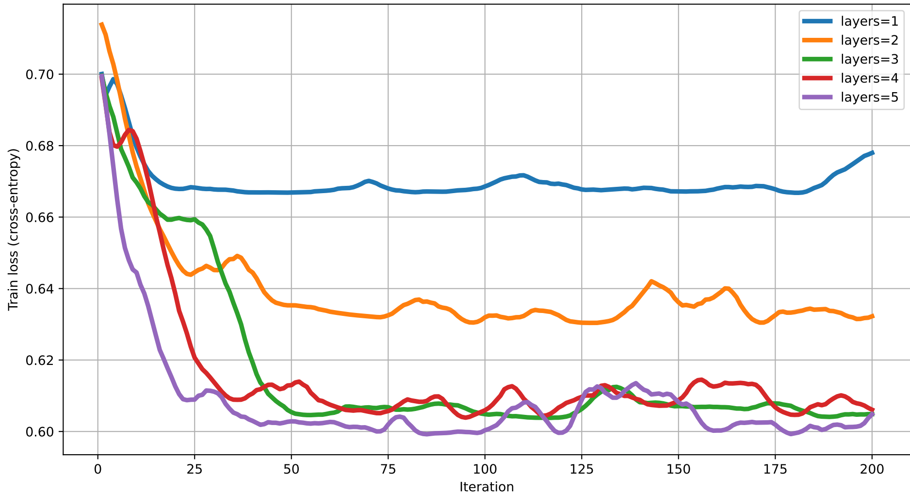
Train loss vs Iteration (dim=10) rot=RX, ent=chain, gate=CZ
