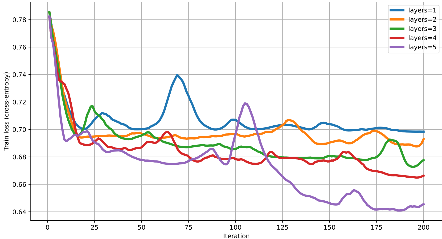
Train loss vs Iteration (dim=9) rot=RX, ent=full, gate=CZ
