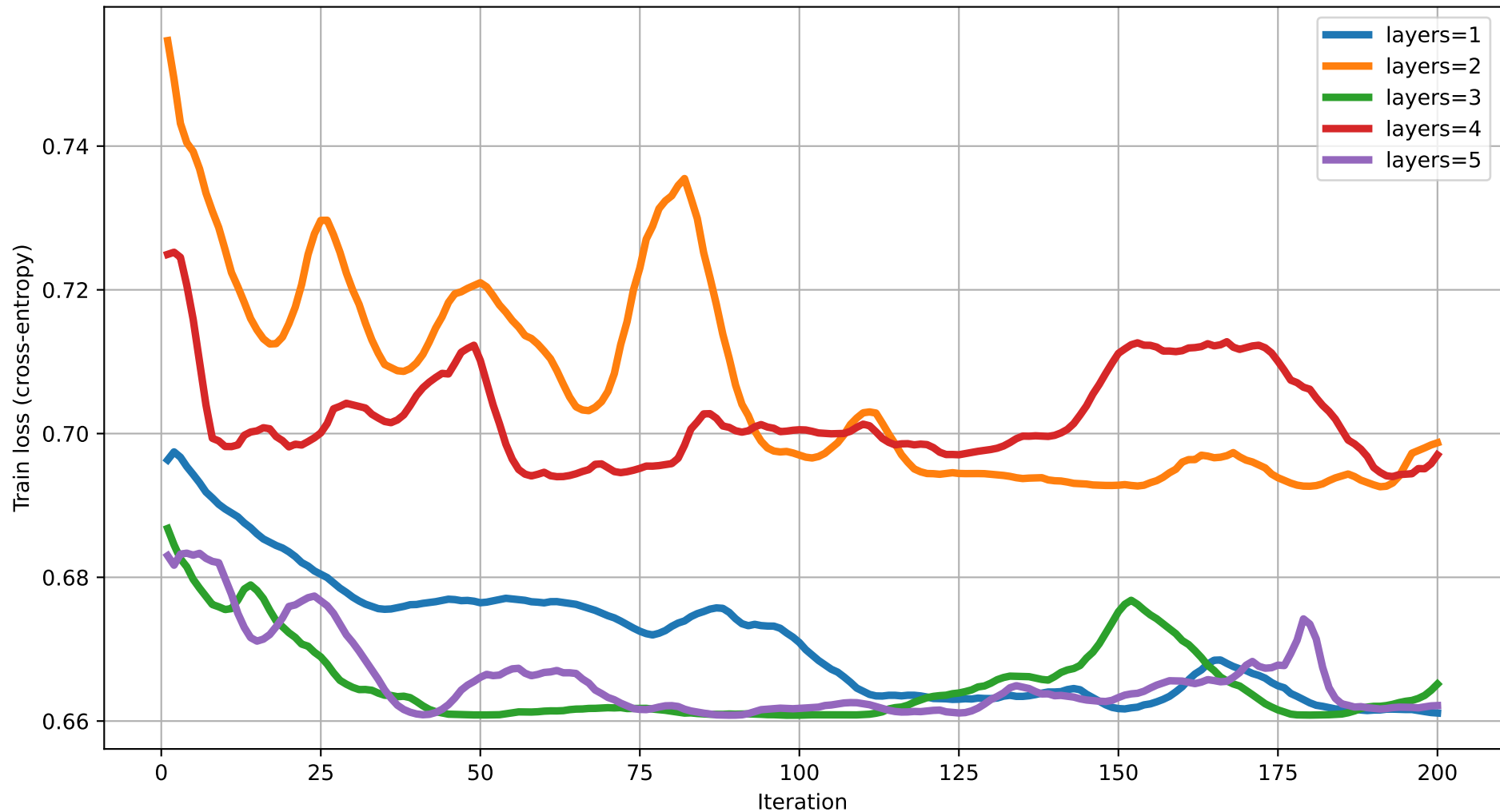
Train loss vs Iteration (dim=5) rot=RX, ent=chain, gate=IsingXX
