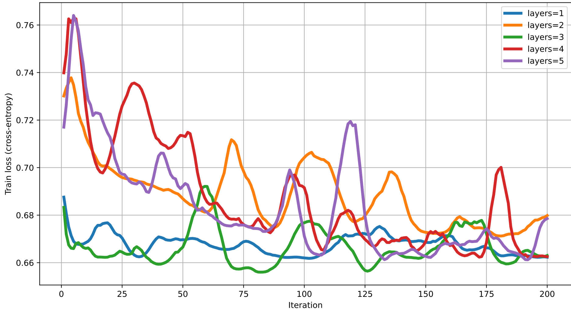
Train loss vs Iteration (dim=11) rot=RY, ent=ring, gate=IsingXX
