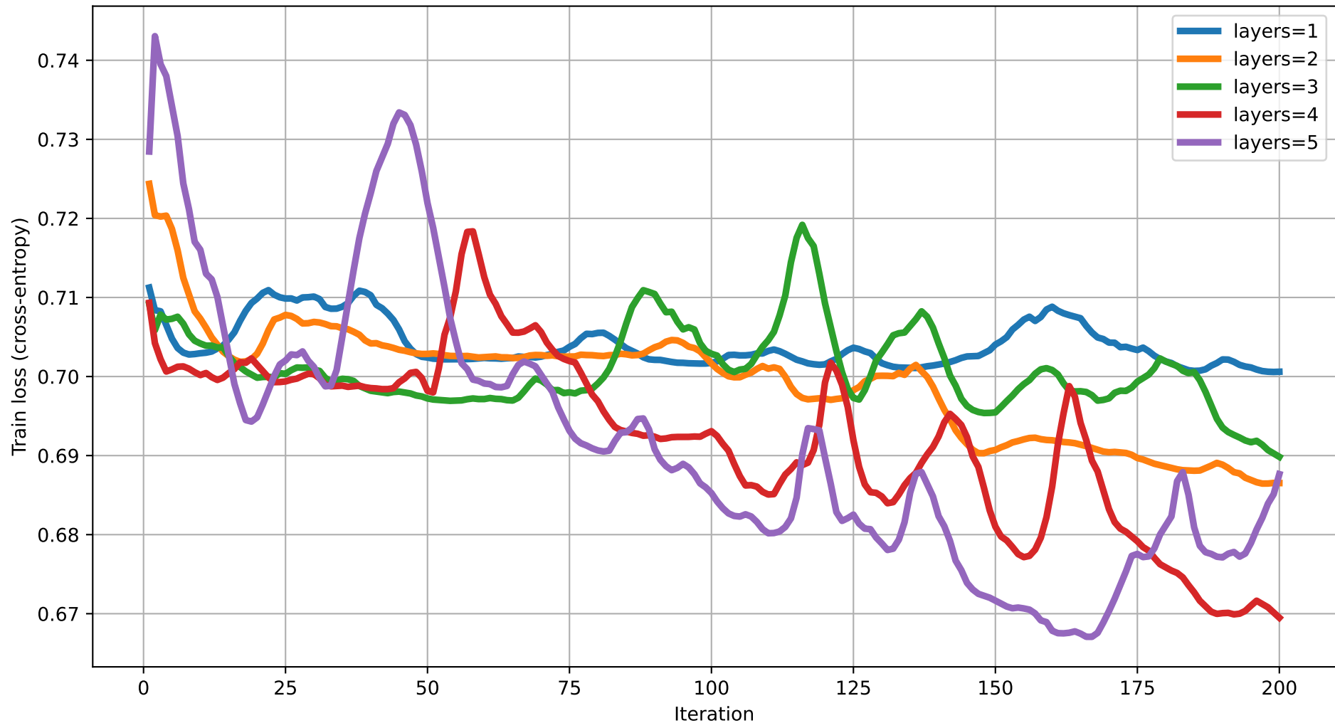
Train loss vs Iteration (dim=11) rot=Rot, ent=ring, gate=CZ
