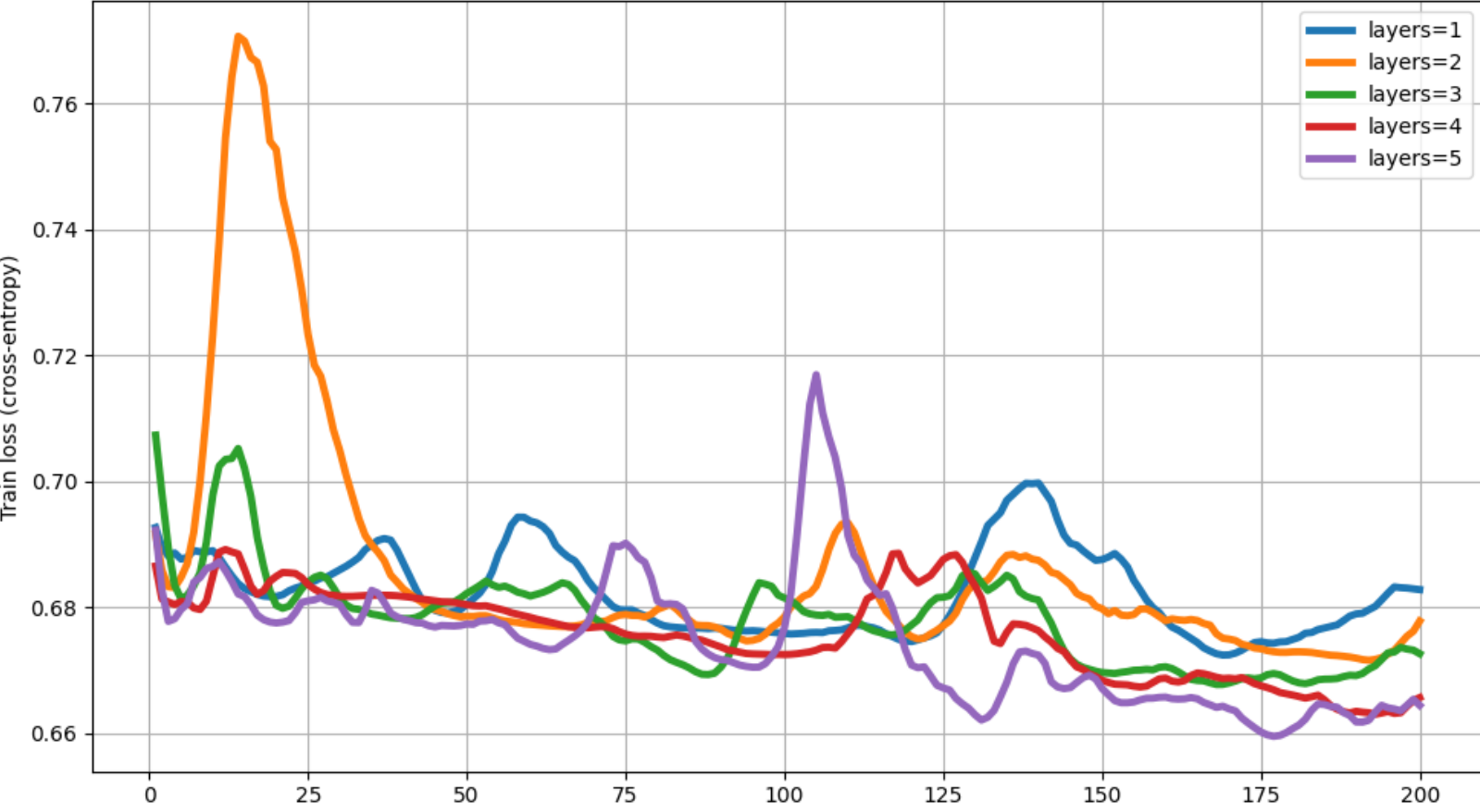
Train loss vs Iteration for different num_layers (dim=13)
