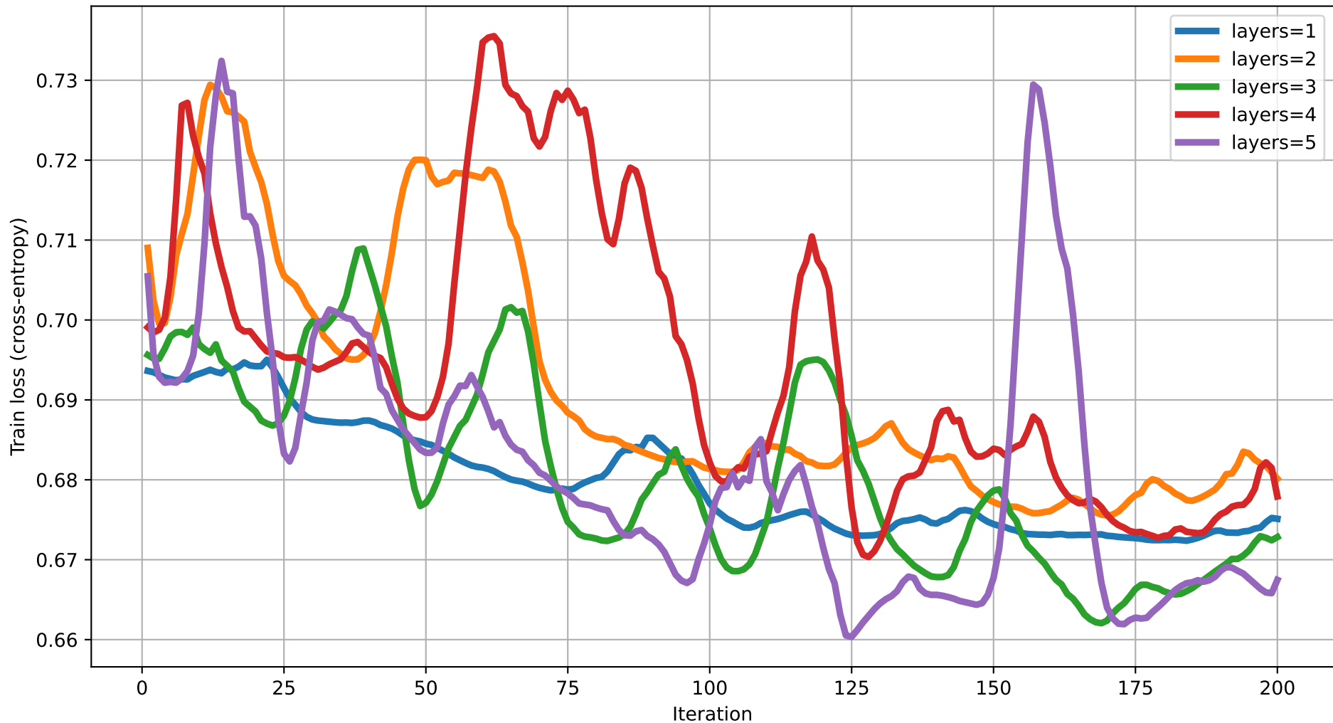
Train loss vs Iteration (dim=12) rot=RYZ, ent=chain, gate=IsingXX
