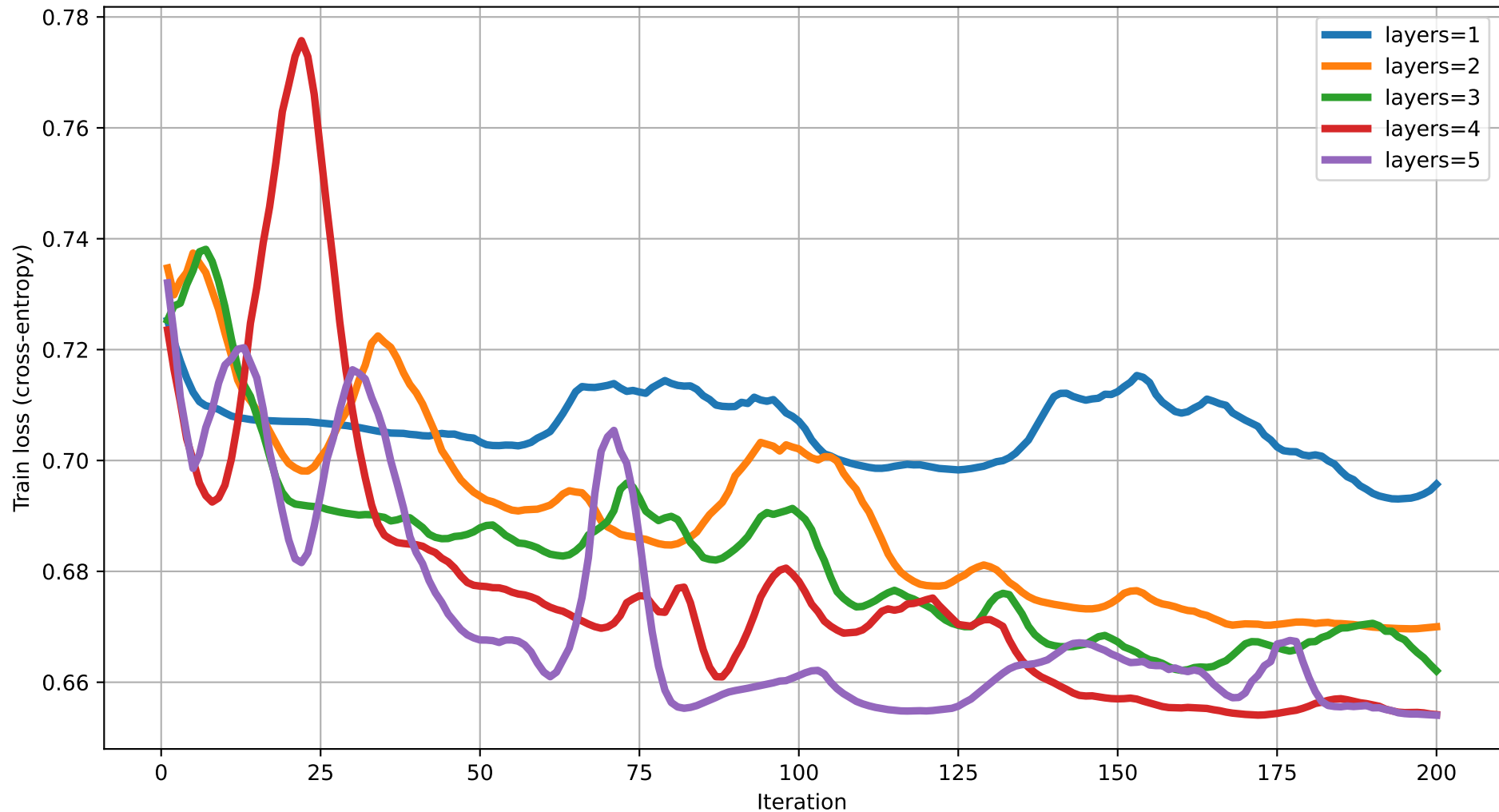
Train loss vs Iteration (dim=10) rot=RX, ent=chain, gate=CNOT
