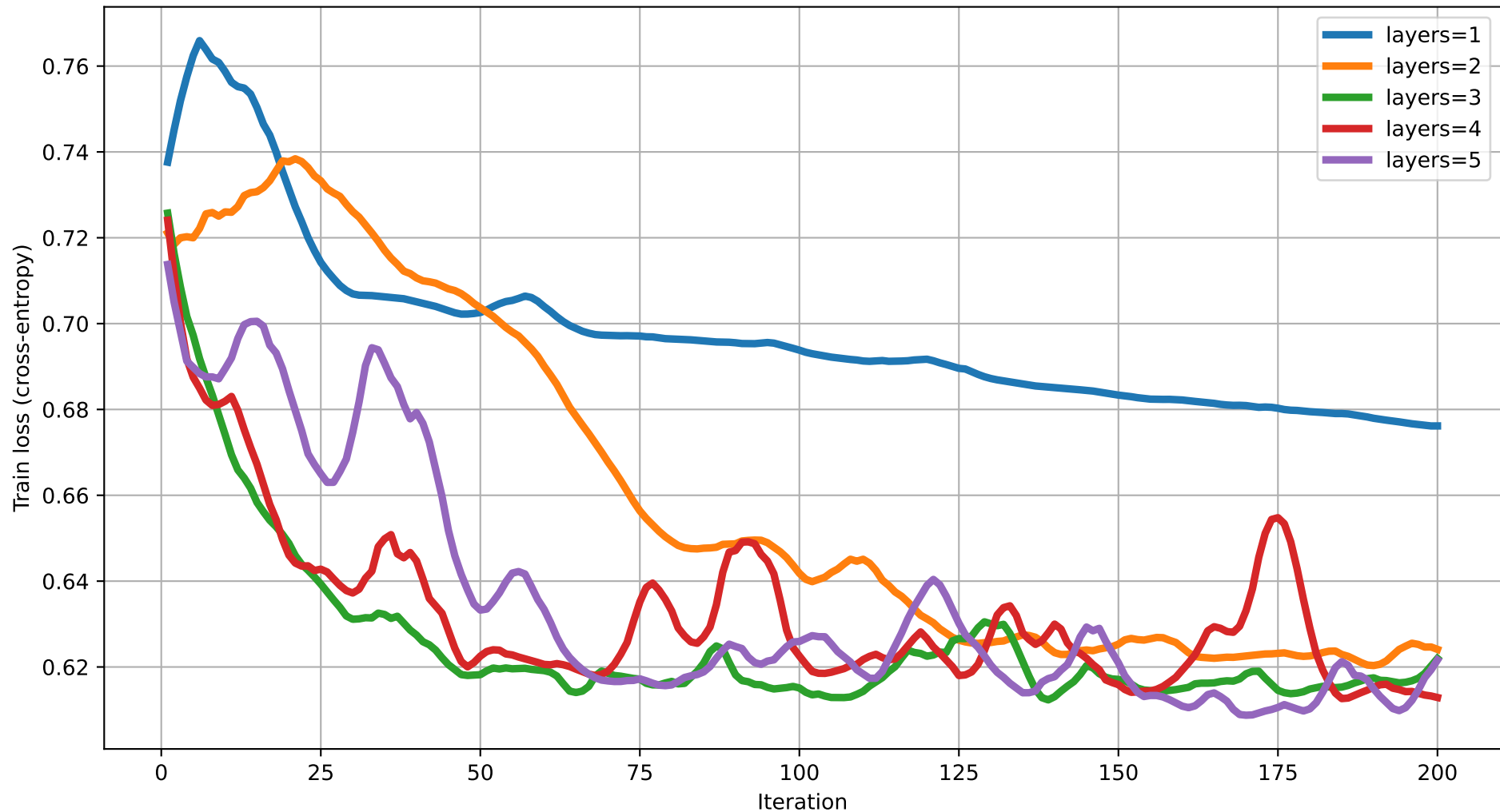
Train loss vs Iteration (dim=6) rot=RYZ, ent=full, gate=CNOT
