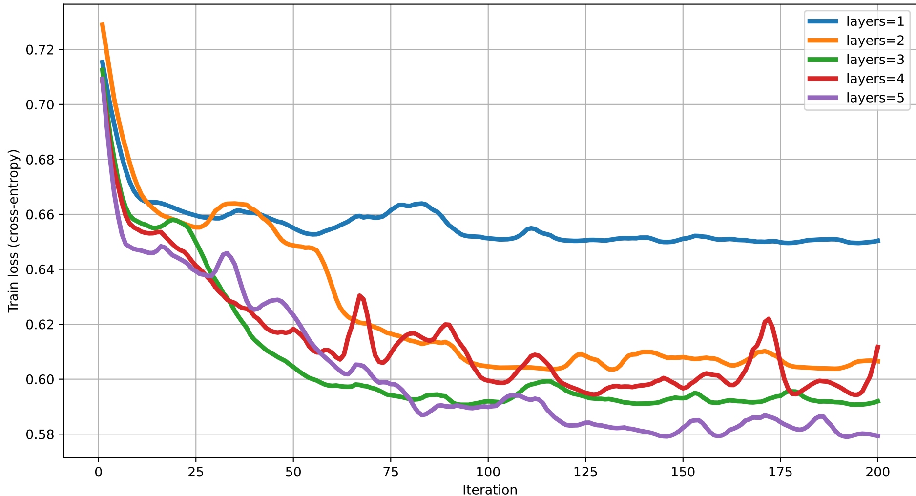
Train loss vs Iteration (degree=4) rot=RY, ent=full, gate=CZ
