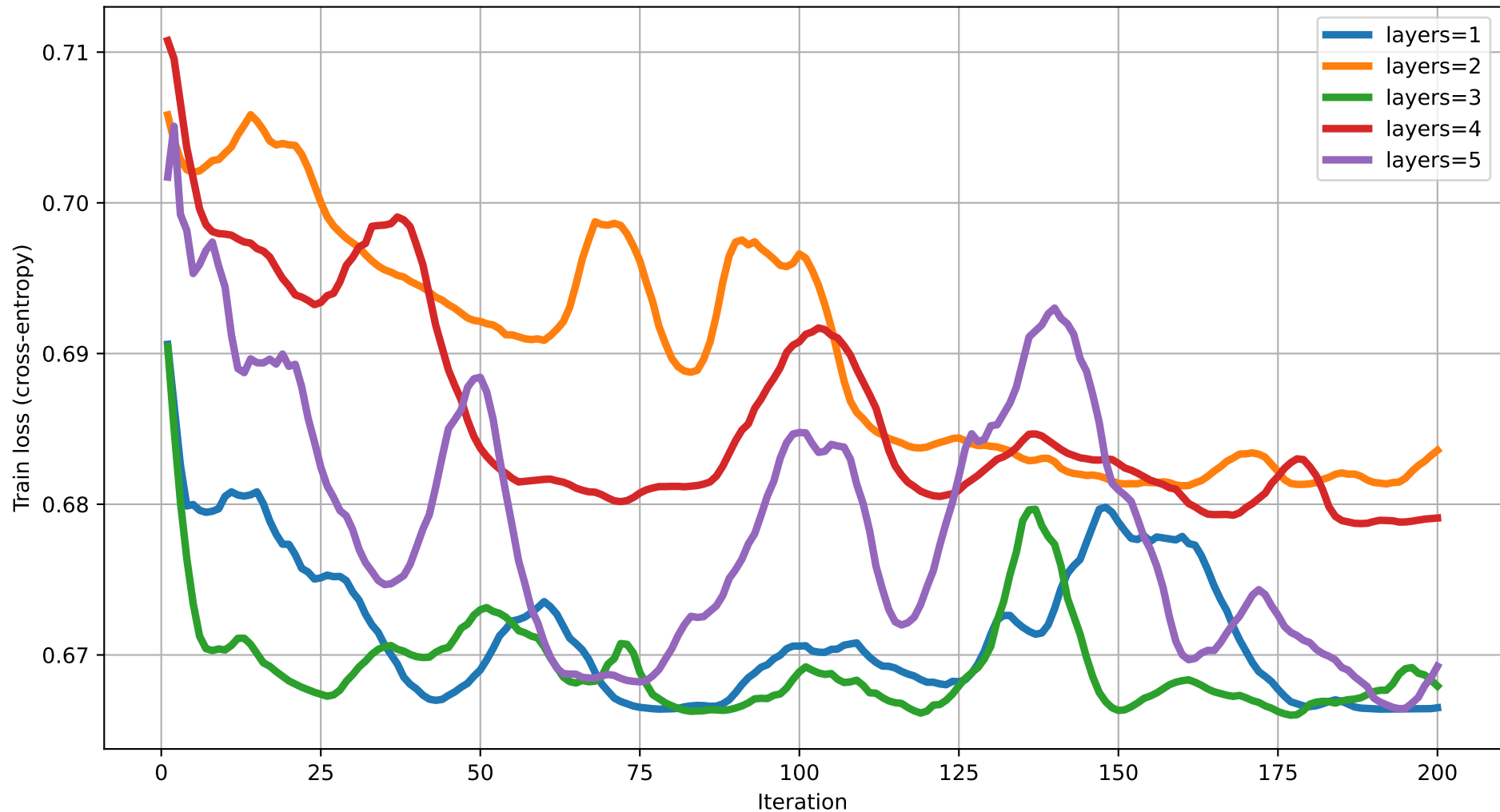
Train loss vs Iteration (dim=12) rot=RZ, ent=ring, gate=IsingXX
