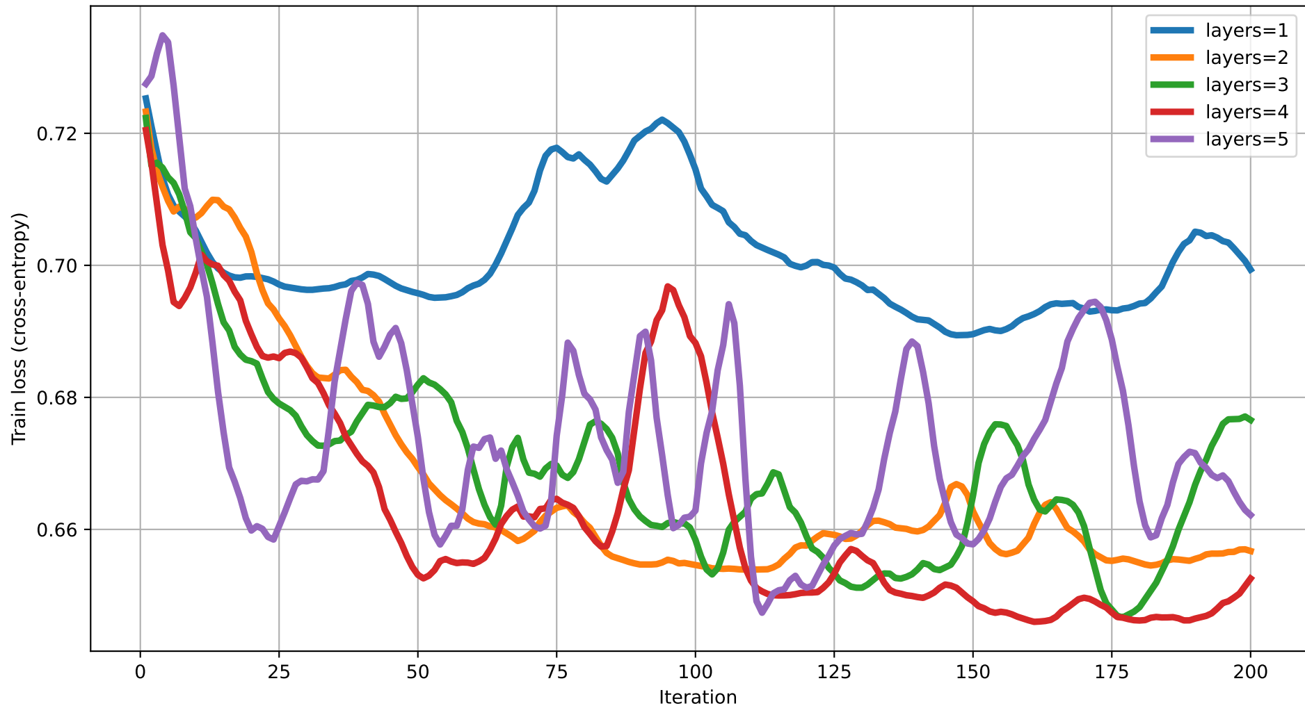
Train loss vs Iteration (dim=5) rot=Rot, ent=ring, gate=CZ
