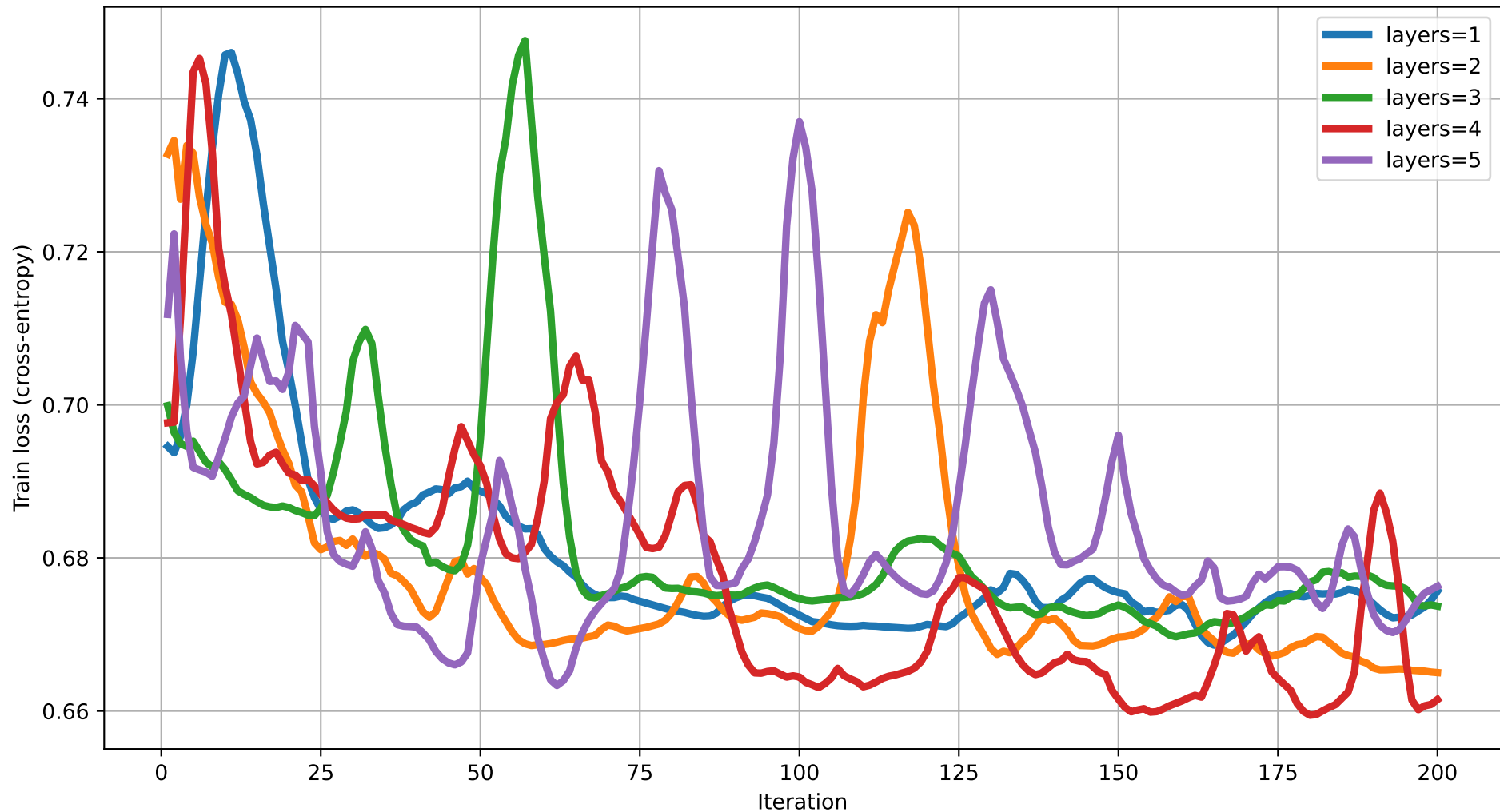
Train loss vs Iteration (dim=11) rot=Rot, ent=chain, gate=IsingXX
