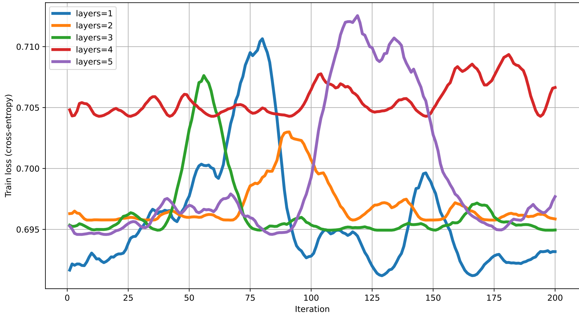
Train loss vs Iteration (dim=20) rot=RZ, ent=ring, gate=CNOT
