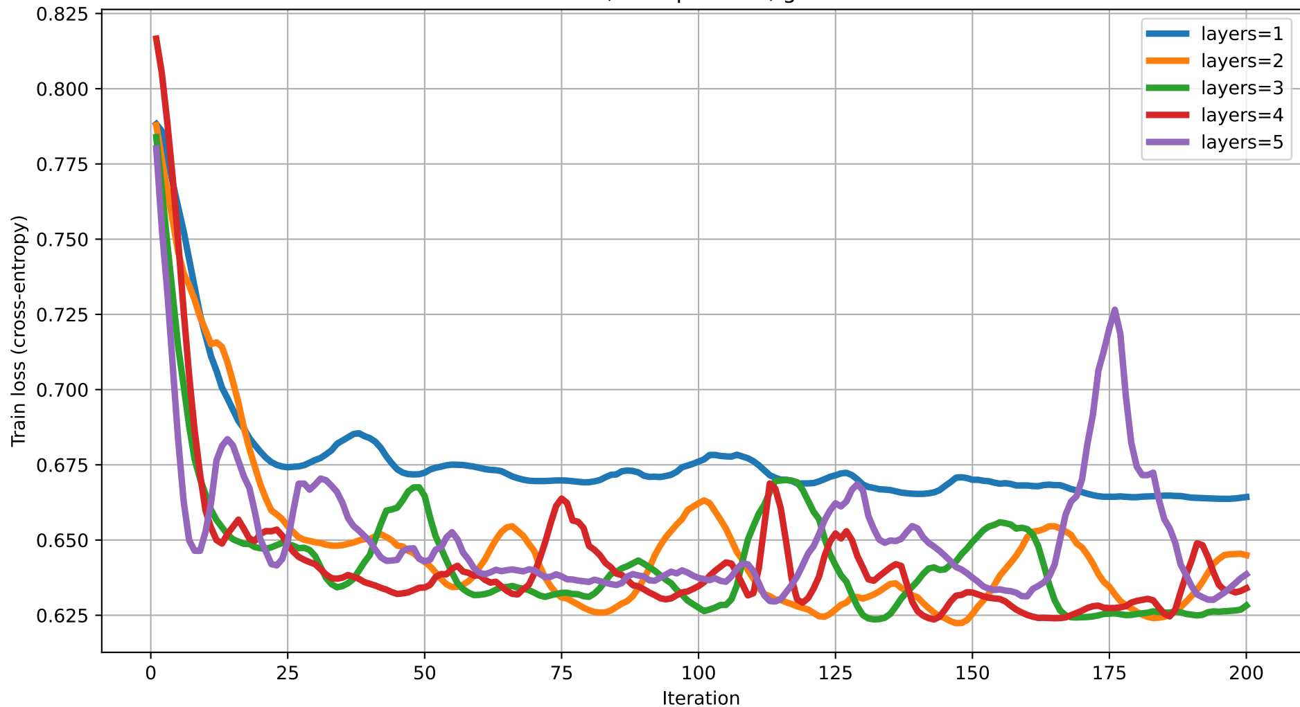
Train loss vs Iteration (dim=4) rot=Rot, ent=pairwise, gate=CZ
