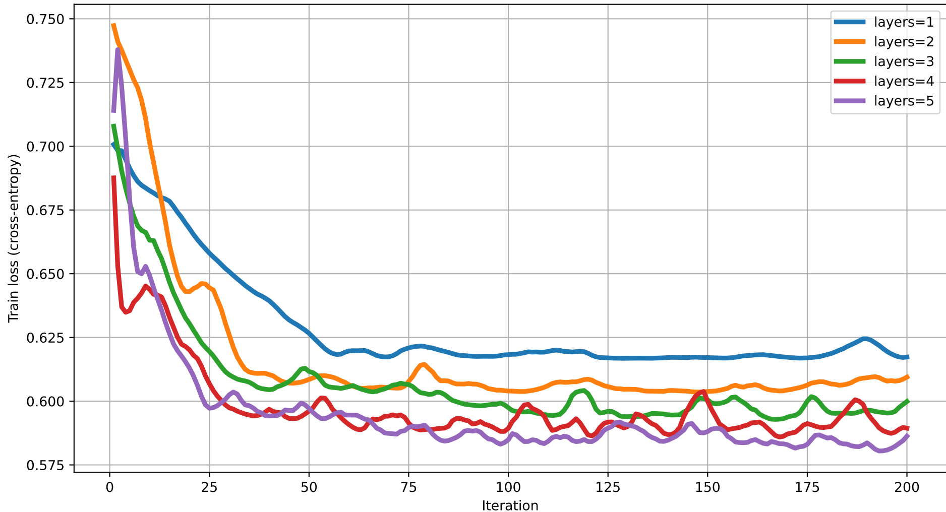
Train loss vs Iteration (degree=3) rot=Rot, ent=chain, gate=IsingXX
