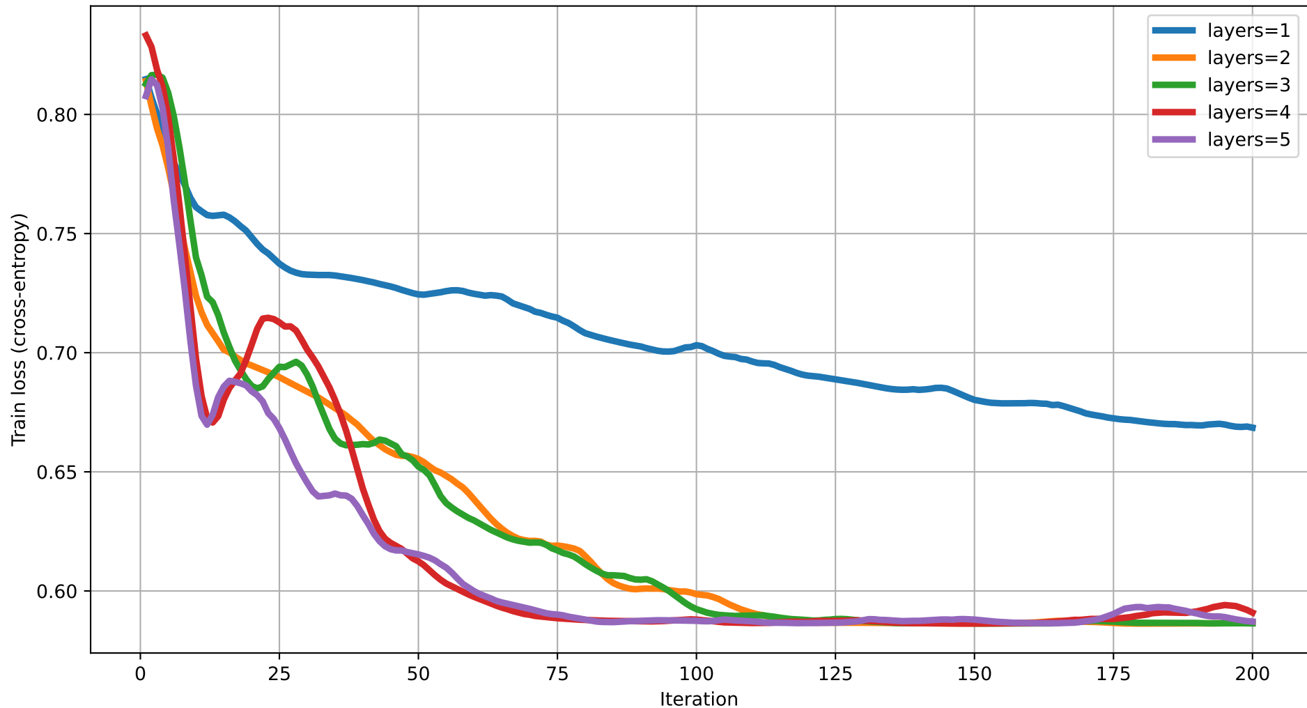
Train loss vs Iteration (dim=2) rot=RX, ent=pairwise, gate=CNOT
