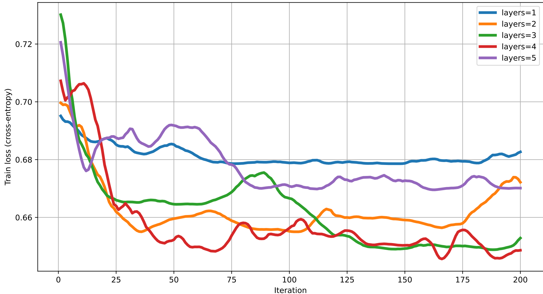
Train loss vs Iteration (dim=7) rot=RX, ent=ring, gate=CNOT
