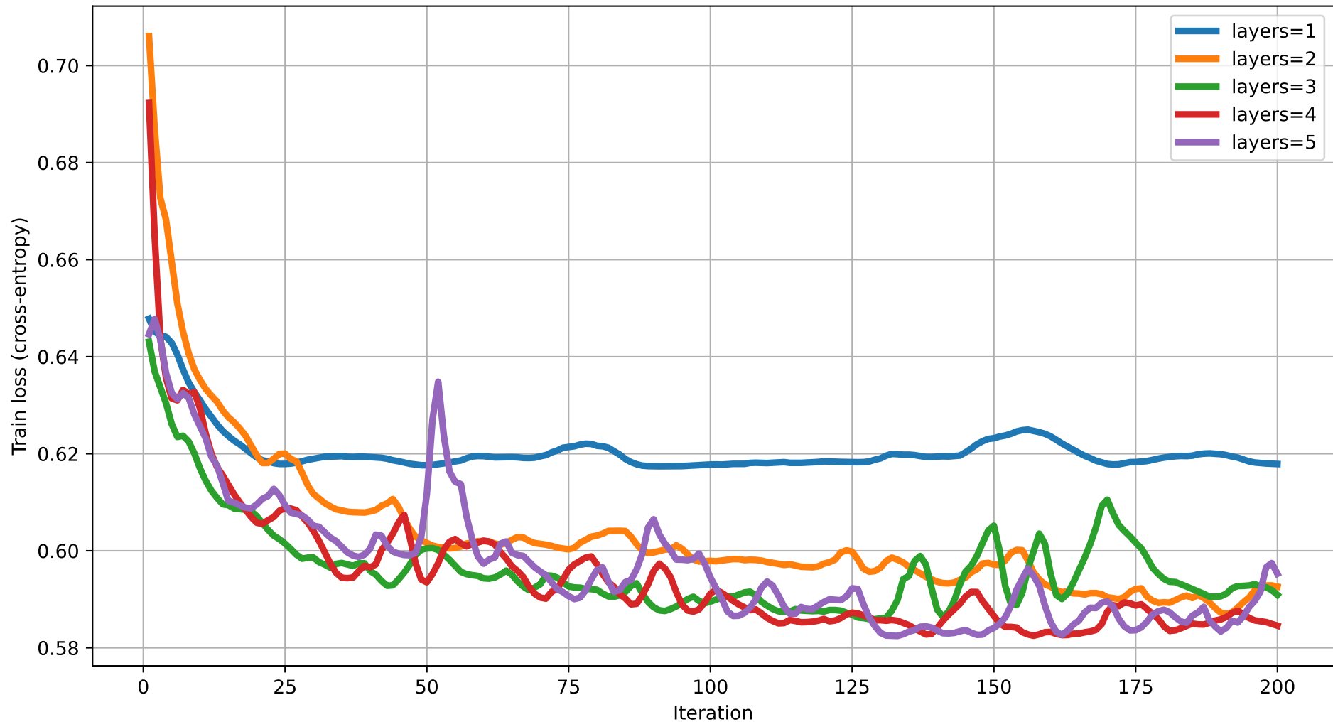
Train loss vs Iteration (degree=4) rot=Rot, ent=ring, gate=IsingXX
