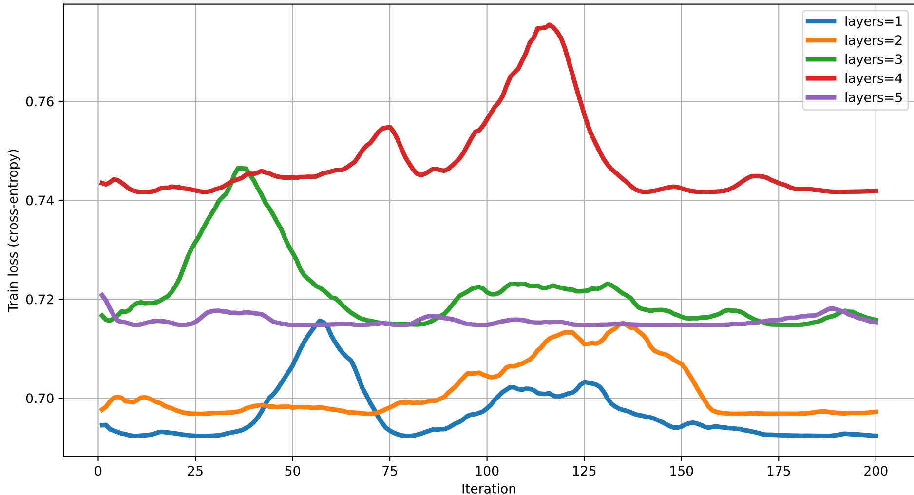
Train loss vs Iteration (dim=9) rot=RZ, ent=ring, gate=CNOT
