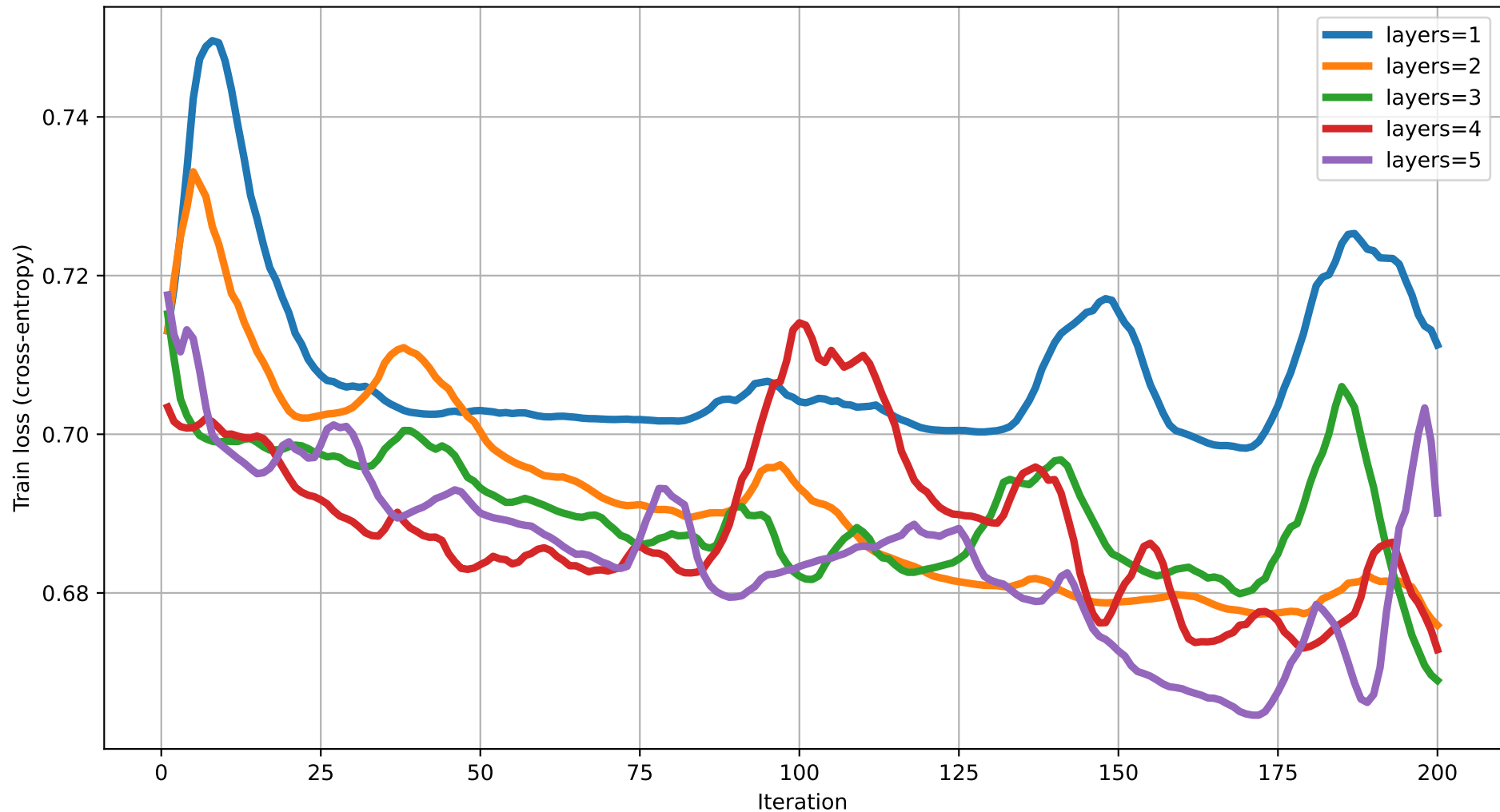
Train loss vs Iteration (dim=12) rot=RY, ent=full, gate=CZ
