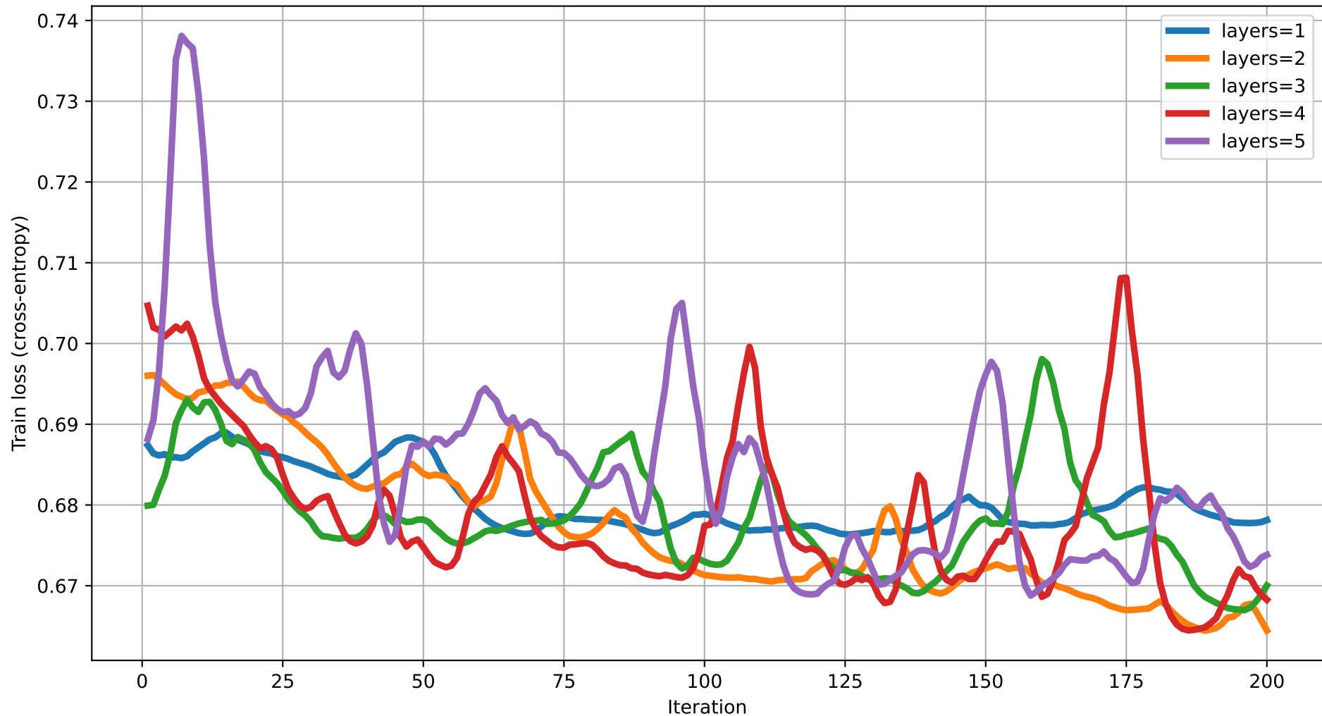
Train loss vs Iteration (dim=19) rot=Rot, ent=ring, gate=CNOT
