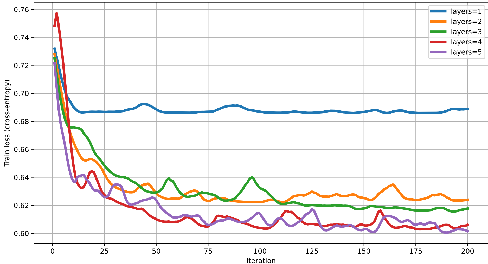
Train loss vs Iteration (degree=2) rot=RYZ, ent=full, gate=CZ
