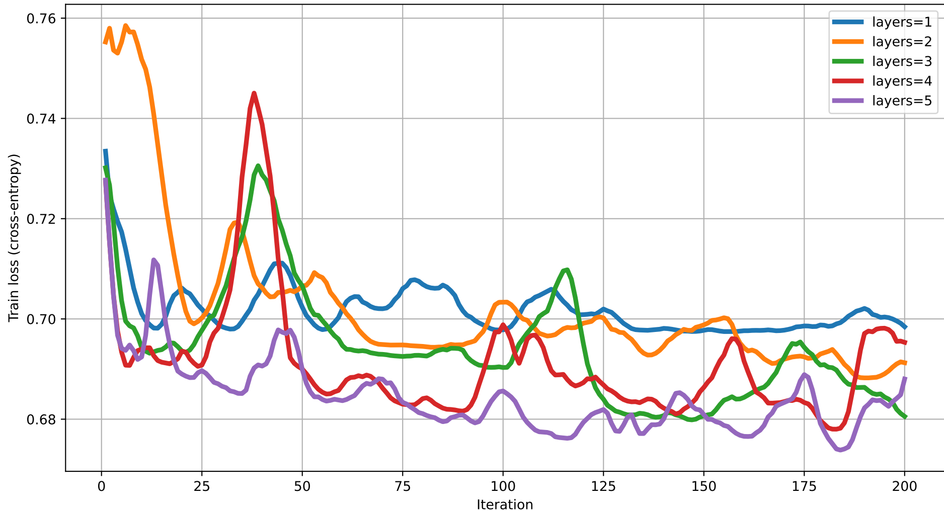
Train loss vs Iteration (dim=19) rot=Rot, ent=full, gate=CZ
