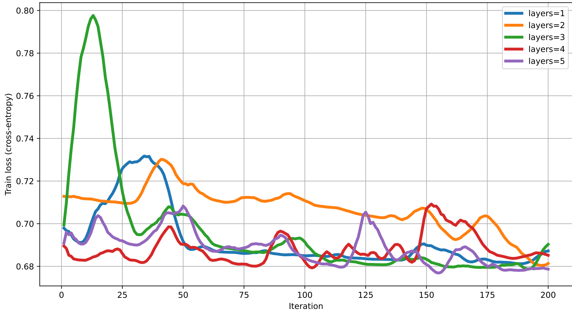
Train loss vs Iteration (dim=13) rot=RZ, ent=pairwise, gate=IsingXX
