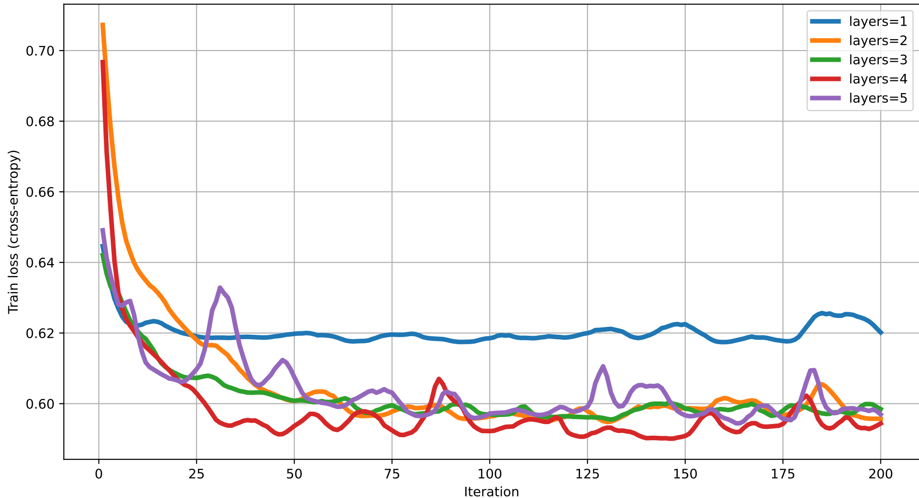
Train loss vs Iteration (degree=4) rot=RY, ent=ring, gate=IsingXX
