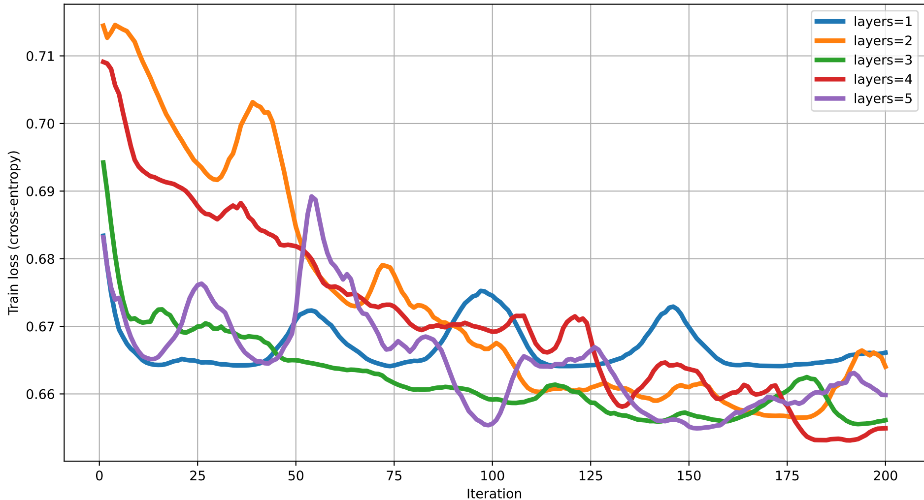
Train loss vs Iteration (dim=6) rot=RZ, ent=full, gate=IsingXX
