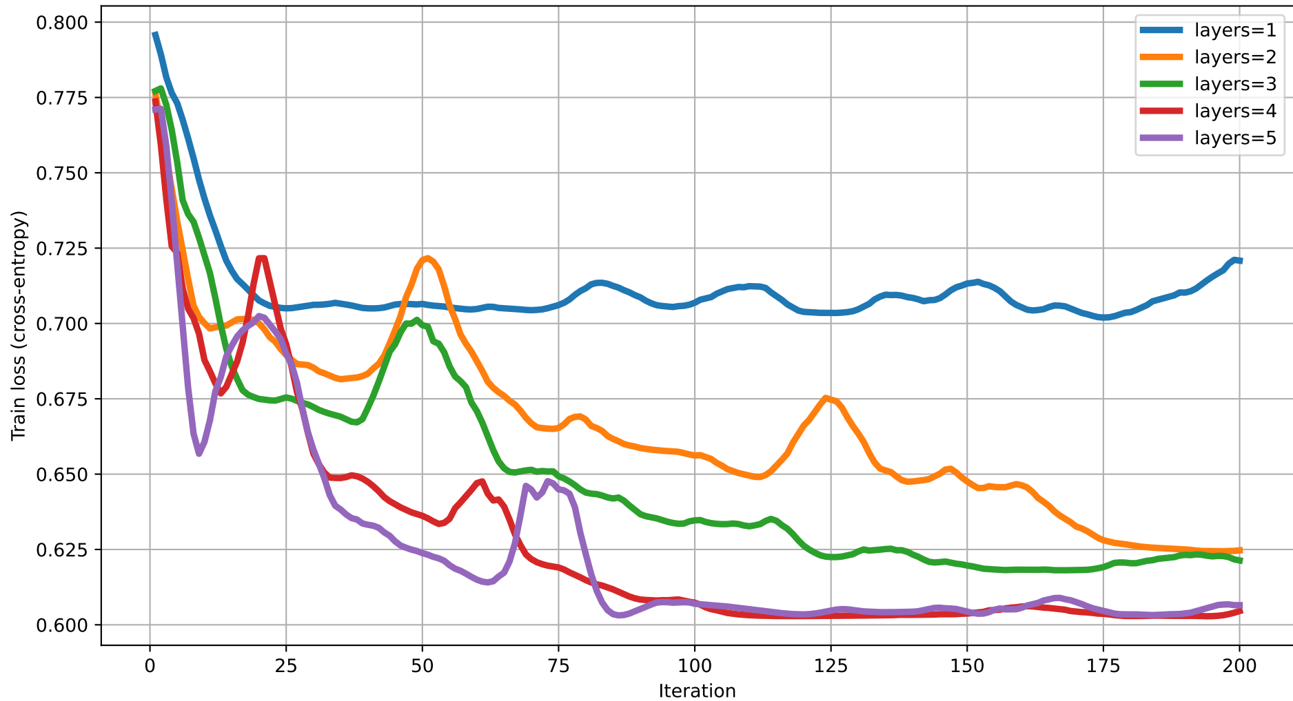
Train loss vs Iteration (dim=4) rot=RX, ent=chain, gate=CNOT
