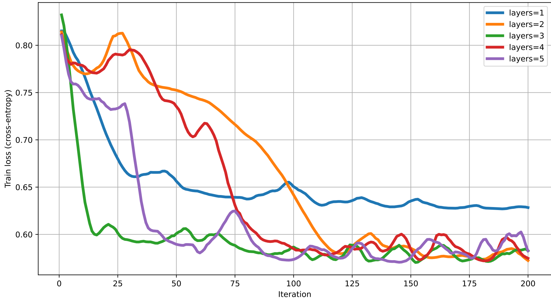
Train loss vs Iteration (dim=2) rot=RYZ, ent=full, gate=CNOT
