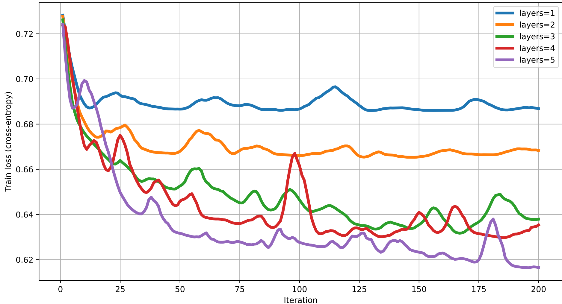
Train loss vs Iteration (degree=2) rot=RY, ent=ring, gate=CZ
