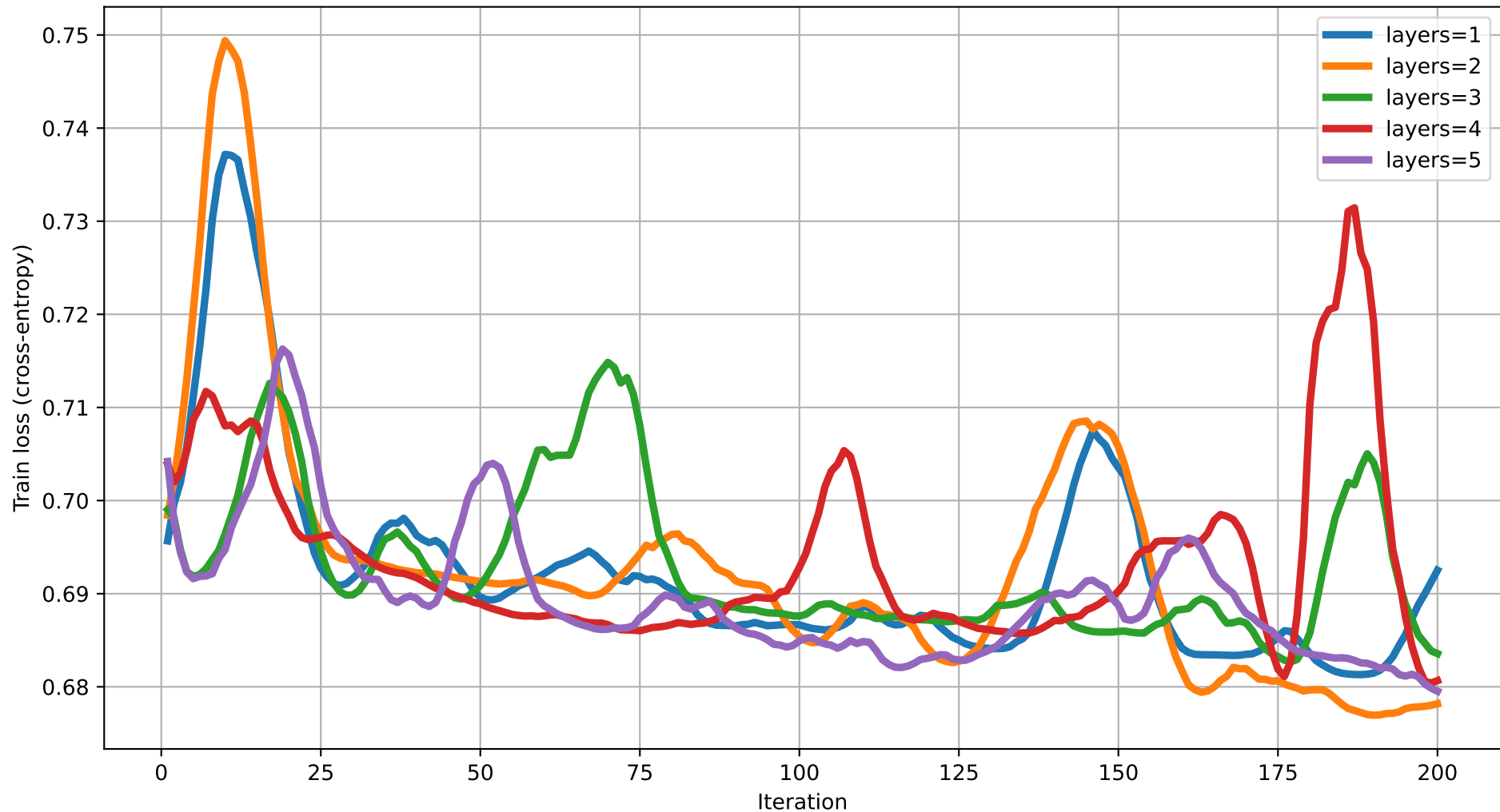
Train loss vs Iteration (dim=14) rot=RZ, ent=chain, gate=IsingXX
