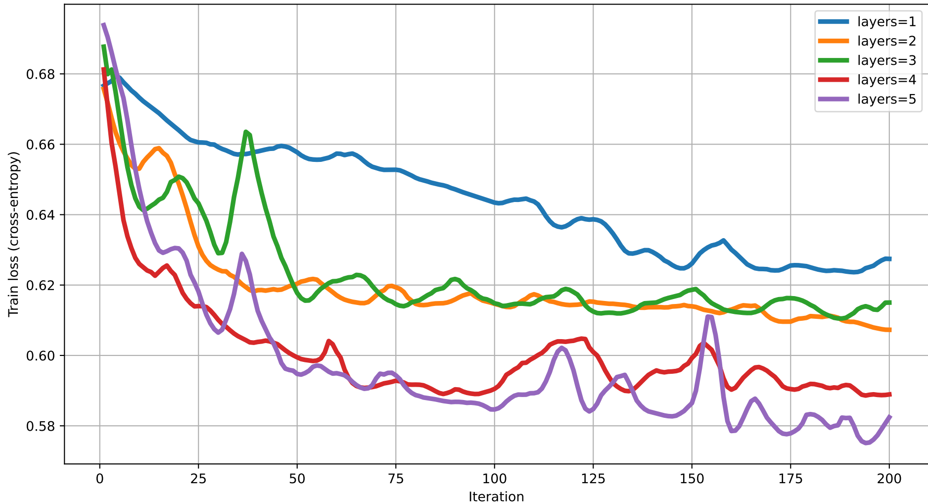
Train loss vs Iteration (degree=4) rot=RY, ent=ring, gate=CNOT
