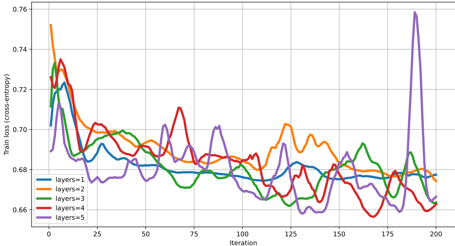
Train loss vs Iteration (dim=3) rot=Rot, ent=chain, gate=IsingXX
