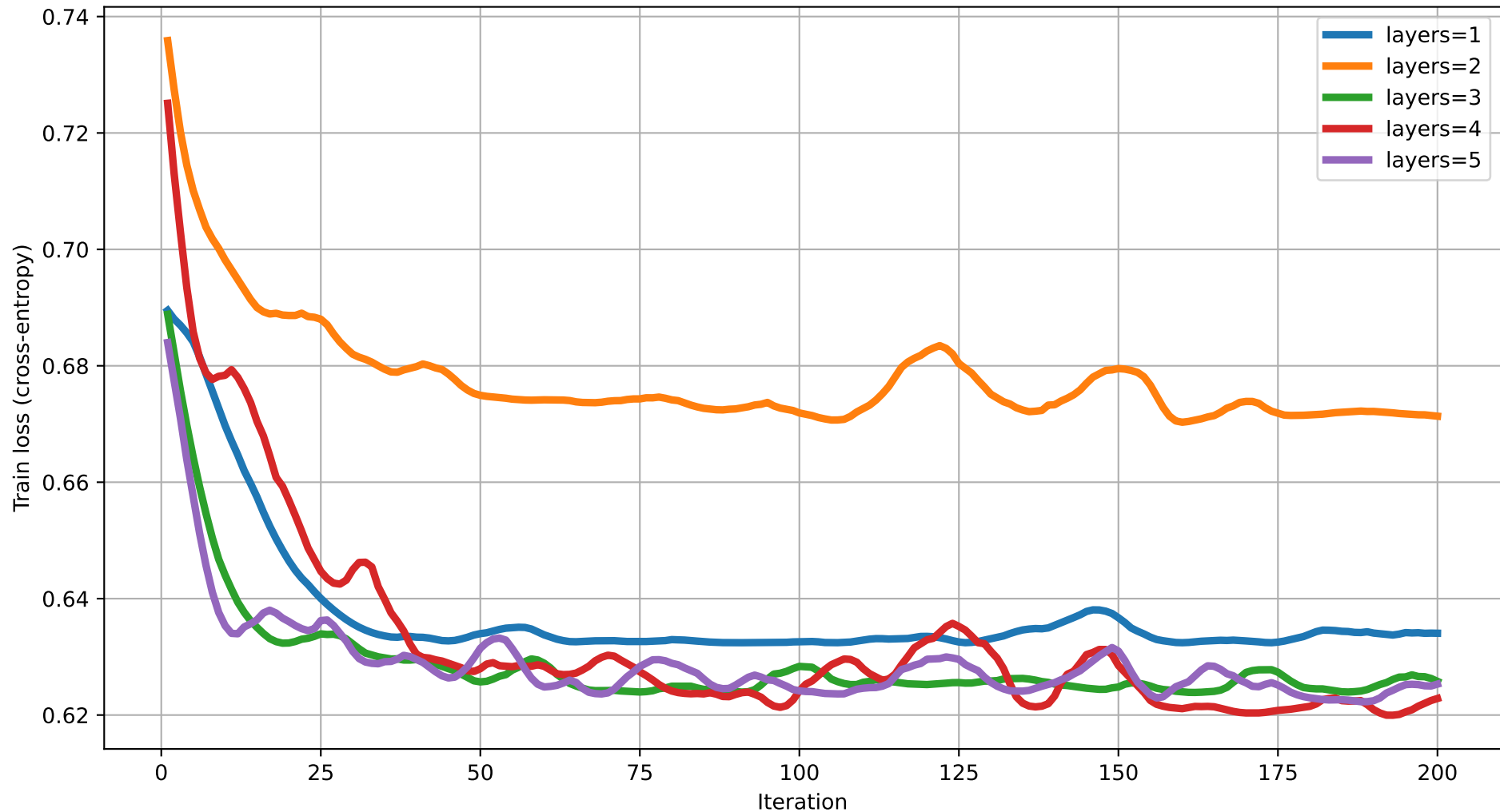
Train loss vs Iteration (degree=2) rot=RZ, ent=chain, gate=IsingXX
