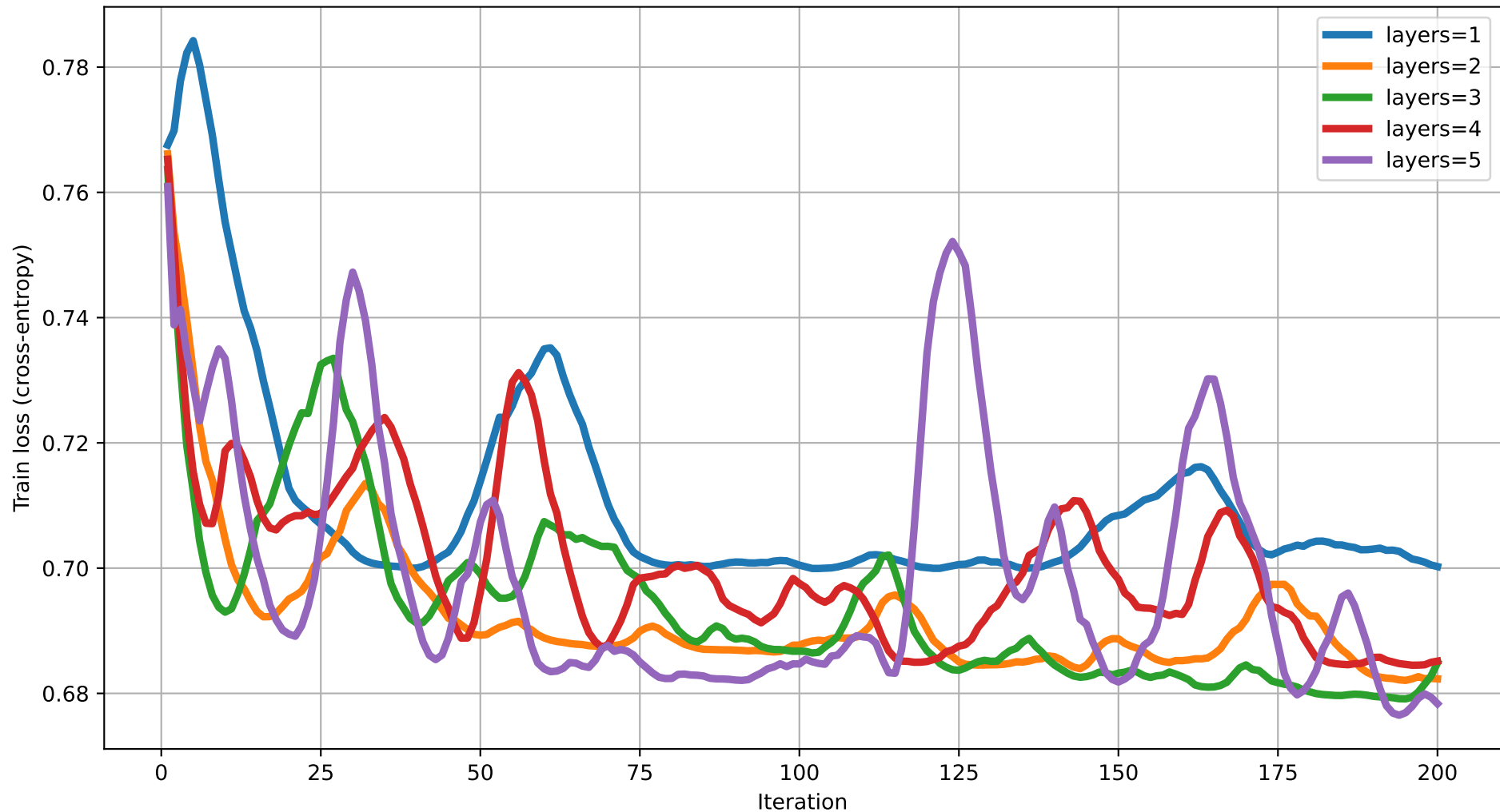
Train loss vs Iteration (dim=17) rot=RY, ent=chain, gate=CZ
