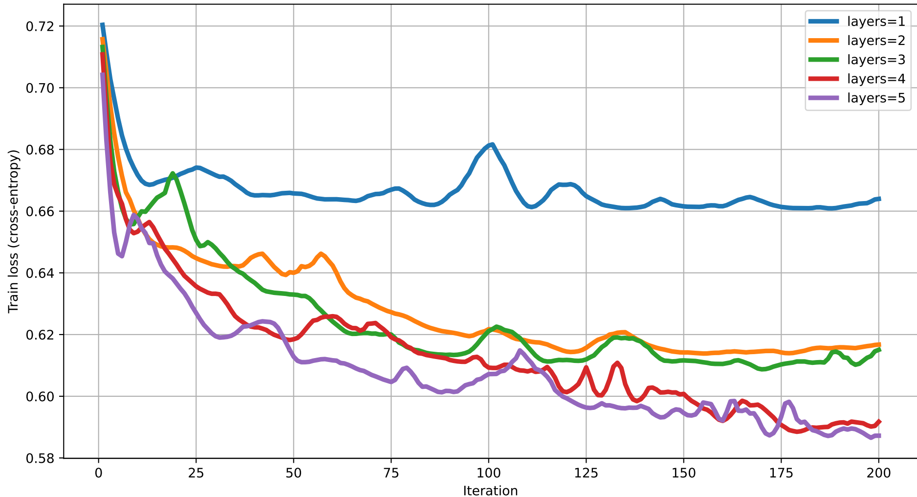
Train loss vs Iteration (degree=3) rot=Rot, ent=chain, gate=CZ
