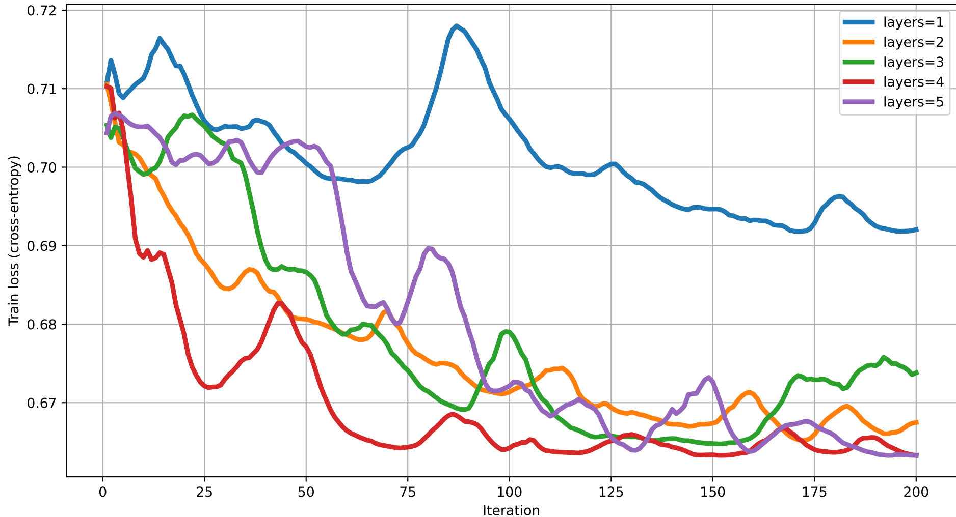
Train loss vs Iteration (dim=12) rot=RX, ent=full, gate=CNOT
