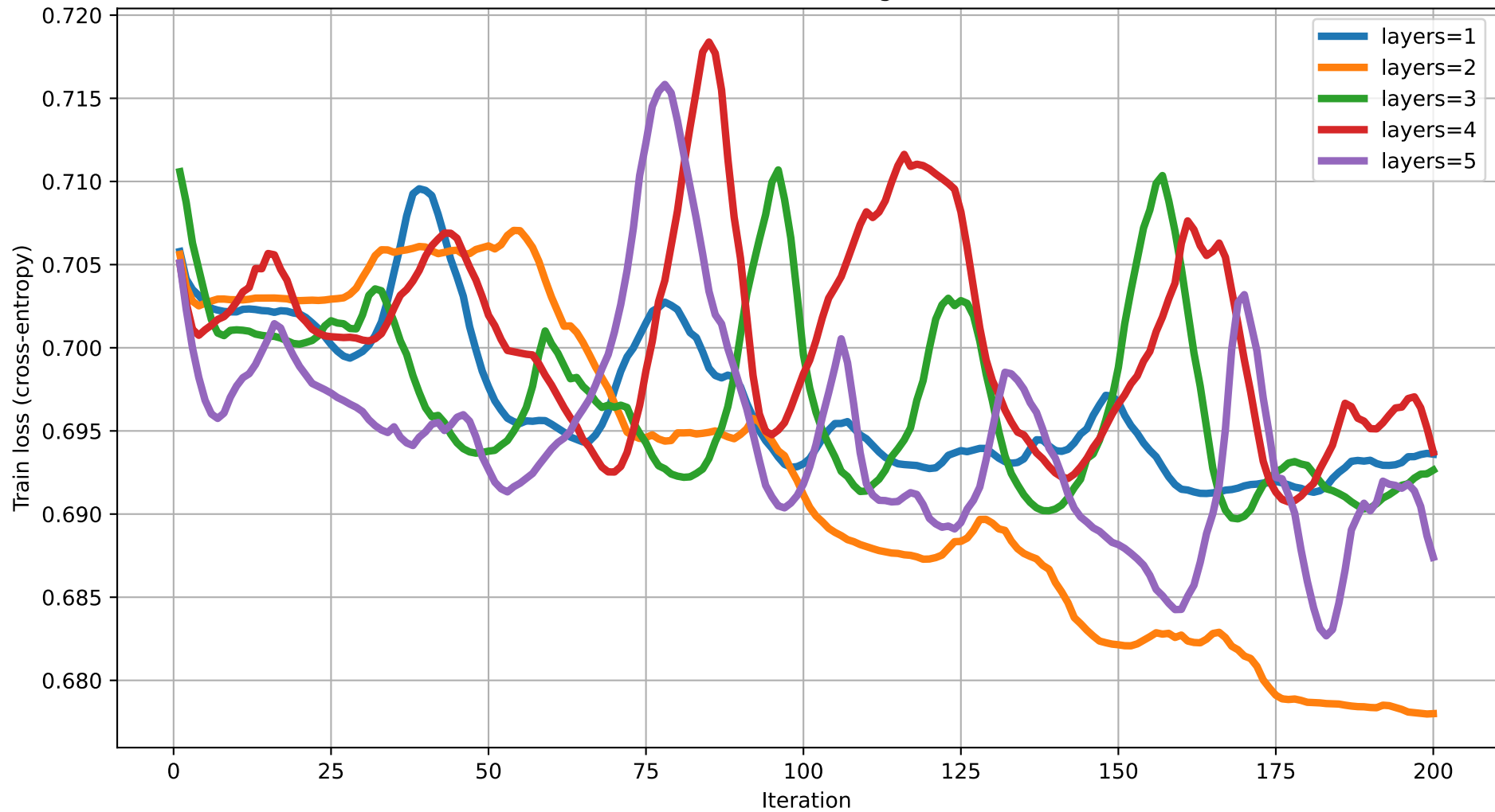
Train loss vs Iteration (dim=12) rot=RX, ent=chain, gate=CZ
