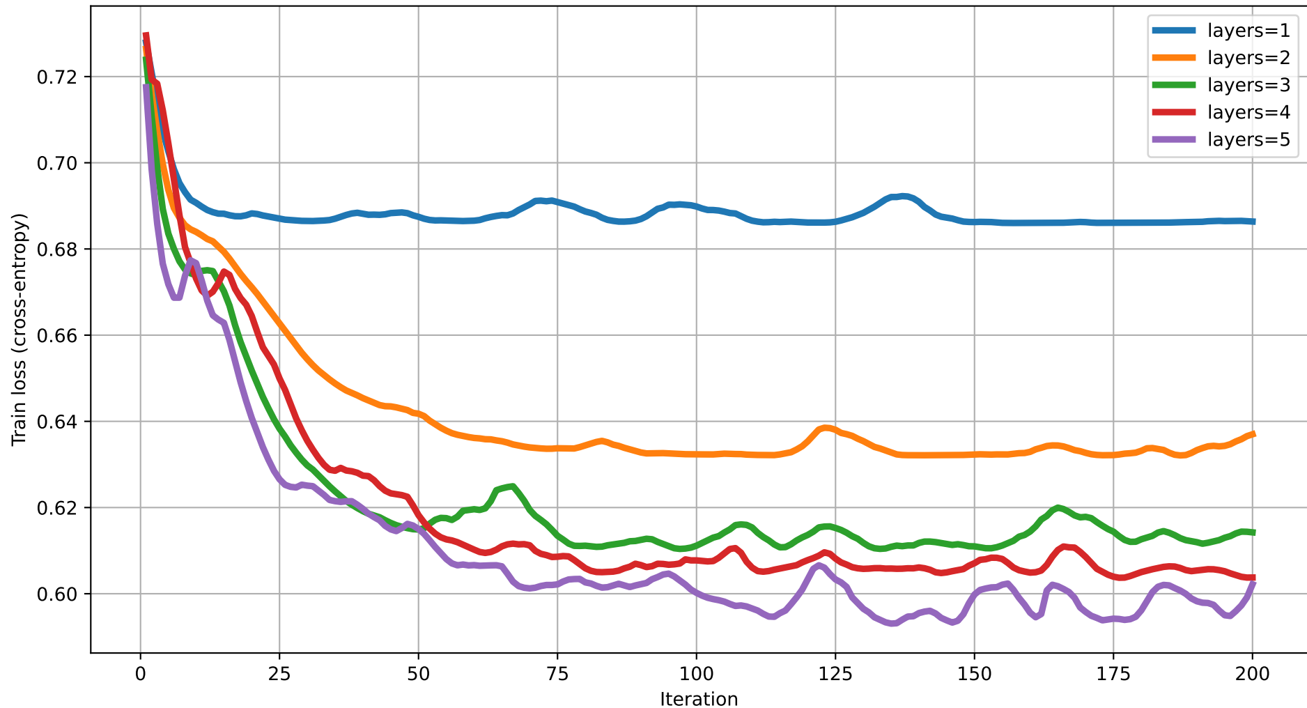
Train loss vs Iteration (degree=2) rot=RYZ, ent=chain, gate=CNOT
