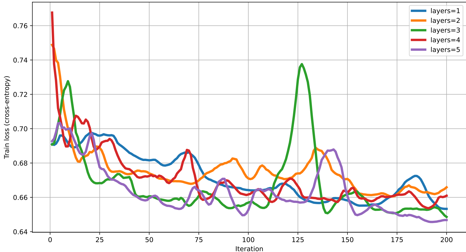
Train loss vs Iteration (dim=9) rot=RYZ, ent=chain, gate=IsingXX
