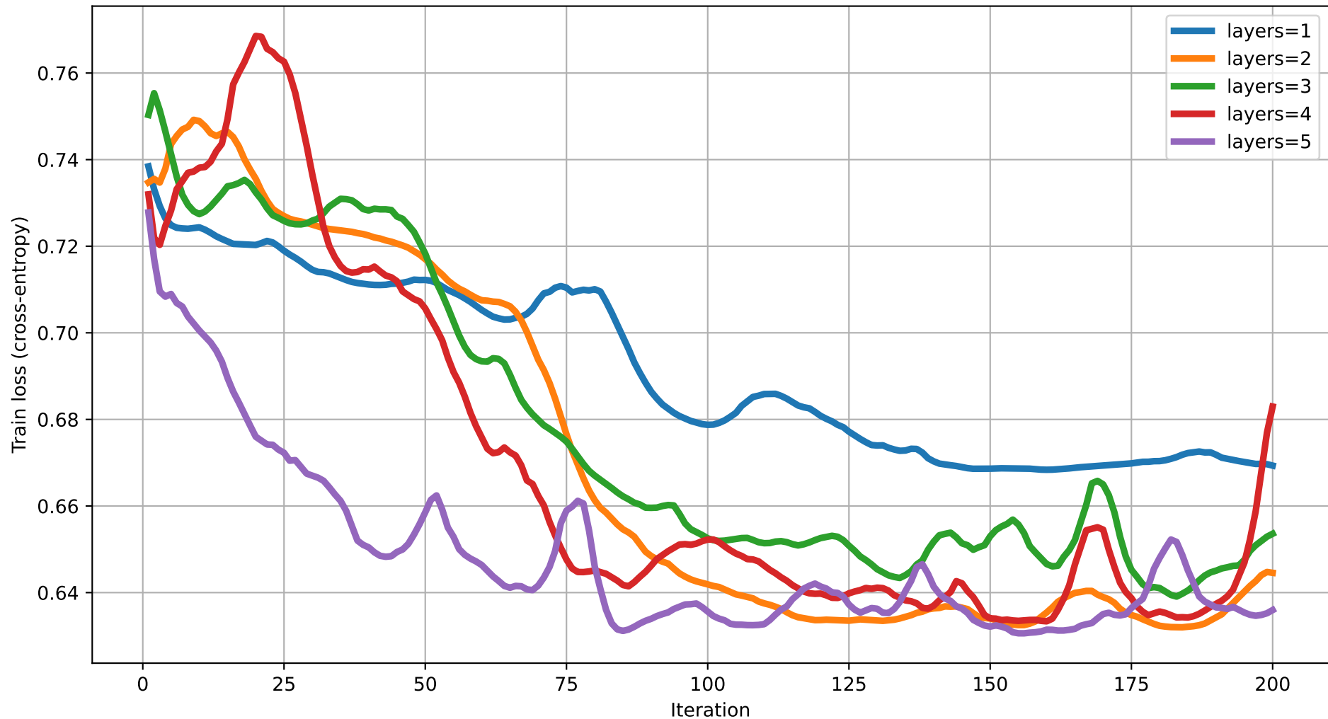
Train loss vs Iteration (dim=3) rot=RYZ, ent=chain, gate=CNOT
