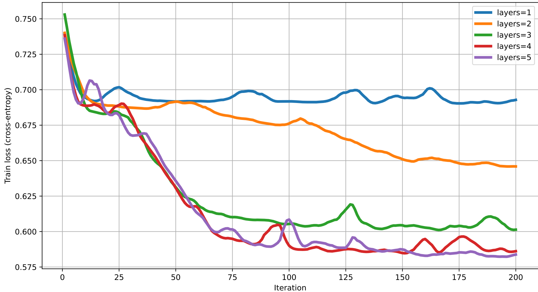
Train loss vs Iteration (degree=5) rot=RYZ, ent=full, gate=CZ
