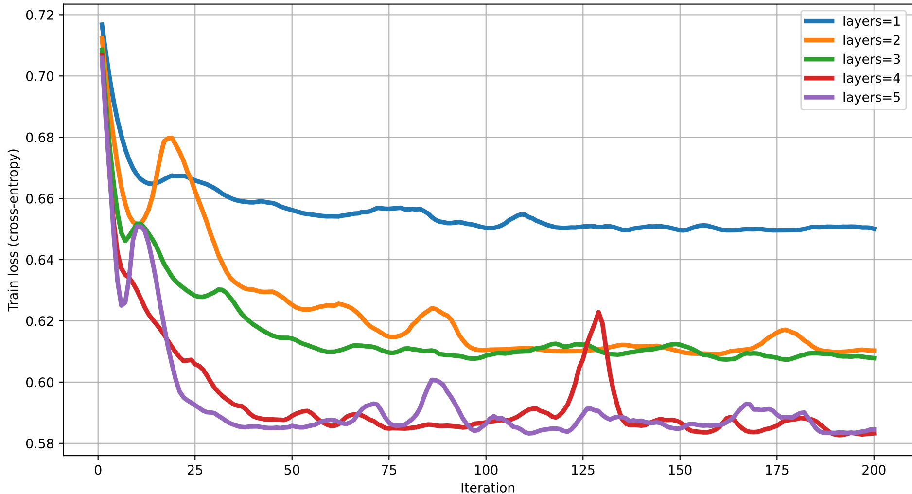
Train loss vs Iteration (degree=4) rot=RY, ent=chain, gate=CNOT
