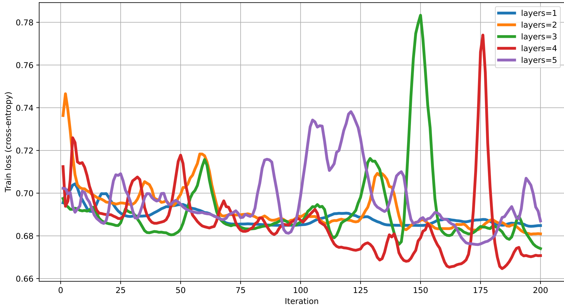
Train loss vs Iteration (dim=19) rot=Rot, ent=chain, gate=IsingXX
