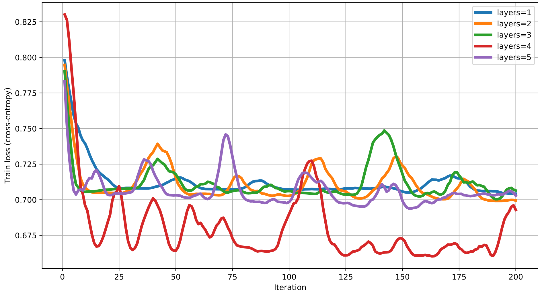
Train loss vs Iteration (dim=8) rot=RY, ent=pairwise, gate=CNOT
