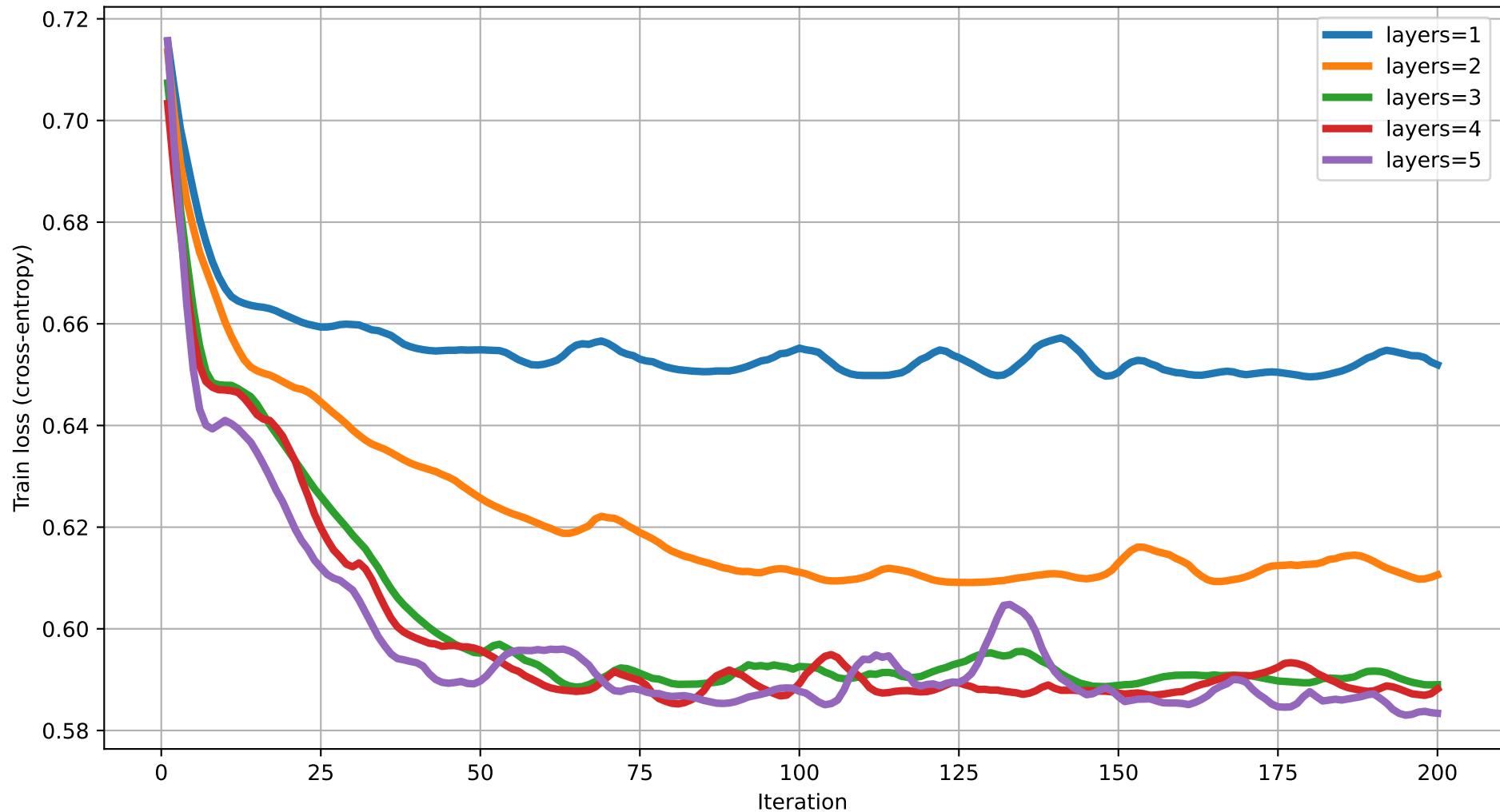
Train loss vs Iteration (degree=4) rot=RYZ, ent=chain, gate=CZ
