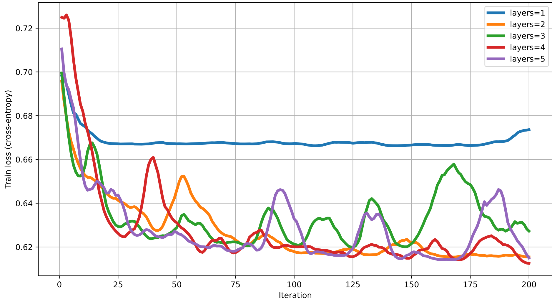
Train loss vs Iteration (dim=10) rot=RY, ent=pairwise, gate=CZ
