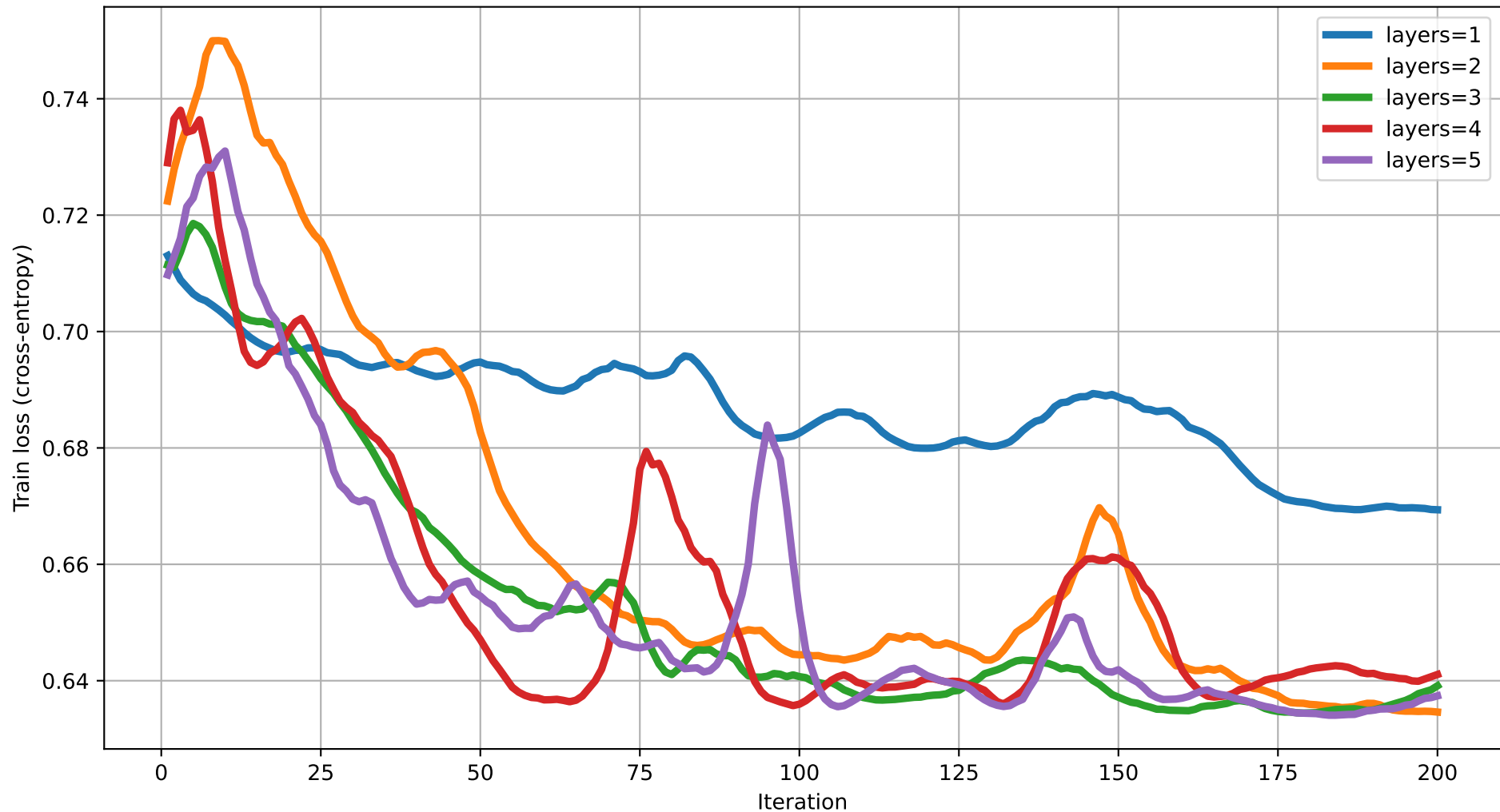
Train loss vs Iteration (dim=7) rot=RYZ, ent=pairwise, gate=CNOT
