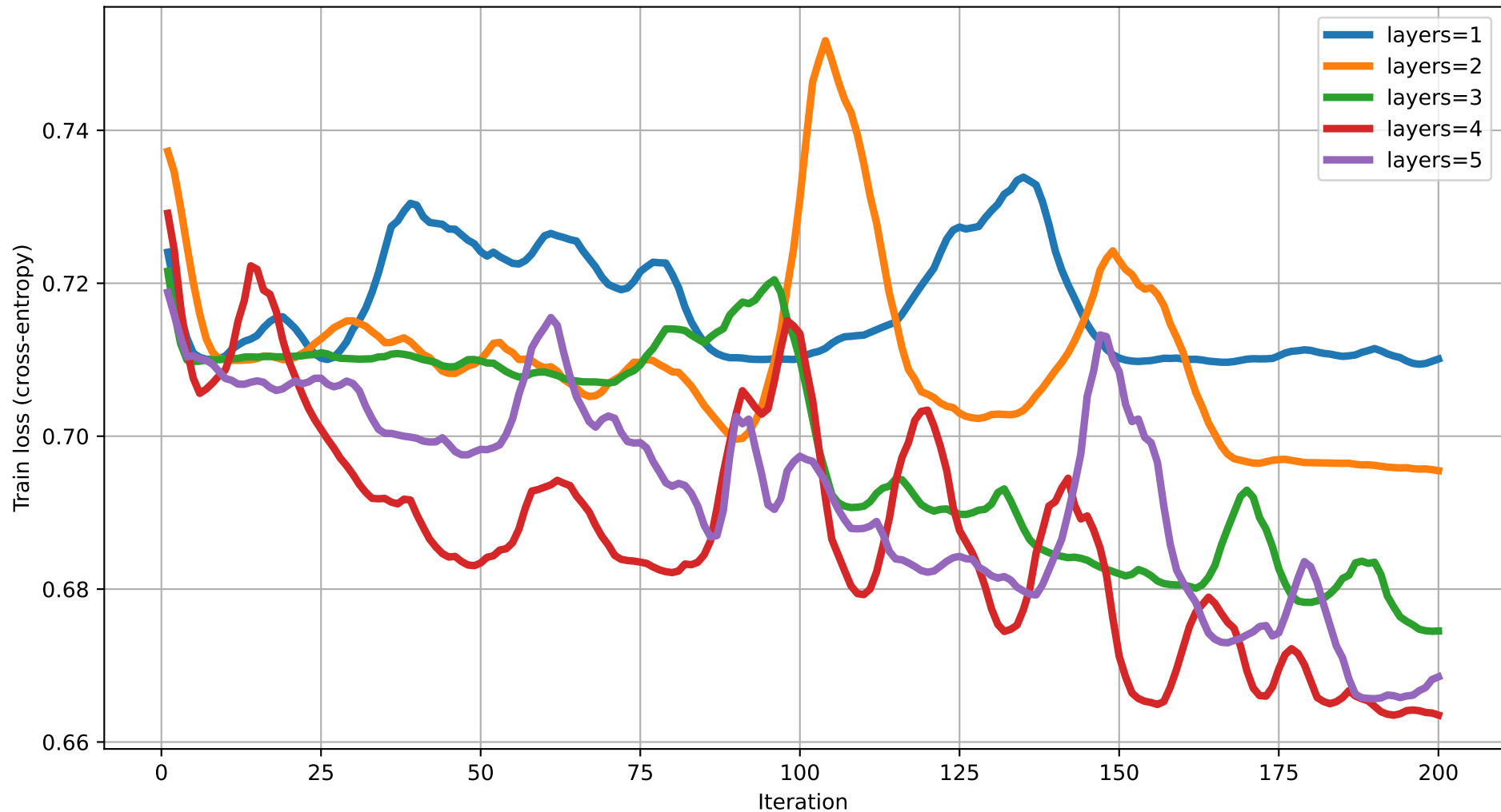
Train loss vs Iteration (dim=10) rot=RYZ, ent=full, gate=CZ
