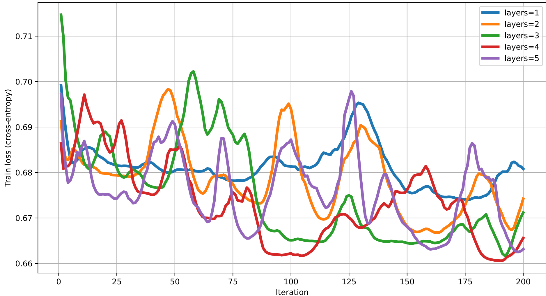
Train loss vs Iteration (dim=13) rot=RY, ent=full, gate=CNOT
