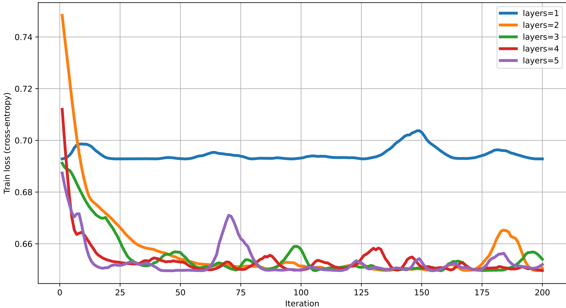
Train loss vs Iteration (degree=4) rot=RY, ent=pairwise, gate=IsingXX
