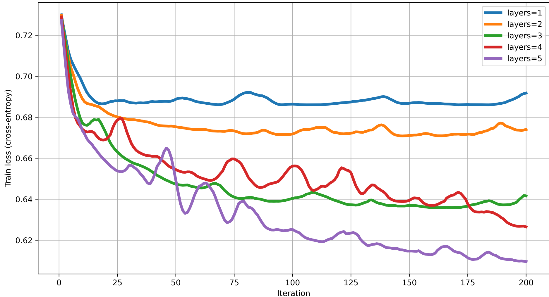
Train loss vs Iteration (degree=2) rot=RX, ent=full, gate=CZ
