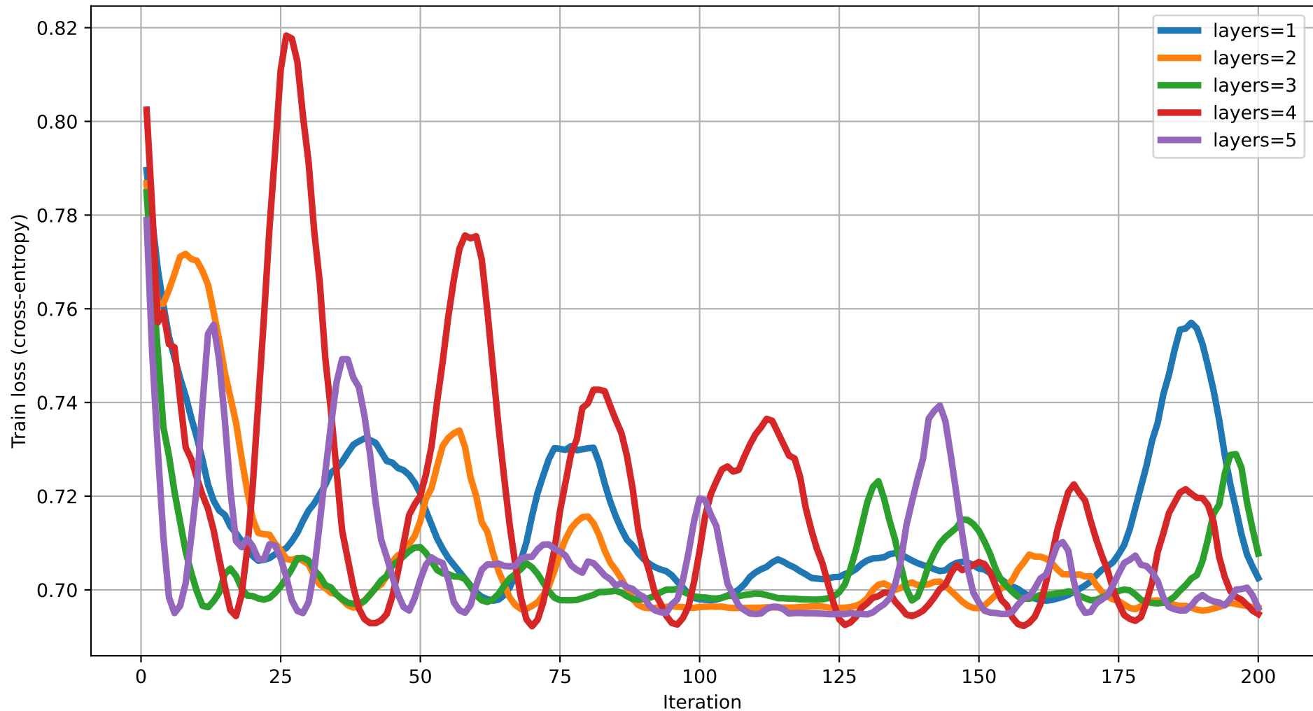
Train loss vs Iteration (dim=2) rot=RYZ, ent=ring, gate=CZ
