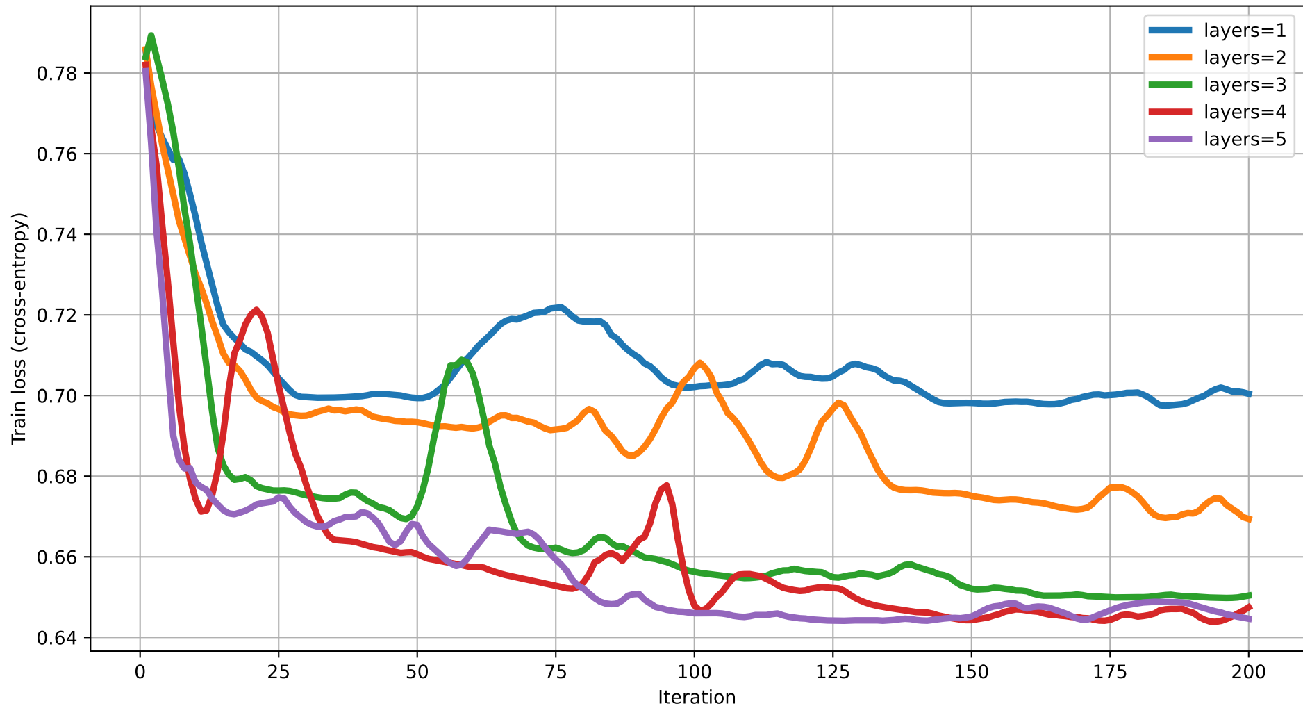
Train loss vs Iteration (dim=9) rot=RX, ent=chain, gate=CNOT
