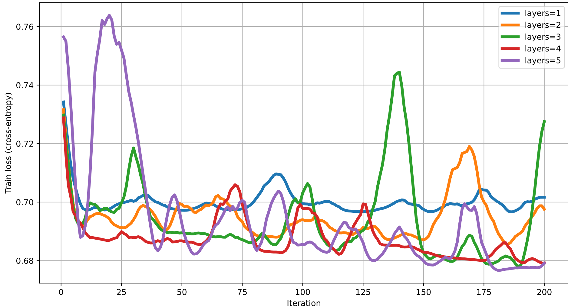
Train loss vs Iteration (dim=18) rot=RY, ent=chain, gate=CZ
