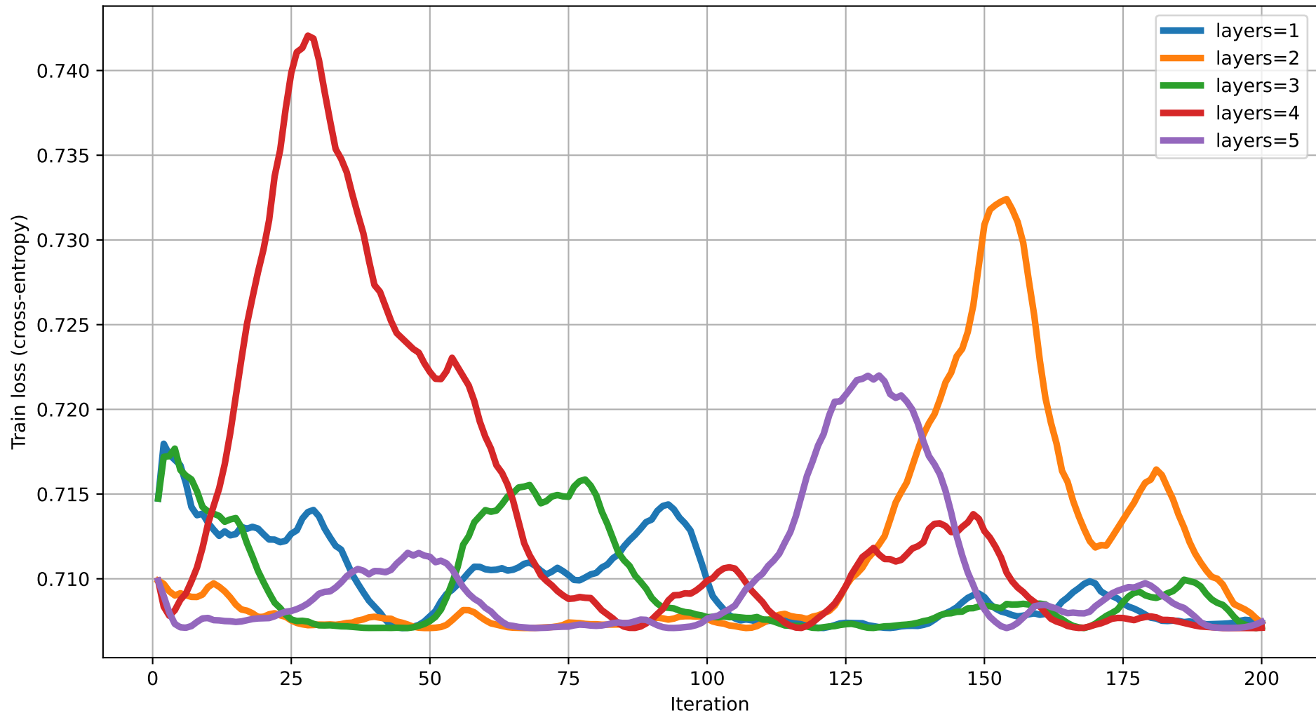
Train loss vs Iteration (dim=6) rot=RZ, ent=pairwise, gate=CNOT
