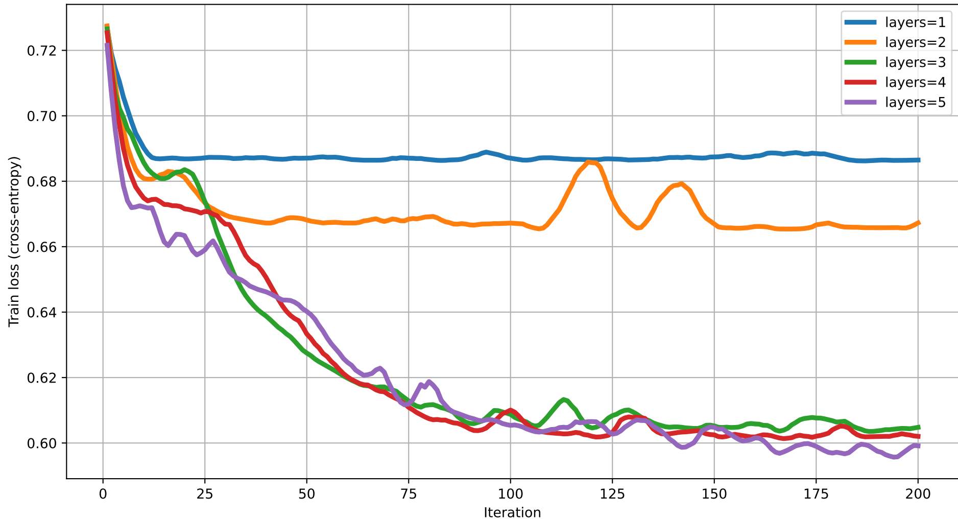
Train loss vs Iteration (degree=2) rot=RYZ, ent=ring, gate=CZ
