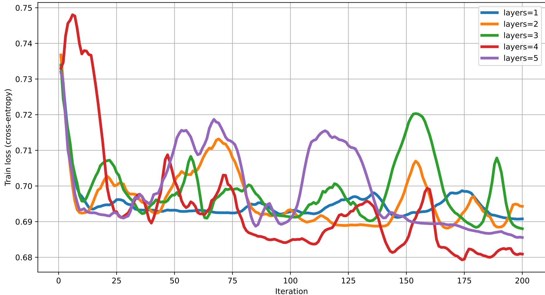
Train loss vs Iteration (dim=16) rot=Rot, ent=ring, gate=CZ
