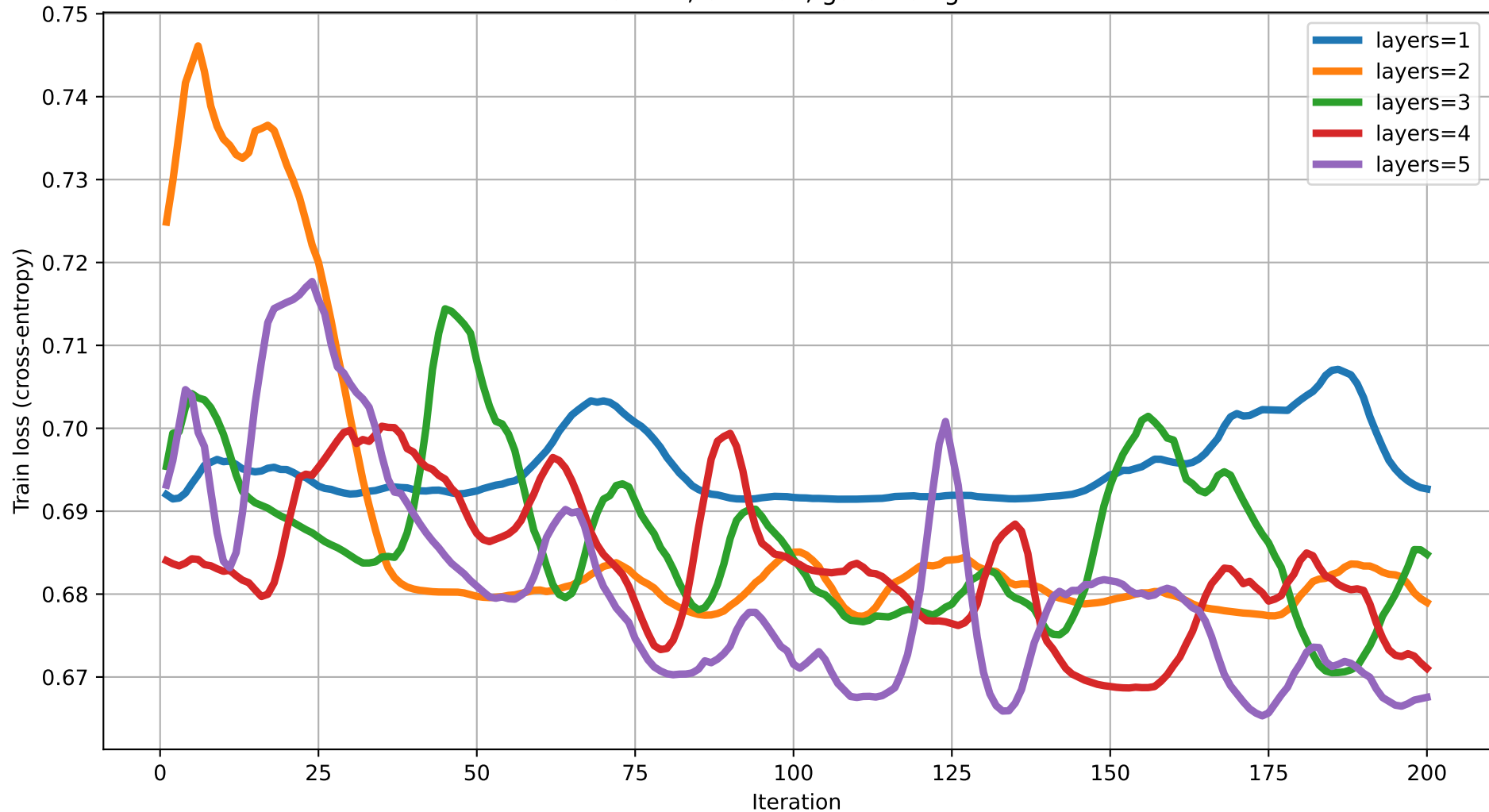
Train loss vs Iteration (dim=15) rot=RY, ent=full, gate=IsingXX
