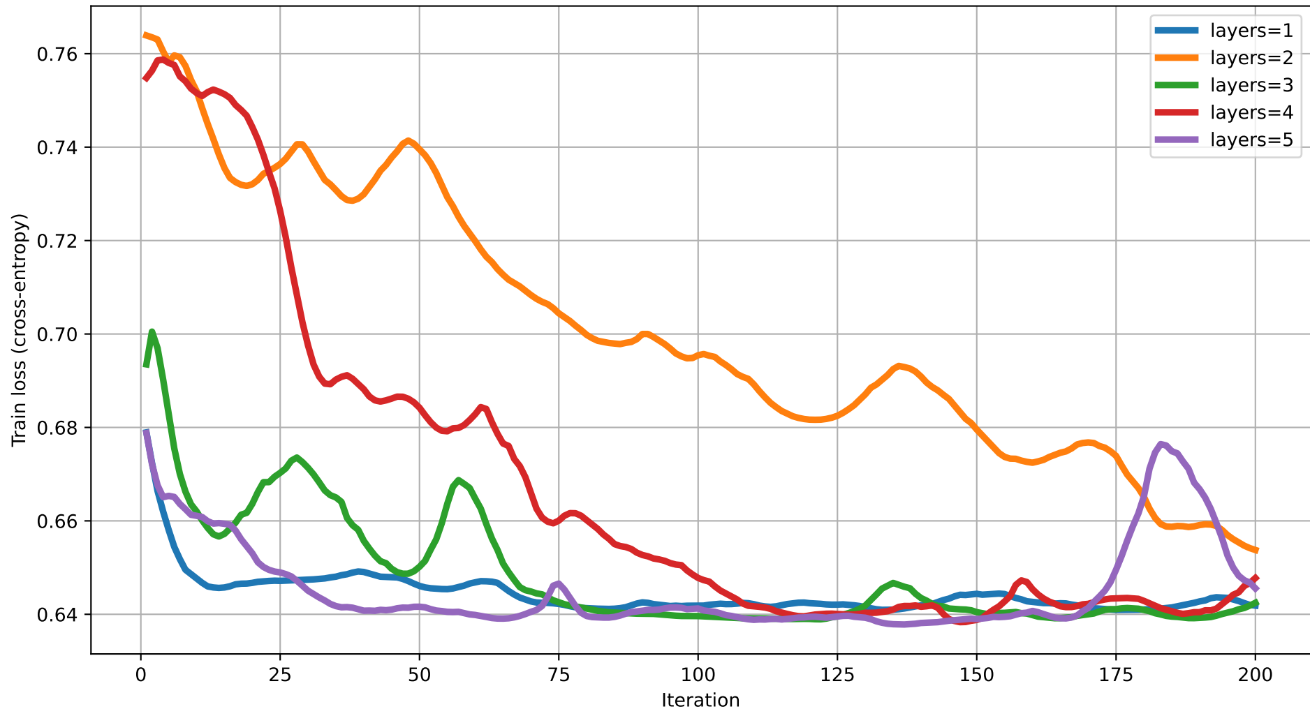
Train loss vs Iteration (dim=5) rot=RZ, ent=ring, gate=IsingXX
