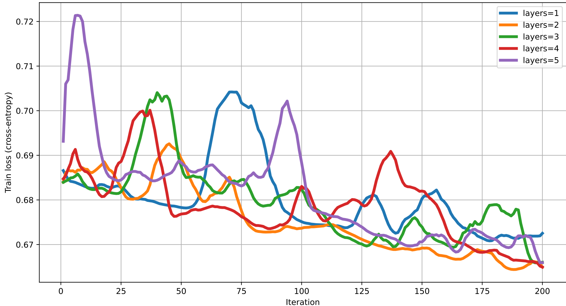
Train loss vs Iteration (dim=15) rot=RYZ, ent=full, gate=CZ
