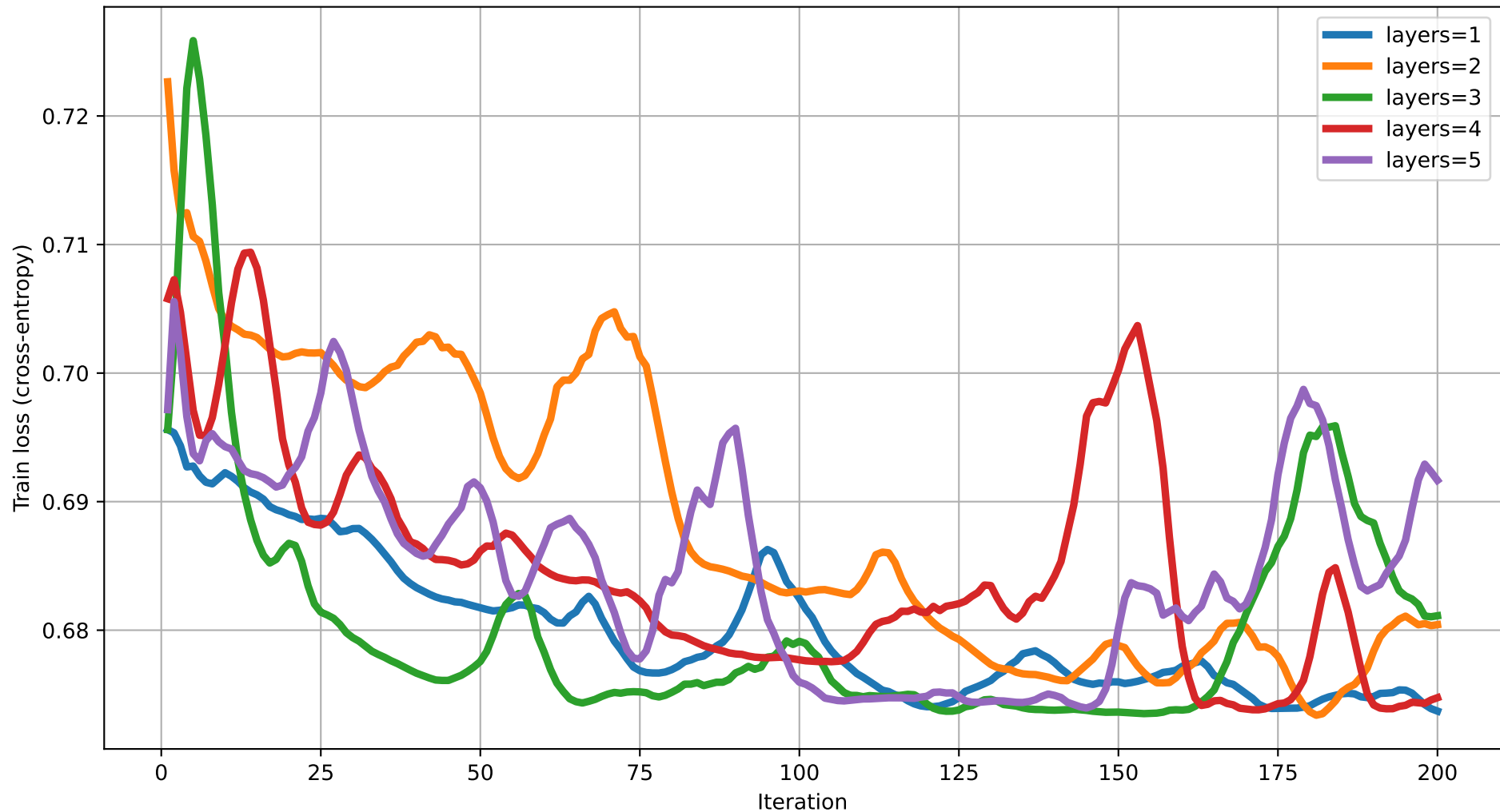
Train loss vs Iteration (dim=11) rot=RZ, ent=pairwise, gate=IsingXX
