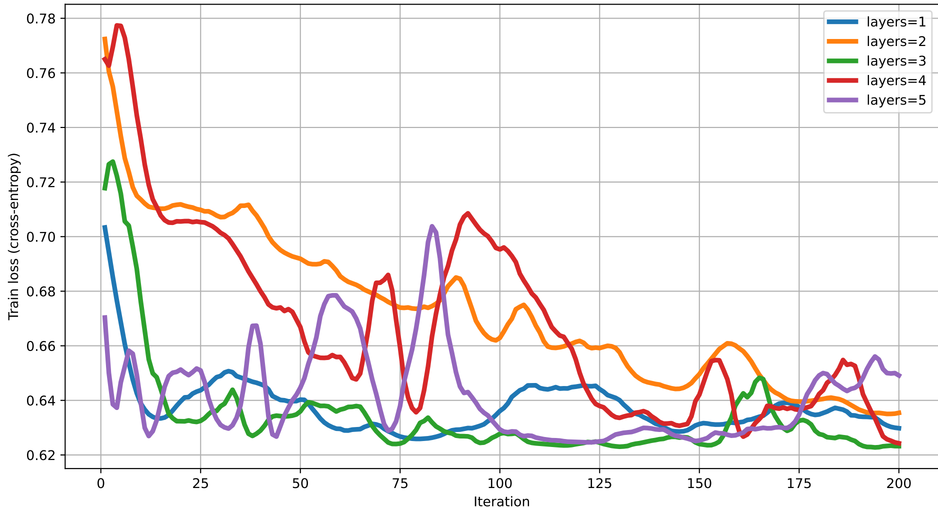
Train loss vs Iteration (dim=4) rot=RY, ent=ring, gate=IsingXX
