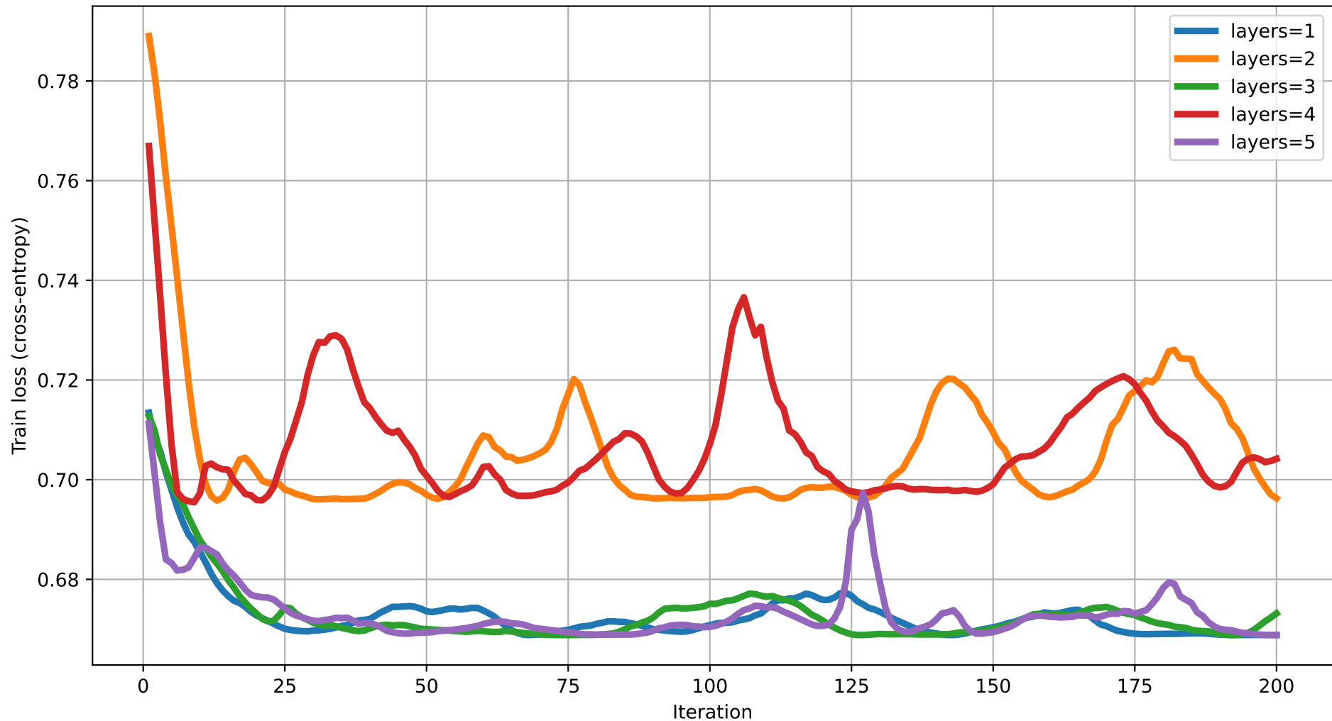
Train loss vs Iteration (dim=17) rot=RX, ent=ring, gate=IsingXX
