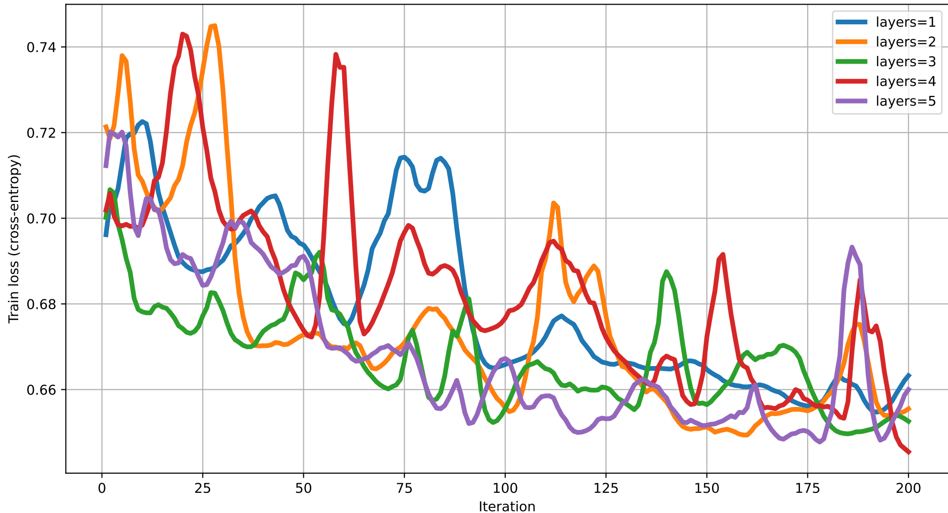
Train loss vs Iteration (dim=6) rot=Rot, ent=chain, gate=IsingXX
