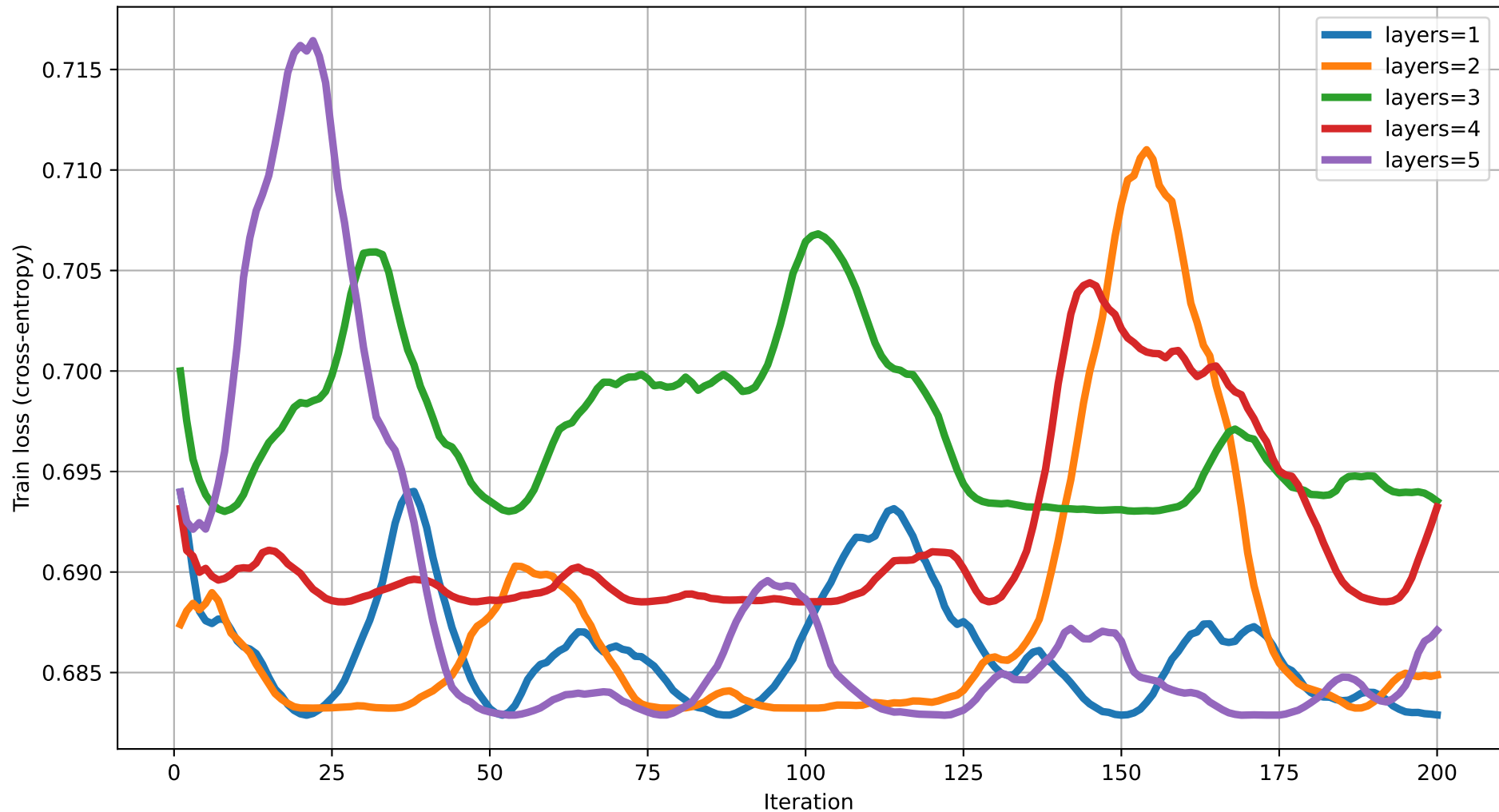
Train loss vs Iteration (dim=16) rot=RZ, ent=ring, gate=CNOT
