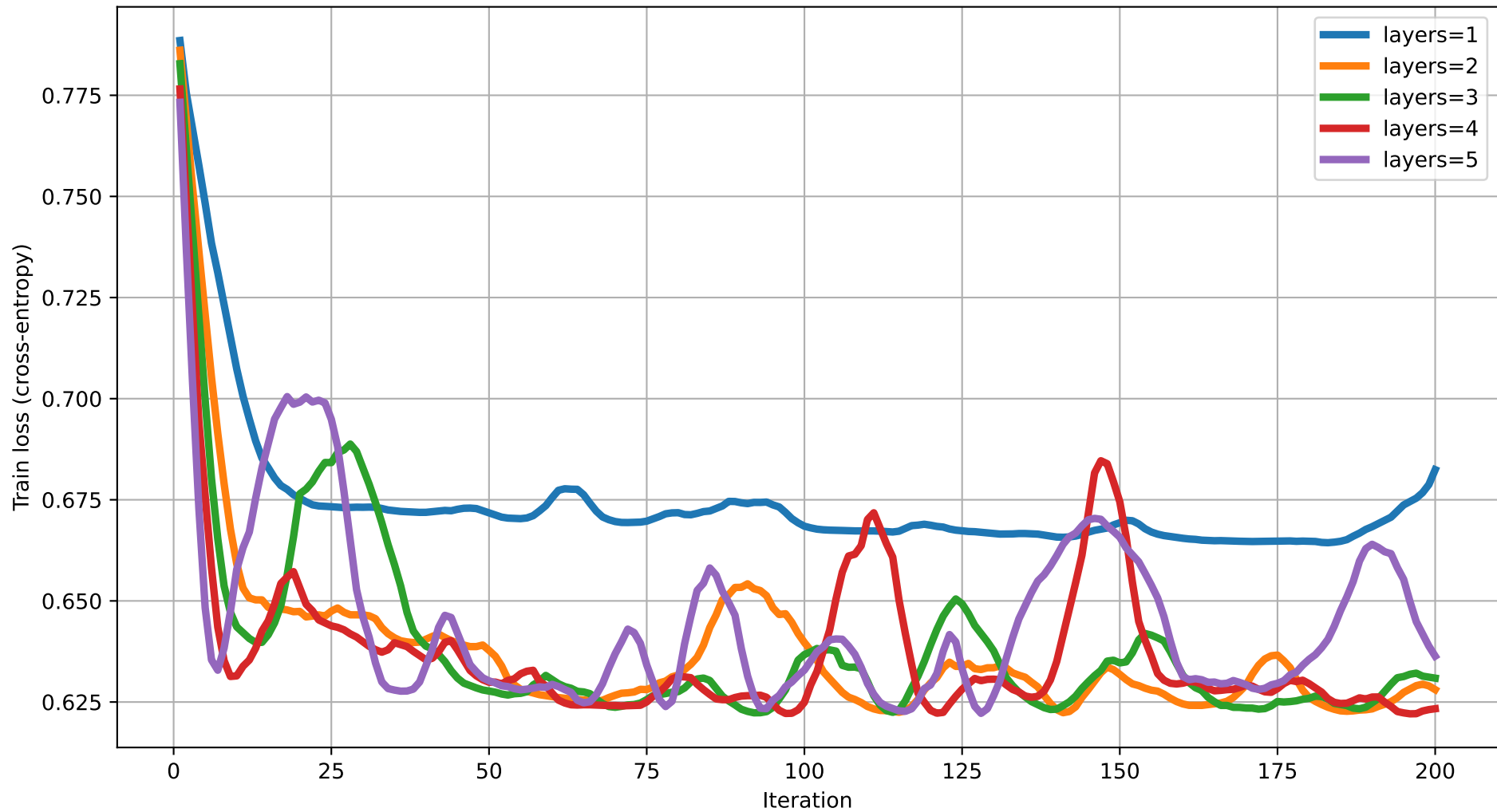
Train loss vs Iteration (dim=4) rot=RY, ent=pairwise, gate=CNOT
