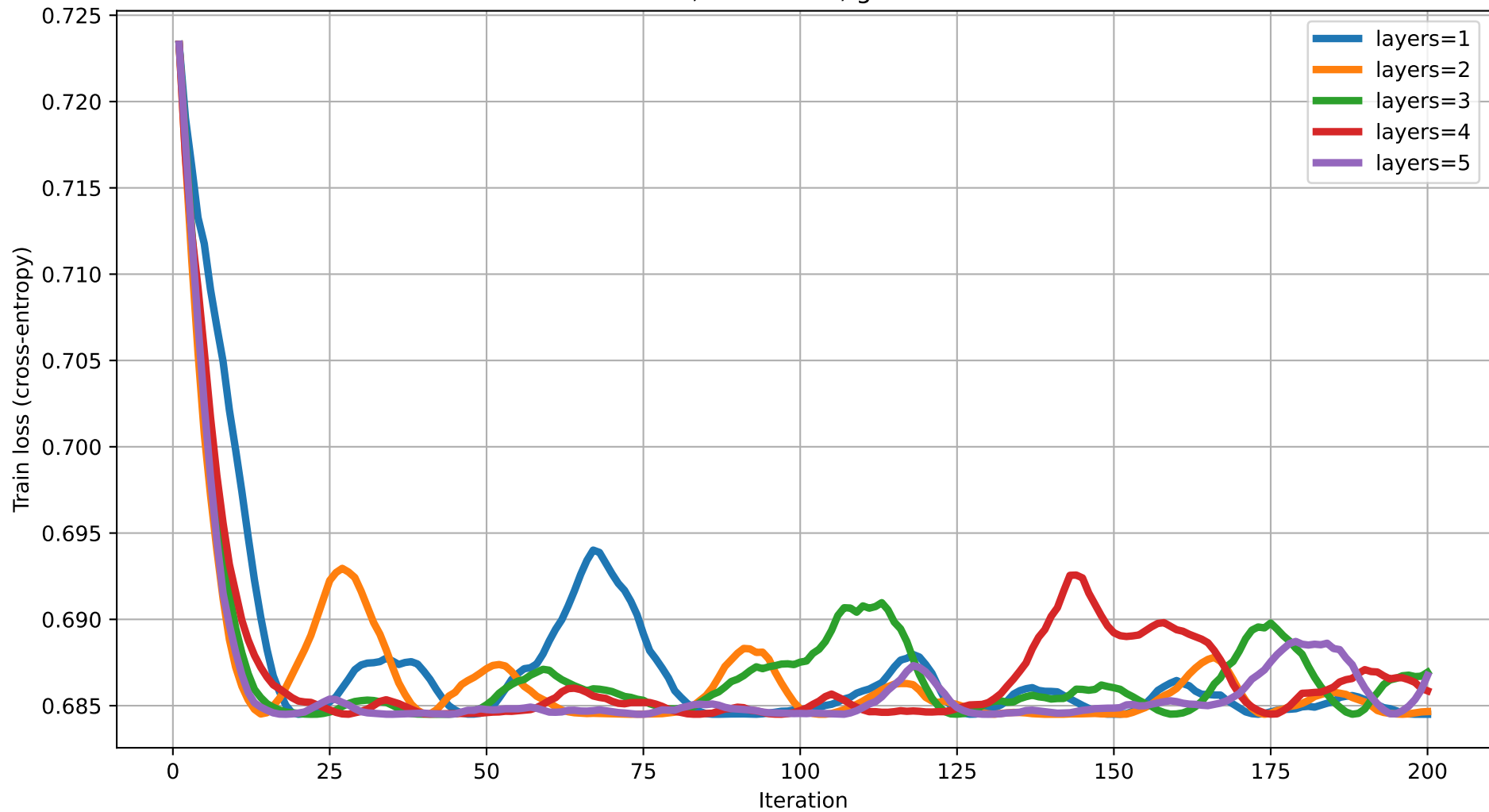
Train loss vs Iteration (degree=3) rot=RZ, ent=chain, gate=CNOT
