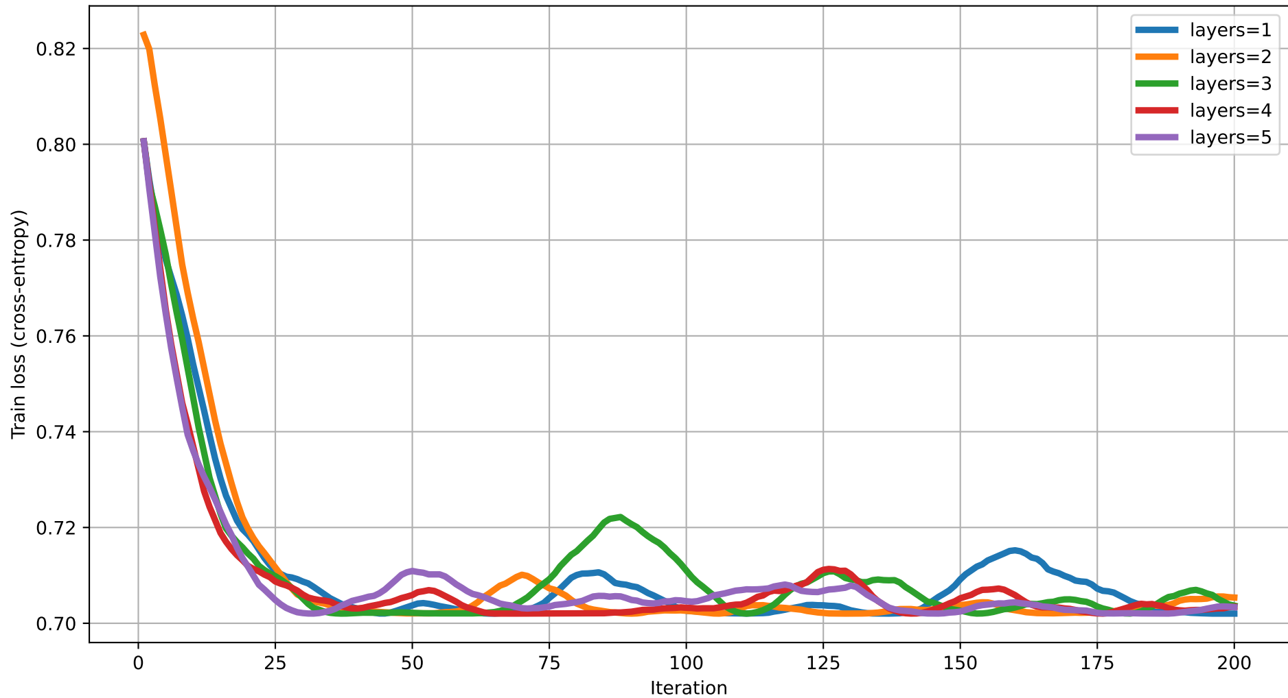
Train loss vs Iteration (dim=8) rot=RZ, ent=full, gate=CZ
