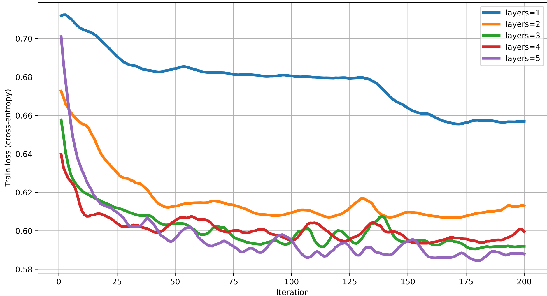
Train loss vs Iteration (degree=5) rot=RY, ent=ring, gate=CNOT
