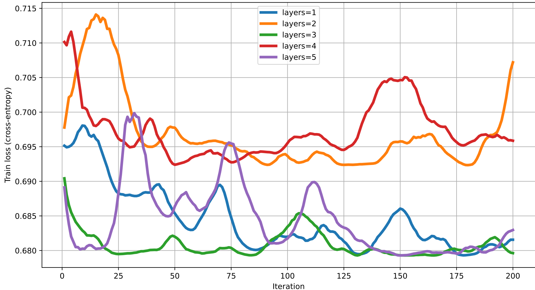
Train loss vs Iteration (dim=14) rot=RX, ent=chain, gate=IsingXX
