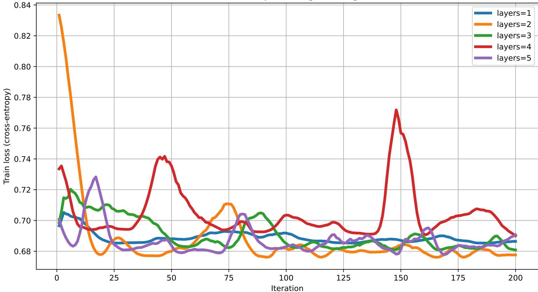
Train loss vs Iteration (dim=16) rot=RY, ent=pairwise, gate=IsingXX
