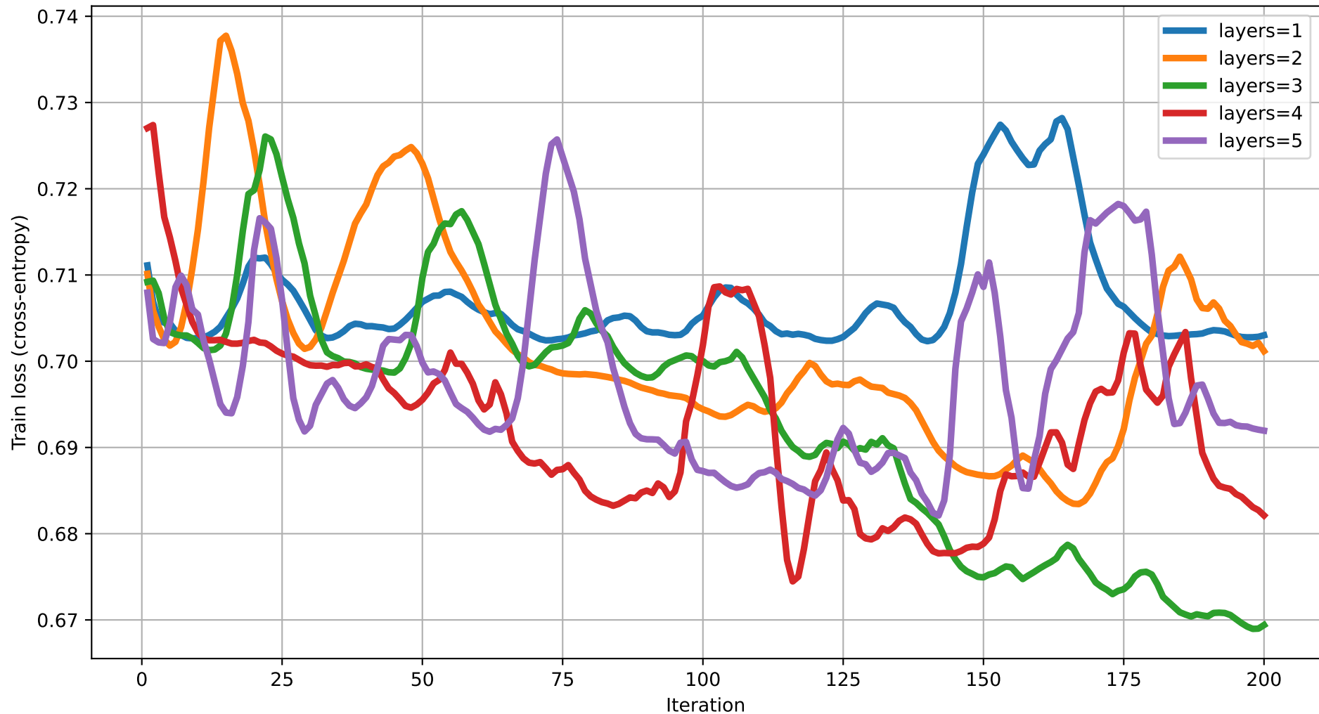
Train loss vs Iteration (dim=11) rot=Rot, ent=full, gate=CZ
