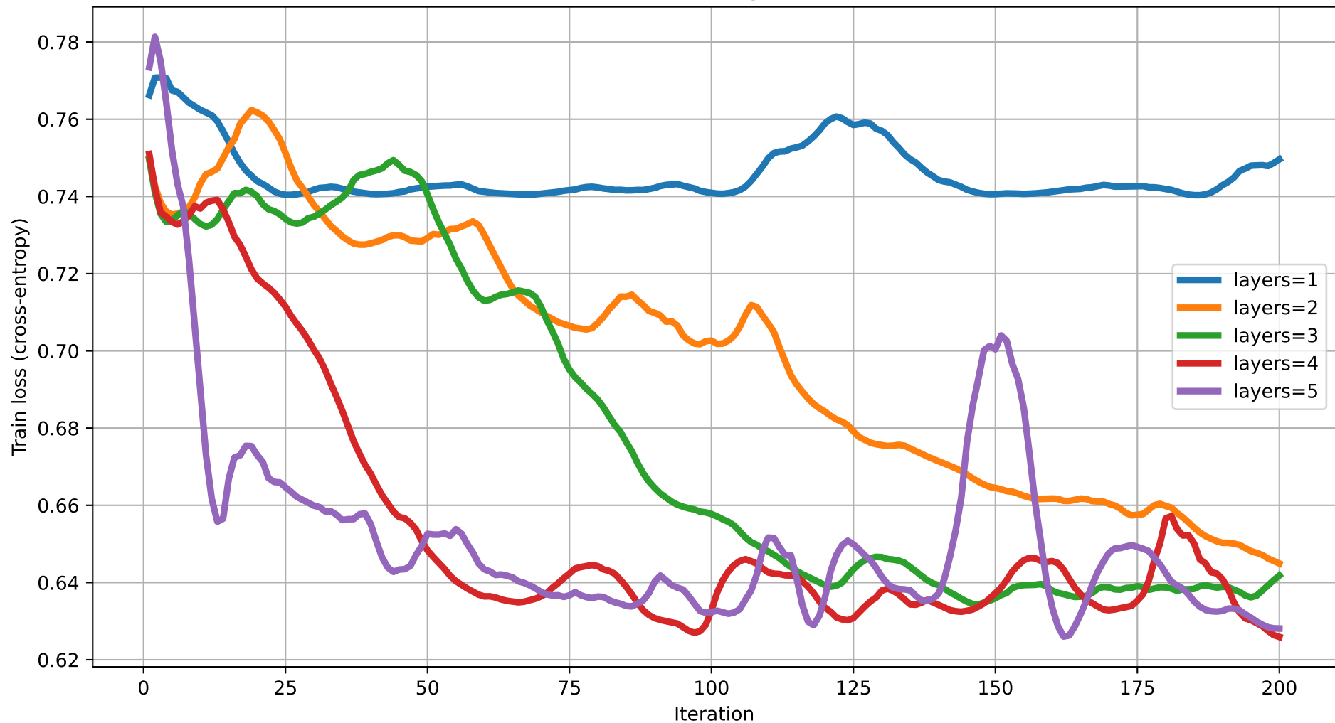
Train loss vs Iteration (dim=5) rot=RY, ent=full, gate=CNOT
