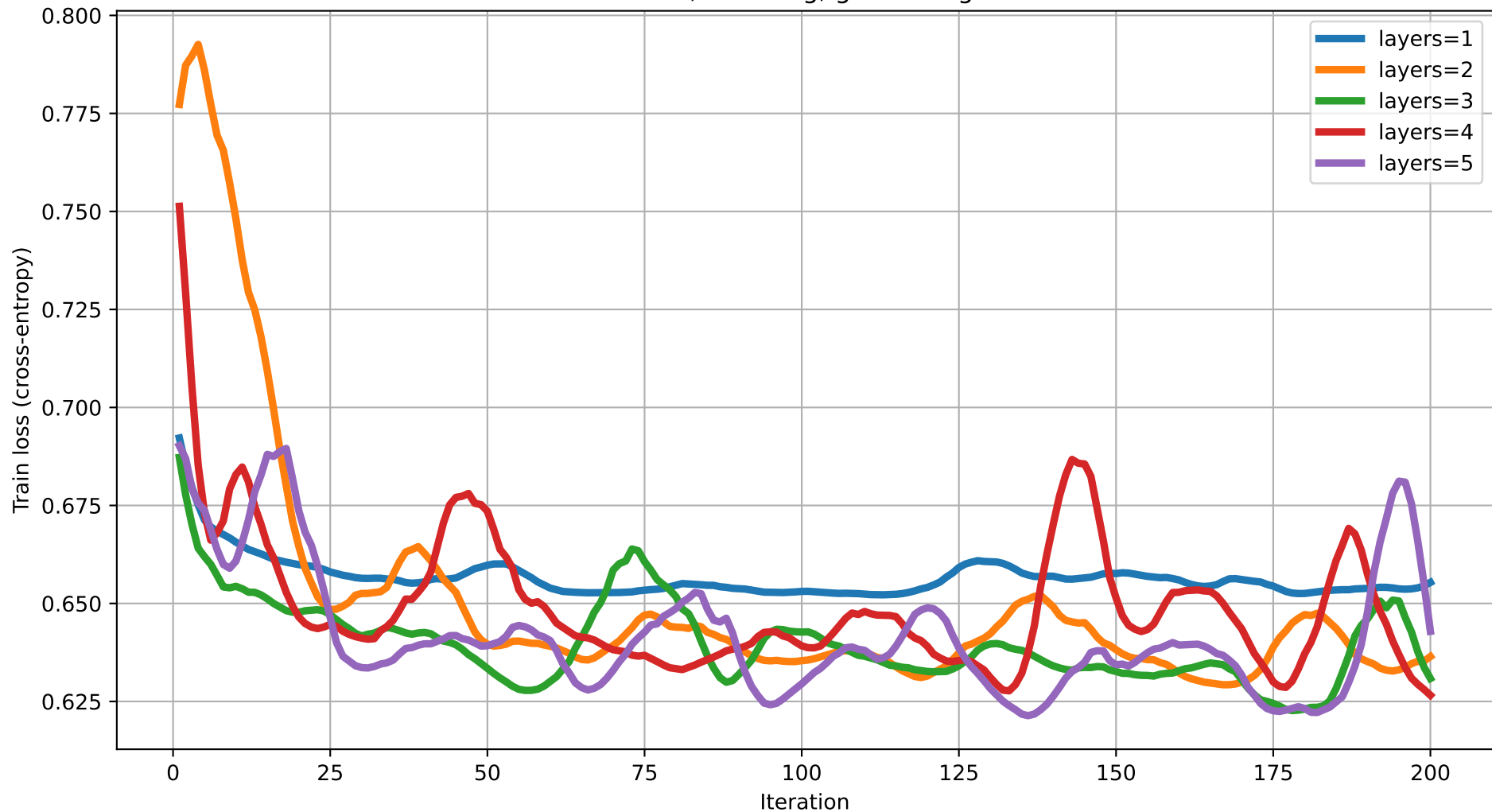
Train loss vs Iteration (dim=8) rot=RY, ent=ring, gate=IsingXX
