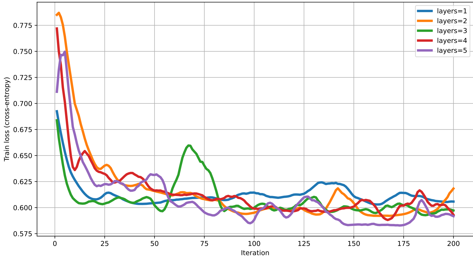
Train loss vs Iteration (dim=4) rot=RY, ent=ring, gate=lsingXX
