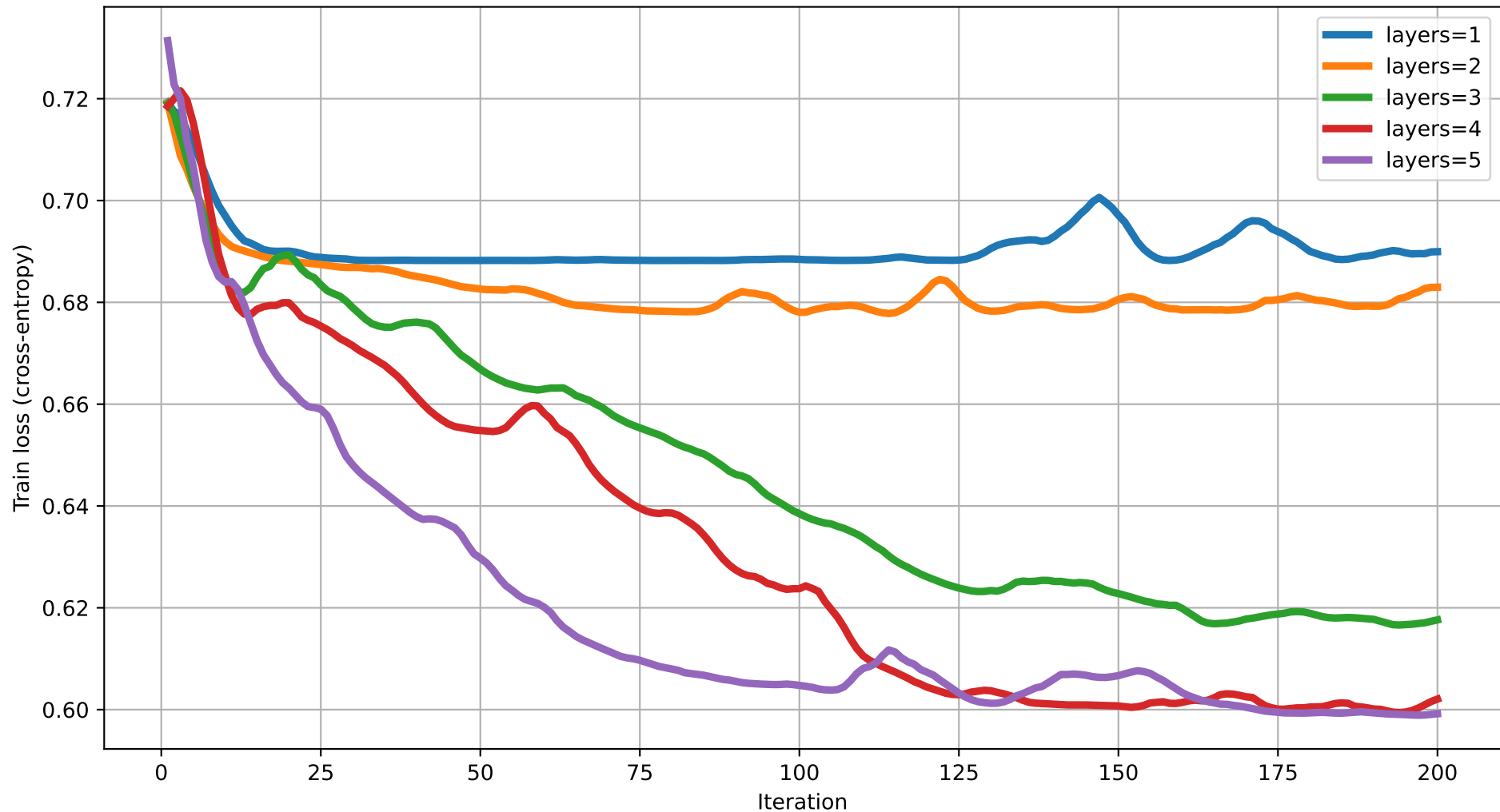
Train loss vs Iteration (degree=4) rot=RX, ent=ring, gate=CZ
