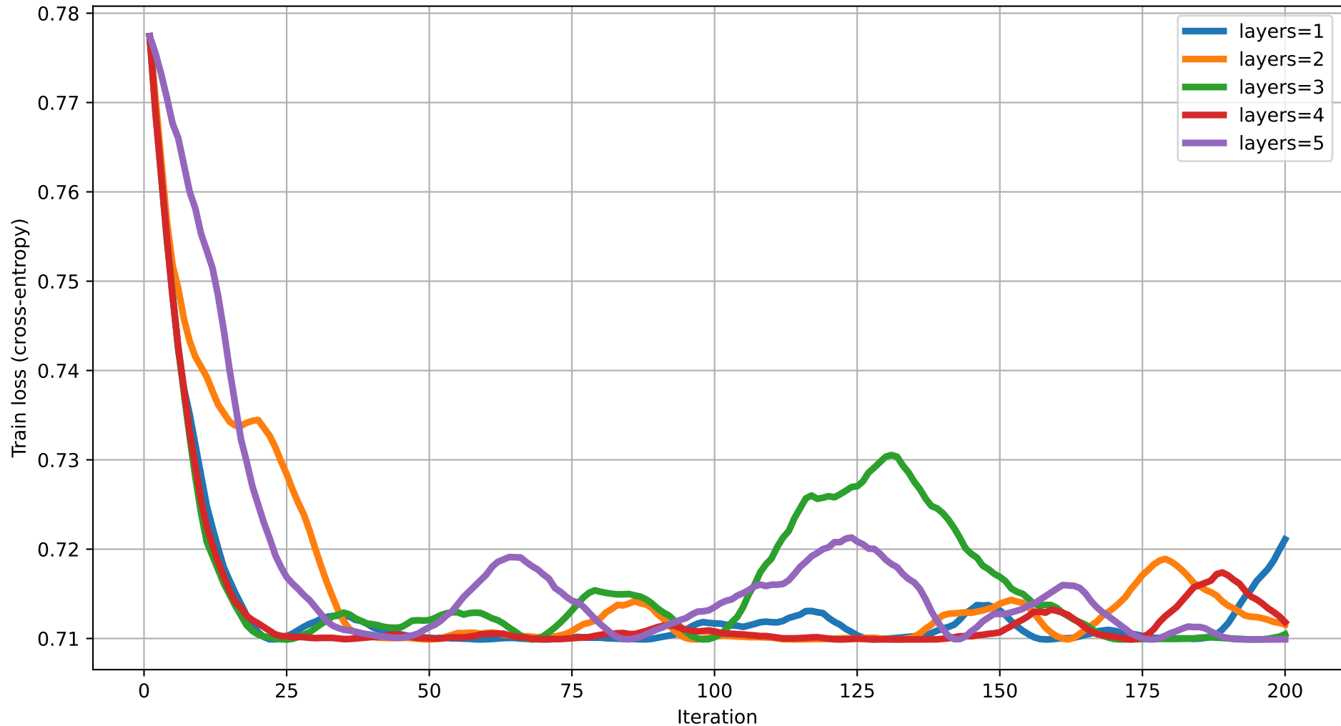
Train loss vs Iteration (dim=4) rot=RZ, ent=full, gate=CNOT
