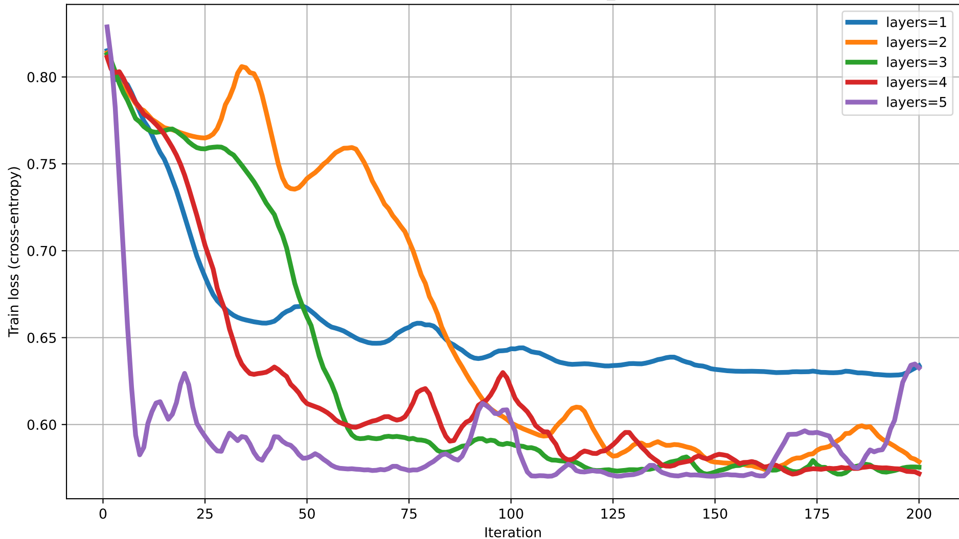
Train loss vs Iteration for different num_layers (dim=2)
