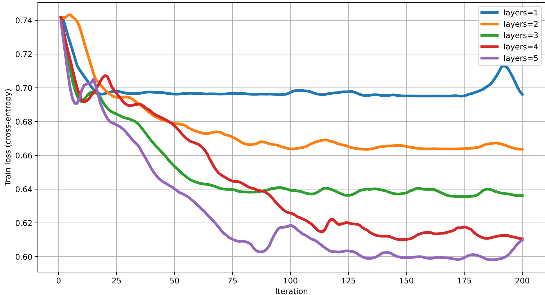
Train loss vs Iteration (degree=5) rot=RX, ent=full, gate=CZ
