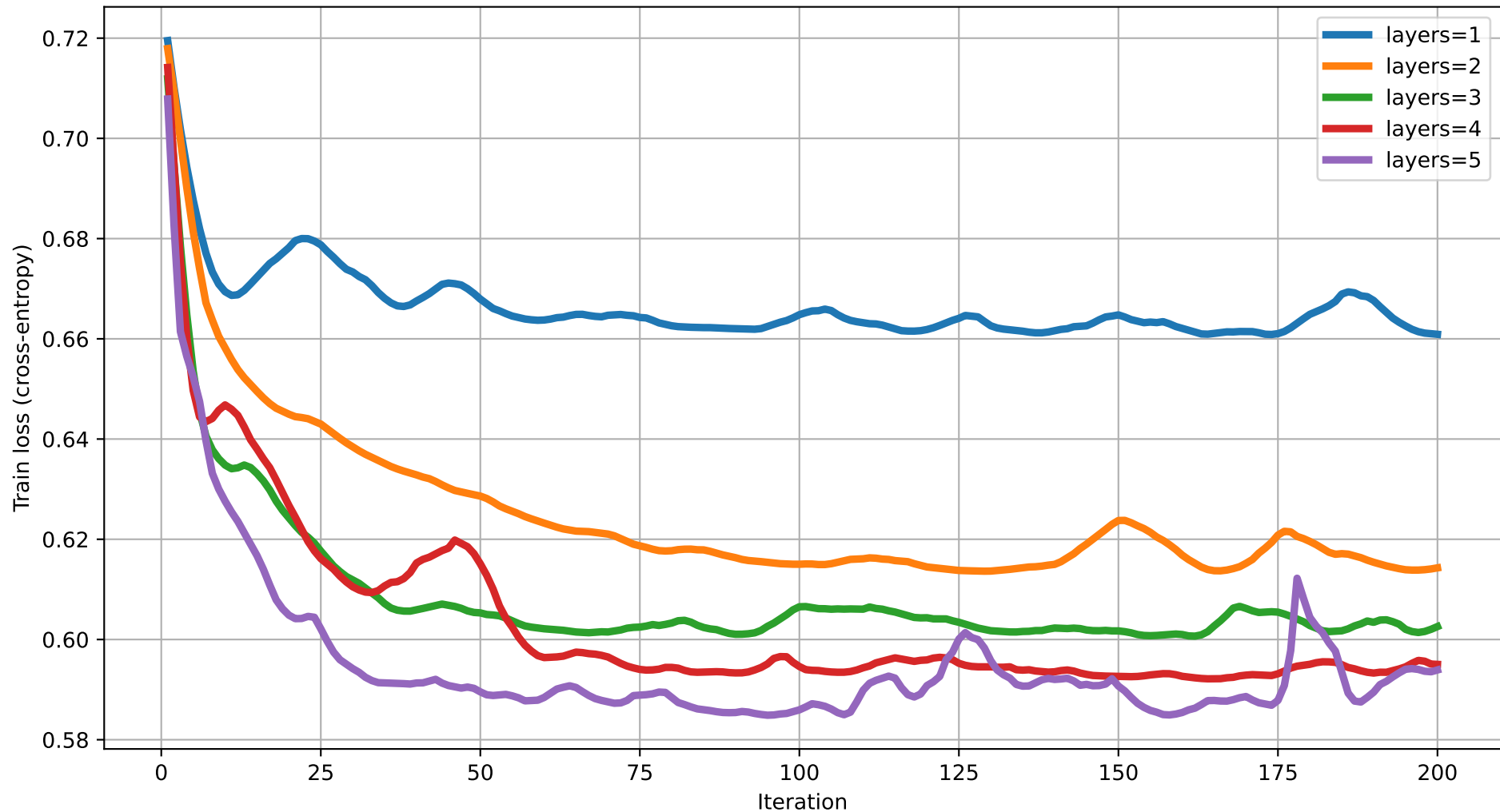
Train loss vs Iteration (degree=3) rot=RYZ, ent=chain, gate=CNOT
