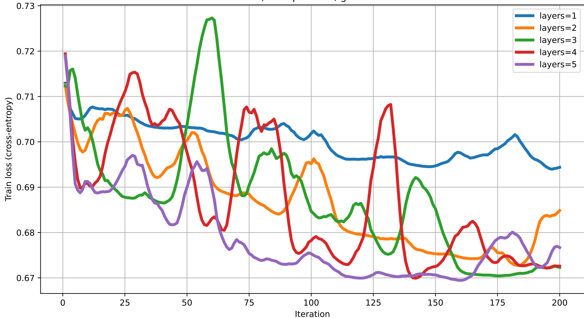
Train loss vs Iteration (dim=11) rot=RX, ent=pairwise, gate=CNOT
