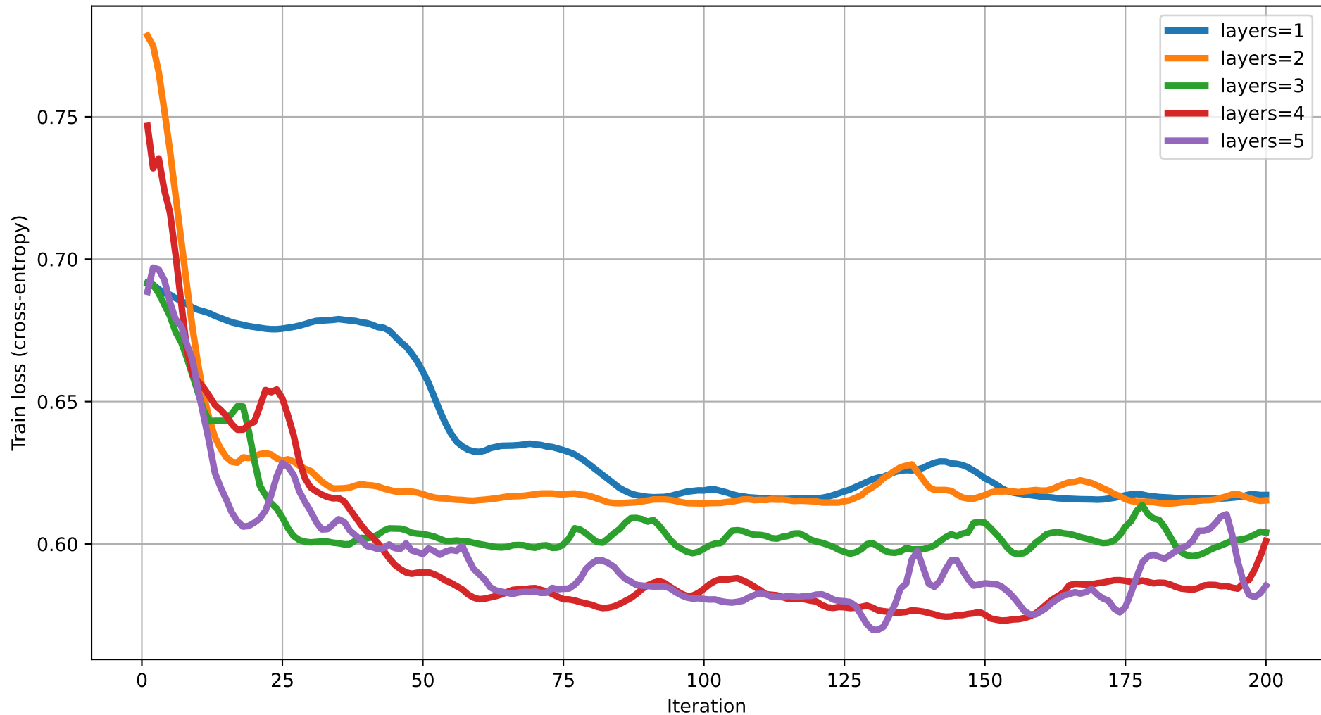
Train loss vs Iteration (dim=18) rot=Rot, ent=chain, gate=IsingXX
