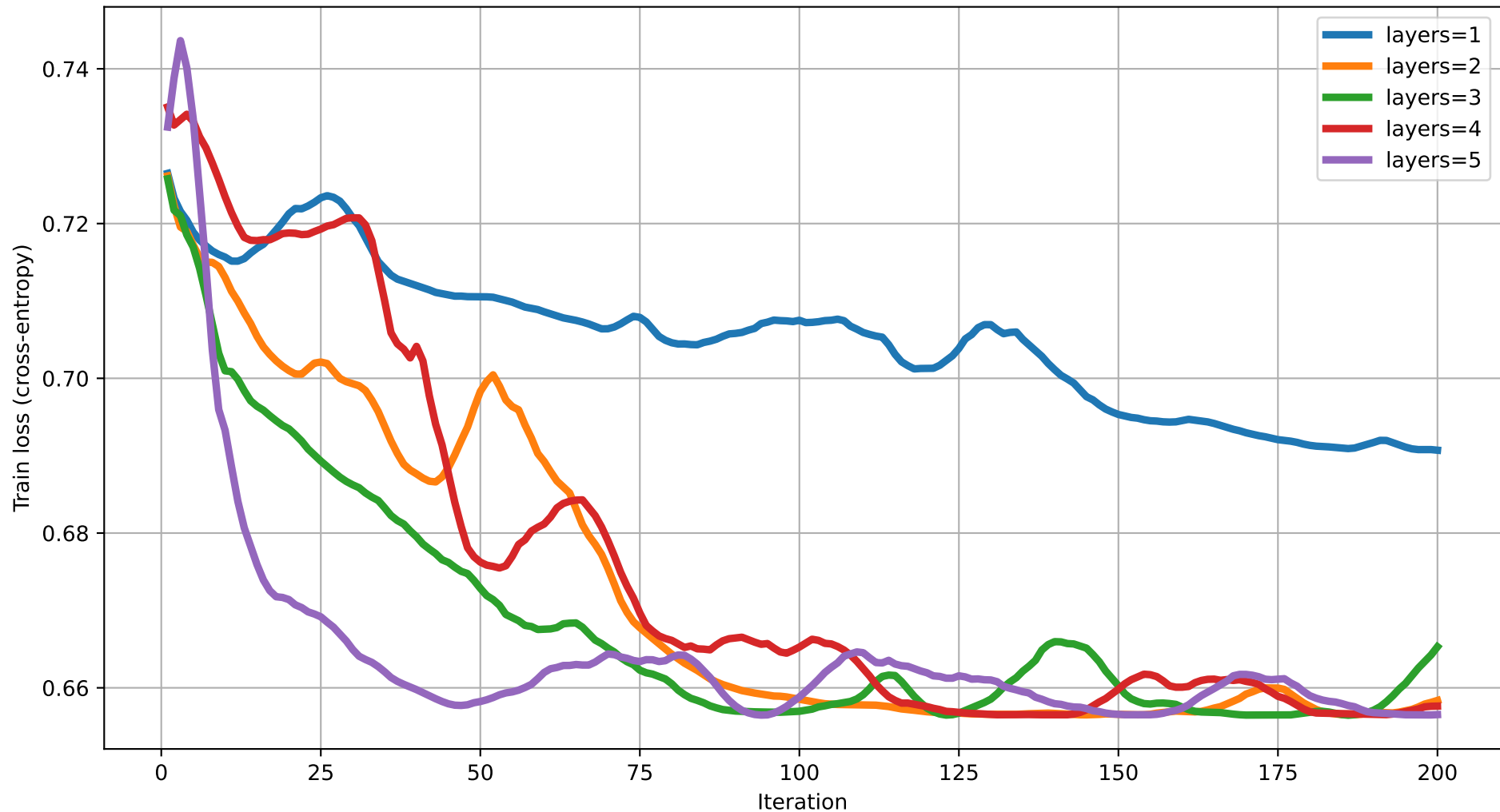
Train loss vs Iteration (dim=6) rot=RX, ent=pairwise, gate=CNOT
