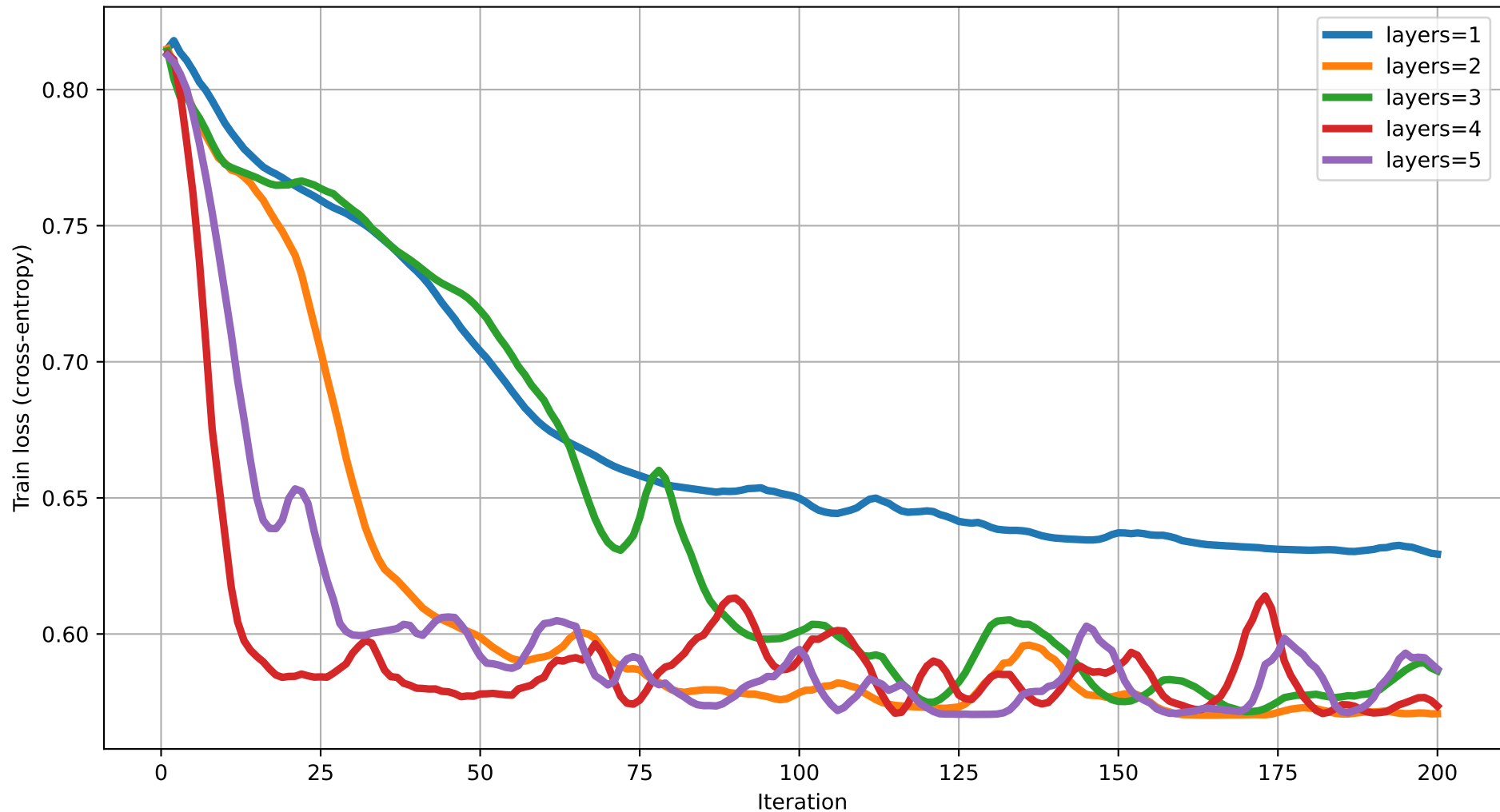
Train loss vs Iteration (dim=2) rot=RYZ, ent=full, gate=CZ
