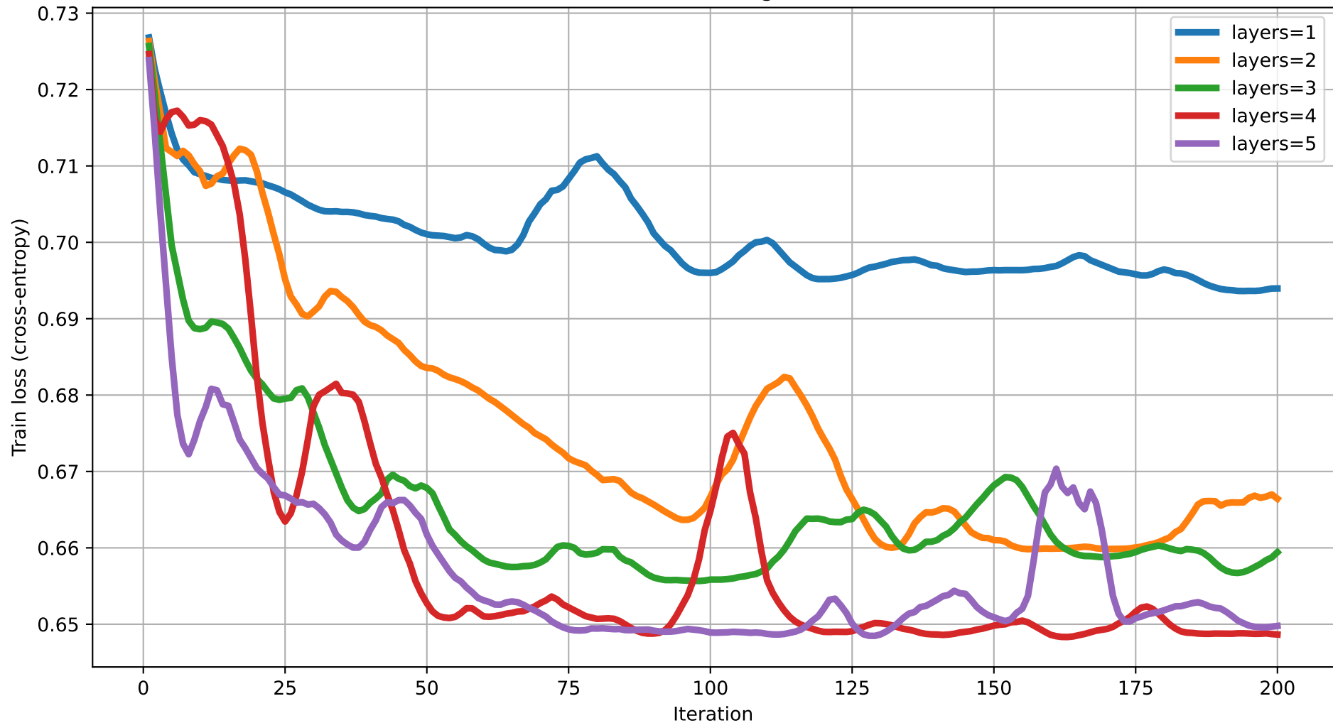
Train loss vs Iteration (dim=5) rot=RX, ent=chain, gate=CNOT
