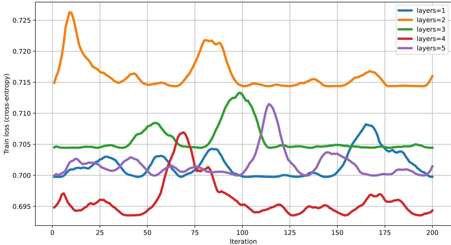
Train loss vs Iteration (dim=17) rot=RZ, ent=ring, gate=CNOT
