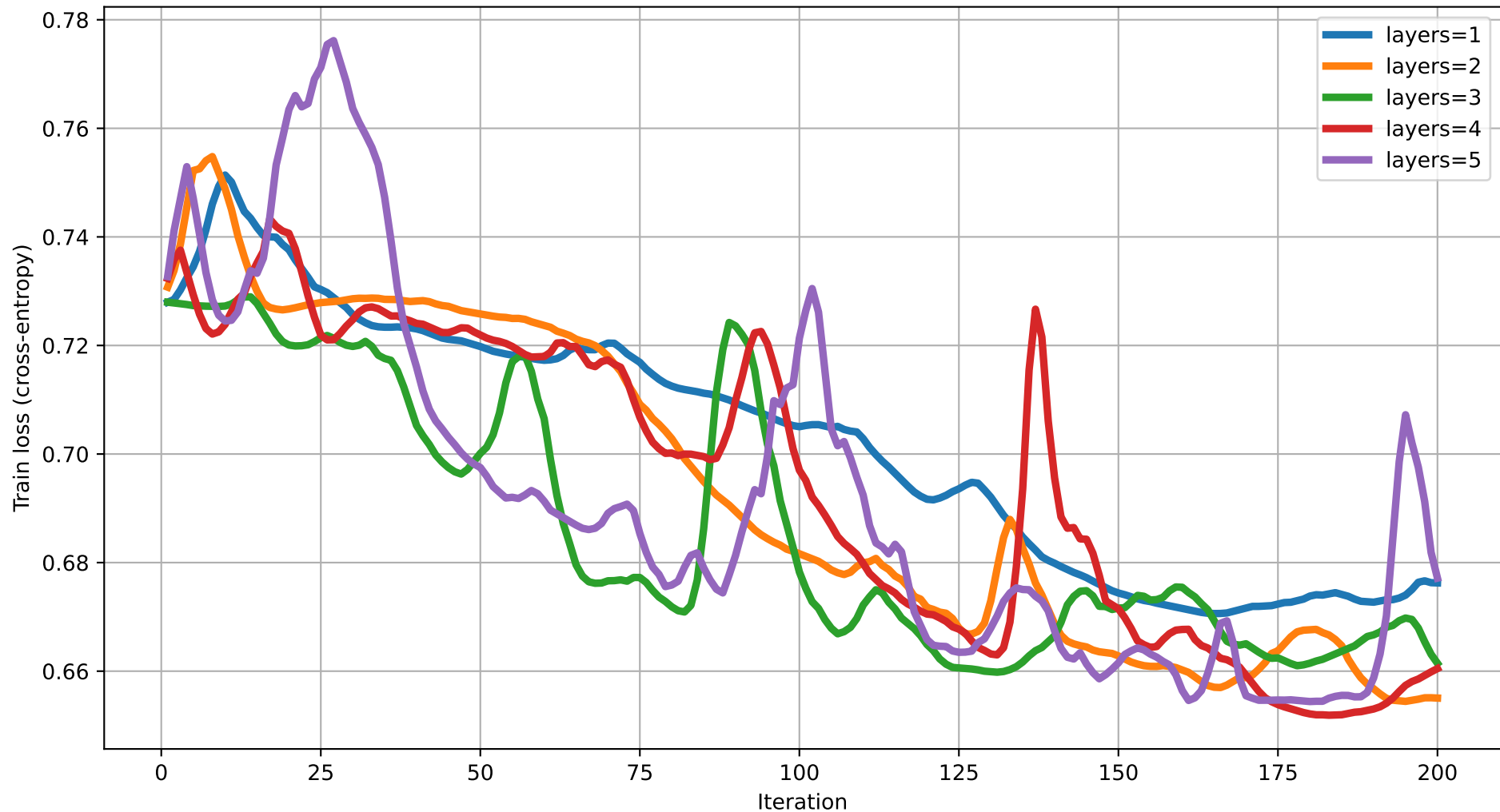
Train loss vs Iteration (dim=7) rot=Rot, ent=pairwise, gate=CZ
