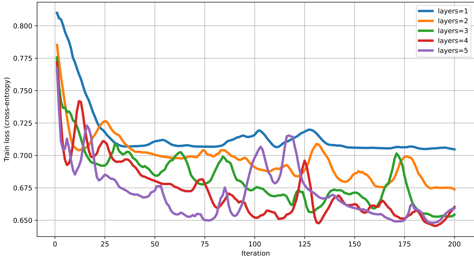
Train loss vs Iteration (dim=9) rot=Rot, ent=chain, gate=CNOT
