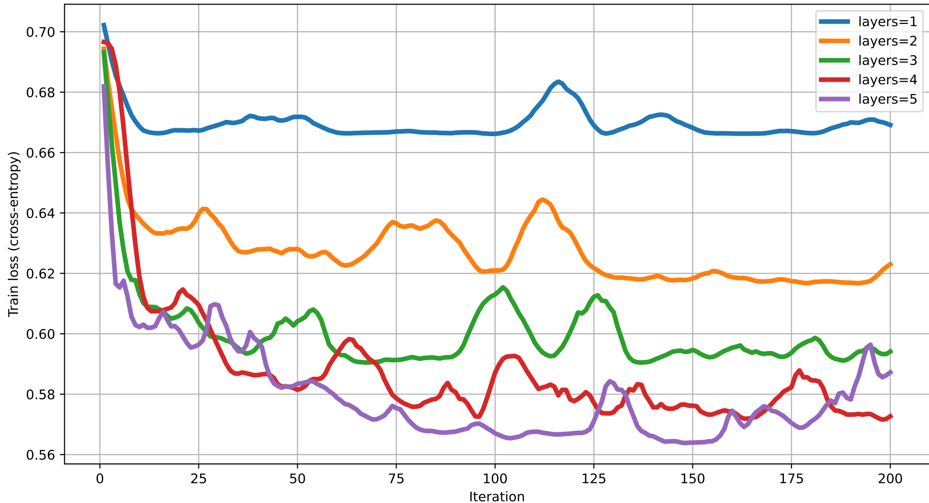
Train loss vs Iteration (dim=10) rot=Rot, ent=chain, gate=CNOT
