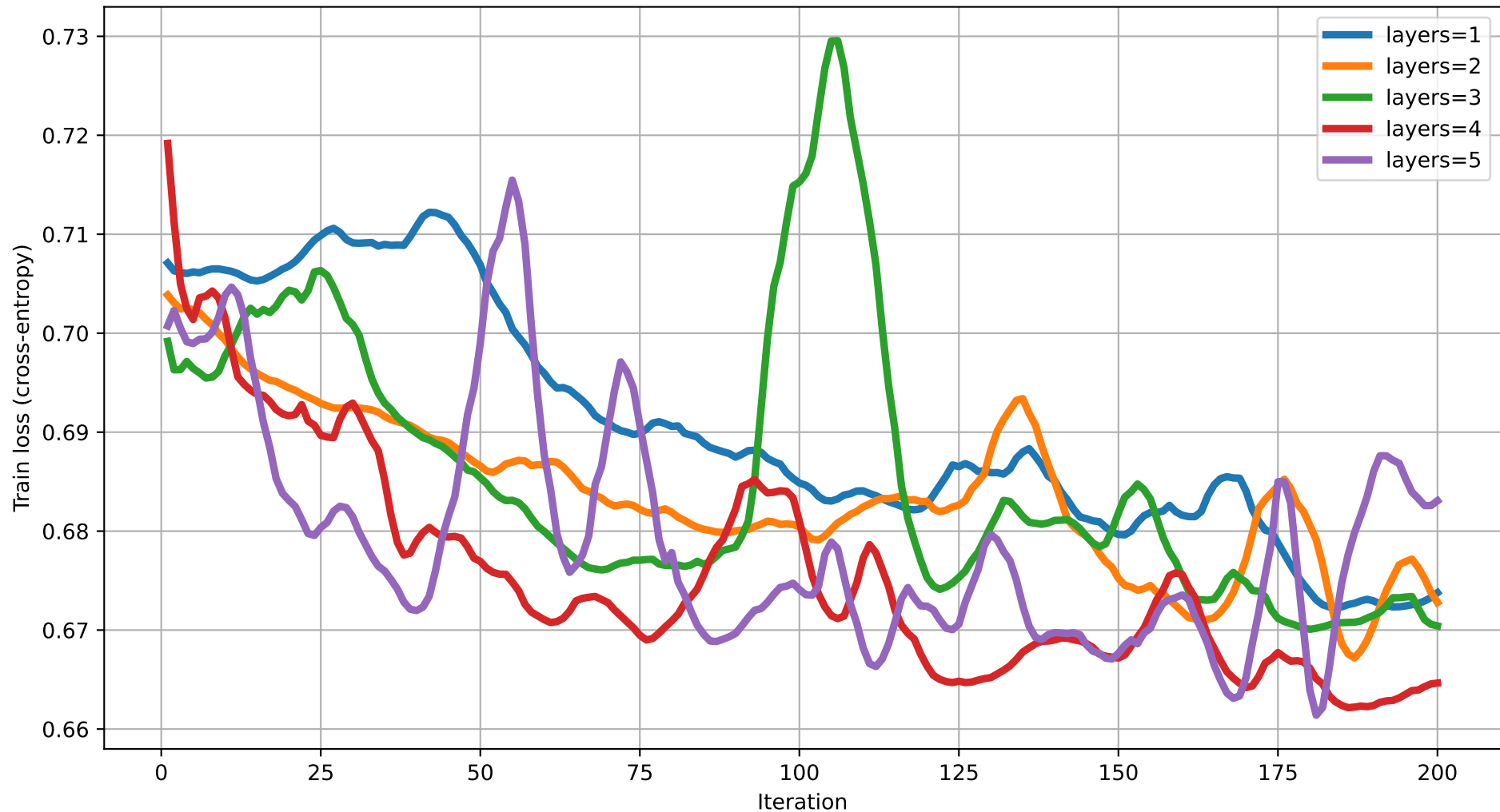
Train loss vs Iteration (dim=12) rot=RYZ, ent=ring, gate=CNOT
