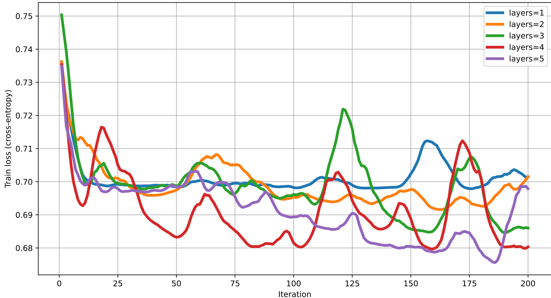
Train loss vs Iteration (dim=19) rot=RX, ent=full, gate=CZ
