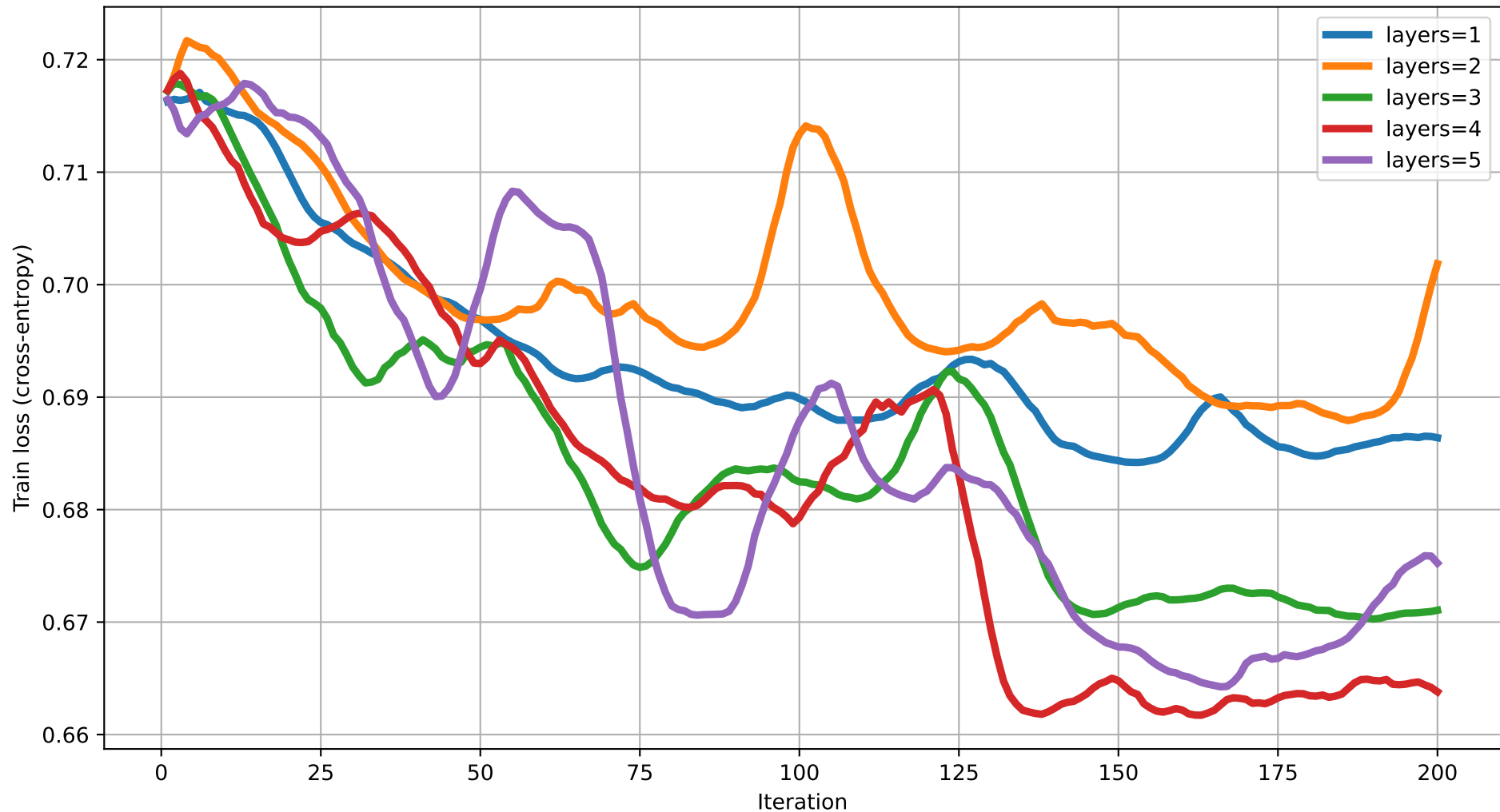
Train loss vs Iteration (dim=7) rot=RX, ent=chain, gate=CZ
