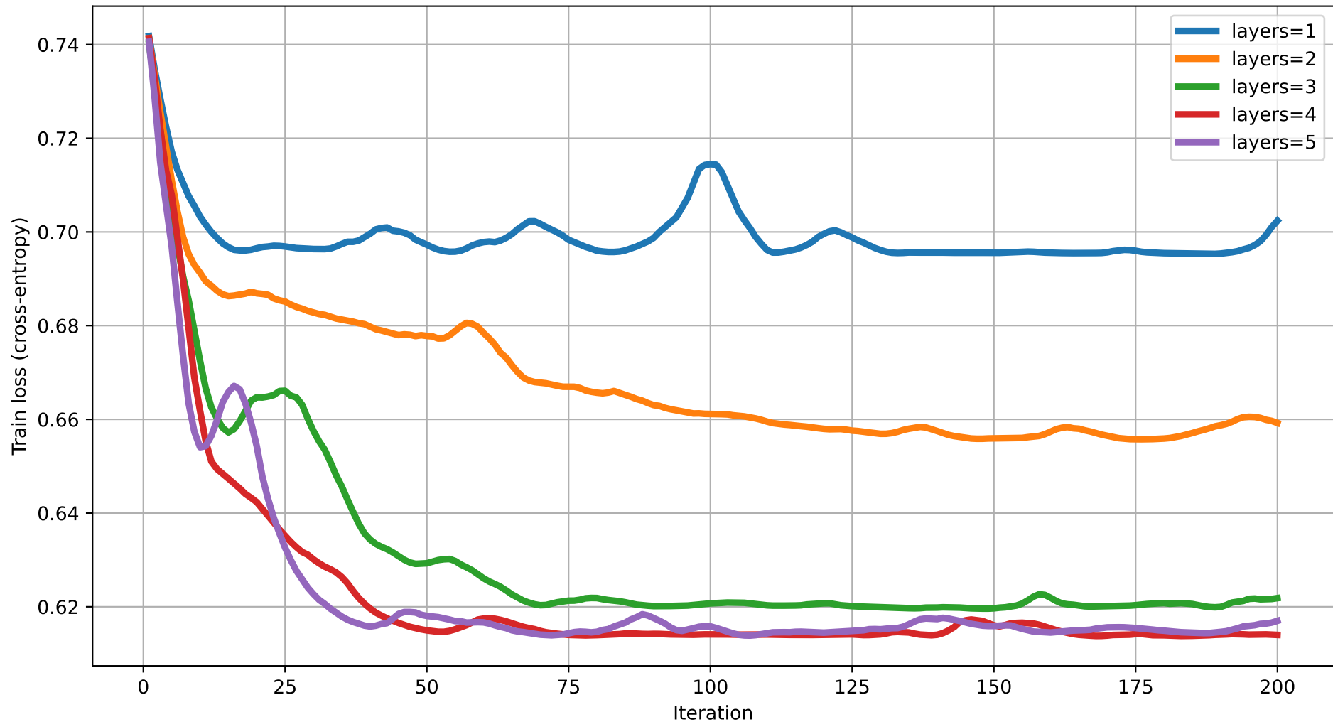
Train loss vs Iteration (degree=5) rot=RX, ent=chain, gate=CNOT
