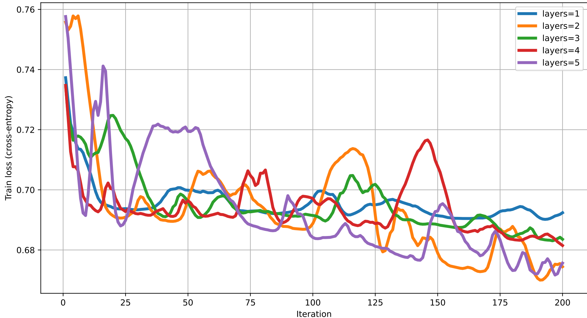
Train loss vs Iteration (dim=16) rot=Rot, ent=chain, gate=CZ
