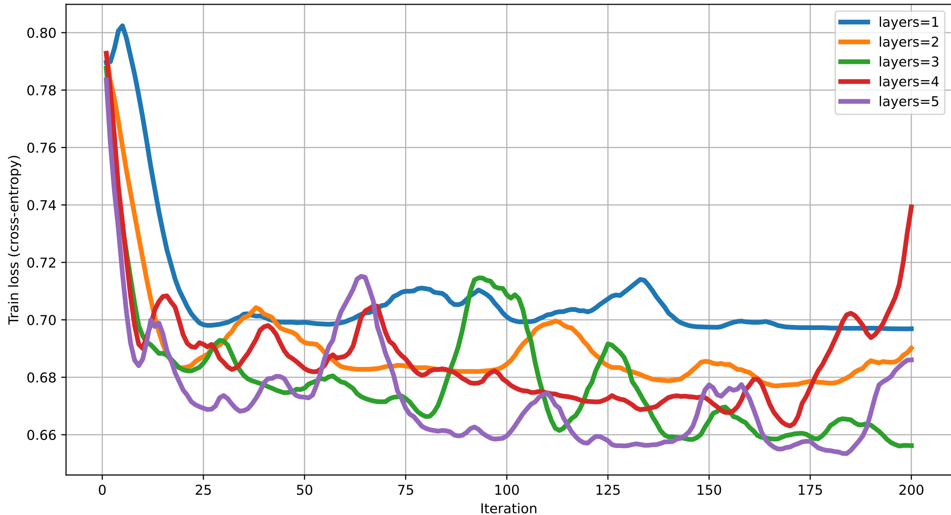
Train loss vs Iteration (dim=2) rot=RYZ, ent=chain, gate=CZ
