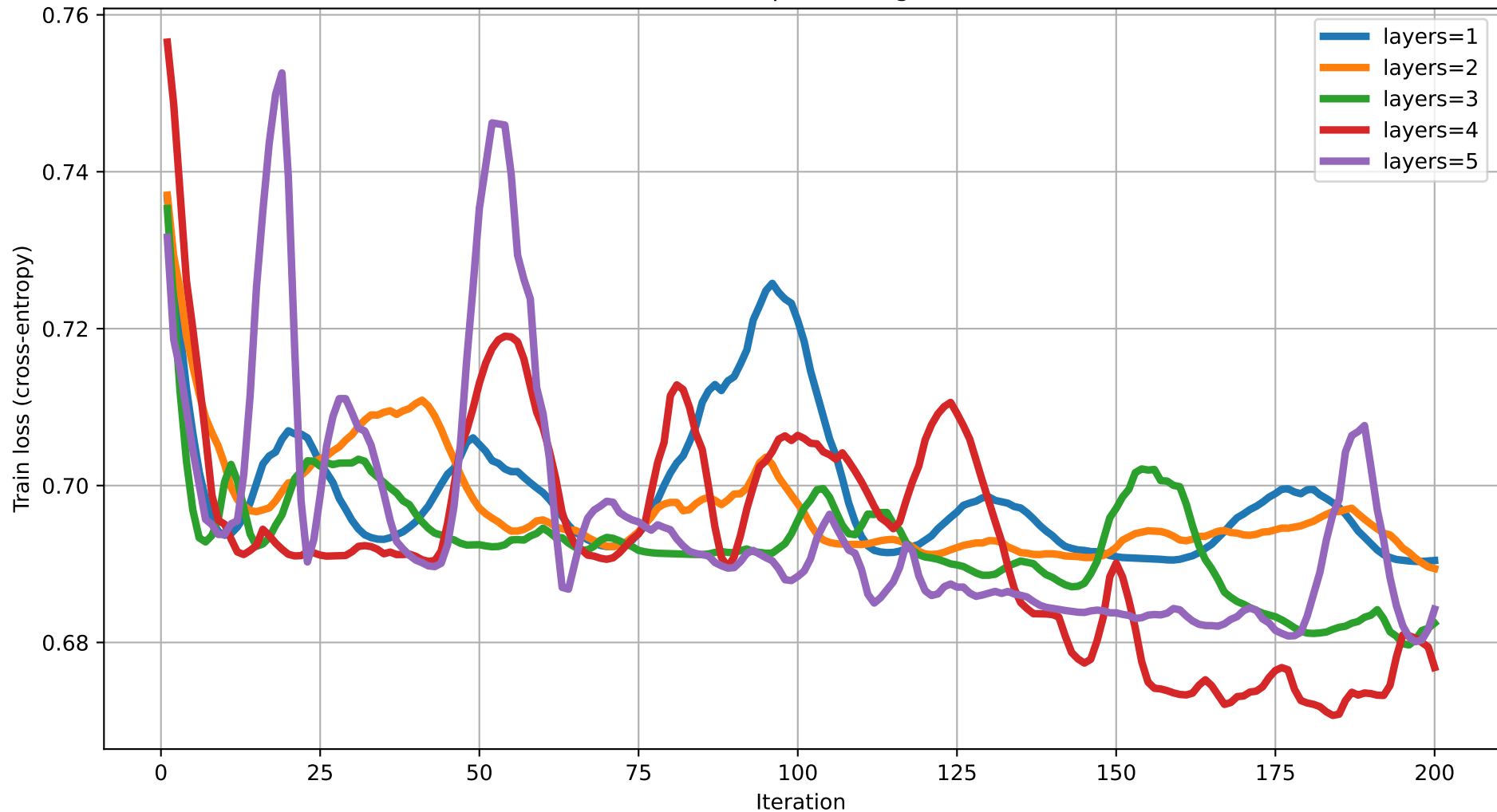
Train loss vs Iteration (dim=16) rot=Rot, ent=pairwise, gate=CZ
