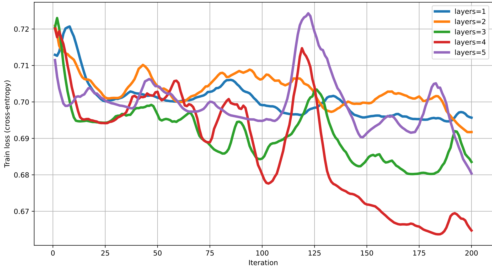
Train loss vs Iteration (dim=11) rot=RX, ent=full, gate=CZ
