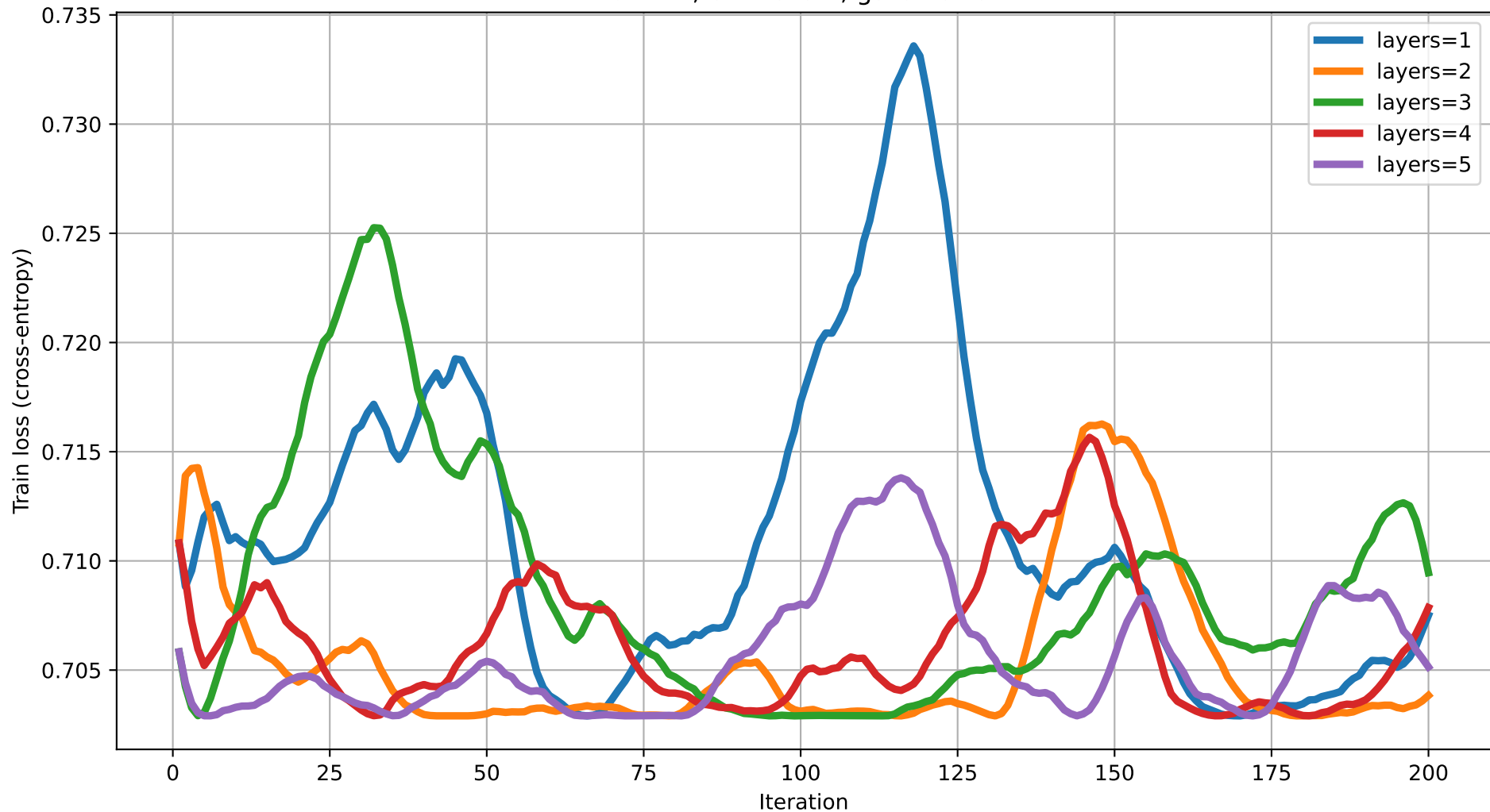
Train loss vs Iteration (dim=12) rot=RZ, ent=chain, gate=CNOT
