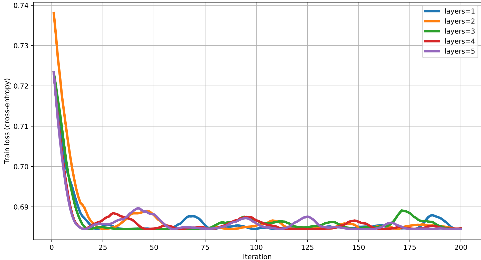
Train loss vs Iteration (degree=3) rot=RZ, ent=pairwise, gate=CNOT
