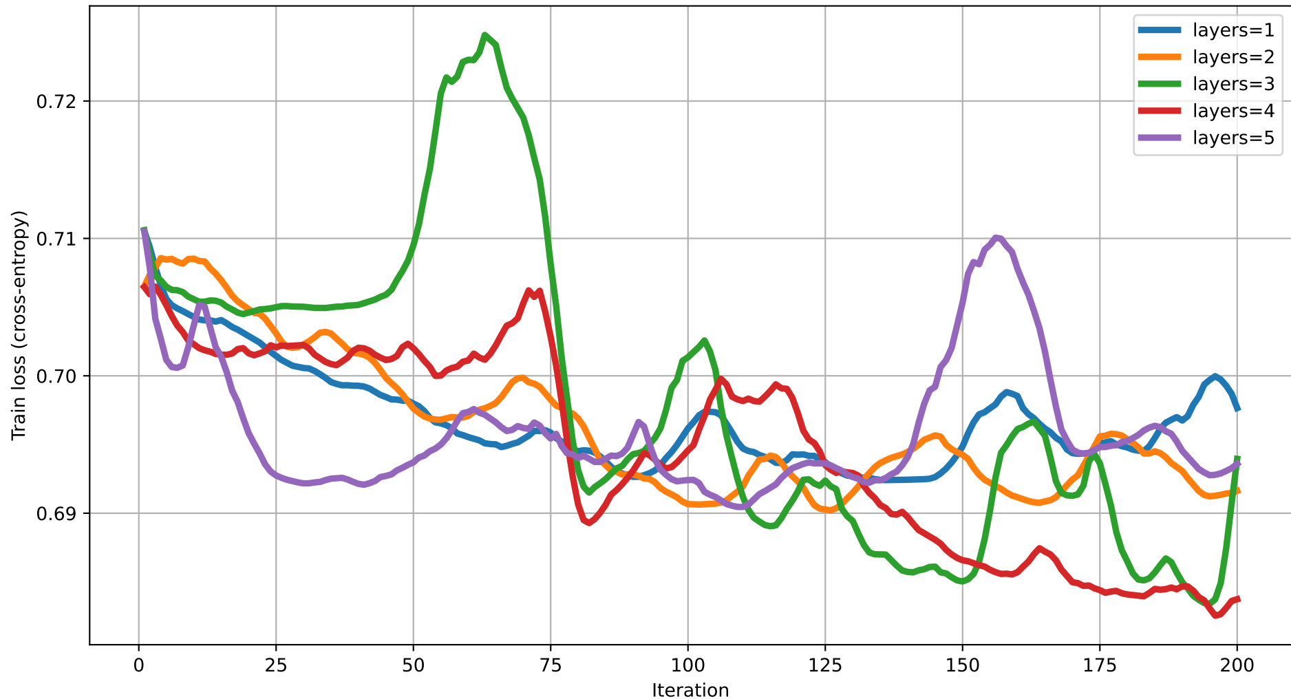
Train loss vs Iteration (dim=14) rot=RX, ent=pairwise, gate=CZ
