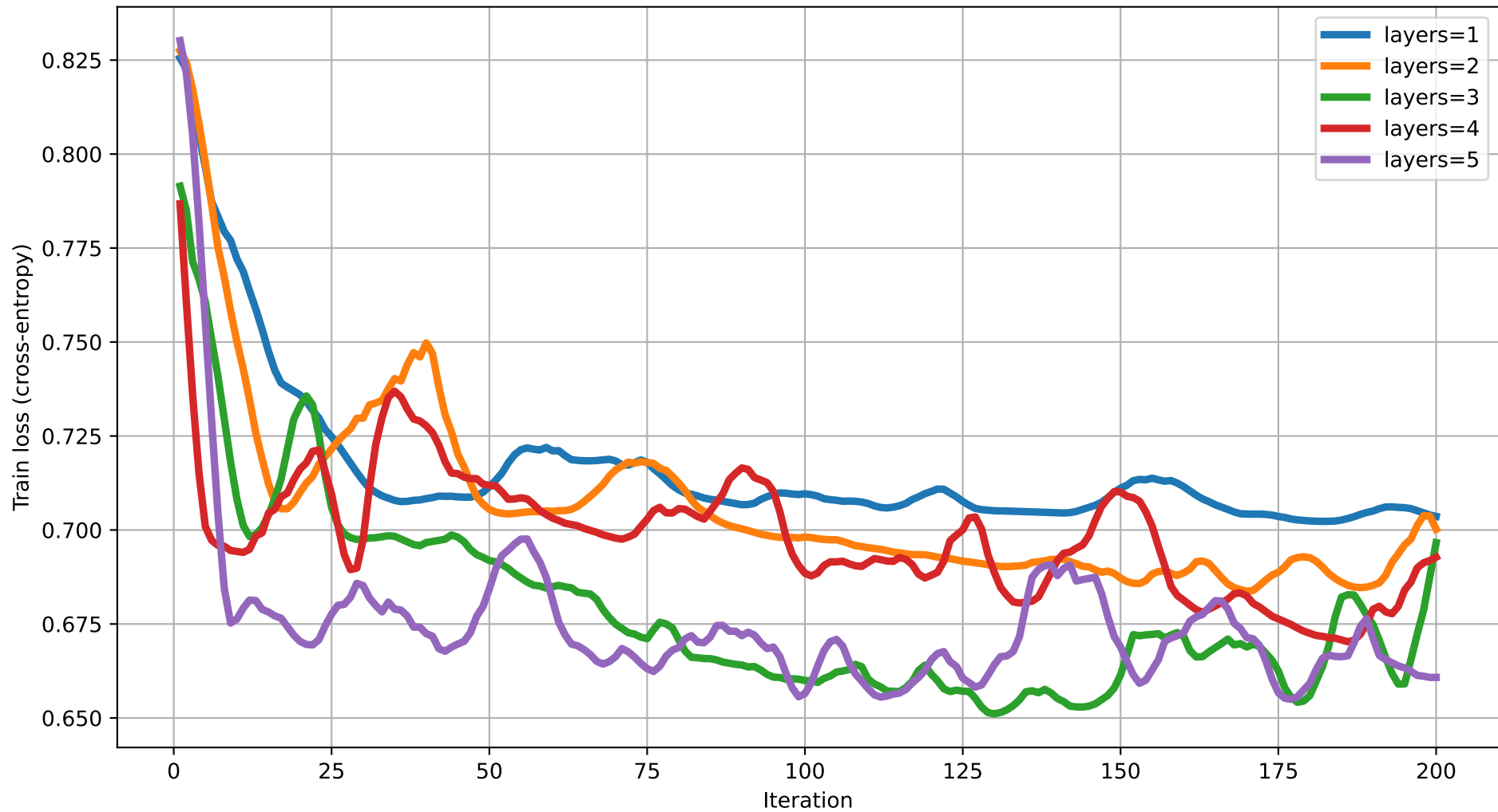
Train loss vs Iteration (dim=8) rot=Rot, ent=full, gate=CNOT
