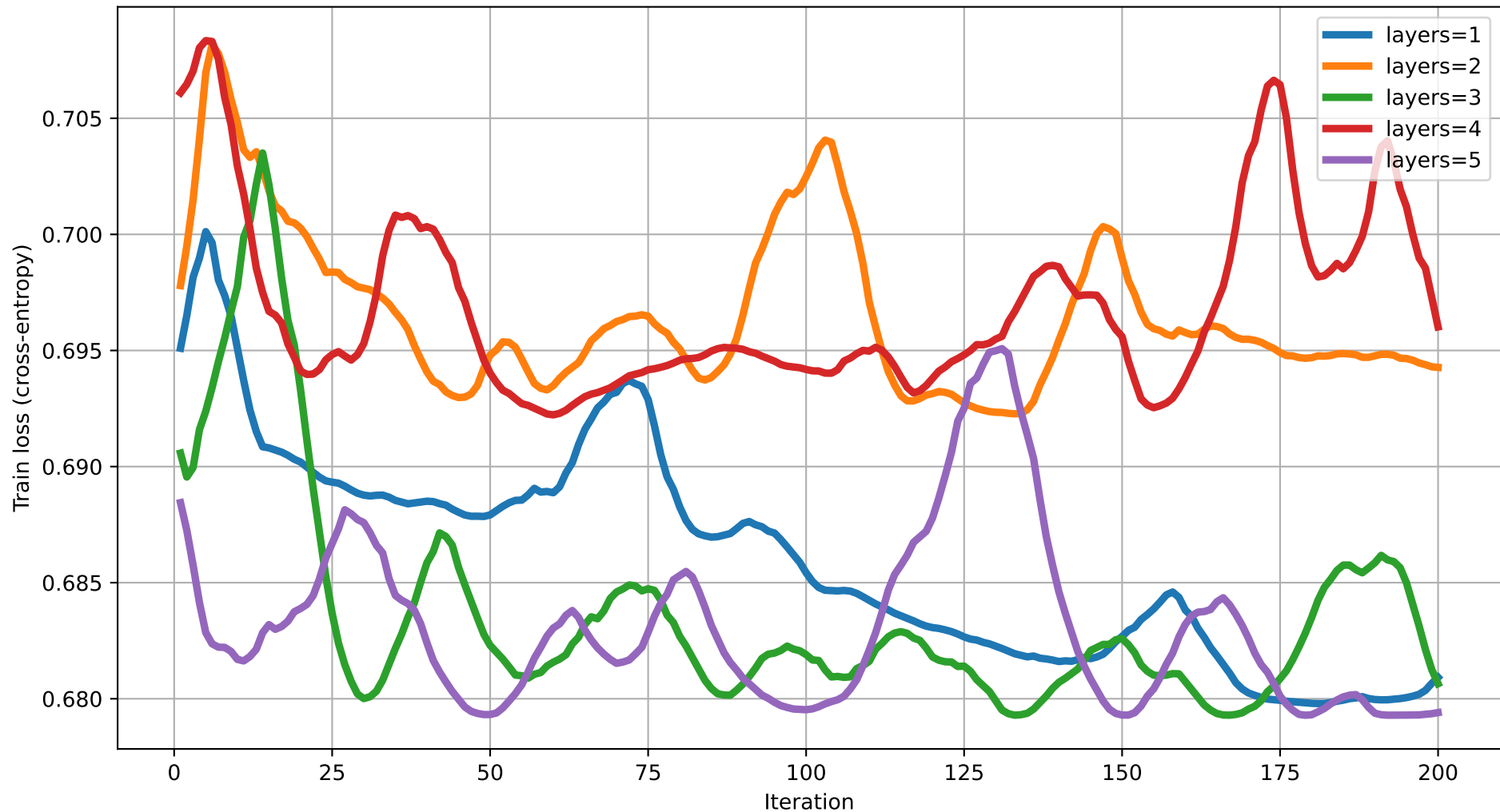
Train loss vs Iteration (dim=14) rot=RX, ent=pairwise, gate=IsingXX
