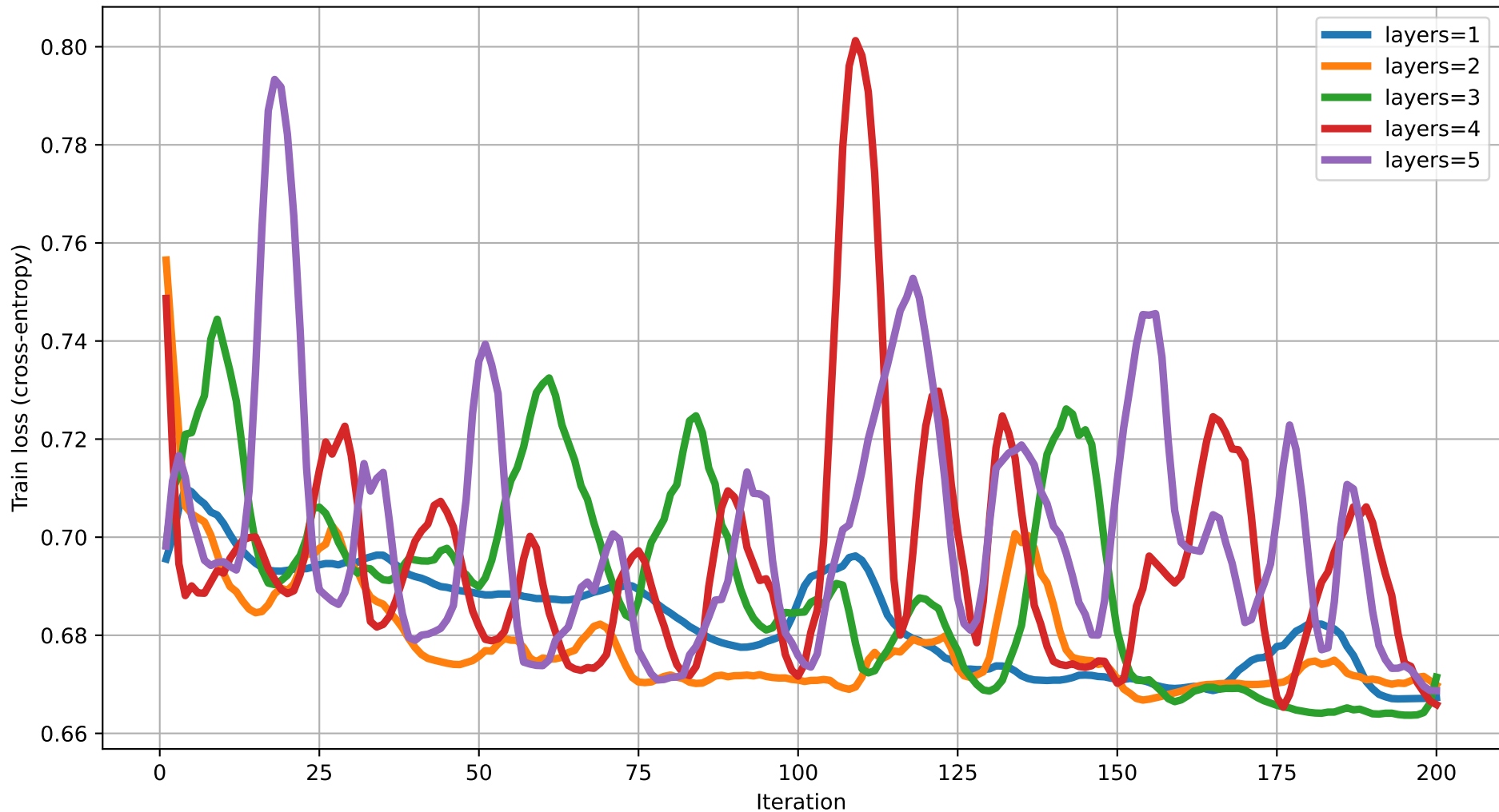
Train loss vs Iteration (dim=17) rot=Rot, ent=pairwise, gate=IsingXX
