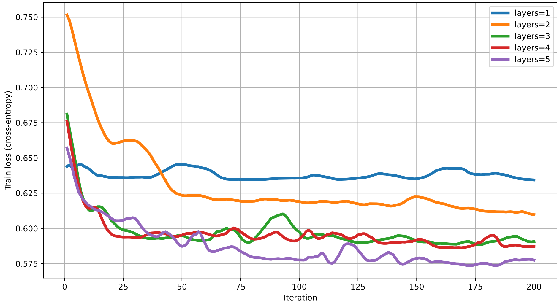
Train loss vs Iteration (degree=3) rot=RY, ent=ring, gate=CNOT
