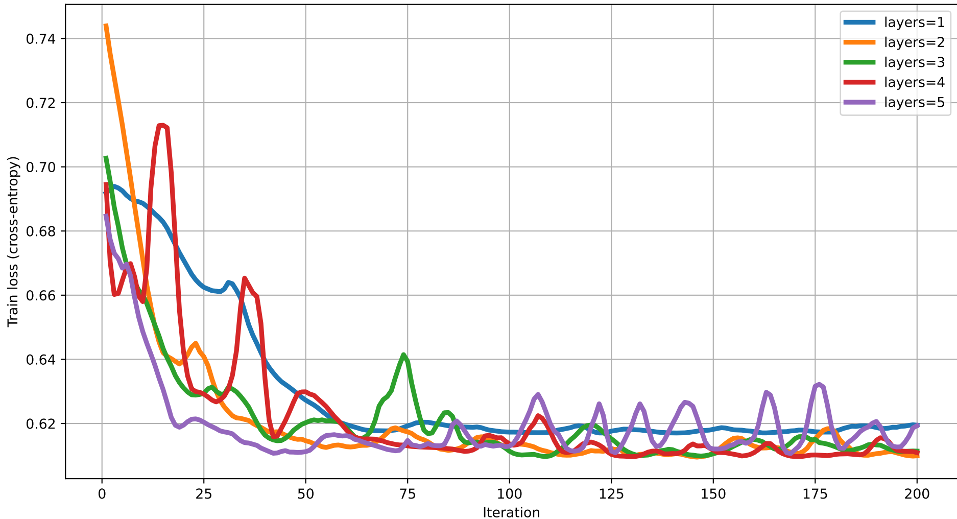
Train loss vs Iteration (degree=4) rot=Rot, ent=pairwise, gate=IsingXX
