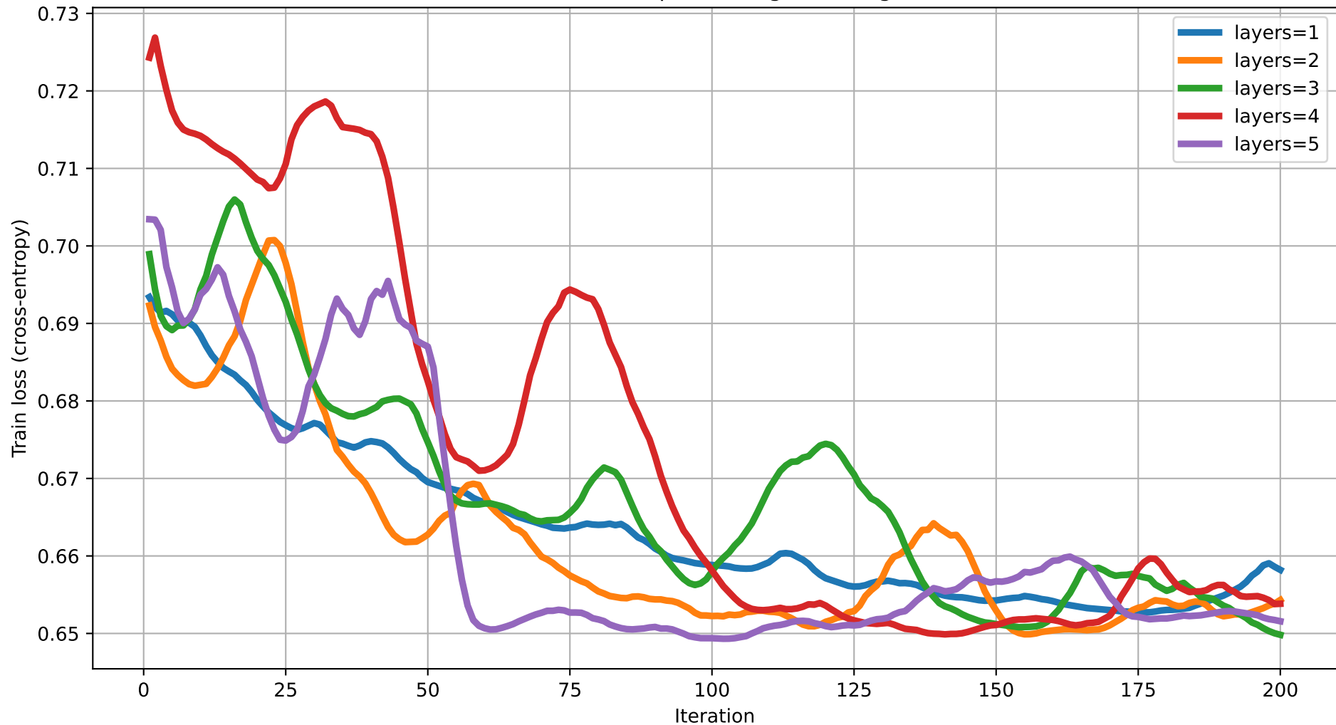
Train loss vs Iteration (dim=7) rot=RZ, ent=pairwise, gate=IsingXX
