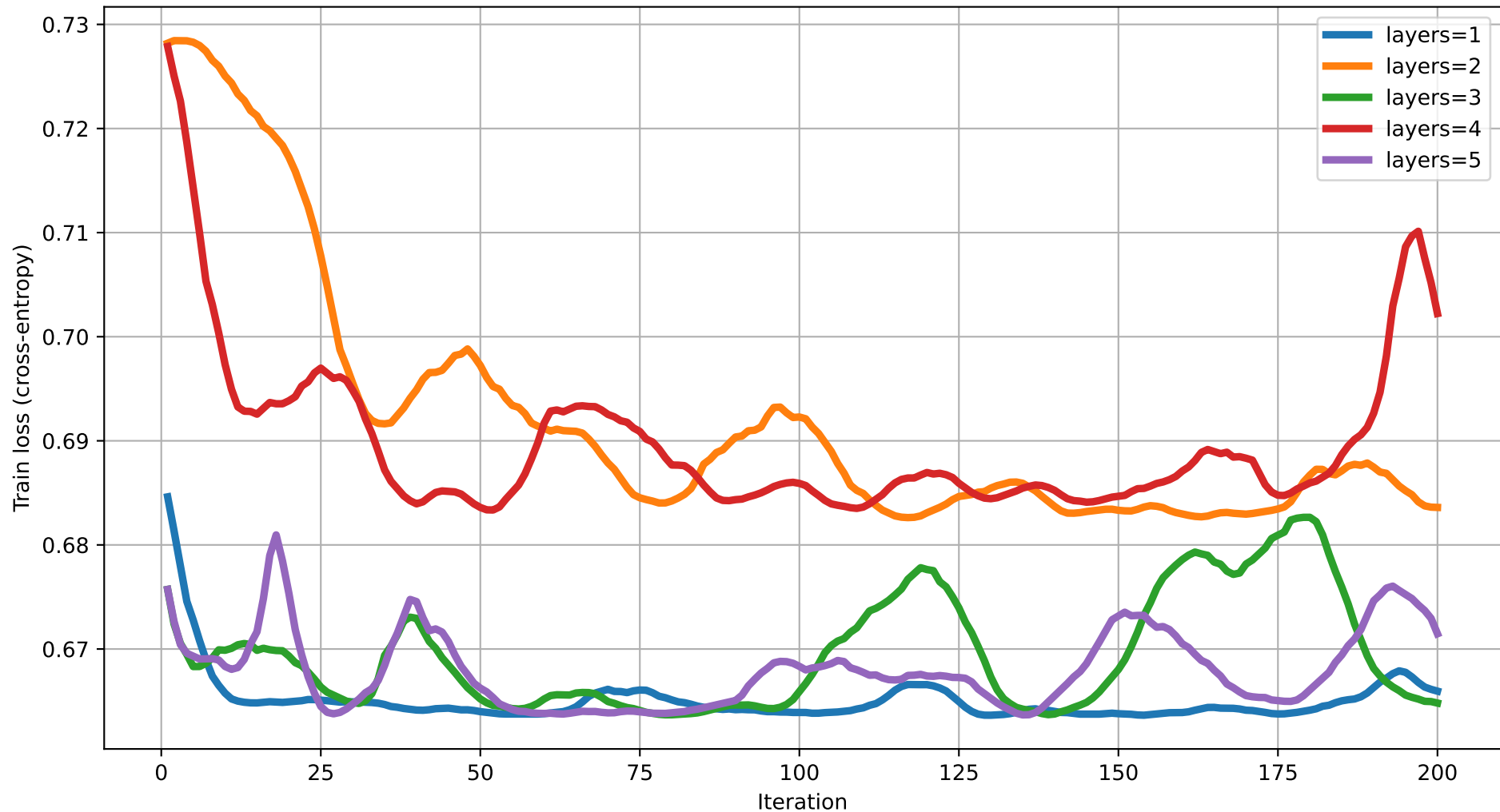
Train loss vs Iteration (dim=7) rot=RX, ent=ring, gate=IsingXX
