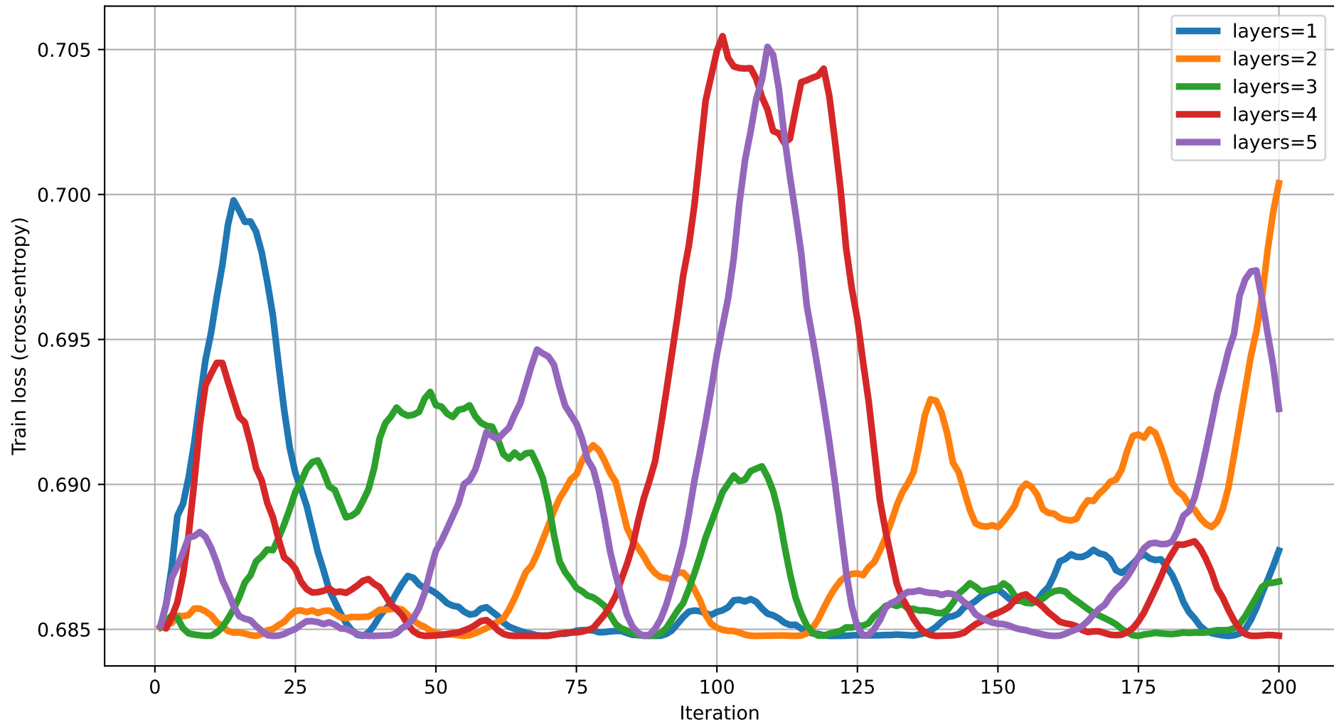
Train loss vs Iteration (dim=15) rot=RZ, ent=pairwise, gate=CNOT
