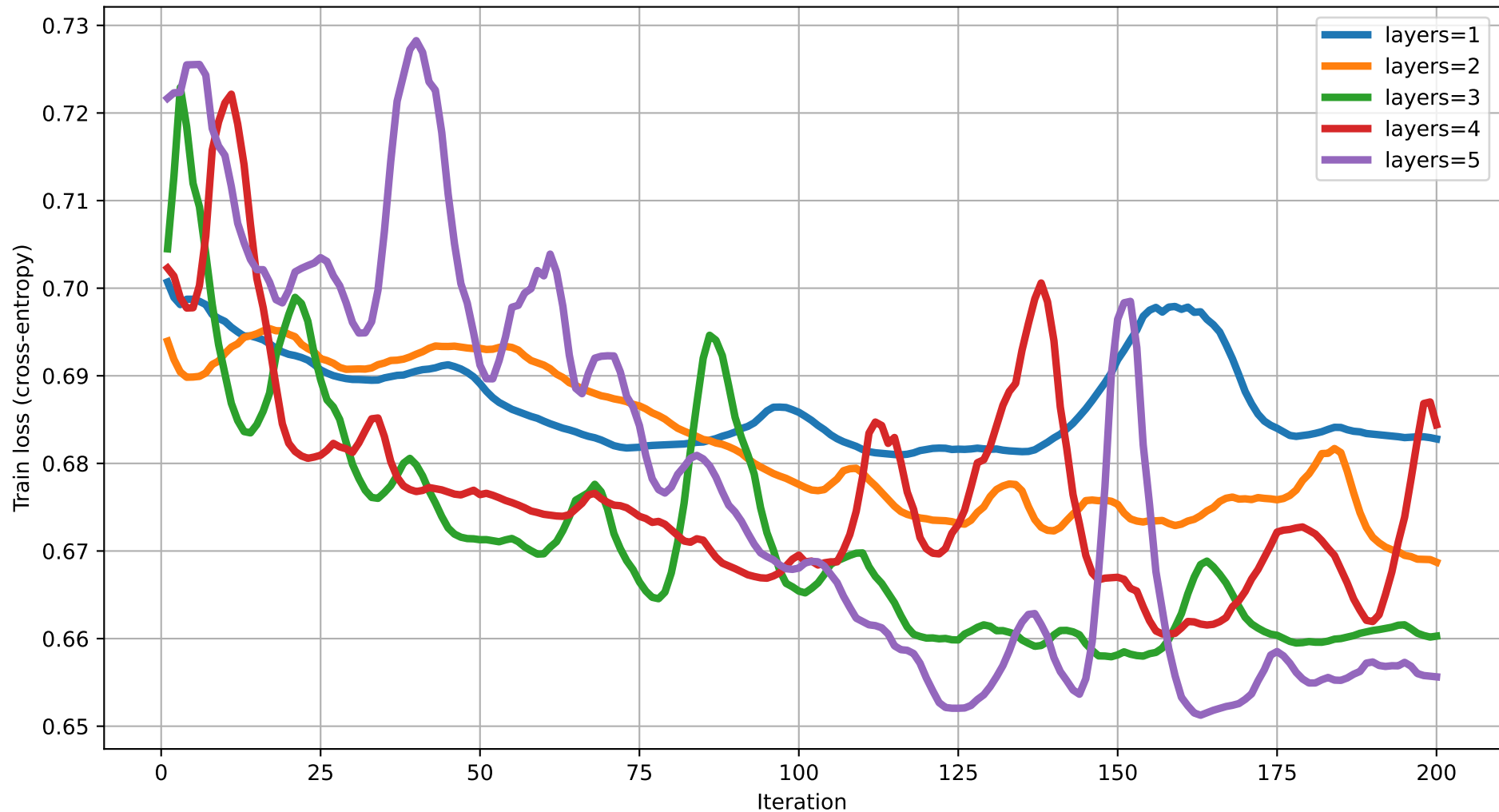
Train loss vs Iteration (dim=11) rot=RY, ent=ring, gate=CNOT
