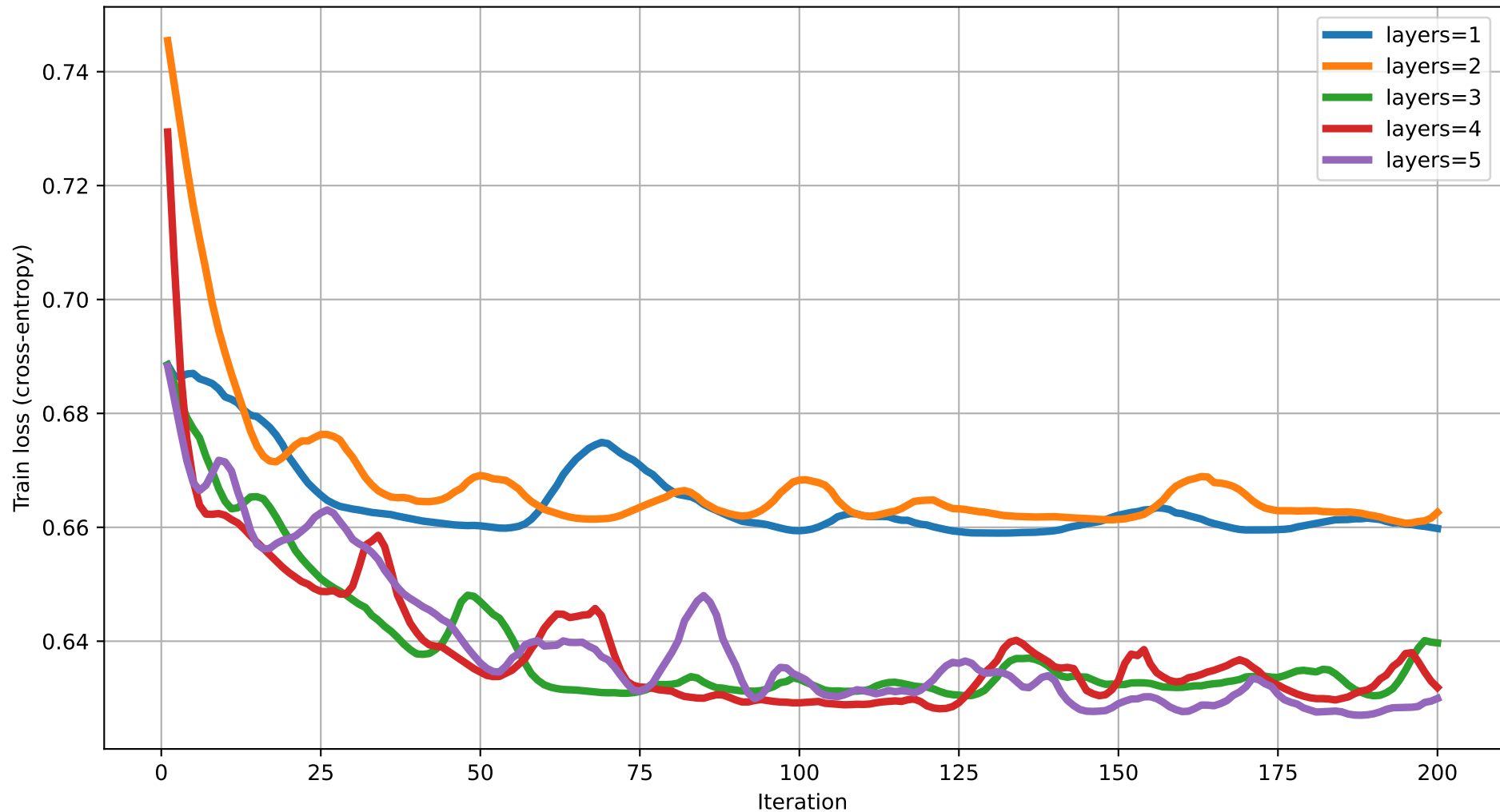
Train loss vs Iteration (degree=5) rot=RZ, ent=full, gate=IsingXX
