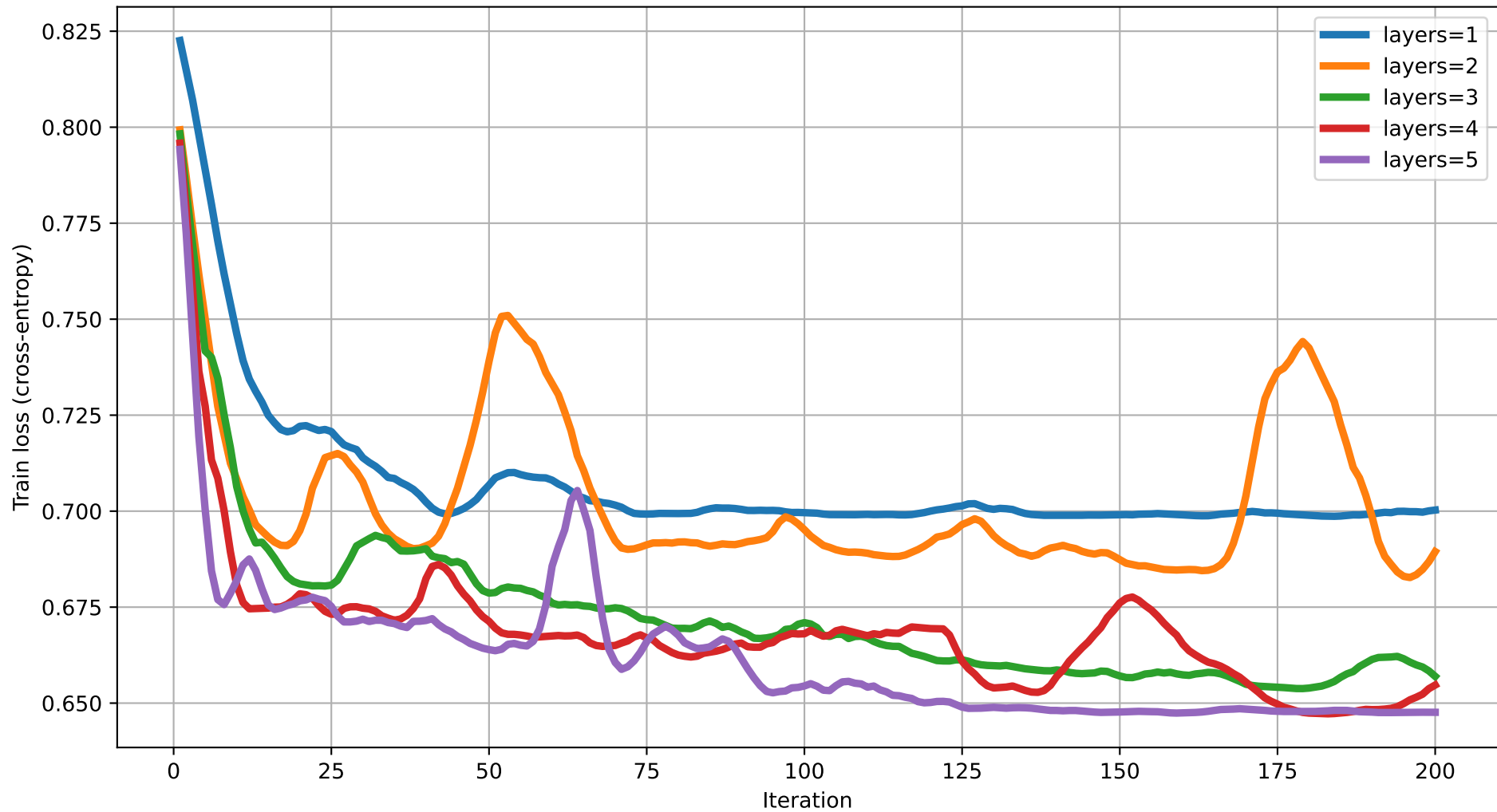
Train loss vs Iteration (dim=8) rot=RX, ent=chain, gate=CNOT
