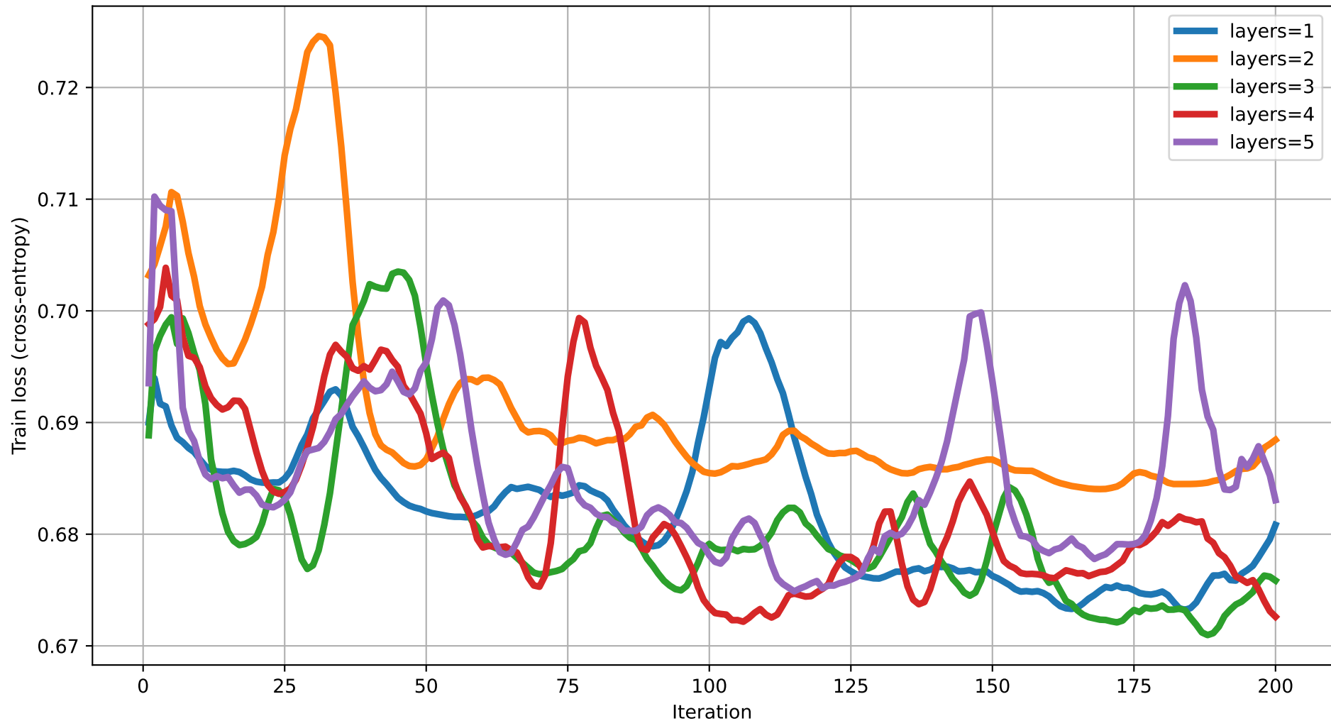
Train loss vs Iteration (dim=14) rot=RY, ent=ring, gate=IsingXX
