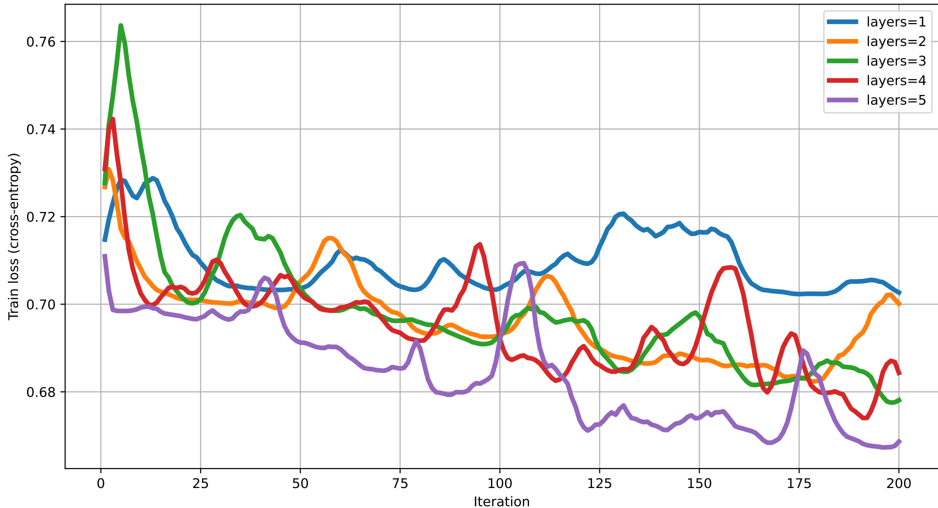
Train loss vs Iteration (dim=11) rot=RY, ent=chain, gate=CZ
