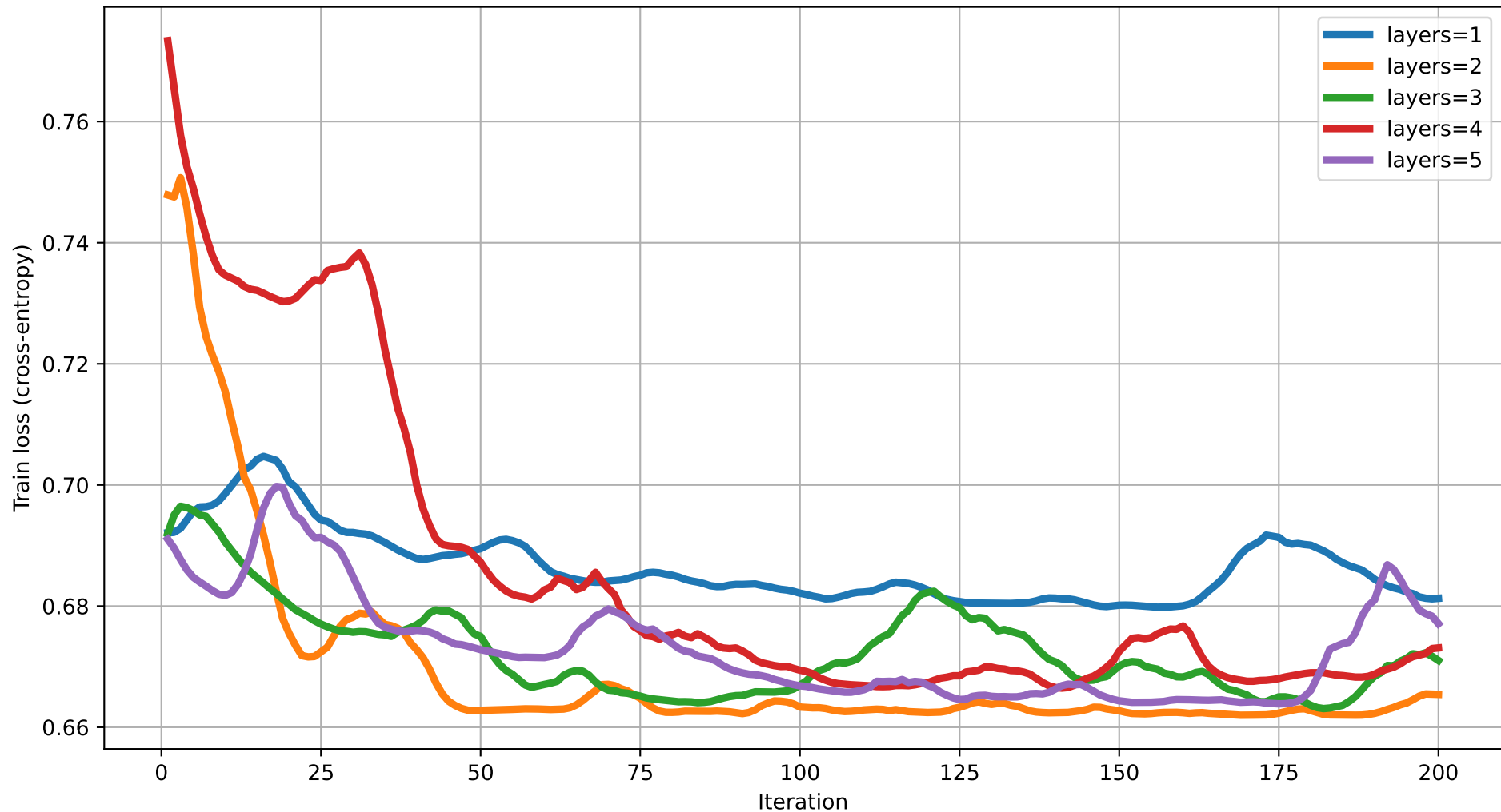
Train loss vs Iteration (dim=9) rot=RZ, ent=pairwise, gate=IsingXX
