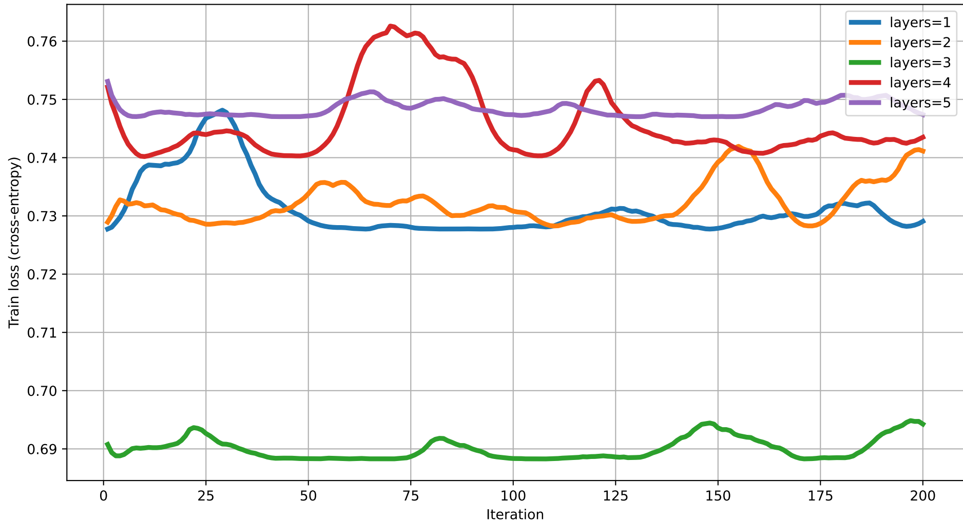
Train loss vs Iteration (dim=6) rot=RZ, ent=ring, gate=CNOT
