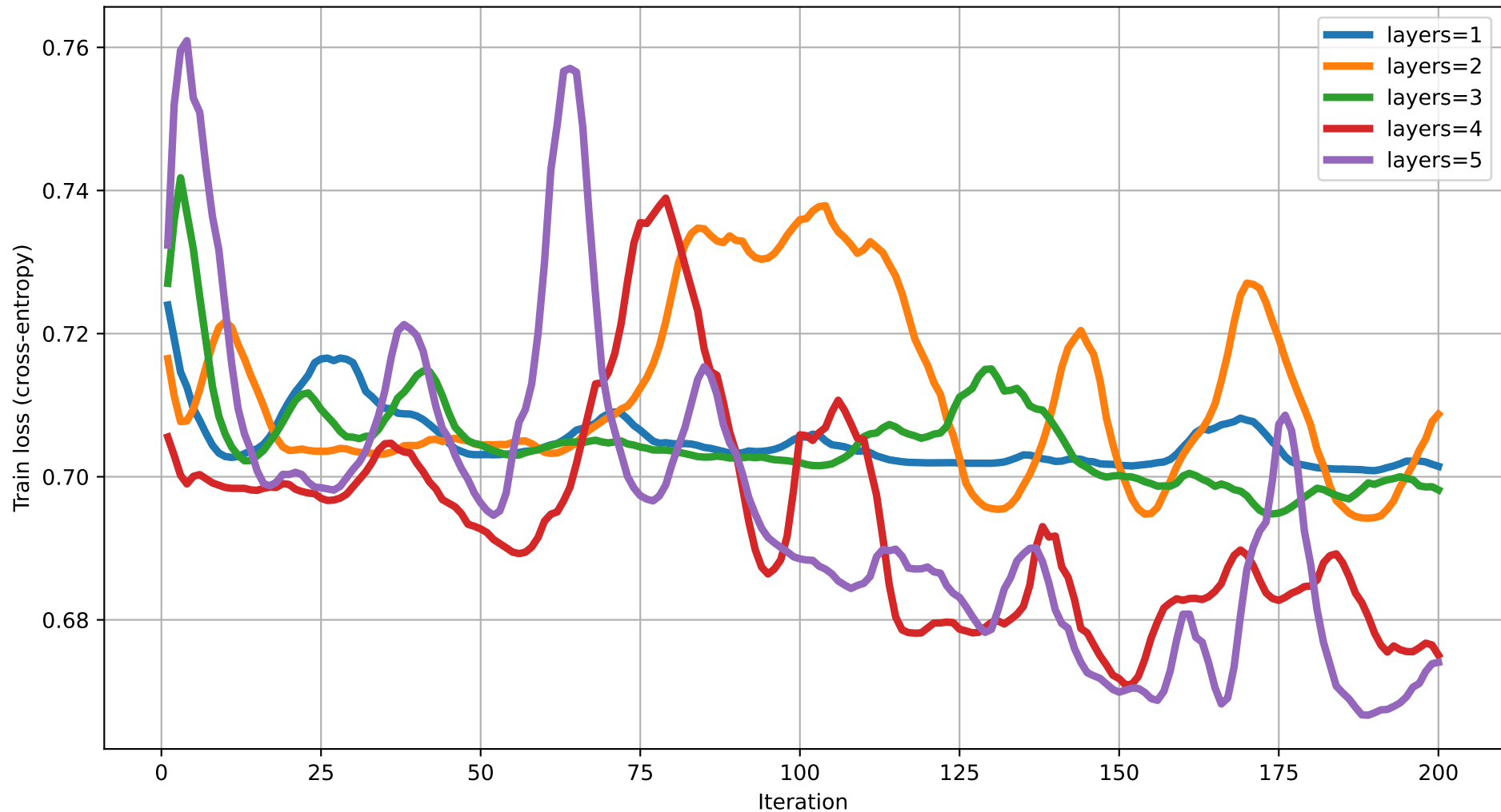
Train loss vs Iteration (dim=11) rot=RYZ, ent=chain, gate=CZ
