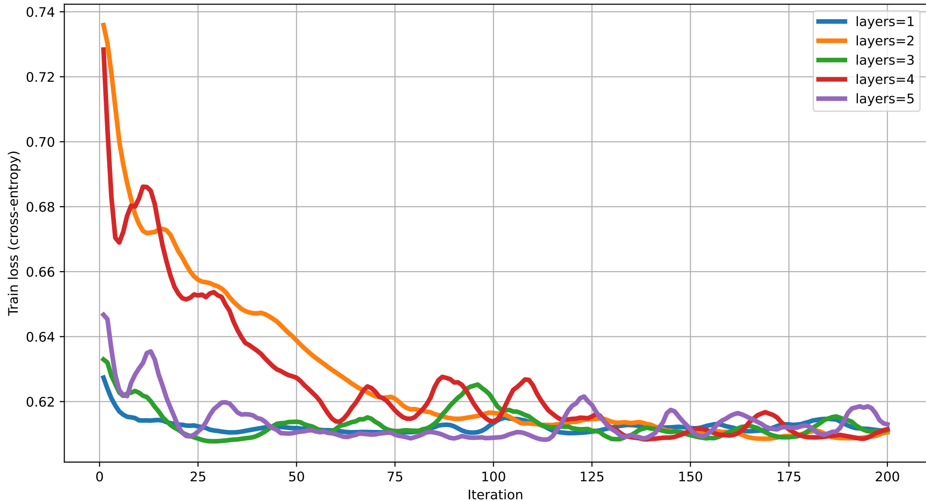
Train loss vs Iteration (degree=5) rot=RY, ent=ring, gate=IsingXX
