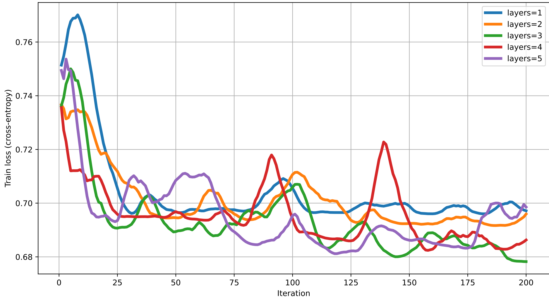
Train loss vs Iteration (dim=18) rot=RX, ent=ring, gate=CZ
