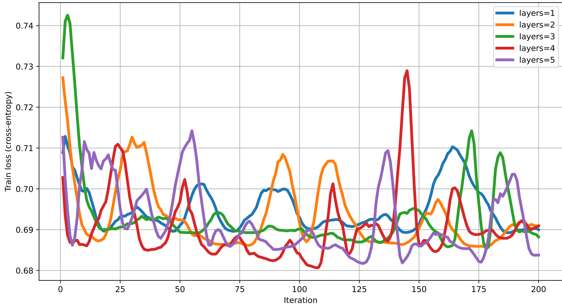
Train loss vs Iteration (dim=20) rot=Rot, ent=pairwise, gate=CZ
