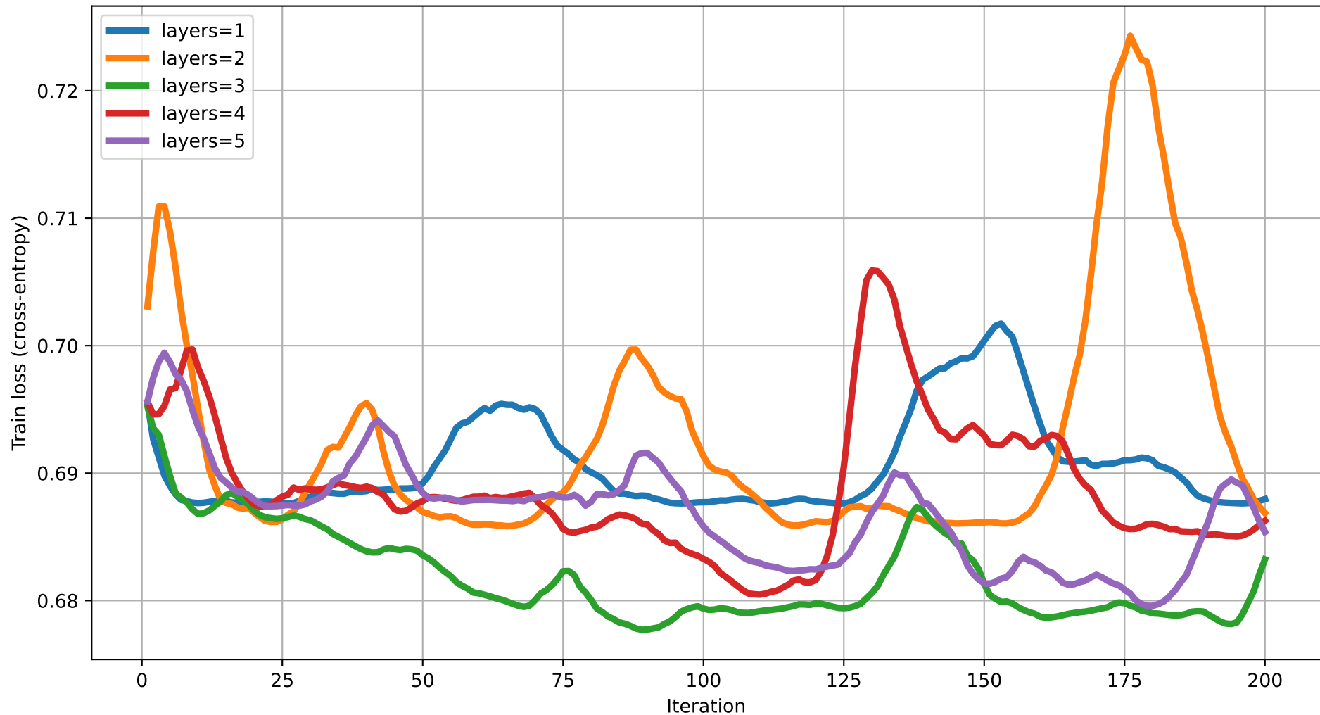
Train loss vs Iteration (dim=13) rot=RX, ent=chain, gate=CZ
