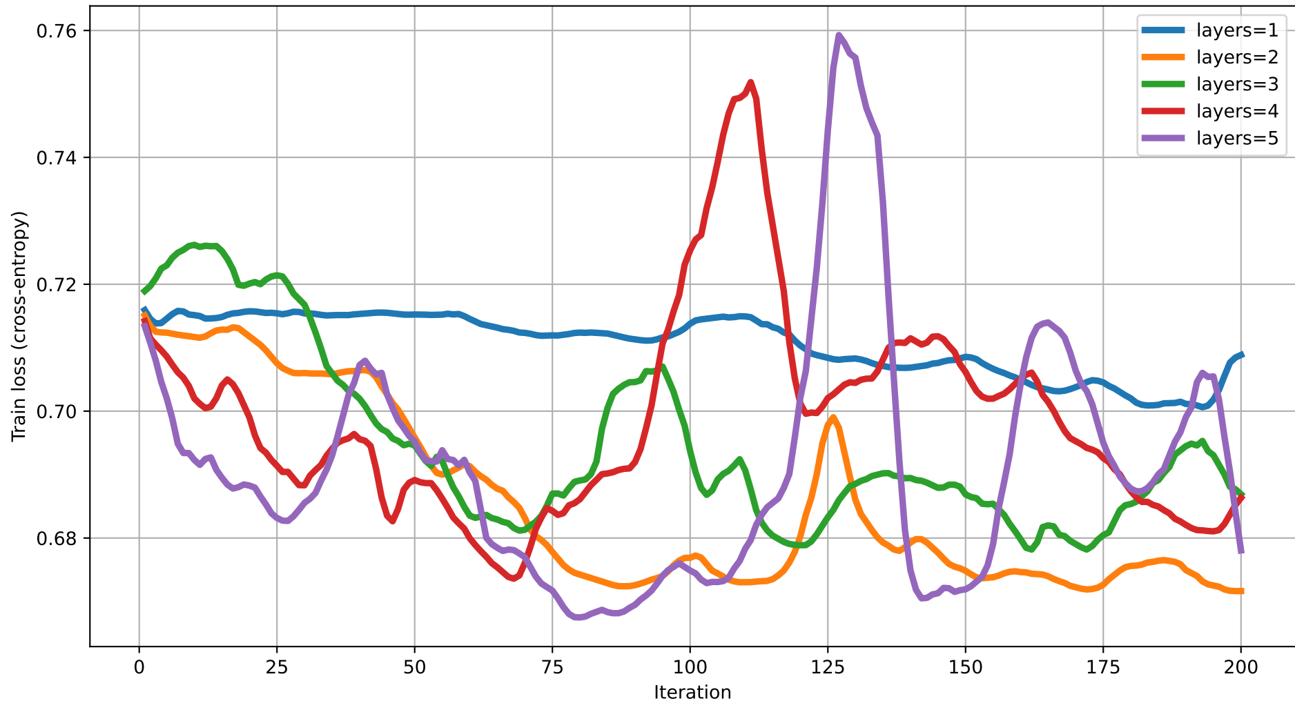
Train loss vs Iteration (dim=3) rot=Rot, ent=chain, gate=CZ
