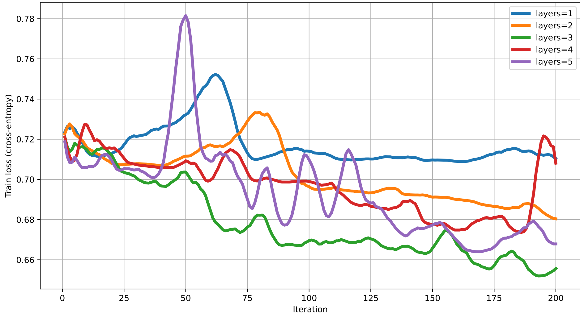
Train loss vs Iteration (dim=10) rot=RY, ent=full, gate=CZ
