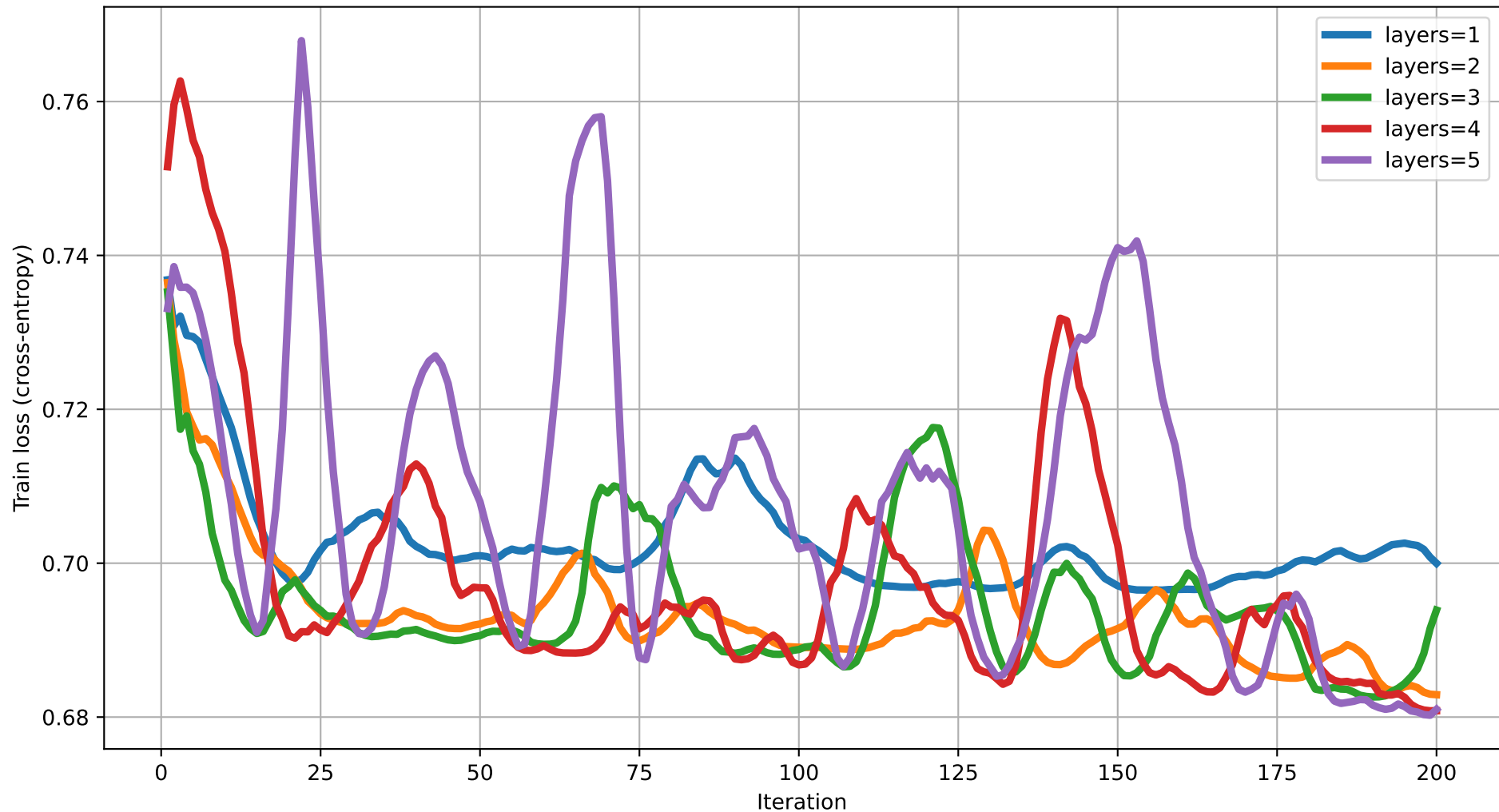
Train loss vs Iteration (dim=18) rot=RX, ent=pairwise, gate=CNOT
