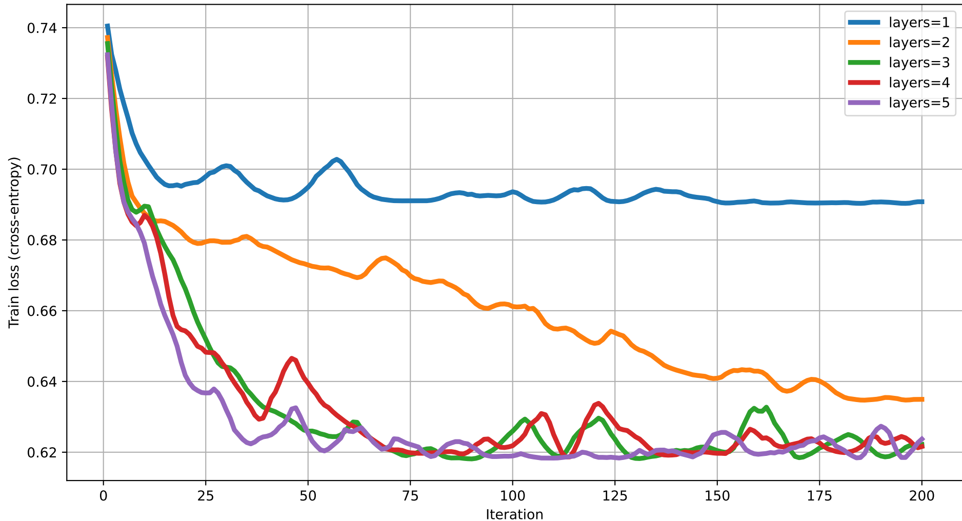
Train loss vs Iteration (degree=5) rot=RYZ, ent=pairwise, gate=CZ
