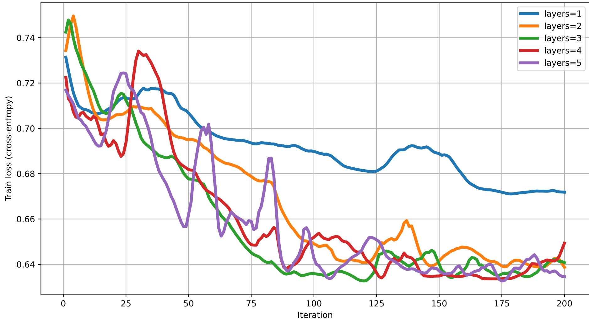
Train loss vs Iteration (dim=6) rot=Rot, ent=pairwise, gate=CNOT
