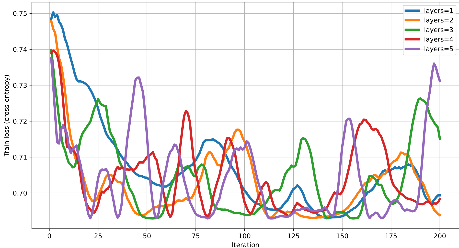
Train loss vs Iteration (dim=3) rot=RX, ent=ring, gate=CZ
