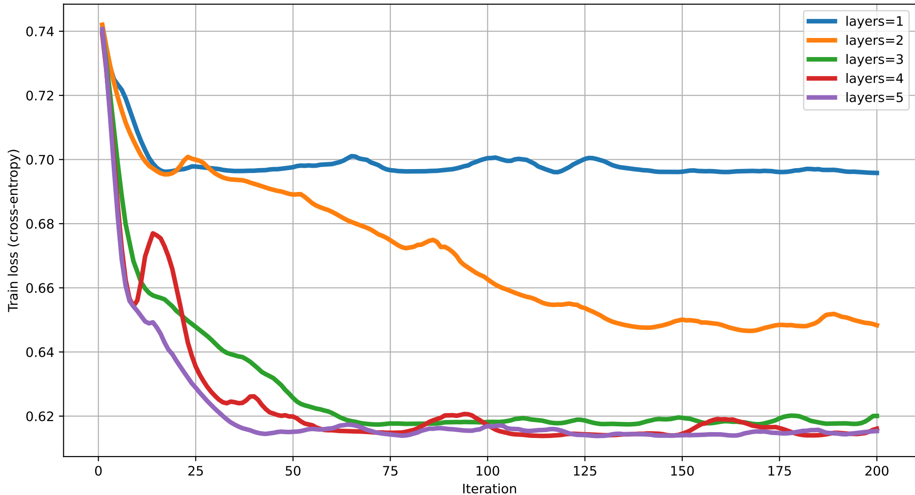
Train loss vs Iteration (degree=5) rot=RX, ent=full, gate=CNOT
