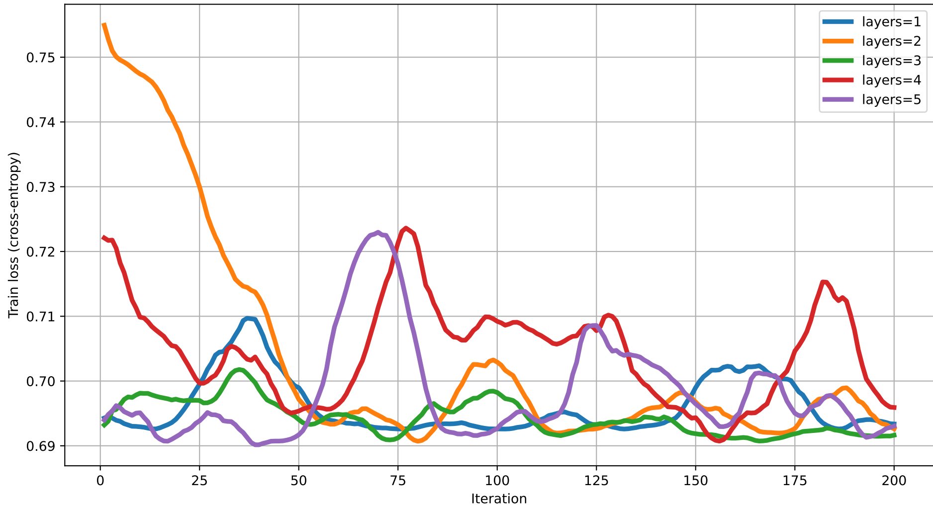
Train loss vs Iteration (dim=3) rot=RY, ent=chain, gate=IsingXX
