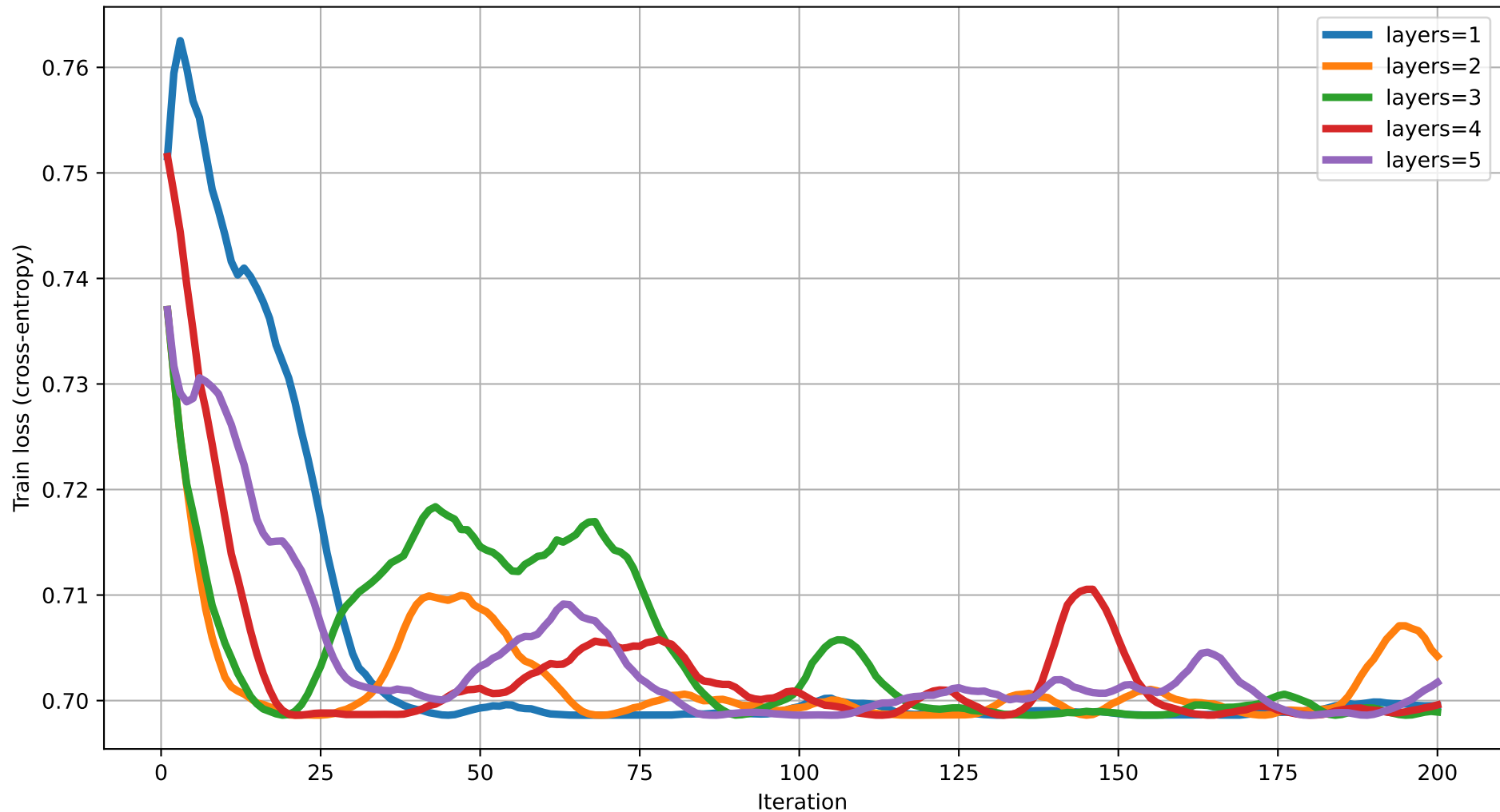
Train loss vs Iteration (dim=18) rot=RZ, ent=full, gate=CZ
