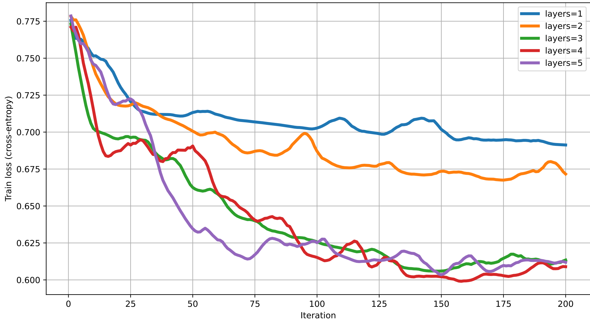
Train loss vs Iteration (dim=9) rot=RY, ent=ring, gate=CZ
