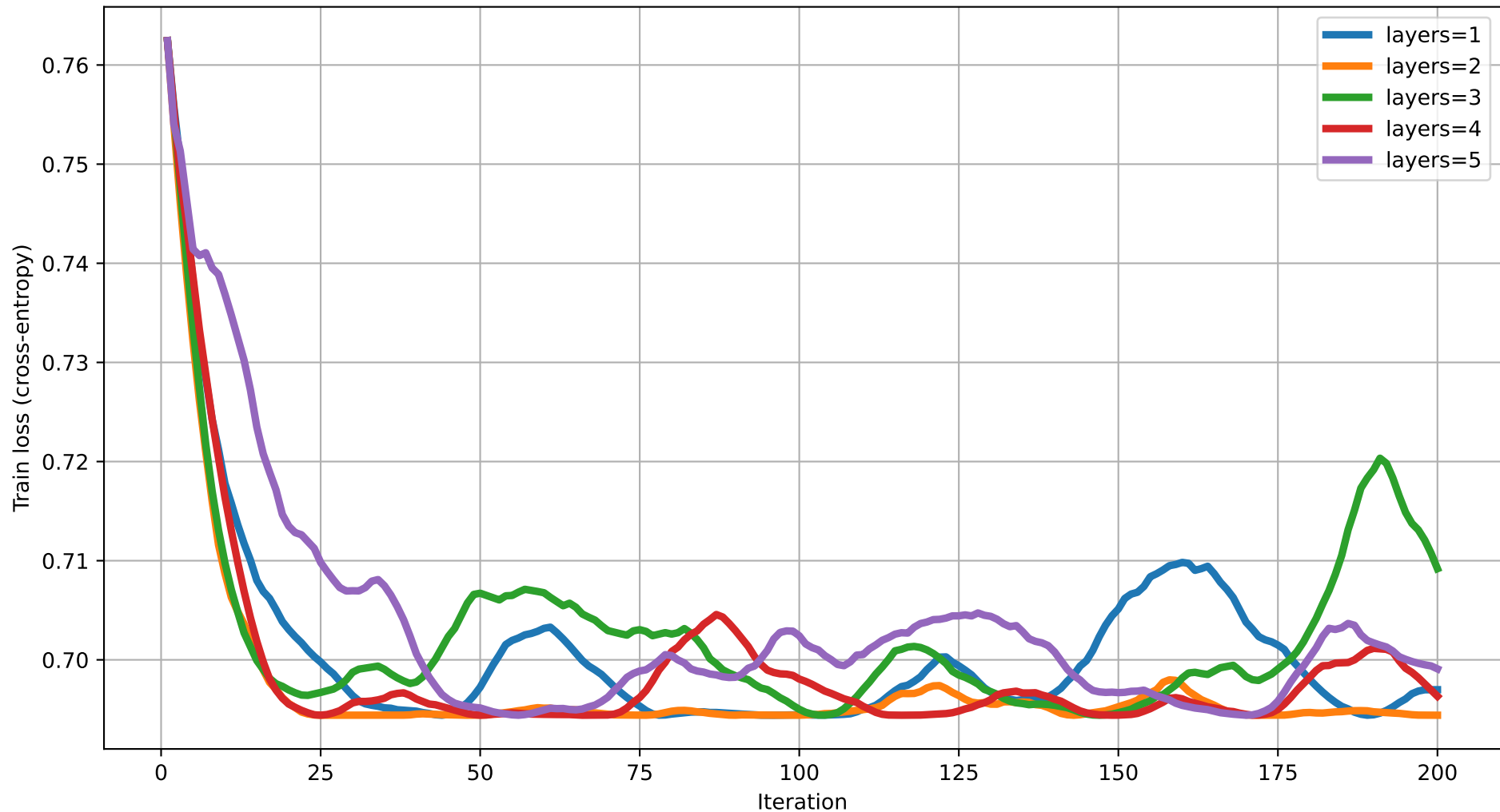
Train loss vs Iteration (dim=8) rot=RZ, ent=pairwise, gate=CNOT
