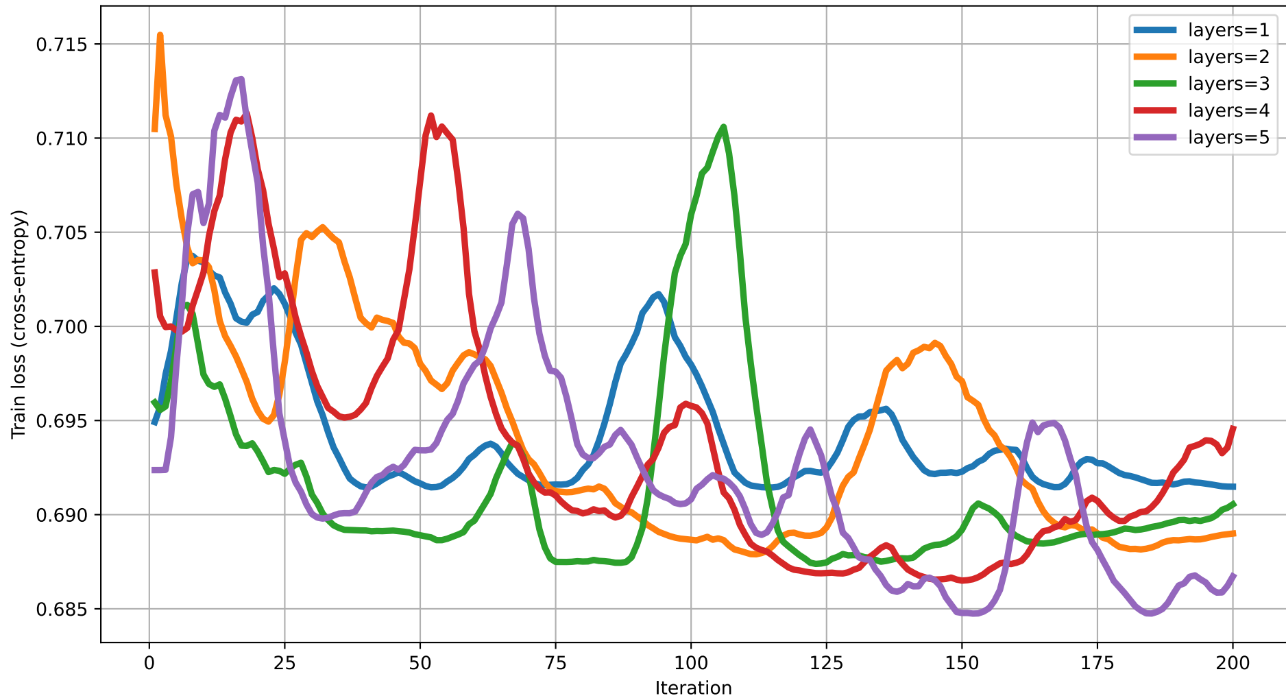
Train loss vs Iteration (dim=12) rot=RY, ent=full, gate=IsingXX
