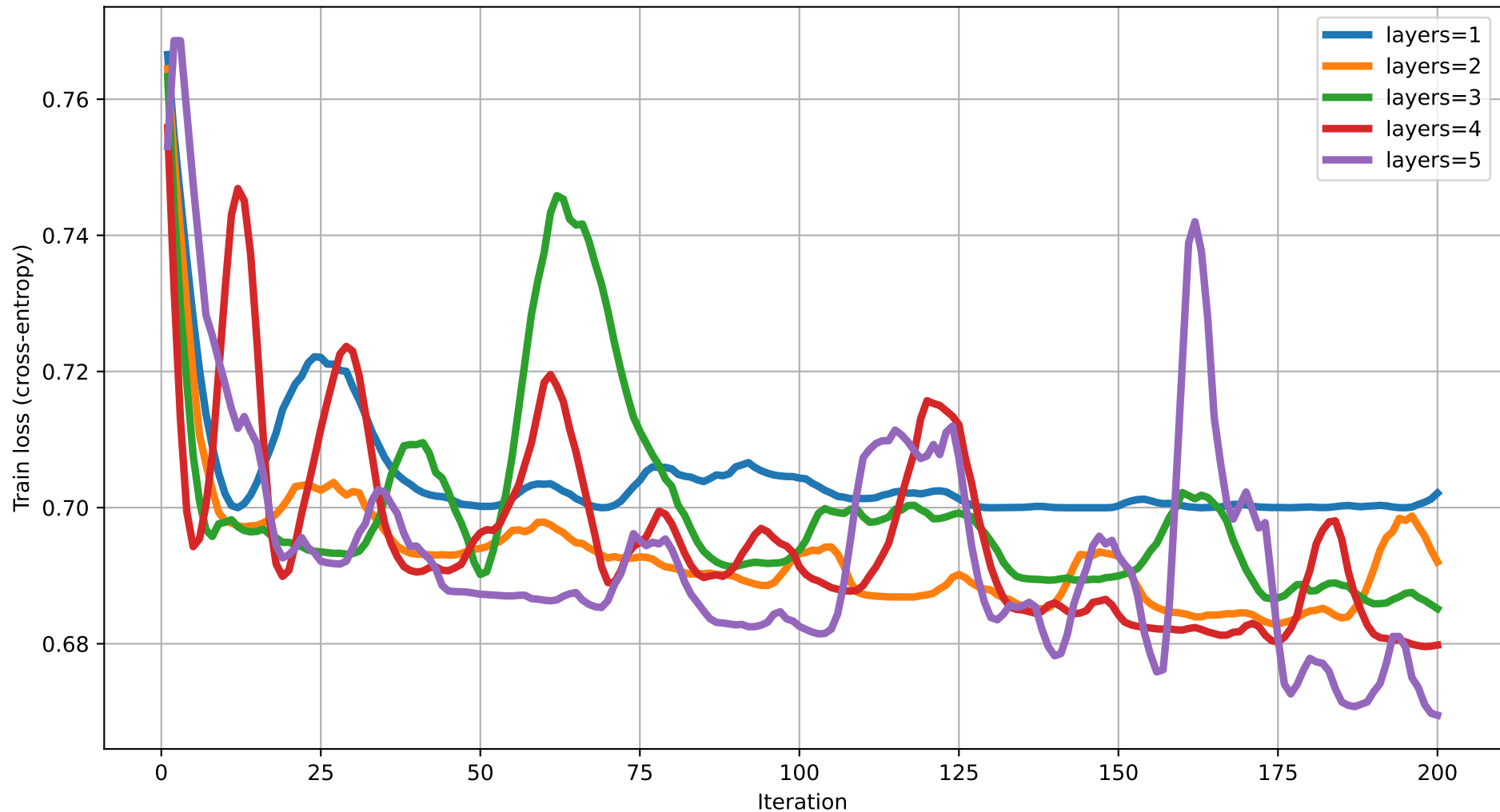
Train loss vs Iteration (dim=17) rot=RYZ, ent=pairwise, gate=CNOT
