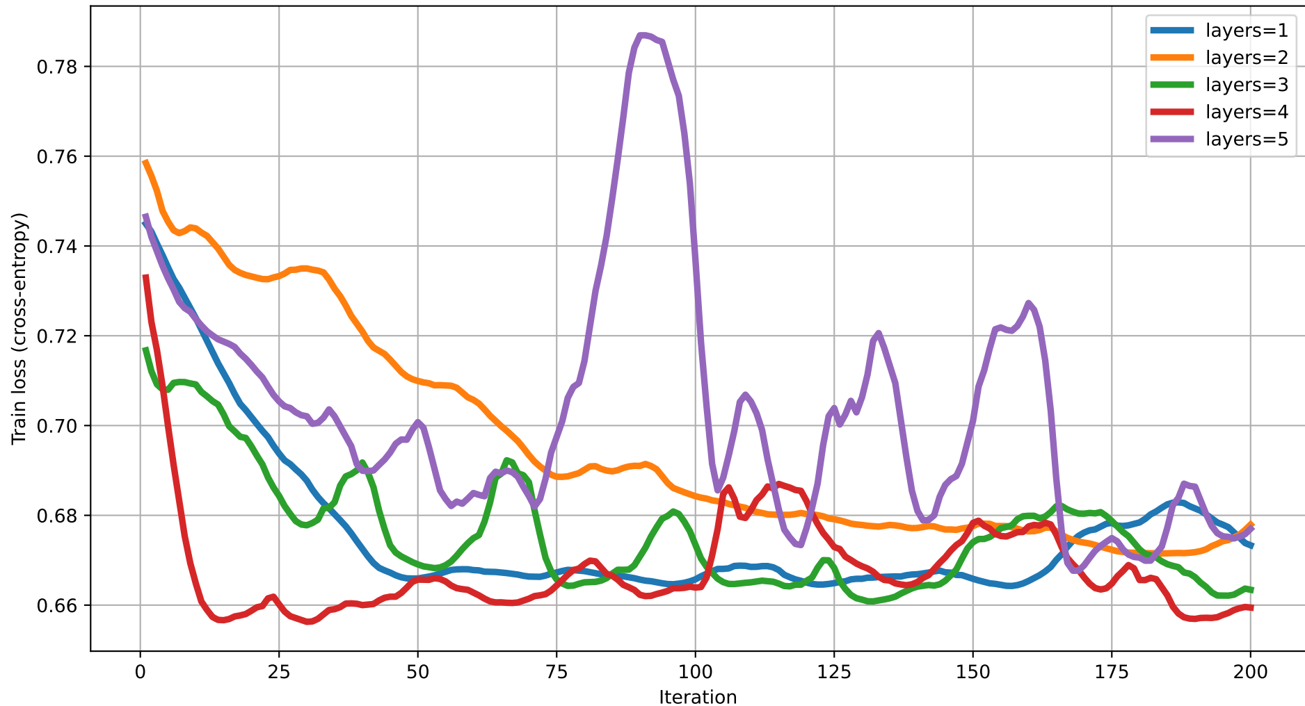
Train loss vs Iteration (dim=3) rot=Rot, ent=ring, gate=CNOT
