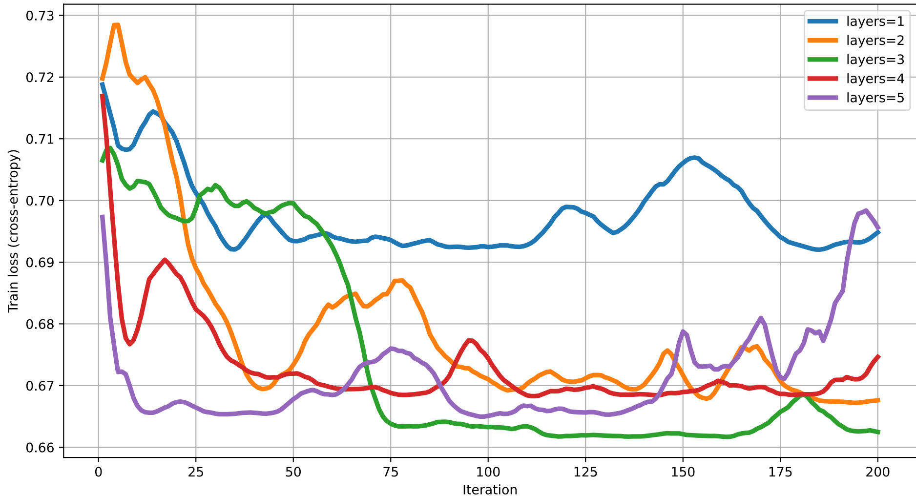
Train loss vs Iteration (dim=5) rot=RX, ent=ring, gate=CNOT
