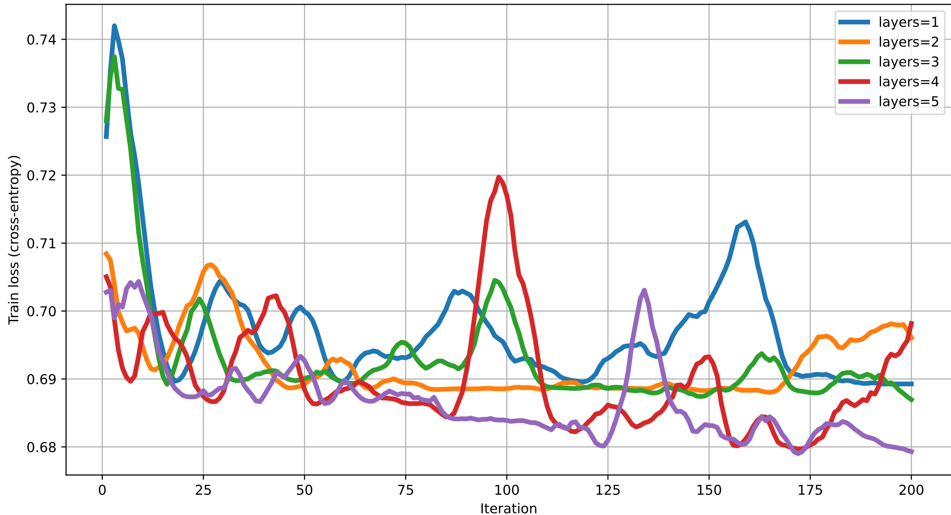
Train loss vs Iteration (dim=20) rot=RY, ent=ring, gate=CZ
