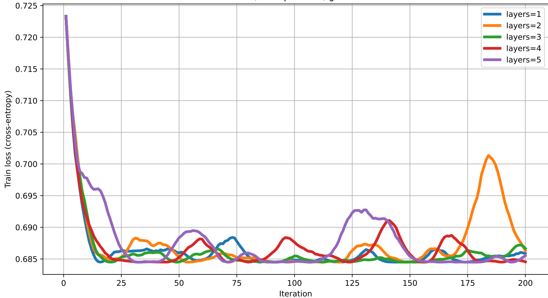
Train loss vs Iteration (degree=3) rot=RZ, ent=pairwise, gate=CZ
