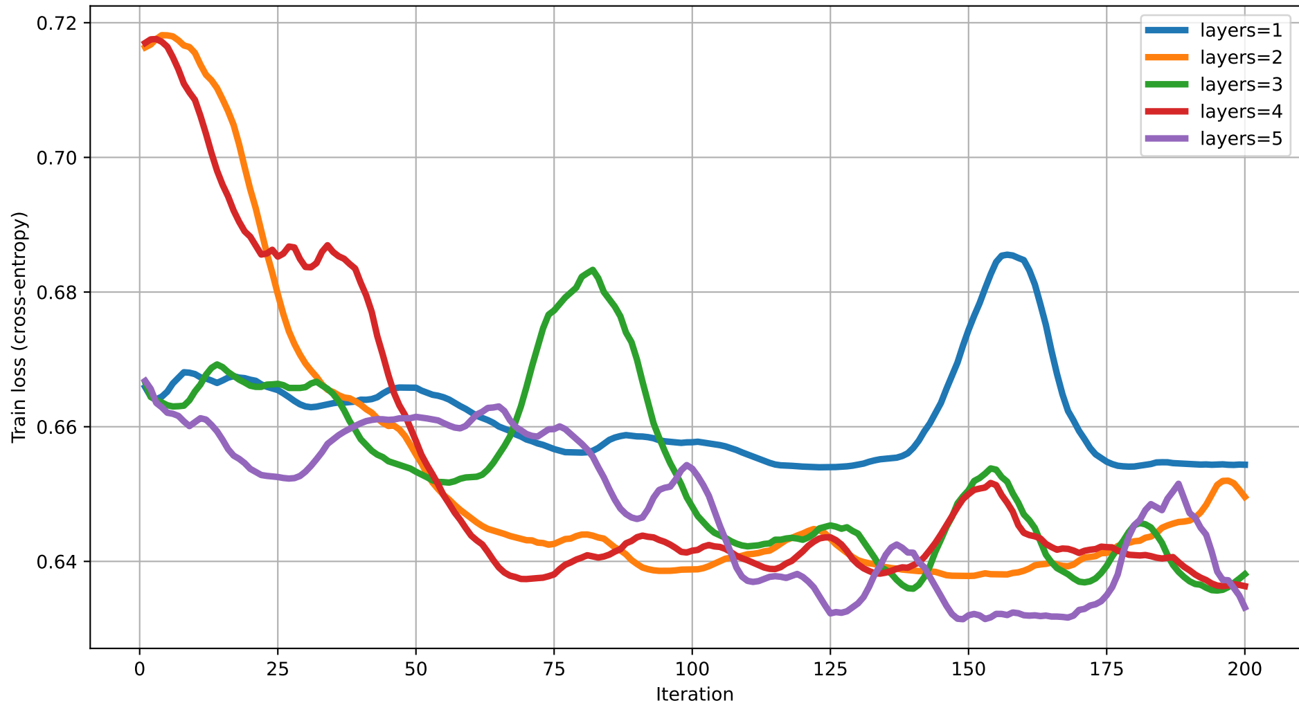
Train loss vs Iteration (dim=7) rot=RZ, ent=full, gate=IsingXX
