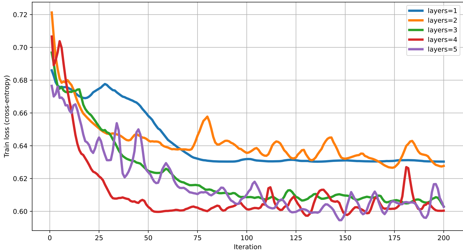
Train loss vs Iteration (degree=2) rot=Rot, ent=ring, gate=IsingXX
