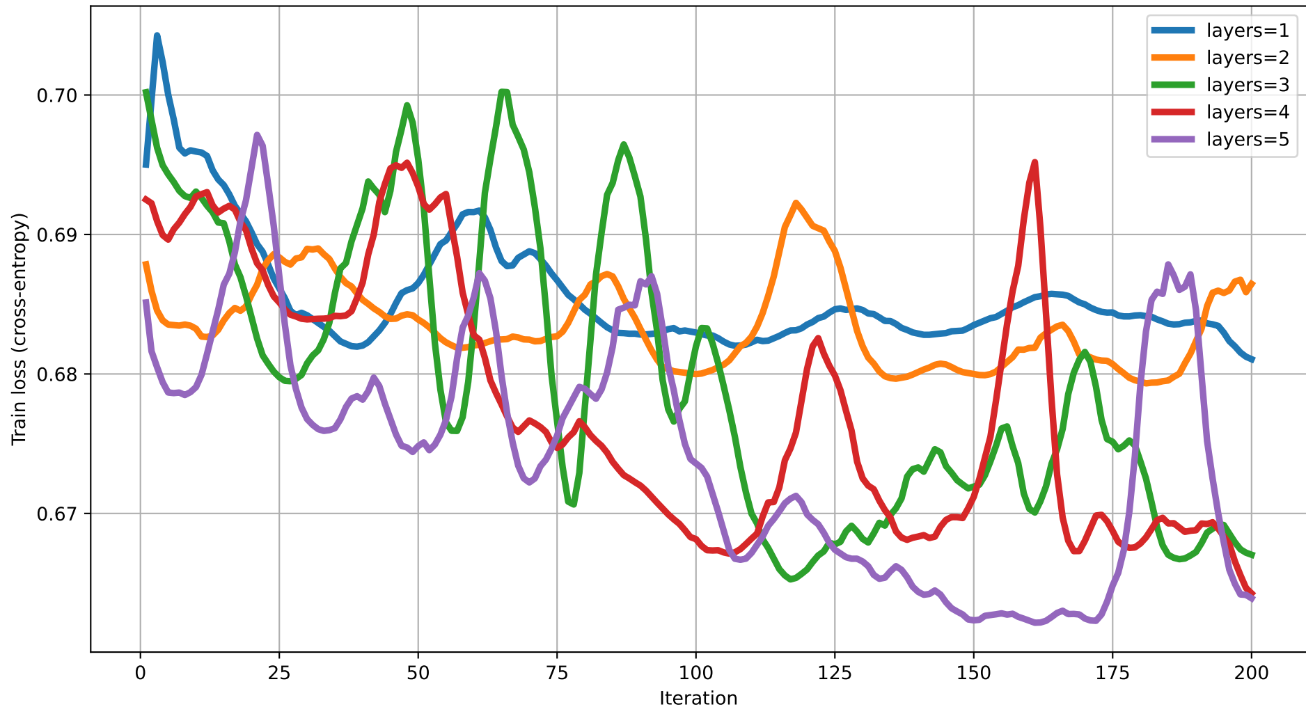
Train loss vs Iteration (dim=16) rot=RY, ent=ring, gate=CNOT
