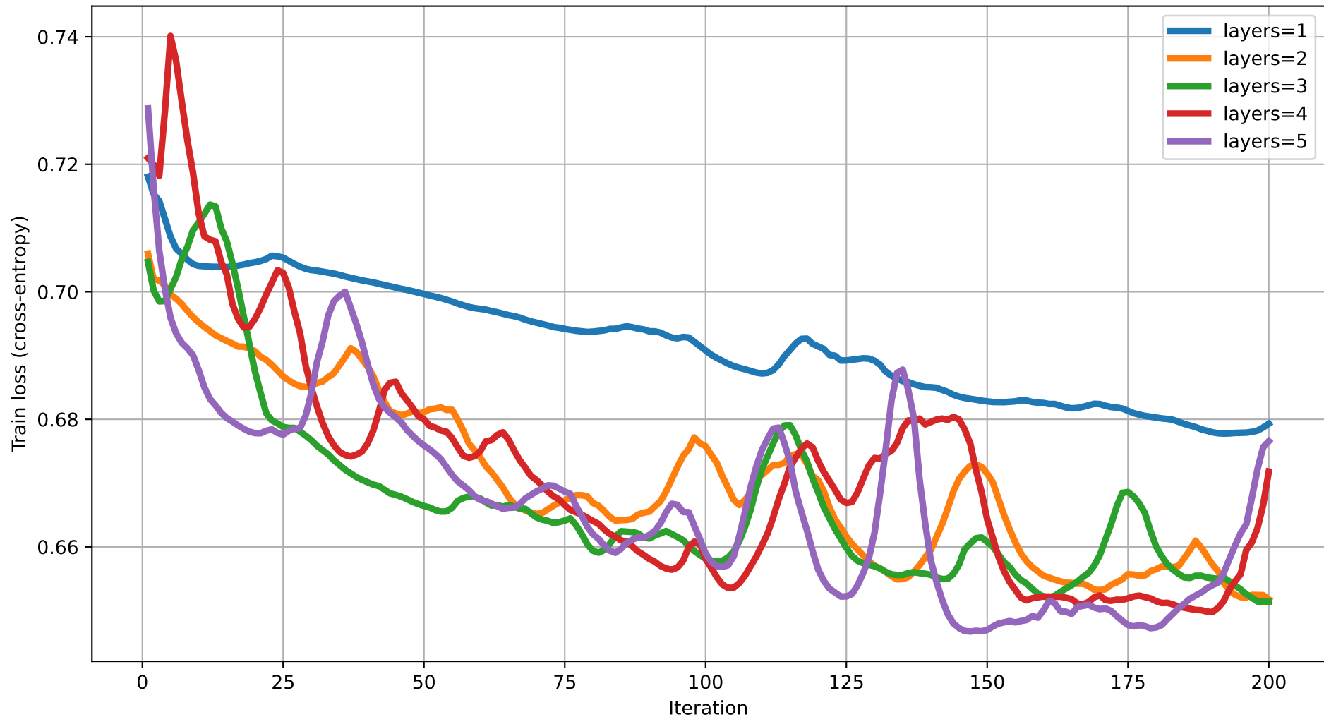
Train loss vs Iteration (dim=6) rot=RY, ent=chain, gate=CZ
