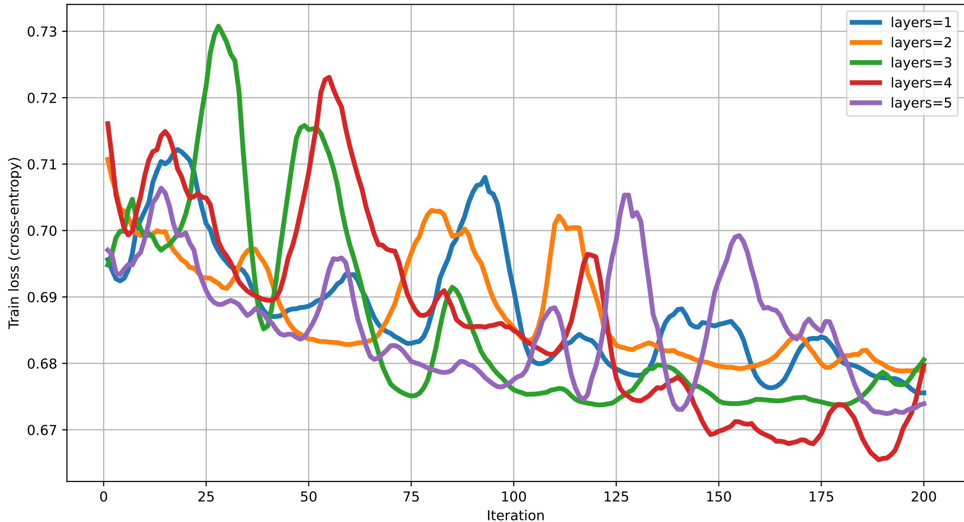
Train loss vs Iteration (dim=12) rot=RZ, ent=chain, gate=IsingXX
