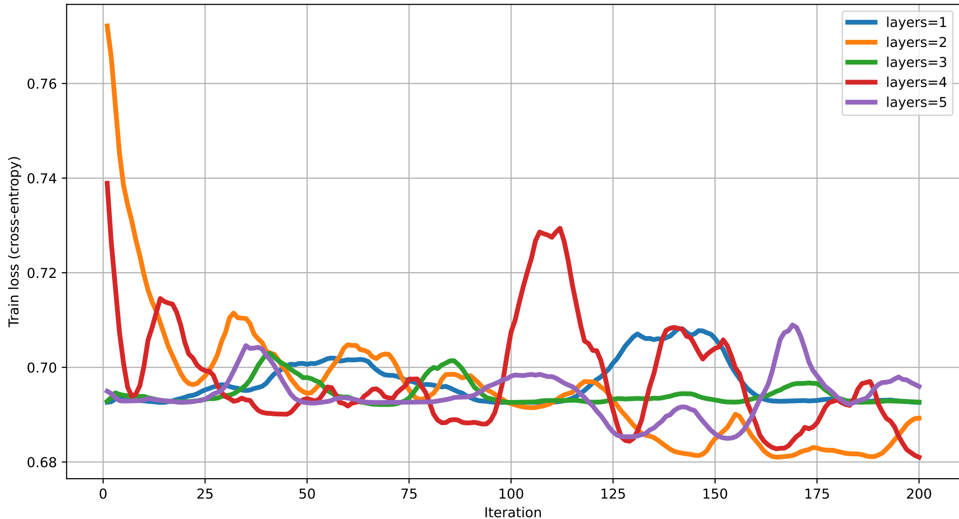
Train loss vs Iteration (dim=19) rot=RY, ent=chain, gate=IsingXX
