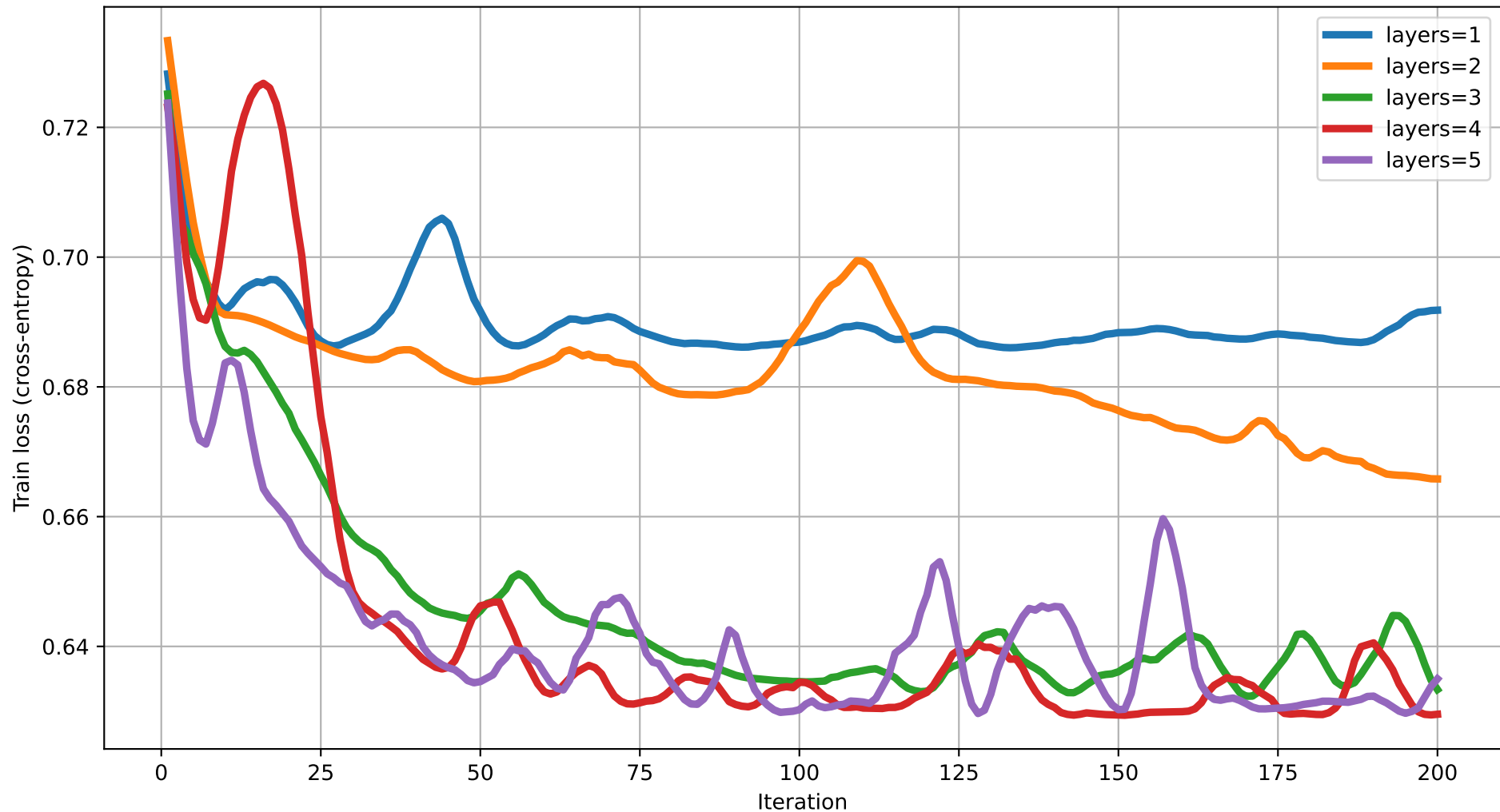
Train loss vs Iteration (degree=2) rot=RY, ent=pairwise, gate=CZ
