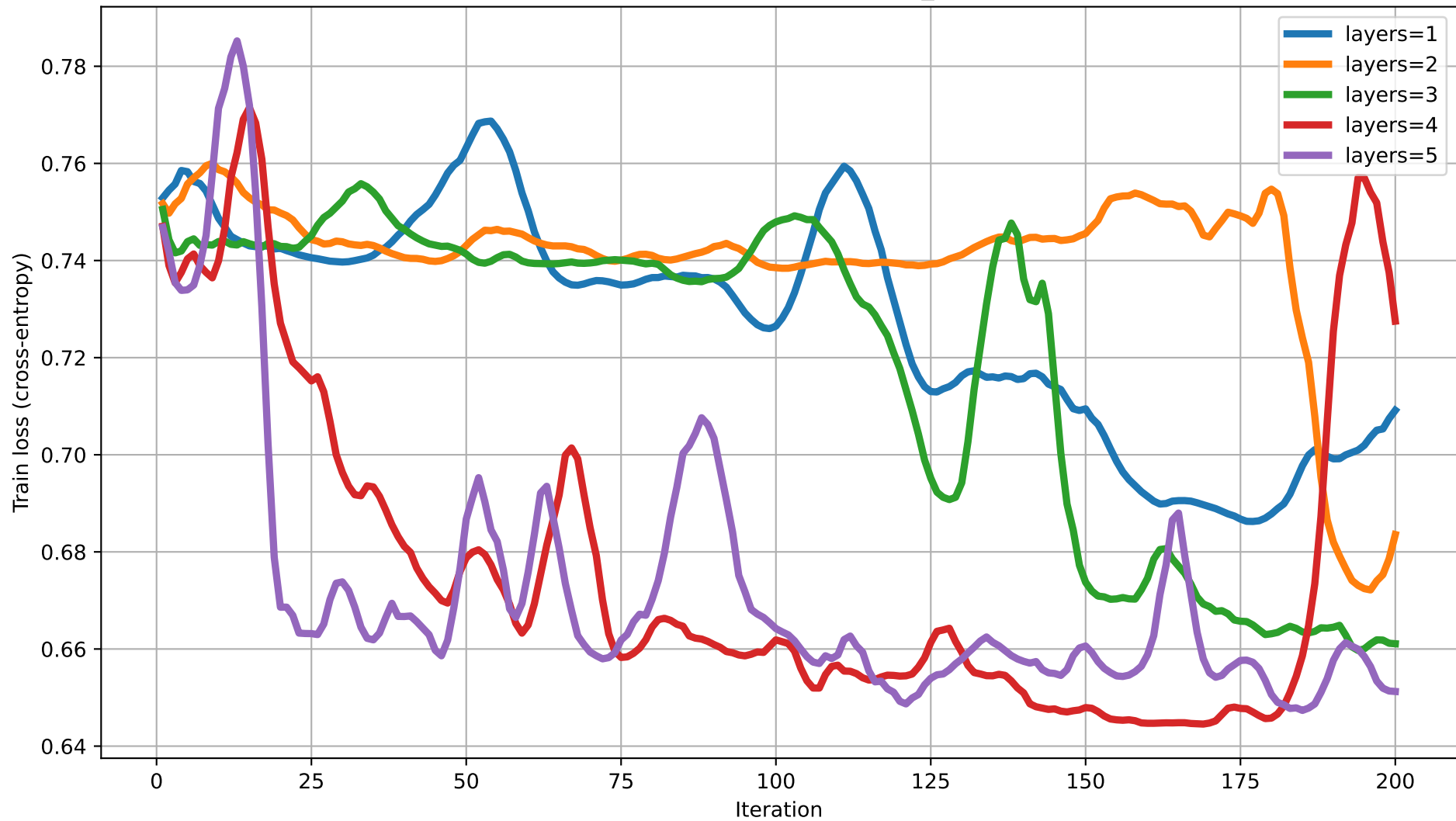
Train loss vs Iteration for different num_layers (dim=5)
