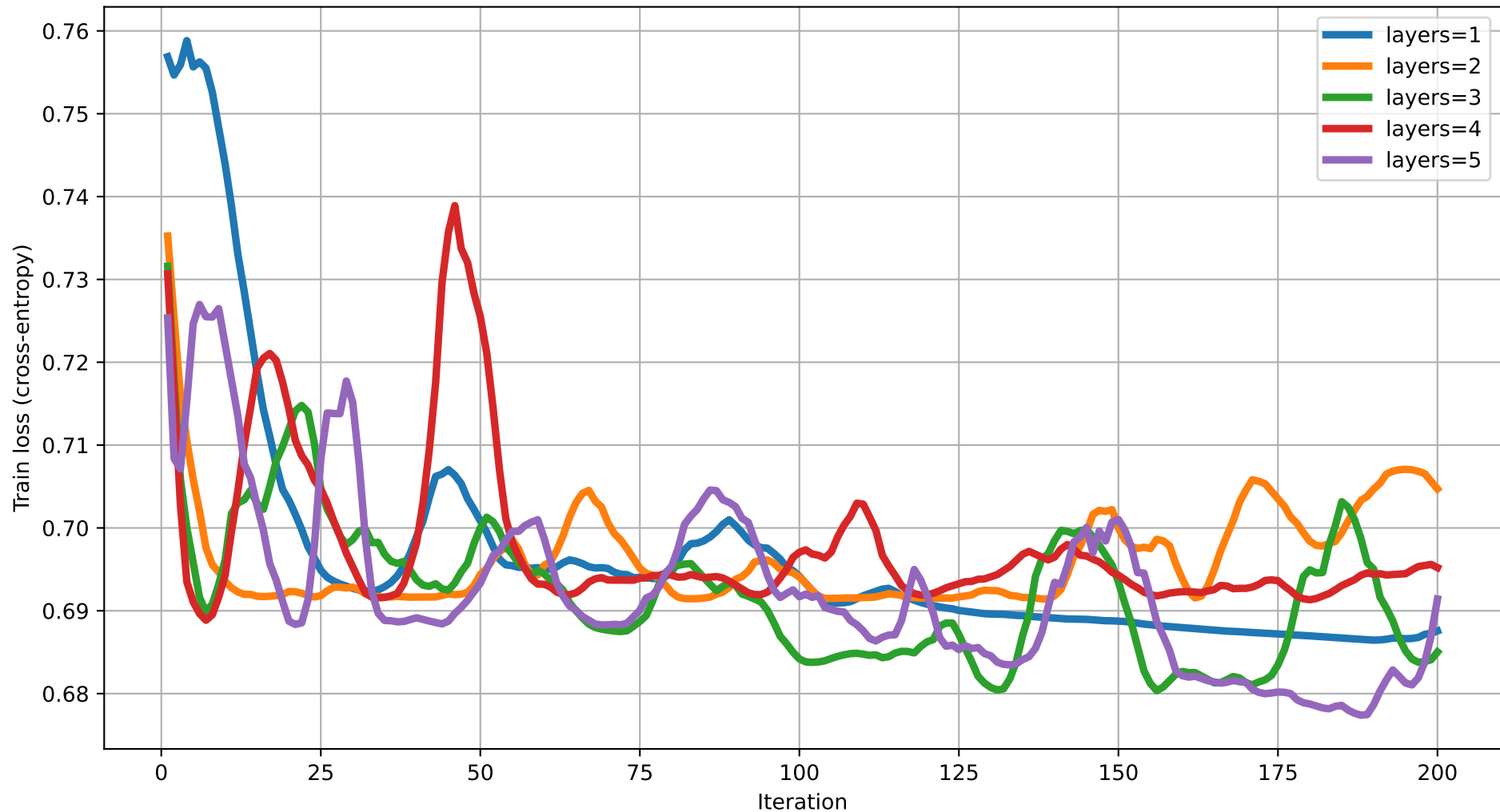
Train loss vs Iteration (dim=16) rot=RYZ, ent=full, gate=CNOT
