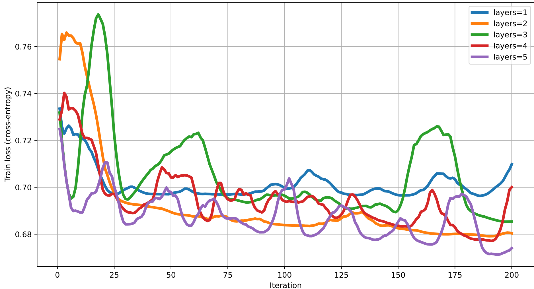
Train loss vs Iteration (dim=18) rot=RYZ, ent=full, gate=CZ
