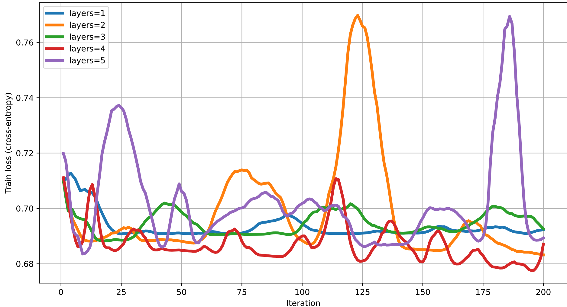
Train loss vs Iteration (dim=20) rot=RX, ent=pairwise, gate=CNOT
