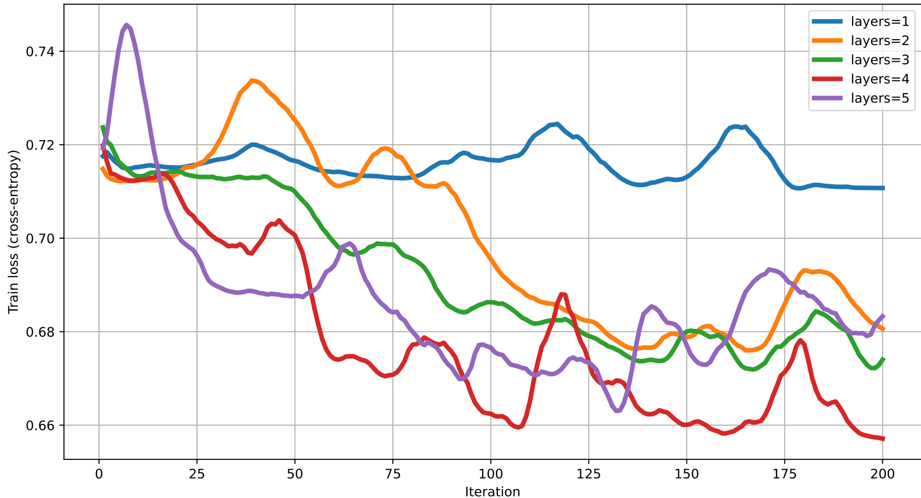
Train loss vs Iteration (dim=3) rot=RY, ent=chain, gate=CZ
