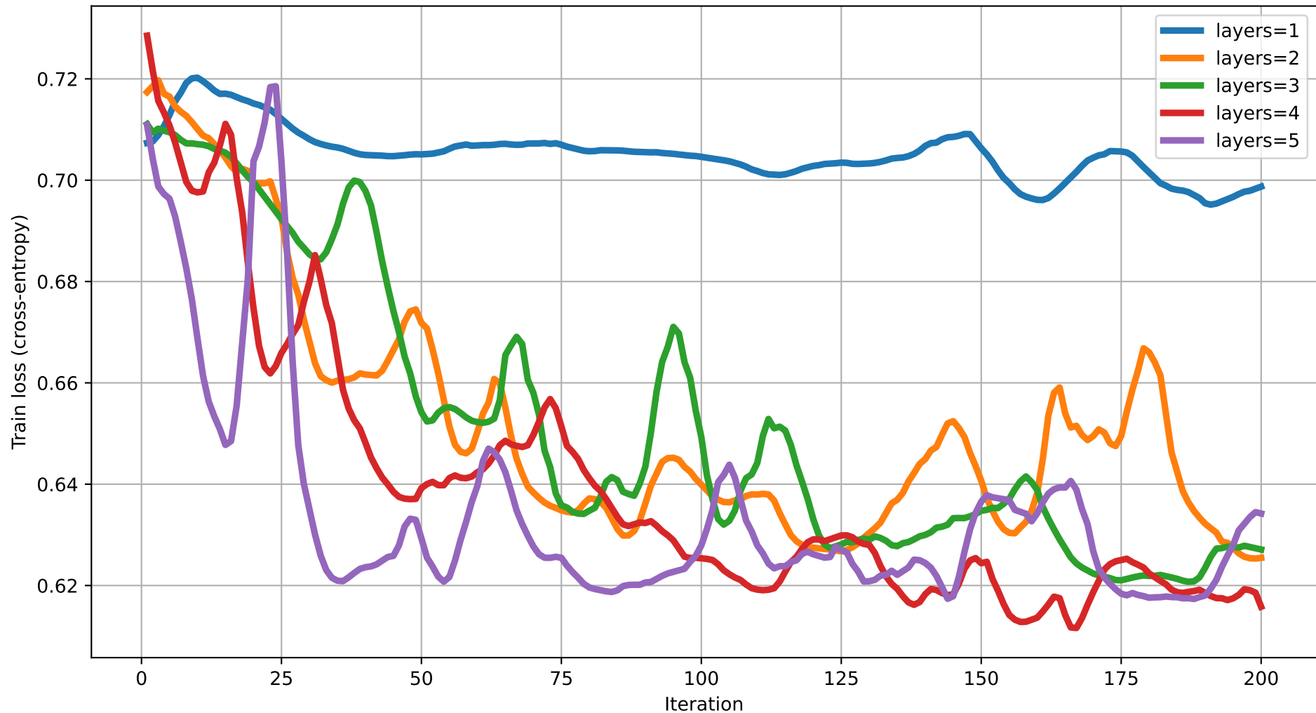
Train loss vs Iteration (dim=4) rot=Rot, ent=ring, gate=CNOT
