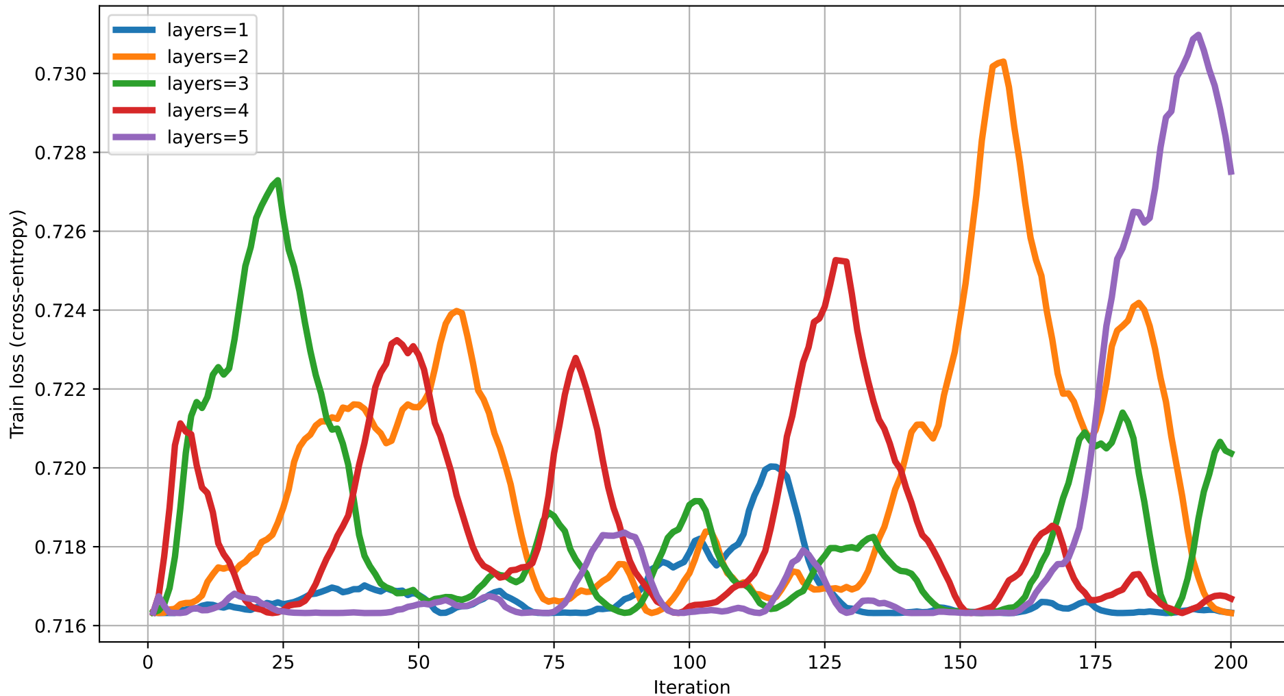
Train loss vs Iteration (dim=7) rot=RZ, ent=pairwise, gate=CNOT
