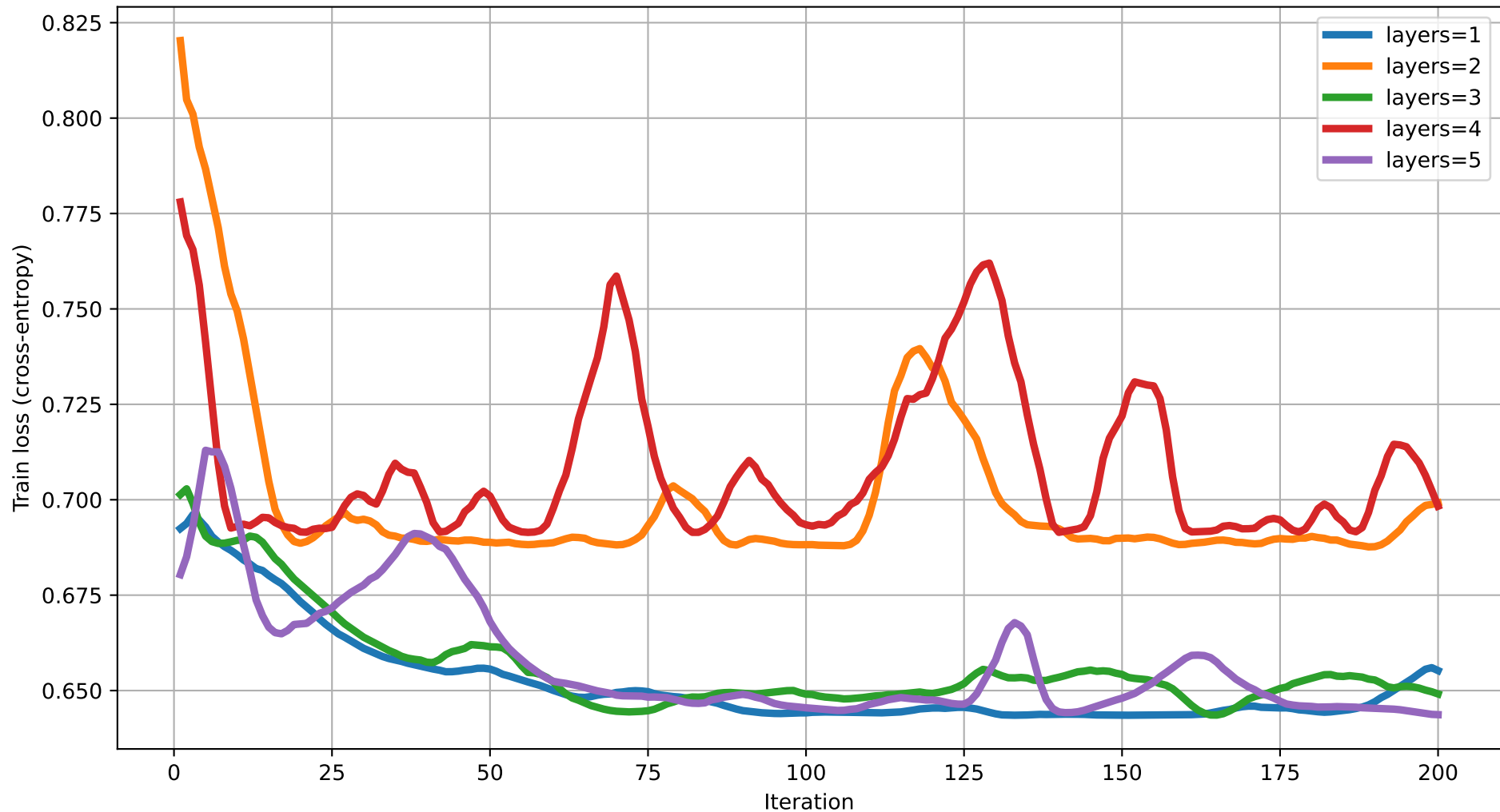
Train loss vs Iteration (dim=8) rot=RX, ent=chain, gate=IsingXX
