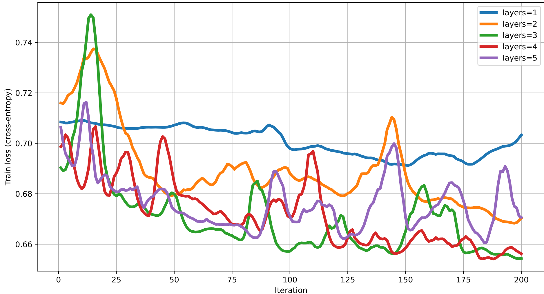
Train loss vs Iteration (dim=8) rot=Rot, ent=ring, gate=CNOT
