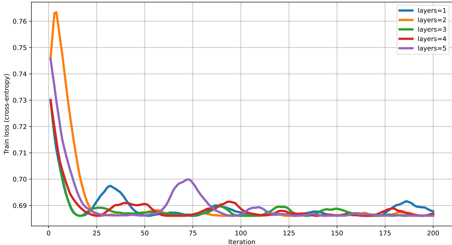
Train loss vs Iteration (degree=2) rot=RZ, ent=chain, gate=CNOT
