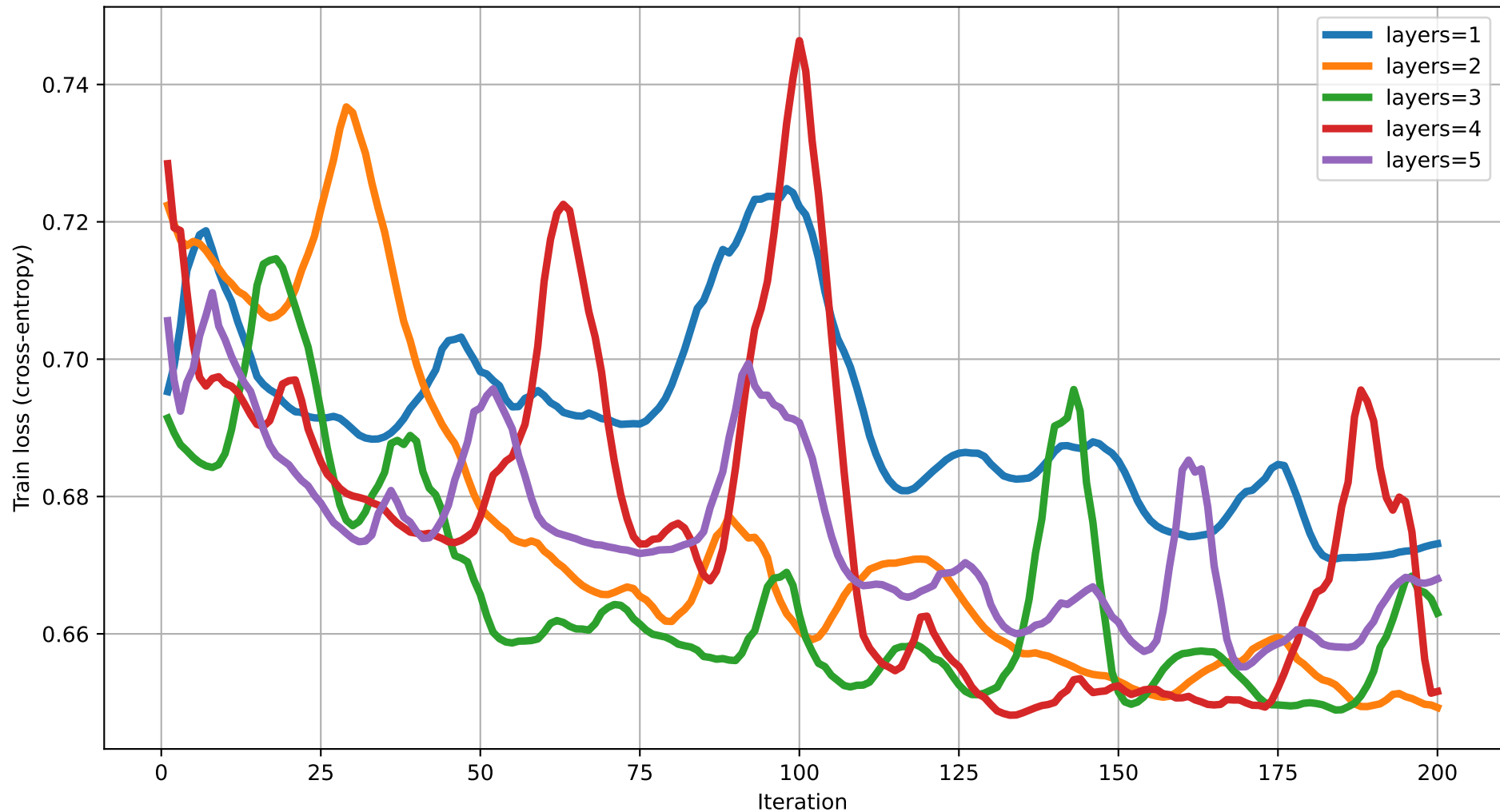
Train loss vs Iteration (dim=6) rot=RYZ, ent=pairwise, gate=IsingXX
