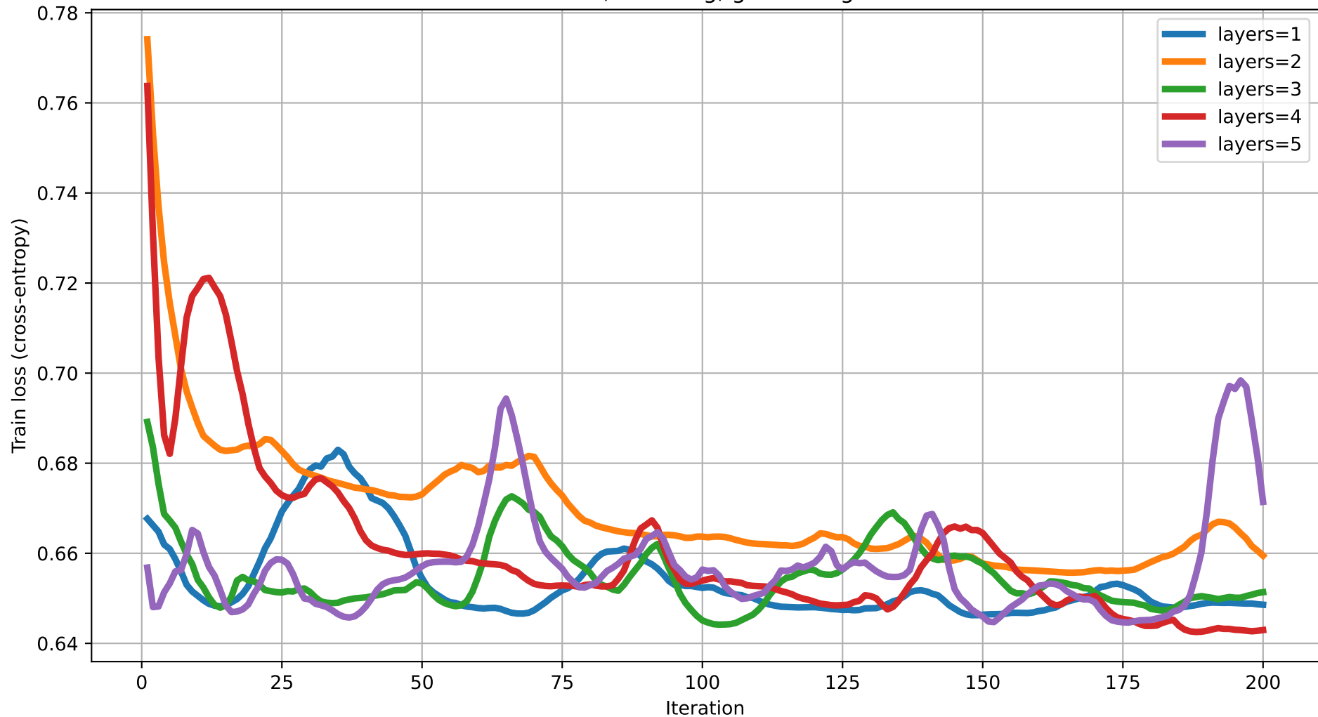
Train loss vs Iteration (dim=9) rot=RY, ent=ring, gate=IsingXX
