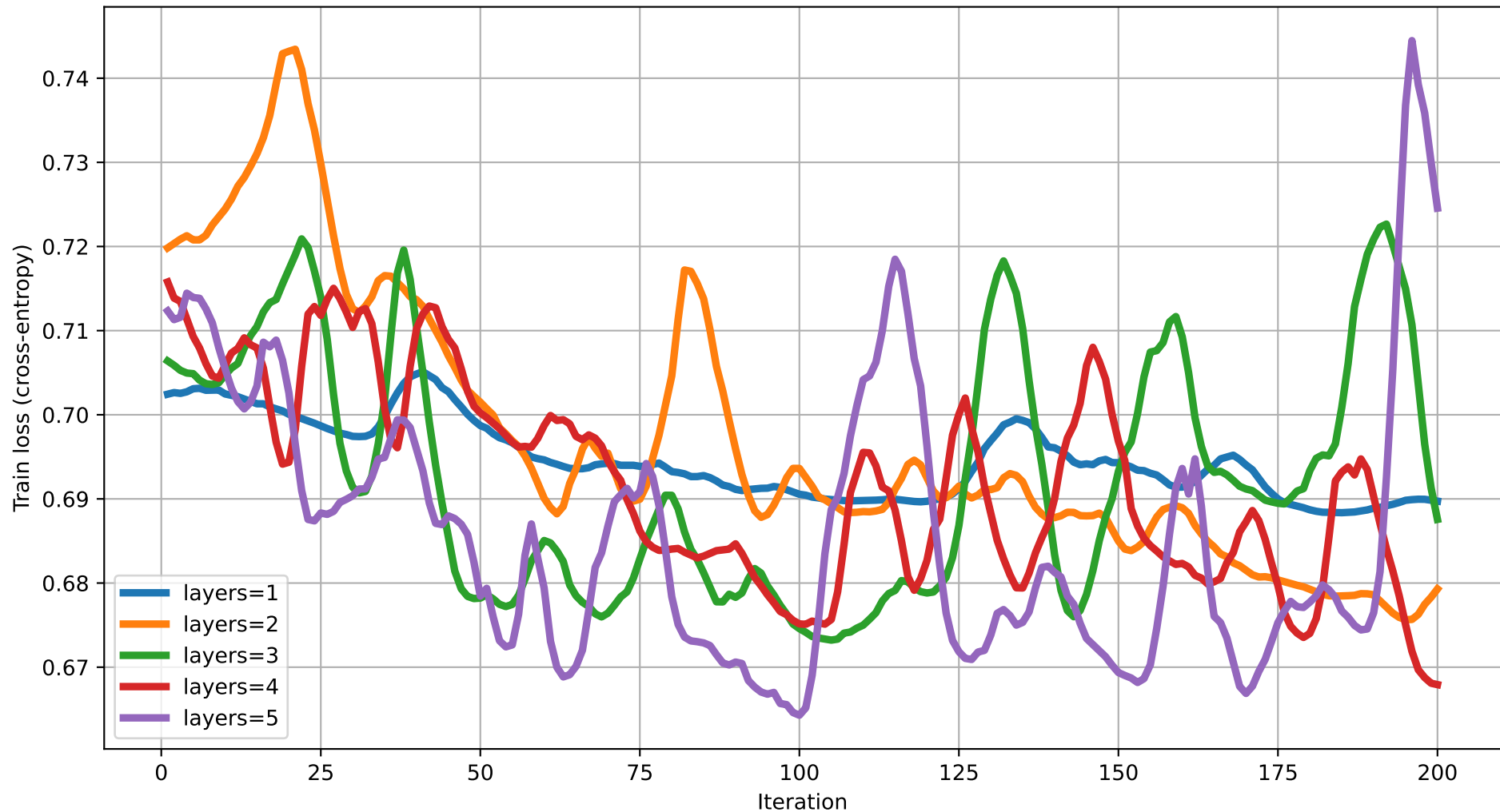
Train loss vs Iteration (dim=15) rot=Rot, ent=ring, gate=CNOT
