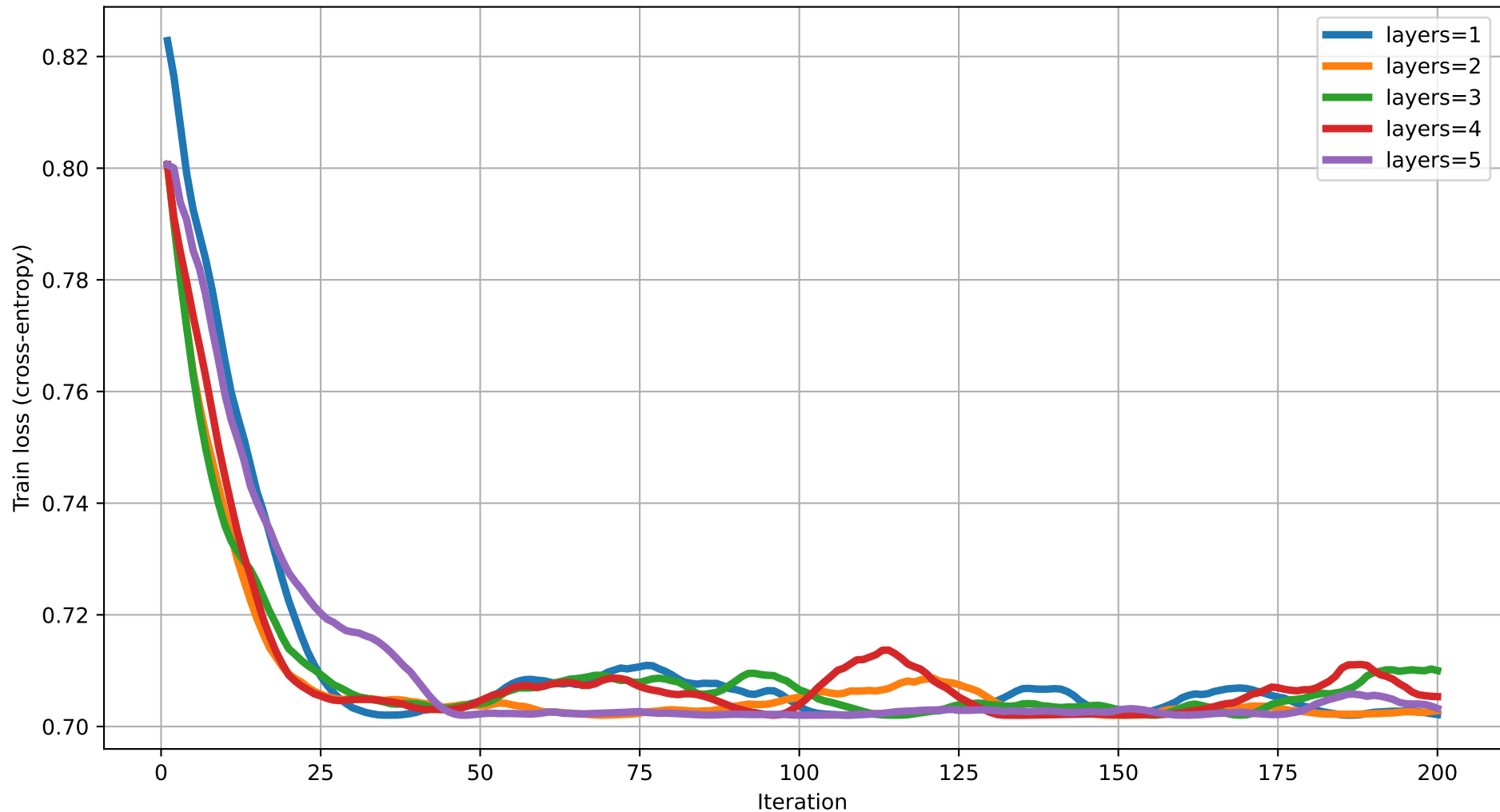
Train loss vs Iteration (dim=8) rot=RZ, ent=chain, gate=CZ
