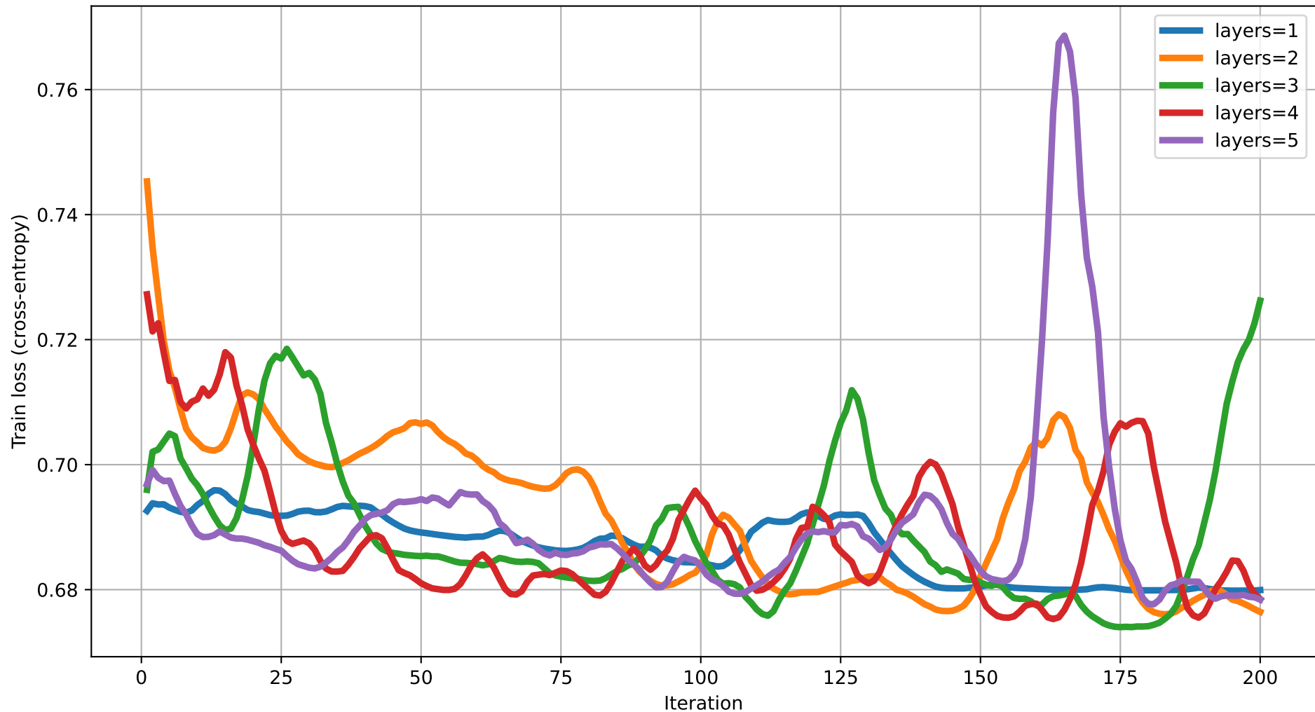
Train loss vs Iteration (dim=20) rot=RZ, ent=chain, gate=IsingXX
