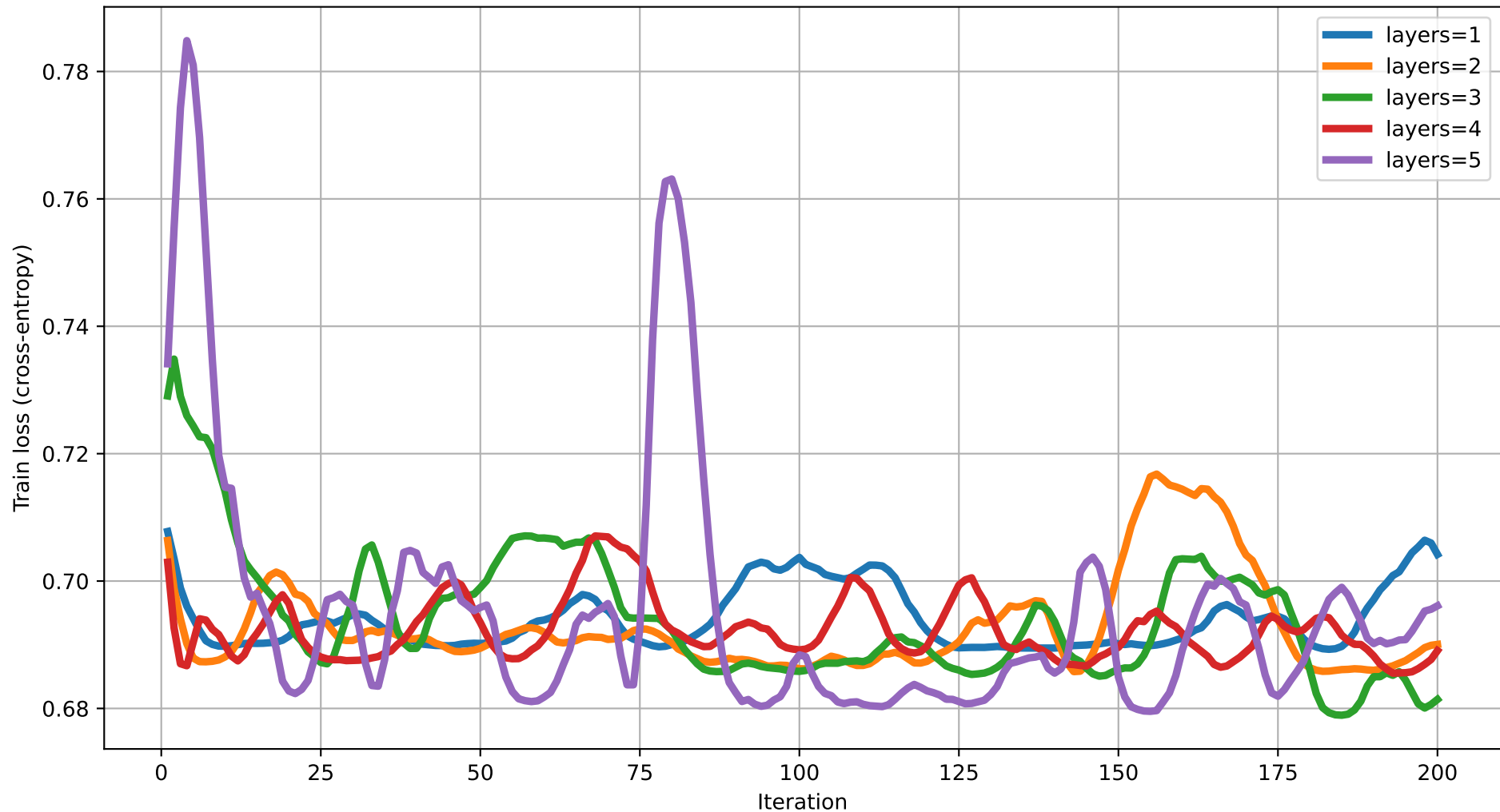
Train loss vs Iteration (dim=20) rot=Rot, ent=chain, gate=CZ
