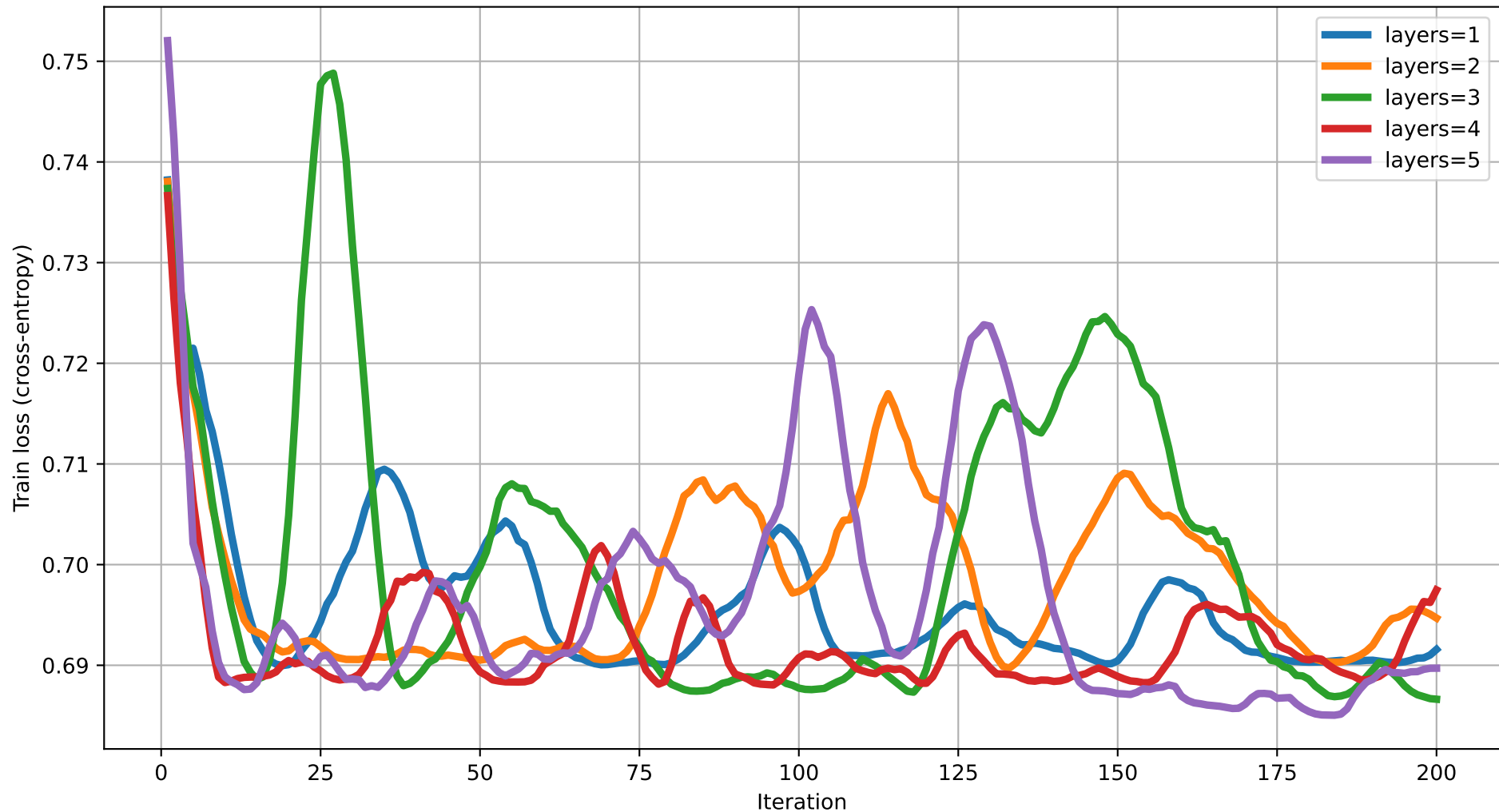
Train loss vs Iteration (dim=16) rot=RX, ent=ring, gate=CZ
