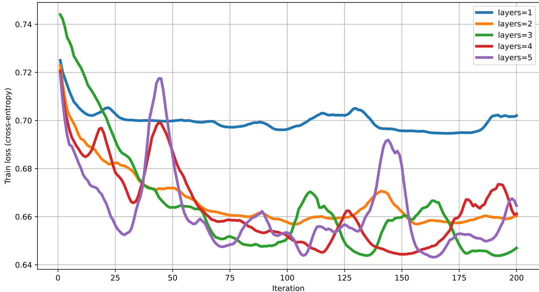
Train loss vs Iteration (dim=5) rot=RYZ, ent=chain, gate=CZ
