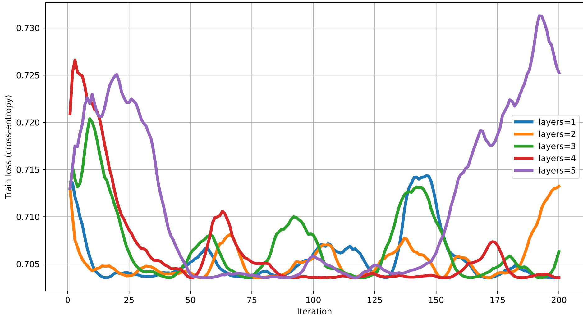
Train loss vs Iteration (dim=11) rot=RZ, ent=chain, gate=CNOT
