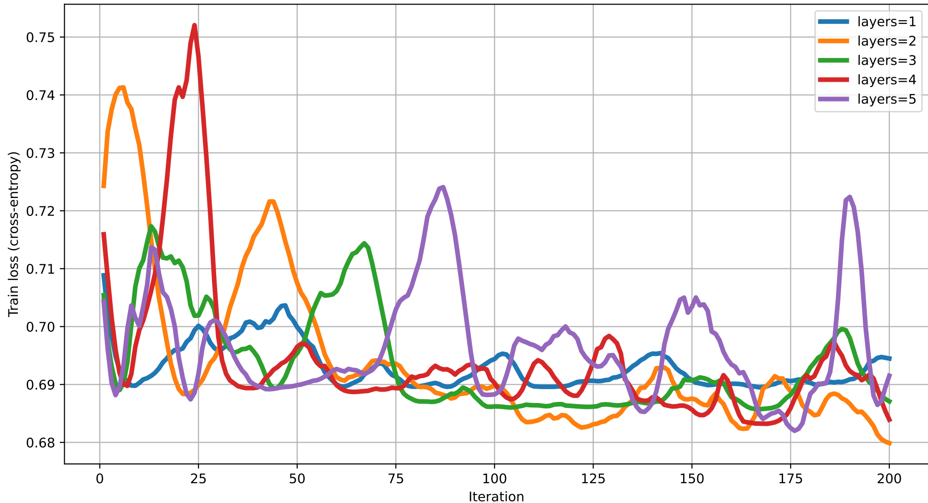
Train loss vs Iteration (dim=20) rot=RYZ, ent=full, gate=CZ
