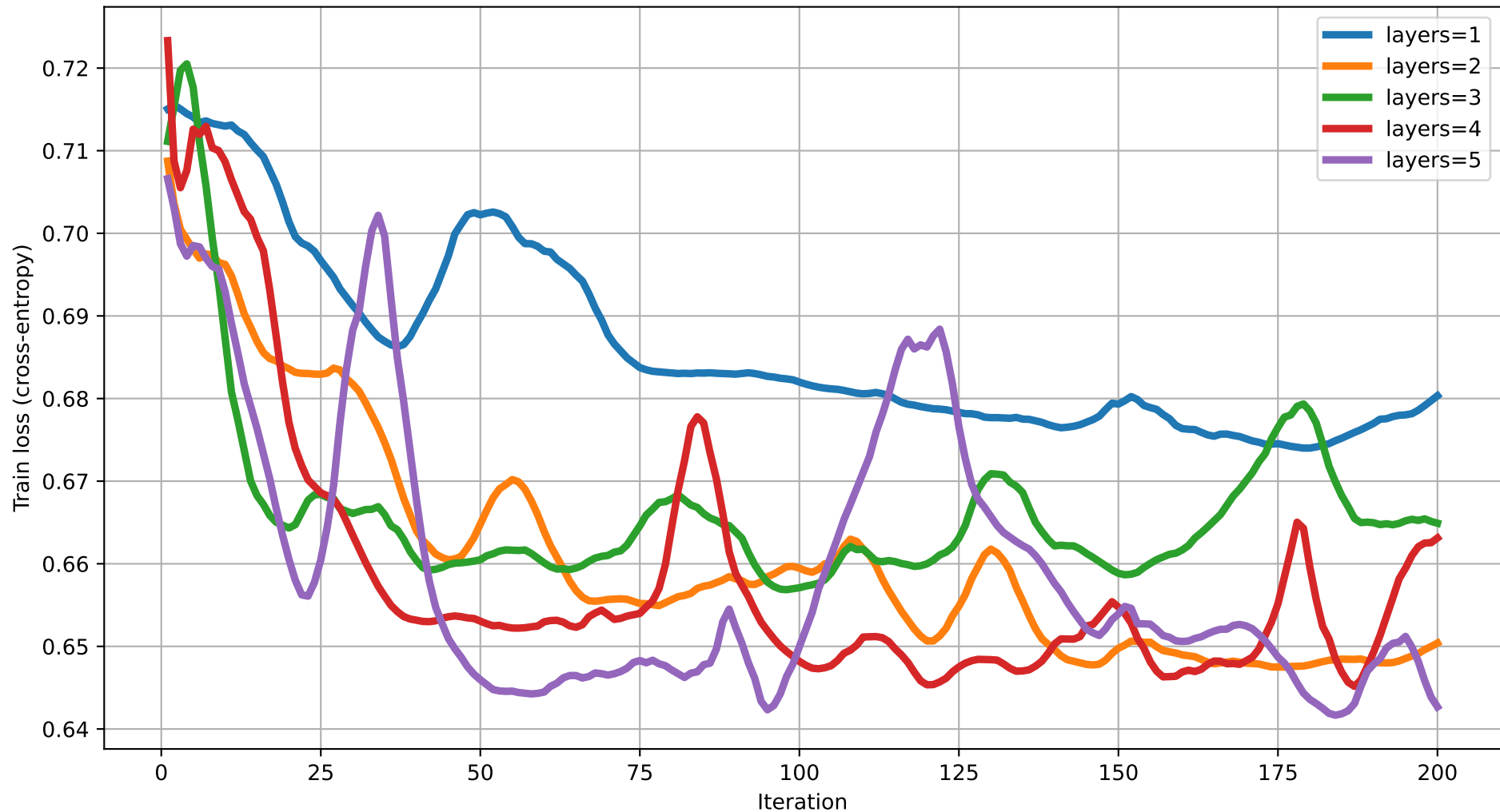
Train loss vs Iteration (dim=5) rot=RY, ent=ring, gate=CNOT
