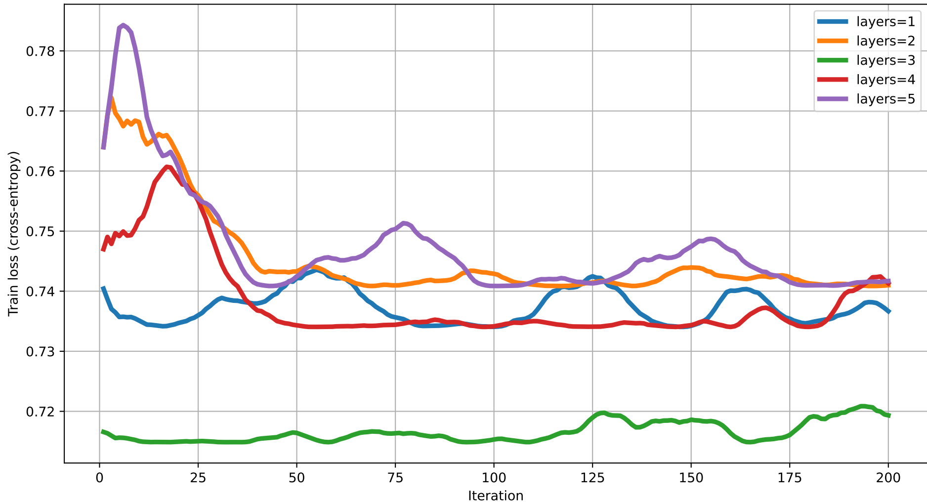
Train loss vs Iteration (dim=3) rot=RZ, ent=ring, gate=CNOT
