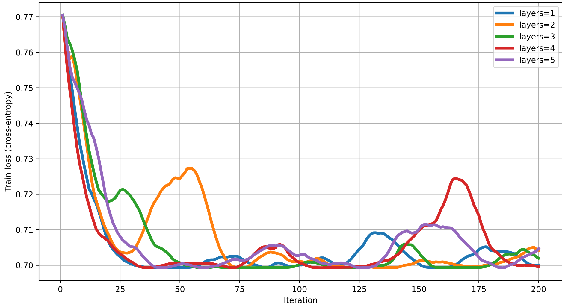
Train loss vs Iteration (dim=17) rot=RZ, ent=pairwise, gate=CNOT
