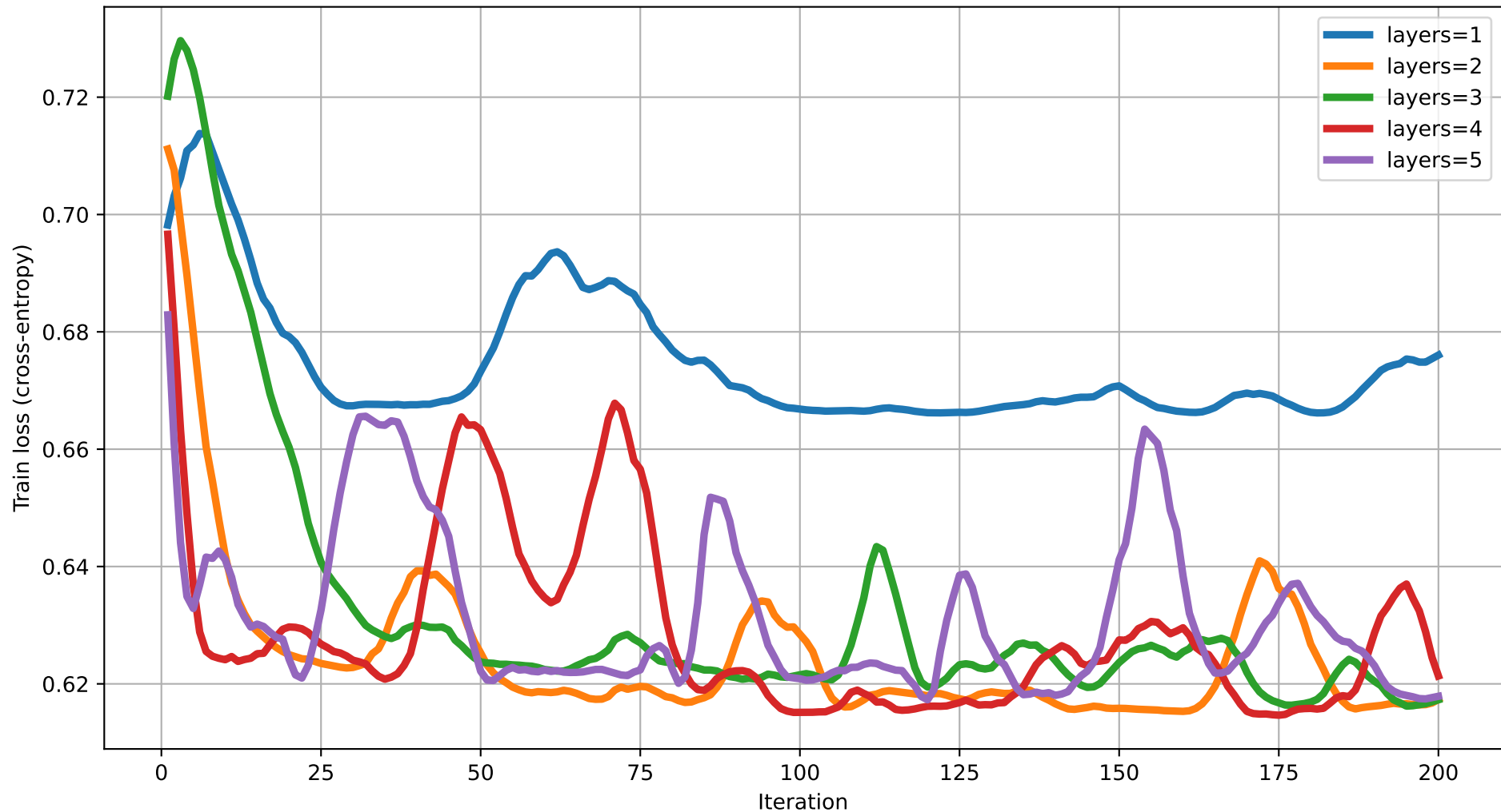
Train loss vs Iteration (dim=10) rot=RYZ, ent=pairwise, gate=CNOT
