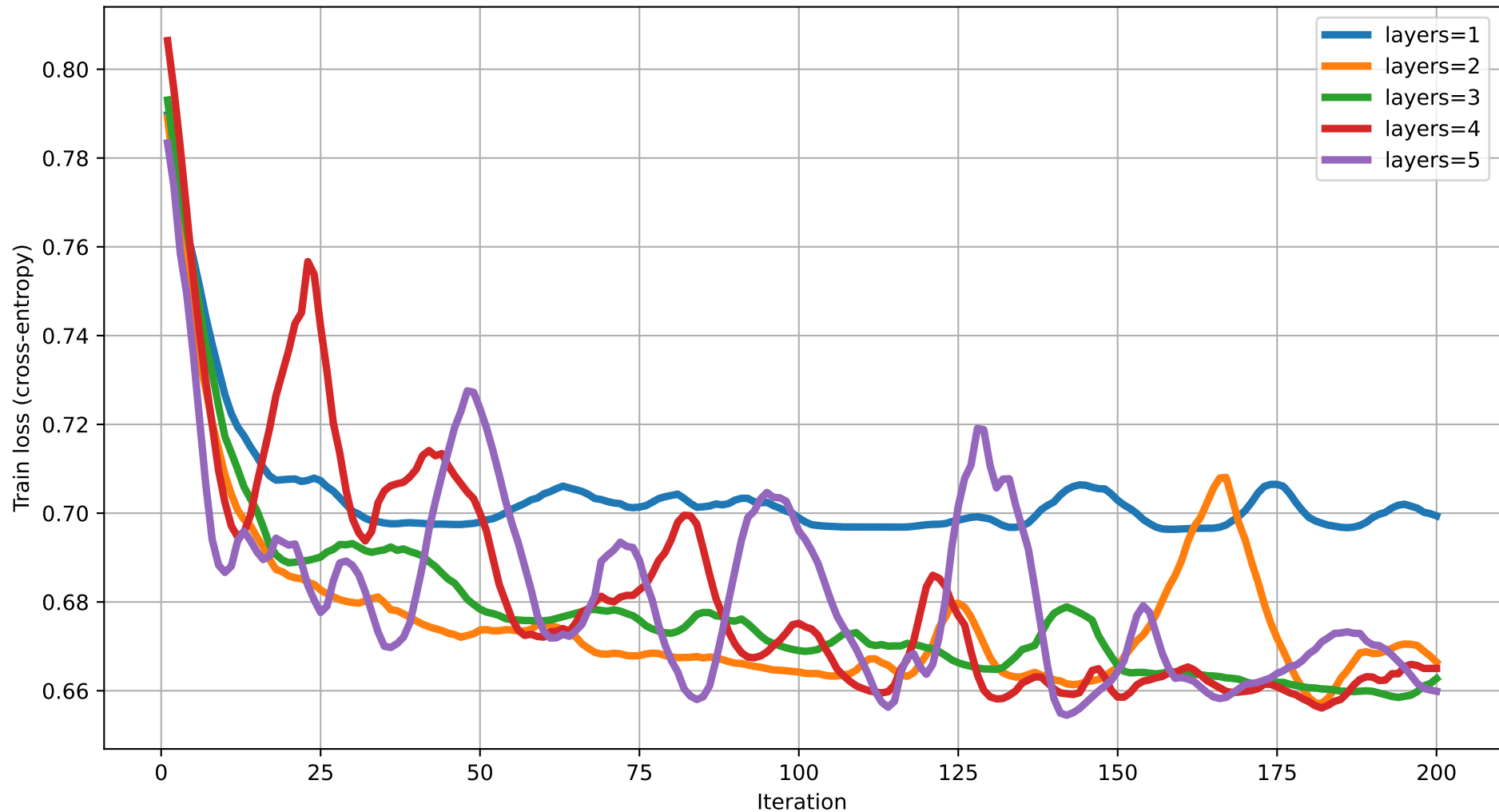
Train loss vs Iteration (dim=2) rot=Rot, ent=chain, gate=CZ
