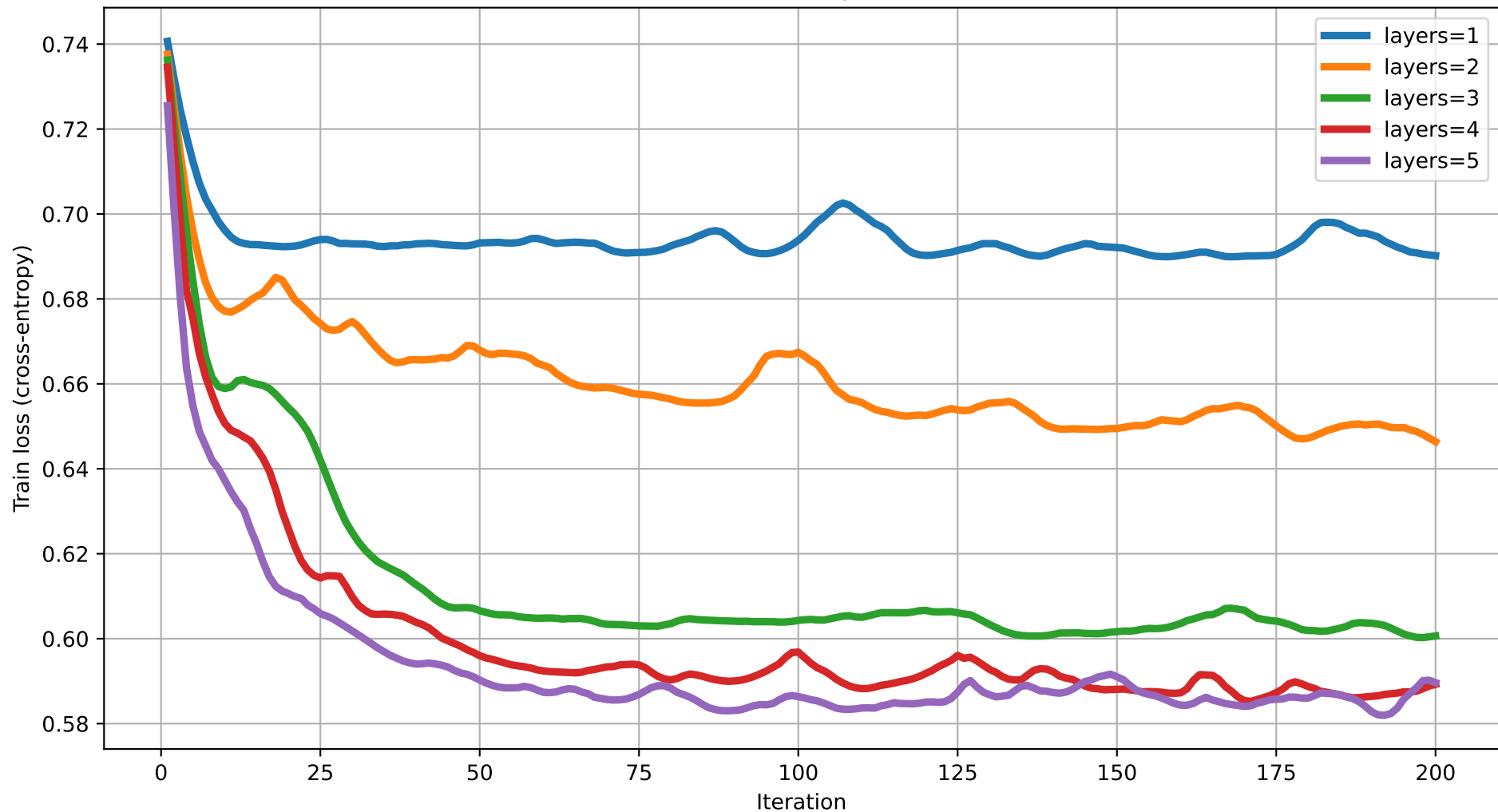
Train loss vs Iteration (degree=5) rot=RY, ent=full, gate=CNOT
