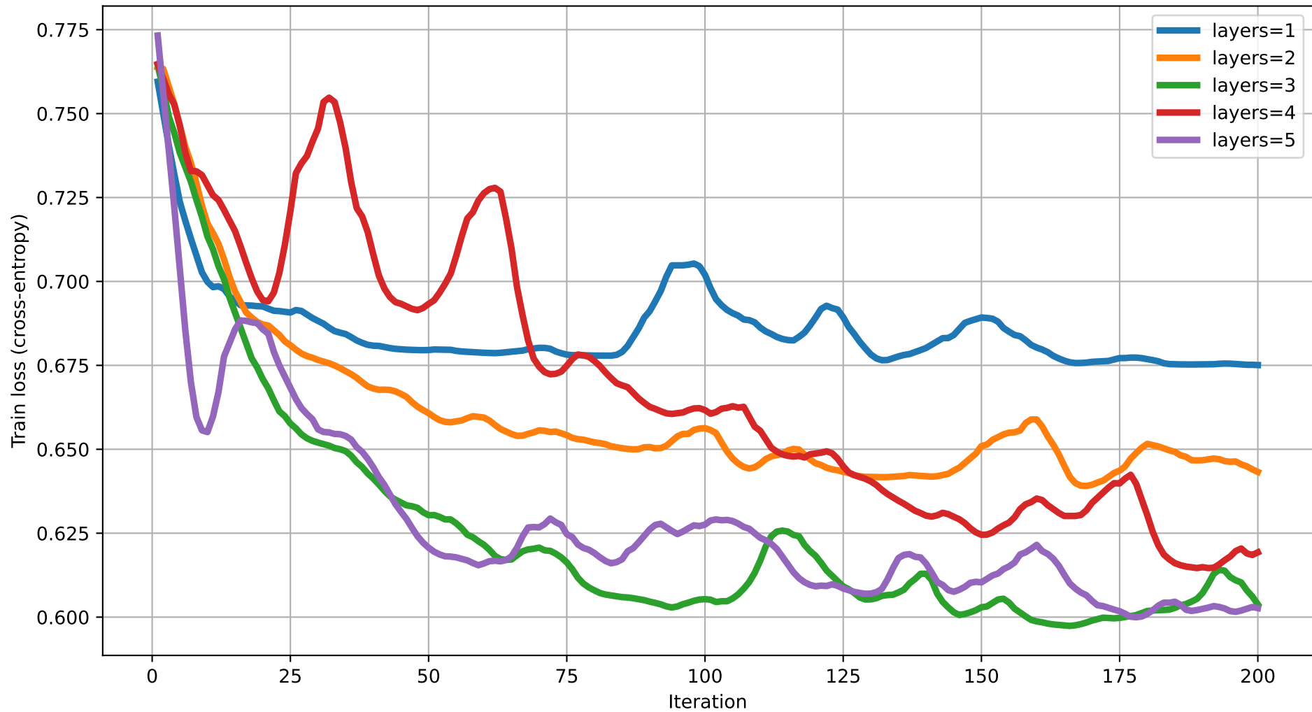
Train loss vs Iteration (dim=8) rot=RY, ent=full, gate=CZ
