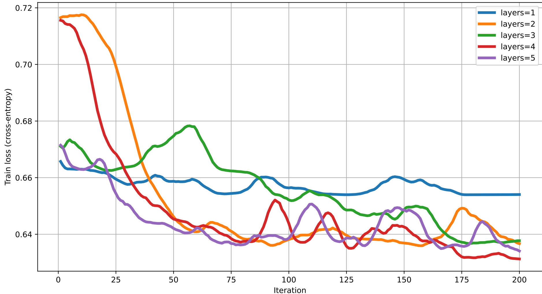
Train loss vs Iteration (dim=7) rot=RZ, ent=ring, gate=IsingXX
