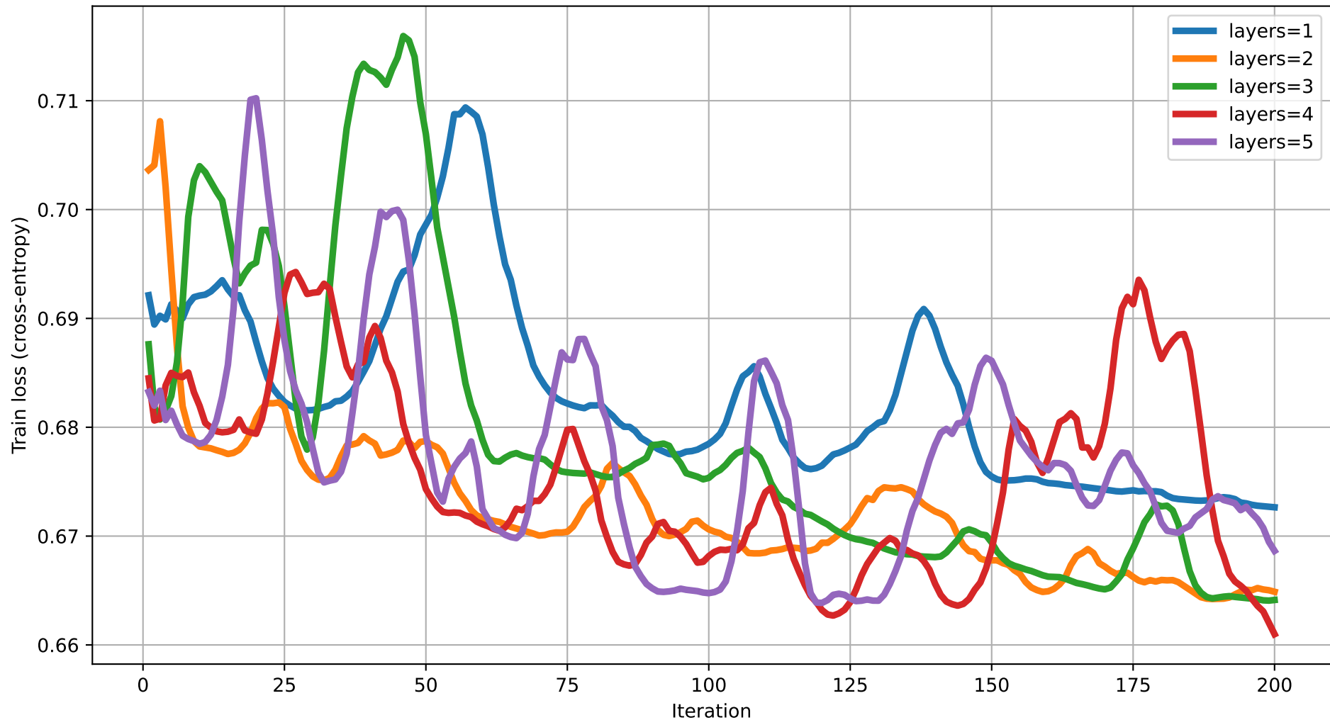
Train loss vs Iteration (dim=13) rot=RYZ, ent=chain, gate=CNOT
