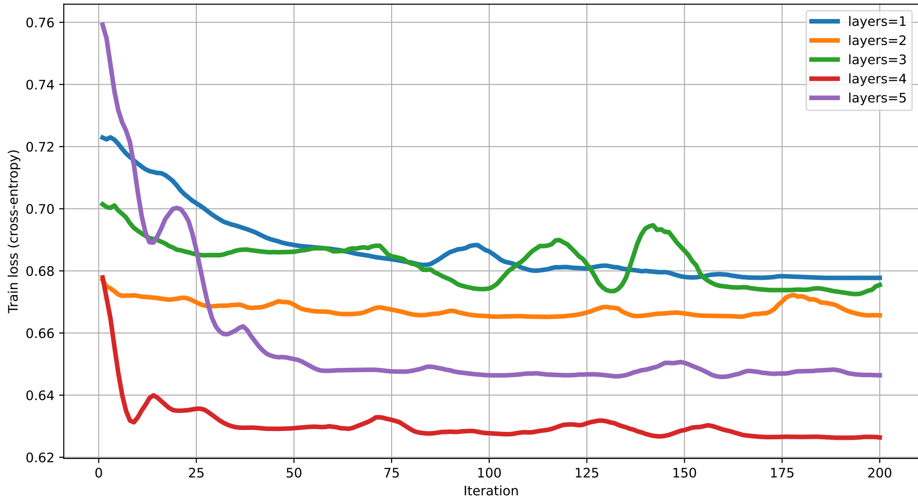
Train loss vs Iteration (degree=2) rot=RX, ent=ring, gate=CNOT
