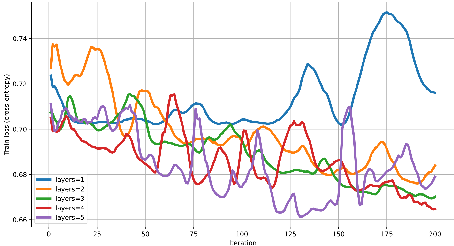
Train loss vs Iteration (dim=11) rot=Rot, ent=full, gate=CNOT
