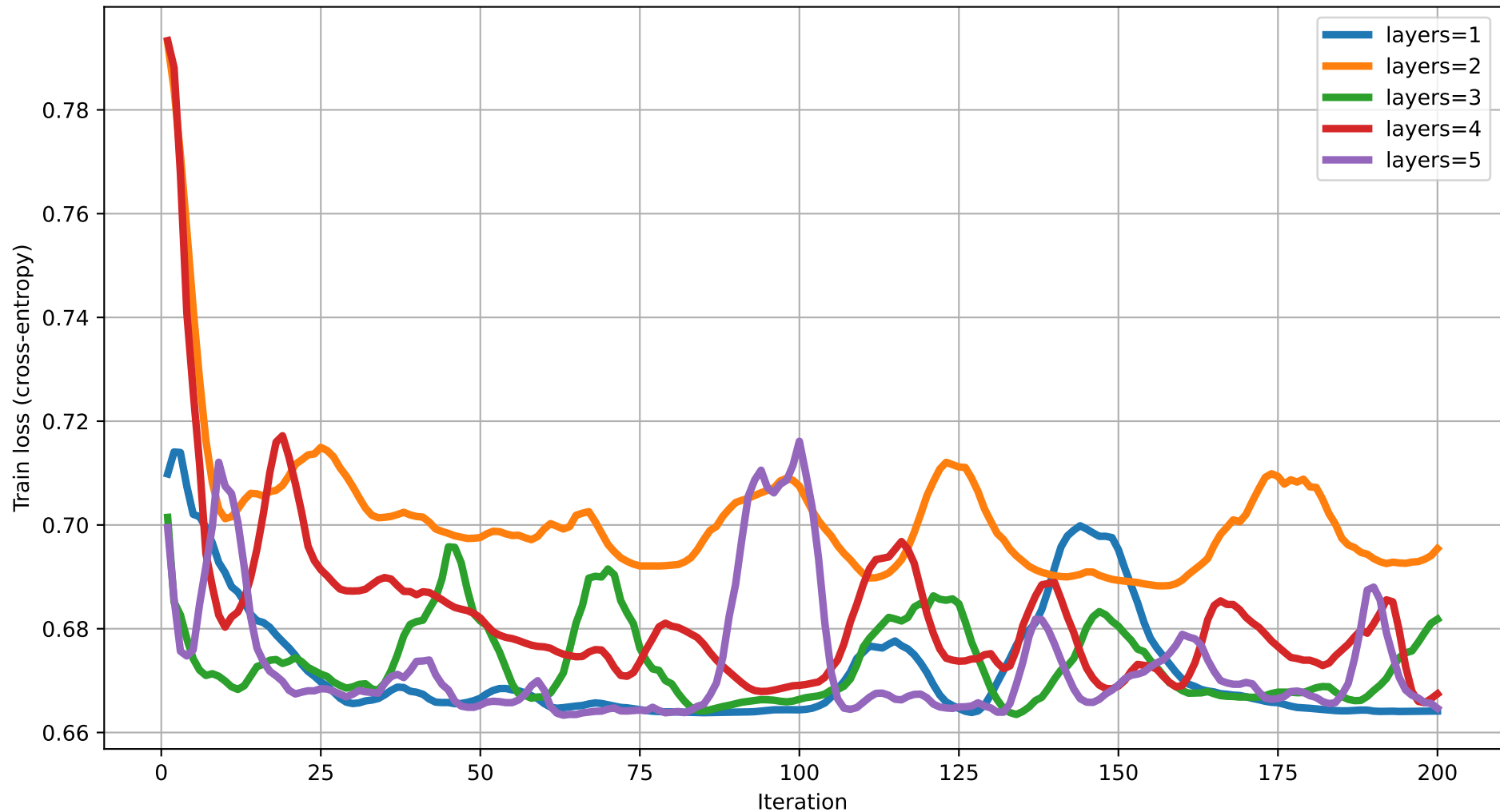
Train loss vs Iteration (dim=17) rot=RYZ, ent=ring, gate=IsingXX
