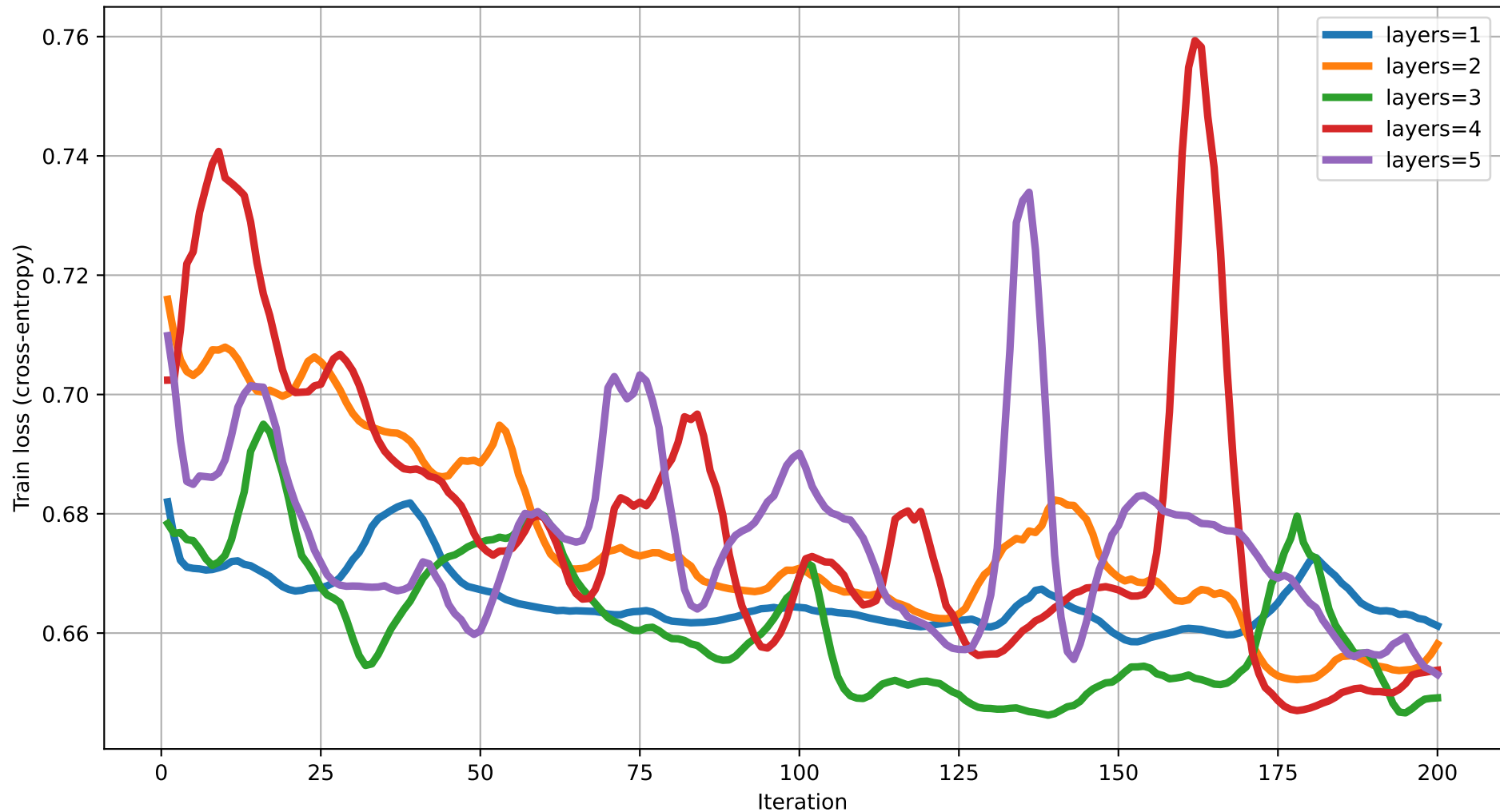
Train loss vs Iteration (dim=6) rot=RYZ, ent=ring, gate=IsingXX
