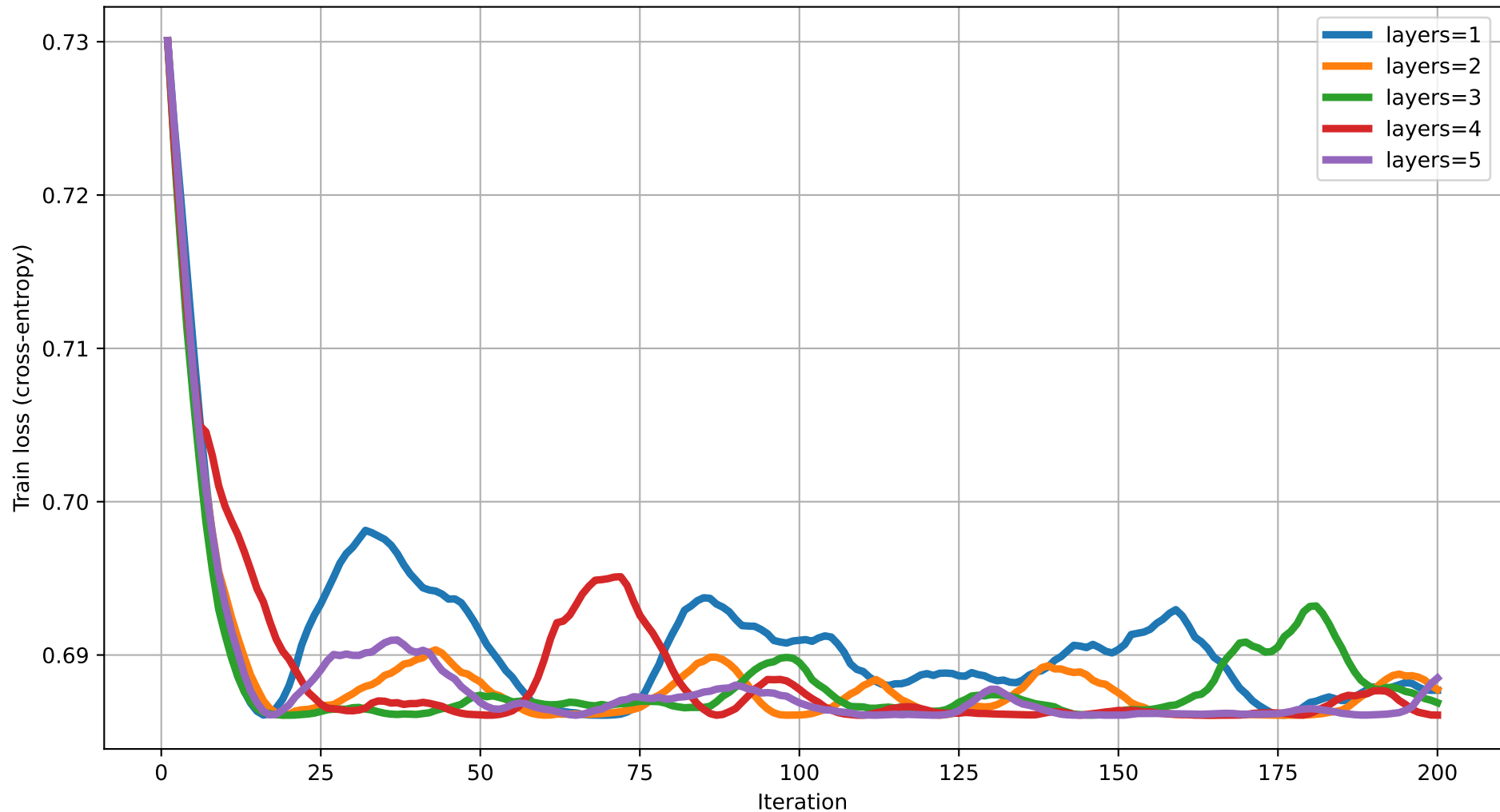
Train loss vs Iteration (degree=2) rot=RZ, ent=pairwise, gate=CNOT
