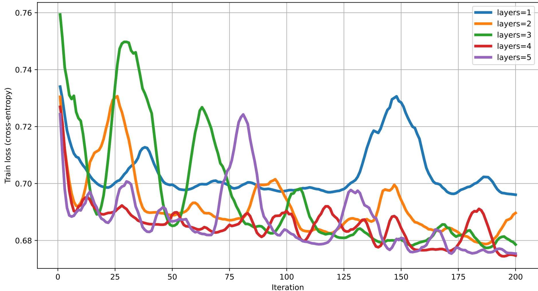
Train loss vs Iteration (dim=19) rot=RY, ent=pairwise, gate=CZ
