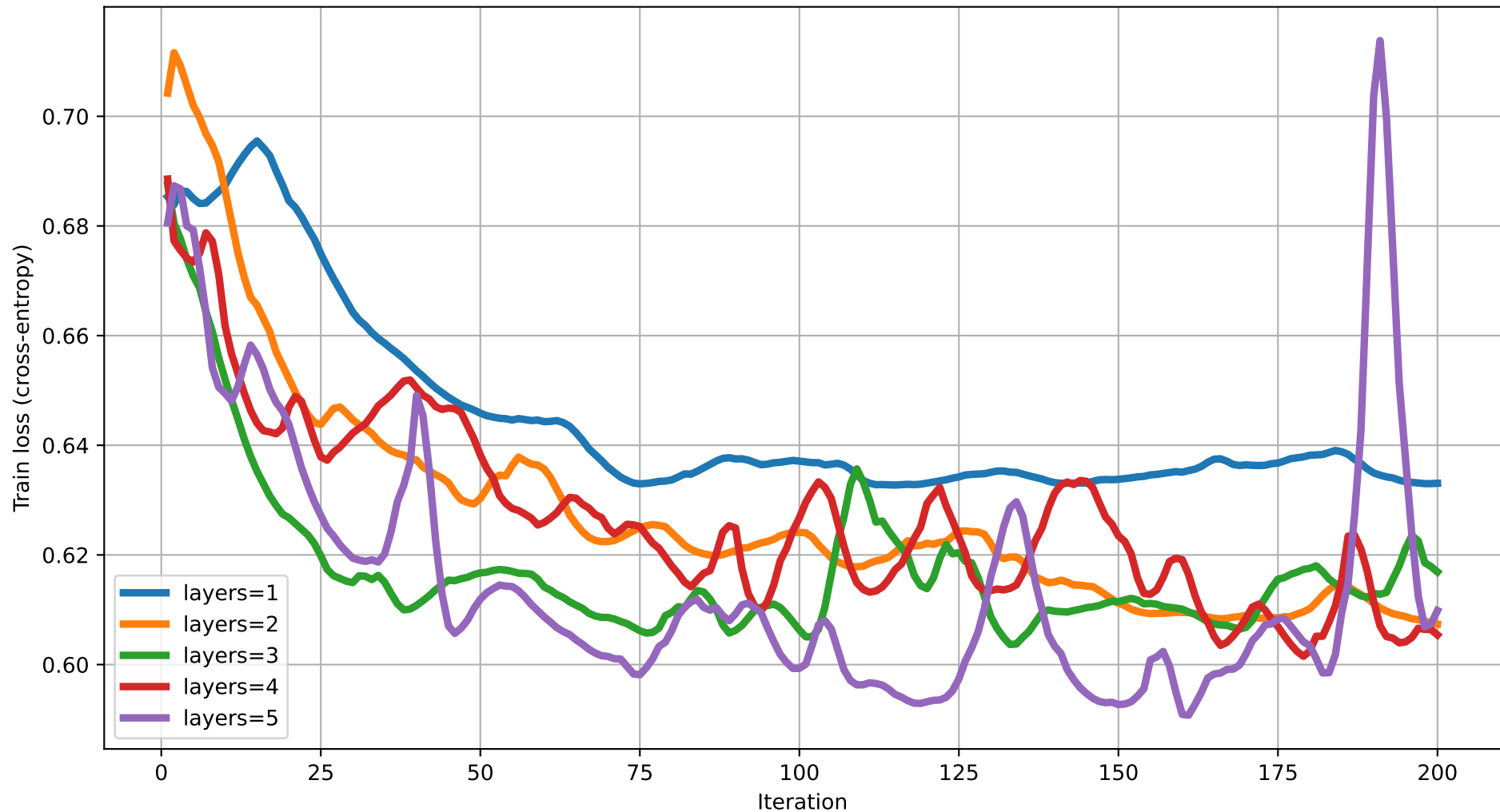
Train loss vs Iteration (dim=13) rot=Rot, ent=chain, gate=IsingXX
