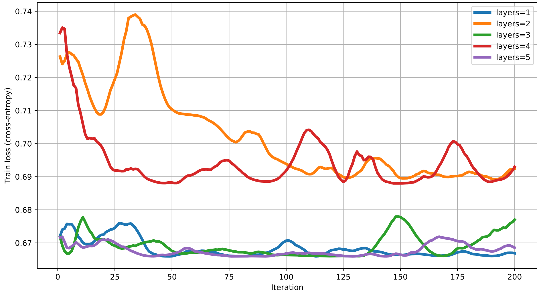
Train loss vs Iteration (dim=6) rot=RX, ent=ring, gate=IsingXX
