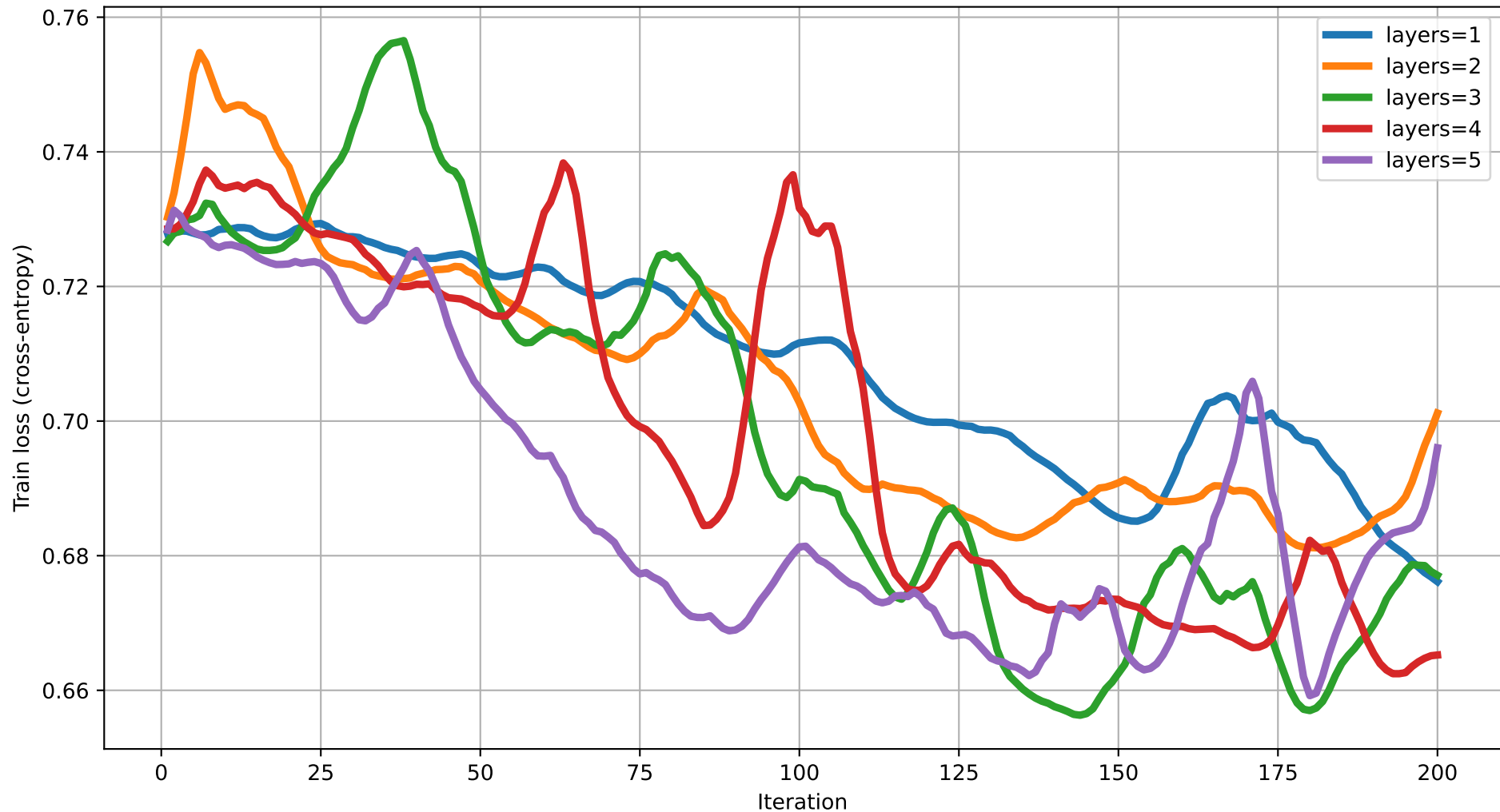
Train loss vs Iteration (dim=7) rot=RYZ, ent=ring, gate=CZ
