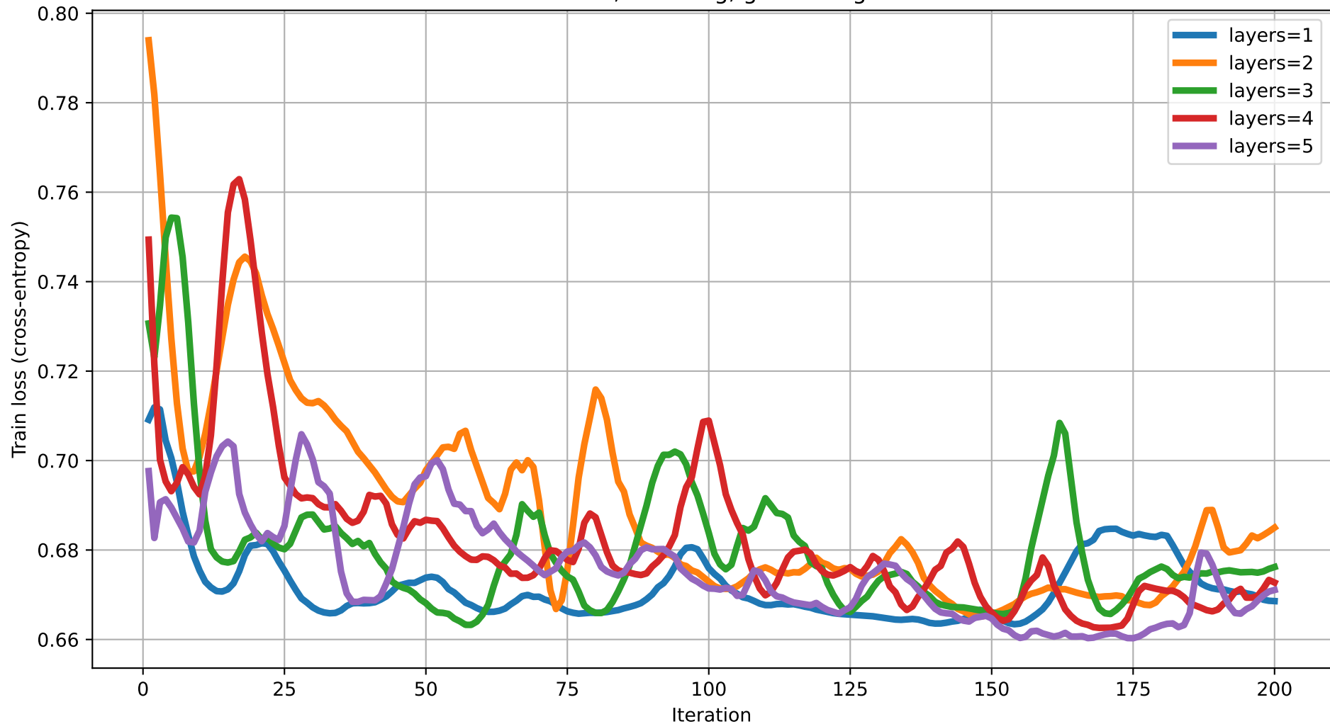
Train loss vs Iteration (dim=17) rot=Rot, ent=ring, gate=IsingXX
