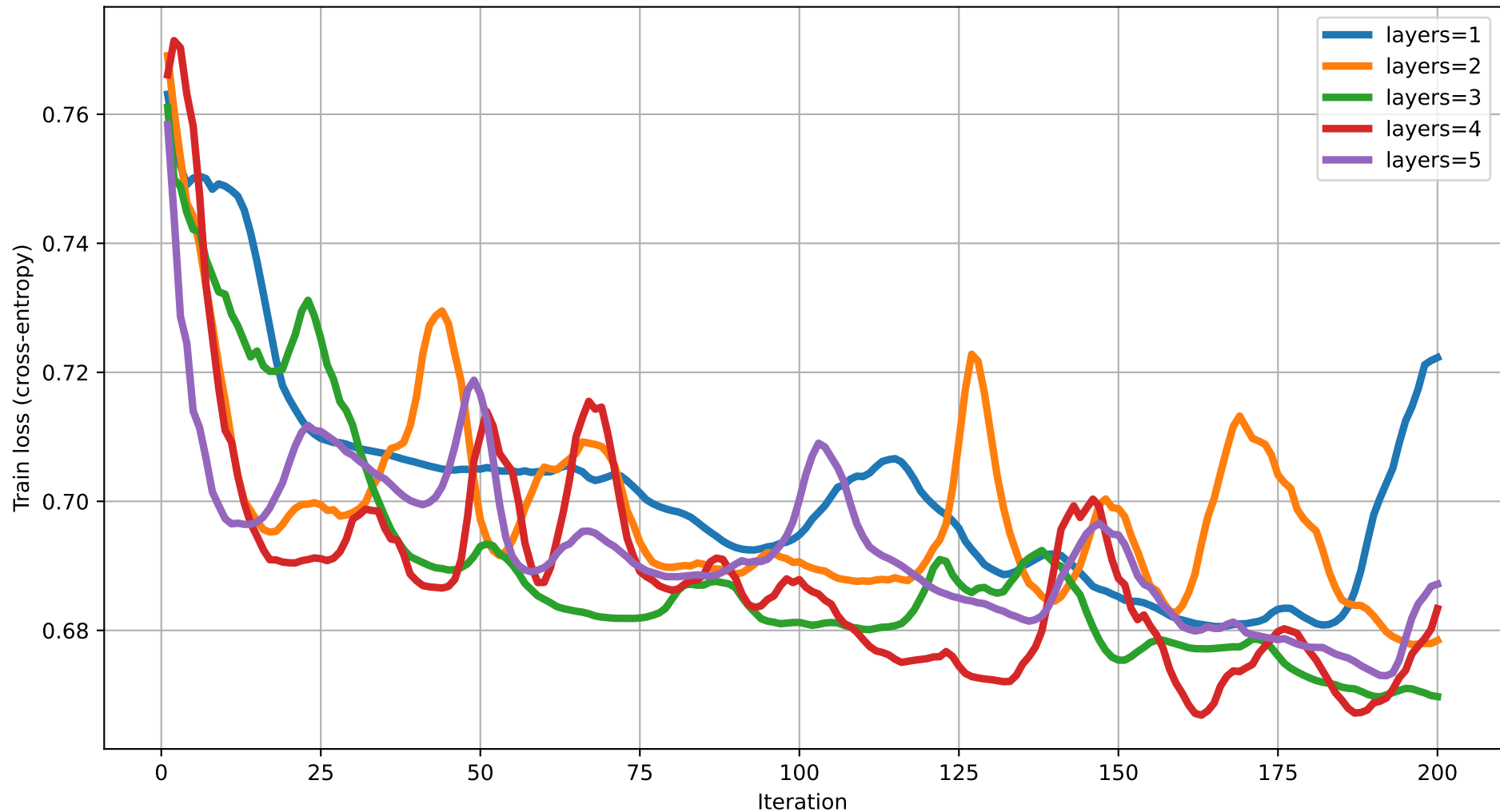
Train loss vs Iteration (dim=17) rot=RZ, ent=full, gate=IsingXX
