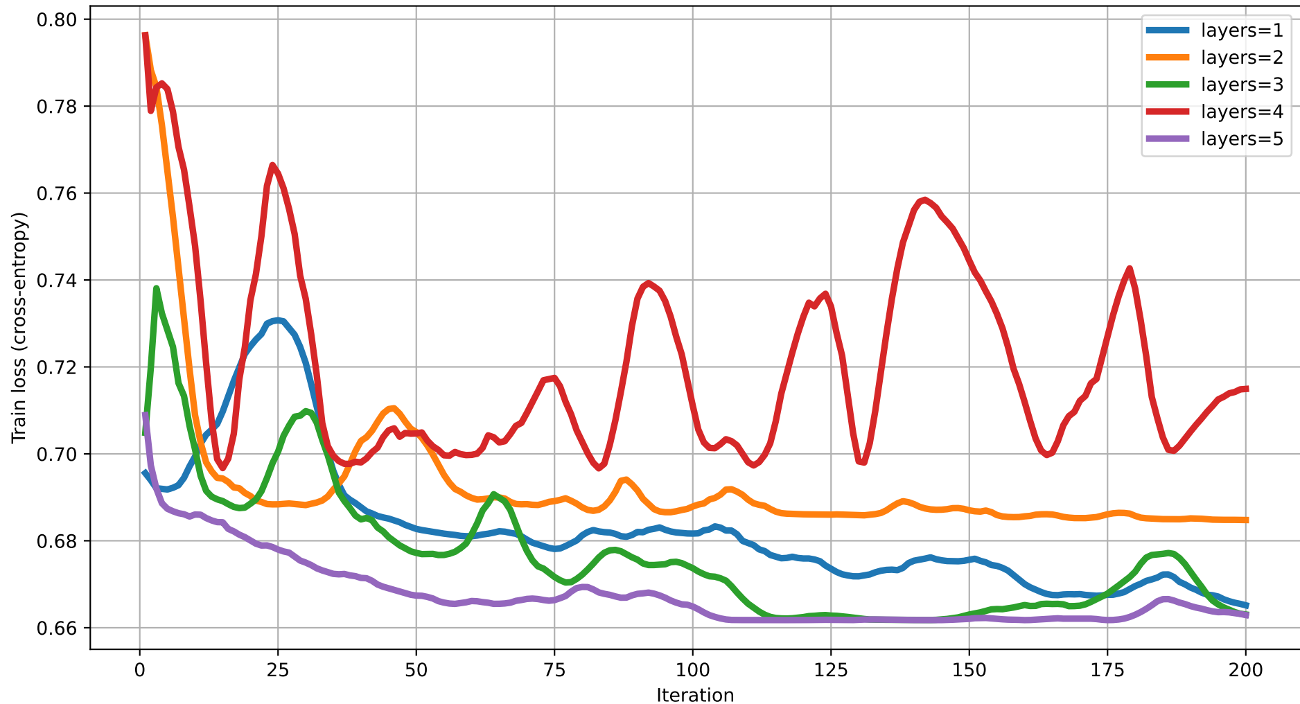
Train loss vs Iteration (dim=8) rot=RX, ent=full, gate=IsingXX
