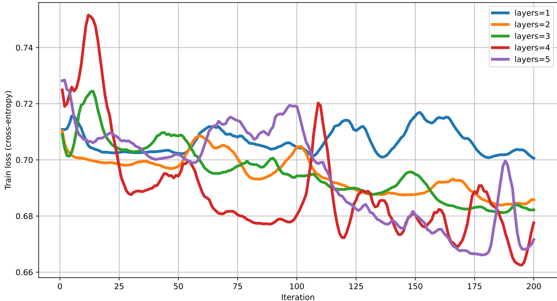
Train loss vs Iteration (dim=11) rot=RY, ent=full, gate=CZ
