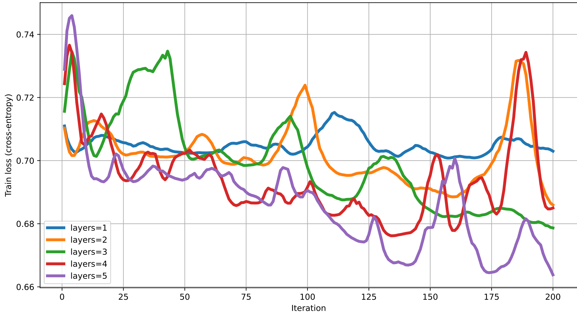
Train loss vs Iteration (dim=11) rot=RYZ, ent=ring, gate=CZ
