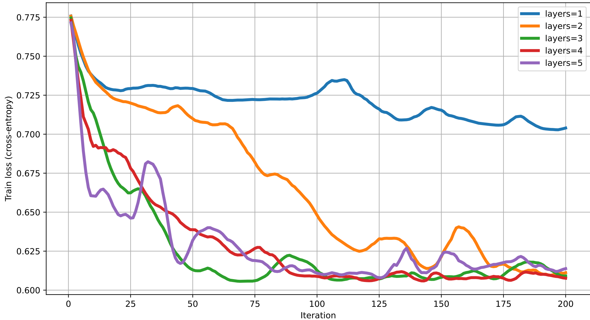
Train loss vs Iteration (dim=9) rot=RY, ent=pairwise, gate=CNOT
