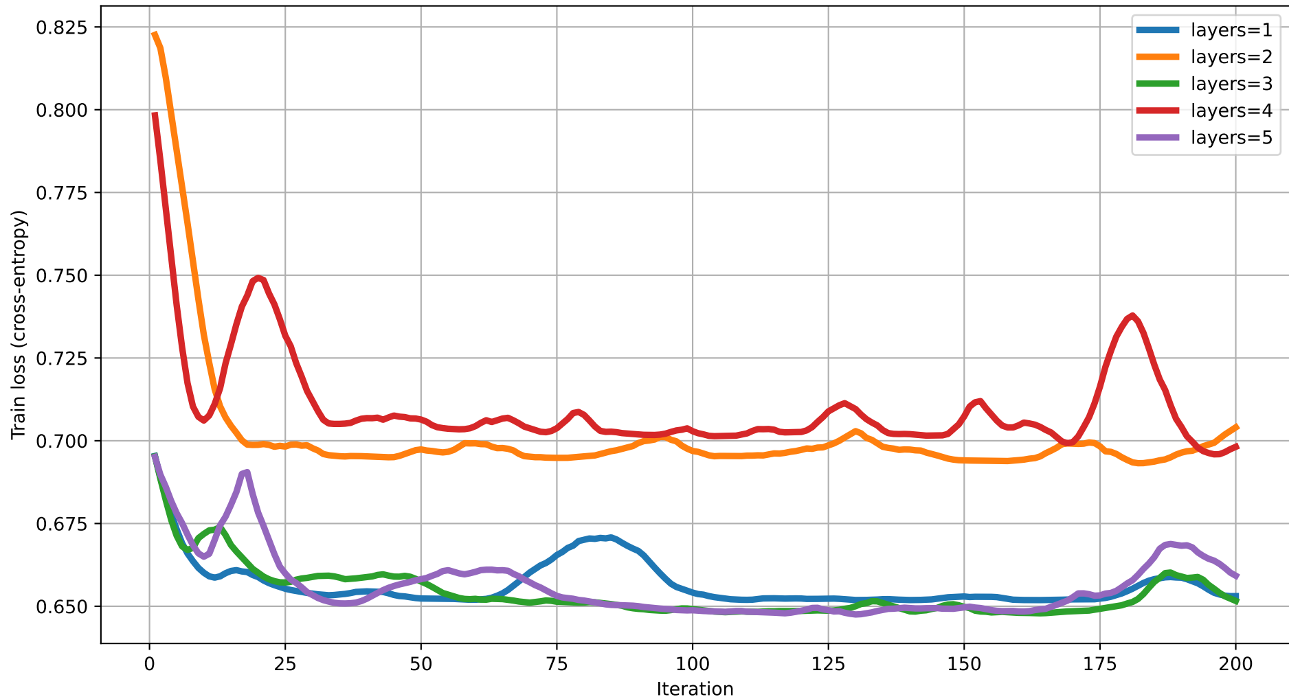
Train loss vs Iteration (dim=8) rot=RZ, ent=ring, gate=IsingXX
