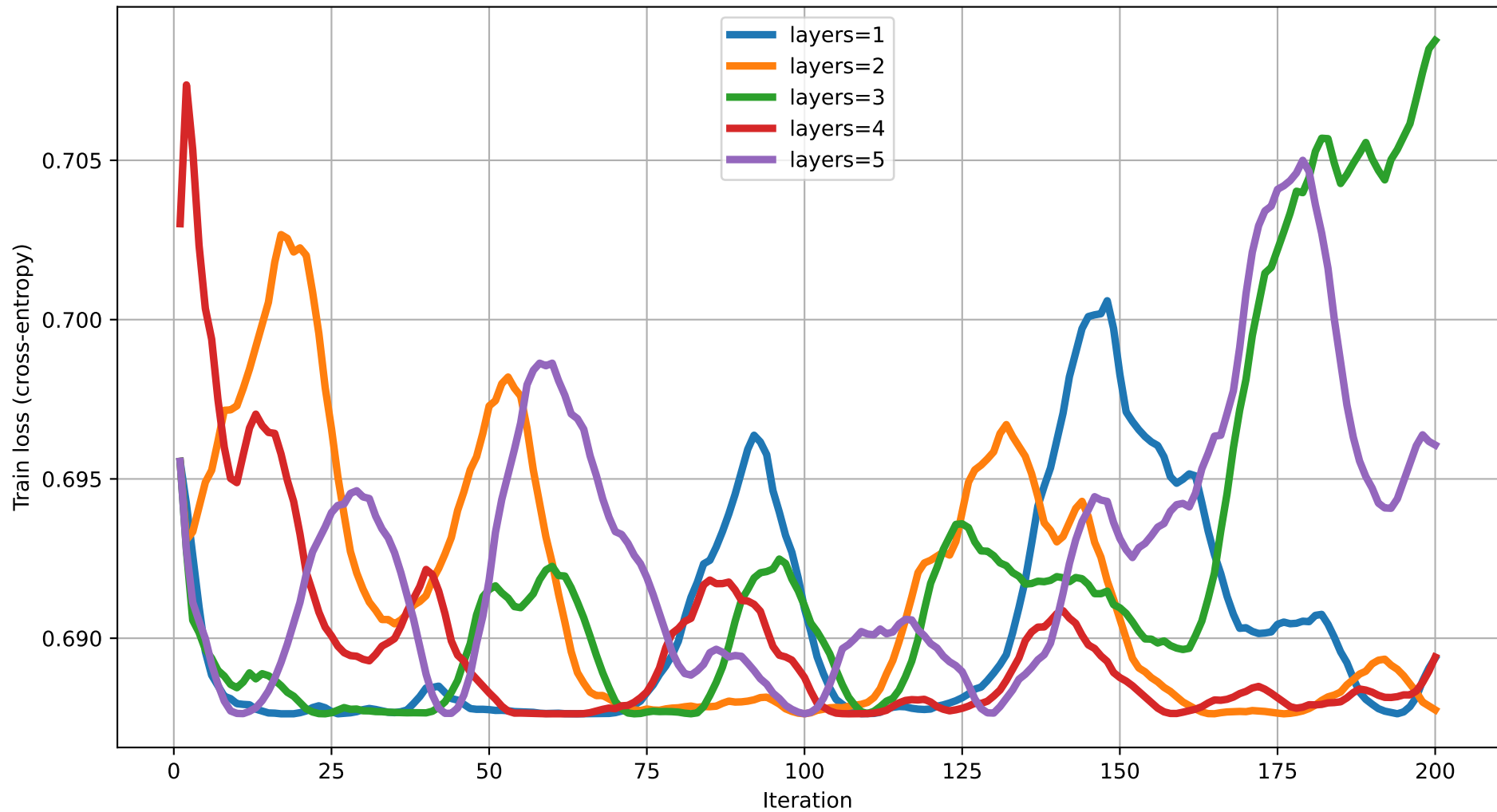
Train loss vs Iteration (dim=13) rot=RZ, ent=chain, gate=CZ
