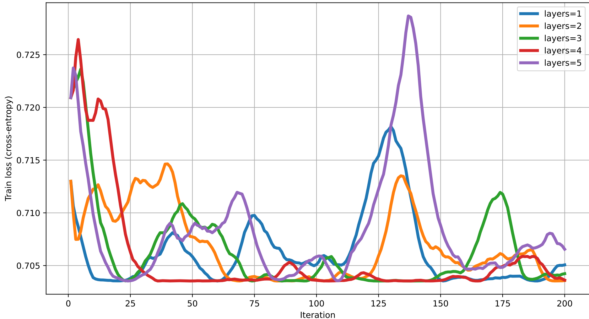
Train loss vs Iteration (dim=11) rot=RZ, ent=full, gate=CZ
