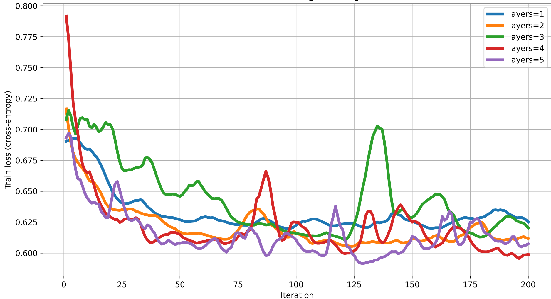
Train loss vs Iteration (dim=9) rot=Rot, ent=full, gate=IsingXX
