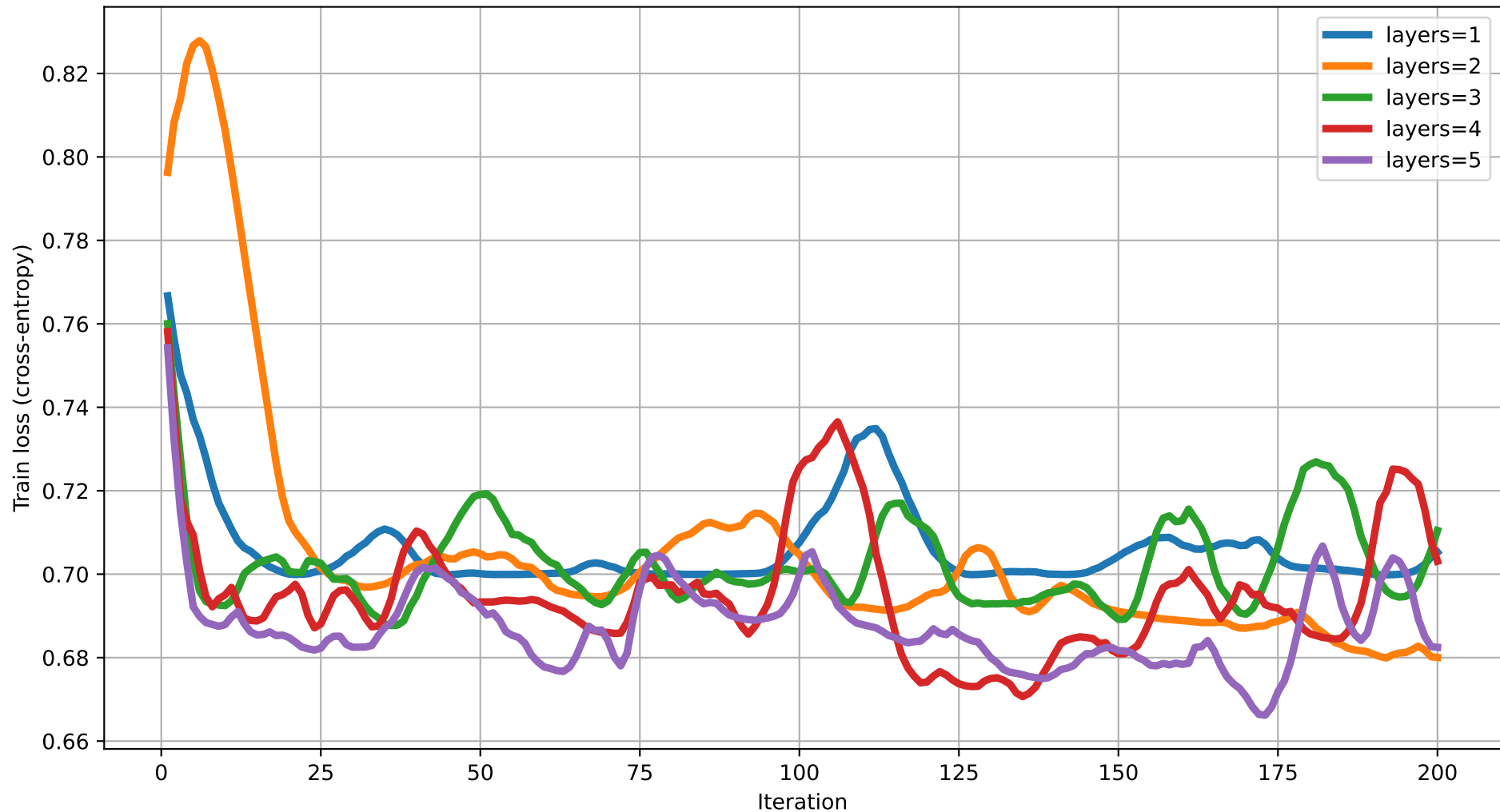
Train loss vs Iteration (dim=17) rot=Rot, ent=full, gate=CNOT
