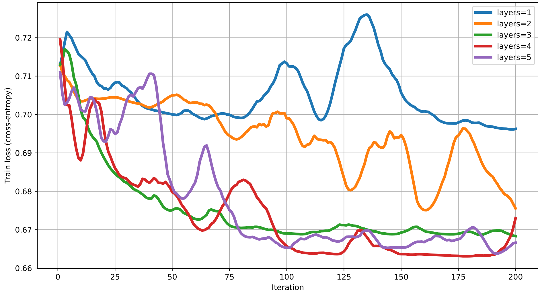
Train loss vs Iteration (dim=11) rot=RX, ent=chain, gate=CNOT
