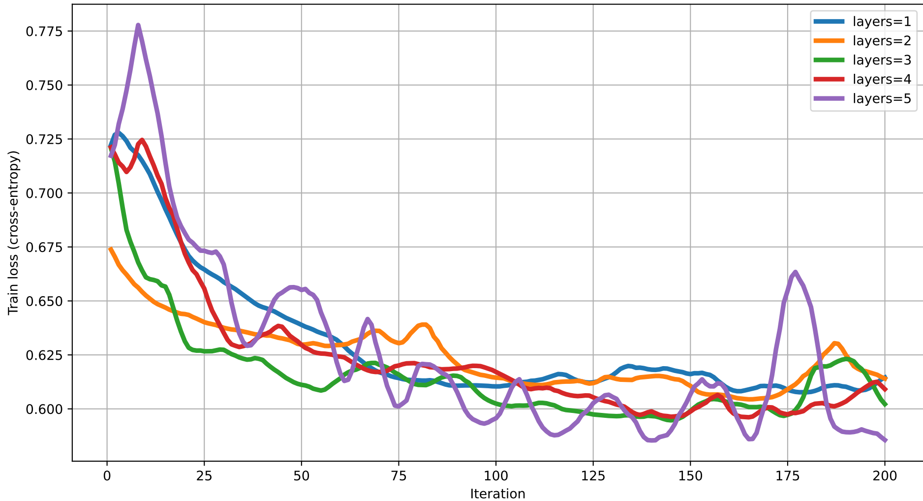
Train loss vs Iteration (dim=4) rot=RYZ, ent=ring, gate=CNOT
