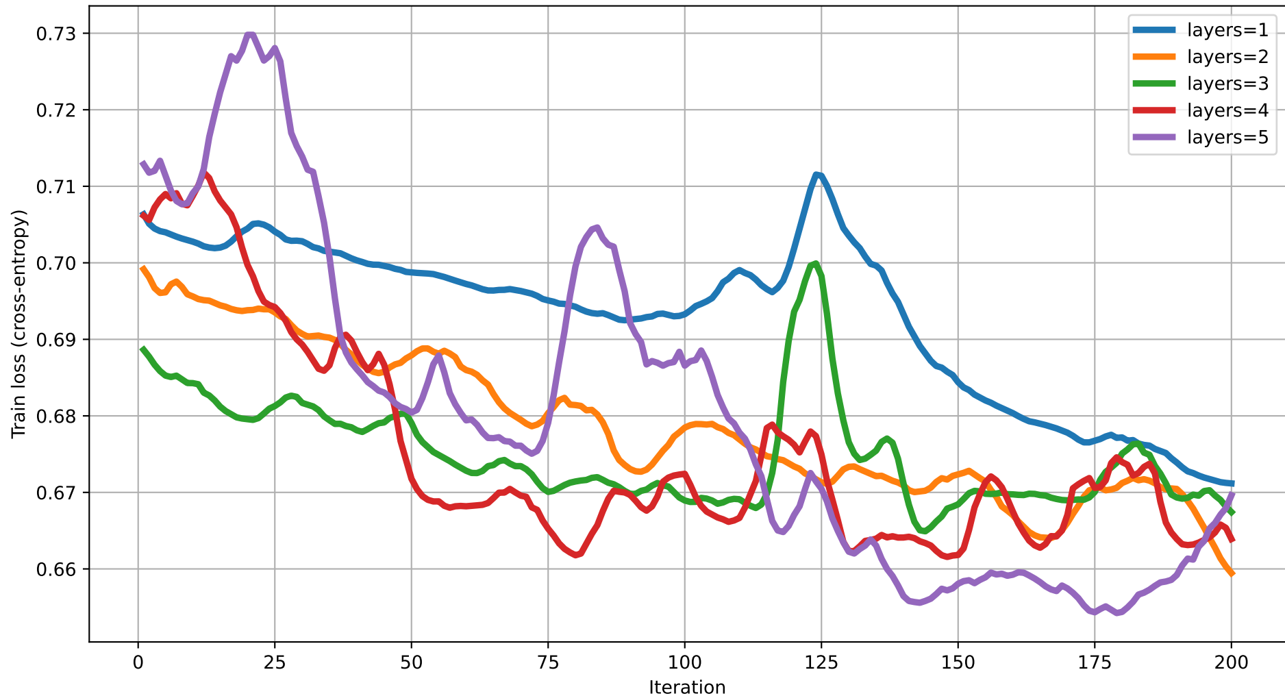
Train loss vs Iteration (dim=10) rot=RYZ, ent=ring, gate=CNOT
