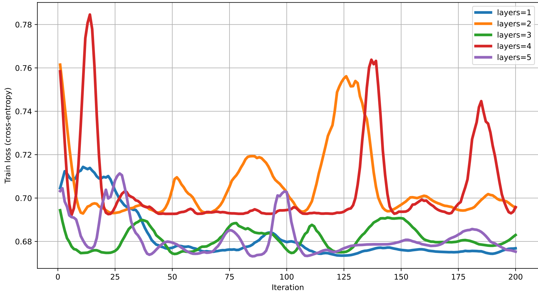
Train loss vs Iteration (dim=8) rot=RX, ent=ring, gate=lsingXX
