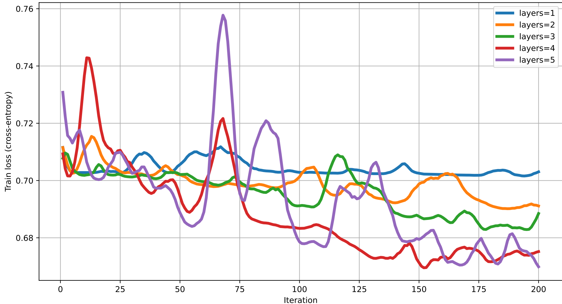
Train loss vs Iteration (dim=11) rot=RY, ent=ring, gate=CZ
