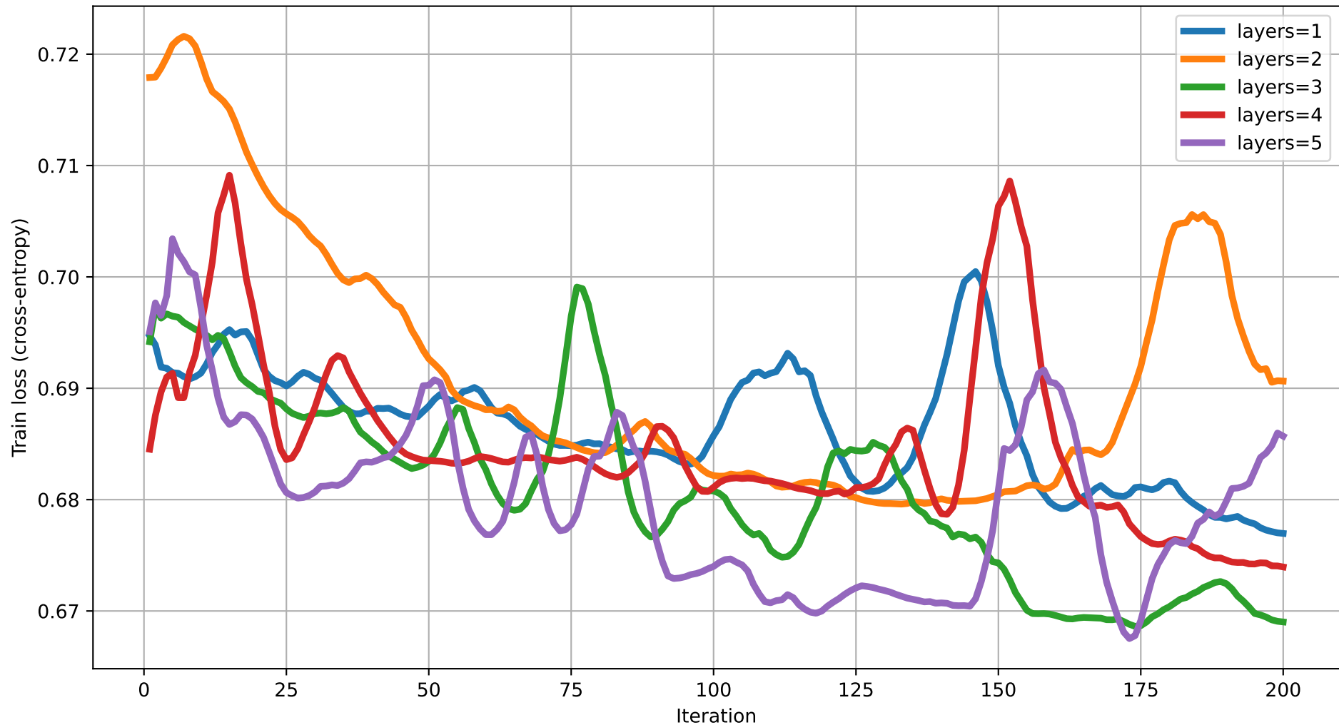
Train loss vs Iteration (dim=15) rot=RZ, ent=chain, gate=IsingXX
