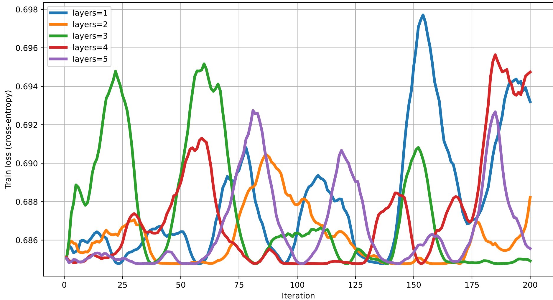
Train loss vs Iteration (dim=15) rot=RZ, ent=full, gate=CNOT
