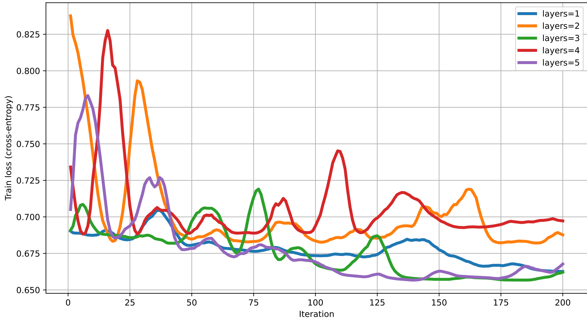
Train loss vs Iteration (dim=16) rot=RX, ent=pairwise, gate=IsingXX
