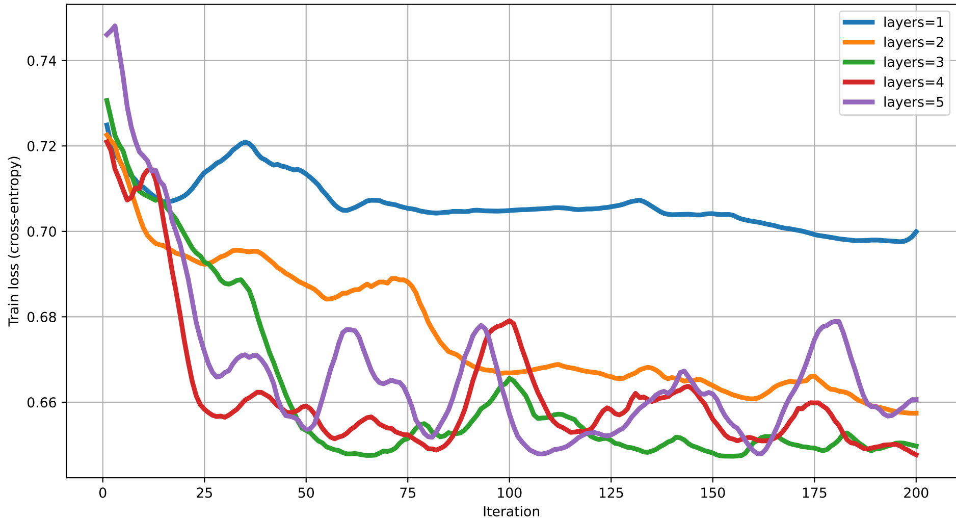
Train loss vs Iteration (dim=5) rot=RY, ent=full, gate=CZ
