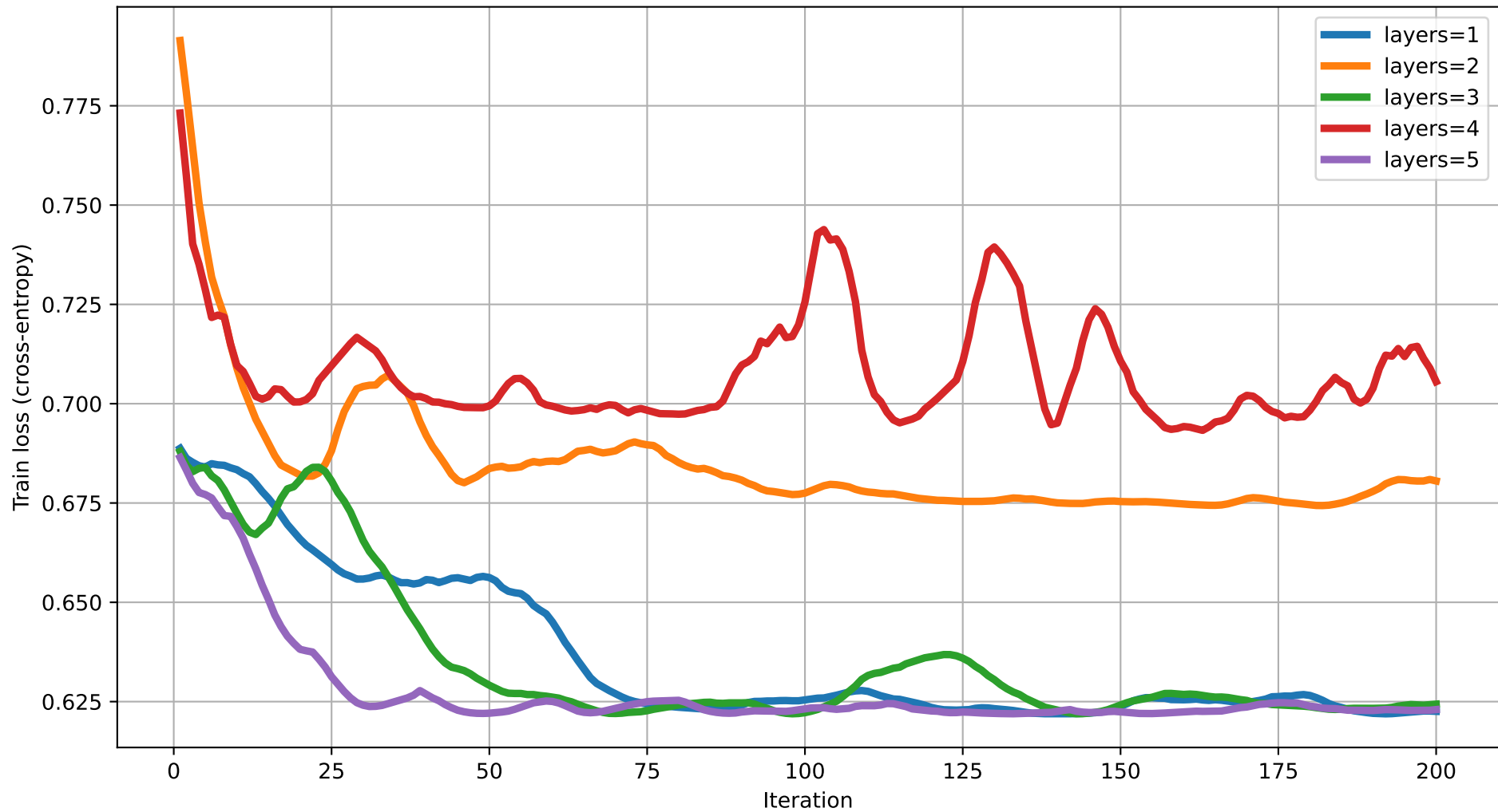
Train loss vs Iteration (dim=4) rot=RX, ent=chain, gate=IsingXX
