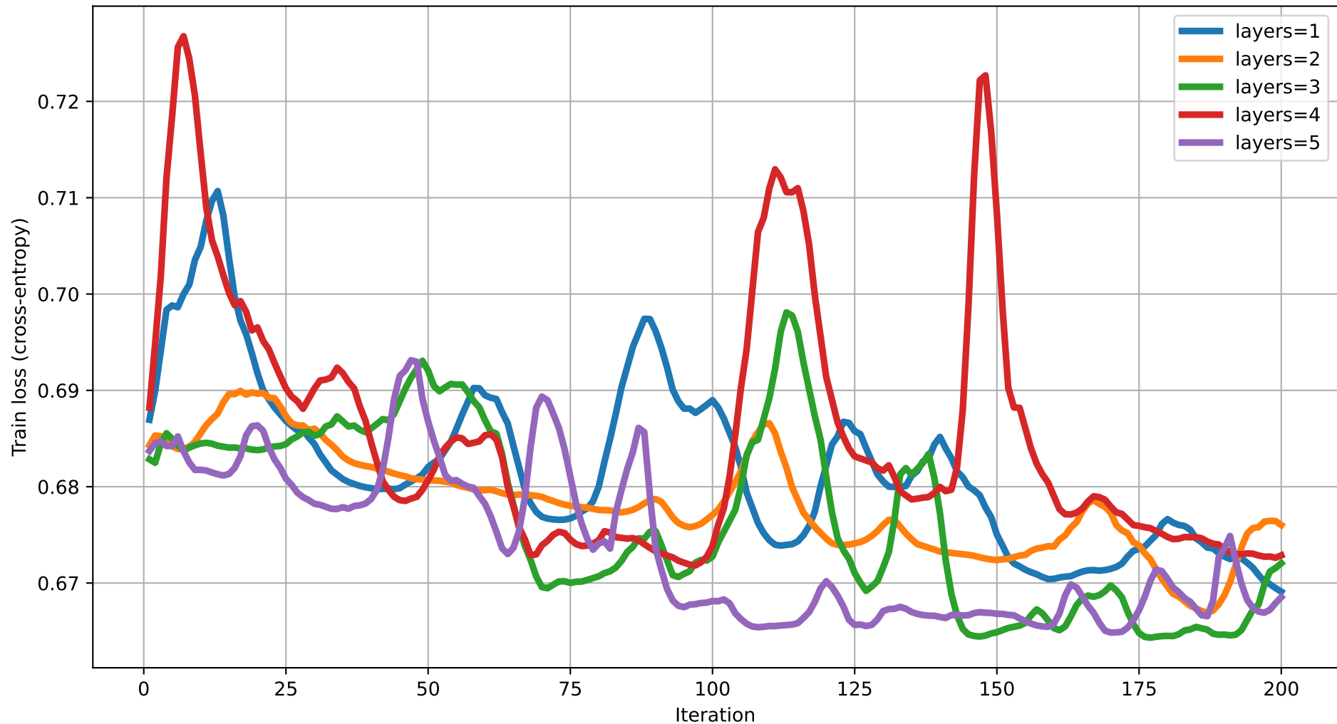
Train loss vs Iteration (dim=15) rot=Rot, ent=ring, gate=CZ
