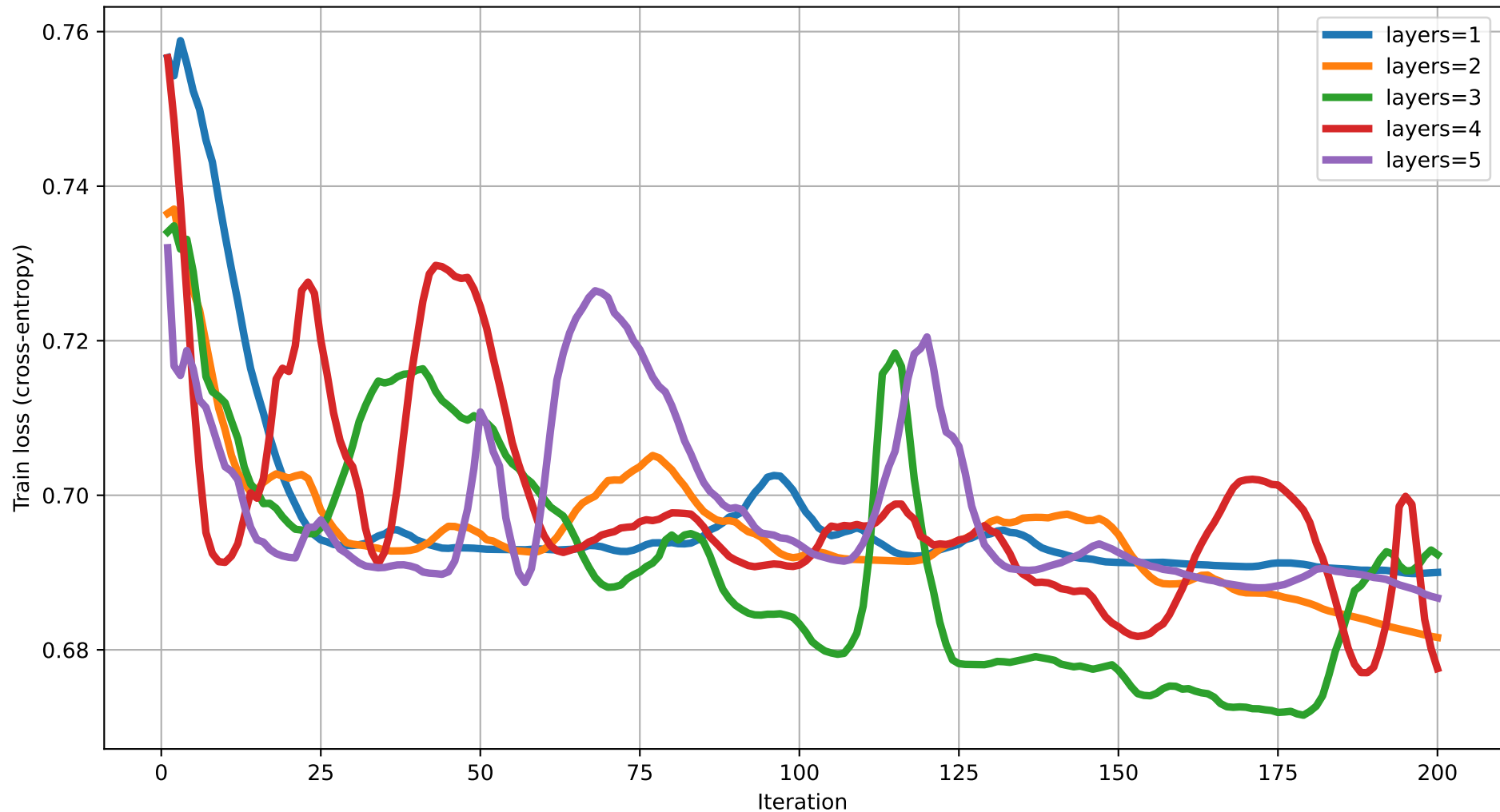
Train loss vs Iteration (dim=16) rot=RY, ent=pairwise, gate=CZ
