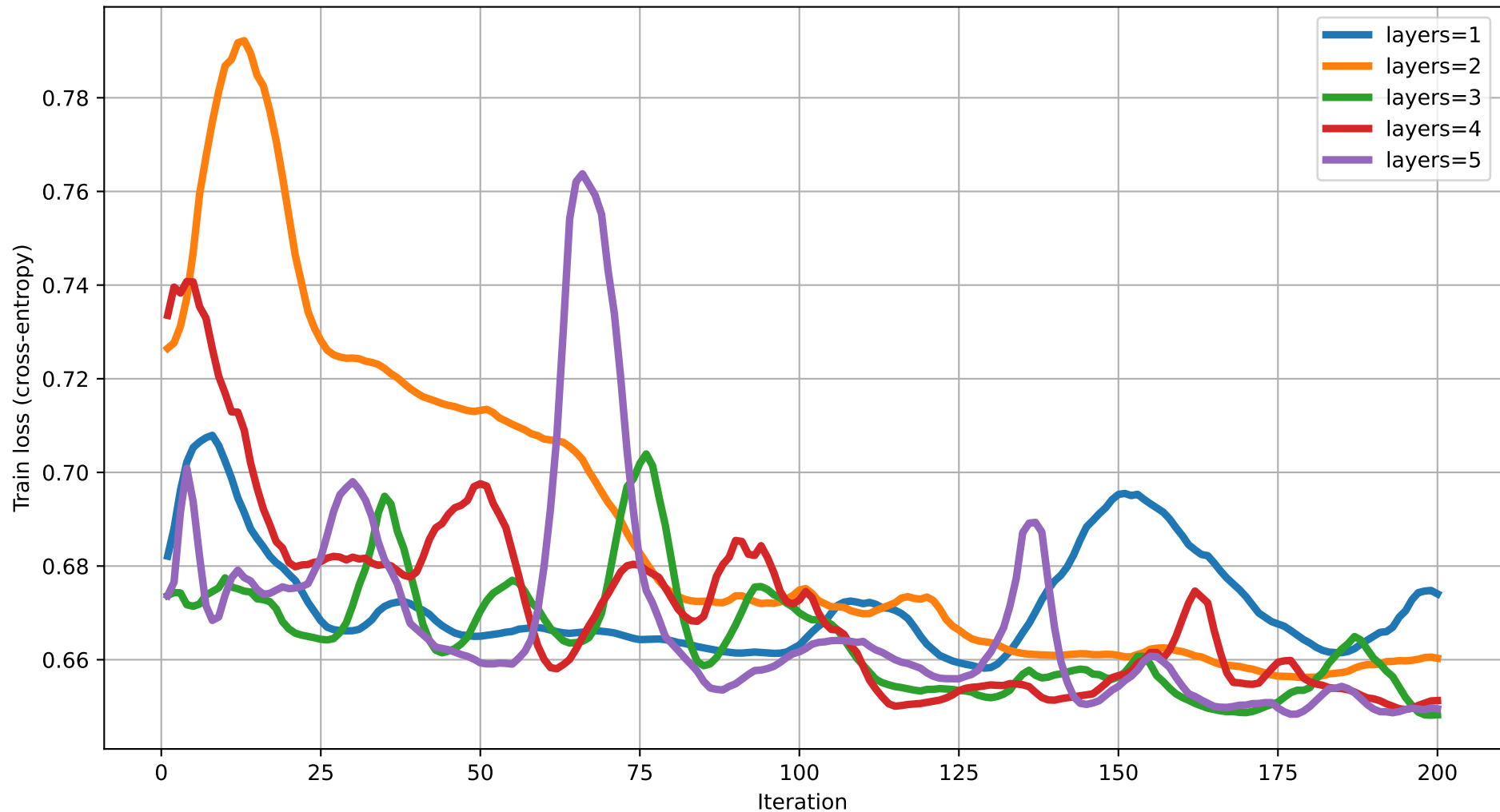
Train loss vs Iteration (dim=7) rot=RY, ent=ring, gate=IsingXX
