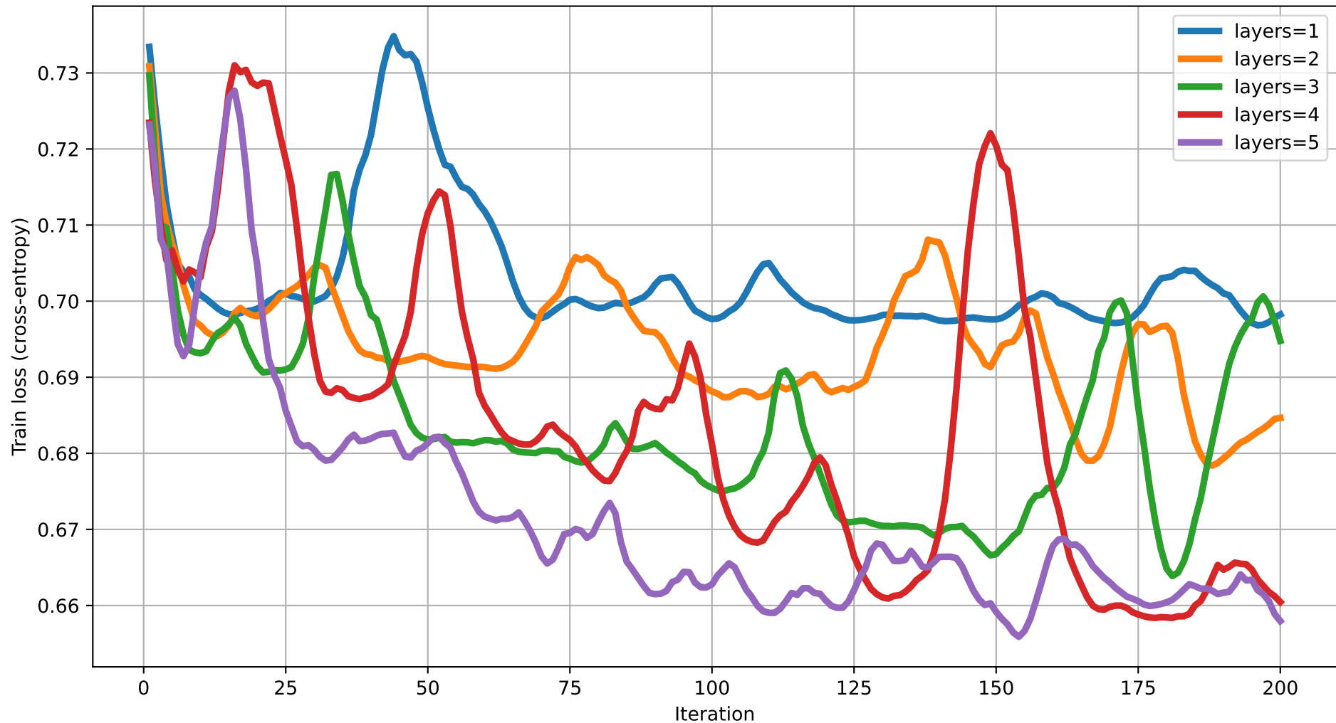
Train loss vs Iteration (dim=19) rot=RY, ent=full, gate=CNOT
