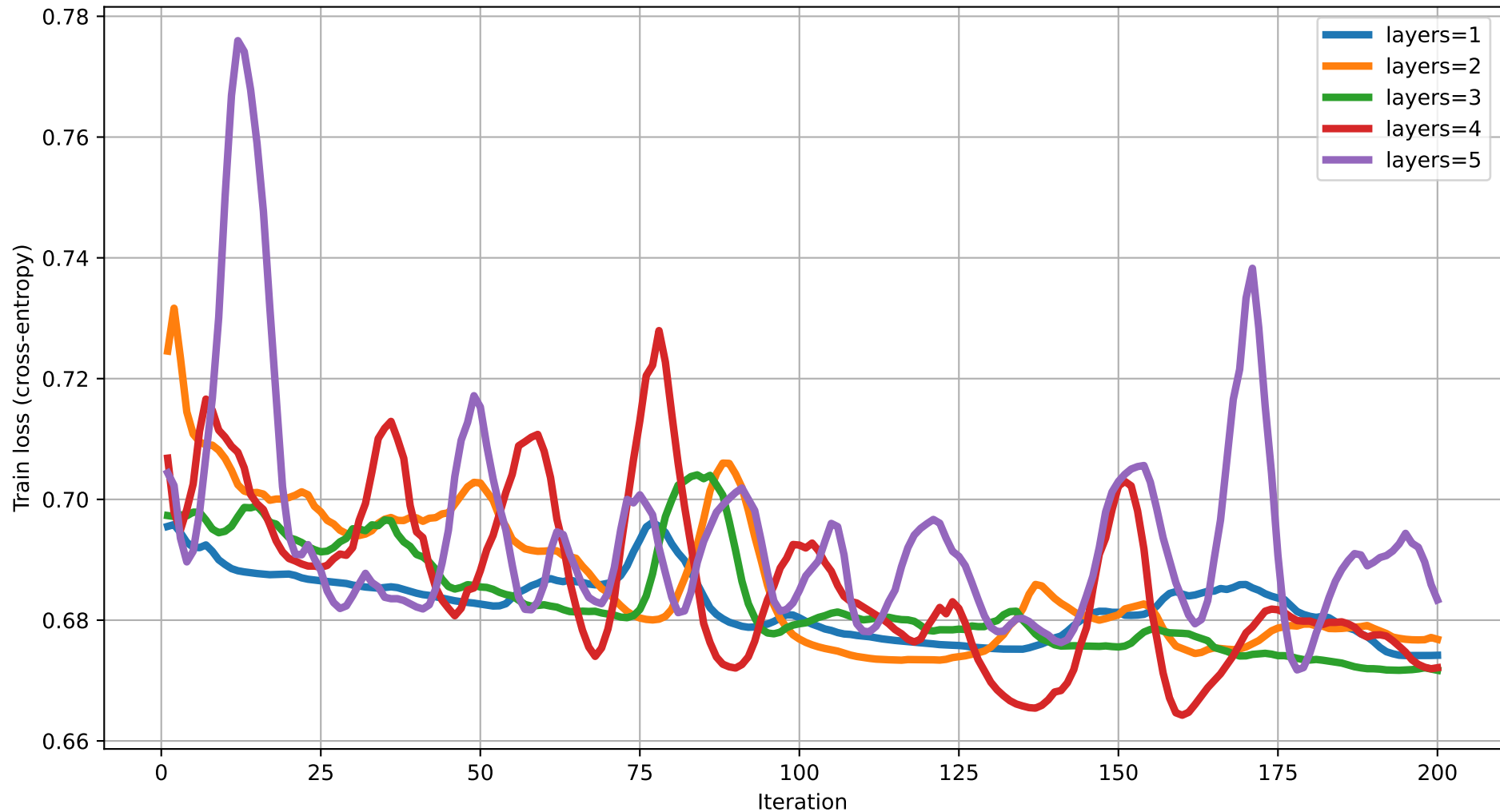
Train loss vs Iteration (dim=12) rot=RYZ, ent=pairwise, gate=IsingXX
