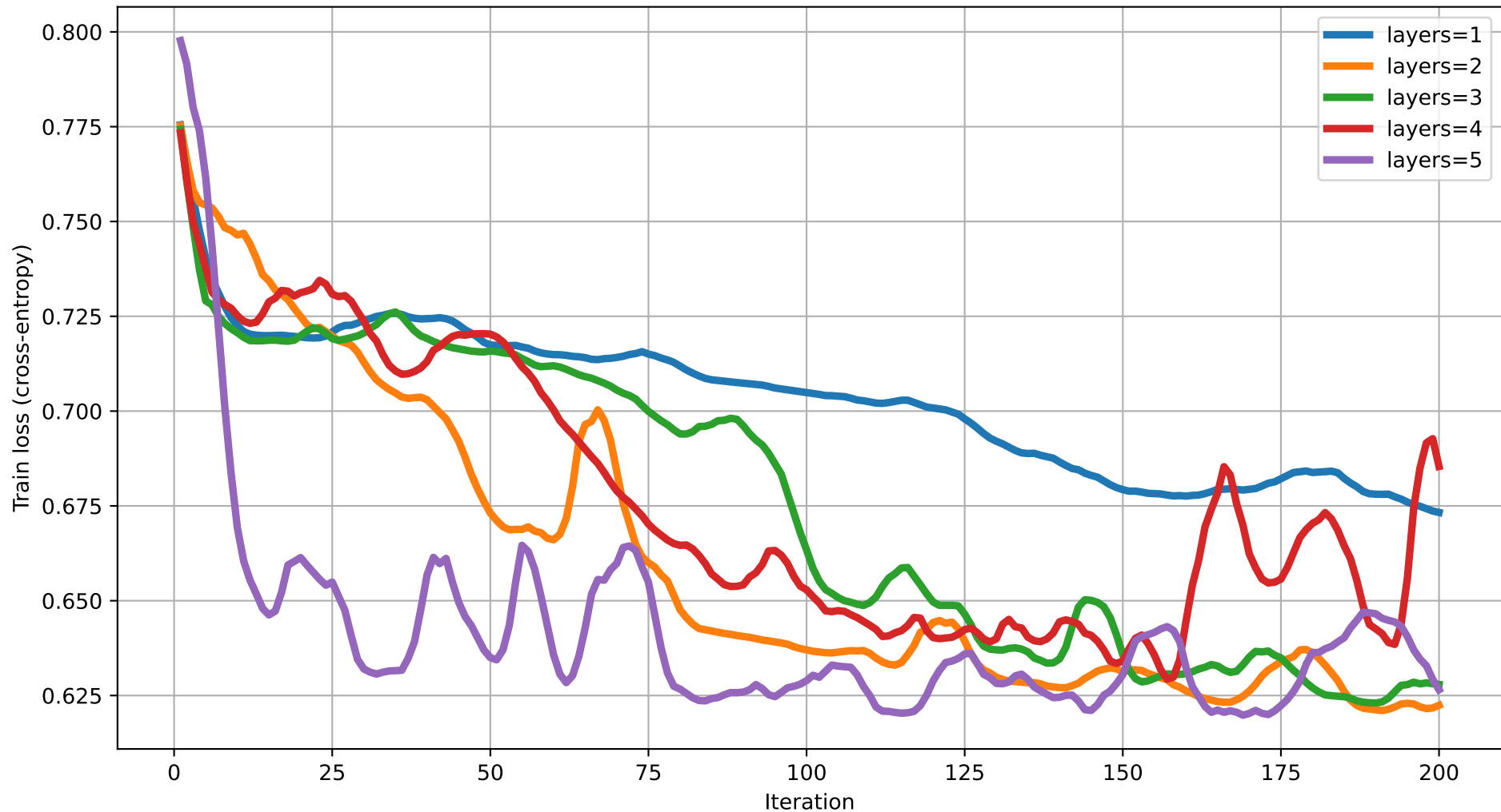
Train loss vs Iteration (dim=4) rot=Rot, ent=chain, gate=CZ
