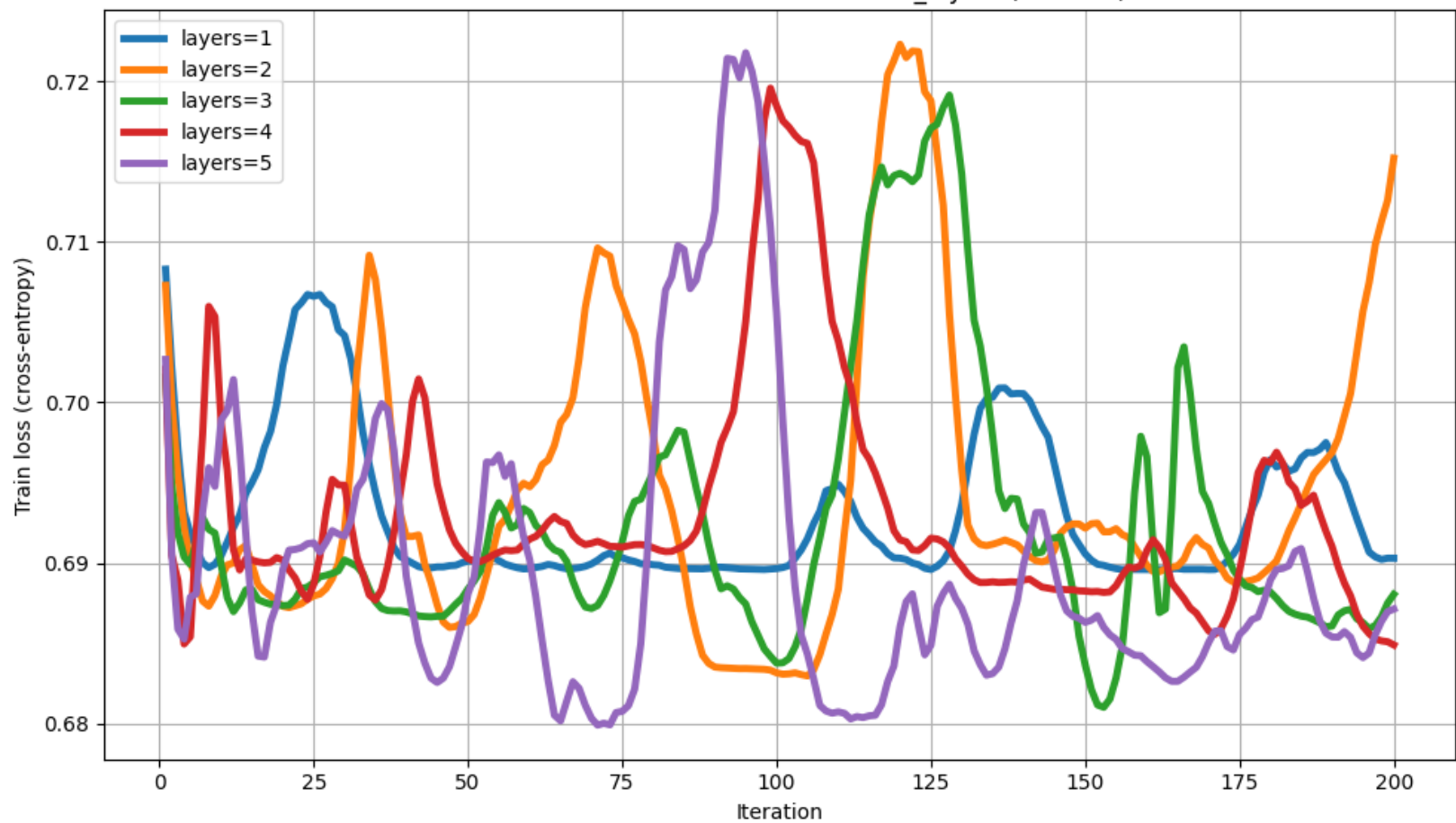
Train loss vs Iteration for different num_layers (dim=20)
