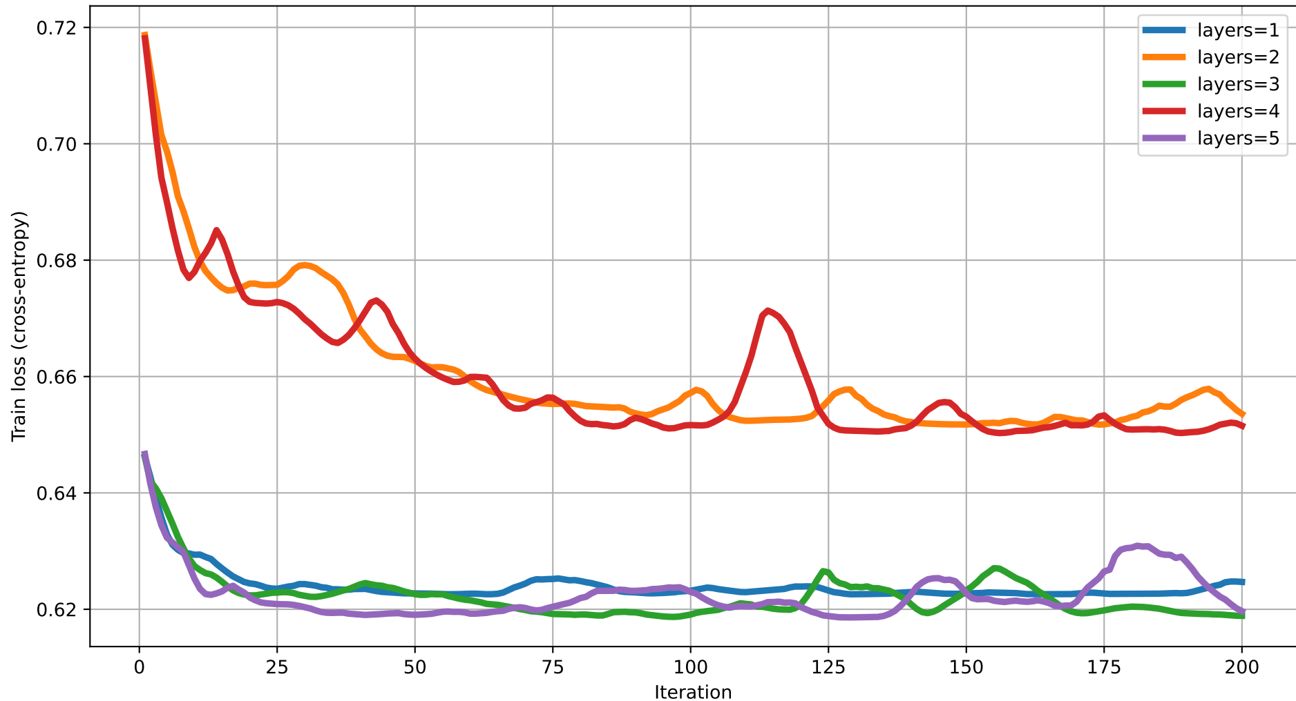
Train loss vs Iteration (degree=4) rot=RZ, ent=ring, gate=IsingXX
