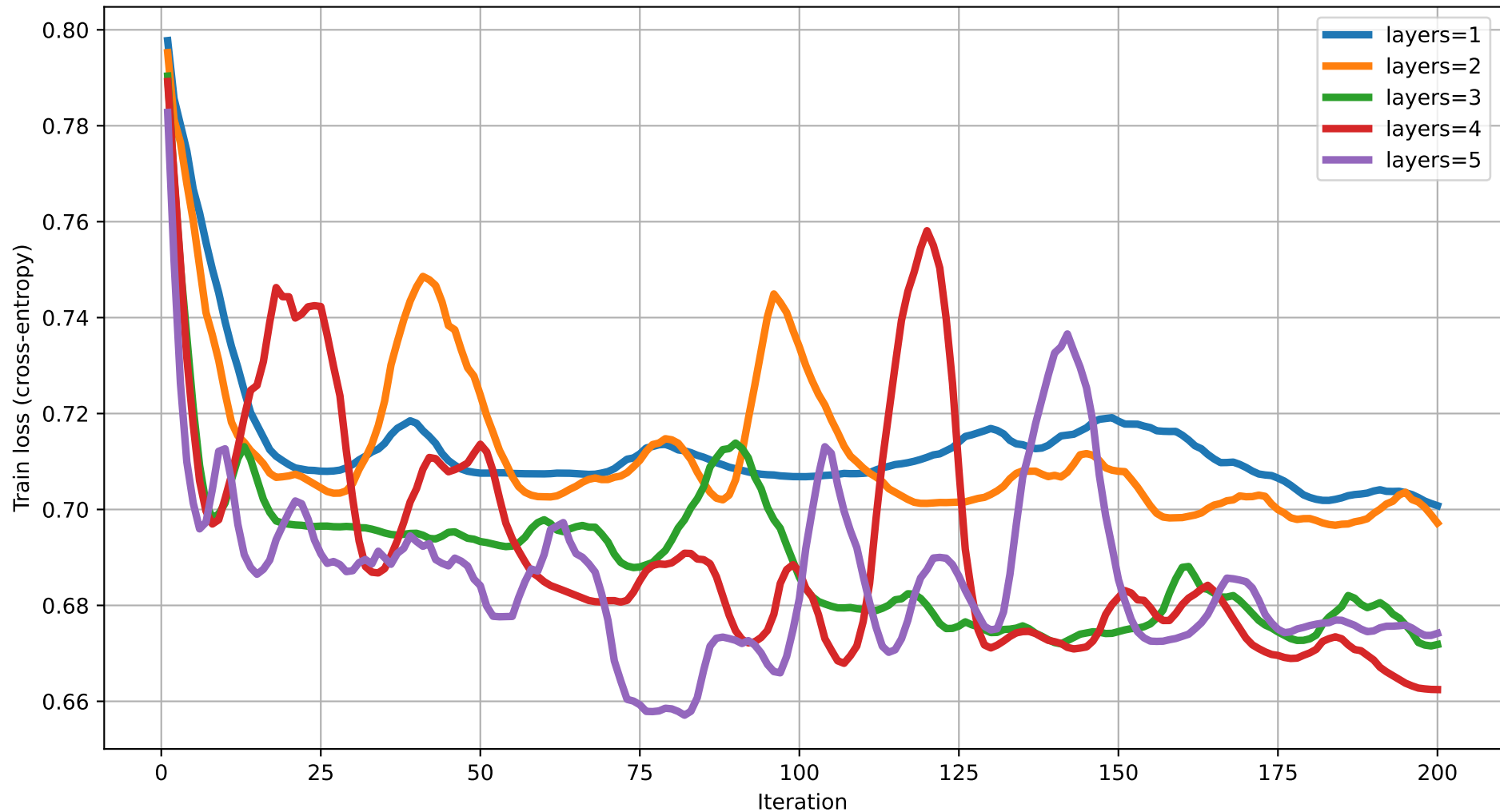
Train loss vs Iteration (dim=8) rot=RYZ, ent=full, gate=CNOT
