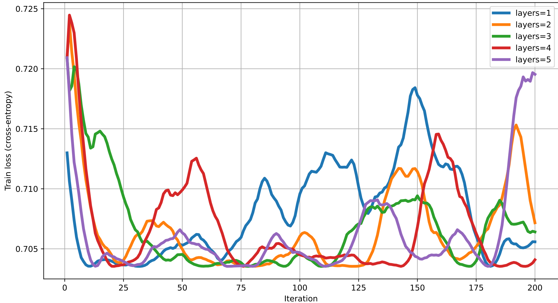
Train loss vs Iteration (dim=11) rot=RZ, ent=chain, gate=CZ
