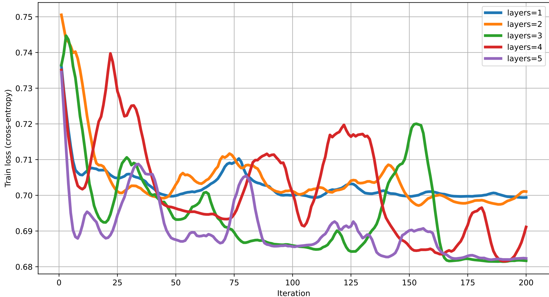
Train loss vs Iteration (dim=19) rot=RX, ent=ring, gate=CZ
