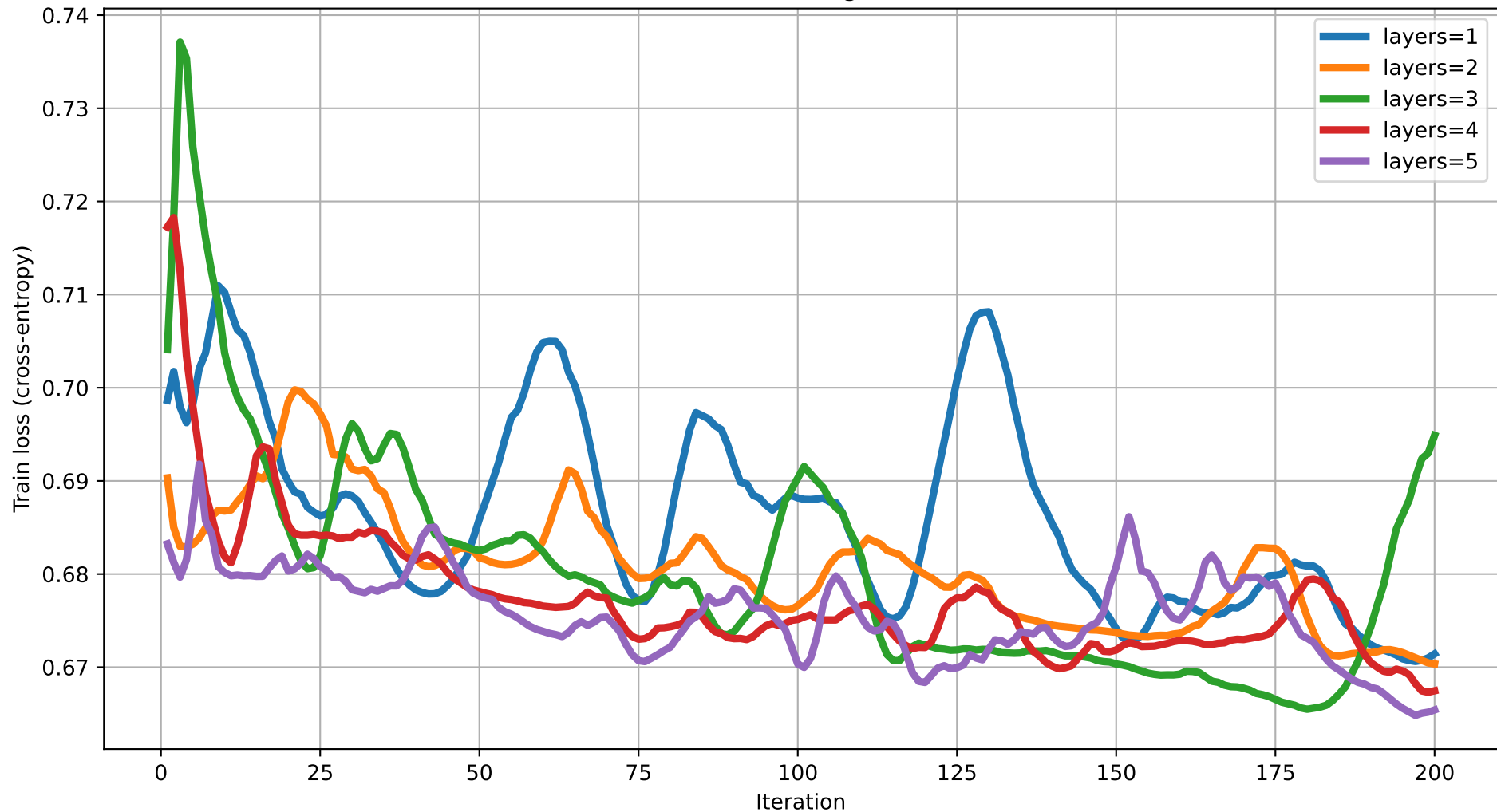
Train loss vs Iteration (dim=13) rot=Rot, ent=full, gate=CNOT
