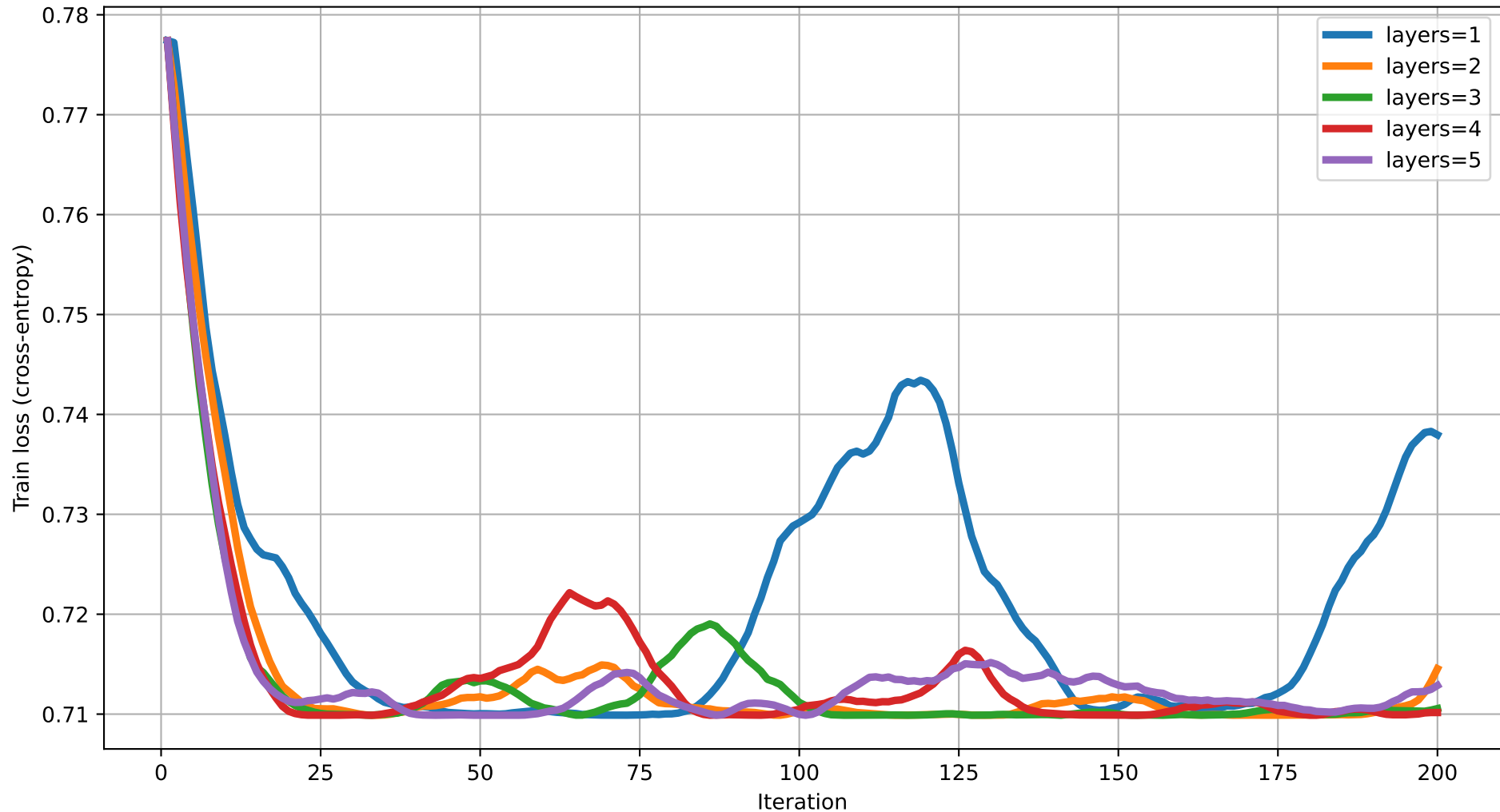
Train loss vs Iteration (dim=4) rot=RZ, ent=pairwise, gate=CNOT
