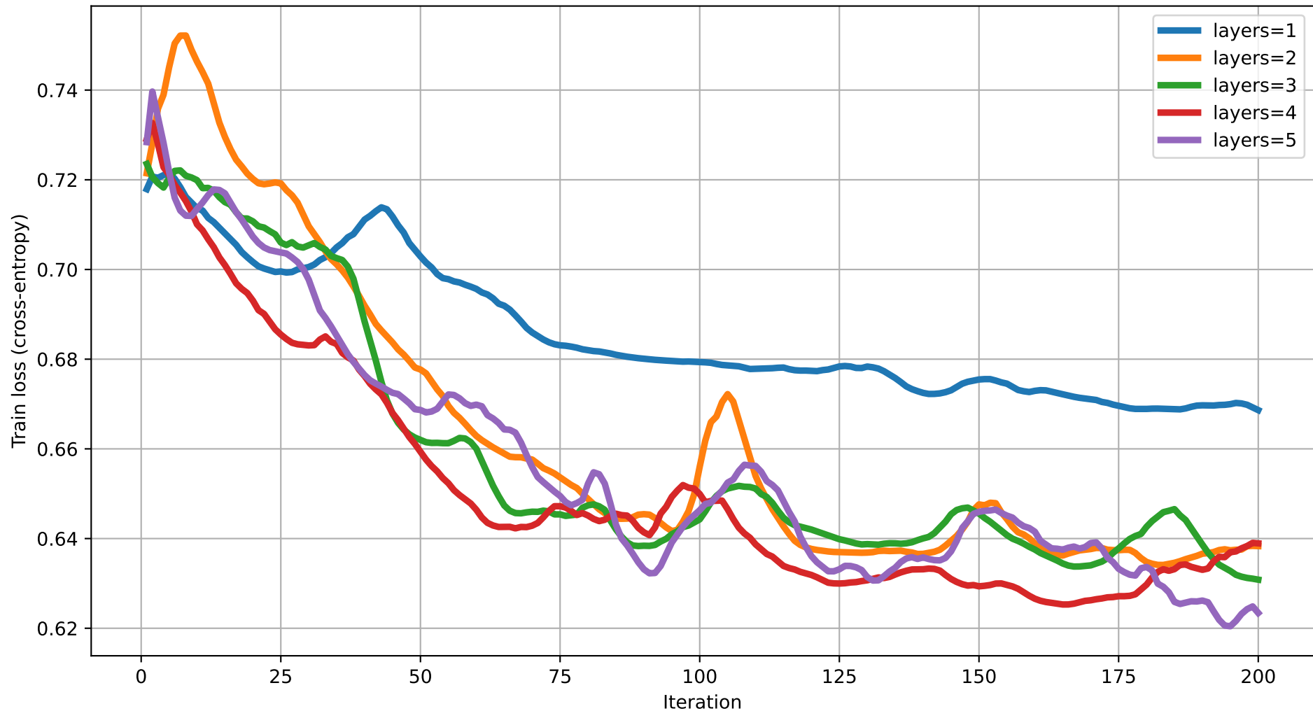
Train loss vs Iteration (dim=7) rot=RYZ, ent=chain, gate=CNOT
