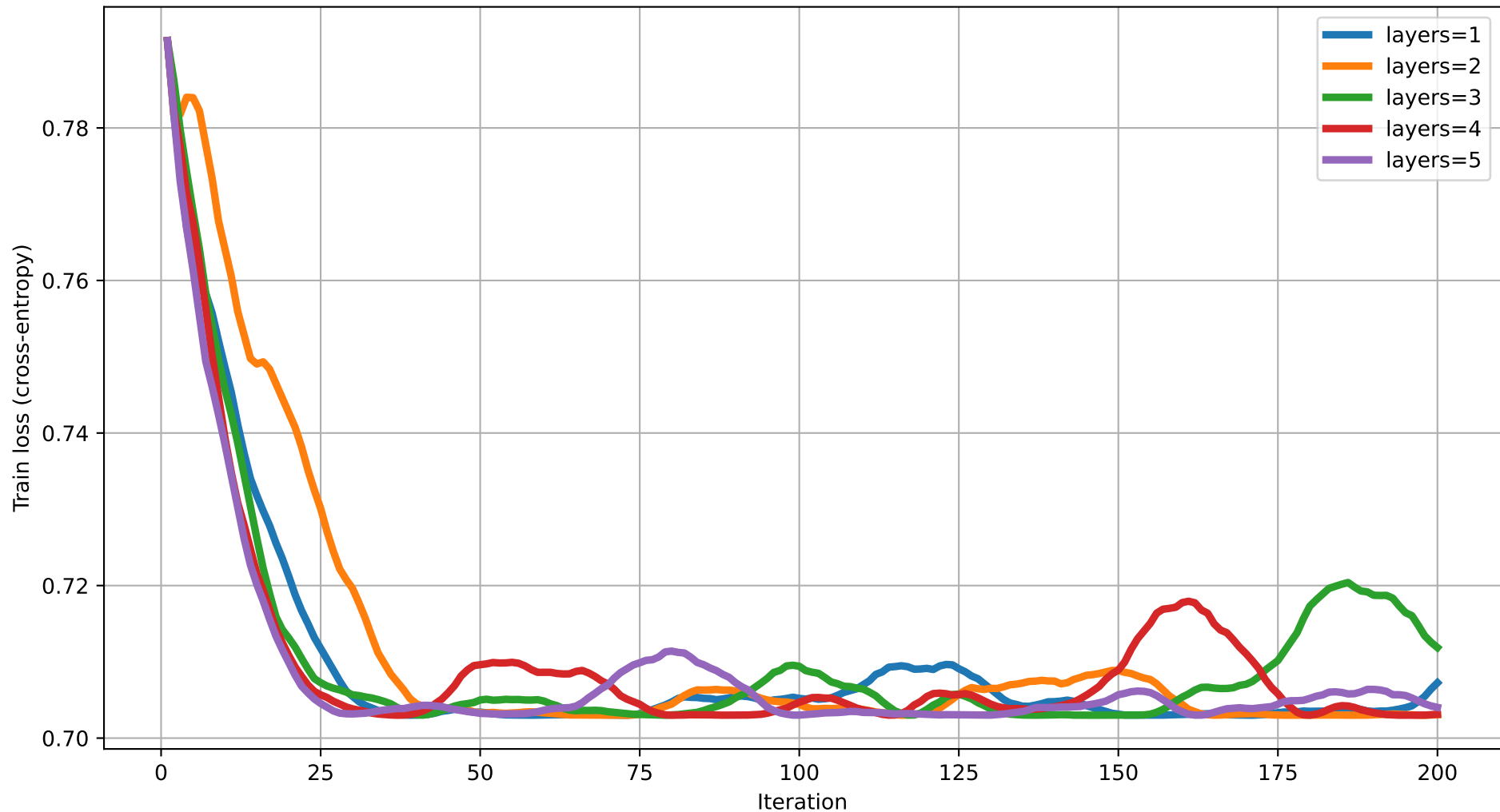
Train loss vs Iteration (dim=2) rot=RZ, ent=pairwise, gate=CNOT
