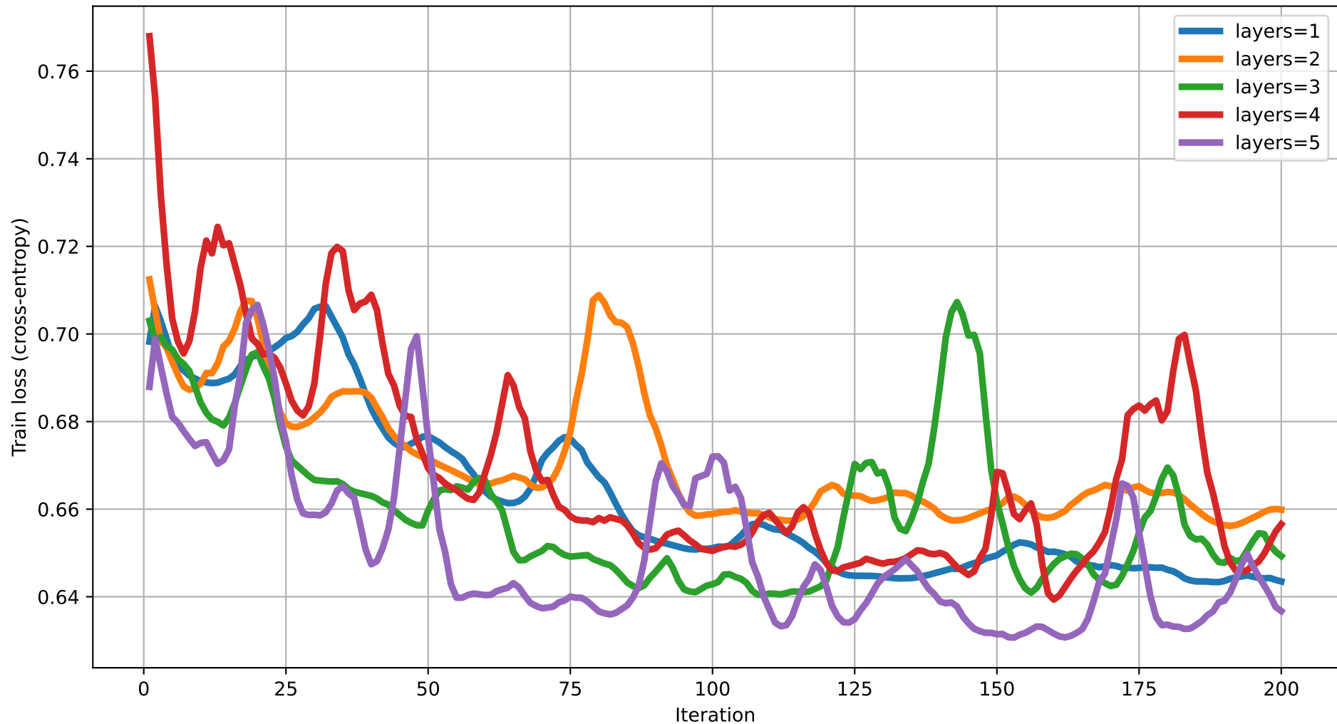
Train loss vs Iteration (dim=5) rot=Rot, ent=chain, gate=IsingXX
