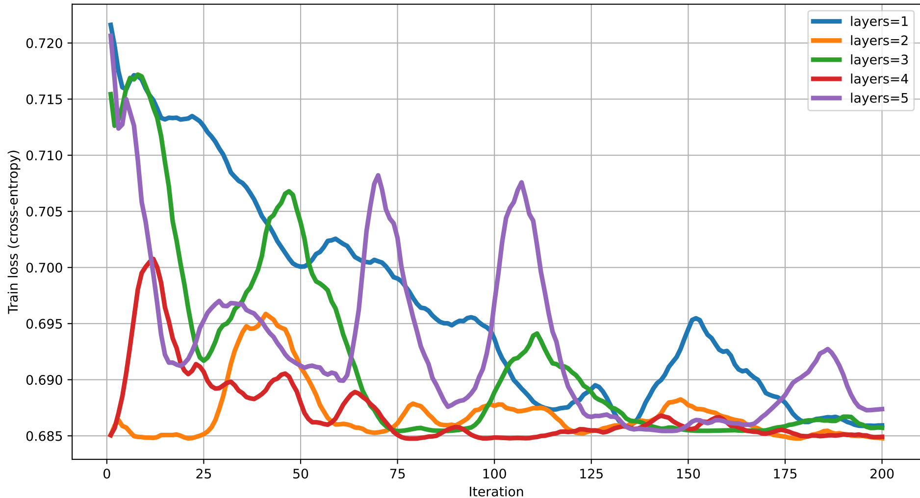
Train loss vs Iteration (dim=15) rot=RX, ent=ring, gate=IsingXX
