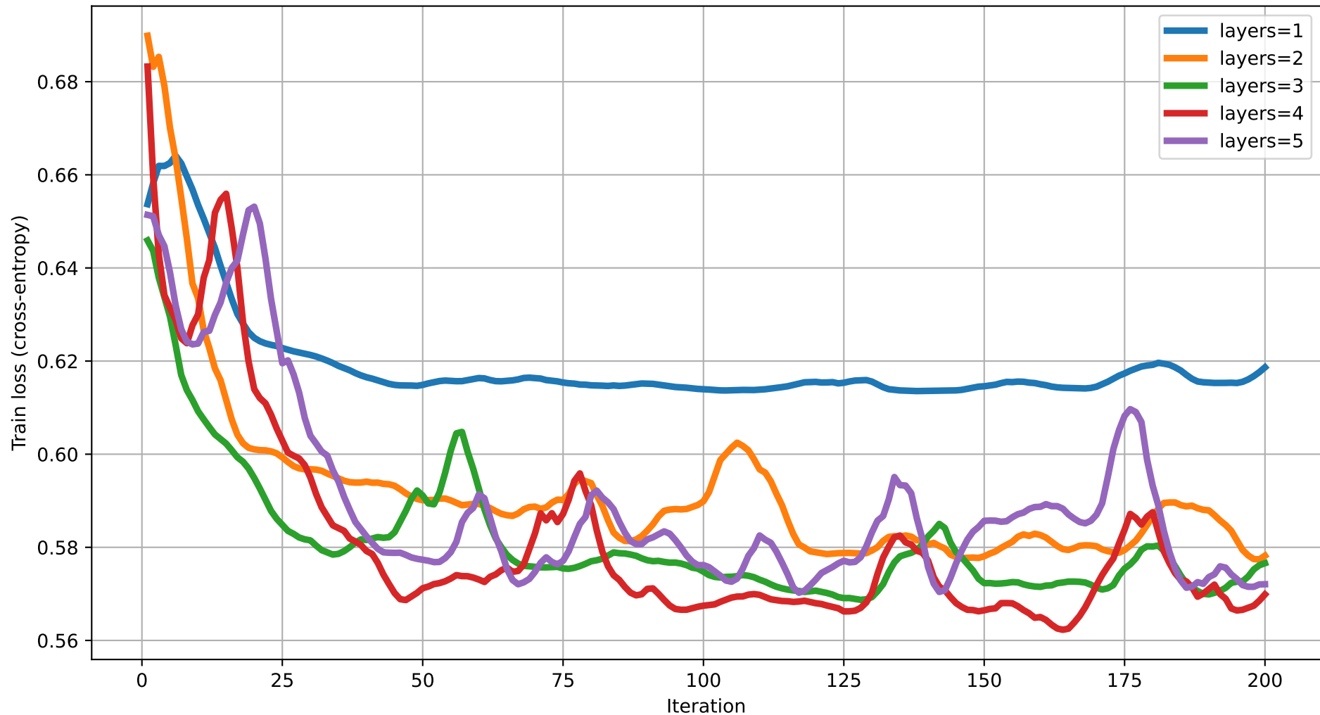
Train loss vs Iteration (dim=10) rot=RYZ, ent=ring, gate=IsingXX
