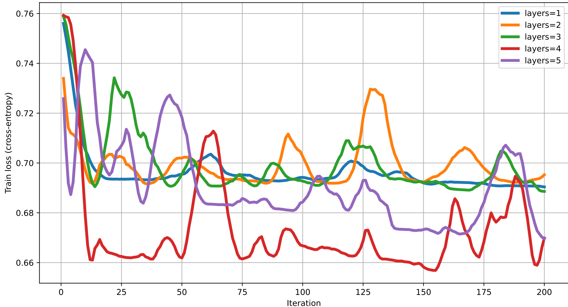
Train loss vs Iteration (dim=16) rot=RY, ent=full, gate=CNOT
