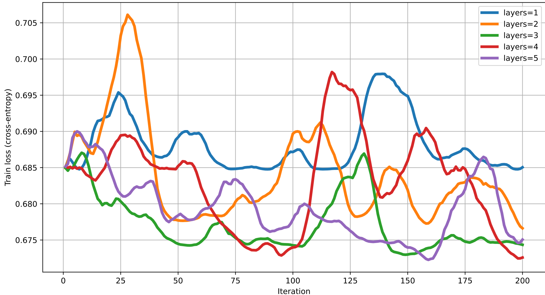
Train loss vs Iteration (dim=15) rot=RX, ent=ring, gate=CZ
