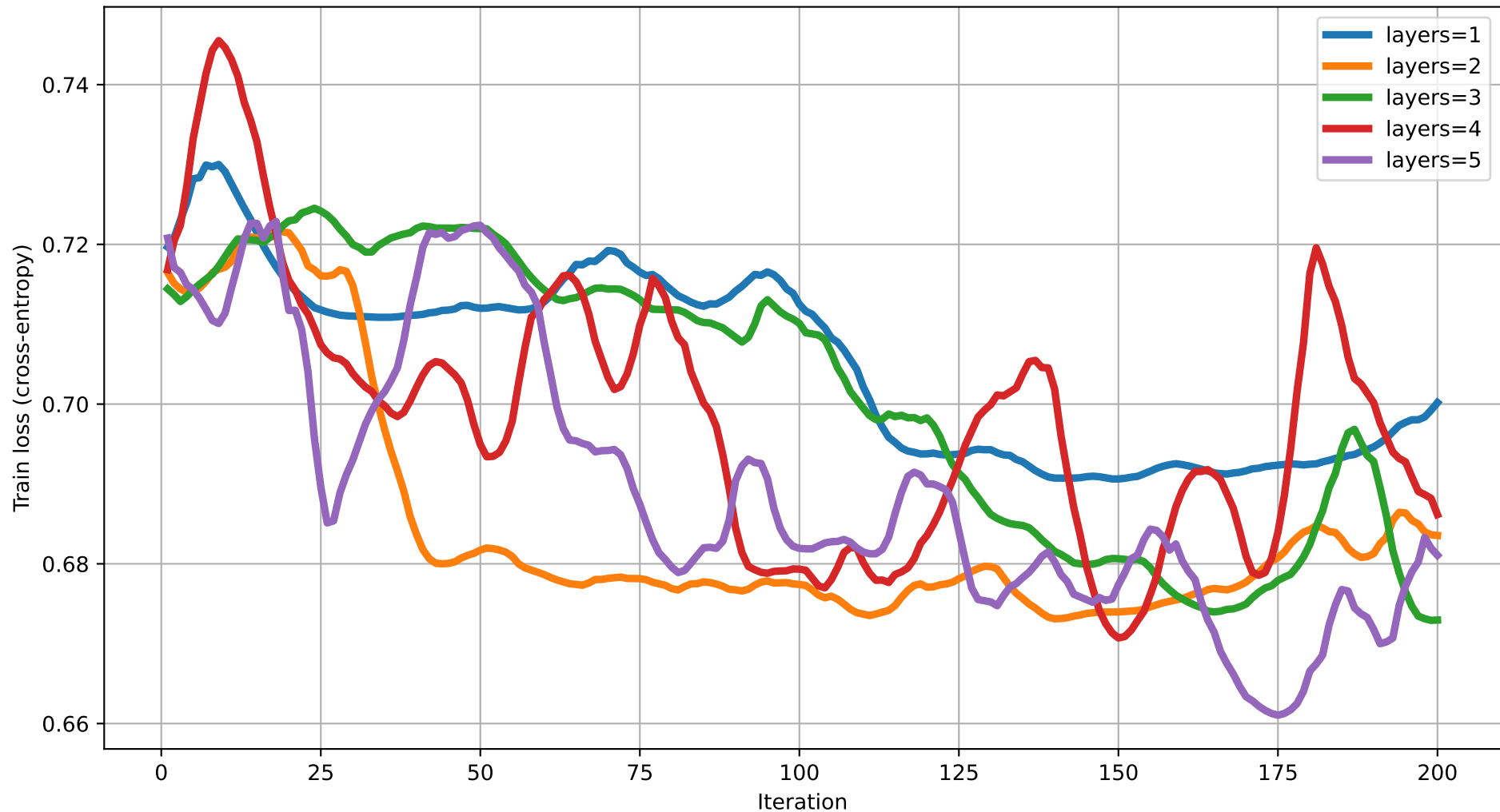
Train loss vs Iteration (dim=3) rot=Rot, ent=full, gate=CZ
