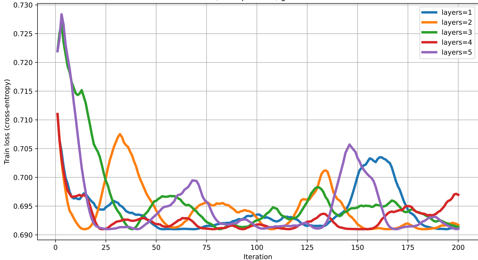
Train loss vs Iteration (dim=20) rot=RZ, ent=pairwise, gate=CNOT
