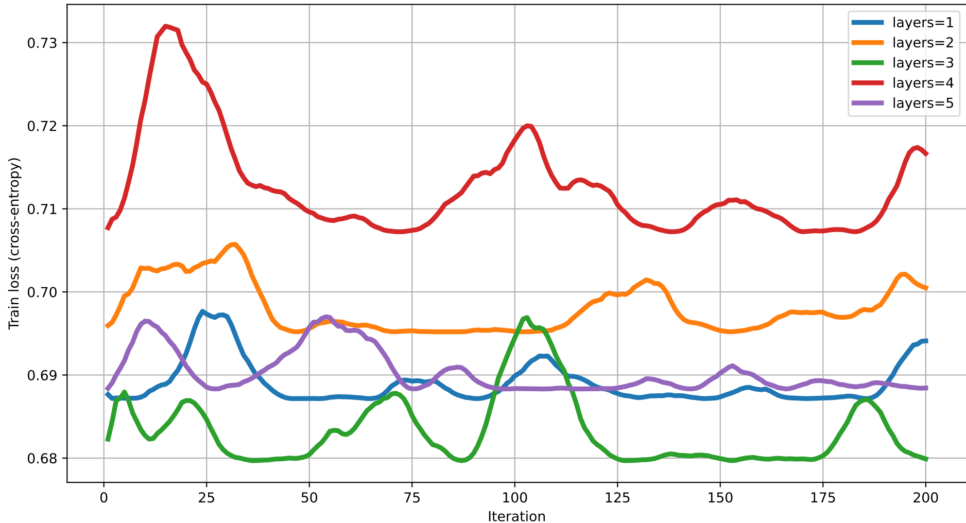
Train loss vs Iteration (dim=19) rot=RZ, ent=ring, gate=CNOT
