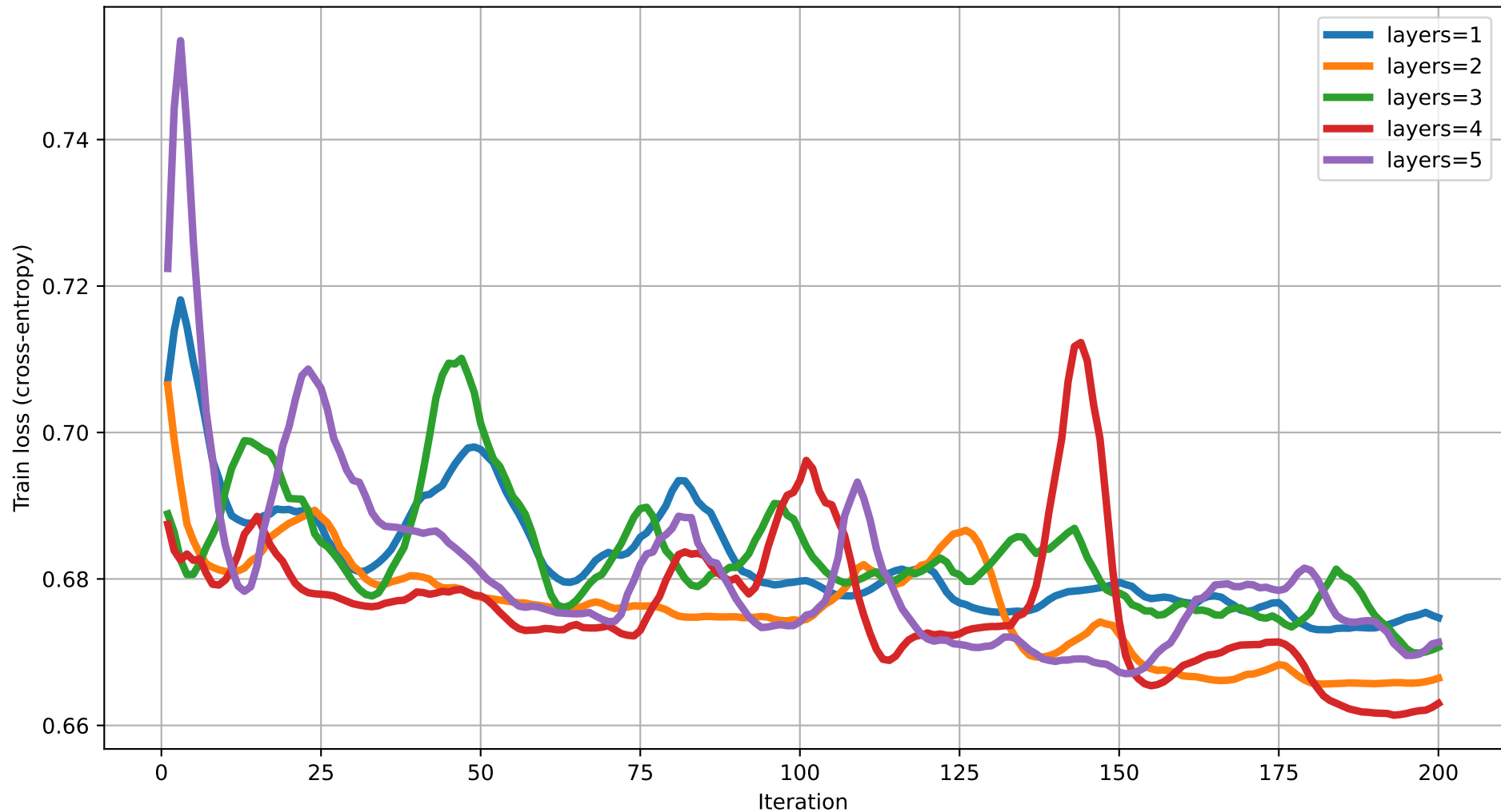
Train loss vs Iteration (dim=13) rot=RY, ent=pairwise, gate=CZ
