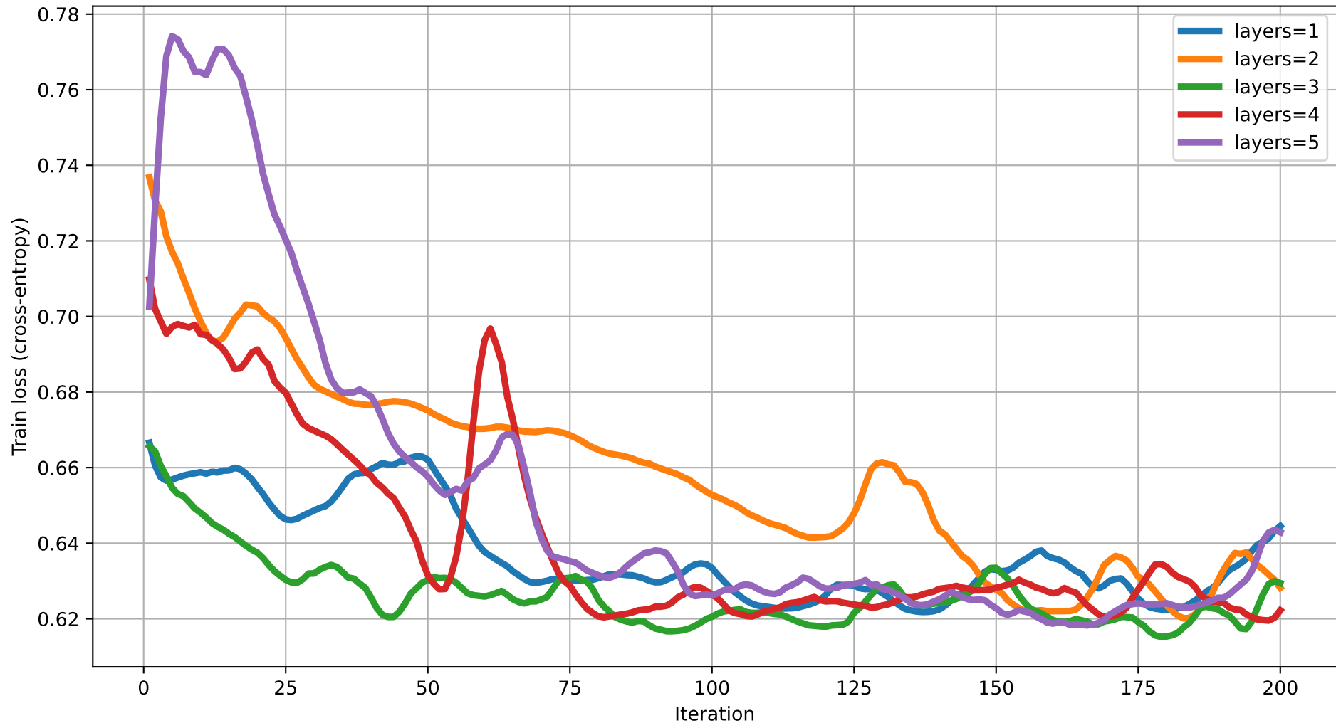
Train loss vs Iteration (dim=6) rot=RY, ent=full, gate=IsingXX
