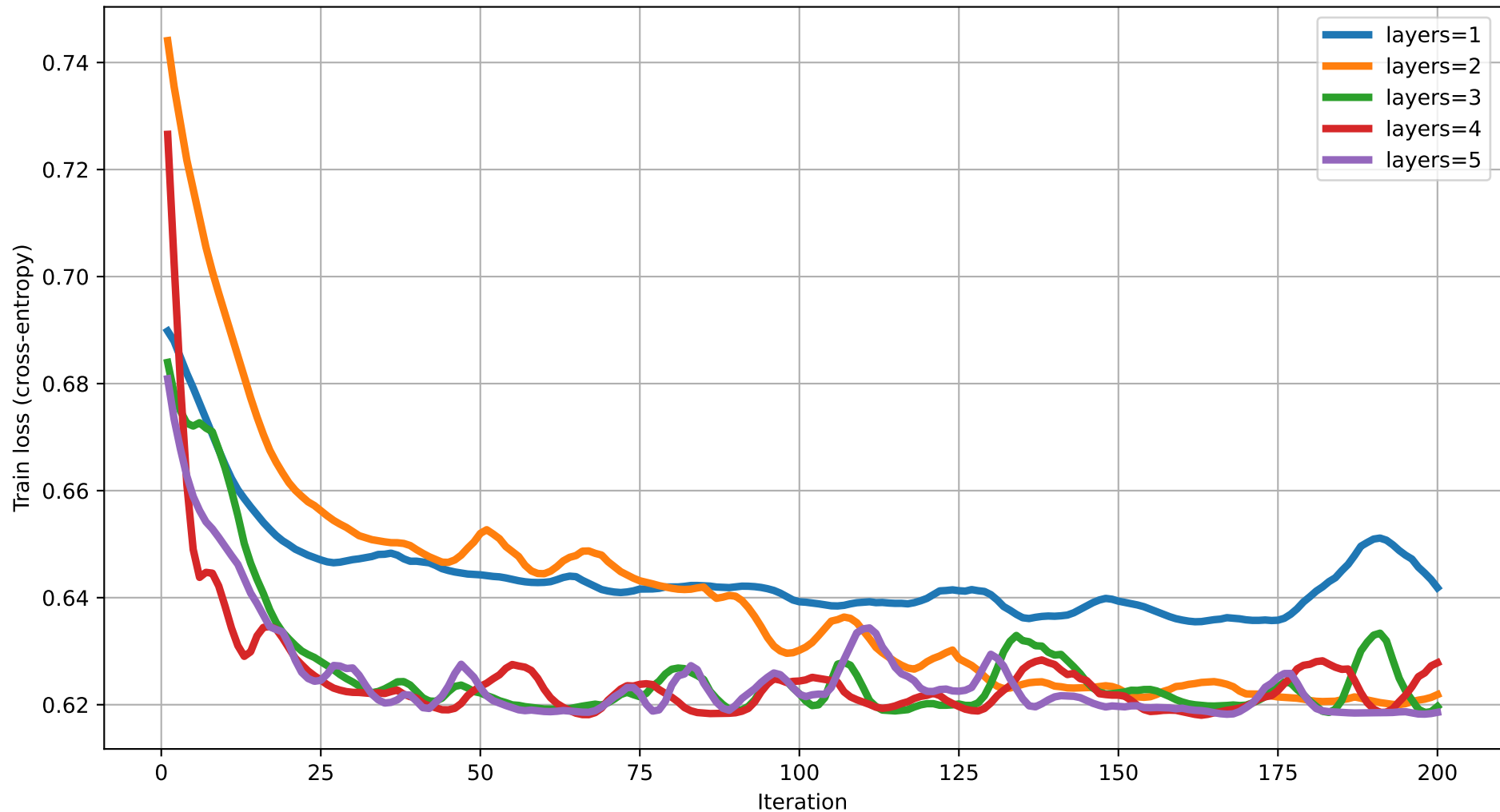
Train loss vs Iteration (degree=5) rot=RYZ, ent=pairwise, gate=IsingXX
