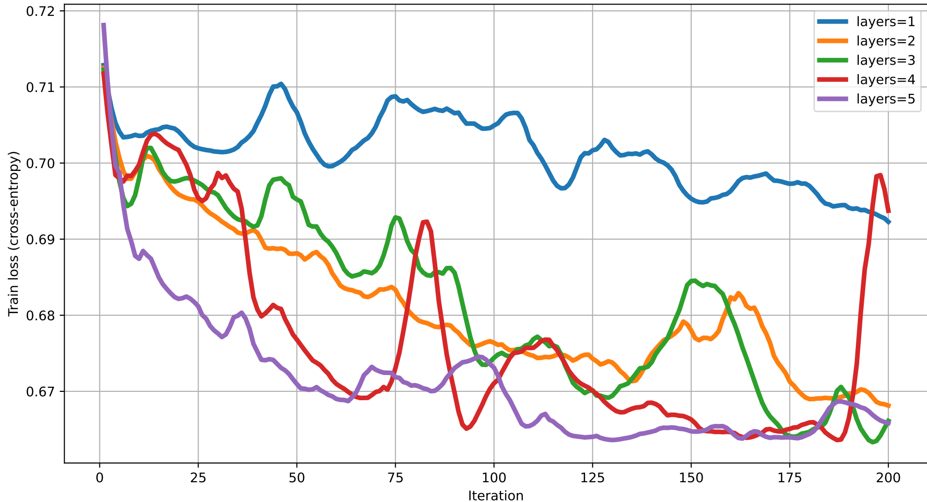
Train loss vs Iteration (dim=11) rot=RX, ent=full, gate=CNOT
