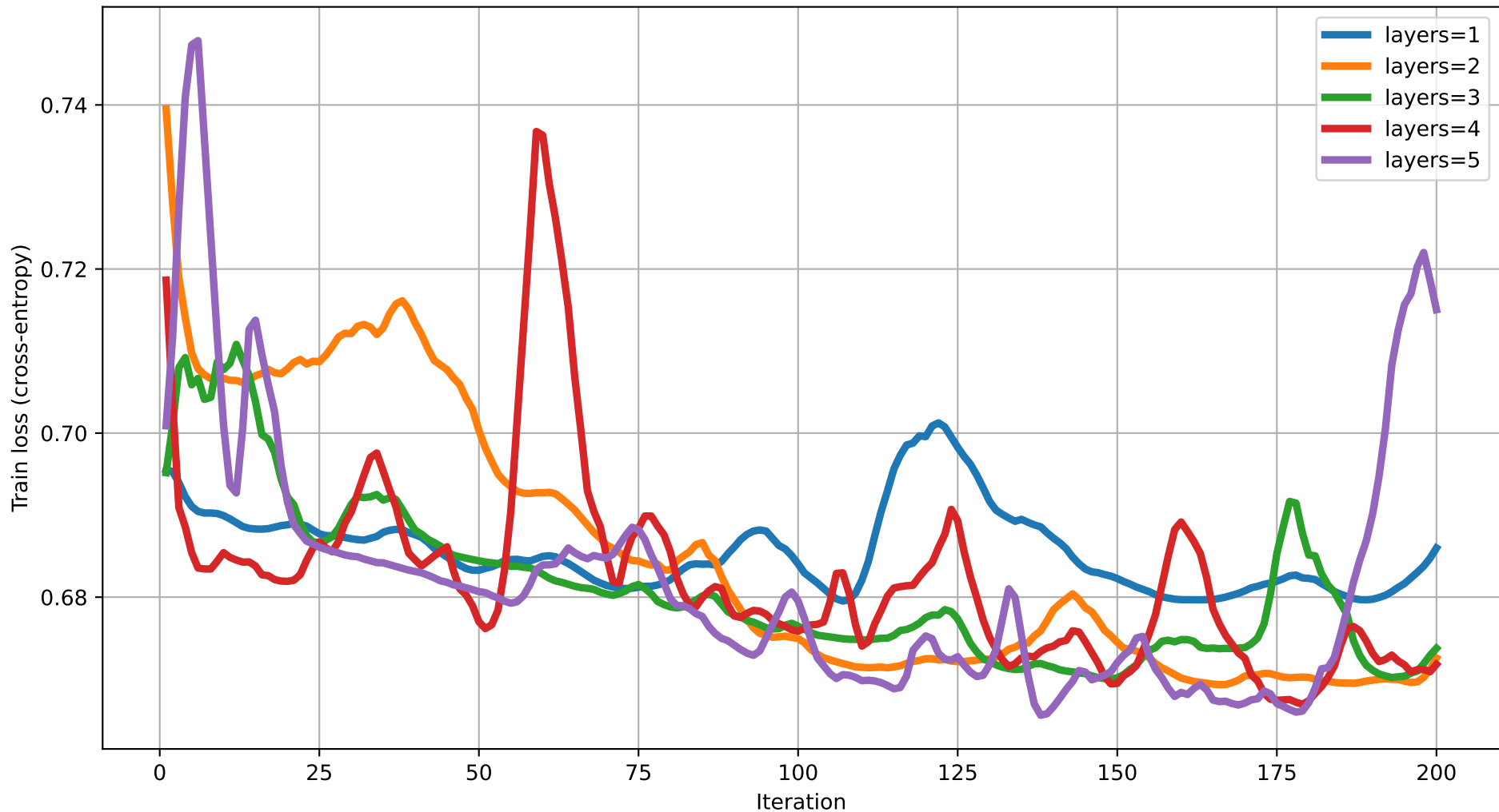
Train loss vs Iteration (dim=20) rot=RYZ, ent=chain, gate=IsingXX
