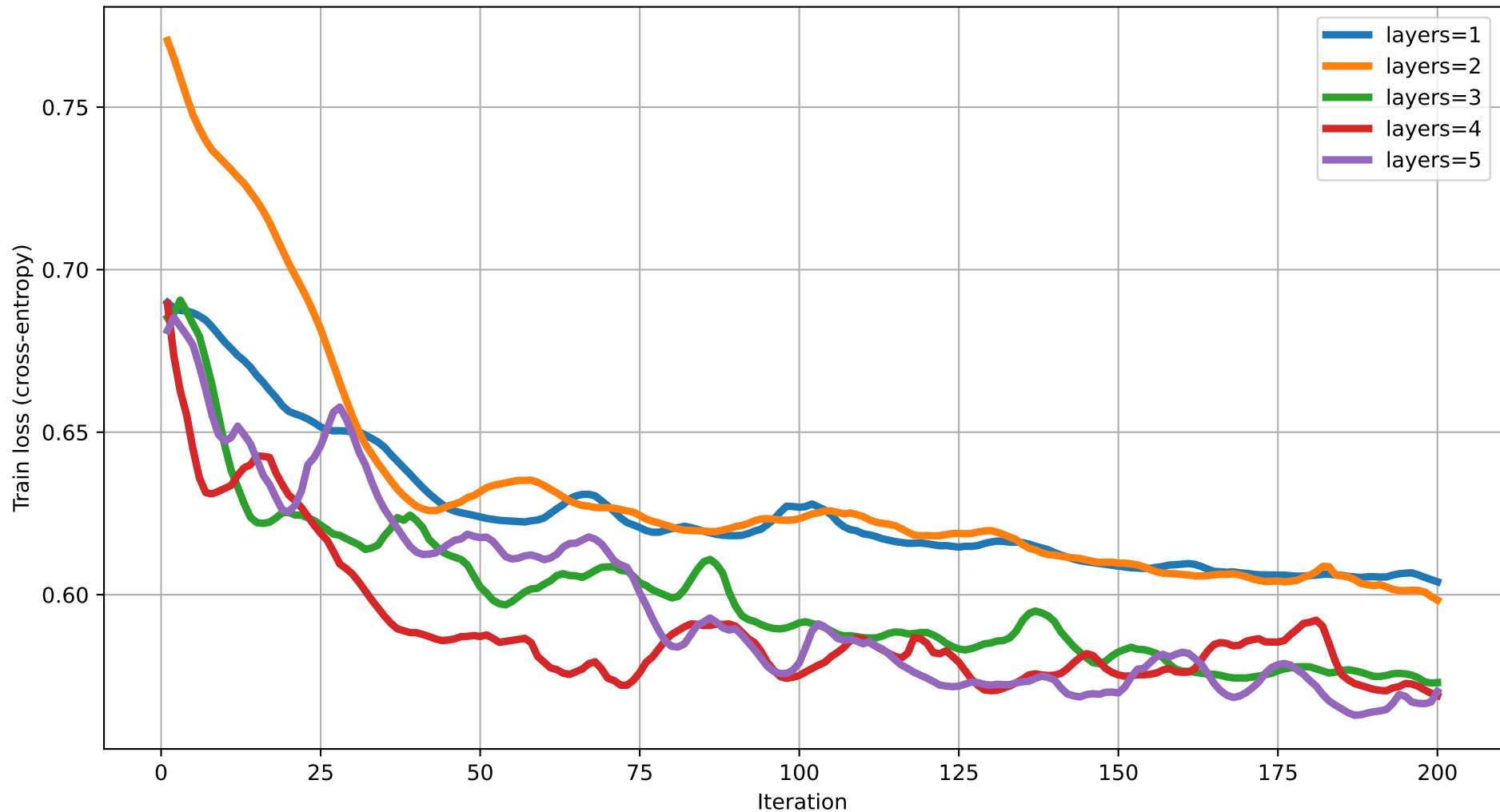
Train loss vs Iteration (dim=10) rot=RYZ, ent=full, gate=IsingXX
