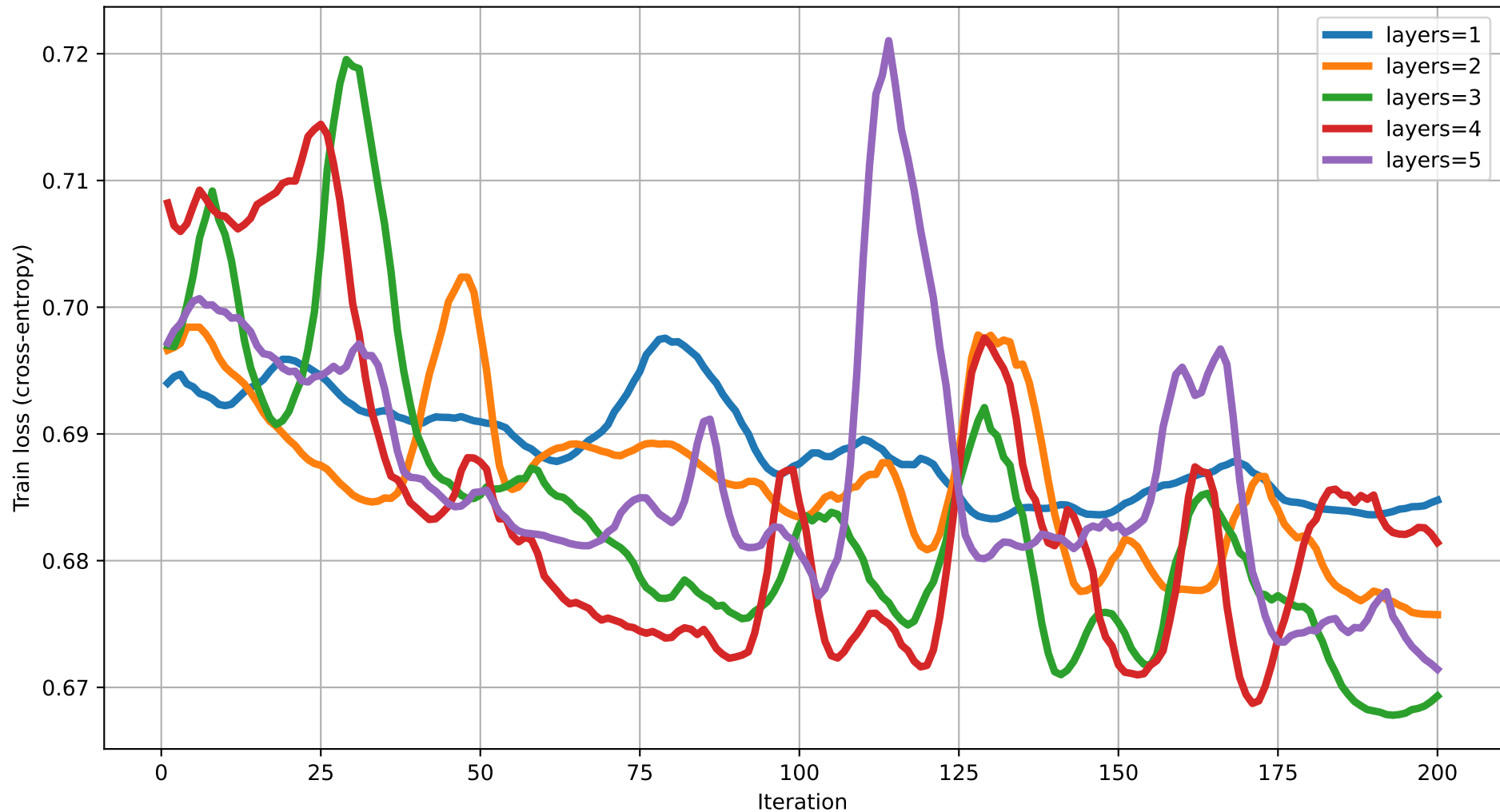
Train loss vs Iteration (dim=20) rot=RYZ, ent=ring, gate=CNOT
