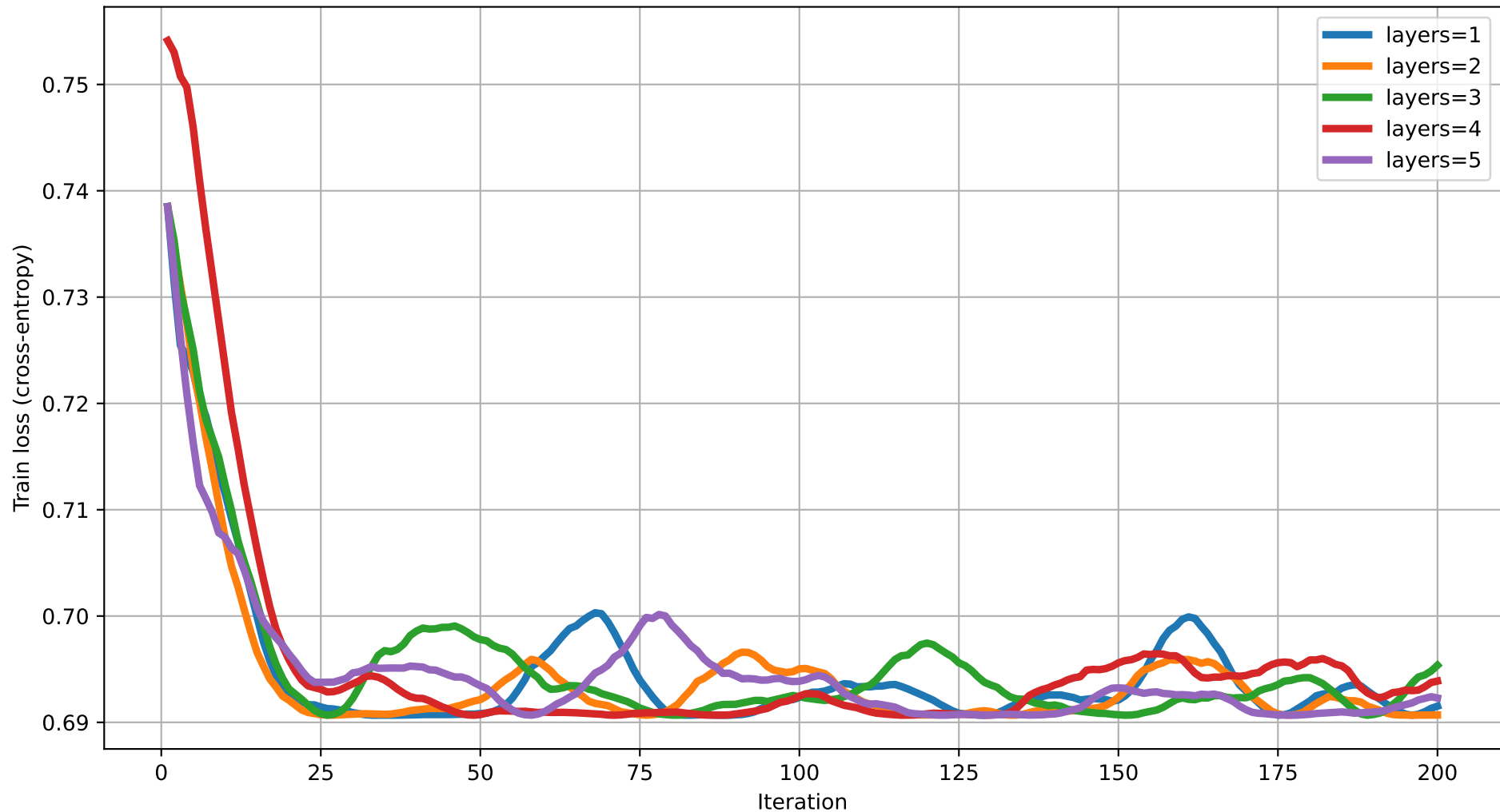
Train loss vs Iteration (dim=16) rot=RZ, ent=pairwise, gate=CNOT
