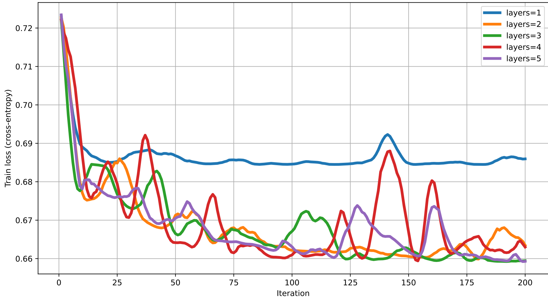
Train loss vs Iteration (degree=3) rot=RX, ent=pairwise, gate=CZ
