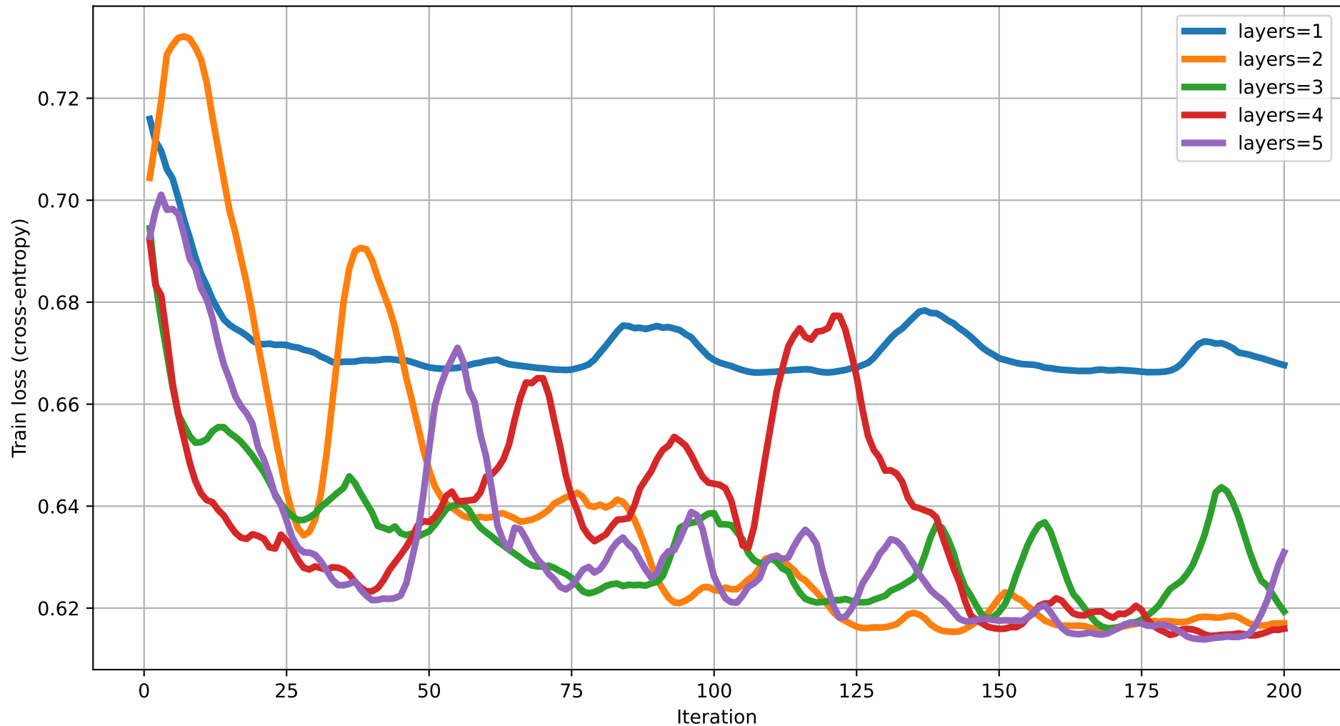
Train loss vs Iteration (dim=10) rot=Rot, ent=pairwise, gate=CZ
