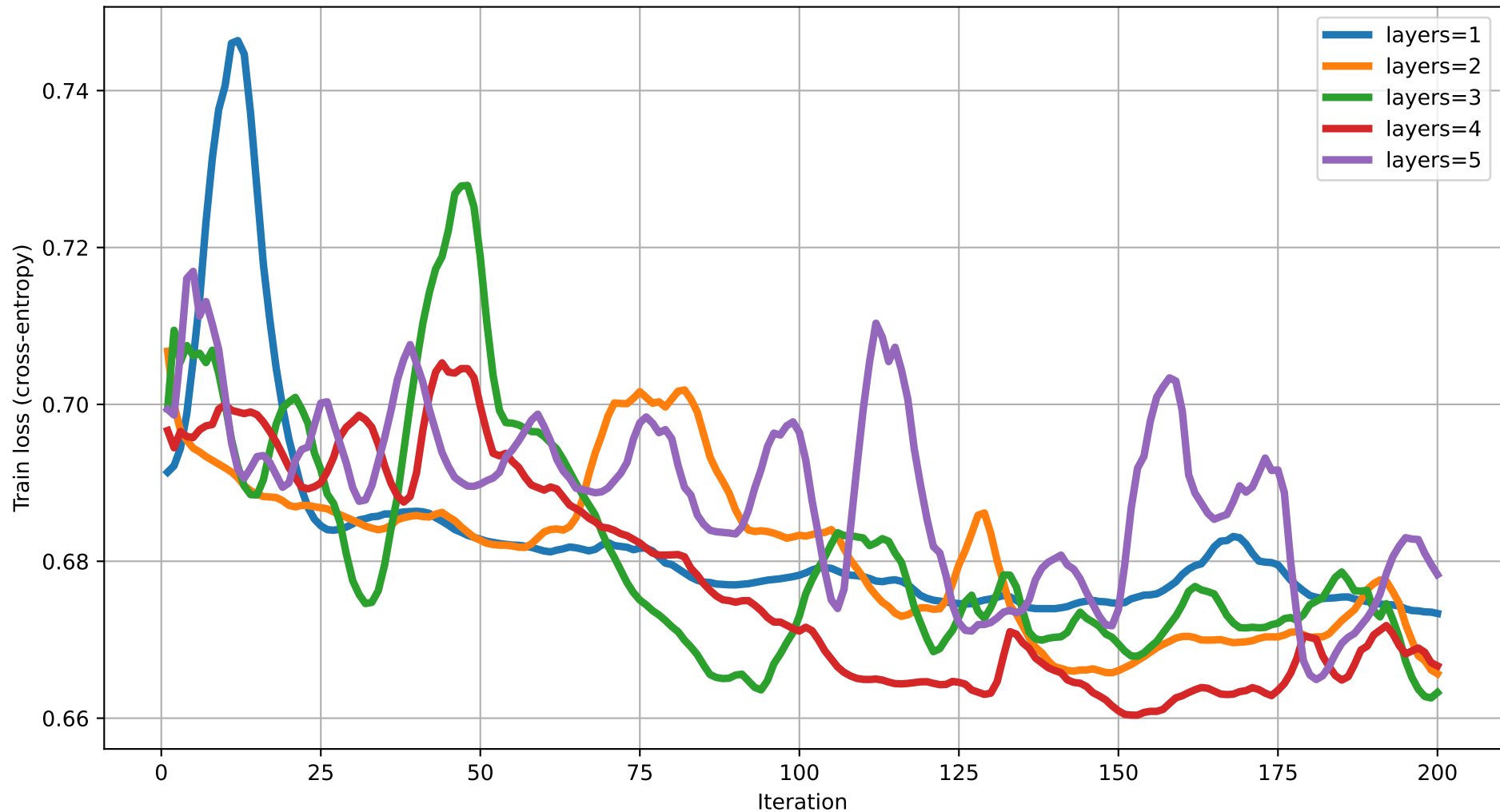
Train loss vs Iteration (dim=12) rot=RYZ, ent=full, gate=IsingXX
