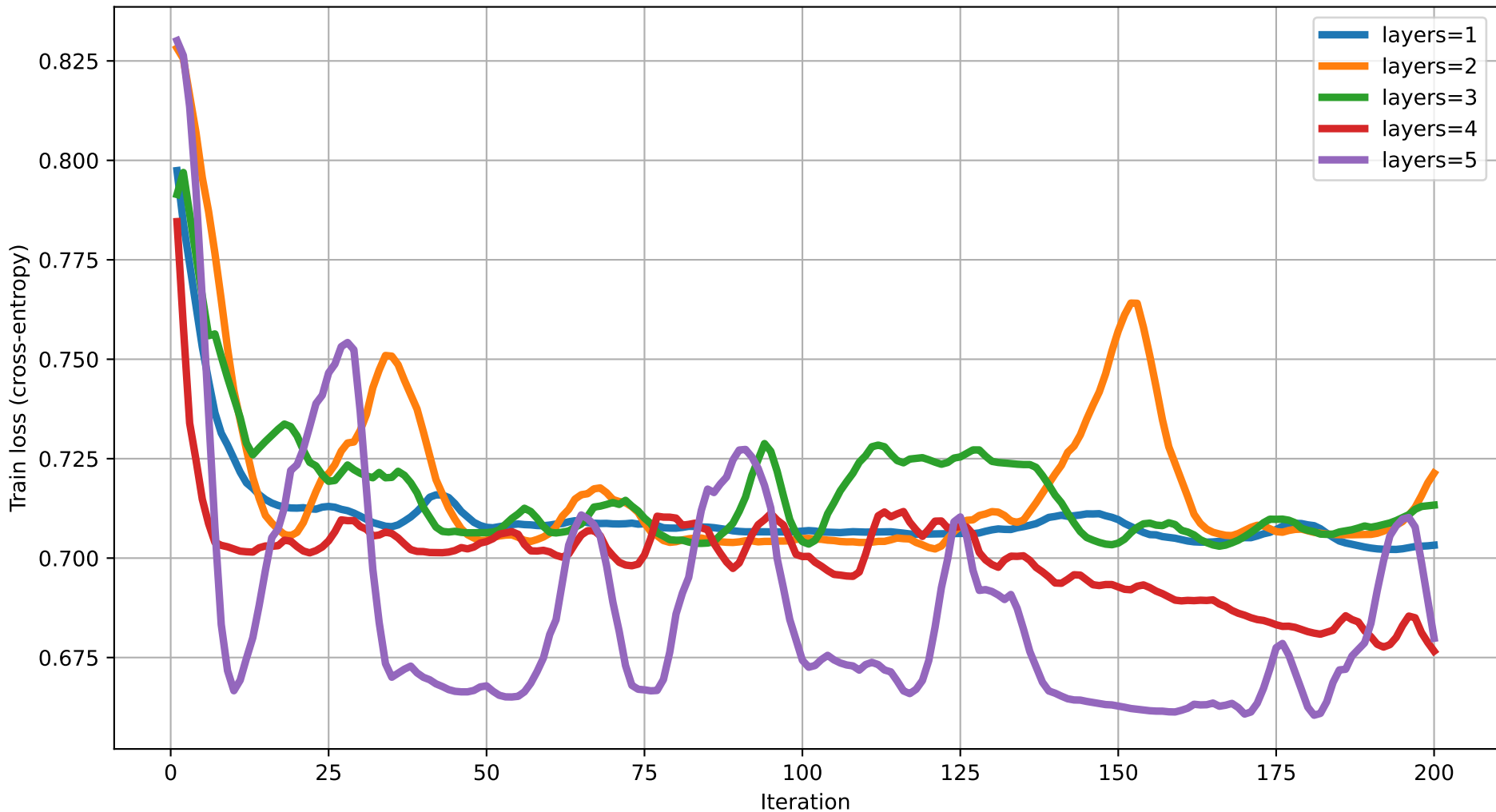
Train loss vs Iteration (dim=8) rot=RYZ, ent=pairwise, gate=CNOT
