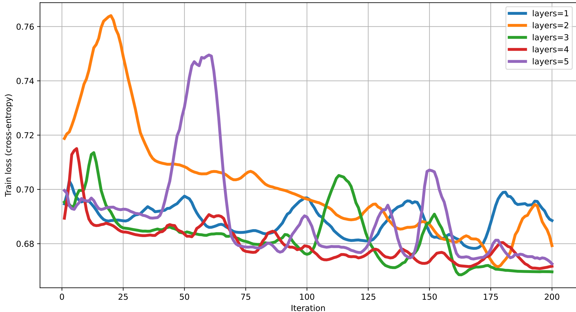
Train loss vs Iteration (dim=15) rot=RZ, ent=pairwise, gate=IsingXX
