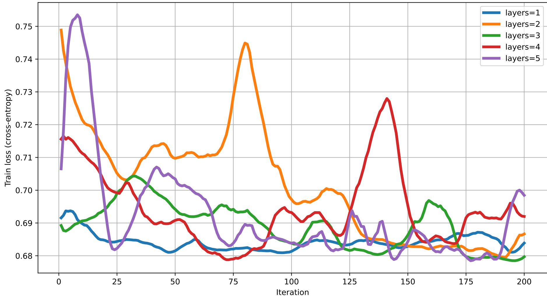
Train loss vs Iteration (dim=3) rot=RZ, ent=chain, gate=IsingXX
