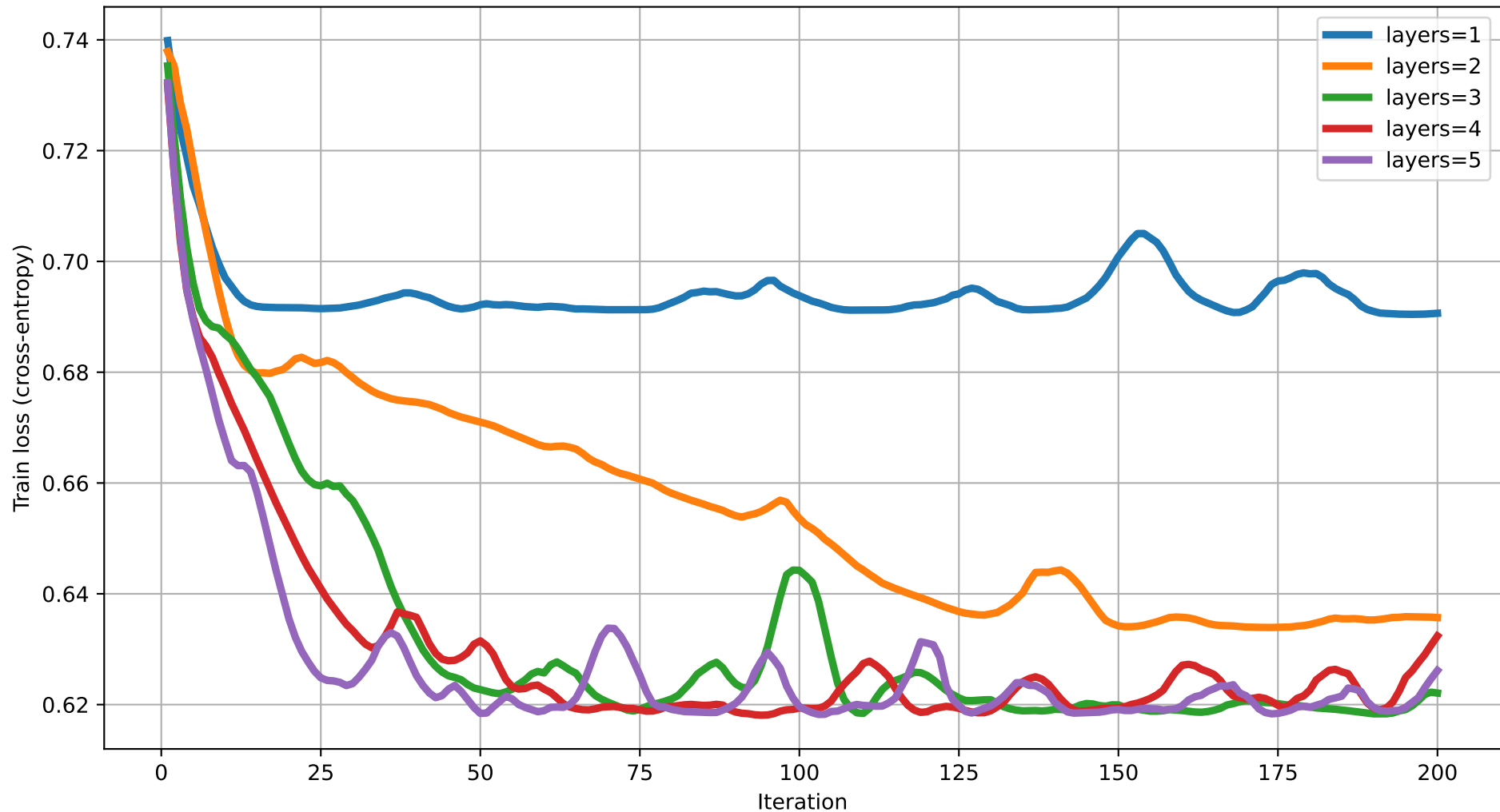
Train loss vs Iteration (degree=5) rot=RY, ent=pairwise, gate=CZ
