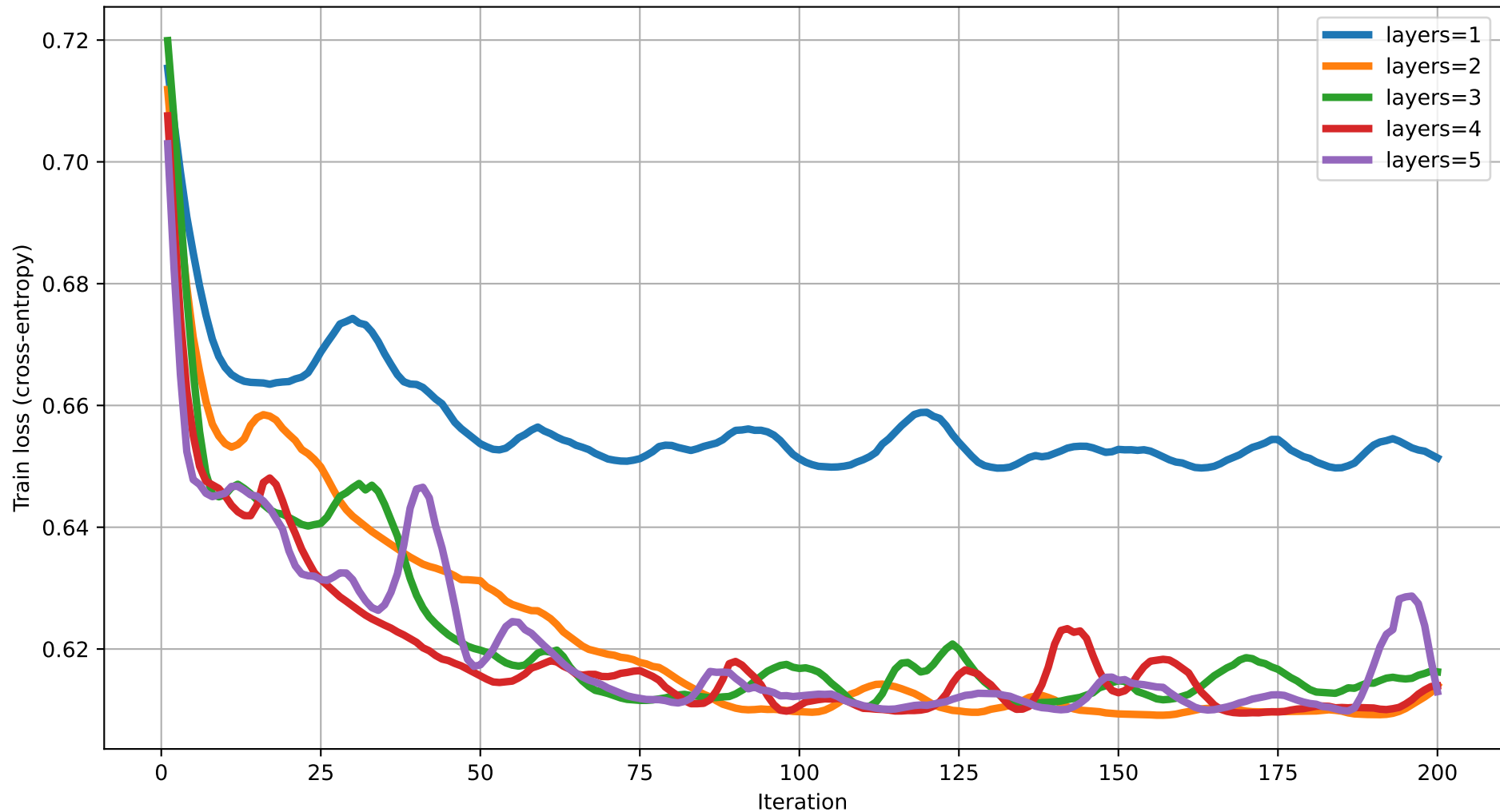
Train loss vs Iteration (degree=4) rot=RY, ent=pairwise, gate=CZ
