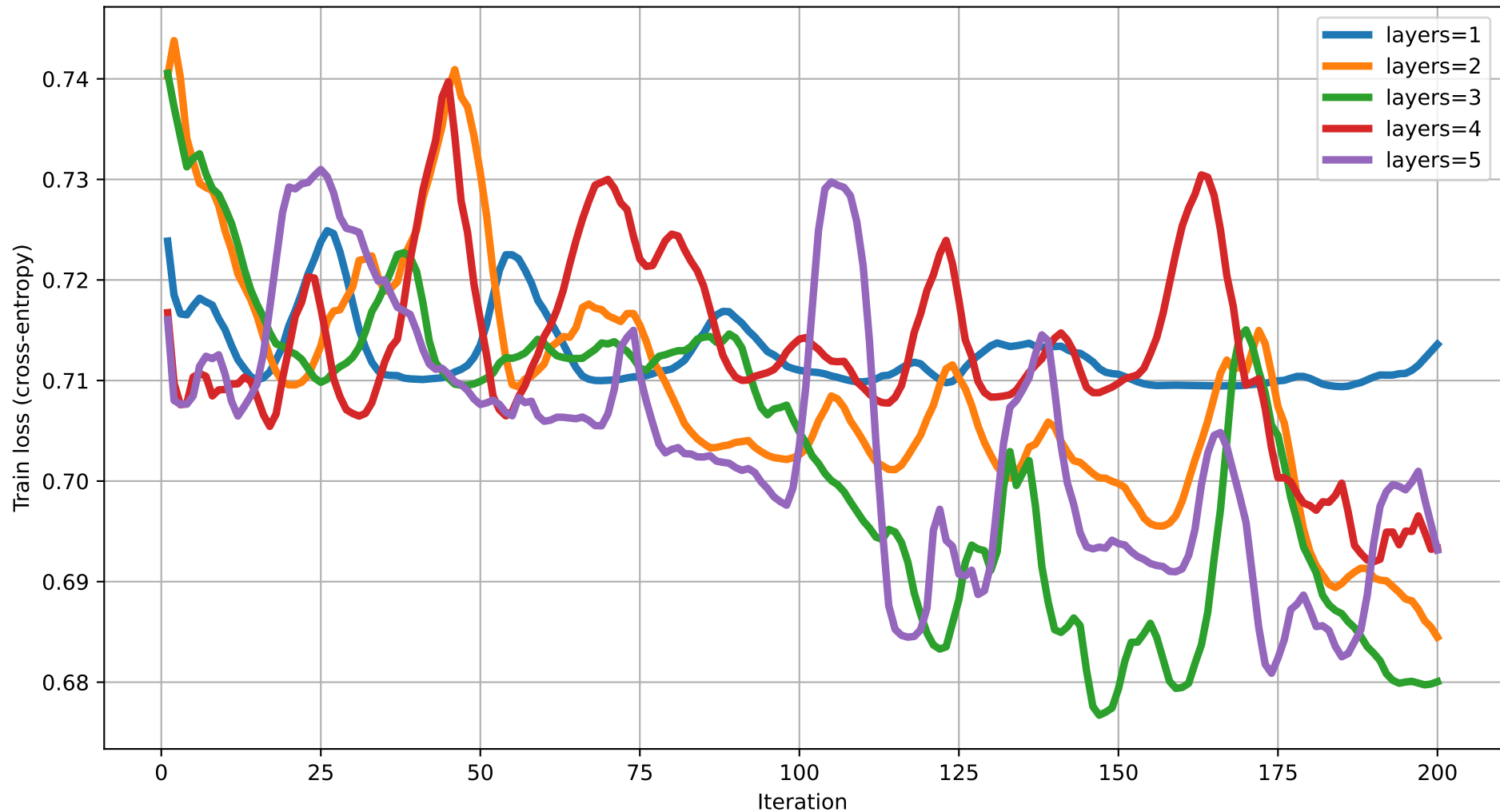
Train loss vs Iteration (dim=10) rot=Rot, ent=pairwise, gate=CNOT
