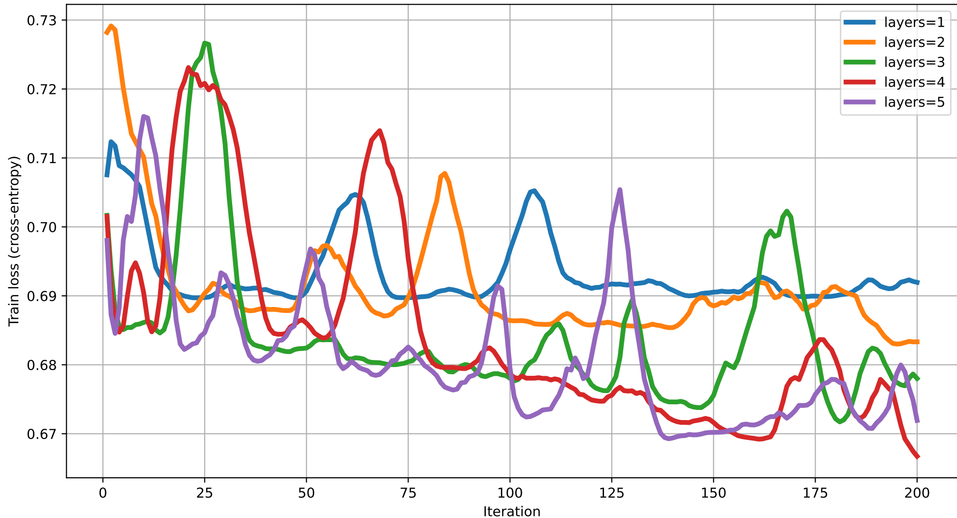
Train loss vs Iteration (dim=20) rot=RYZ, ent=chain, gate=CNOT
