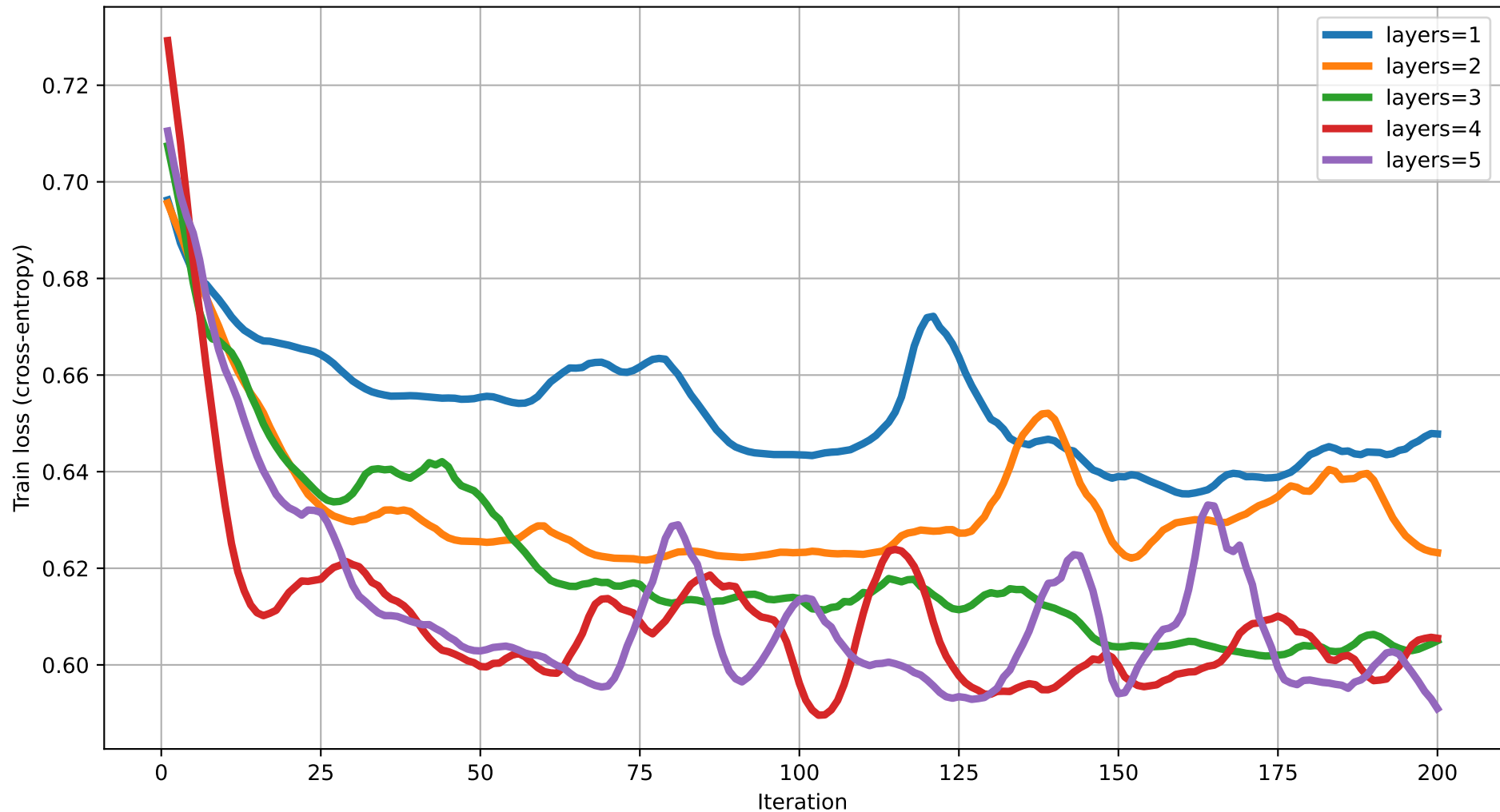
Train loss vs Iteration (dim=9) rot=RY, ent=ring, gate=CNOT
