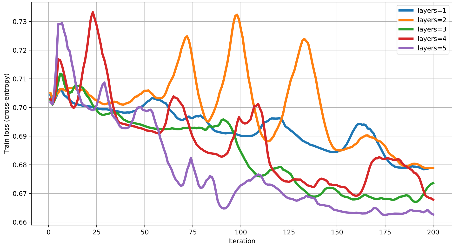
Train loss vs Iteration (dim=14) rot=RY, ent=chain, gate=CZ
