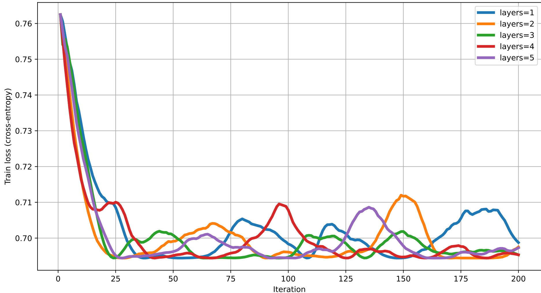
Train loss vs Iteration (dim=8) rot=RZ, ent=full, gate=CNOT
