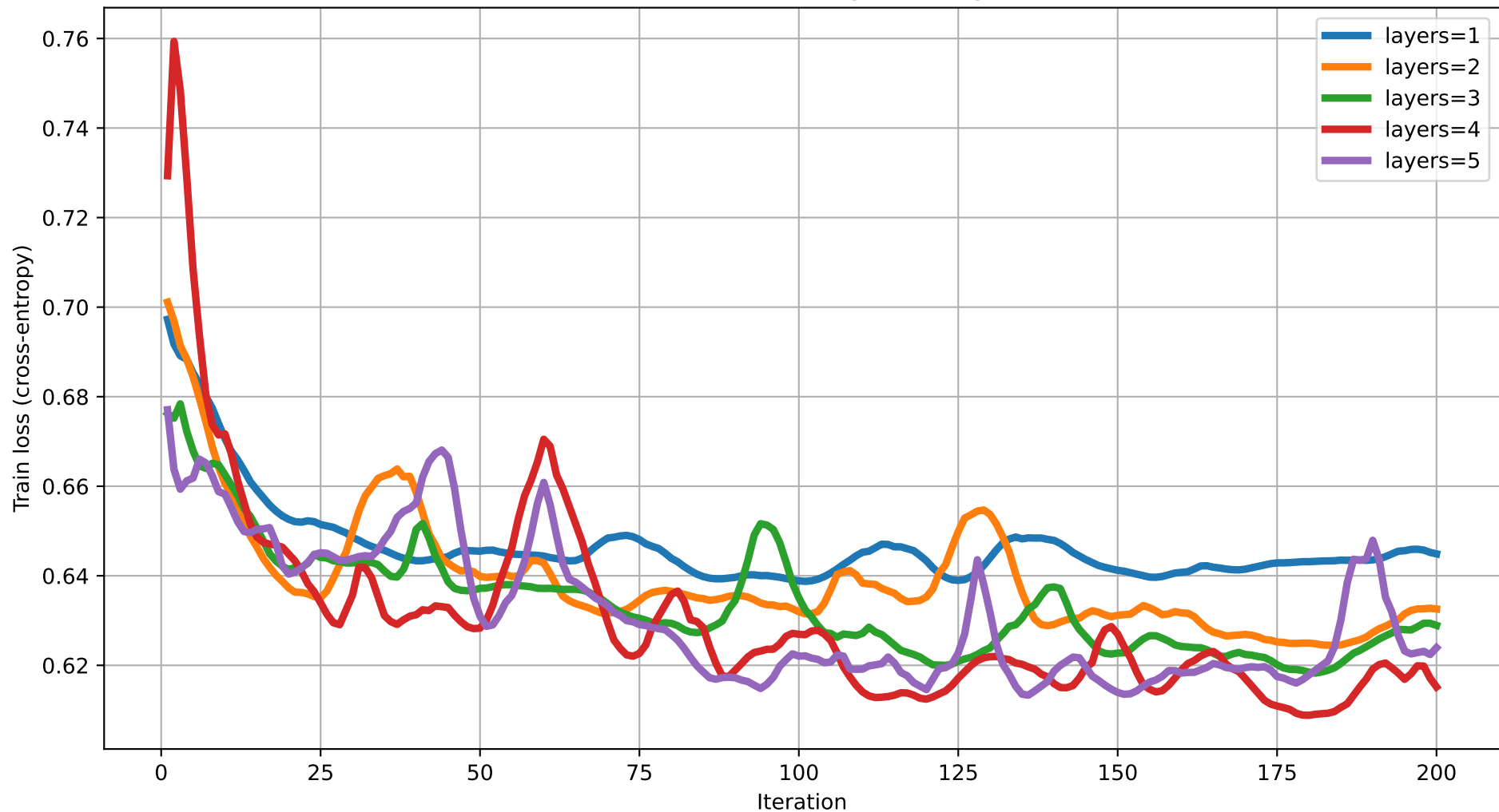
Train loss vs Iteration (dim=14) rot=Rot, ent=chain, gate=IsingXX
