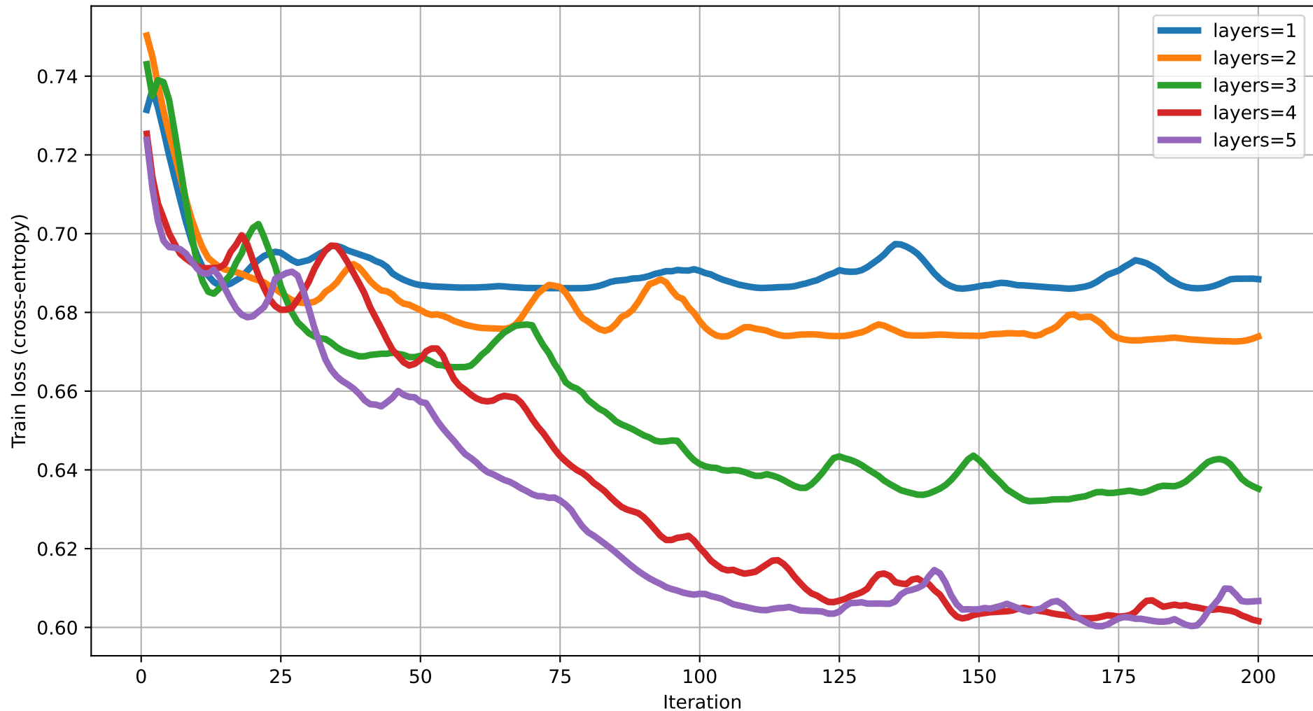
Train loss vs Iteration (degree=2) rot=RYZ, ent=chain, gate=CZ
