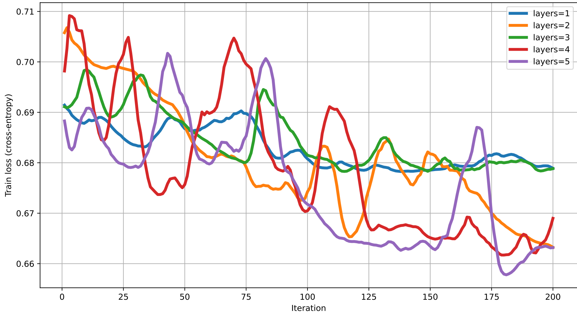
Train loss vs Iteration (dim=18) rot=RY, ent=ring, gate=CNOT
