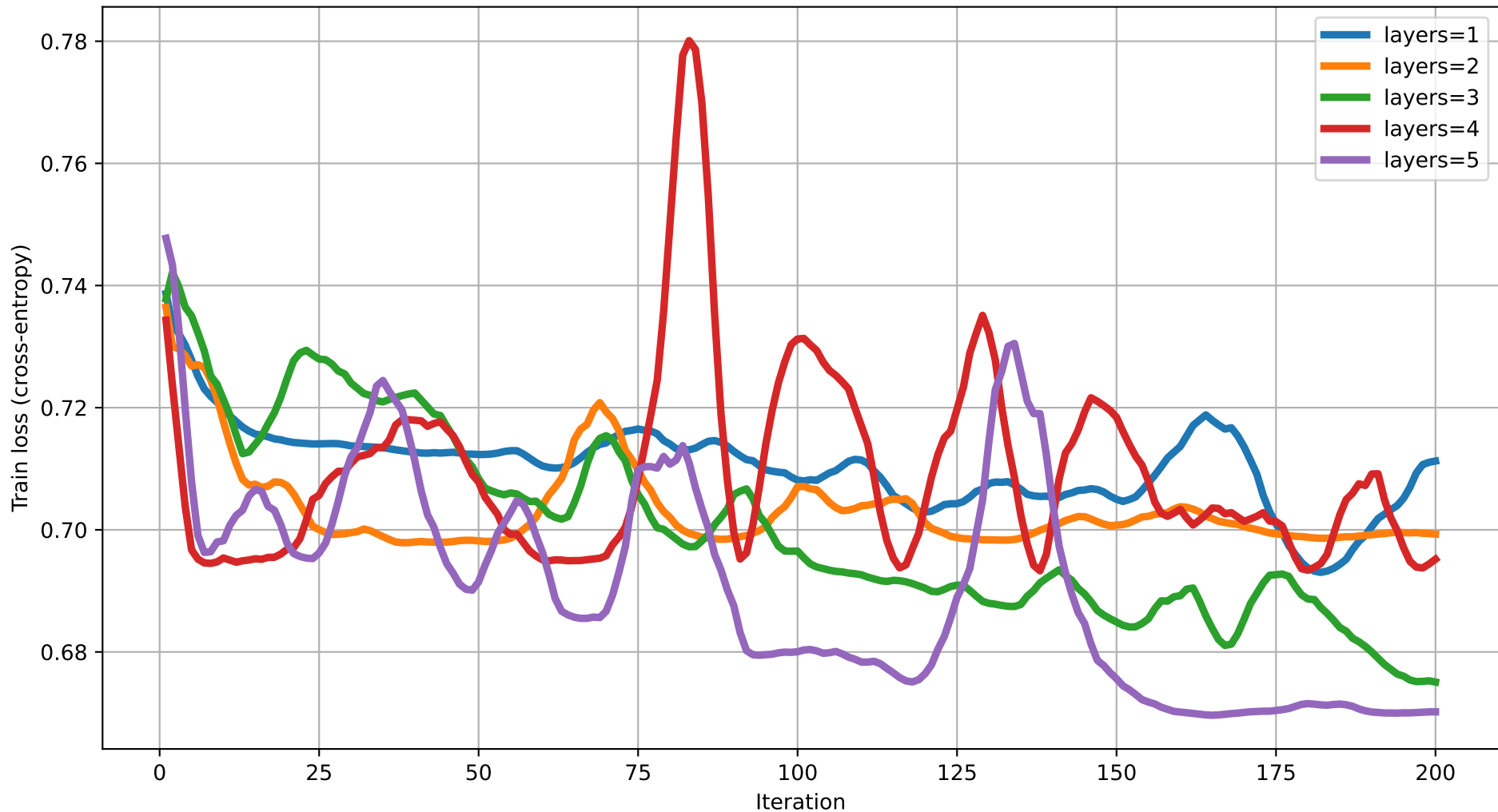
Train loss vs Iteration (dim=18) rot=RX, ent=full, gate=IsingXX
