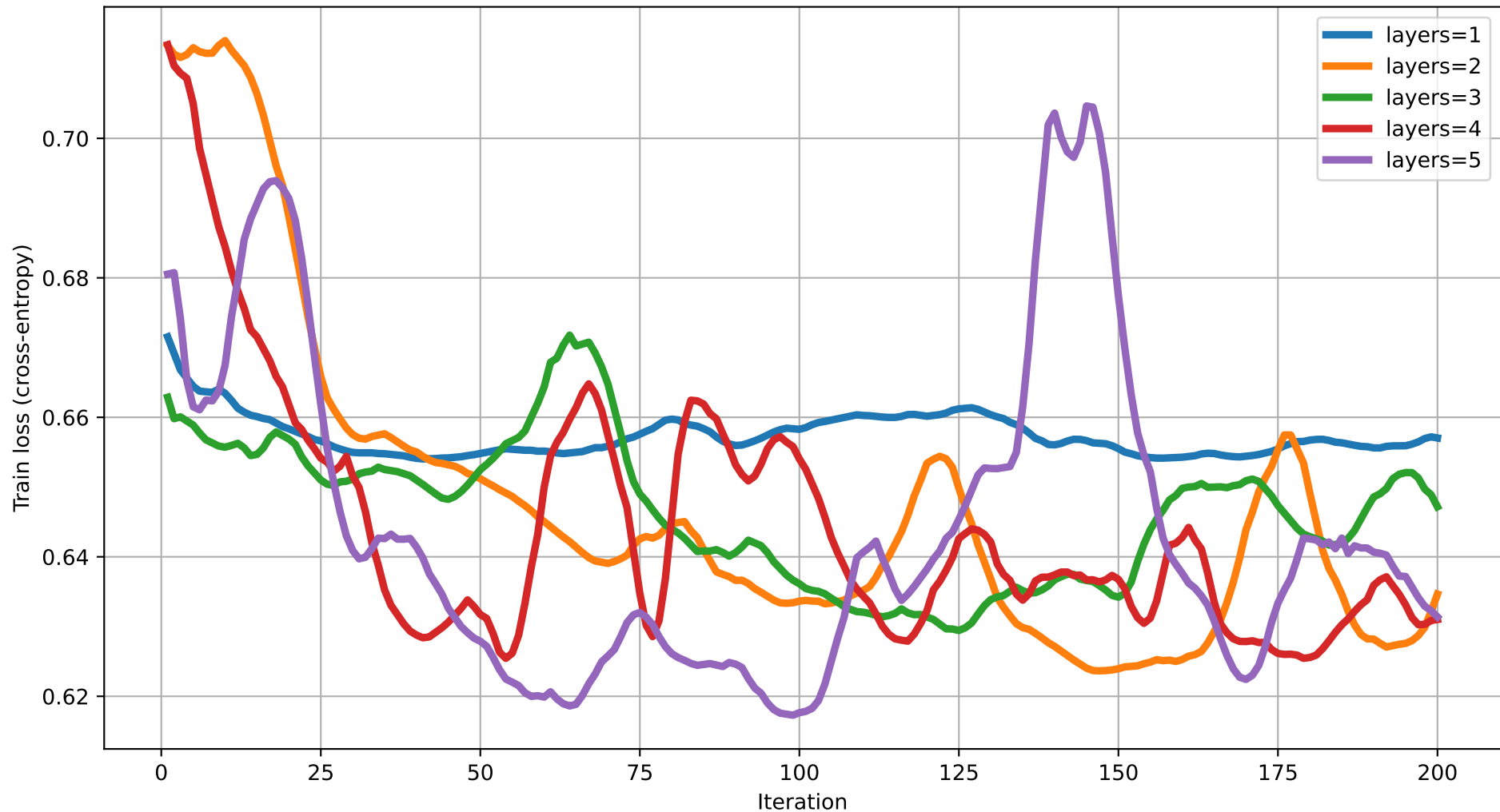
Train loss vs Iteration (dim=7) rot=RYZ, ent=full, gate=IsingXX
