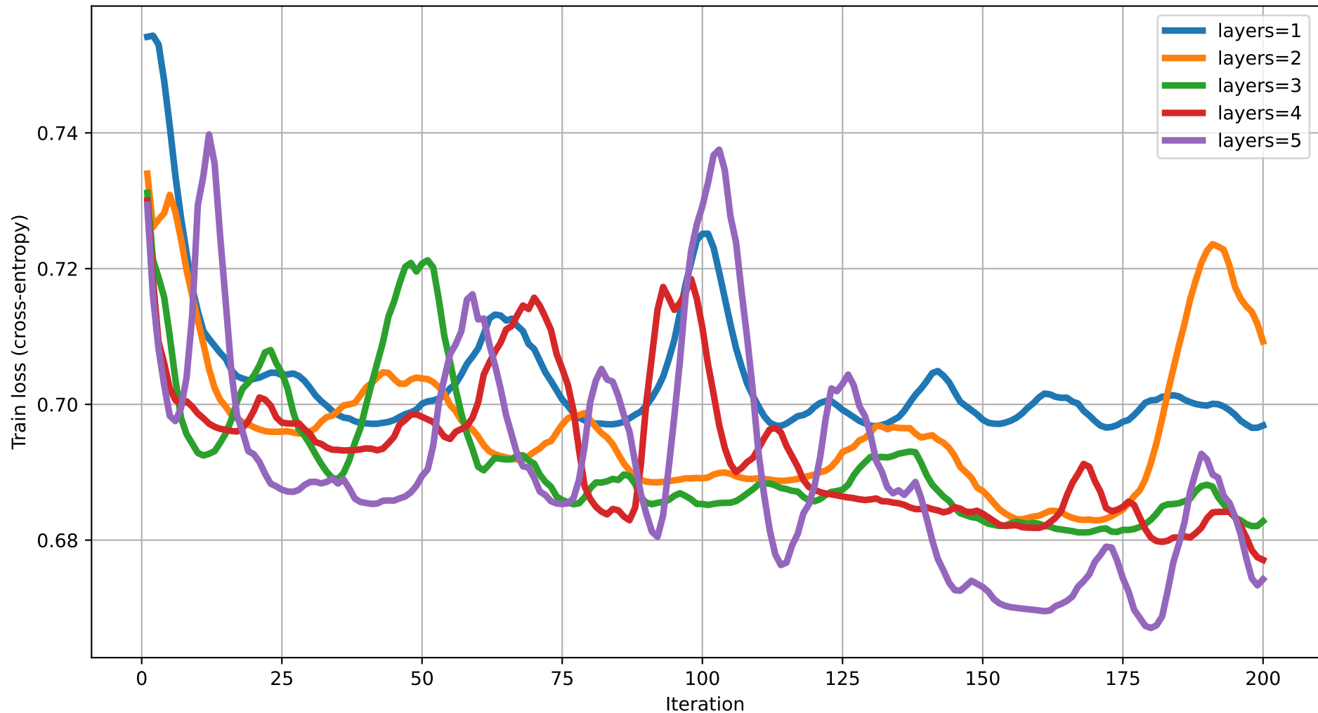
Train loss vs Iteration (dim=18) rot=RY, ent=full, gate=CZ
