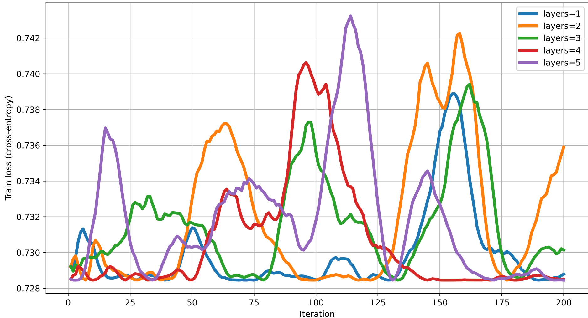
Train loss vs Iteration (dim=7) rot=RZ, ent=full, gate=CNOT
