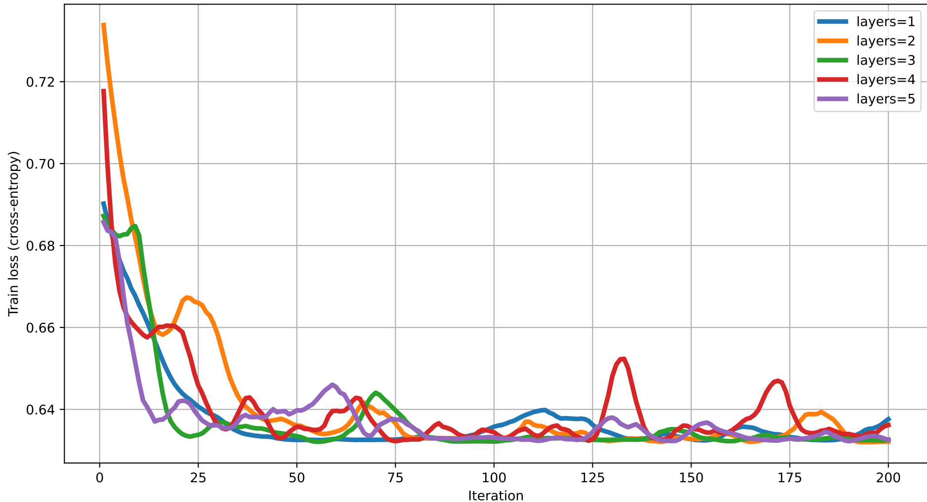
Train loss vs Iteration (degree=2) rot=RZ, ent=pairwise, gate=IsingXX
