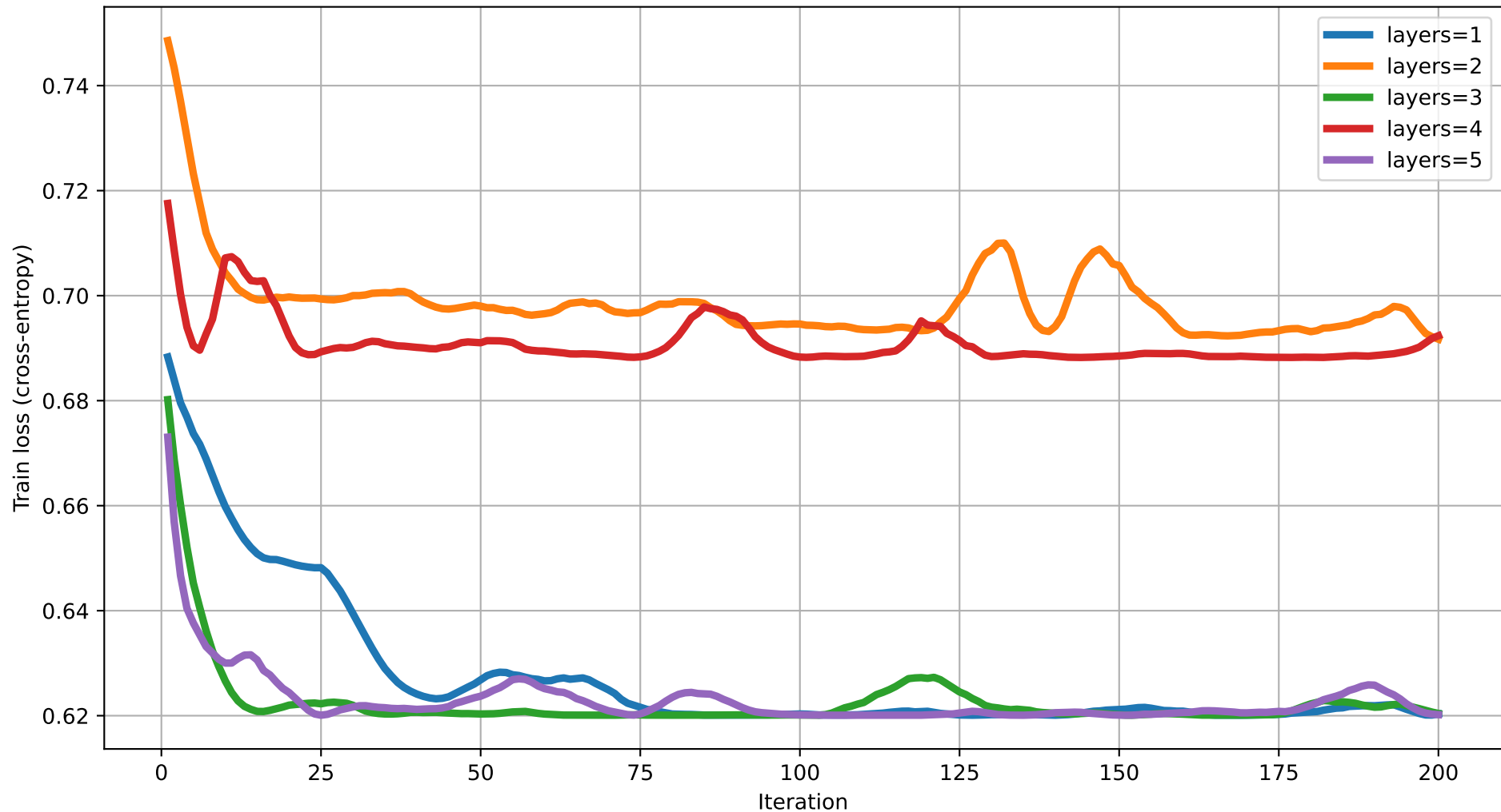
Train loss vs Iteration (degree=4) rot=RX, ent=pairwise, gate=IsingXX
