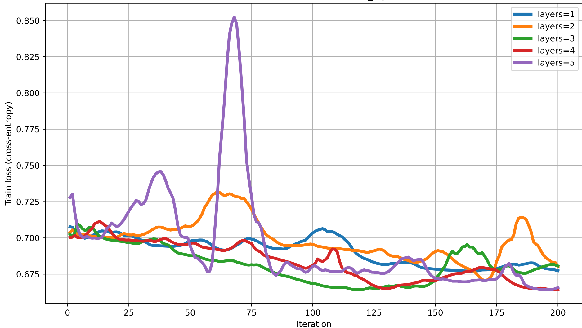
Train loss vs Iteration for different num_layers (dim=14)
