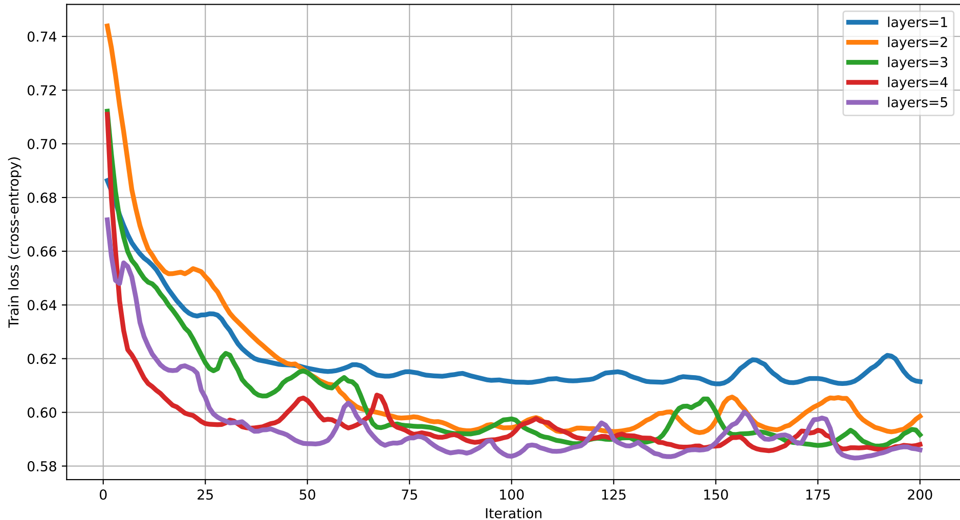
Train loss vs Iteration (degree=4) rot=RYZ, ent=full, gate=IsingXX
