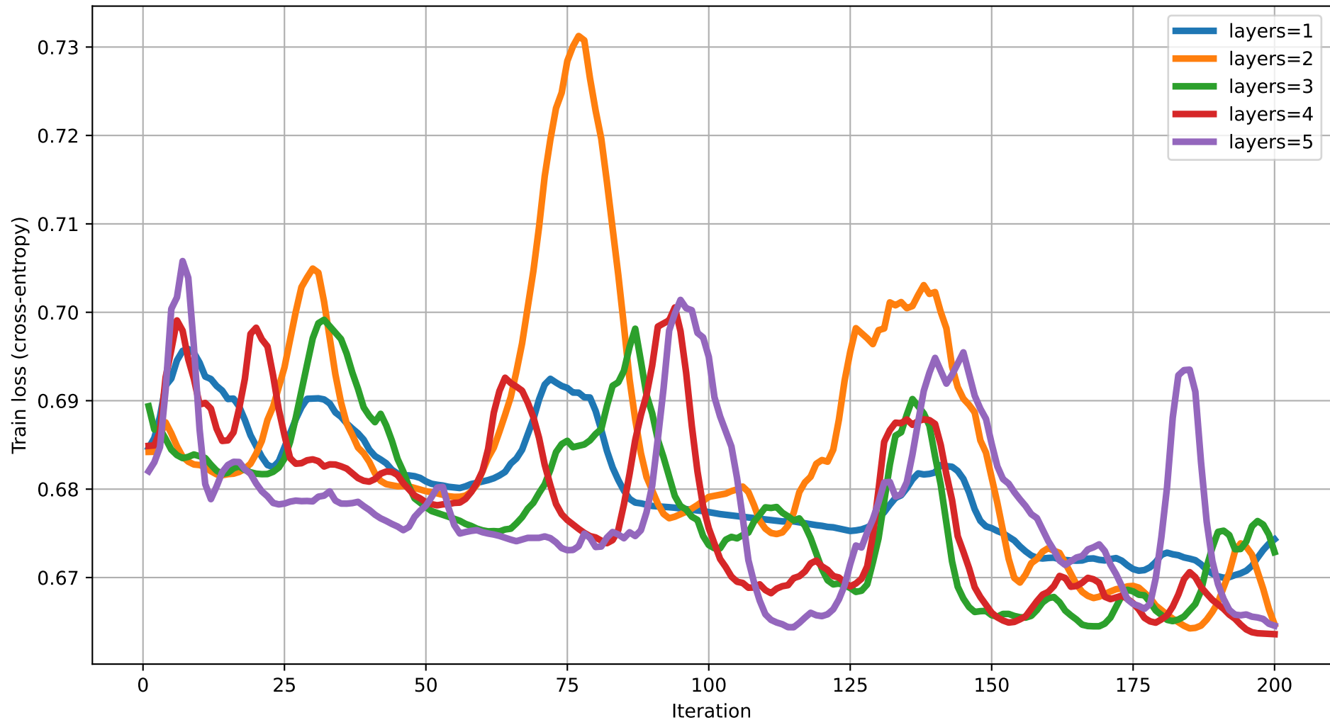
Train loss vs Iteration (dim=15) rot=Rot, ent=full, gate=CNOT
