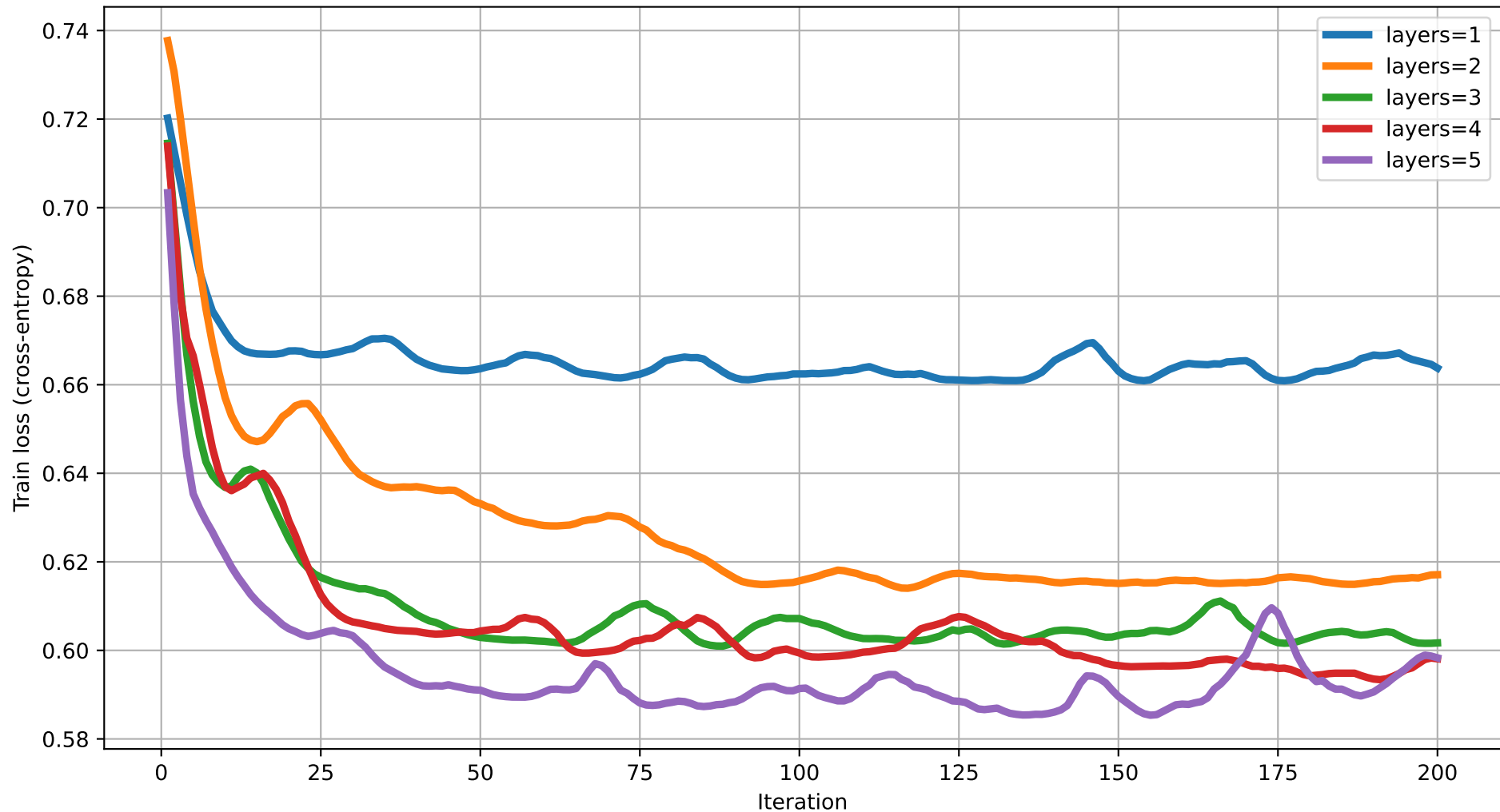
Train loss vs Iteration (degree=3) rot=RY, ent=chain, gate=CNOT
