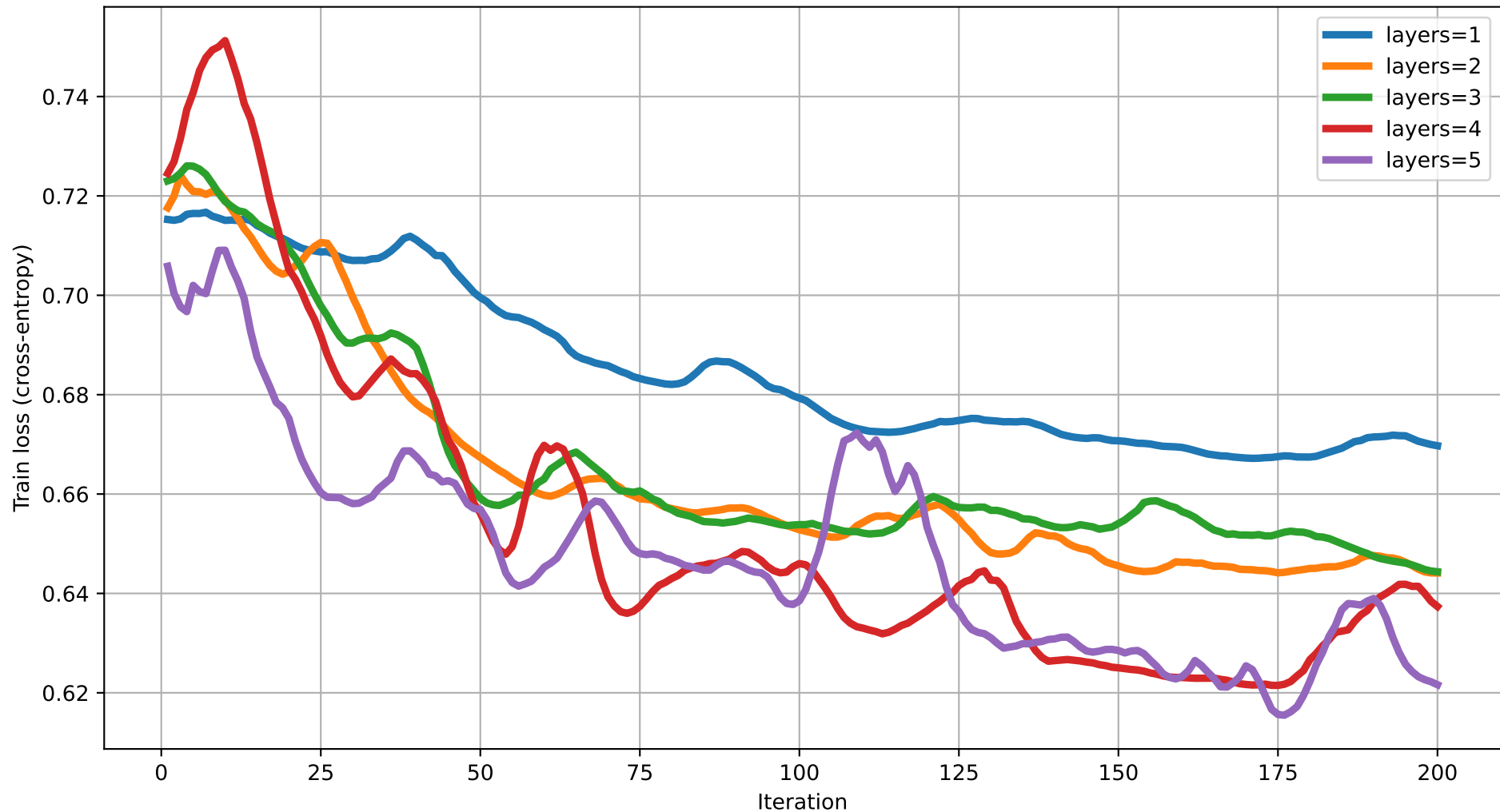
Train loss vs Iteration (dim=7) rot=RY, ent=full, gate=CZ
