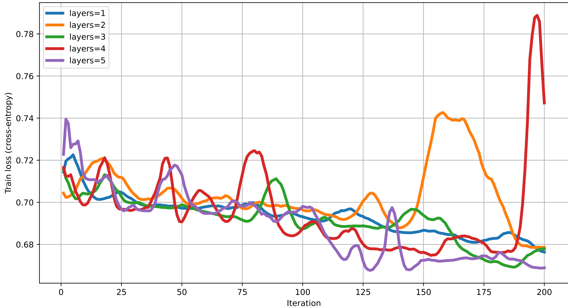
Train loss vs Iteration (dim=14) rot=Rot, ent=pairwise, gate=CZ
