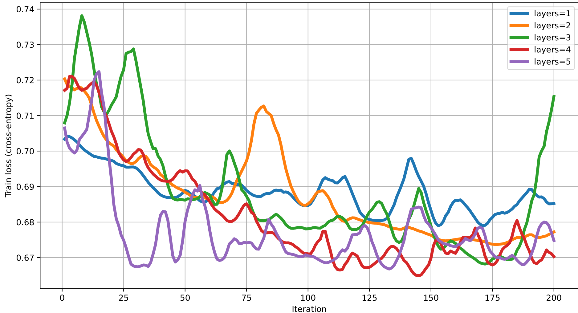
Train loss vs Iteration (dim=15) rot=RYZ, ent=ring, gate=CNOT
