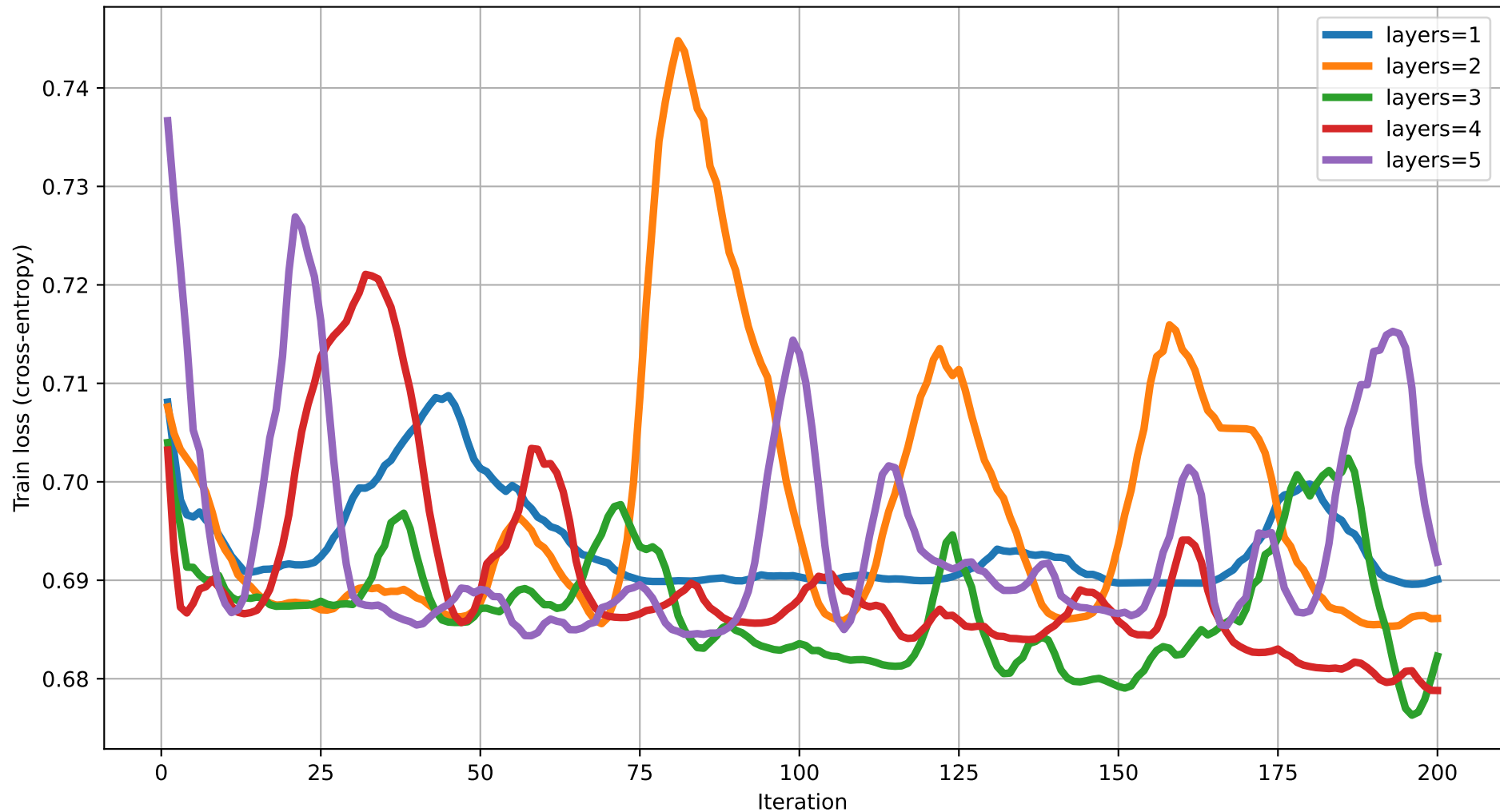
Train loss vs Iteration (dim=20) rot=YRZ, ent=chain, gate=CZ
