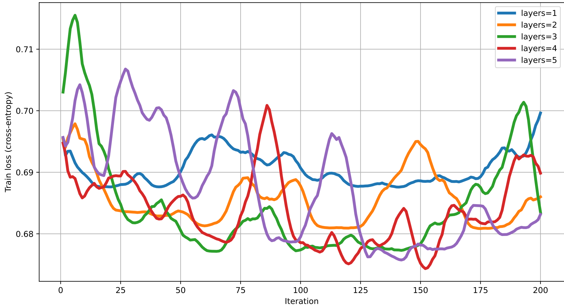
Train loss vs Iteration (dim=13) rot=RX, ent=full, gate=CZ
