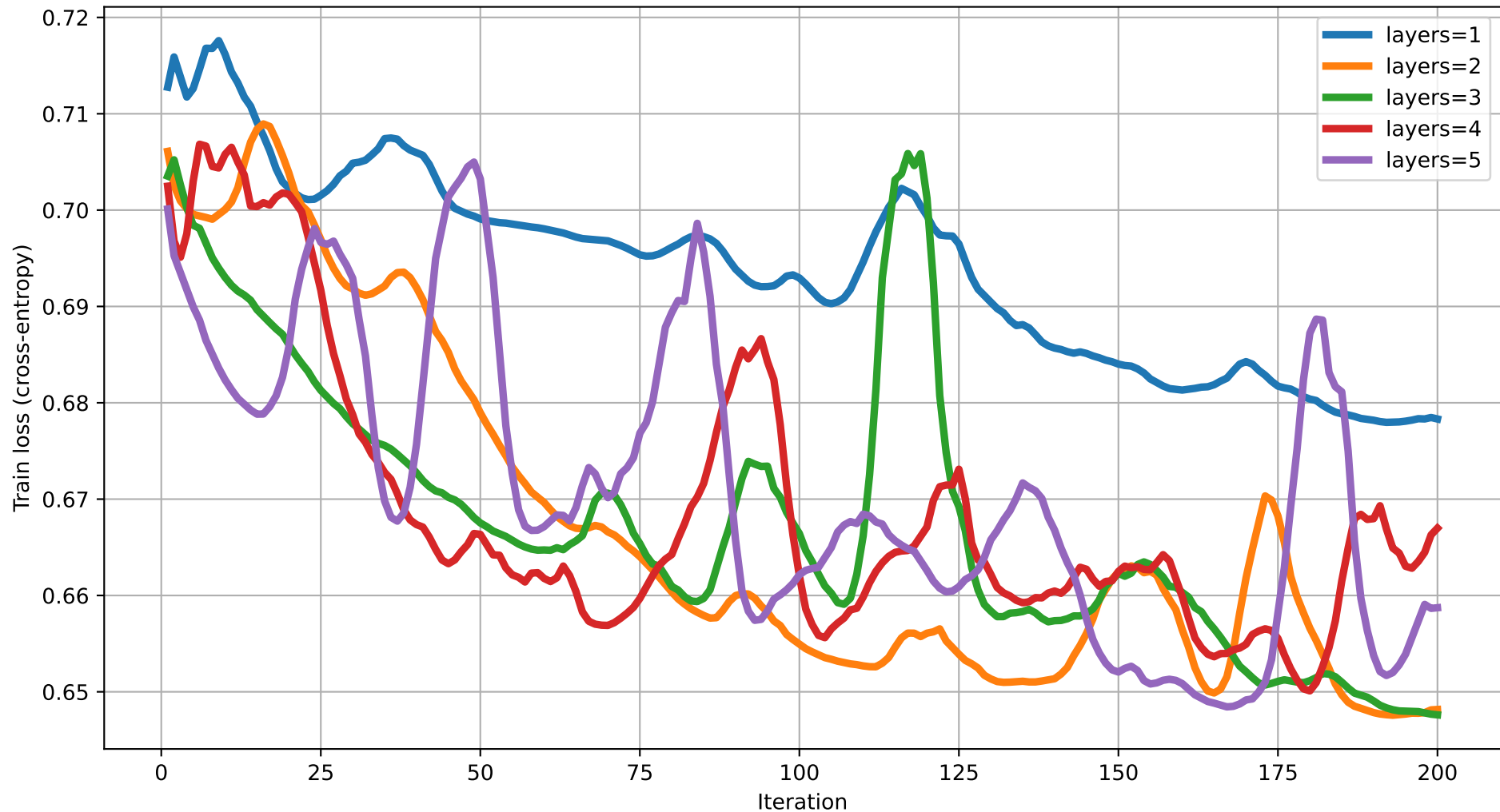
Train loss vs Iteration (dim=6) rot=RYZ, ent=chain, gate=CZ
