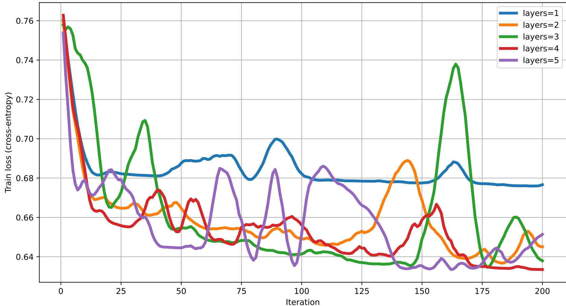
Train loss vs Iteration (dim=8) rot=RY, ent=pairwise, gate=CZ
