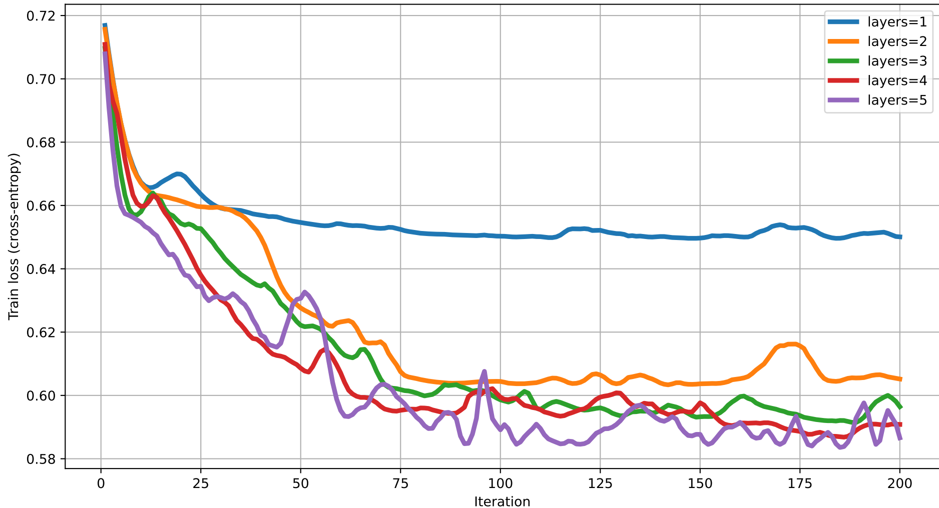
Train loss vs Iteration (degree=4) rot=Rot, ent=full, gate=CZ
