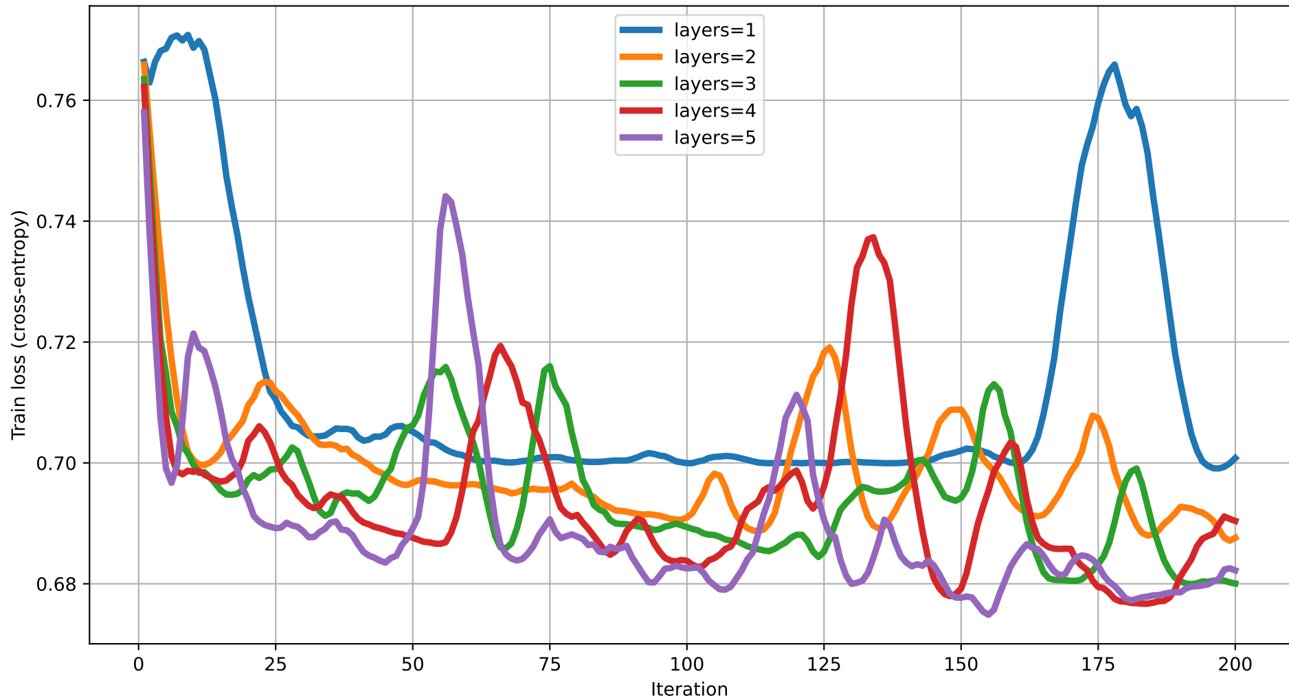
Train loss vs Iteration (dim=17) rot=Rot, ent=ring, gate=CZ
