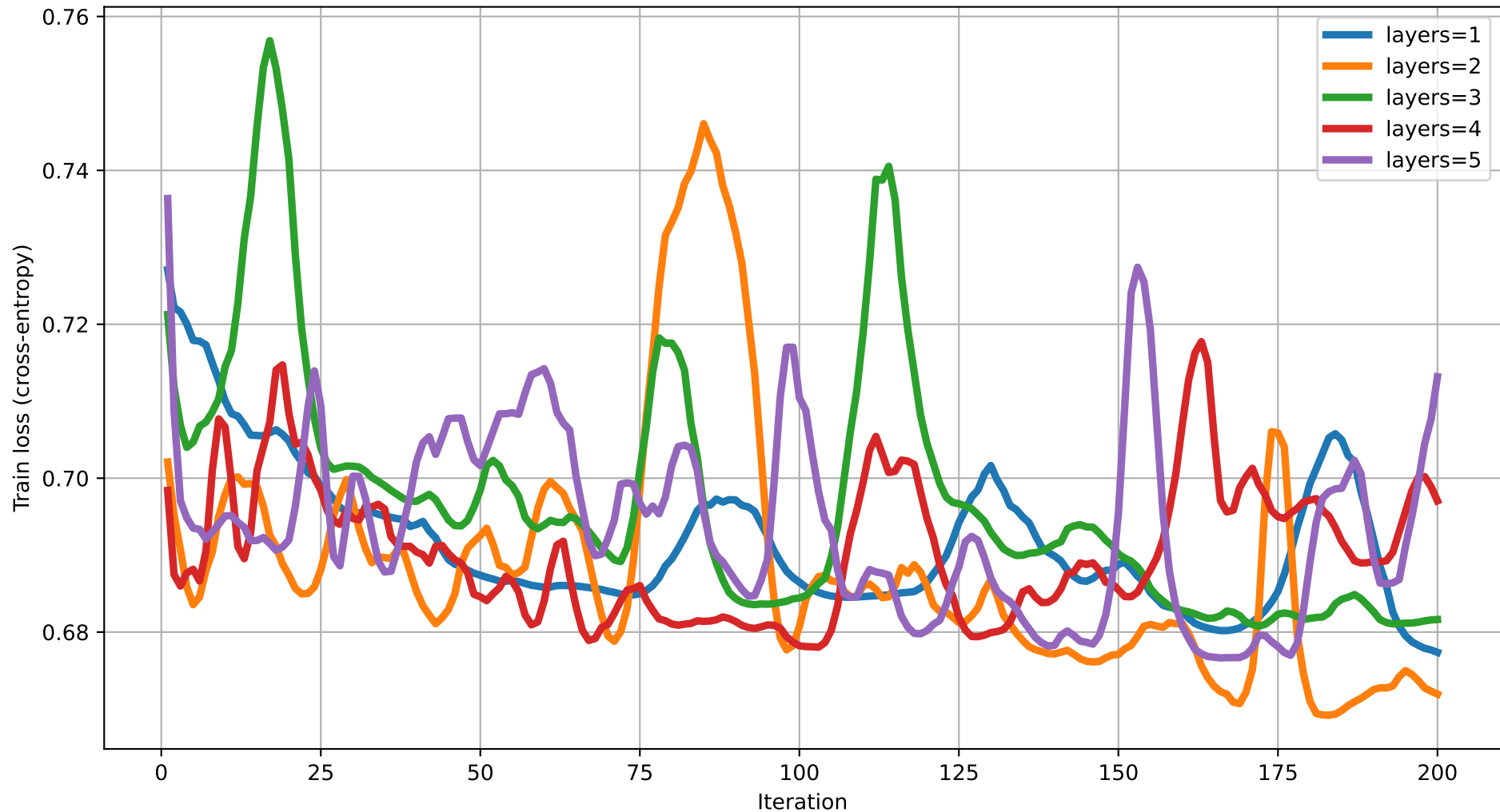
Train loss vs Iteration (dim=20) rot=Rot, ent=full, gate=IsingXX
