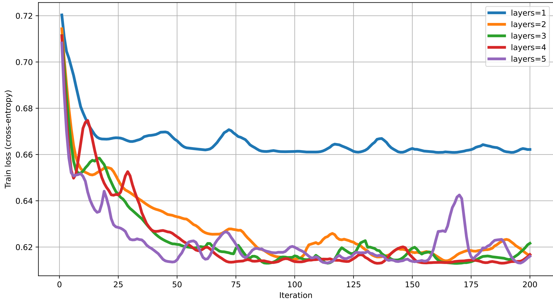
Train loss vs Iteration (degree=3) rot=Rot, ent=pairwise, gate=CZ
