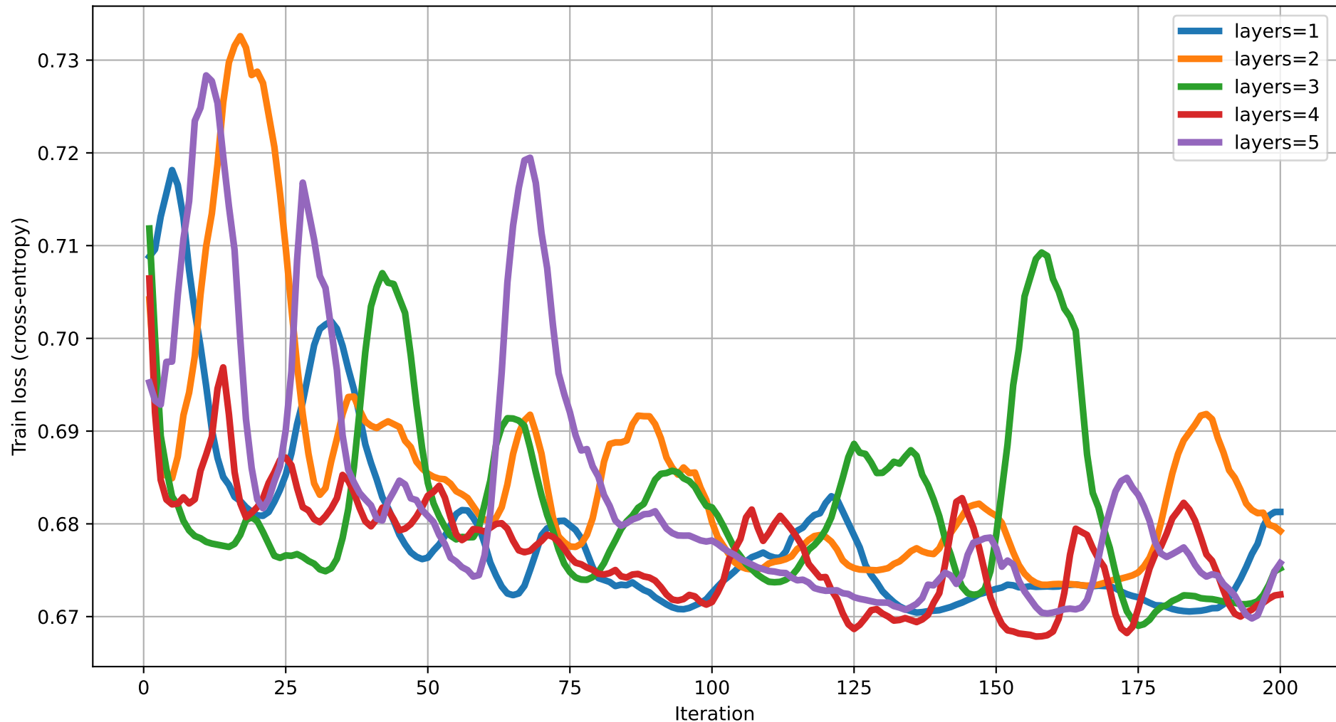
Train loss vs Iteration (dim=20) rot=RYZ, ent=ring, gate=IsingXX
