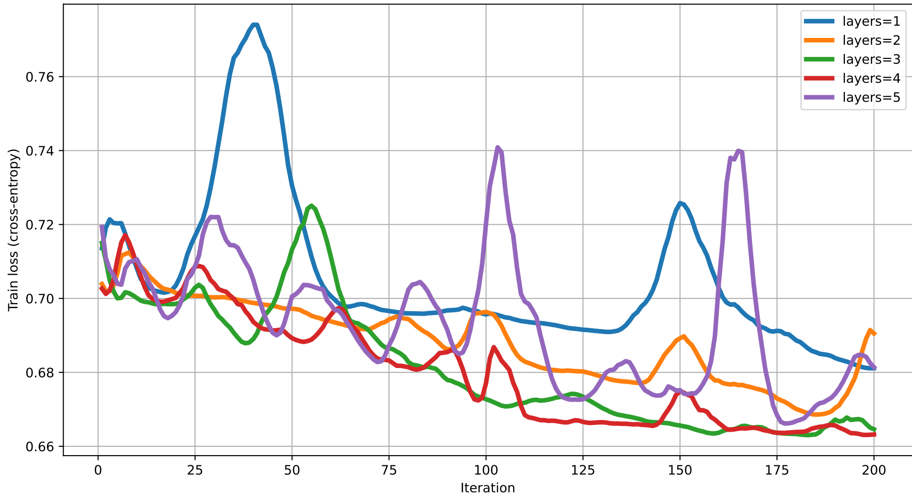
Train loss vs Iteration (dim=14) rot=RY, ent=pairwise, gate=CZ
