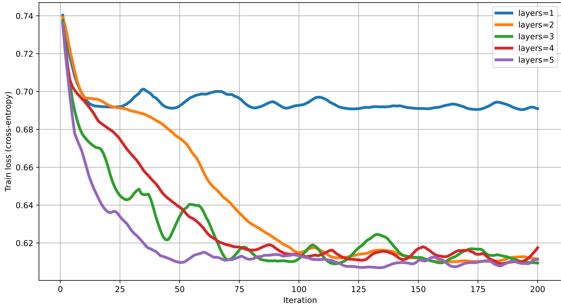
Train loss vs Iteration (degree=5) rot=RY, ent=ring, gate=CZ
