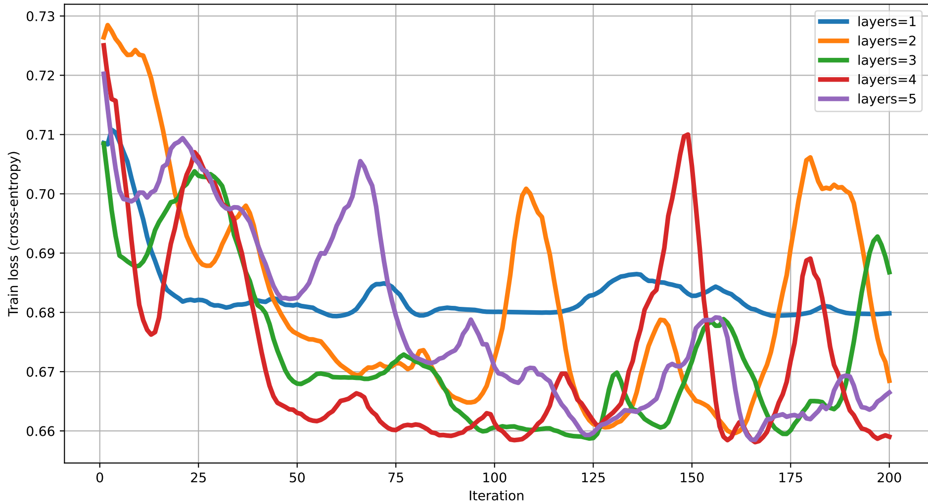
Train loss vs Iteration (dim=5) rot=RZ, ent=full, gate=IsingXX
