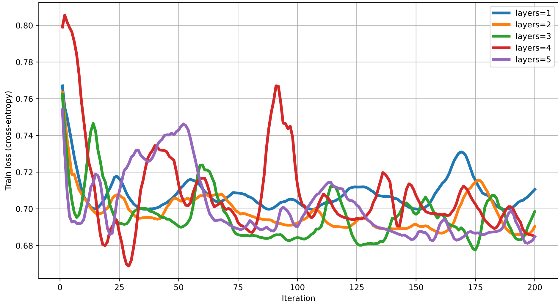
Train loss vs Iteration (dim=17) rot=Rot, ent=chain, gate=CNOT
