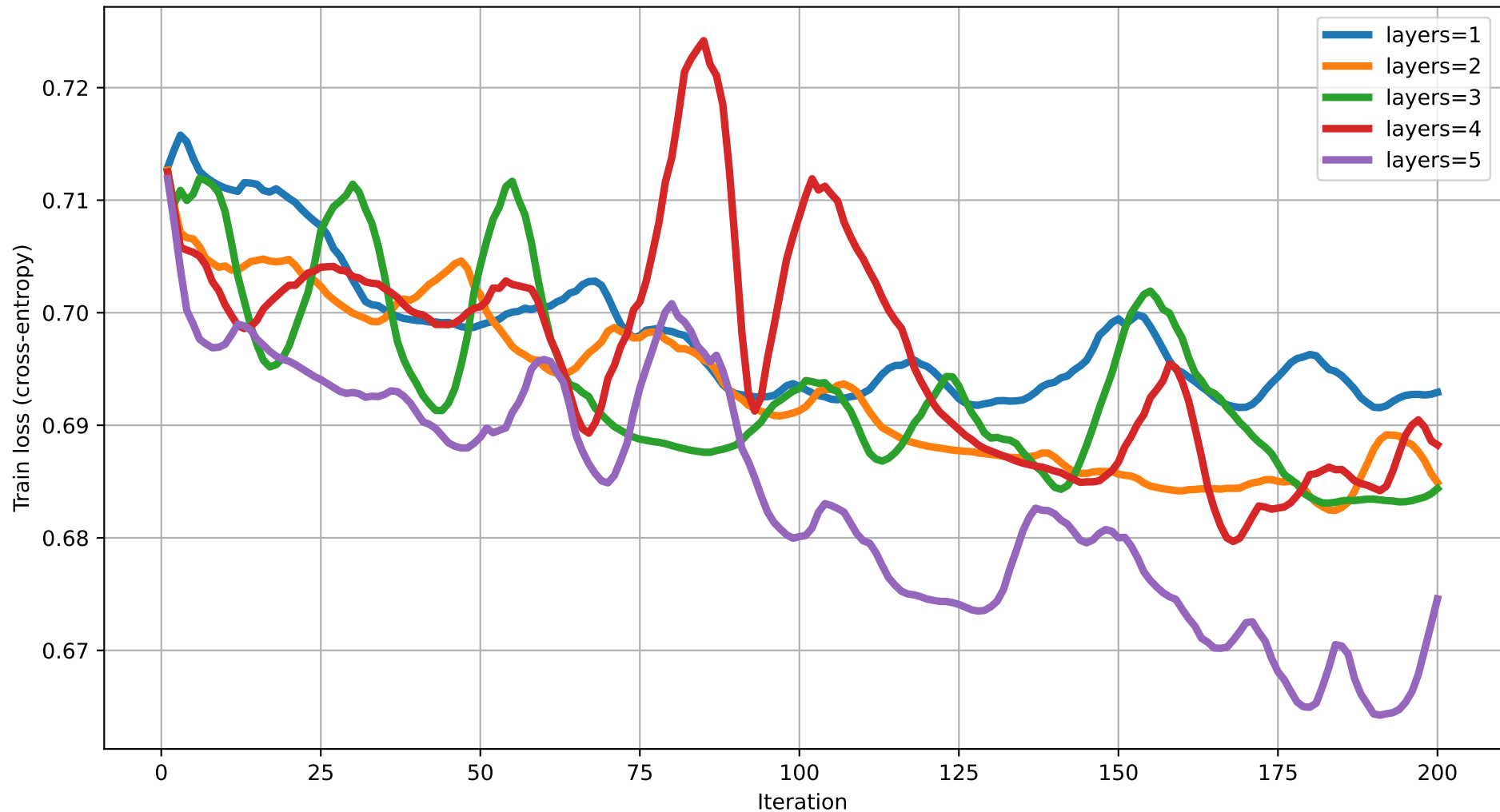
Train loss vs Iteration (dim=11) rot=RX, ent=ring, gate=CZ
