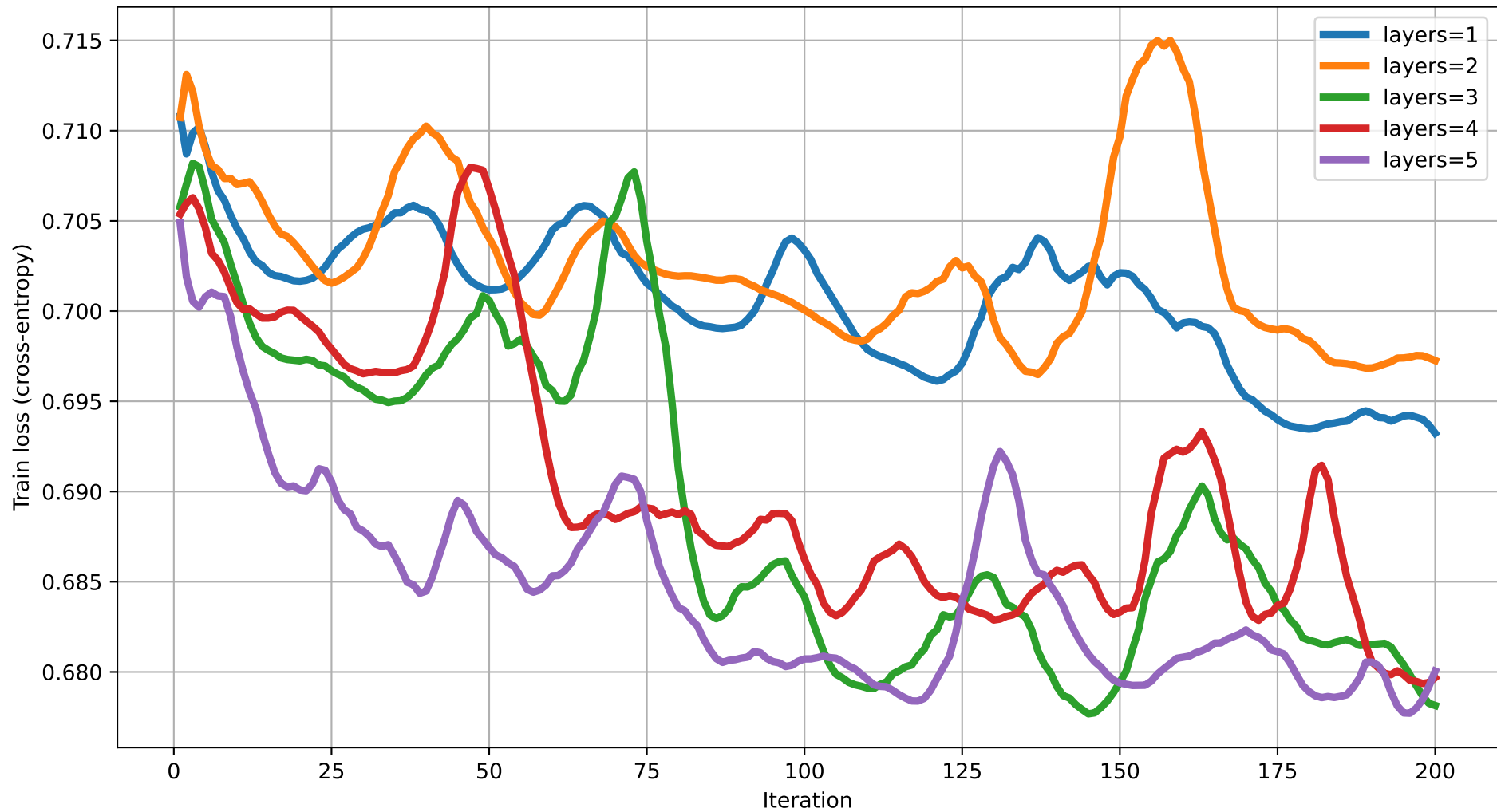
Train loss vs Iteration (dim=12) rot=RX, ent=full, gate=CZ
