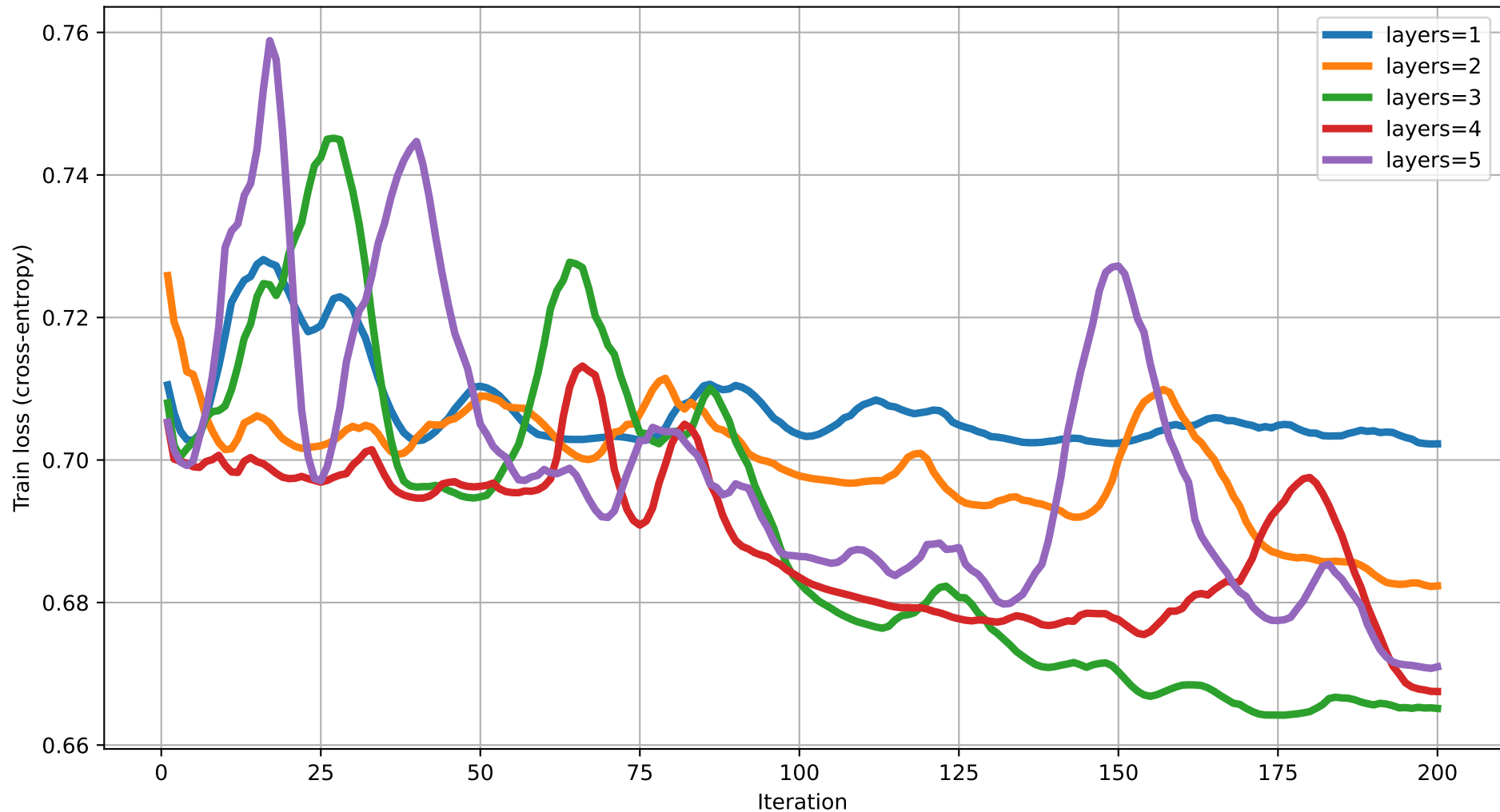
Train loss vs Iteration (dim=11) rot=RY, ent=pairwise, gate=CNOT
