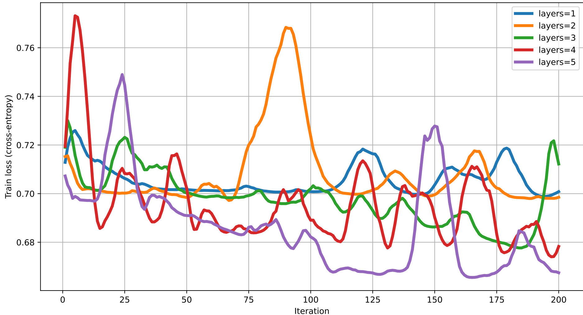
Train loss vs Iteration (dim=12) rot=RYZ, ent=pairwise, gate=CNOT
