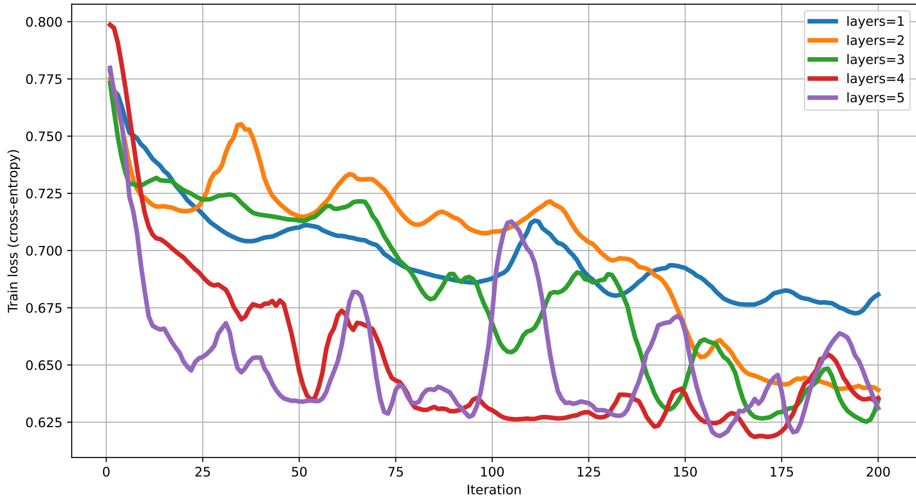
Train loss vs Iteration (dim=4) rot=RYZ, ent=pairwise, gate=CZ
