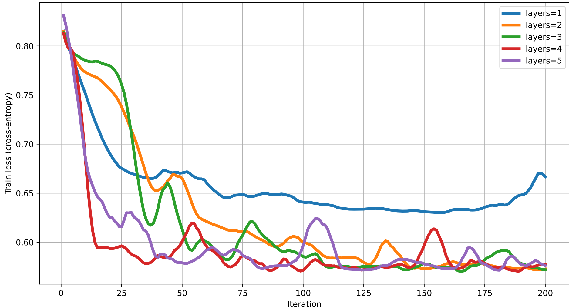
Train loss vs Iteration (dim=2) rot=RYZ, ent=pairwise, gate=CZ
