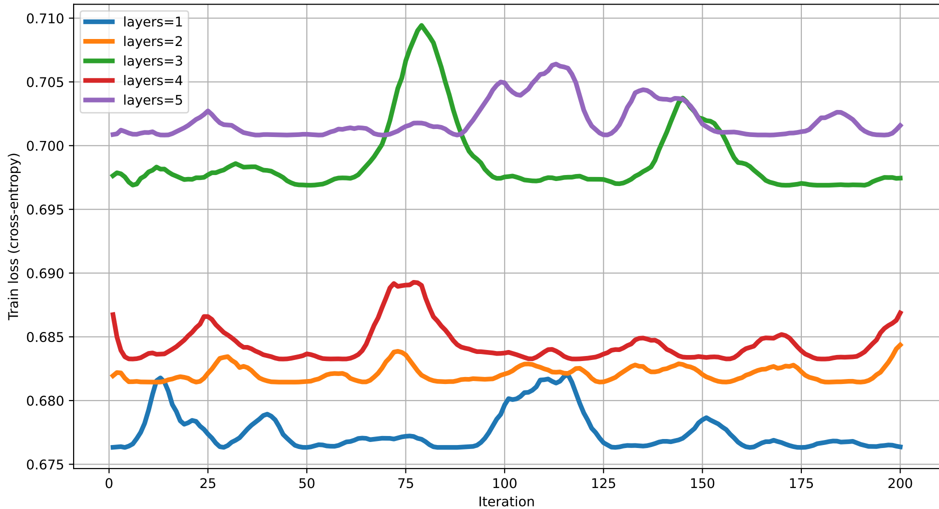
Train loss vs Iteration (degree=4) rot=RZ, ent=ring, gate=CNOT
