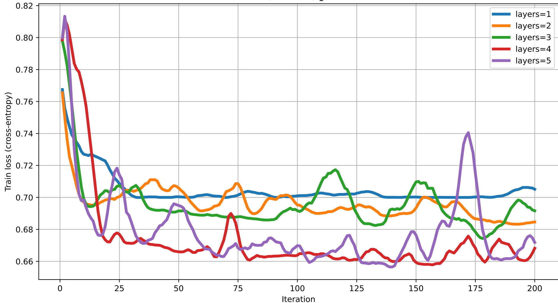
Train loss vs Iteration (dim=17) rot=RYZ, ent=full, gate=CNOT
