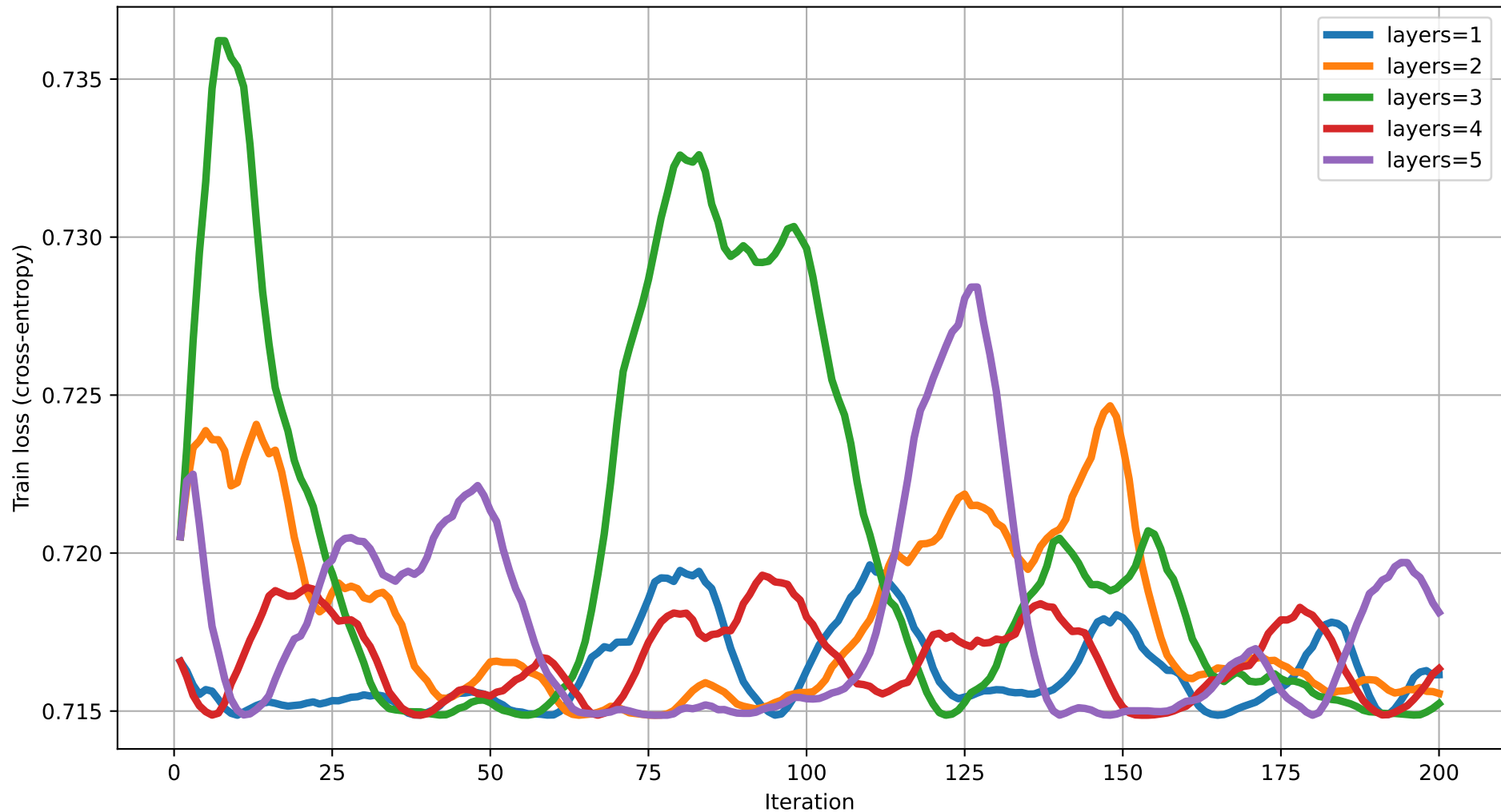
Train loss vs Iteration (dim=3) rot=RZ, ent=pairwise, gate=CZ
