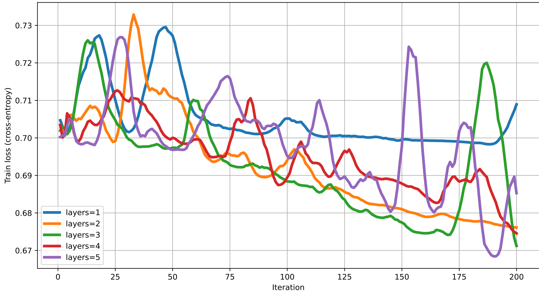
Train loss vs Iteration (dim=12) rot=RYZ, ent=chain, gate=CNOT
