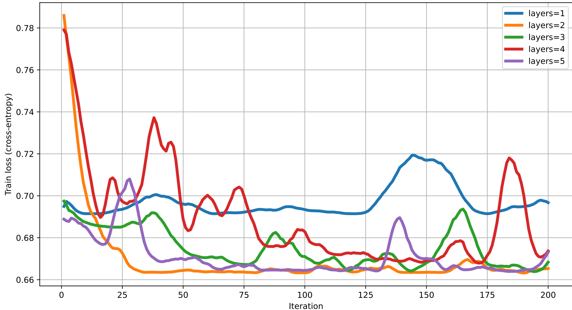
Train loss vs Iteration (dim=4) rot=RY, ent=chain, gate=IsingXX
