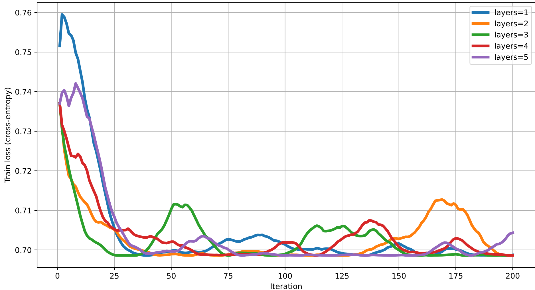
Train loss vs Iteration (dim=18) rot=RZ, ent=full, gate=CNOT
