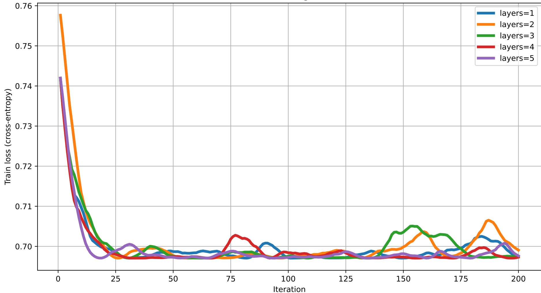
Train loss vs Iteration (degree=5) rot=RZ, ent=full, gate=CNOT
