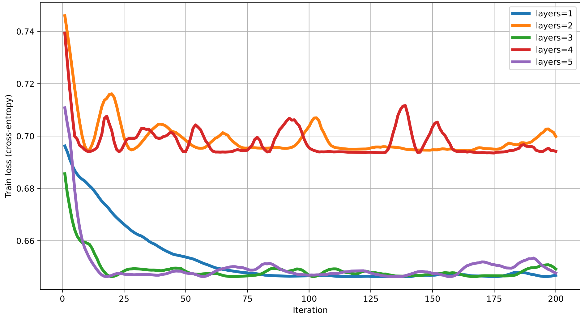
Train loss vs Iteration (degree=5) rot=RX, ent=full, gate=IsingXX
