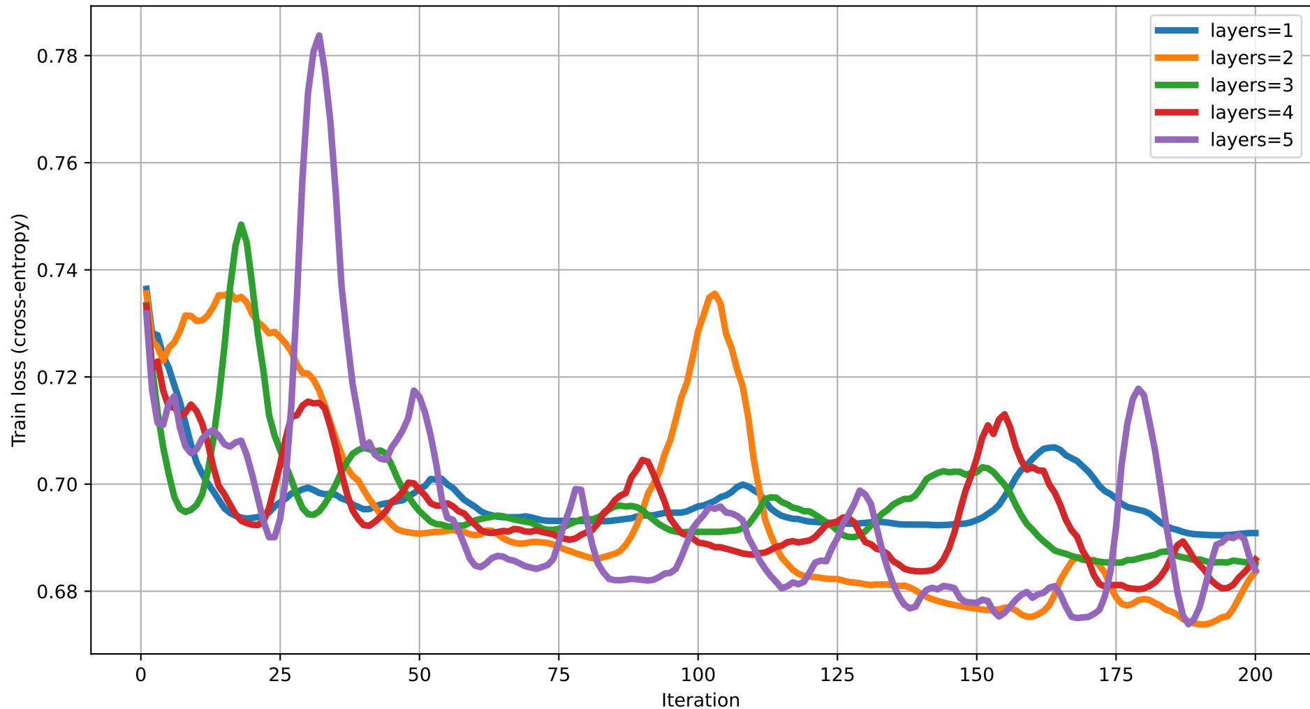
Train loss vs Iteration (dim=16) rot=RYZ, ent=ring, gate=CZ
