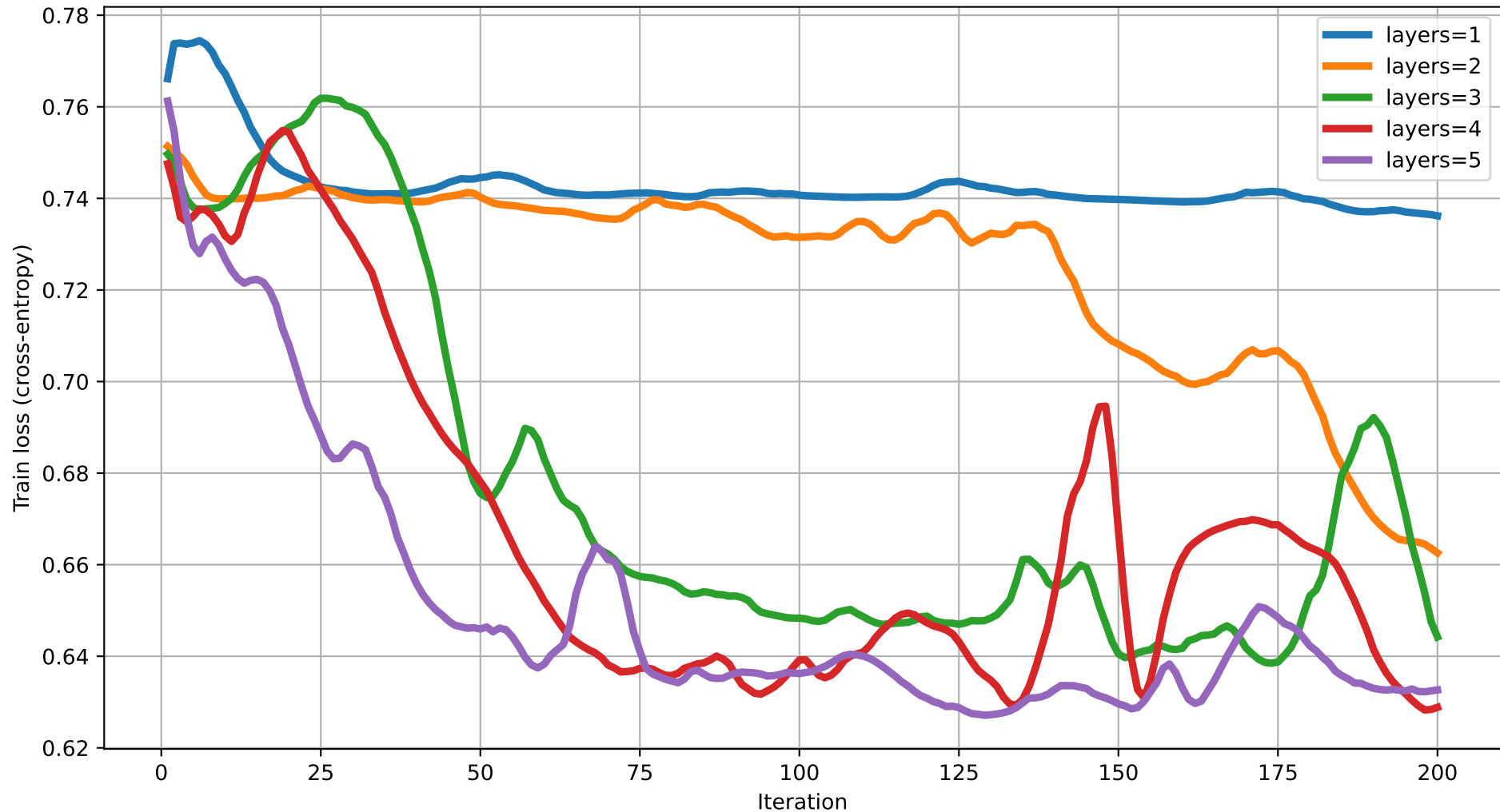
Train loss vs Iteration (dim=5) rot=RY, ent=chain, gate=CNOT
