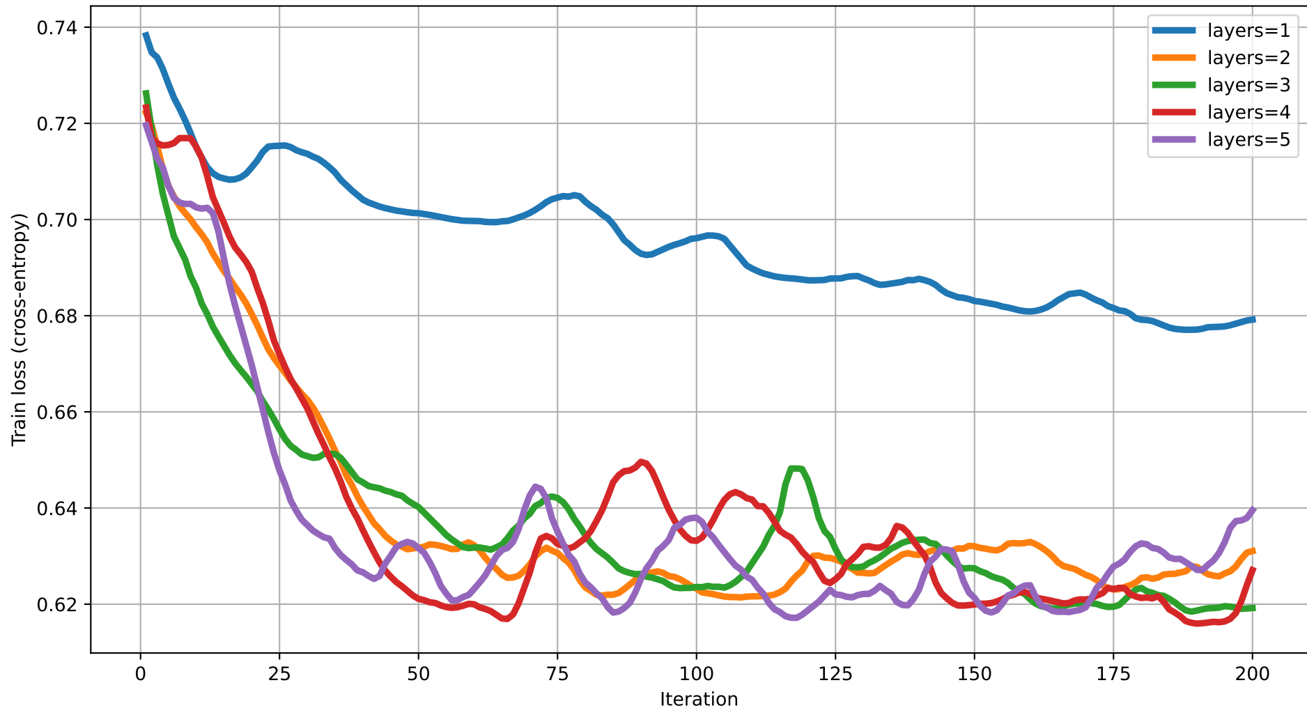
Train loss vs Iteration (dim=6) rot=RY, ent=ring, gate=CZ
