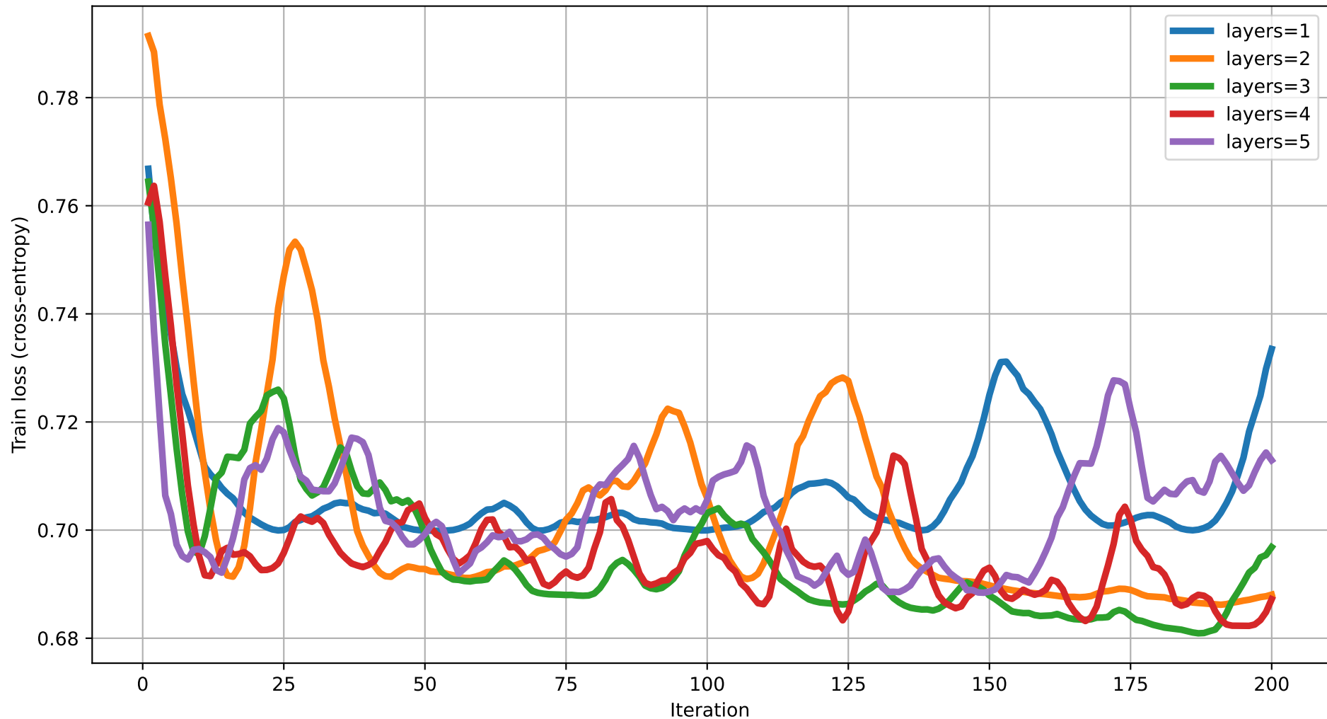
Train loss vs Iteration (dim=17) rot=Rot, ent=full, gate=CZ
