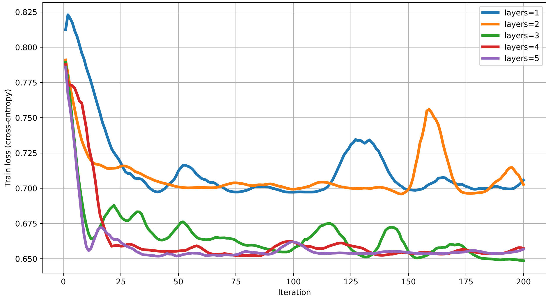
Train loss vs Iteration (dim=4) rot=RX, ent=full, gate=CNOT
