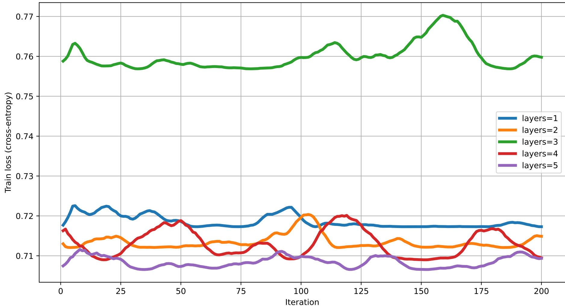
Train loss vs Iteration (dim=10) rot=RZ, ent=ring, gate=CNOT
