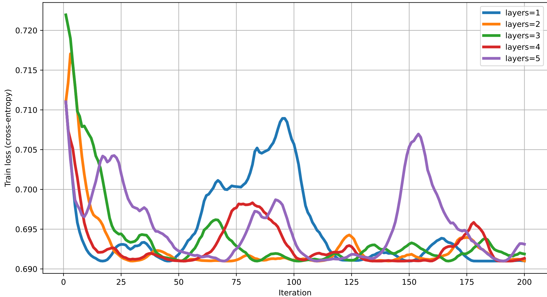
Train loss vs Iteration (dim=20) rot=RZ, ent=chain, gate=CNOT
