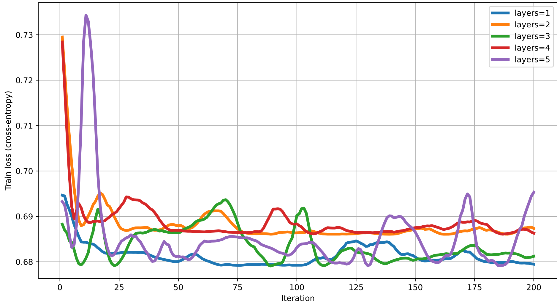
Train loss vs Iteration (degree=2) rot=RX, ent=ring, gate=IsingXX
