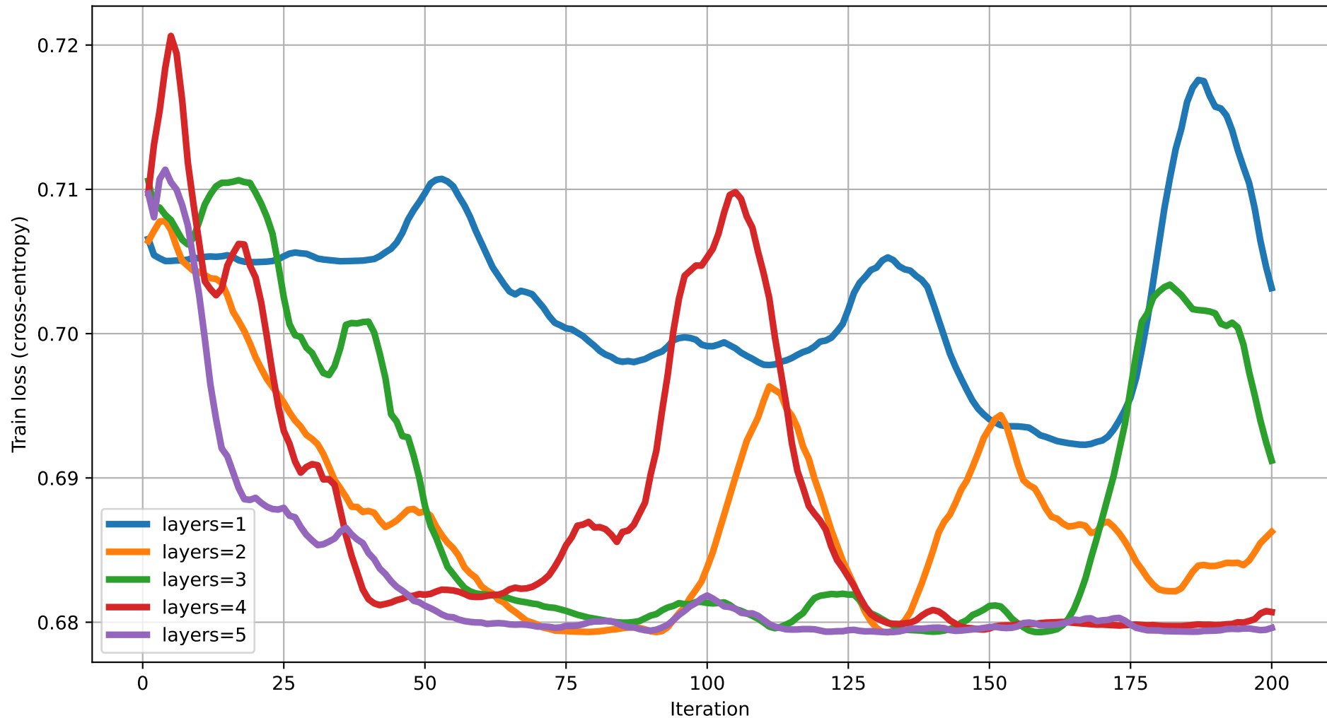
Train loss vs Iteration (dim=14) rot=RX, ent=pairwise, gate=CNOT
