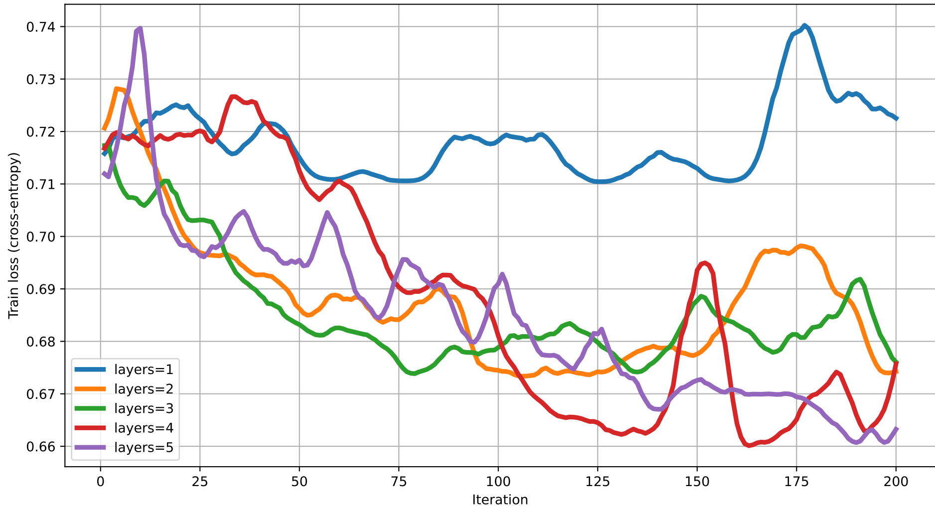
Train loss vs Iteration (dim=3) rot=RYZ, ent=full, gate=CNOT
