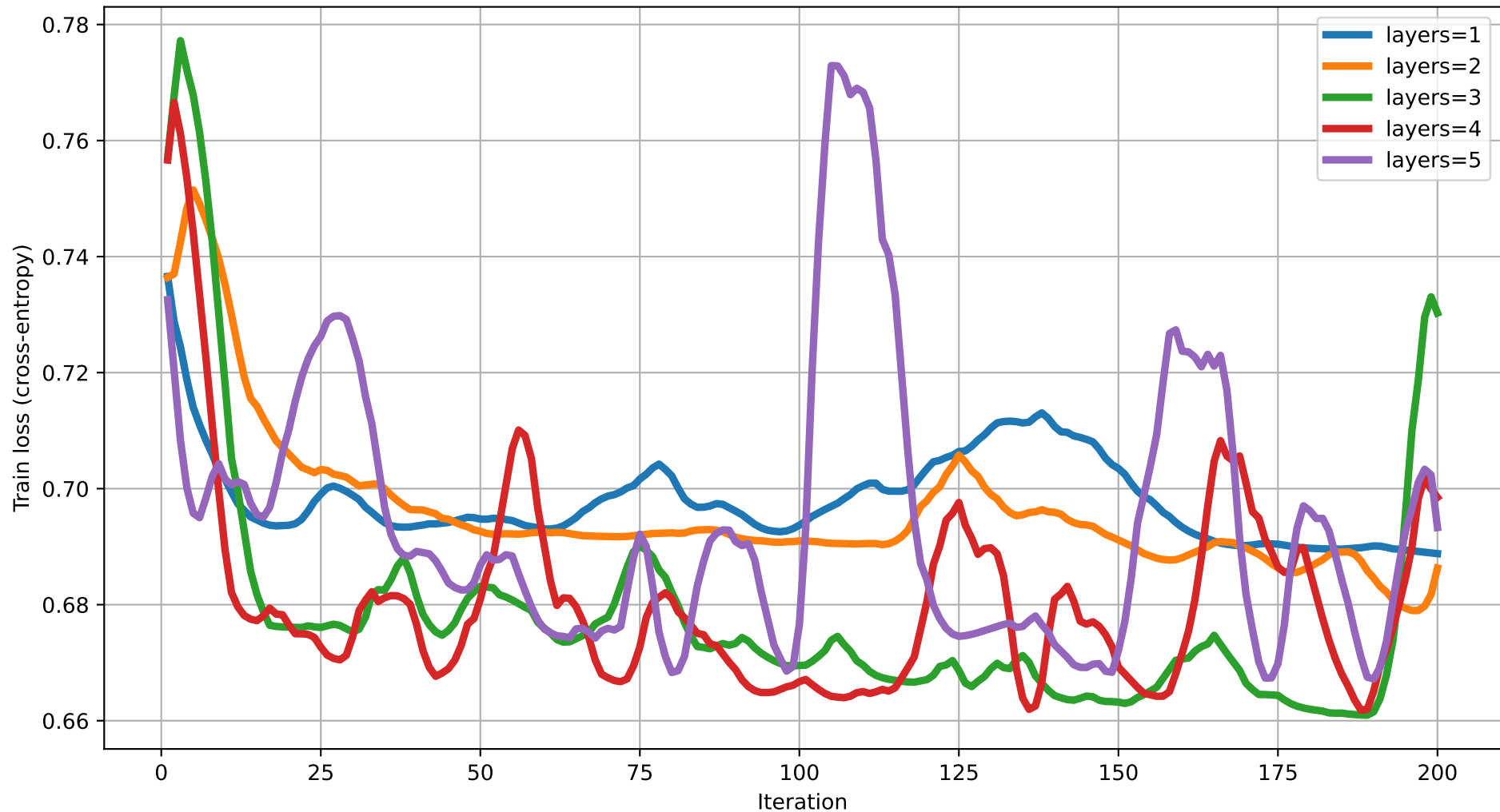
Train loss vs Iteration (dim=16) rot=RYZ, ent=chain, gate=CZ
