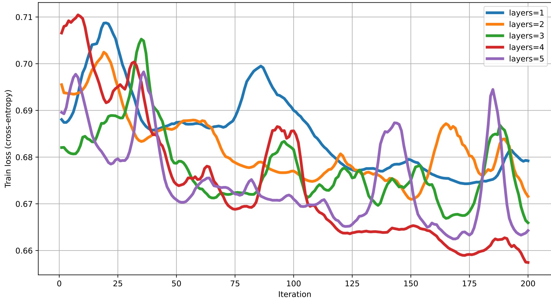
Train loss vs Iteration (dim=19) rot=RY, ent=ring, gate=CNOT
