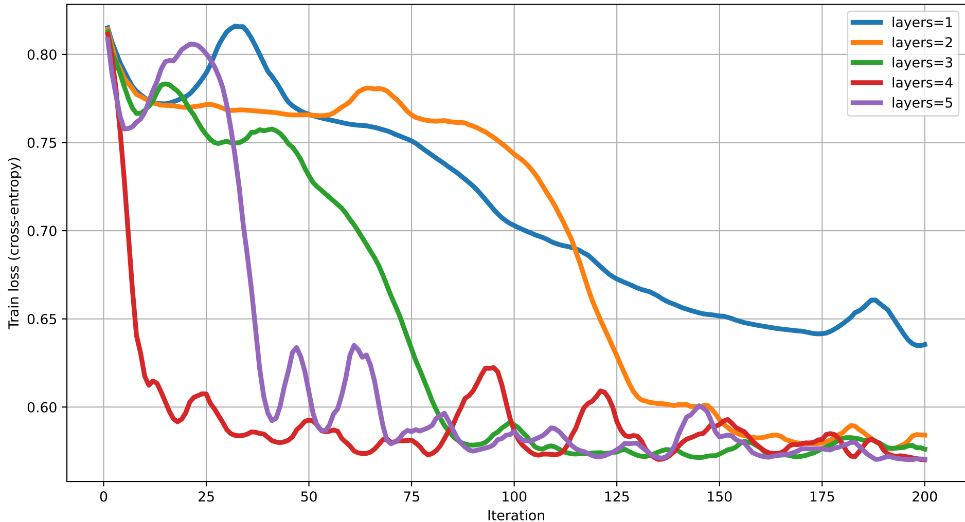
Train loss vs Iteration (dim=2) rot=RY, ent=pairwise, gate=CNOT
