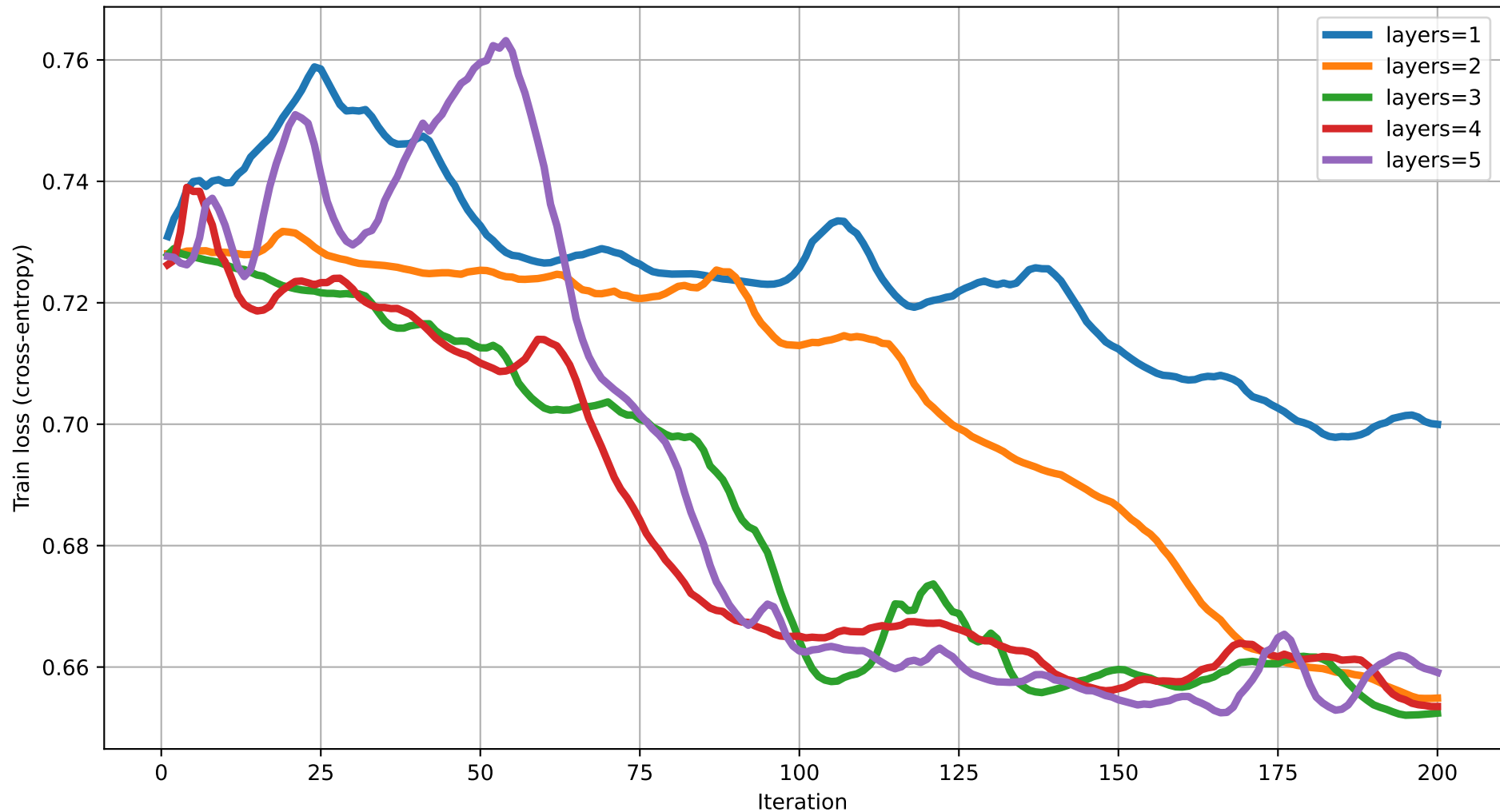
Train loss vs Iteration (dim=7) rot=RY, ent=chain, gate=CZ
