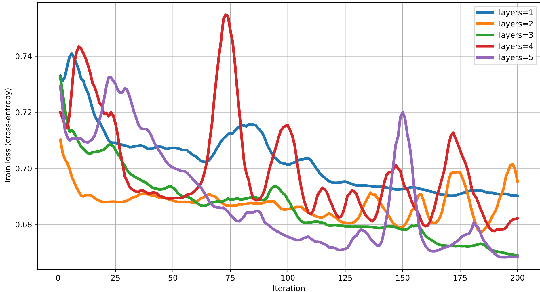
Train loss vs Iteration (dim=20) rot=RZ, ent=full, gate=IsingXX
