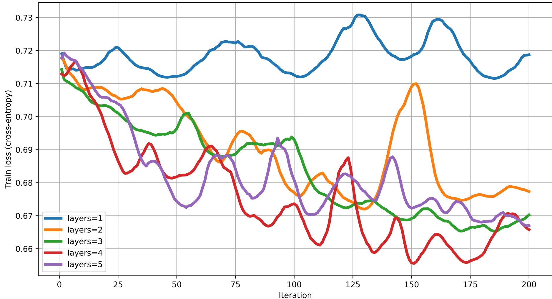
Train loss vs Iteration (dim=3) rot=RY, ent=chain, gate=CNOT
