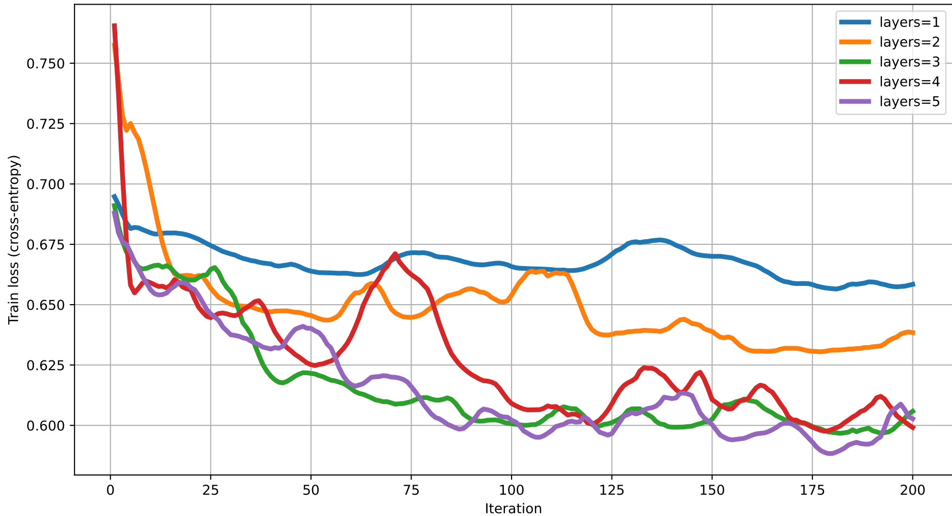
Train loss vs Iteration (dim=8) rot=RYZ, ent=ring, gate=IsingXX
