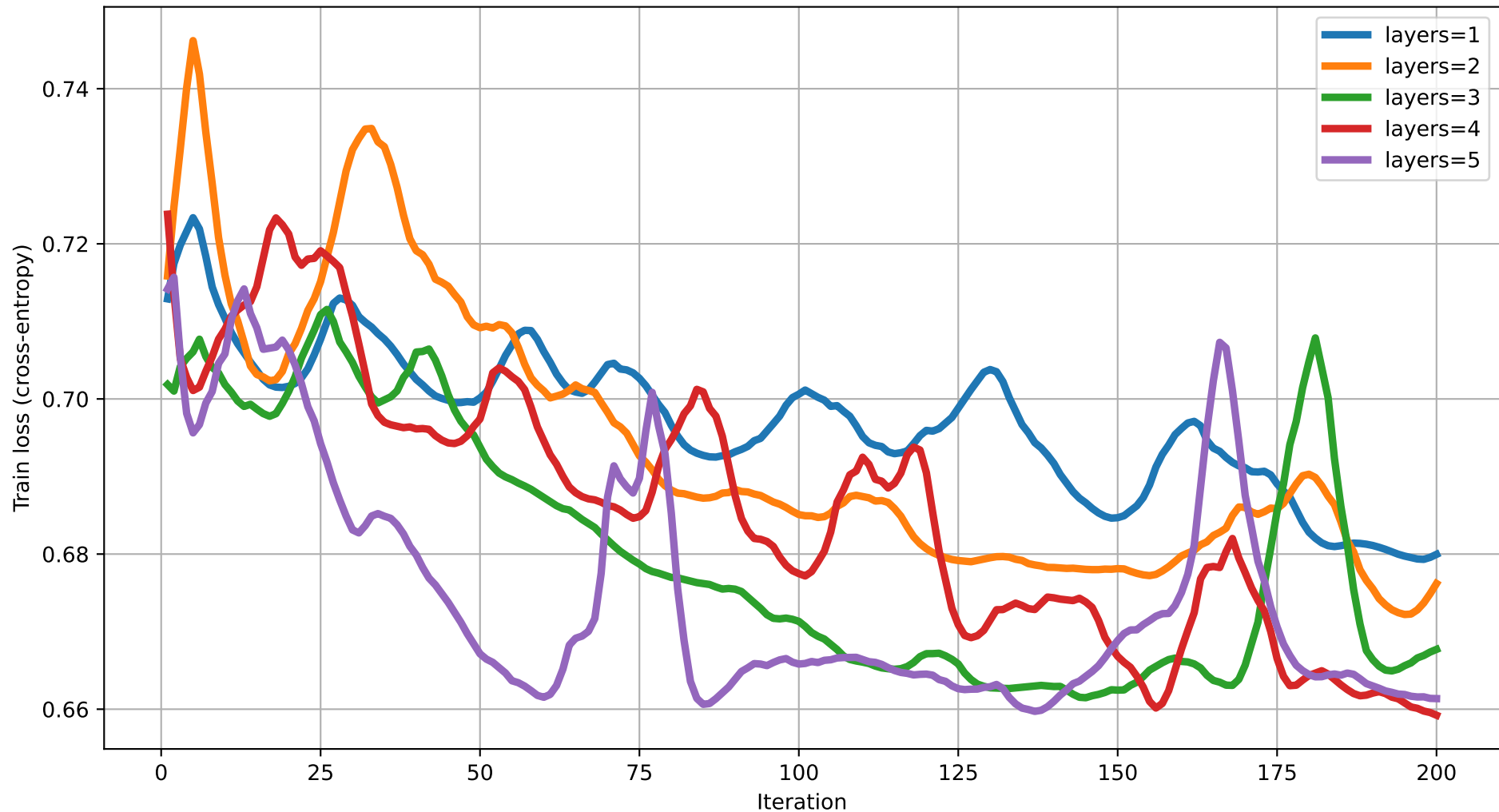
Train loss vs Iteration (dim=14) rot=RY, ent=full, gate=CNOT
