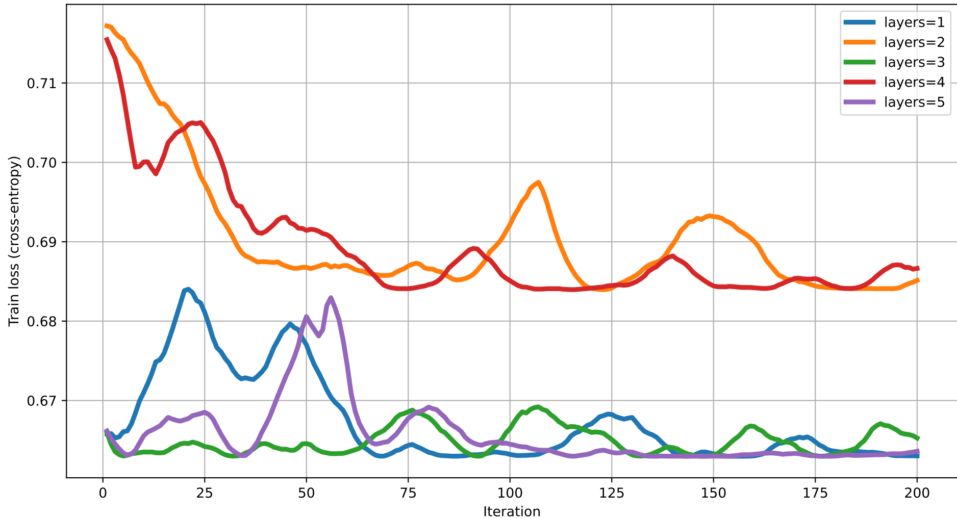
Train loss vs Iteration (dim=7) rot=RX, ent=full, gate=IsingXX
