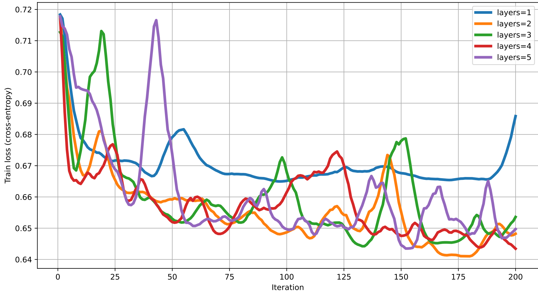
Train loss vs Iteration (dim=5) rot=RYZ, ent=full, gate=IsingXX
