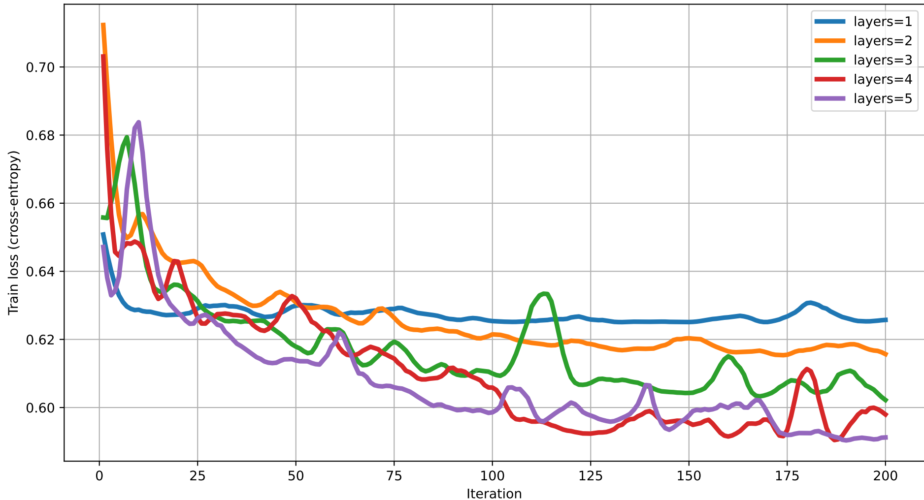
Train loss vs Iteration (degree=3) rot=RY, ent=ring, gate=IsingXX
