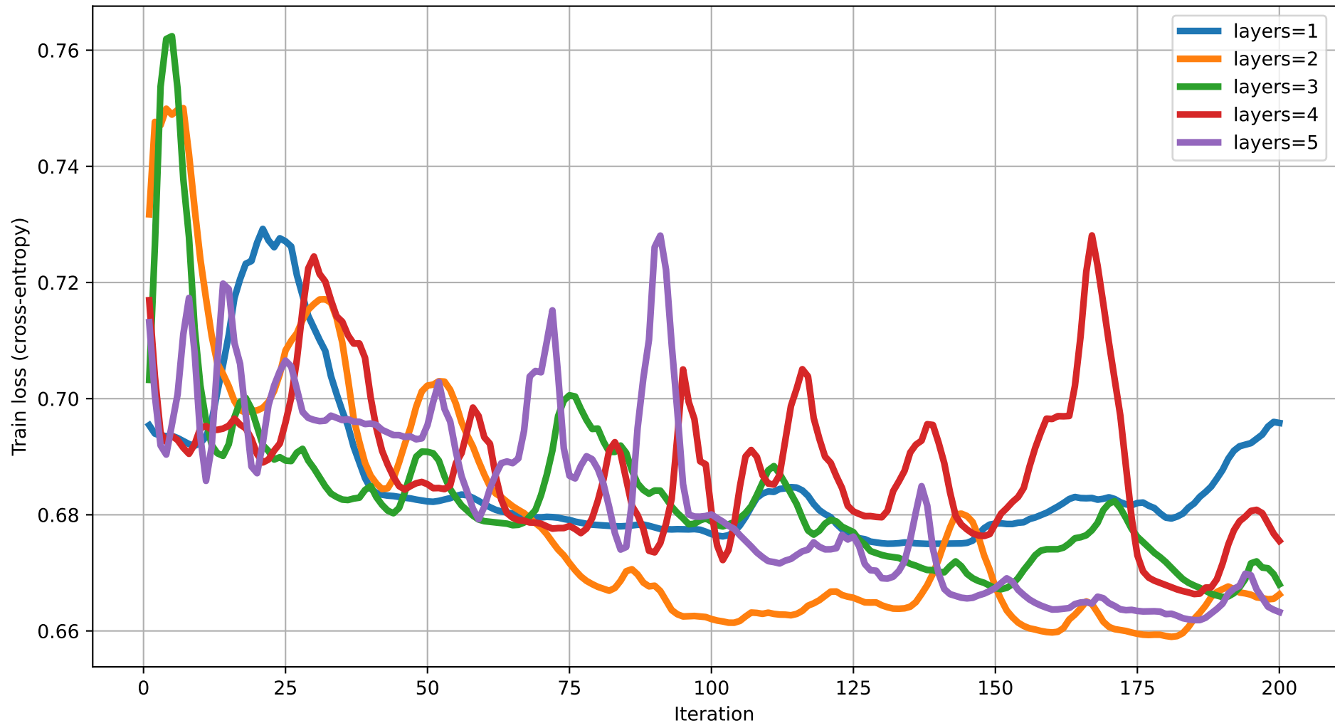
Train loss vs Iteration (dim=12) rot=Rot, ent=chain, gate=IsingXX
