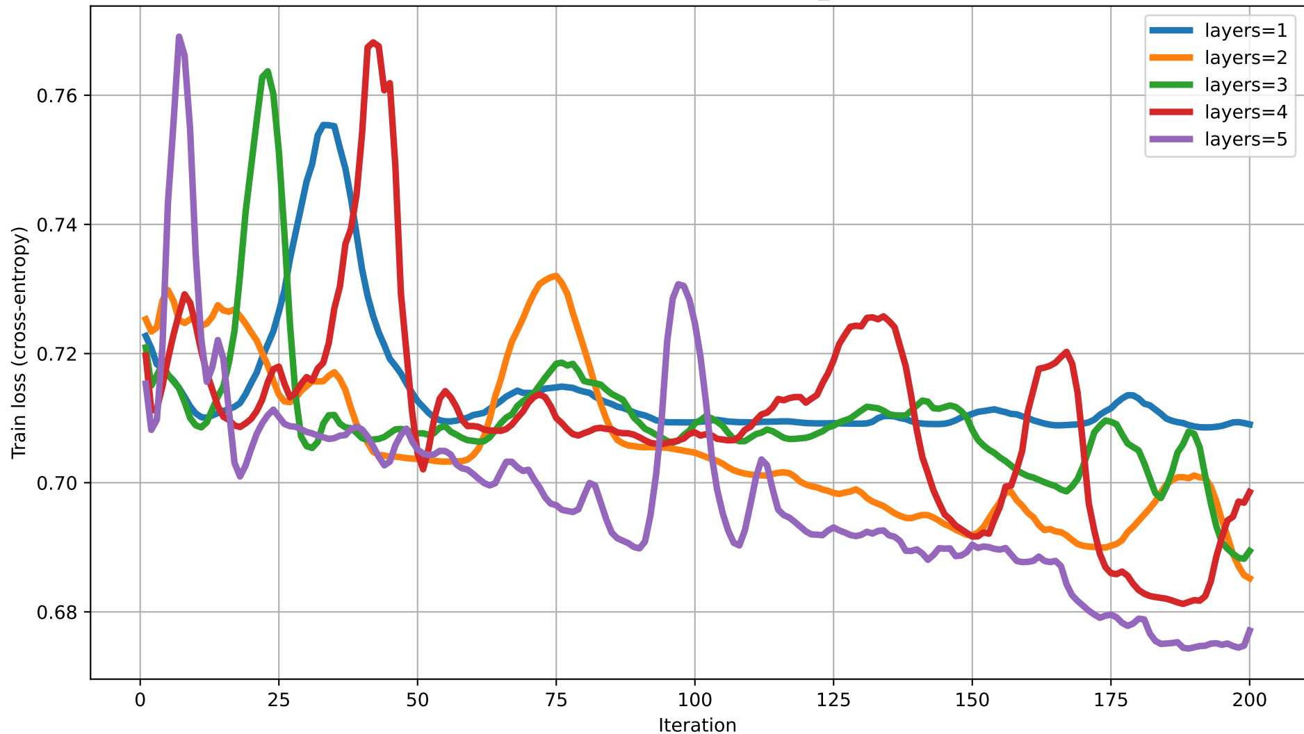
Train loss vs Iteration for different num_layers (dim=10)
