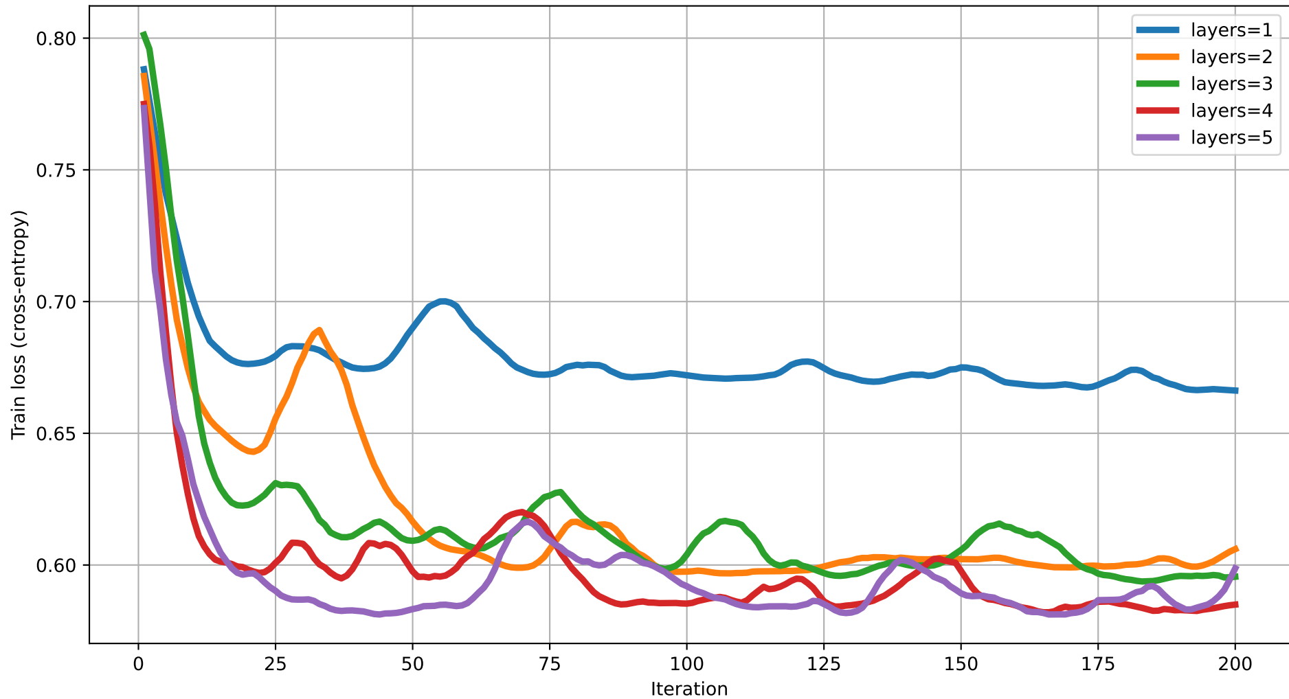
Train loss vs Iteration (dim=4) rot=RY, ent=full, gate=CNOT
