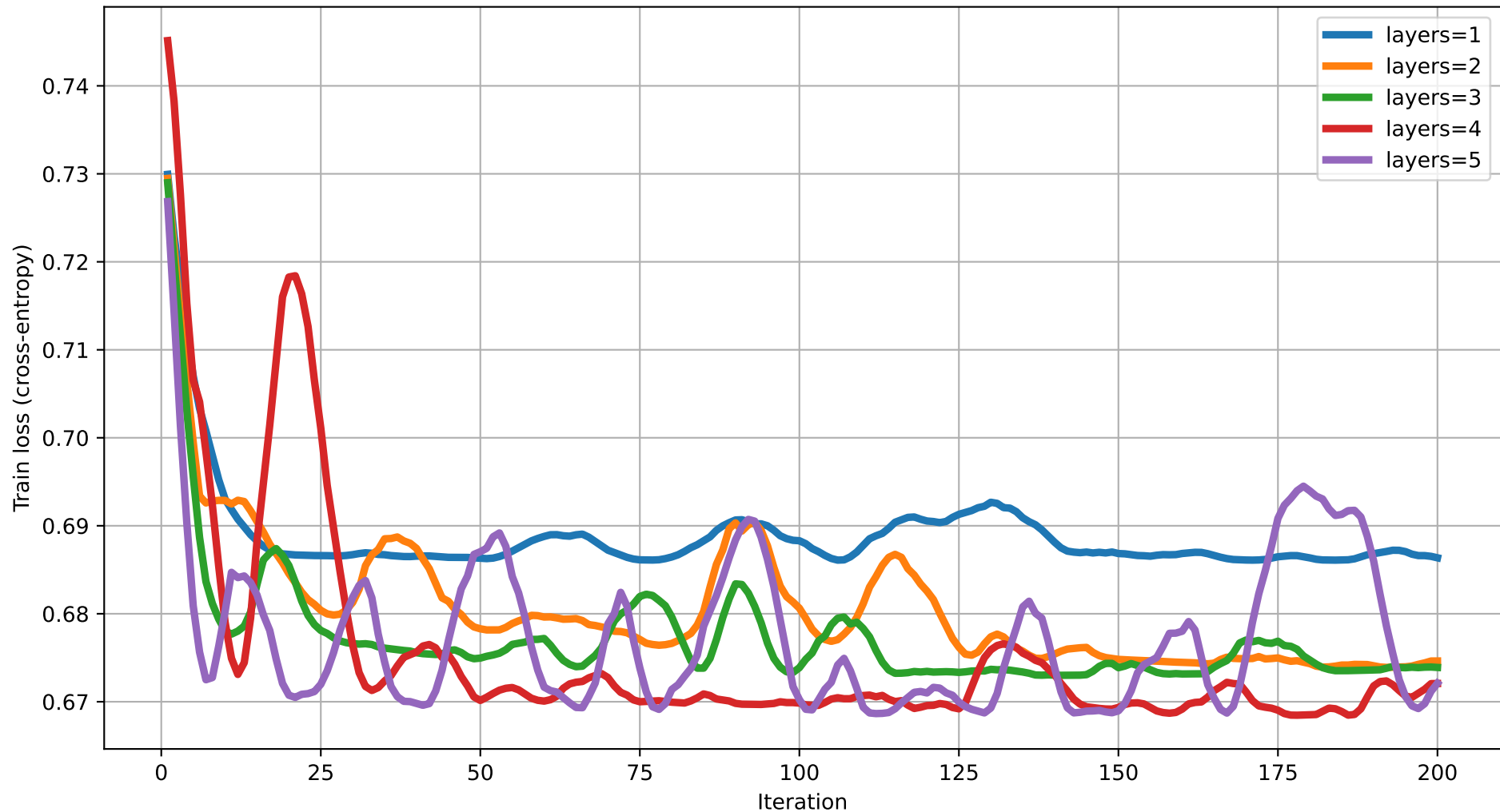
Train loss vs Iteration (degree=2) rot=RX, ent=chain, gate=CNOT
