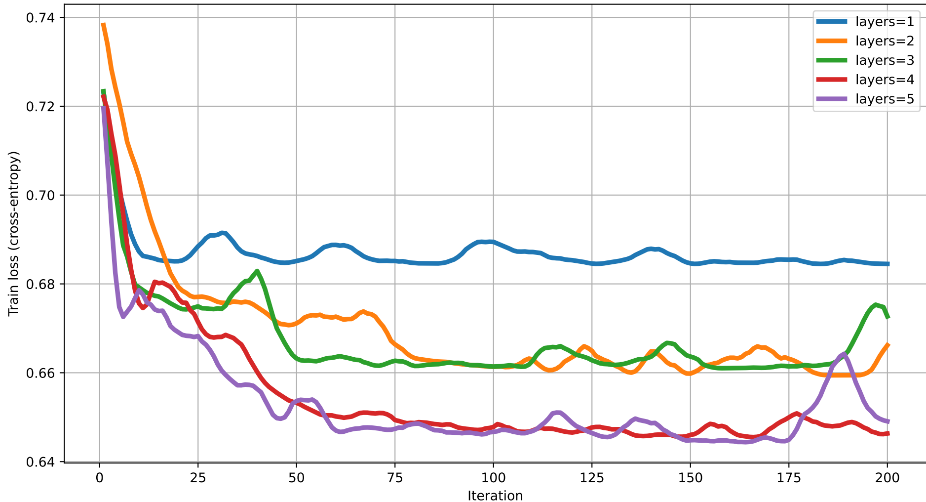
Train loss vs Iteration (degree=3) rot=RX, ent=chain, gate=CZ
