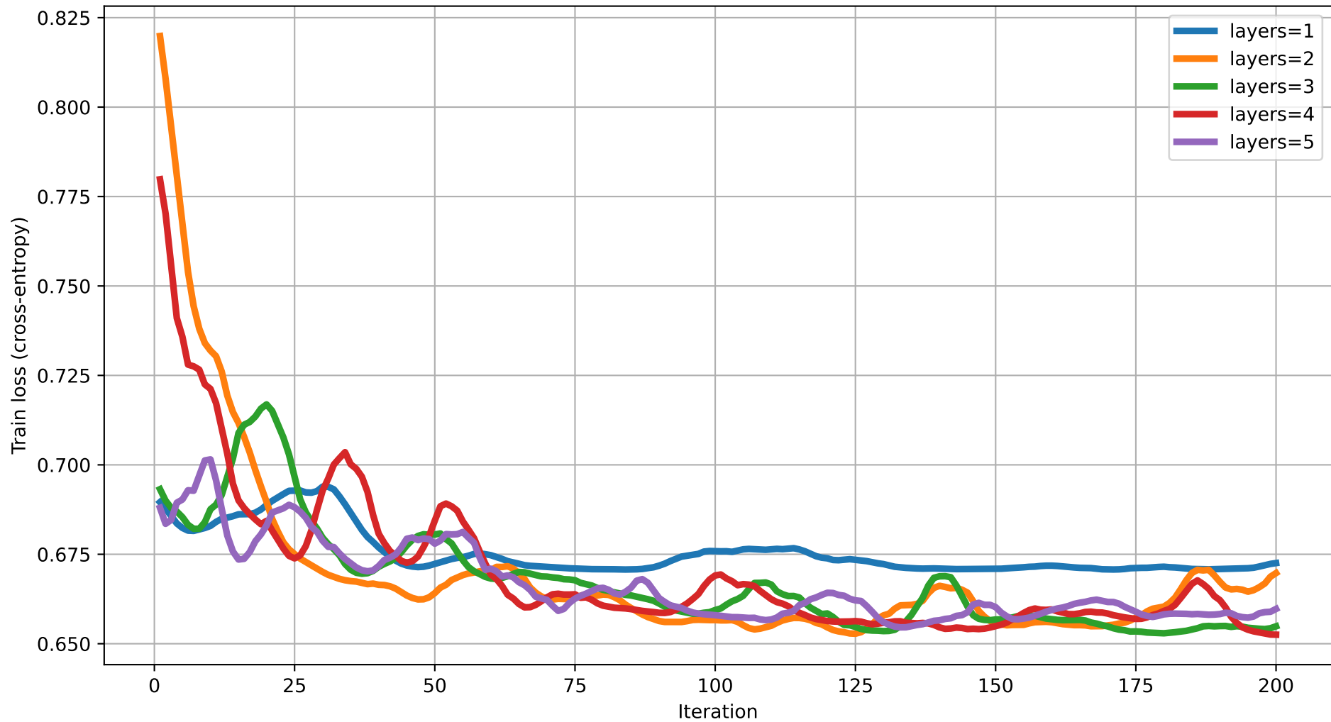
Train loss vs Iteration (dim=8) rot=RZ, ent=full, gate=IsingXX
