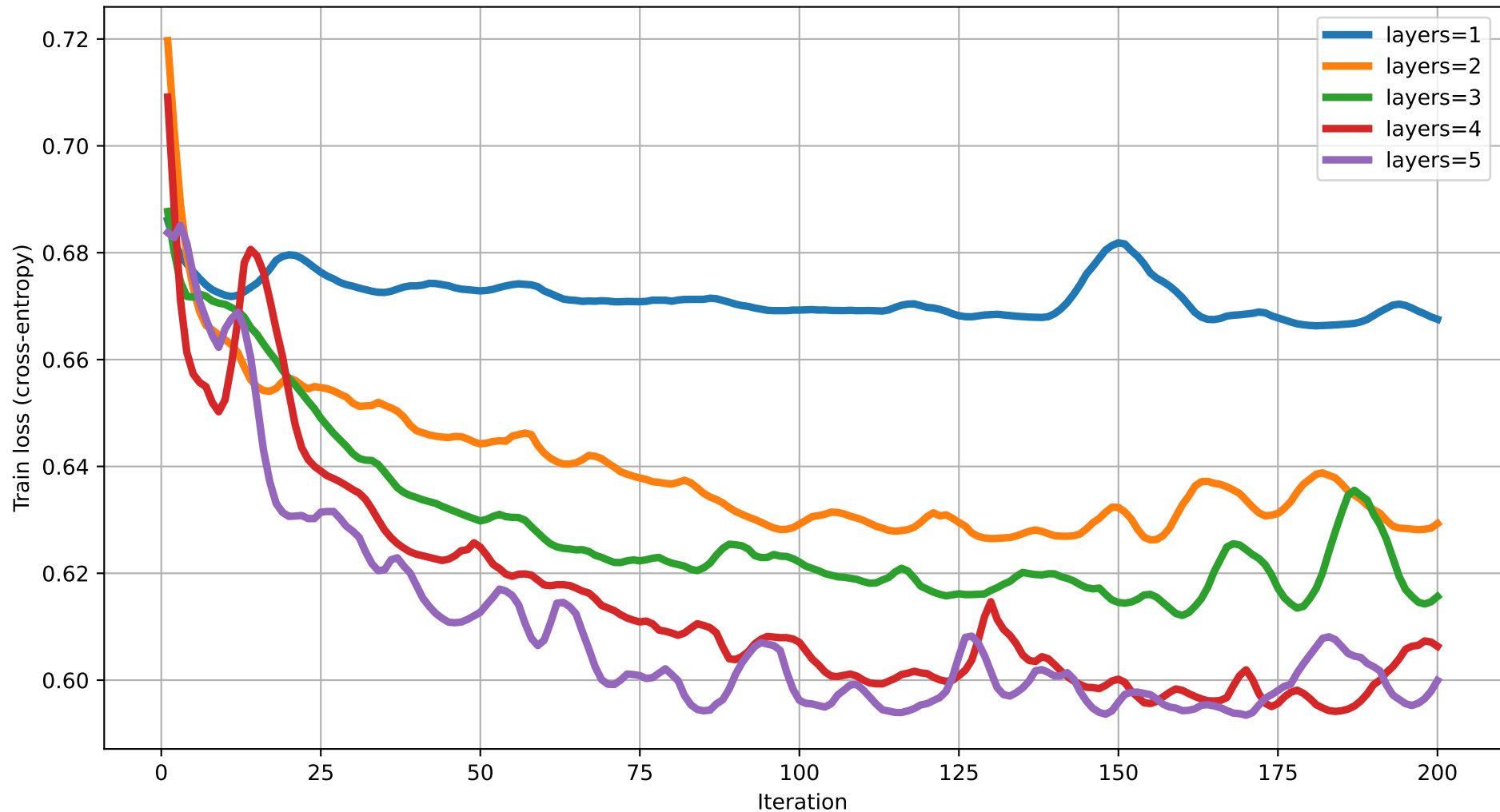
Train loss vs Iteration (degree=2) rot=RYZ, ent=ring, gate=IsingXX
