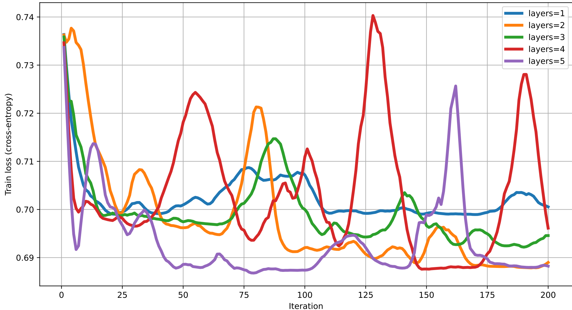
Train loss vs Iteration (dim=19) rot=RX, ent=pairwise, gate=CZ
