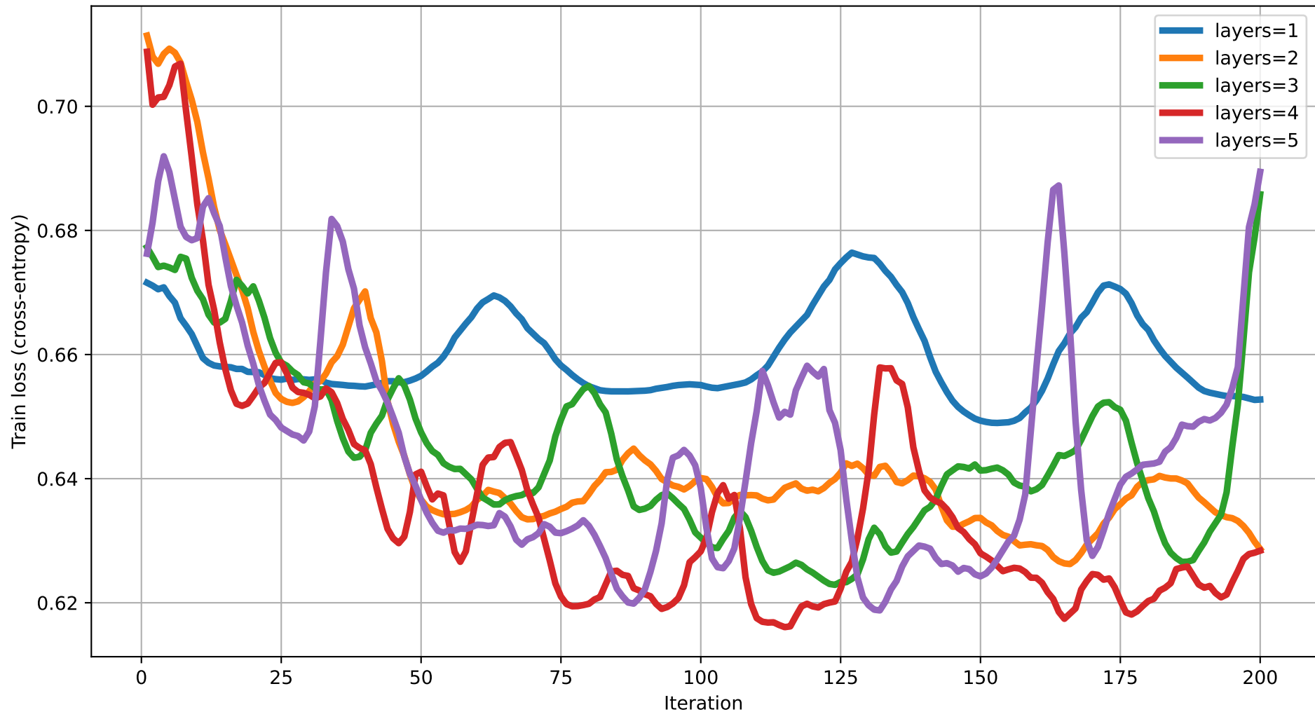
Train loss vs Iteration (dim=7) rot=Rot, ent=ring, gate=IsingXX
