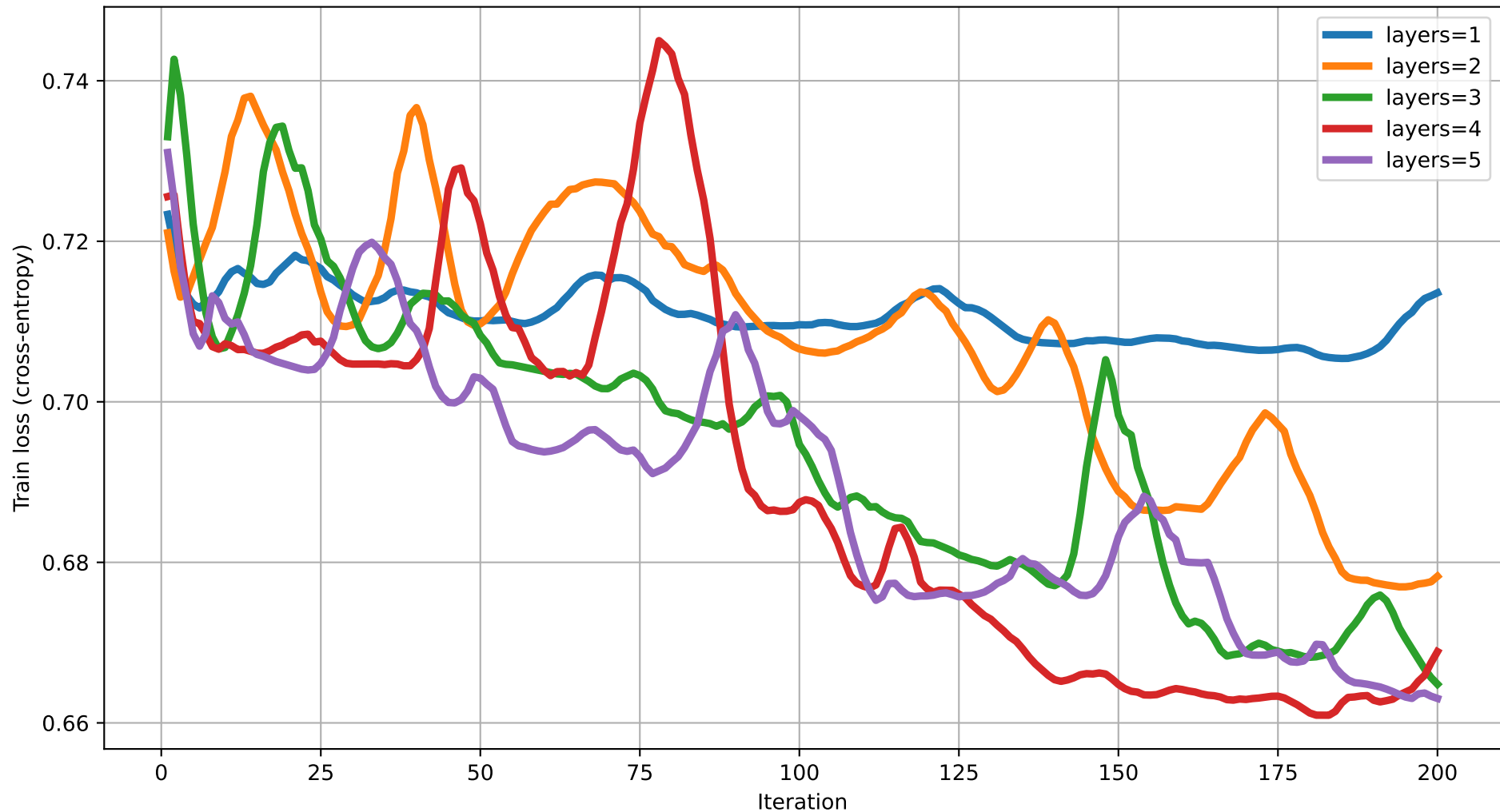
Train loss vs Iteration (dim=10) rot=RYZ, ent=chain, gate=CNOT
