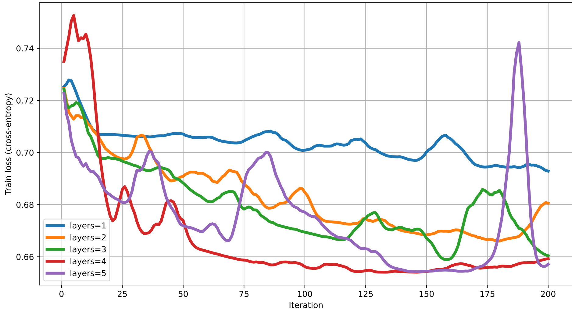
Train loss vs Iteration (dim=10) rot=RX, ent=full, gate=CNOT
