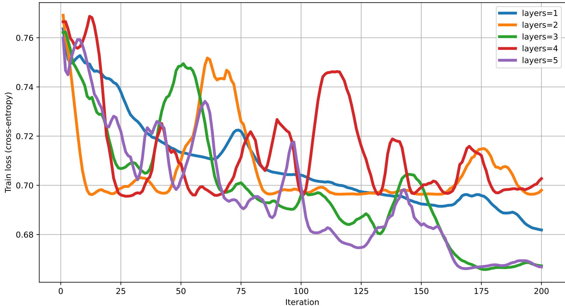
Train loss vs Iteration (dim=17) rot=RX, ent=full, gate=IsingXX
