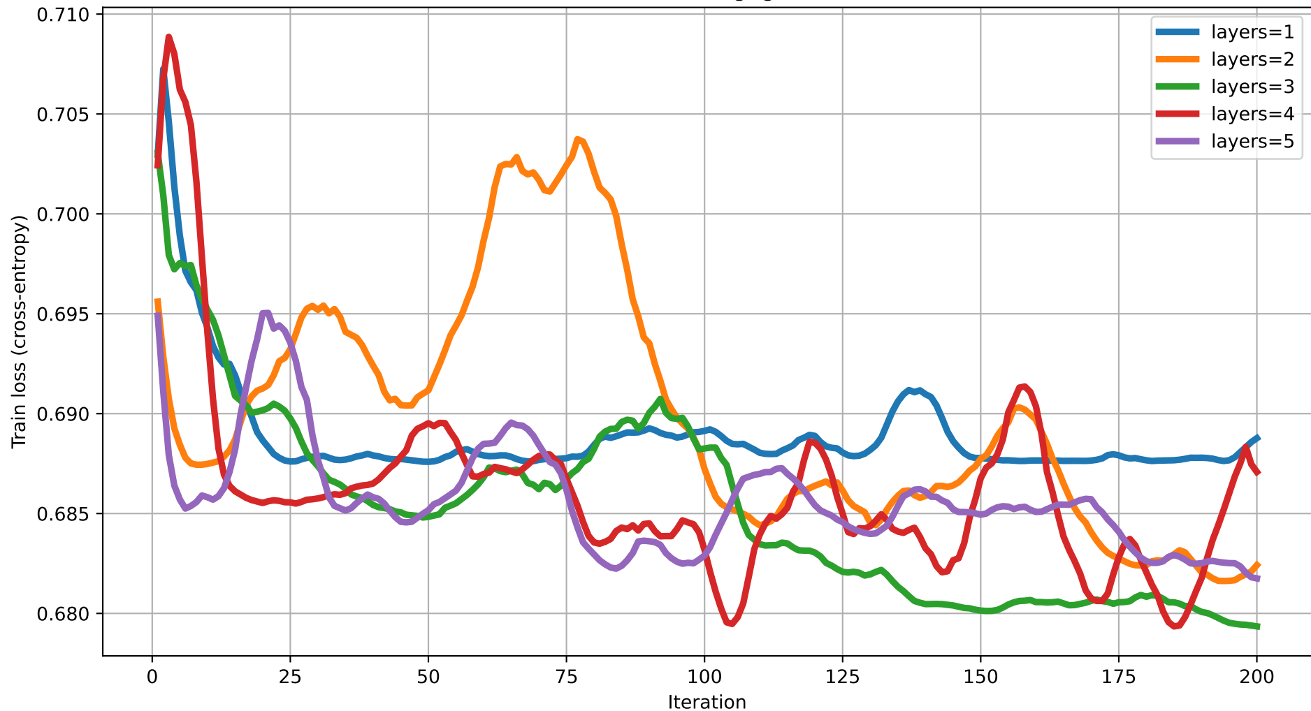
Train loss vs Iteration (dim=13) rot=RX, ent=ring, gate=CZ
