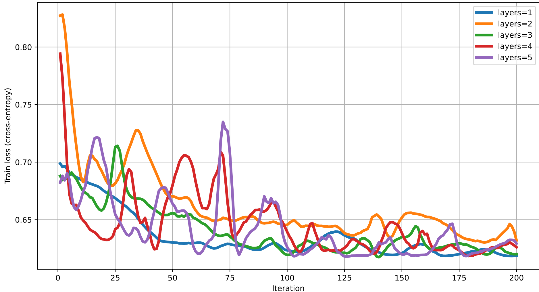
Train loss vs Iteration (dim=4) rot=Rot, ent=pairwise, gate=IsingXX
