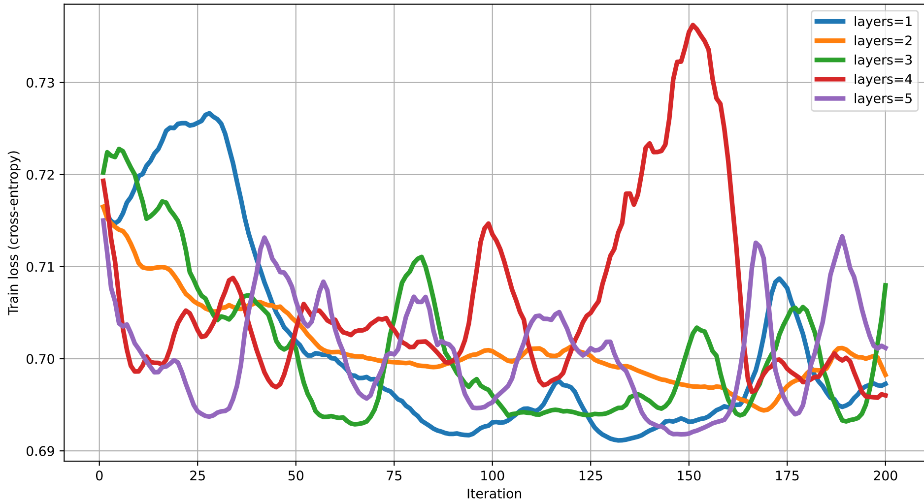
Train loss vs Iteration (dim=3) rot=RX, ent=pairwise, gate=CNOT
