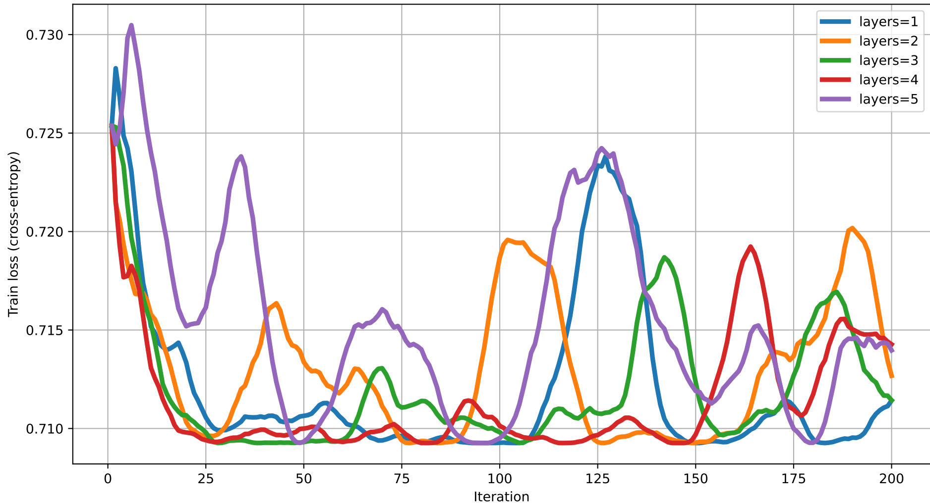
Train loss vs Iteration (dim=10) rot=RZ, ent=chain, gate=CNOT
