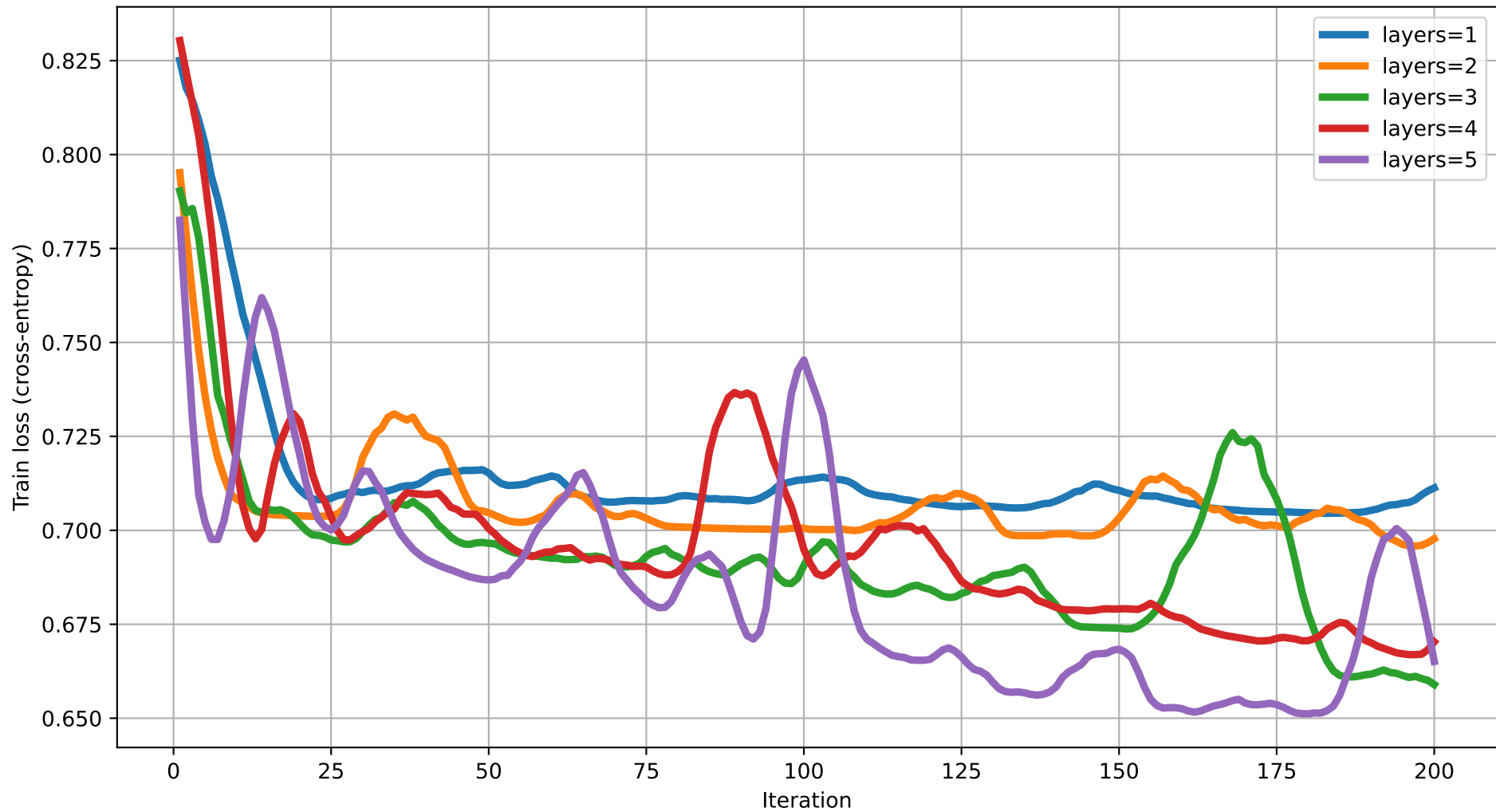
Train loss vs Iteration (dim=8) rot=RY, ent=full, gate=CNOT
