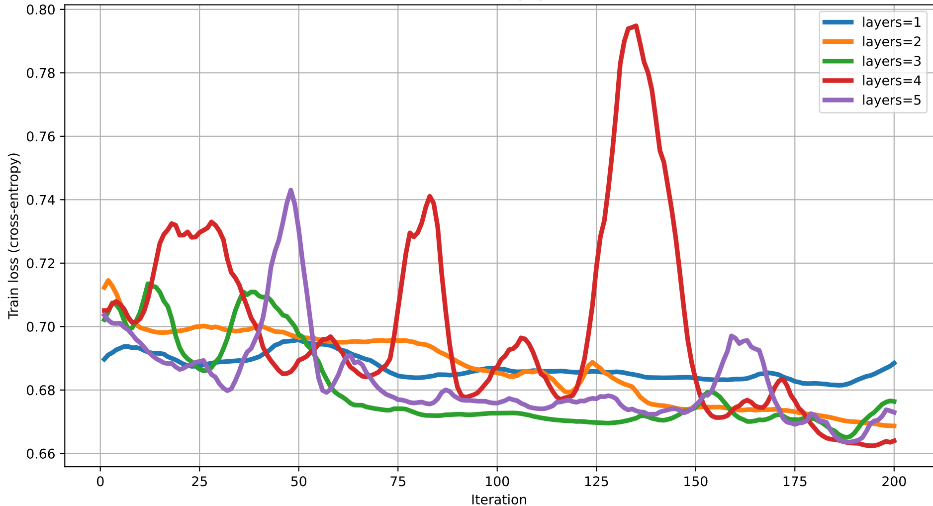
Train loss vs Iteration (dim=13) rot=RYZ, ent=ring, gate=CNOT
