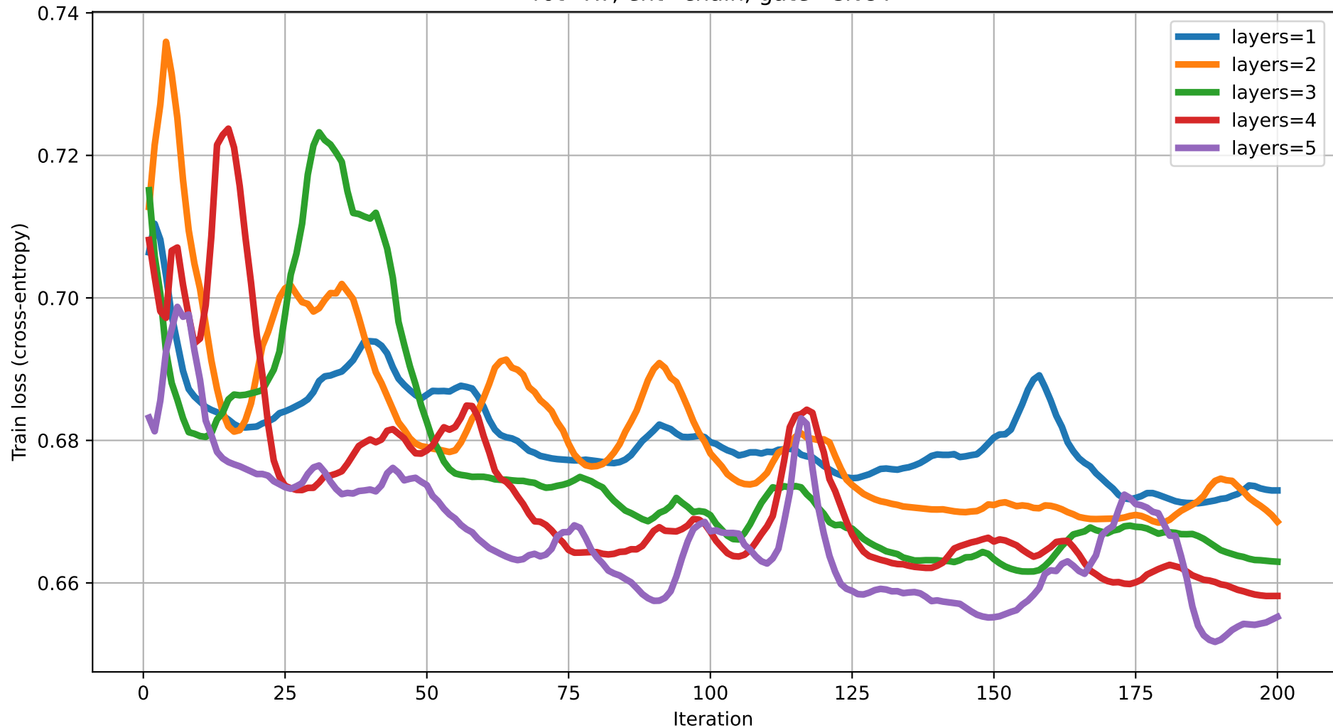
Train loss vs Iteration (dim=13) rot=RY, ent=chain, gate=CNOT
