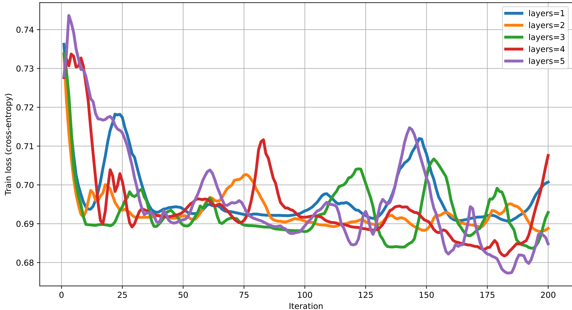
Train loss vs Iteration (dim=16) rot=Rot, ent=full, gate=CNOT
