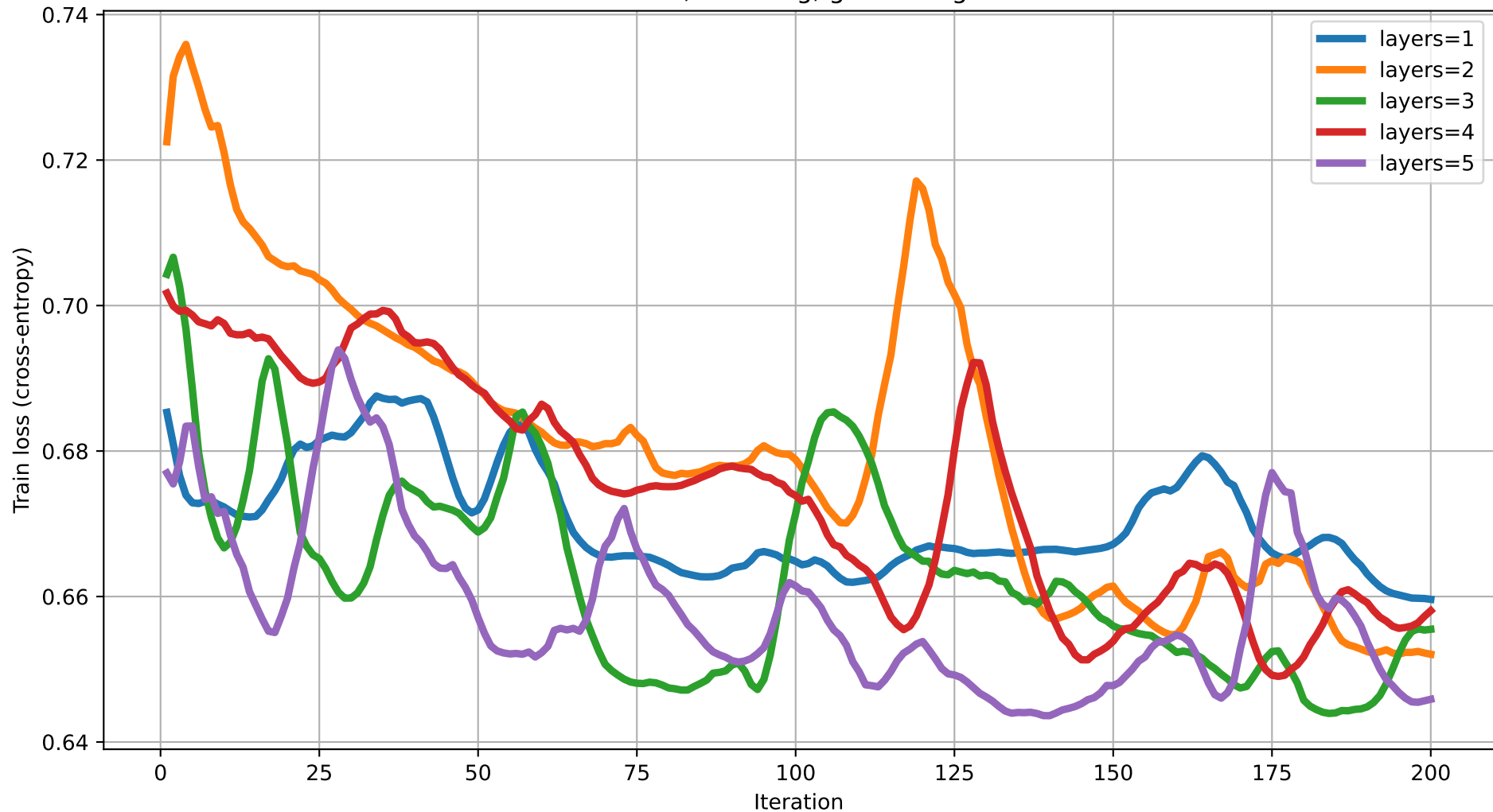
Train loss vs Iteration (dim=6) rot=RY, ent=ring, gate=IsingXX
