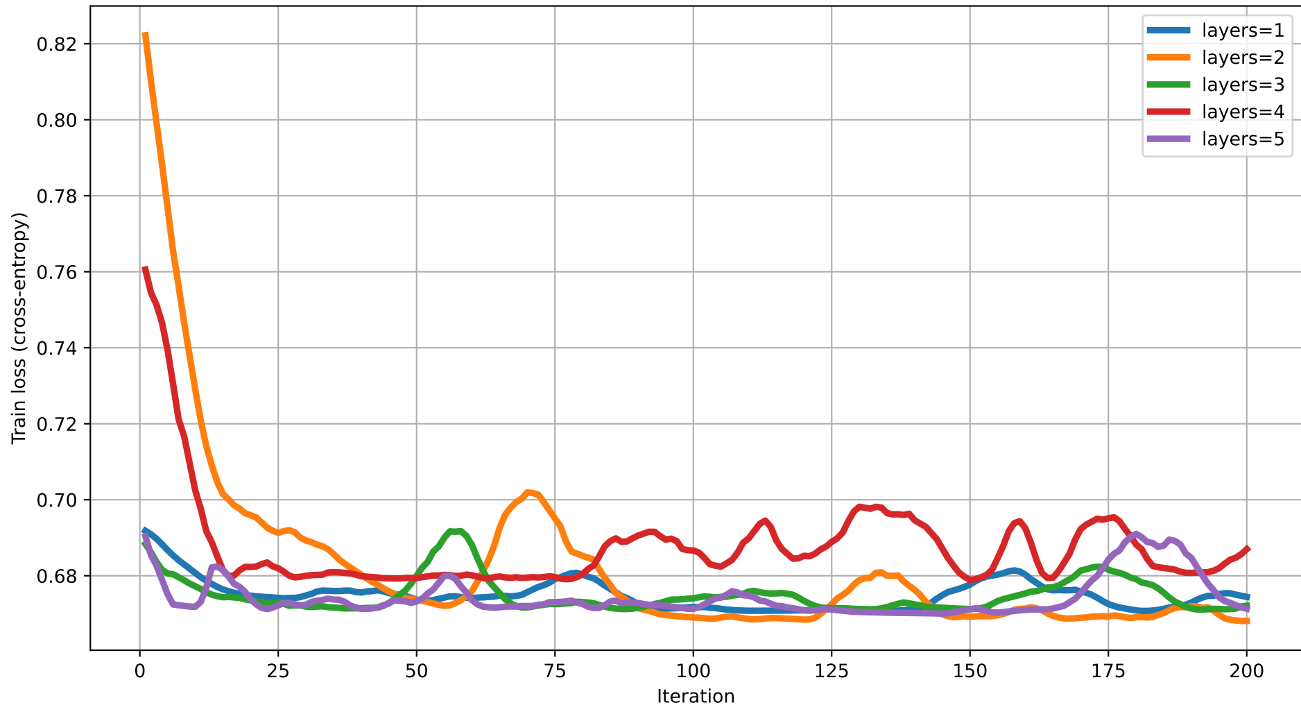
Train loss vs Iteration (dim=8) rot=RZ, ent=pairwise, gate=IsingXX
