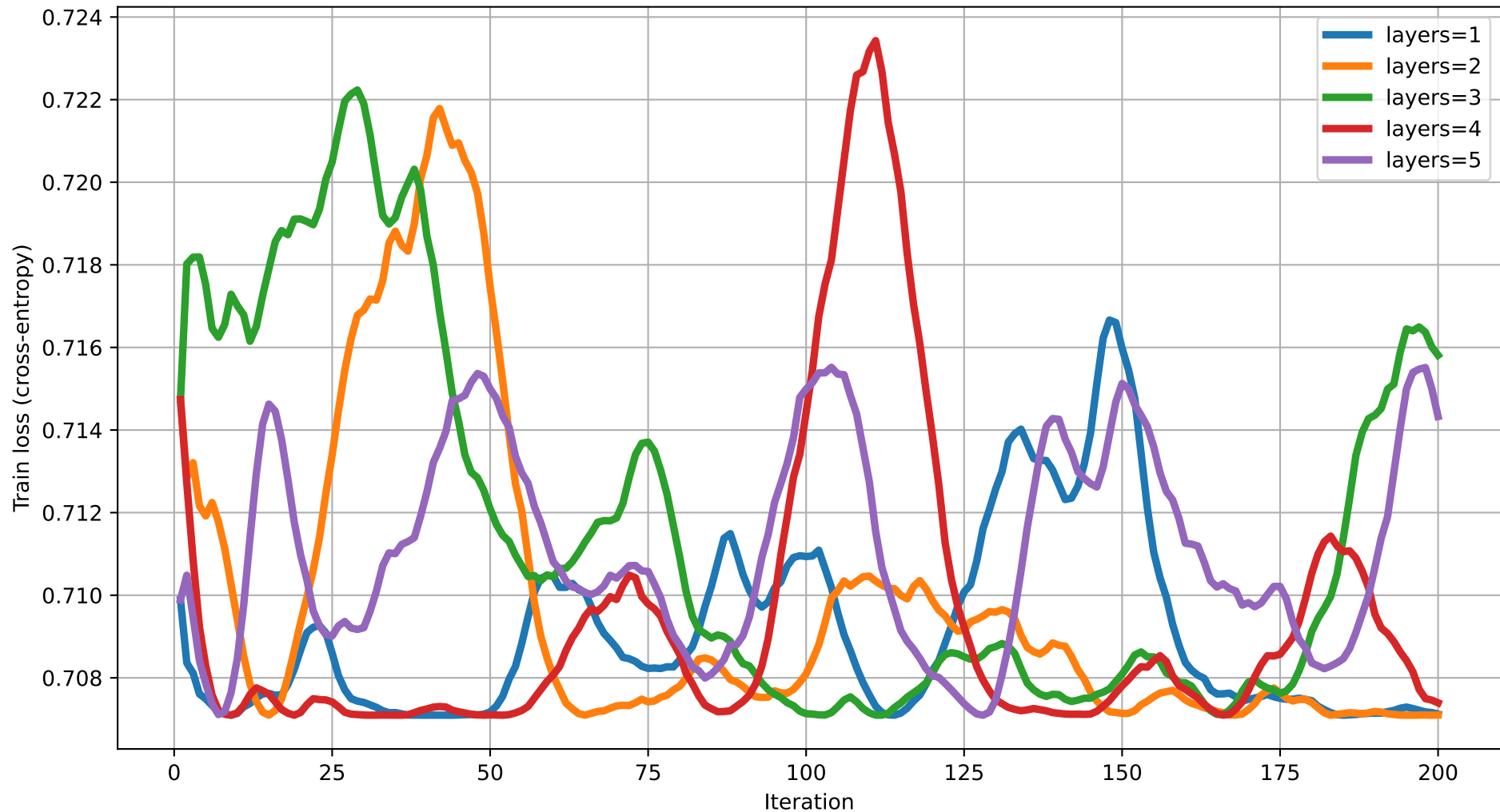
Train loss vs Iteration (dim=6) rot=RZ, ent=pairwise, gate=CZ
