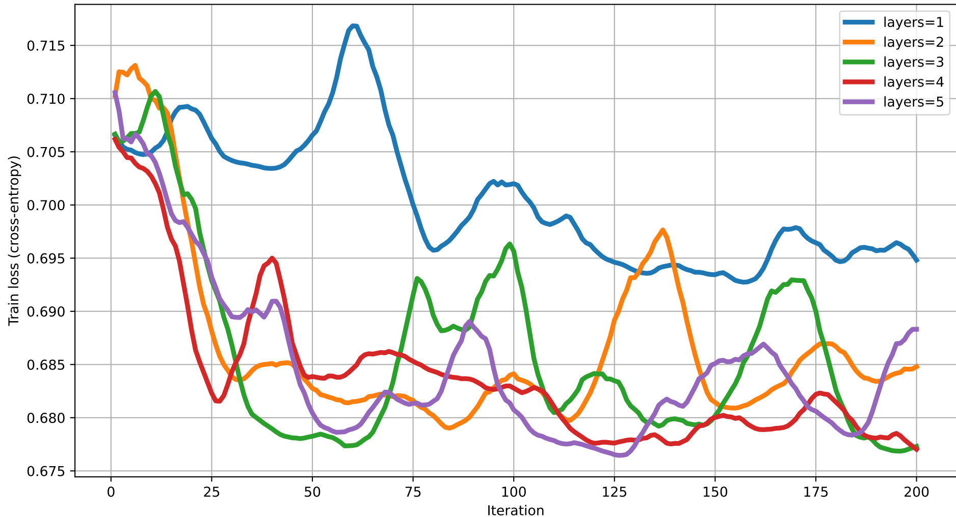
Train loss vs Iteration (dim=14) rot=RX, ent=ring, gate=CZ
