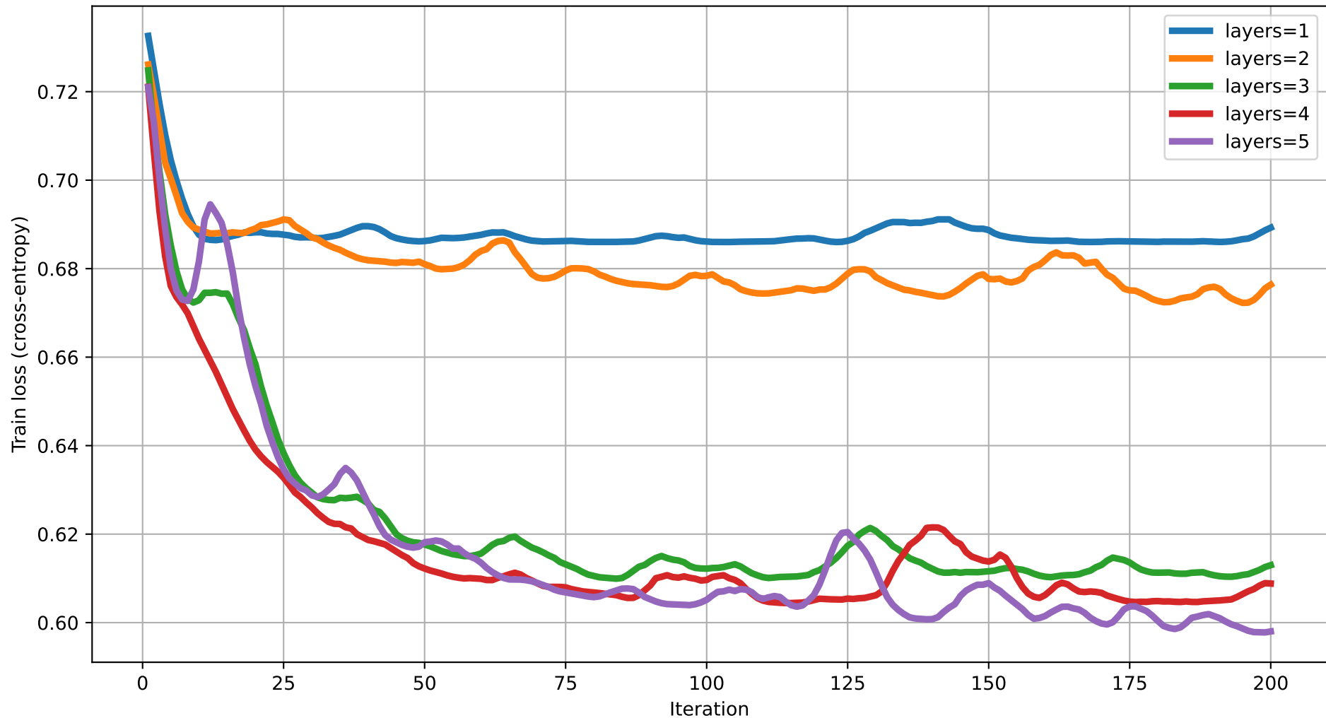
Train loss vs Iteration (degree=2) rot=RY, ent=chain, gate=CNOT
