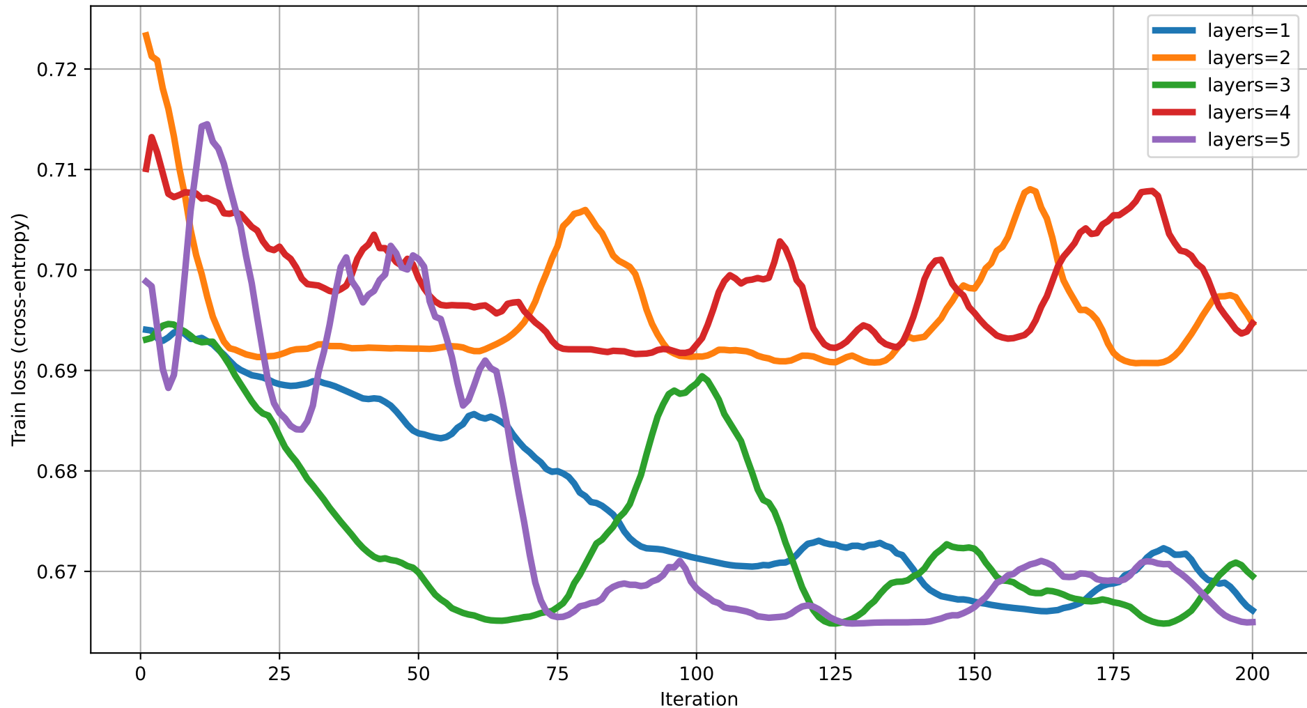
Train loss vs Iteration (dim=12) rot=RX, ent=full, gate=IsingXX
