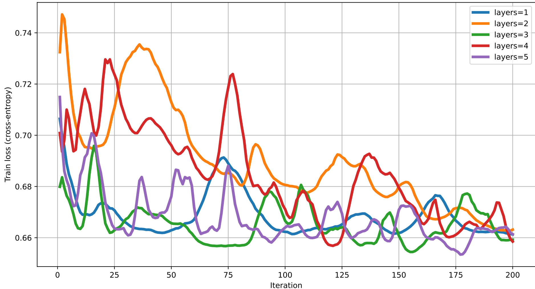
Train loss vs Iteration (dim=11) rot=Rot, ent=ring, gate=IsingXX
