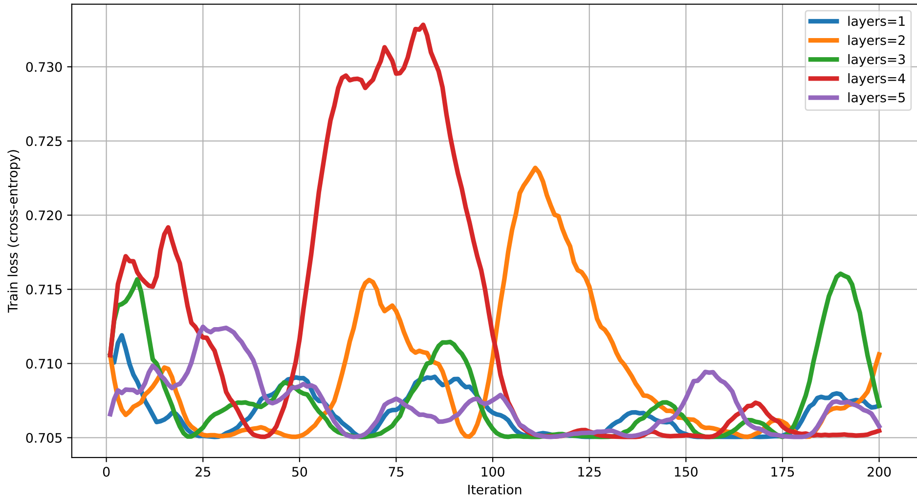
Train loss vs Iteration (dim=14) rot=RZ, ent=full, gate=CNOT
