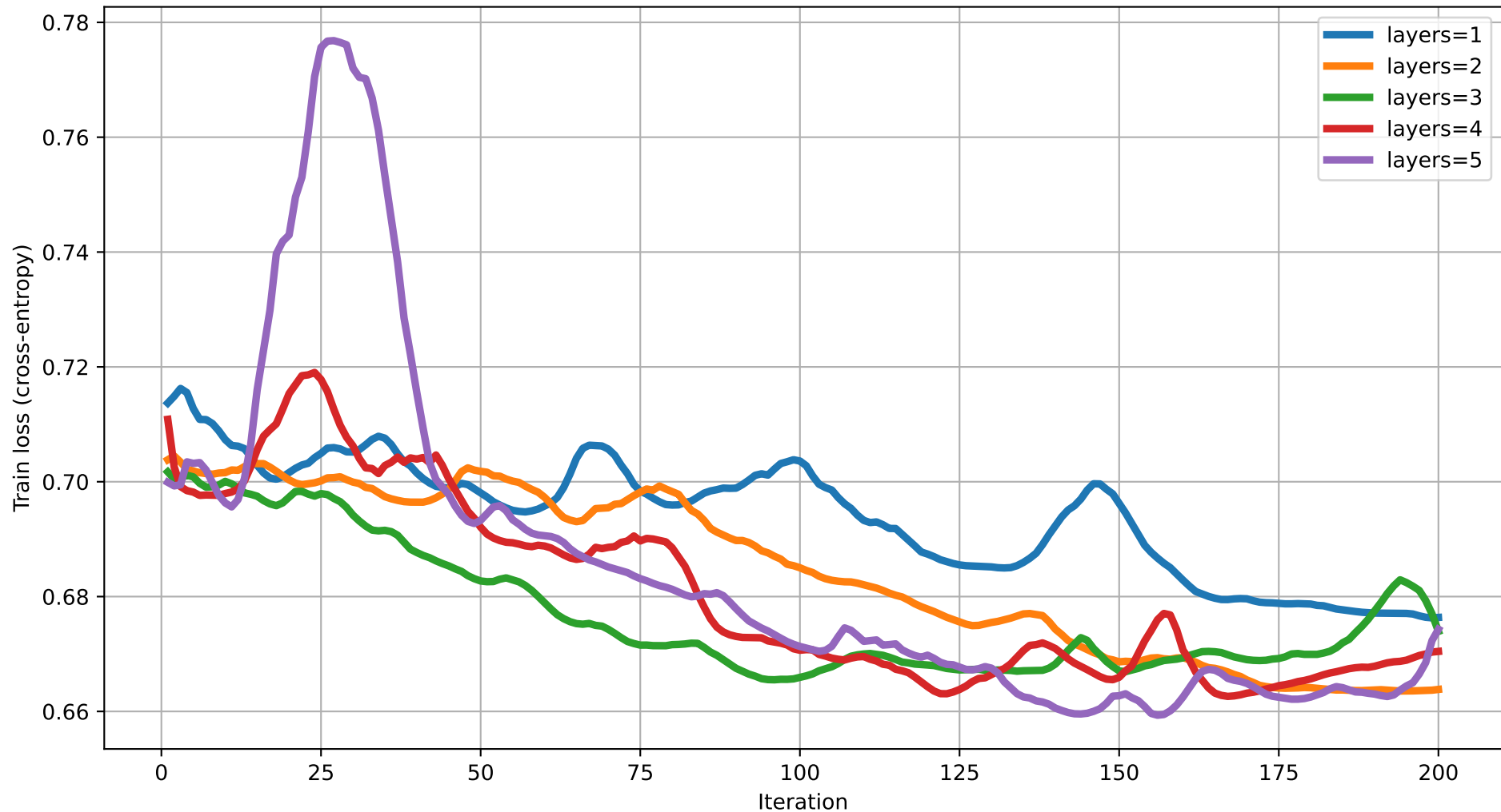
Train loss vs Iteration (dim=14) rot=RY, ent=chain, gate=CNOT
