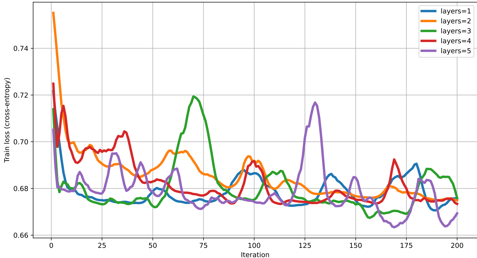
Train loss vs Iteration (dim=18) rot=RYZ, ent=ring, gate=IsingXX
