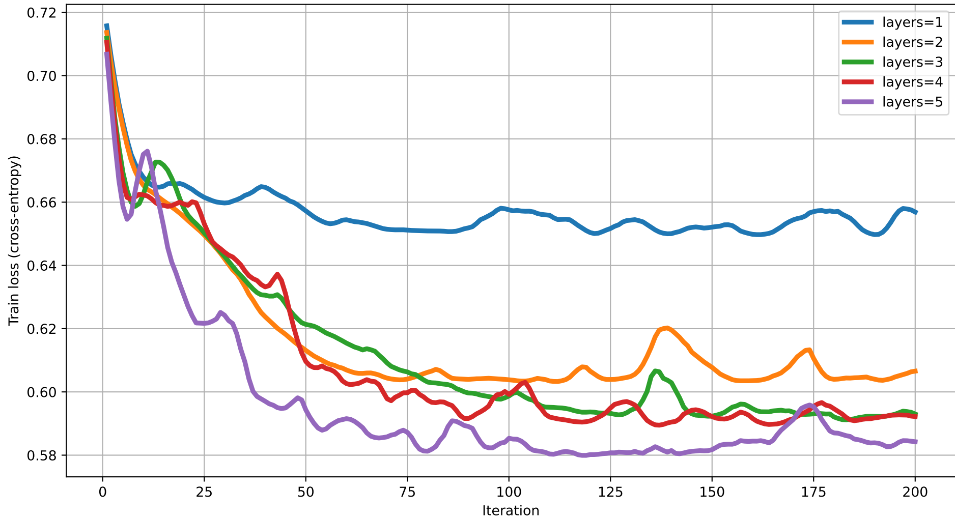
Train loss vs Iteration (degree=4) rot=RYZ, ent=full, gate=CZ
