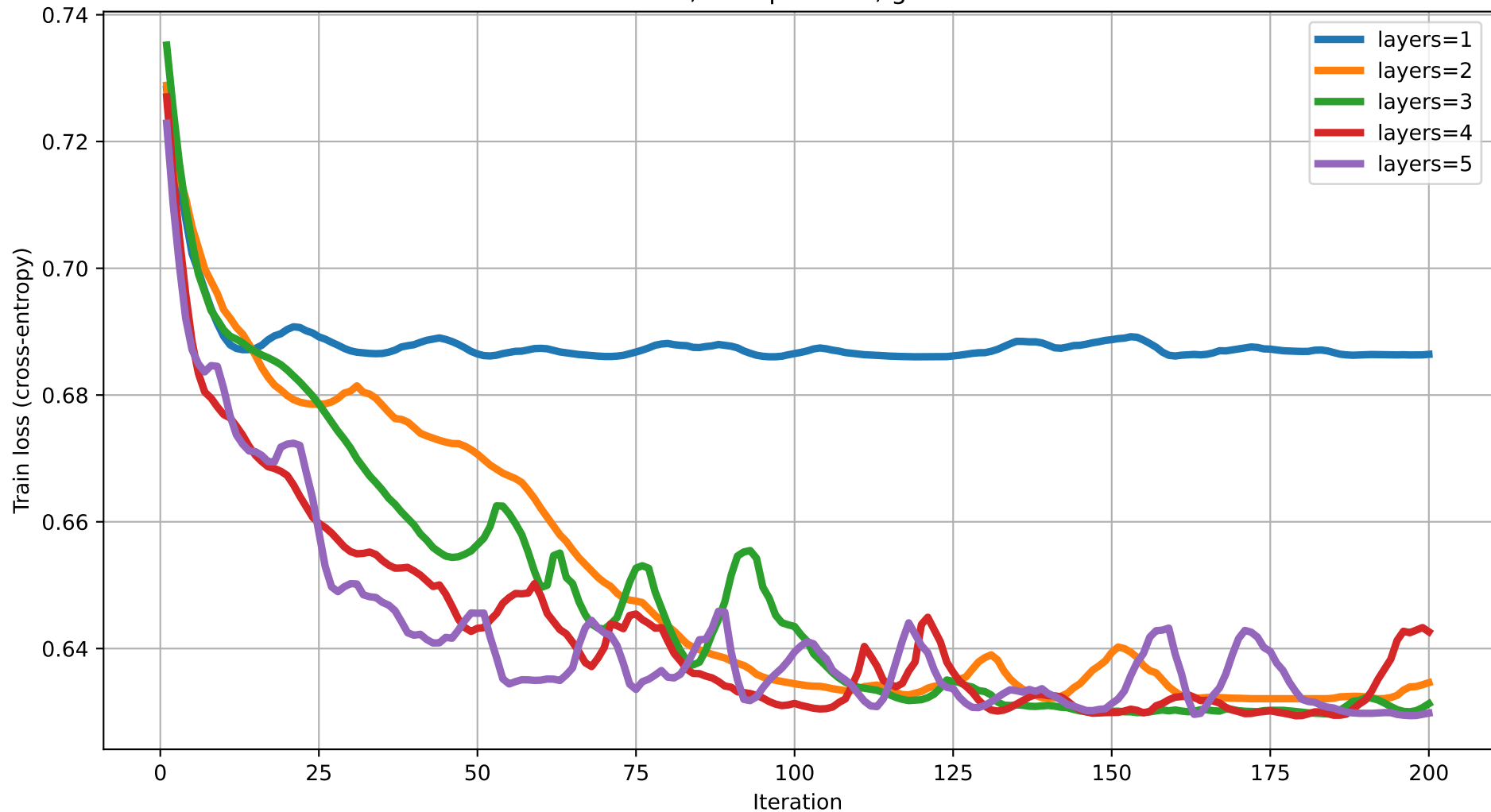
Train loss vs Iteration (degree=2) rot=Rot, ent=pairwise, gate=CZ
