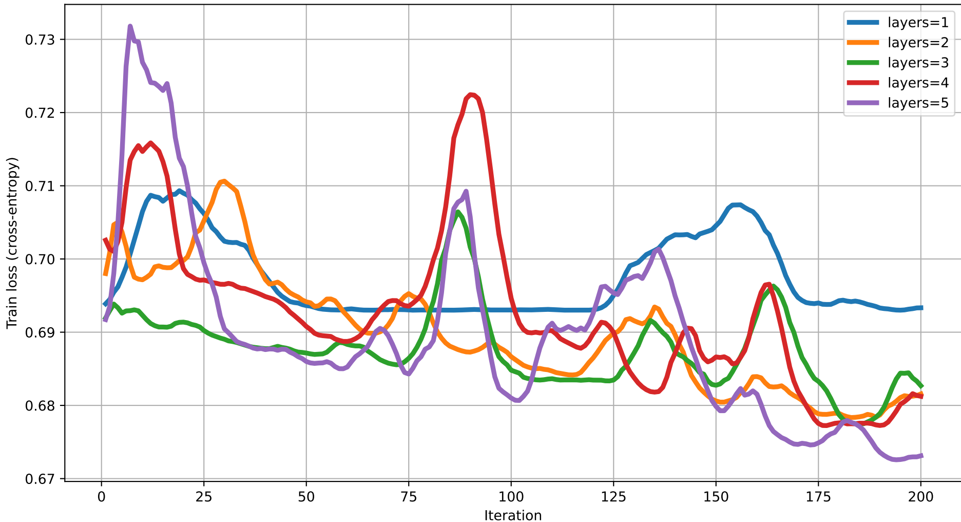
Train loss vs Iteration (dim=14) rot=RY, ent=pairwise, gate=IsingXX
