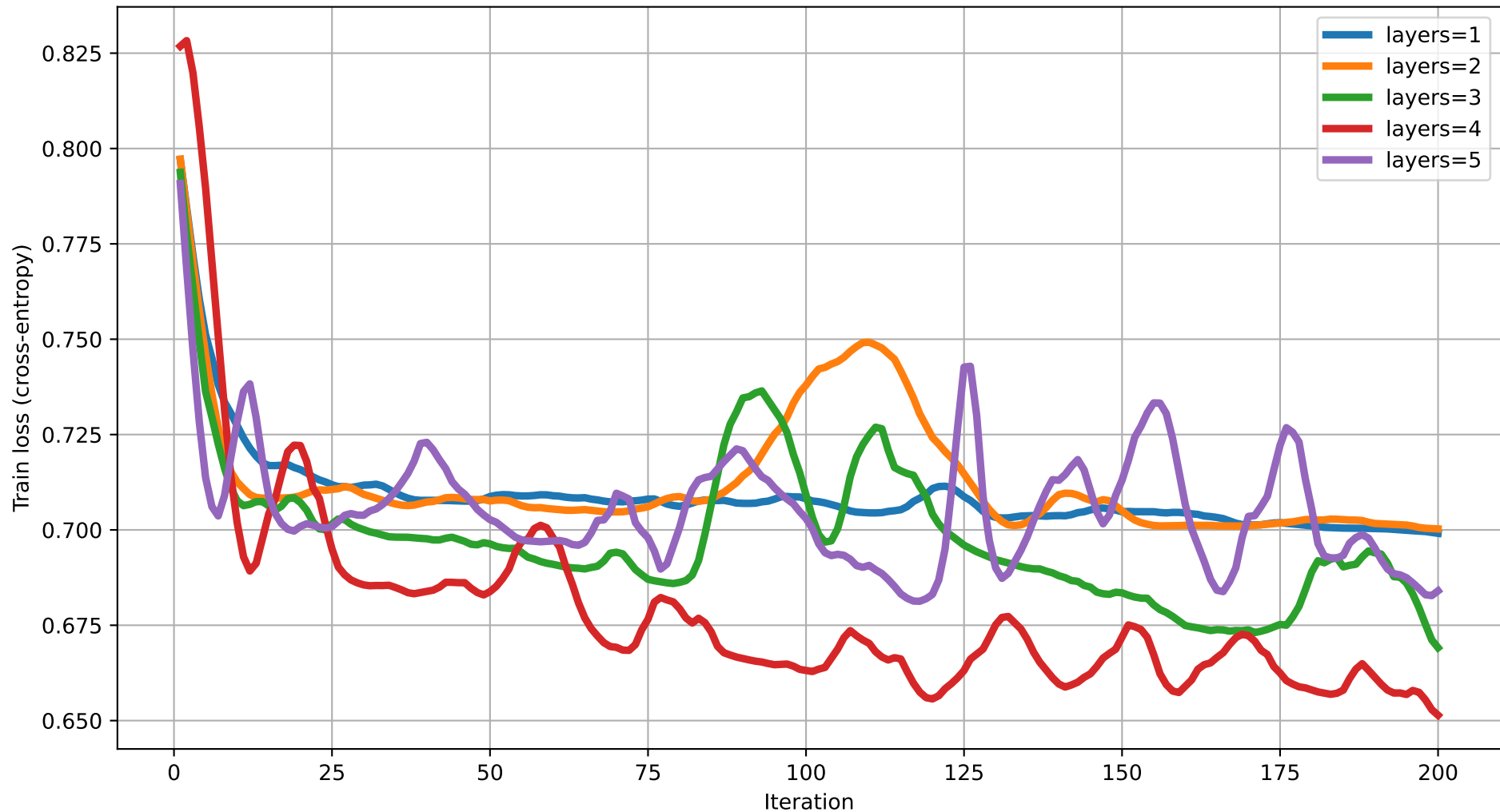
Train loss vs Iteration (dim=8) rot=Rot, ent=full, gate=CZ
