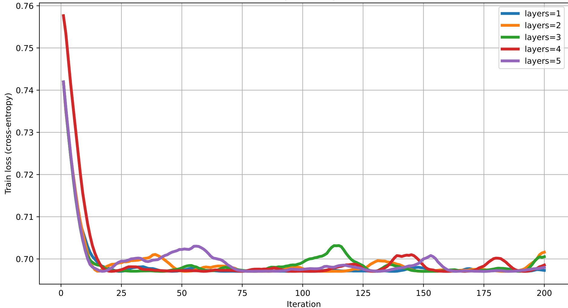
Train loss vs Iteration (degree=5) rot=RZ, ent=pairwise, gate=CNOT
