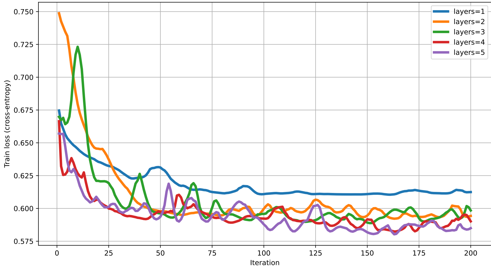
Train loss vs Iteration (degree=4) rot=Rot, ent=full, gate=IsingXX
