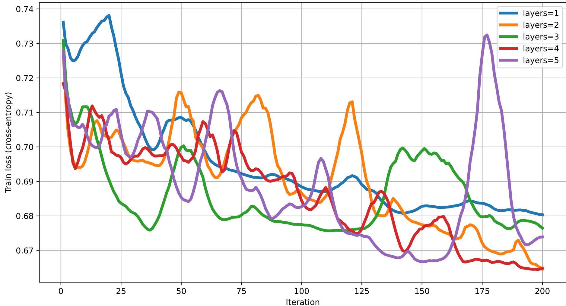
Train loss vs Iteration (dim=18) rot=RY, ent=full, gate=IsingXX
