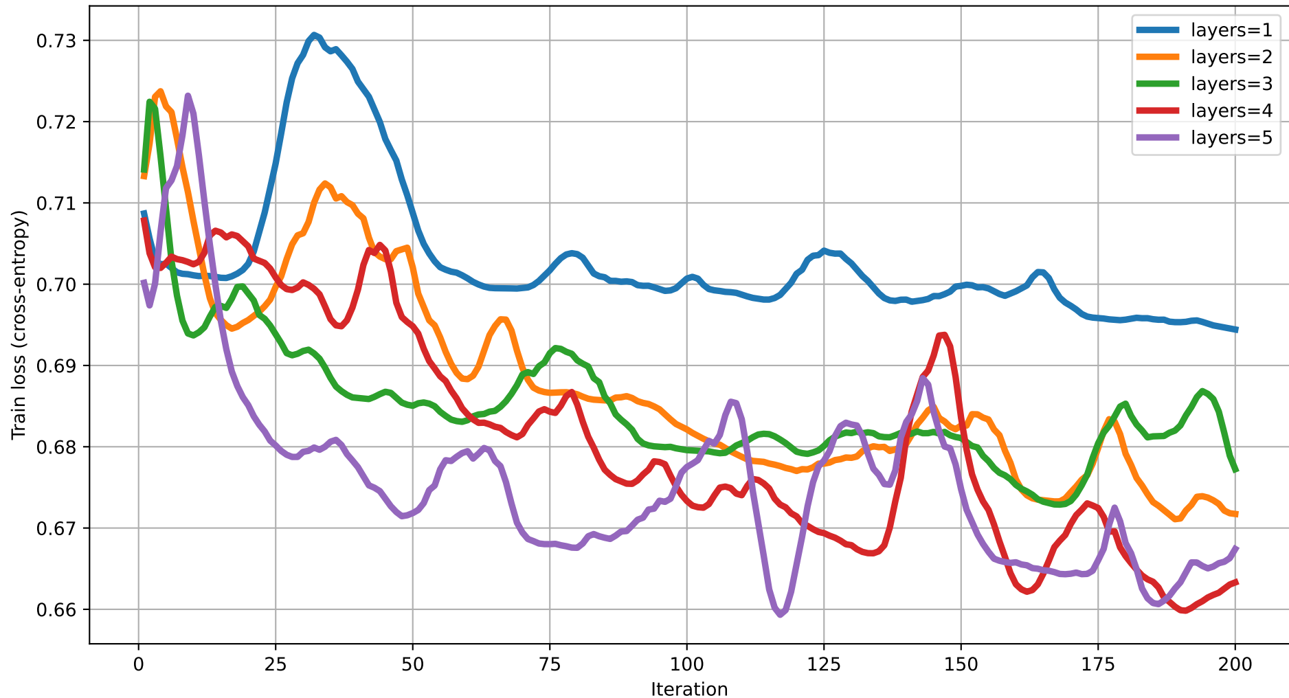
Train loss vs Iteration (dim=12) rot=RY, ent=ring, gate=CZ
