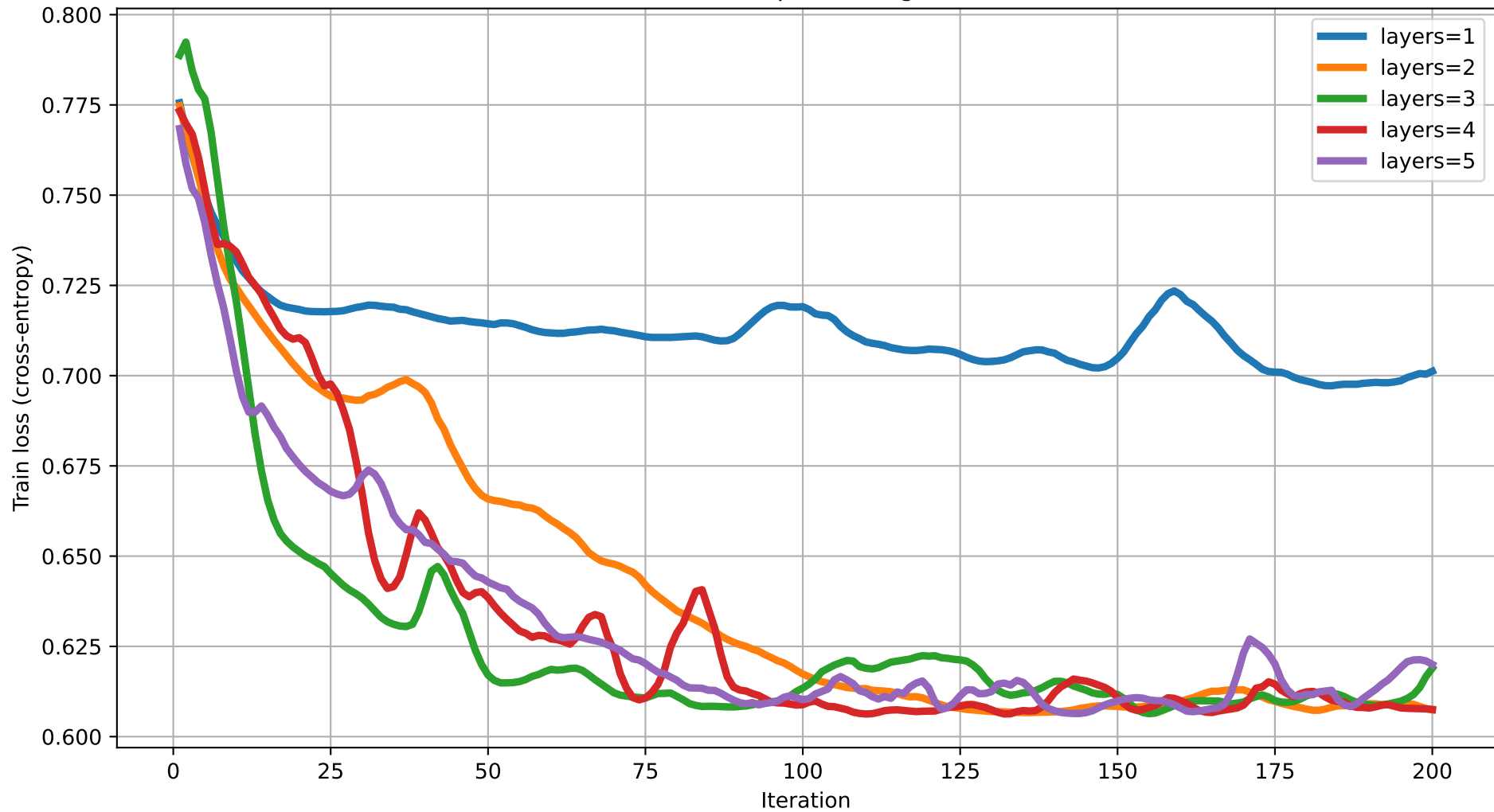
Train loss vs Iteration (dim=9) rot=Rot, ent=pairwise, gate=CZ
