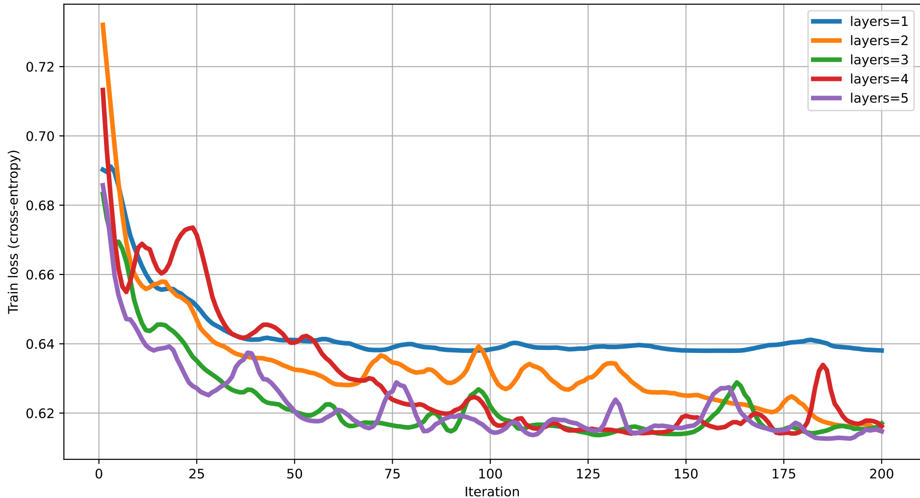
Train loss vs Iteration (degree=2) rot=RZ, ent=full, gate=IsingXX
