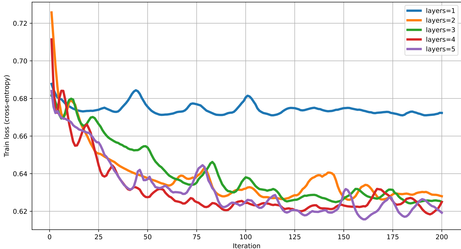
Train loss vs Iteration (degree=2) rot=RY, ent=ring, gate=IsingXX
