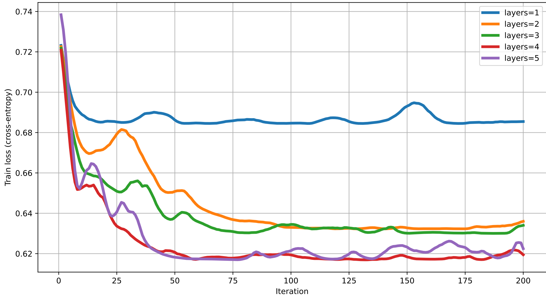
Train loss vs Iteration (degree=3) rot=RX, ent=full, gate=CNOT
