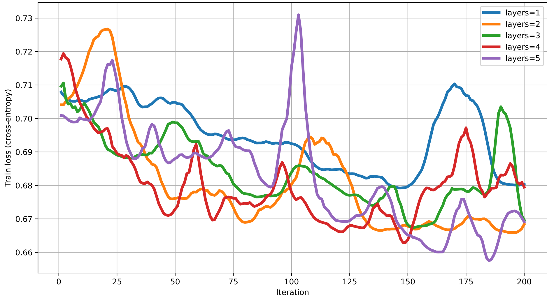
Train loss vs Iteration (dim=12) rot=RY, ent=ring, gate=CNOT
