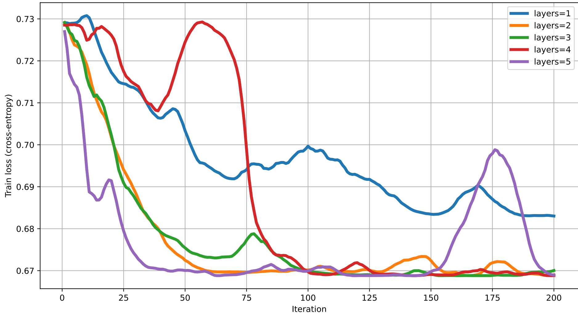
Train loss vs Iteration (dim=7) rot=RX, ent=pairwise, gate=CNOT
