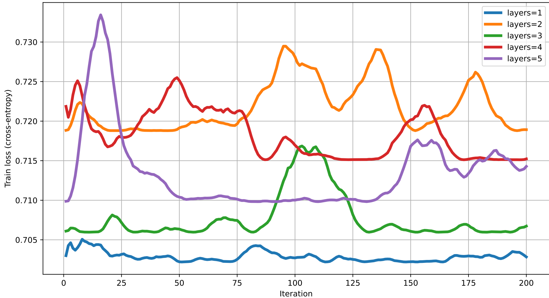
Train loss vs Iteration (dim=15) rot=RZ, ent=ring, gate=CNOT
