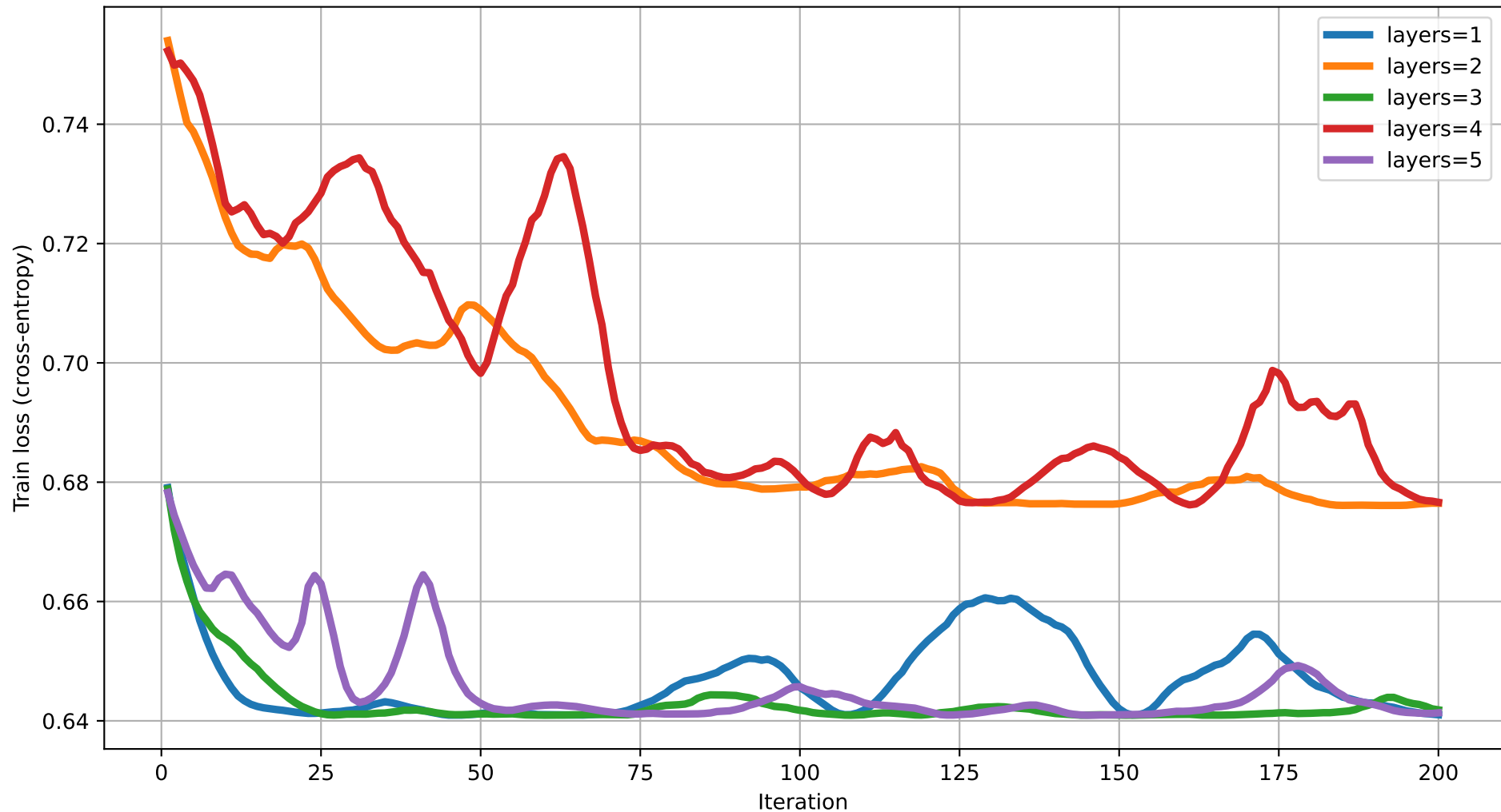
Train loss vs Iteration (dim=5) rot=RX, ent=full, gate=IsingXX
