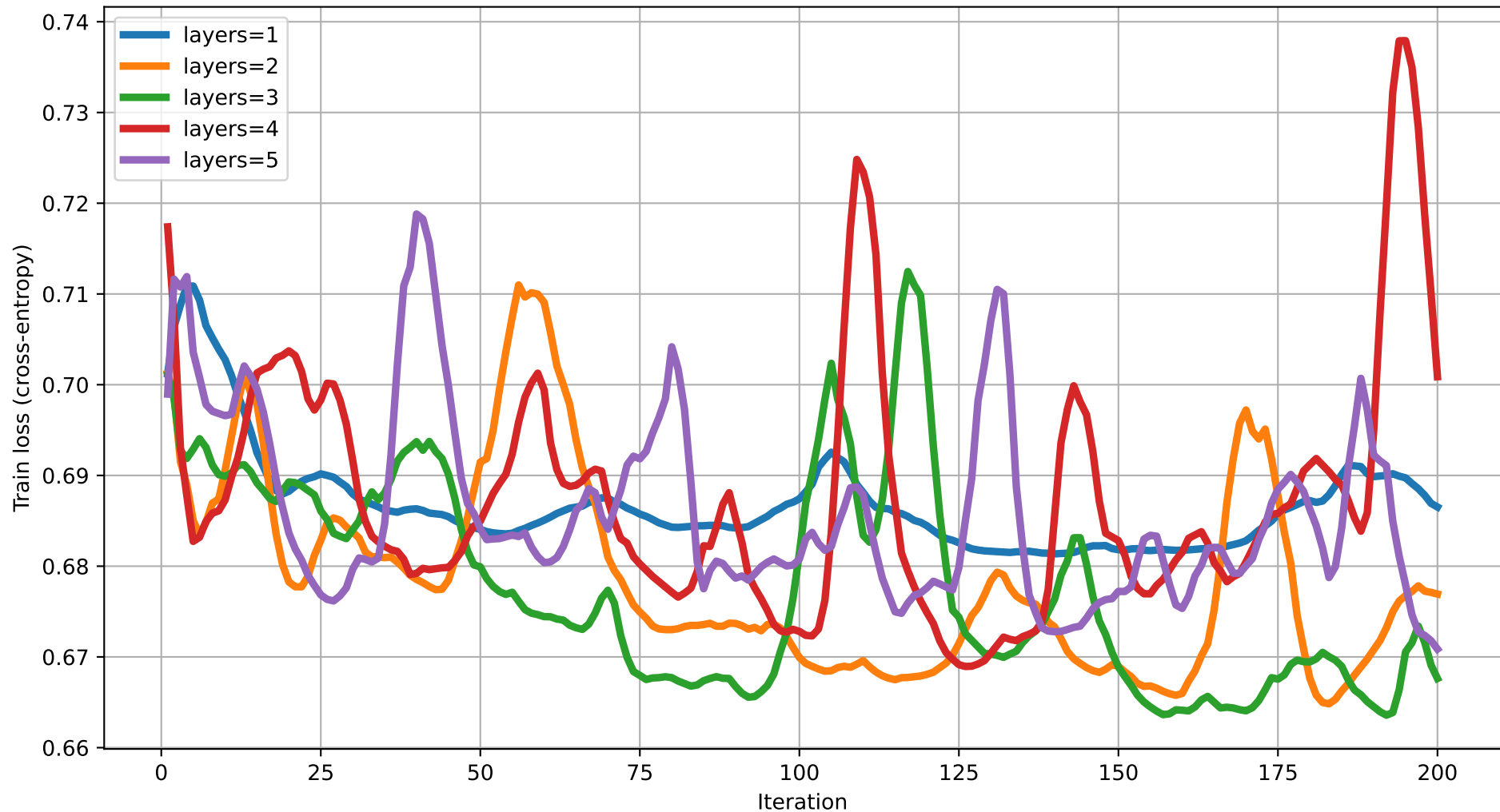
Train loss vs Iteration (dim=13) rot=Rot, ent=ring, gate=IsingXX
