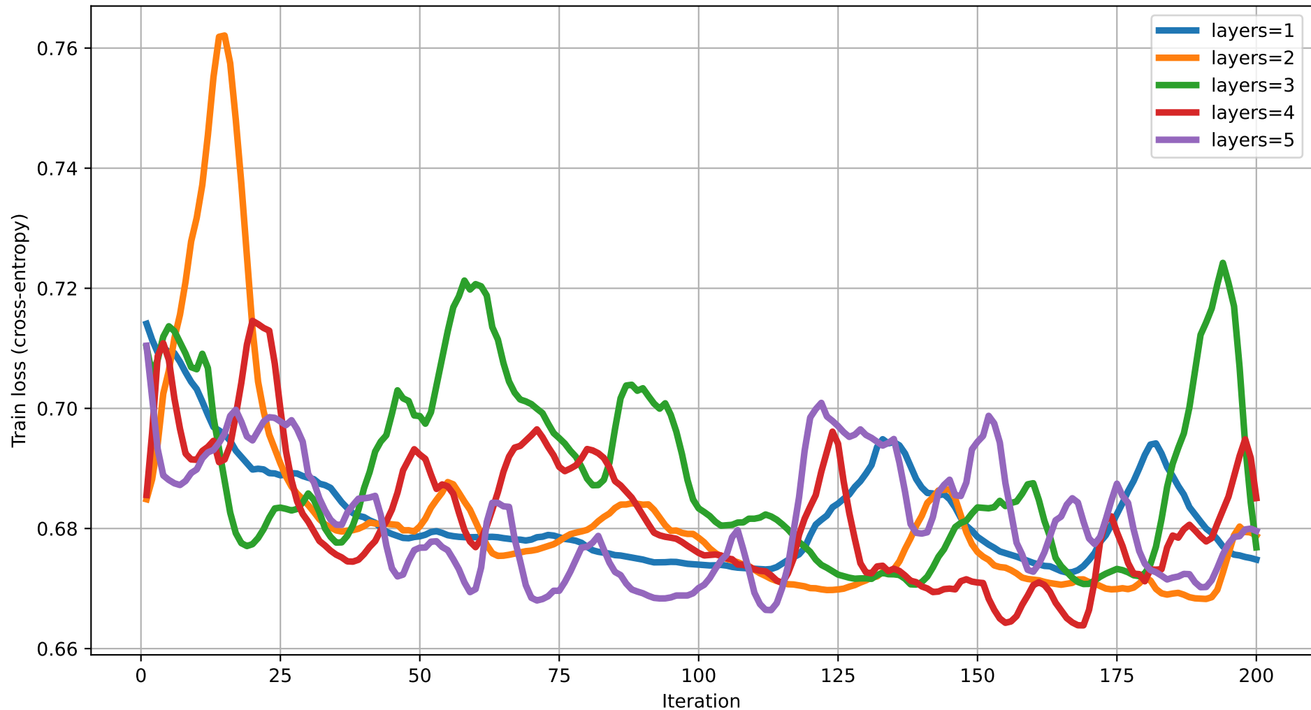
Train loss vs Iteration (dim=15) rot=Rot, ent=ring, gate=IsingXX
