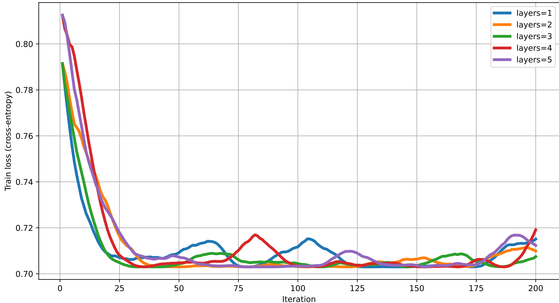
Train loss vs Iteration (dim=2) rot=RZ, ent=full, gate=CZ
