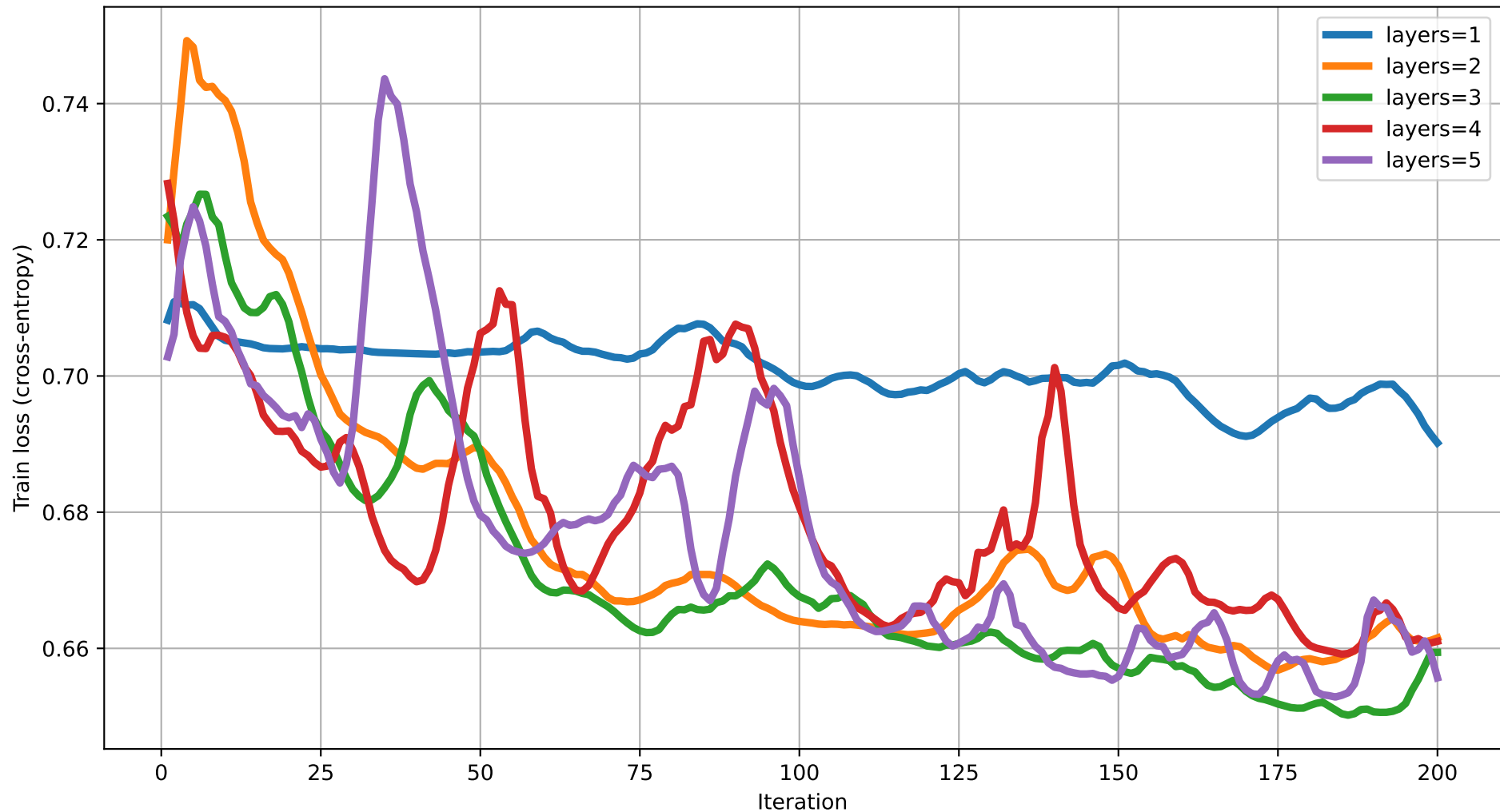
Train loss vs Iteration (dim=6) rot=Rot, ent=pairwise, gate=CZ
