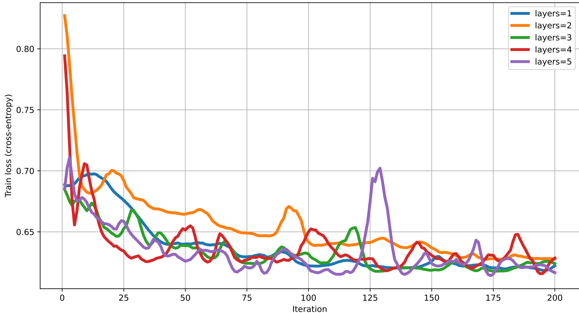
Train loss vs Iteration (dim=4) rot=Rot, ent=chain, gate=IsingXX
