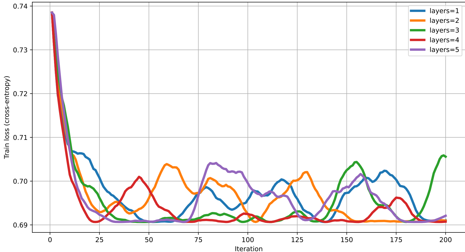
Train loss vs Iteration (dim=16) rot=RZ, ent=ring, gate=CZ
