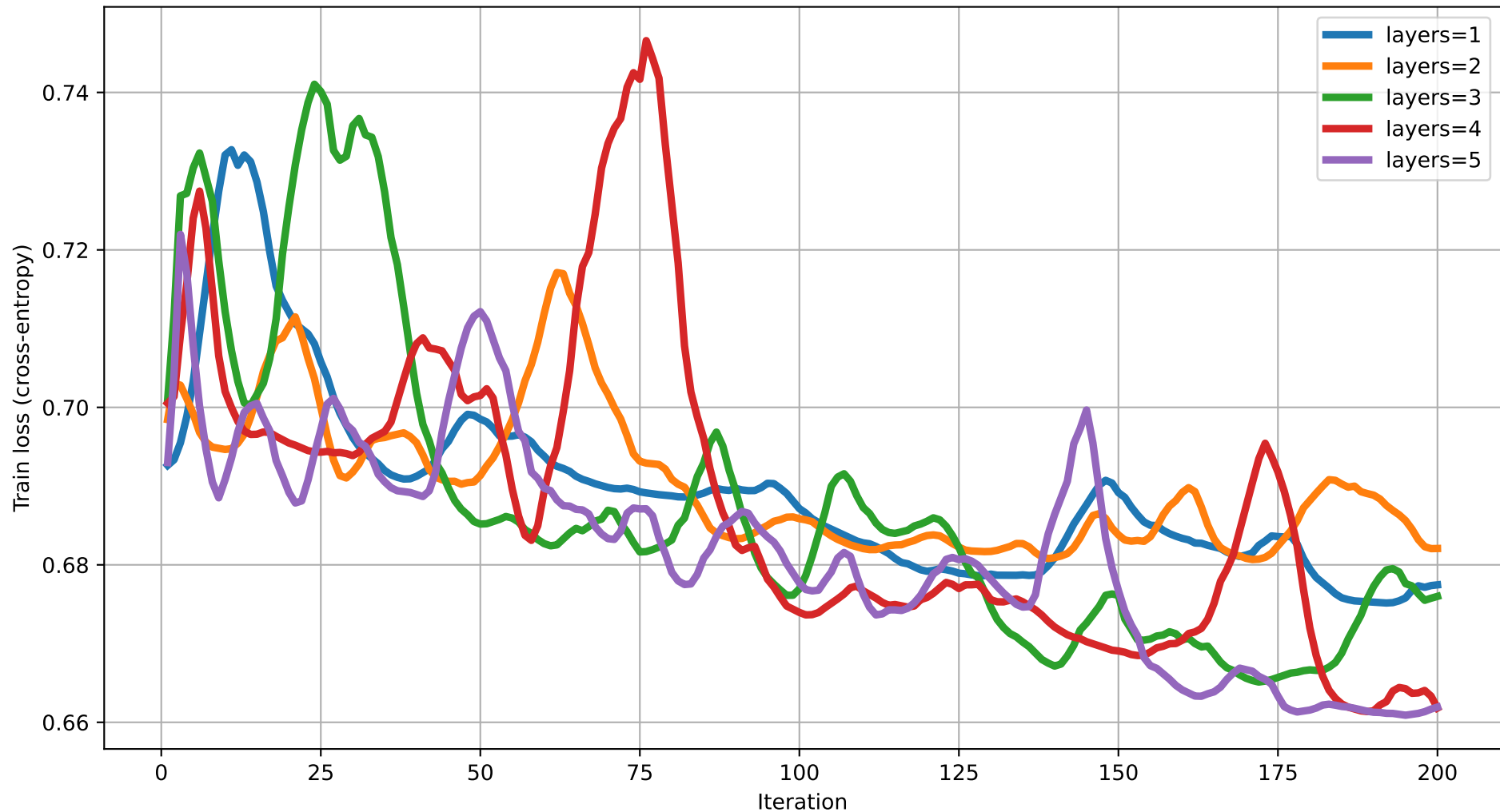
Train loss vs Iteration (dim=14) rot=RYZ, ent=chain, gate=IsingXX
