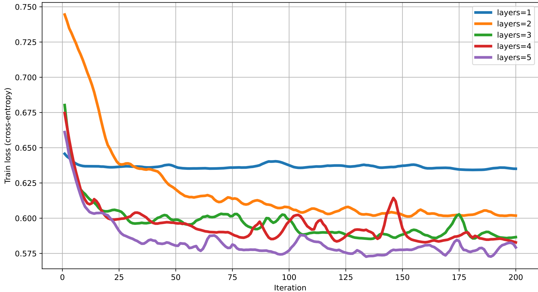
Train loss vs Iteration (degree=3) rot=Rot, ent=ring, gate=CNOT
