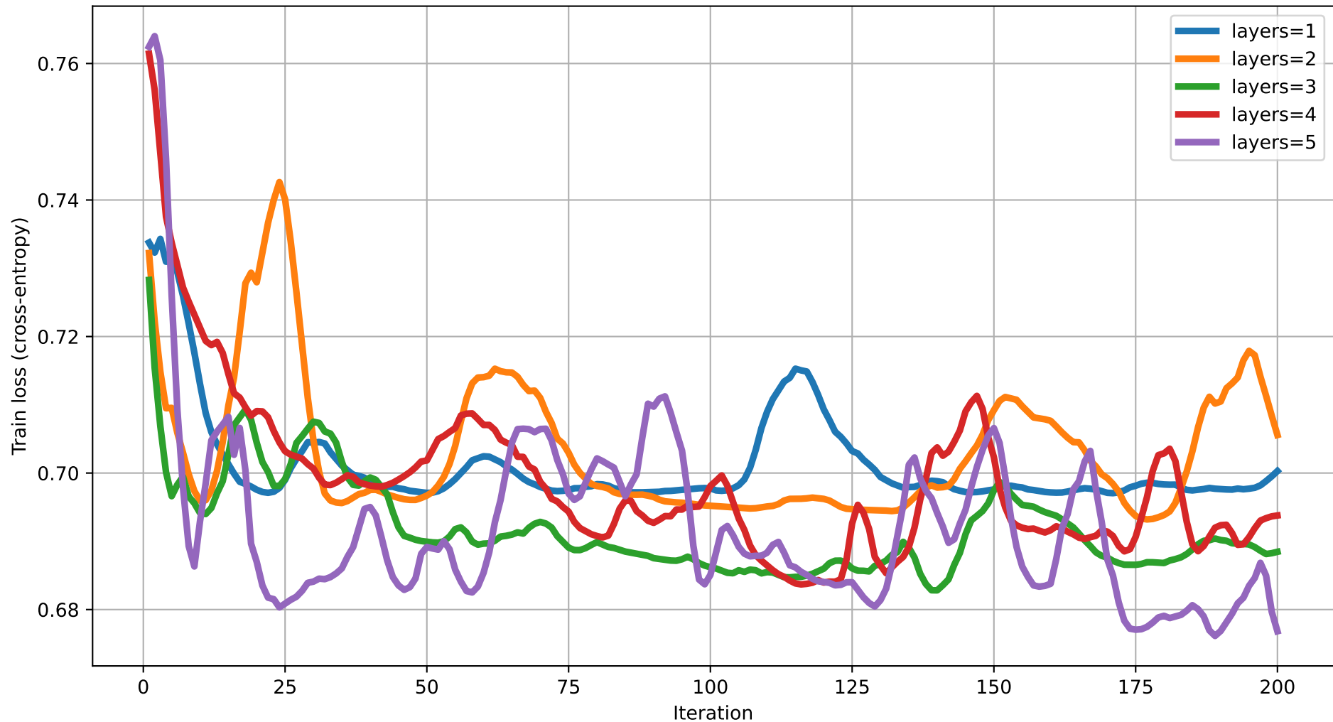
Train loss vs Iteration (dim=18) rot=Rot, ent=full, gate=CNOT
