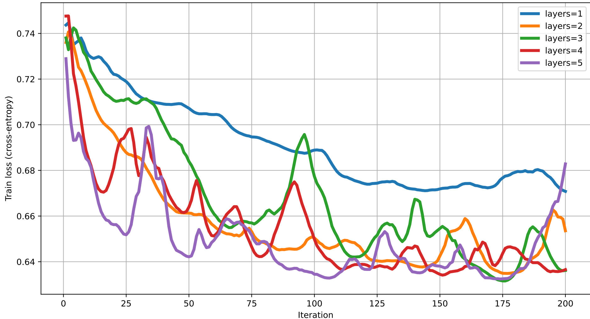
Train loss vs Iteration (dim=3) rot=Rot, ent=pairwise, gate=CZ
