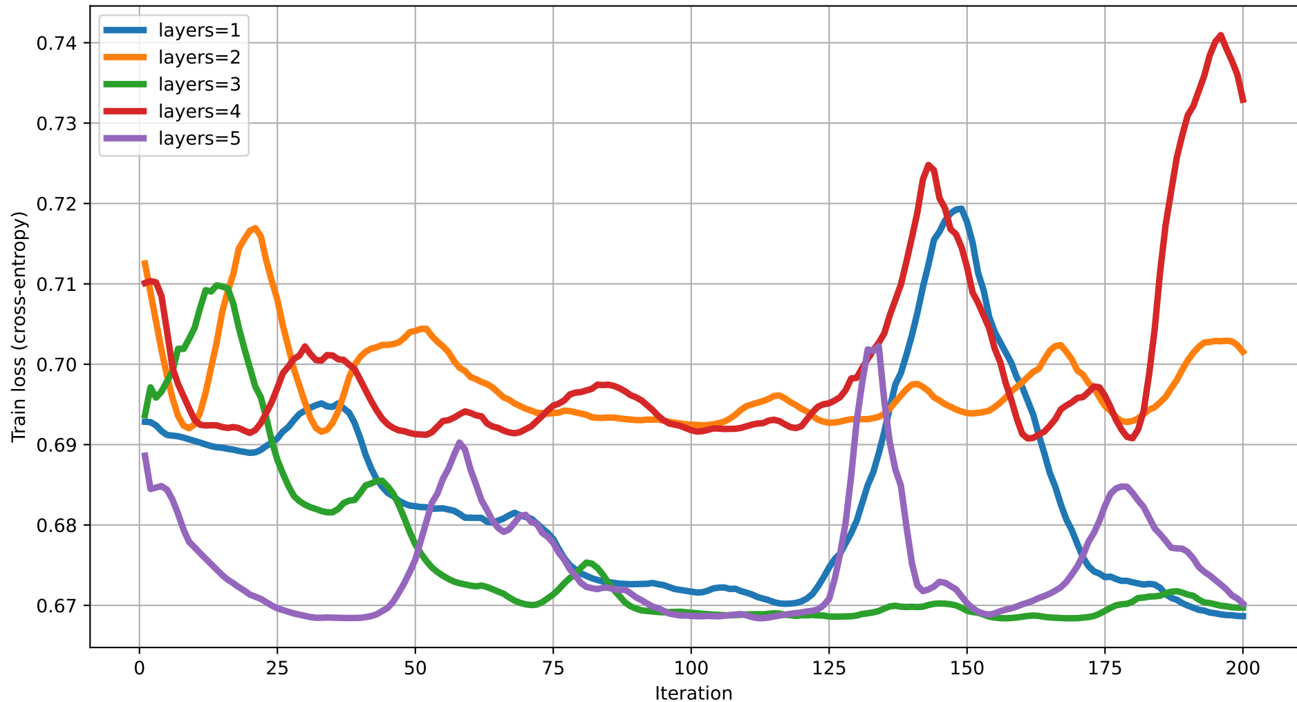
Train loss vs Iteration (dim=12) rot=RX, ent=chain, gate=IsingXX
