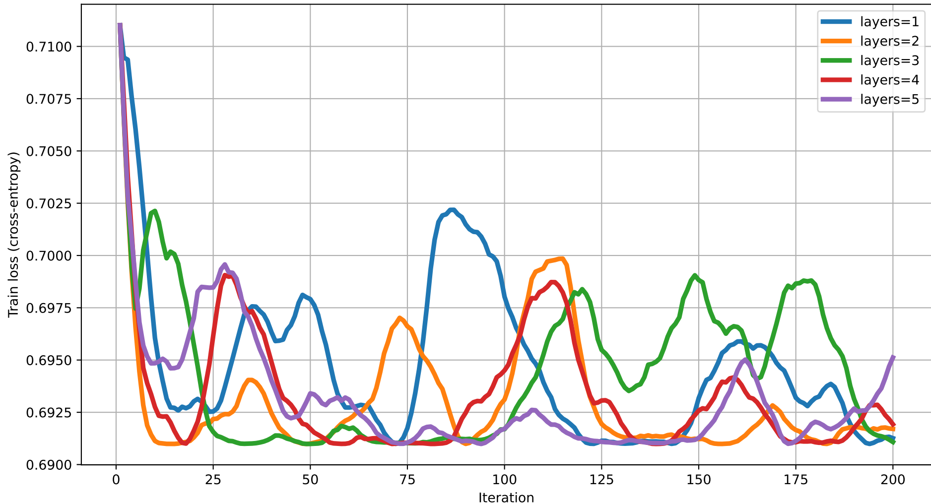
Train loss vs Iteration (dim=20) rot=RZ, ent=ring, gate=CZ
