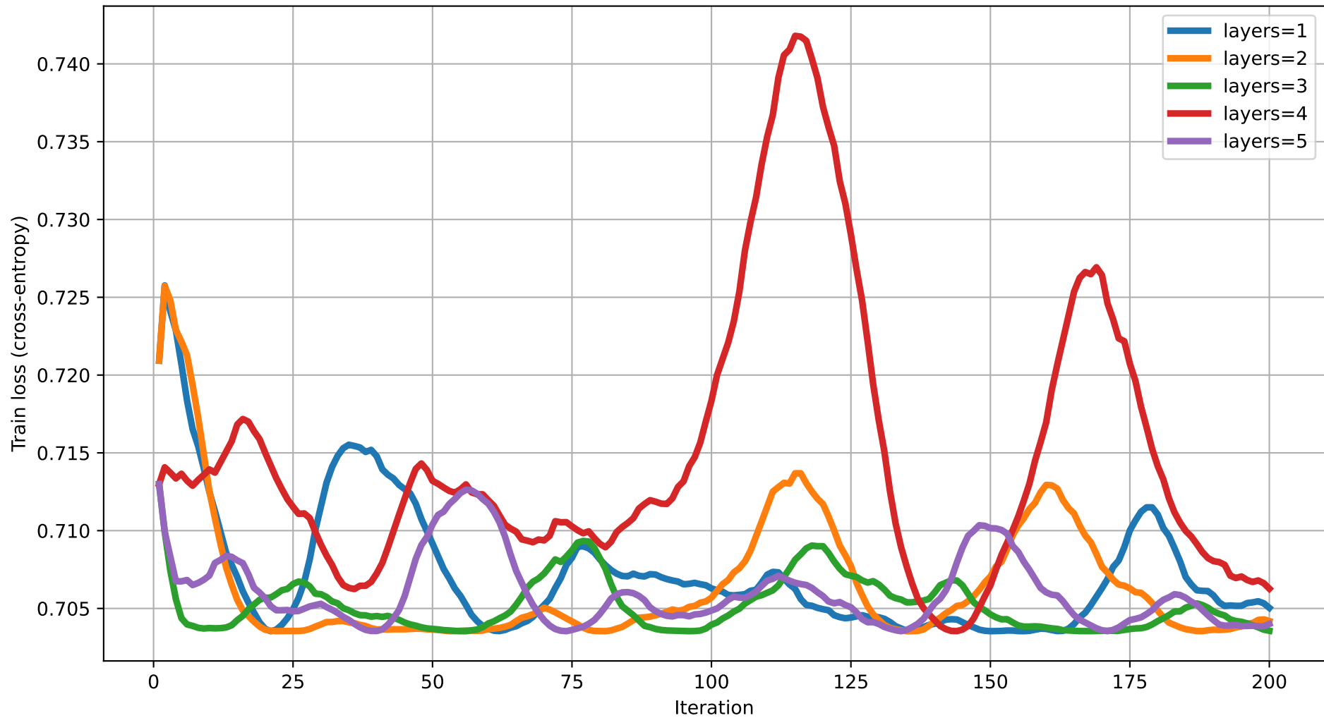
Train loss vs Iteration (dim=11) rot=RZ, ent=pairwise, gate=CNOT
