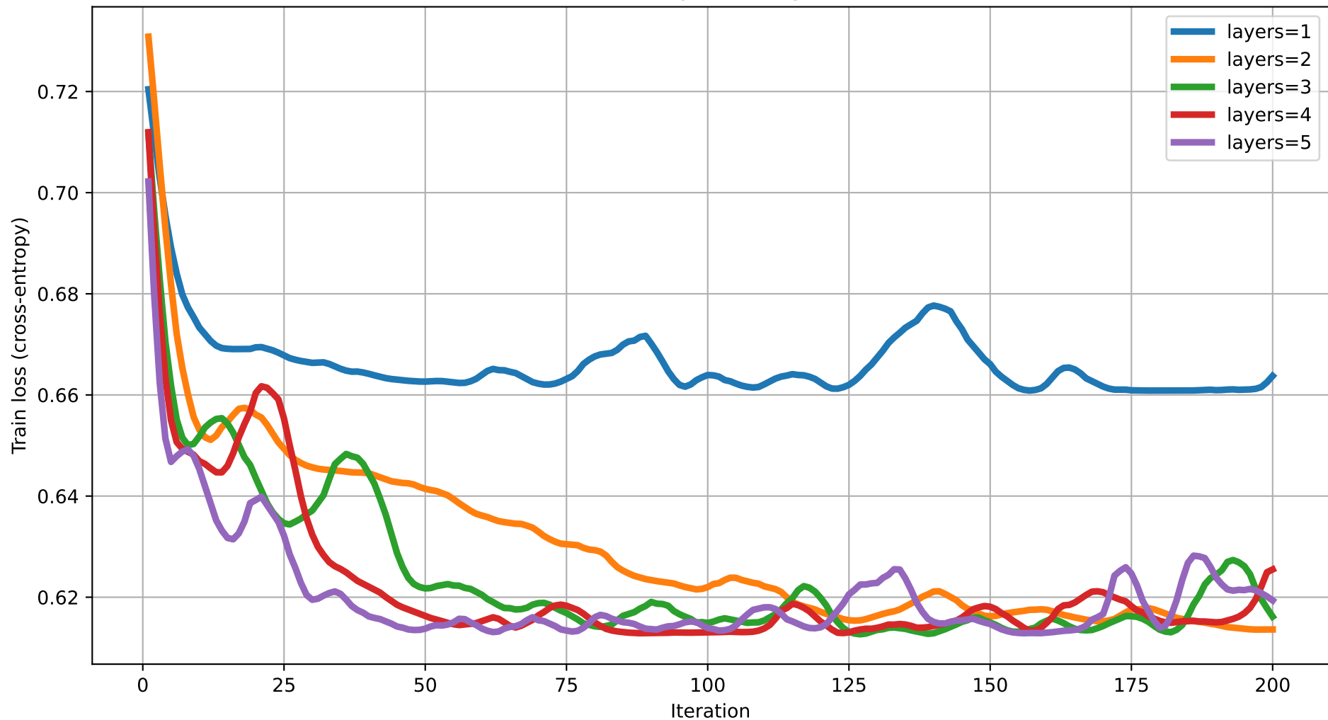
Train loss vs Iteration (degree=3) rot=RY, ent=pairwise, gate=CZ
