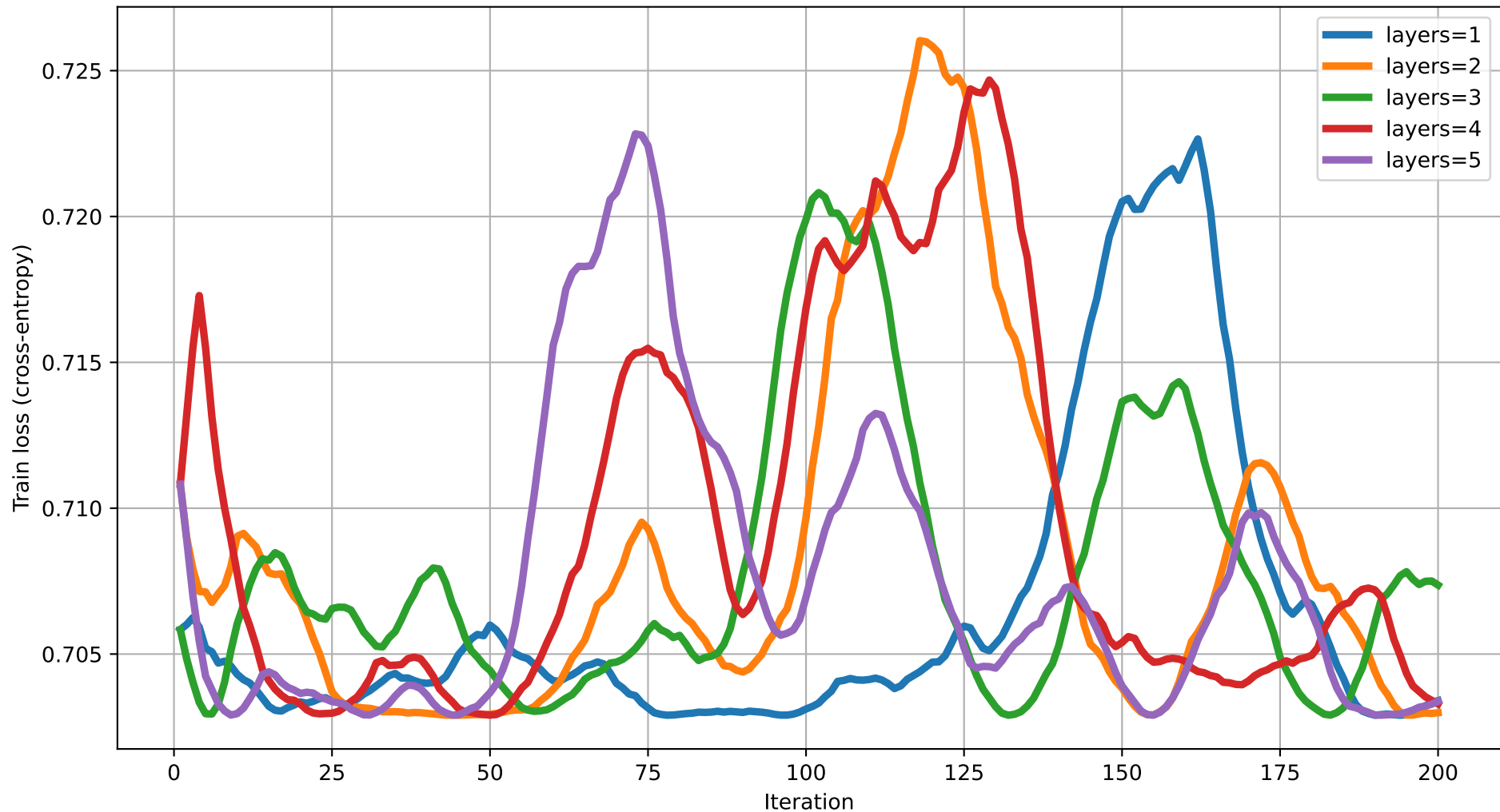
Train loss vs Iteration (dim=12) rot=RZ, ent=full, gate=CNOT
