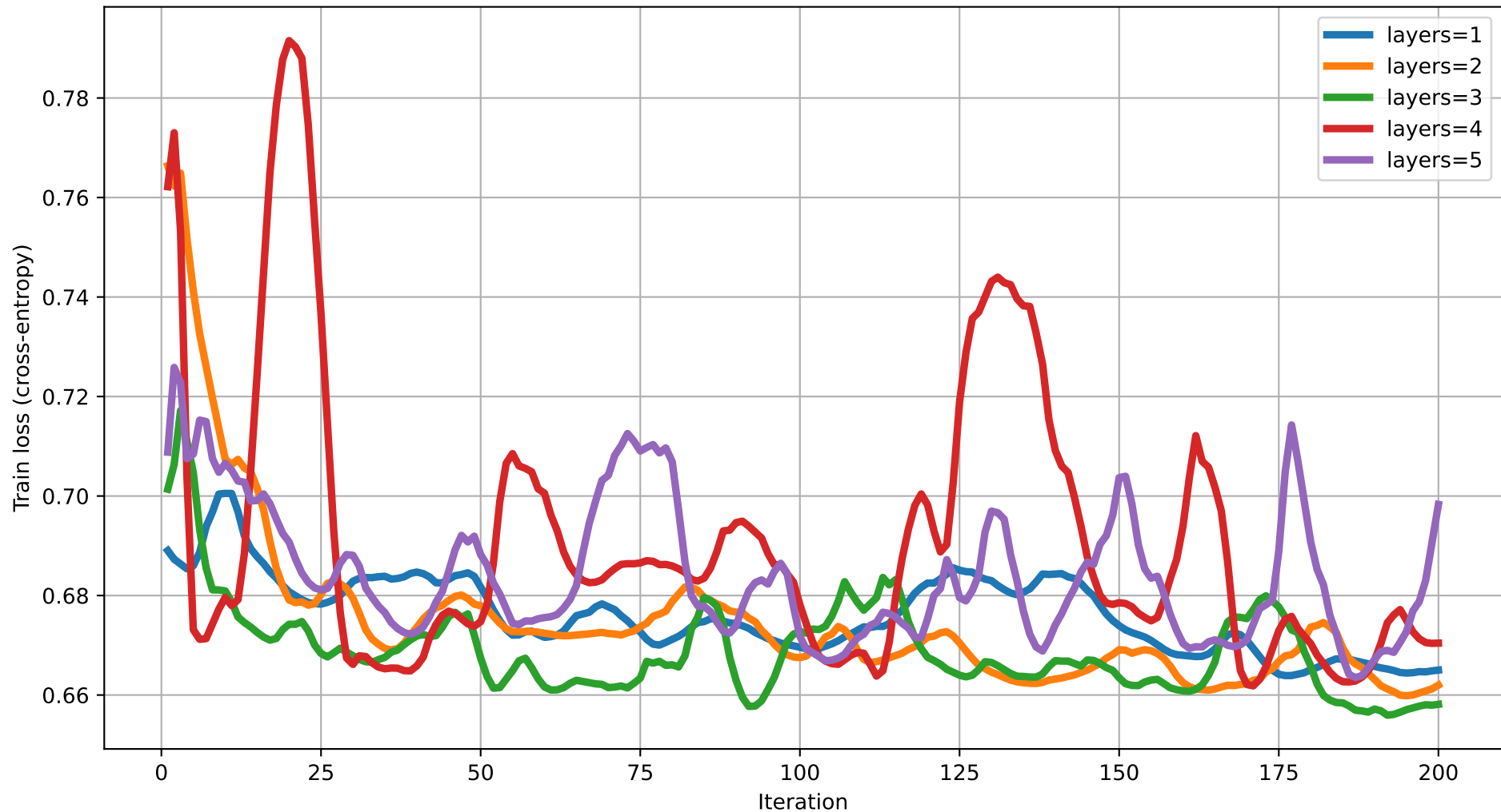
Train loss vs Iteration (dim=10) rot=Rot, ent=full, gate=IsingXX
