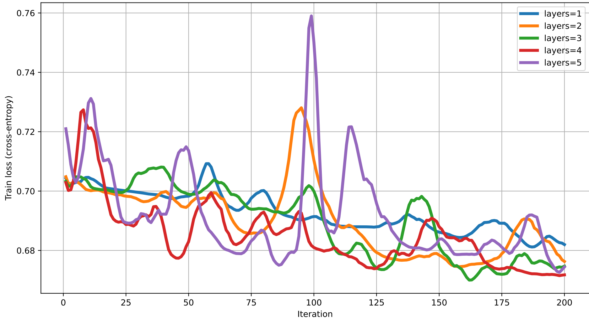
Train loss vs Iteration (dim=14) rot=Rot, ent=ring, gate=CZ
