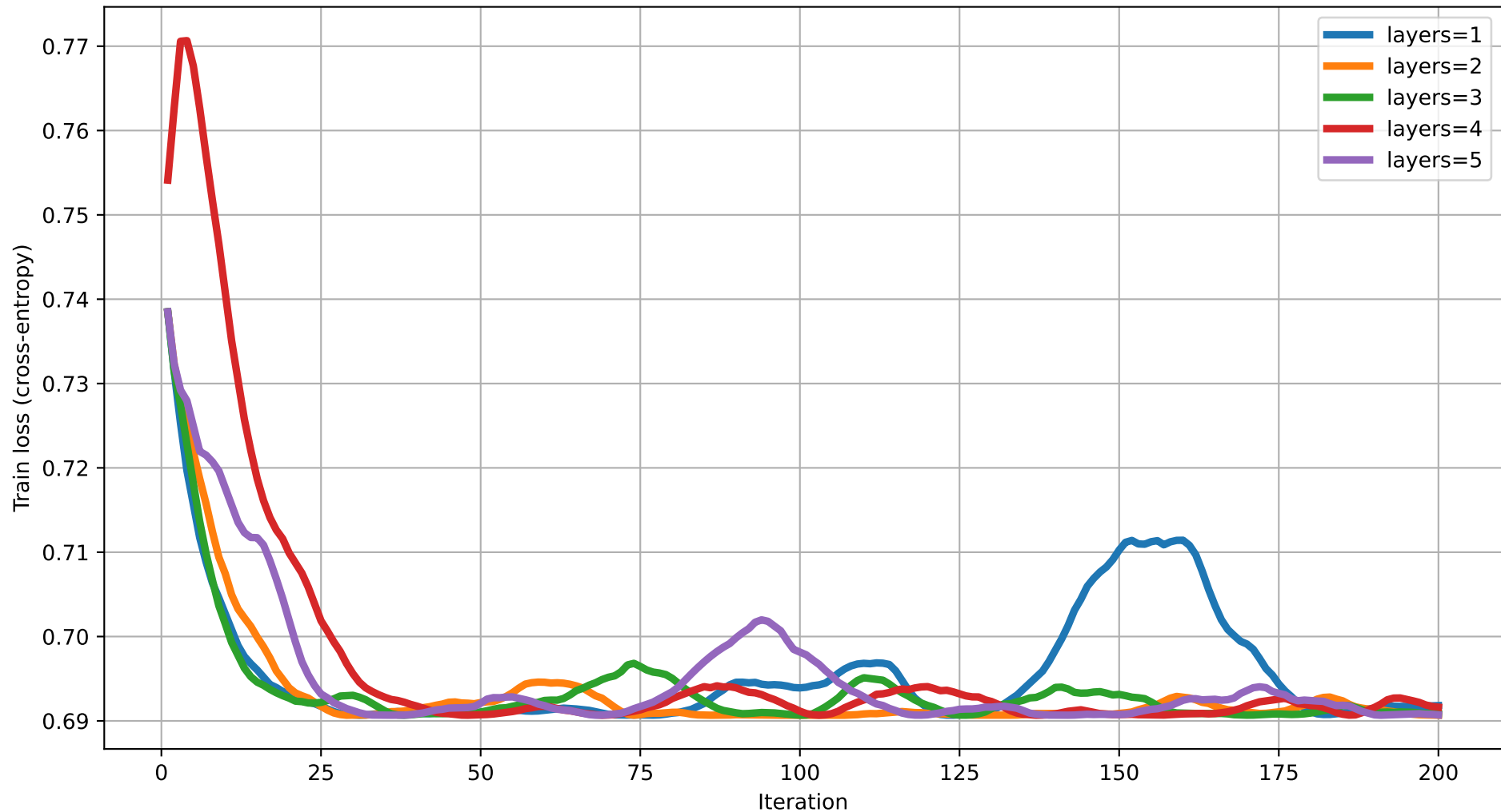
Train loss vs Iteration (dim=16) rot=RZ, ent=full, gate=CZ
