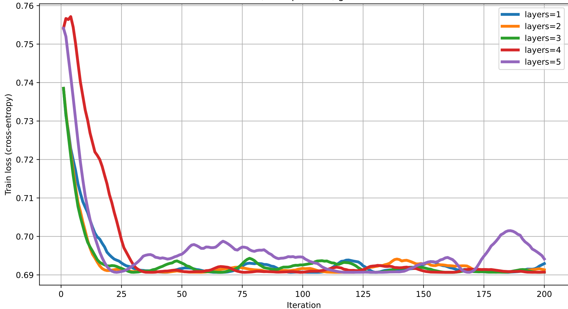
Train loss vs Iteration (dim=16) rot=RZ, ent=pairwise, gate=CZ
