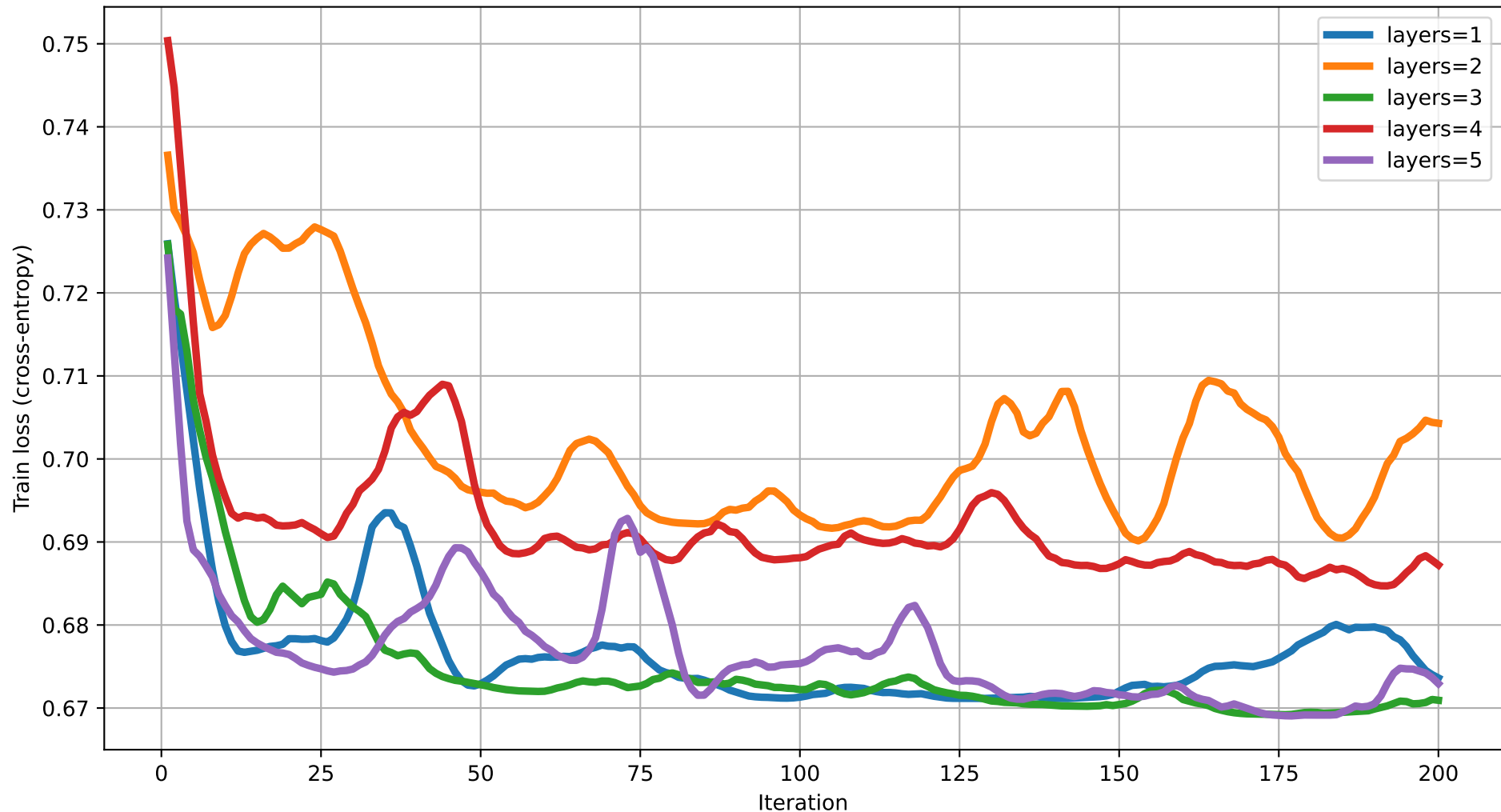
Train loss vs Iteration (dim=18) rot=RZ, ent=ring, gate=IsingXX
