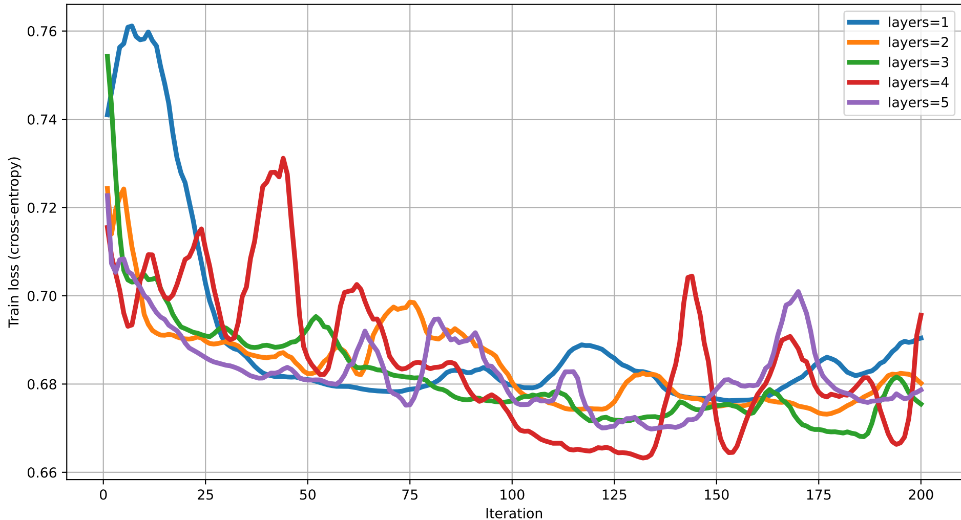
Train loss vs Iteration (dim=19) rot=RYZ, ent=full, gate=IsingXX
