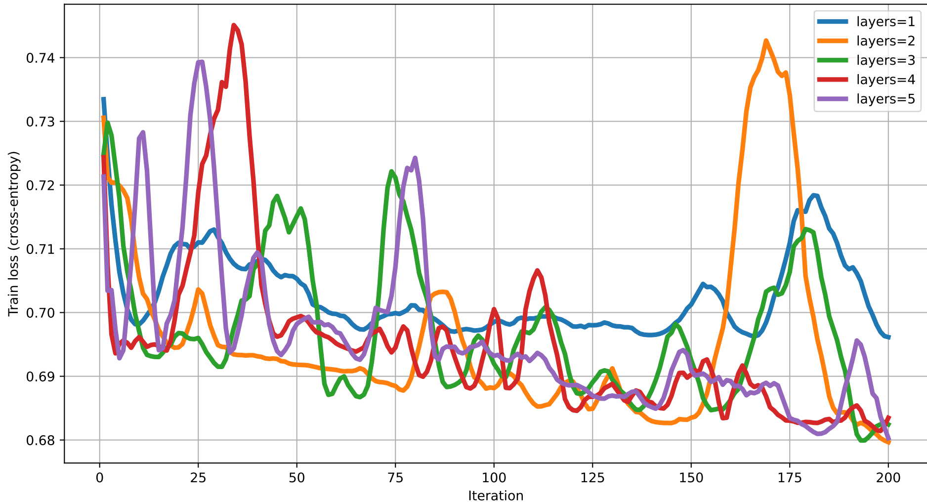
Train loss vs Iteration (dim=19) rot=Rot, ent=pairwise, gate=CNOT
