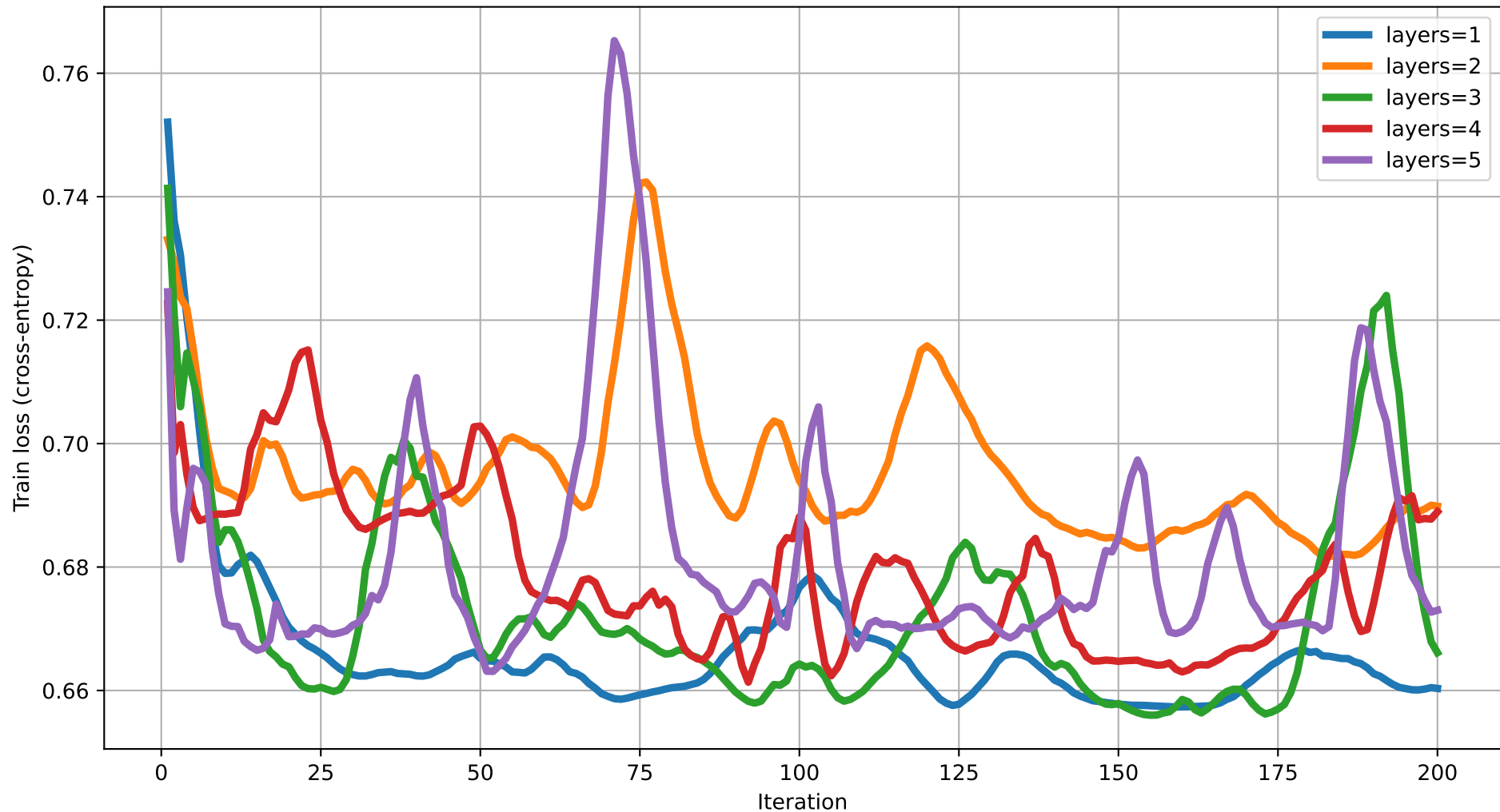
Train loss vs Iteration (dim=16) rot=Rot, ent=ring, gate=IsingXX
