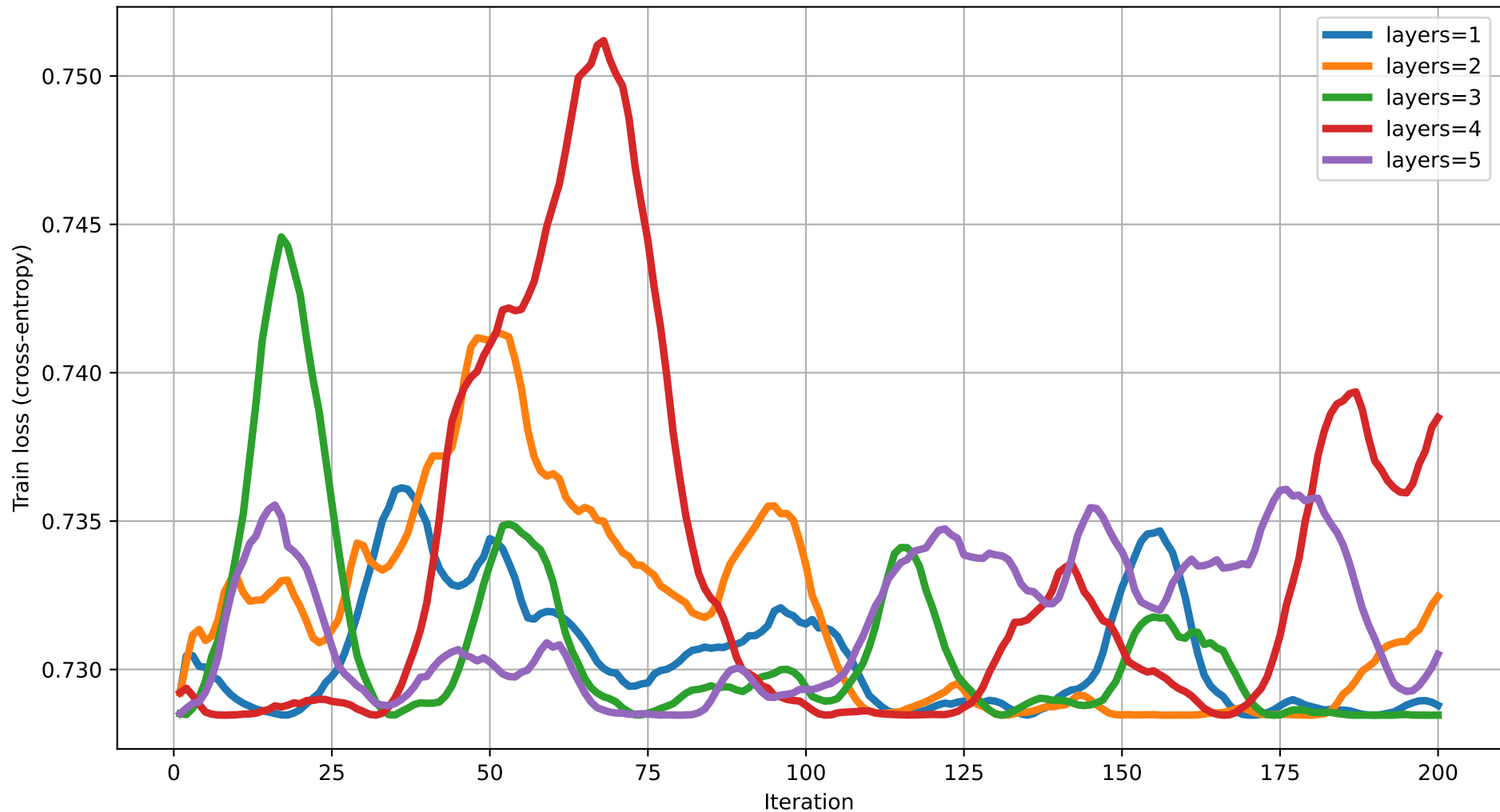
Train loss vs Iteration (dim=7) rot=RZ, ent=chain, gate=CNOT
