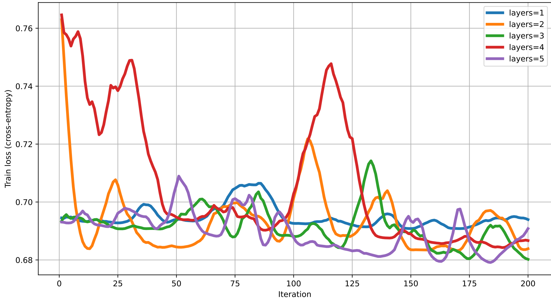
Train loss vs Iteration (dim=17) rot=RZ, ent=pairwise, gate=IsingXX
