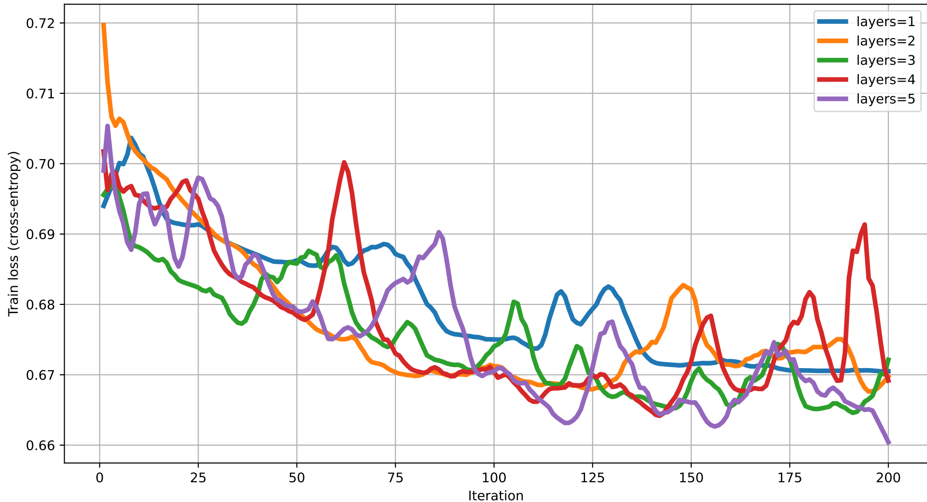
Train loss vs Iteration (dim=11) rot=RYZ, ent=chain, gate=IsingXX
