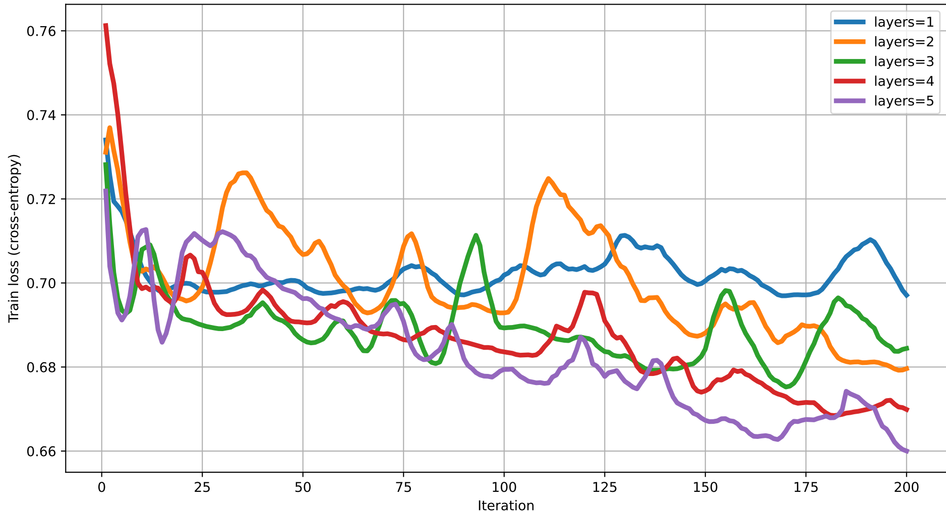
Train loss vs Iteration (dim=19) rot=RYZ, ent=full, gate=CNOT
