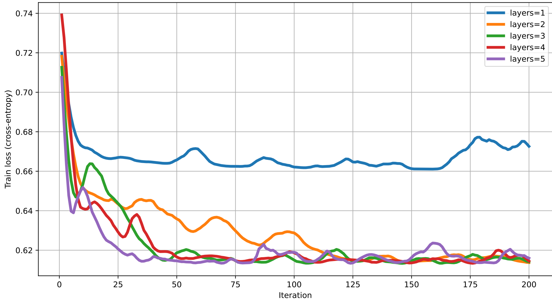
Train loss vs Iteration (degree=3) rot=RYZ, ent=pairwise, gate=CNOT
