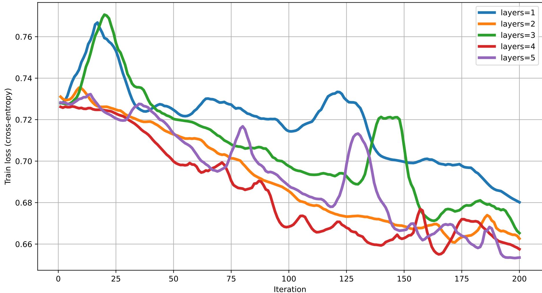
Train loss vs Iteration (dim=7) rot=RYZ, ent=full, gate=CZ
