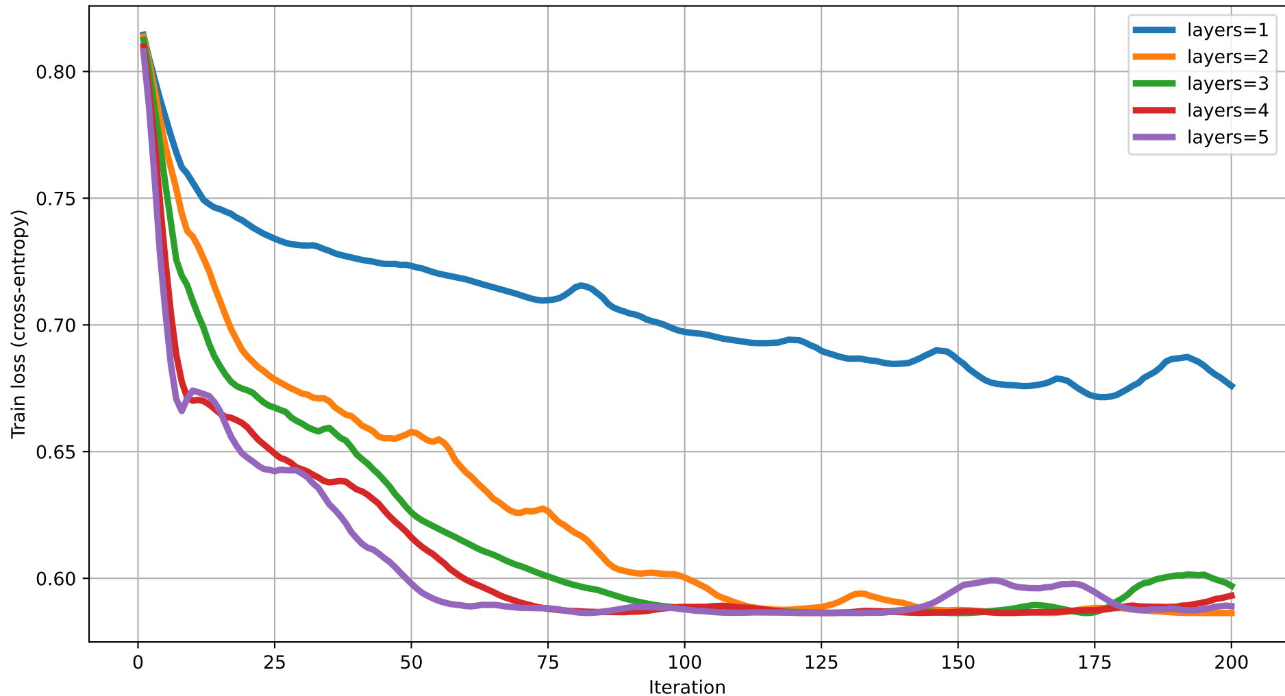
Train loss vs Iteration (dim=2) rot=RX, ent=full, gate=CNOT
