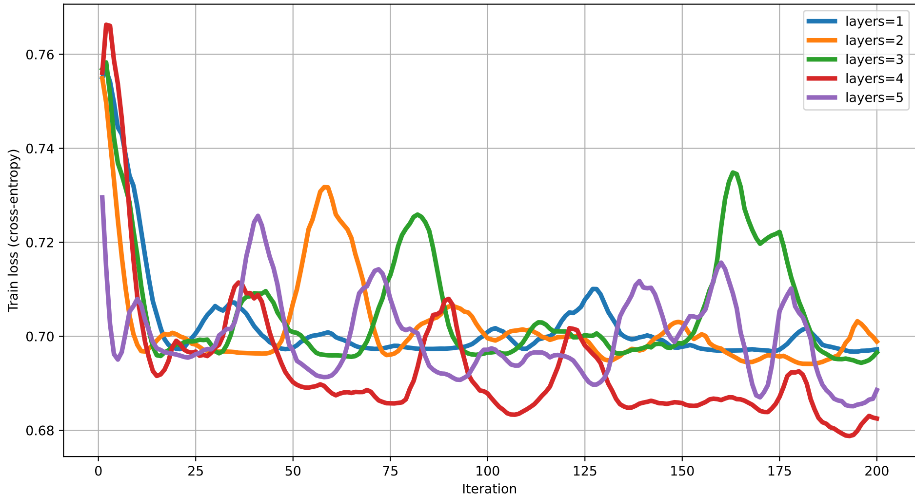
Train loss vs Iteration (dim=18) rot=RY, ent=ring, gate=CZ
