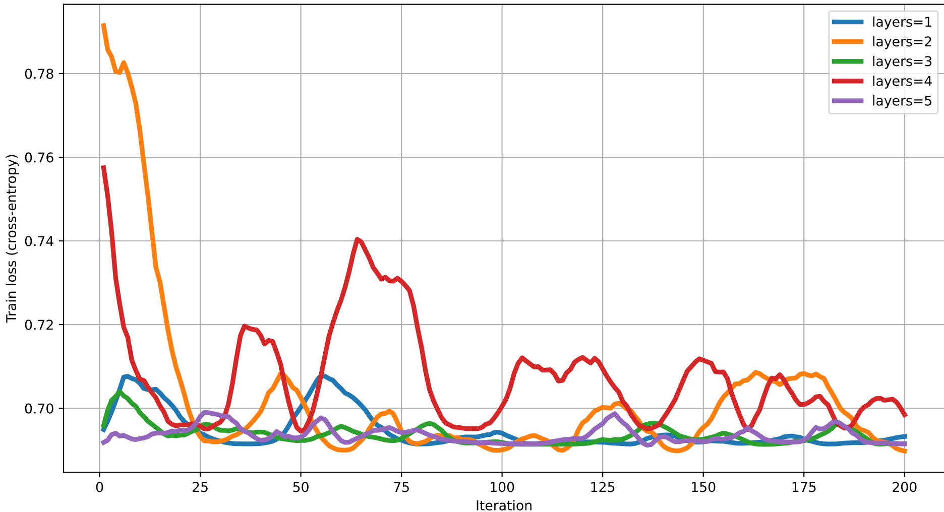
Train loss vs Iteration (dim=18) rot=RY, ent=pairwise, gate=IsingXX
