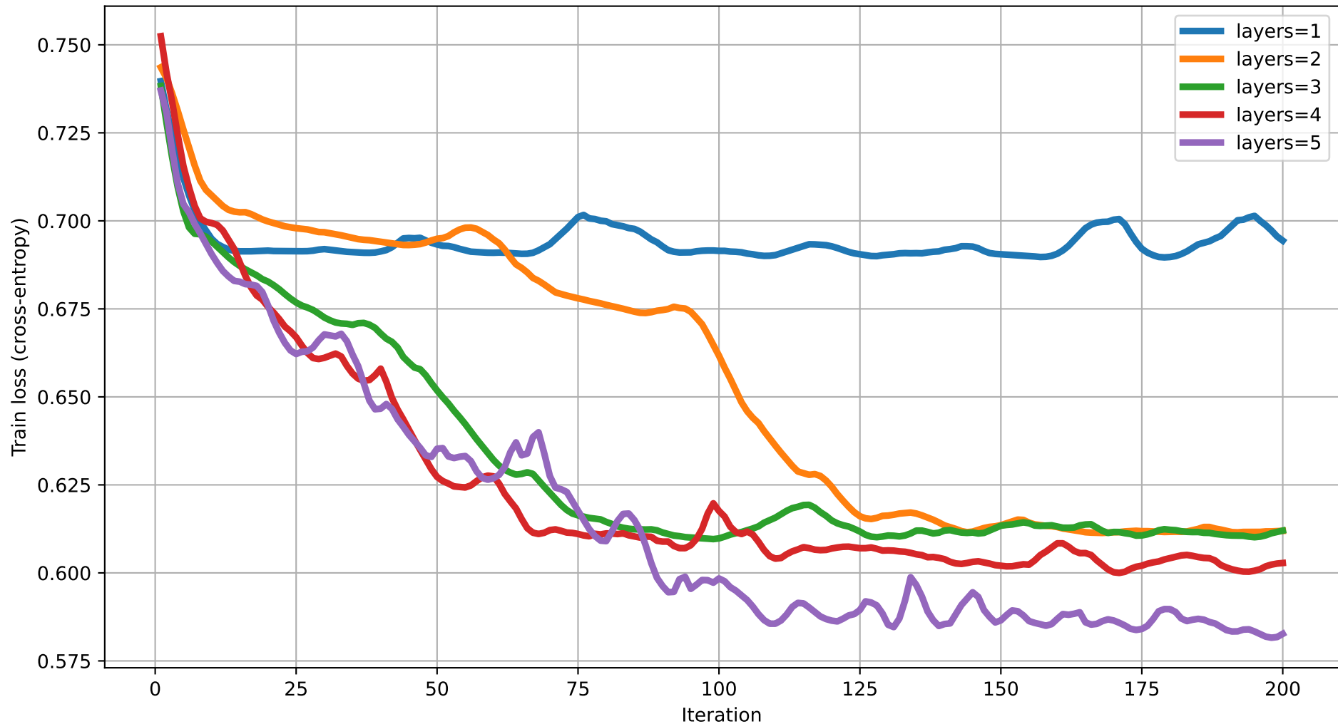
Train loss vs Iteration (degree=5) rot=Rot, ent=ring, gate=CZ
