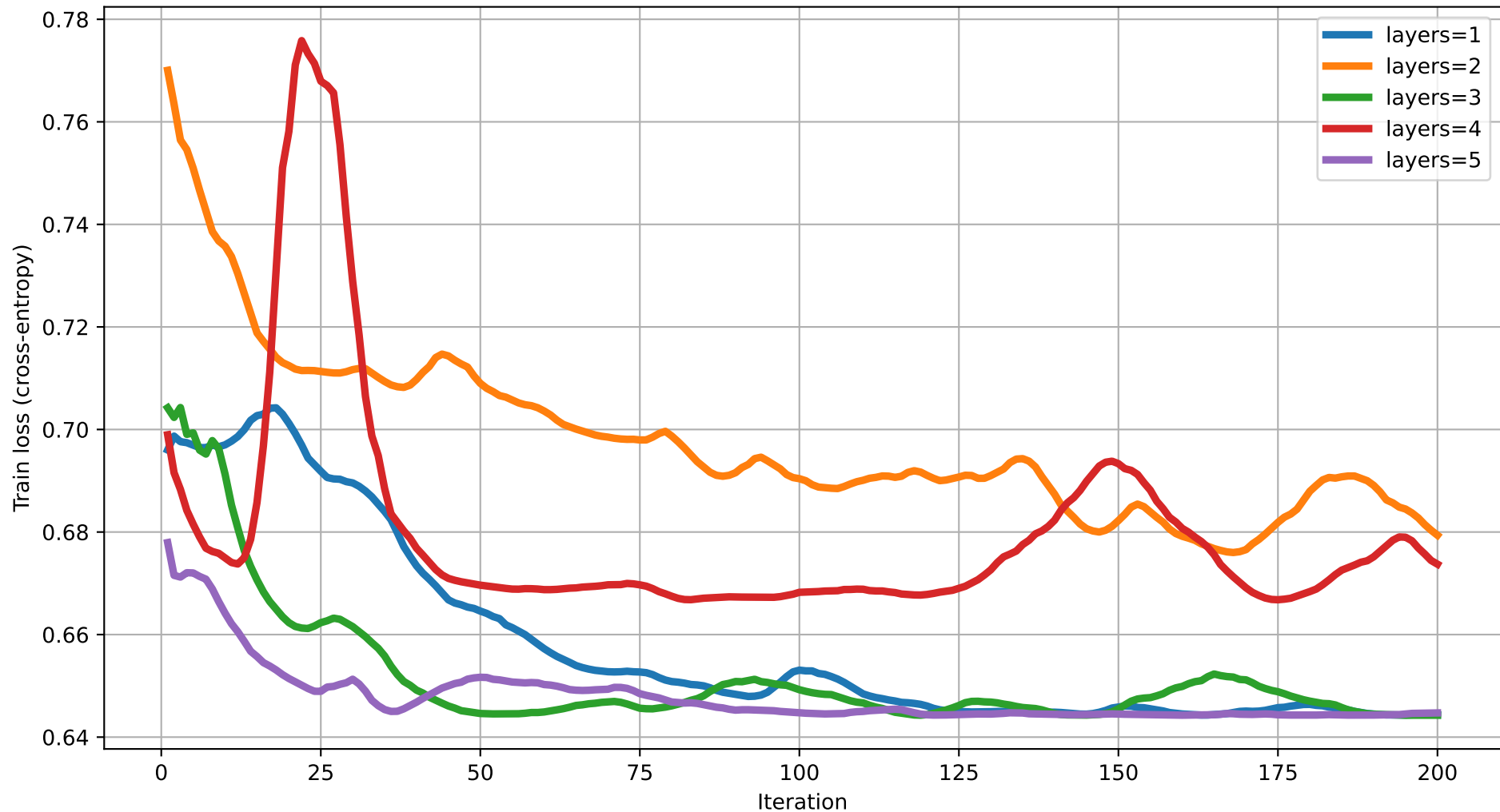
Train loss vs Iteration (dim=10) rot=RX, ent=pairwise, gate=IsingXX
