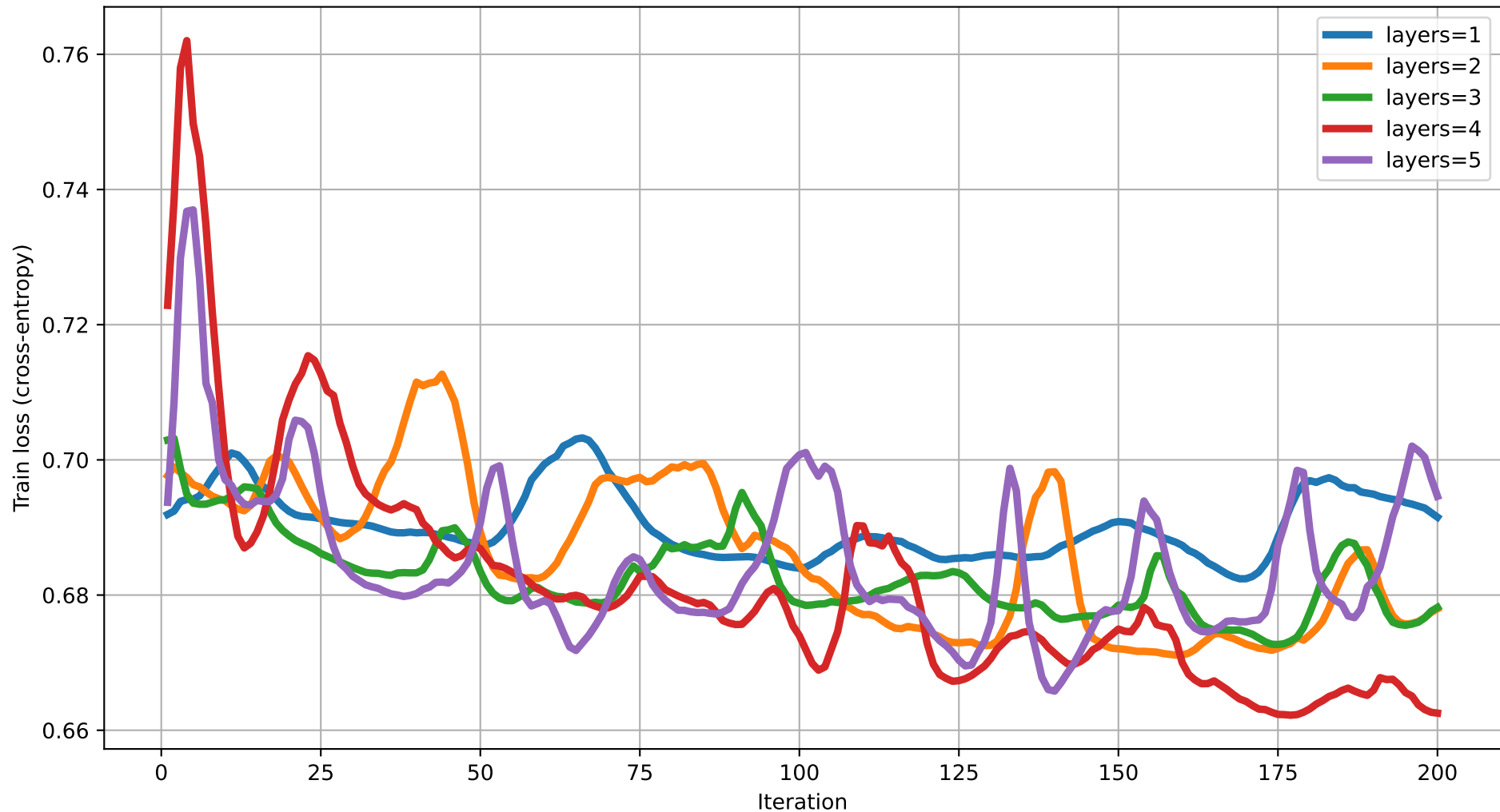
Train loss vs Iteration (dim=14) rot=RYZ, ent=full, gate=IsingXX
