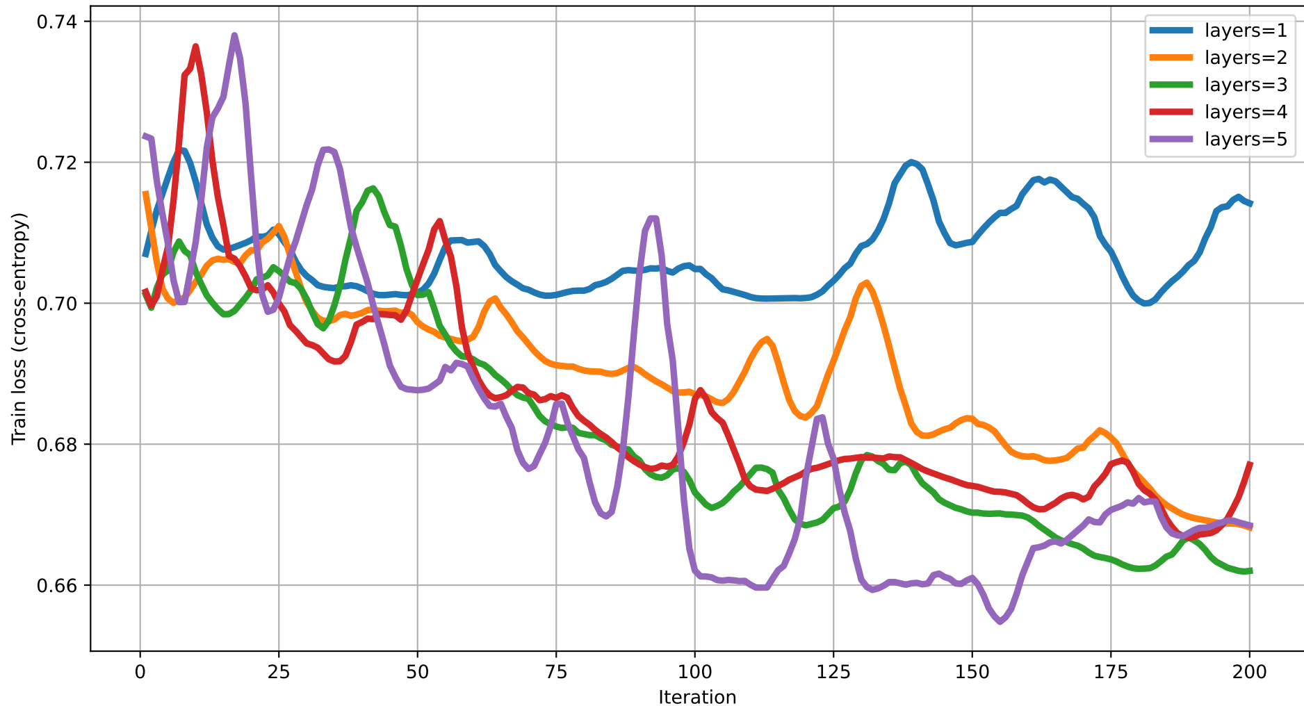
Train loss vs Iteration (dim=12) rot=RY, ent=full, gate=CNOT
