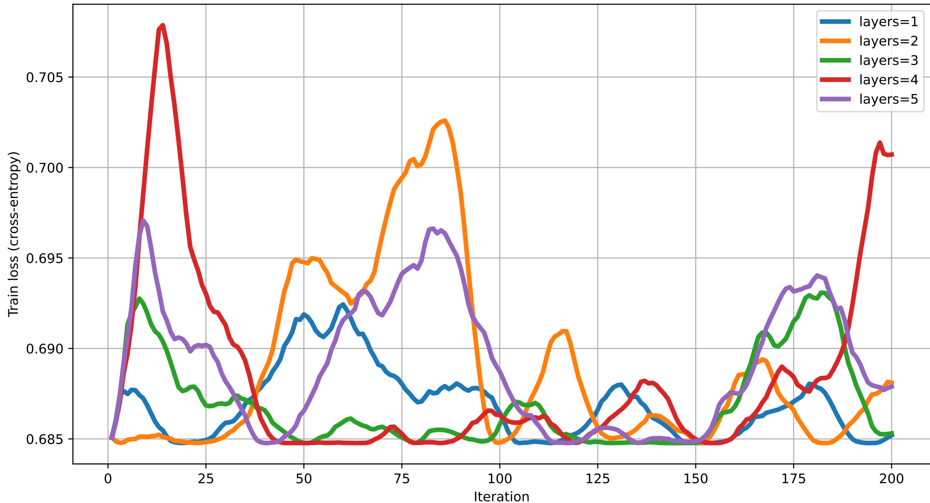
Train loss vs Iteration (dim=15) rot=RZ, ent=chain, gate=CZ
