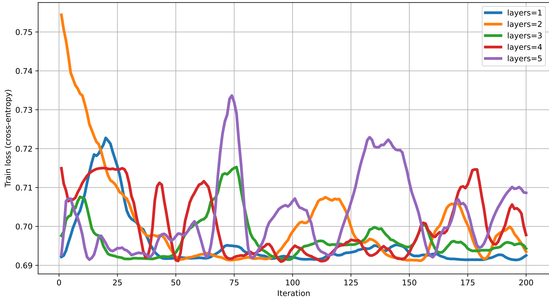
Train loss vs Iteration (dim=3) rot=RX, ent=full, gate=IsingXX
