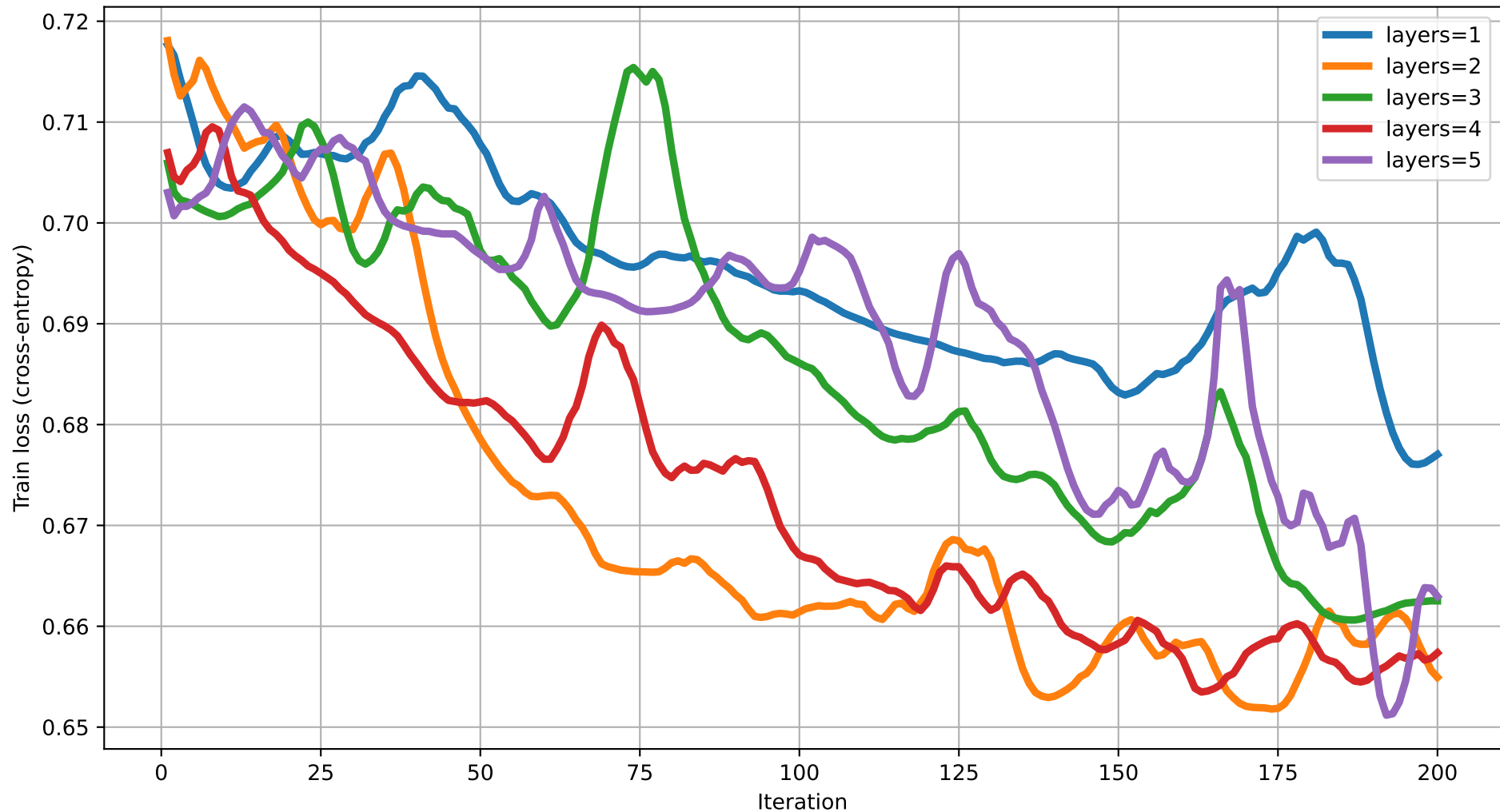
Train loss vs Iteration (dim=6) rot=RYZ, ent=ring, gate=CZ
