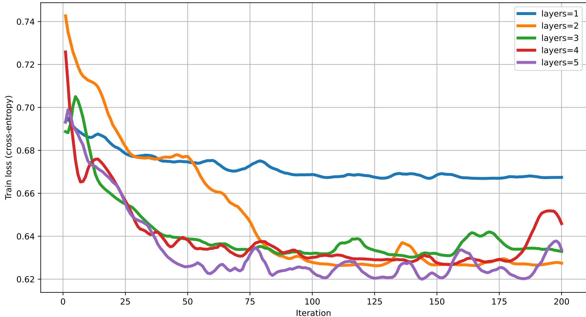
Train loss vs Iteration (degree=3) rot=RZ, ent=full, gate=IsingXX
