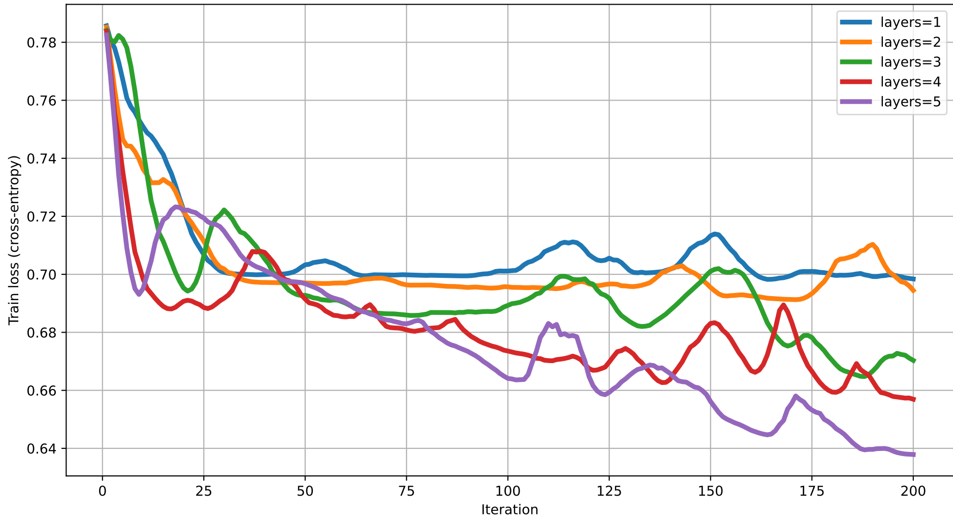
Train loss vs Iteration (dim=9) rot=RX, ent=ring, gate=CZ
