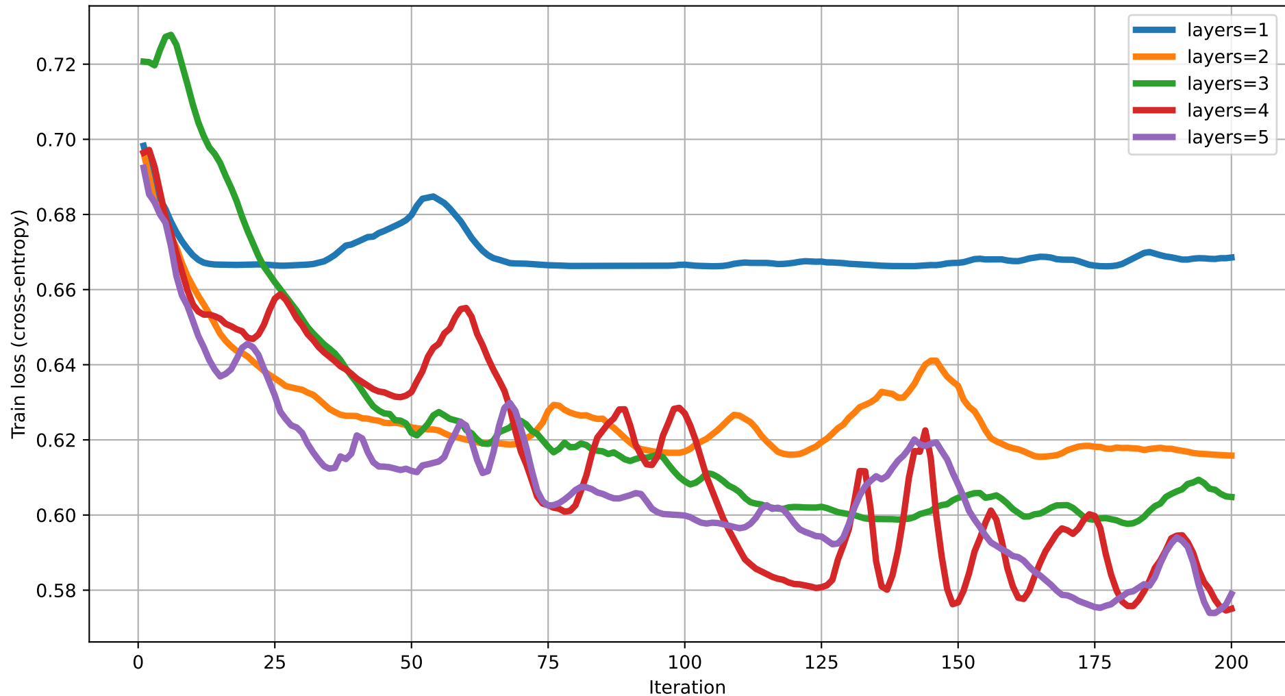
Train loss vs Iteration (dim=10) rot=Rot, ent=chain, gate=CZ
