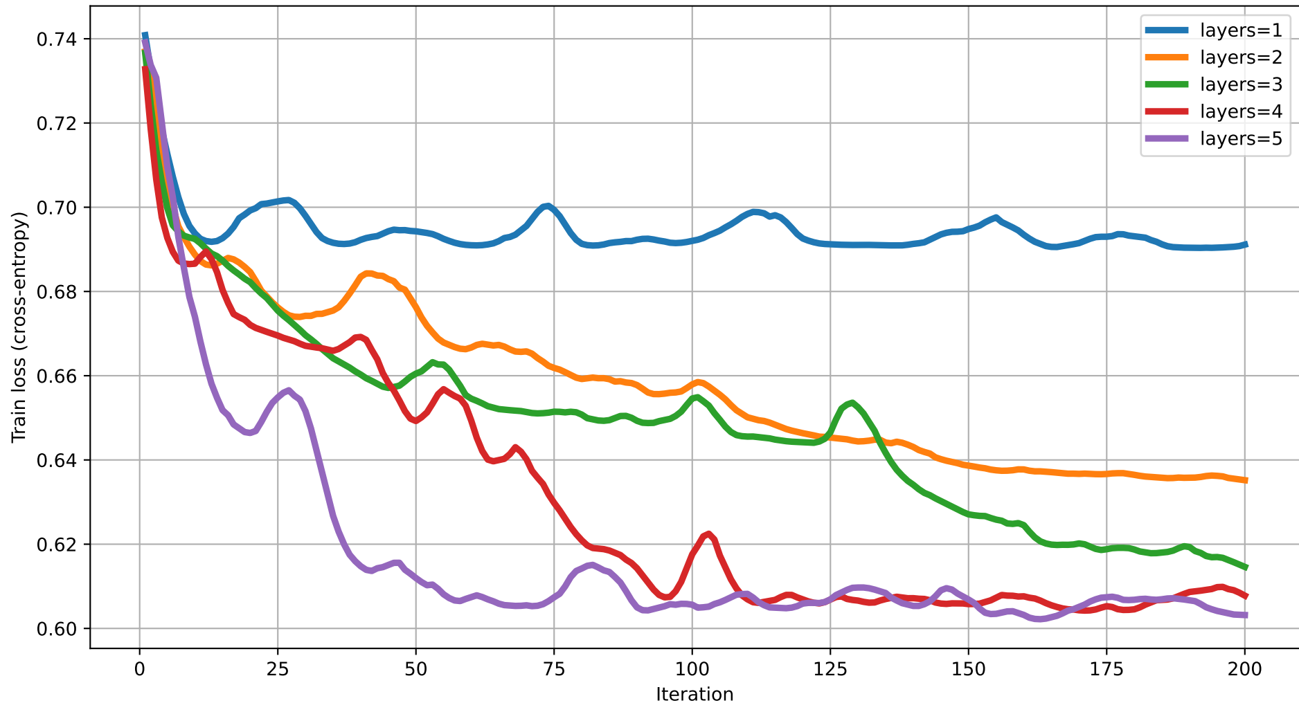
Train loss vs Iteration (degree=5) rot=RY, ent=chain, gate=CZ
