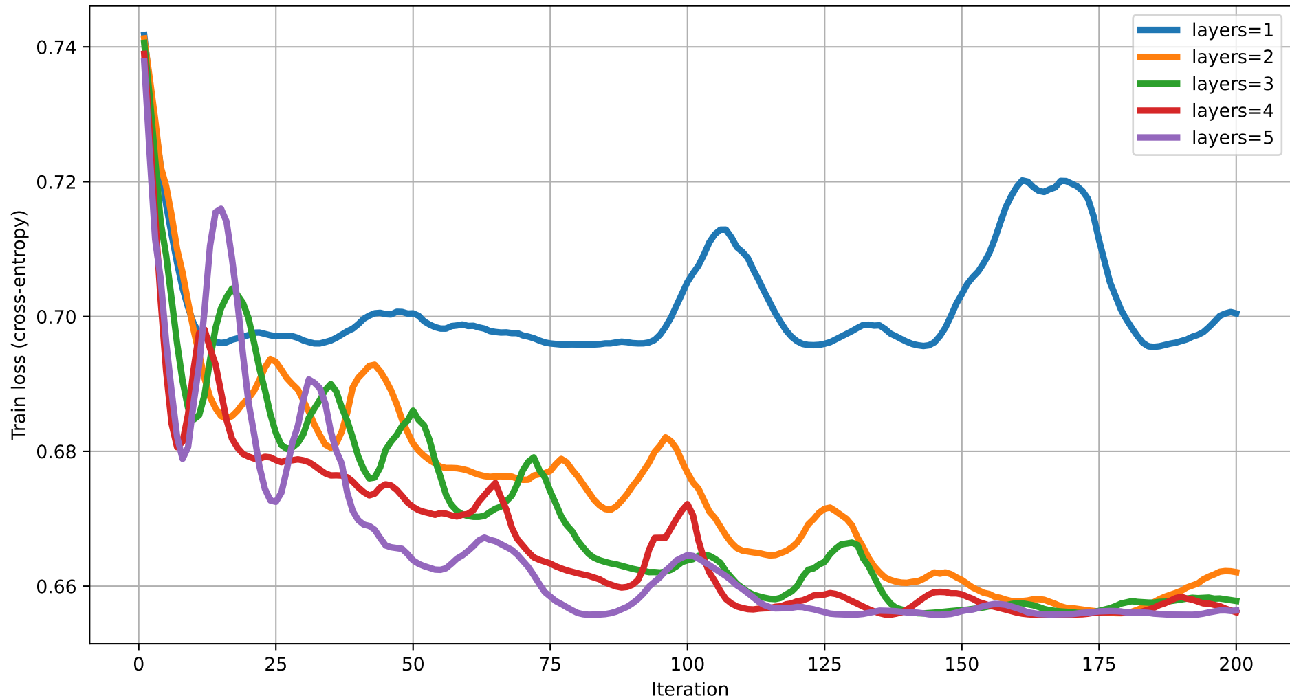
Train loss vs Iteration (degree=5) rot=RX, ent=pairwise, gate=CNOT
