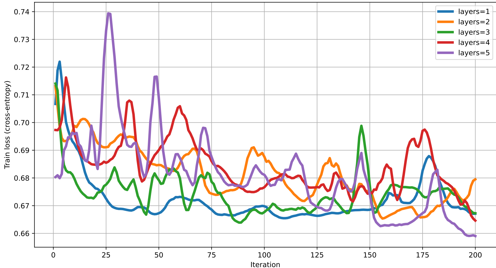
Train loss vs Iteration (dim=12) rot=Rot, ent=ring, gate=IsingXX
