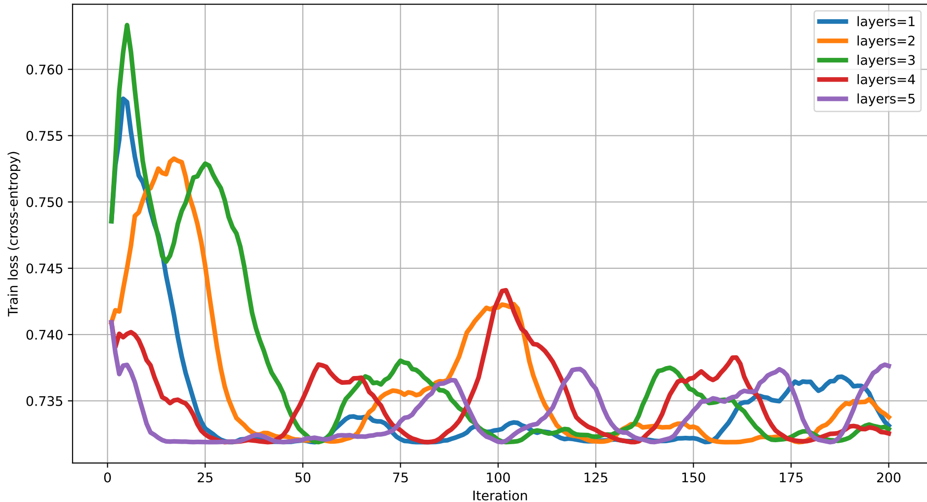
Train loss vs Iteration (dim=3) rot=RZ, ent=full, gate=CZ
