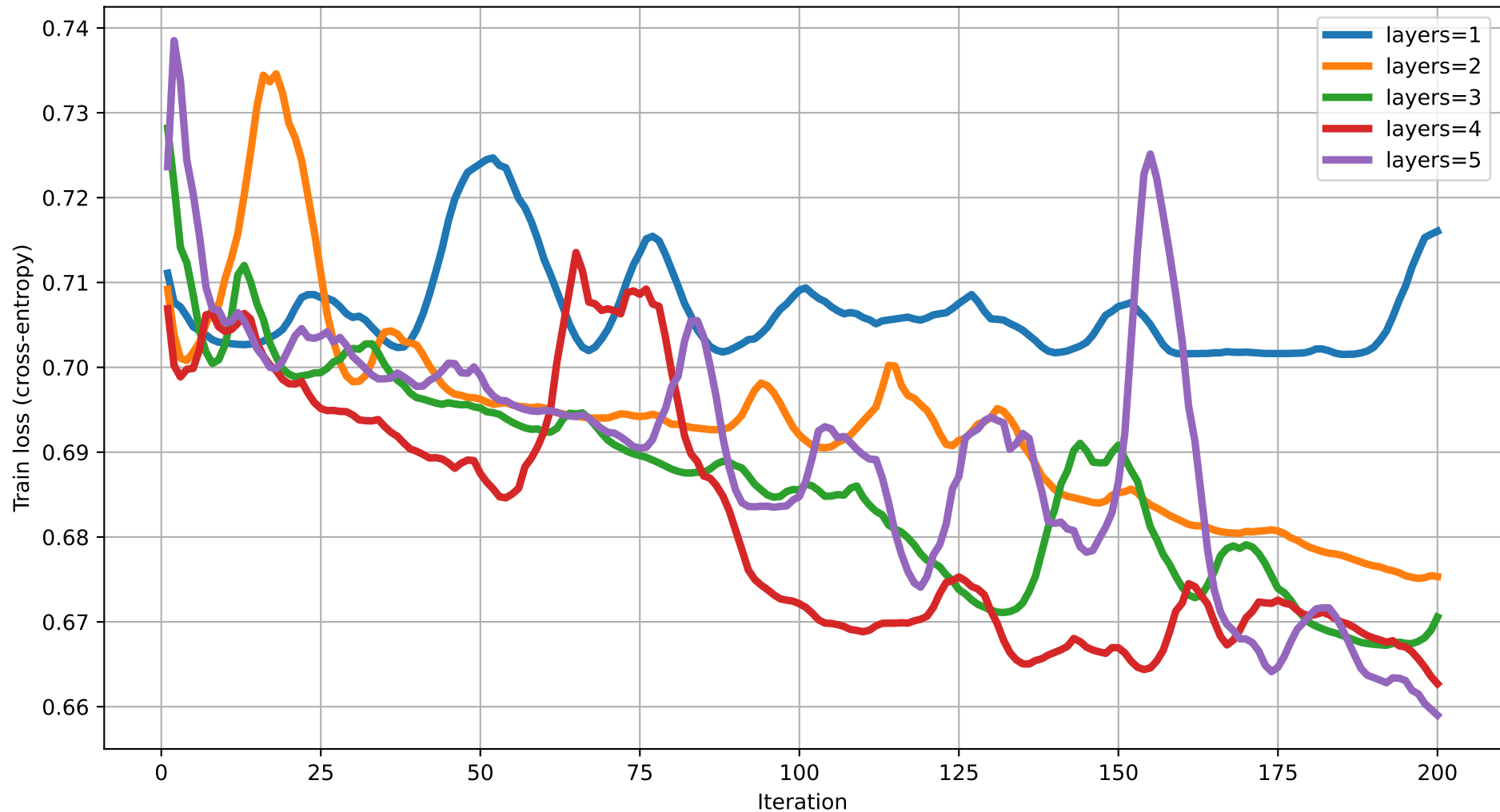
Train loss vs Iteration (dim=11) rot=RYZ, ent=chain, gate=CNOT
