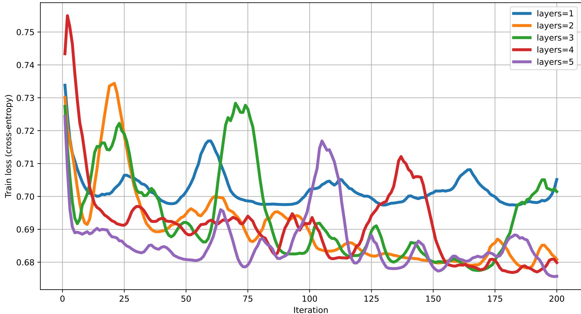
Train loss vs Iteration (dim=19) rot=RY, ent=chain, gate=CZ
