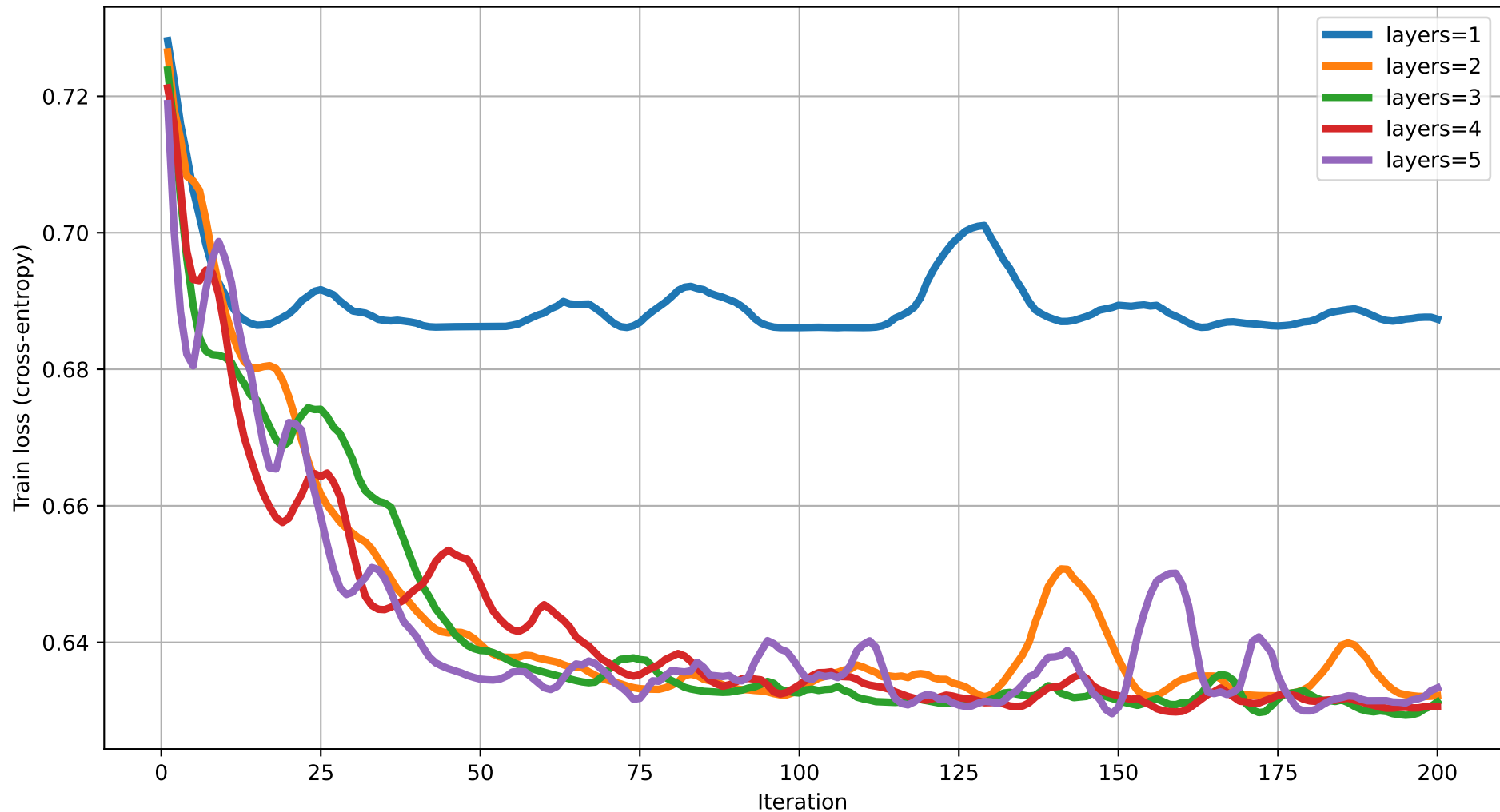
Train loss vs Iteration (degree=2) rot=YRZ, ent=pairwise, gate=CNOT
