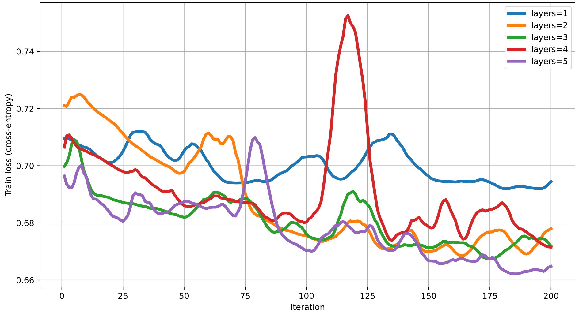
Train loss vs Iteration (dim=14) rot=RY, ent=ring, gate=CNOT
