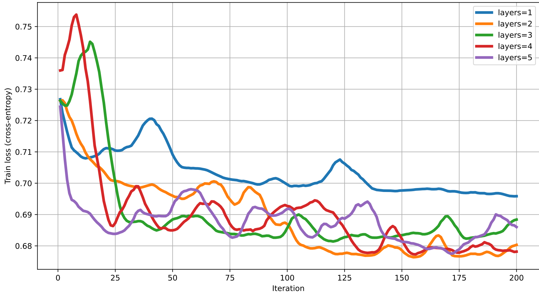
Train loss vs Iteration (dim=5) rot=RX, ent=pairwise, gate=CZ
