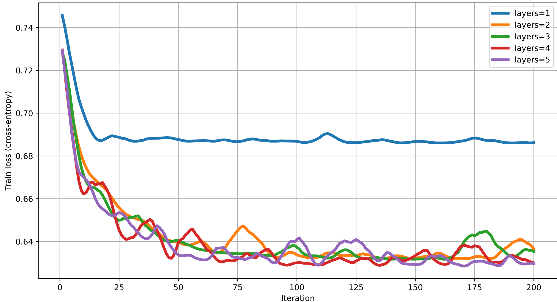
Train loss vs Iteration (degree=2) rot=RX, ent=chain, gate=CZ
