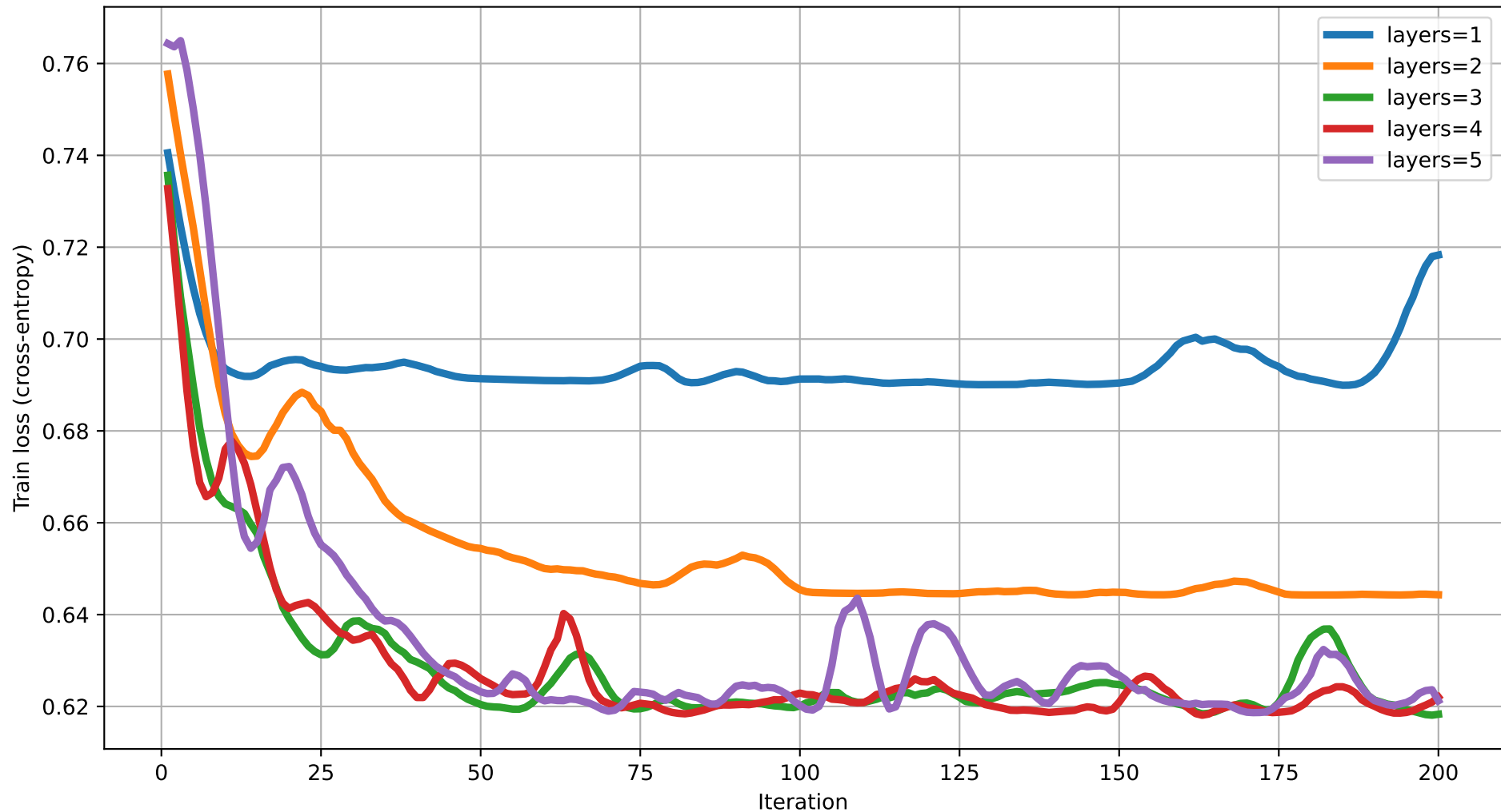
Train loss vs Iteration (degree=5) rot=RYZ, ent=pairwise, gate=CNOT
