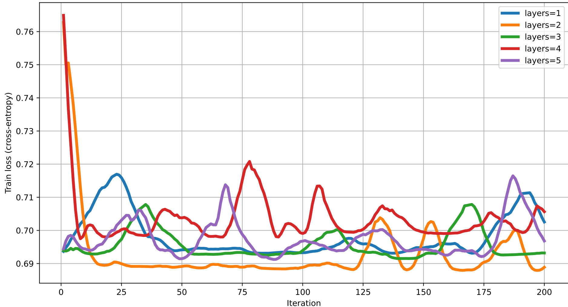
Train loss vs Iteration (dim=17) rot=RY, ent=chain, gate=IsingXX
