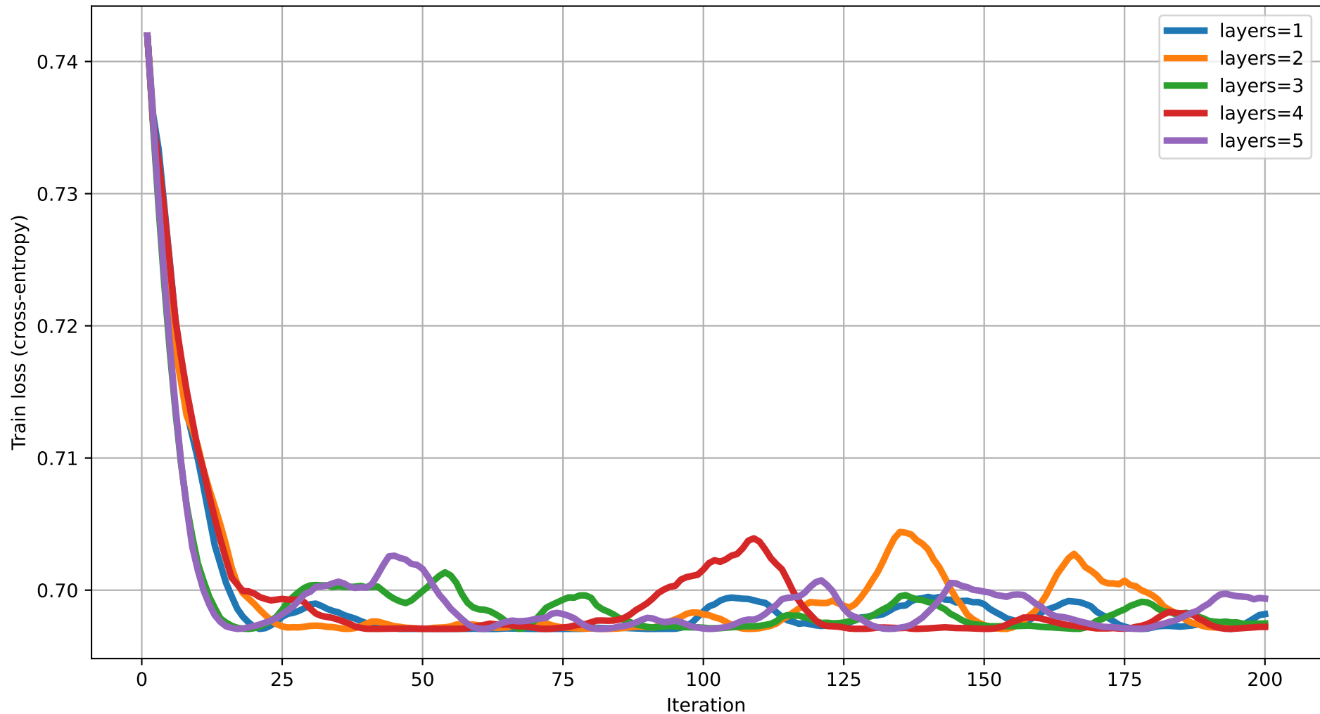
Train loss vs Iteration (degree=5) rot=RZ, ent=full, gate=CZ
