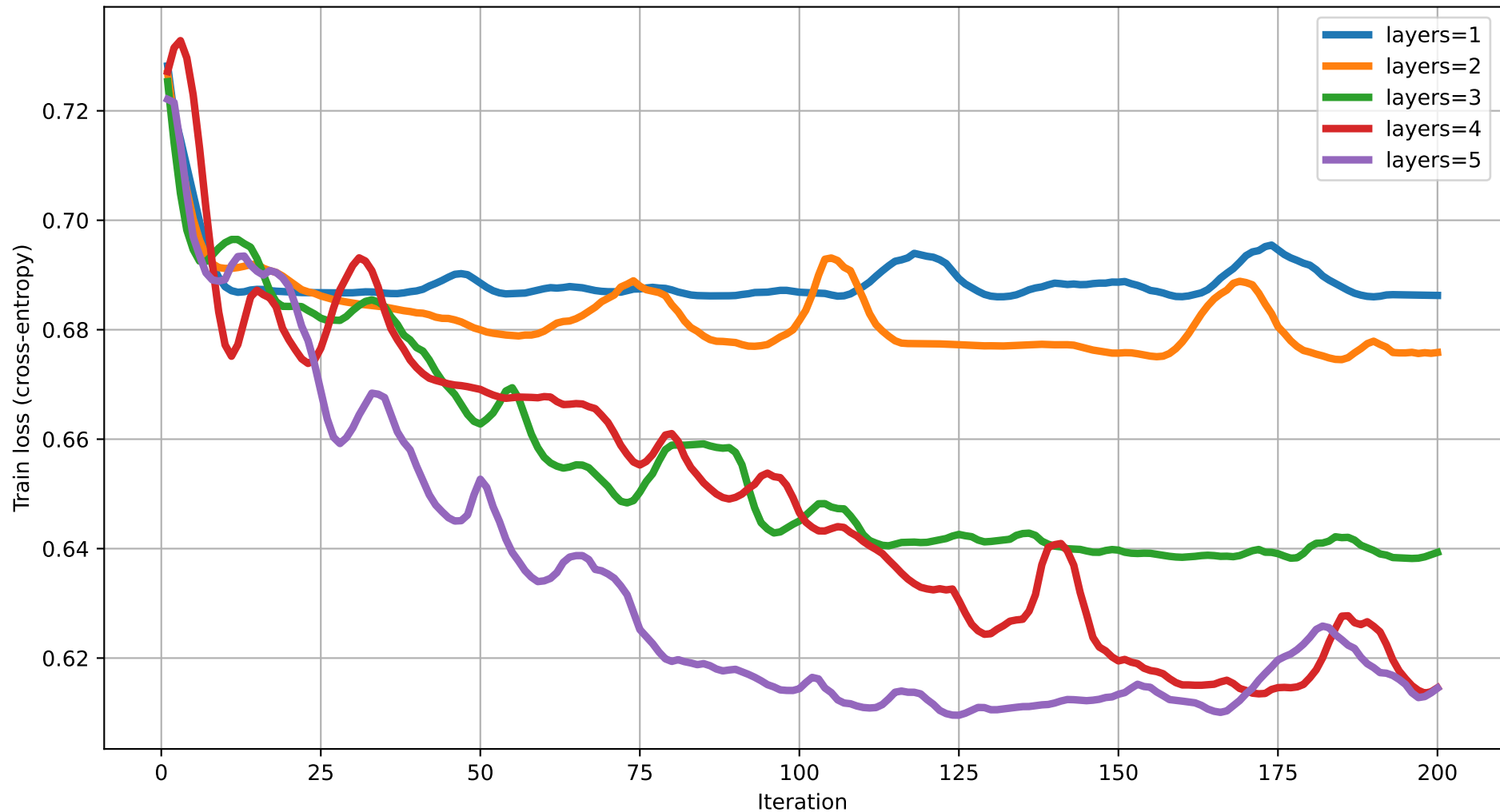
Train loss vs Iteration (degree=2) rot=RY, ent=chain, gate=CZ
