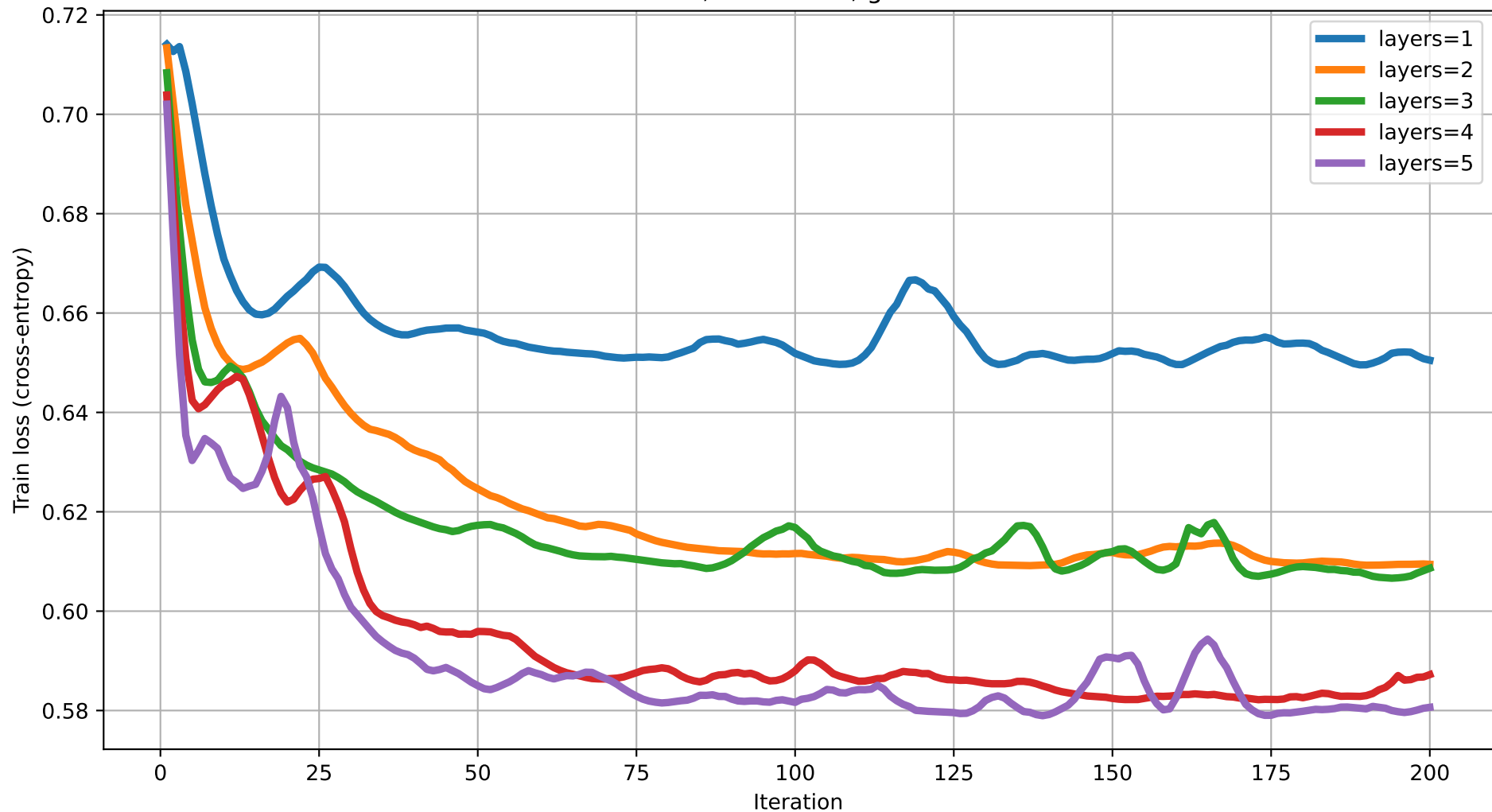
Train loss vs Iteration (degree=4) rot=RYZ, ent=chain, gate=CNOT
