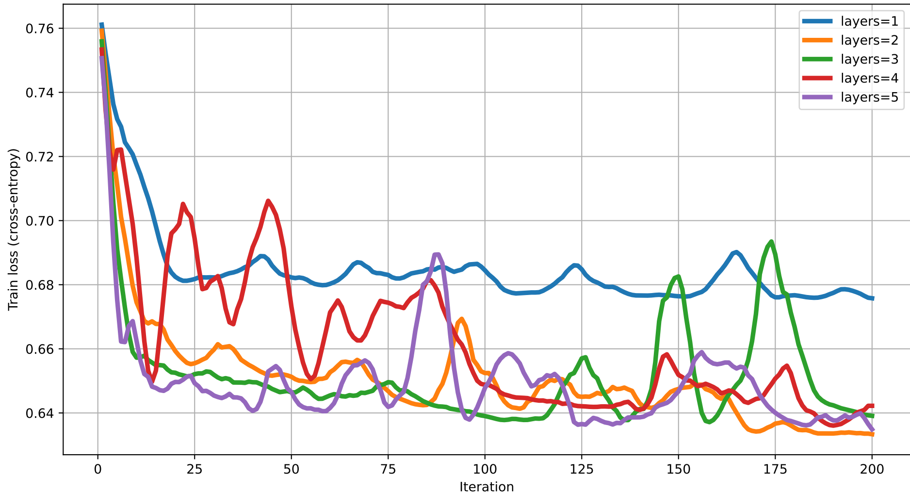
Train loss vs Iteration (dim=8) rot=Rot, ent=pairwise, gate=CNOT
