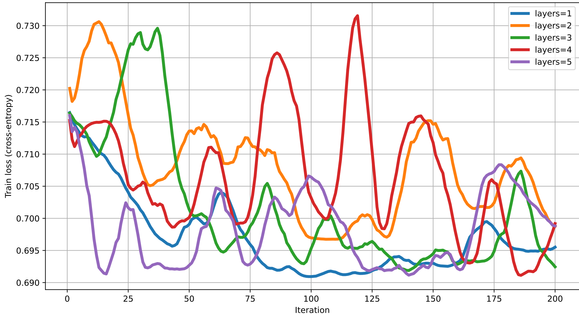
Train loss vs Iteration (dim=3) rot=RX, ent=chain, gate=CNOT
