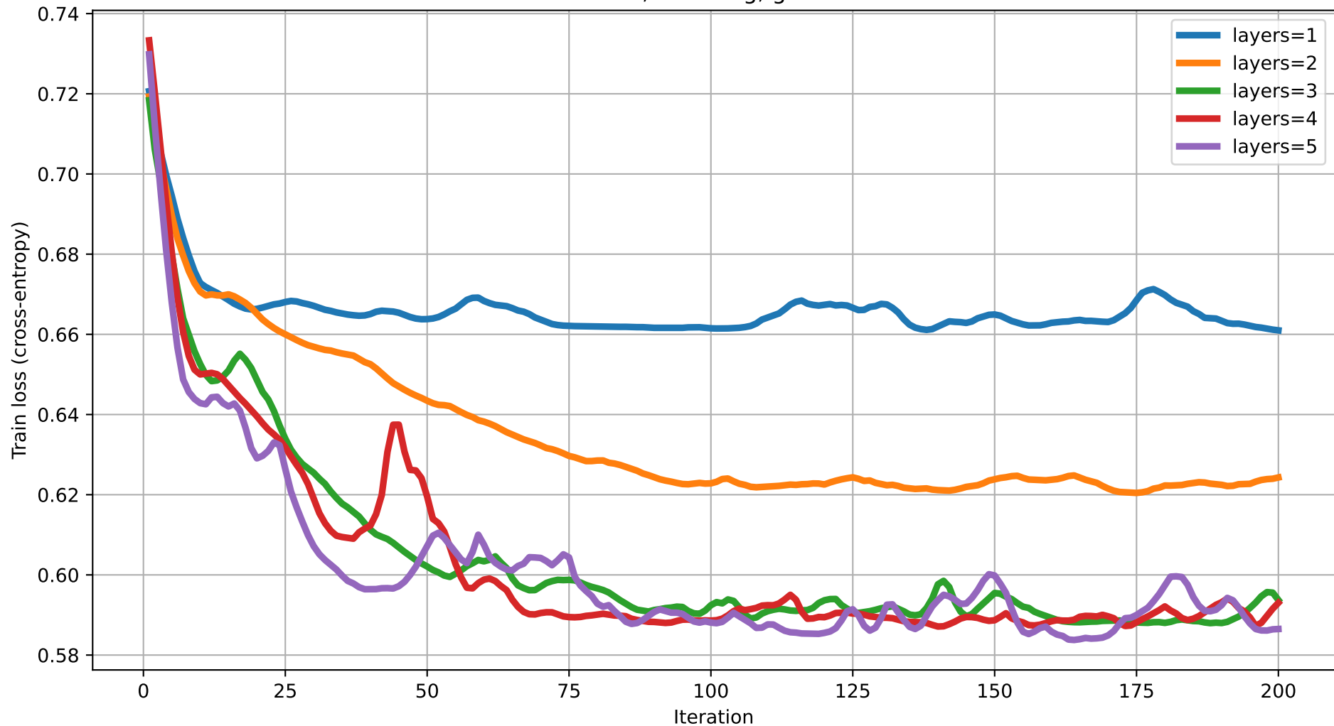
Train loss vs Iteration (degree=3) rot=Rot, ent=ring, gate=CZ
