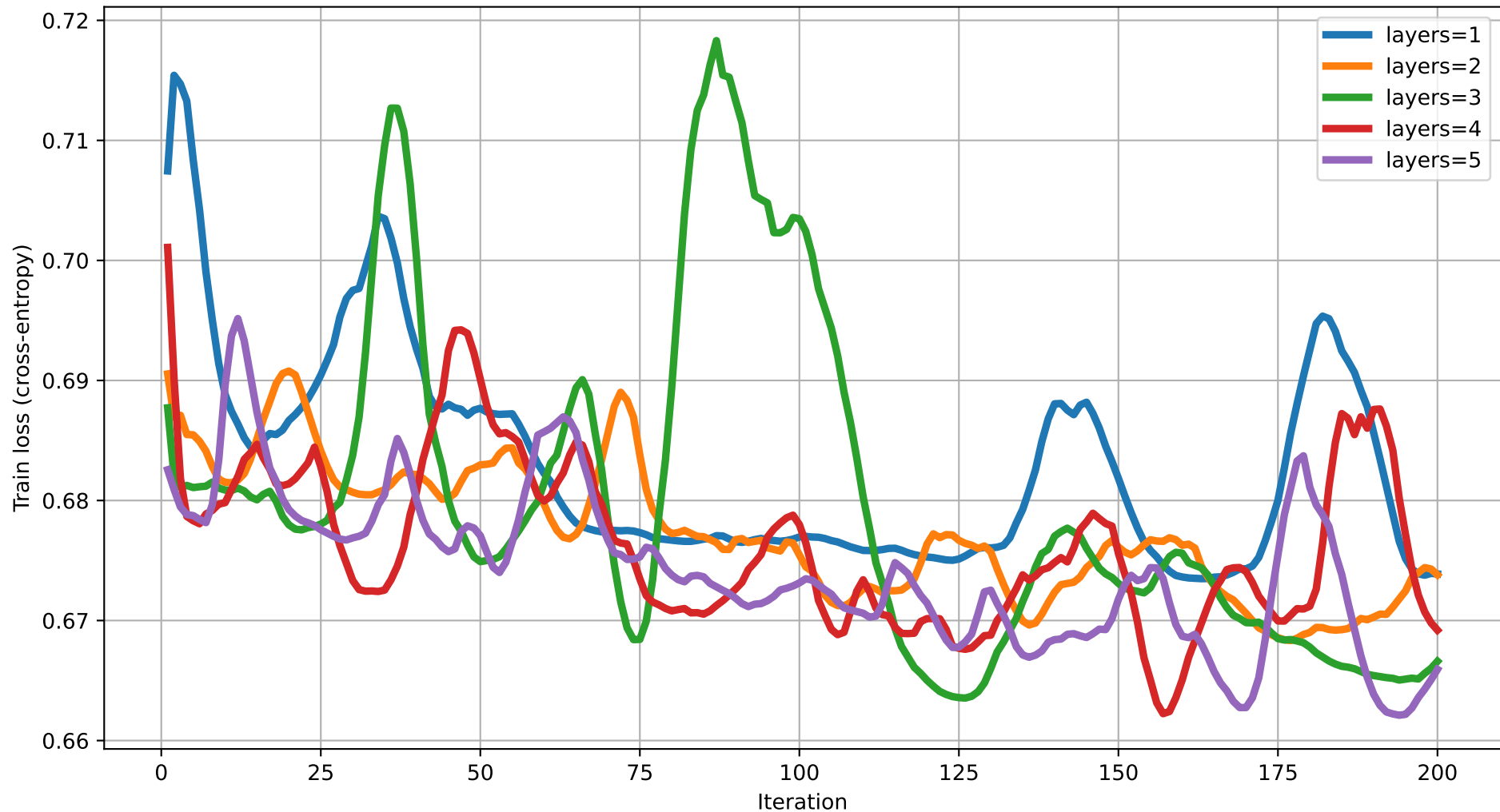
Train loss vs Iteration (dim=13) rot=RYZ, ent=full, gate=CNOT
