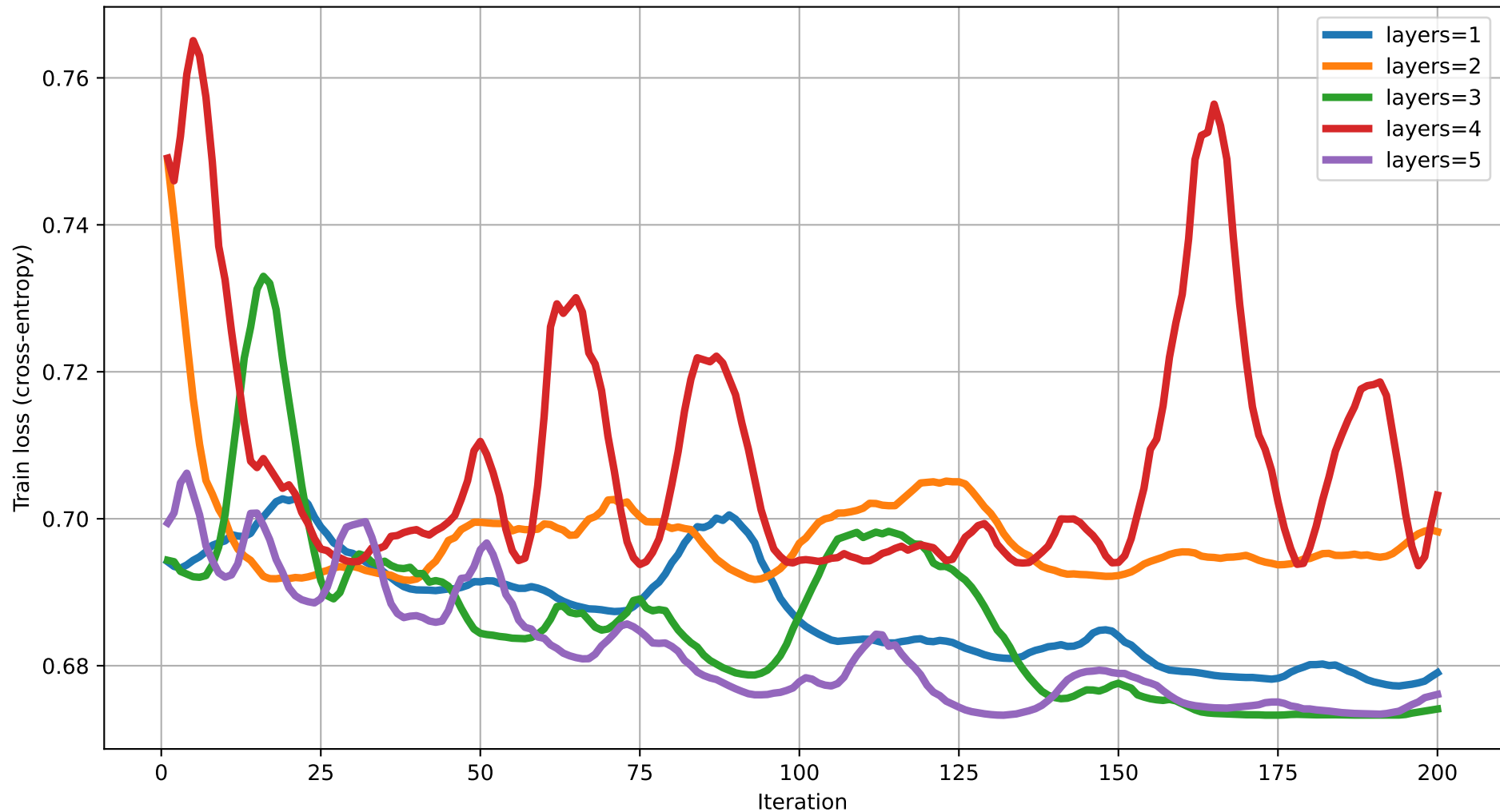
Train loss vs Iteration (dim=19) rot=RX, ent=chain, gate=IsingXX
