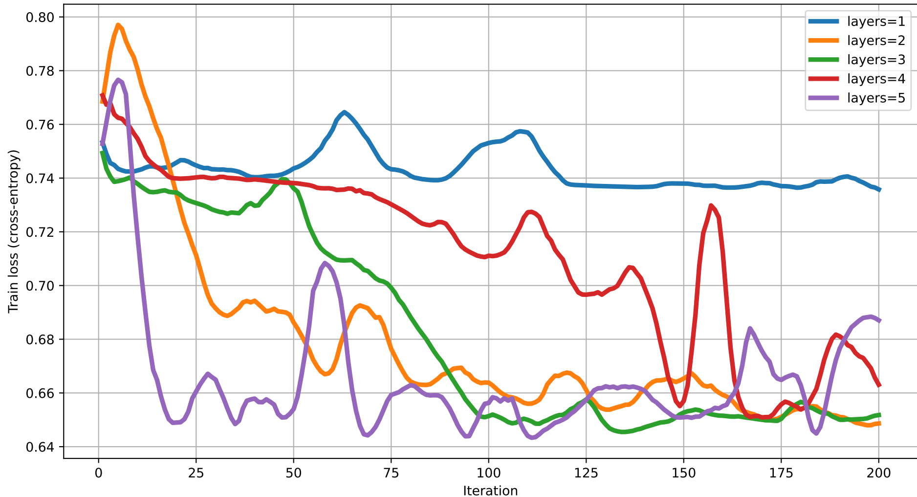
Train loss vs Iteration (dim=5) rot=RY, ent=pairwise, gate=CNOT
