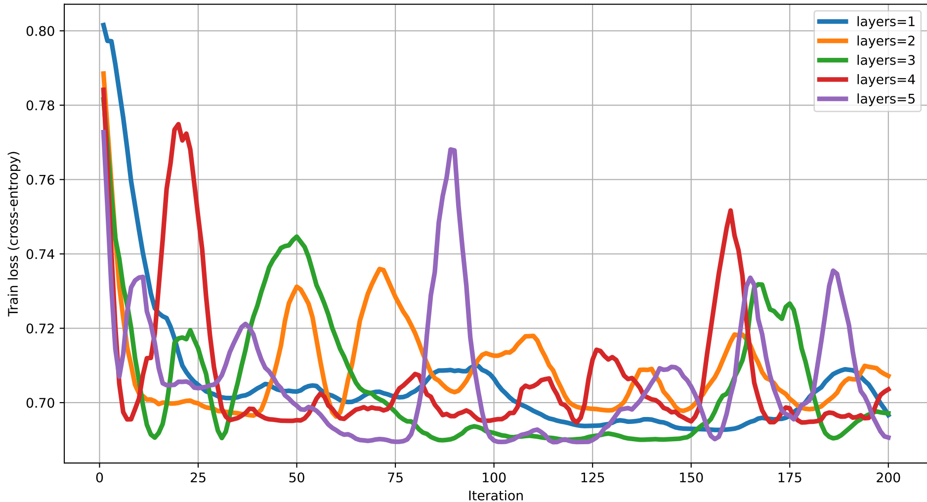
Train loss vs Iteration (dim=2) rot=RYZ, ent=ring, gate=IsingXX
