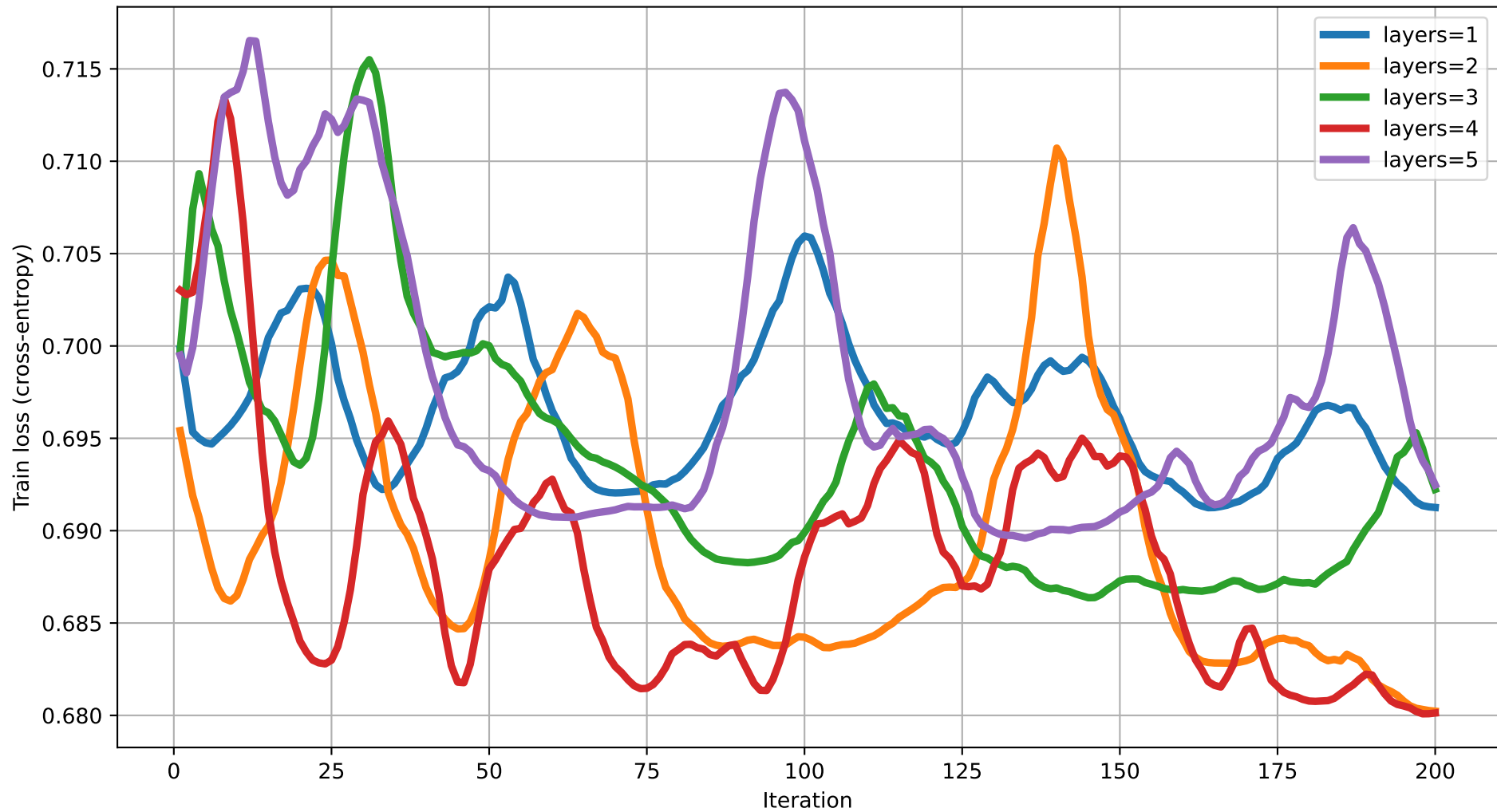
Train loss vs Iteration (dim=13) rot=RZ, ent=ring, gate=IsingXX
