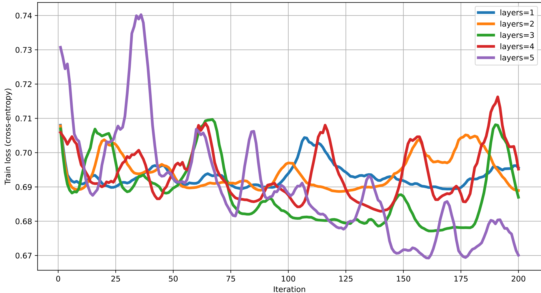
Train loss vs Iteration (dim=20) rot=RY, ent=full, gate=CZ
