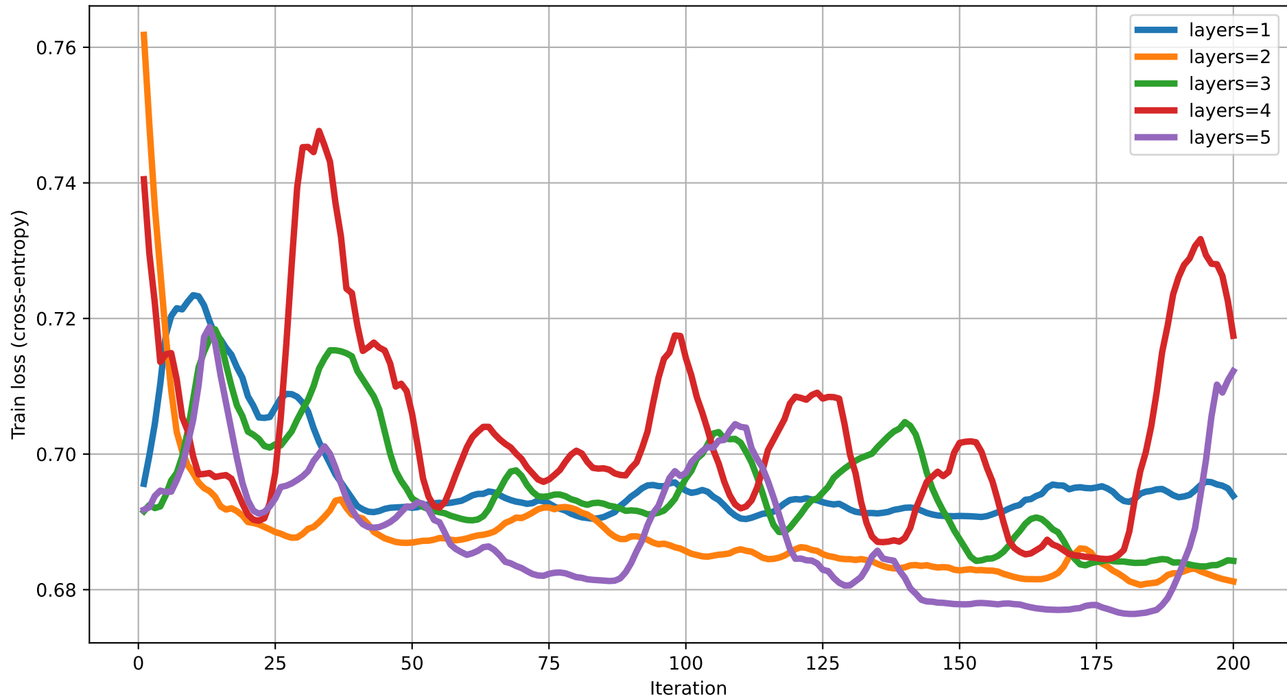
Train loss vs Iteration (dim=18) rot=RZ, ent=chain, gate=IsingXX
