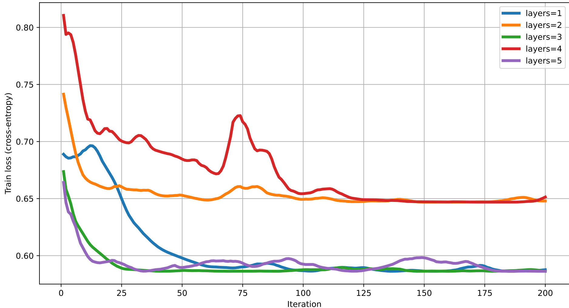
Train loss vs Iteration (dim=2) rot=RX, ent=pairwise, gate=IsingXX
