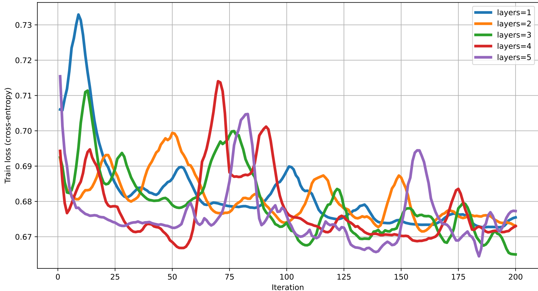
Train loss vs Iteration (dim=13) rot=Rot, ent=full, gate=CZ
