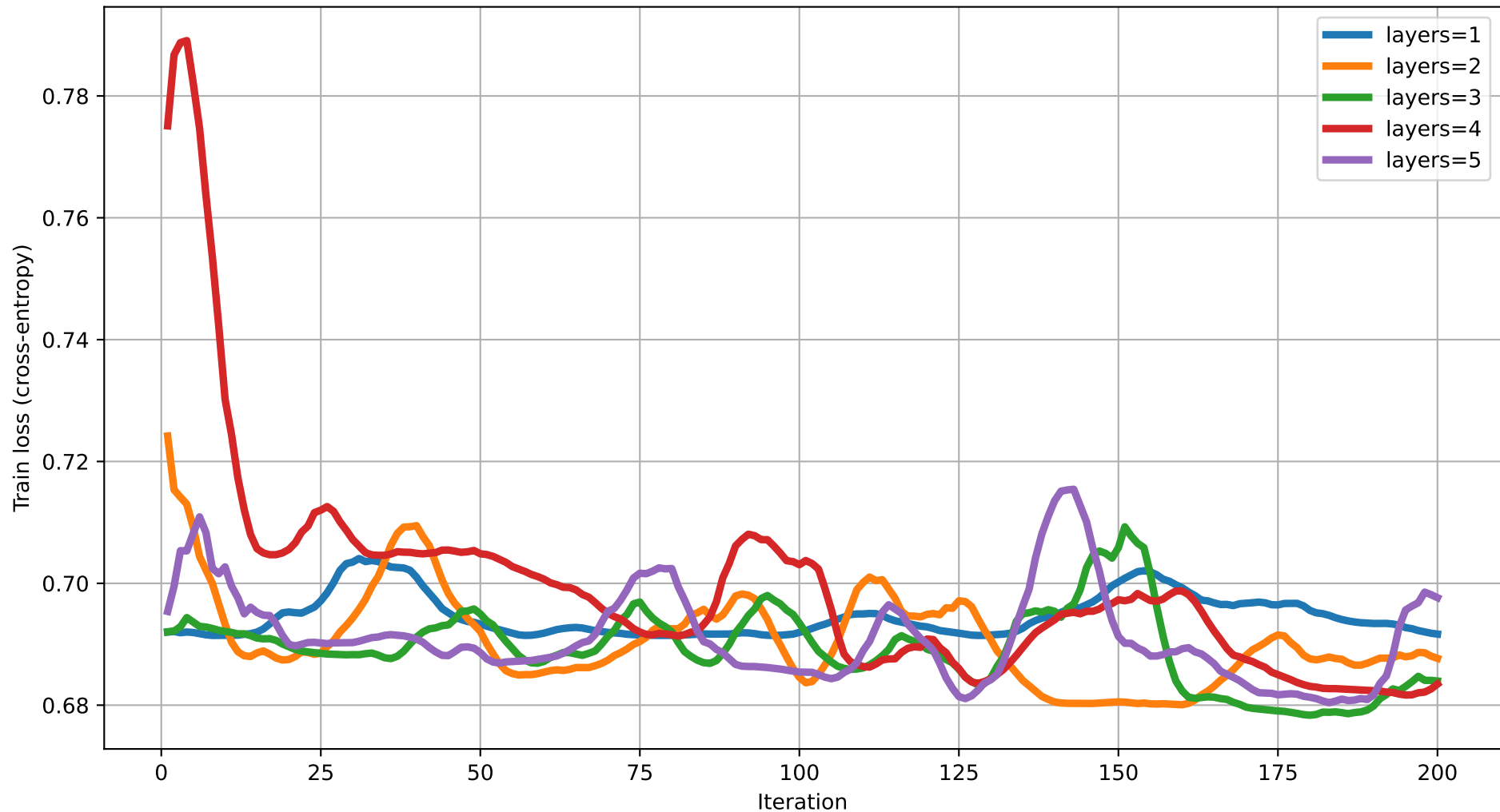
Train loss vs Iteration (dim=9) rot=RY, ent=full, gate=IsingXX
