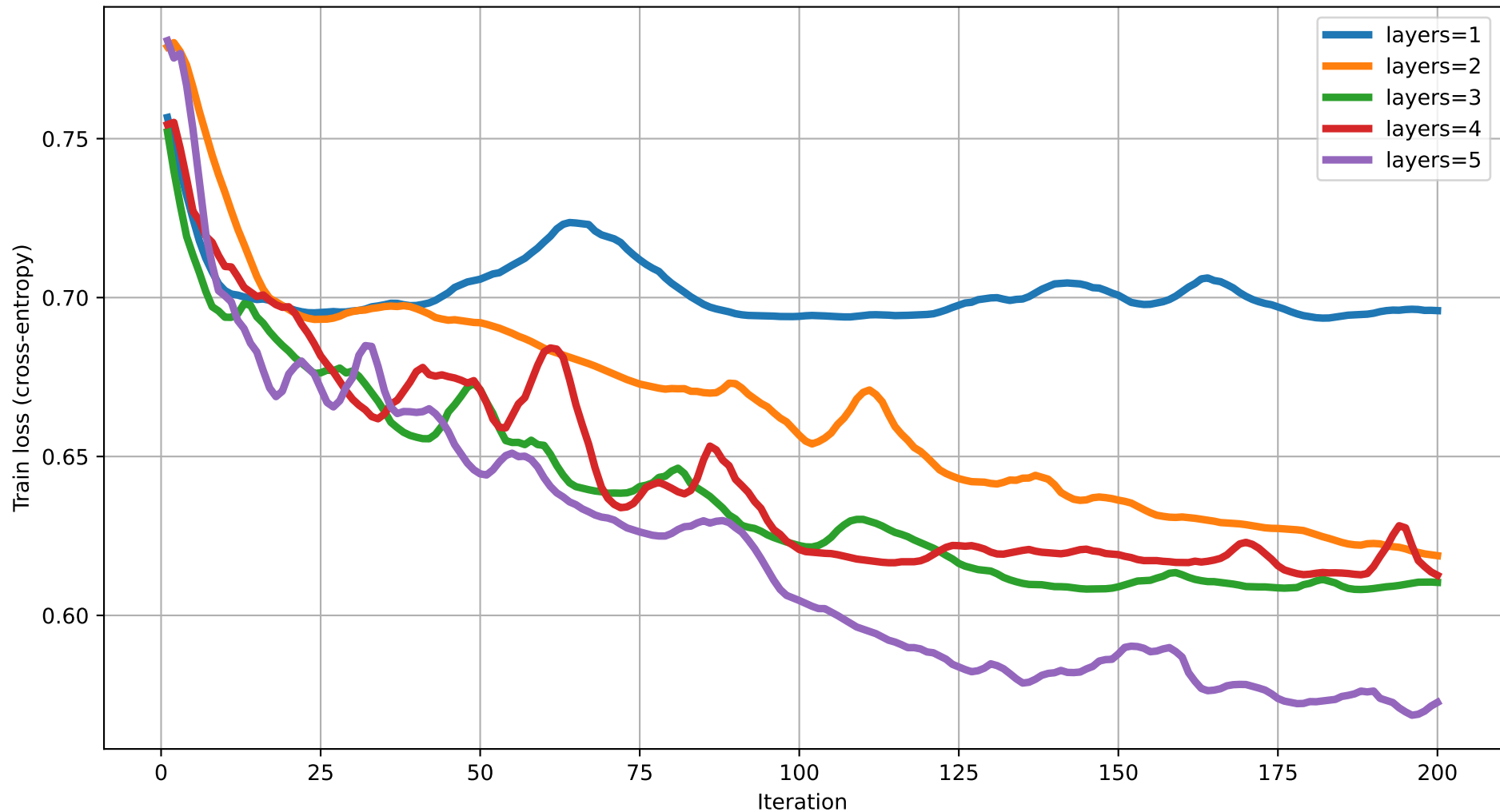
Train loss vs Iteration (dim=18) rot=Rot, ent=chain, gate=CZ
