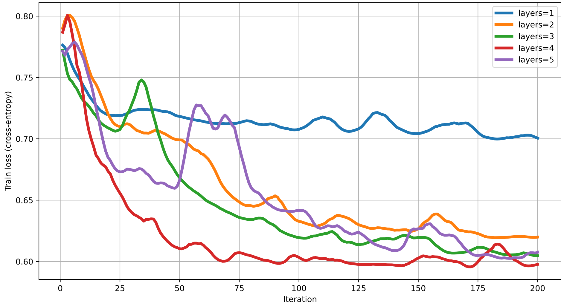
Train loss vs Iteration (dim=9) rot=RYZ, ent=full, gate=CZ
