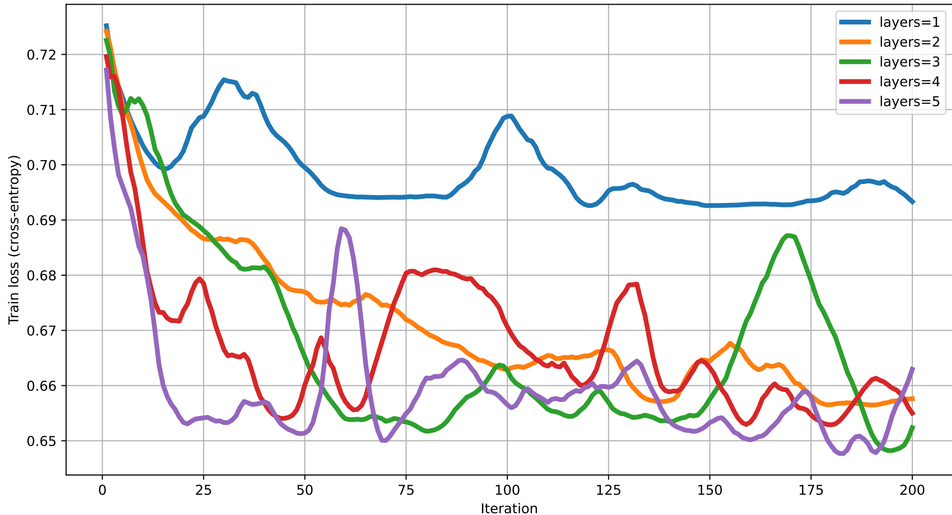
Train loss vs Iteration (dim=5) rot=RYZ, ent=pairwise, gate=CZ
