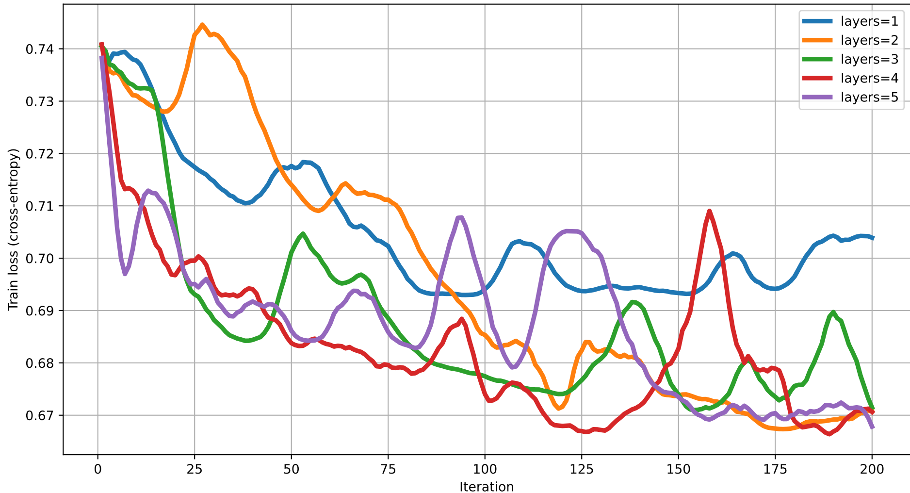
Train loss vs Iteration (dim=3) rot=RX, ent=pairwise, gate=CZ
