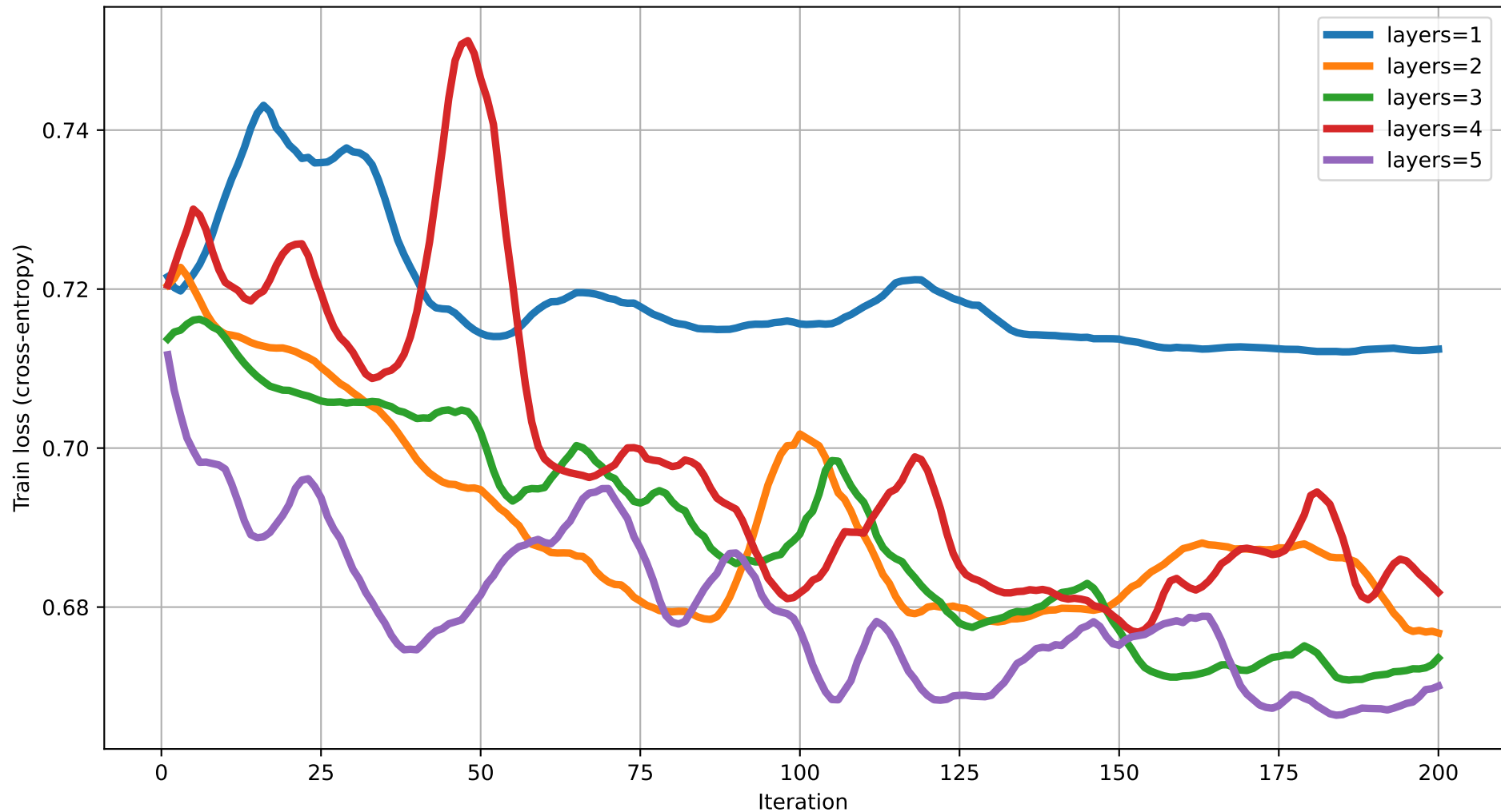
Train loss vs Iteration (dim=3) rot=RYZ, ent=pairwise, gate=CNOT
