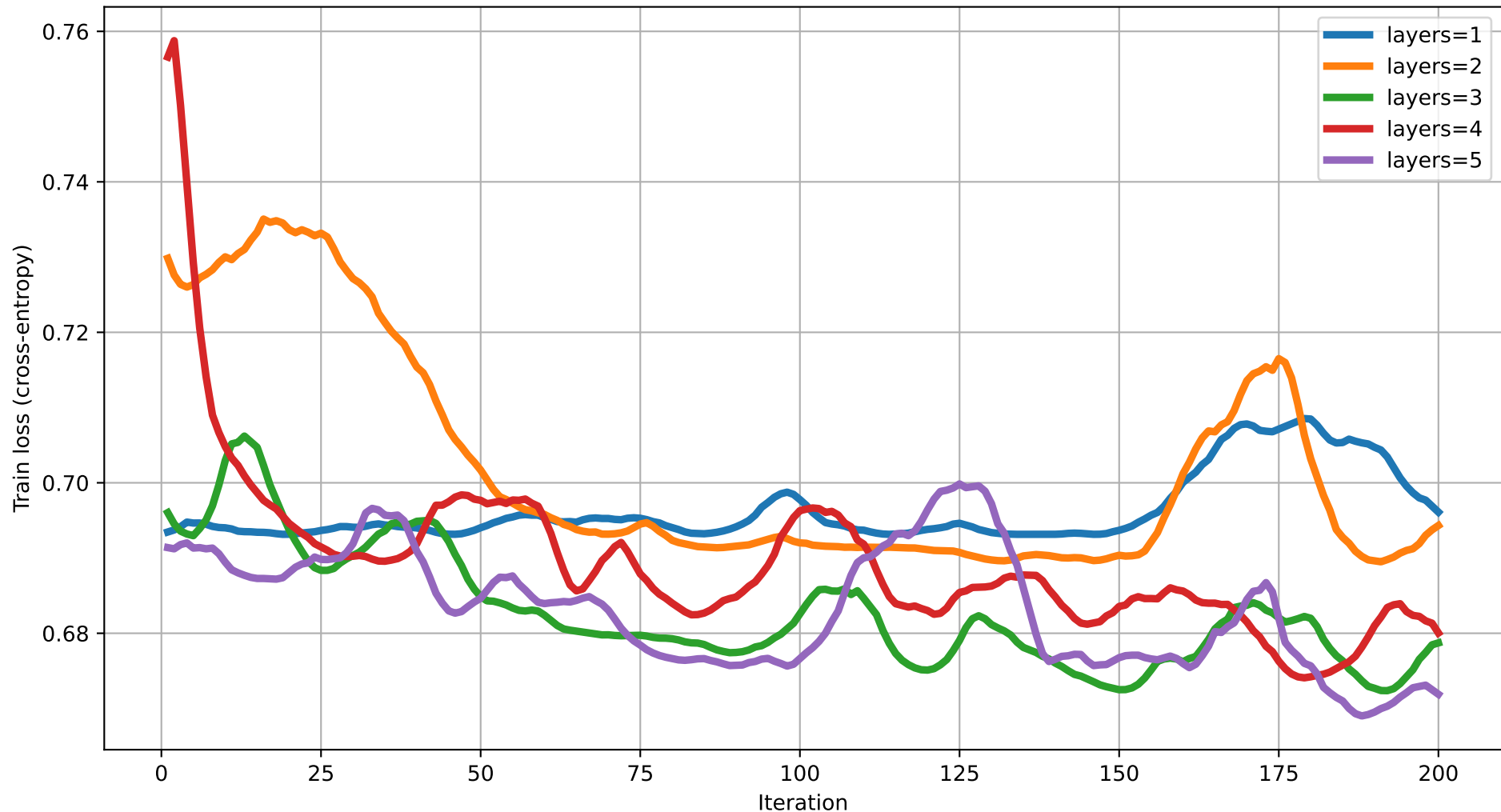
Train loss vs Iteration (dim=3) rot=RY, ent=full, gate=IsingXX
