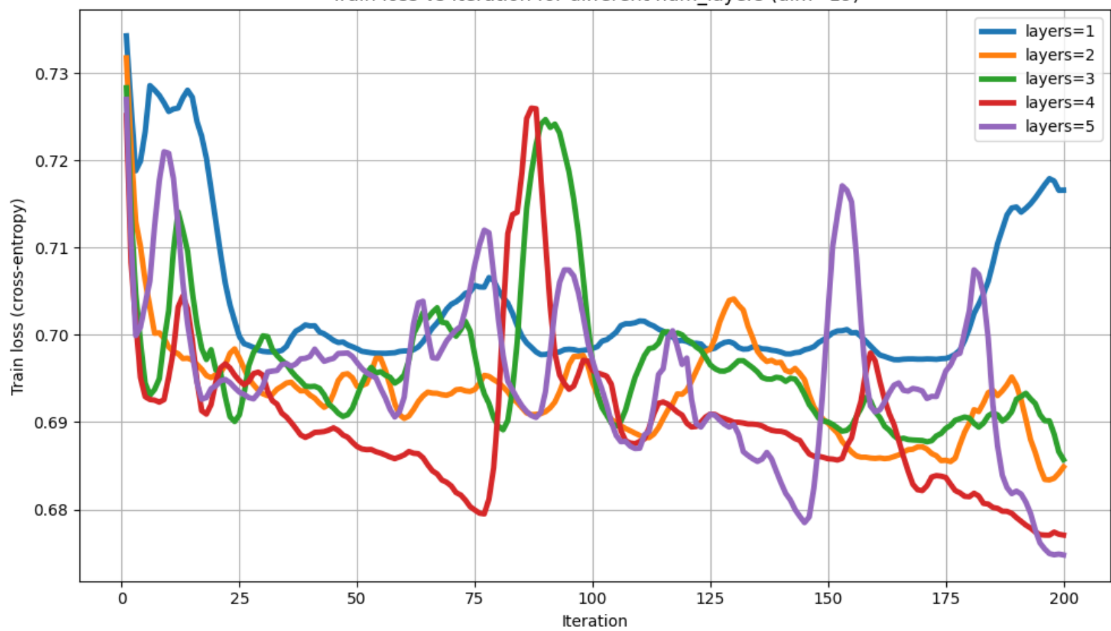
Train loss vs Iteration for different num_layers (dim=19)
