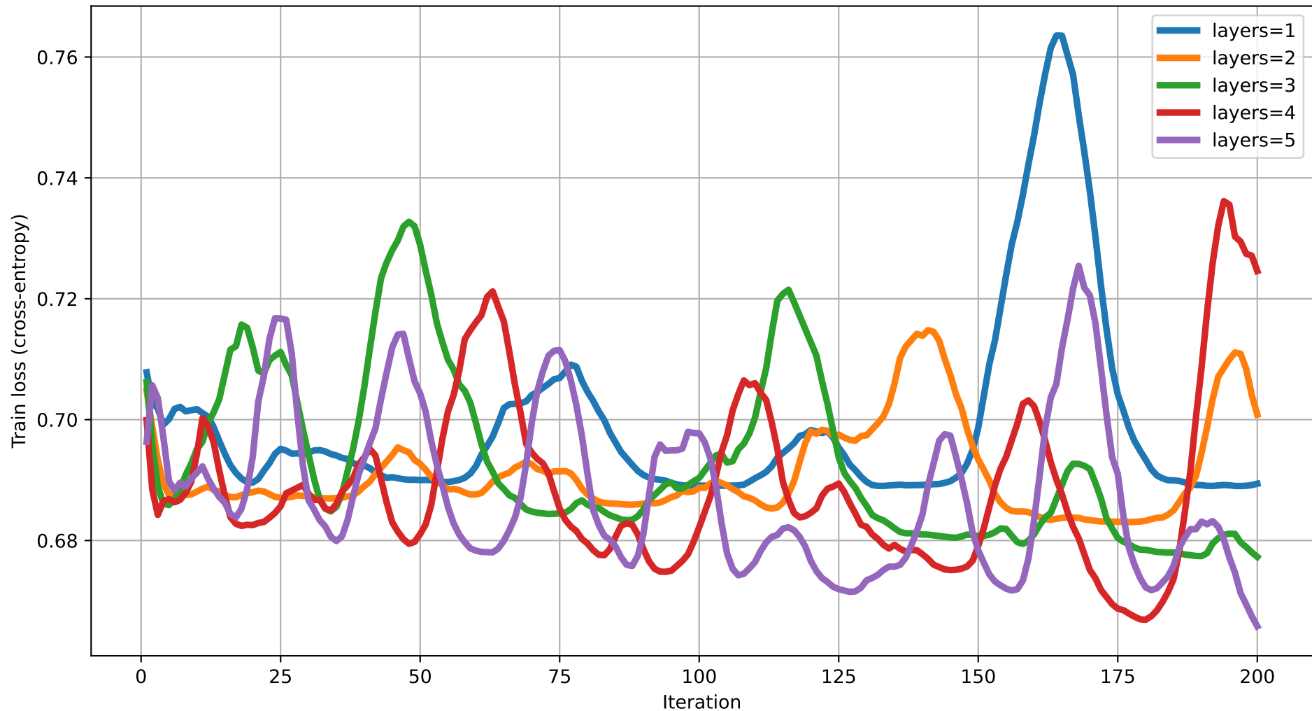
Train loss vs Iteration (dim=20) rot=RY, ent=chain, gate=CNOT
