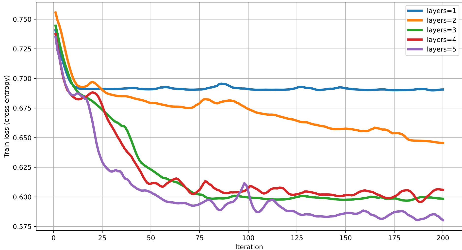
Train loss vs Iteration (degree=5) rot=RY, ent=full, gate=CZ
