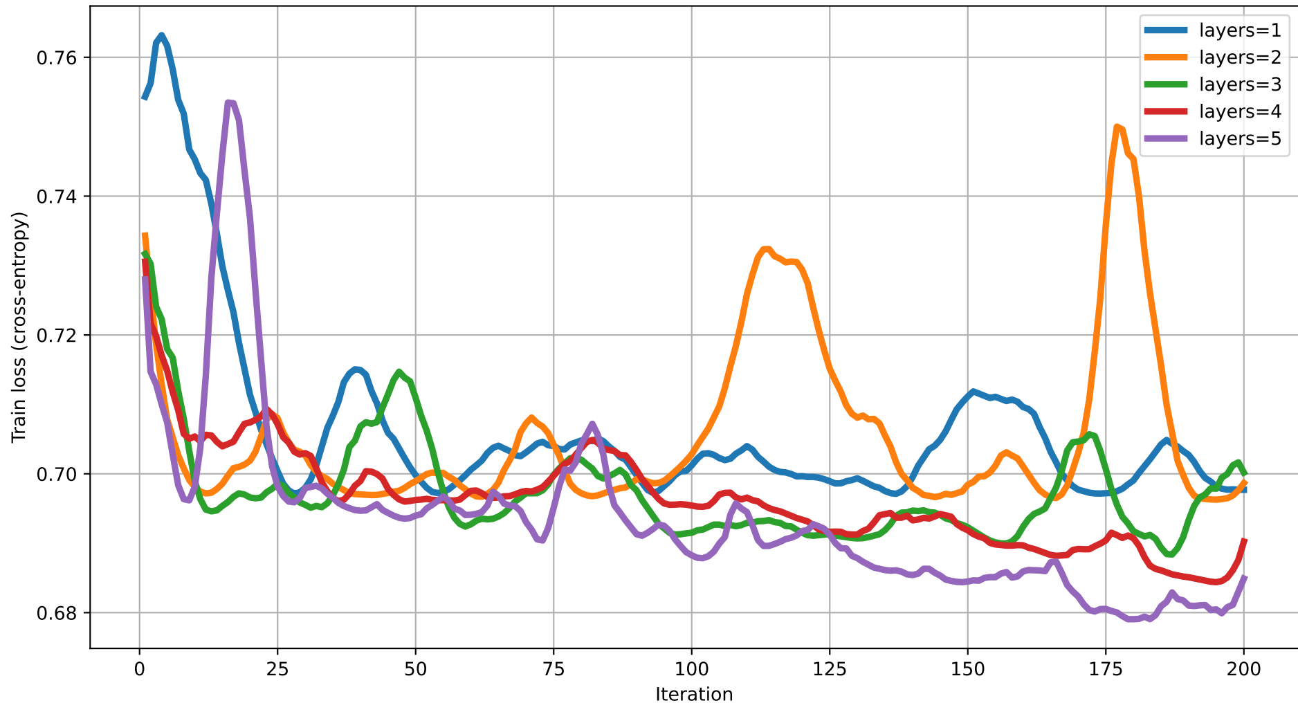
Train loss vs Iteration (dim=18) rot=RYZ, ent=ring, gate=CZ
