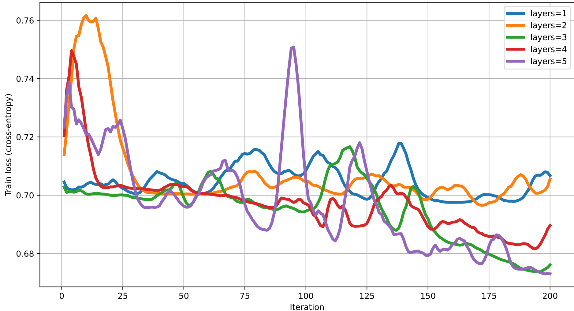
Train loss vs Iteration (dim=12) rot=RY, ent=pairwise, gate=CZ
