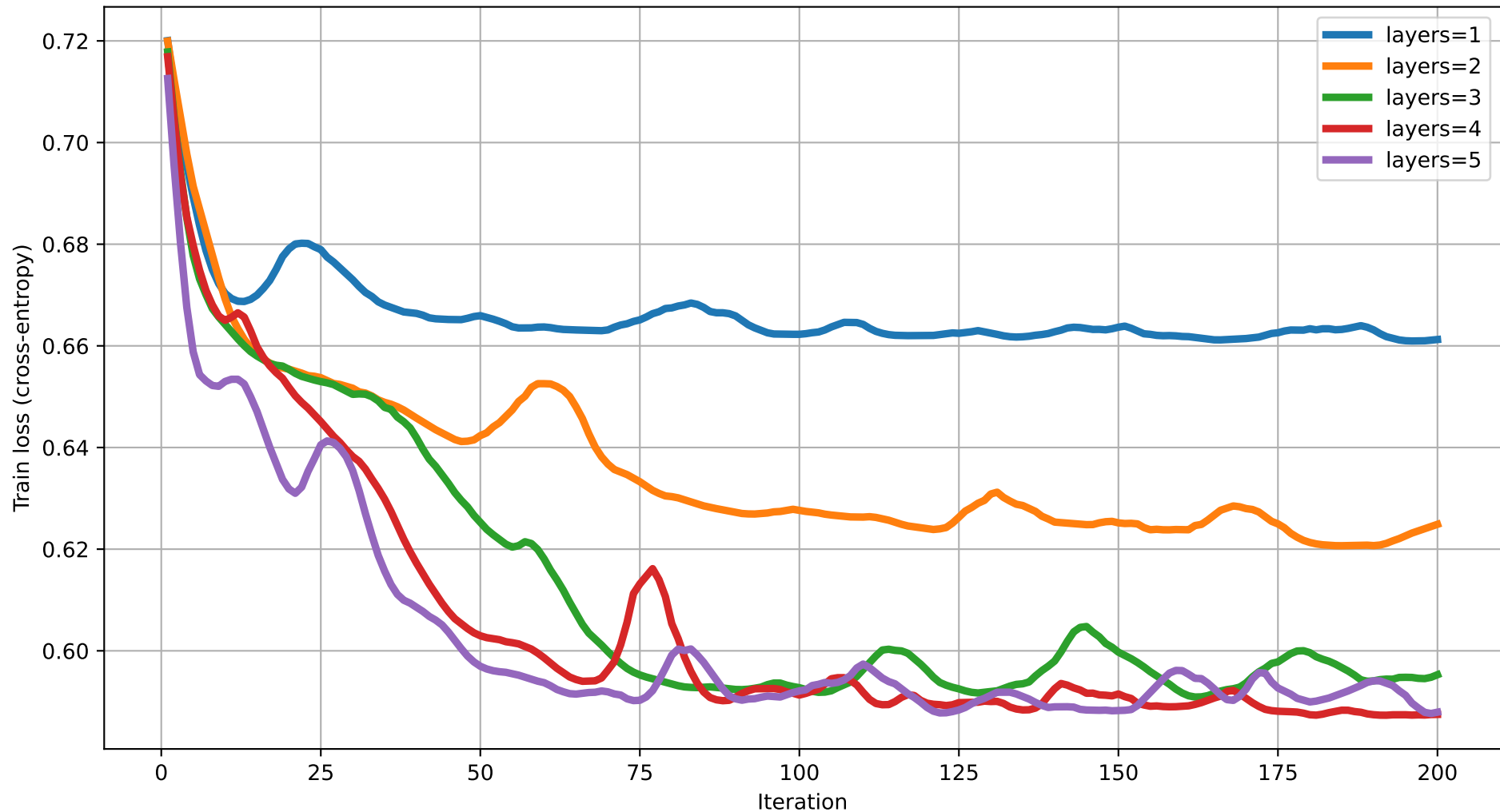
Train loss vs Iteration (degree=3) rot=RY, ent=ring, gate=CZ
