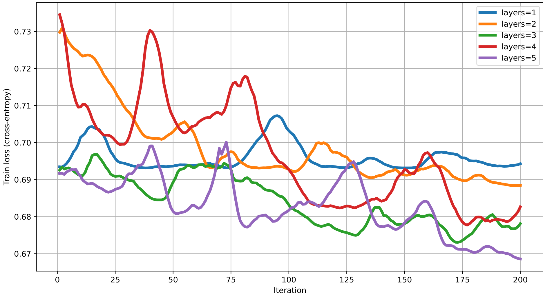
Train loss vs Iteration (dim=3) rot=RY, ent=pairwise, gate=IsingXX
