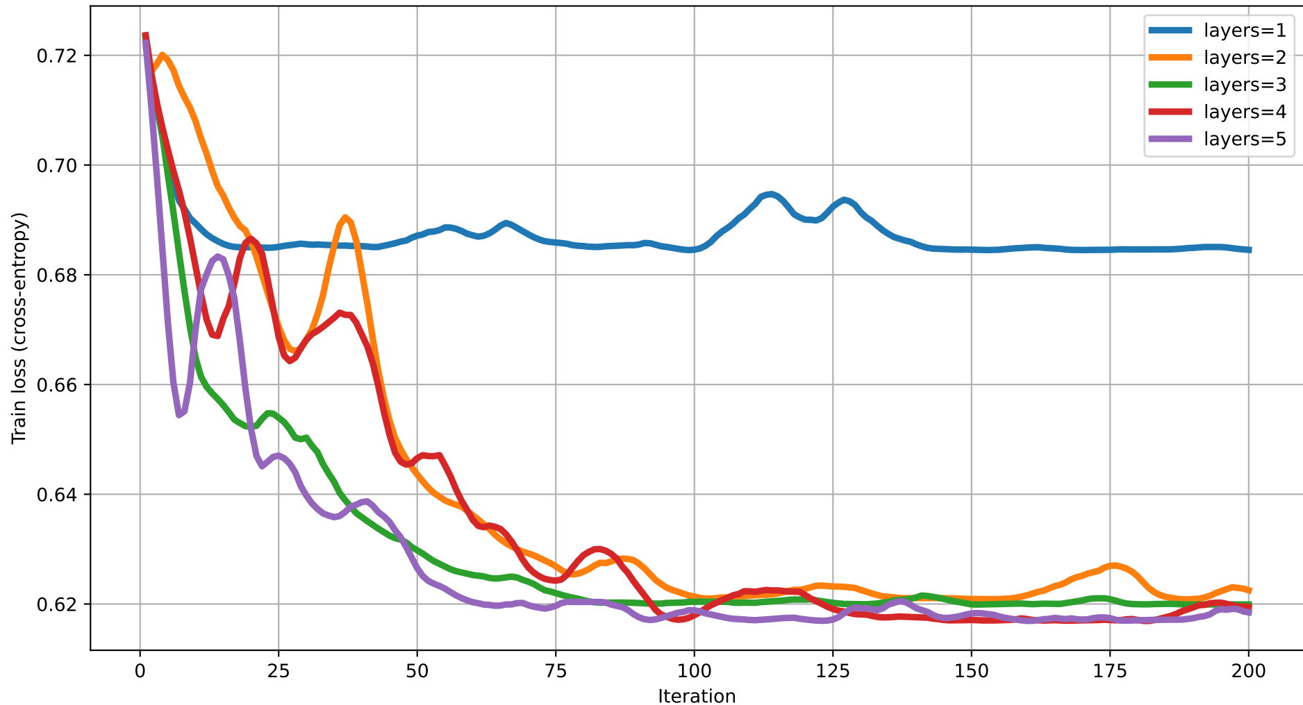
Train loss vs Iteration (degree=3) rot=RX, ent=chain, gate=CNOT
