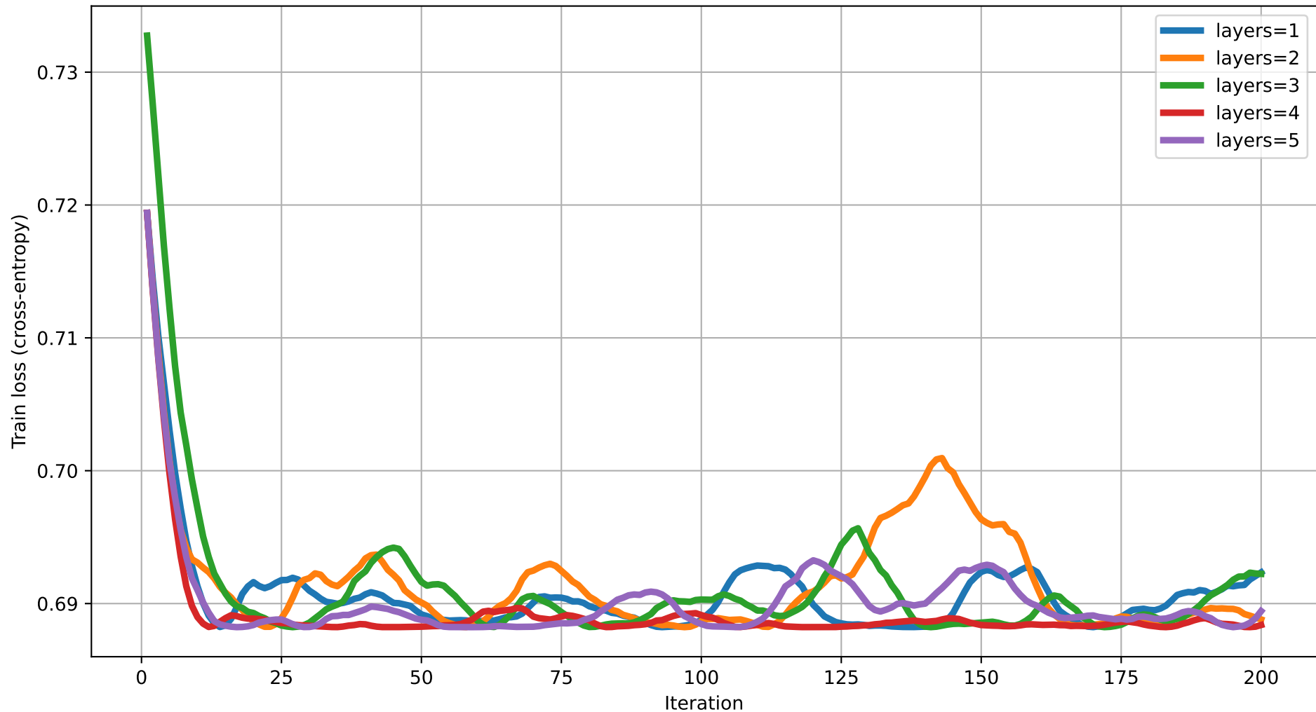
Train loss vs Iteration (degree=4) rot=RZ, ent=pairwise, gate=CZ
