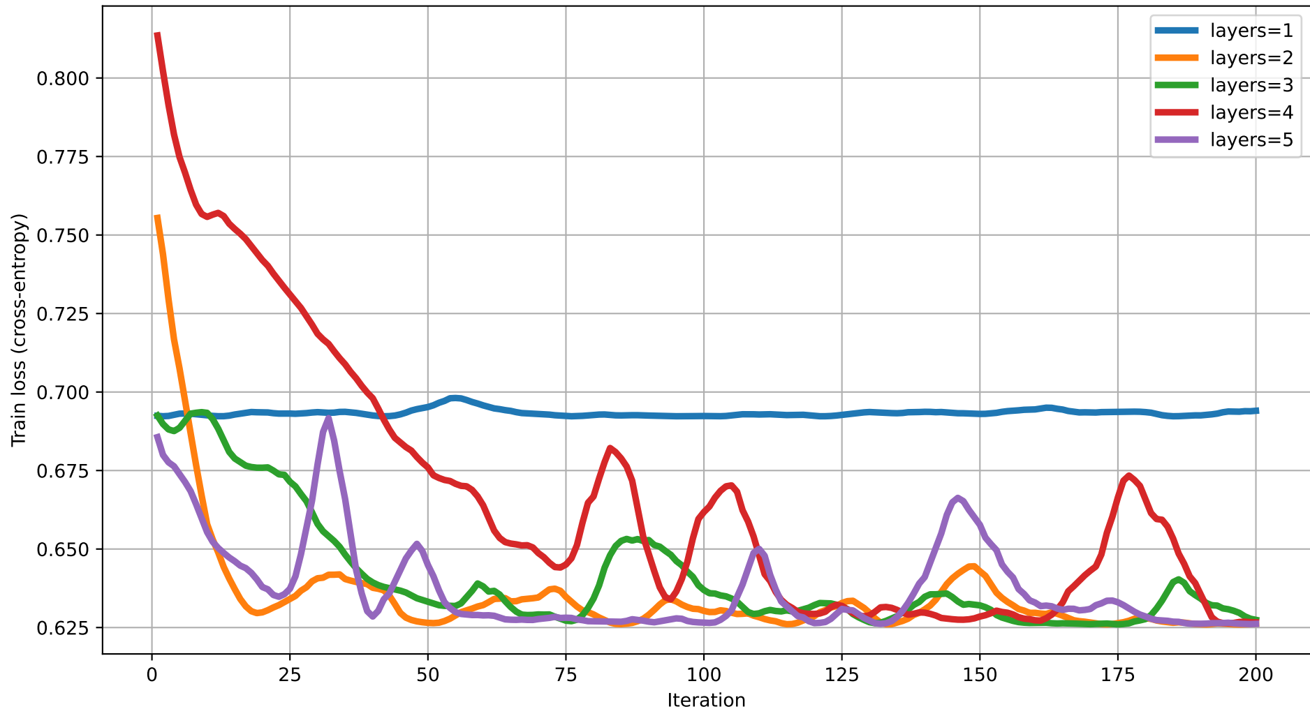
Train loss vs Iteration (dim=2) rot=RY, ent=full, gate=IsingXX
