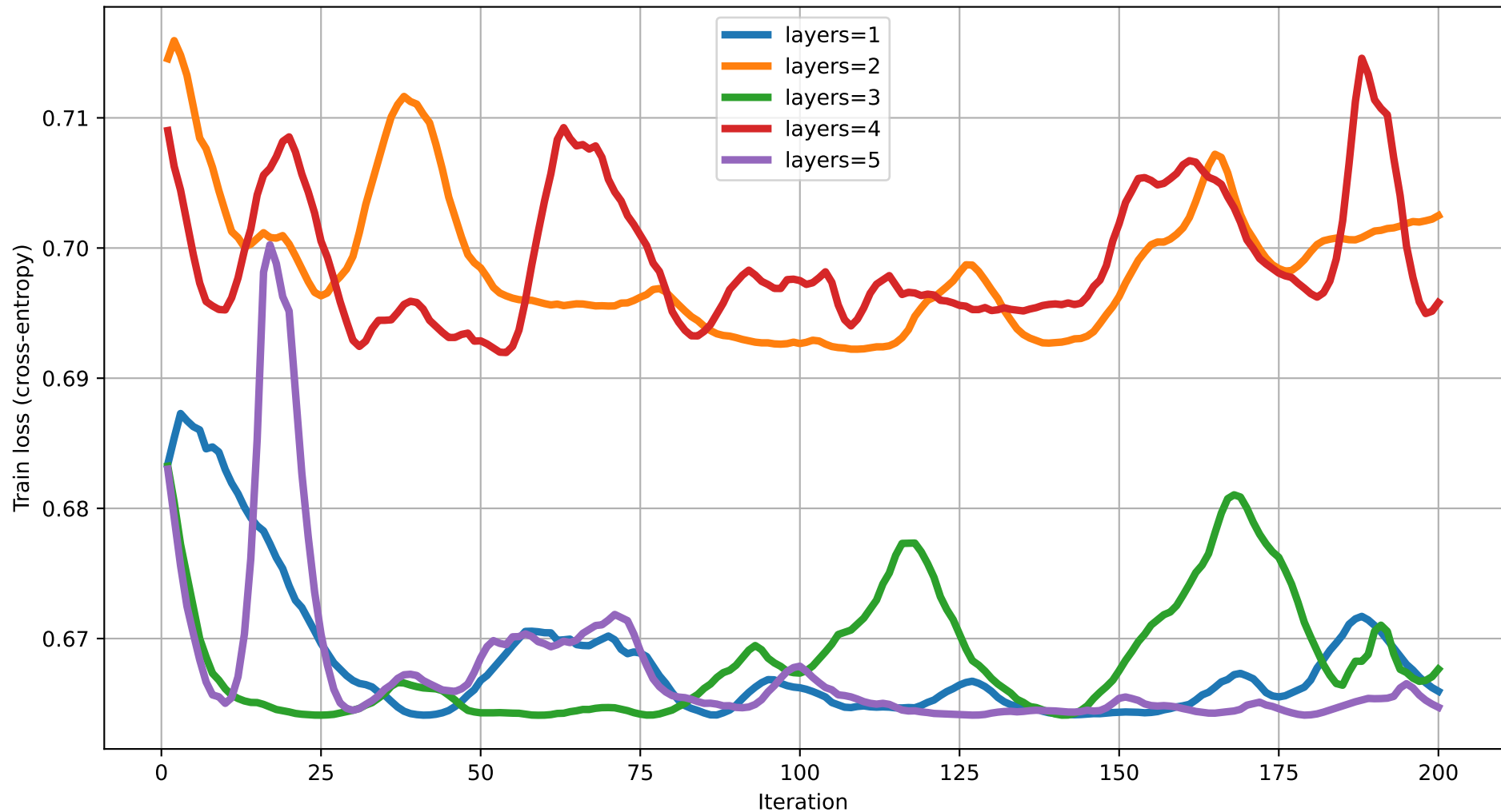
Train loss vs Iteration (dim=6) rot=RX, ent=ring, gate=lsingXX
