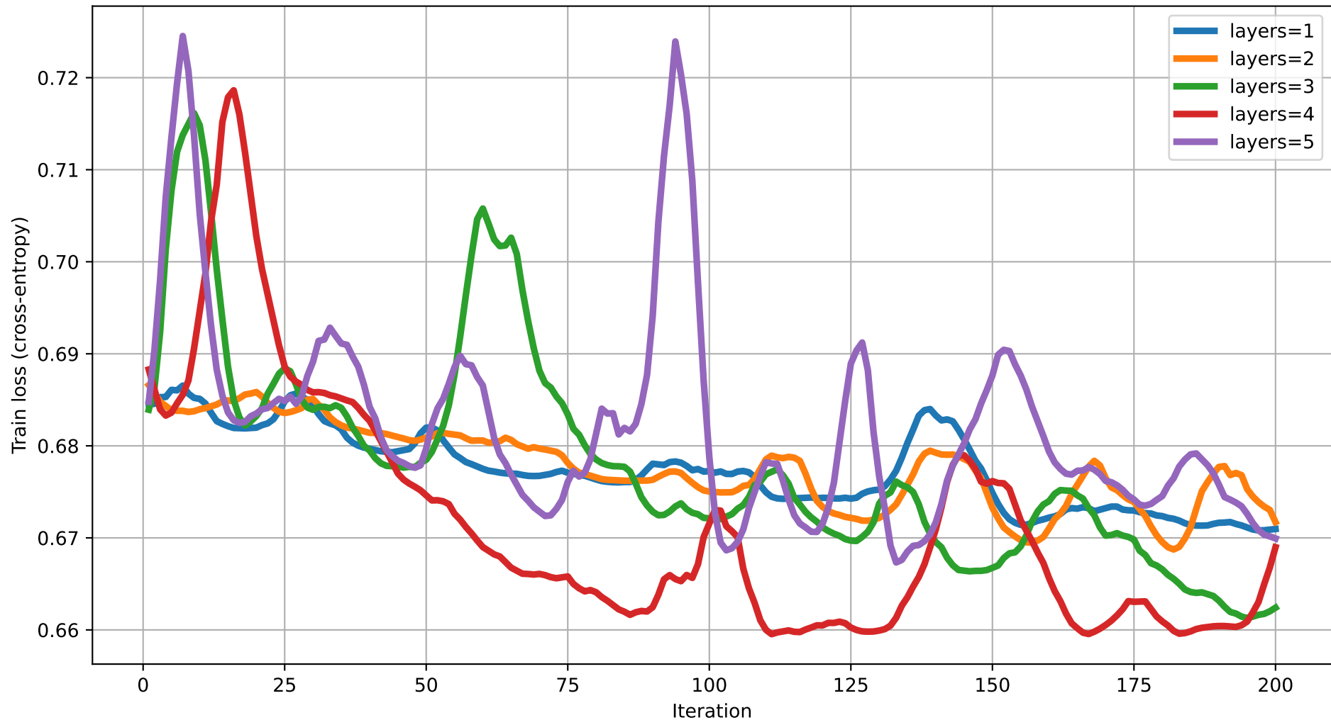
Train loss vs Iteration (dim=15) rot=RY, ent=ring, gate=CZ
