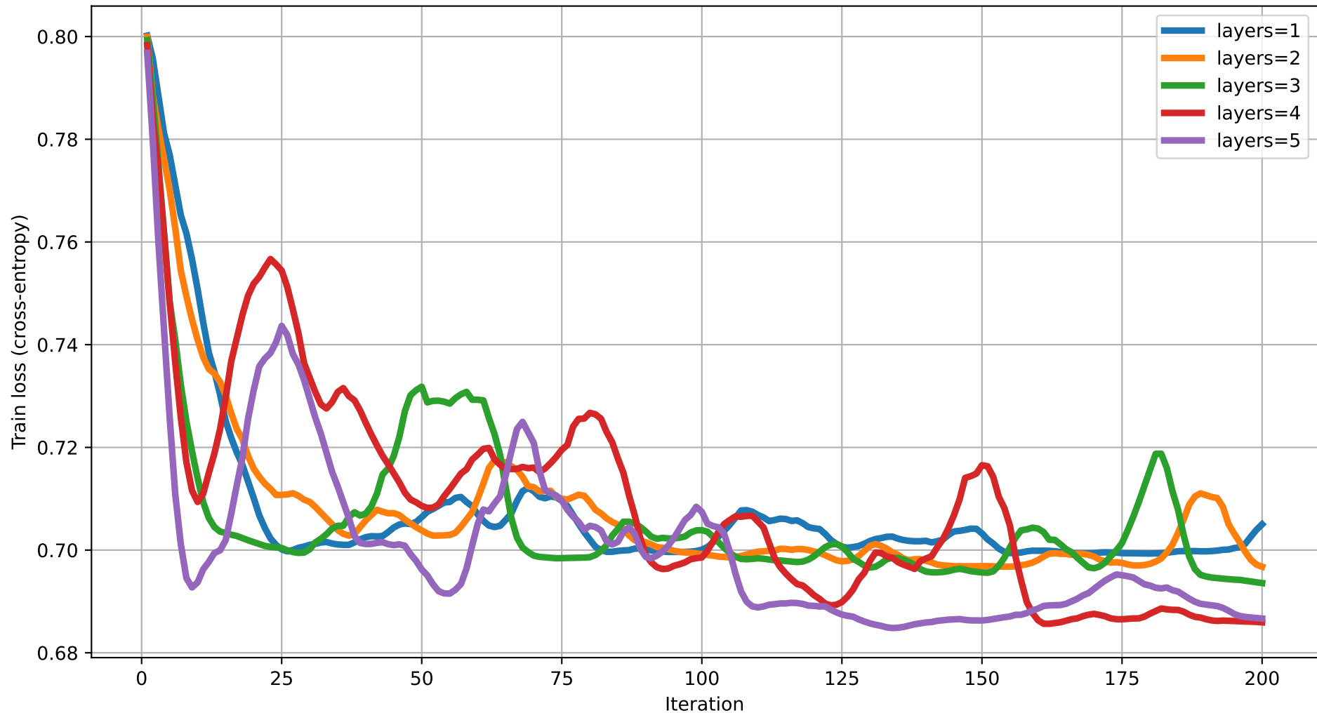
Train loss vs Iteration (dim=8) rot=RX, ent=chain, gate=CZ
