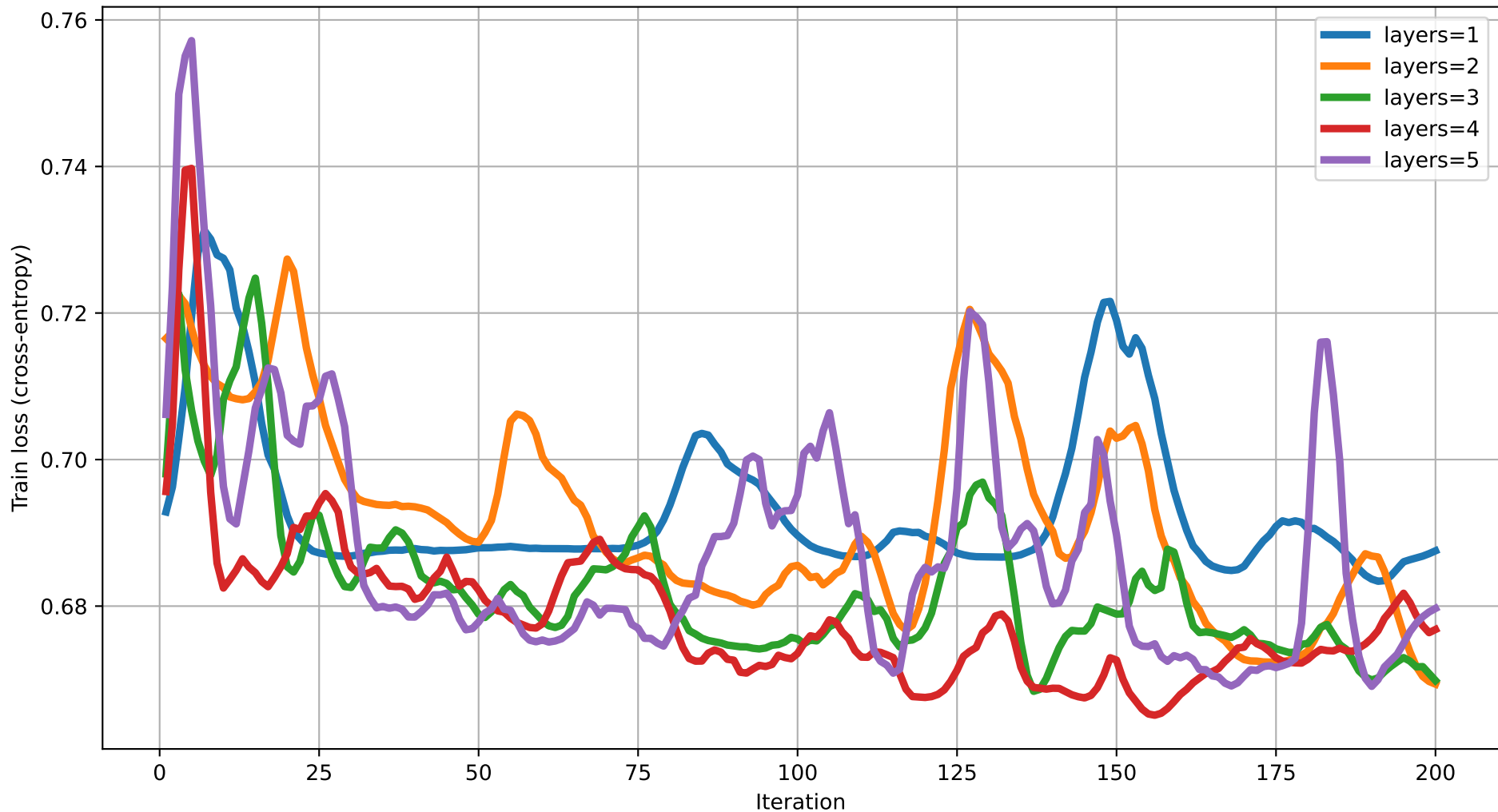
Train loss vs Iteration (dim=15) rot=Rot, ent=pairwise, gate=IsingXX
