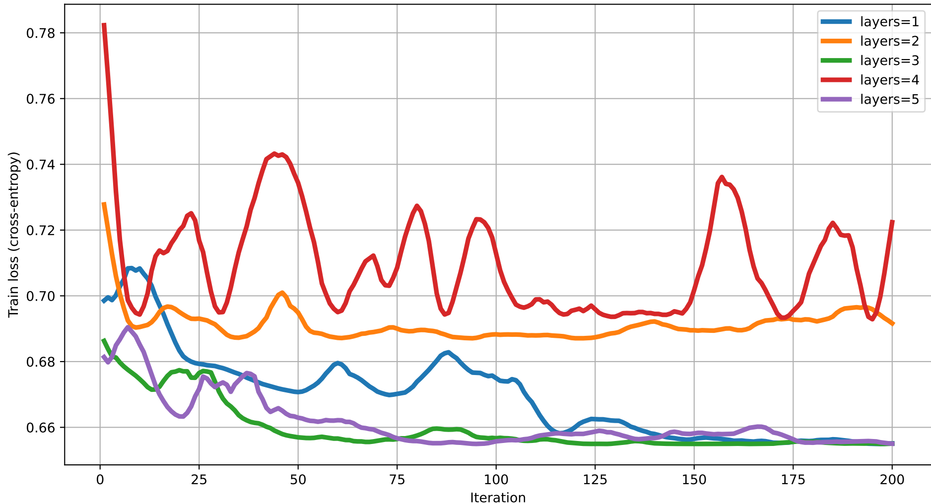
Train loss vs Iteration (dim=9) rot=RX, ent=full, gate=IsingXX
