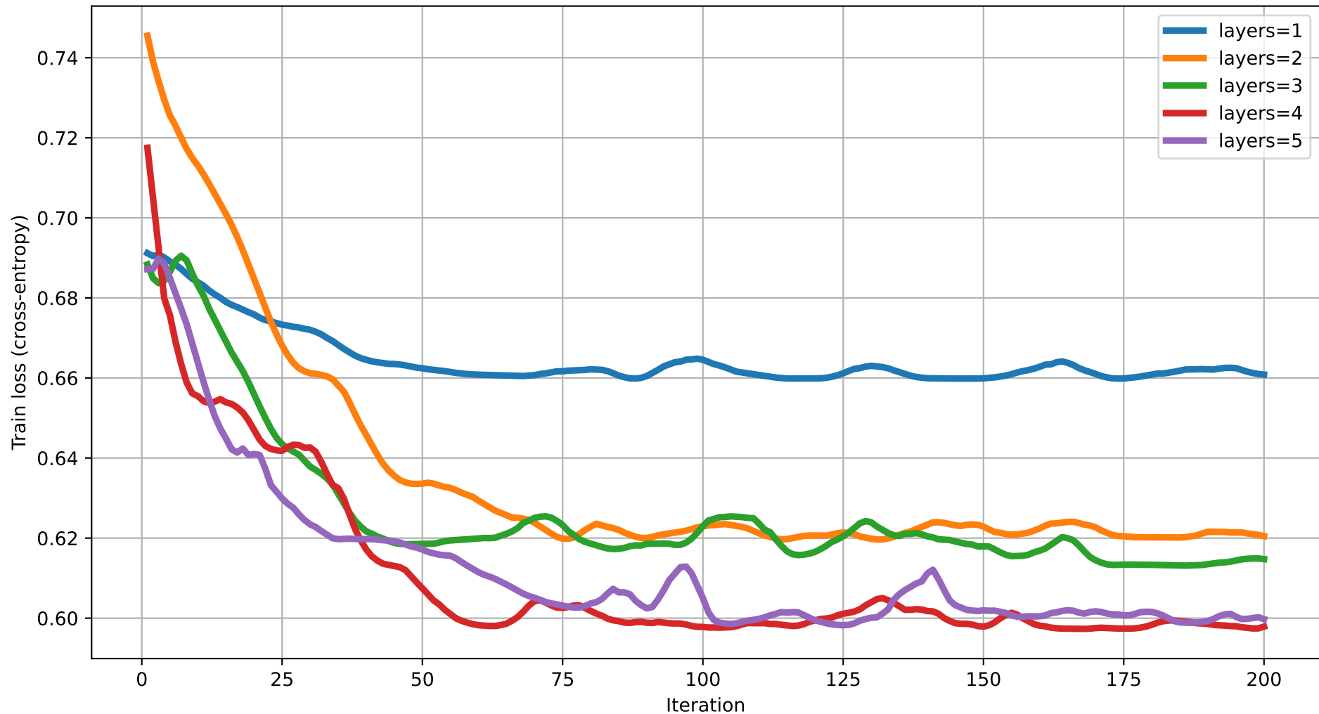
Train loss vs Iteration (degree=3) rot=RZ, ent=chain, gate=IsingXX
