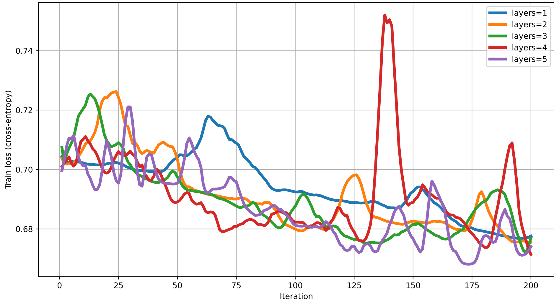
Train loss vs Iteration (dim=14) rot=Rot, ent=full, gate=CNOT
