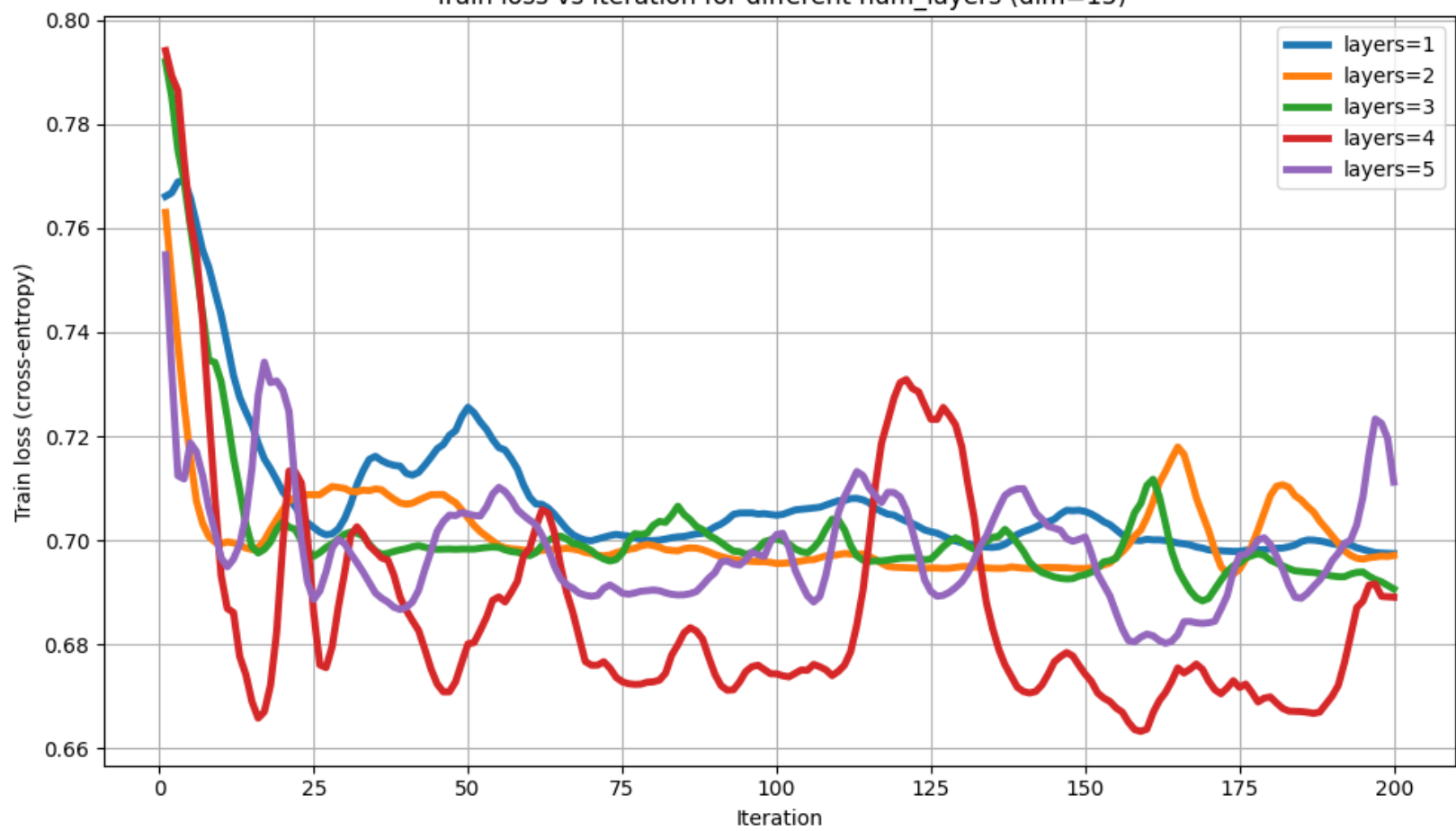
Train loss vs Iteration for different num_layers (dim=15)
