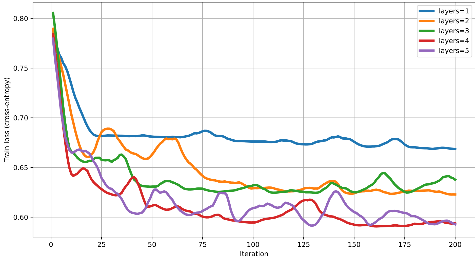
Train loss vs Iteration (dim=4) rot=RY, ent=chain, gate=CZ
