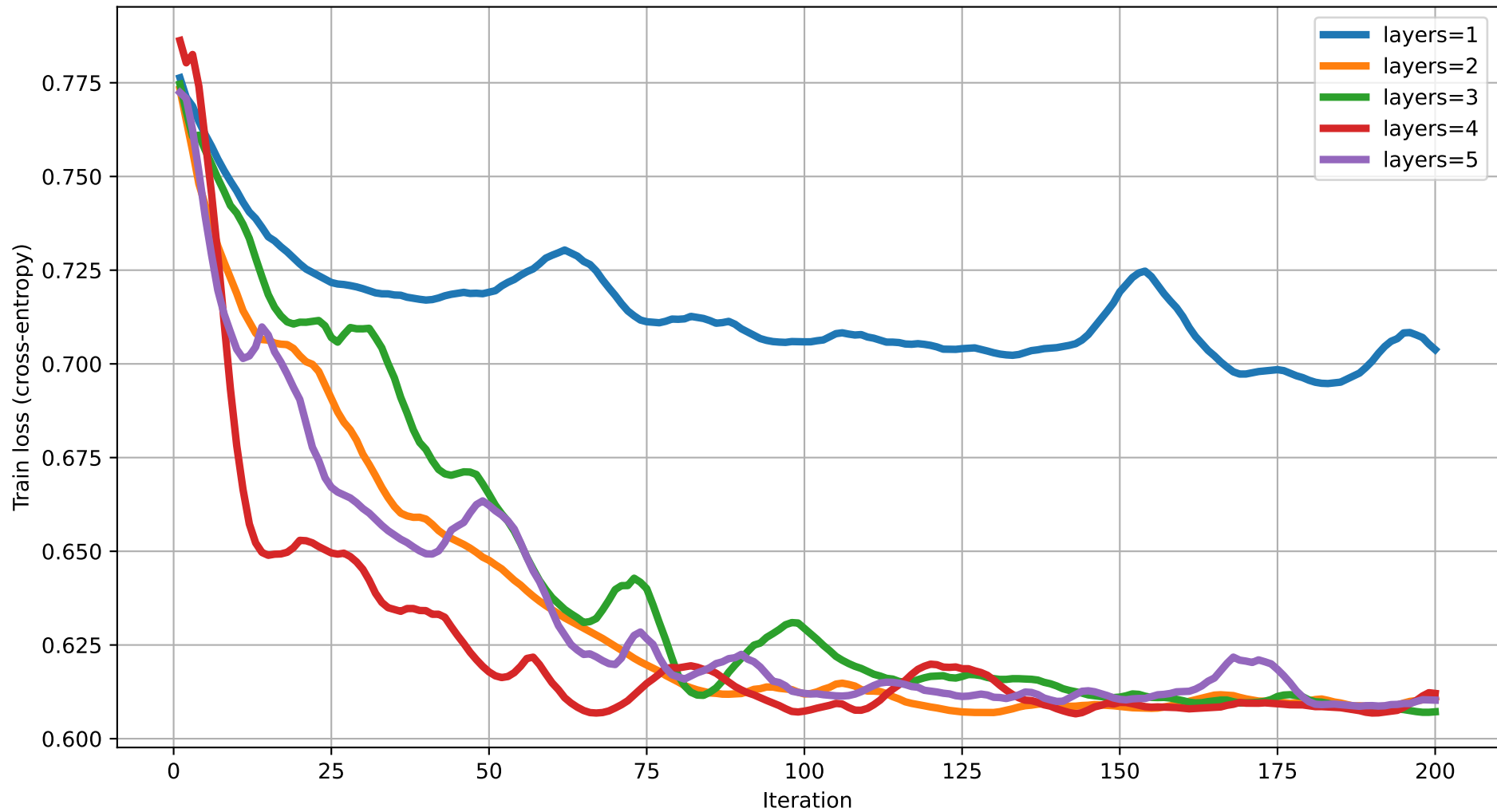
Train loss vs Iteration (dim=9) rot=RYZ, ent=pairwise, gate=CZ
