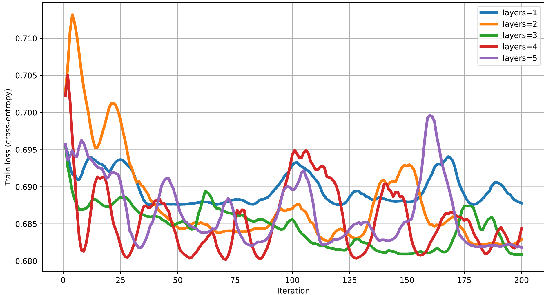
Train loss vs Iteration (dim=13) rot=RX, ent=full, gate=CNOT
