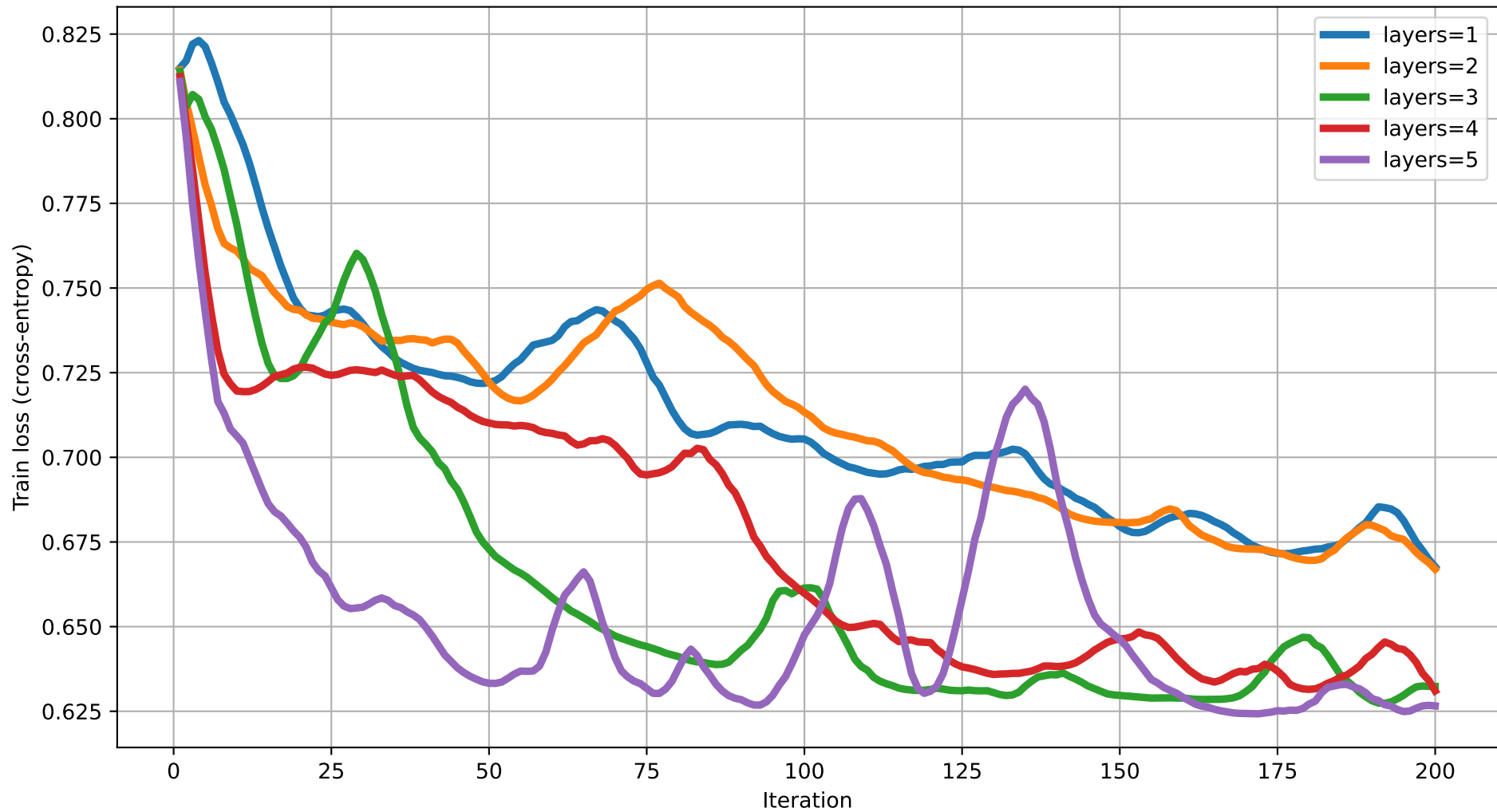
Train loss vs Iteration (dim=2) rot=RX, ent=chain, gate=CZ
