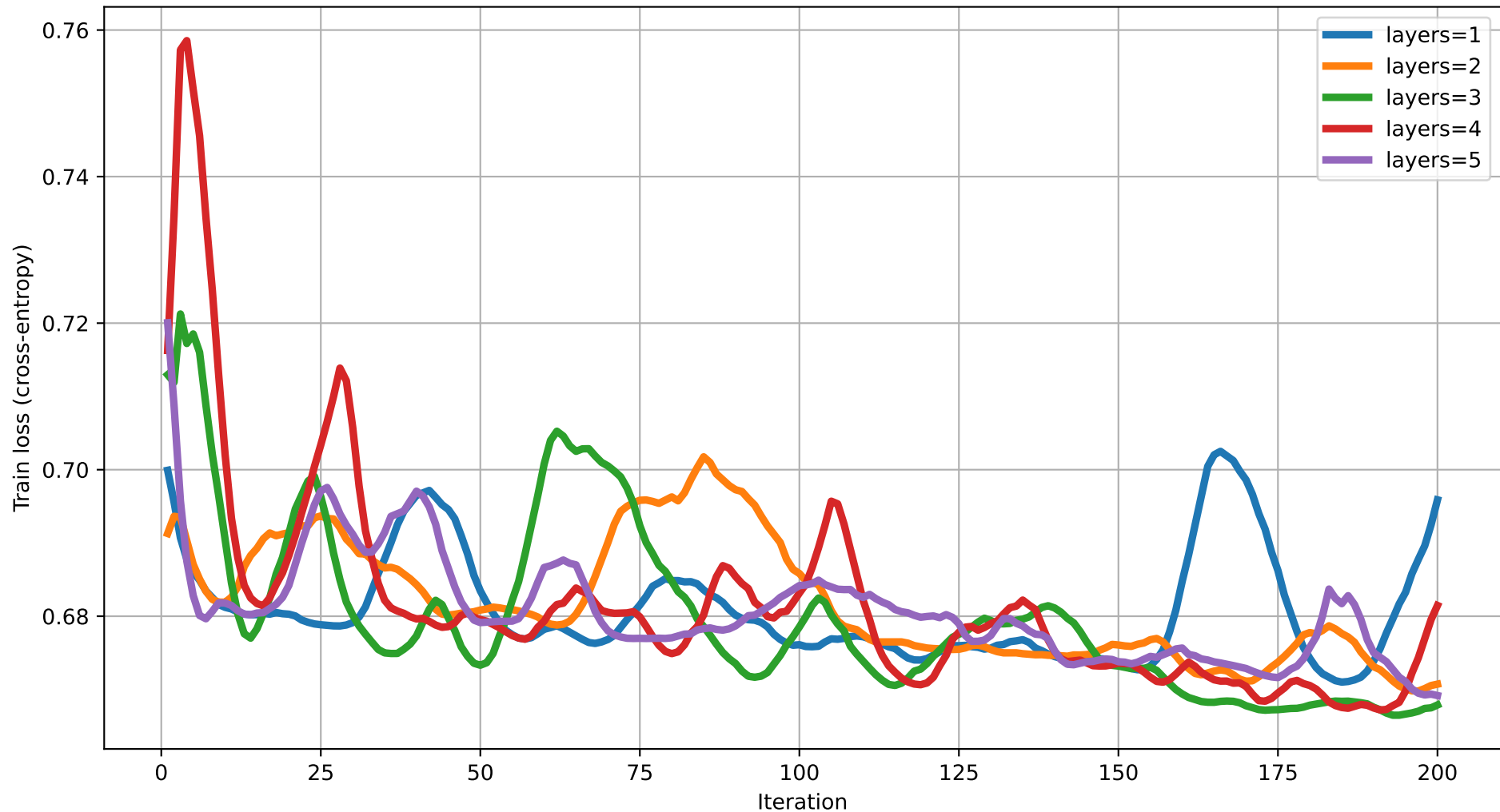
Train loss vs Iteration (dim=13) rot=RY, ent=chain, gate=CZ
