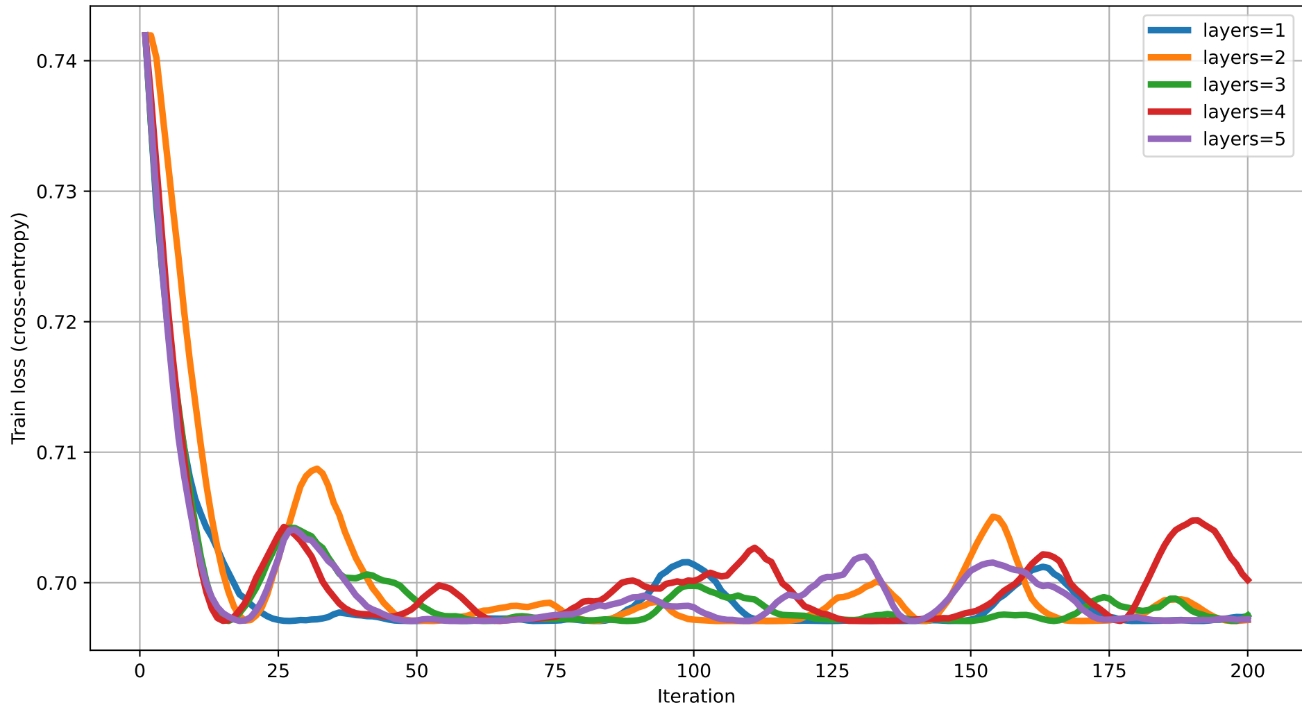
Train loss vs Iteration (degree=5) rot=RZ, ent=pairwise, gate=CZ
