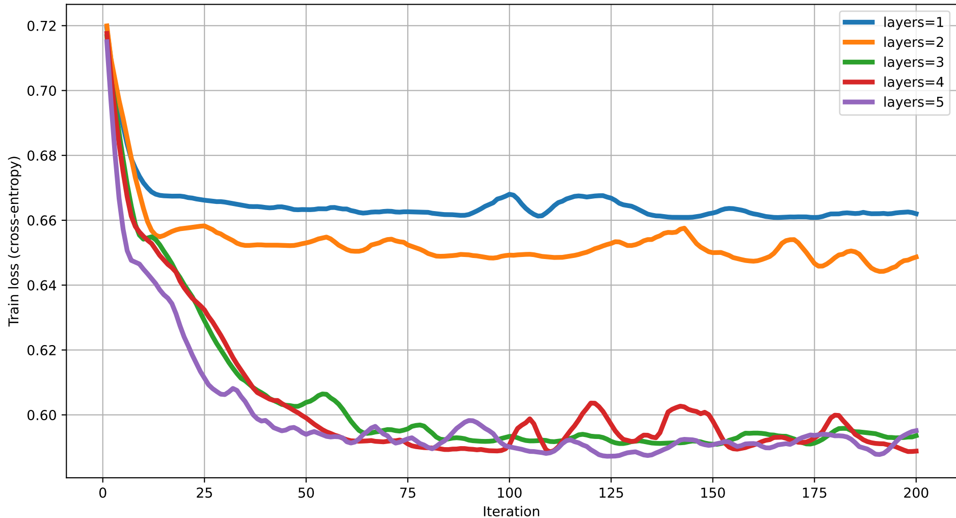
Train loss vs Iteration (degree=3) rot=RYZ, ent=ring, gate=CZ
