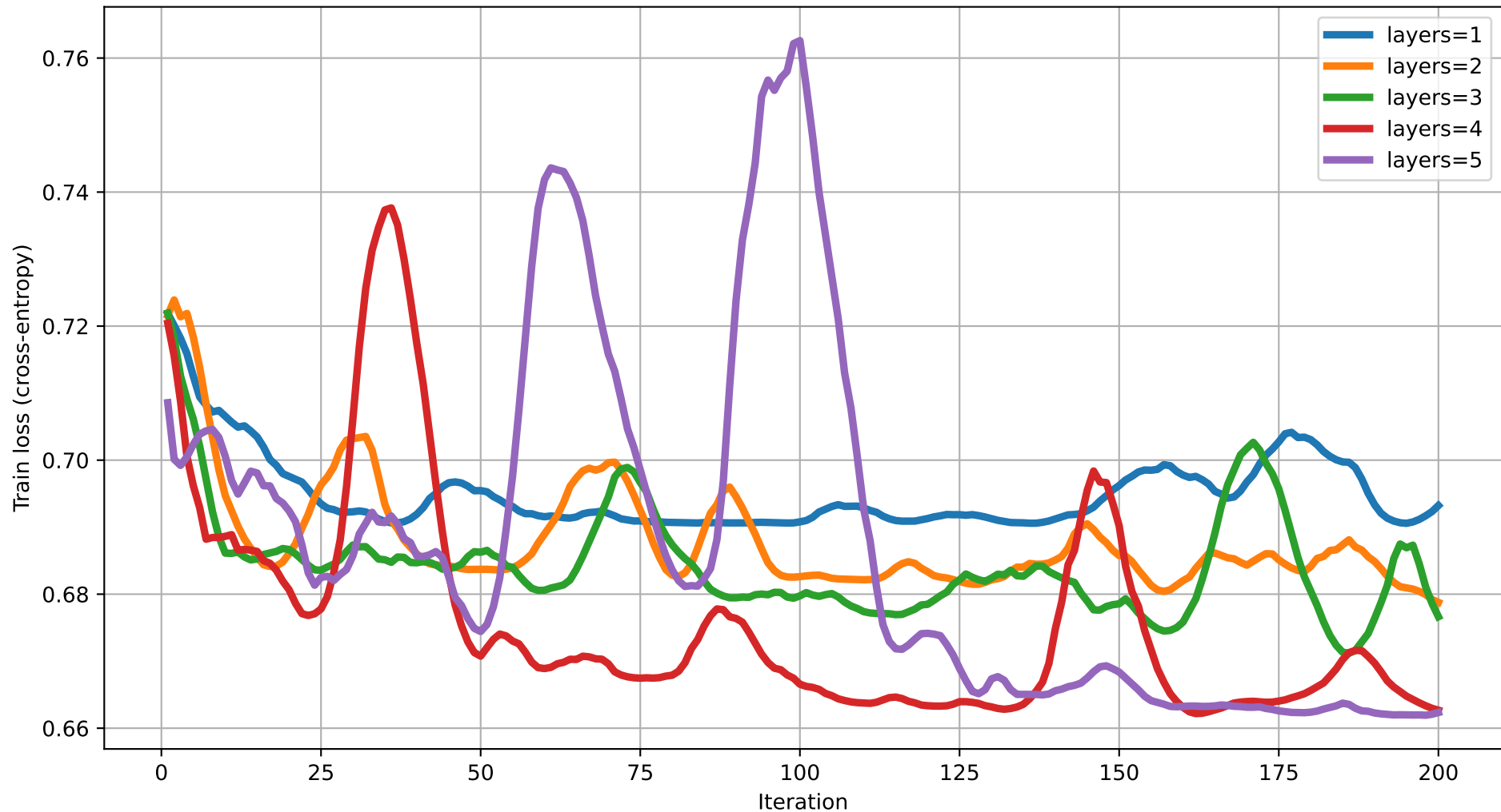
Train loss vs Iteration (dim=20) rot=RX, ent=full, gate=CNOT
