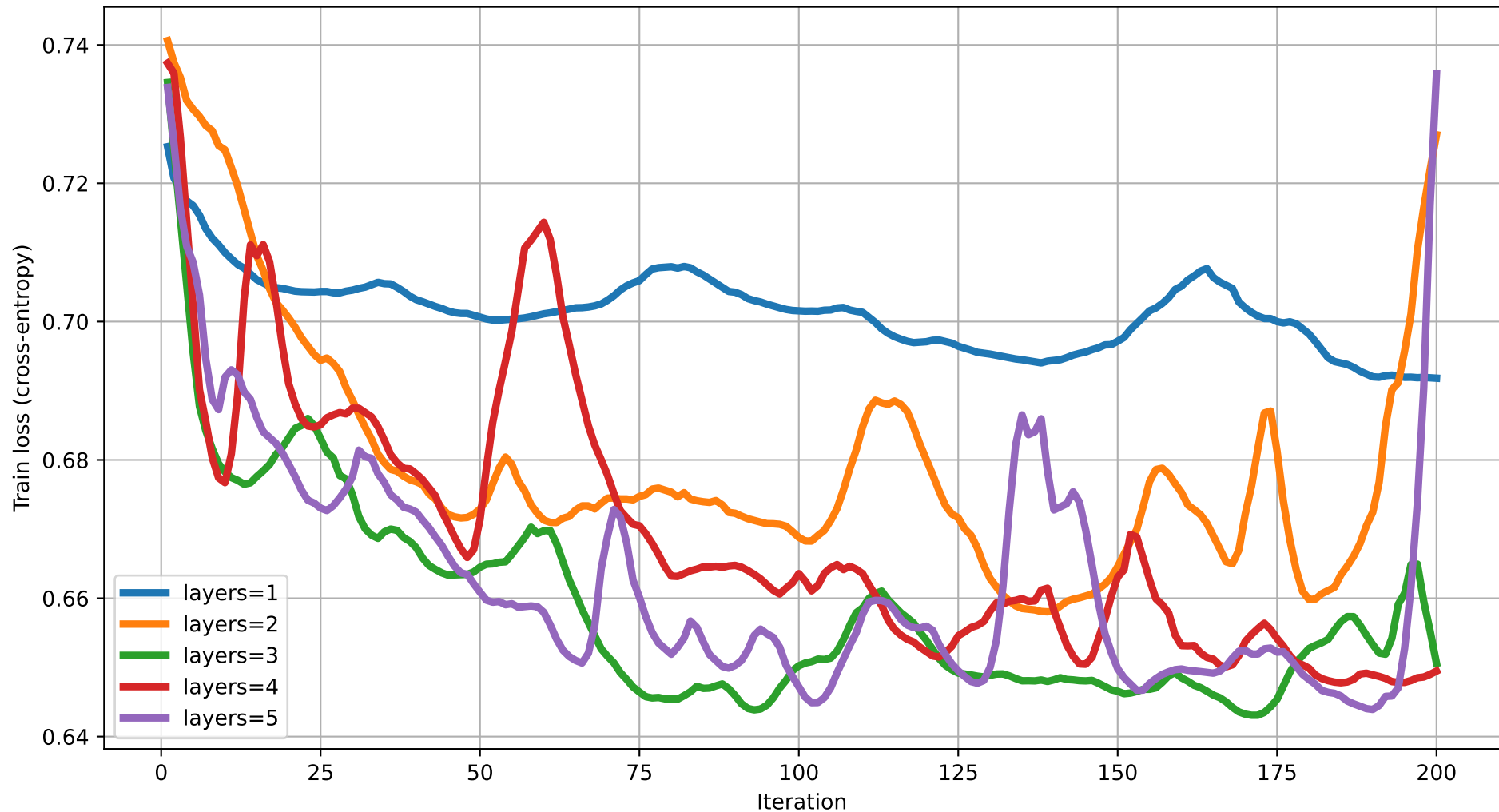
Train loss vs Iteration (dim=5) rot=Rot, ent=full, gate=CNOT
