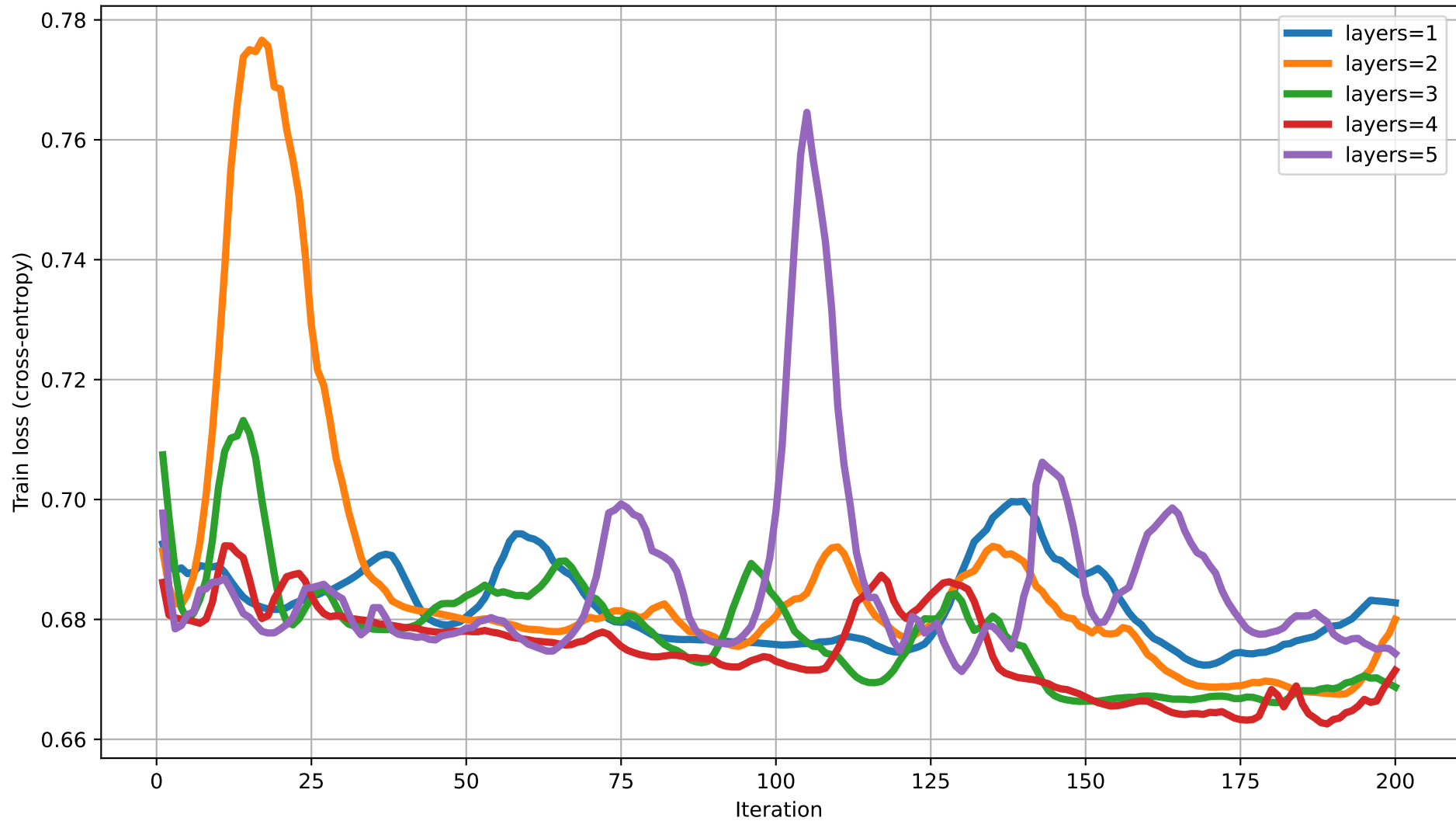
Train loss vs Iteration for different num_layers (dim=13)
