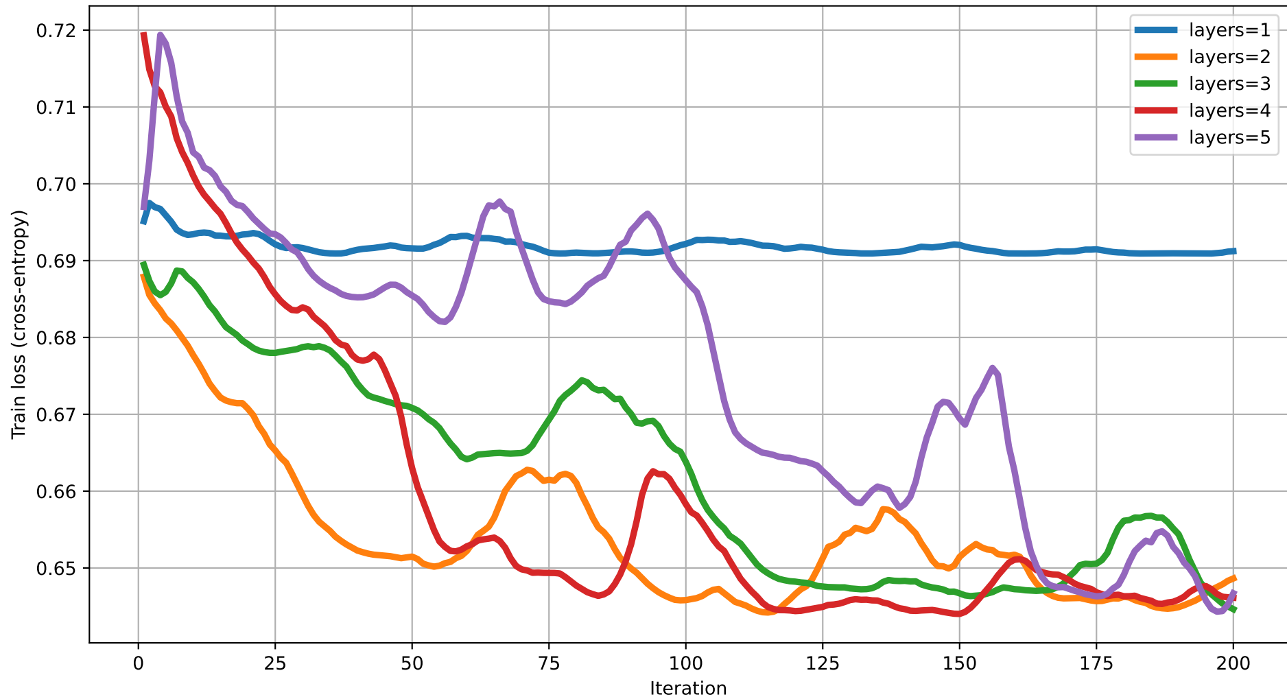
Train loss vs Iteration (dim=7) rot=RY, ent=chain, gate=IsingXX
