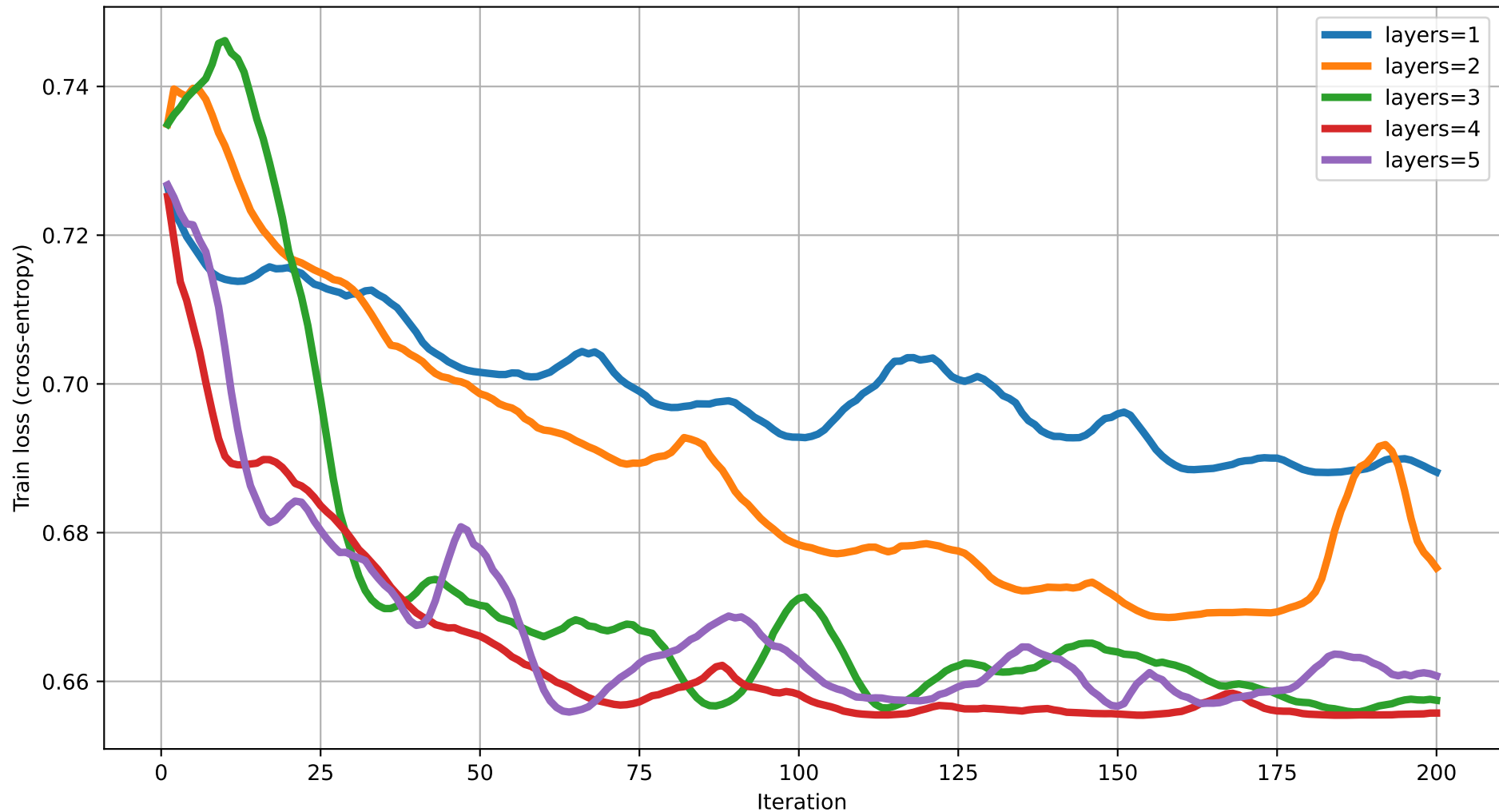
Train loss vs Iteration (dim=6) rot=RX, ent=full, gate=CNOT
