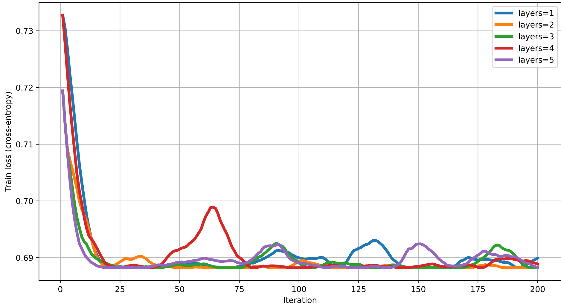
Train loss vs Iteration (degree=4) rot=RZ, ent=chain, gate=CZ
