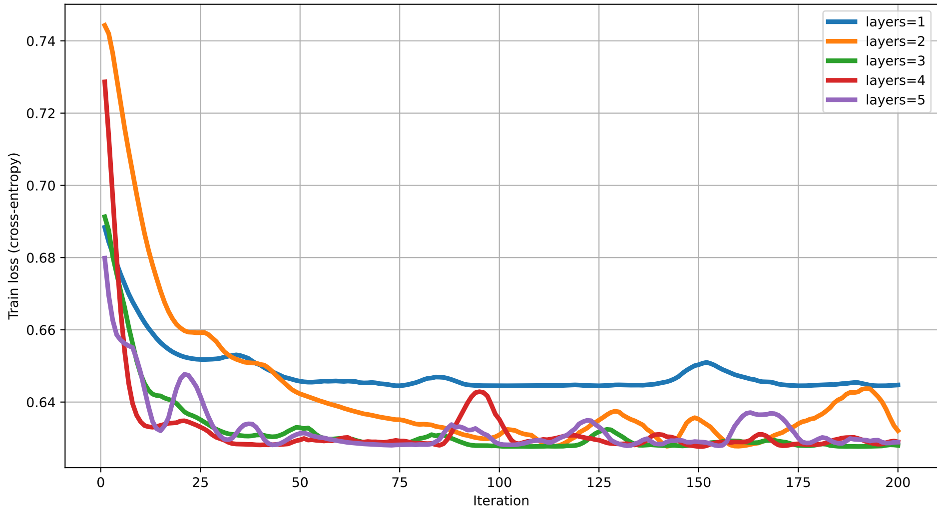
Train loss vs Iteration (degree=5) rot=RZ, ent=pairwise, gate=IsingXX
