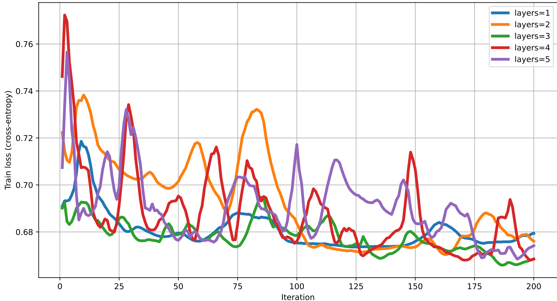
Train loss vs Iteration (dim=11) rot=Rot, ent=pairwise, gate=IsingXX
