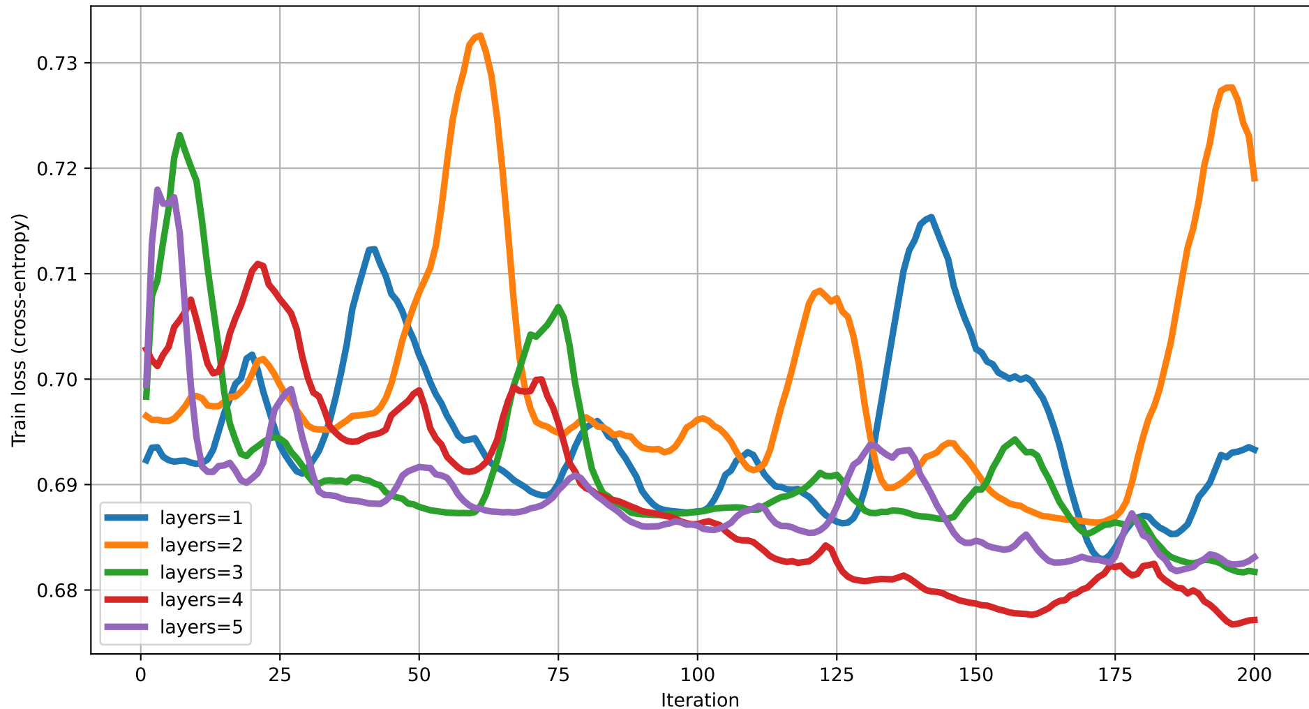
Train loss vs Iteration (dim=14) rot=RZ, ent=pairwise, gate=IsingXX
