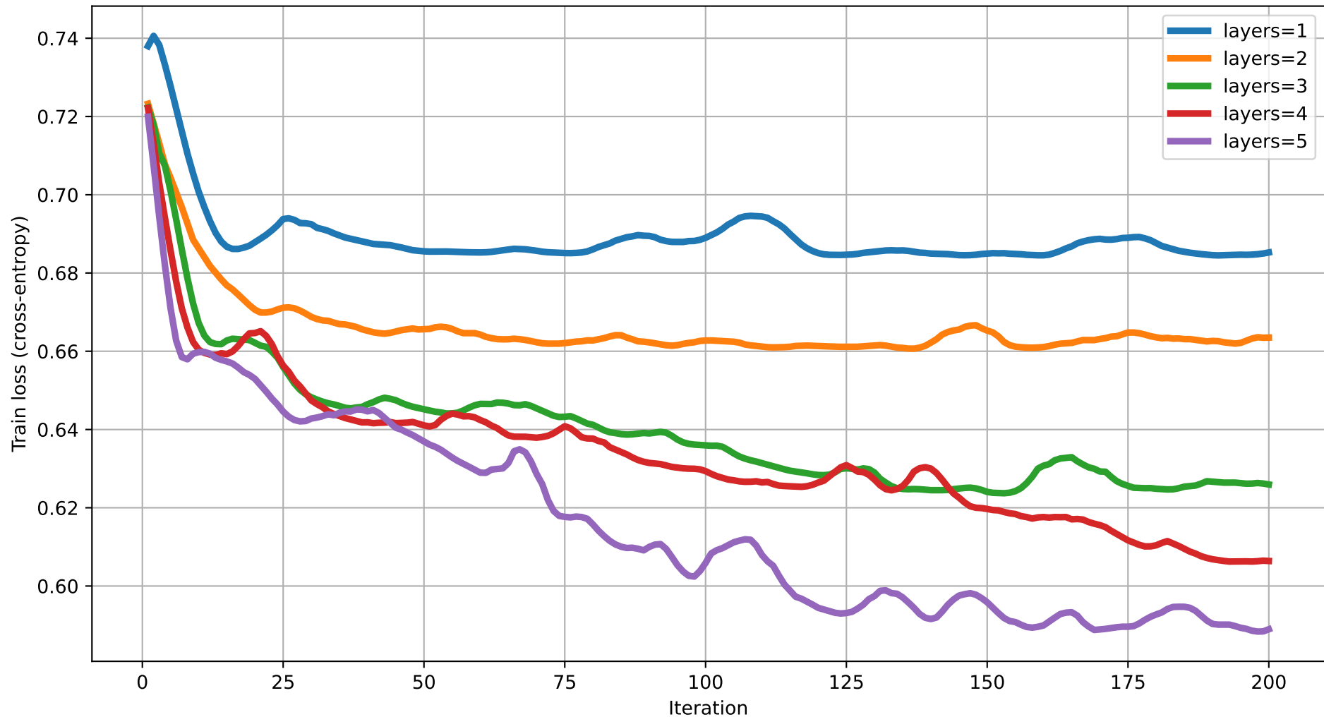
Train loss vs Iteration (degree=3) rot=RX, ent=full, gate=CZ
