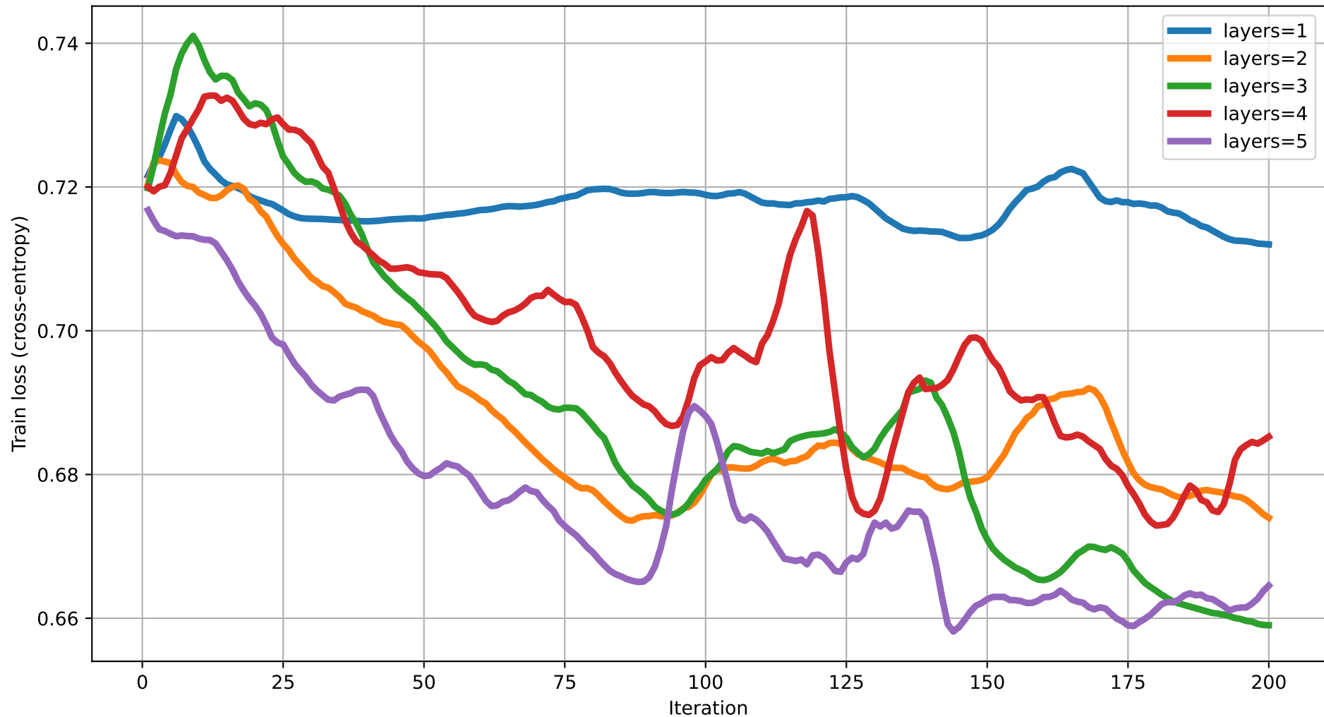
Train loss vs Iteration (dim=3) rot=RY, ent=full, gate=CNOT
