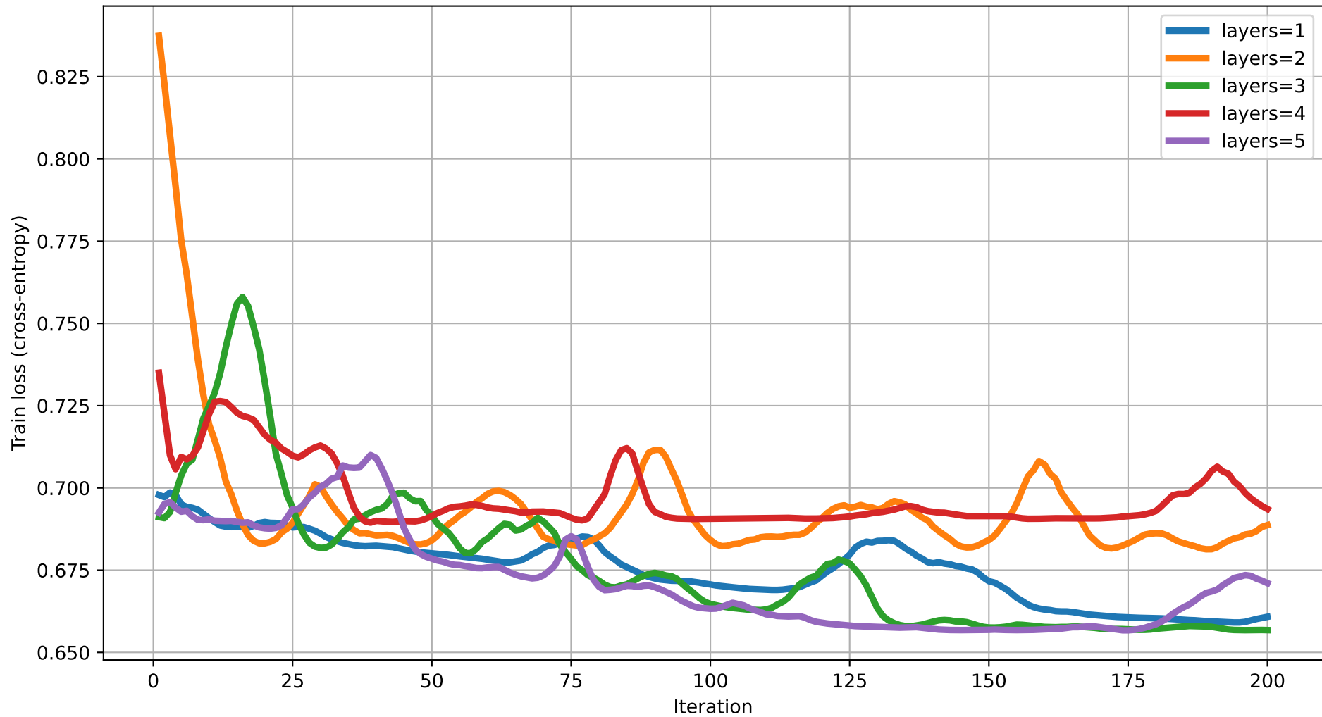
Train loss vs Iteration (dim=16) rot=RX, ent=chain, gate=IsingXX
