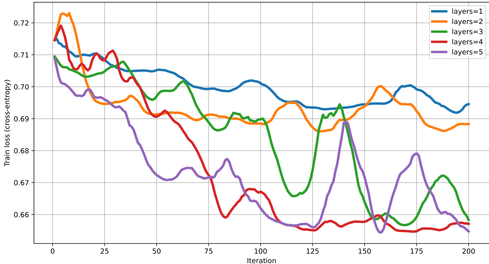
Train loss vs Iteration (dim=6) rot=RX, ent=ring, gate=CZ
