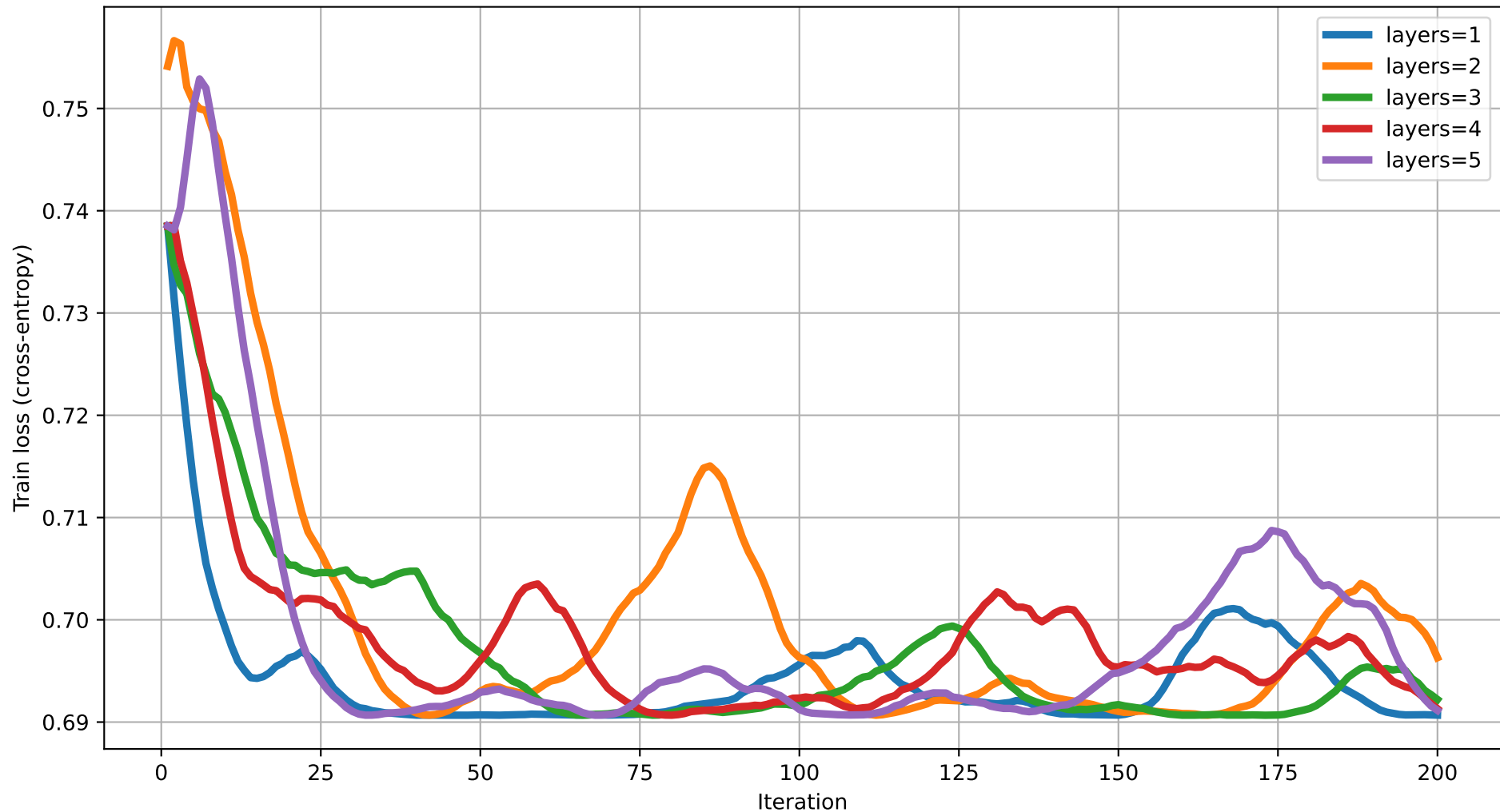
Train loss vs Iteration (dim=16) rot=RZ, ent=chain, gate=CNOT
