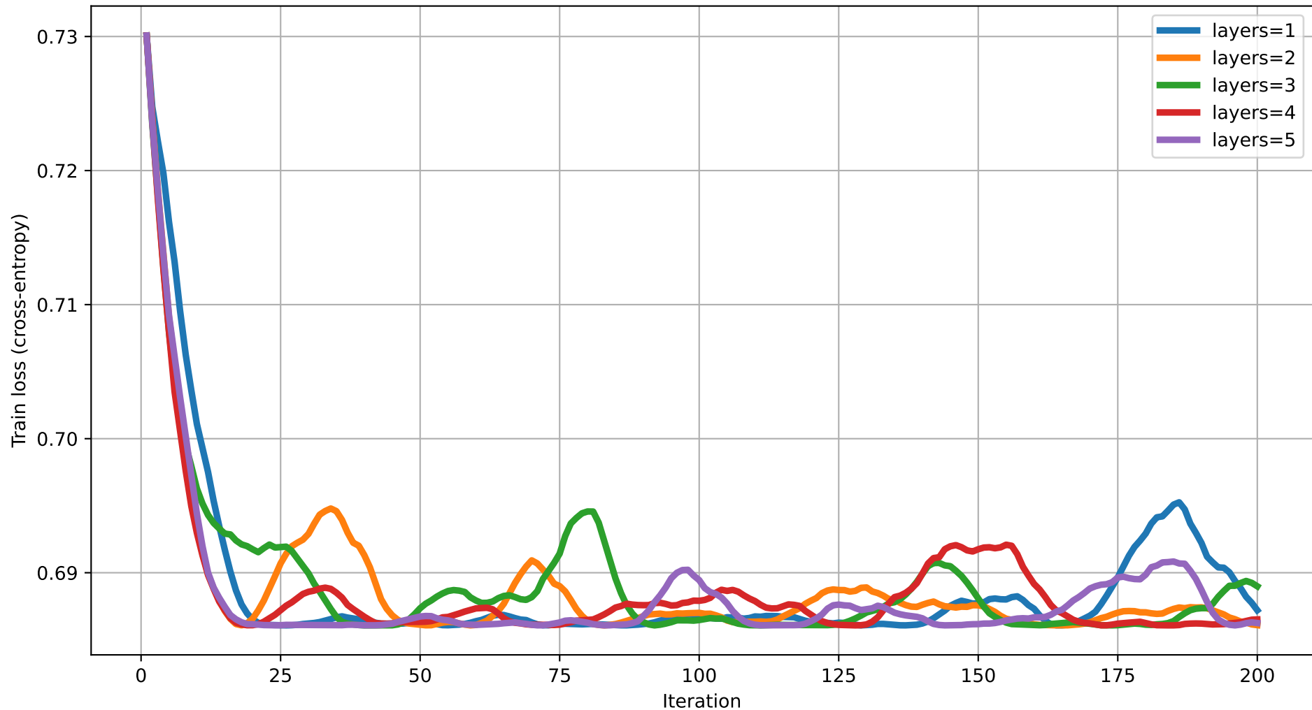
Train loss vs Iteration (degree=2) rot=RZ, ent=full, gate=CNOT
