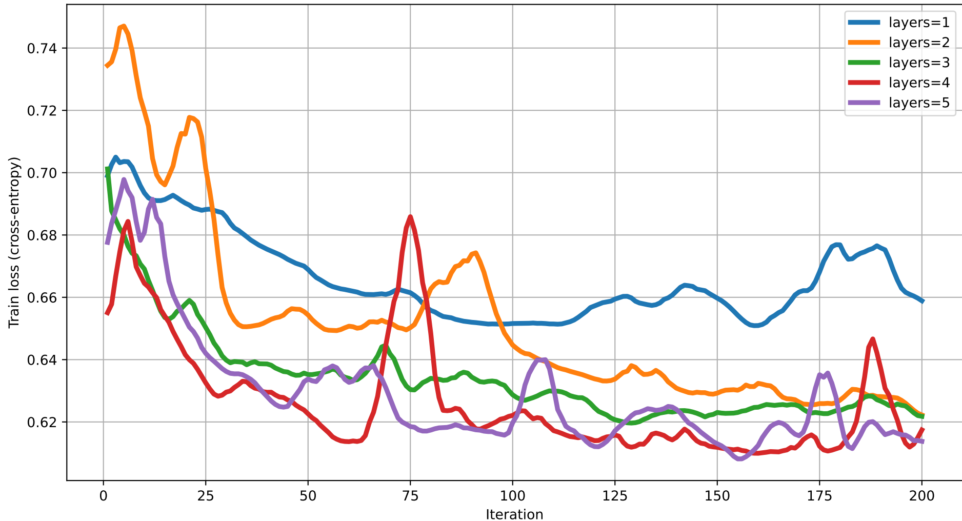
Train loss vs Iteration (dim=15) rot=Rot, ent=chain, gate=IsingXX
