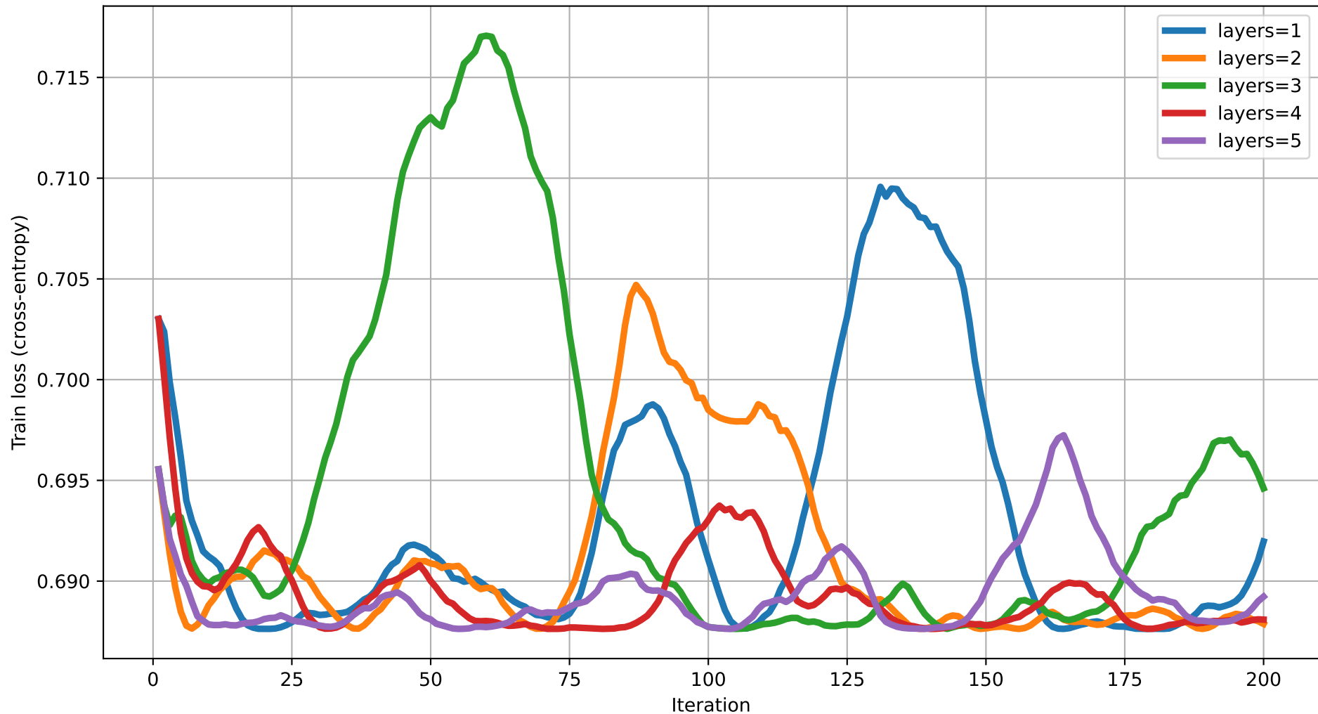
Train loss vs Iteration (dim=13) rot=RZ, ent=pairwise, gate=CZ
