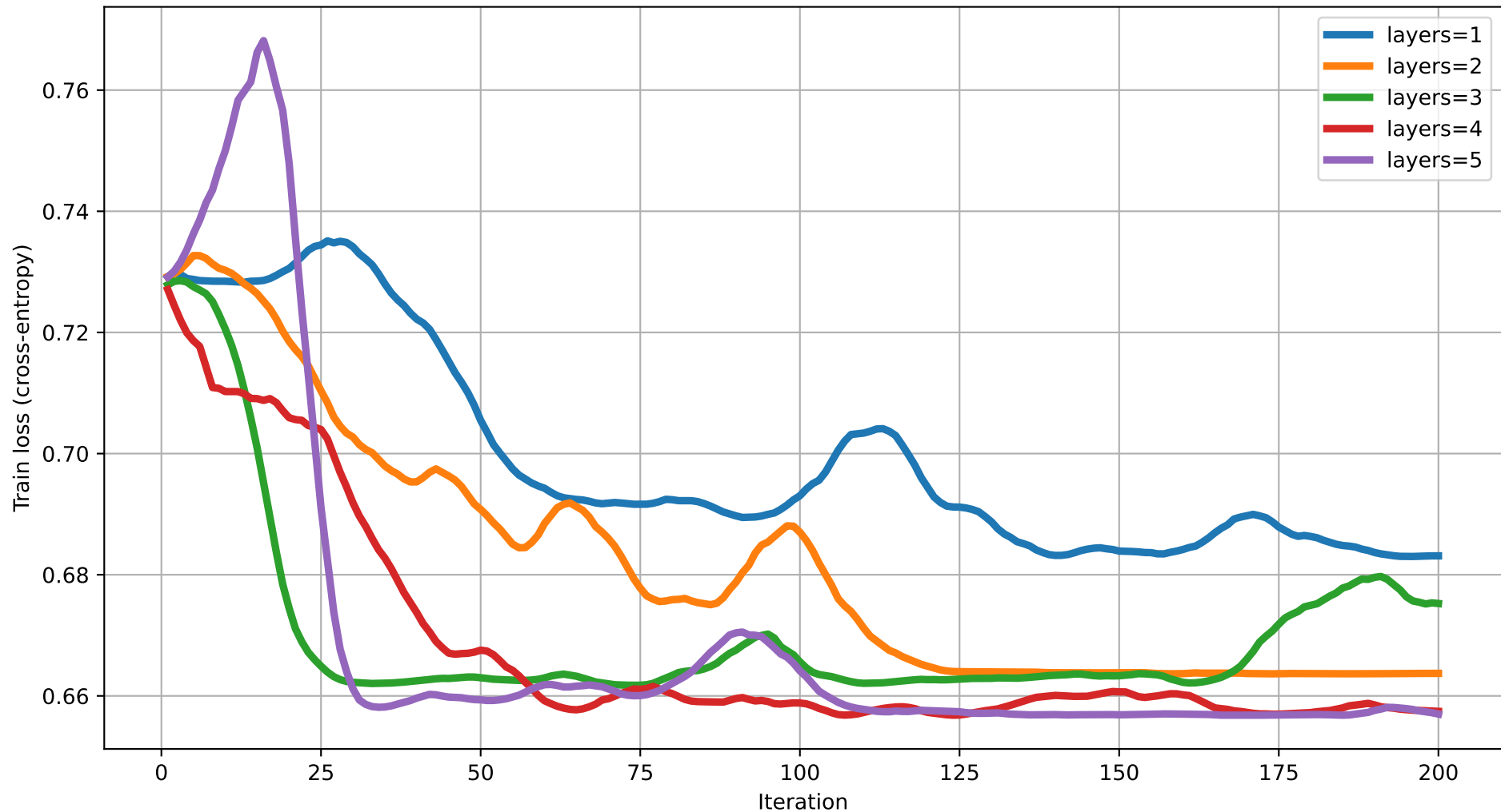
Train loss vs Iteration (dim=7) rot=RX, ent=full, gate=CNOT
