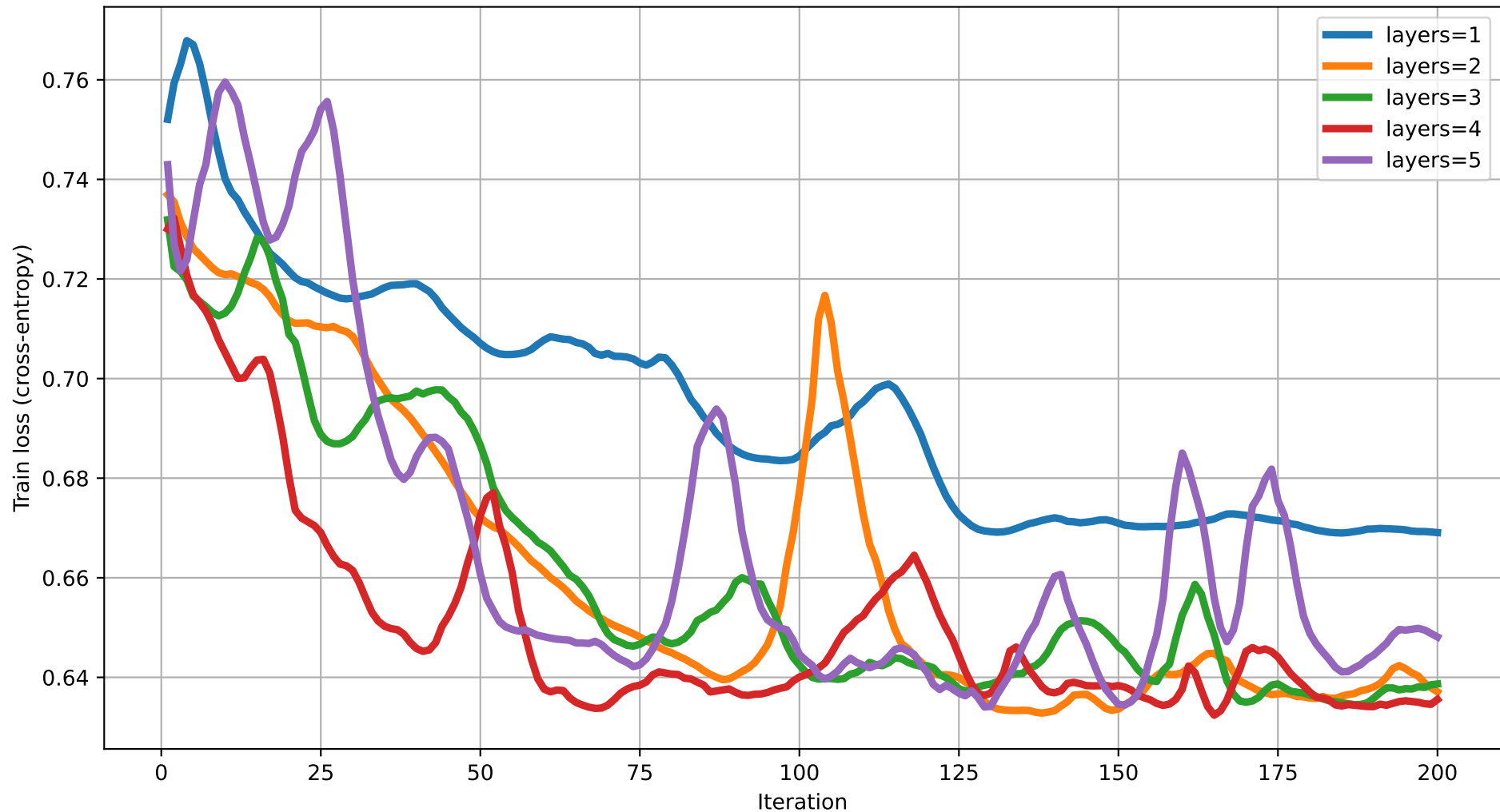
Train loss vs Iteration (dim=3) rot=Rot, ent=full, gate=CNOT
