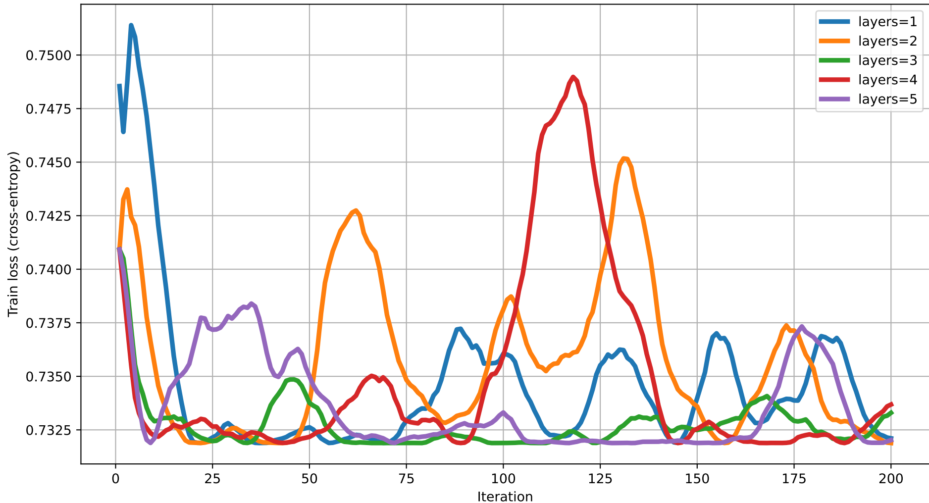
Train loss vs Iteration (dim=3) rot=RZ, ent=ring, gate=CZ
