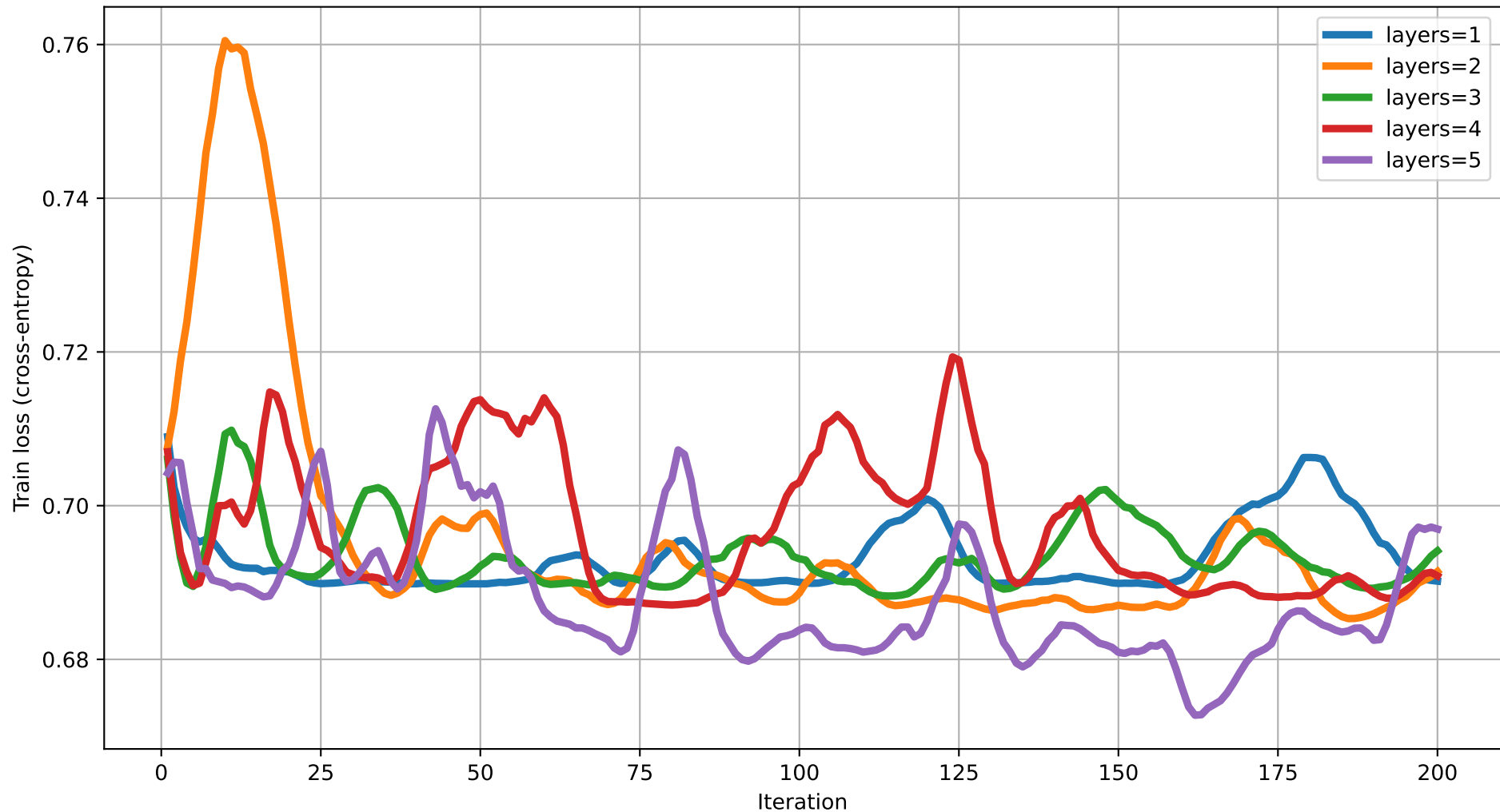
Train loss vs Iteration (dim=20) rot=Rot, ent=full, gate=CZ
