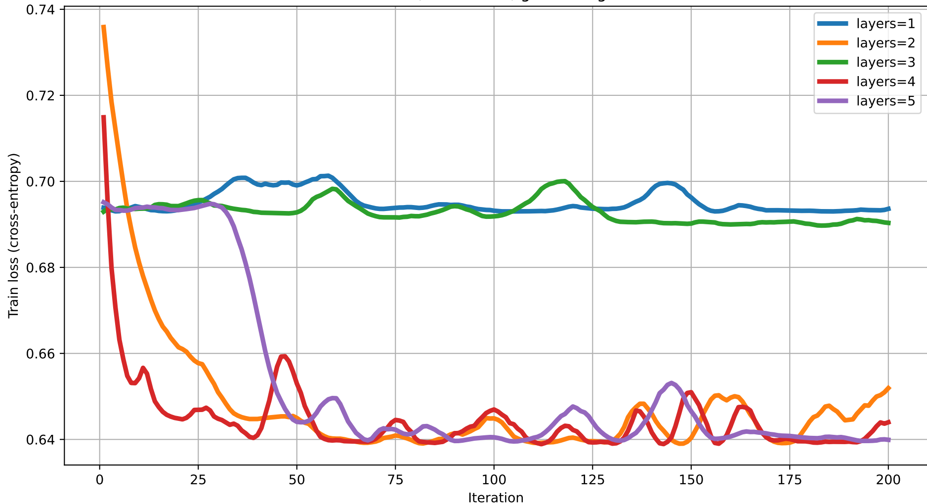
Train loss vs Iteration (degree=2) rot=RY, ent=chain, gate=IsingXX
