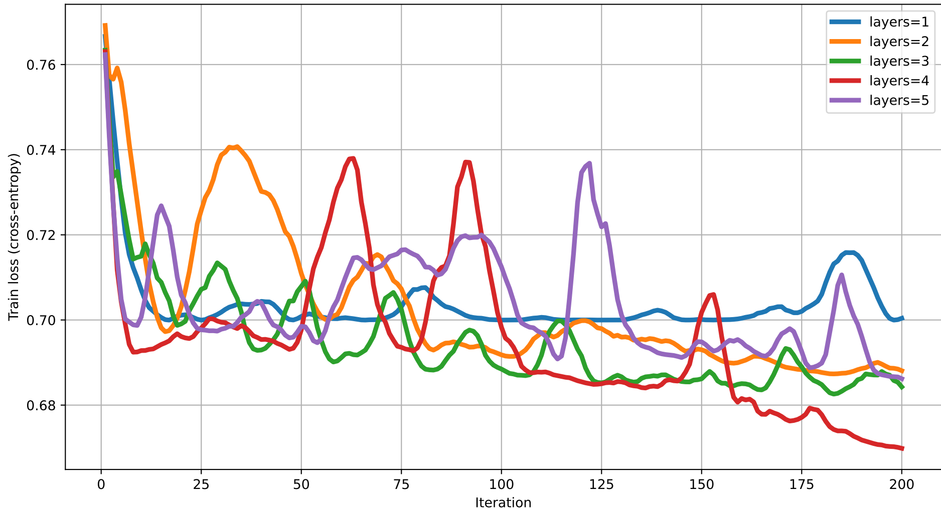
Train loss vs Iteration (dim=17) rot=RYZ, ent=full, gate=CZ
