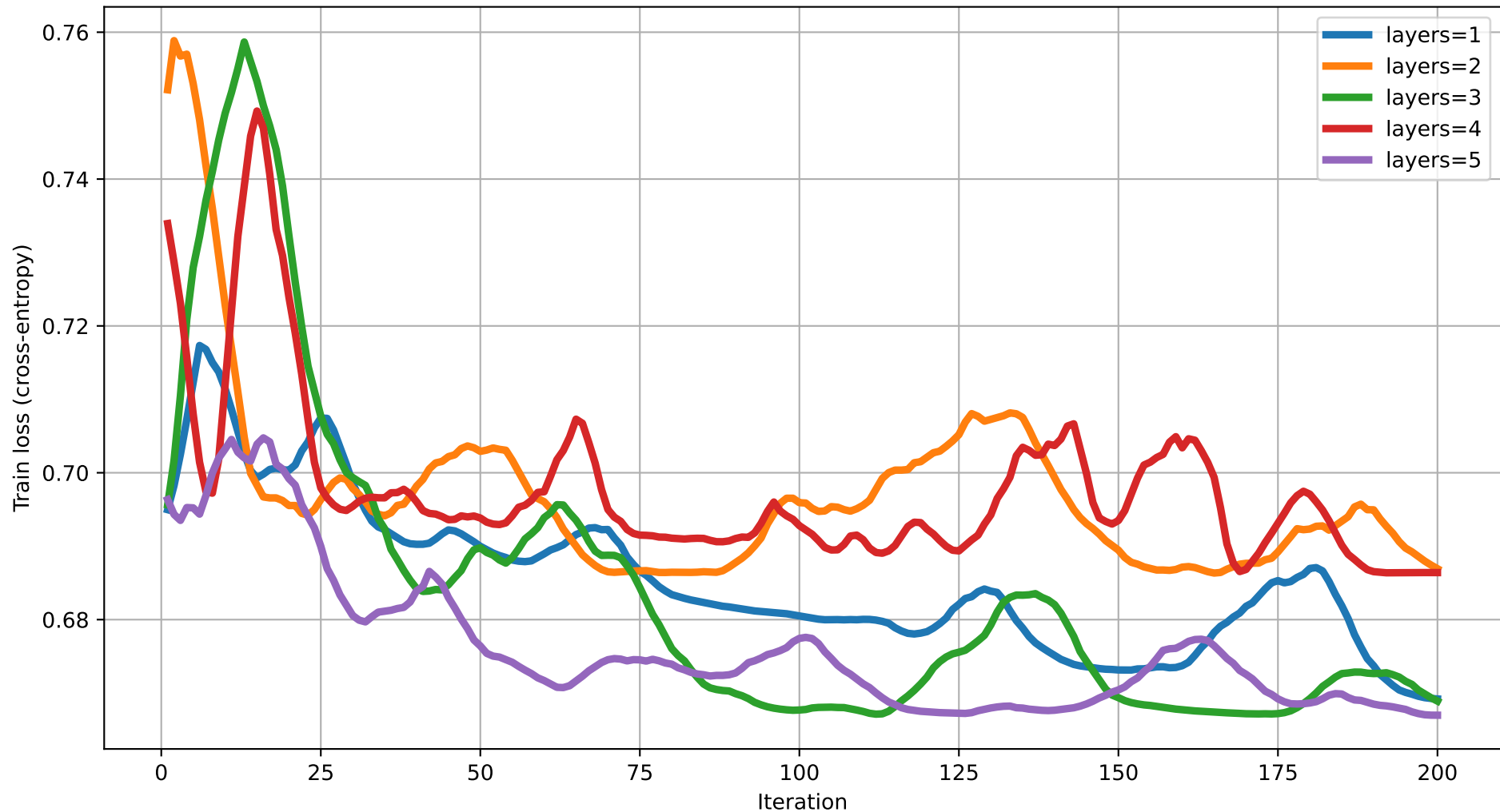
Train loss vs Iteration (dim=10) rot=RX, ent=chain, gate=IsingXX
