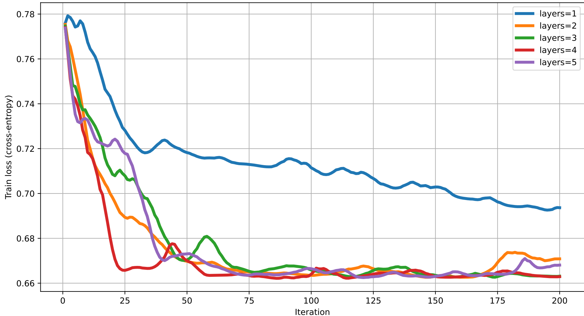
Train loss vs Iteration (dim=9) rot=RX, ent=pairwise, gate=CZ
