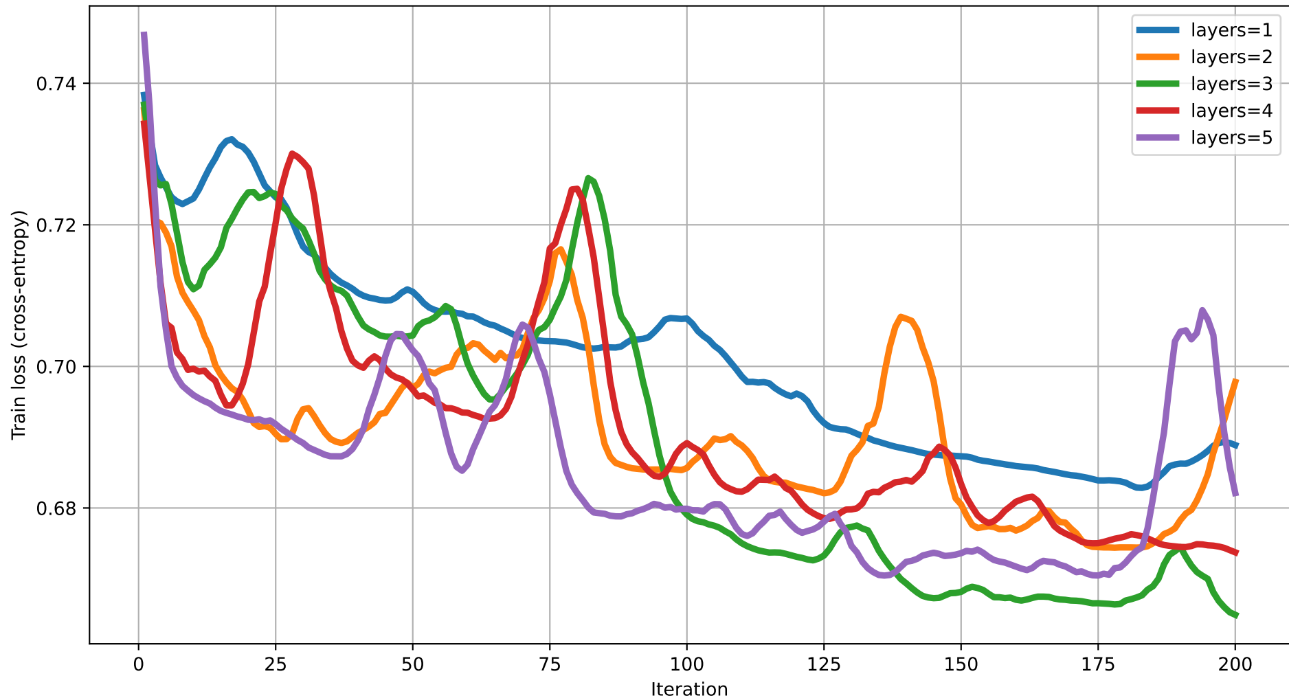
Train loss vs Iteration (dim=18) rot=RZ, ent=full, gate=IsingXX
