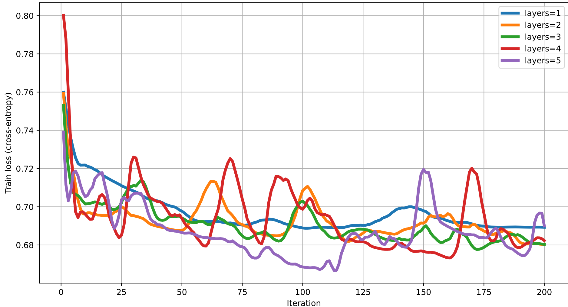
Train loss vs Iteration (dim=17) rot=RYZ, ent=full, gate=IsingXX
