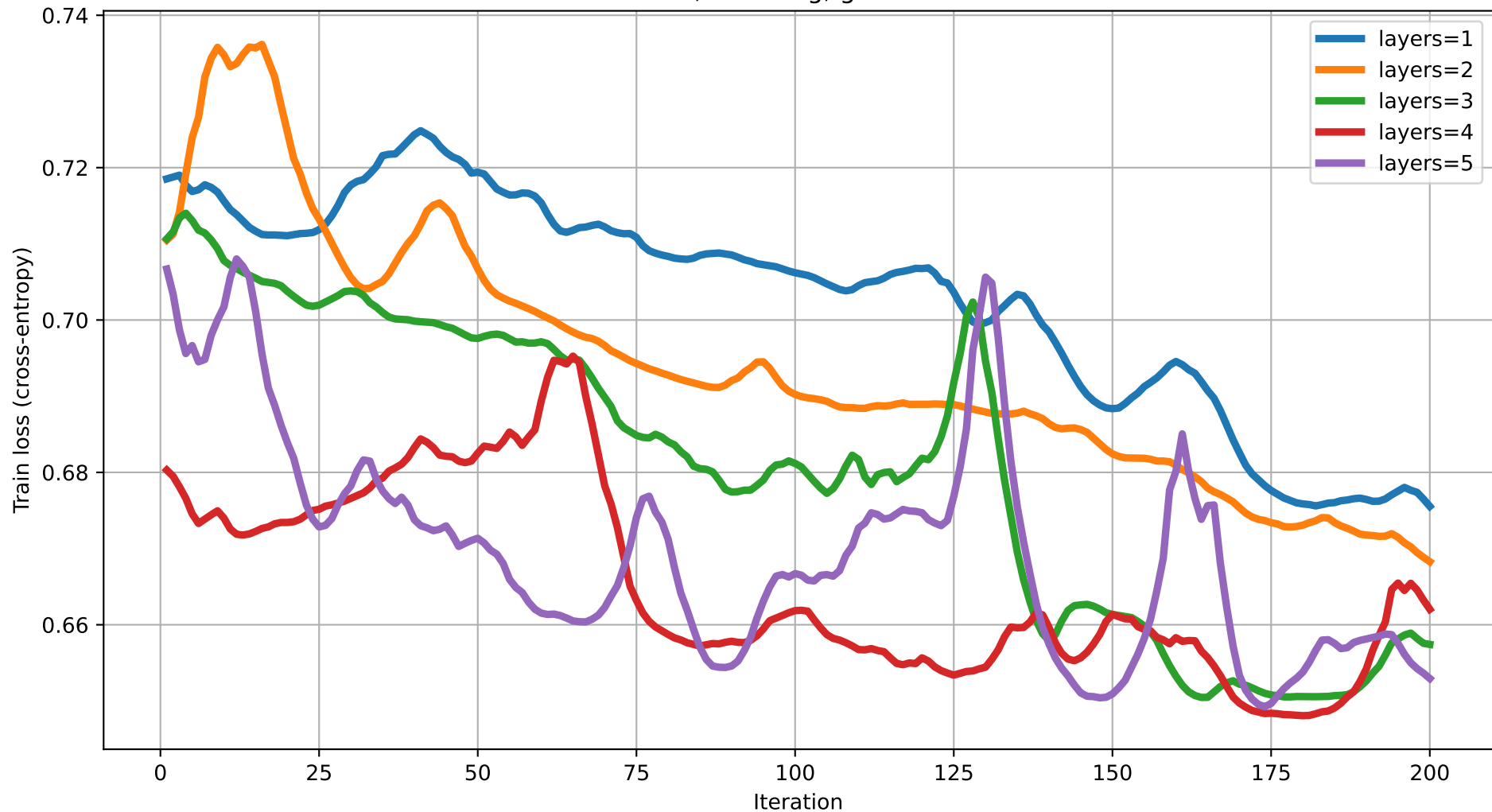
Train loss vs Iteration (dim=7) rot=RY, ent=ring, gate=CNOT
