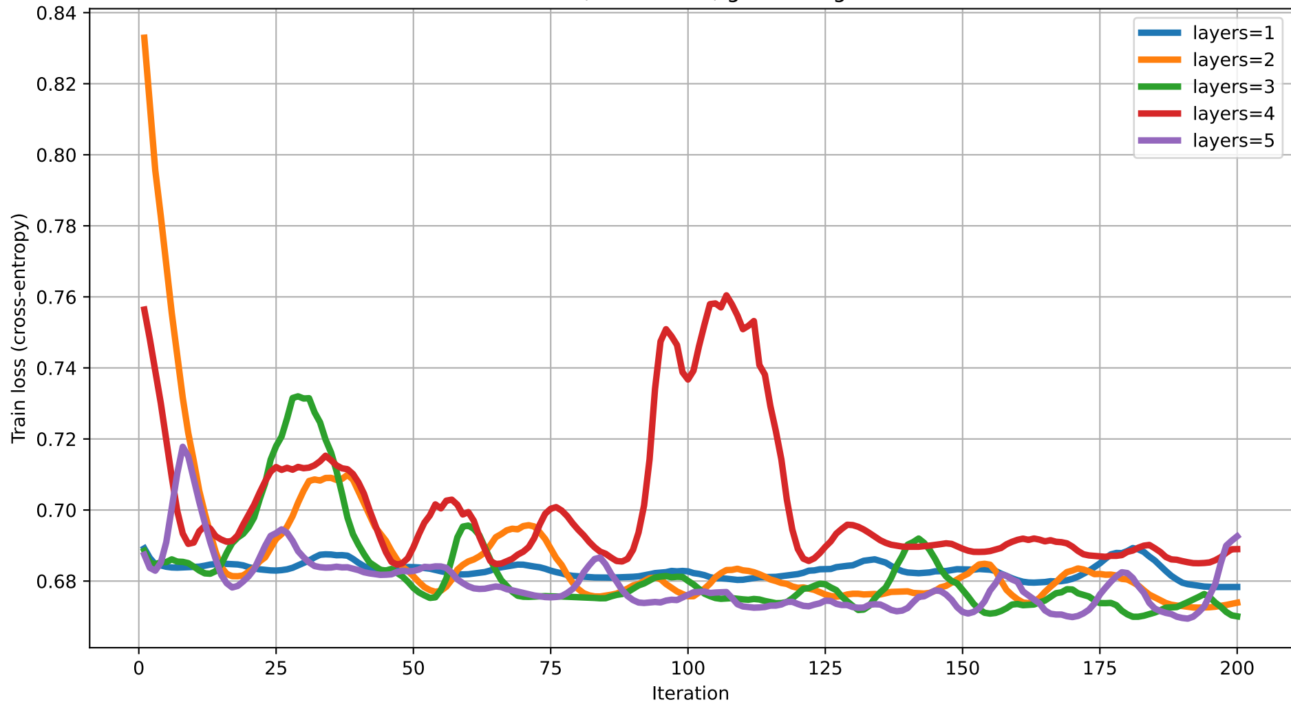
Train loss vs Iteration (dim=16) rot=RZ, ent=chain, gate=IsingXX
