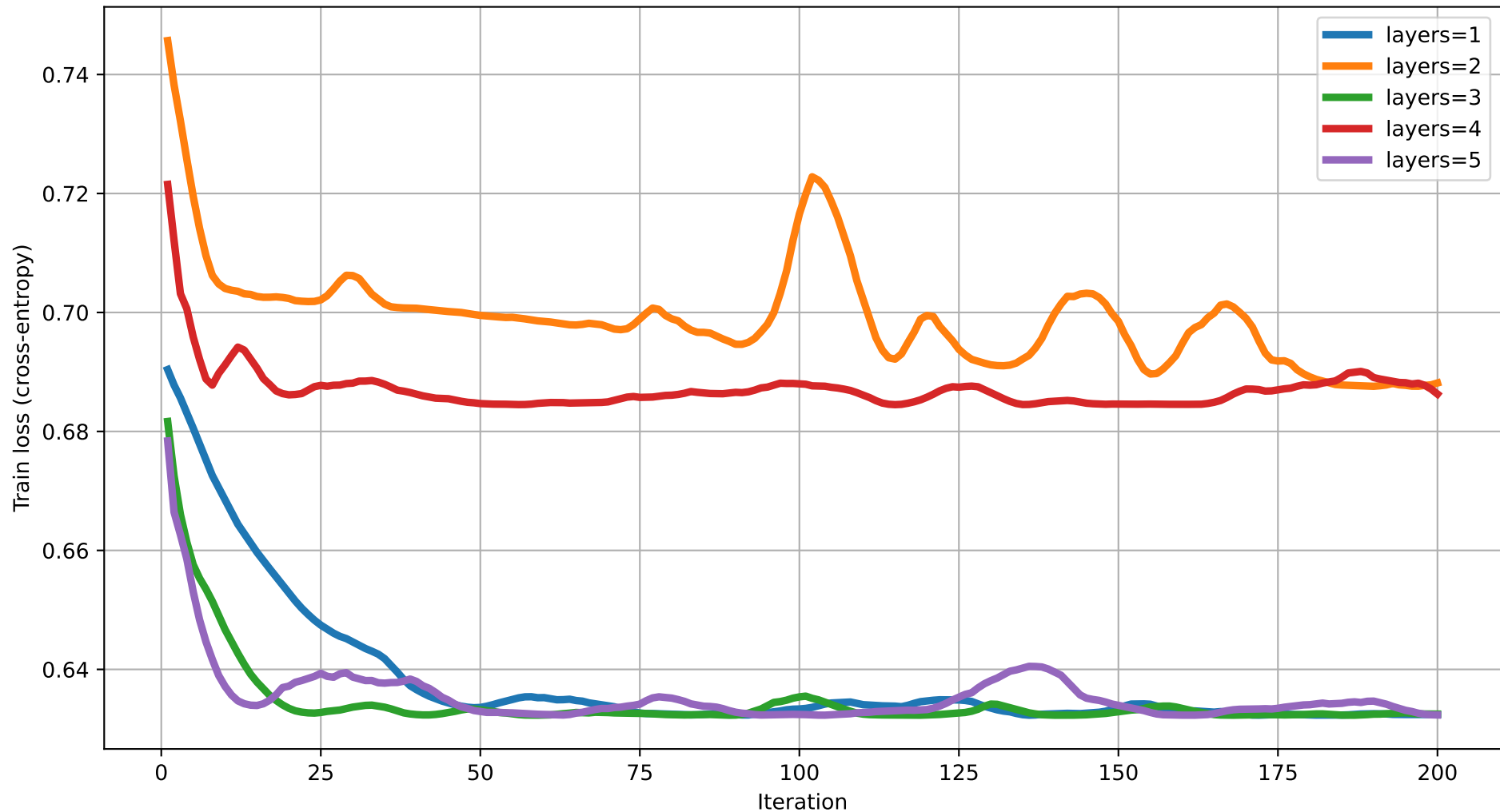
Train loss vs Iteration (degree=3) rot=RX, ent=full, gate=IsingXX
