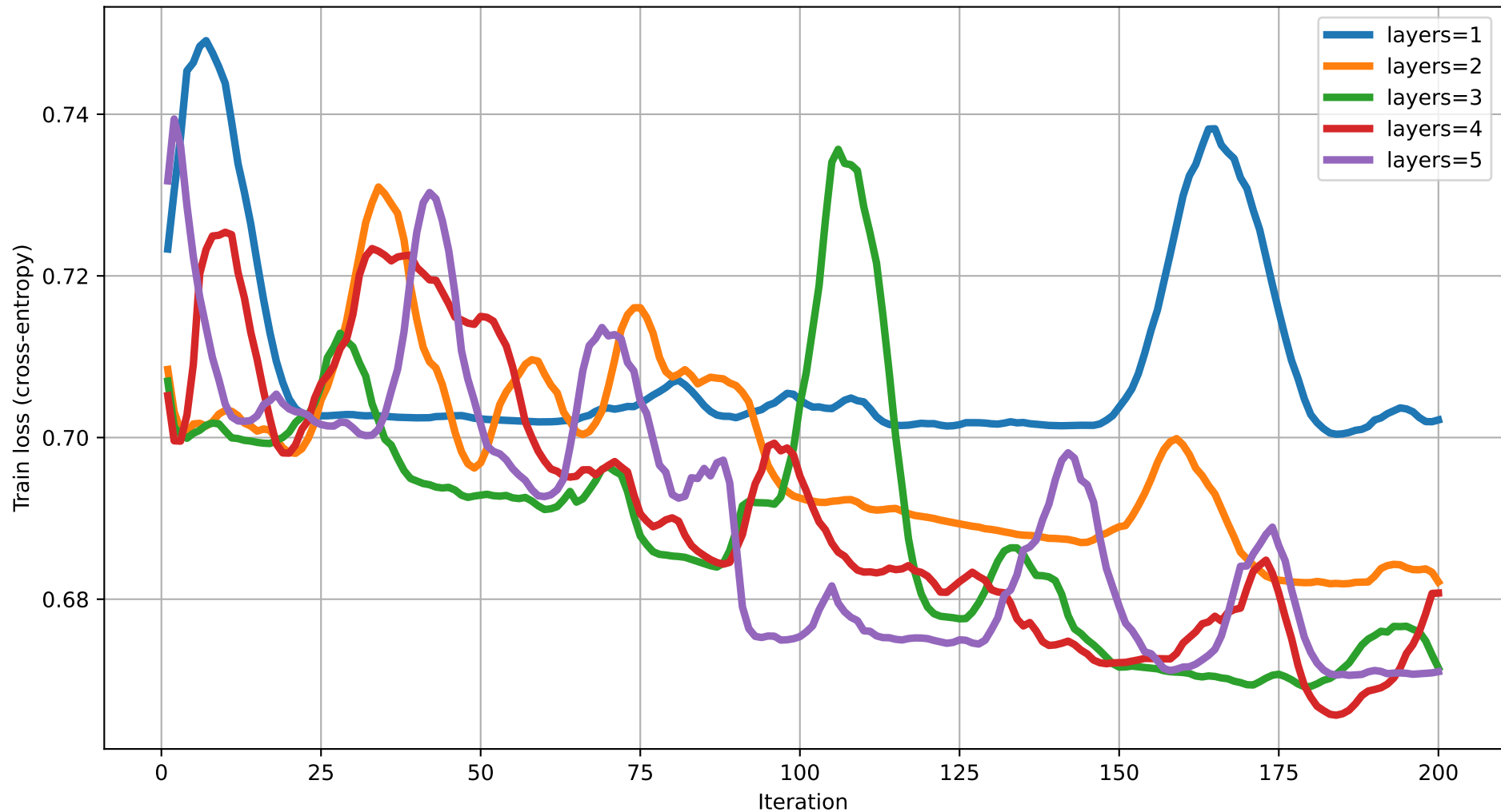
Train loss vs Iteration (dim=11) rot=RYZ, ent=pairwise, gate=CNOT
