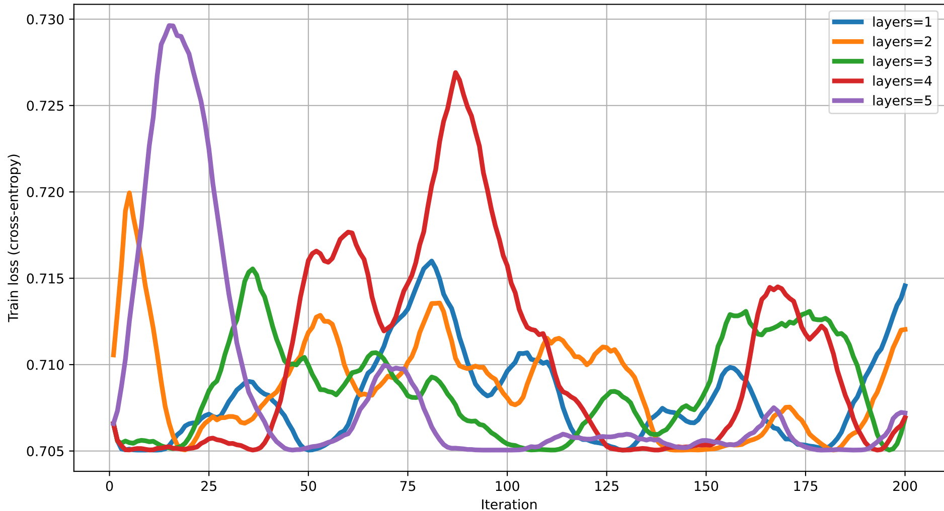
Train loss vs Iteration (dim=14) rot=RZ, ent=pairwise, gate=CNOT
