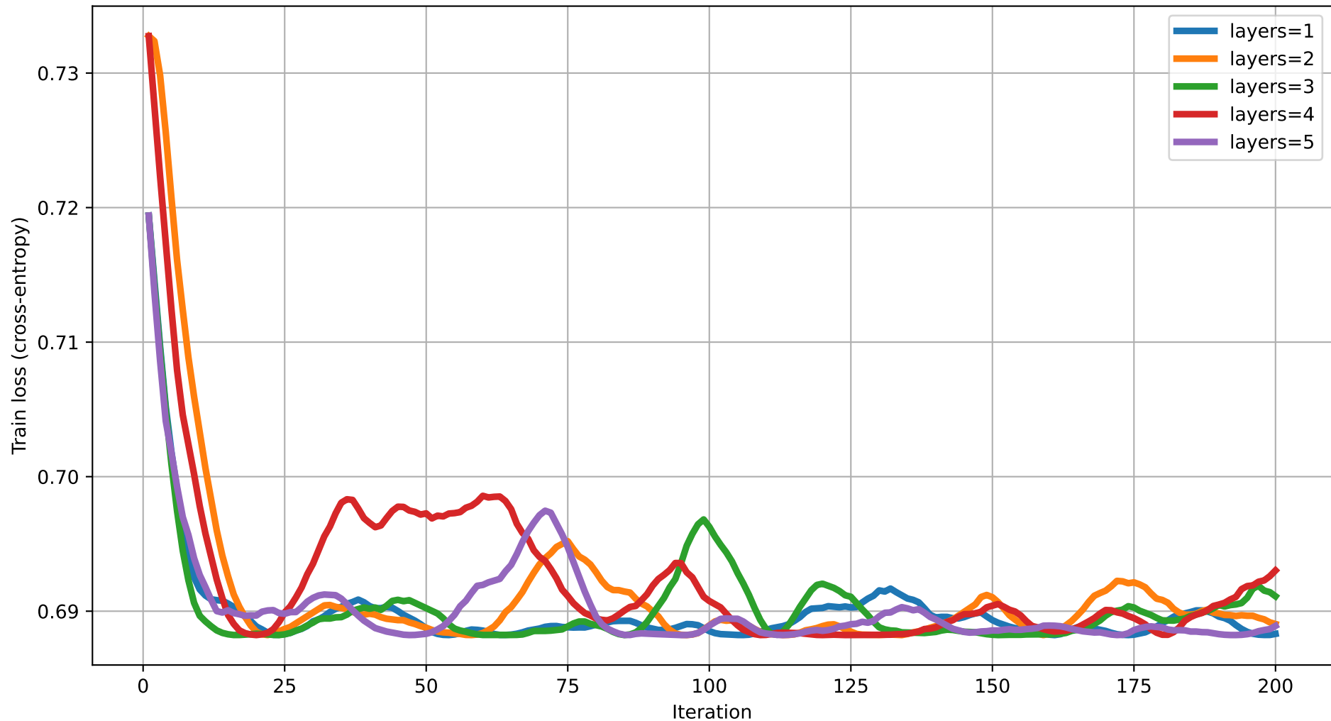
Train loss vs Iteration (degree=4) rot=RZ, ent=full, gate=CNOT
