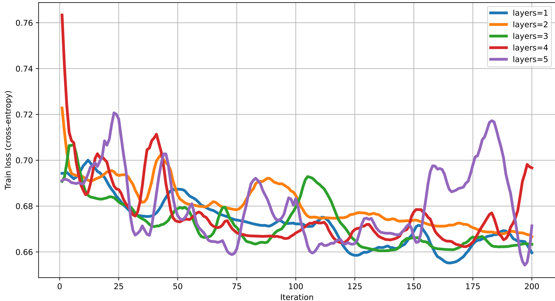
Train loss vs Iteration (dim=9) rot=RYZ, ent=pairwise, gate=IsingXX
