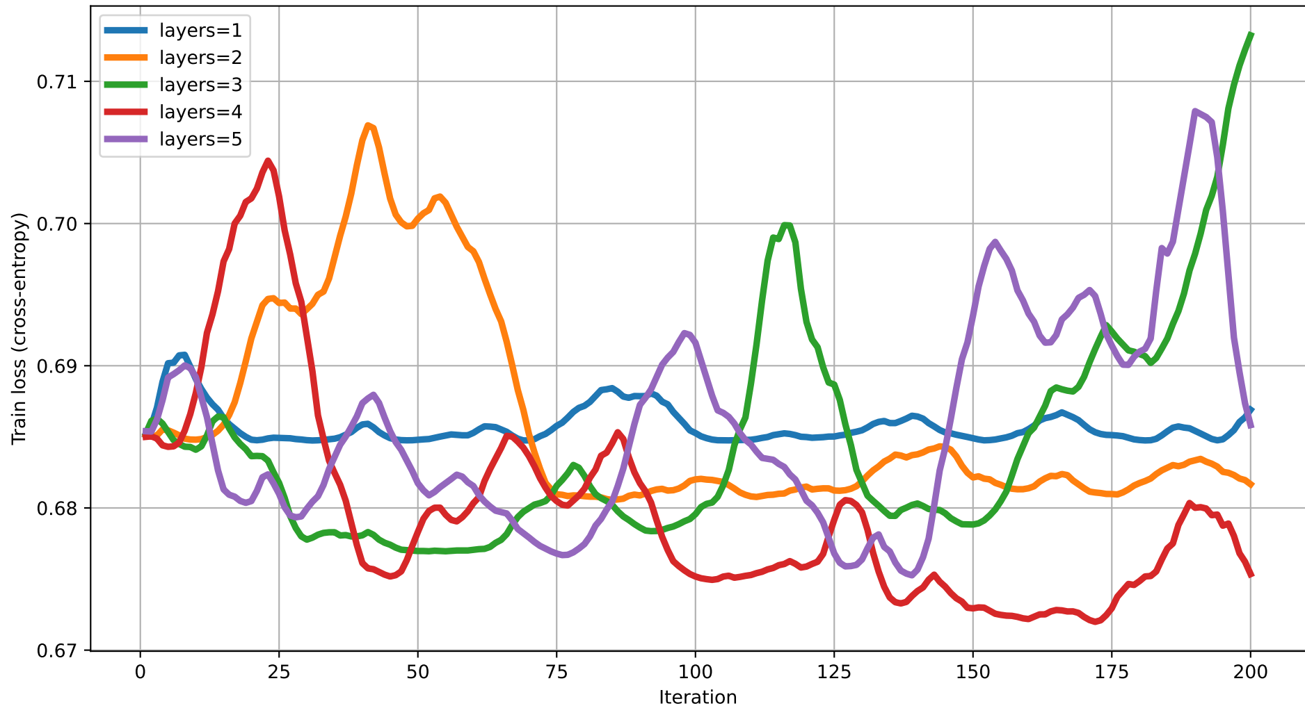
Train loss vs Iteration (dim=15) rot=RX, ent=pairwise, gate=CZ
