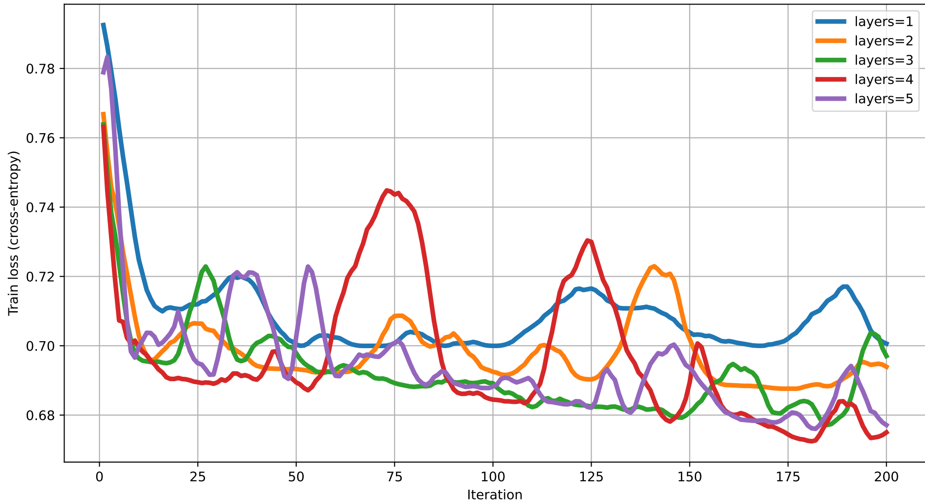
Train loss vs Iteration (dim=17) rot=RY, ent=full, gate=CZ
