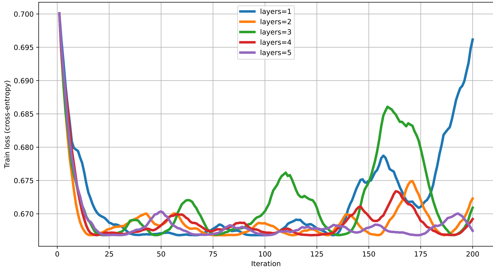
Train loss vs Iteration (dim=10) rot=RZ, ent=pairwise, gate=CNOT
