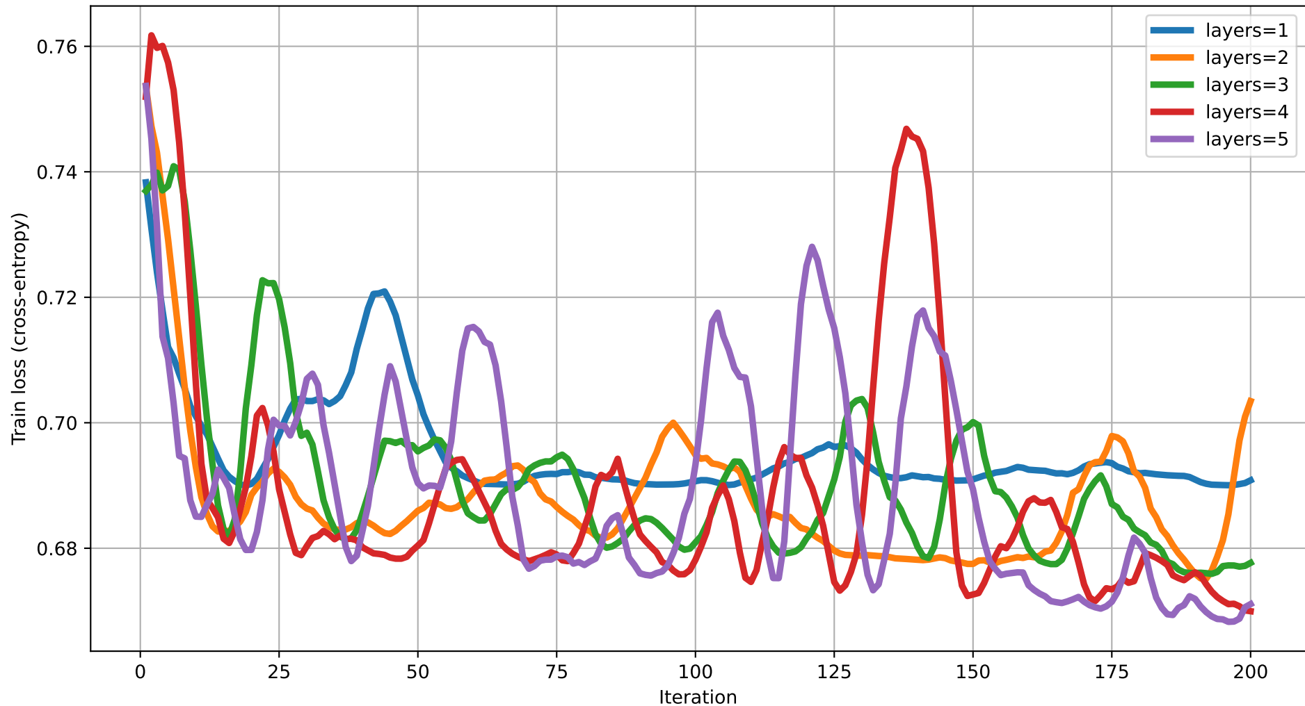
Train loss vs Iteration (dim=16) rot=RX, ent=pairwise, gate=CNOT
