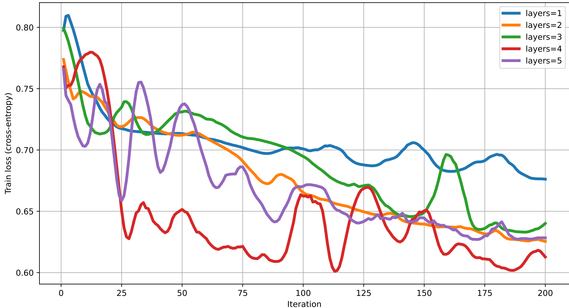
Train loss vs Iteration (dim=4) rot=RYZ, ent=chain, gate=CNOT
