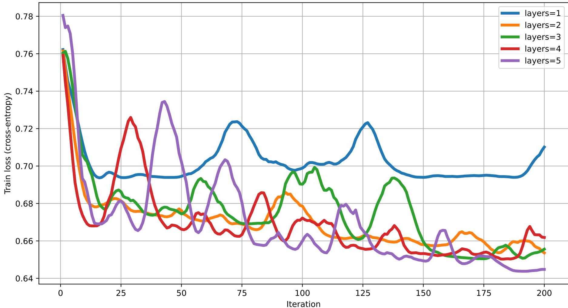
Train loss vs Iteration (dim=8) rot=RX, ent=pairwise, gate=CNOT
