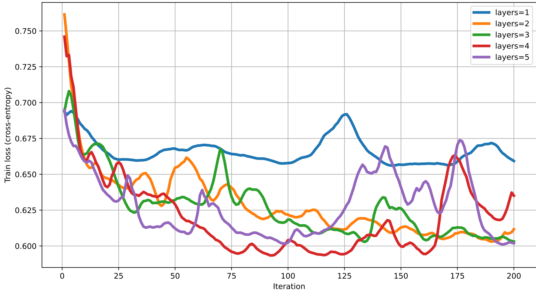
Train loss vs Iteration (dim=8) rot=Rot, ent=ring, gate=IsingXX
