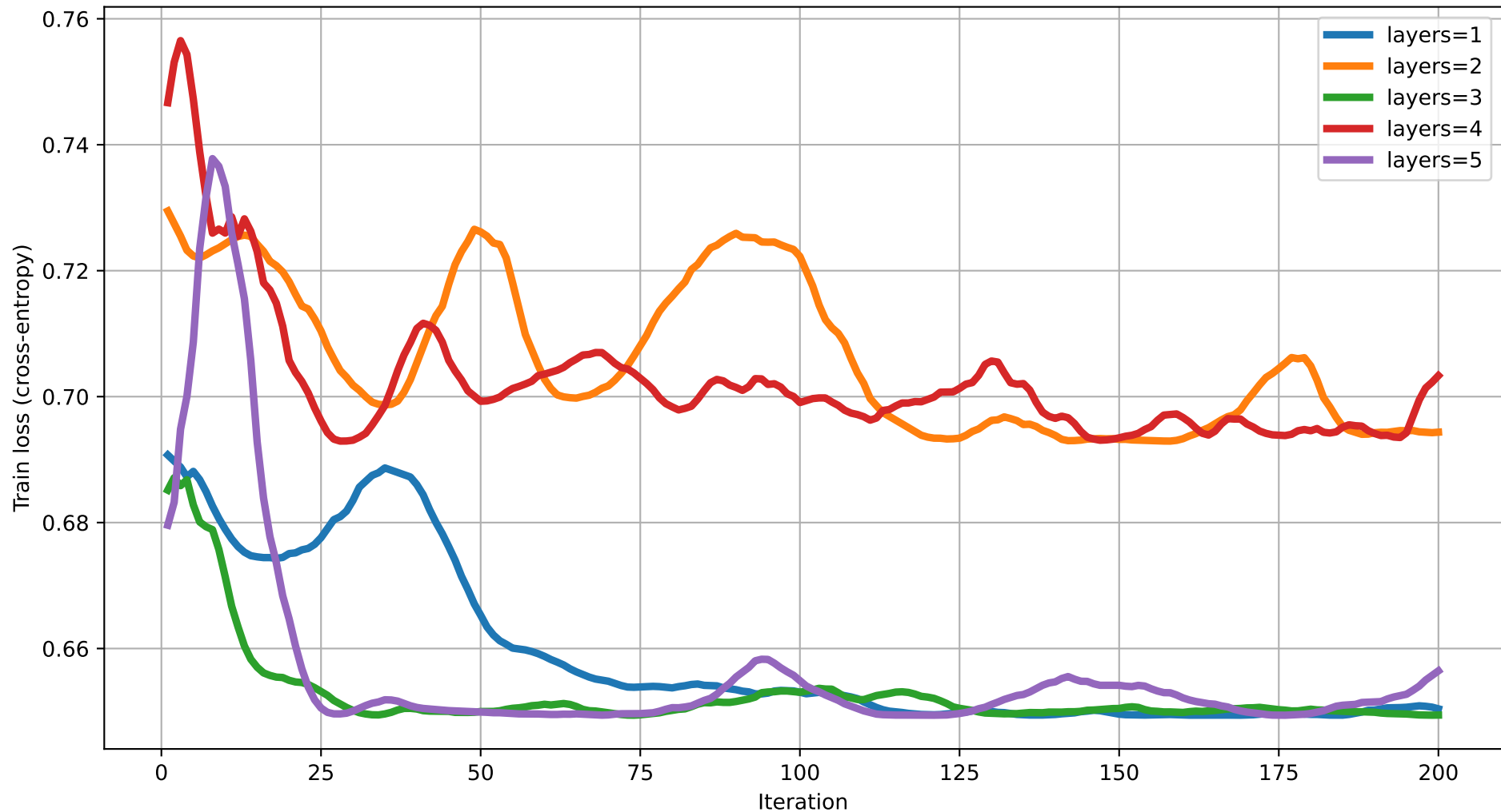
Train loss vs Iteration (dim=3) rot=RX, ent=chain, gate=IsingXX
