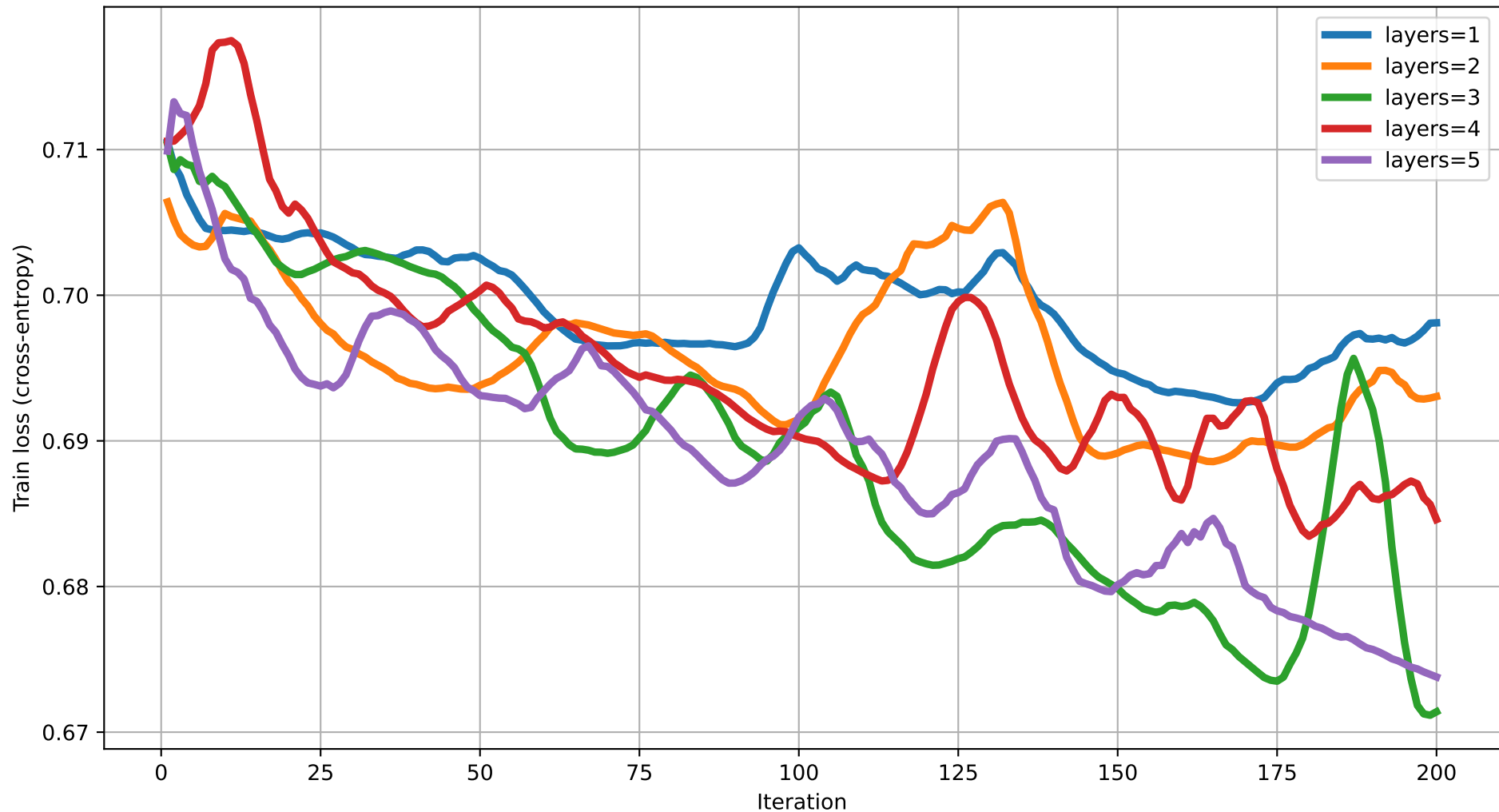
Train loss vs Iteration (dim=14) rot=RX, ent=full, gate=CZ
