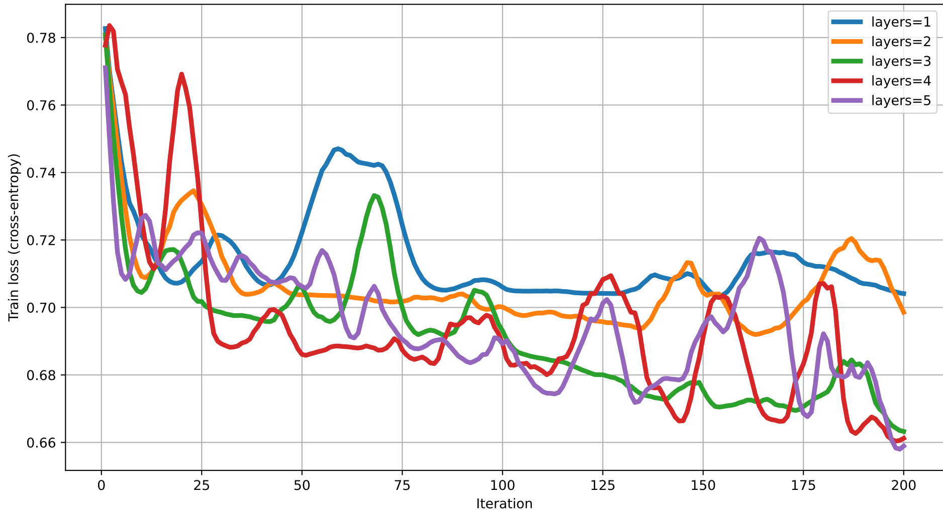
Train loss vs Iteration (dim=9) rot=Rot, ent=chain, gate=CZ
