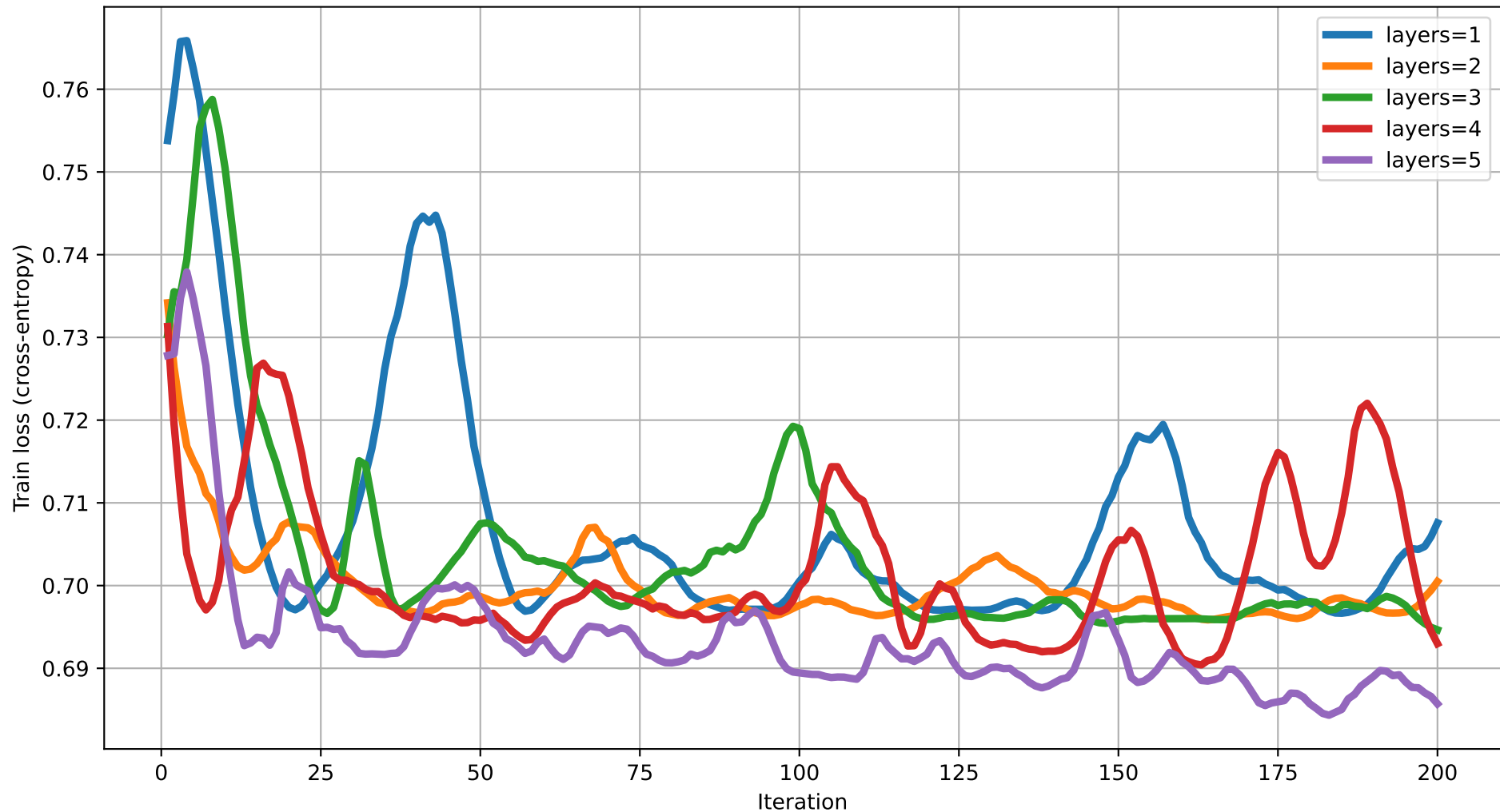
Train loss vs Iteration (dim=18) rot=Rot, ent=ring, gate=CZ
