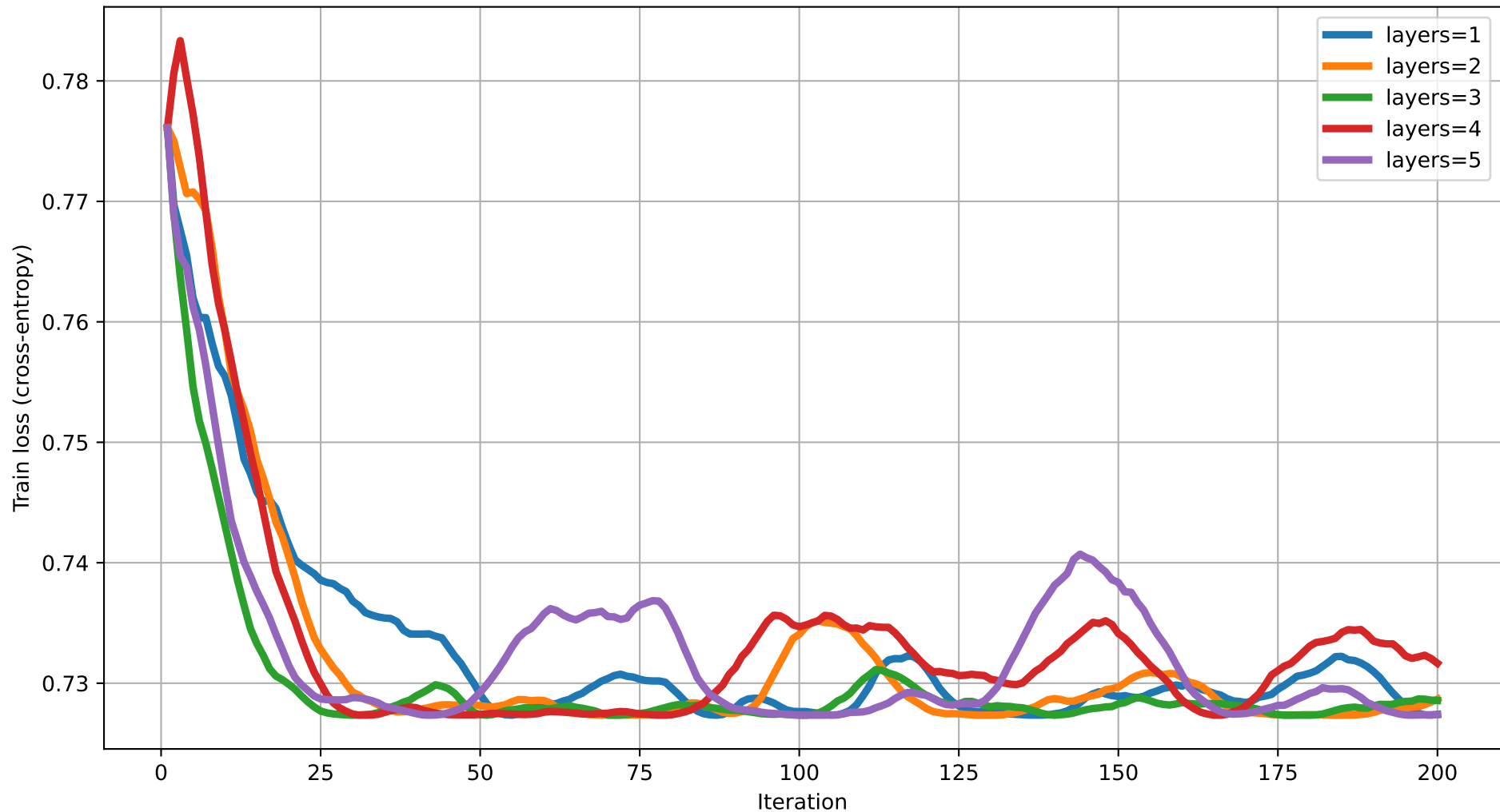
Train loss vs Iteration (dim=9) rot=RZ, ent=full, gate=CNOT
