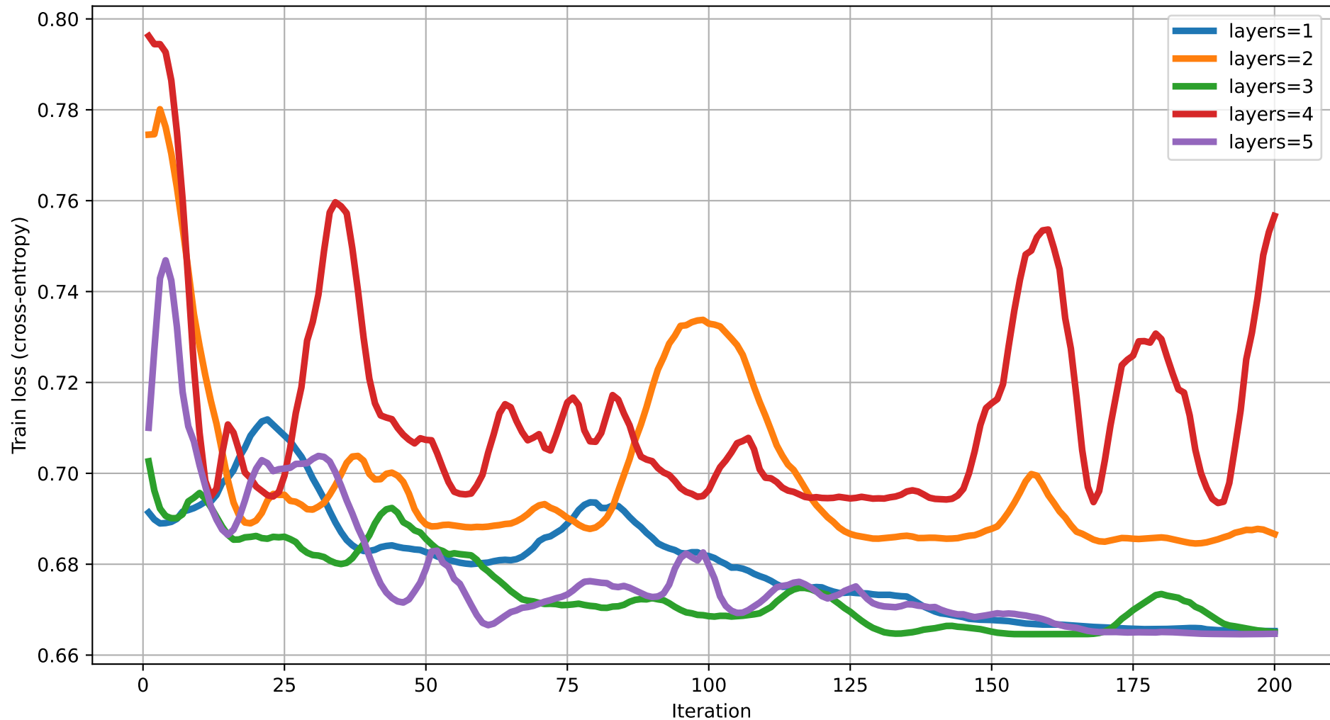
Train loss vs Iteration (dim=8) rot=RX, ent=pairwise, gate=IsingXX
