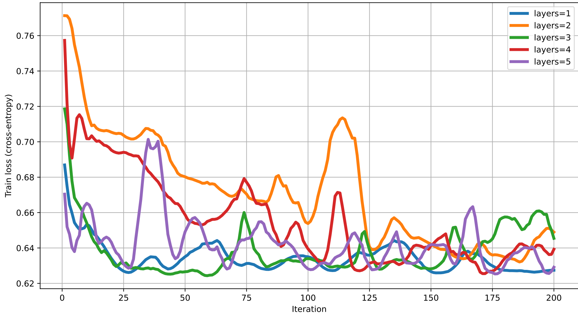
Train loss vs Iteration (dim=4) rot=Rot, ent=full, gate=IsingXX
