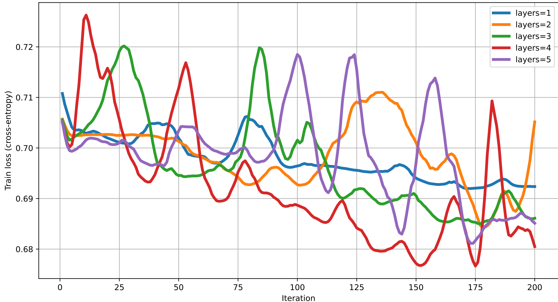
Train loss vs Iteration (dim=12) rot=RX, ent=pairwise, gate=CZ
