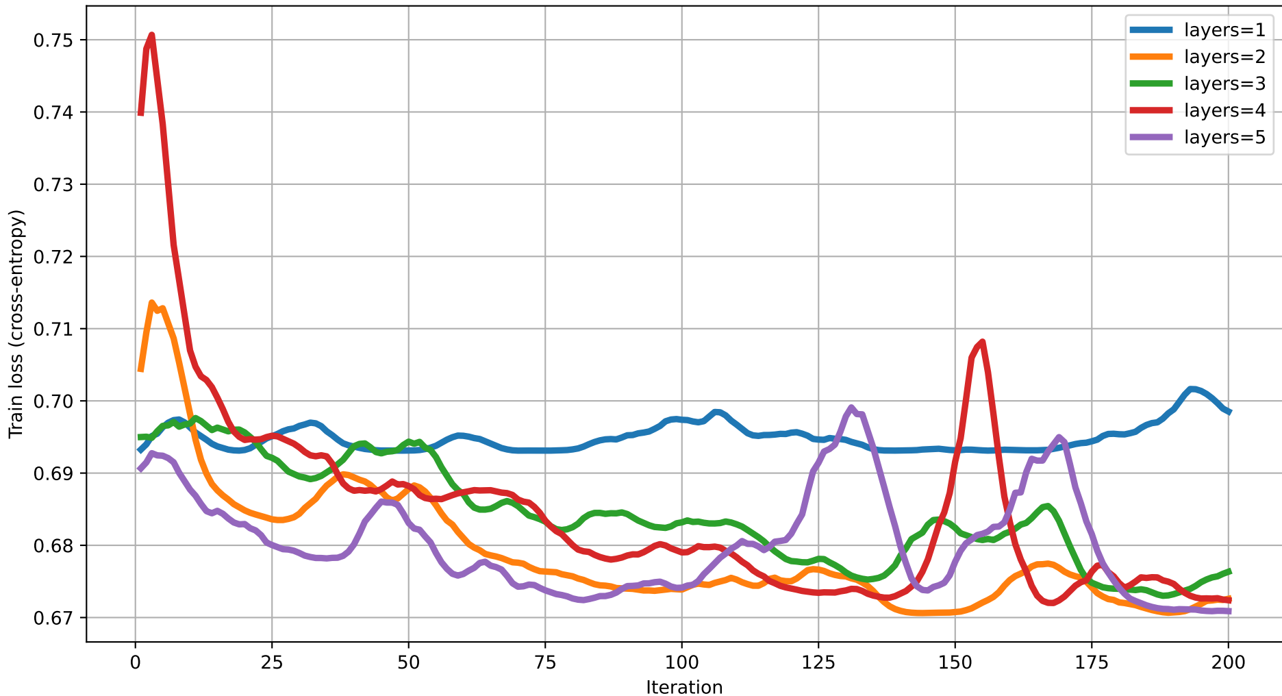
Train loss vs Iteration (dim=6) rot=RY, ent=pairwise, gate=IsingXX
