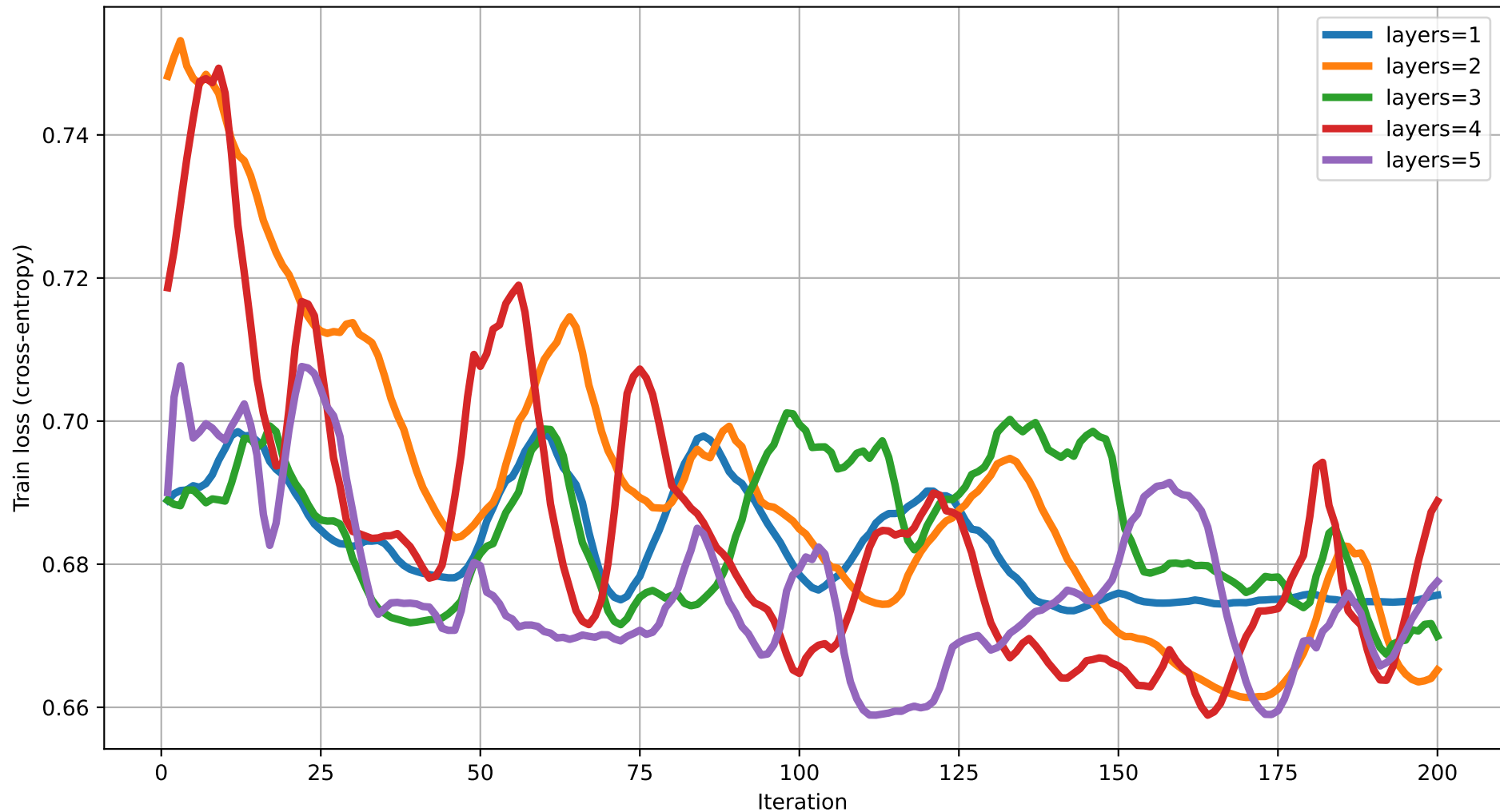
Train loss vs Iteration (dim=3) rot=Rot, ent=pairwise, gate=IsingXX
