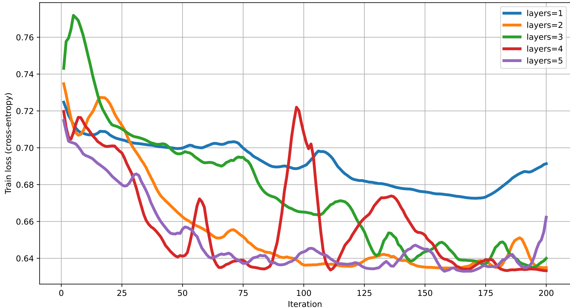
Train loss vs Iteration (dim=6) rot=RY, ent=pairwise, gate=CNOT
