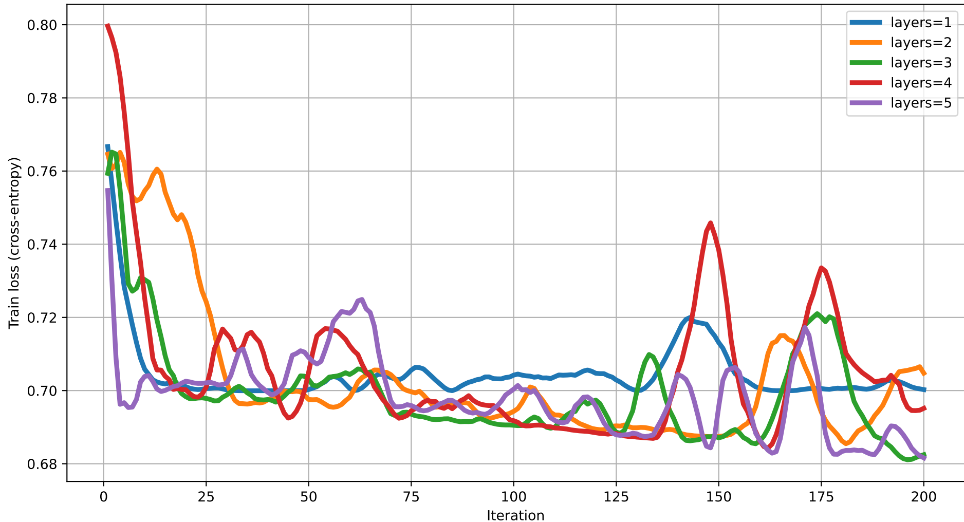
Train loss vs Iteration (dim=17) rot=RY, ent=pairwise, gate=CNOT
