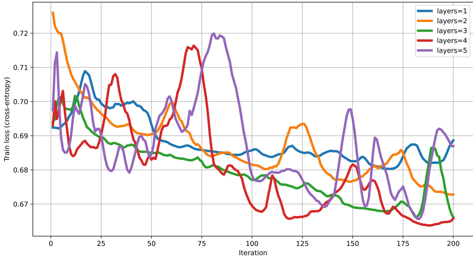
Train loss vs Iteration (dim=15) rot=YRZ, ent=pairwise, gate=IsingXX
