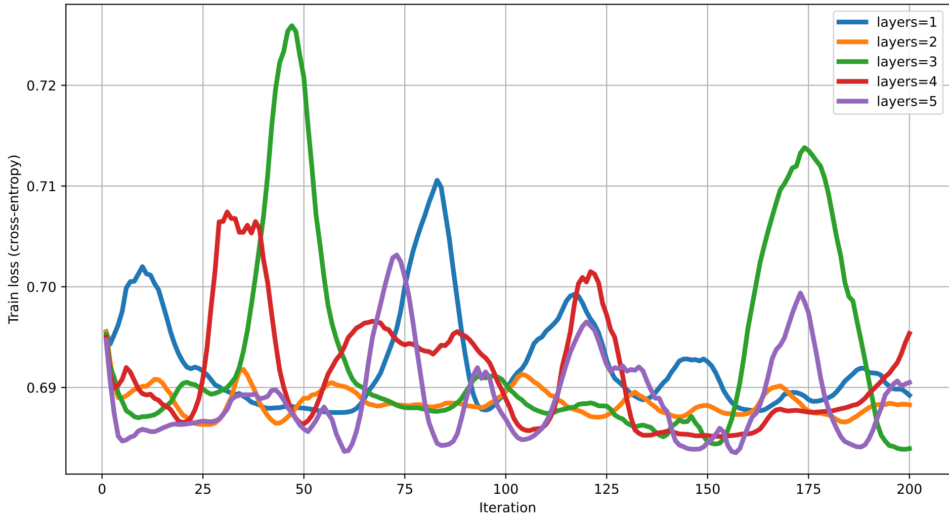
Train loss vs Iteration (dim=13) rot=RX, ent=pairwise, gate=CNOT
