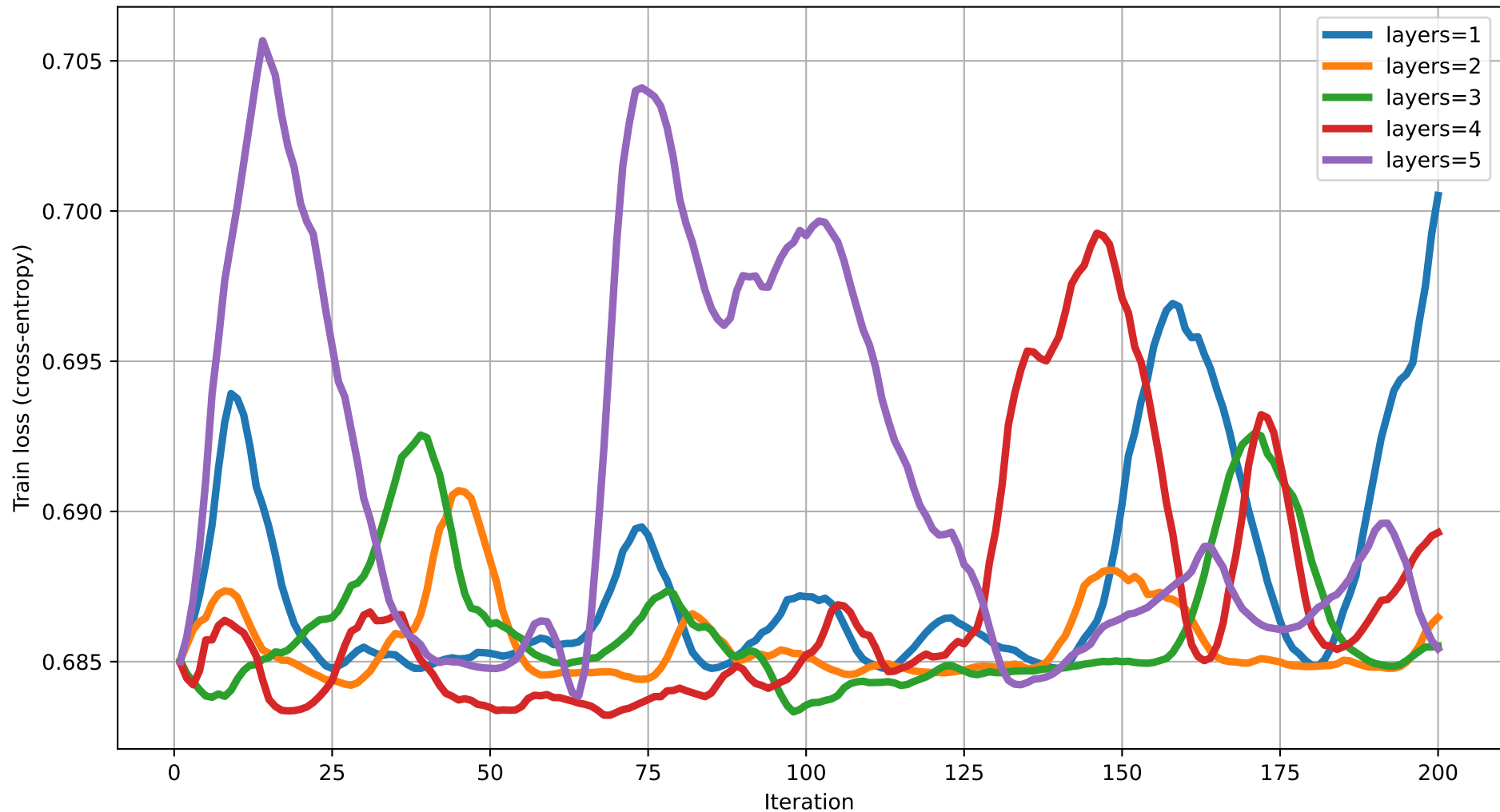
Train loss vs Iteration (dim=15) rot=RX, ent=chain, gate=CNOT
