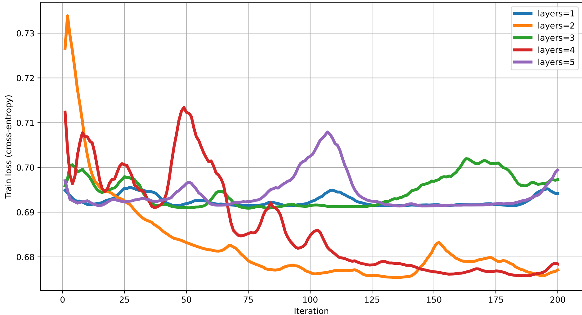
Train loss vs Iteration (dim=12) rot=RY, ent=chain, gate=IsingXX
