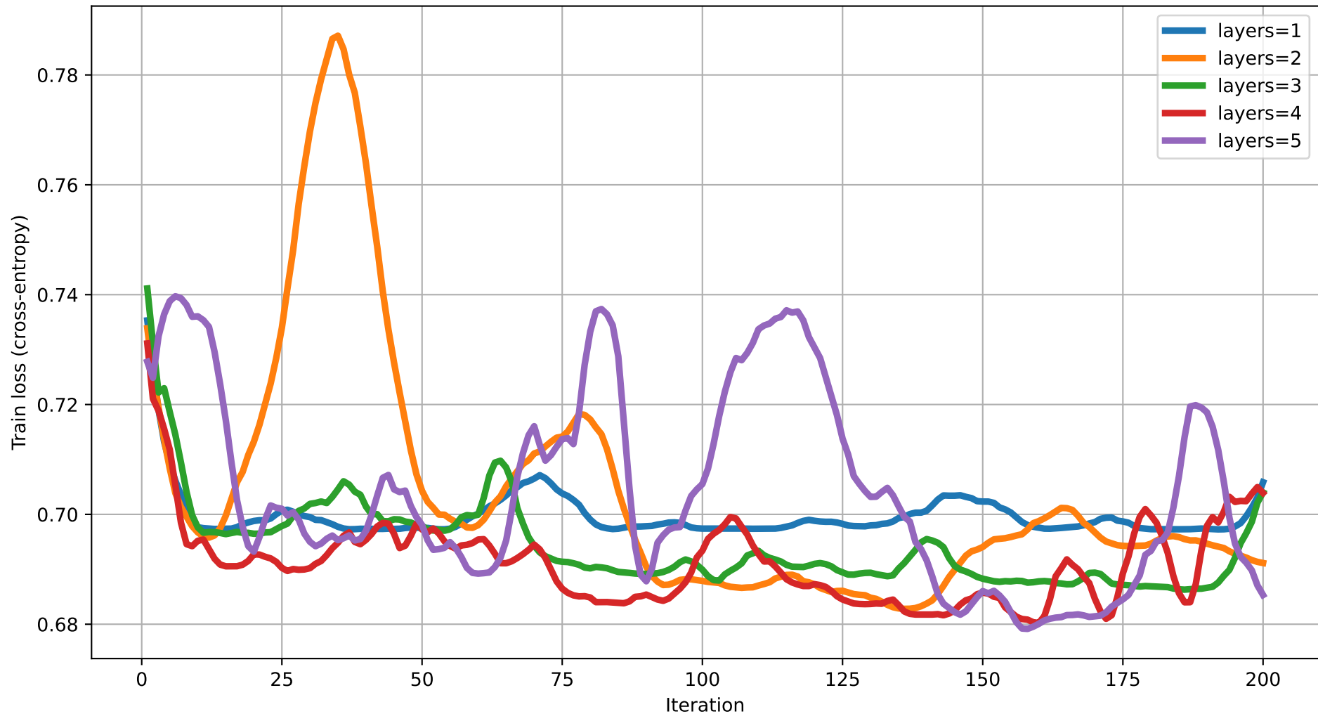
Train loss vs Iteration (dim=18) rot=Rot, ent=full, gate=CZ
