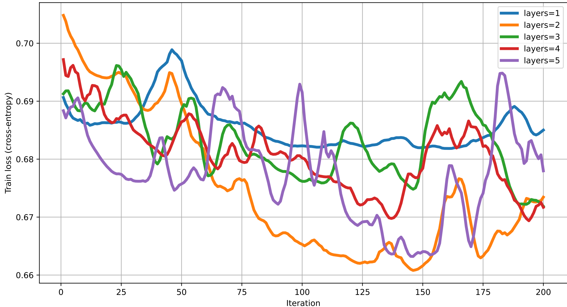
Train loss vs Iteration (dim=18) rot=RYZ, ent=ring, gate=CNOT
