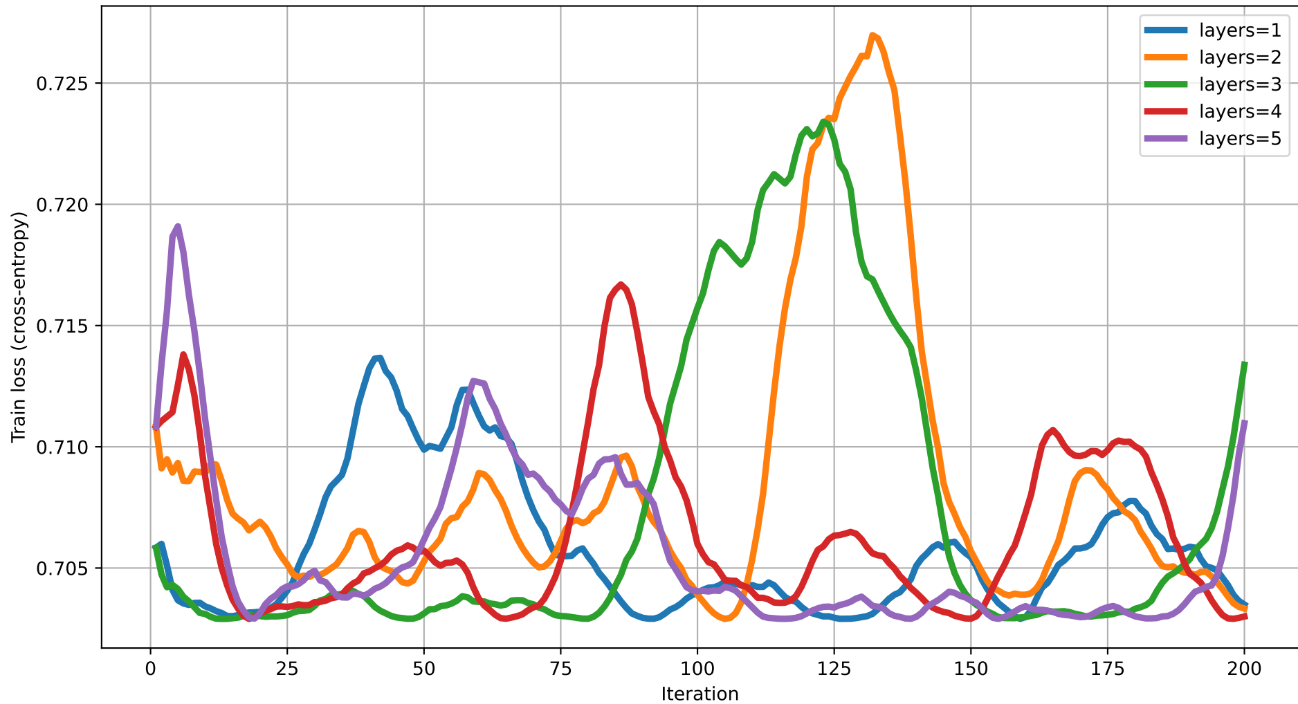
Train loss vs Iteration (dim=12) rot=RZ, ent=chain, gate=CZ
