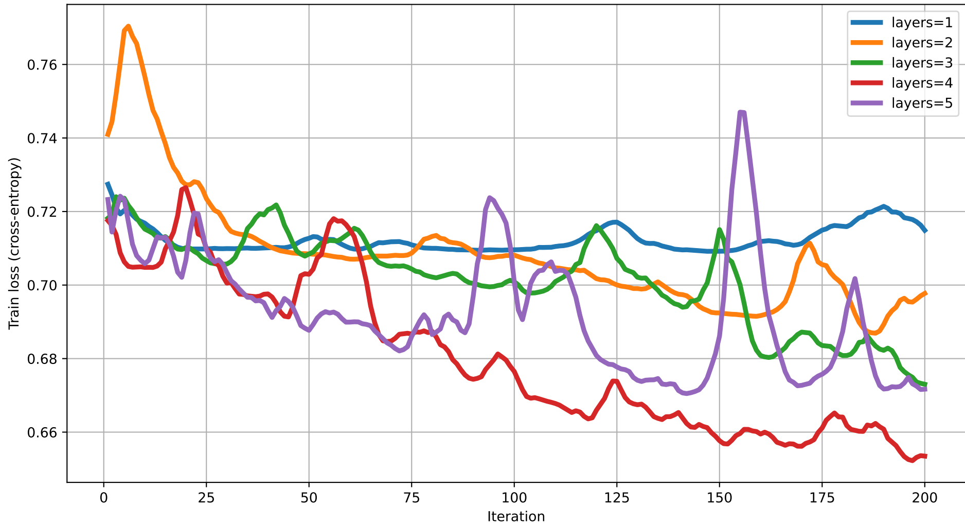
Train loss vs Iteration (dim=10) rot=Rot, ent=full, gate=CNOT
