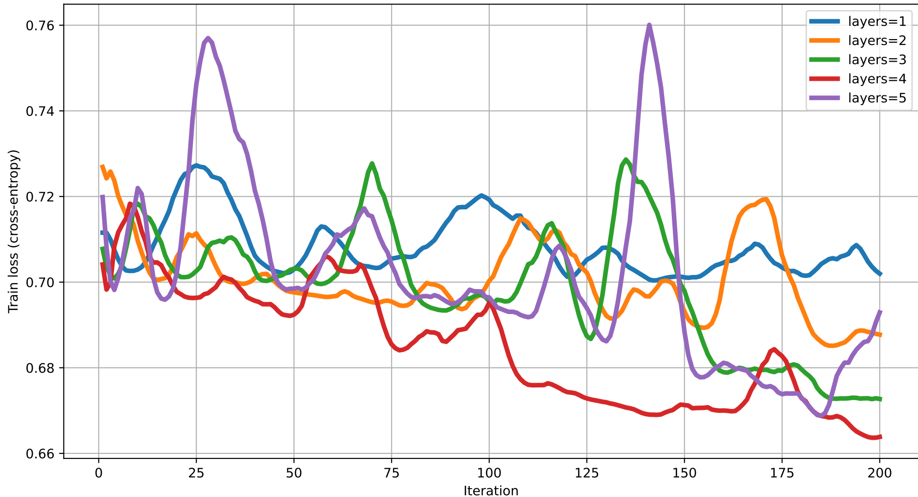
Train loss vs Iteration (dim=11) rot=RY, ent=chain, gate=CNOT
