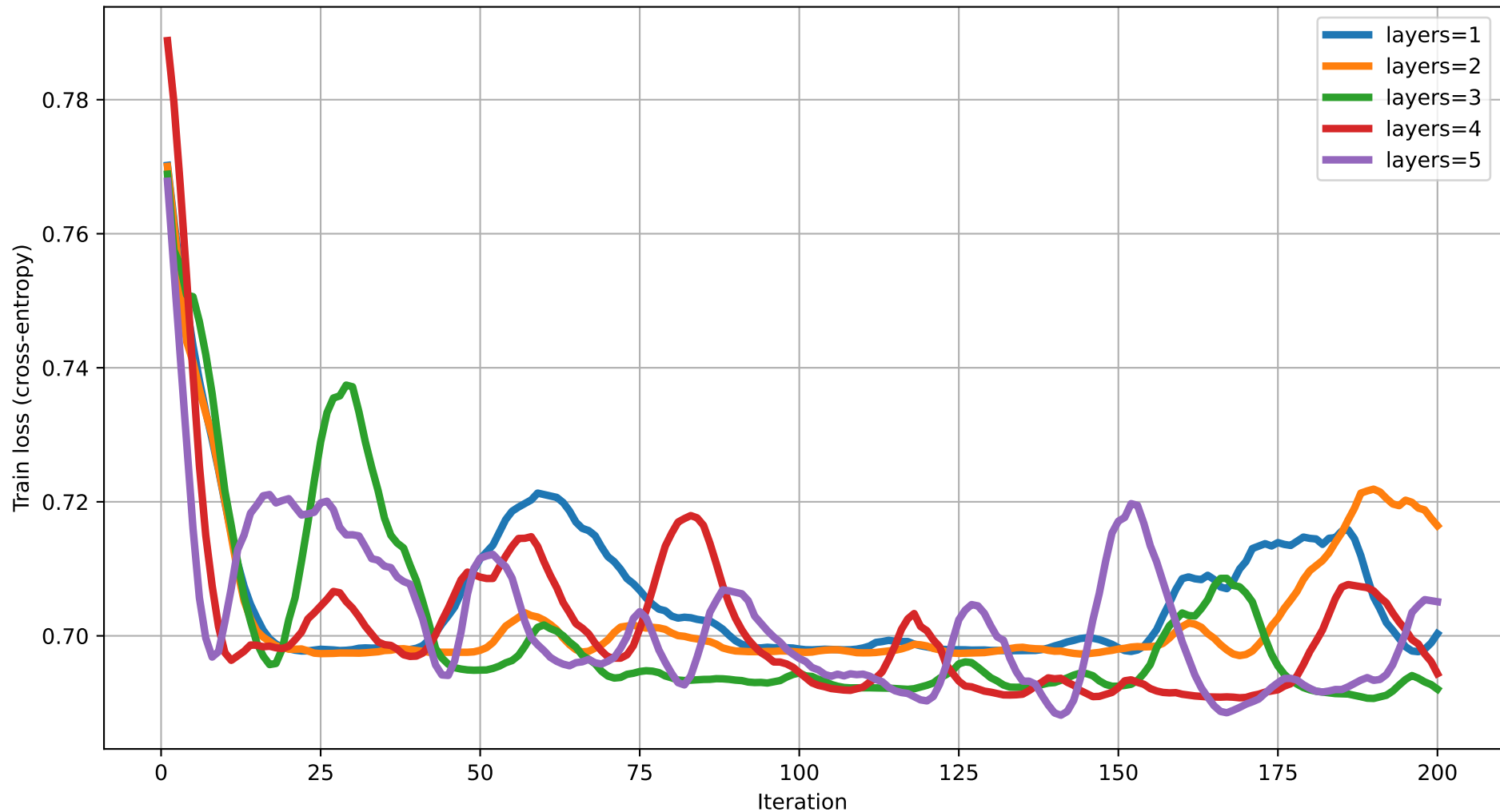
Train loss vs Iteration (dim=17) rot=RX, ent=ring, gate=CZ
