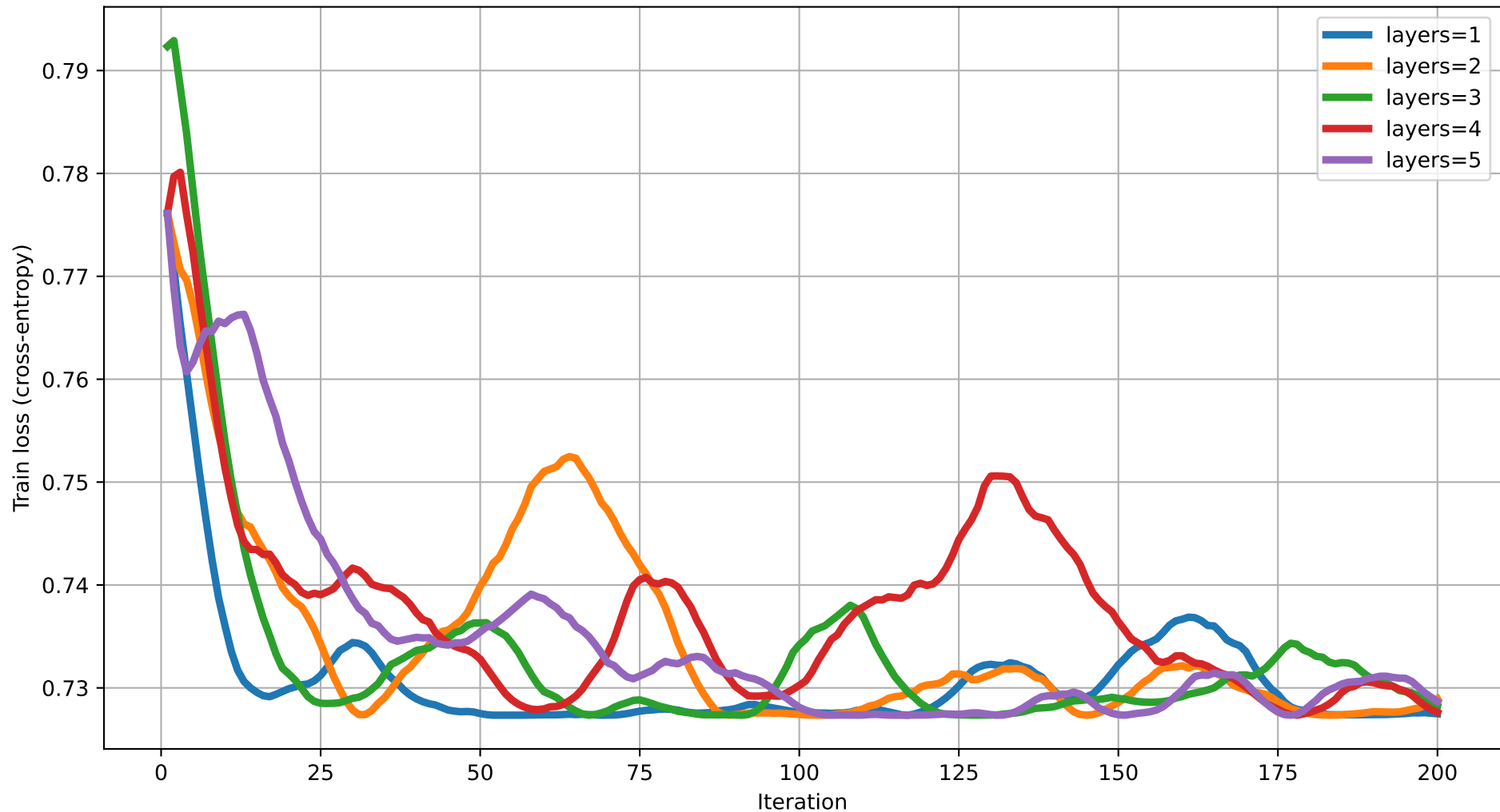
Train loss vs Iteration (dim=9) rot=RZ, ent=ring, gate=CZ
