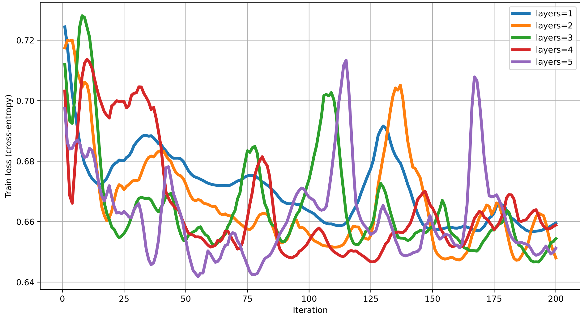
Train loss vs Iteration (dim=5) rot=Rot, ent=full, gate=IsingXX
