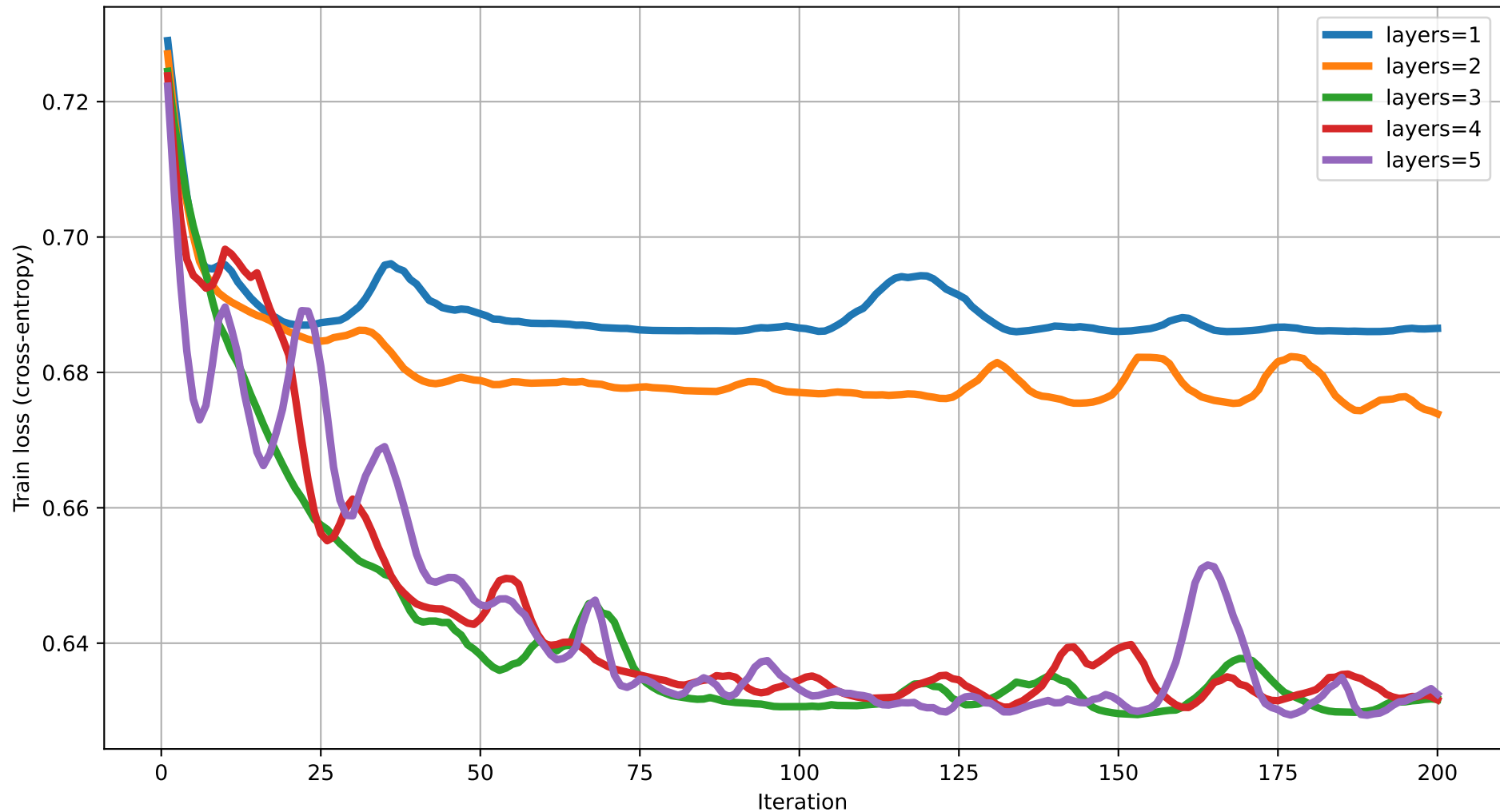
Train loss vs Iteration (degree=2) rot=RYZ, ent=pairwise, gate=CZ
