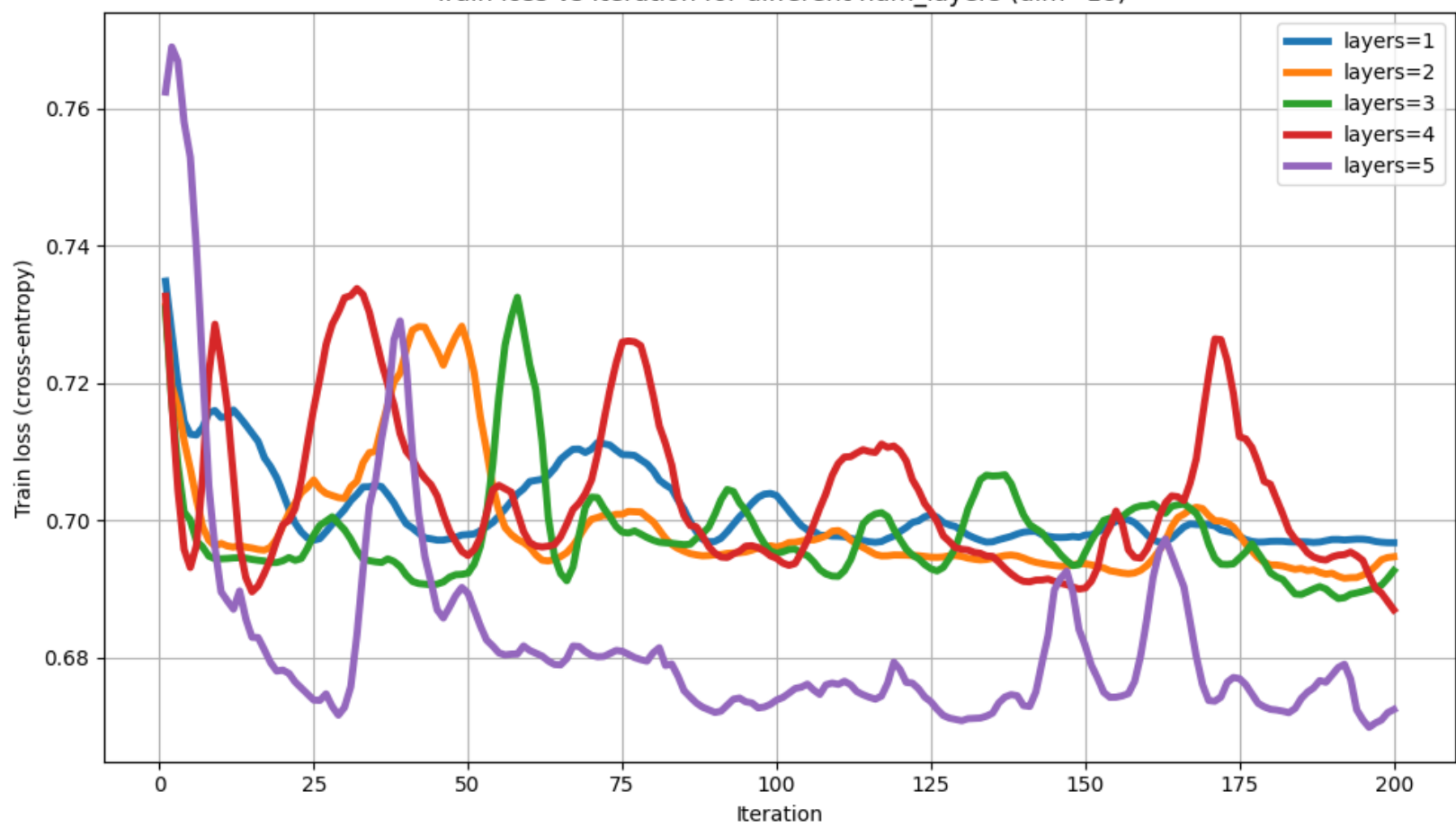
Train loss vs Iteration for different num_layers (dim=18)
