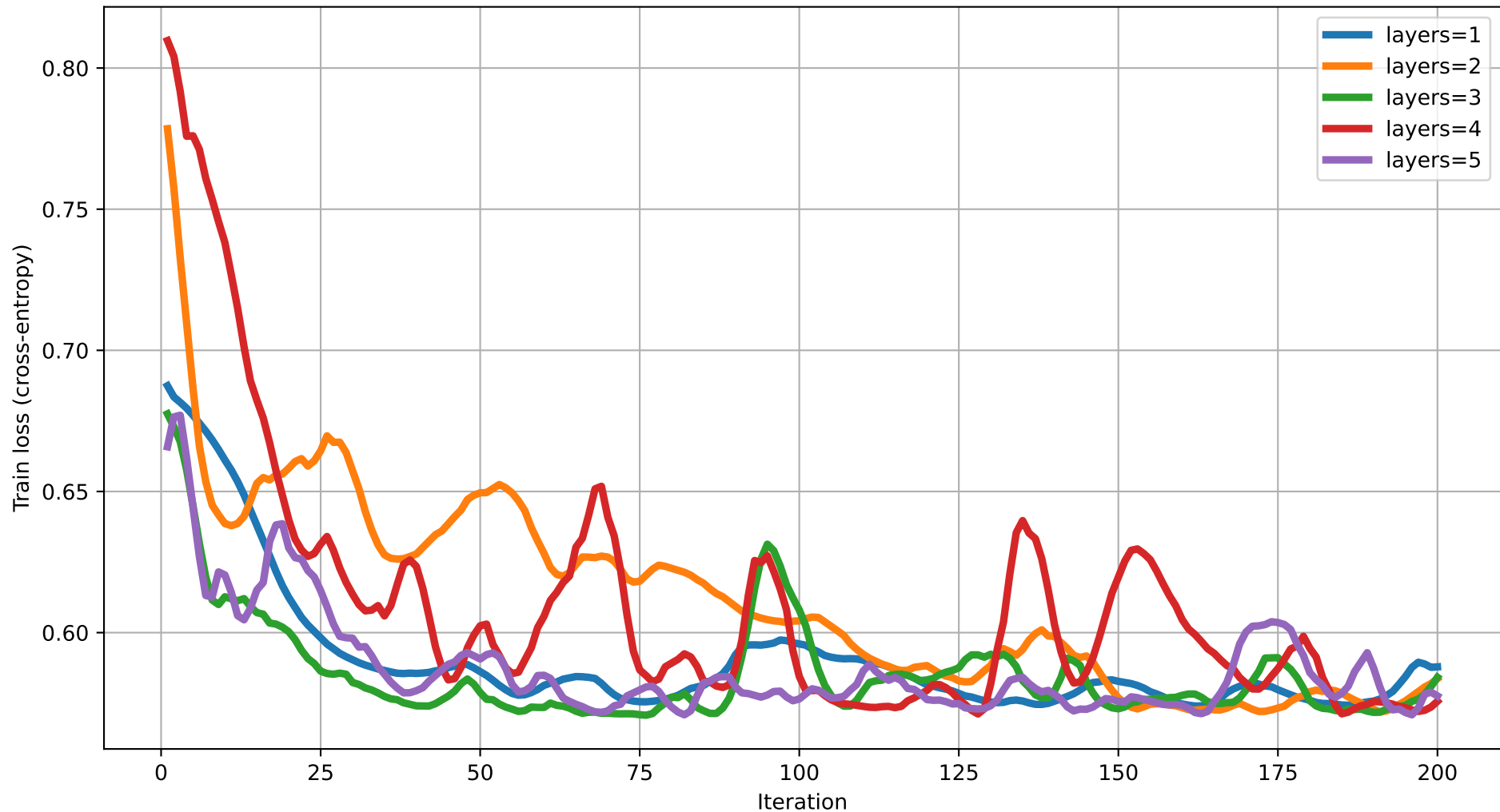
Train loss vs Iteration (dim=2) rot=Rot, ent=full, gate=IsingXX
