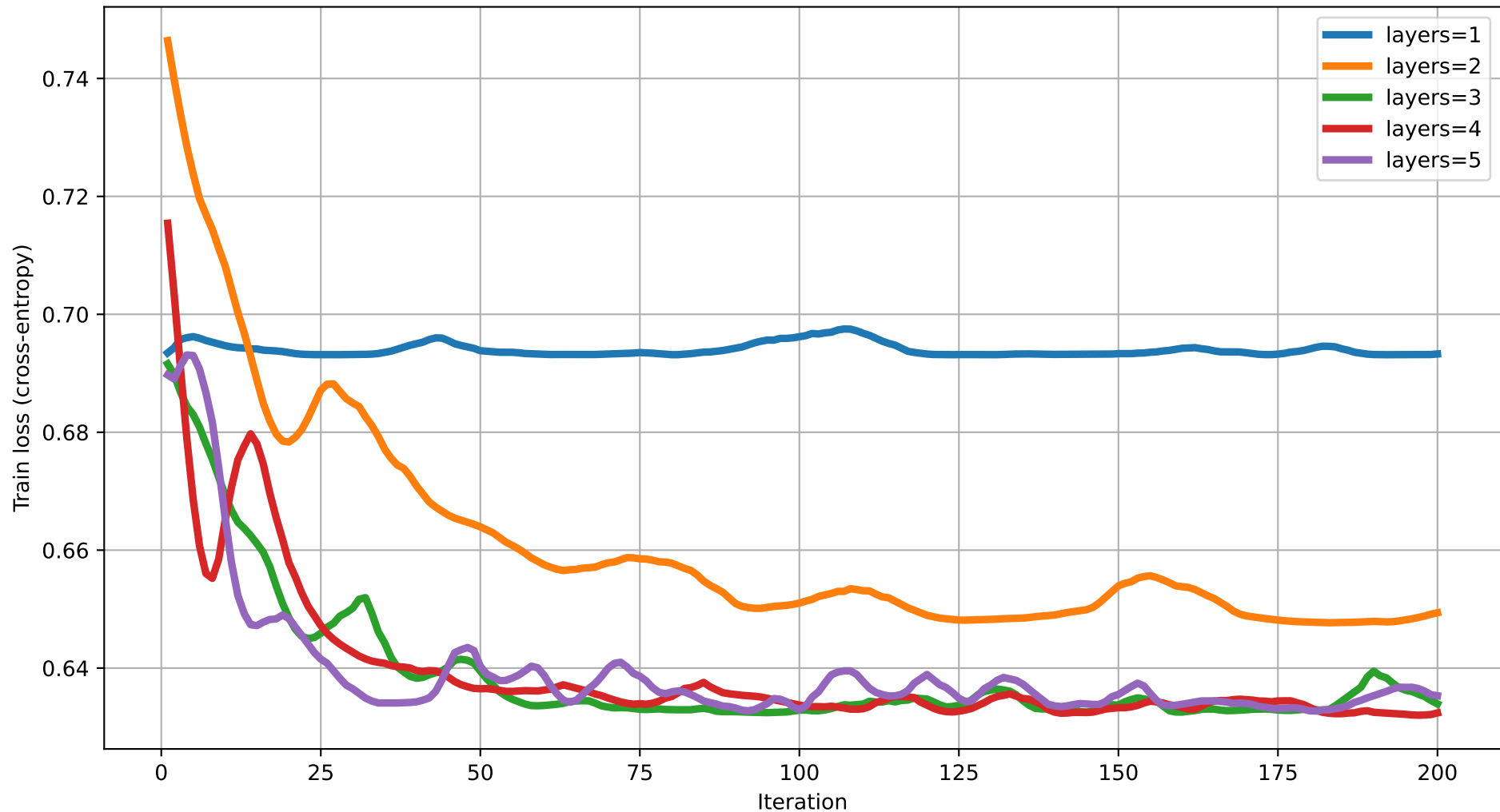
Train loss vs Iteration (degree=3) rot=RY, ent=full, gate=IsingXX
