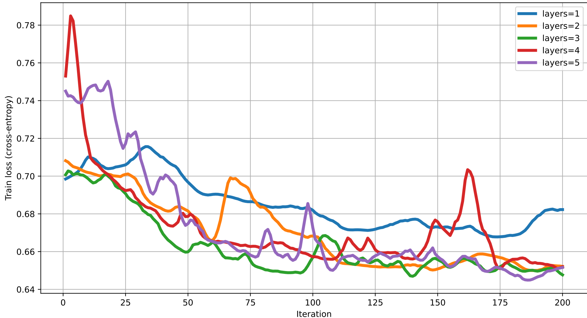
Train loss vs Iteration (dim=6) rot=Rot, ent=ring, gate=CNOT
