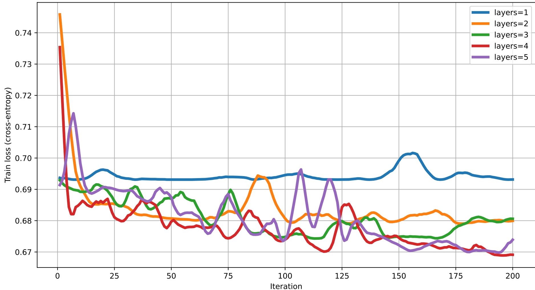
Train loss vs Iteration (degree=5) rot=RY, ent=full, gate=IsingXX
