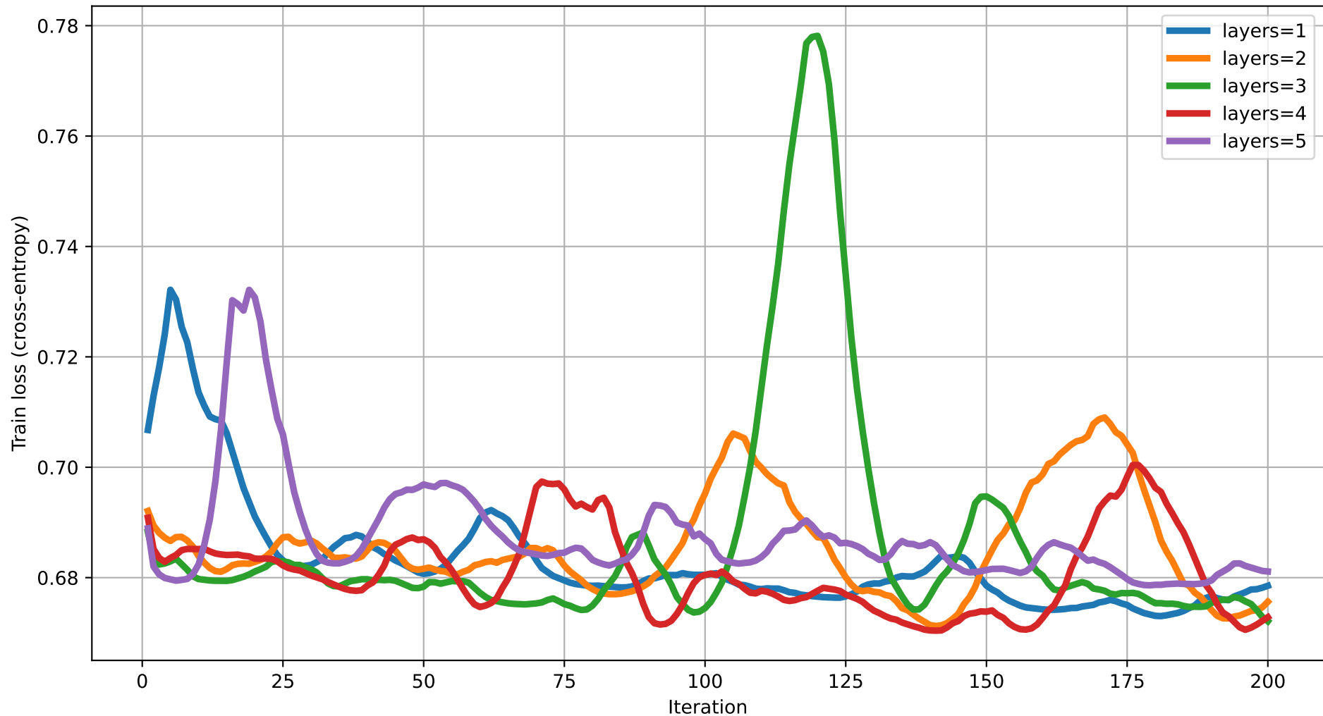
Train loss vs Iteration (dim=13) rot=RY, ent=ring, gate=CZ
