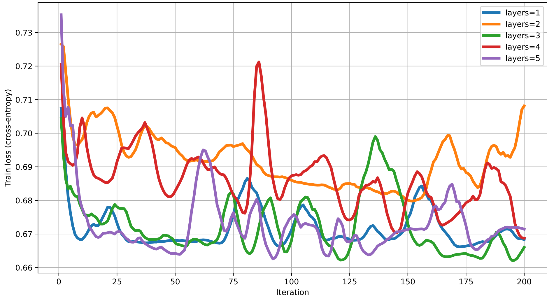
Train loss vs Iteration (dim=19) rot=RY, ent=ring, gate=IsingXX
