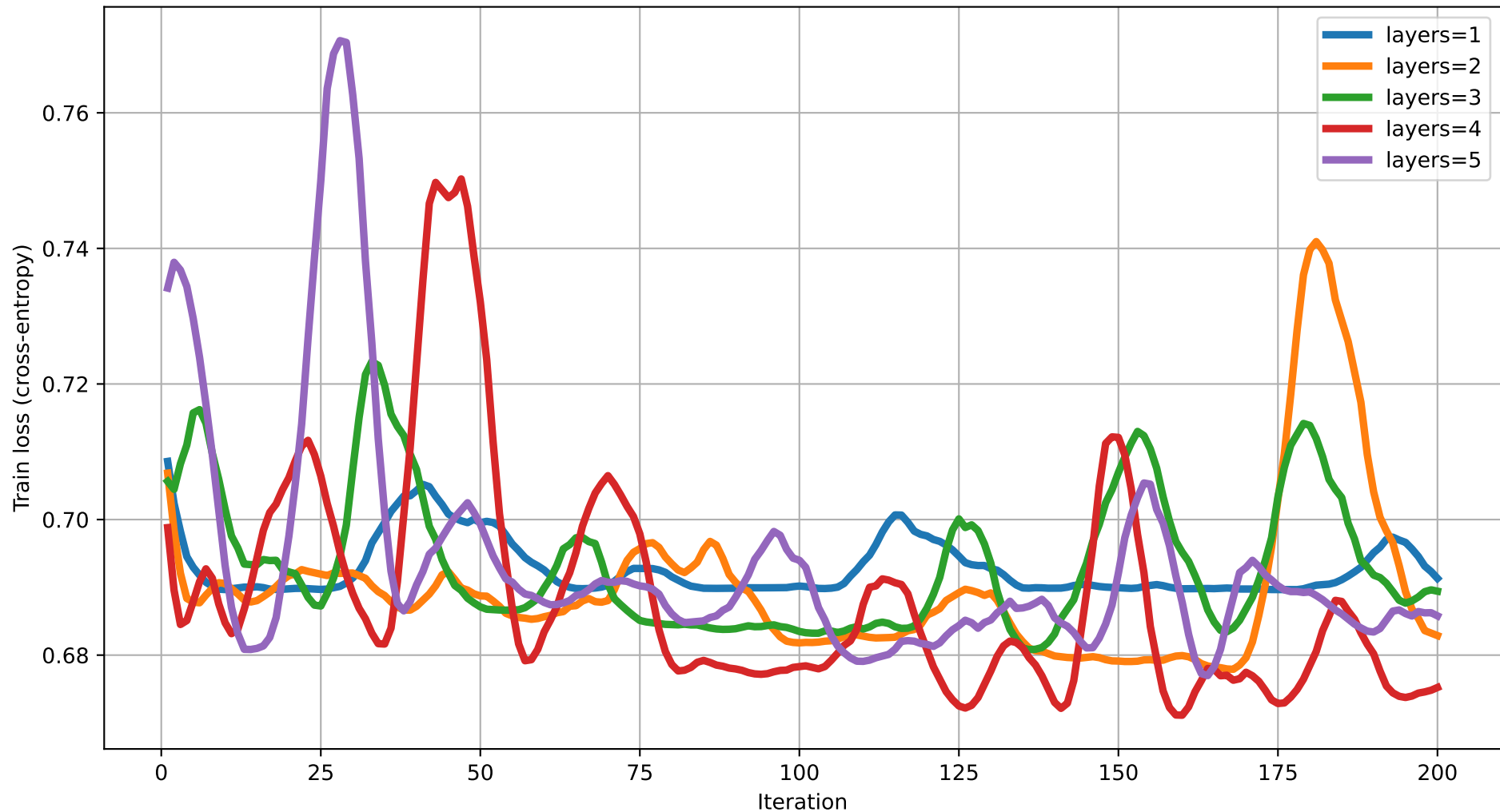
Train loss vs Iteration (dim=20) rot=RY, ent=full, gate=CNOT
