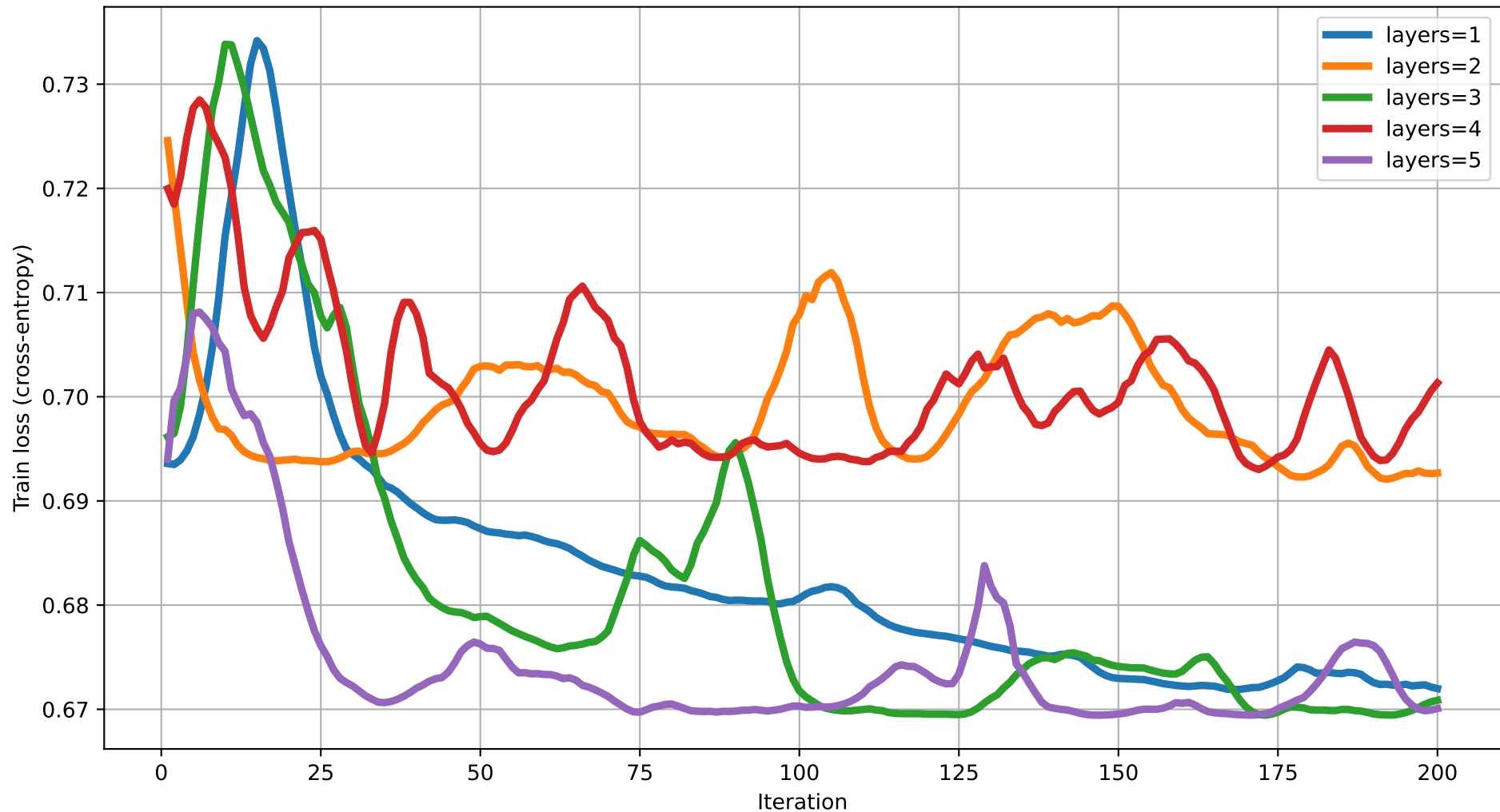
Train loss vs Iteration (dim=11) rot=RX, ent=chain, gate=IsingXX
