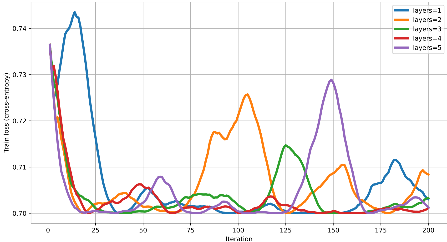
Train loss vs Iteration (dim=19) rot=RZ, ent=chain, gate=CNOT
