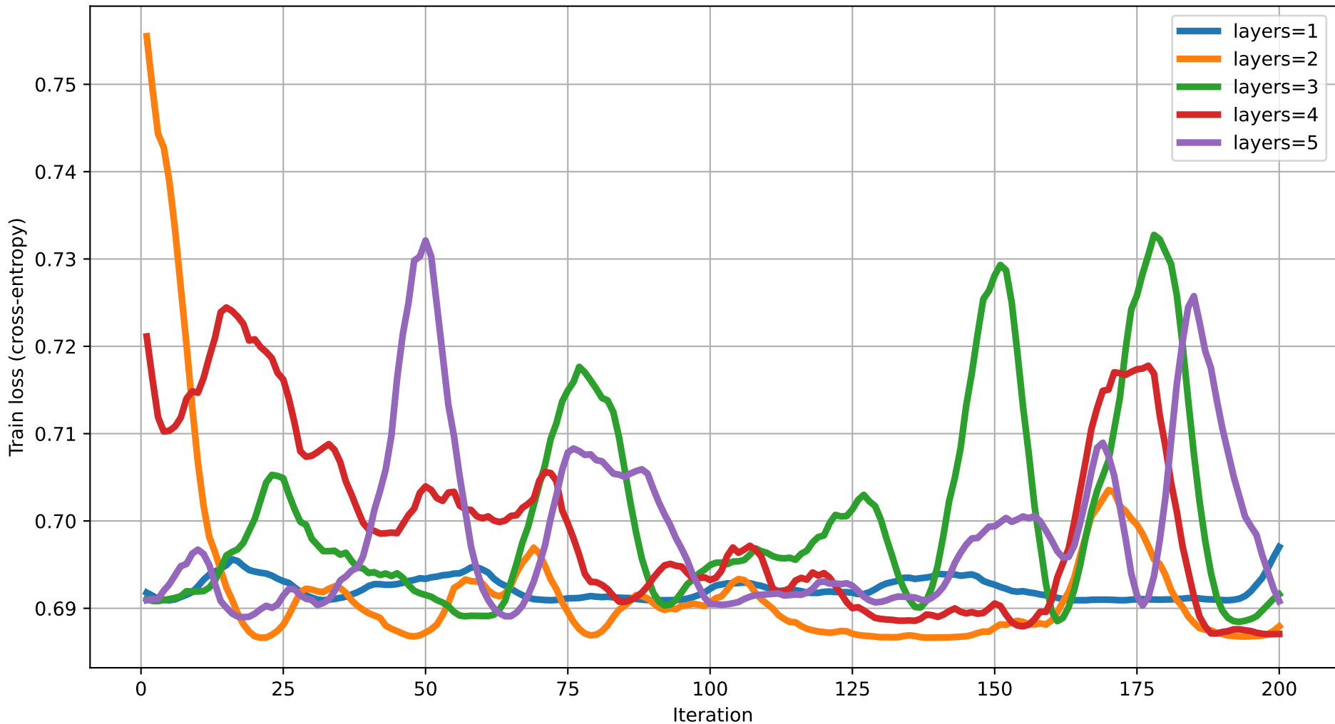
Train loss vs Iteration (dim=10) rot=RY, ent=pairwise, gate=IsingXX
