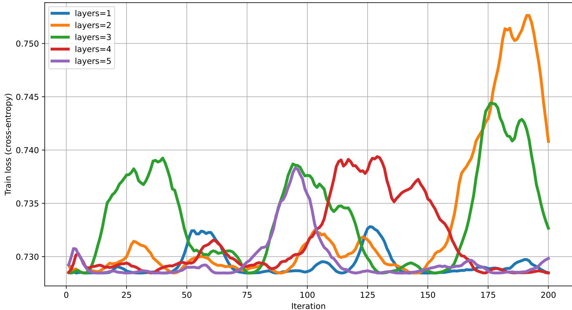
Train loss vs Iteration (dim=7) rot=RZ, ent=pairwise, gate=CZ
