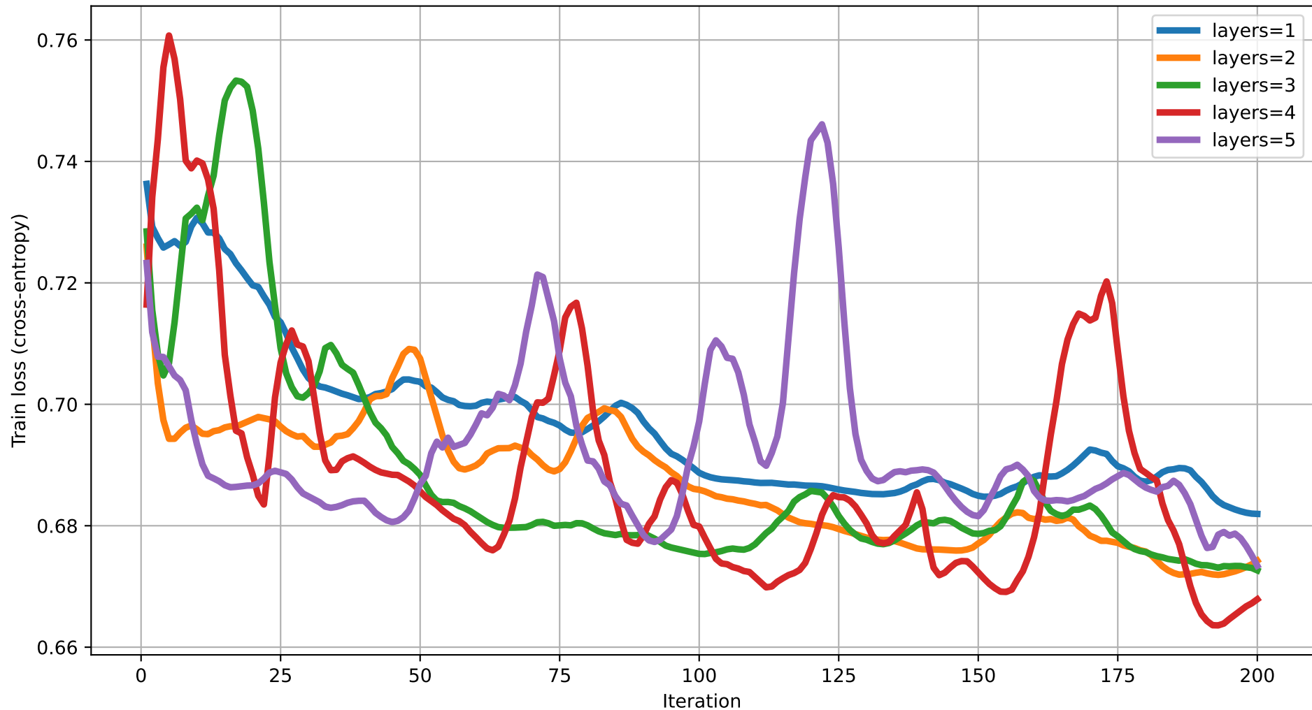
Train loss vs Iteration (dim=18) rot=RYZ, ent=full, gate=IsingXX
