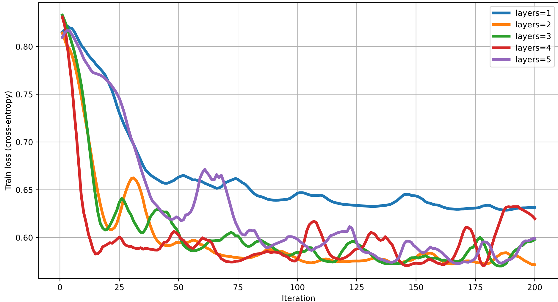
Train loss vs Iteration (dim=2) rot=RYZ, ent=pairwise, gate=CNOT
