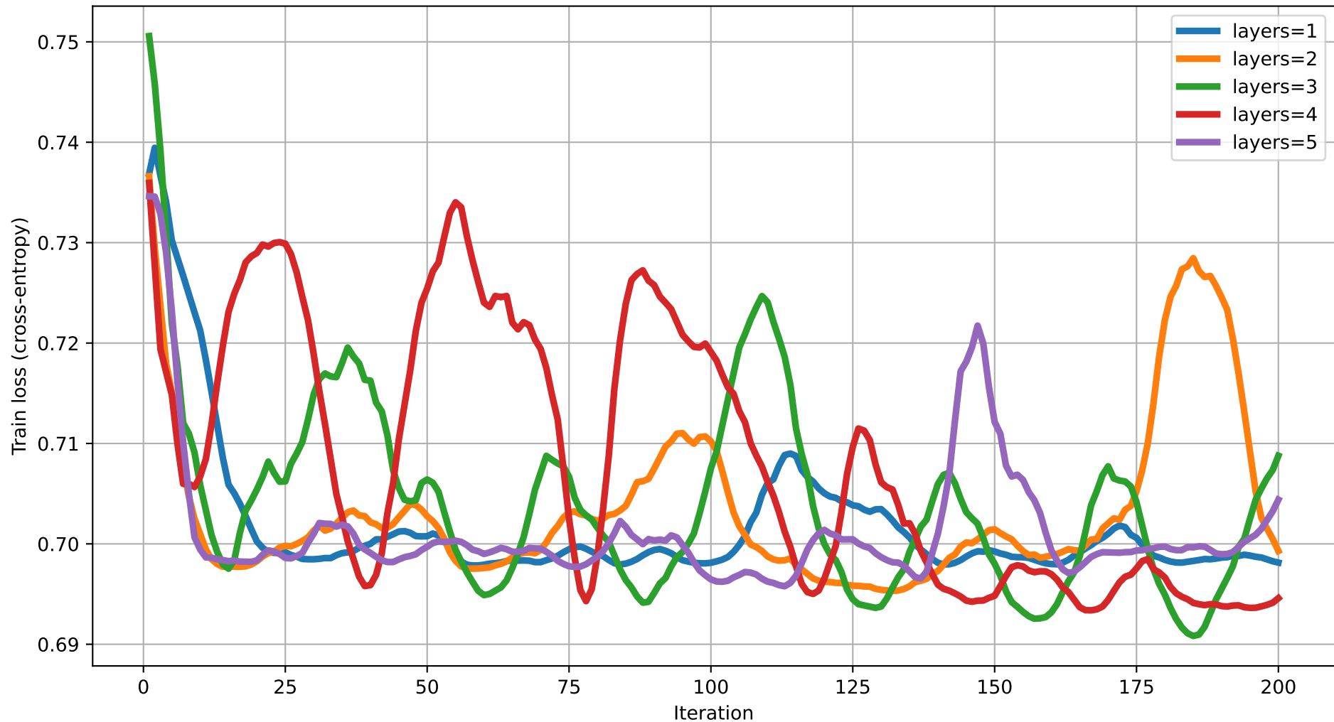
Train loss vs Iteration (dim=18) rot=RX, ent=pairwise, gate=CZ
