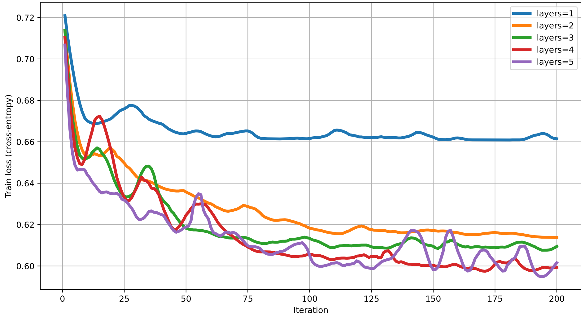
Train loss vs Iteration (degree=3) rot=RYZ, ent=chain, gate=CZ
