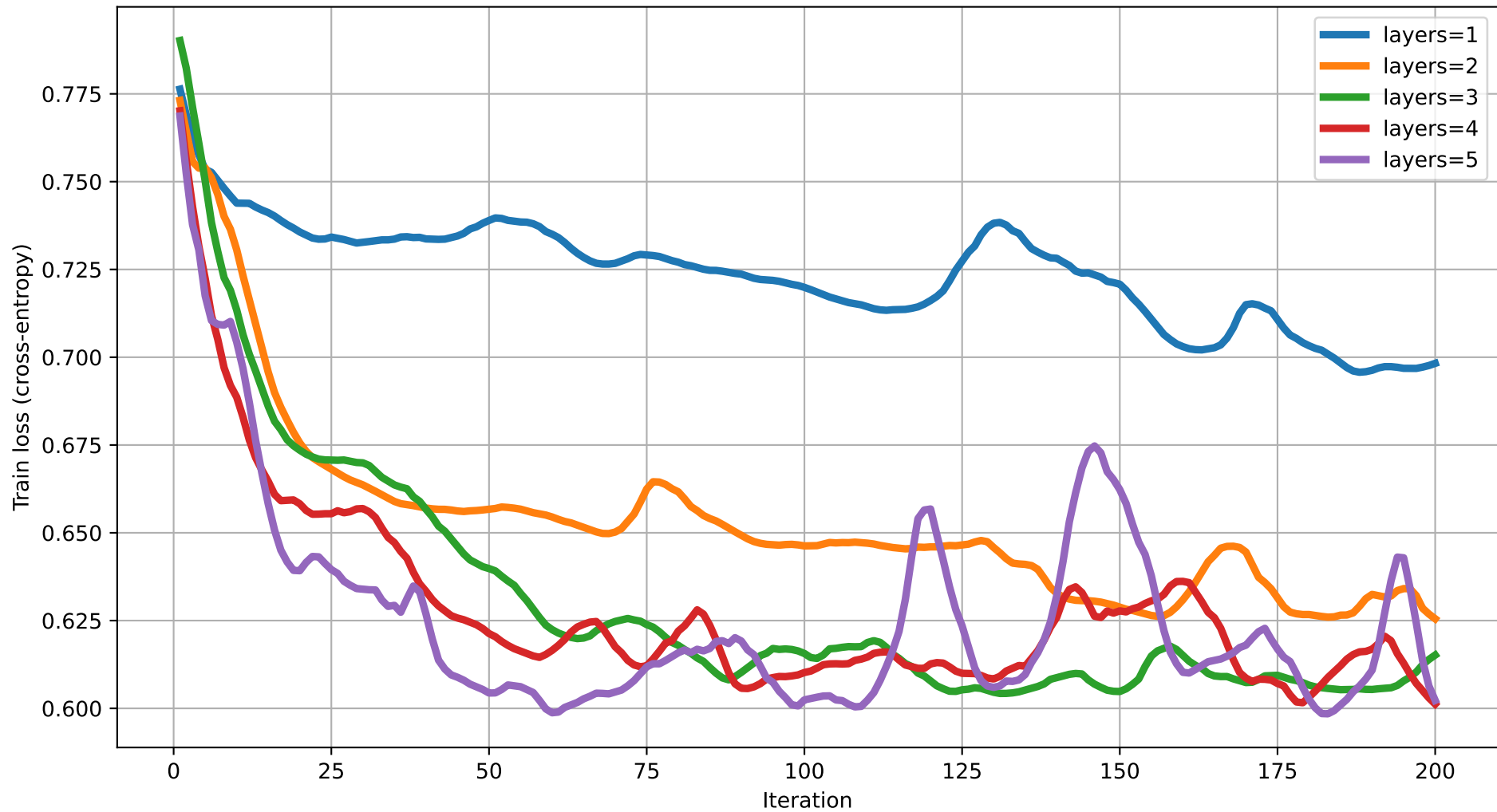
Train loss vs Iteration (dim=9) rot=Rot, ent=full, gate=CZ
