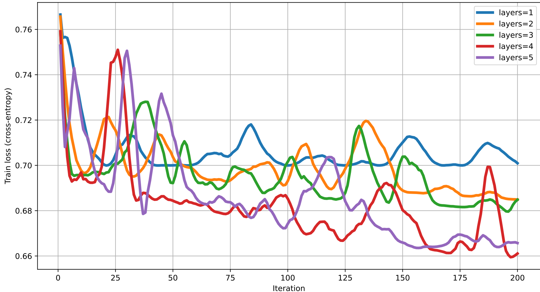
Train loss vs Iteration (dim=17) rot=RYZ, ent=chain, gate=CNOT
