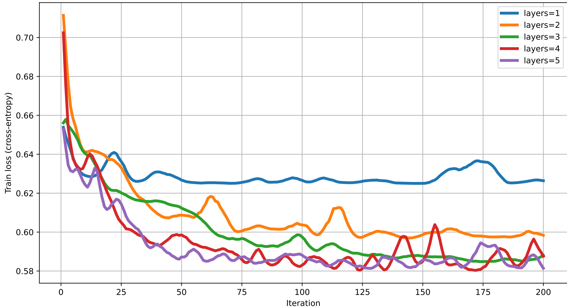
Train loss vs Iteration (degree=3) rot=RYZ, ent=ring, gate=IsingXX
