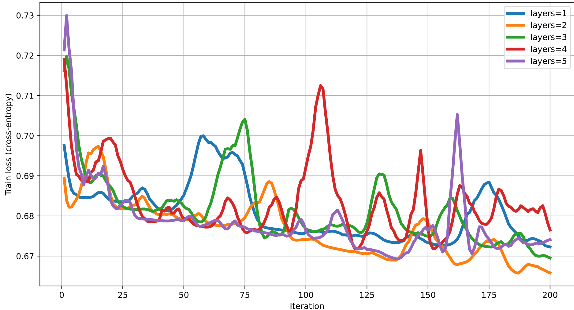
Train loss vs Iteration (dim=13) rot=Rot, ent=pairwise, gate=CNOT
