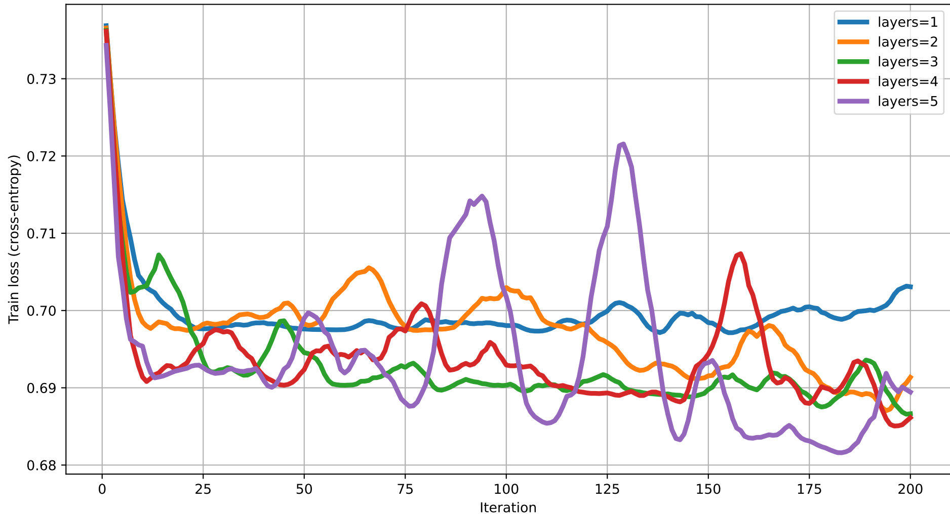
Train loss vs Iteration (dim=18) rot=RX, ent=full, gate=CZ
