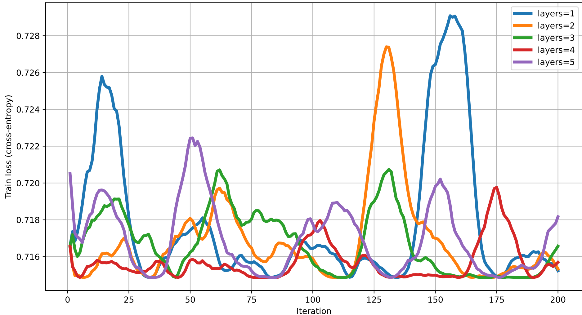
Train loss vs Iteration (dim=3) rot=RZ, ent=chain, gate=CNOT
