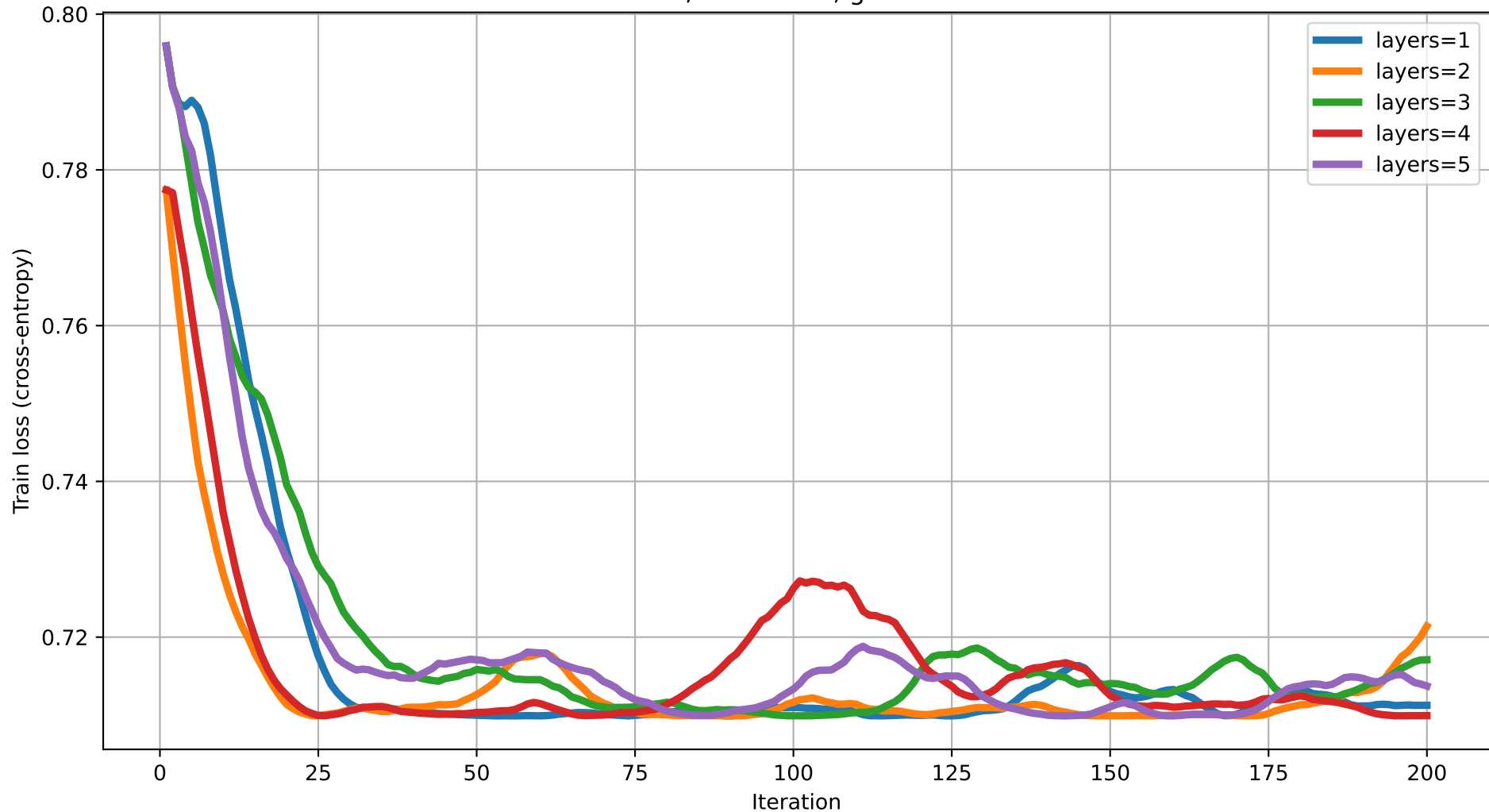
Train loss vs Iteration (dim=4) rot=RZ, ent=chain, gate=CNOT
