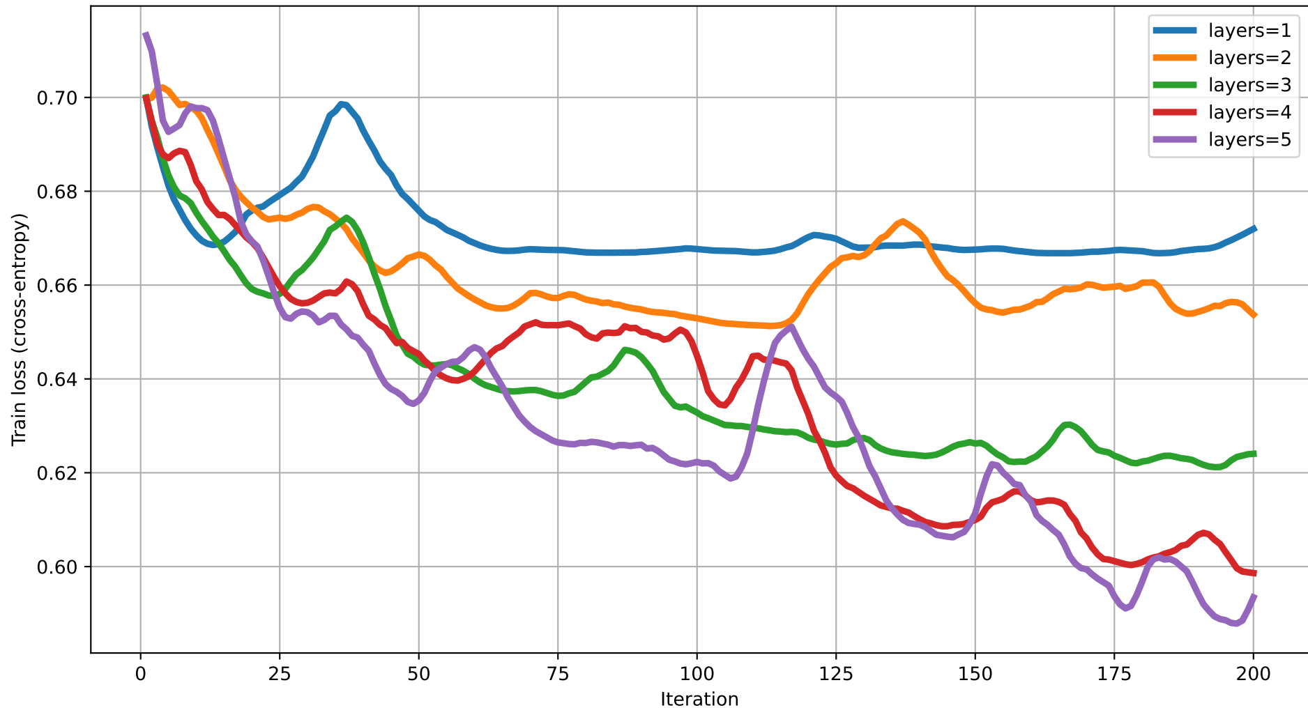
Train loss vs Iteration (dim=10) rot=RX, ent=full, gate=CZ
