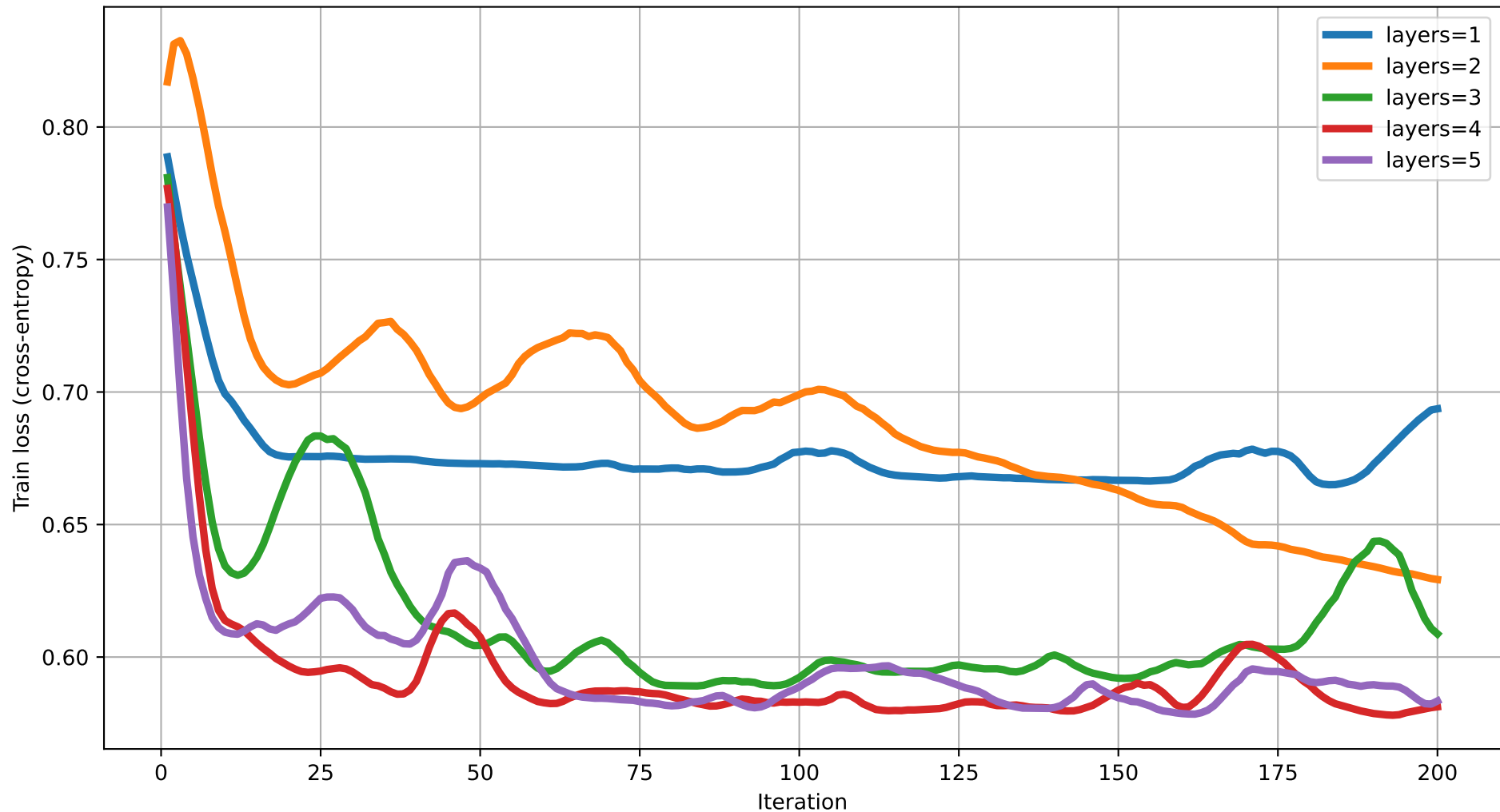
Train loss vs Iteration (dim=4) rot=RY, ent=chain, gate=CNOT
