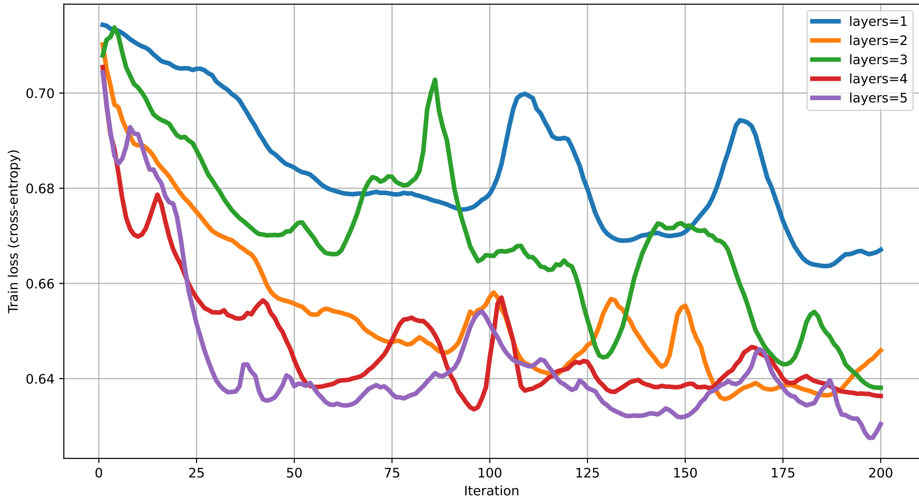
Train loss vs Iteration (dim=7) rot=Rot, ent=chain, gate=CZ
