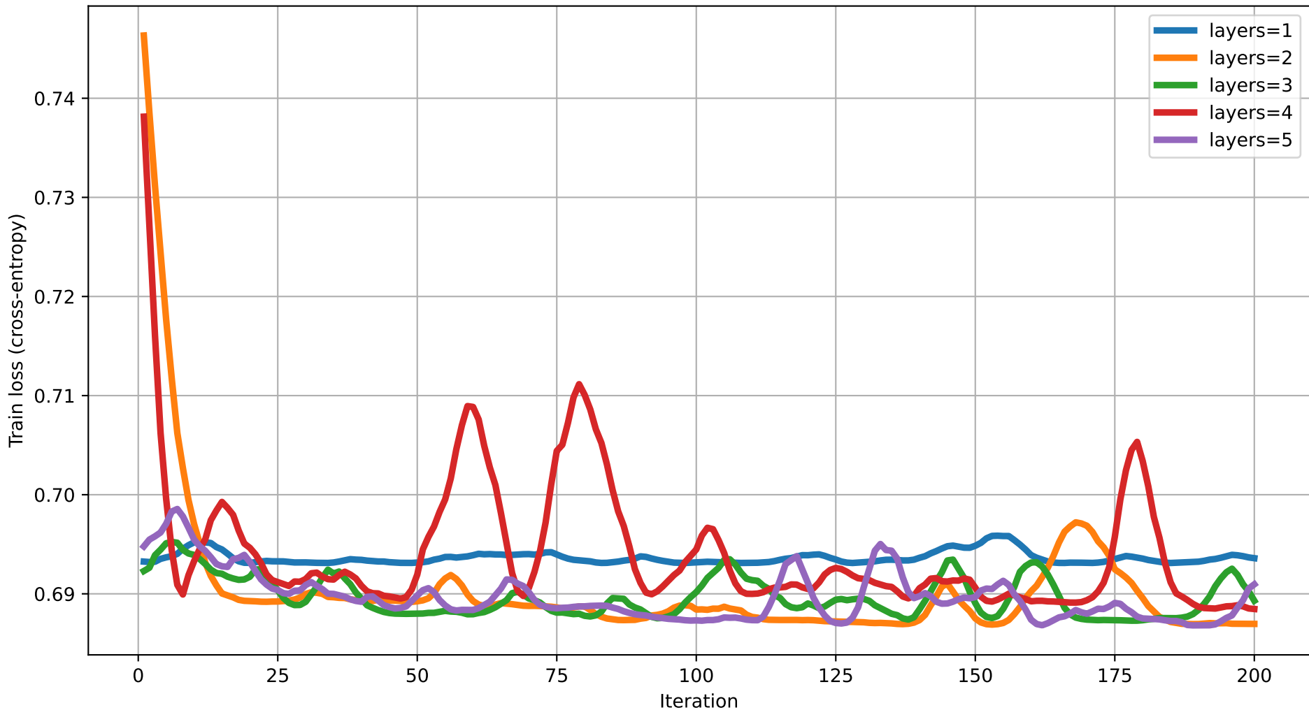
Train loss vs Iteration (degree=5) rot=RY, ent=pairwise, gate=IsingXX
