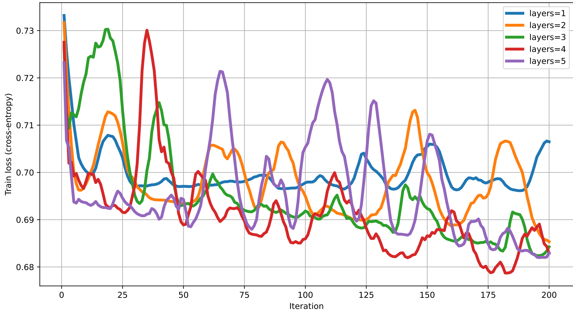
Train loss vs Iteration (dim=18) rot=RYZ, ent=pairwise, gate=CNOT
