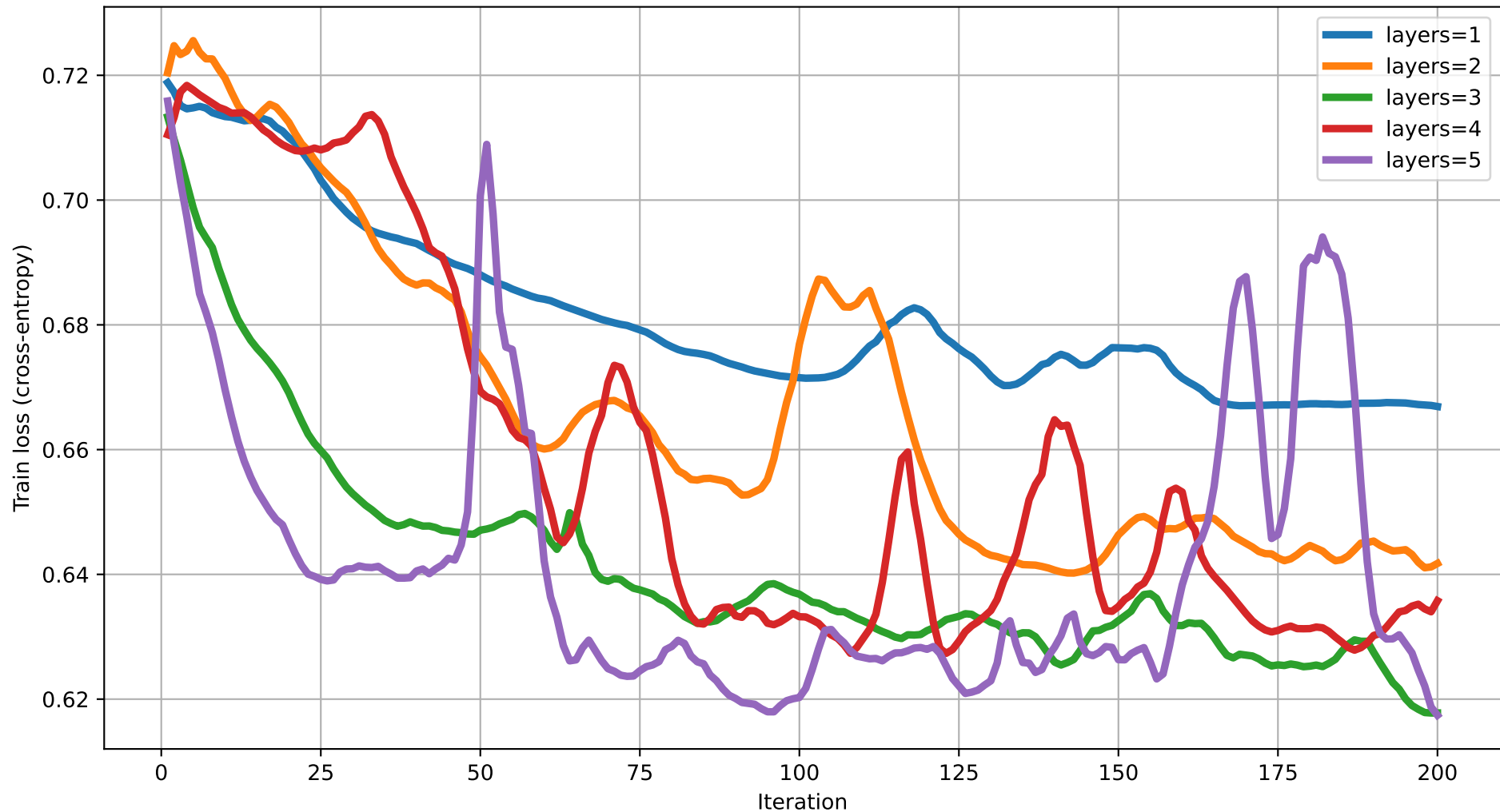
Train loss vs Iteration (dim=7) rot=Rot, ent=full, gate=CNOT
