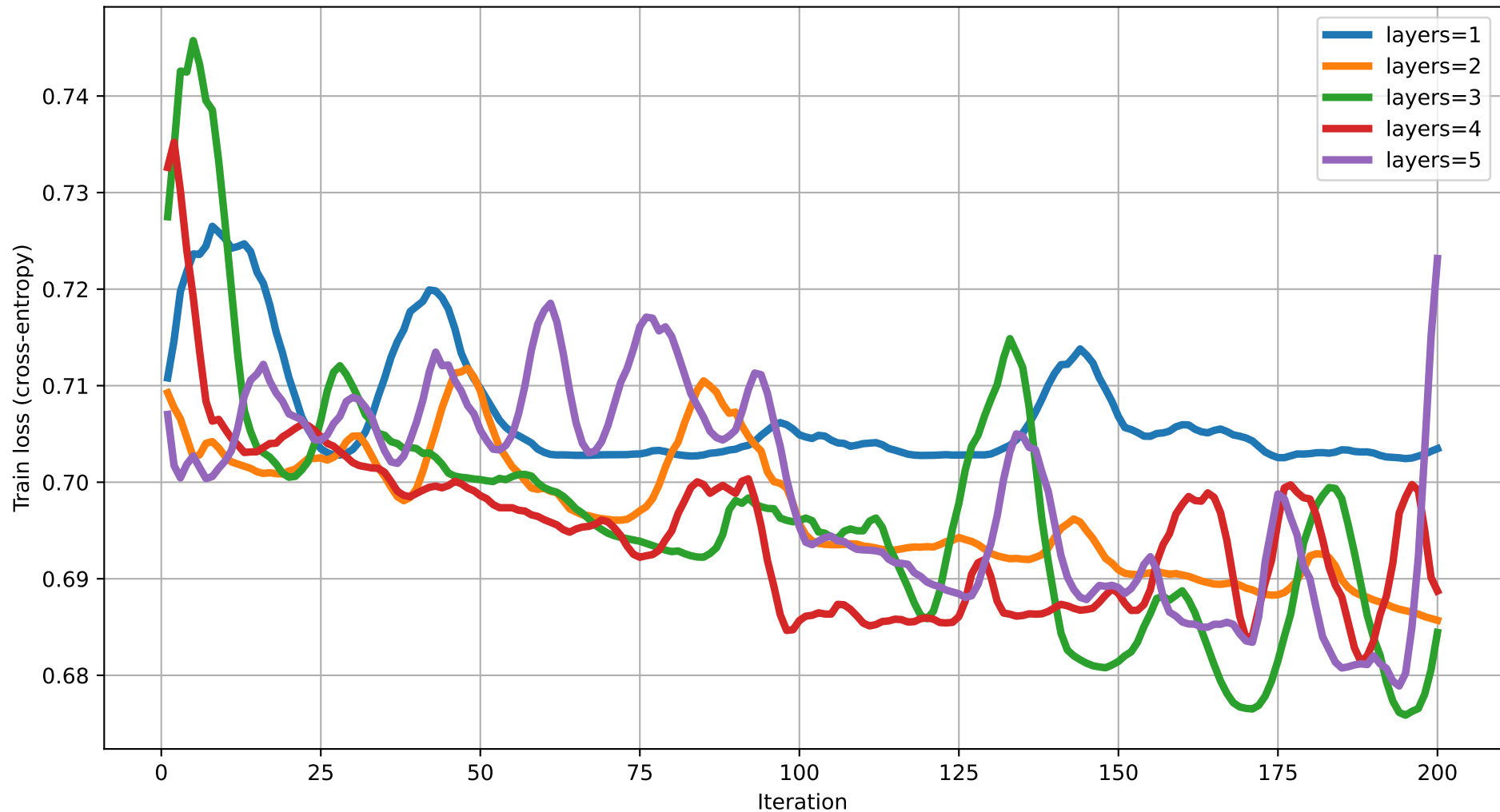
Train loss vs Iteration (dim=11) rot=RY, ent=pairwise, gate=CZ
