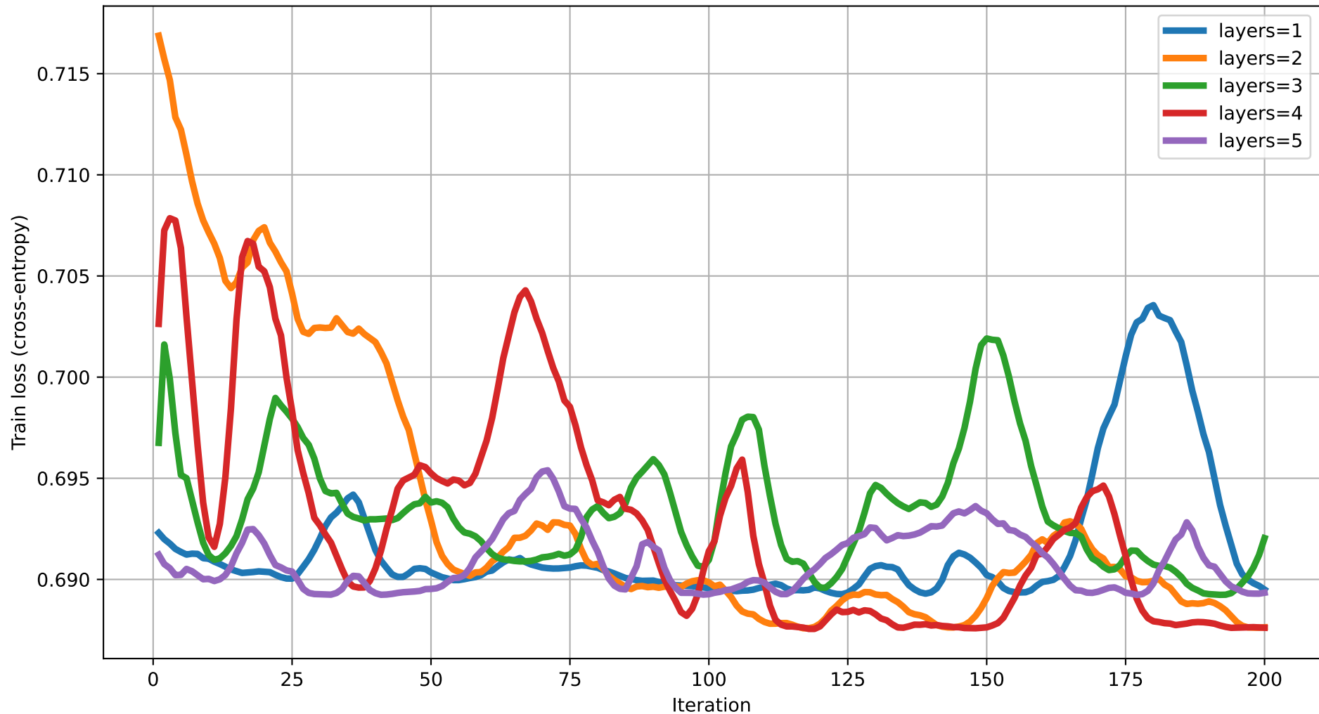
Train loss vs Iteration (dim=13) rot=RX, ent=pairwise, gate=IsingXX
