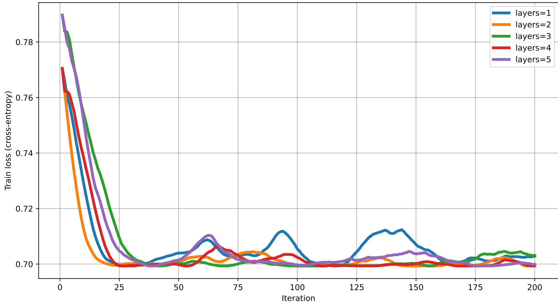
Train loss vs Iteration (dim=17) rot=RZ, ent=full, gate=CNOT
