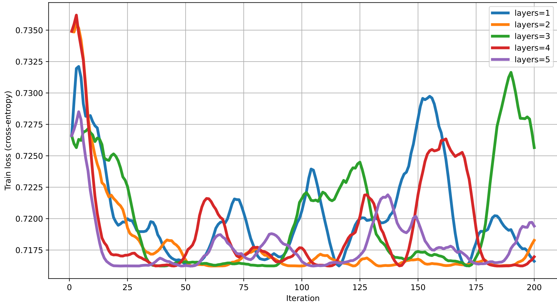
Train loss vs Iteration (dim=6) rot=RZ, ent=ring, gate=CZ
