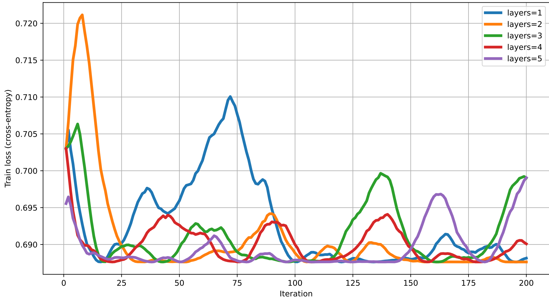
Train loss vs Iteration (dim=13) rot=RZ, ent=full, gate=CNOT
