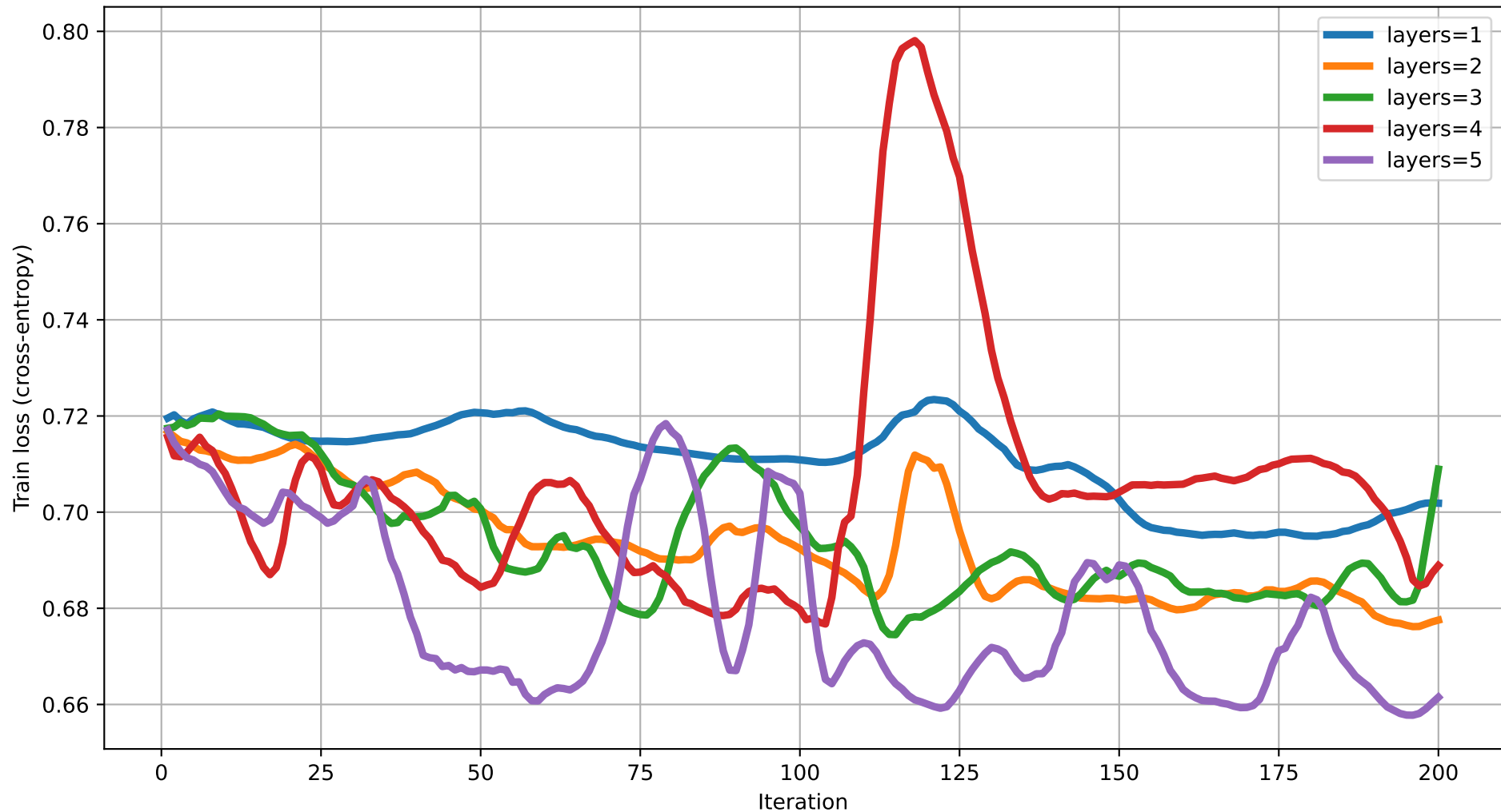
Train loss vs Iteration (dim=3) rot=Rot, ent=pairwise, gate=CNOT
