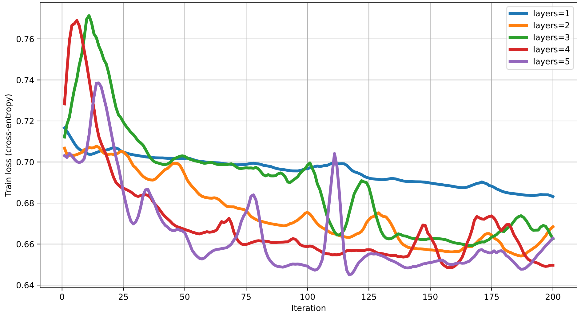
Train loss vs Iteration (dim=6) rot=RY, ent=full, gate=CNOT
