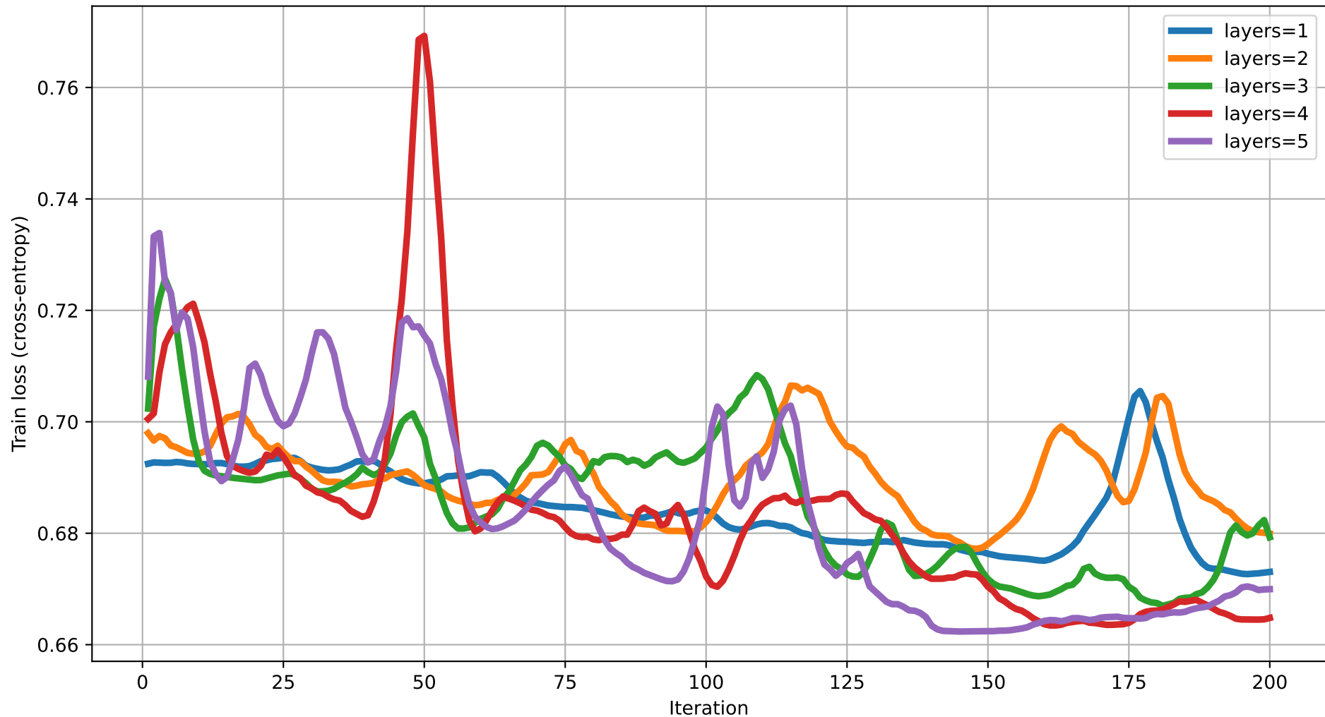
Train loss vs Iteration (dim=14) rot=RYZ, ent=pairwise, gate=IsingXX
