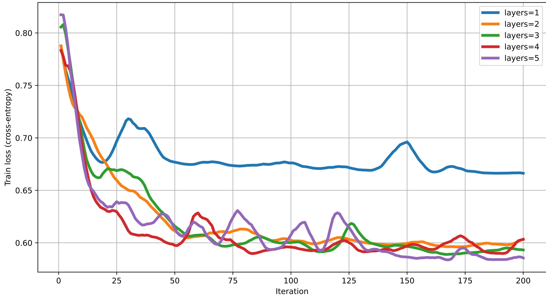
Train loss vs Iteration (dim=4) rot=RYZ, ent=ring, gate=CZ
