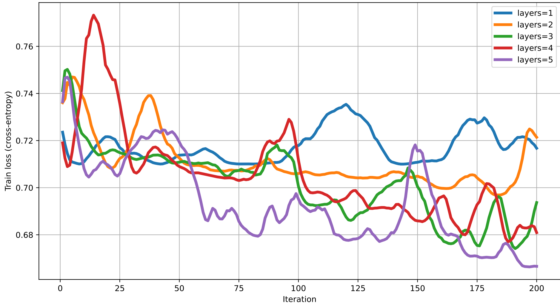
Train loss vs Iteration (dim=10) rot=RYZ, ent=chain, gate=CZ
