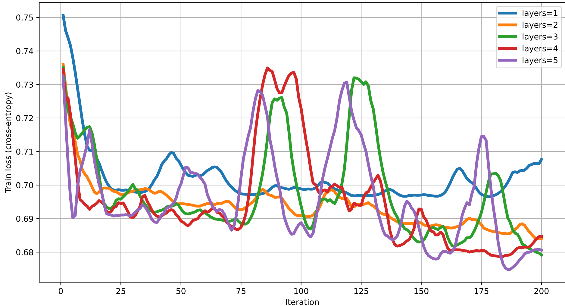
Train loss vs Iteration (dim=19) rot=RX, ent=pairwise, gate=CNOT
