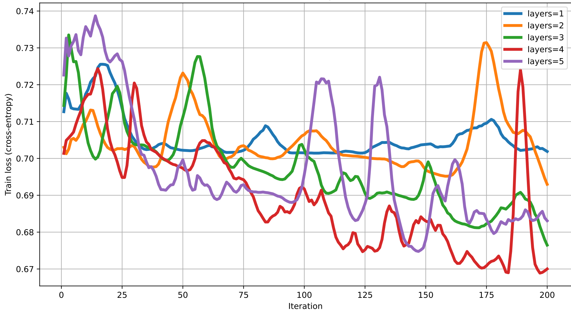
Train loss vs Iteration (dim=12) rot=Rot, ent=chain, gate=CNOT
