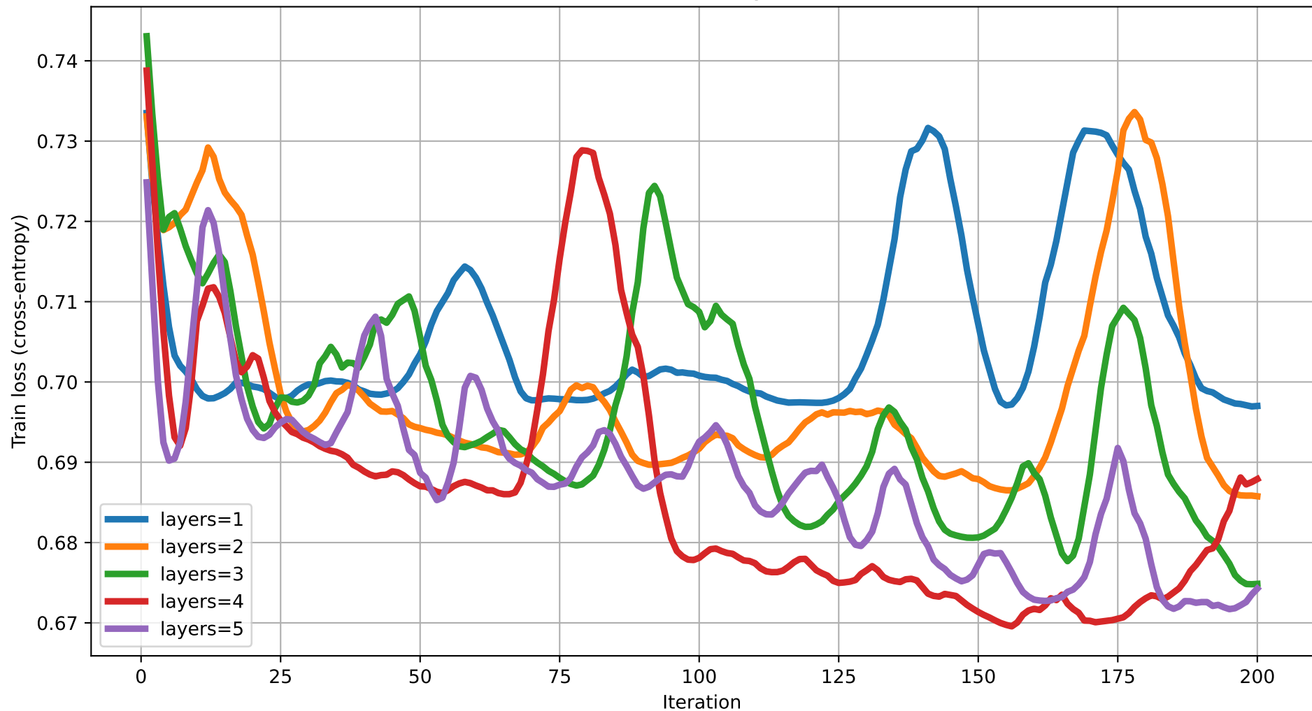
Train loss vs Iteration (dim=19) rot=RY, ent=full, gate=CZ
