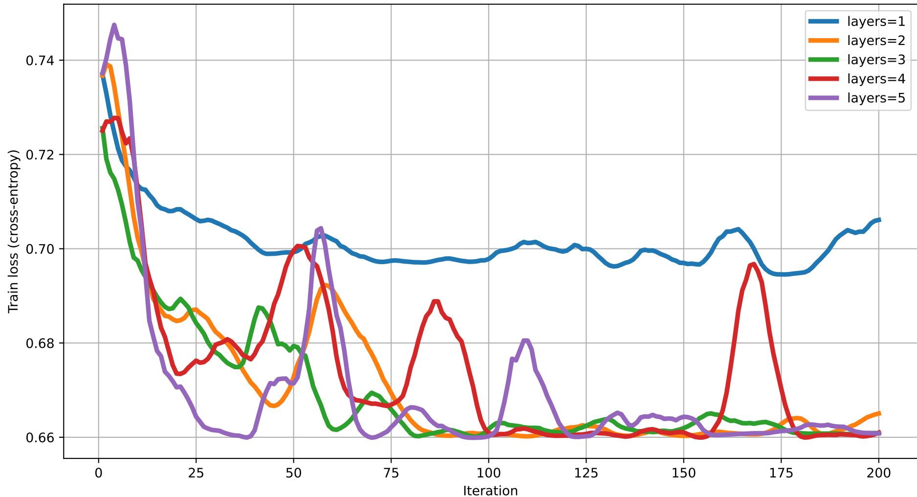
Train loss vs Iteration (dim=5) rot=RX, ent=pairwise, gate=CNOT
