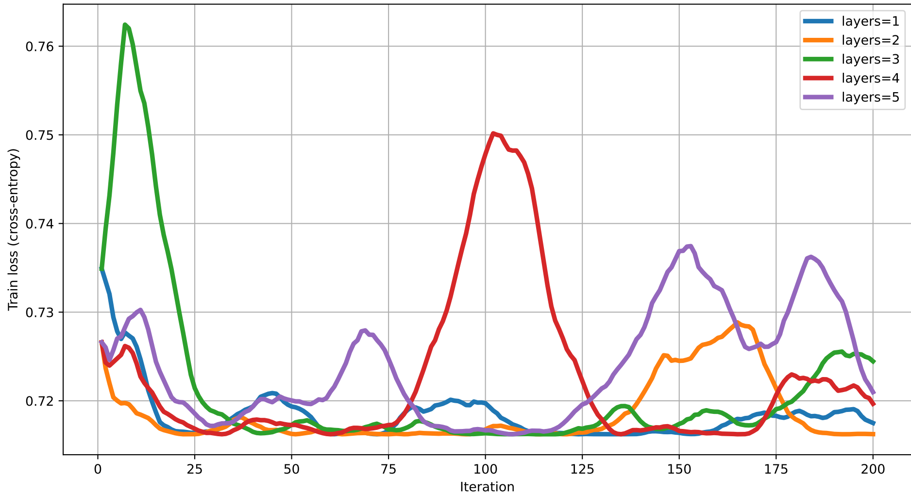
Train loss vs Iteration (dim=6) rot=RZ, ent=full, gate=CZ
