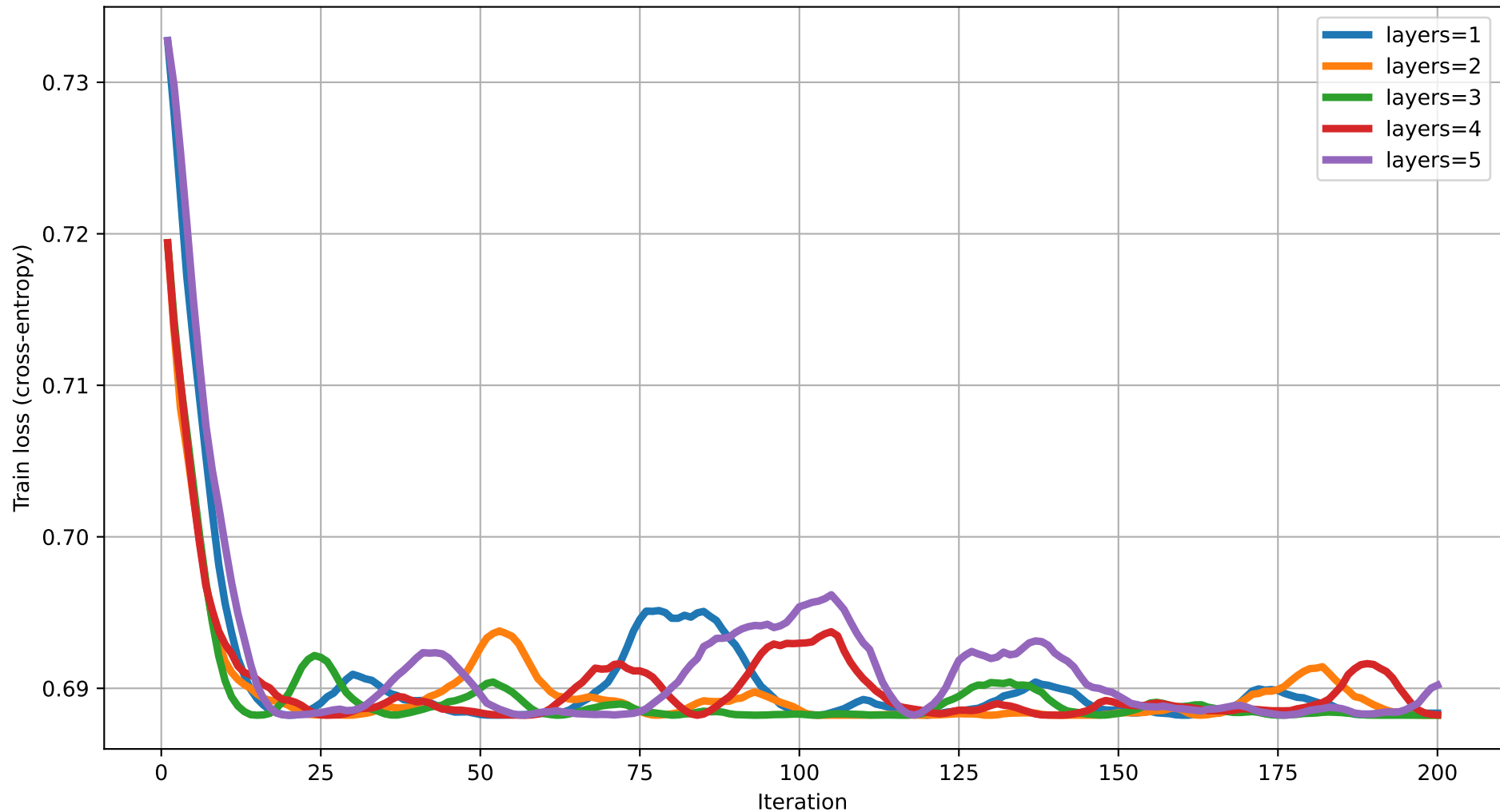
Train loss vs Iteration (degree=4) rot=RZ, ent=full, gate=CZ
