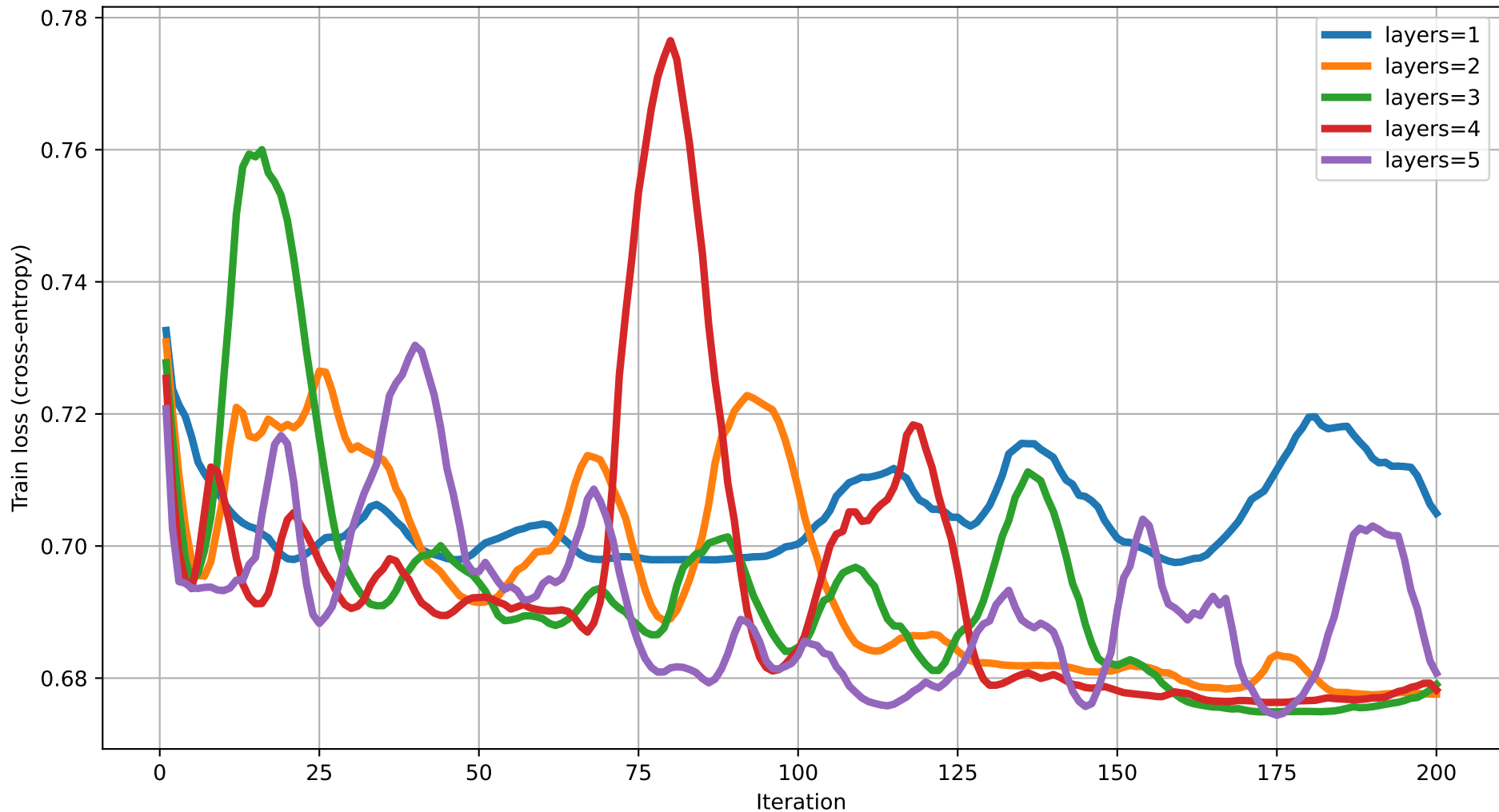
Train loss vs Iteration (dim=19) rot=RY, ent=pairwise, gate=CNOT
