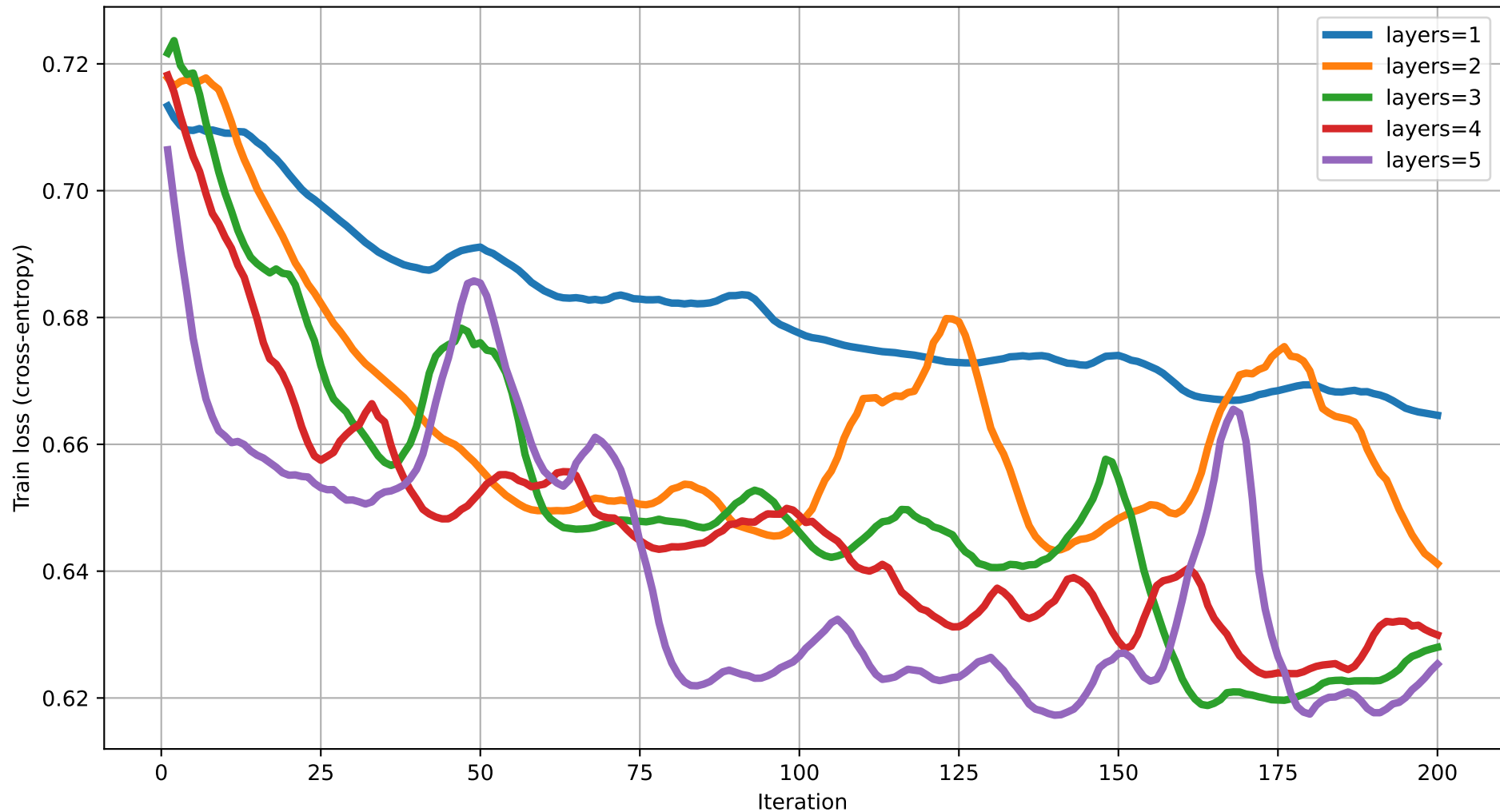
Train loss vs Iteration (dim=7) rot=RY, ent=ring, gate=CZ
