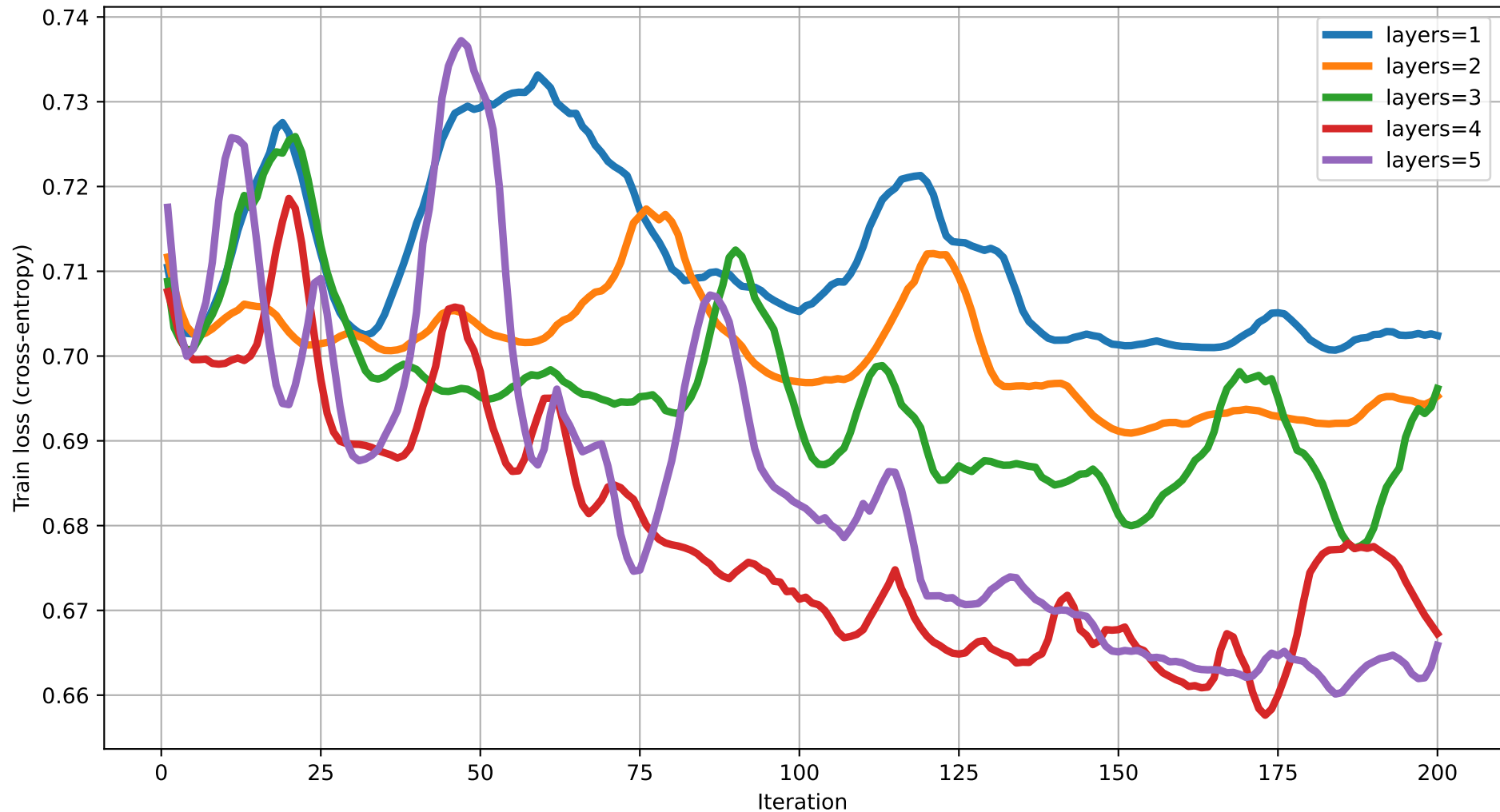
Train loss vs Iteration (dim=11) rot=RYZ, ent=full, gate=CZ
