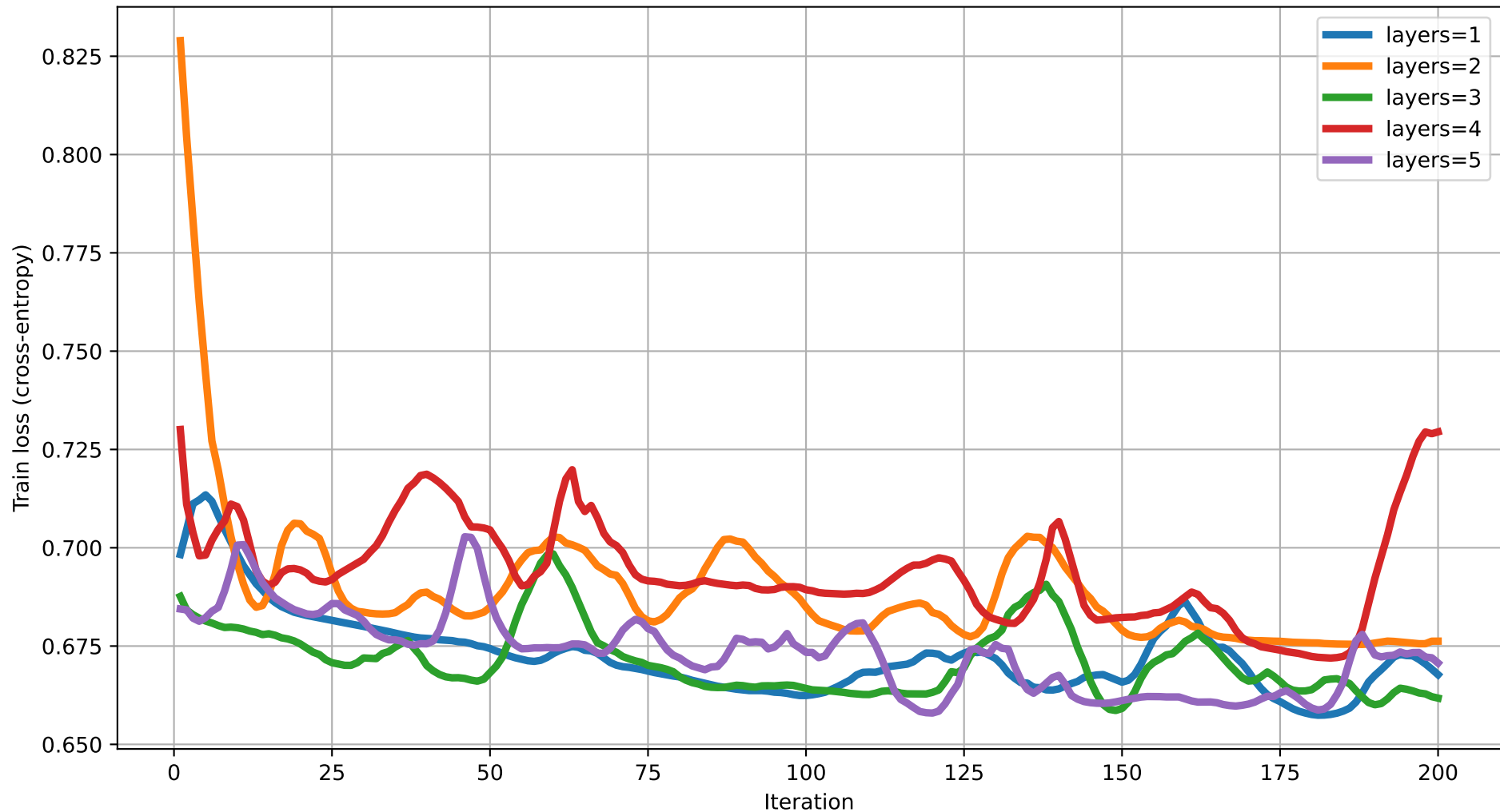
Train loss vs Iteration (dim=16) rot=YRZ, ent=chain, gate=IsingXX
