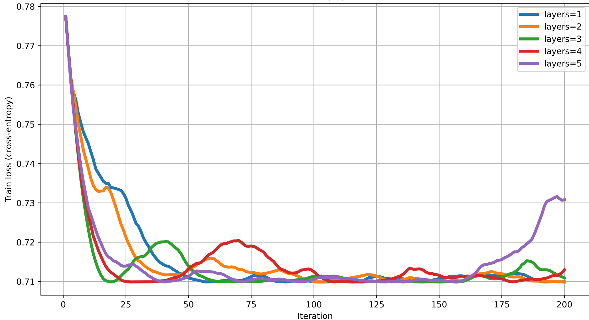
Train loss vs Iteration (dim=4) rot=RZ, ent=ring, gate=CZ
