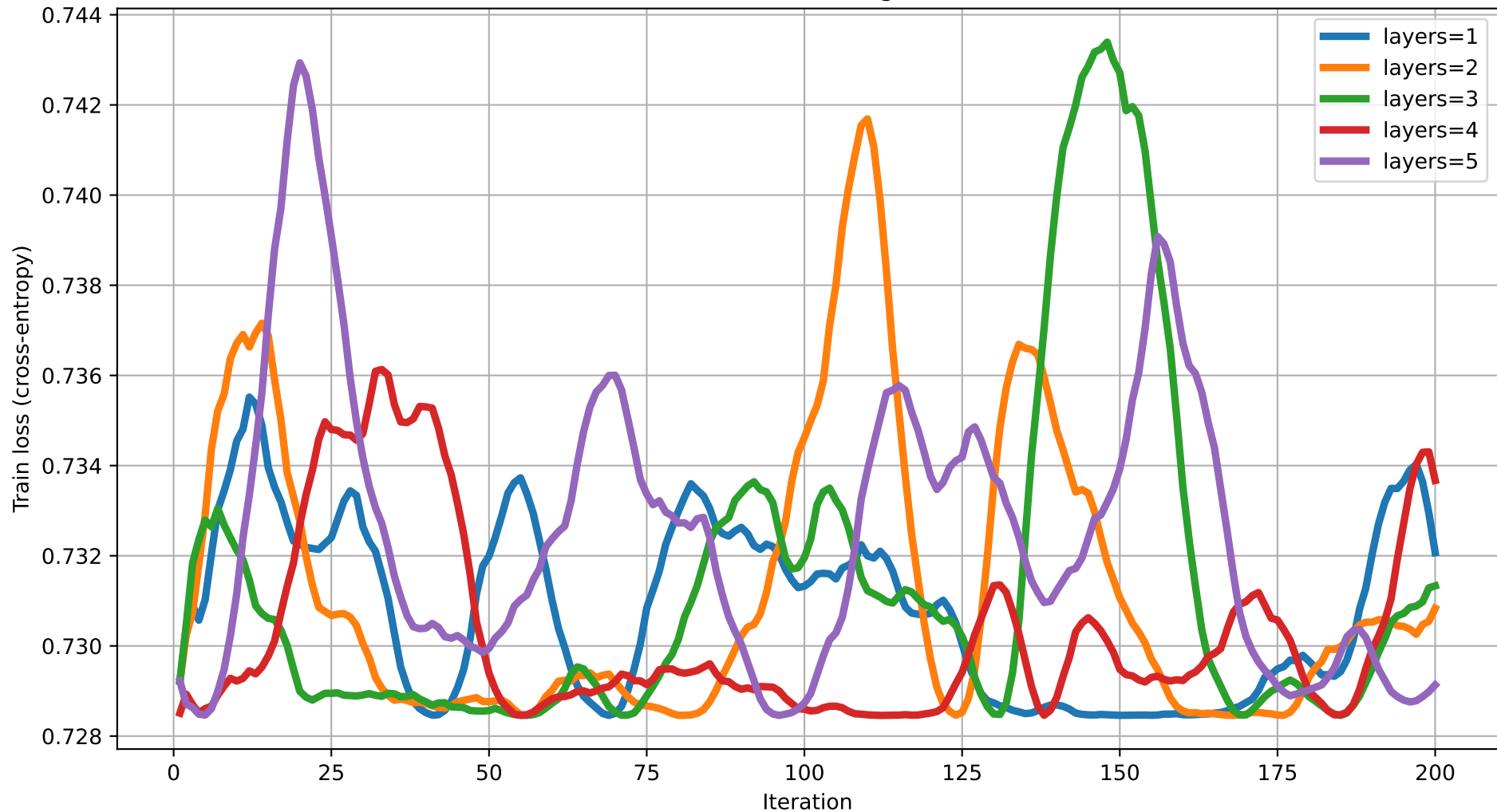
Train loss vs Iteration (dim=7) rot=RZ, ent=chain, gate=CZ
