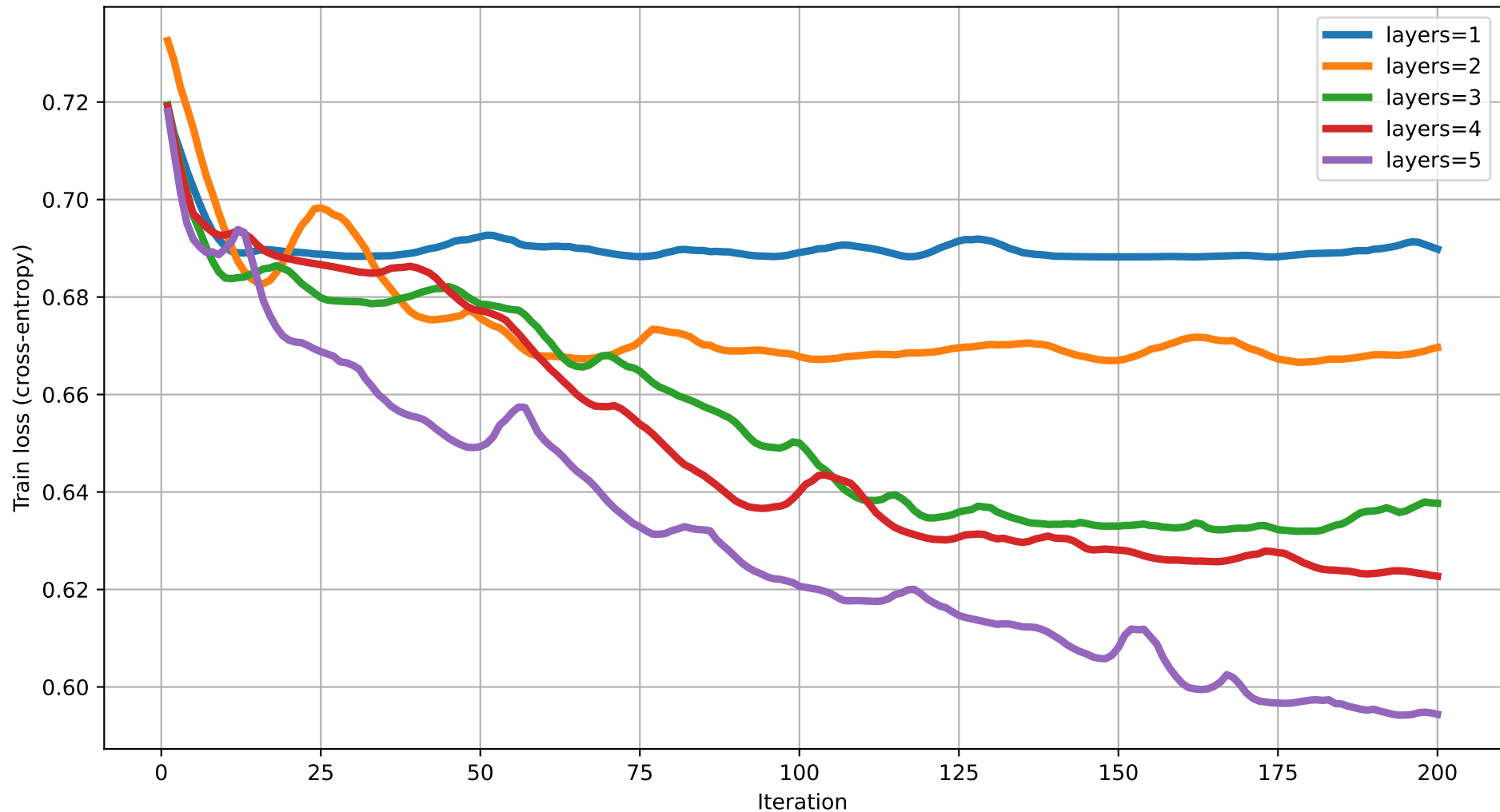
Train loss vs Iteration (degree=4) rot=RX, ent=full, gate=CZ
