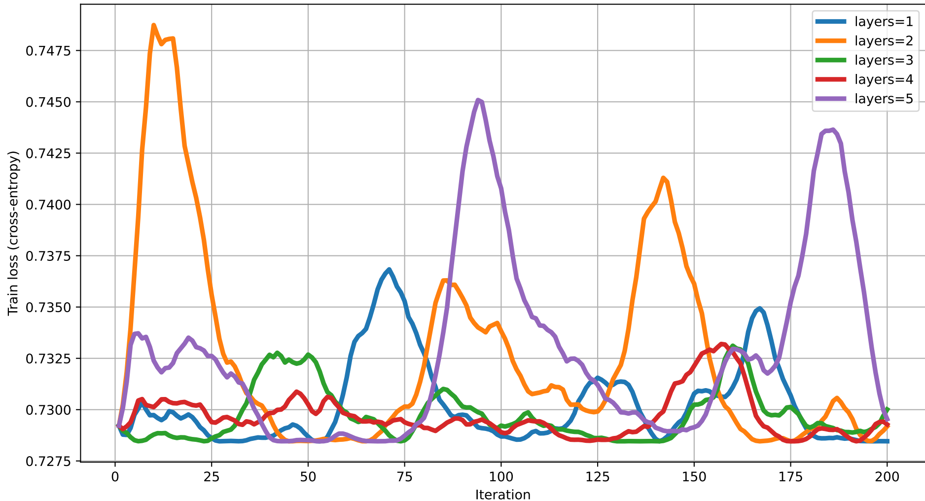
Train loss vs Iteration (dim=7) rot=RZ, ent=full, gate=CZ
