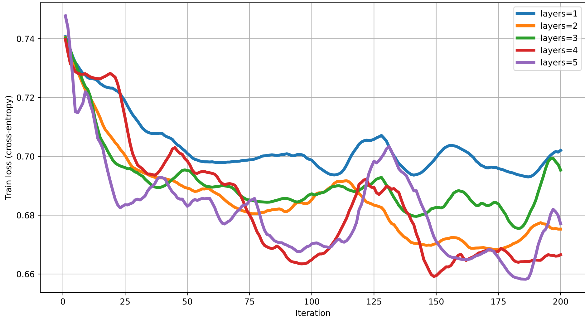
Train loss vs Iteration (dim=3) rot=RX, ent=chain, gate=CZ
