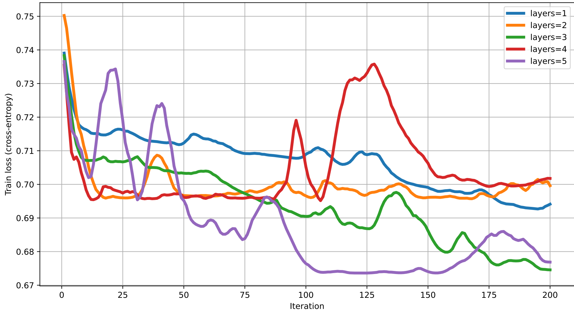
Train loss vs Iteration (dim=19) rot=RX, ent=full, gate=IsingXX
