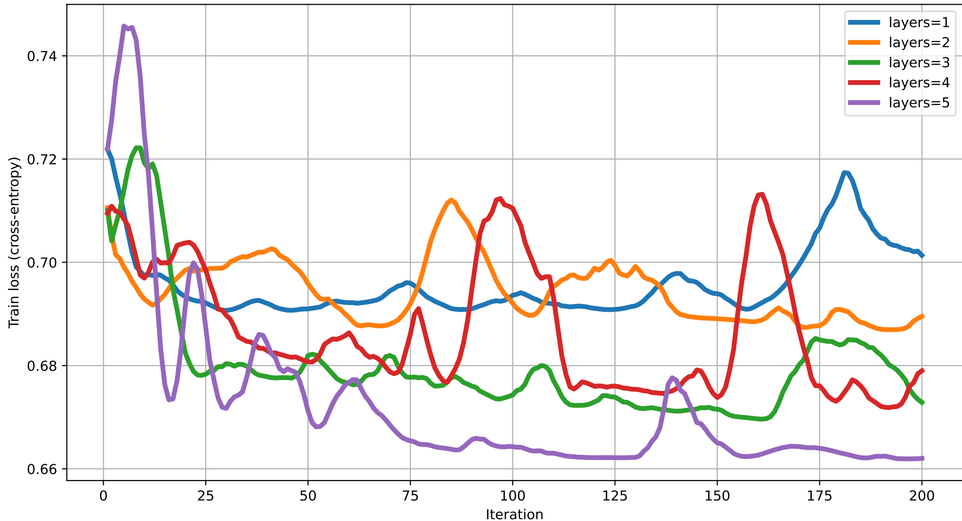
Train loss vs Iteration (dim=20) rot=RX, ent=chain, gate=CNOT
