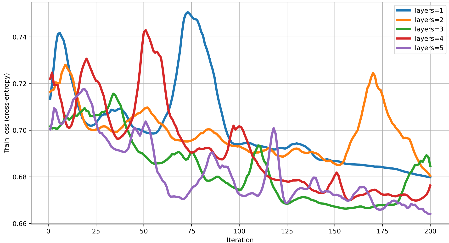
Train loss vs Iteration (dim=14) rot=RYZ, ent=chain, gate=CNOT
