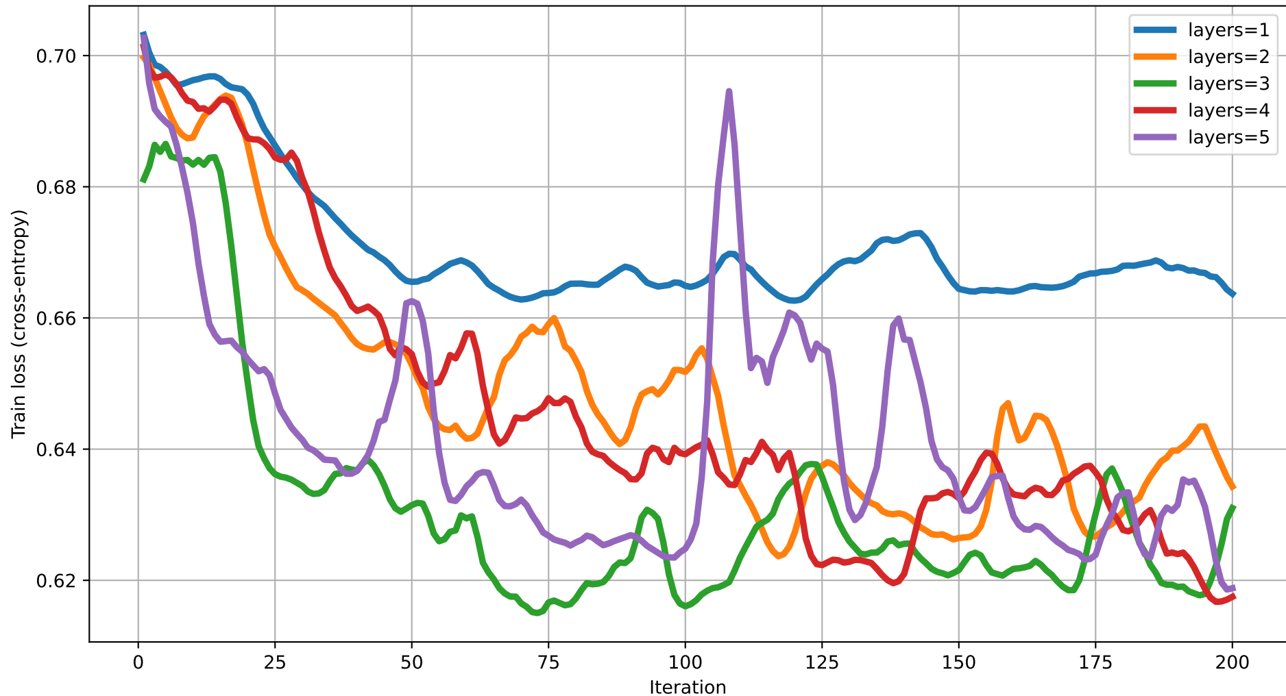
Train loss vs Iteration (dim=16) rot=Rot, ent=ring, gate=CNOT
