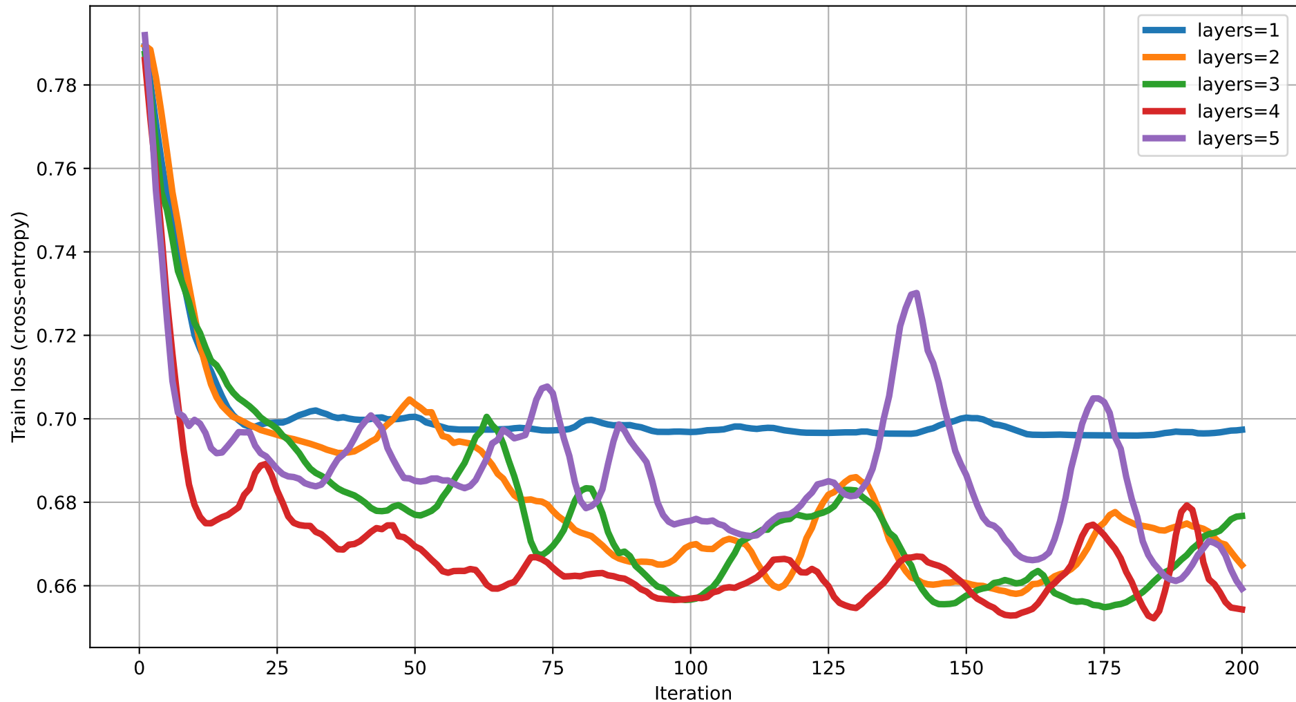
Train loss vs Iteration (dim=2) rot=RY, ent=chain, gate=CZ
