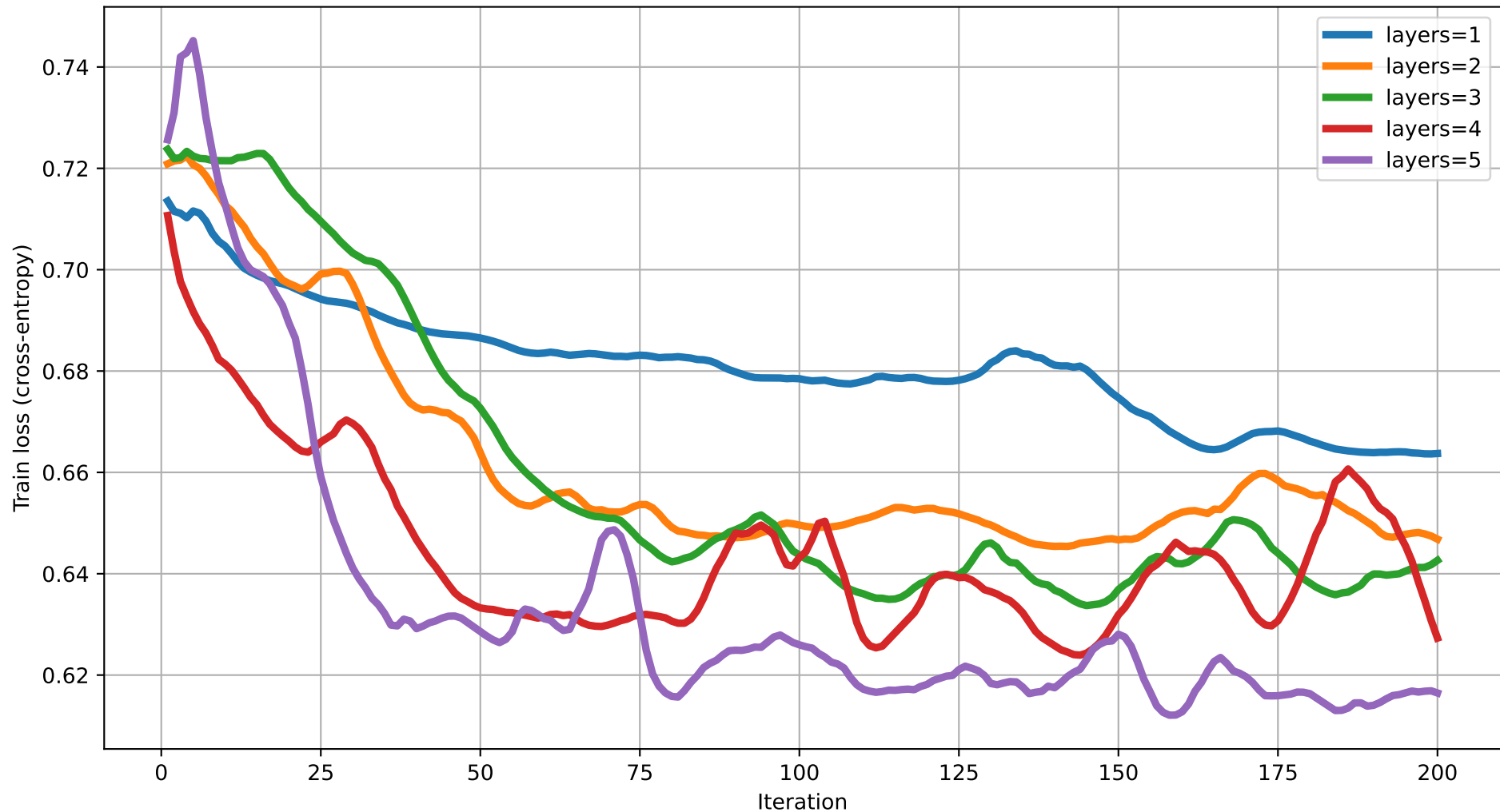
Train loss vs Iteration (dim=7) rot=RY, ent=full, gate=CNOT
