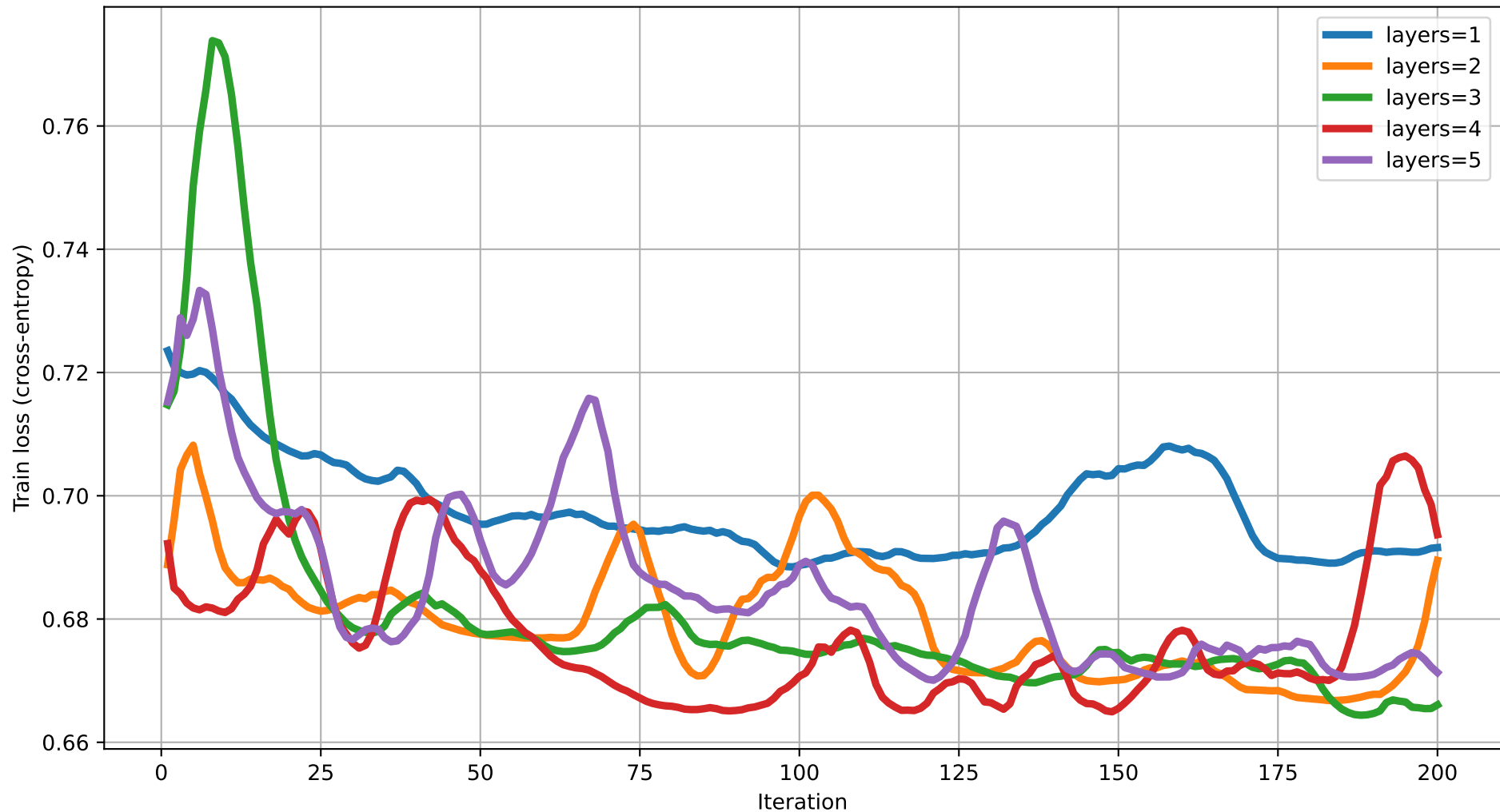
Train loss vs Iteration (dim=15) rot=RY, ent=ring, gate=IsingXX
