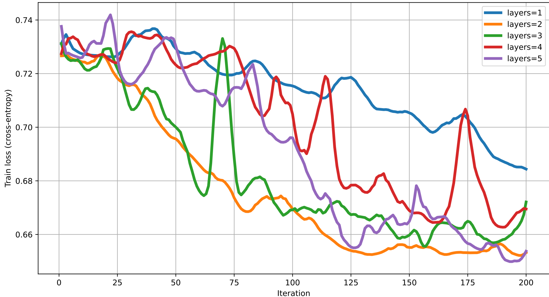
Train loss vs Iteration (dim=7) rot=Rot, ent=chain, gate=CNOT
