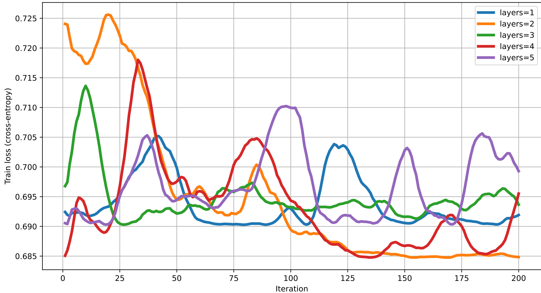
Train loss vs Iteration (dim=15) rot=RX, ent=full, gate=IsingXX
