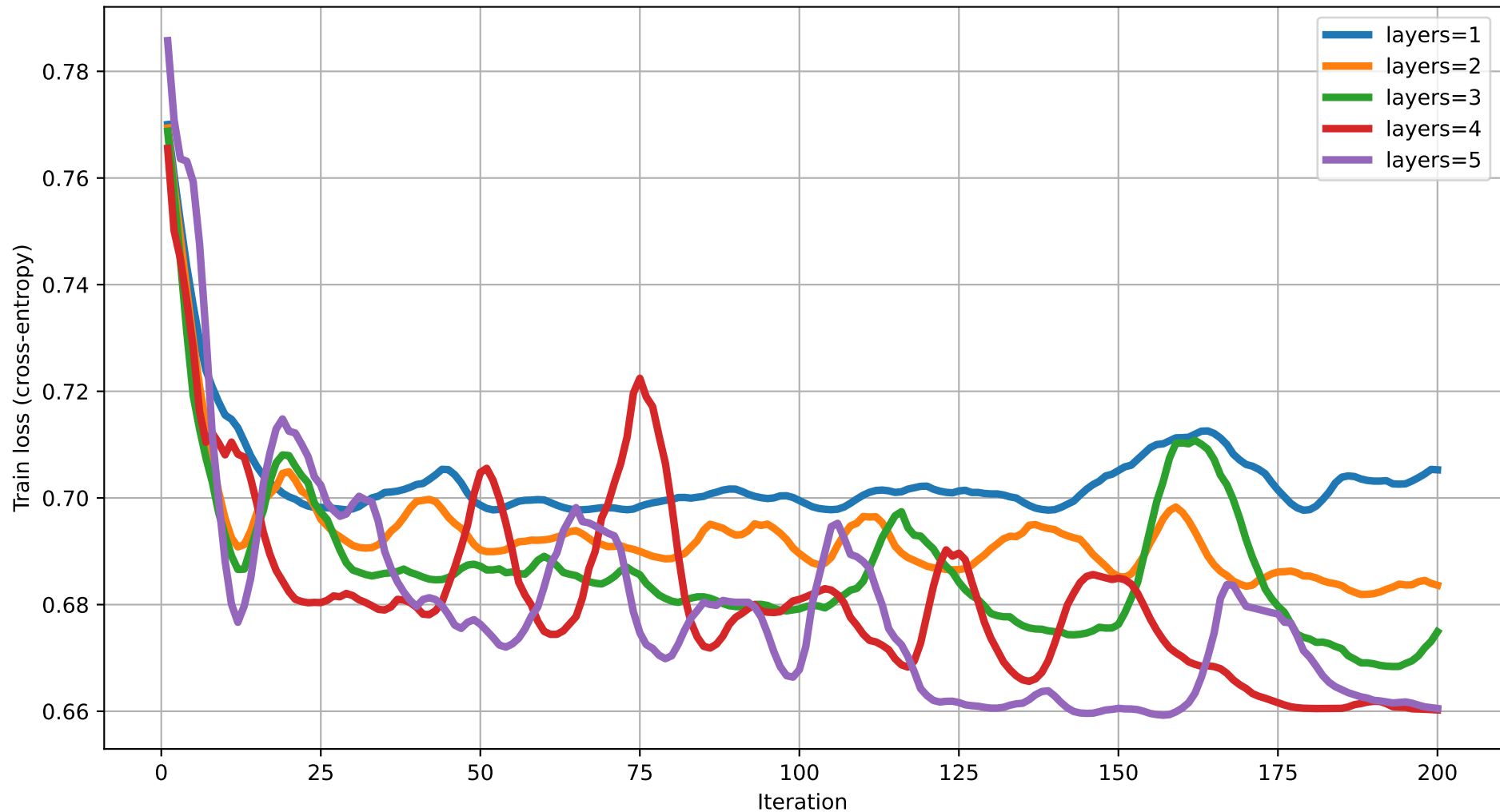
Train loss vs Iteration (dim=17) rot=RX, ent=chain, gate=CNOT
