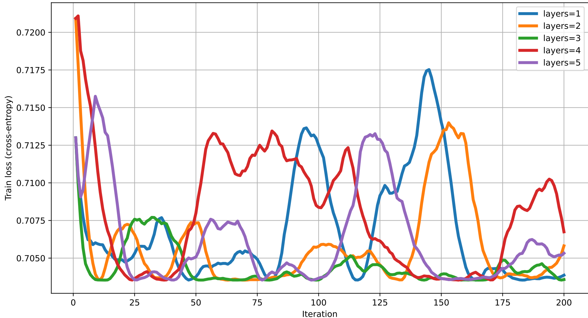
Train loss vs Iteration (dim=11) rot=RZ, ent=pairwise, gate=CZ
