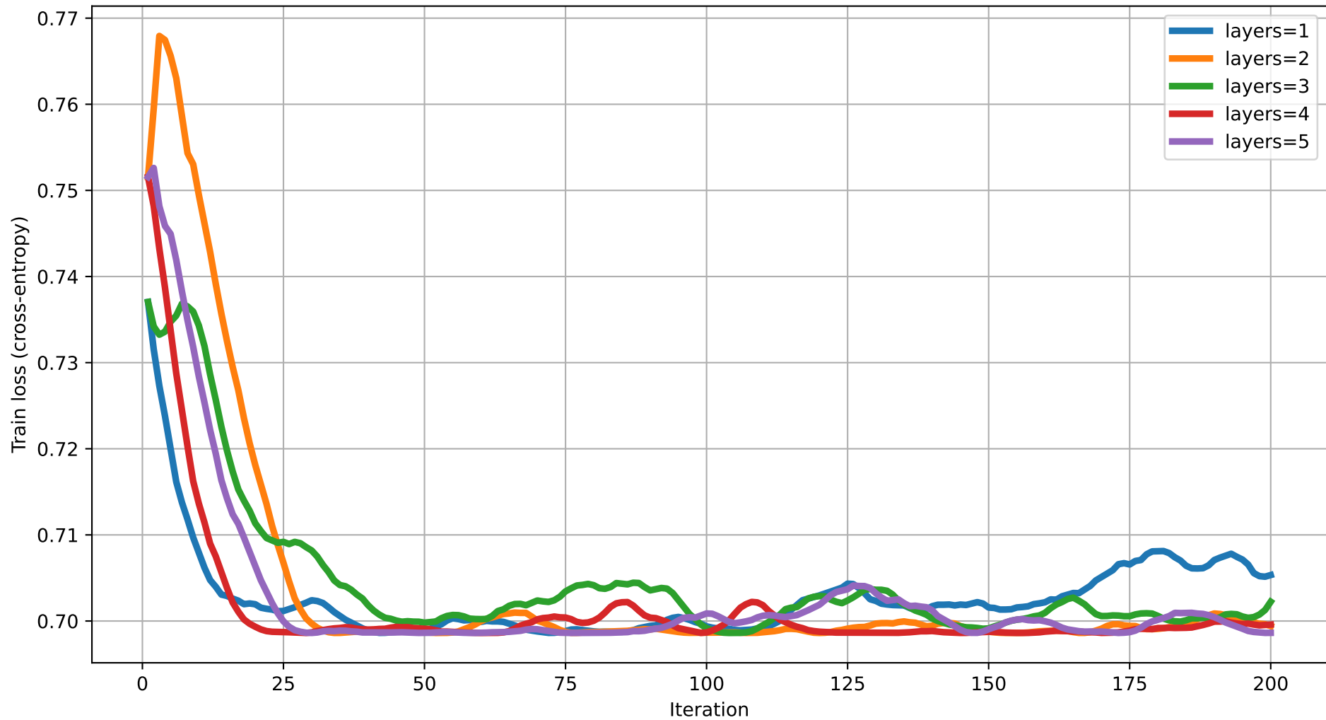
Train loss vs Iteration (dim=18) rot=RZ, ent=chain, gate=CNOT
