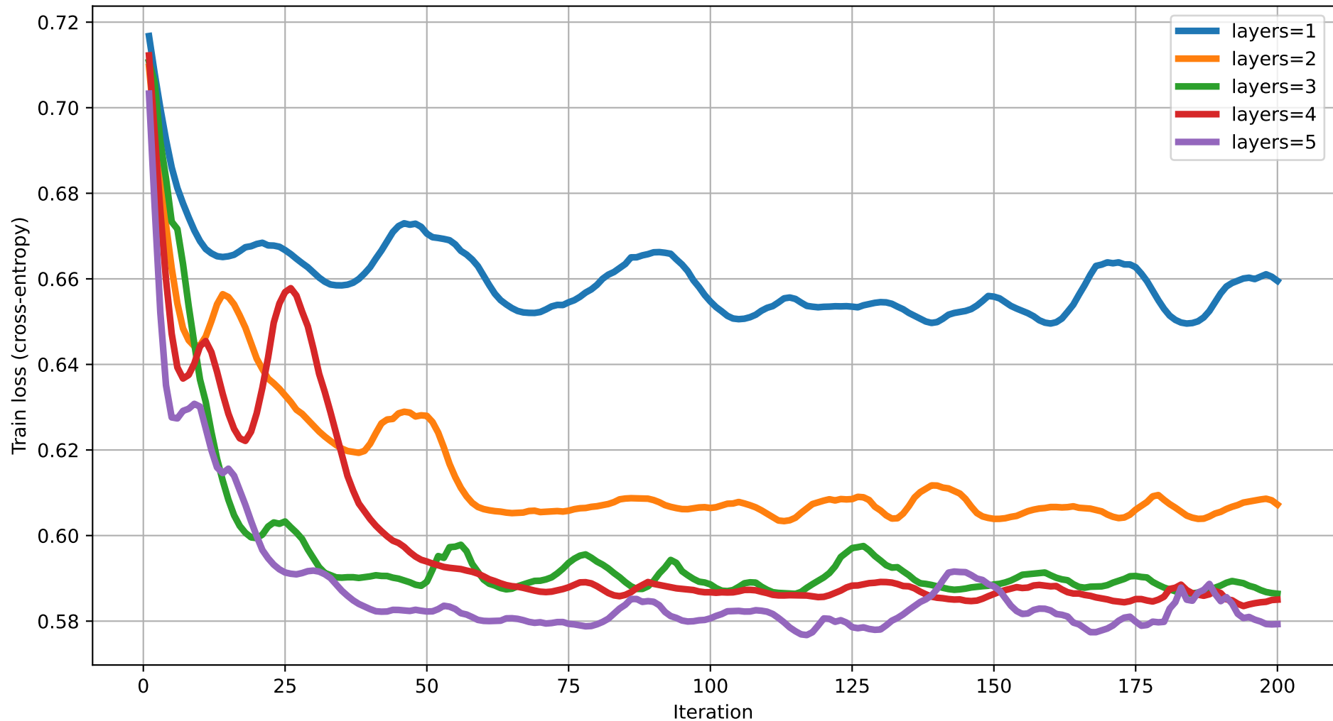
Train loss vs Iteration (degree=4) rot=RYZ, ent=full, gate=CNOT
