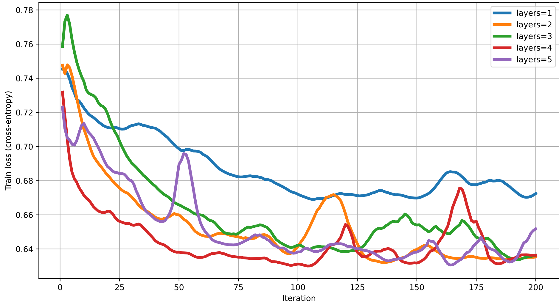
Train loss vs Iteration (dim=3) rot=RYZ, ent=chain, gate=CZ
