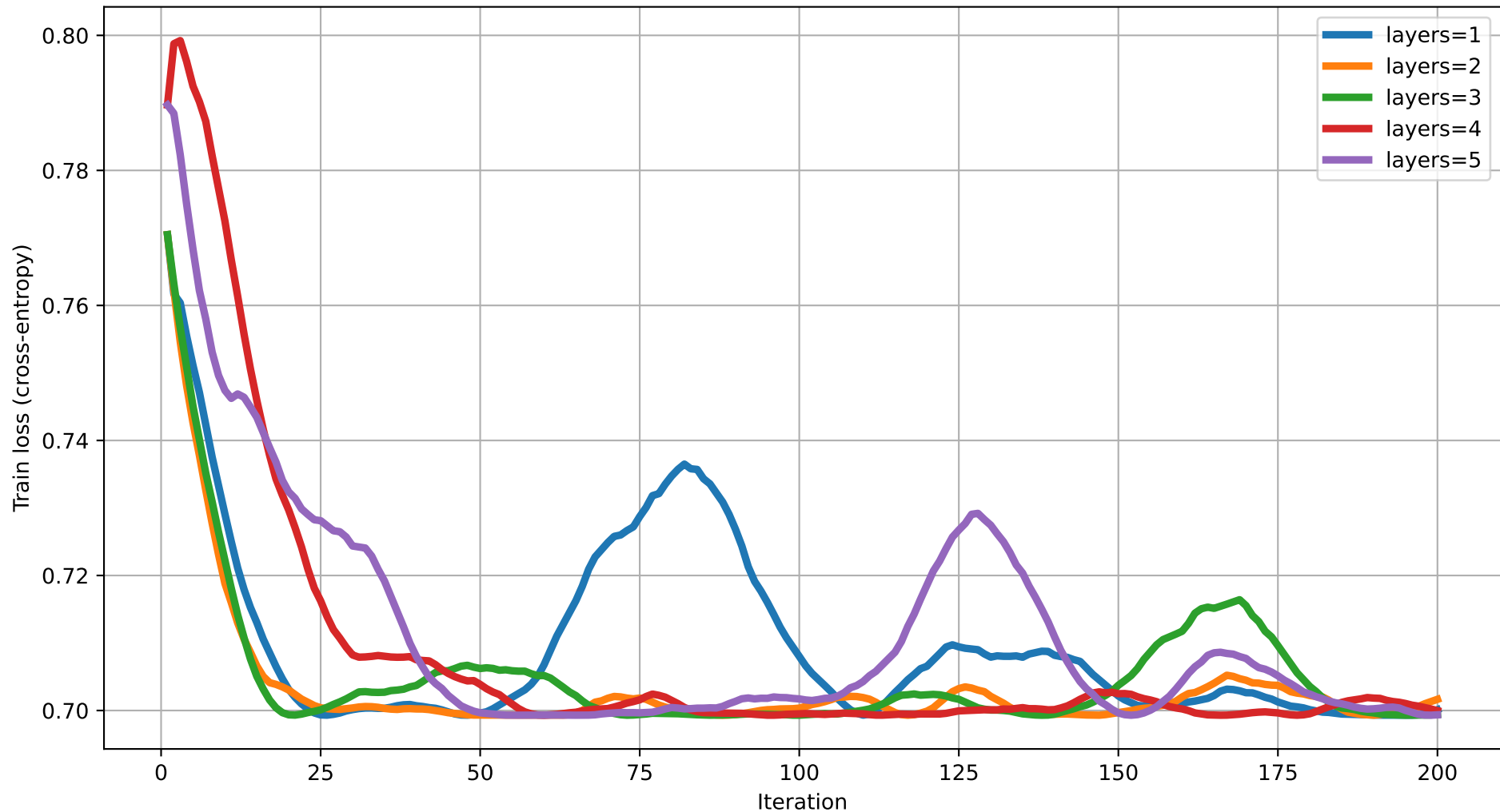
Train loss vs Iteration (dim=17) rot=RZ, ent=chain, gate=CNOT
