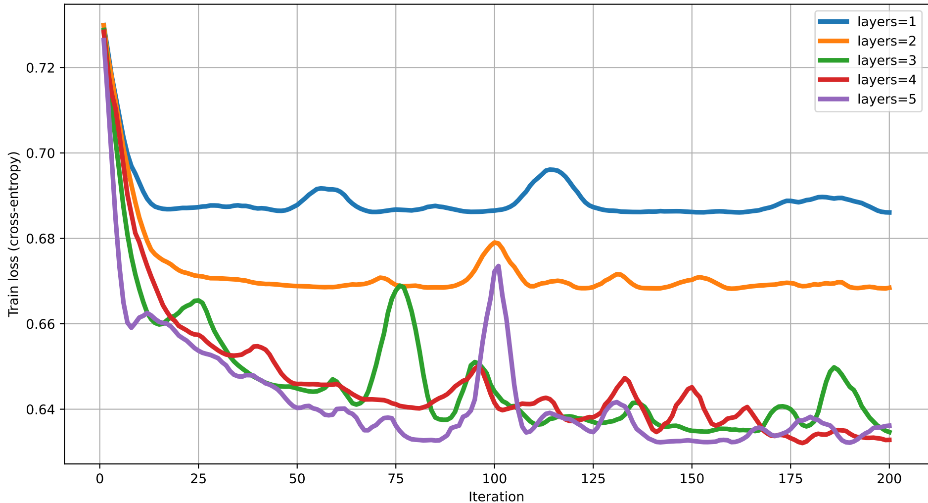
Train loss vs Iteration (degree=2) rot=RX, ent=ring, gate=CZ
