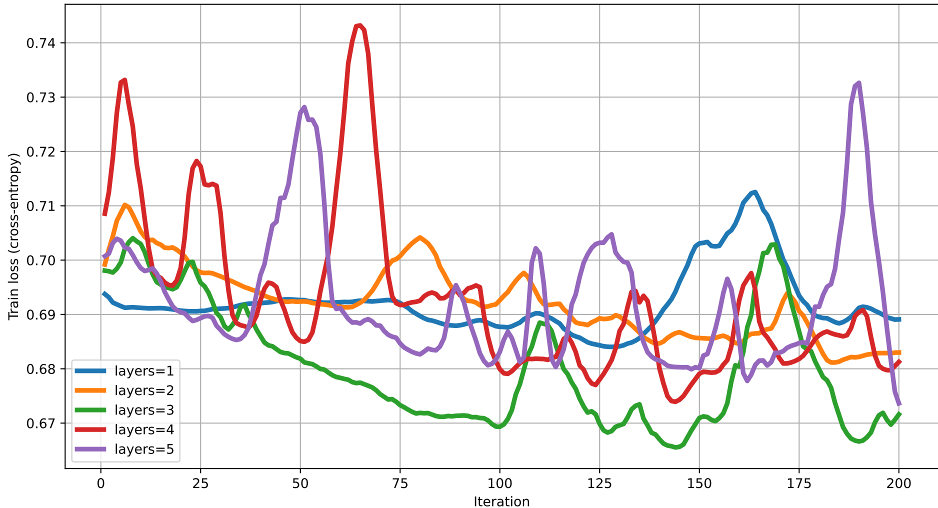
Train loss vs Iteration (dim=20) rot=Rot, ent=ring, gate=CNOT
