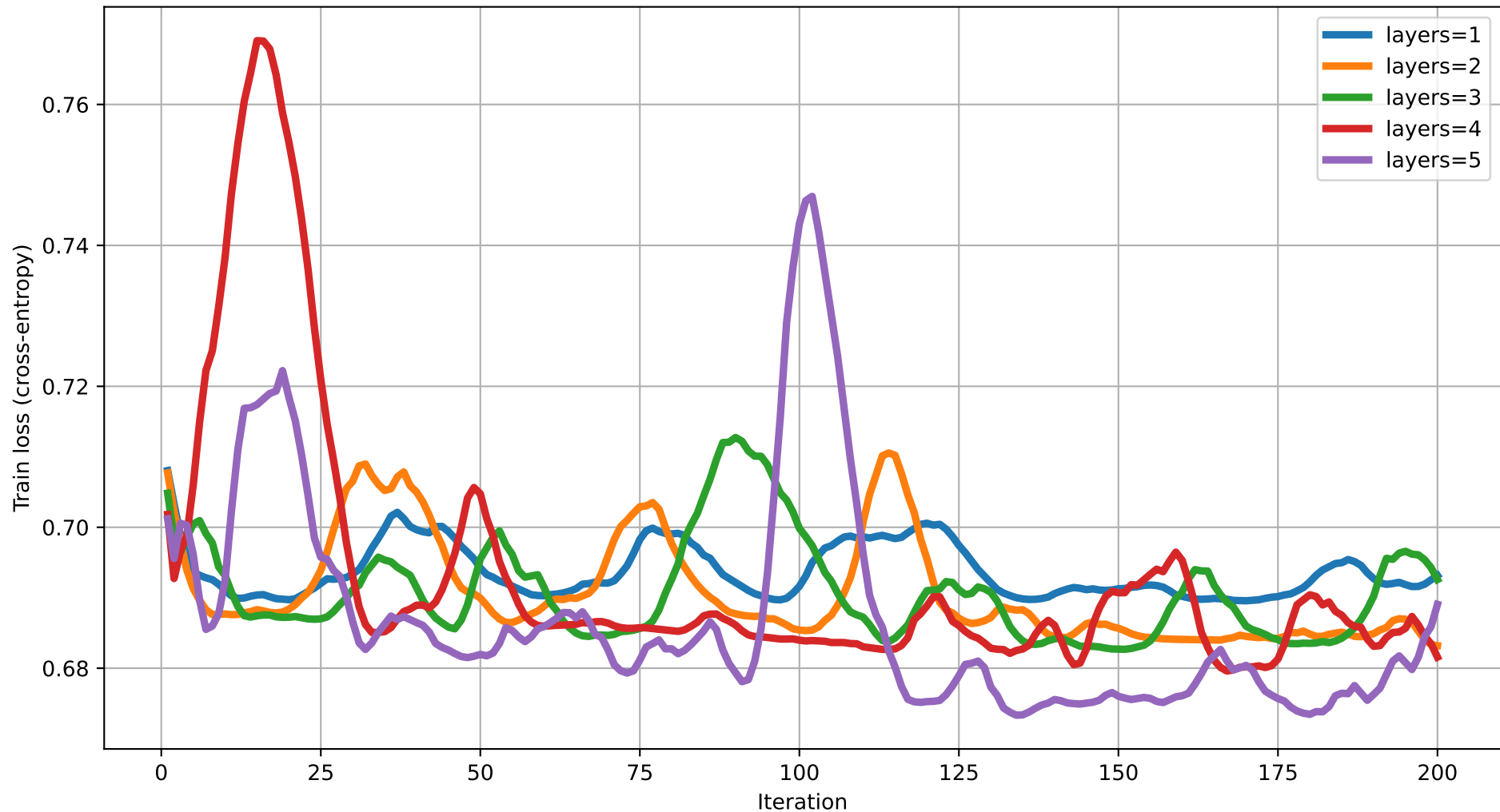
Train loss vs Iteration (dim=20) rot=RY, ent=pairwise, gate=CZ
