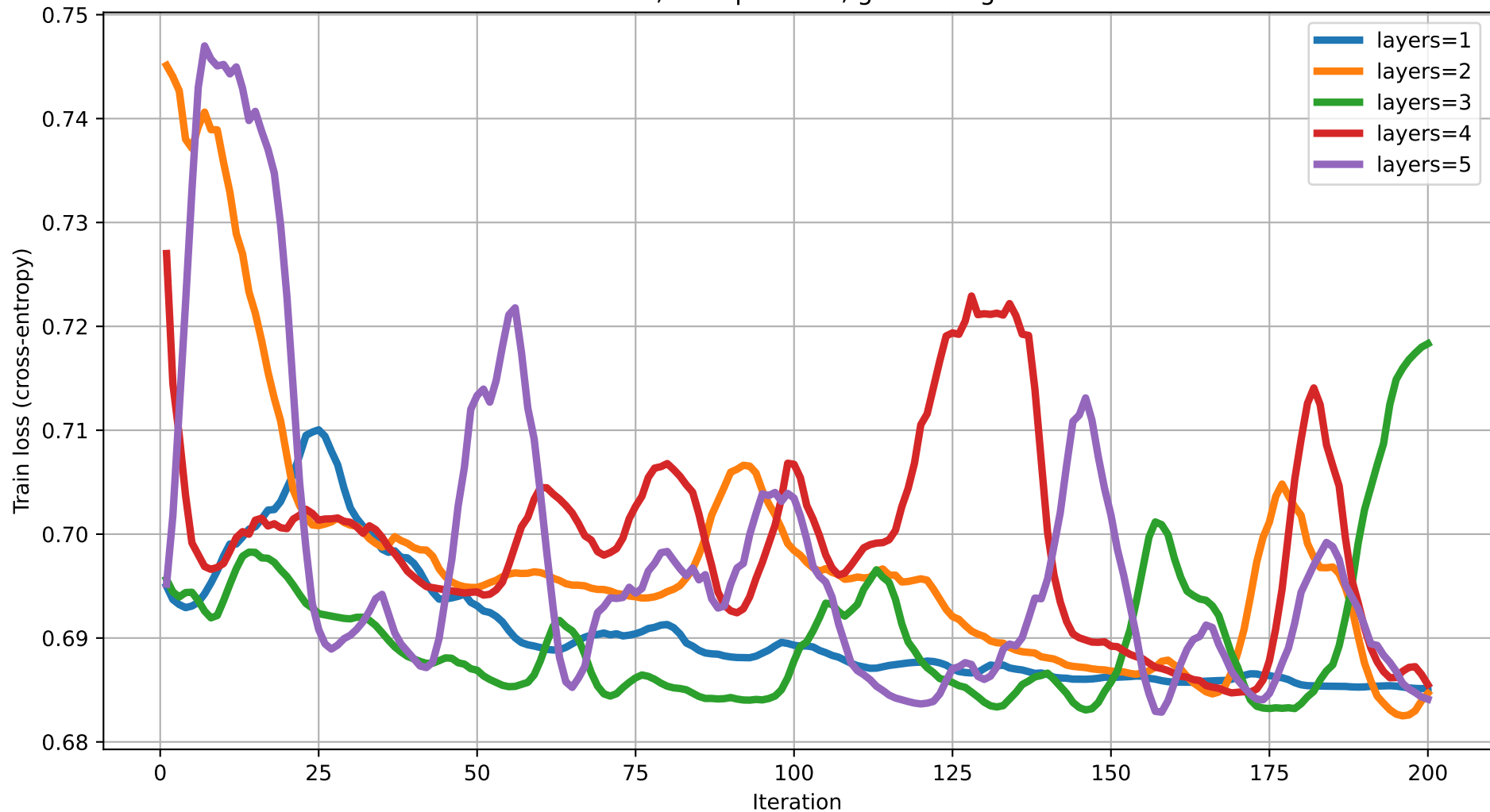
Train loss vs Iteration (dim=19) rot=RZ, ent=pairwise, gate=IsingXX
