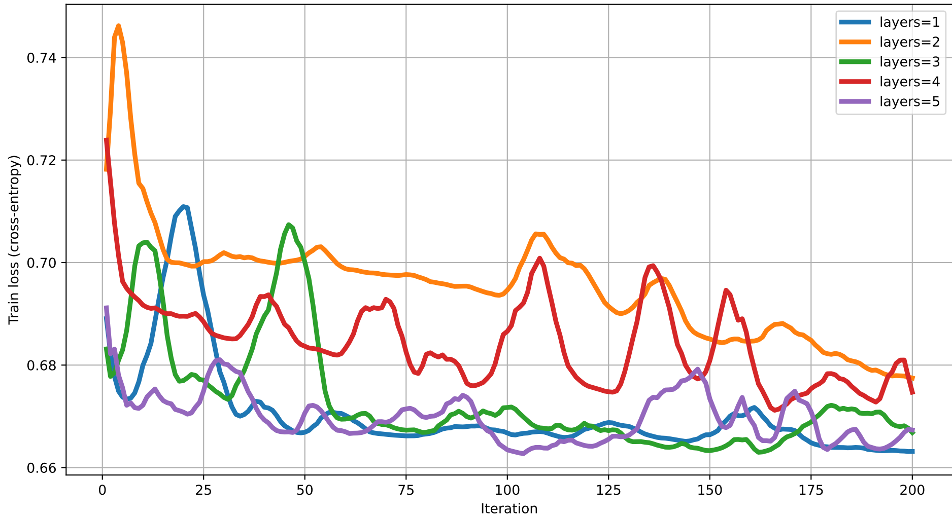
Train loss vs Iteration (dim=12) rot=RY, ent=ring, gate=IsingXX
