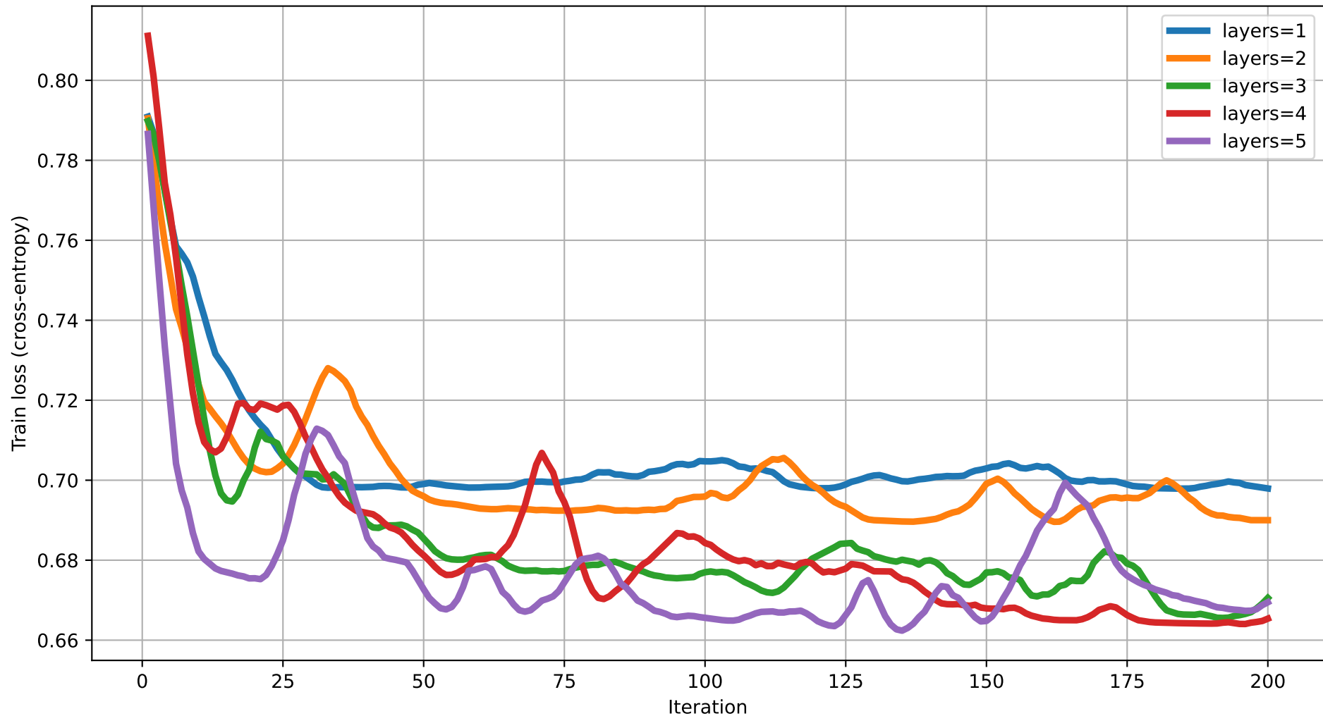
Train loss vs Iteration (dim=4) rot=RX, ent=pairwise, gate=CZ
