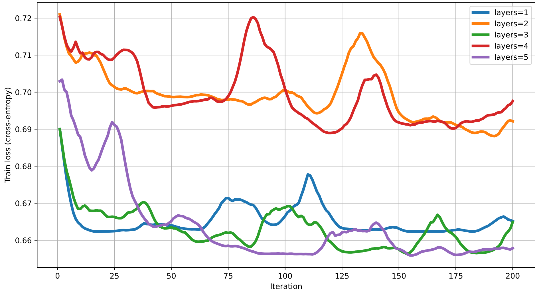
Train loss vs Iteration (dim=11) rot=RZ, ent=ring, gate=IsingXX
