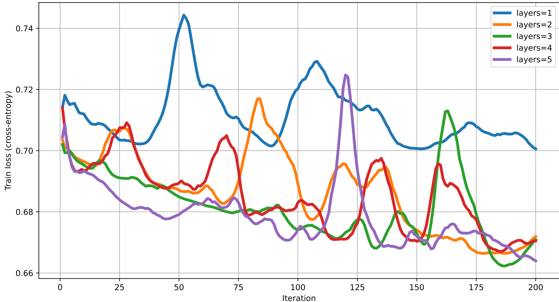
Train loss vs Iteration (dim=12) rot=RYZ, ent=ring, gate=CZ
