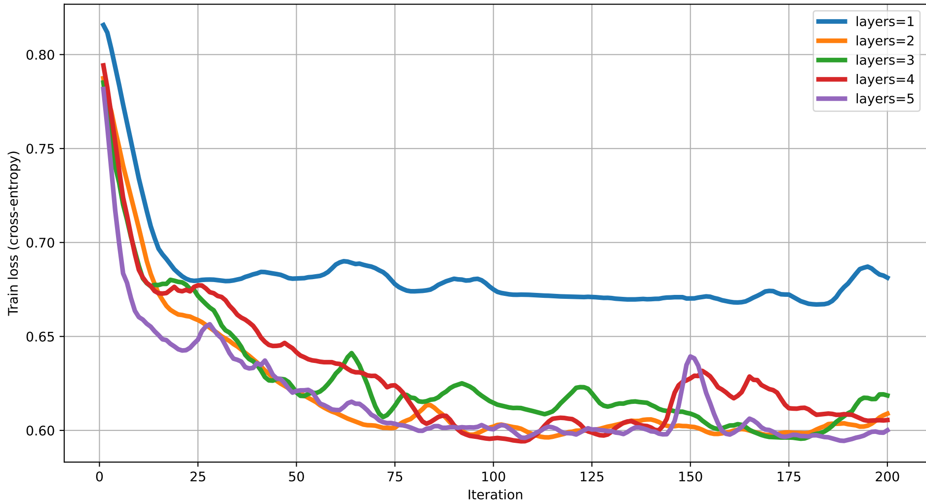
Train loss vs Iteration (dim=4) rot=Rot, ent=ring, gate=CZ
