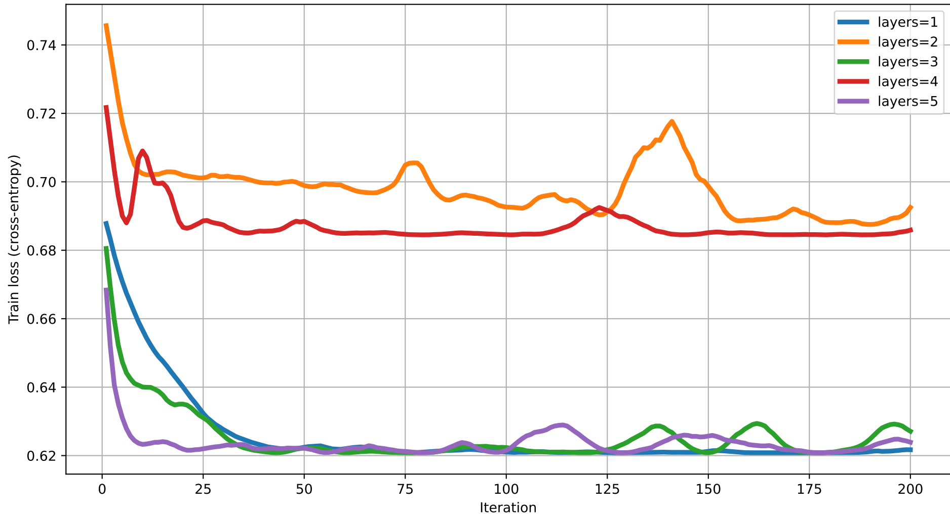
Train loss vs Iteration (degree=3) rot=RX, ent=pairwise, gate=IsingXX
