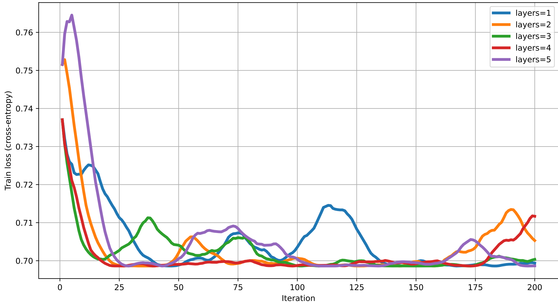
Train loss vs Iteration (dim=18) rot=RZ, ent=ring, gate=CZ
