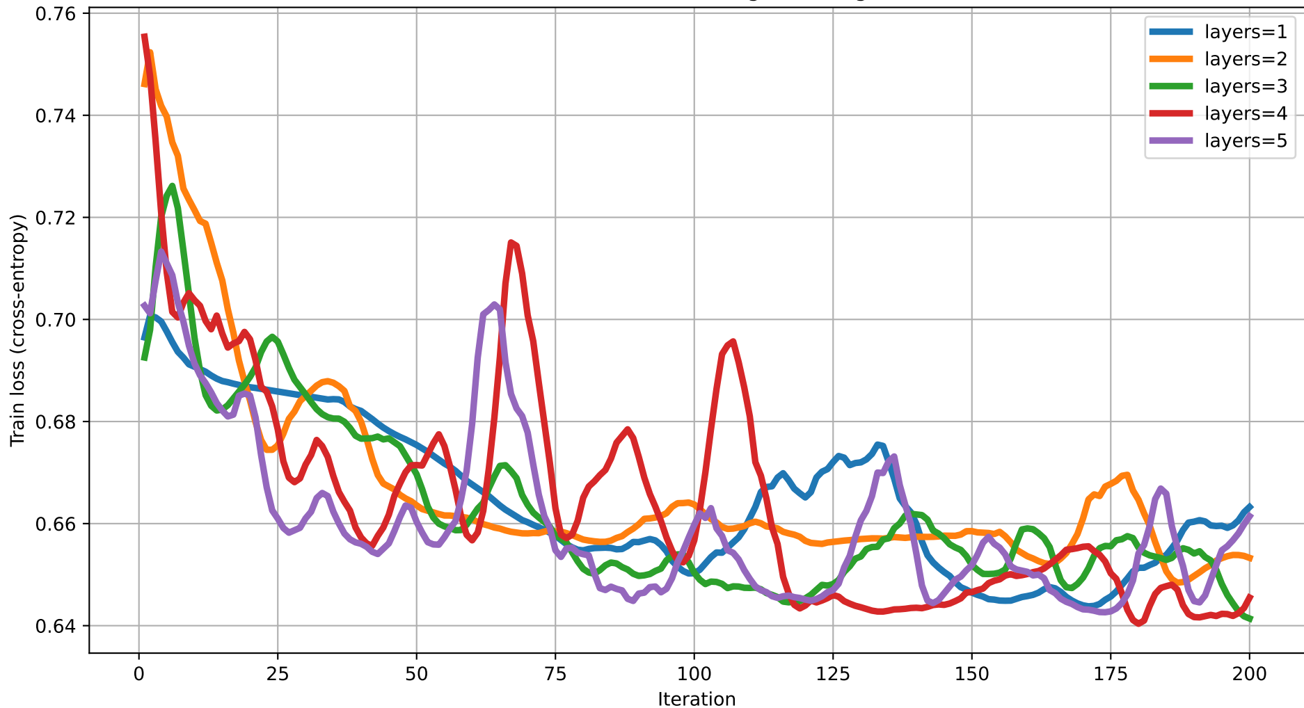
Train loss vs Iteration (dim=5) rot=RYZ, ent=chain, gate=IsingXX
