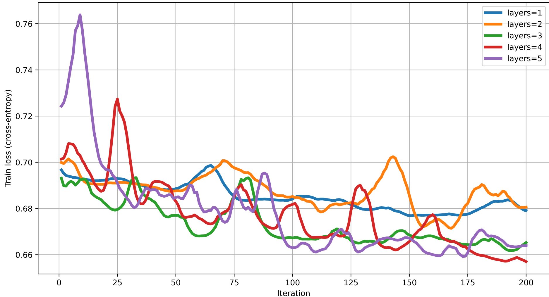
Train loss vs Iteration (dim=11) rot=RYZ, ent=ring, gate=CNOT
