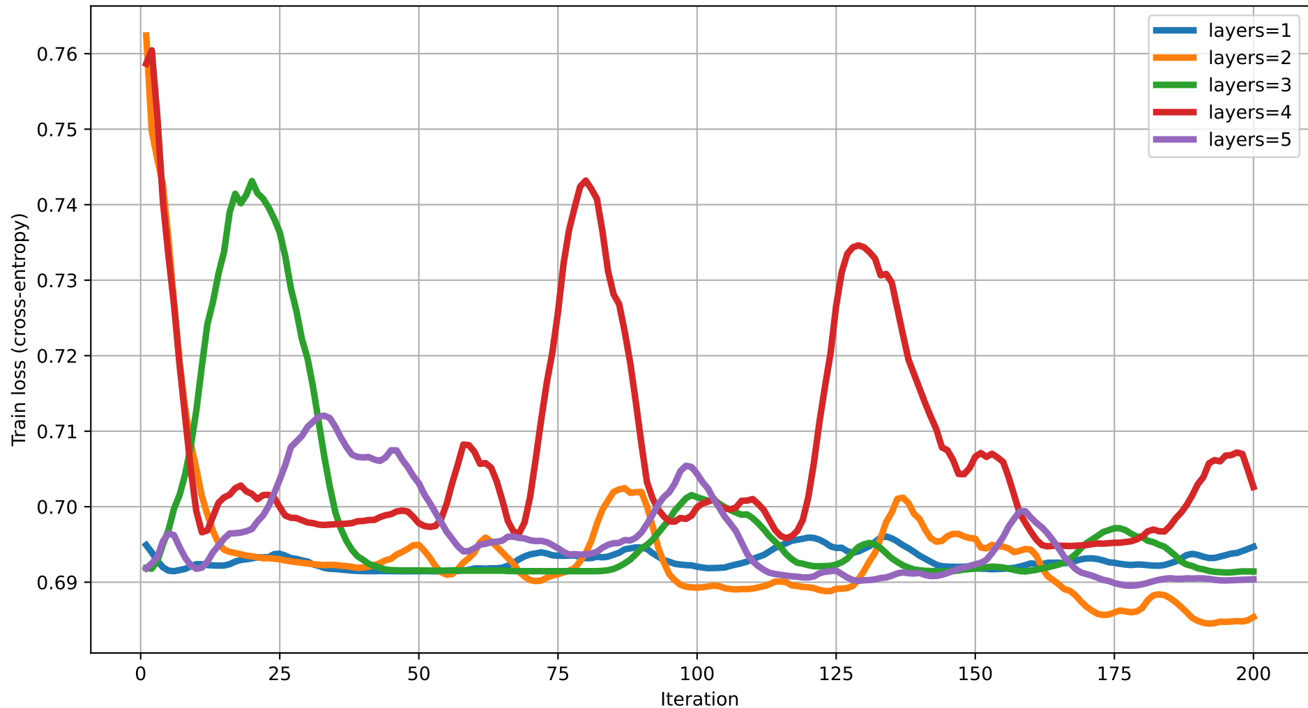
Train loss vs Iteration (dim=18) rot=RY, ent=chain, gate=IsingXX
