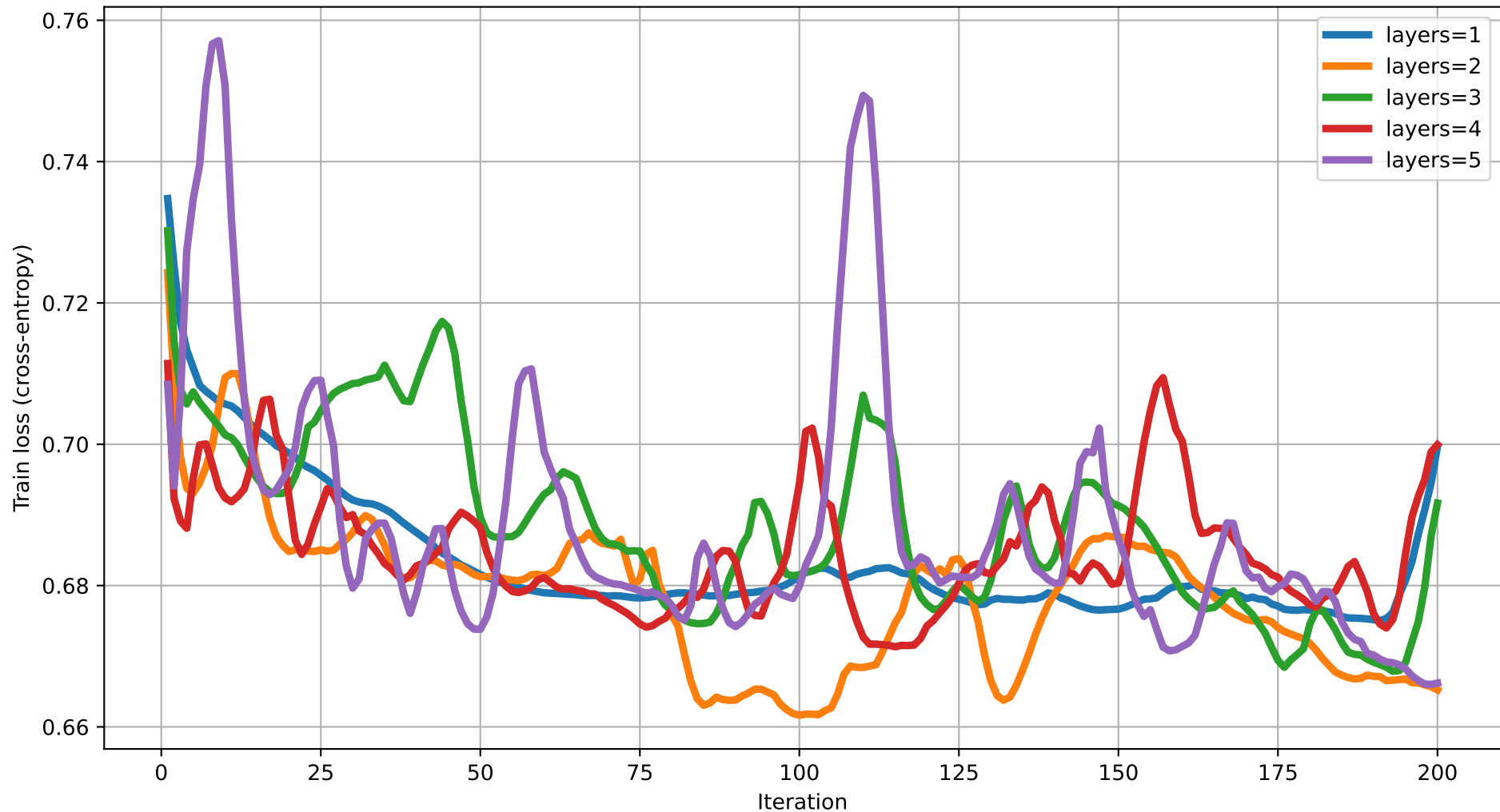
Train loss vs Iteration (dim=19) rot=Rot, ent=full, gate=IsingXX
