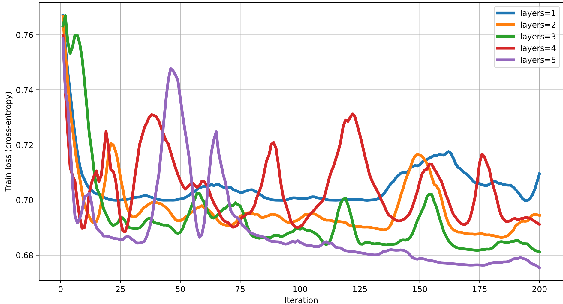
Train loss vs Iteration (dim=17) rot=Rot, ent=pairwise, gate=CZ
