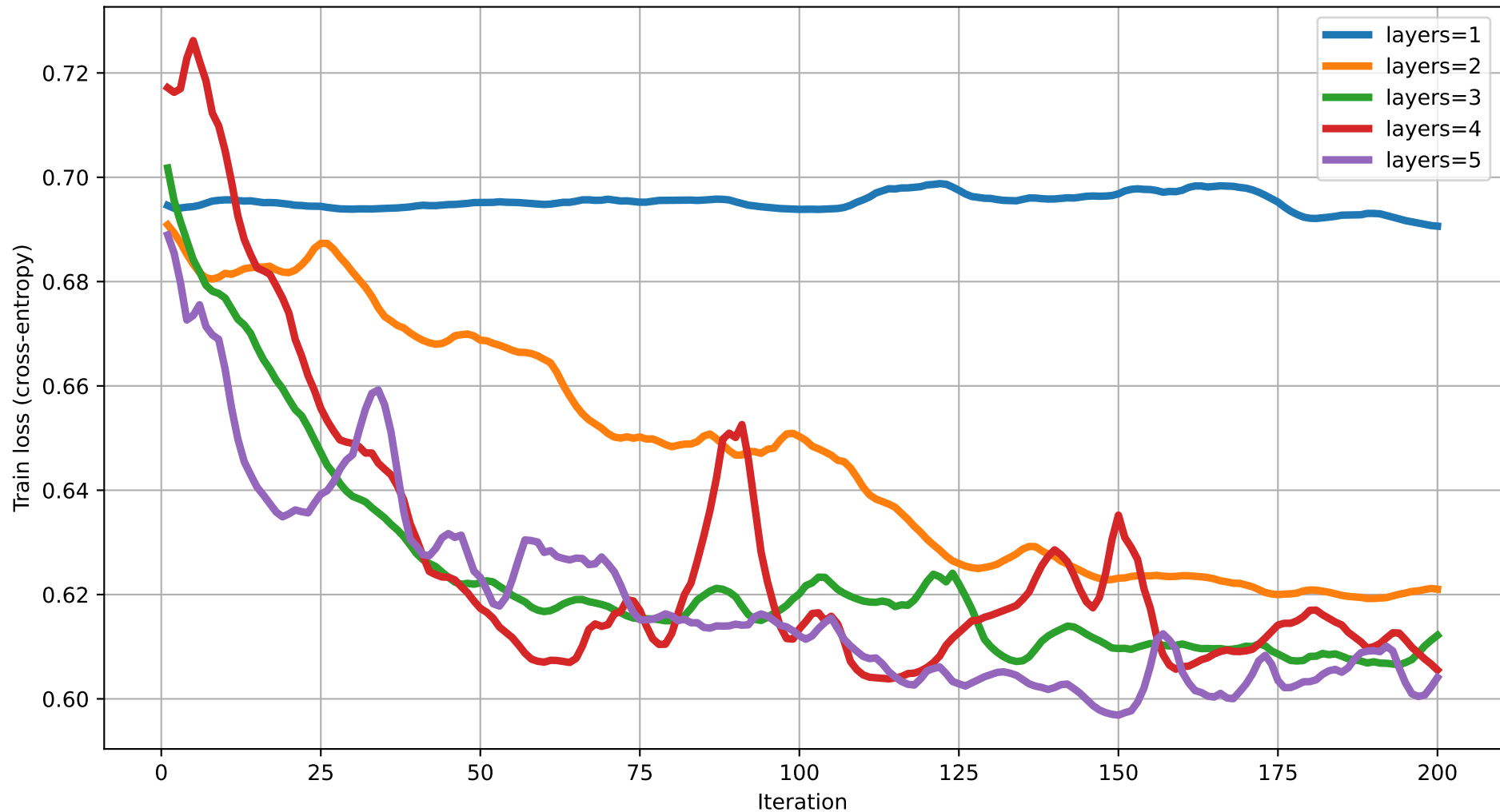
Train loss vs Iteration (dim=14) rot=Rot, ent=ring, gate=CNOT
