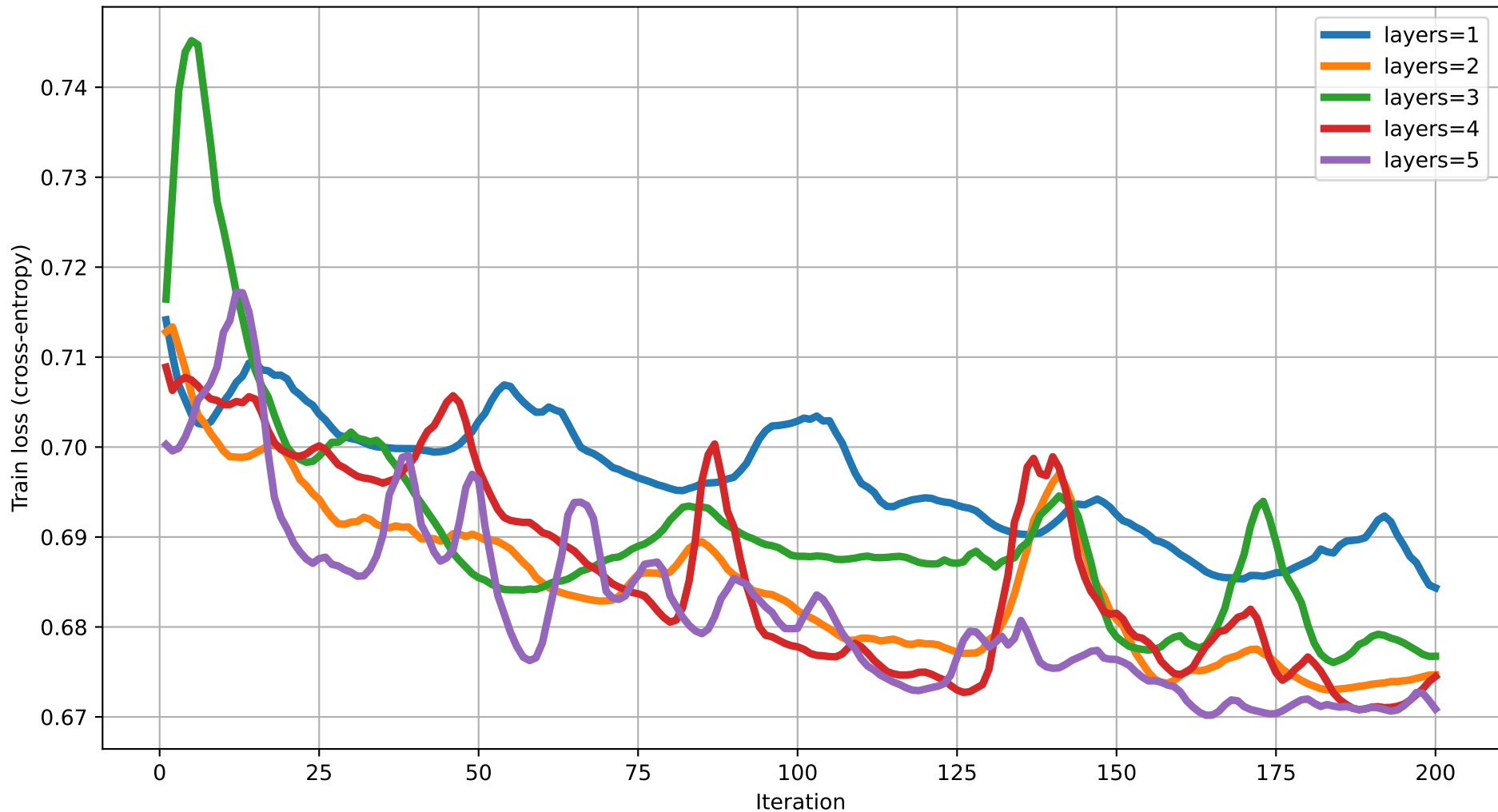
Train loss vs Iteration (dim=14) rot=Rot, ent=full, gate=CZ
