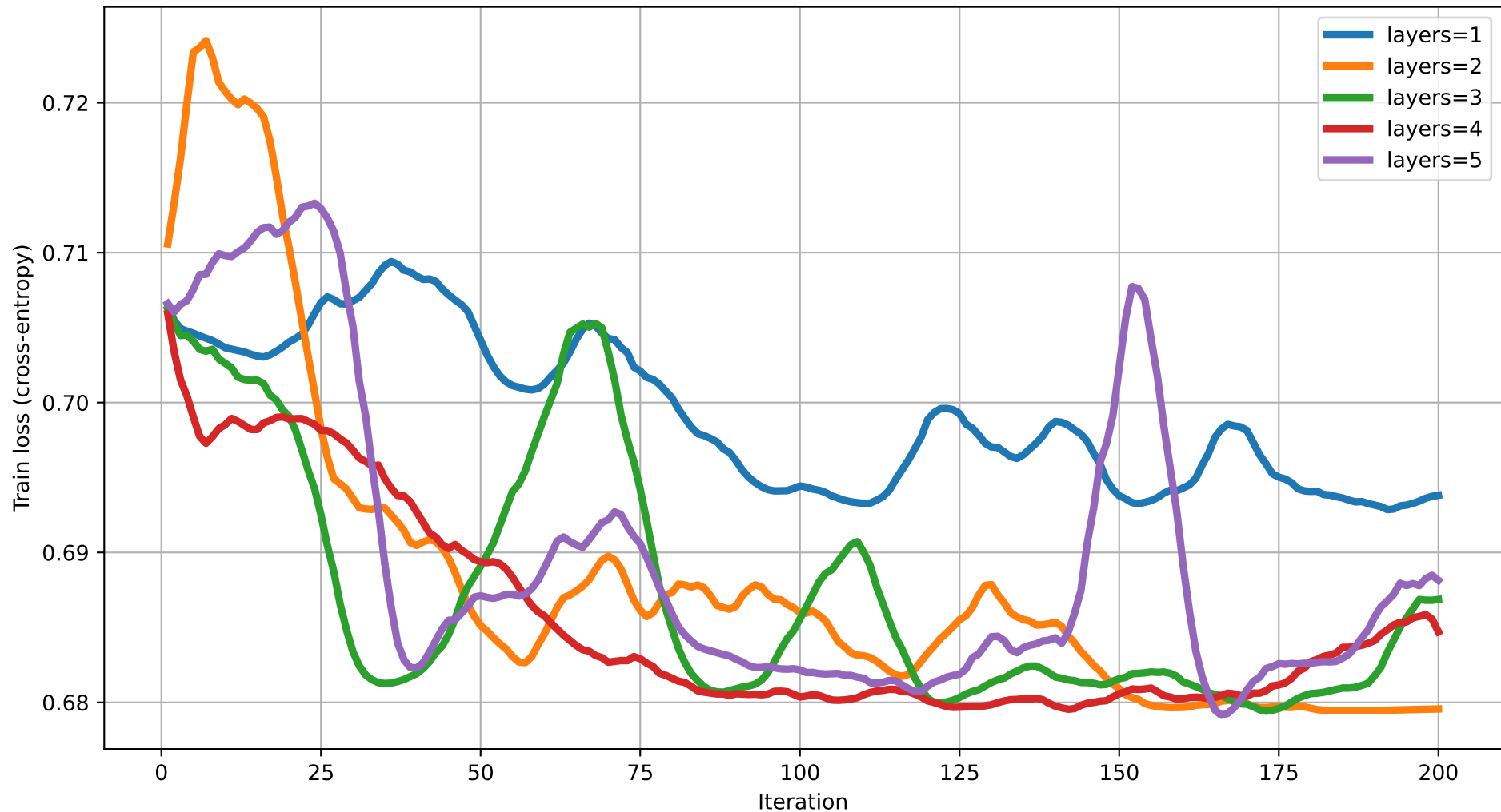
Train loss vs Iteration (dim=14) rot=RX, ent=chain, gate=CNOT
