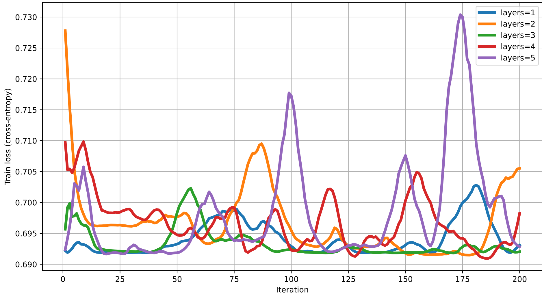
Train loss vs Iteration (dim=11) rot=RY, ent=pairwise, gate=IsingXX
