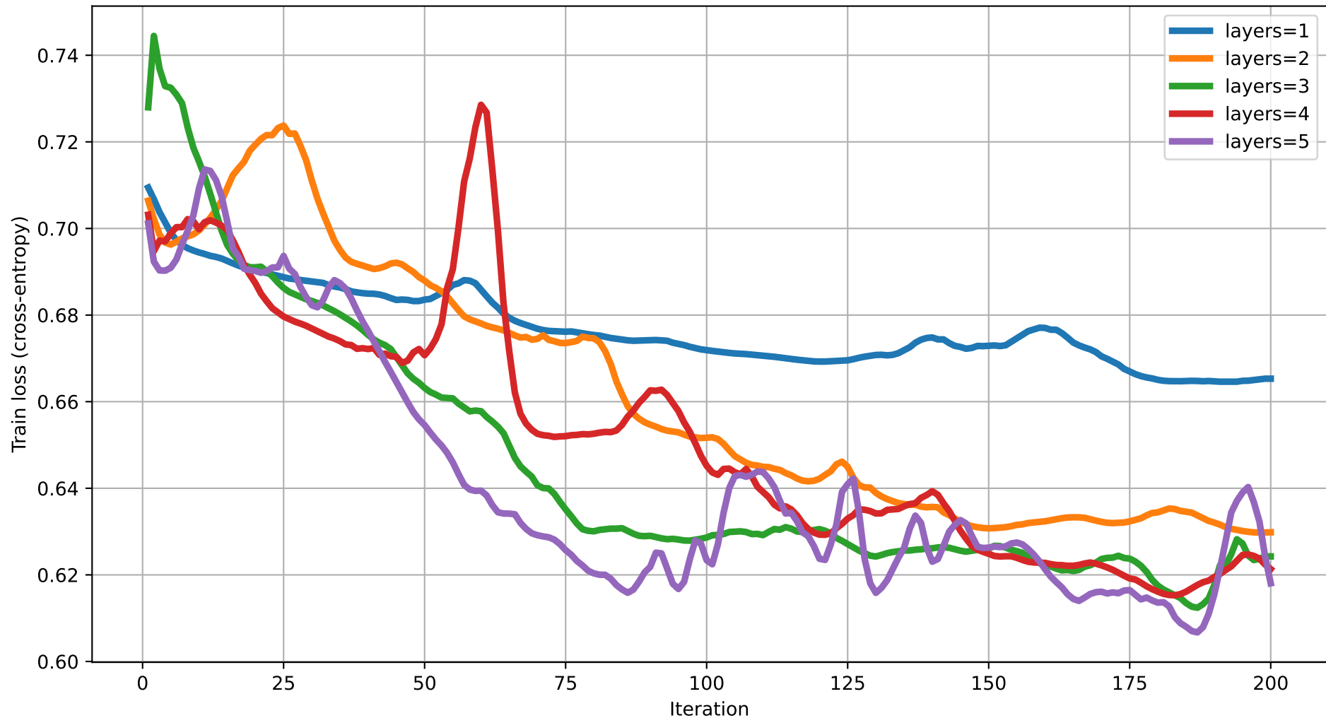
Train loss vs Iteration (dim=13) rot=Rot, ent=chain, gate=CZ
