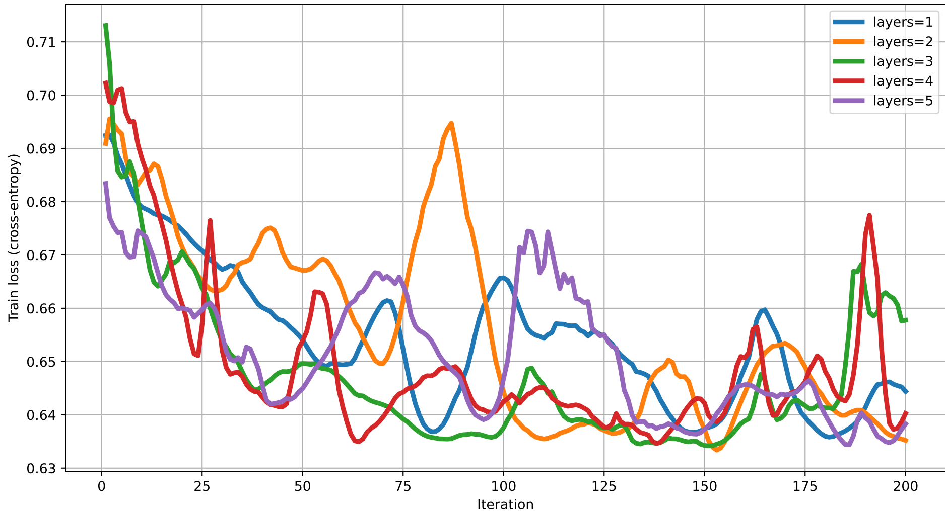
Train loss vs Iteration (dim=7) rot=Rot, ent=pairwise, gate=IsingXX
