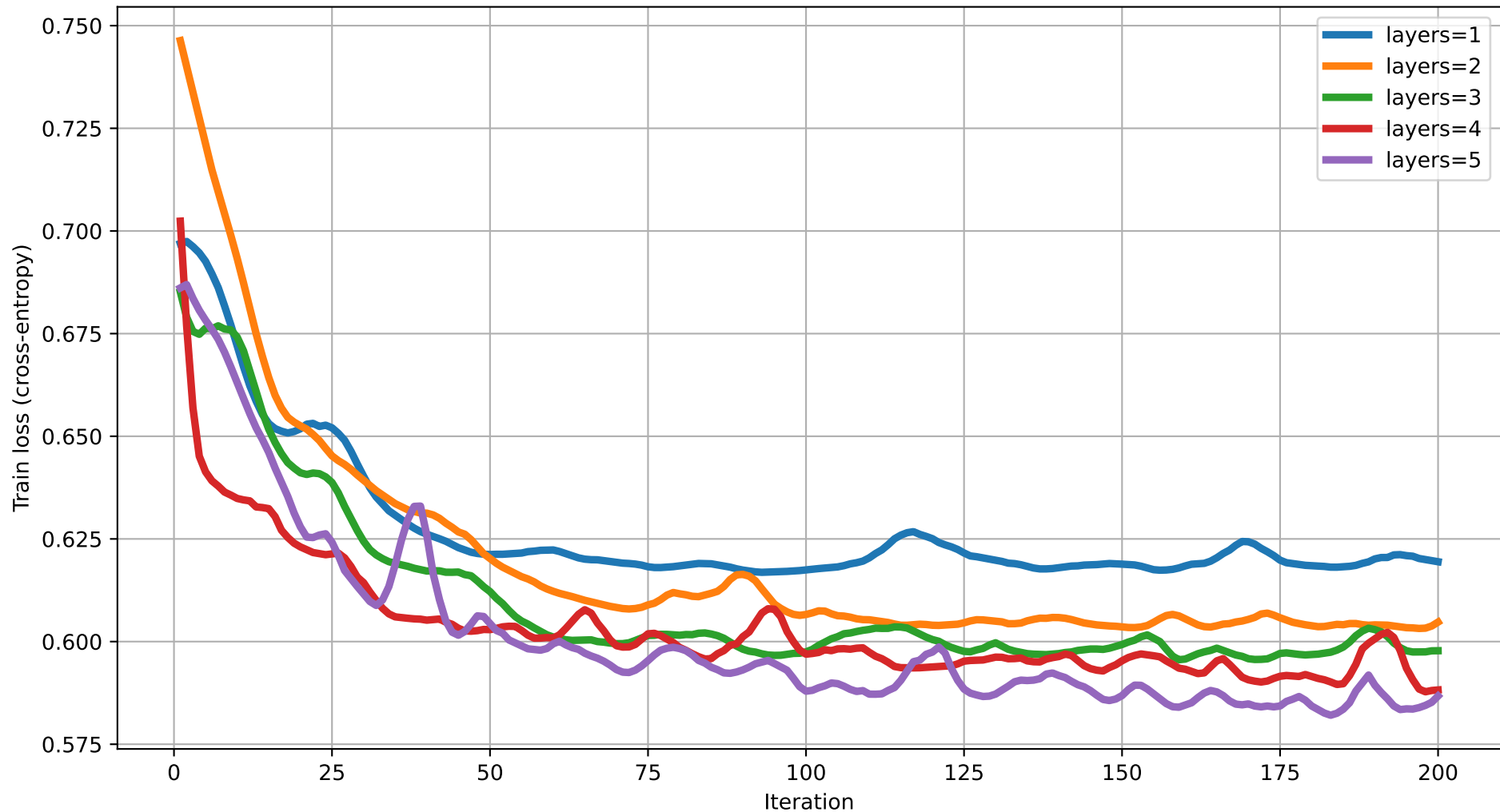
Train loss vs Iteration (degree=3) rot=RYZ, ent=chain, gate=IsingXX
