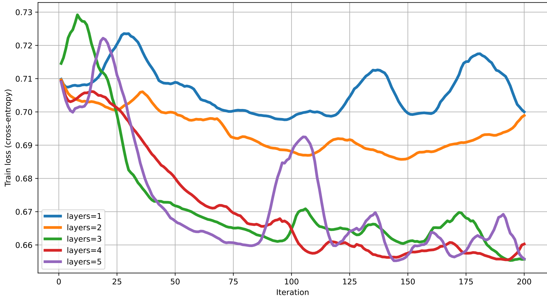
Train loss vs Iteration (dim=6) rot=RX, ent=full, gate=CZ
