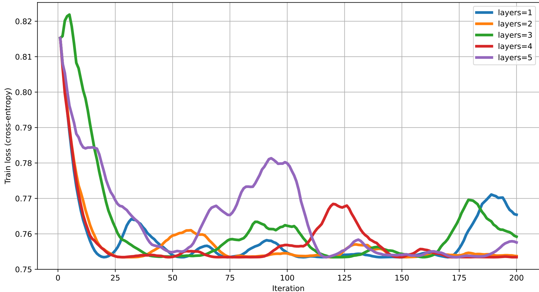
Train loss vs Iteration (dim=2) rot=RZ, ent=pairwise, gate=CZ
