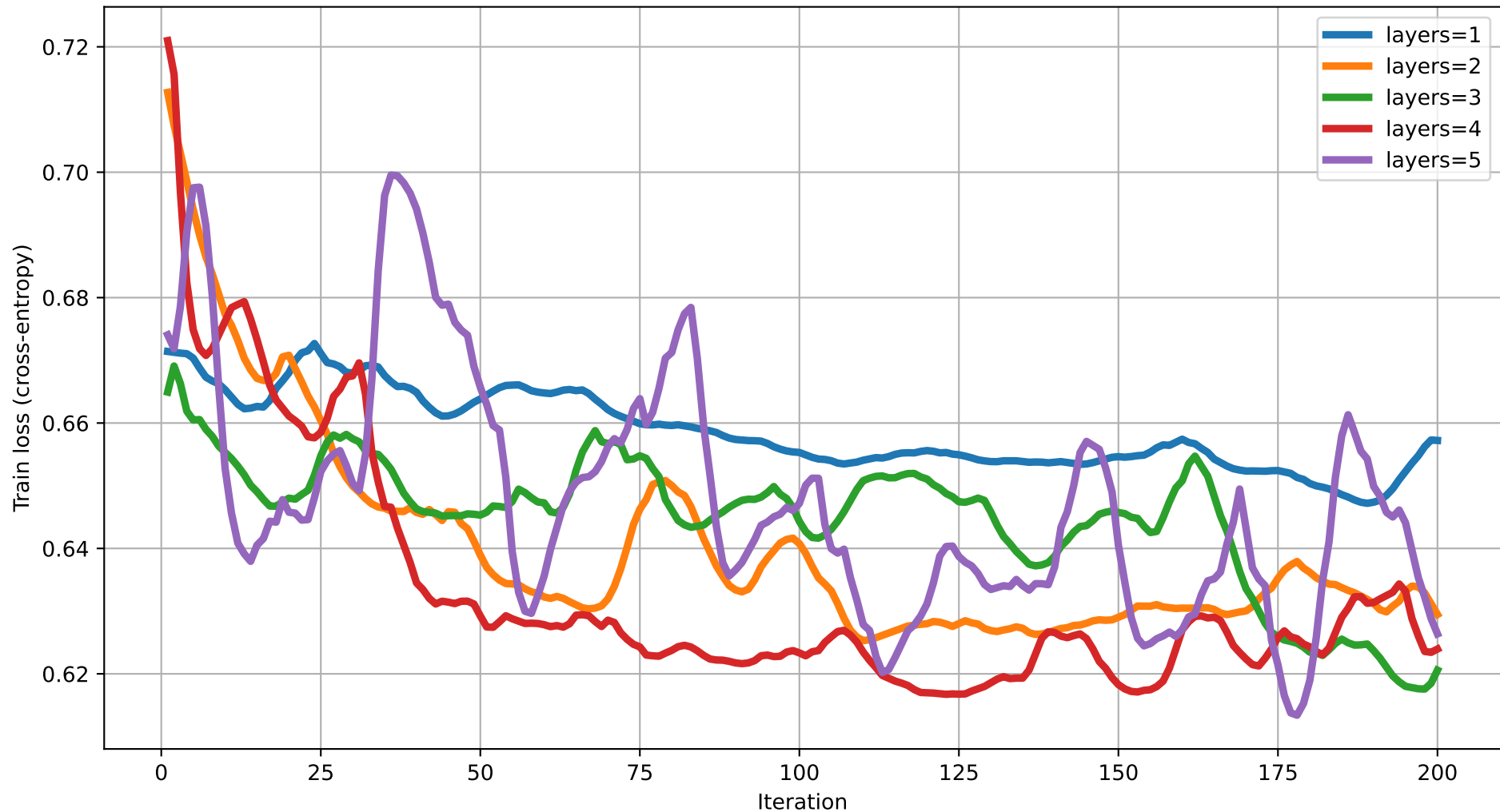
Train loss vs Iteration (dim=7) rot=Rot, ent=full, gate=IsingXX
