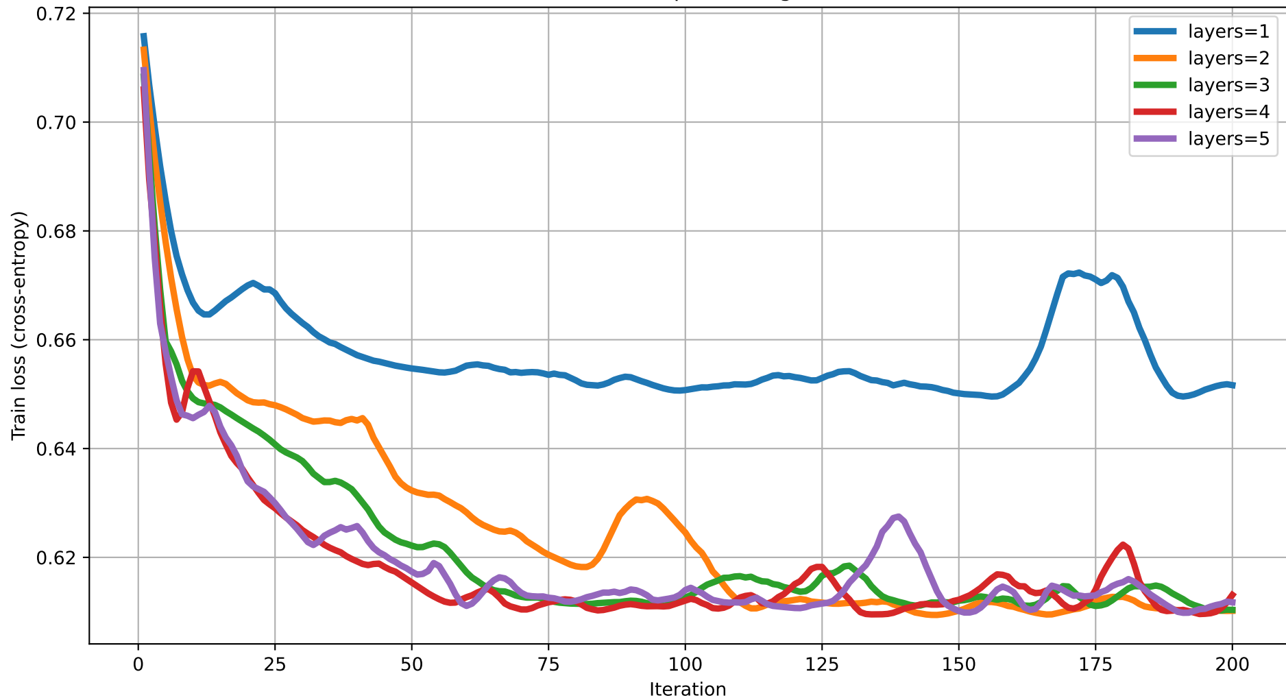
Train loss vs Iteration (degree=4) rot=RYZ, ent=pairwise, gate=CZ
