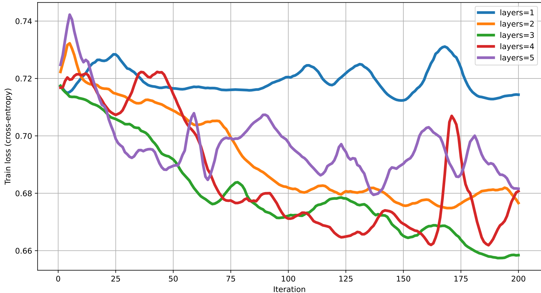
Train loss vs Iteration (dim=3) rot=RYZ, ent=pairwise, gate=CZ
