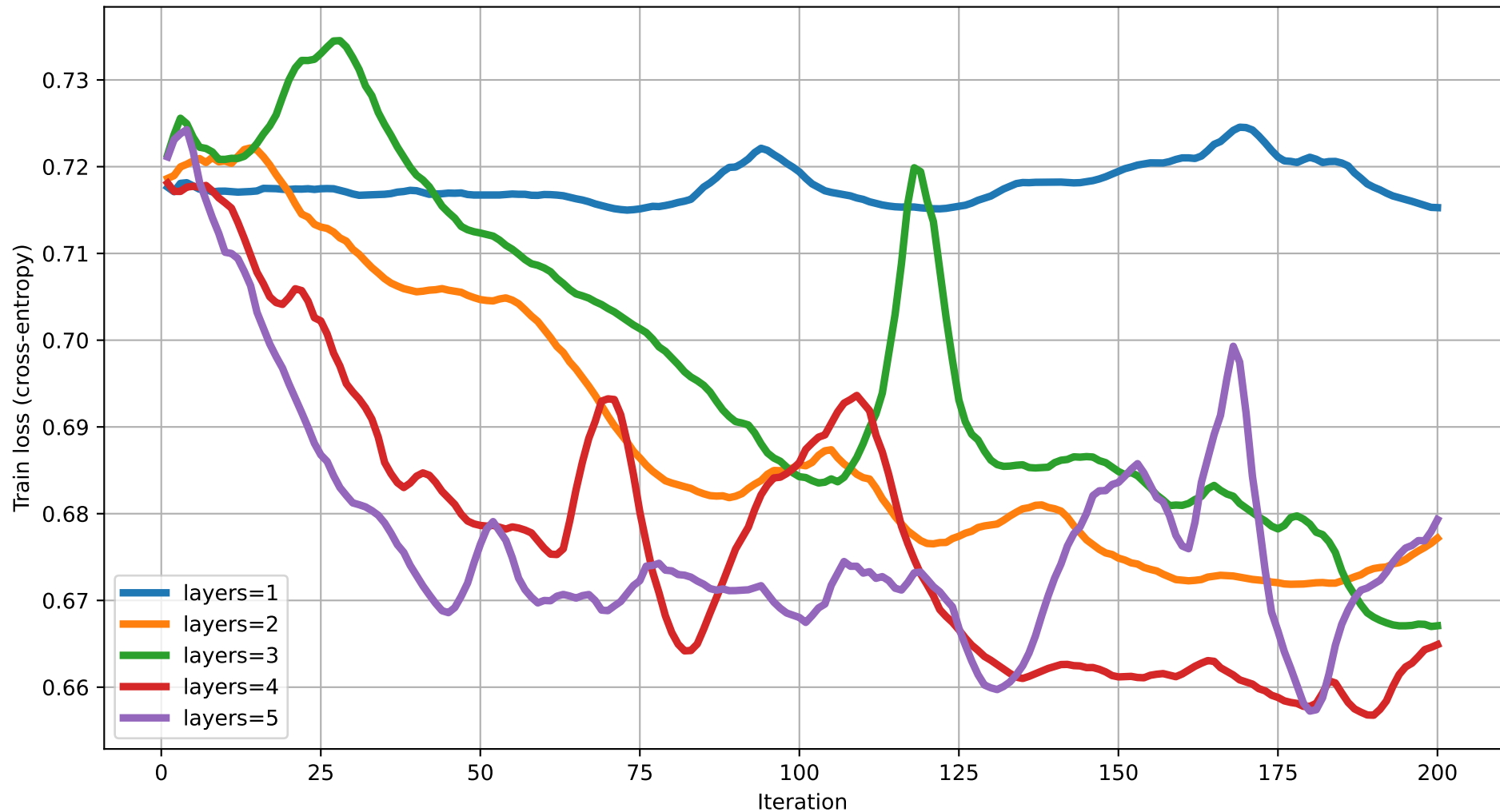
Train loss vs Iteration (dim=3) rot=RY, ent=pairwise, gate=CNOT
