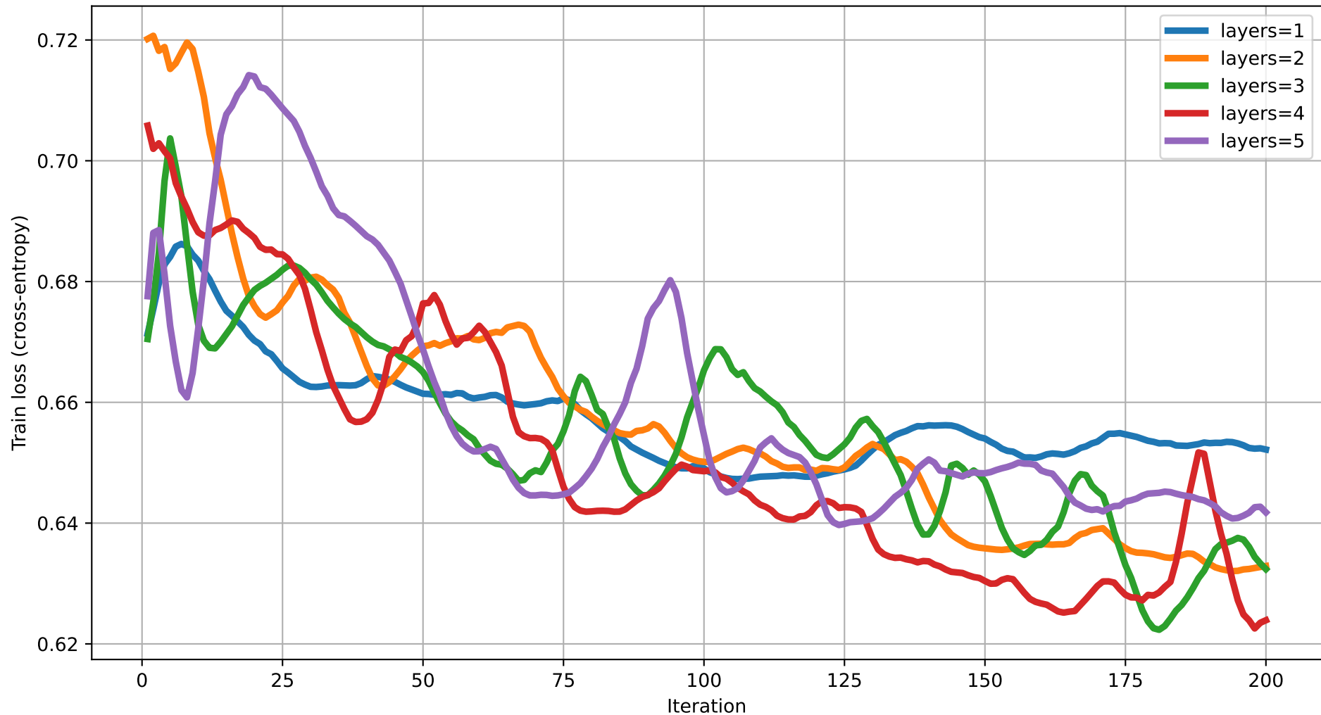
Train loss vs Iteration (dim=7) rot=RY, ent=full, gate=IsingXX
