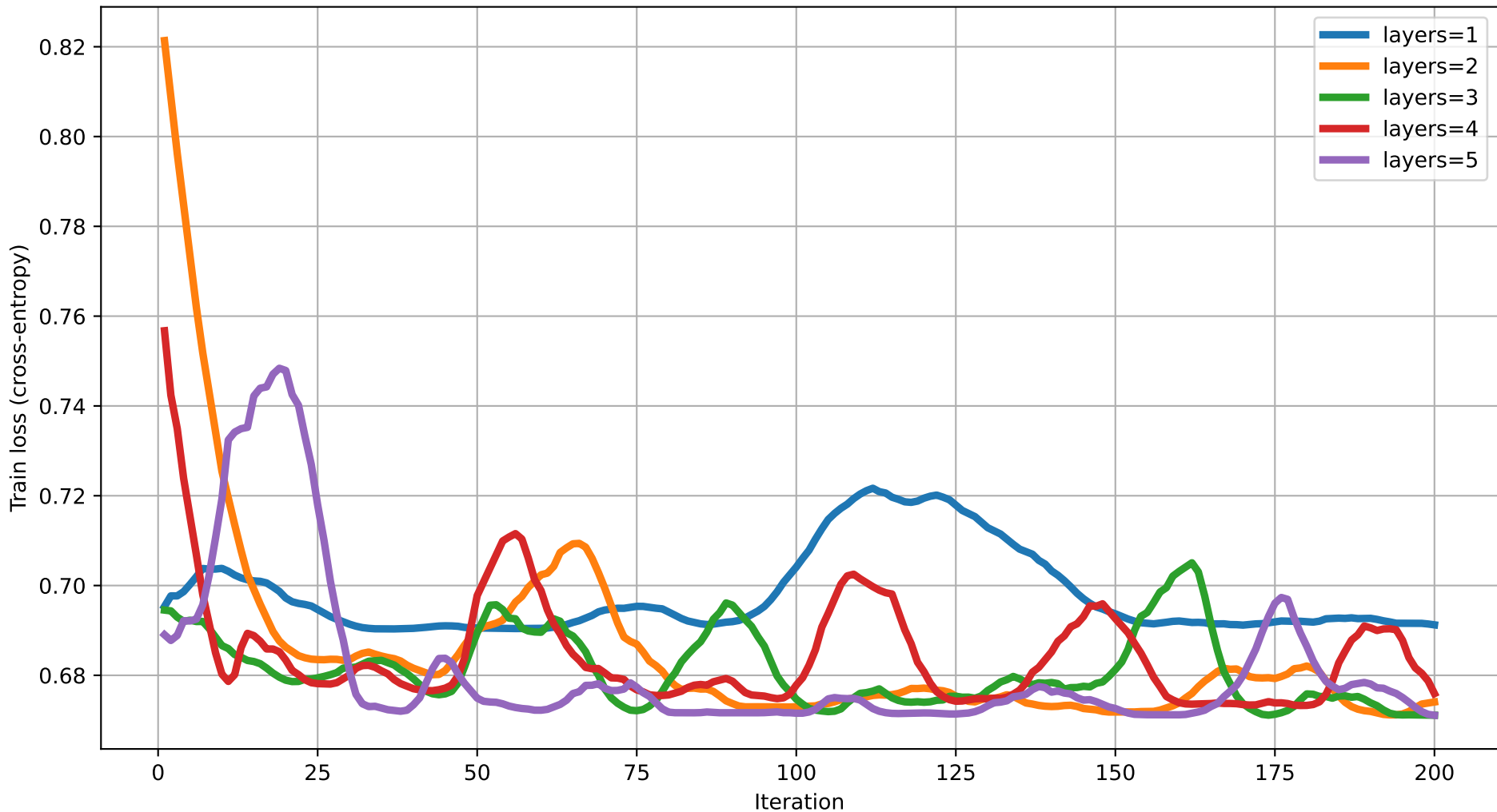
Train loss vs Iteration (dim=8) rot=RY, ent=pairwise, gate=IsingXX
