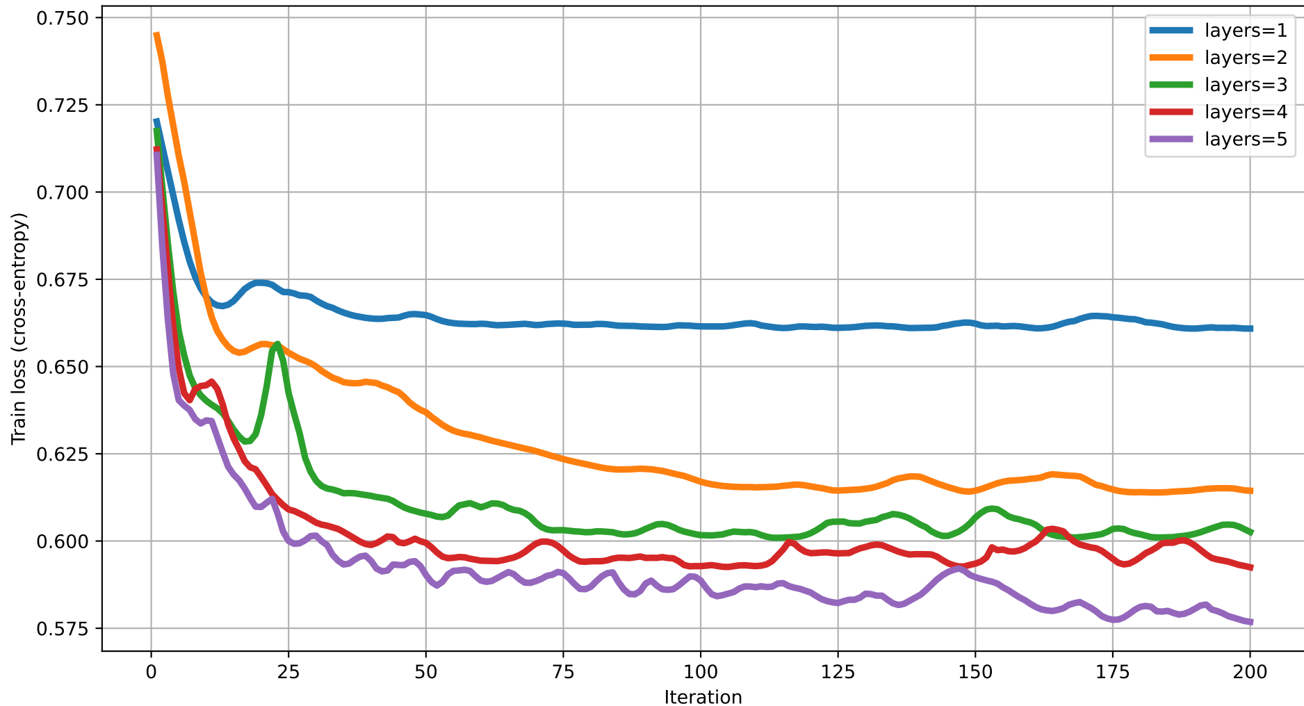
Train loss vs Iteration (degree=3) rot=Rot, ent=chain, gate=CNOT
