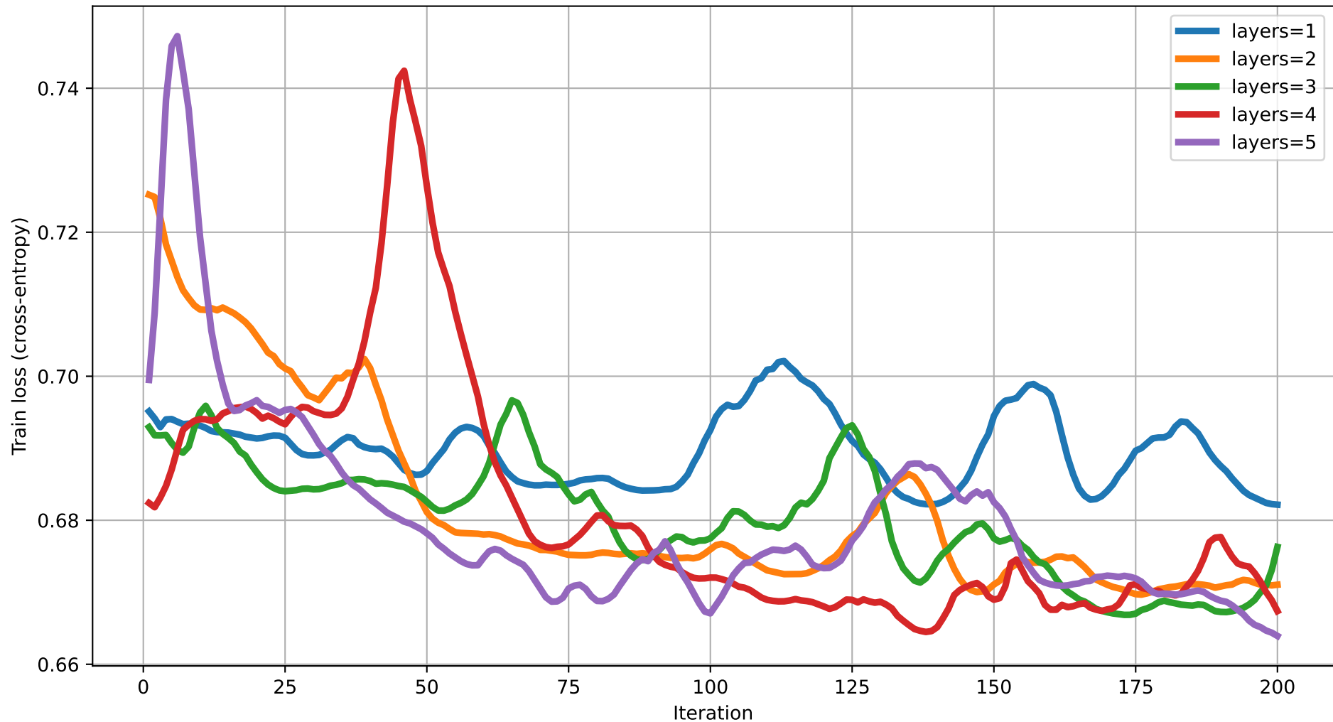
Train loss vs Iteration (dim=15) rot=RZ, ent=full, gate=IsingXX
