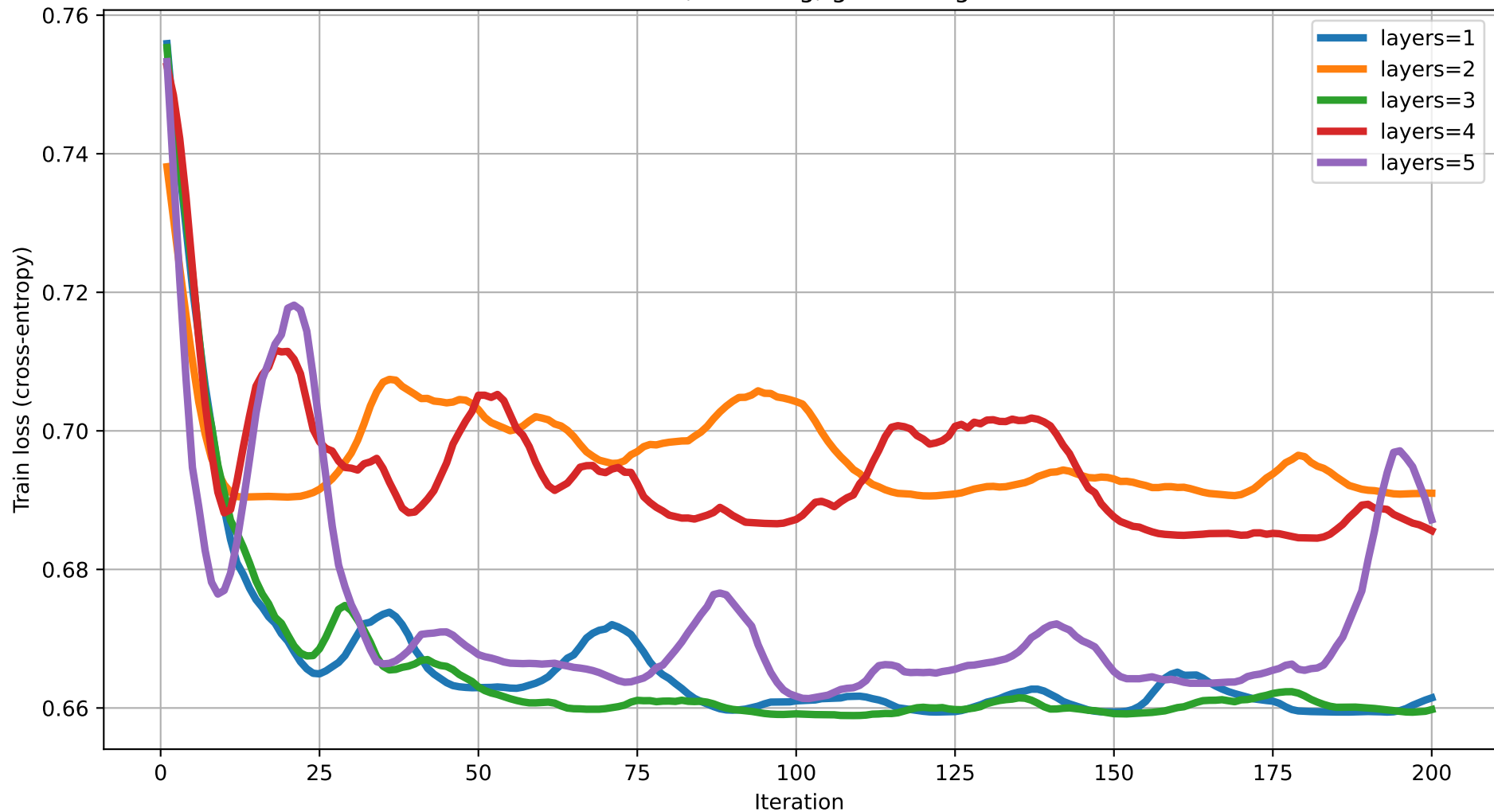
Train loss vs Iteration (dim=16) rot=RZ, ent=ring, gate=IsingXX
