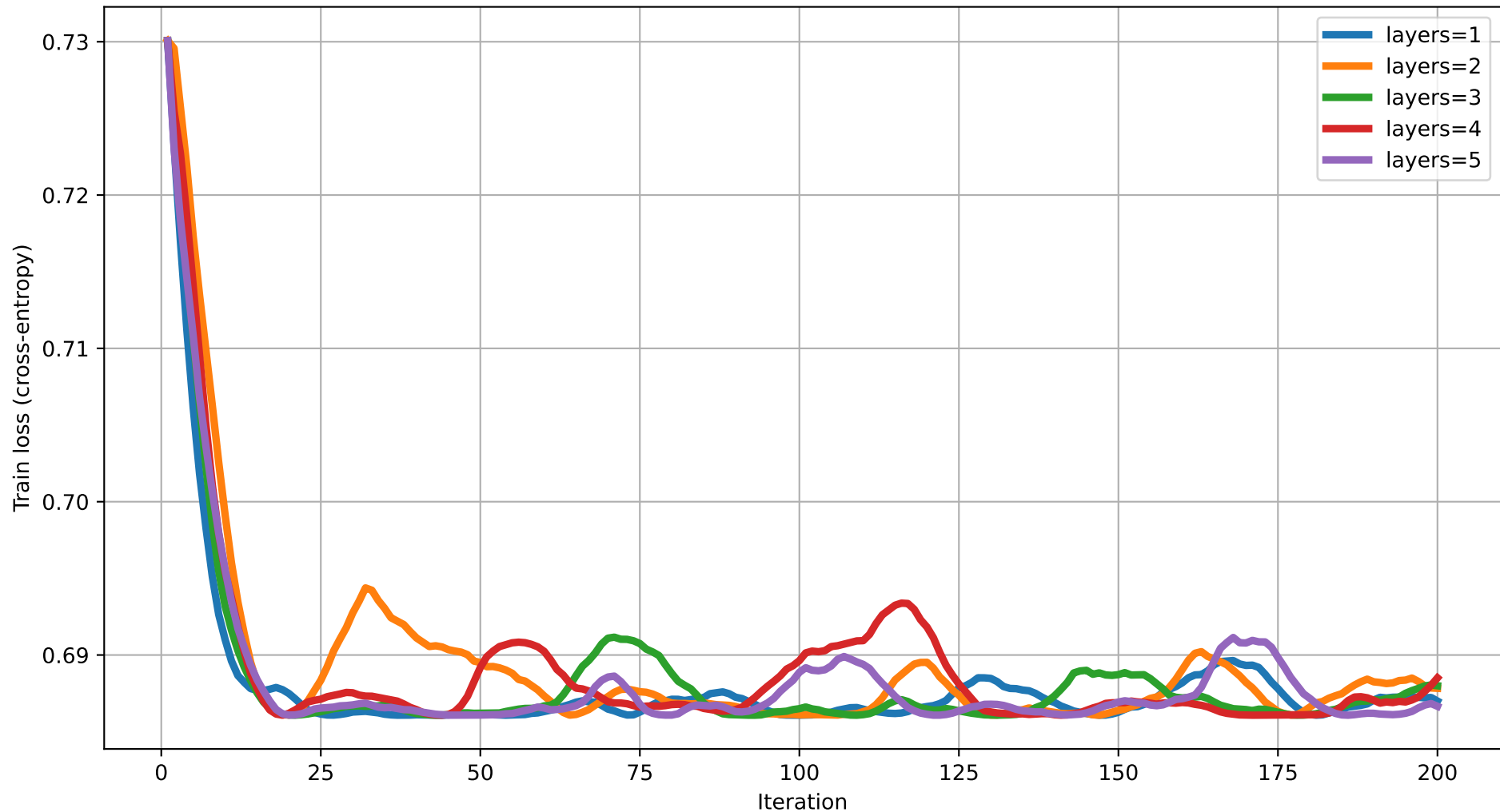
Train loss vs Iteration (degree=2) rot=RZ, ent=pairwise, gate=CZ
