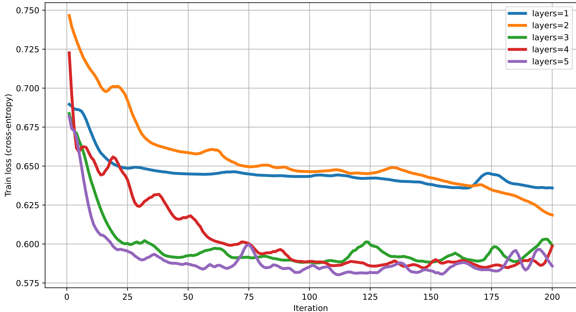
Train loss vs Iteration (degree=5) rot=RYZ, ent=chain, gate=IsingXX
