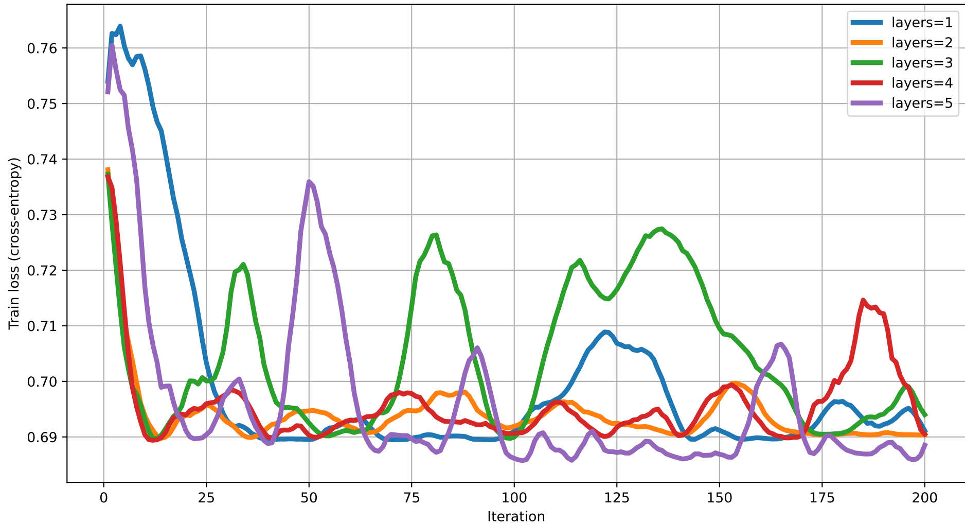
Train loss vs Iteration (dim=16) rot=RX, ent=chain, gate=CZ
