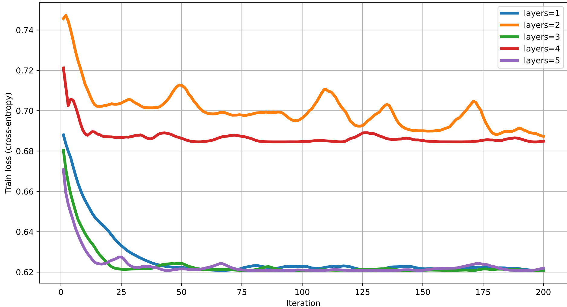
Train loss vs Iteration (degree=3) rot=RX, ent=chain, gate=IsingXX
