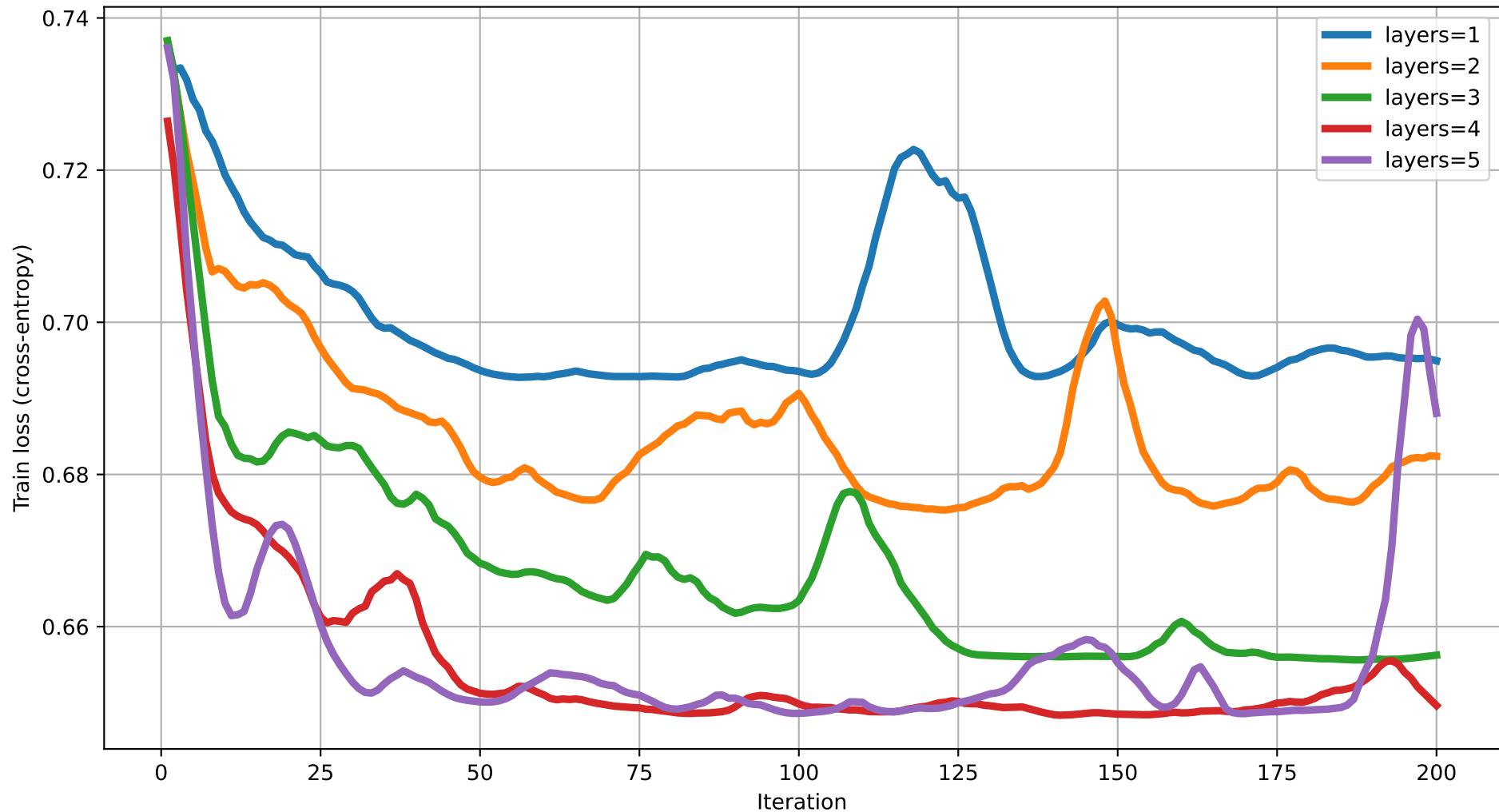
Train loss vs Iteration (dim=5) rot=RX, ent=full, gate=CNOT
