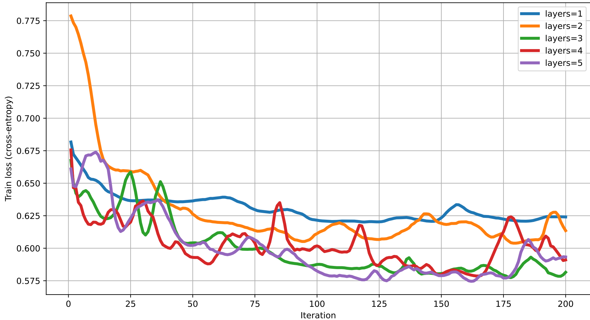
Train loss vs Iteration (dim=10) rot=Rot, ent=chain, gate=IsingXX
