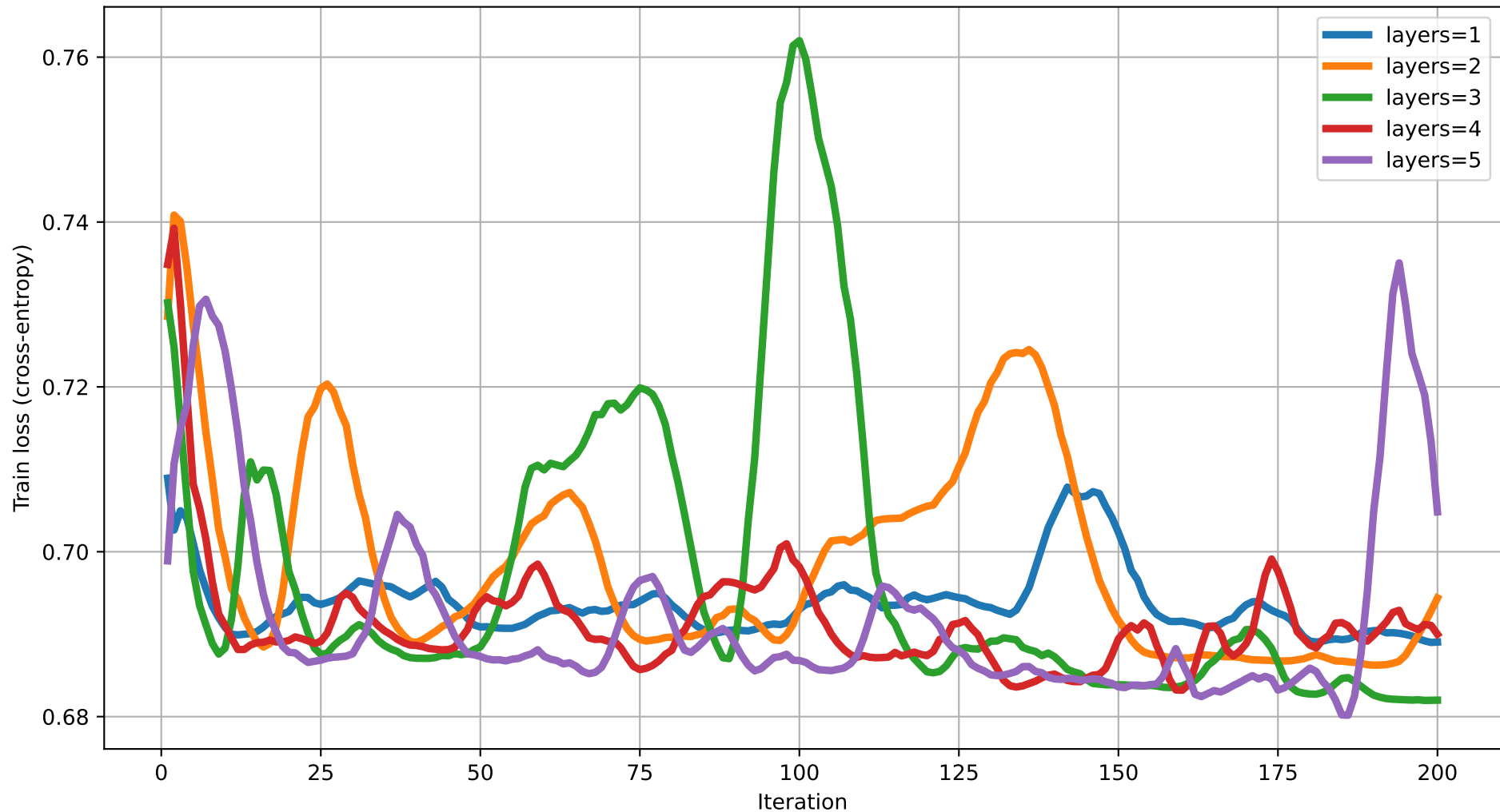
Train loss vs Iteration (dim=20) rot=RYZ, ent=pairwise, gate=CNOT
