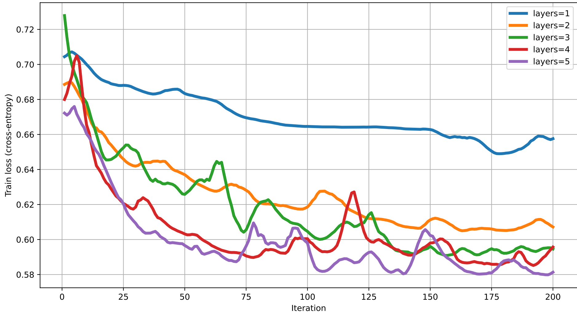
Train loss vs Iteration (dim=13) rot=Rot, ent=ring, gate=CNOT
