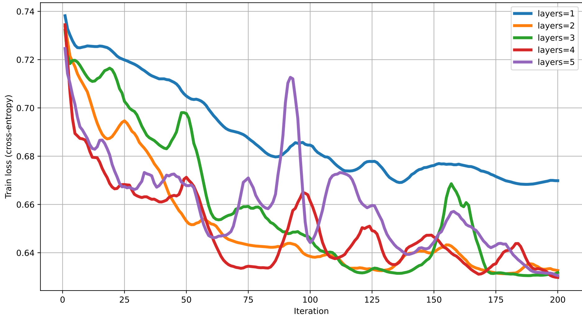
Train loss vs Iteration (dim=3) rot=RY, ent=full, gate=CZ
