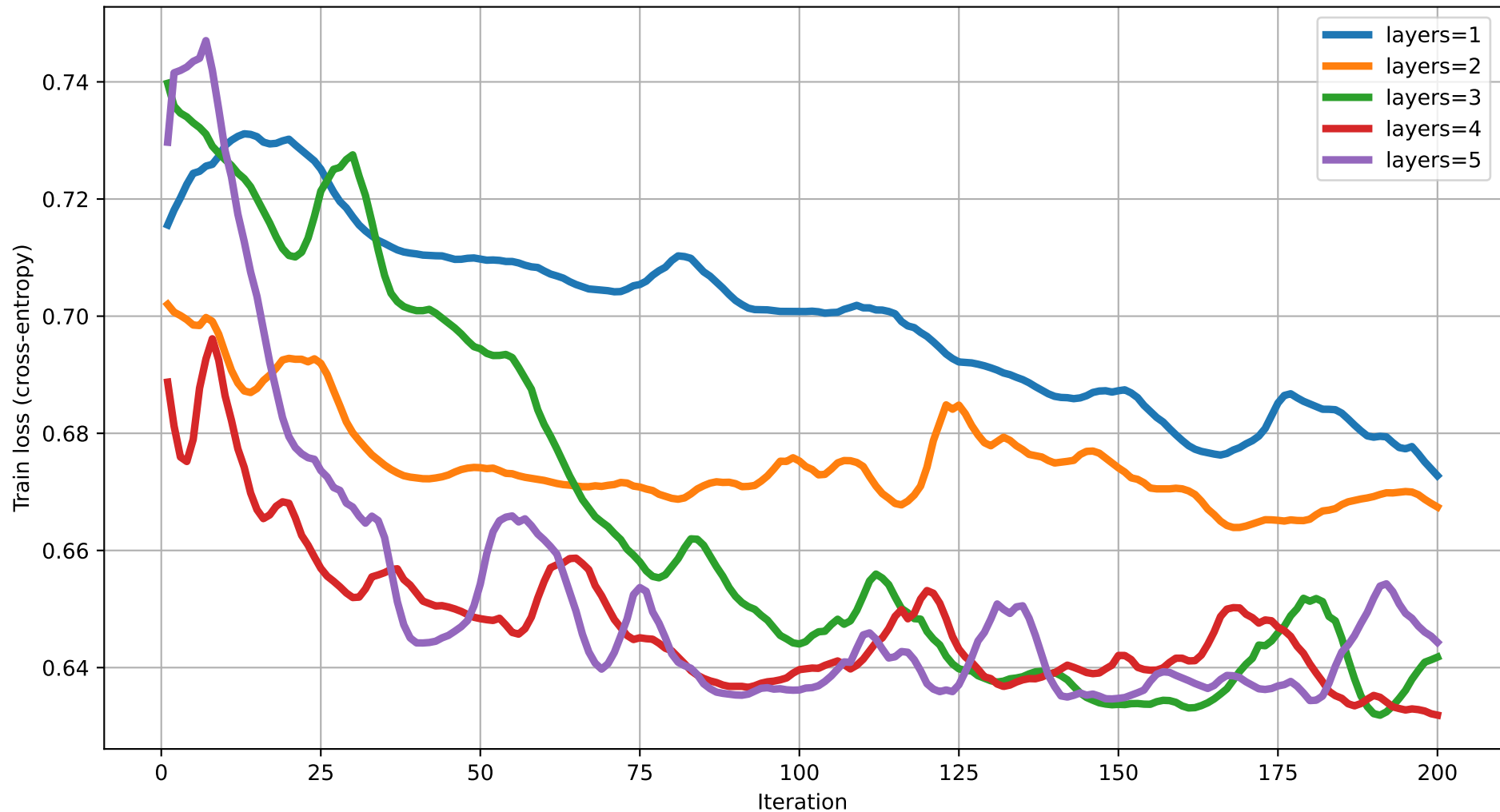
Train loss vs Iteration (dim=5) rot=RYZ, ent=ring, gate=CNOT
