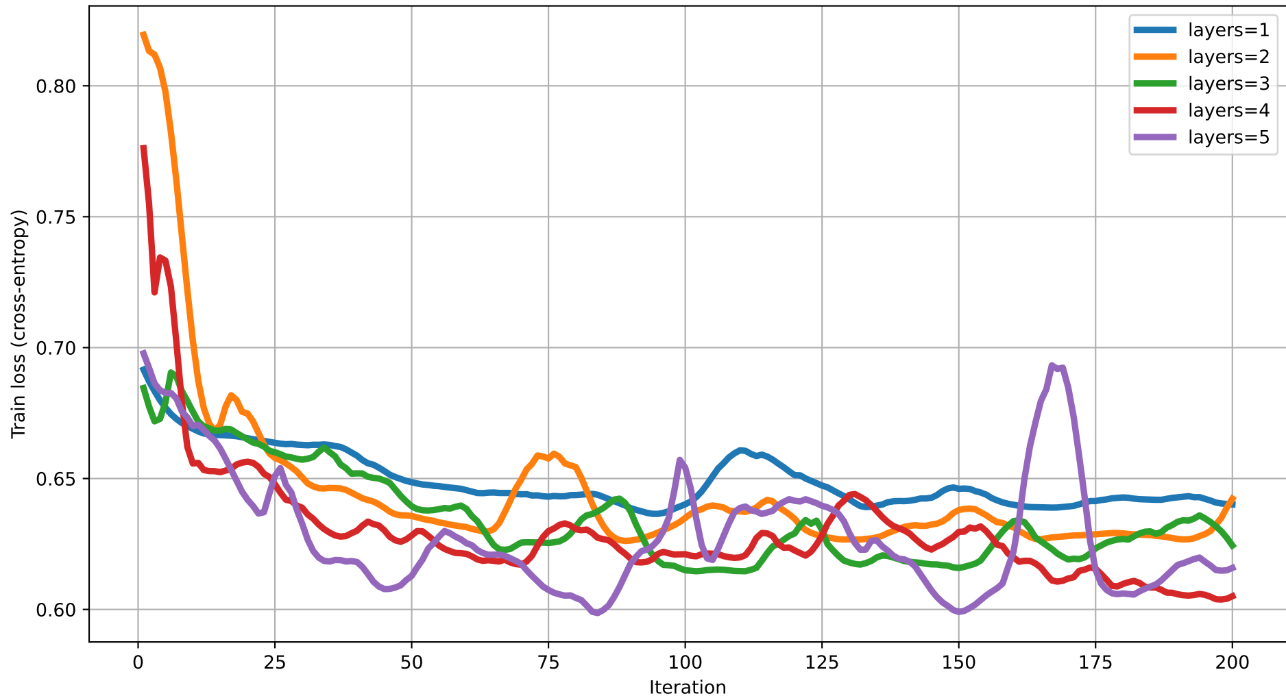
Train loss vs Iteration (dim=8) rot=Rot, ent=chain, gate=IsingXX
