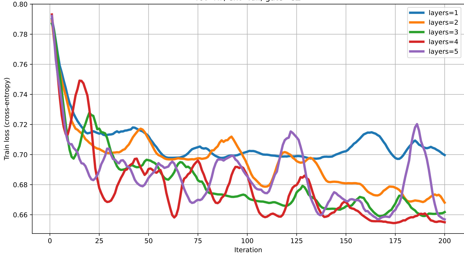
Train loss vs Iteration (dim=2) rot=RY, ent=full, gate=CZ
