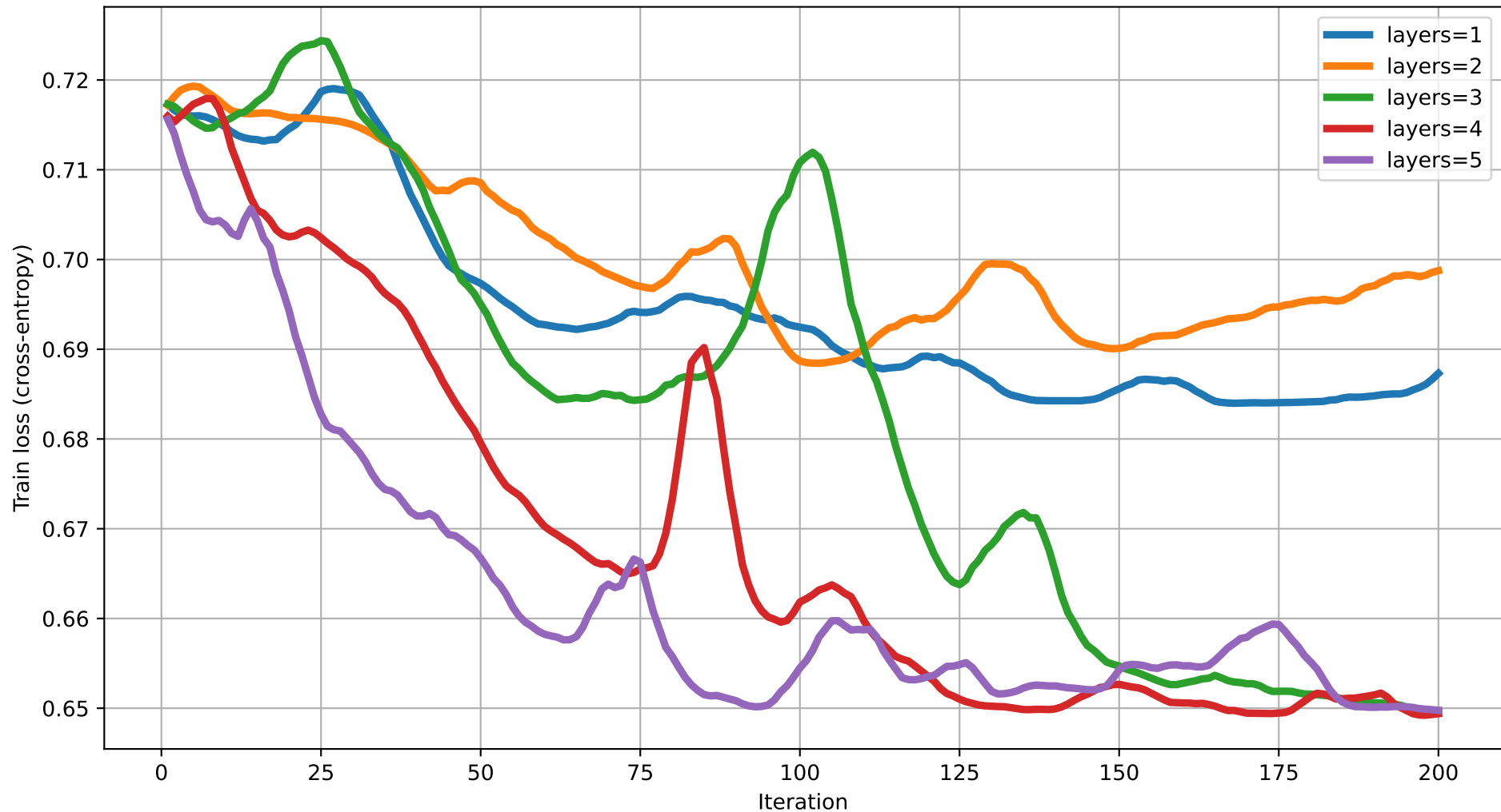
Train loss vs Iteration (dim=7) rot=RX, ent=pairwise, gate=CZ
