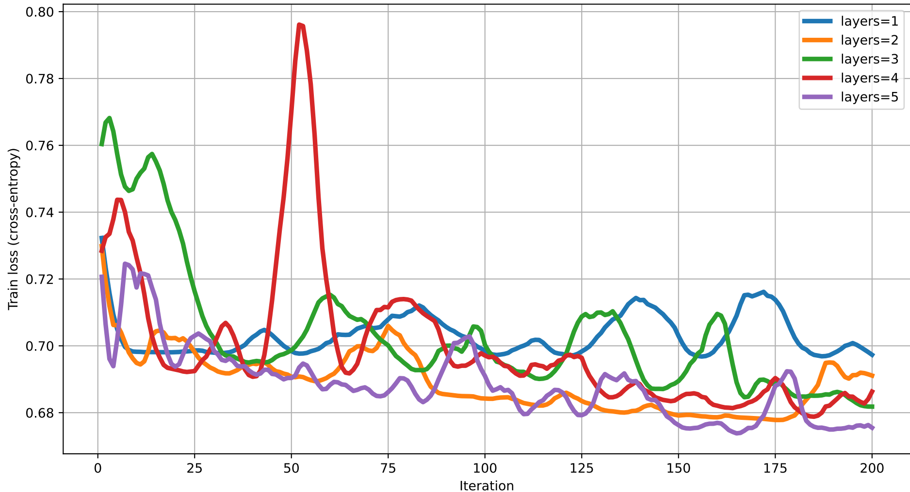
Train loss vs Iteration (dim=19) rot=RYZ, ent=pairwise, gate=CNOT
