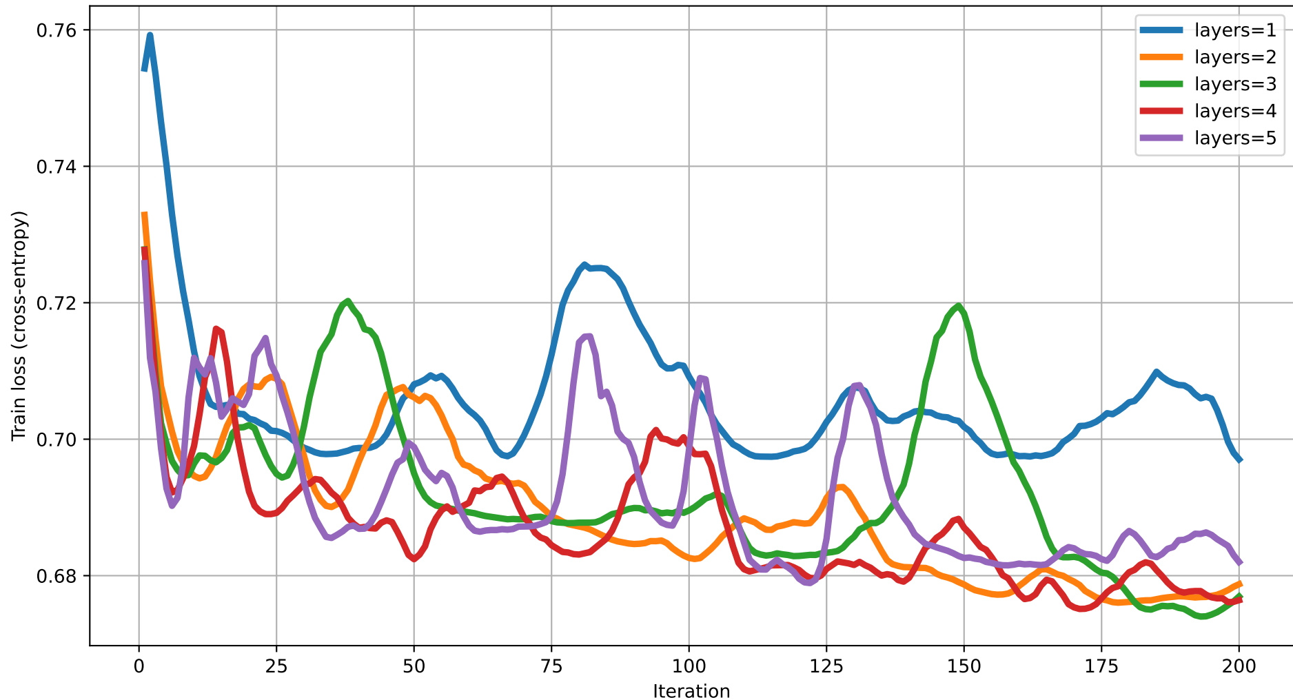
Train loss vs Iteration (dim=19) rot=RYZ, ent=full, gate=CZ
