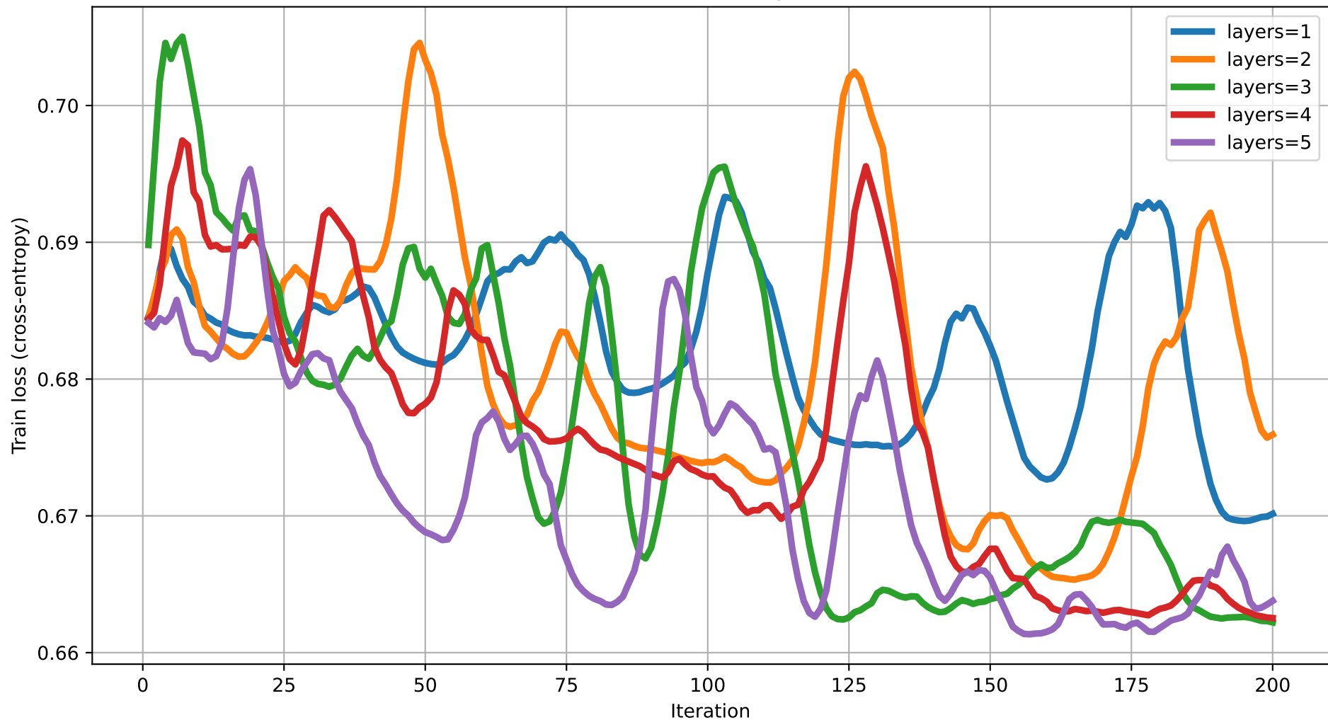
Train loss vs Iteration (dim=15) rot=RY, ent=chain, gate=CZ
