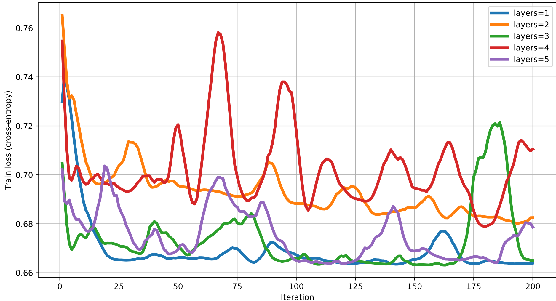
Train loss vs Iteration (dim=17) rot=RY, ent=ring, gate=IsingXX
