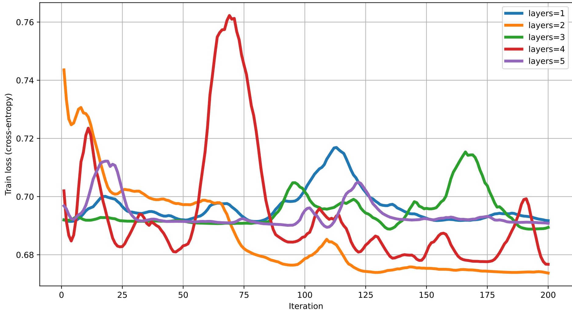
Train loss vs Iteration (dim=20) rot=RY, ent=chain, gate=IsingXX
