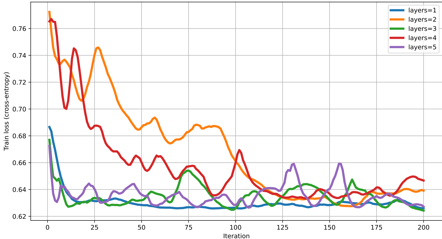
Train loss vs Iteration (dim=4) rot=RYZ, ent=ring, gate=IsingXX
