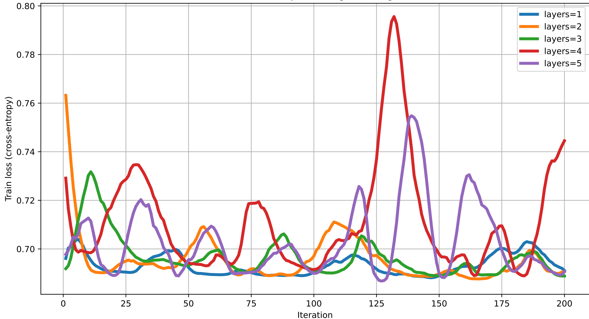
Train loss vs Iteration (dim=18) rot=RZ, ent=pairwise, gate=IsingXX
