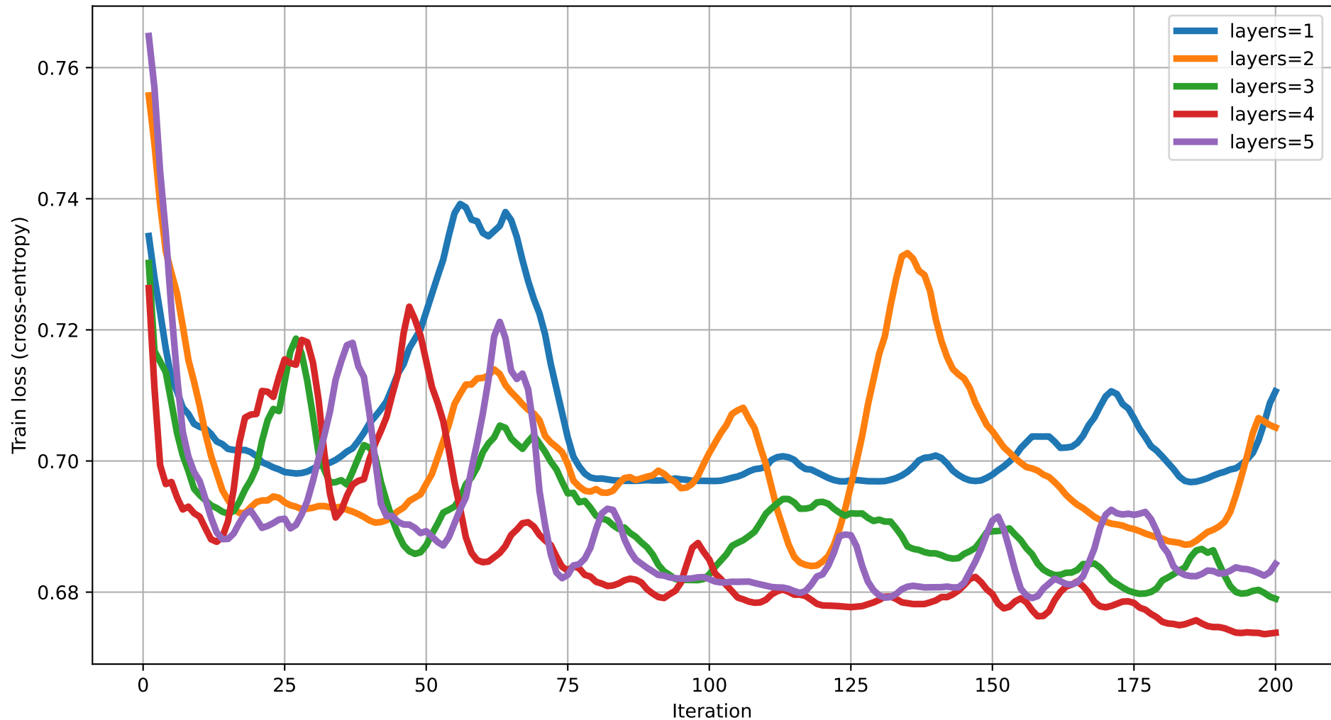
Train loss vs Iteration (dim=19) rot=Rot, ent=chain, gate=CZ
