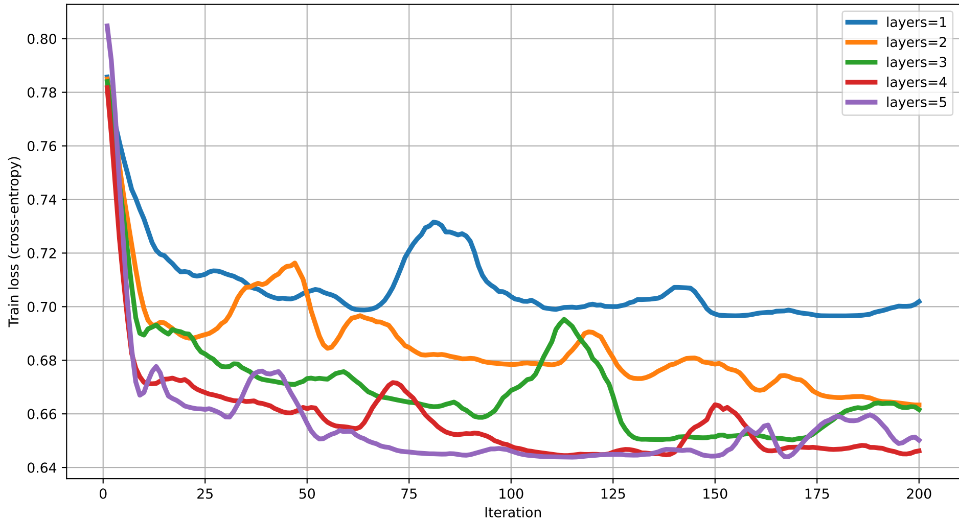
Train loss vs Iteration (dim=9) rot=RX, ent=full, gate=CNOT
