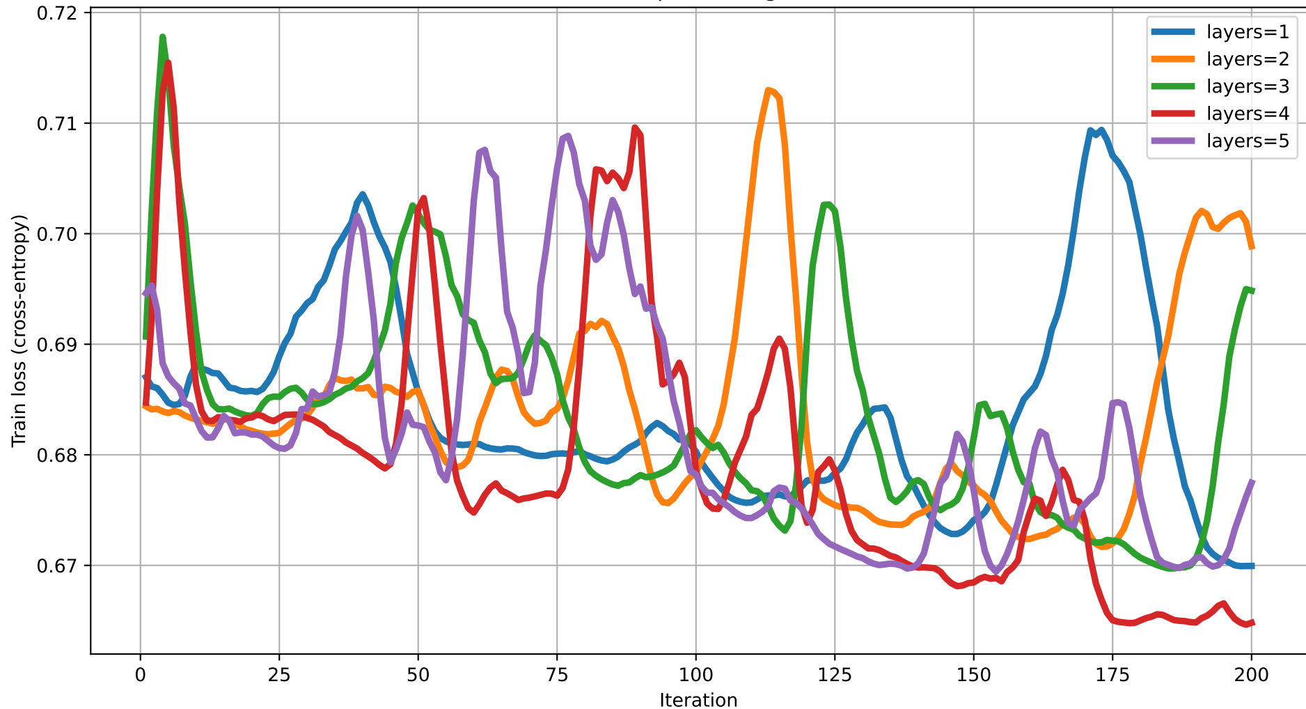
Train loss vs Iteration (dim=15) rot=Rot, ent=pairwise, gate=CNOT
