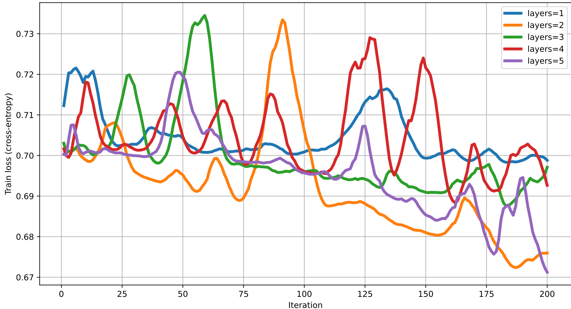
Train loss vs Iteration (dim=12) rot=RYZ, ent=chain, gate=CZ
