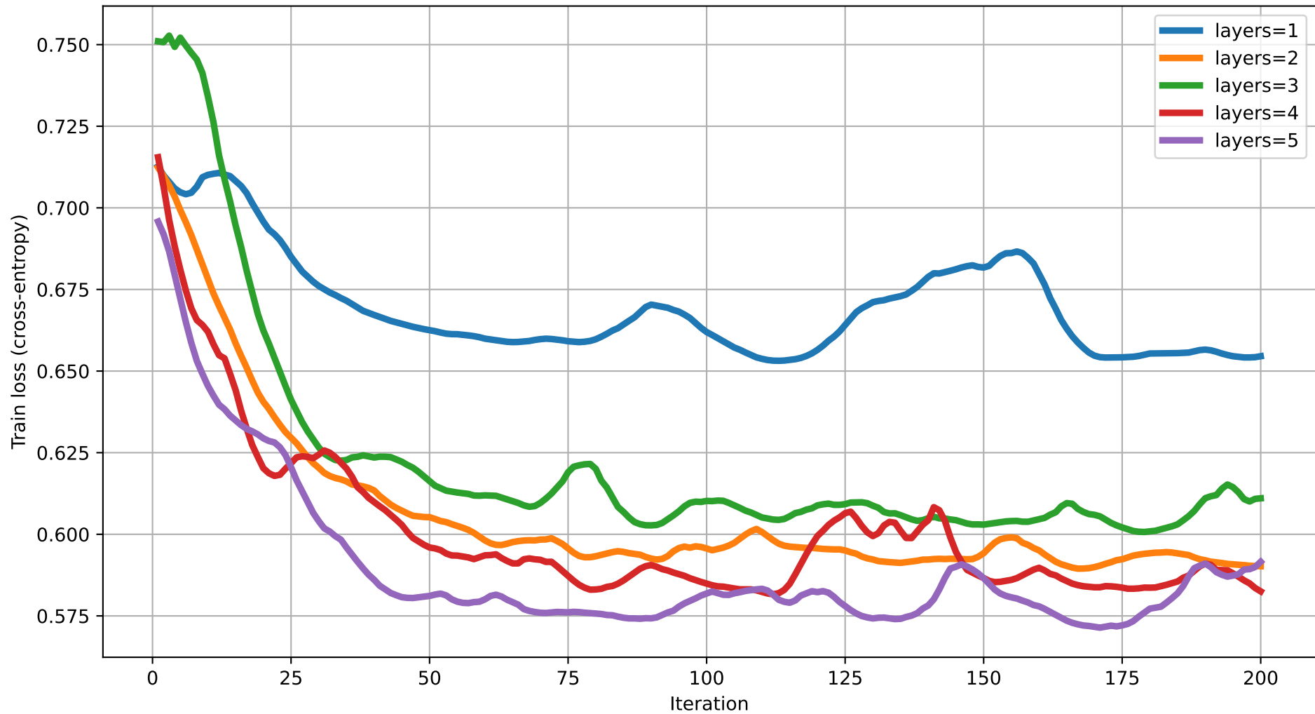
Train loss vs Iteration (dim=10) rot=RY, ent=ring, gate=CNOT
