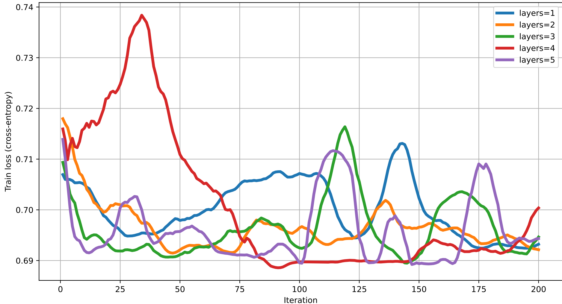
Train loss vs Iteration (dim=4) rot=RX, ent=ring, gate=CNOT
