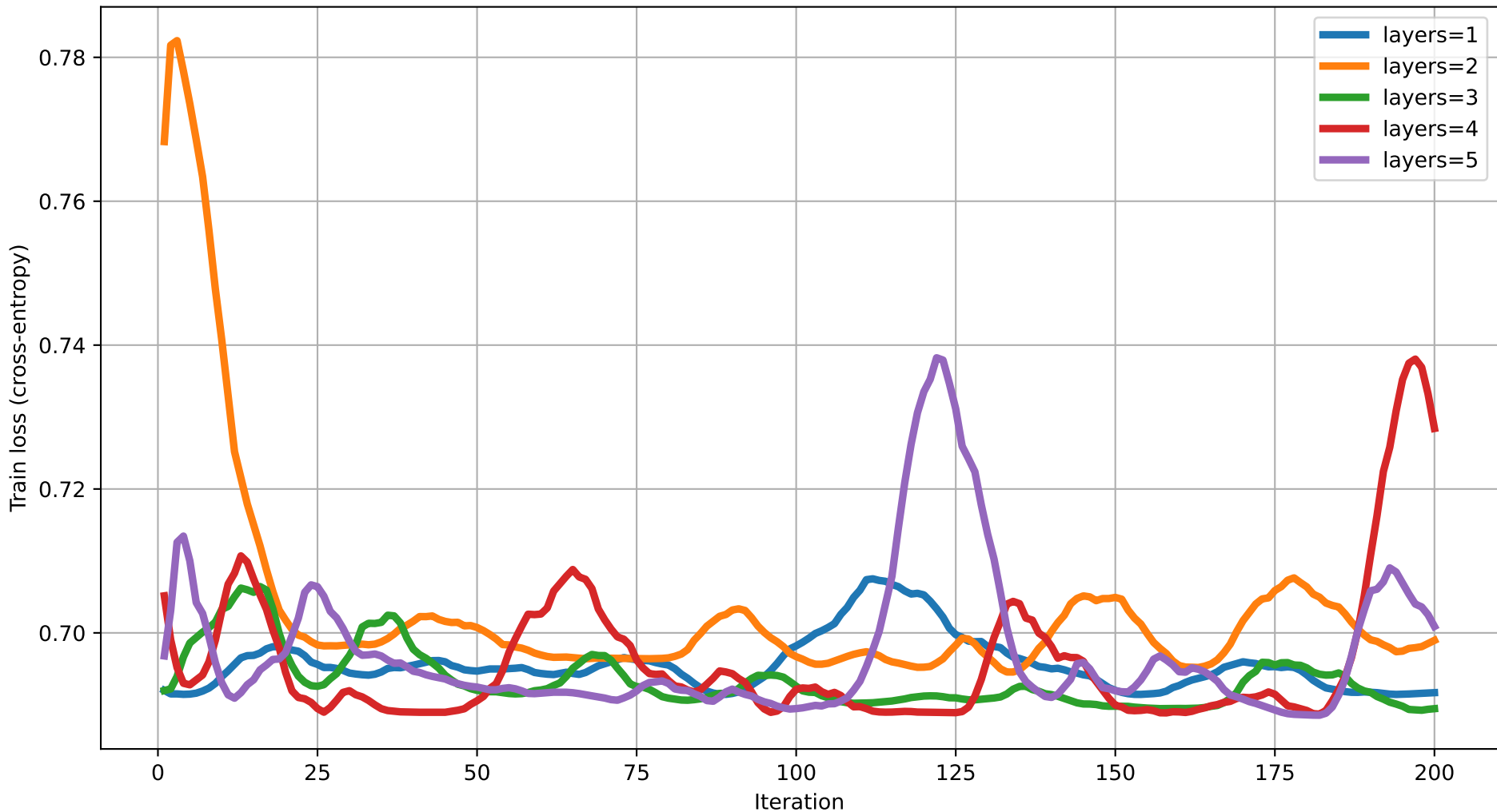
Train loss vs Iteration (dim=20) rot=RY, ent=pairwise, gate=IsingXX
