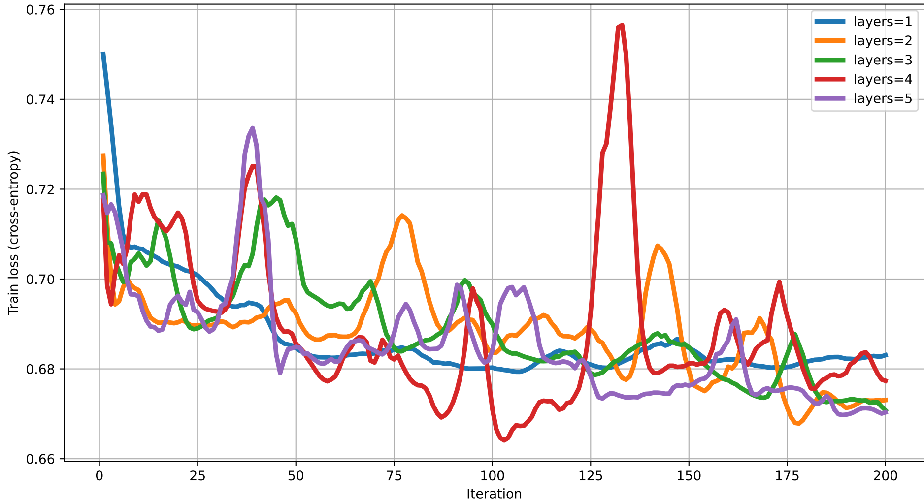
Train loss vs Iteration (dim=18) rot=Rot, ent=full, gate=IsingXX
