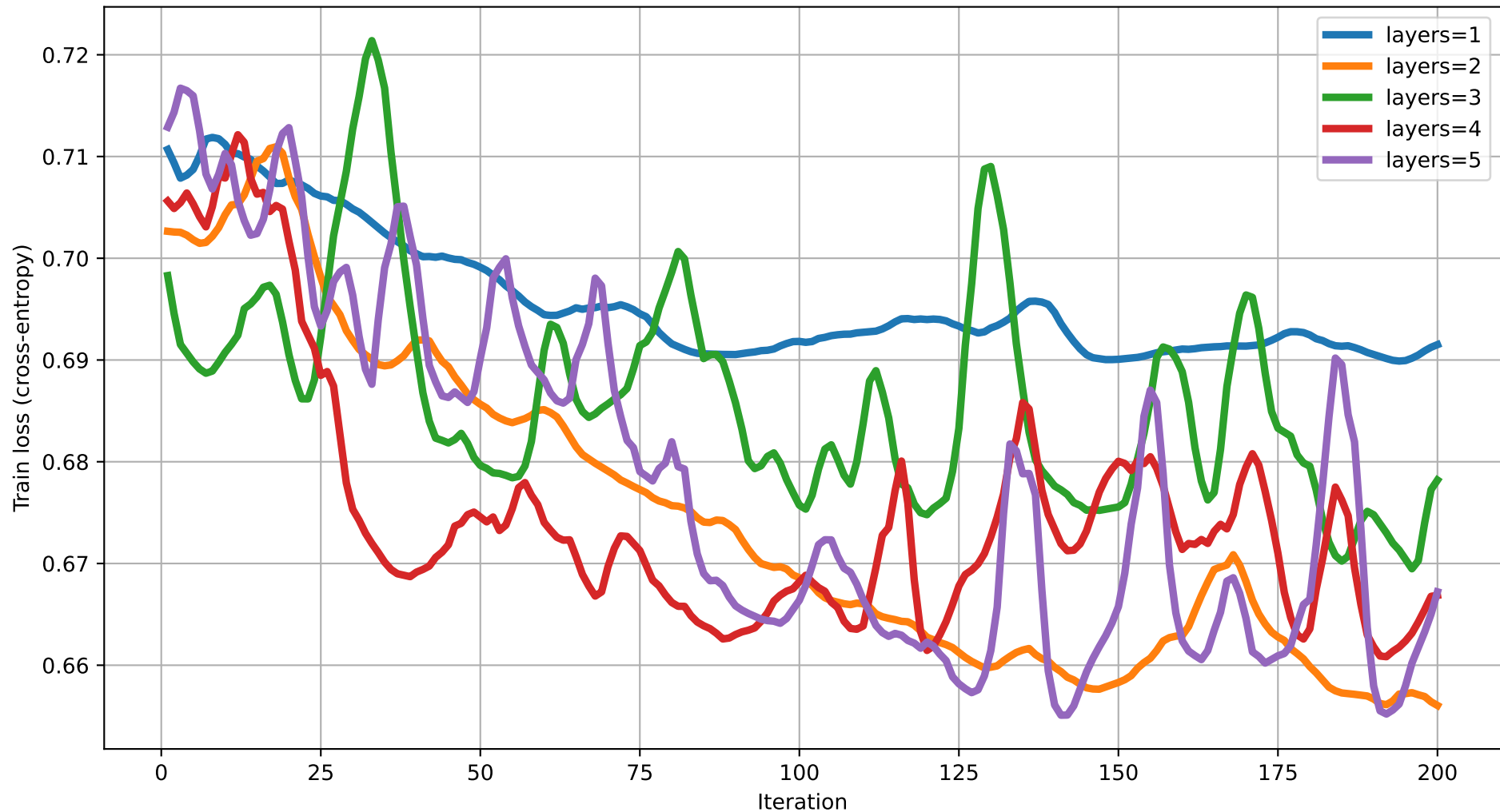
Train loss vs Iteration (dim=10) rot=Rot, ent=ring, gate=CNOT
