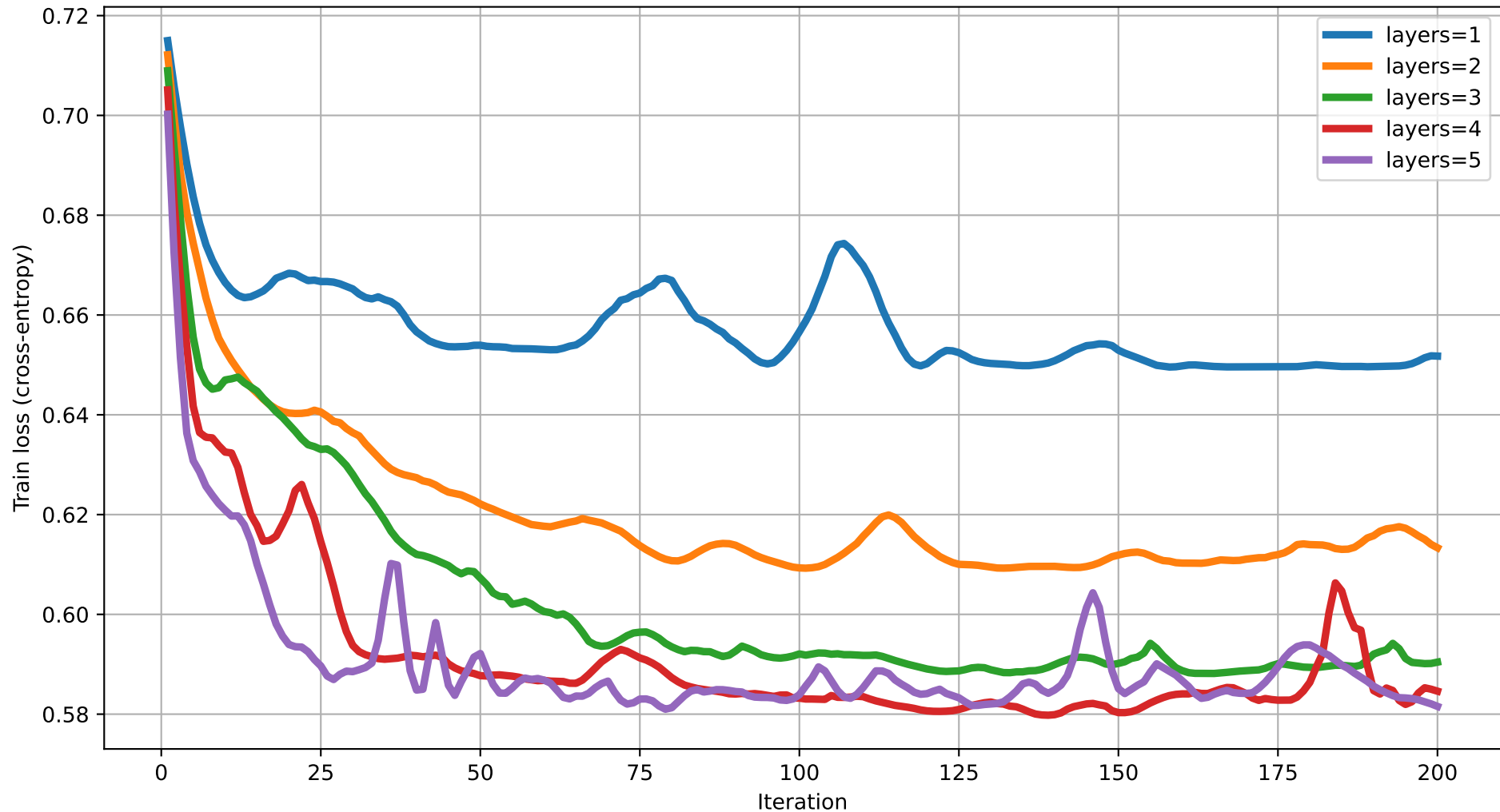
Train loss vs Iteration (degree=4) rot=Rot, ent=chain, gate=CNOT
