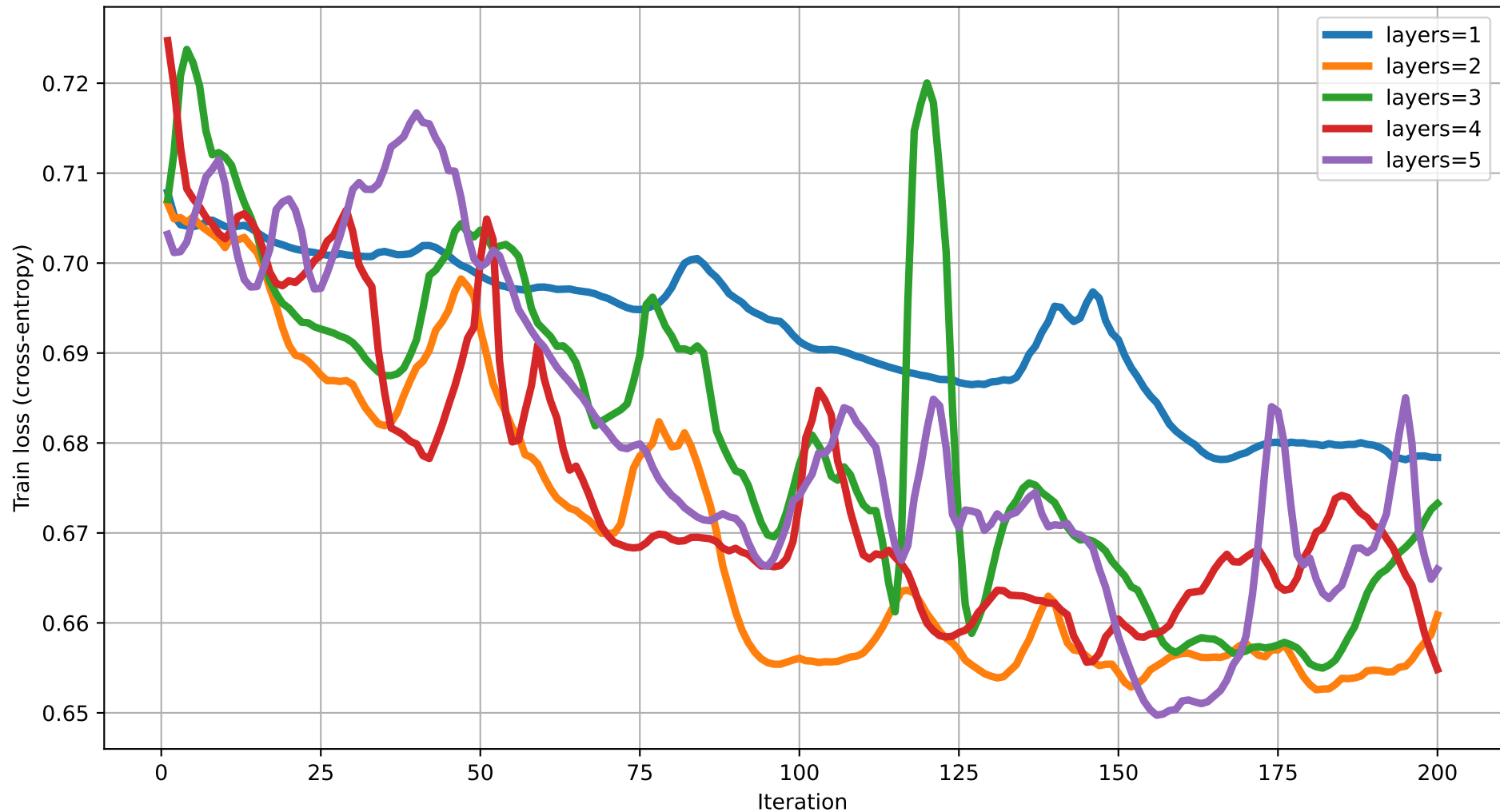
Train loss vs Iteration (dim=6) rot=Rot, ent=chain, gate=CNOT
