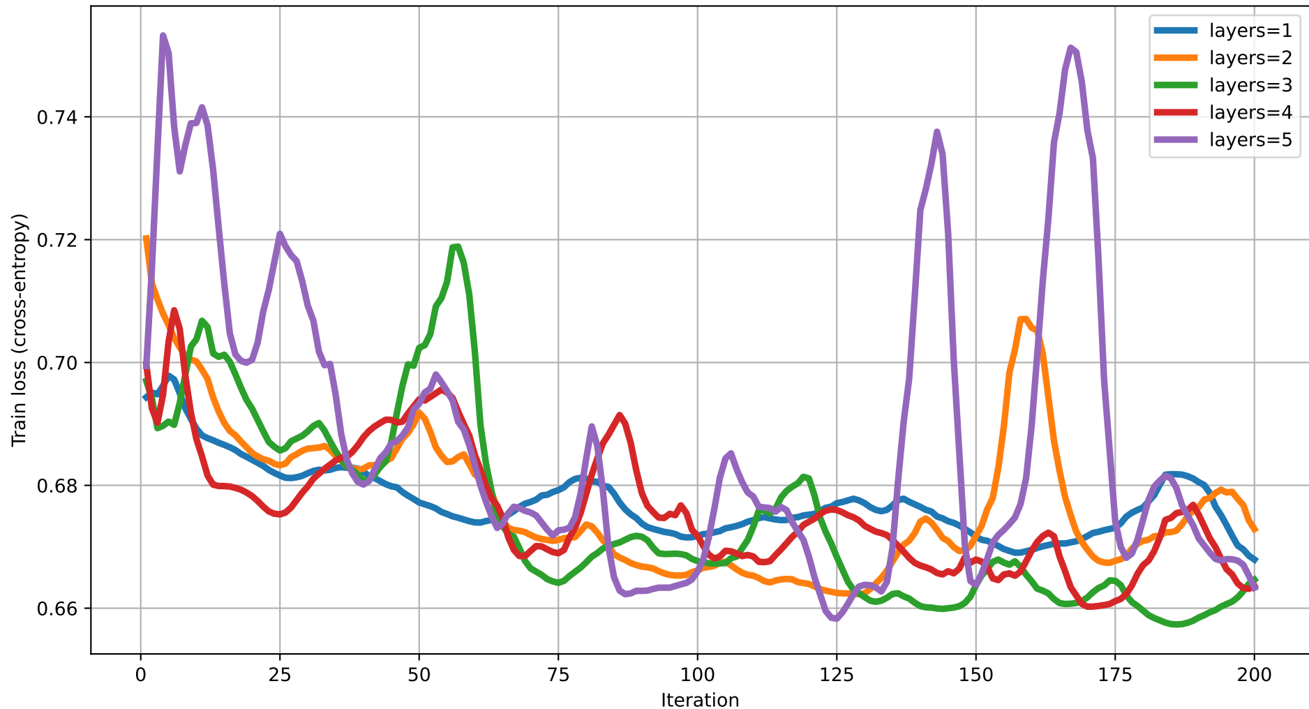
Train loss vs Iteration (dim=11) rot=RYZ, ent=full, gate=IsingXX
