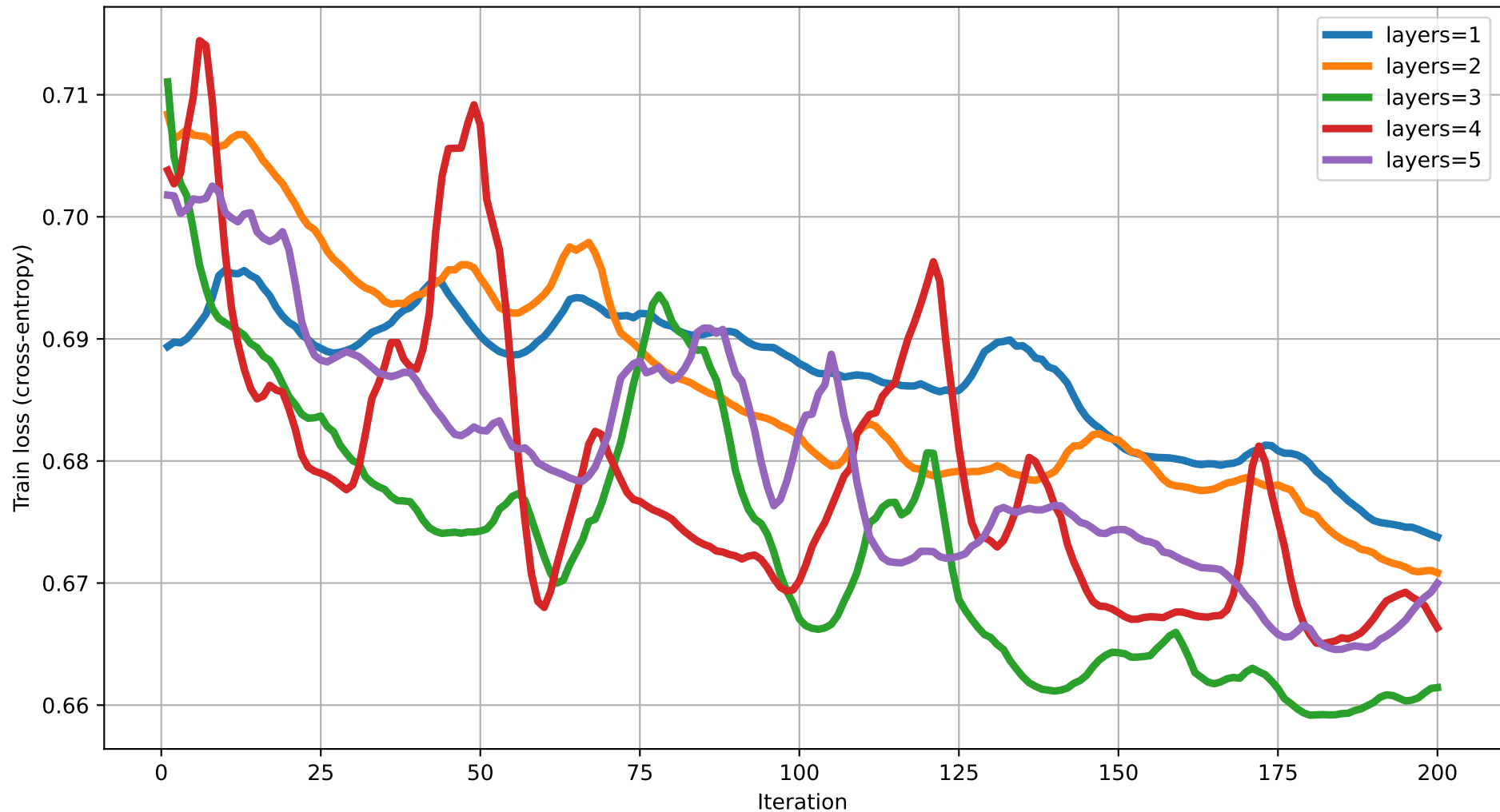
Train loss vs Iteration (dim=13) rot=RY, ent=ring, gate=CNOT
