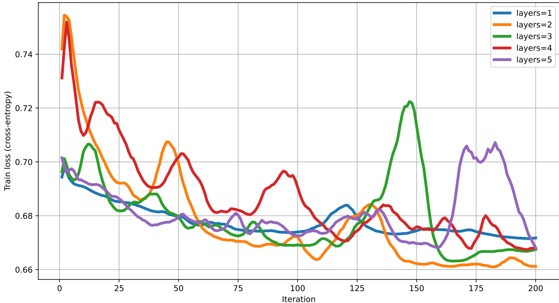
Train loss vs Iteration (dim=11) rot=RZ, ent=full, gate=IsingXX
