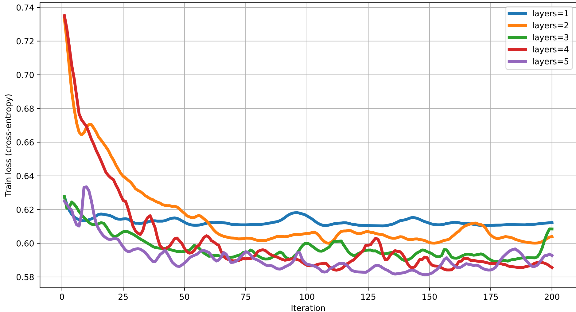
Train loss vs Iteration (degree=5) rot=Rot, ent=ring, gate=IsingXX
