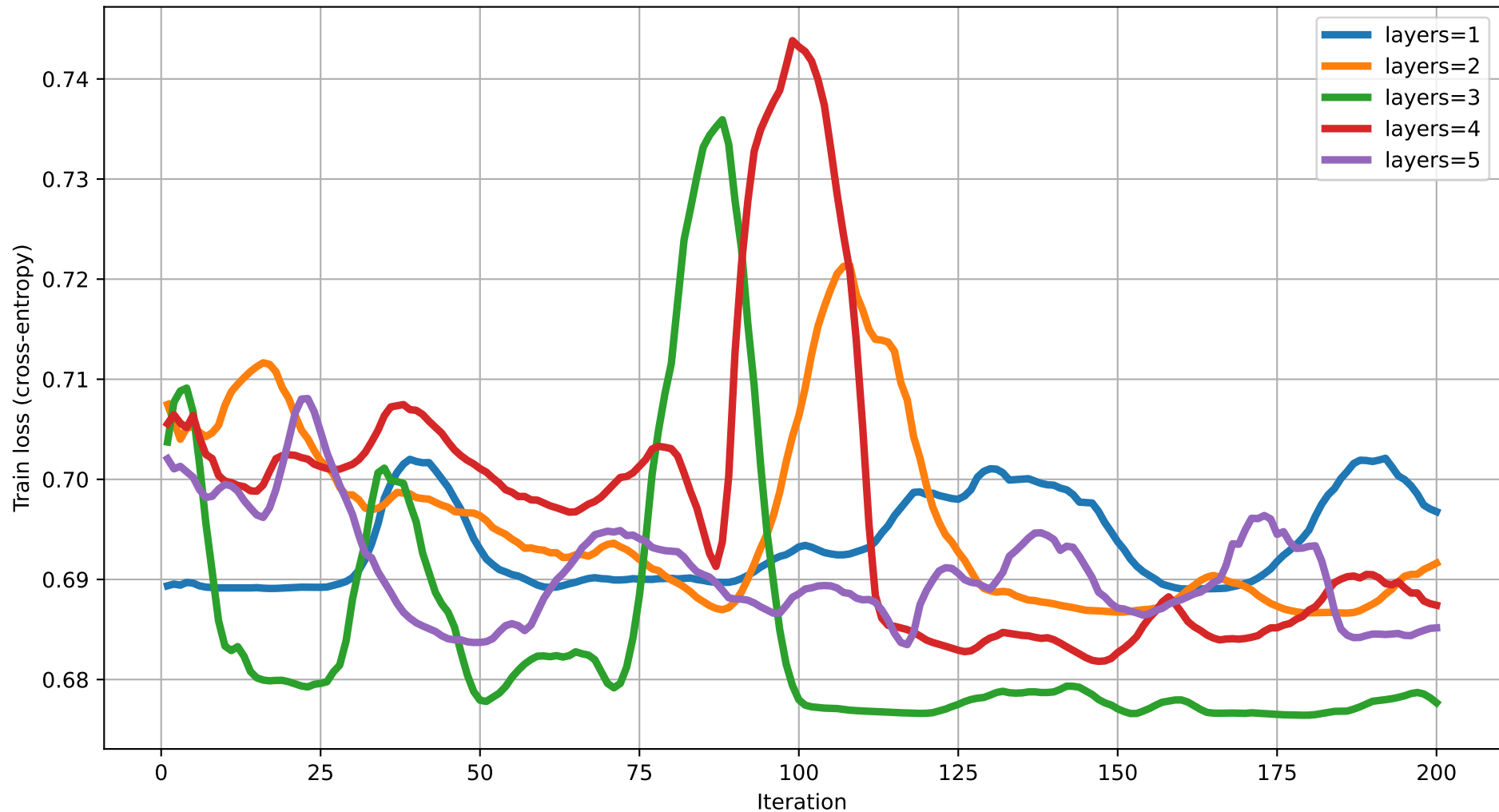
Train loss vs Iteration (dim=13) rot=RX, ent=ring, gate=CNOT
