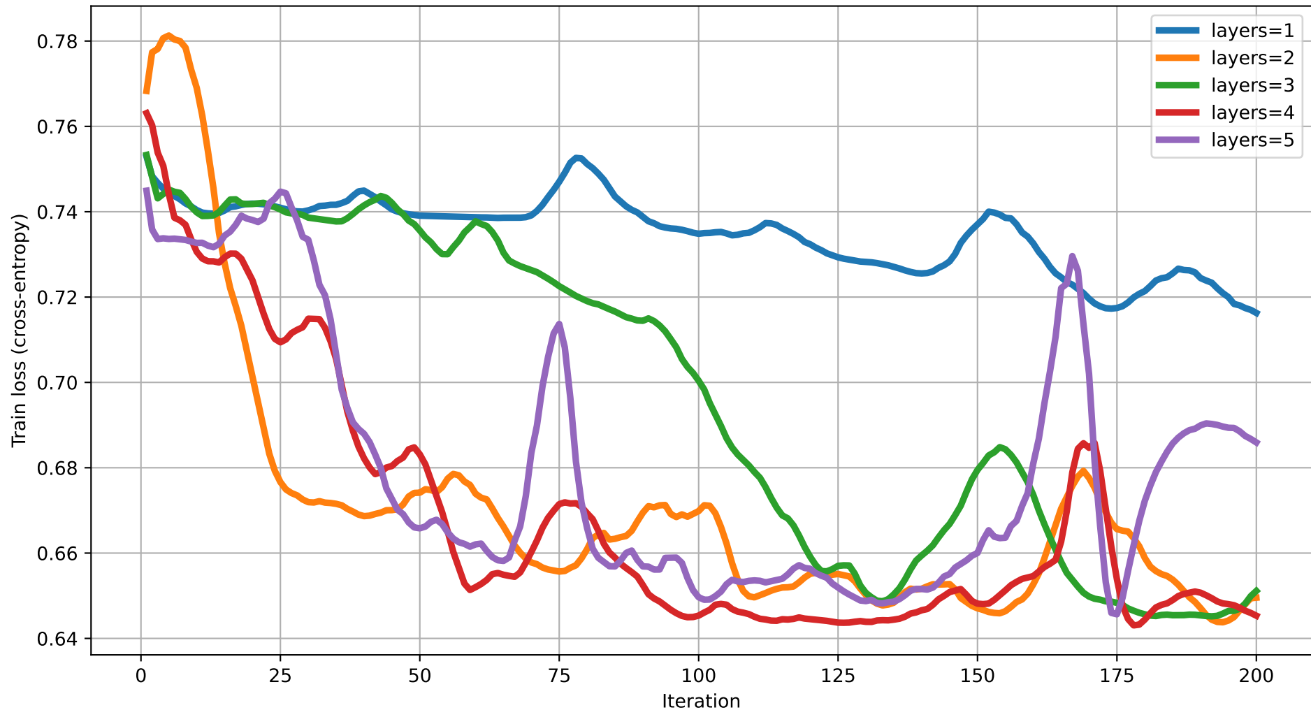
Train loss vs Iteration (dim=5) rot=RYZ, ent=pairwise, gate=CNOT
