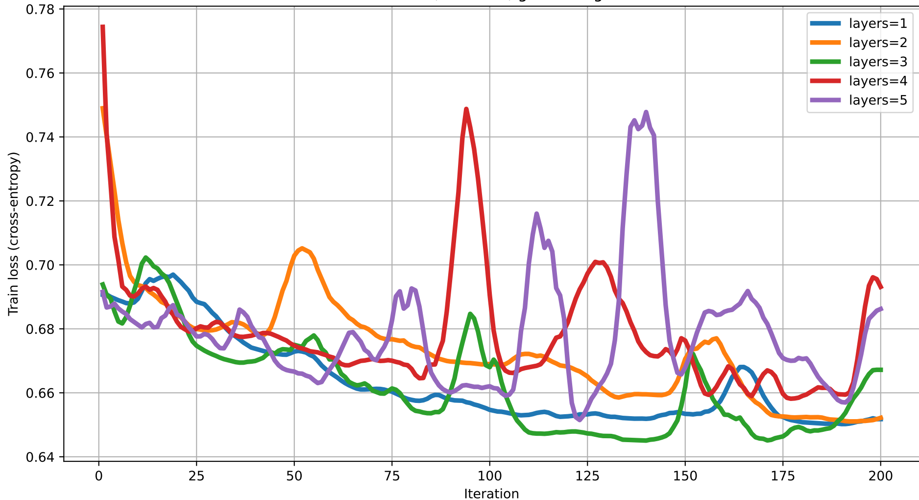
Train loss vs Iteration (dim=9) rot=RYZ, ent=full, gate=IsingXX
