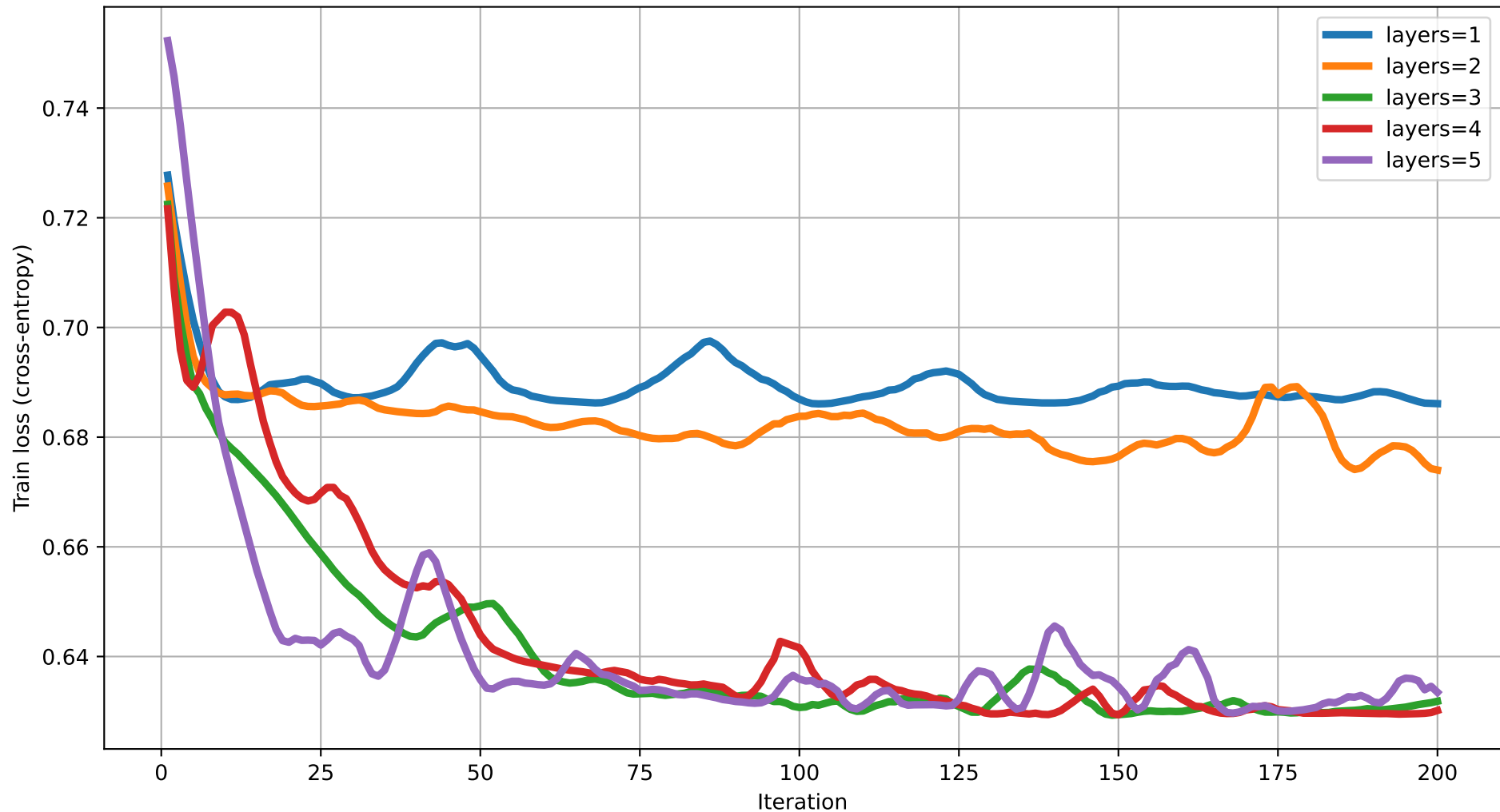
Train loss vs Iteration (degree=2) rot=RY, ent=pairwise, gate=CNOT
