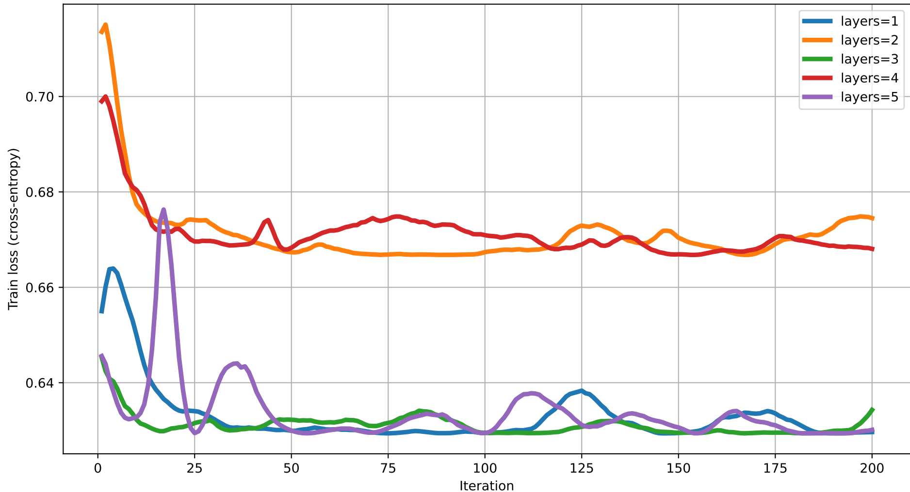
Train loss vs Iteration (dim=10) rot=RX, ent=ring, gate=IsingXX
