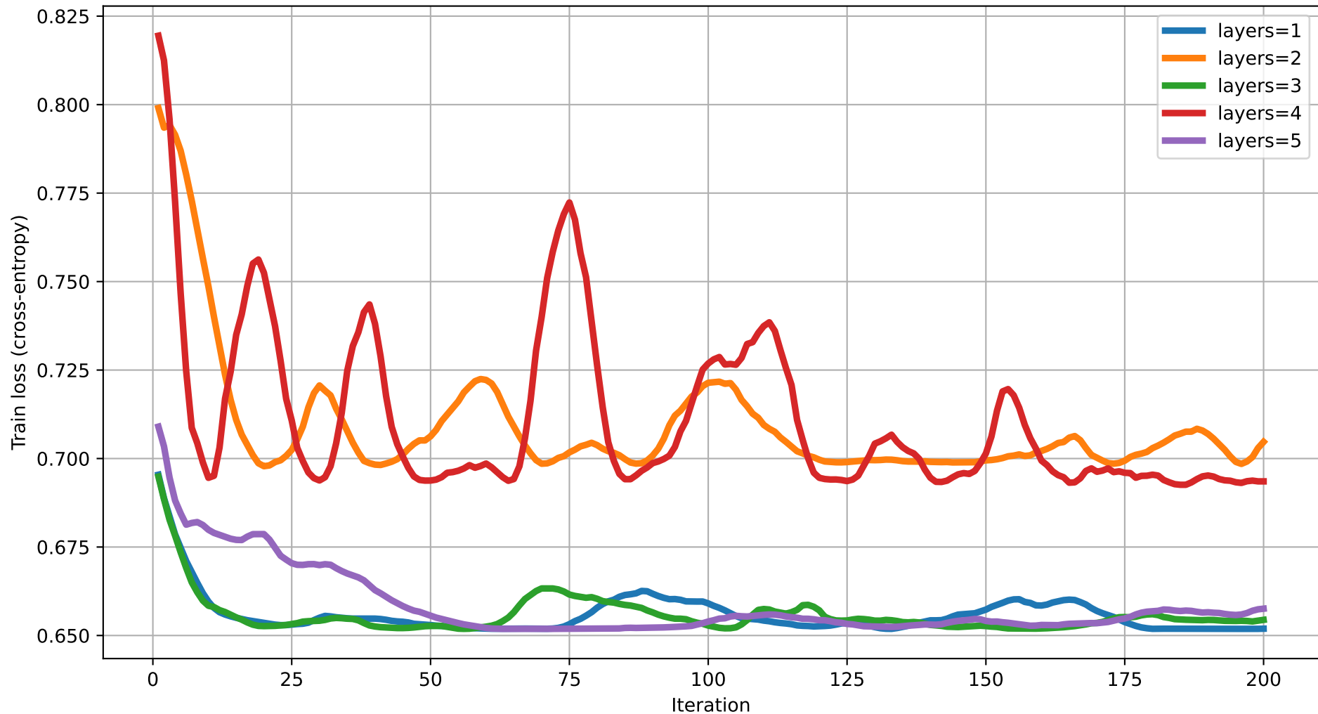
Train loss vs Iteration (dim=8) rot=RX, ent=ring, gate=IsingXX
