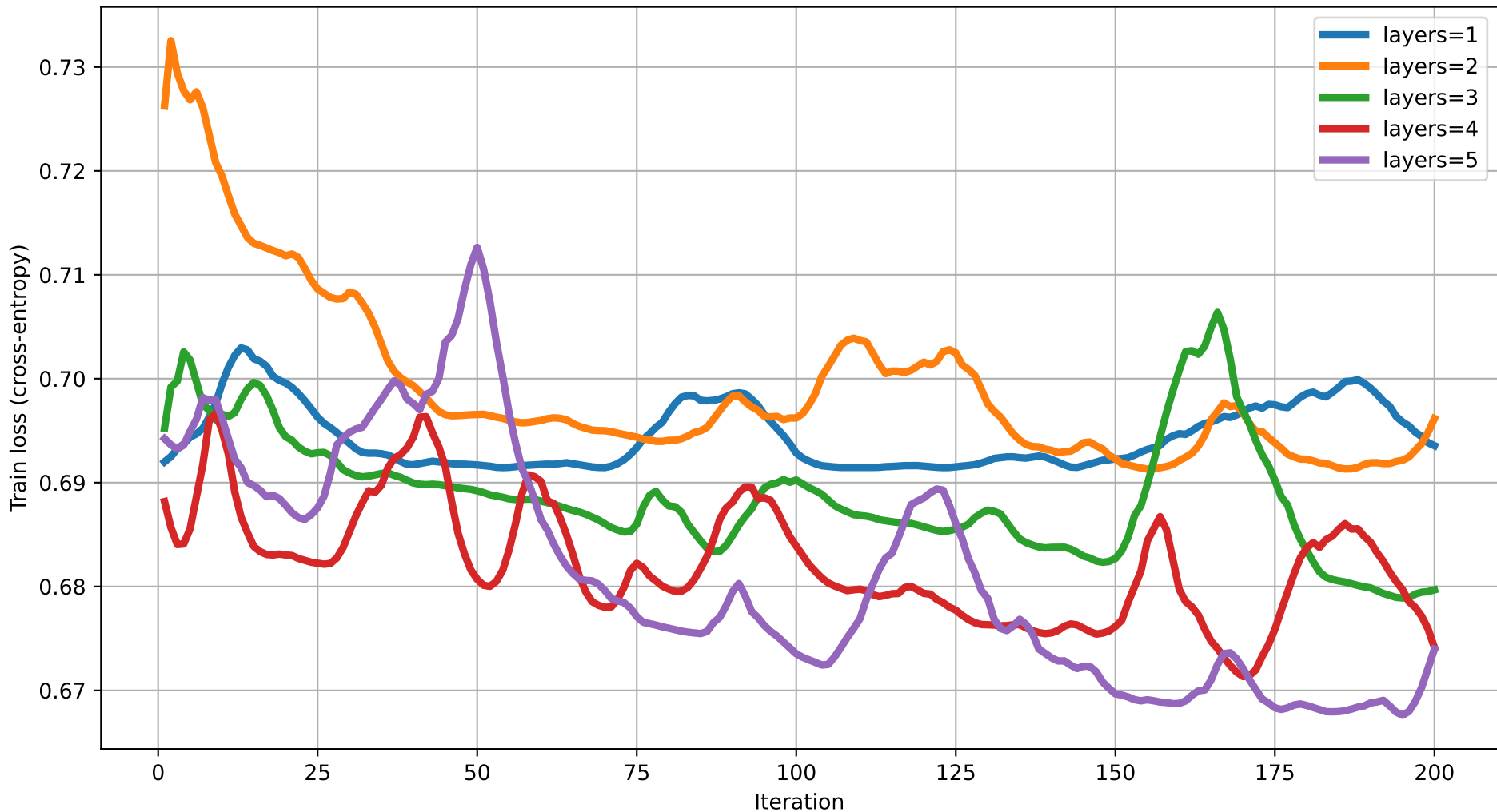
Train loss vs Iteration (dim=15) rot=RY, ent=pairwise, gate=IsingXX
