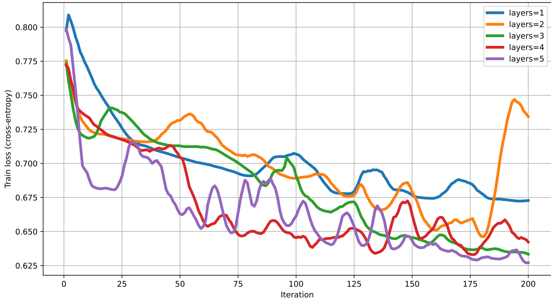
Train loss vs Iteration (dim=4) rot=Rot, ent=full, gate=CZ
