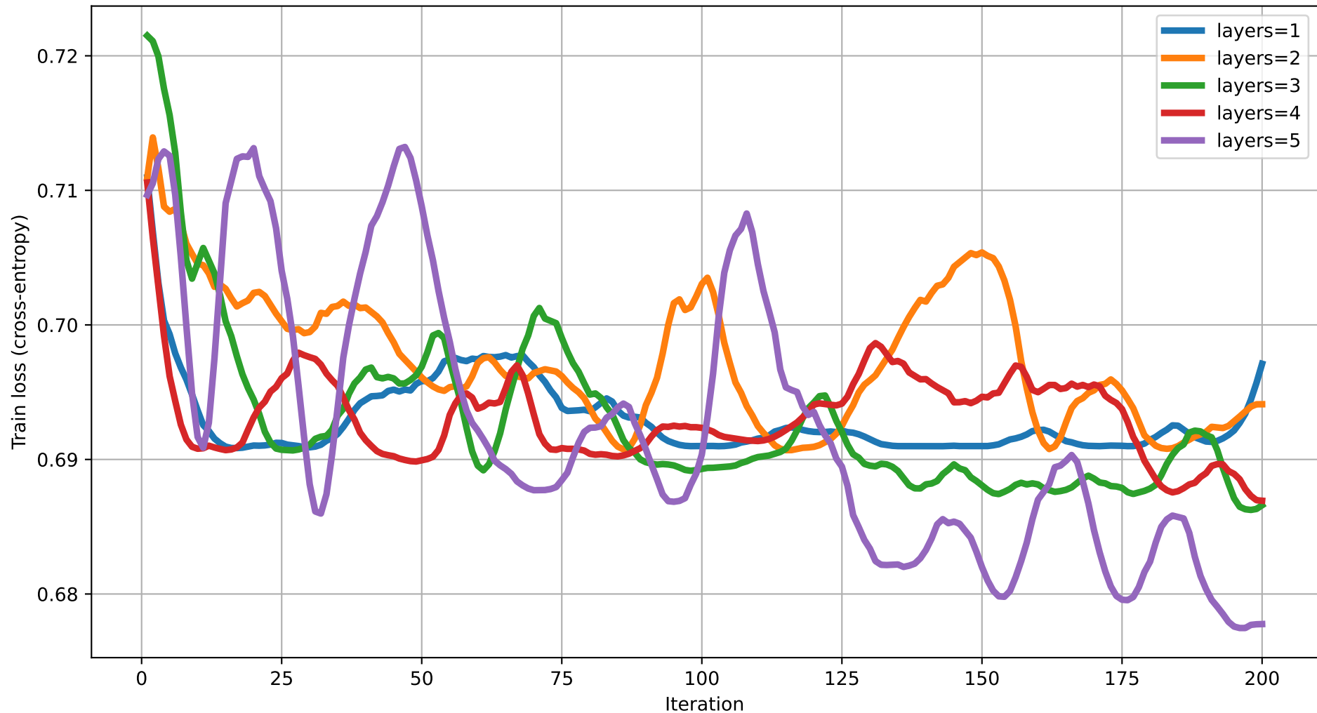
Train loss vs Iteration (dim=20) rot=RX, ent=full, gate=CZ
