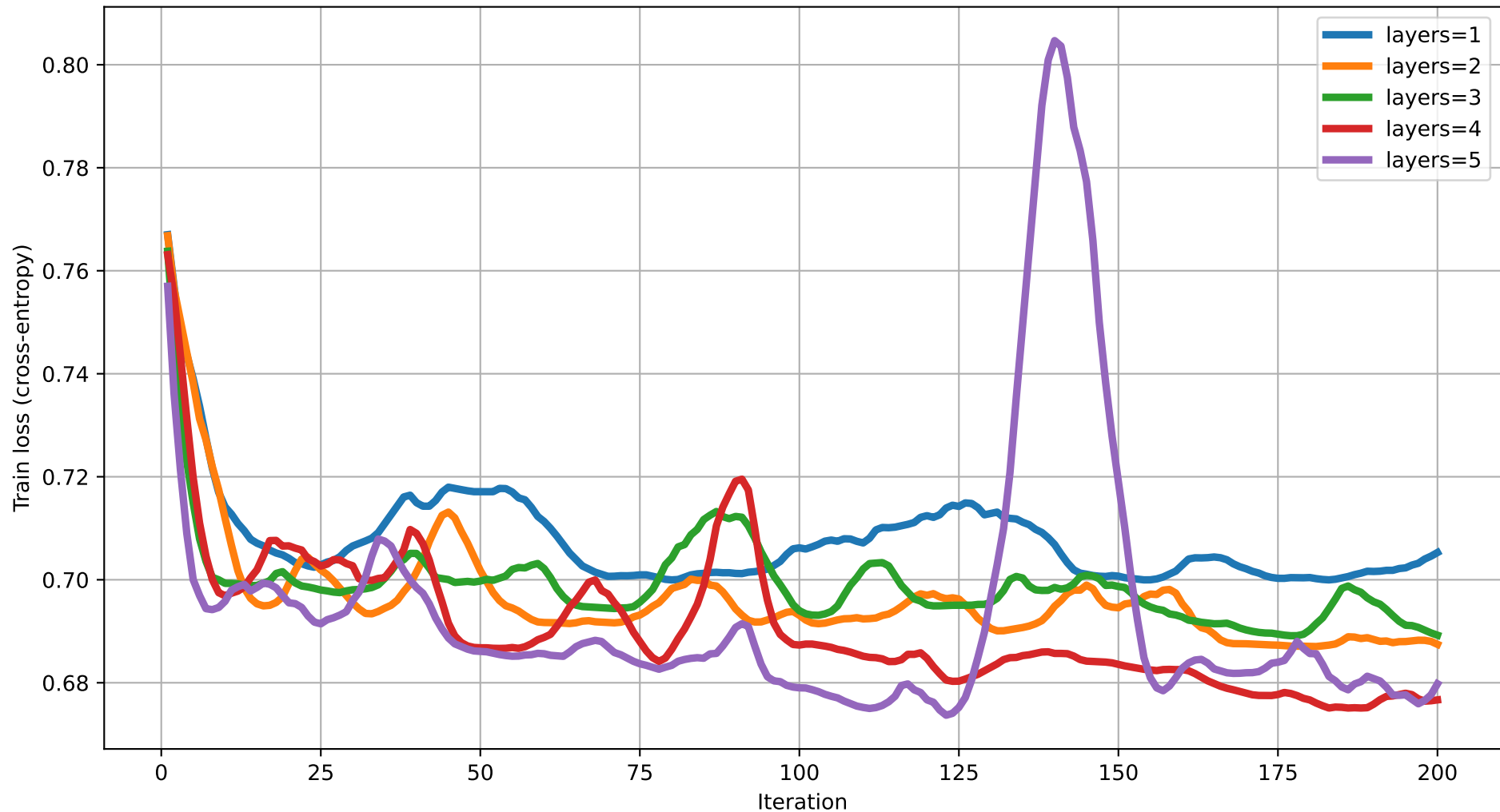
Train loss vs Iteration (dim=17) rot=RY, ent=ring, gate=CZ
