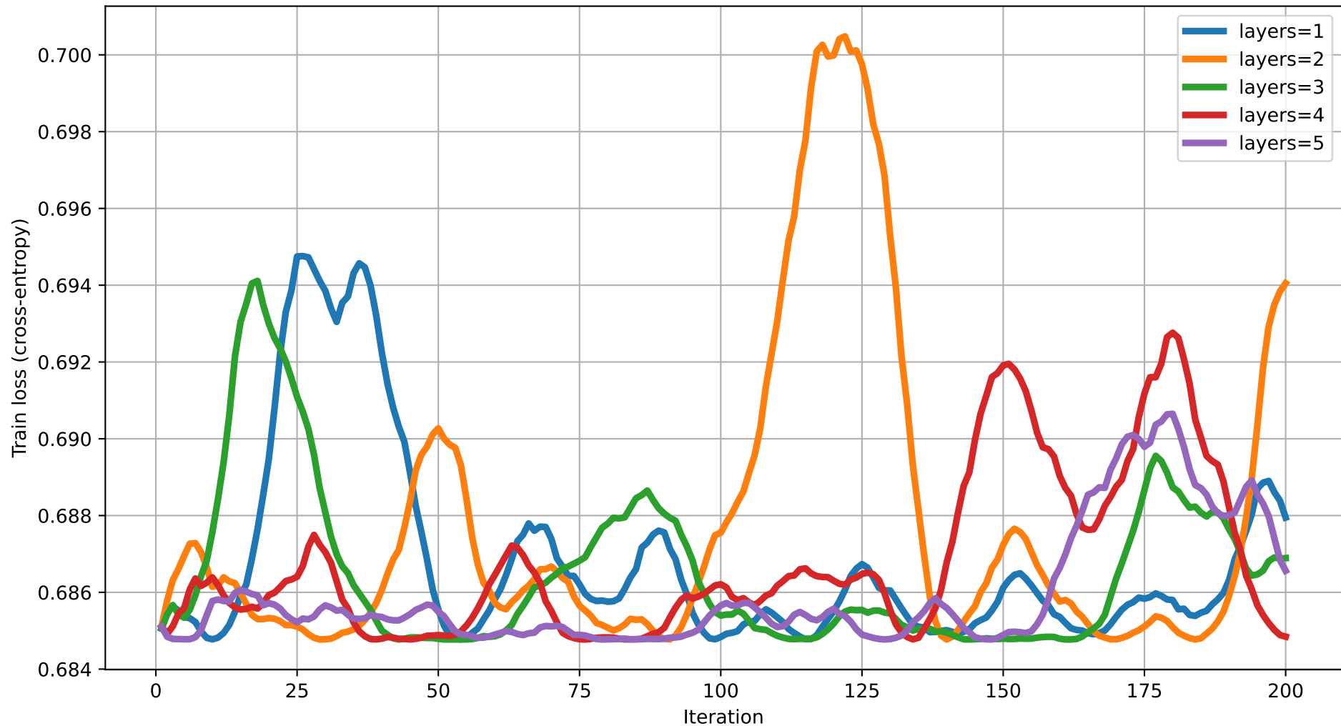
Train loss vs Iteration (dim=15) rot=RZ, ent=full, gate=CZ
