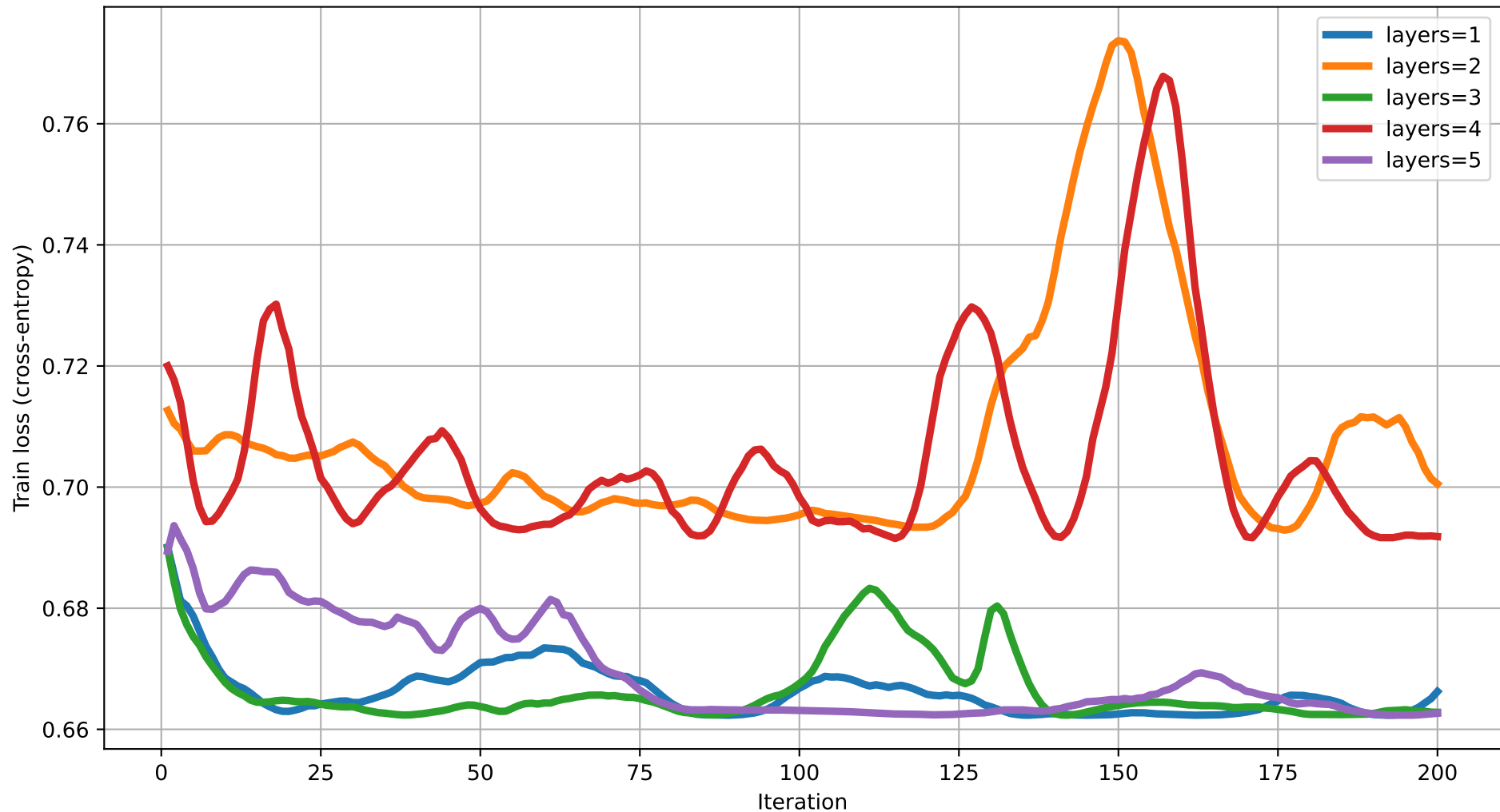
Train loss vs Iteration (dim=11) rot=RX, ent=ring, gate=IsingXX
