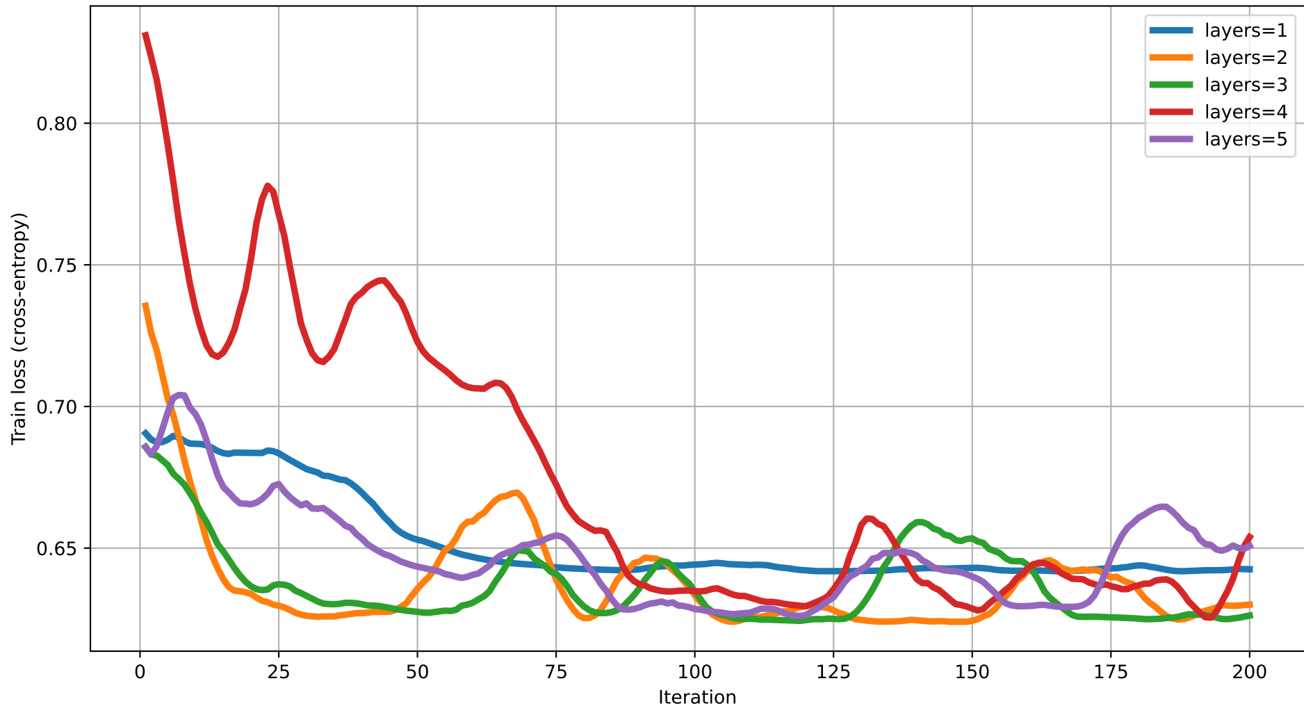
Train loss vs Iteration (dim=2) rot=RZ, ent=pairwise, gate=IsingXX
