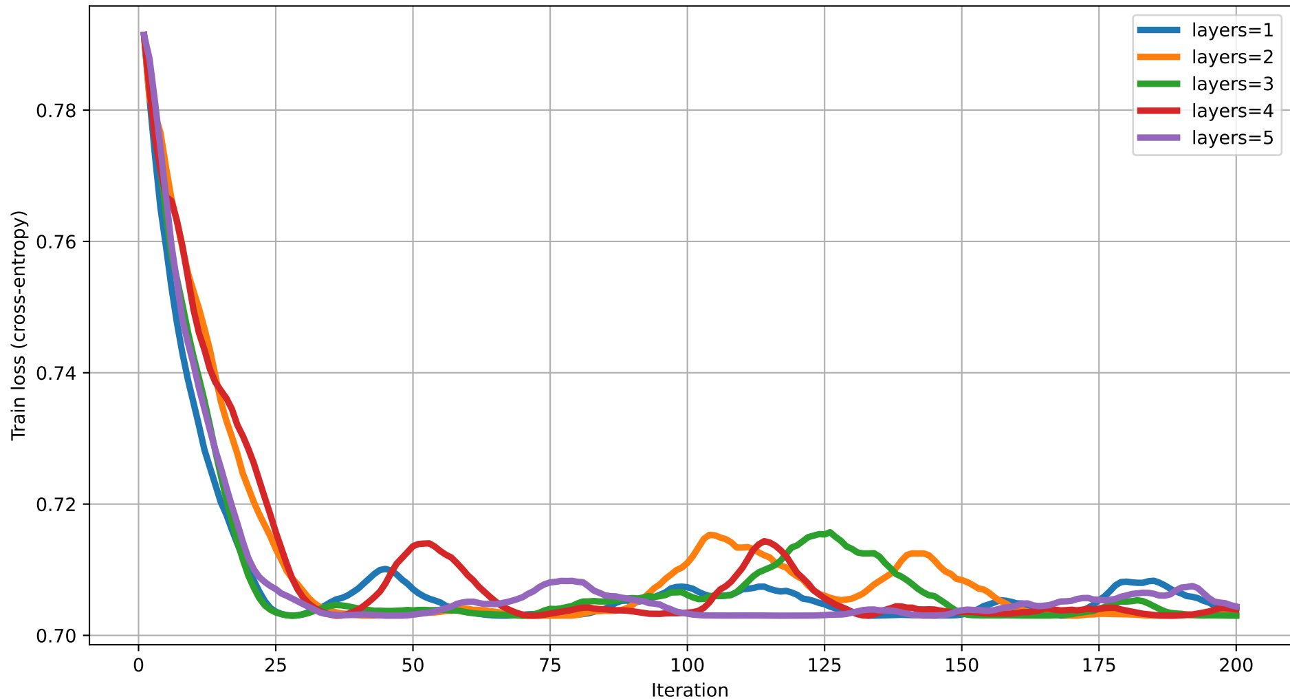
Train loss vs Iteration (dim=2) rot=RZ, ent=ring, gate=CZ
