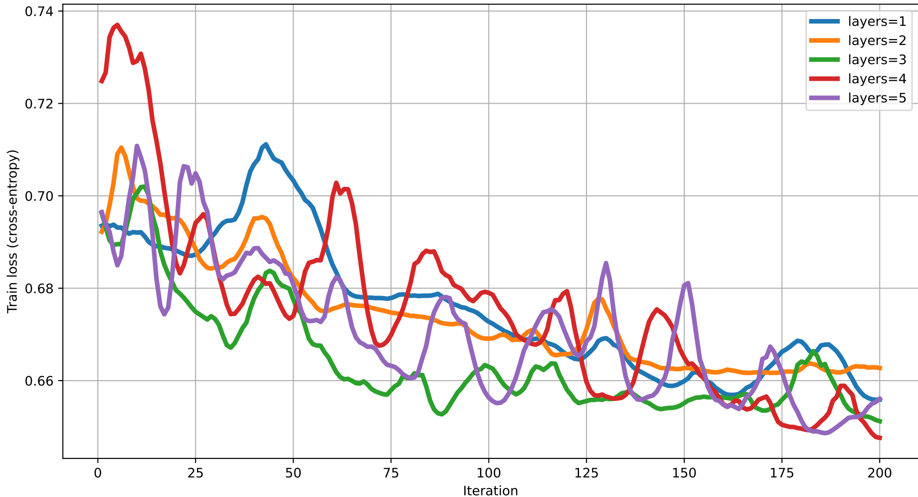
Train loss vs Iteration (dim=7) rot=RYZ, ent=chain, gate=IsingXX
