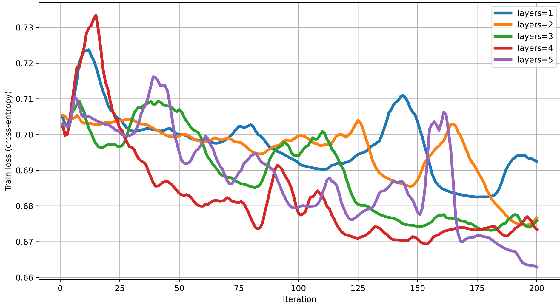
Train loss vs Iteration (dim=14) rot=RYZ, ent=ring, gate=CZ
