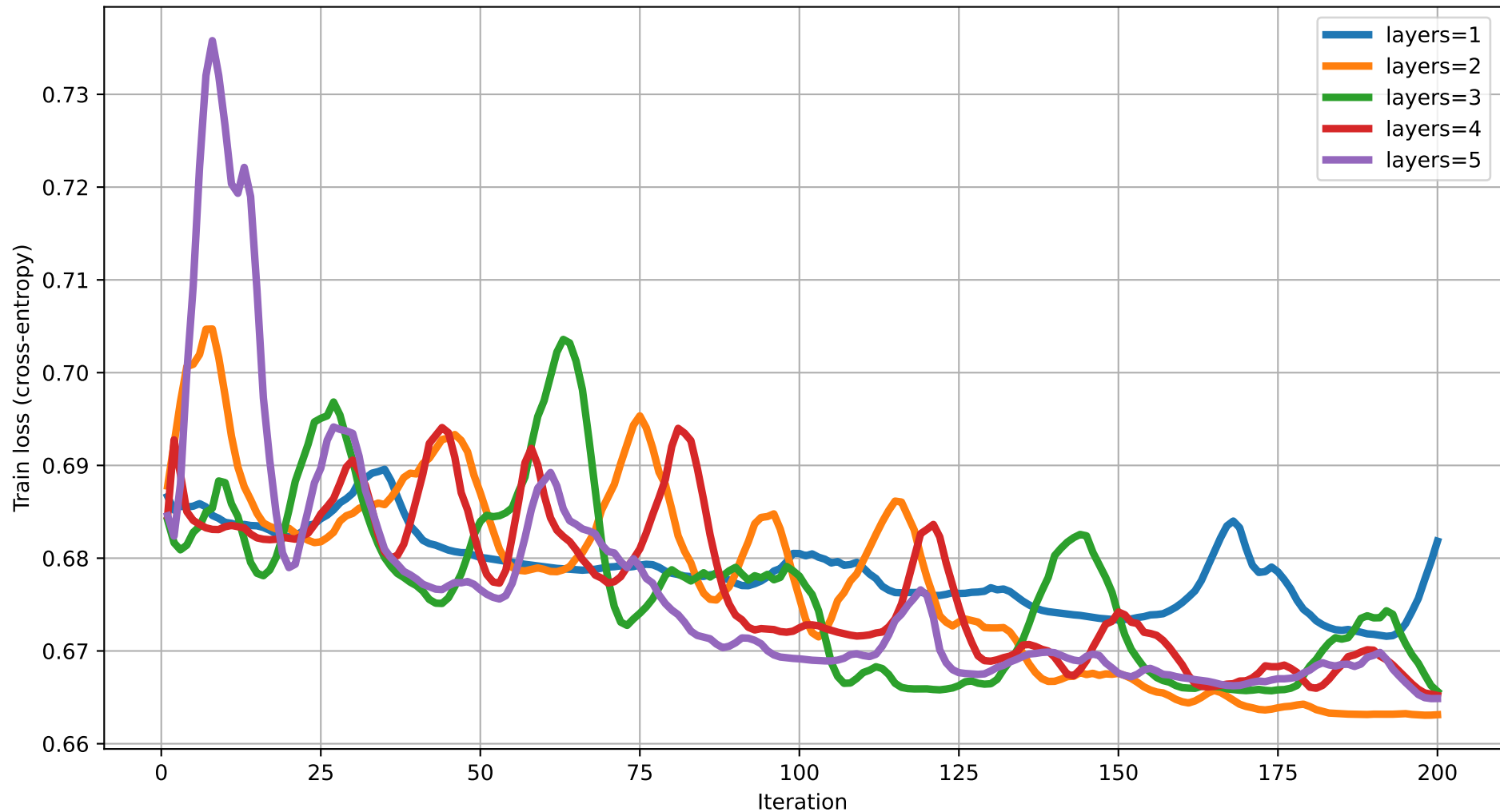
Train loss vs Iteration (dim=15) rot=RYZ, ent=pairwise, gate=CNOT
