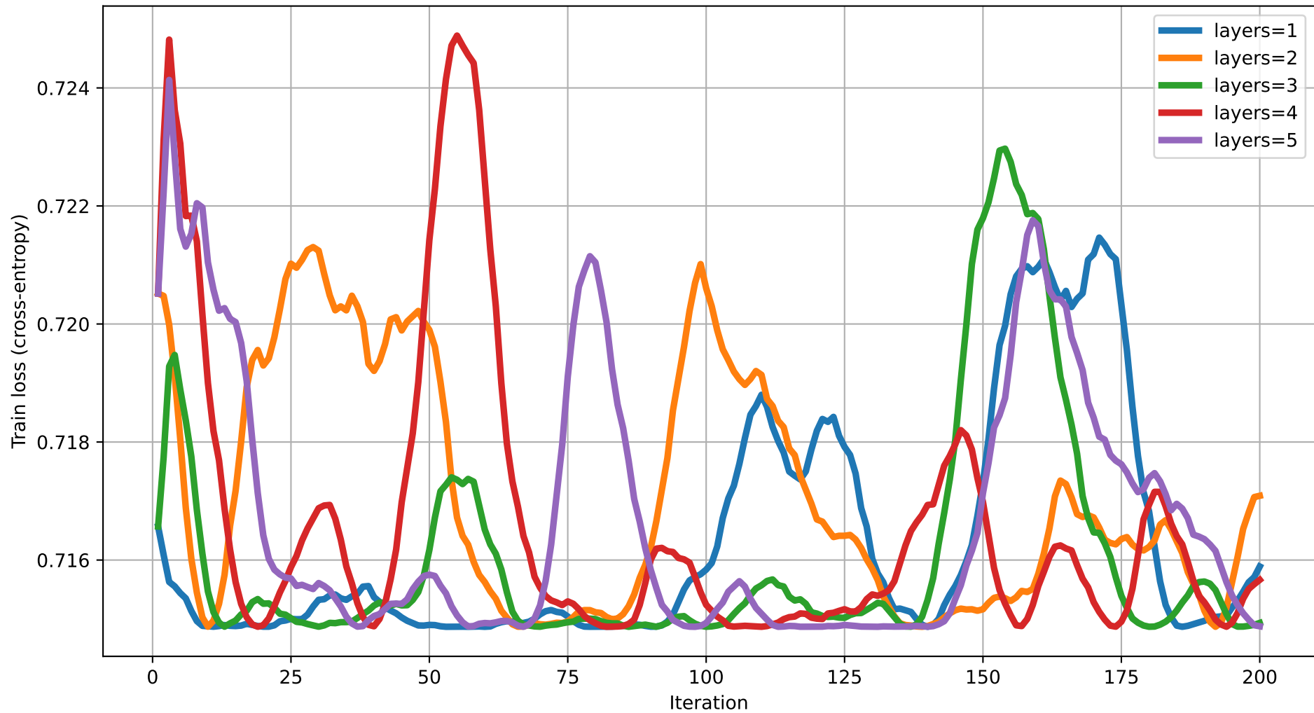
Train loss vs Iteration (dim=3) rot=RZ, ent=pairwise, gate=CNOT
