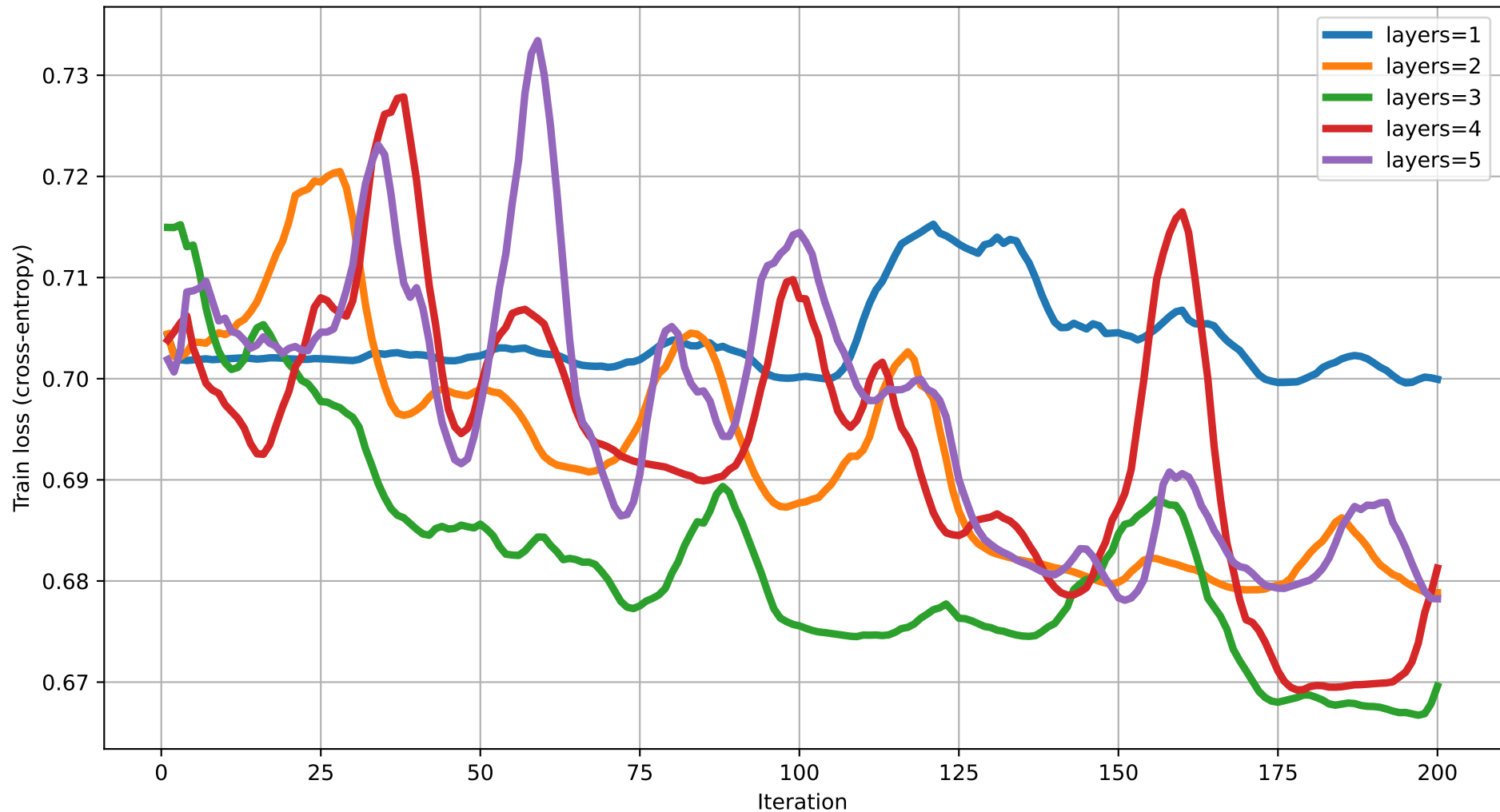
Train loss vs Iteration (dim=12) rot=RYZ, ent=full, gate=CZ
