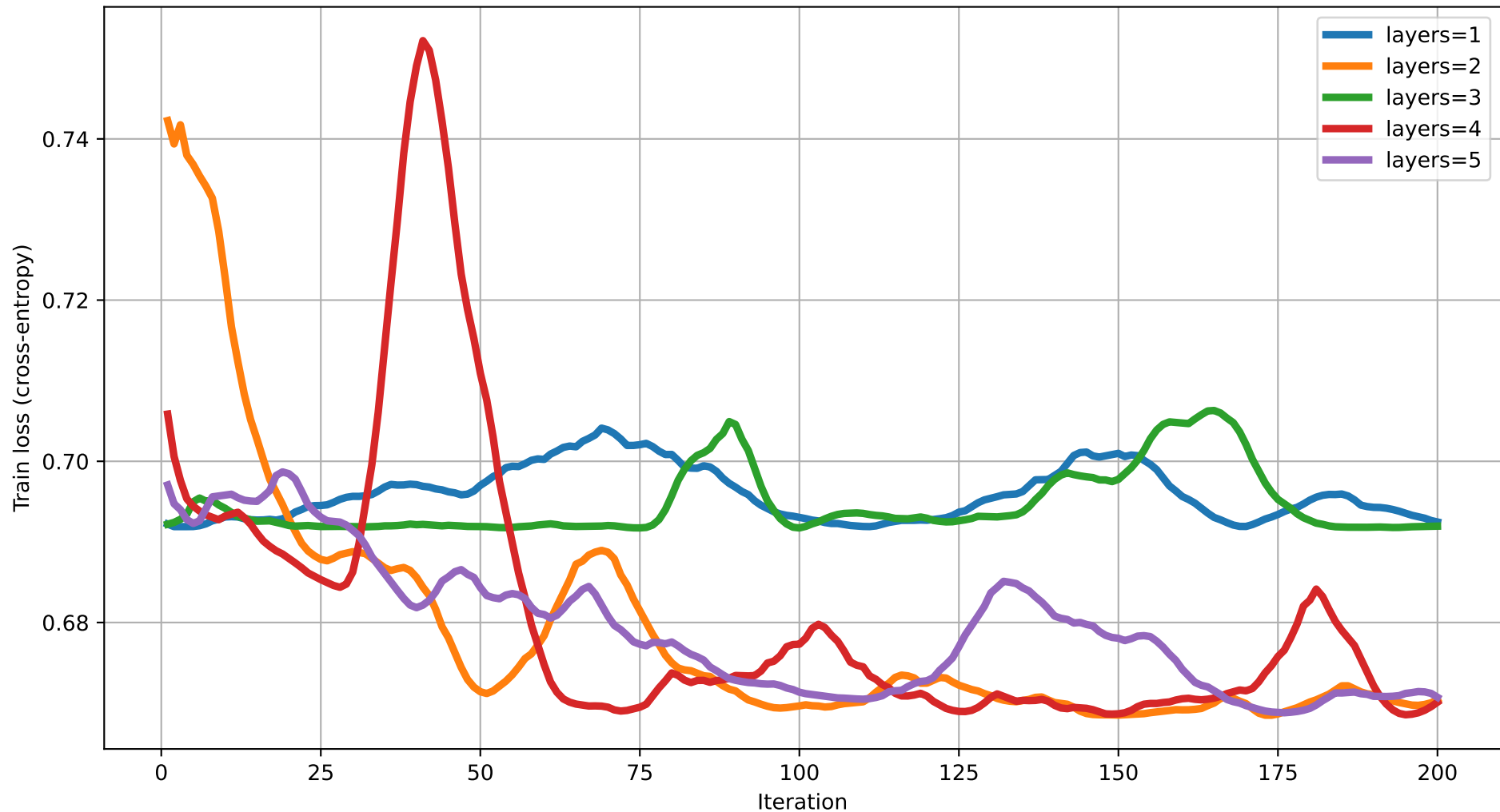
Train loss vs Iteration (dim=11) rot=RY, ent=chain, gate=IsingXX
