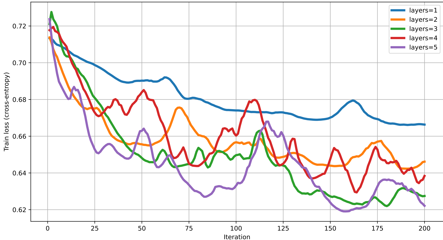
Train loss vs Iteration (dim=7) rot=Rot, ent=full, gate=CZ
