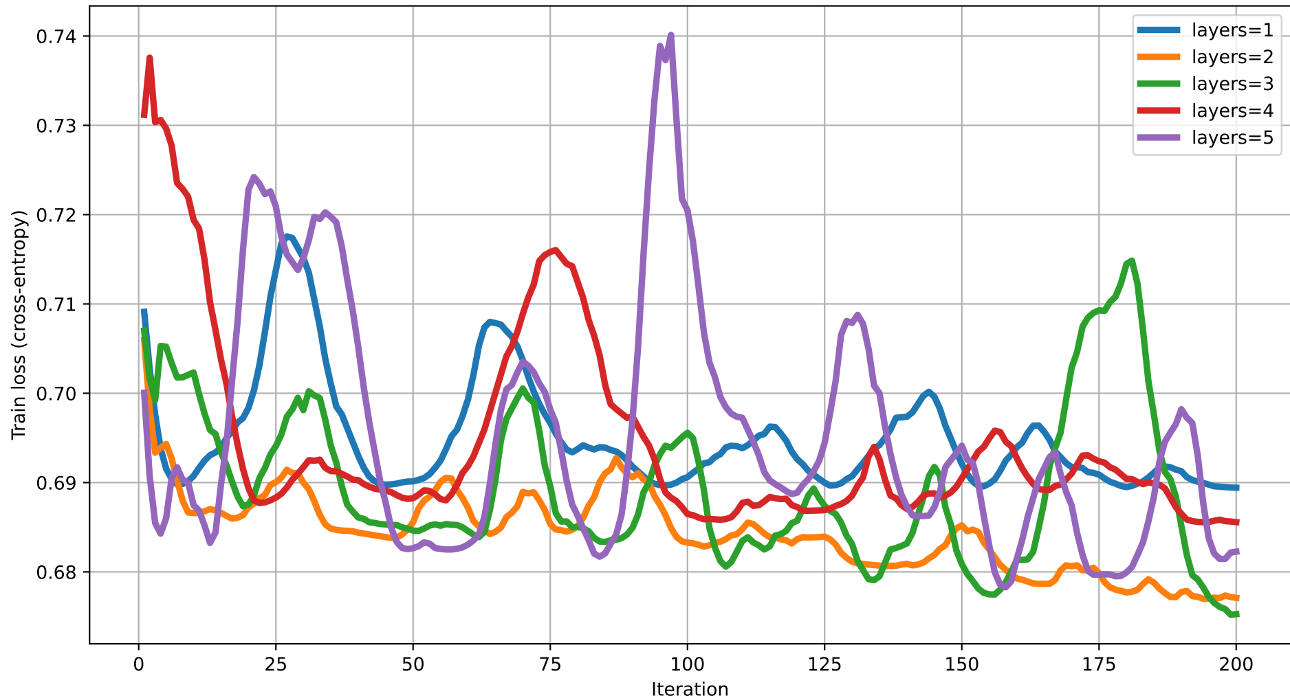
Train loss vs Iteration (dim=20) rot=RYZ, ent=full, gate=CNOT
