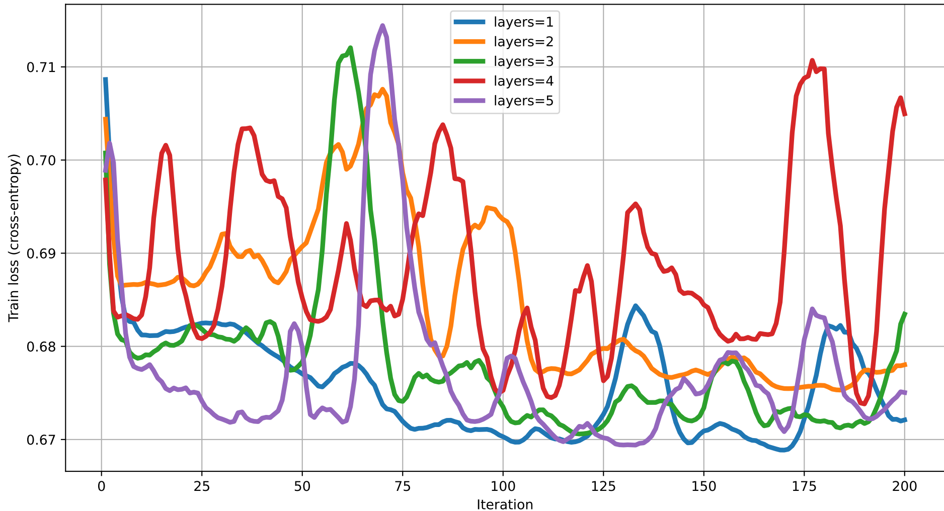
Train loss vs Iteration (dim=20) rot=RY, ent=ring, gate=IsingXX
