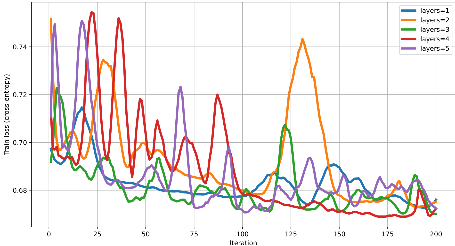
Train loss vs Iteration (dim=18) rot=Rot, ent=pairwise, gate=IsingXX
