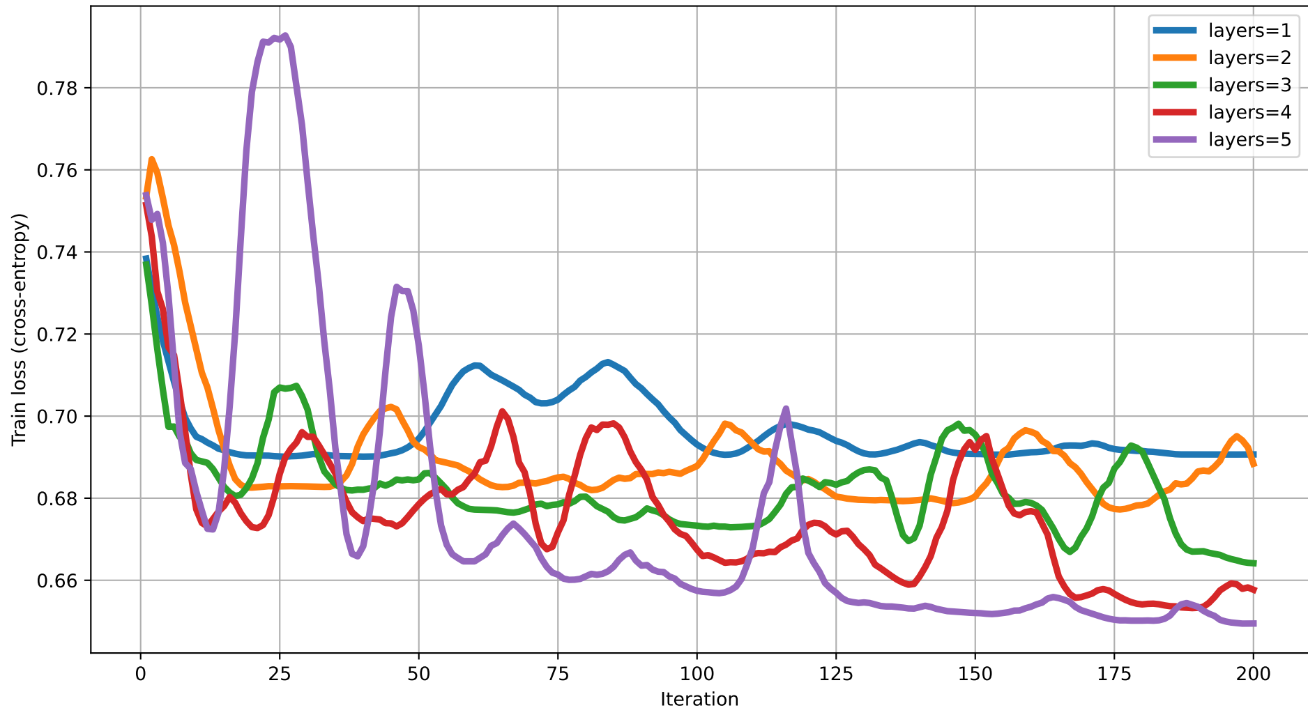
Train loss vs Iteration (dim=16) rot=RX, ent=full, gate=CNOT
