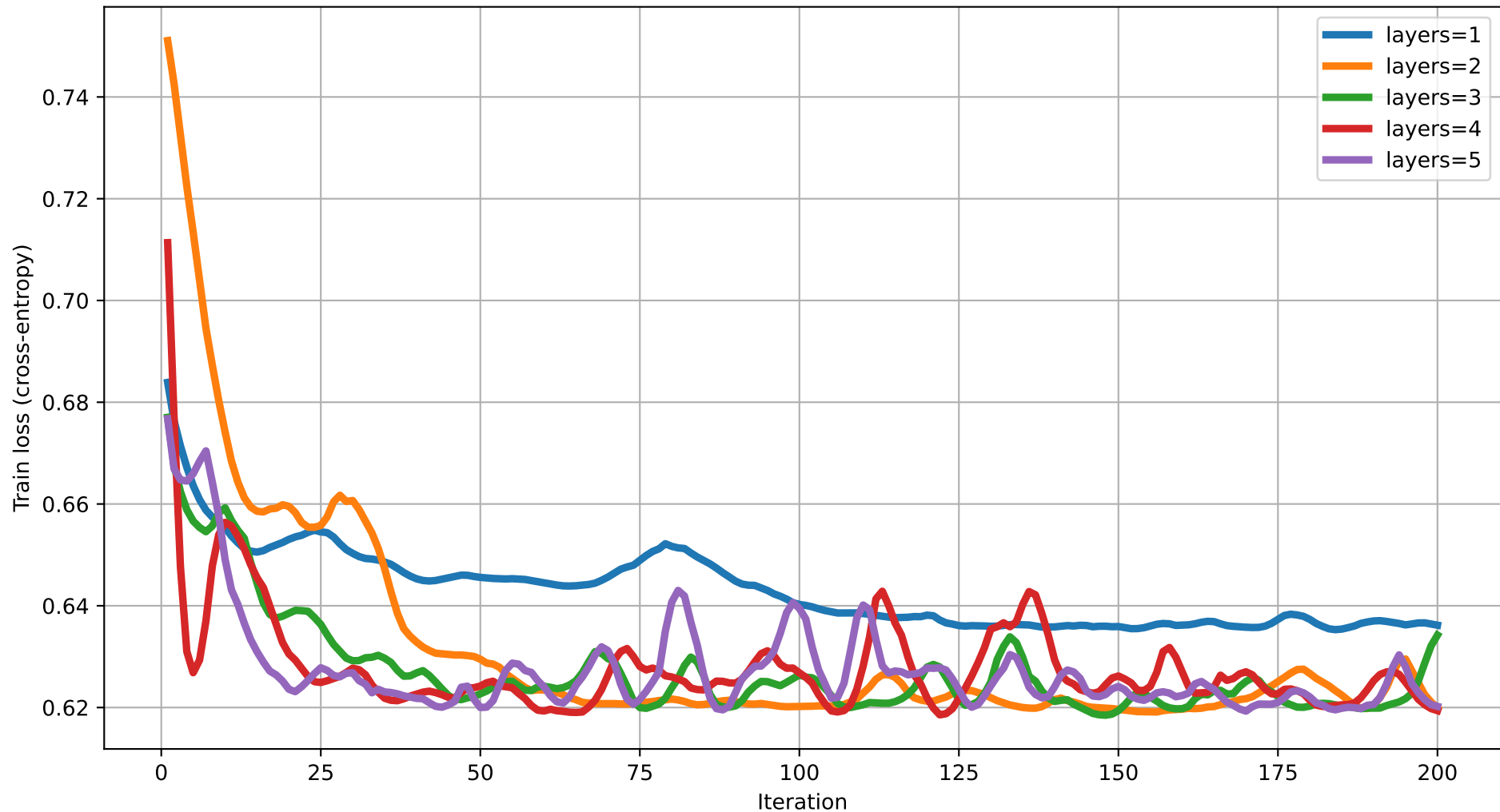
Train loss vs Iteration (degree=5) rot=Rot, ent=pairwise, gate=IsingXX
