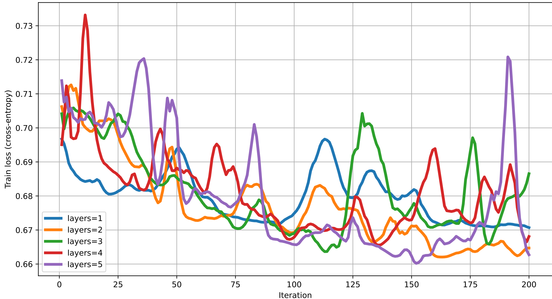
Train loss vs Iteration (dim=12) rot=Rot, ent=full, gate=IsingXX
