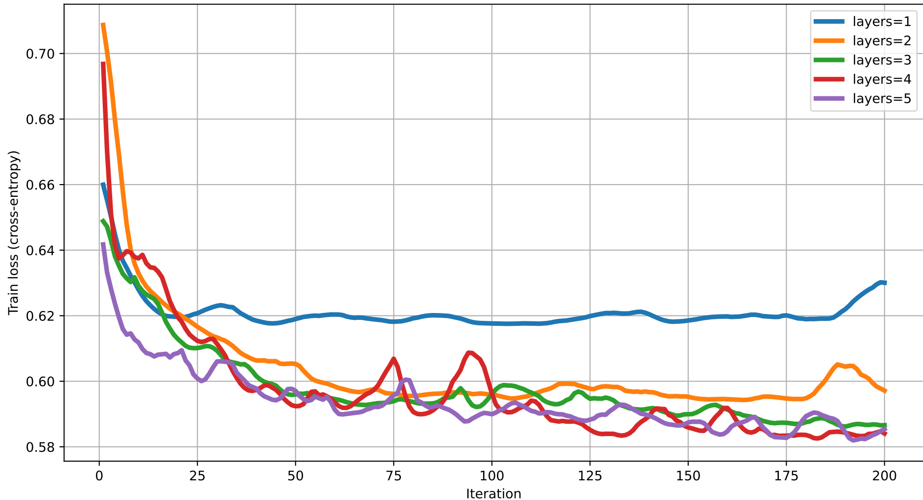
Train loss vs Iteration (degree=4) rot=RYZ, ent=ring, gate=IsingXX
