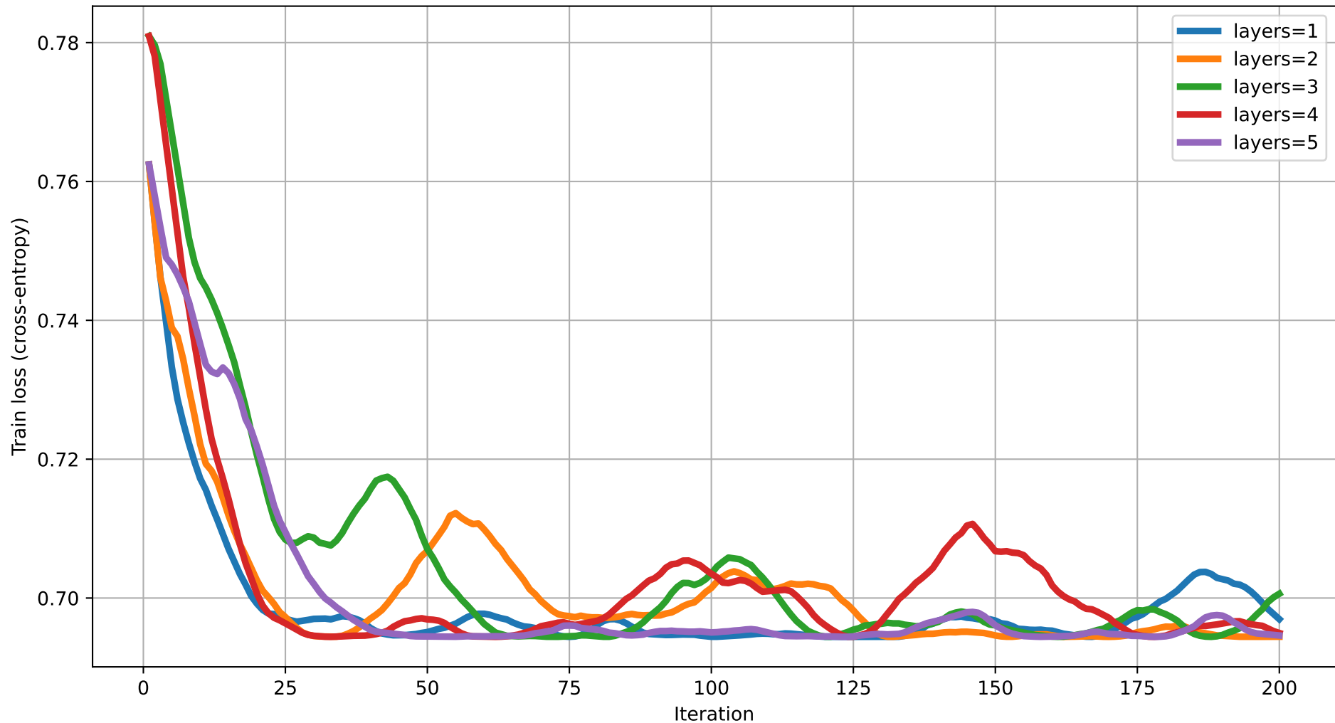
Train loss vs Iteration (dim=8) rot=RZ, ent=chain, gate=CNOT
