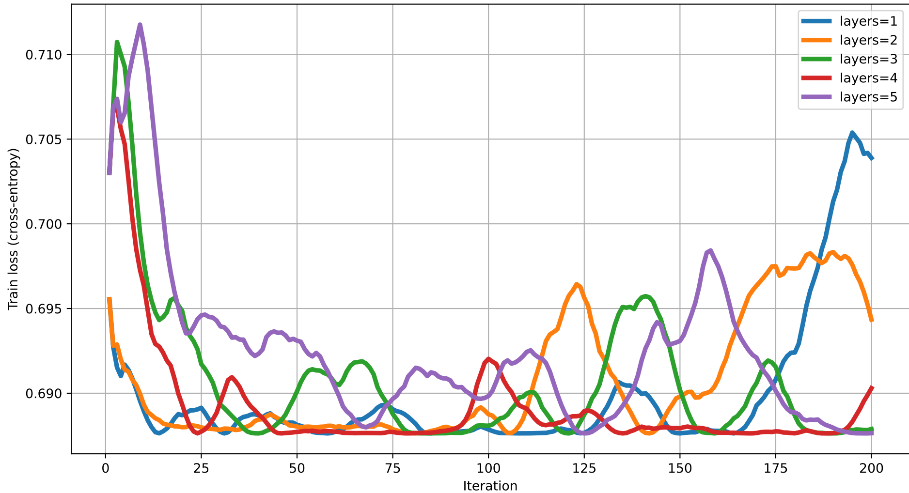
Train loss vs Iteration (dim=13) rot=RZ, ent=pairwise, gate=CNOT
