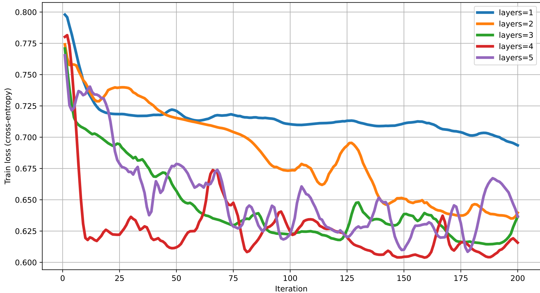
Train loss vs Iteration (dim=4) rot=Rot, ent=full, gate=CNOT
