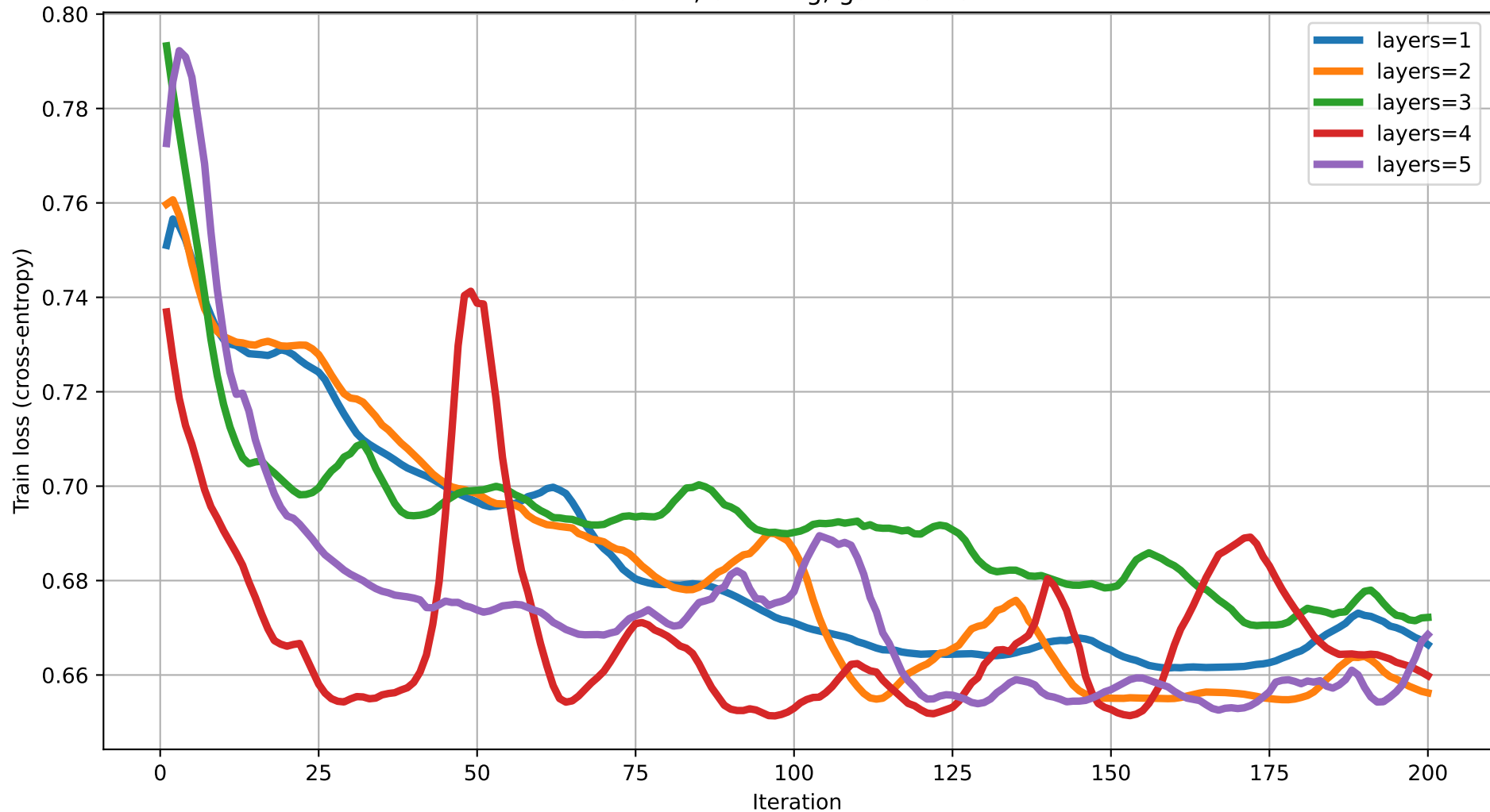
Train loss vs Iteration (dim=2) rot=RY, ent=ring, gate=CNOT
