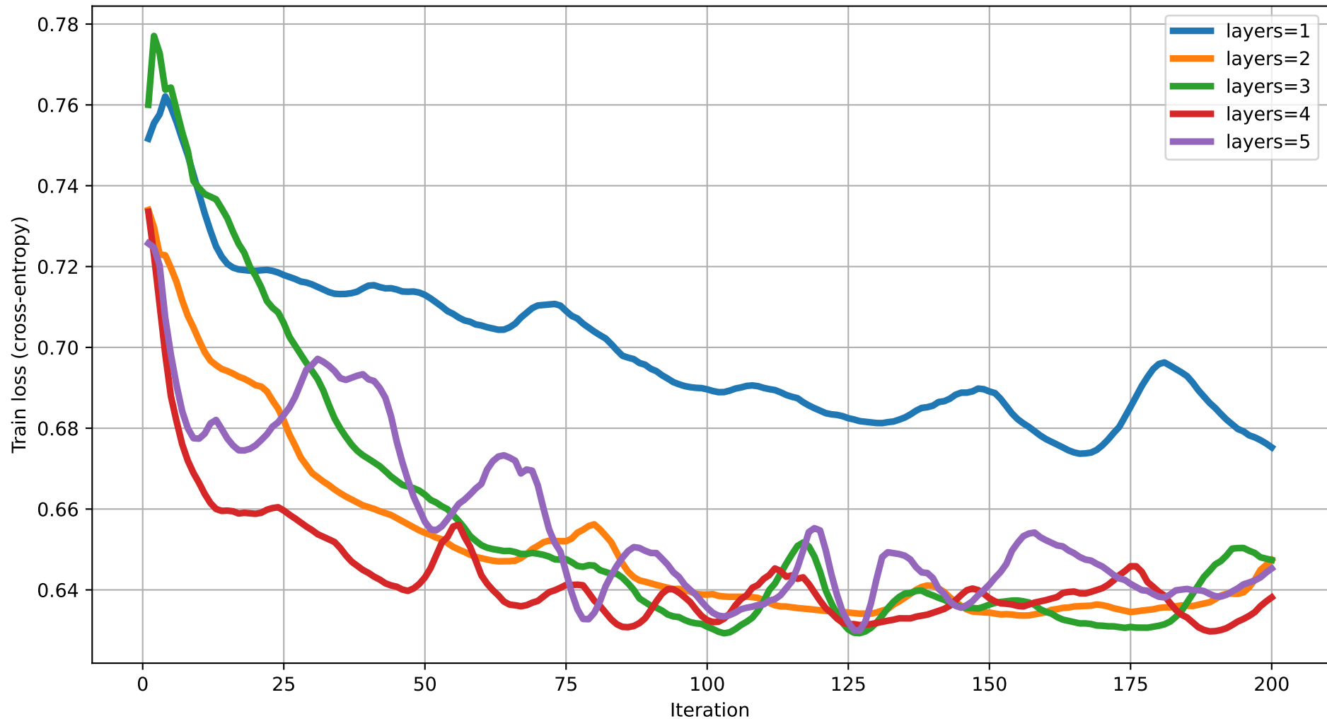
Train loss vs Iteration (dim=3) rot=RY, ent=pairwise, gate=CZ
