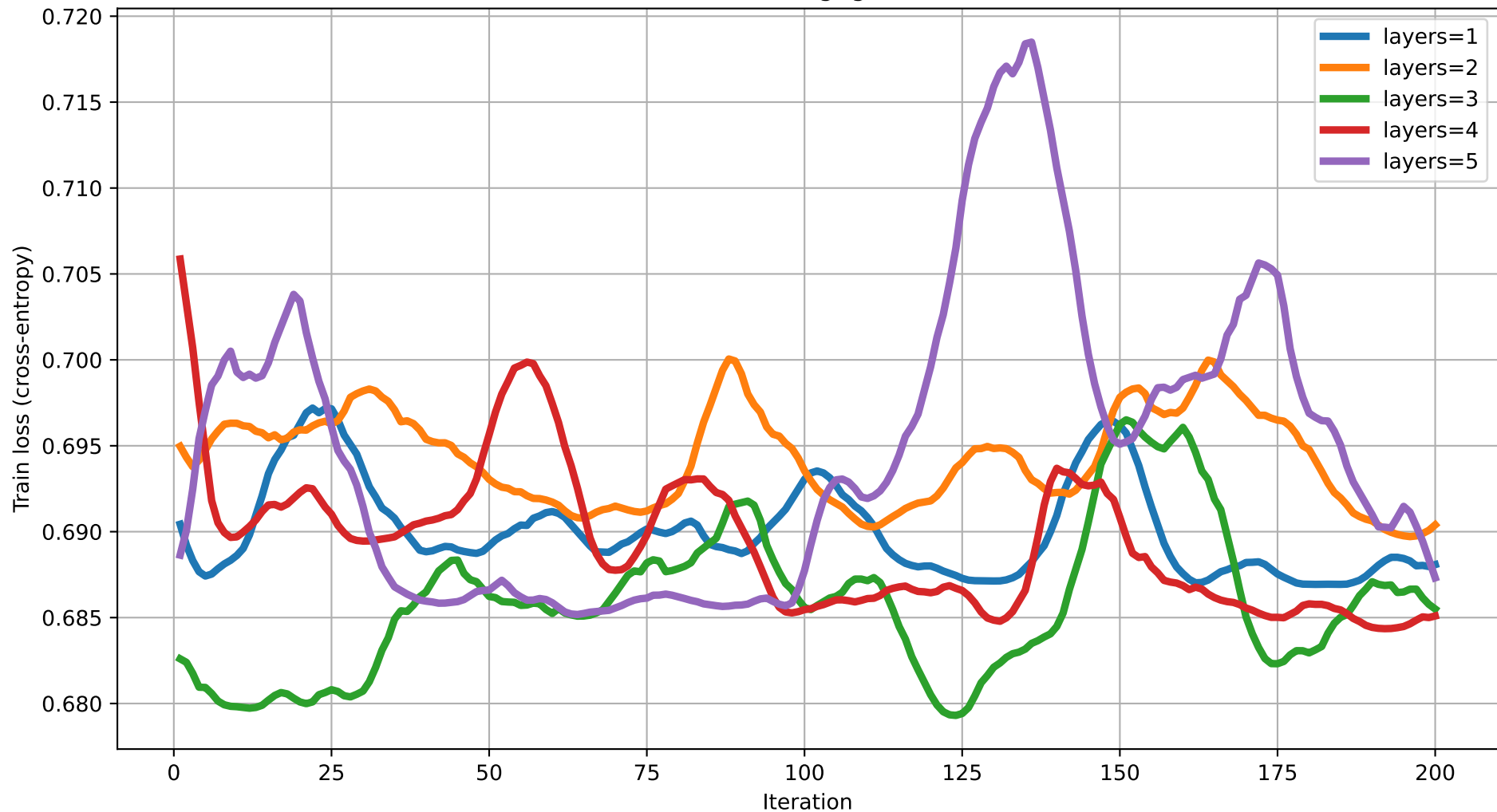
Train loss vs Iteration (dim=19) rot=RX, ent=ring, gate=CNOT
