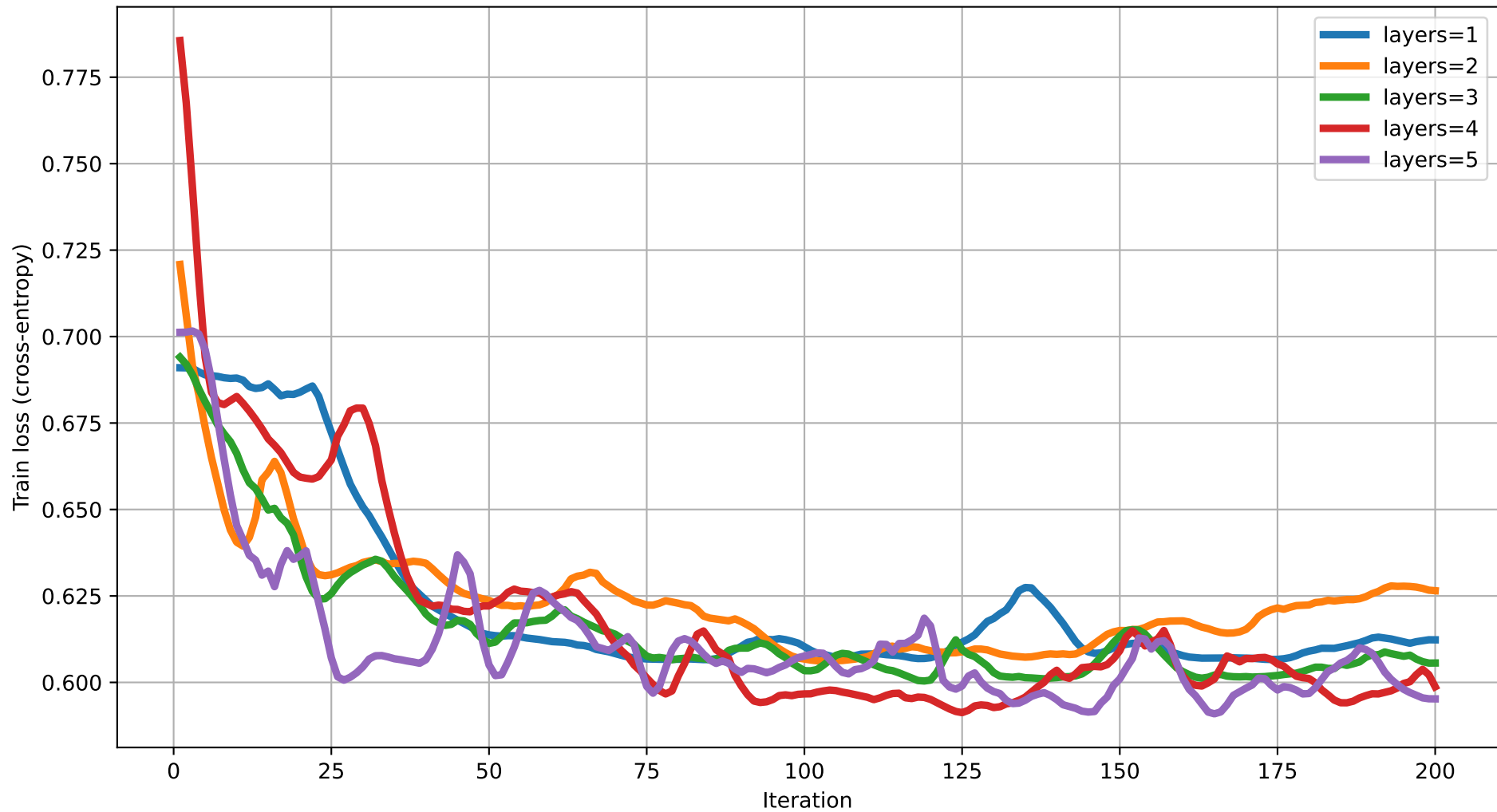
Train loss vs Iteration (dim=9) rot=Rot, ent=chain, gate=IsingXX
