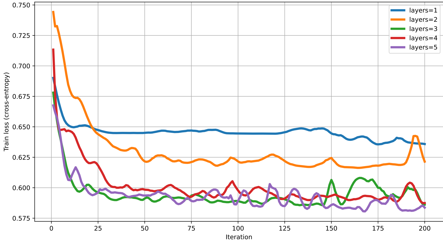
Train loss vs Iteration (degree=5) rot=Rot, ent=chain, gate=IsingXX
