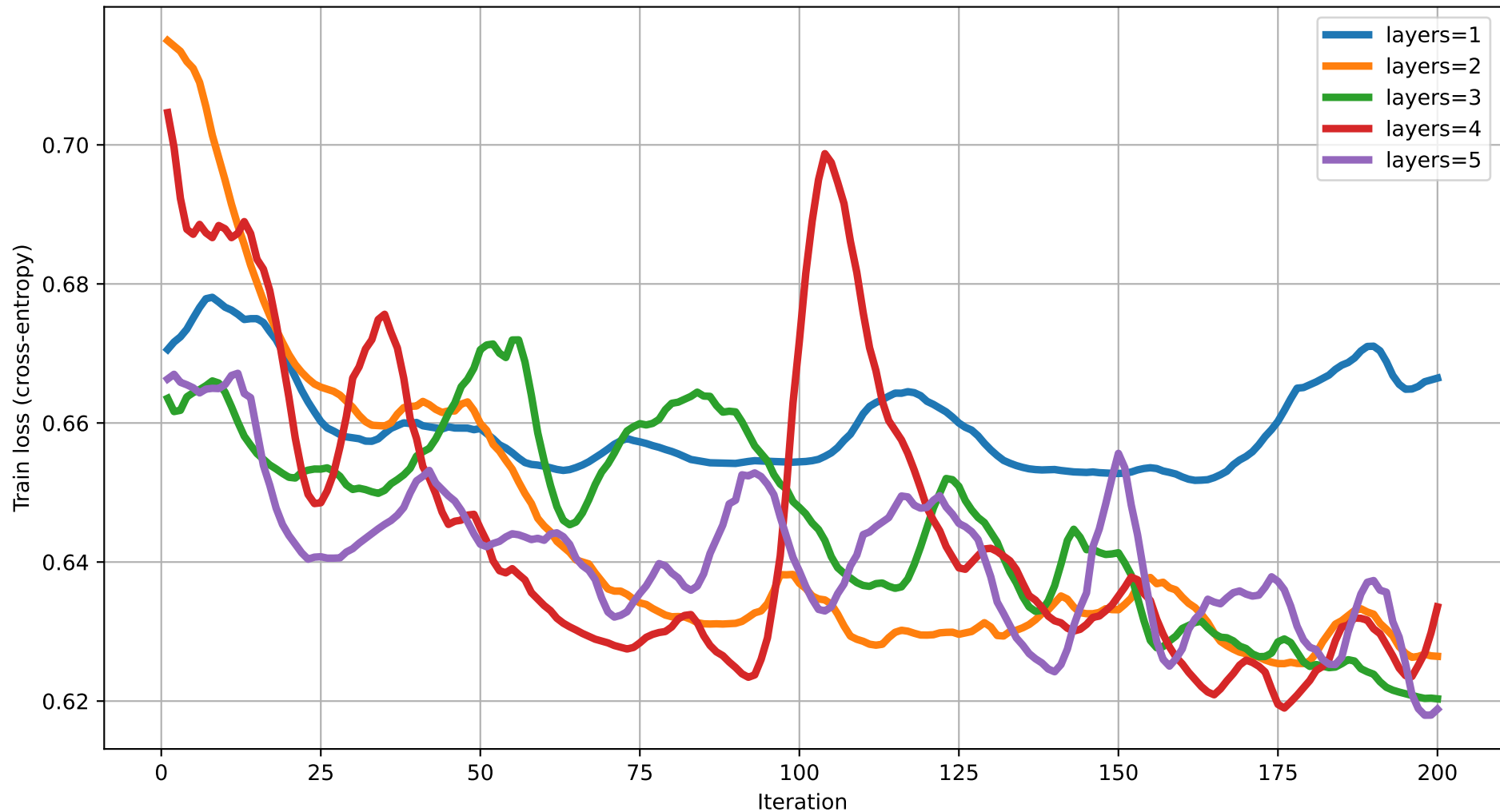
Train loss vs Iteration (dim=7) rot=RYZ, ent=ring, gate=IsingXX
