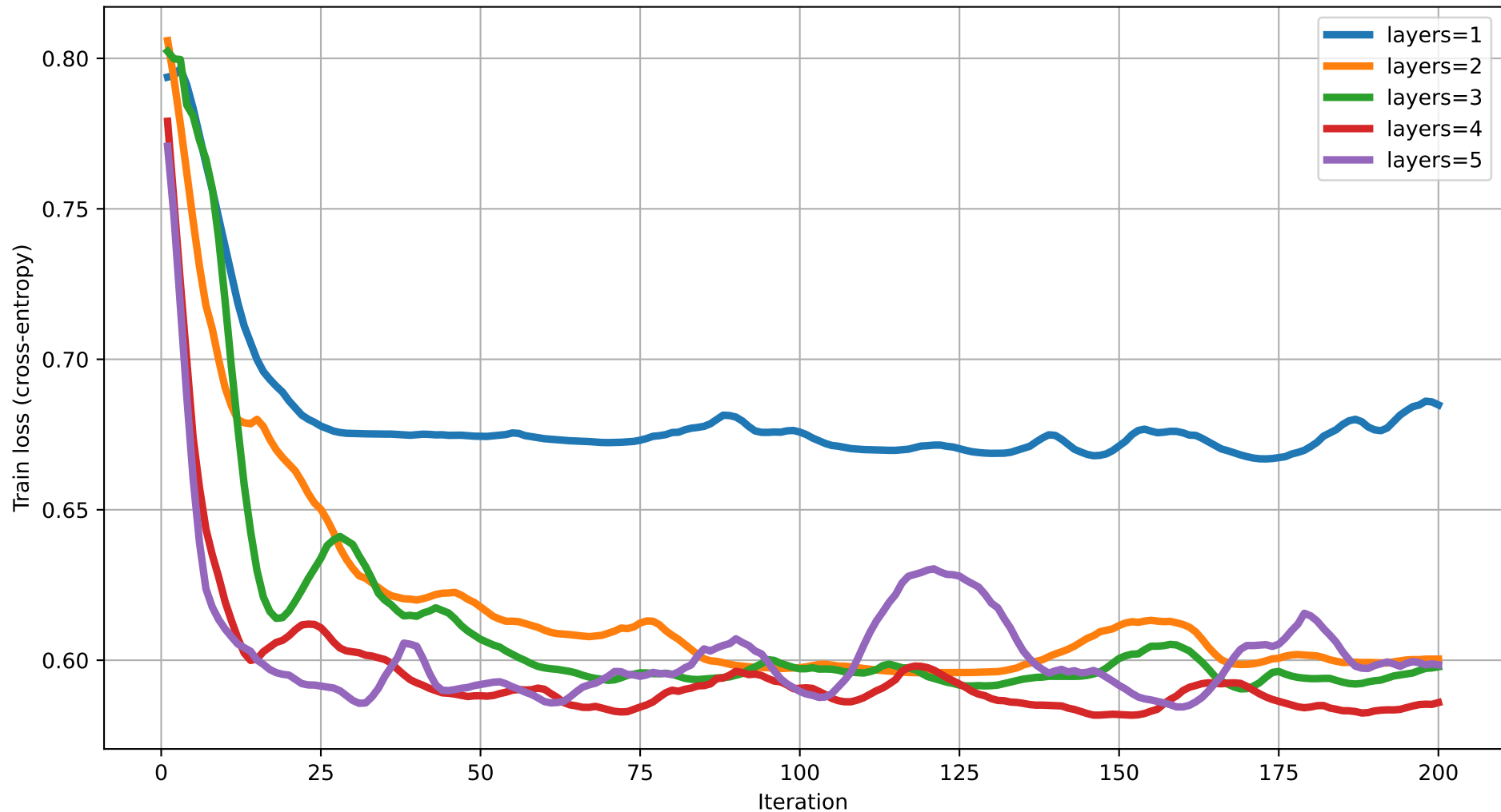
Train loss vs Iteration (dim=4) rot=RYZ, ent=full, gate=CNOT
