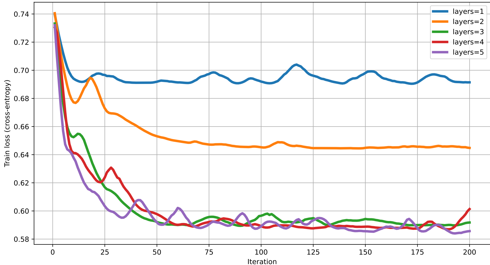
Train loss vs Iteration (degree=5) rot=RYZ, ent=chain, gate=CNOT
