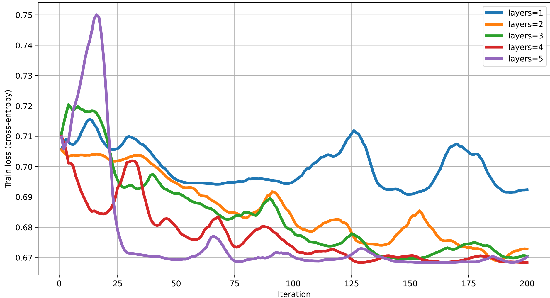
Train loss vs Iteration (dim=12) rot=RX, ent=pairwise, gate=CNOT
