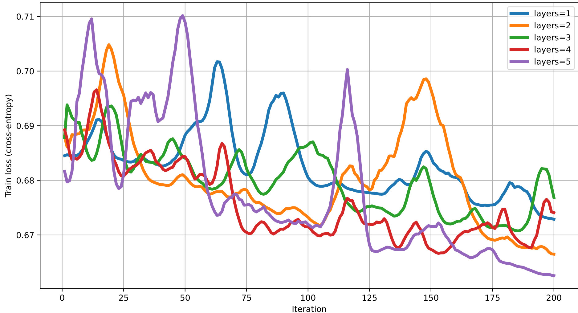
Train loss vs Iteration (dim=15) rot=RYZ, ent=ring, gate=CZ
