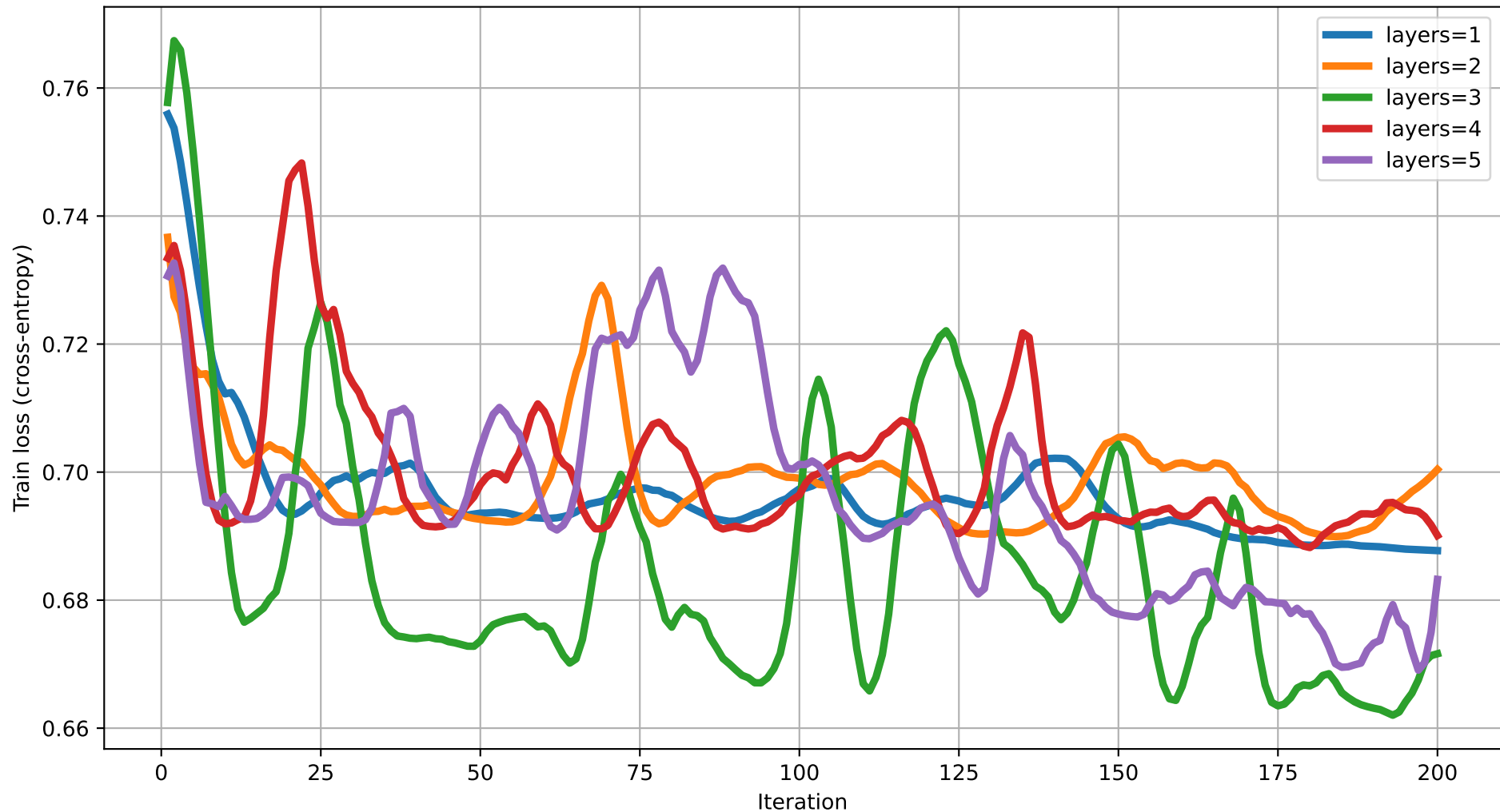
Train loss vs Iteration (dim=16) rot=RY, ent=chain, gate=CZ
