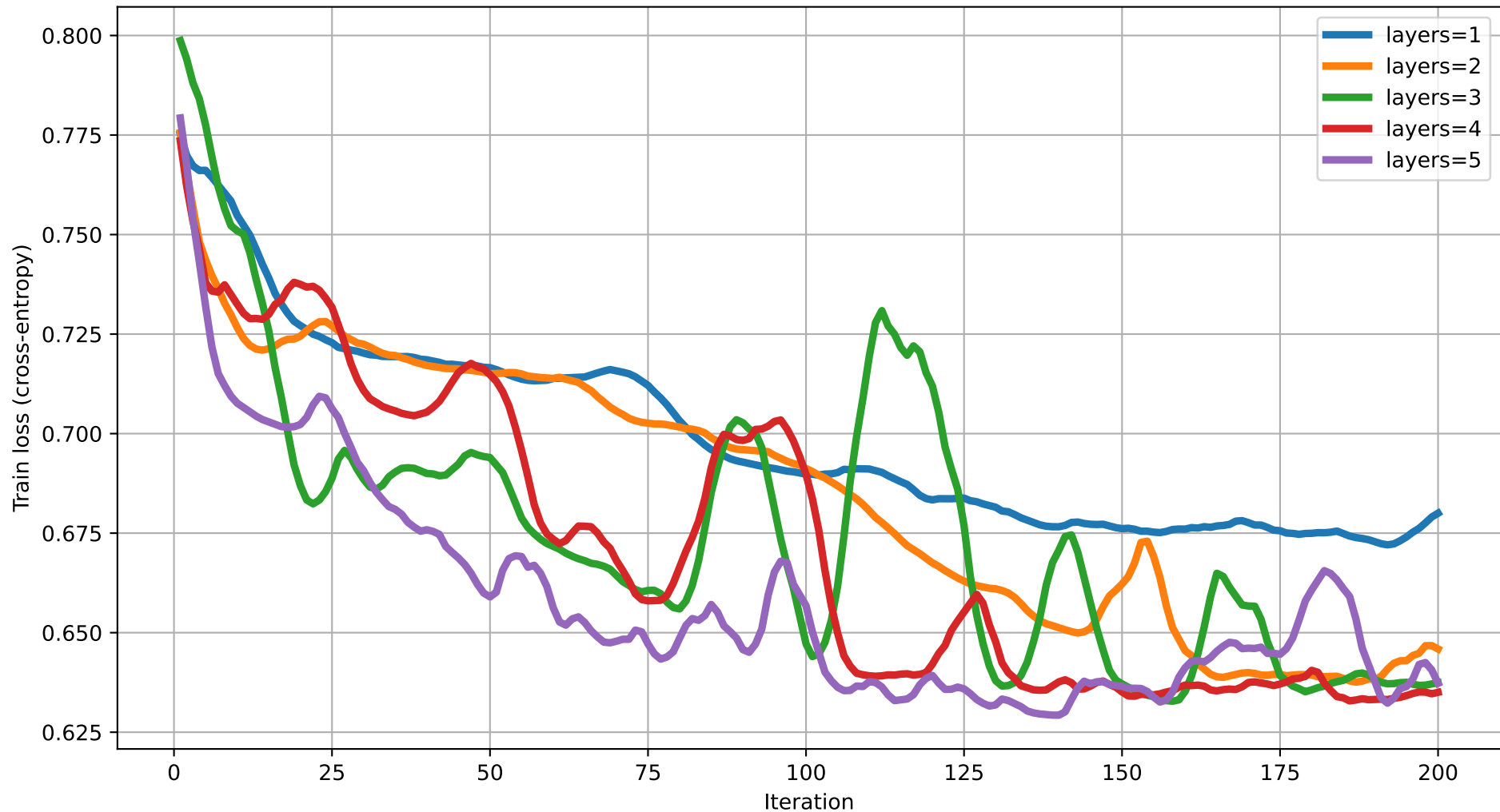
Train loss vs Iteration (dim=4) rot=RY, ent=ring, gate=CZ
