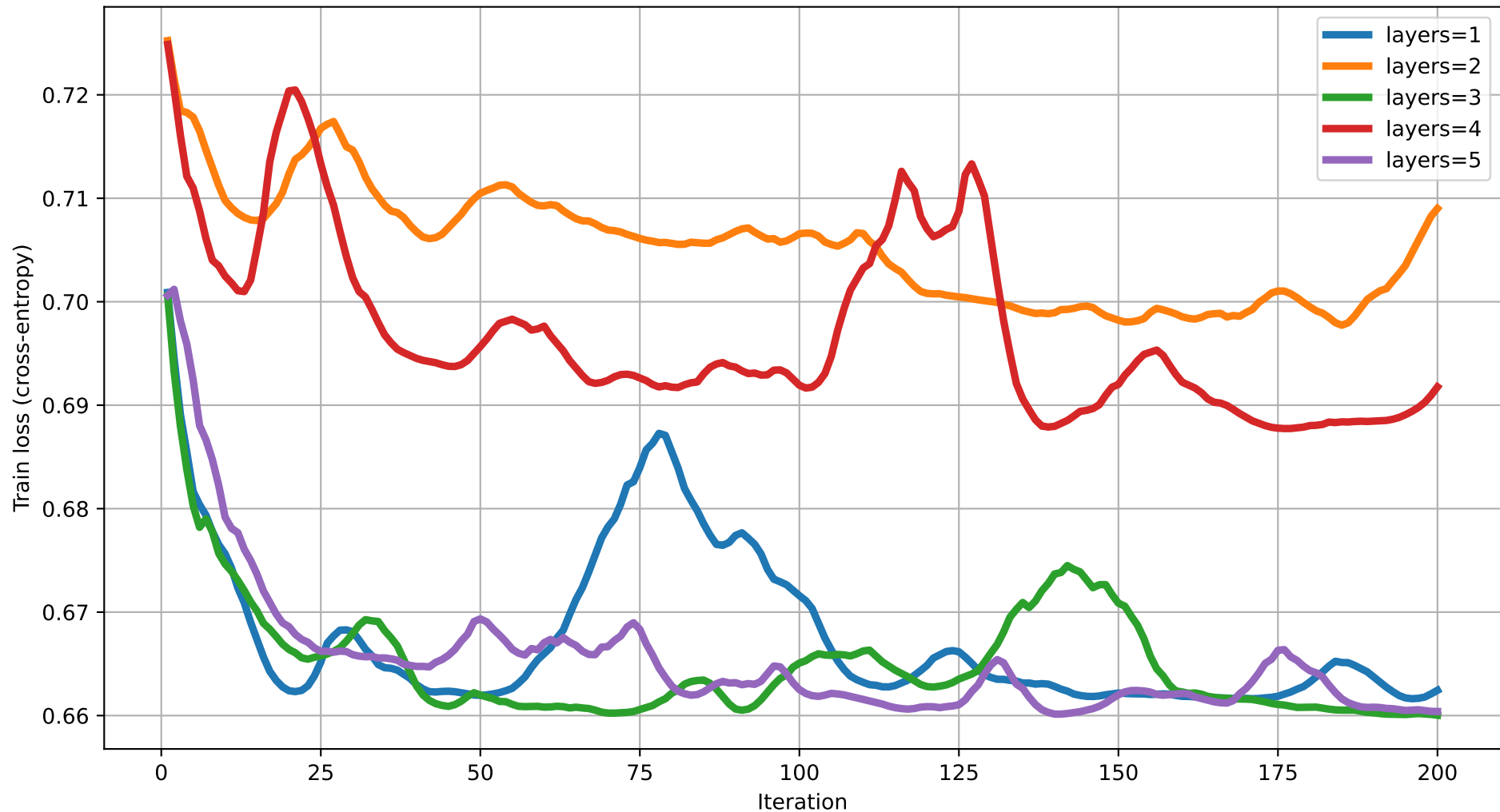
Train loss vs Iteration (dim=10) rot=RZ, ent=ring, gate=IsingXX
