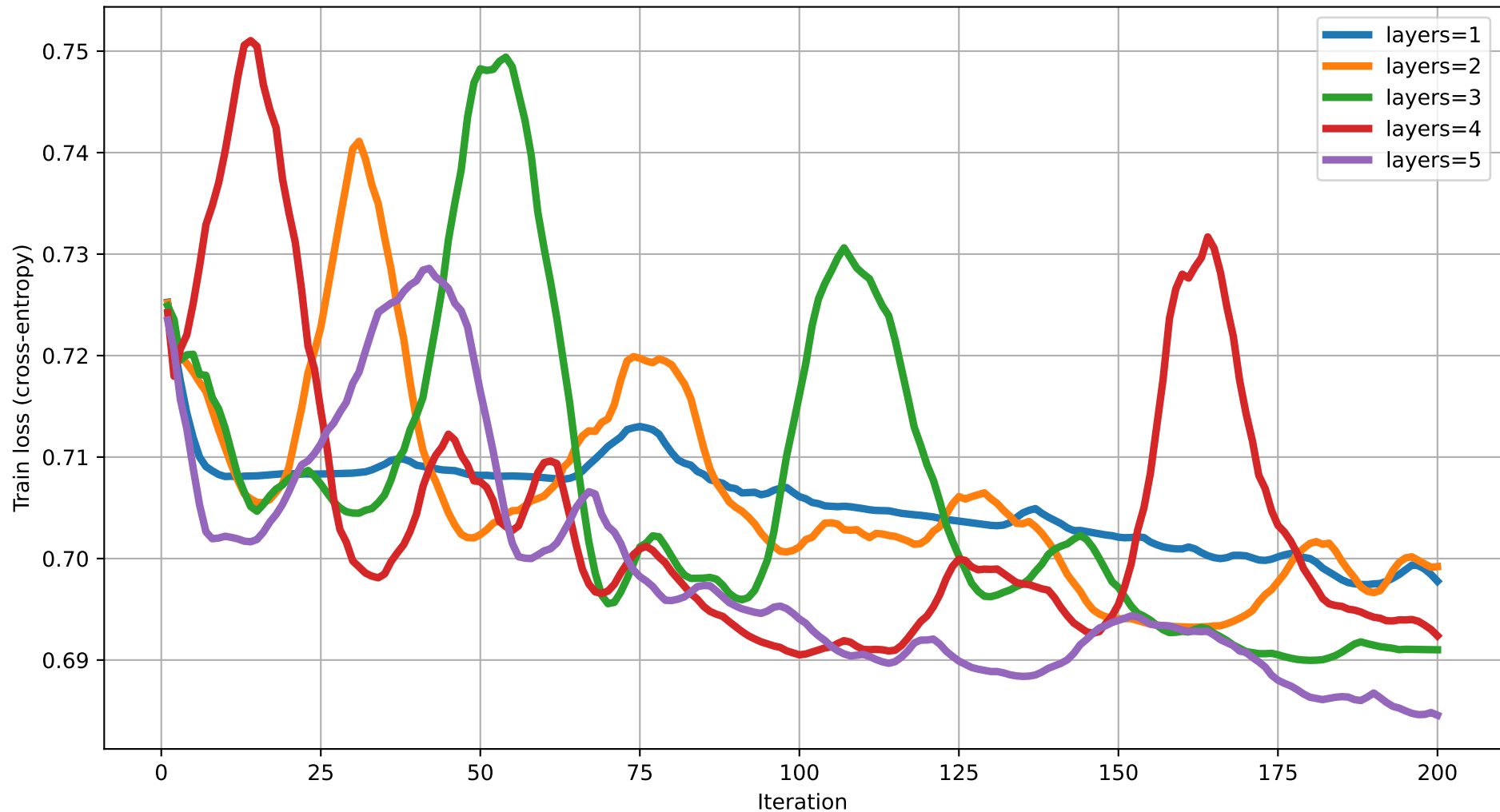
Train loss vs Iteration (dim=10) rot=RX, ent=pairwise, gate=CZ
