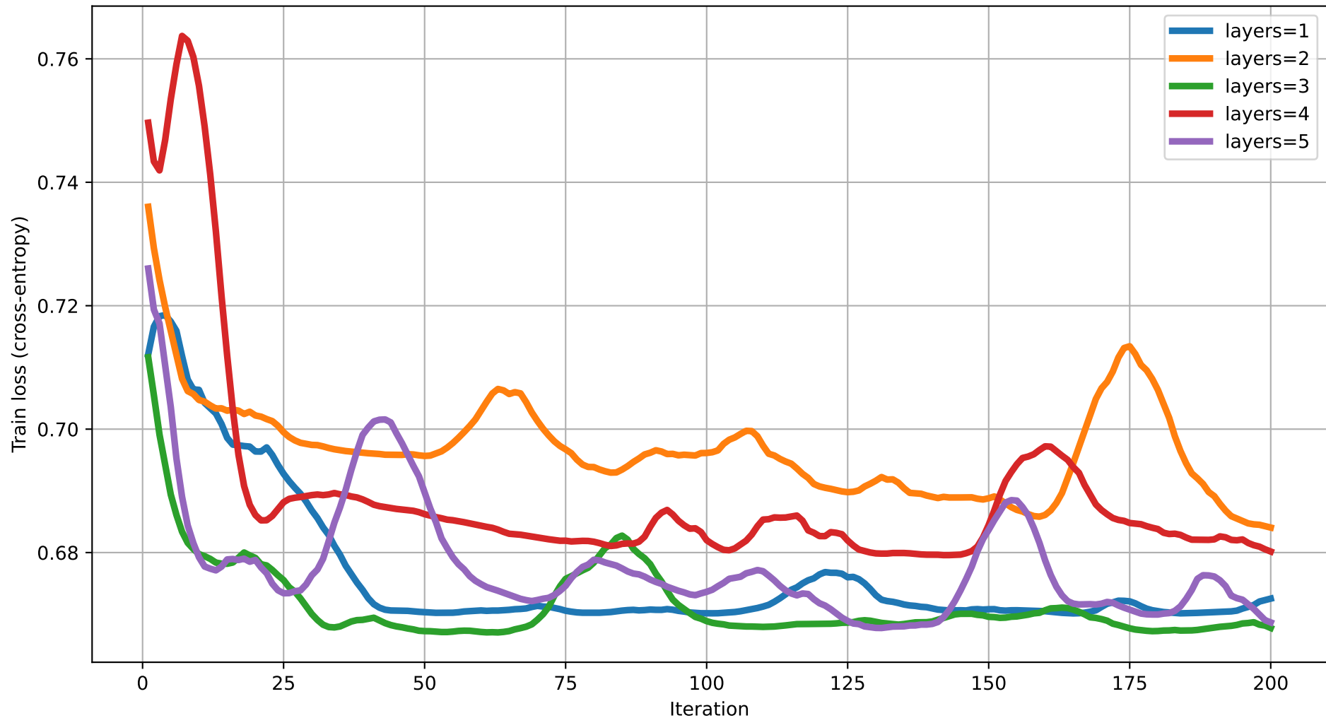
Train loss vs Iteration (dim=19) rot=RZ, ent=ring, gate=IsingXX
