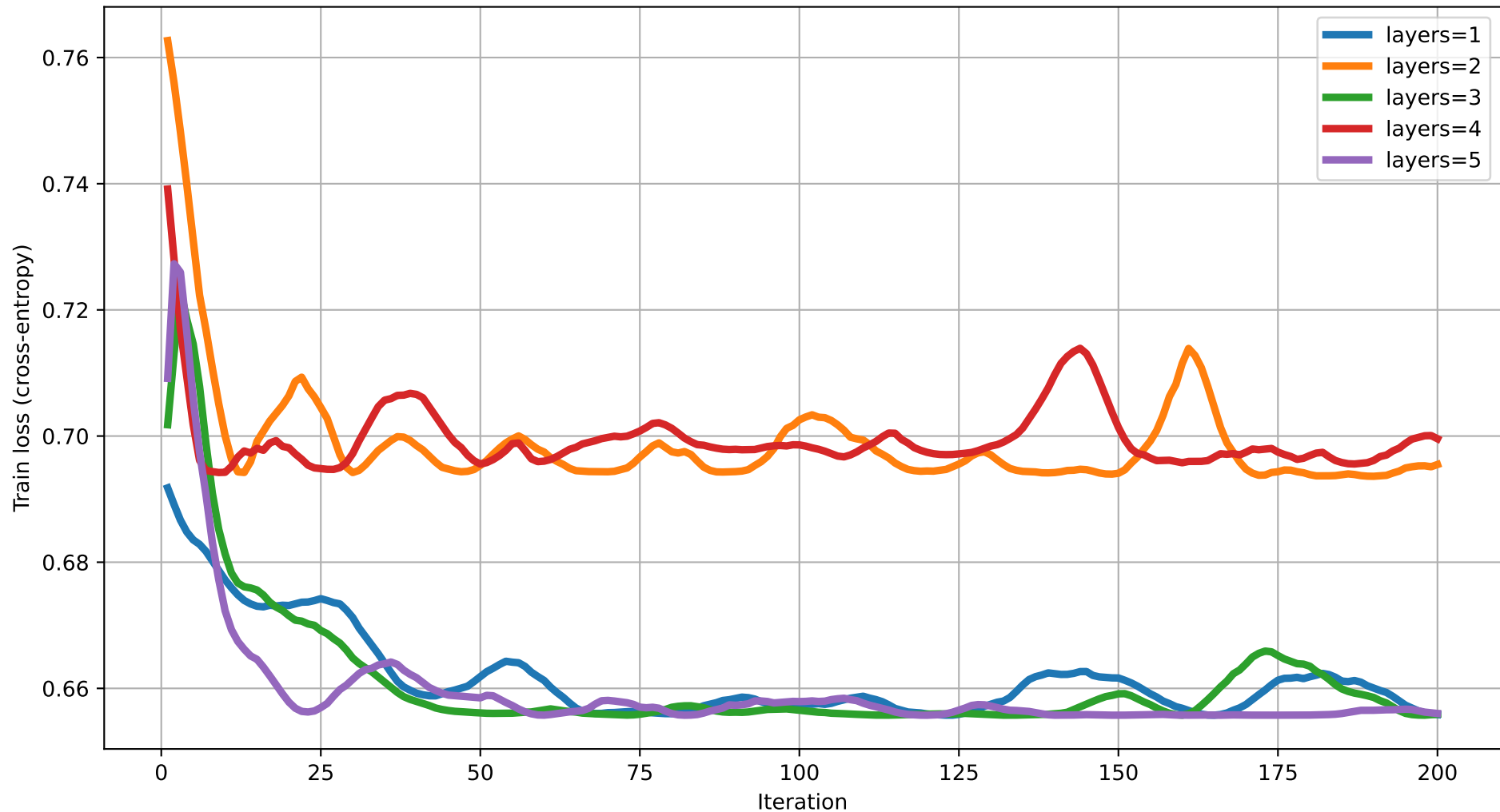
Train loss vs Iteration (degree=5) rot=RX, ent=pairwise, gate=IsingXX
