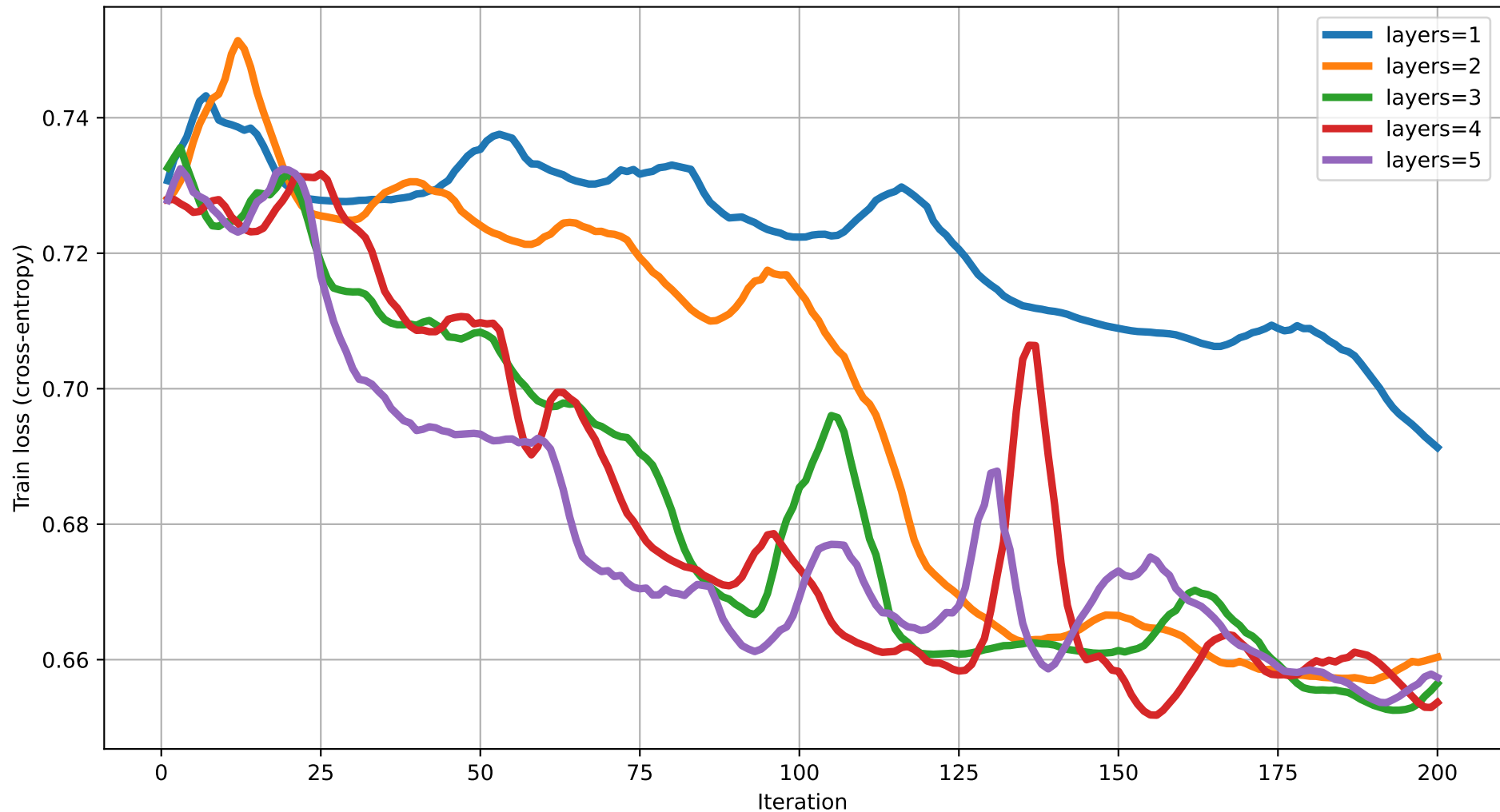
Train loss vs Iteration (dim=7) rot=RYZ, ent=chain, gate=CZ
