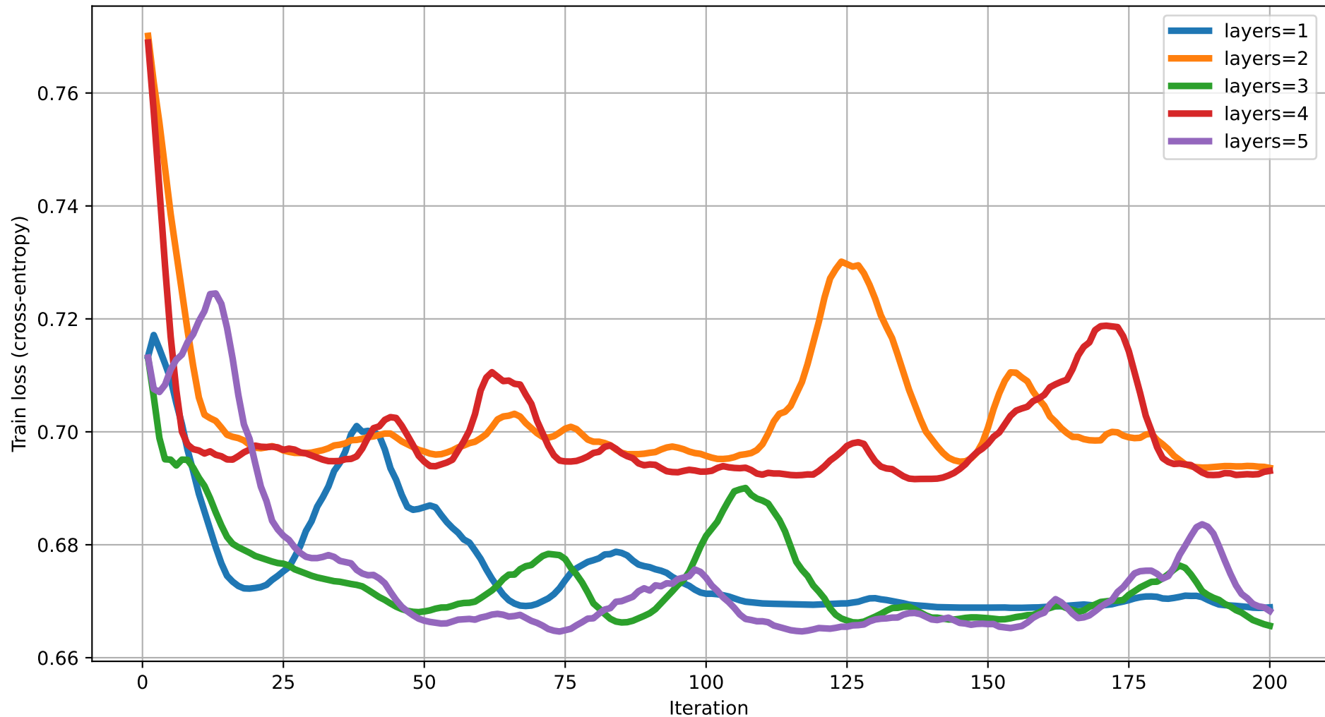
Train loss vs Iteration (dim=17) rot=RZ, ent=ring, gate=IsingXX
