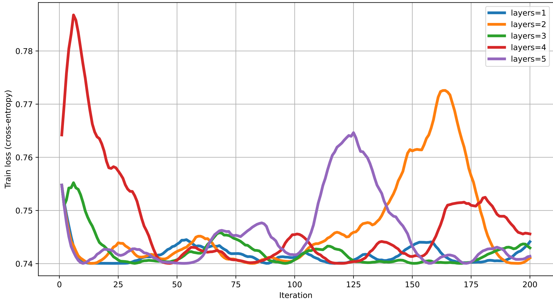
Train loss vs Iteration (dim=5) rot=RZ, ent=ring, gate=CZ
