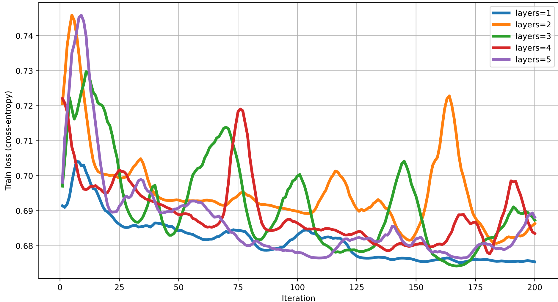
Train loss vs Iteration (dim=12) rot=RZ, ent=pairwise, gate=IsingXX
