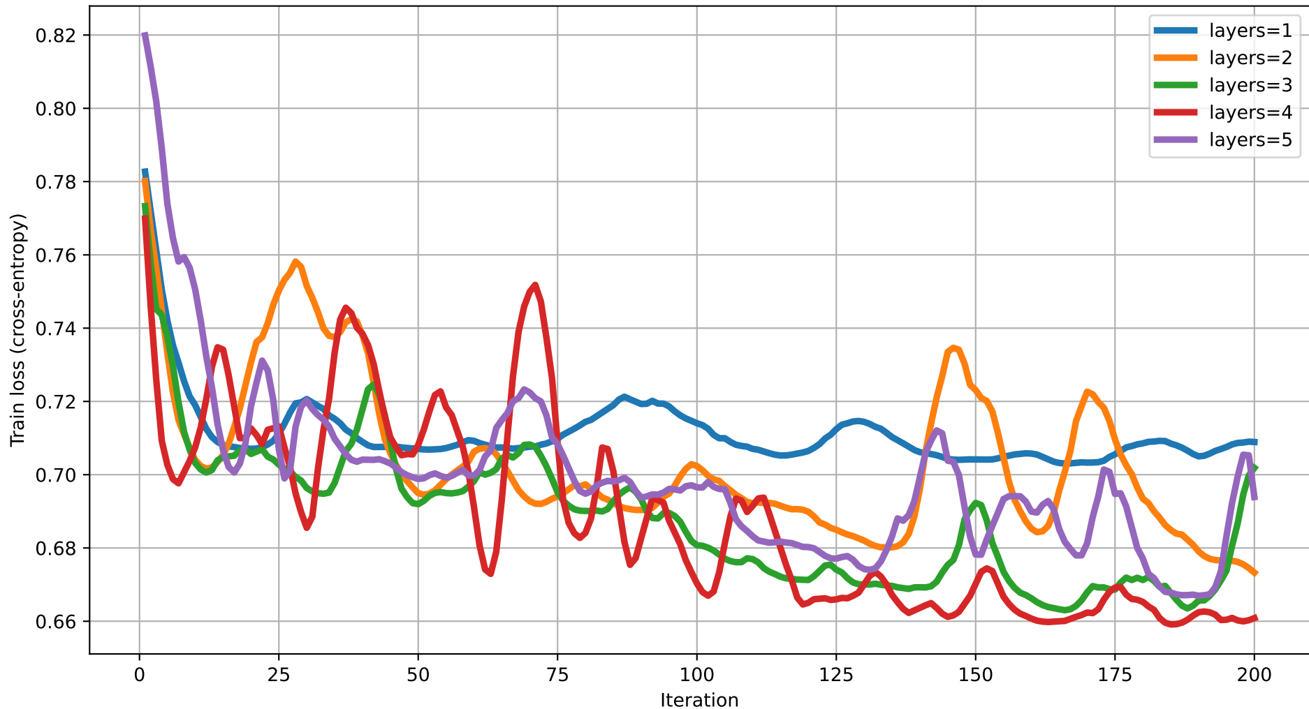
Train loss vs Iteration (dim=9) rot=Rot, ent=pairwise, gate=CNOT
