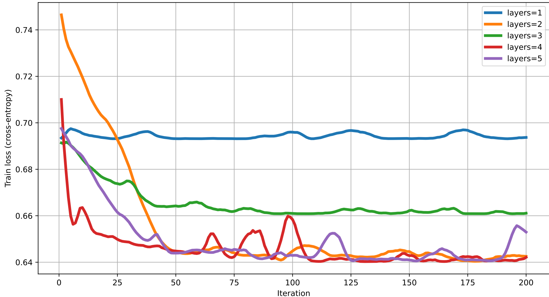
Train loss vs Iteration (degree=3) rot=RY, ent=chain, gate=IsingXX
