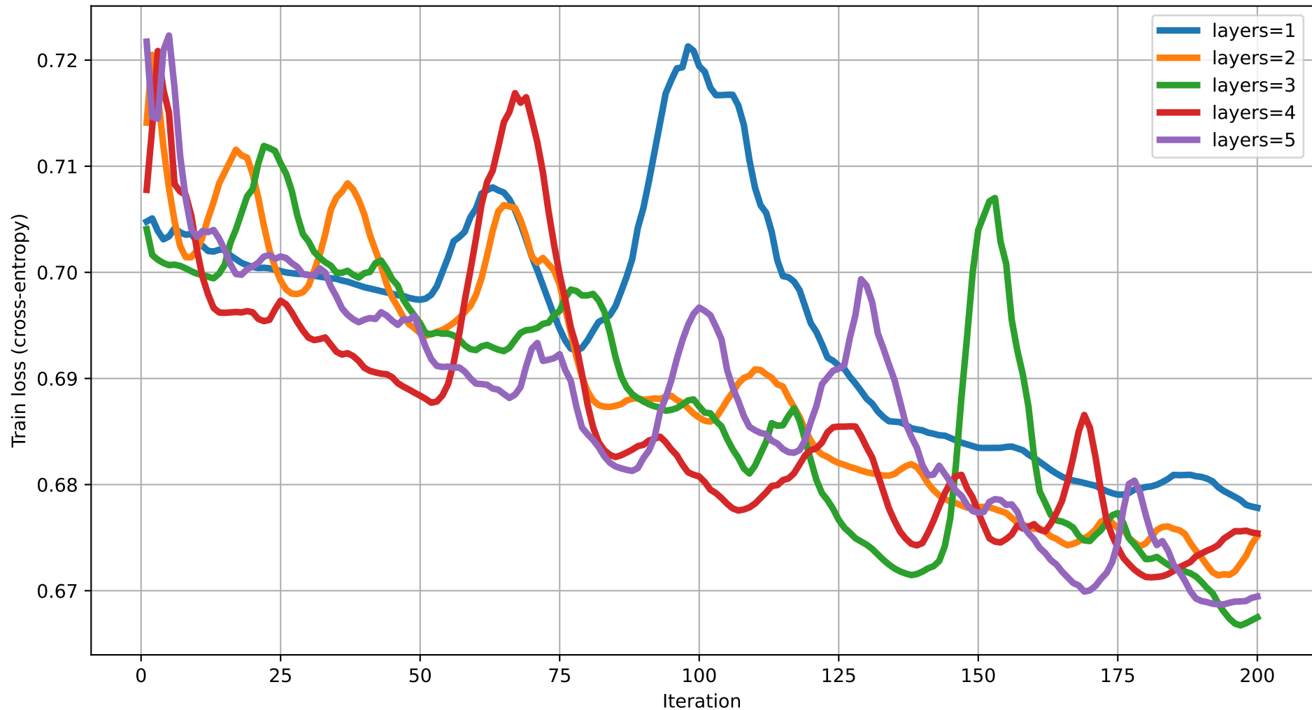
Train loss vs Iteration (dim=14) rot=RYZ, ent=pairwise, gate=CZ
