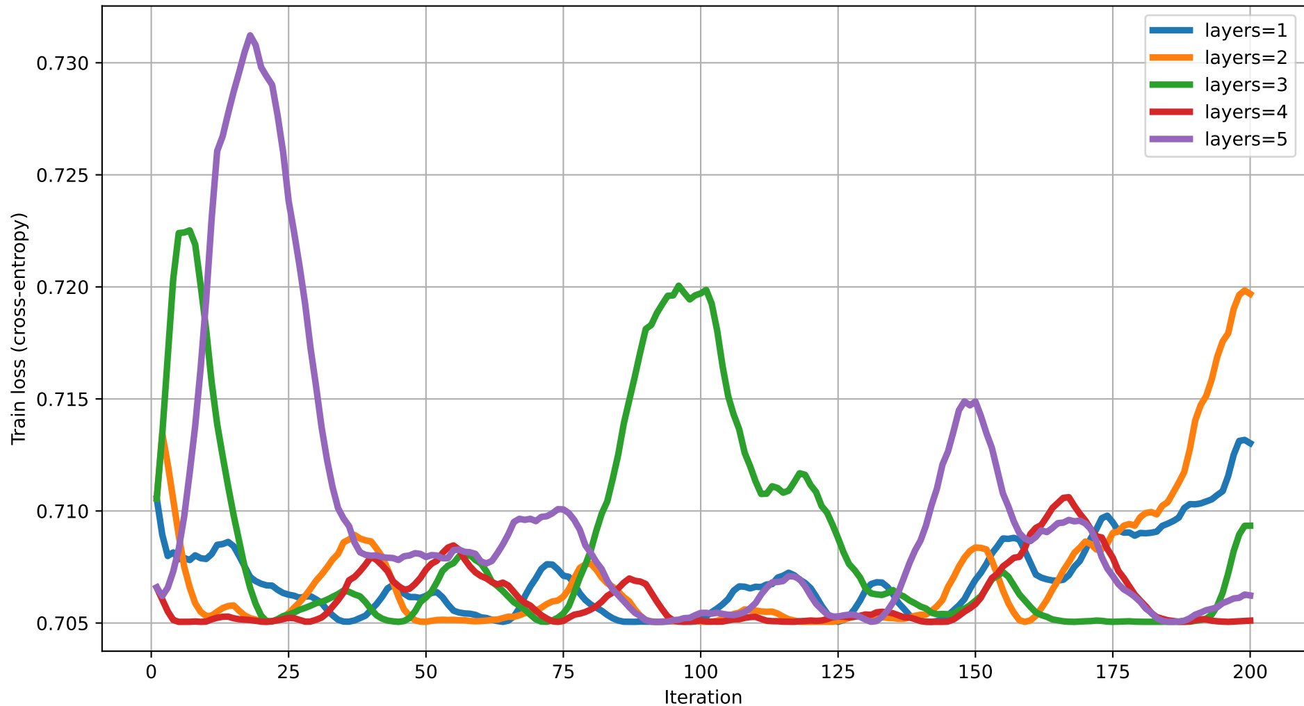
Train loss vs Iteration (dim=14) rot=RZ, ent=pairwise, gate=CZ
