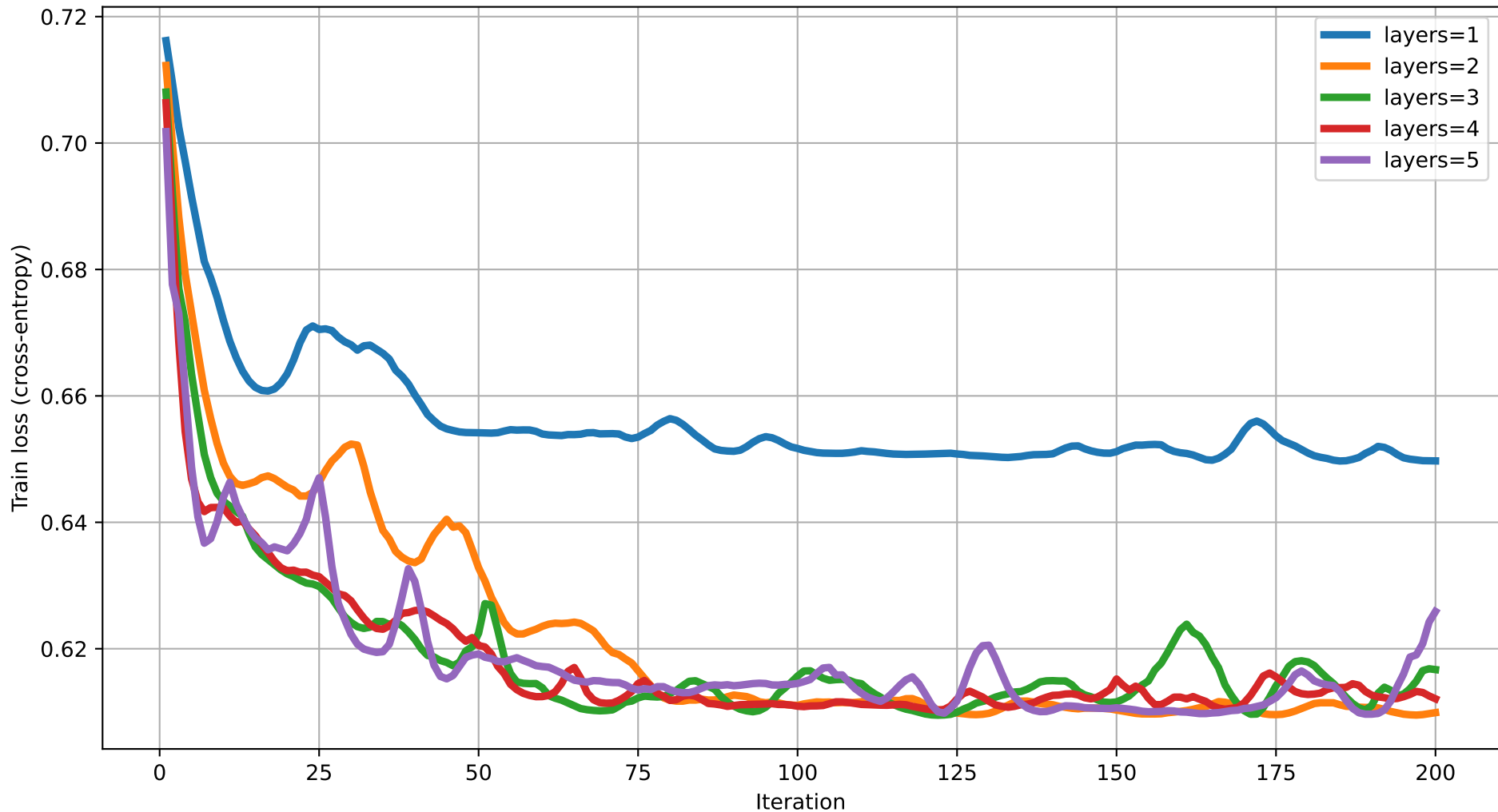
Train loss vs Iteration (degree=4) rot=Rot, ent=pairwise, gate=CNOT
