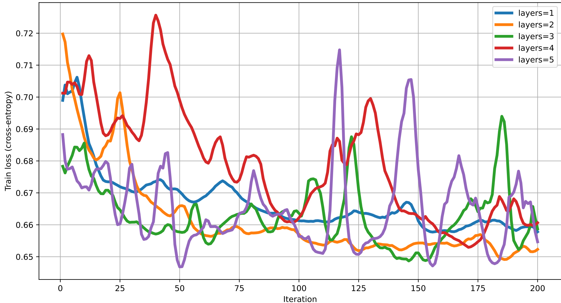
Train loss vs Iteration (dim=6) rot=Rot, ent=full, gate=IsingXX
