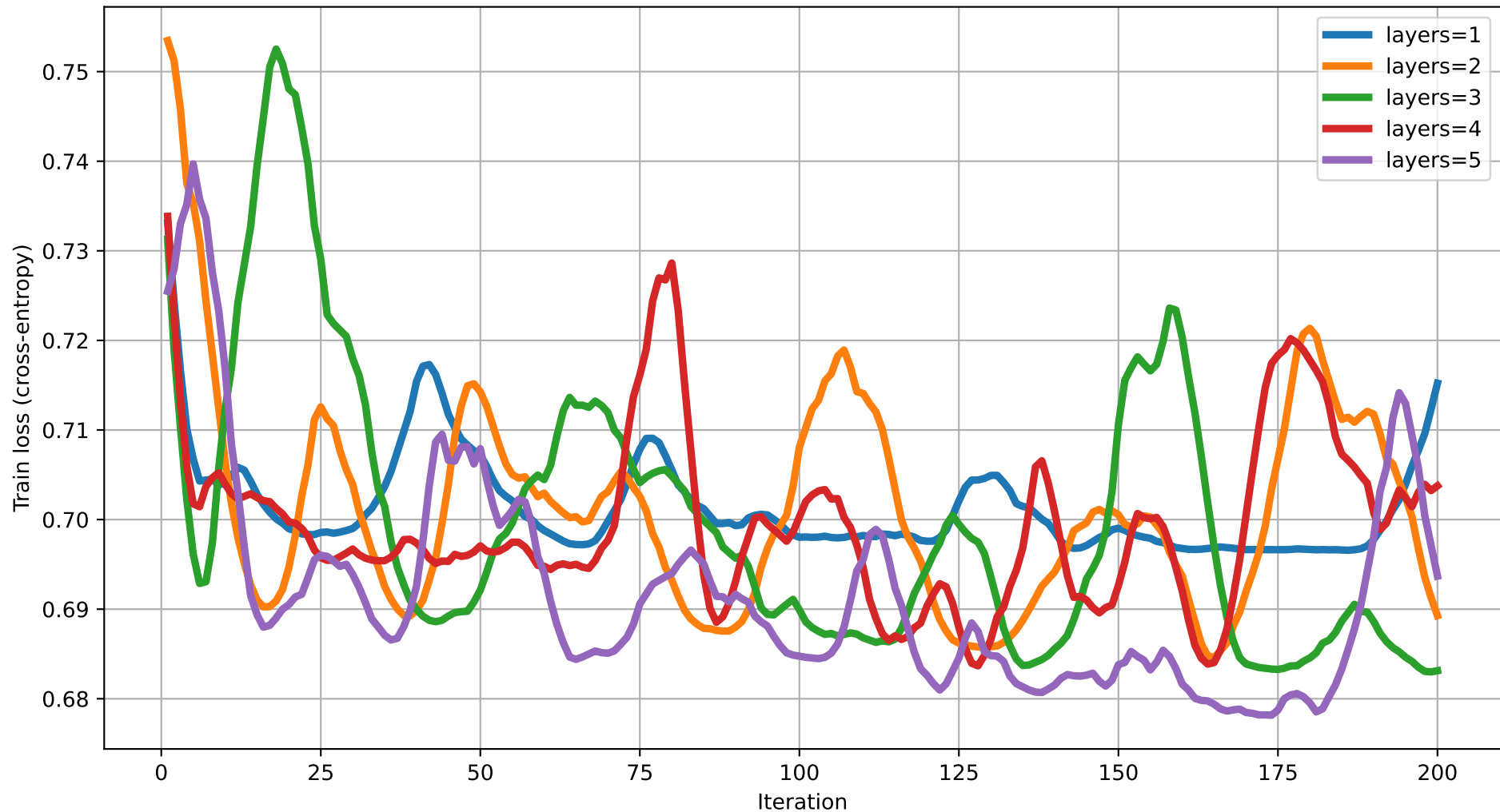
Train loss vs Iteration (dim=18) rot=RY, ent=pairwise, gate=CZ
