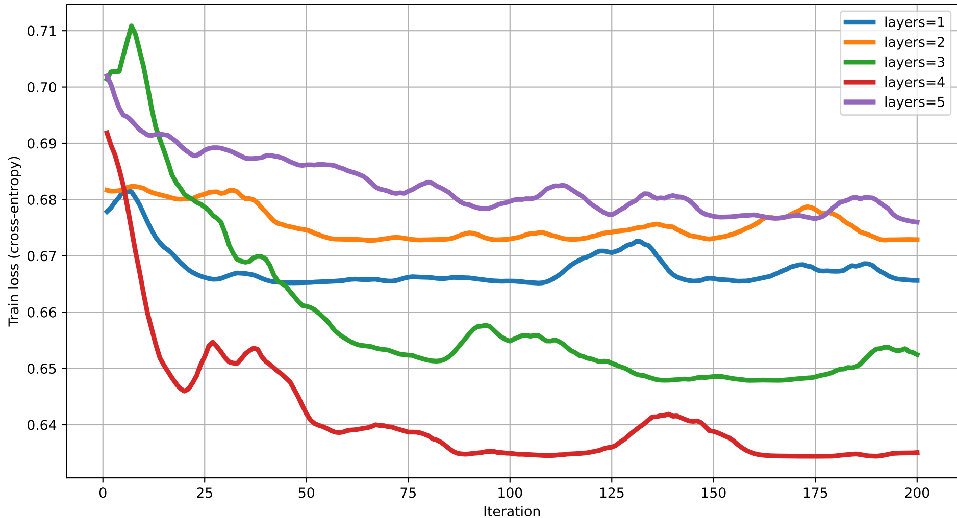
Train loss vs Iteration (degree=4) rot=RX, ent=ring, gate=CNOT
