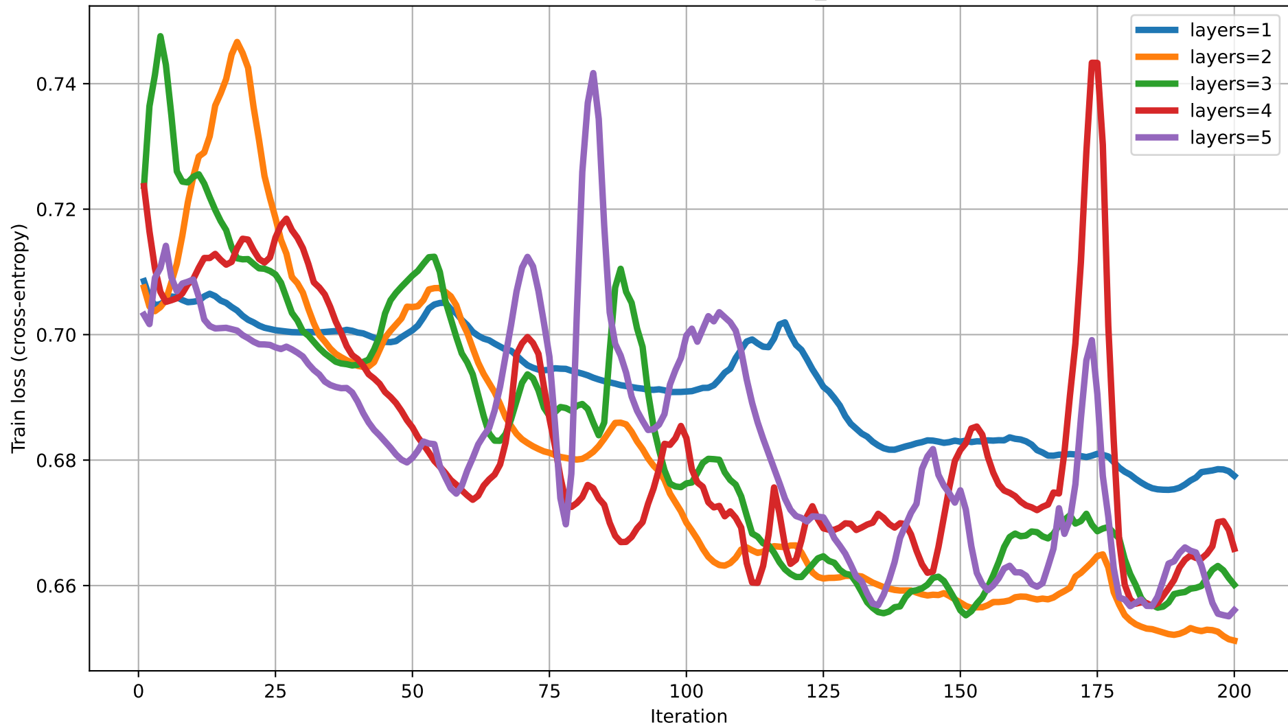
Train loss vs Iteration for different num_layers (dim=6)
