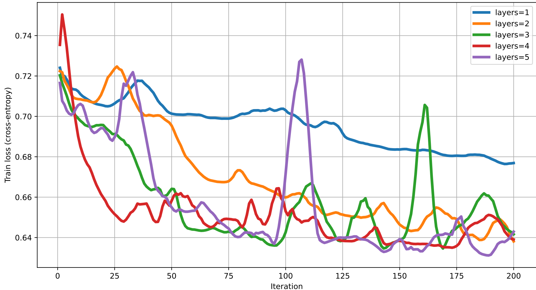
Train loss vs Iteration (dim=6) rot=Rot, ent=chain, gate=CZ
