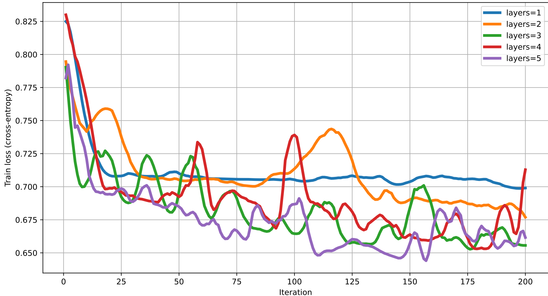
Train loss vs Iteration (dim=8) rot=Rot, ent=chain, gate=CNOT
