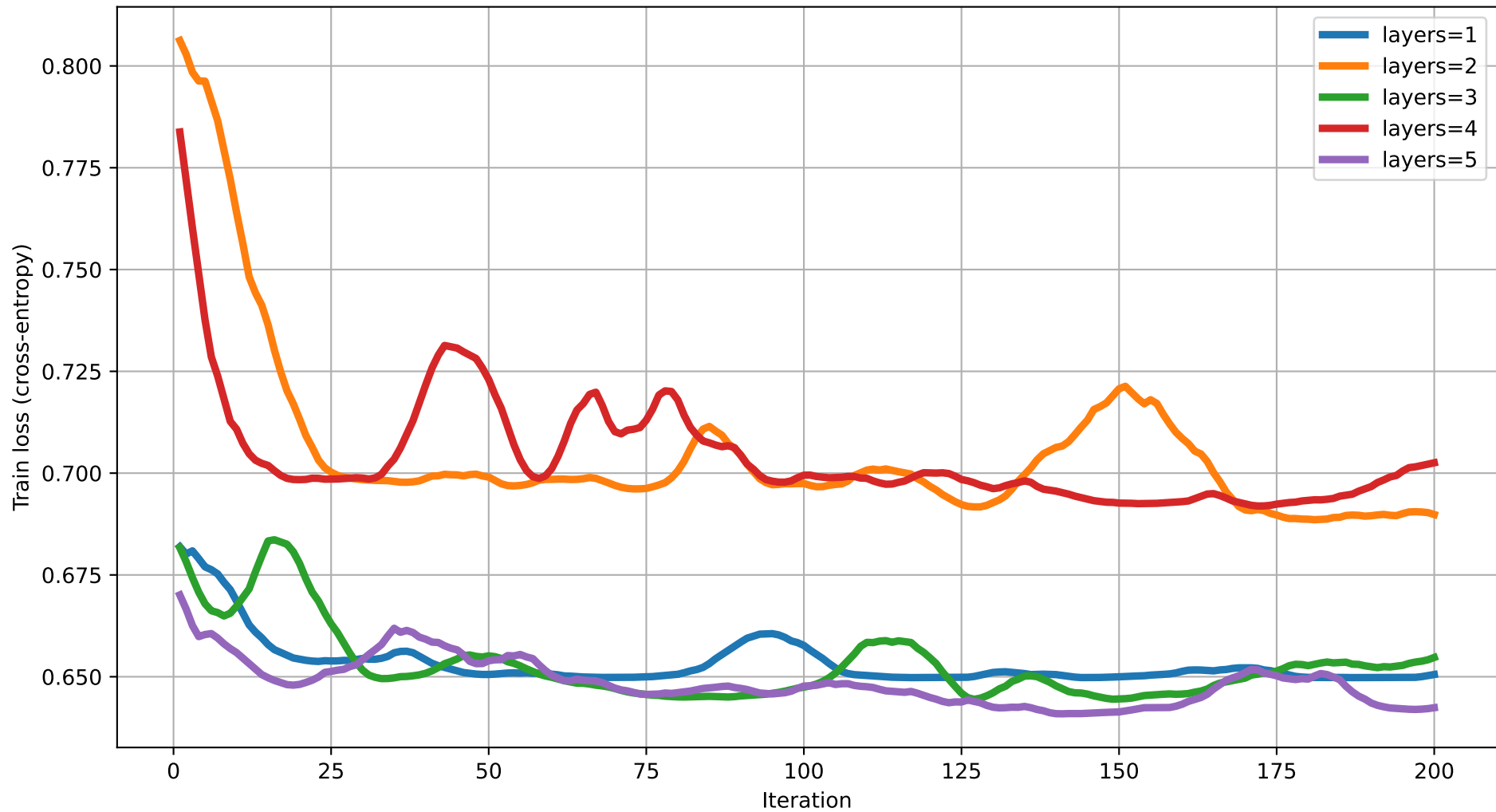
Train loss vs Iteration (dim=9) rot=RZ, ent=ring, gate=IsingXX
