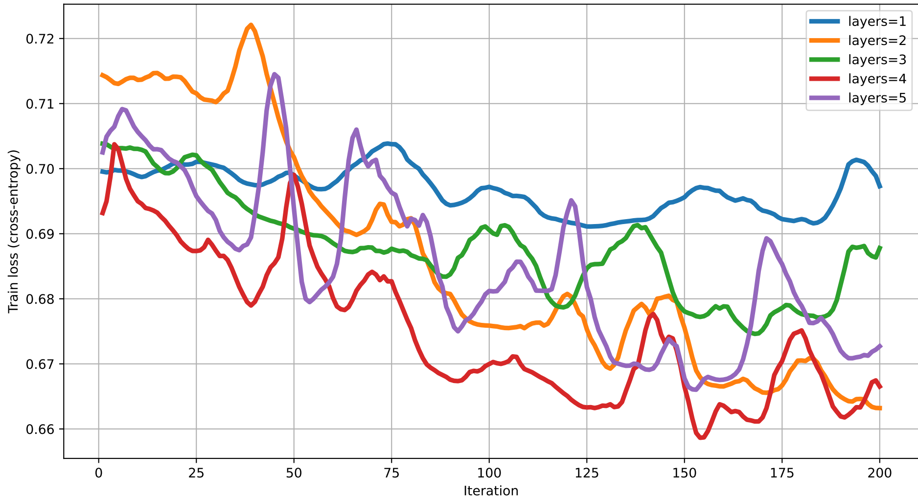
Train loss vs Iteration (dim=17) rot=RY, ent=ring, gate=CNOT
