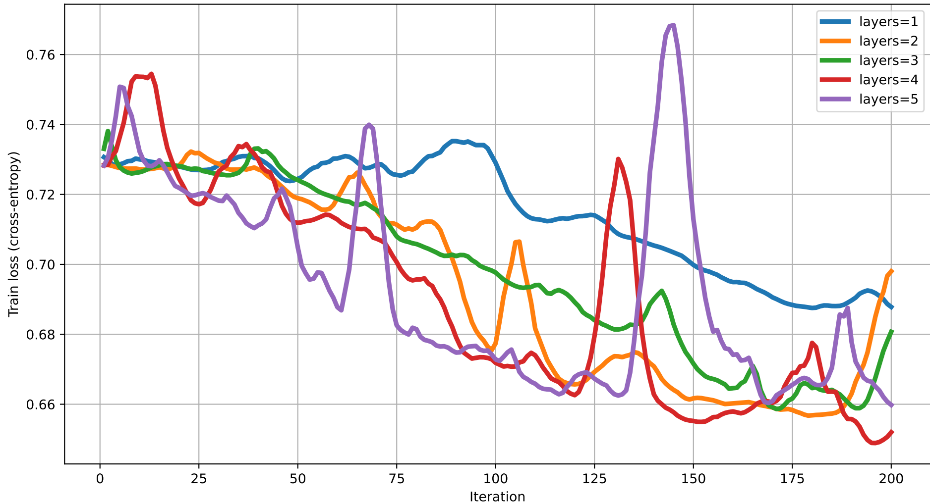
Train loss vs Iteration (dim=7) rot=Rot, ent=ring, gate=CZ
