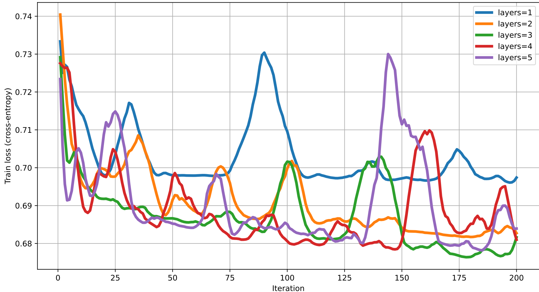
Train loss vs Iteration (dim=19) rot=RYZ, ent=chain, gate=CZ
