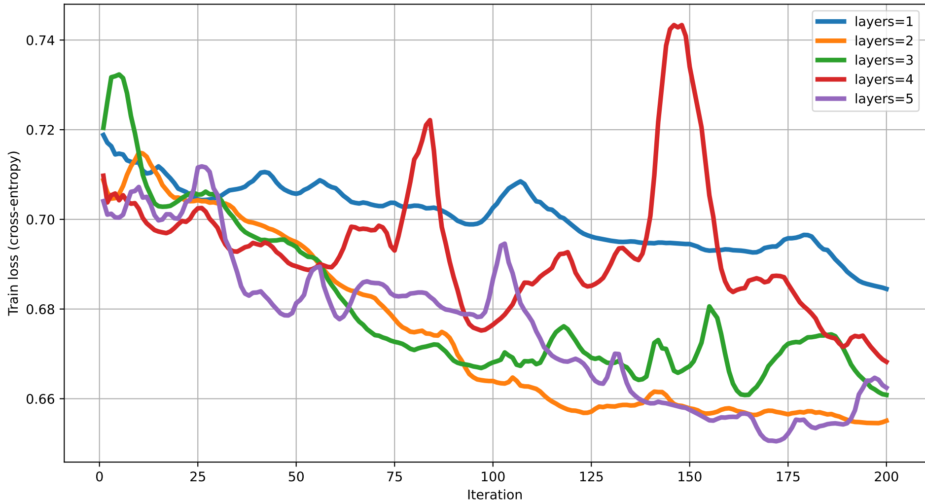
Train loss vs Iteration (dim=6) rot=Rot, ent=ring, gate=CZ
