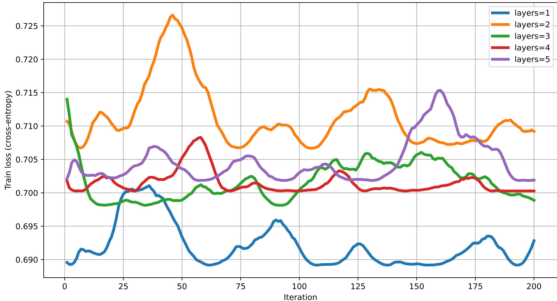
Train loss vs Iteration (dim=13) rot=RZ, ent=ring, gate=CNOT
