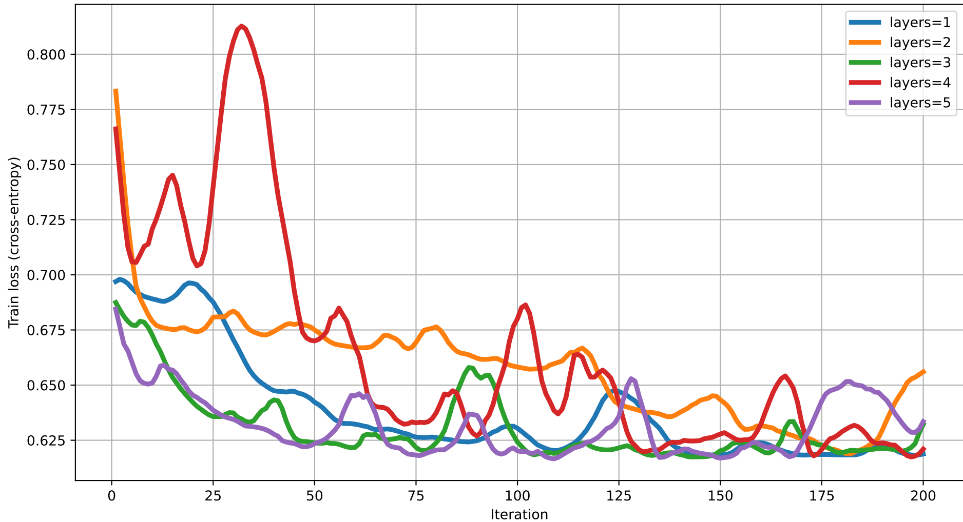
Train loss vs Iteration (dim=4) rot=RYZ, ent=pairwise, gate=IsingXX
