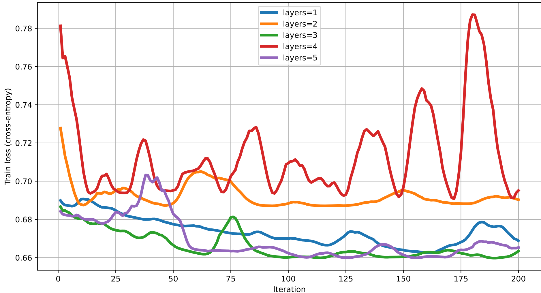
Train loss vs Iteration (dim=9) rot=RX, ent=pairwise, gate=IsingXX
