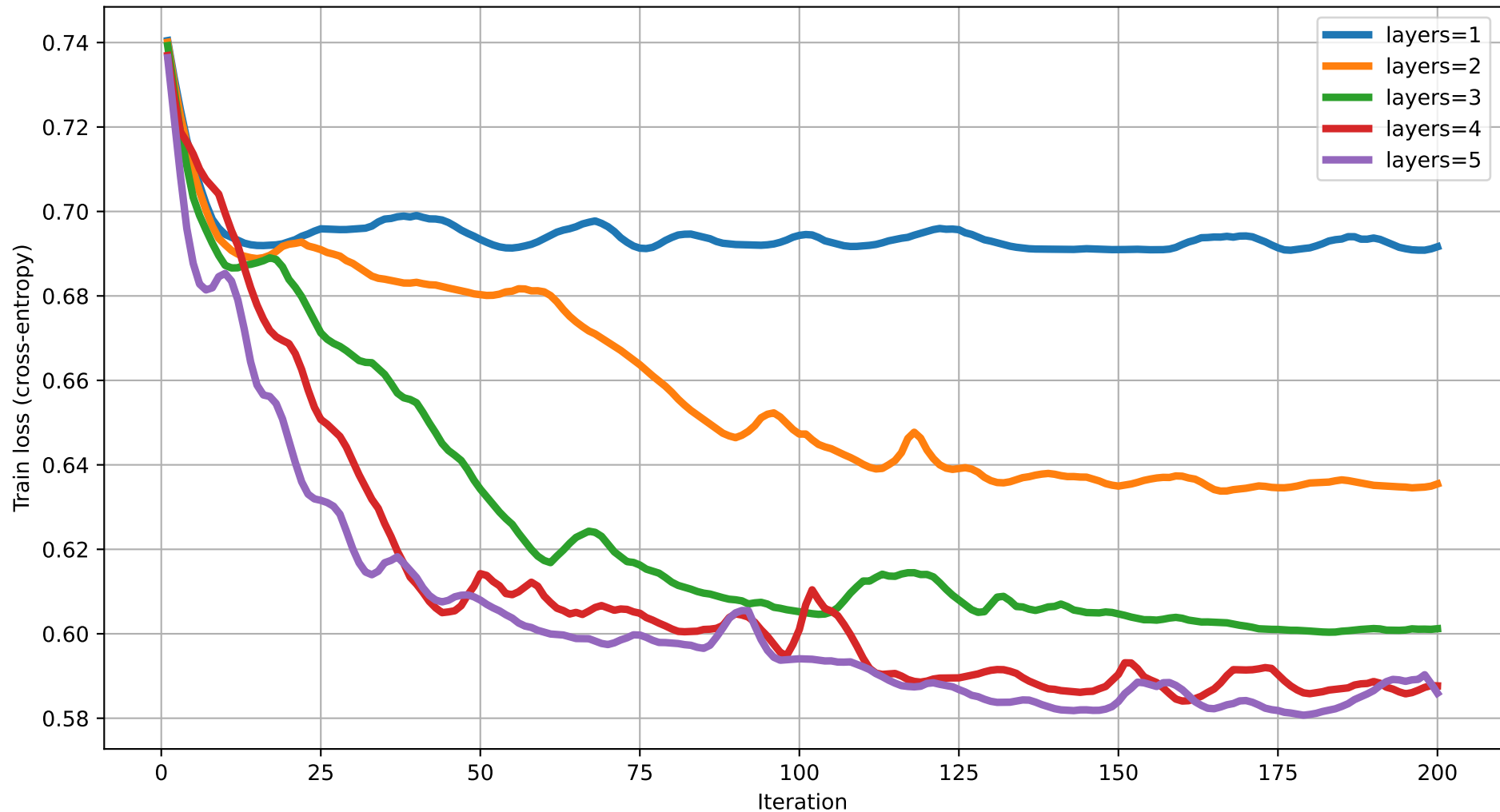
Train loss vs Iteration (degree=5) rot=Rot, ent=full, gate=CZ
