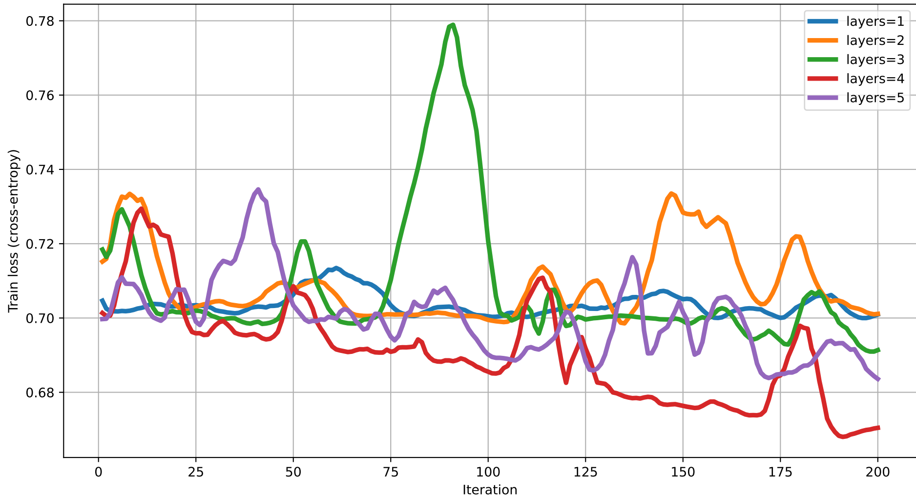
Train loss vs Iteration (dim=12) rot=Rot, ent=pairwise, gate=CNOT
