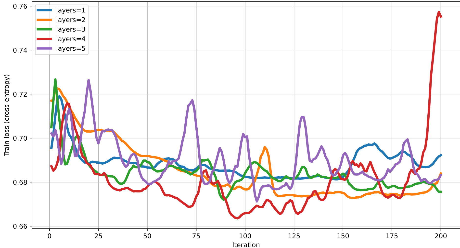
Train loss vs Iteration (dim=15) rot=Rot, ent=full, gate=IsingXX
