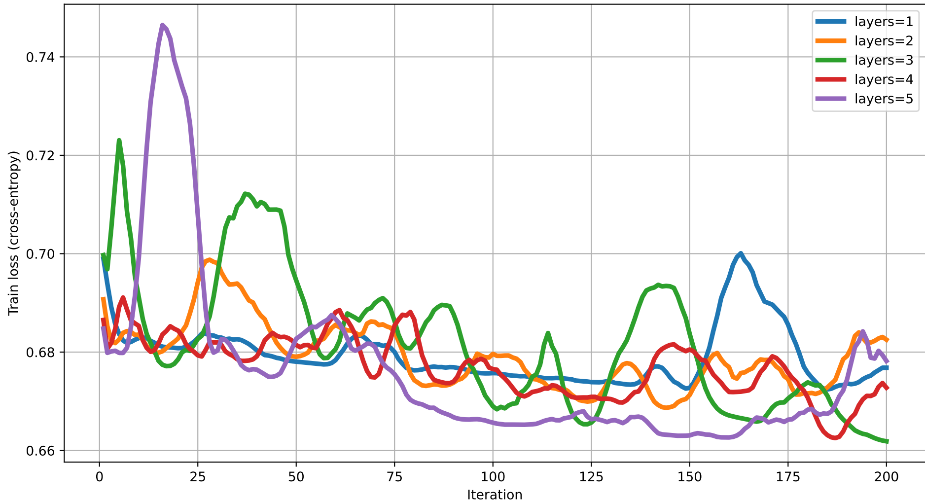
Train loss vs Iteration (dim=13) rot=RYZ, ent=pairwise, gate=CNOT
