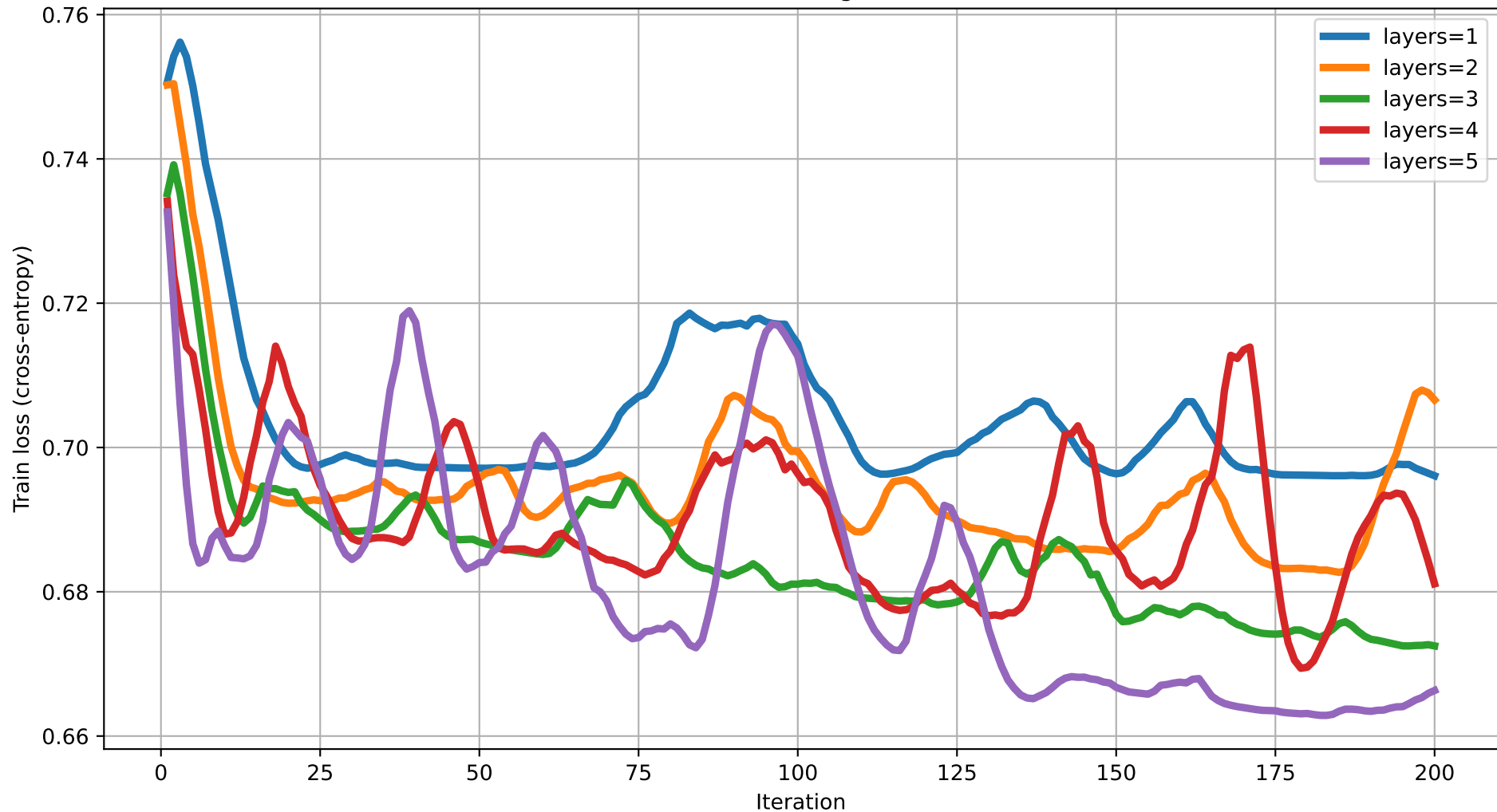
Train loss vs Iteration (dim=19) rot=RX, ent=full, gate=CNOT
