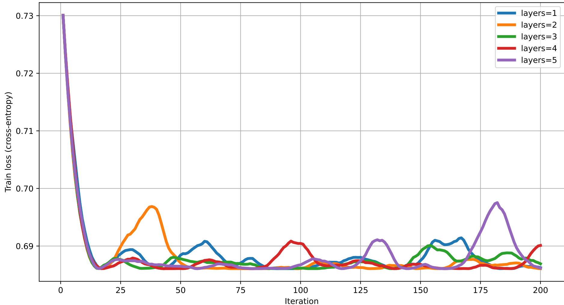
Train loss vs Iteration (degree=2) rot=RZ, ent=chain, gate=CZ
