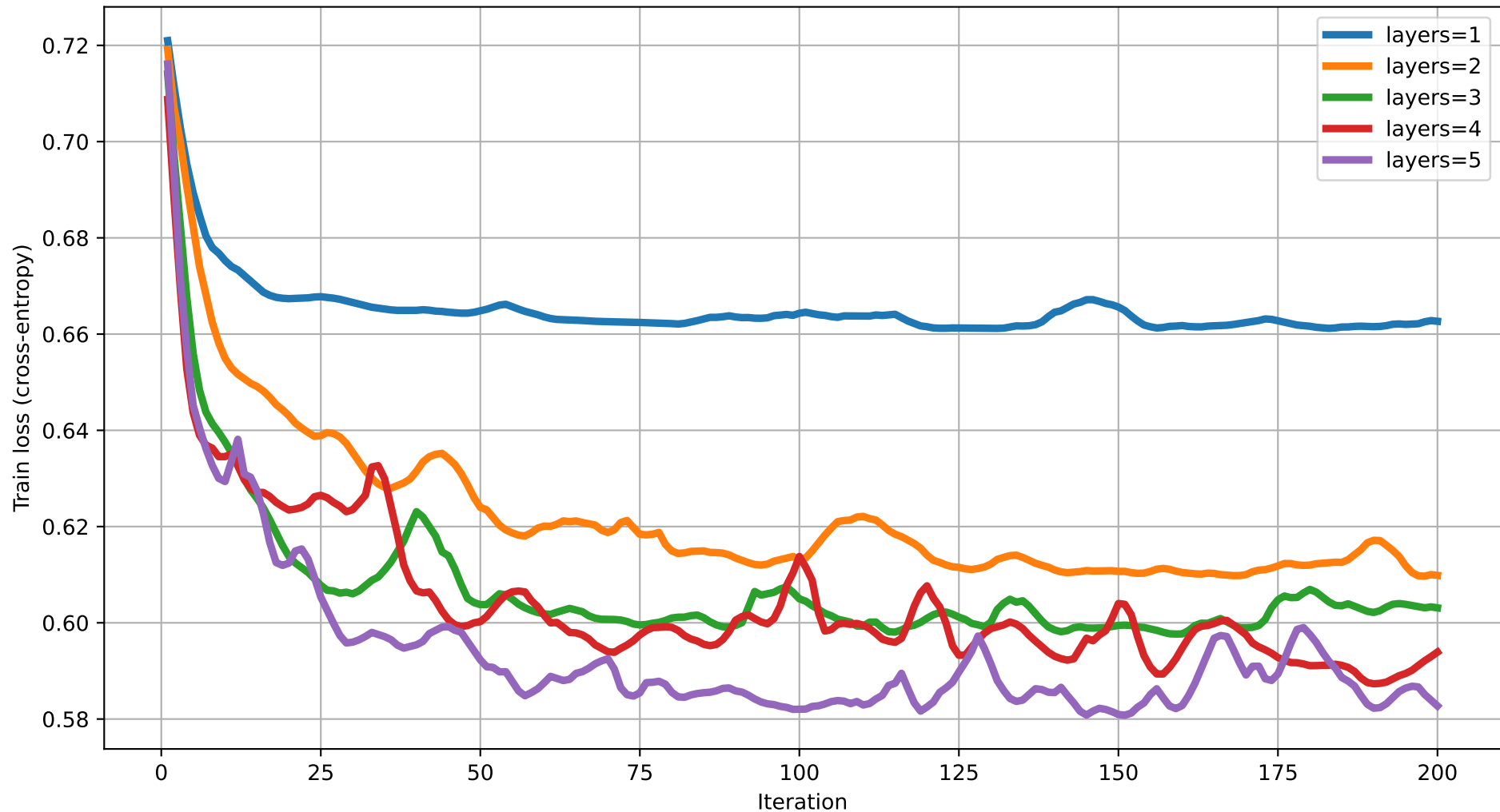
Train loss vs Iteration (degree=3) rot=Rot, ent=full, gate=CNOT
