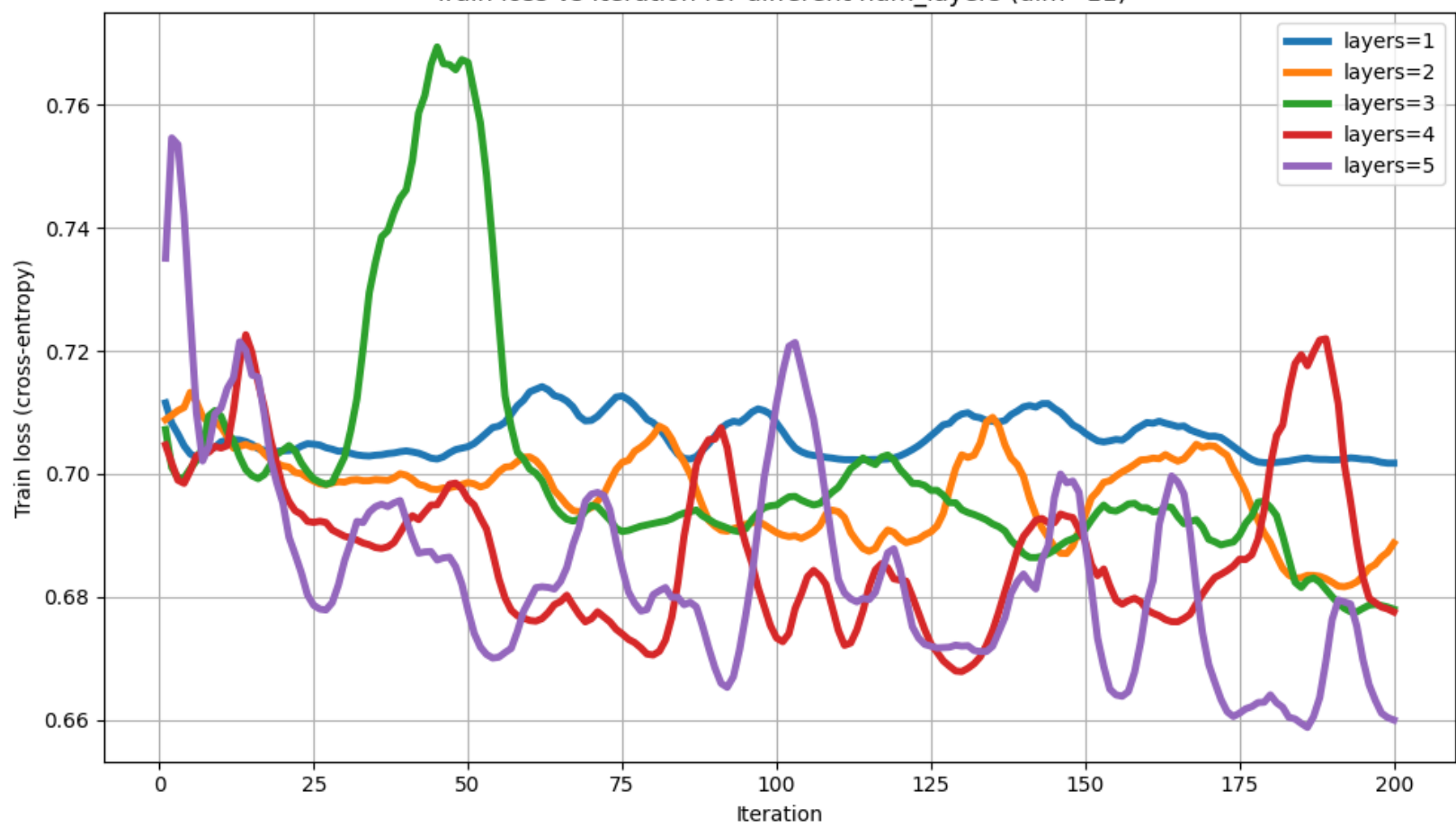
Train loss vs Iteration for different num_layers (dim=11)
