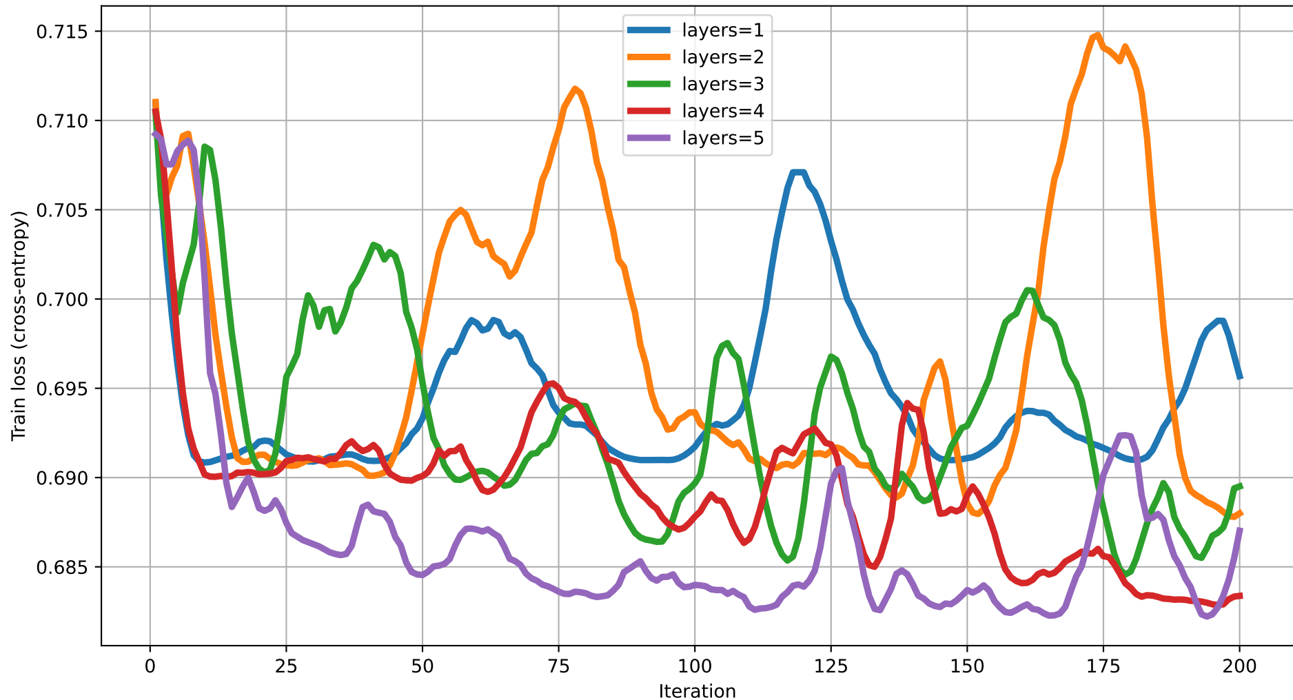
Train loss vs Iteration (dim=20) rot=RX, ent=pairwise, gate=CZ
