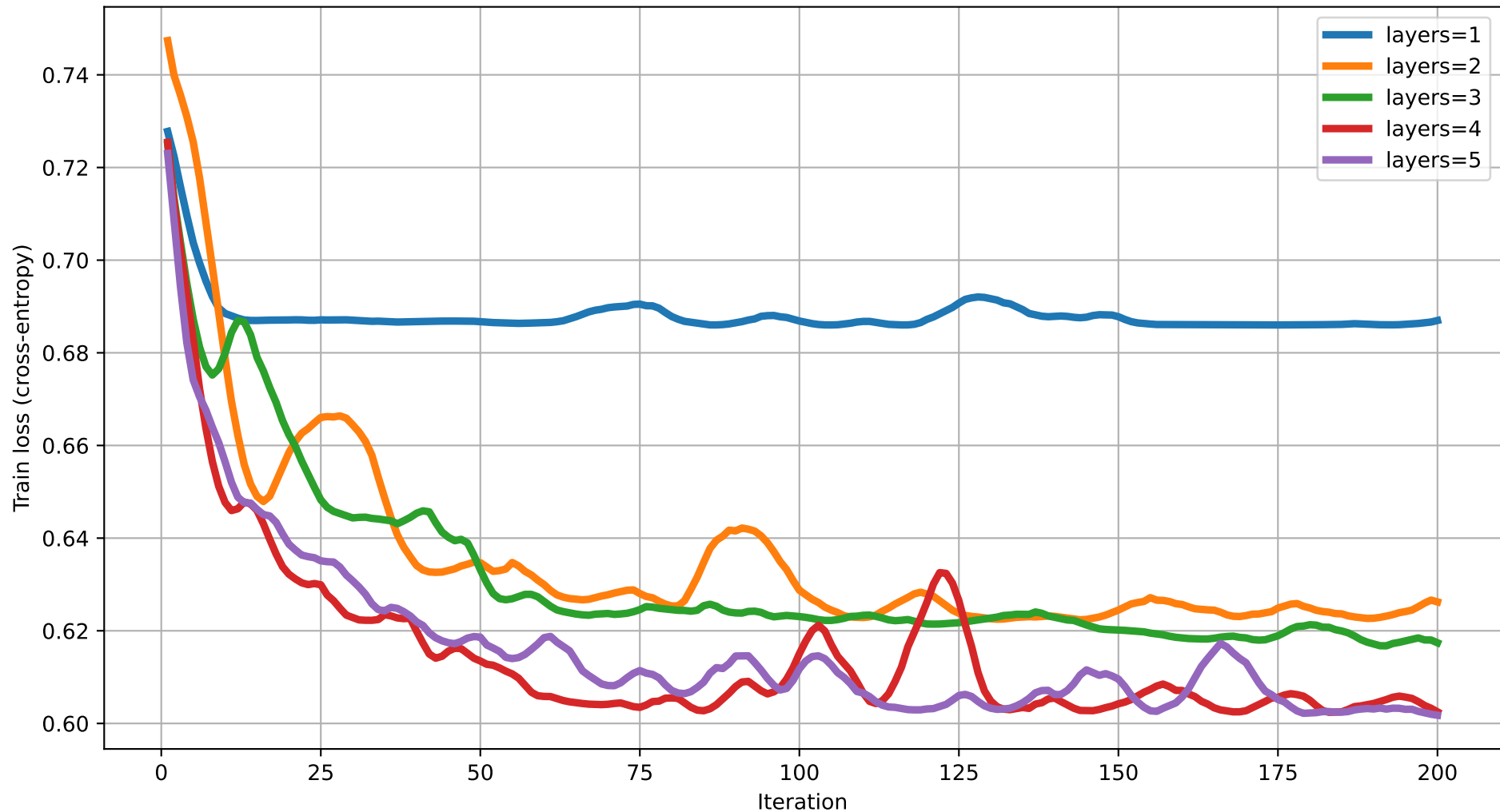
Train loss vs Iteration (degree=2) rot=RY, ent=full, gate=CZ
