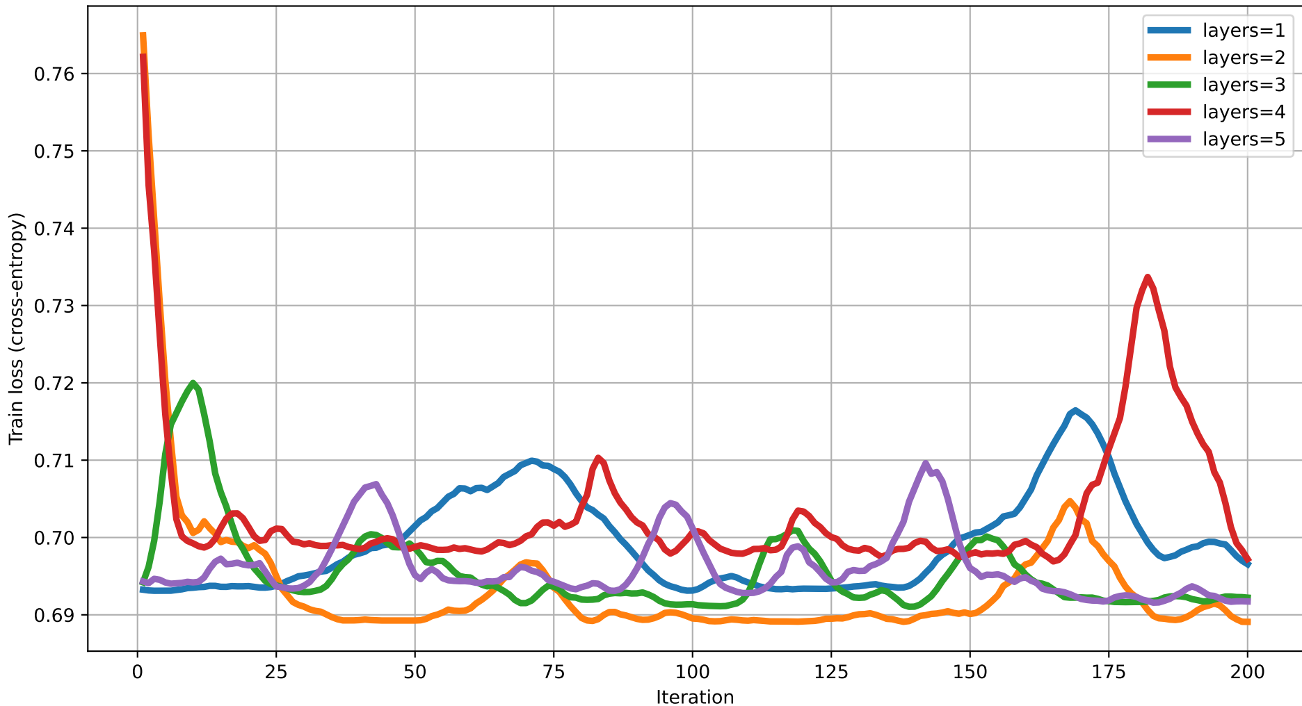
Train loss vs Iteration (dim=17) rot=RY, ent=pairwise, gate=IsingXX
