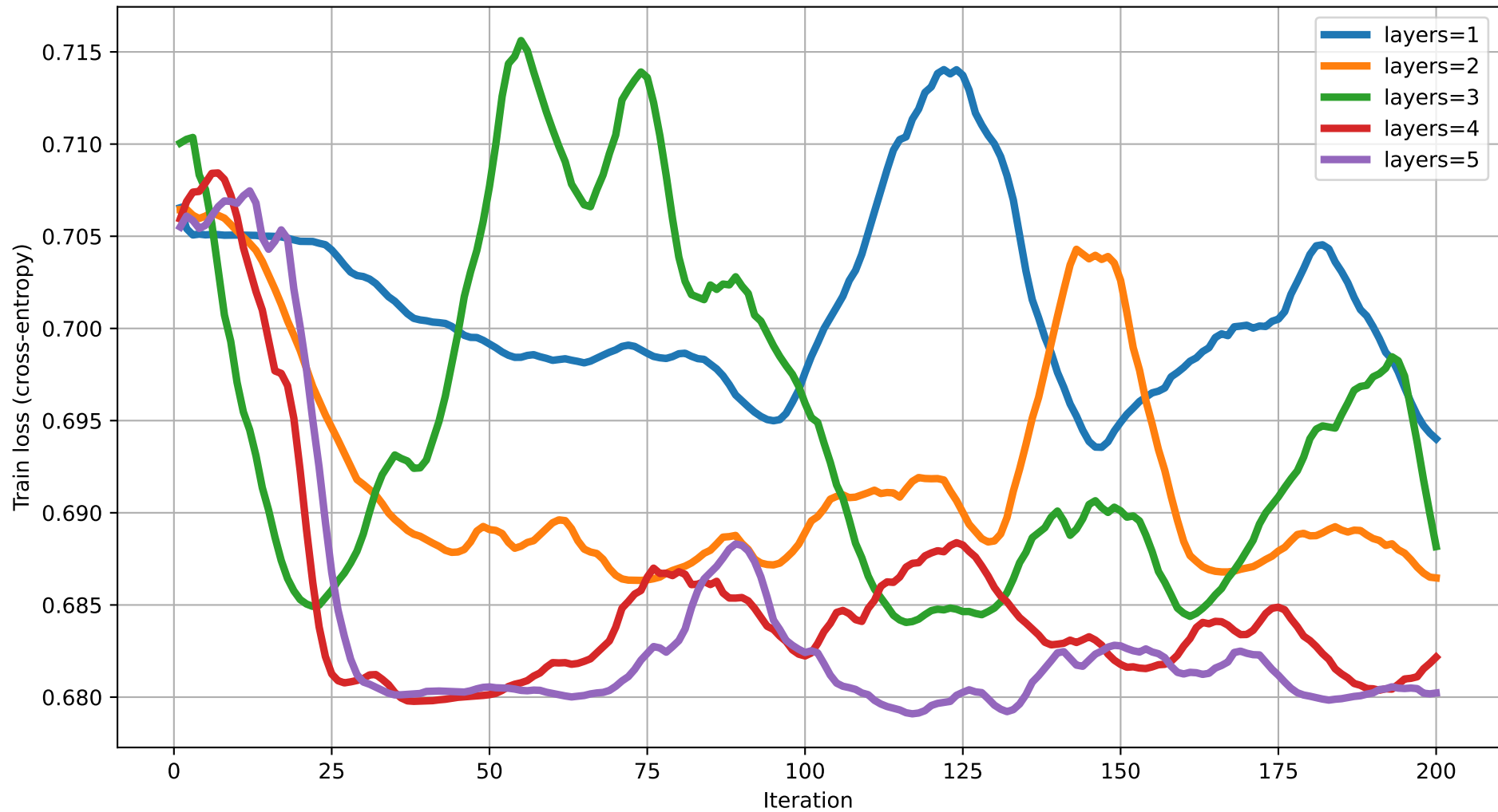
Train loss vs Iteration (dim=14) rot=RX, ent=full, gate=CNOT
