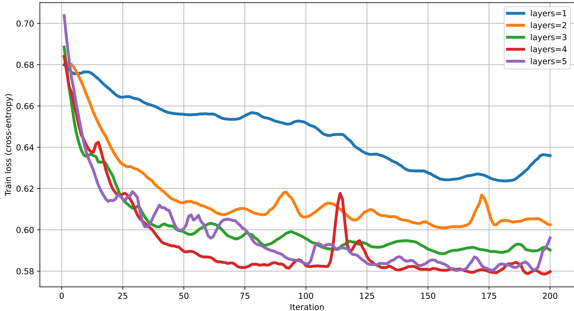
Train loss vs Iteration (degree=4) rot=Rot, ent=ring, gate=CNOT
