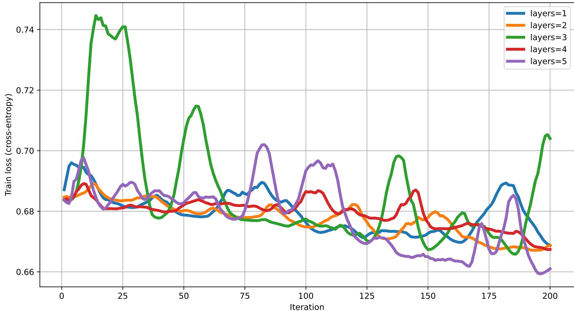
Train loss vs Iteration (dim=15) rot=RY, ent=full, gate=CZ
