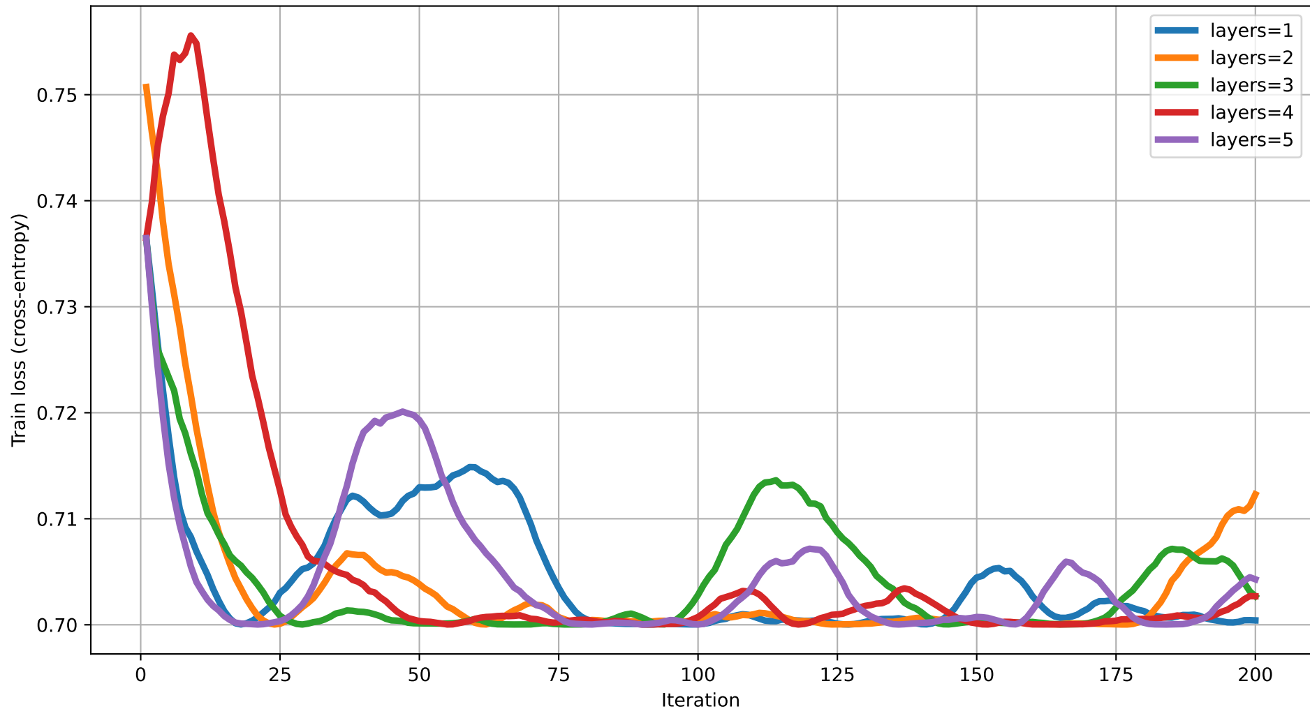
Train loss vs Iteration (dim=19) rot=RZ, ent=chain, gate=CZ
