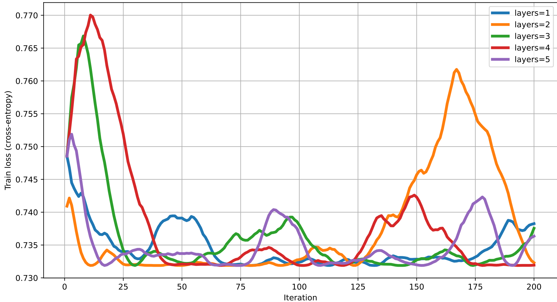
Train loss vs Iteration (dim=3) rot=RZ, ent=full, gate=CNOT
