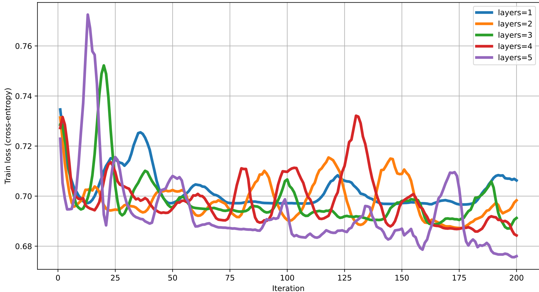
Train loss vs Iteration (dim=18) rot=Rot, ent=pairwise, gate=CNOT
