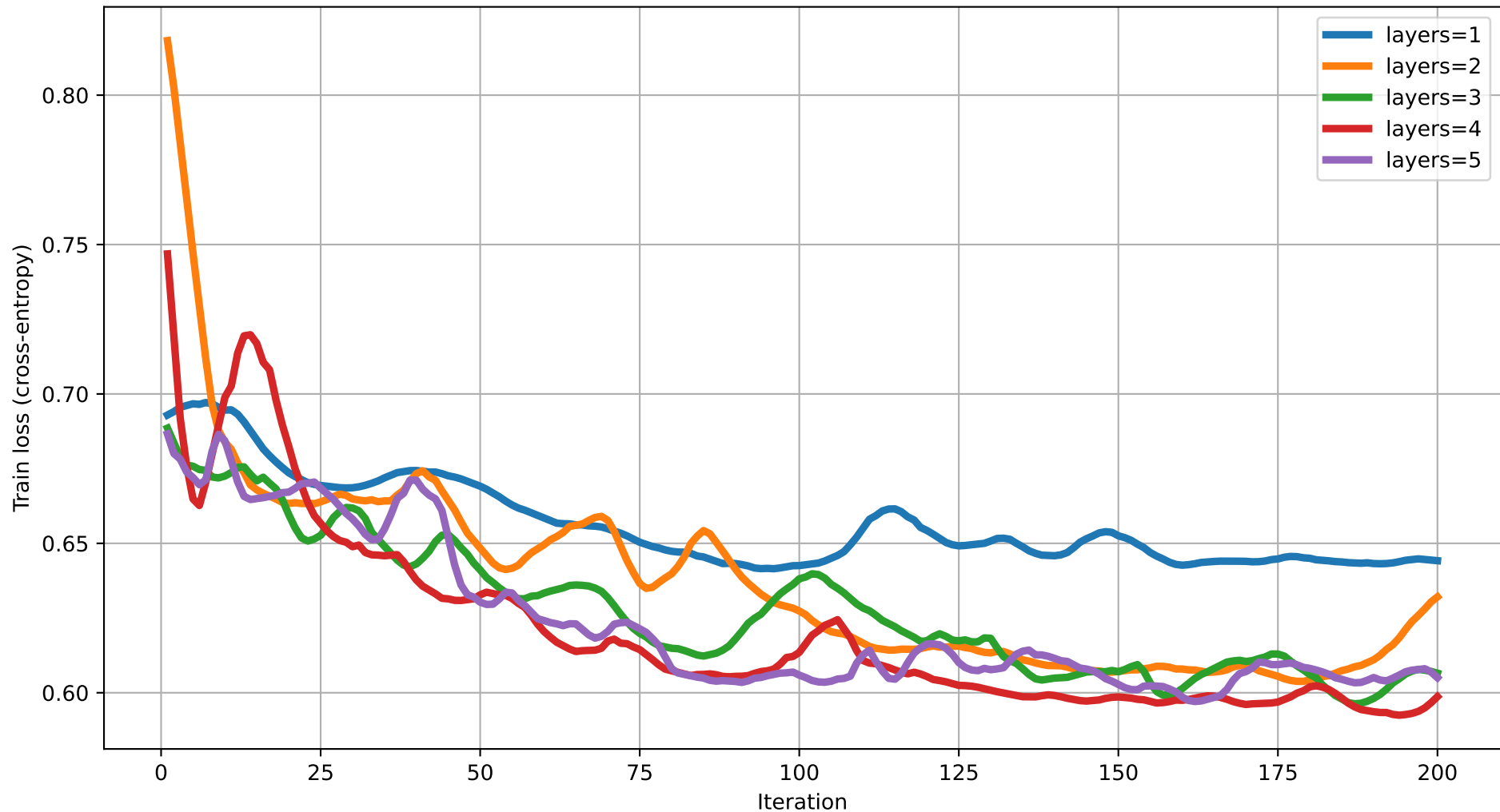
Train loss vs Iteration (dim=8) rot=RYZ, ent=full, gate=IsingXX
