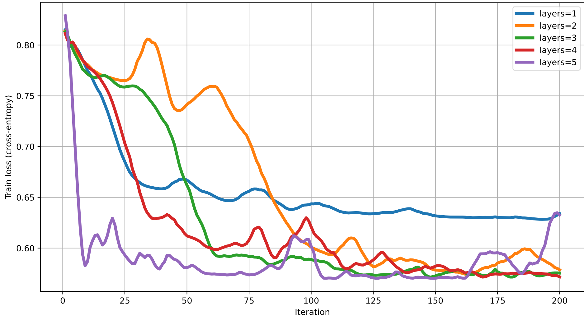
Train loss vs Iteration (dim=2) rot=Rot, ent=chain, gate=CNOT
