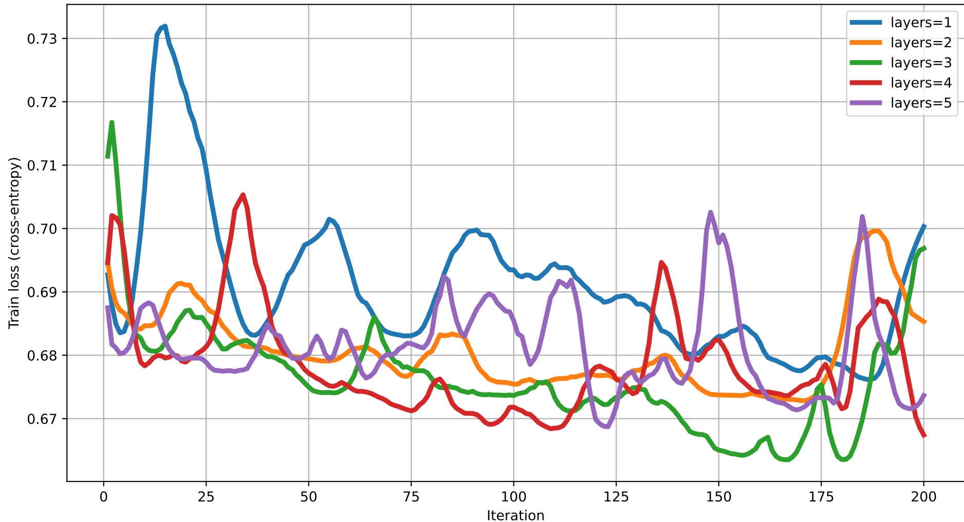
Train loss vs Iteration (dim=13) rot=Rot, ent=ring, gate=CZ
