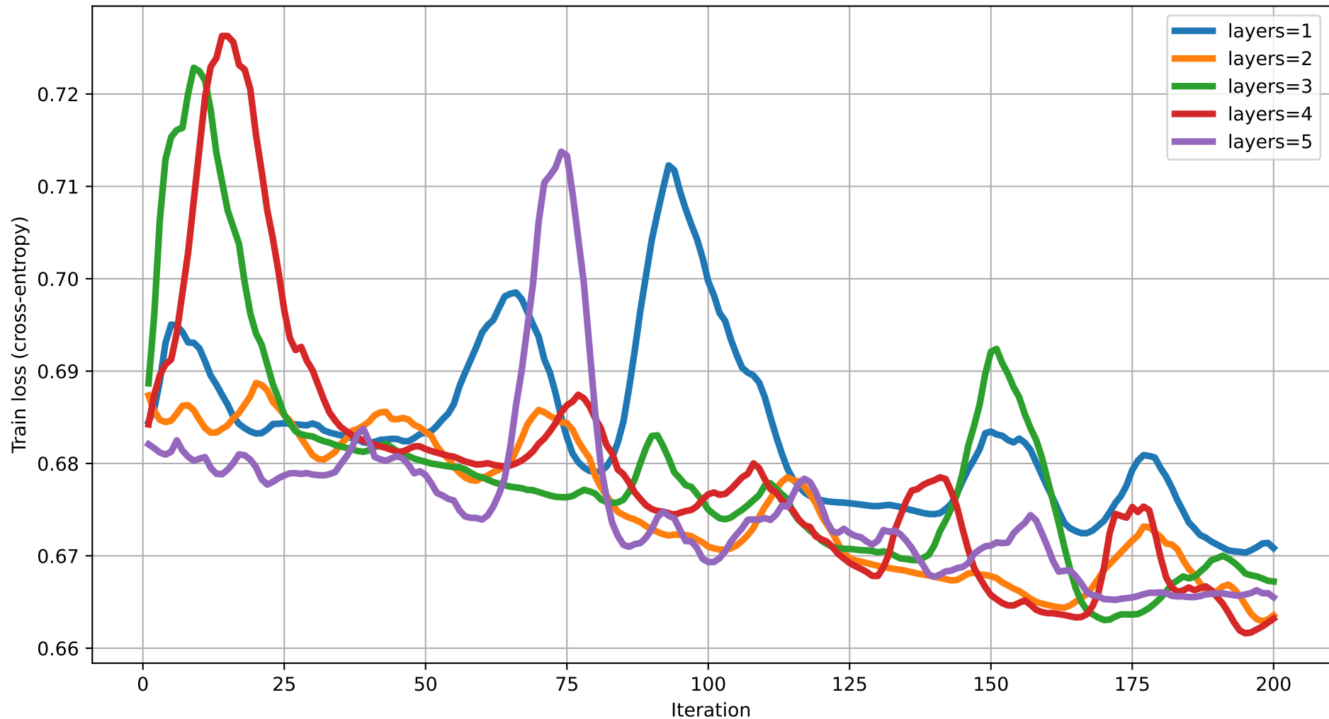
Train loss vs Iteration (dim=15) rot=RYZ, ent=chain, gate=CZ
