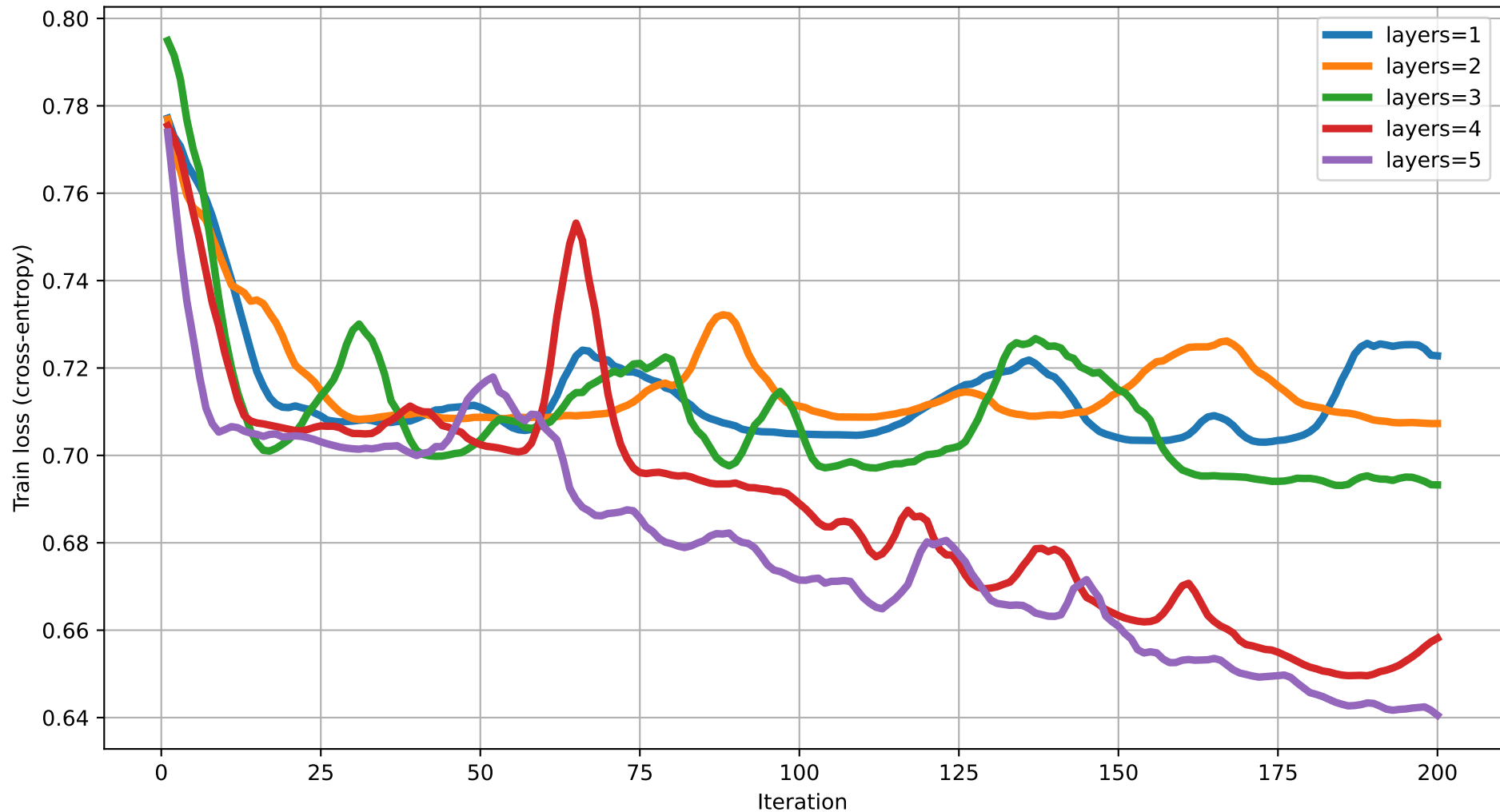
Train loss vs Iteration (dim=4) rot=RX, ent=chain, gate=CZ
