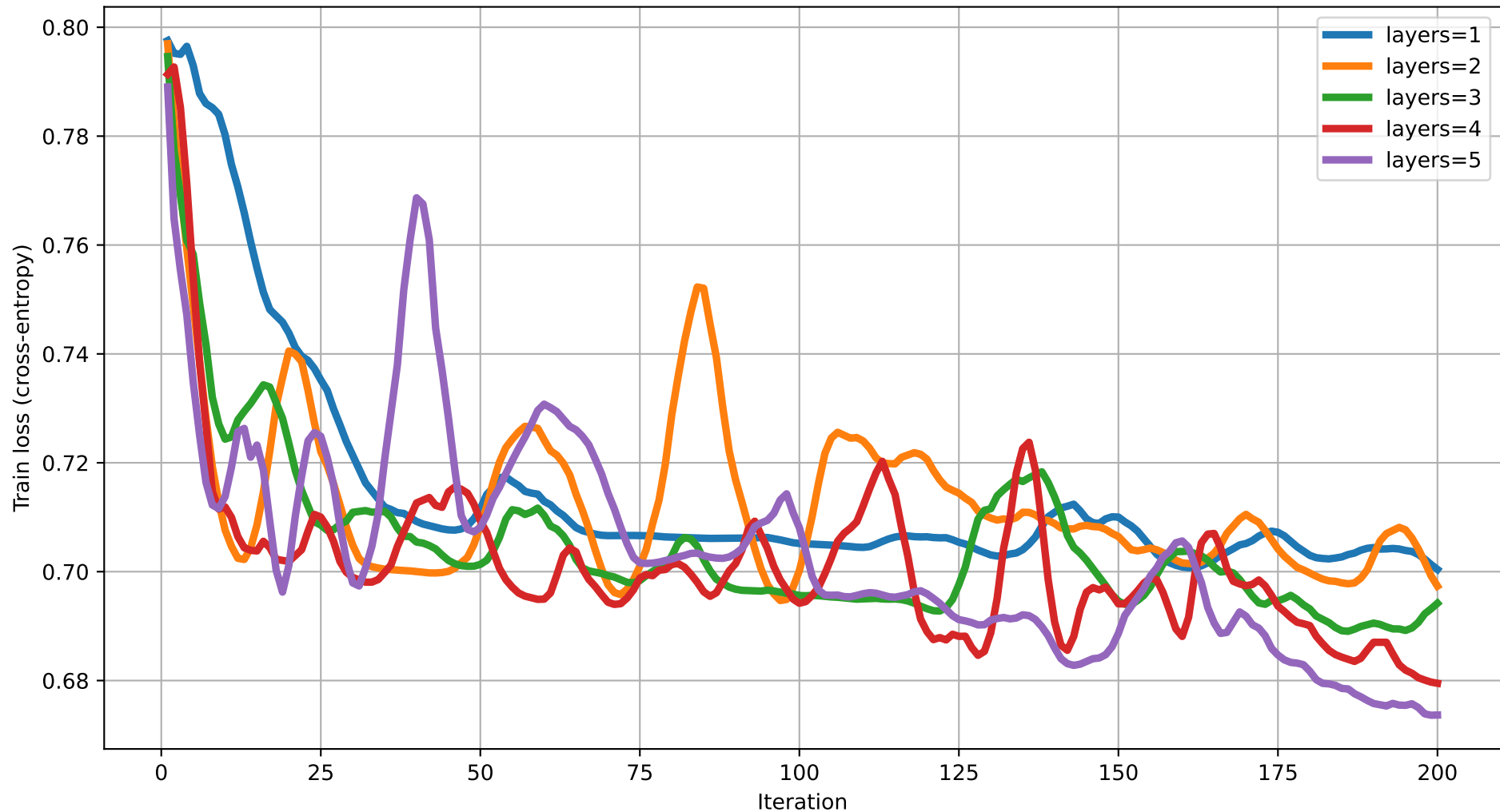
Train loss vs Iteration (dim=8) rot=Rot, ent=chain, gate=CZ
