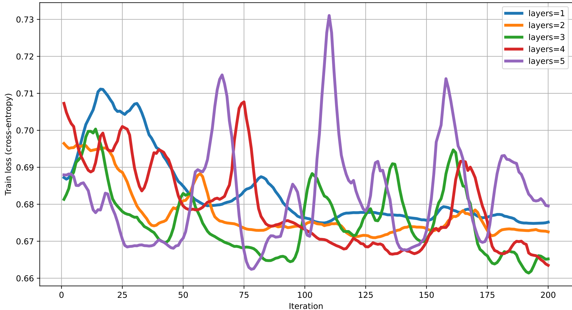
Train loss vs Iteration (dim=19) rot=RYZ, ent=ring, gate=CNOT
