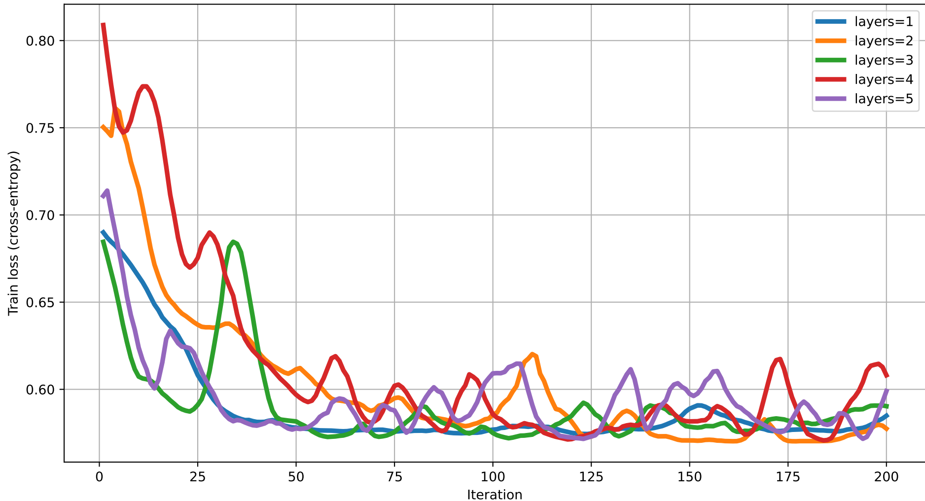
Train loss vs Iteration (dim=2) rot=RYZ, ent=pairwise, gate=IsingXX
