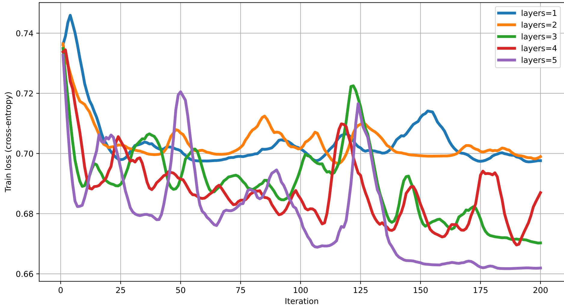
Train loss vs Iteration (dim=19) rot=RX, ent=chain, gate=CNOT
