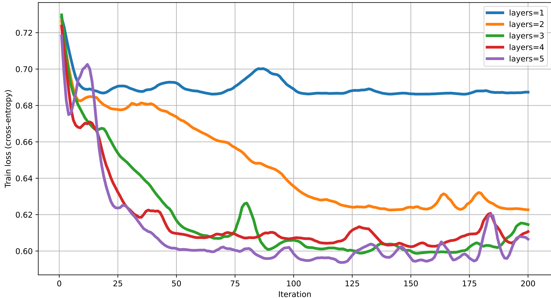
Train loss vs Iteration (degree=2) rot=RY, ent=full, gate=CNOT
