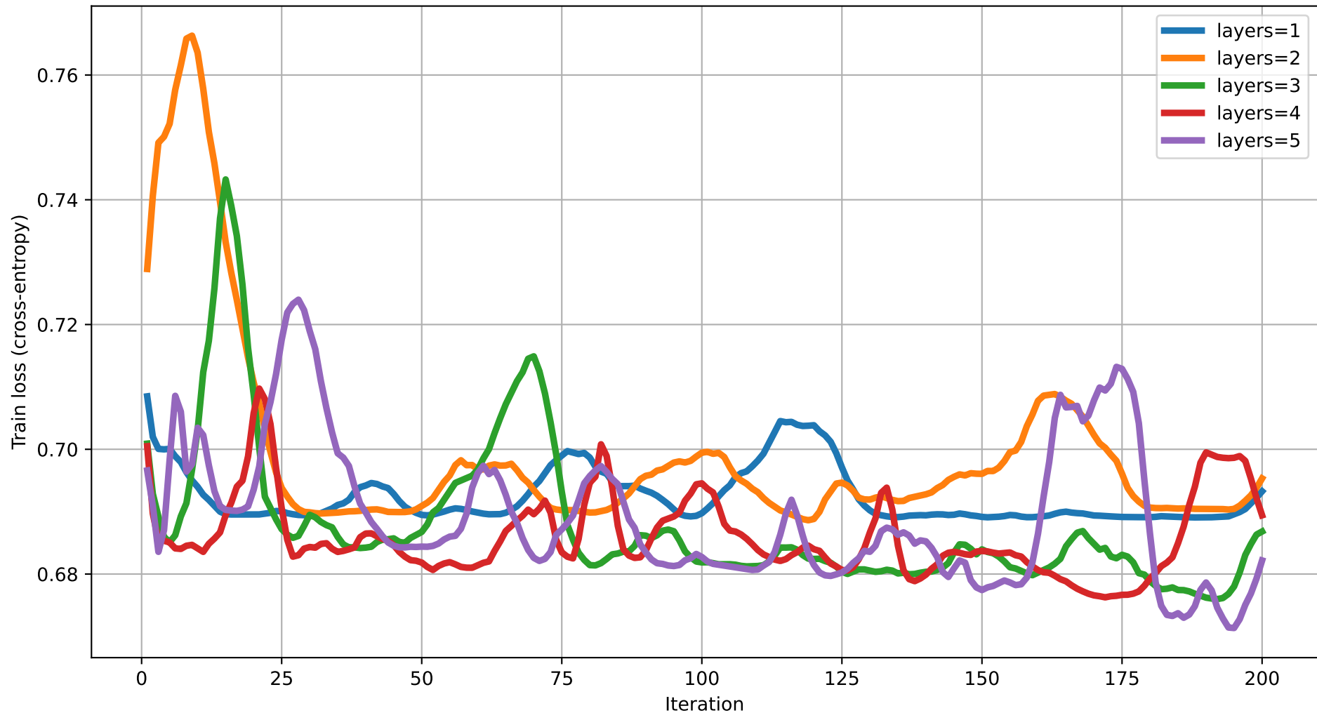
Train loss vs Iteration (dim=20) rot=Rot, ent=chain, gate=CNOT
