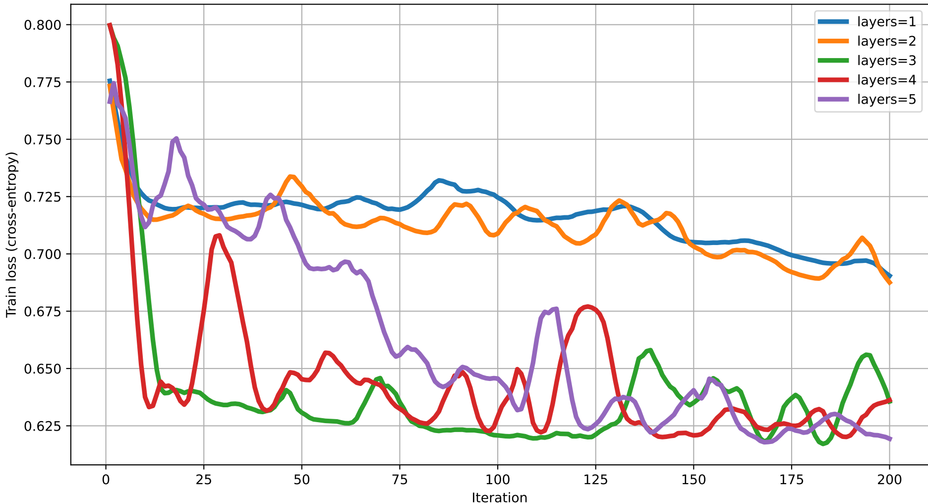
Train loss vs Iteration (dim=4) rot=RYZ, ent=pairwise, gate=CNOT
