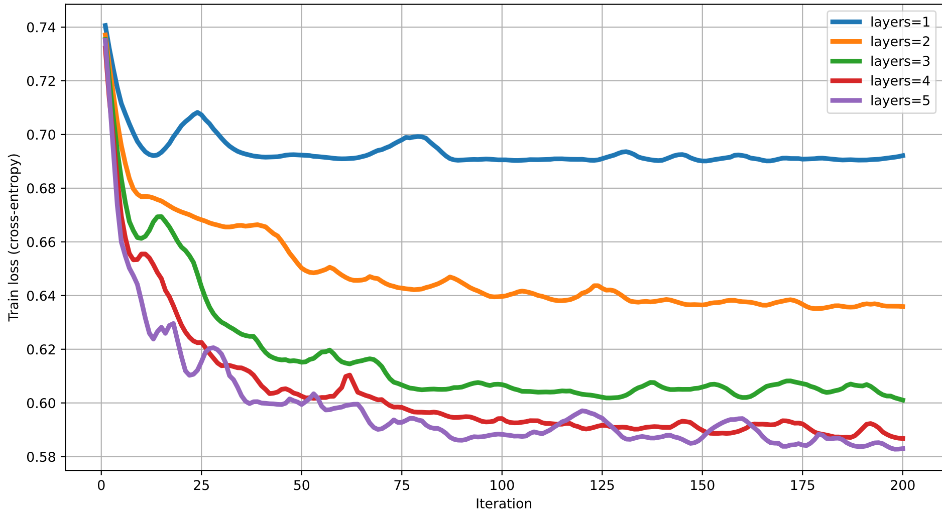
Train loss vs Iteration (degree=5) rot=Rot, ent=full, gate=CNOT
