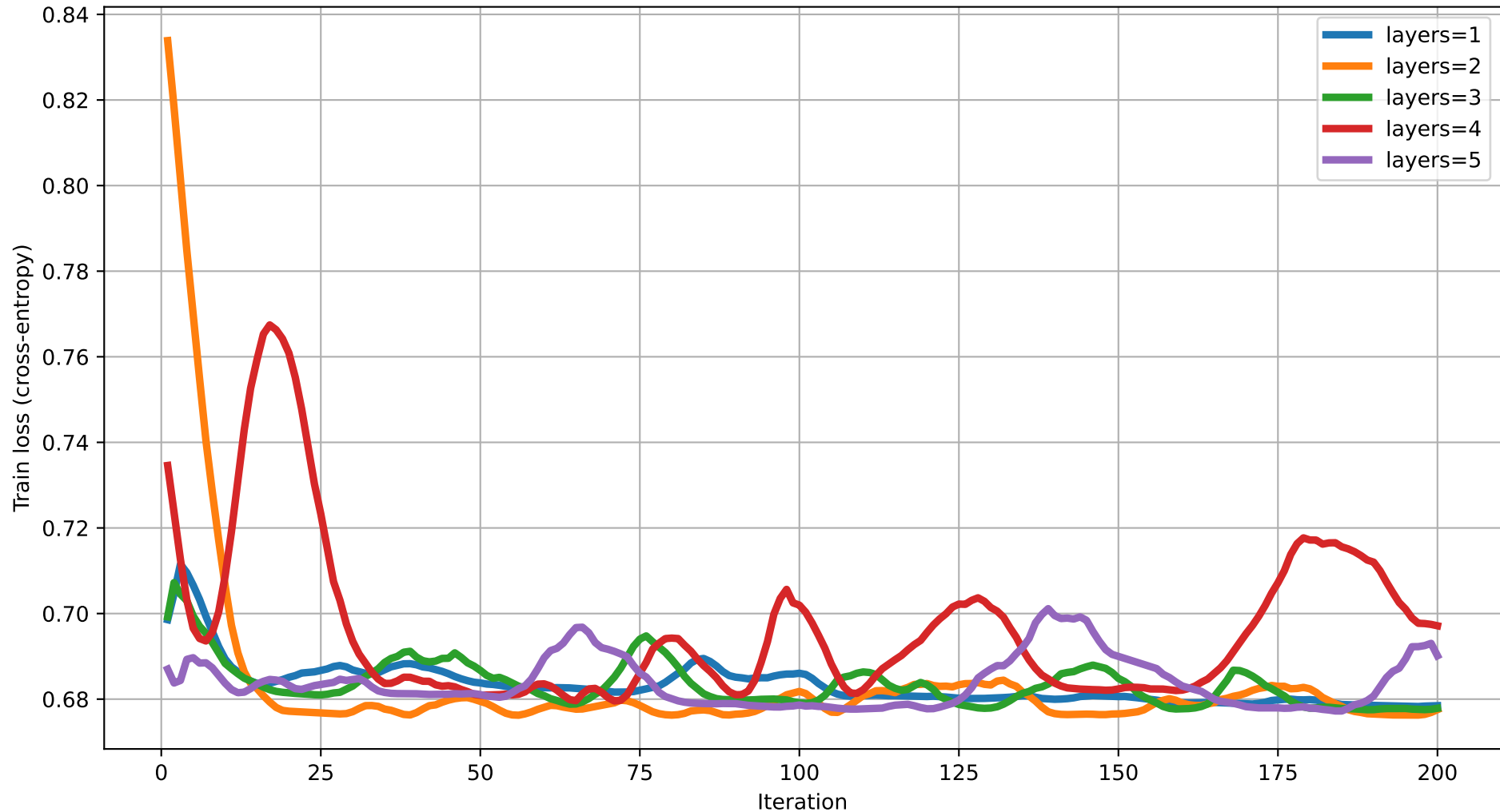
Train loss vs Iteration (dim=16) rot=RZ, ent=pairwise, gate=IsingXX
