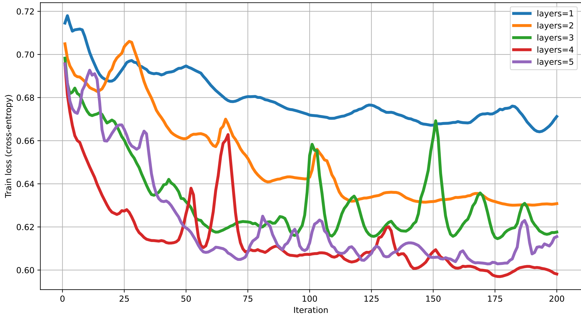
Train loss vs Iteration (dim=13) rot=Rot, ent=chain, gate=CNOT
