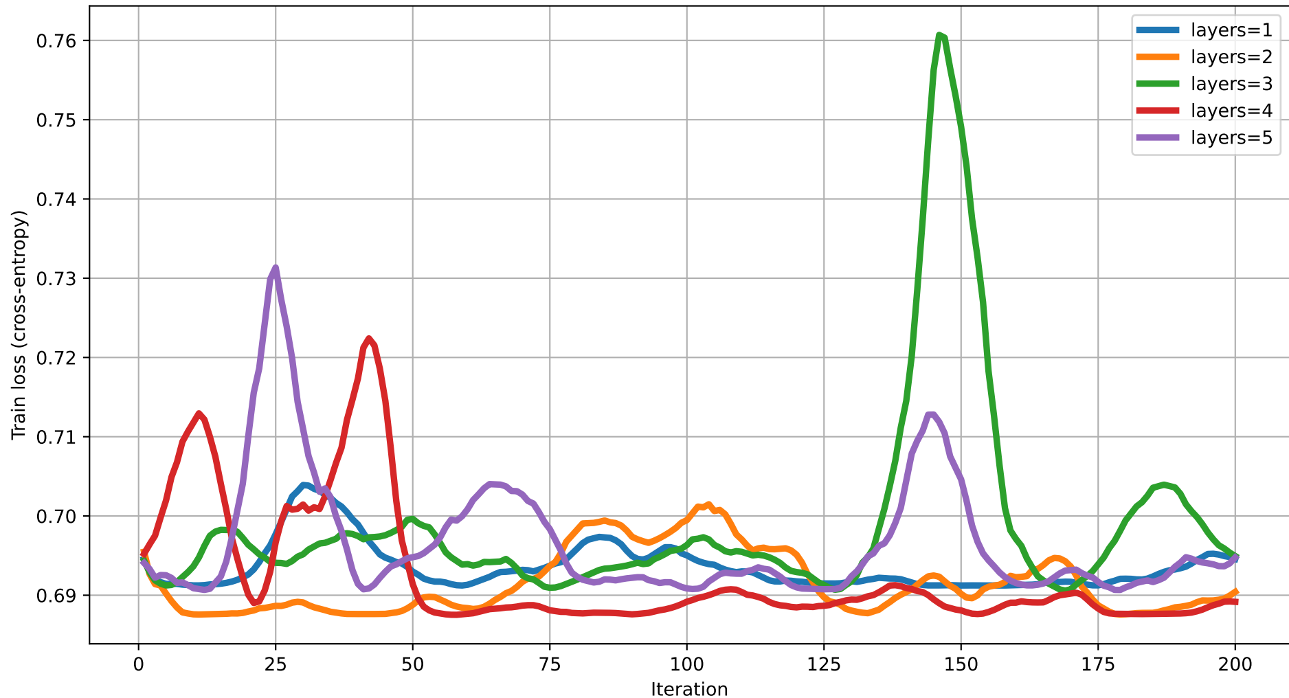
Train loss vs Iteration (dim=13) rot=RX, ent=ring, gate=IsingXX
