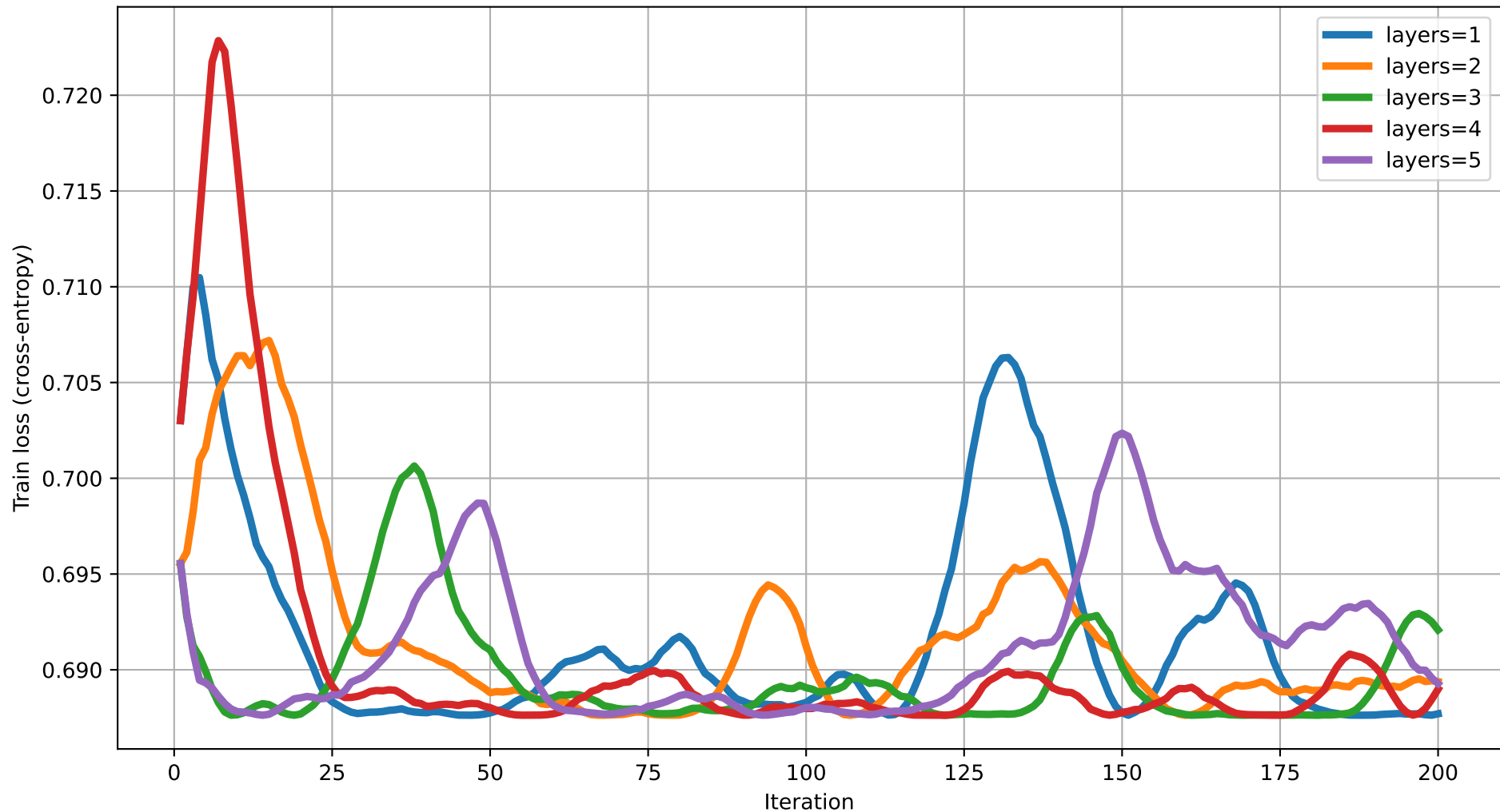
Train loss vs Iteration (dim=13) rot=RZ, ent=full, gate=CZ
