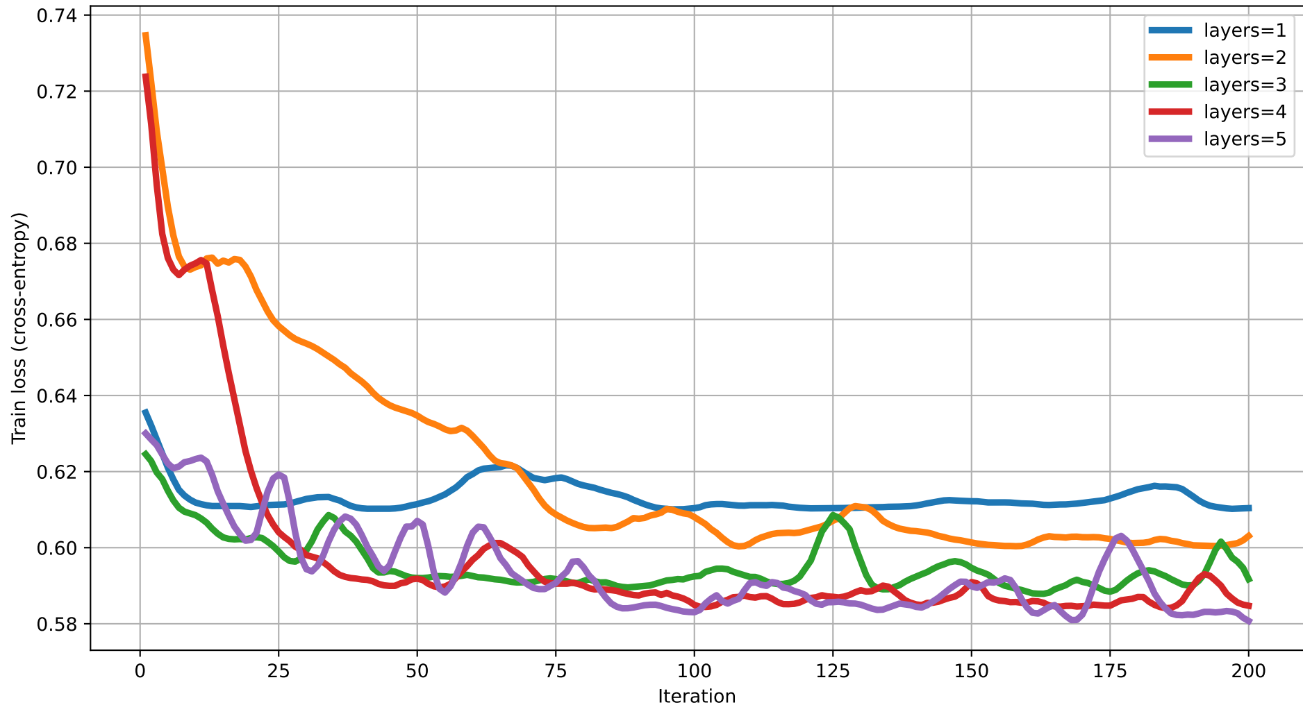
Train loss vs Iteration (degree=5) rot=RYZ, ent=ring, gate=IsingXX
