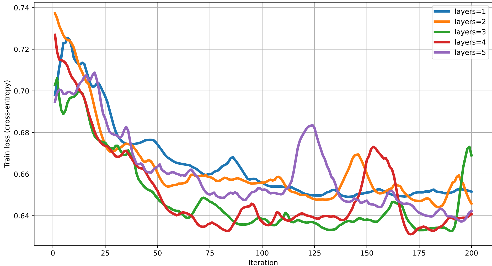
Train loss vs Iteration (dim=3) rot=RYZ, ent=pairwise, gate=IsingXX
