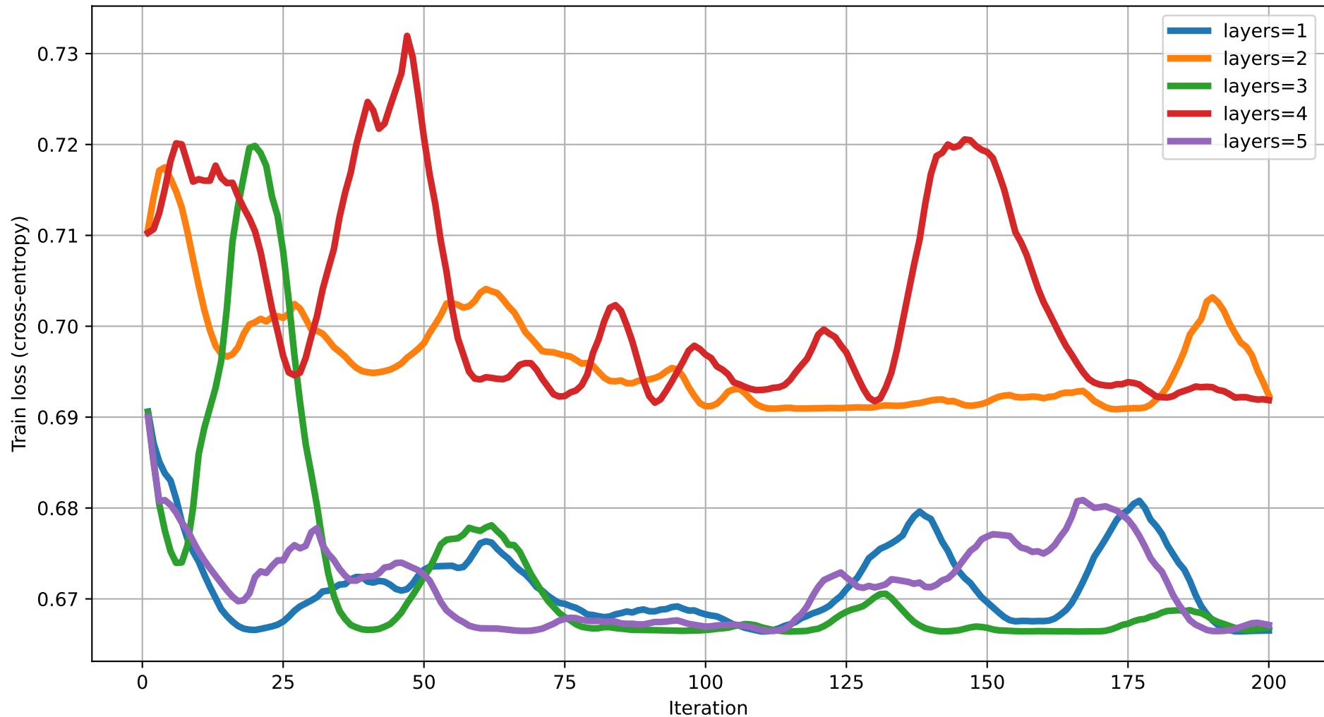
Train loss vs Iteration (dim=12) rot=RX, ent=ring, gate=IsingXX
