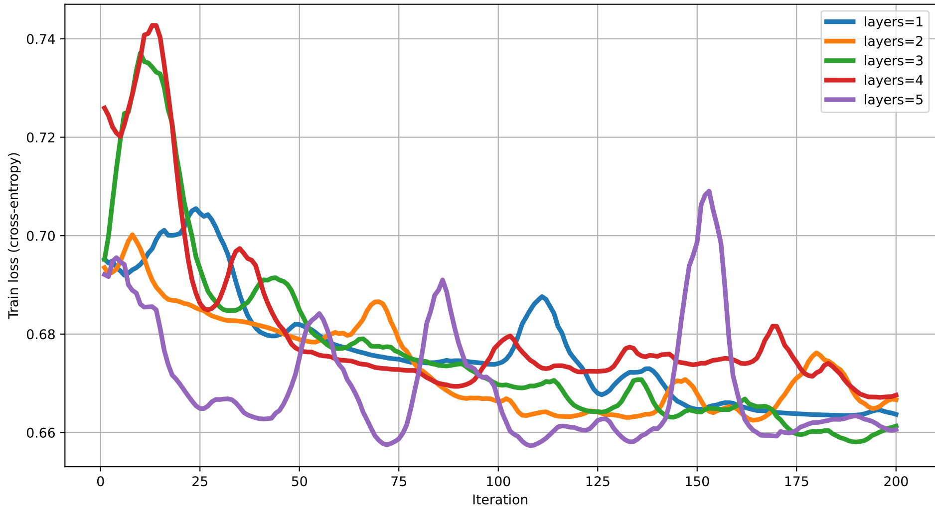
Train loss vs Iteration (dim=7) rot=RZ, ent=chain, gate=IsingXX
