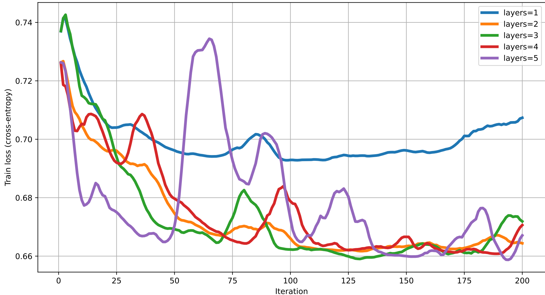
Train loss vs Iteration (dim=5) rot=RX, ent=full, gate=CZ
