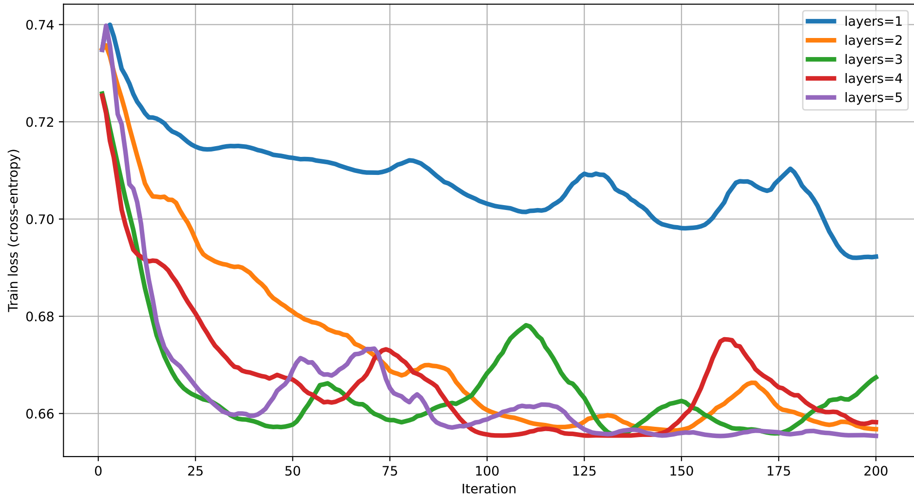
Train loss vs Iteration (dim=6) rot=RX, ent=chain, gate=CNOT
