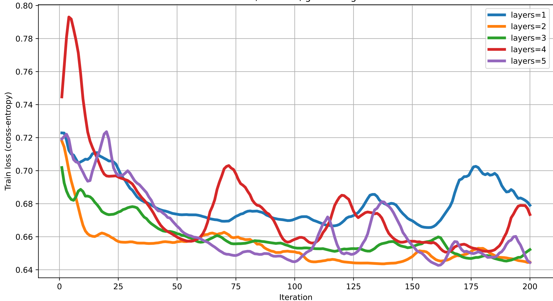
Train loss vs Iteration (dim=5) rot=RY, ent=full, gate=IsingXX
