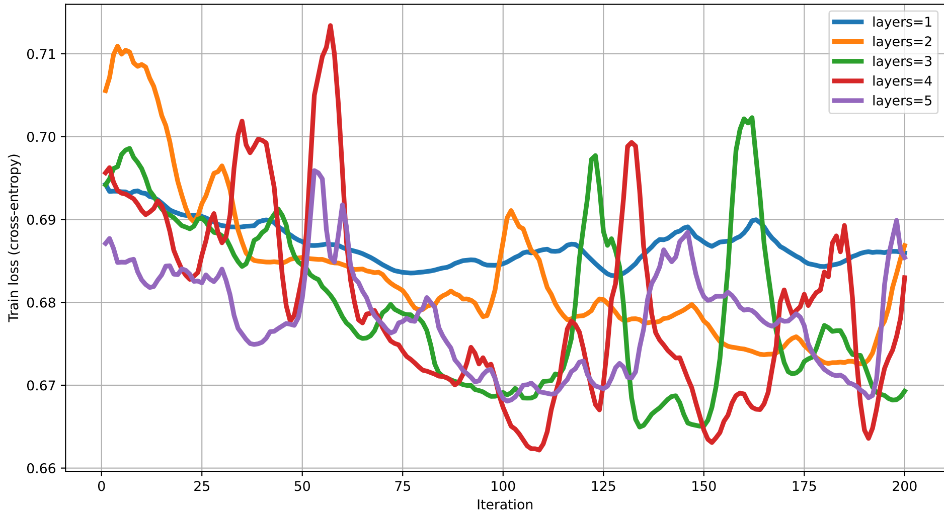
Train loss vs Iteration (dim=18) rot=Rot, ent=ring, gate=CNOT
