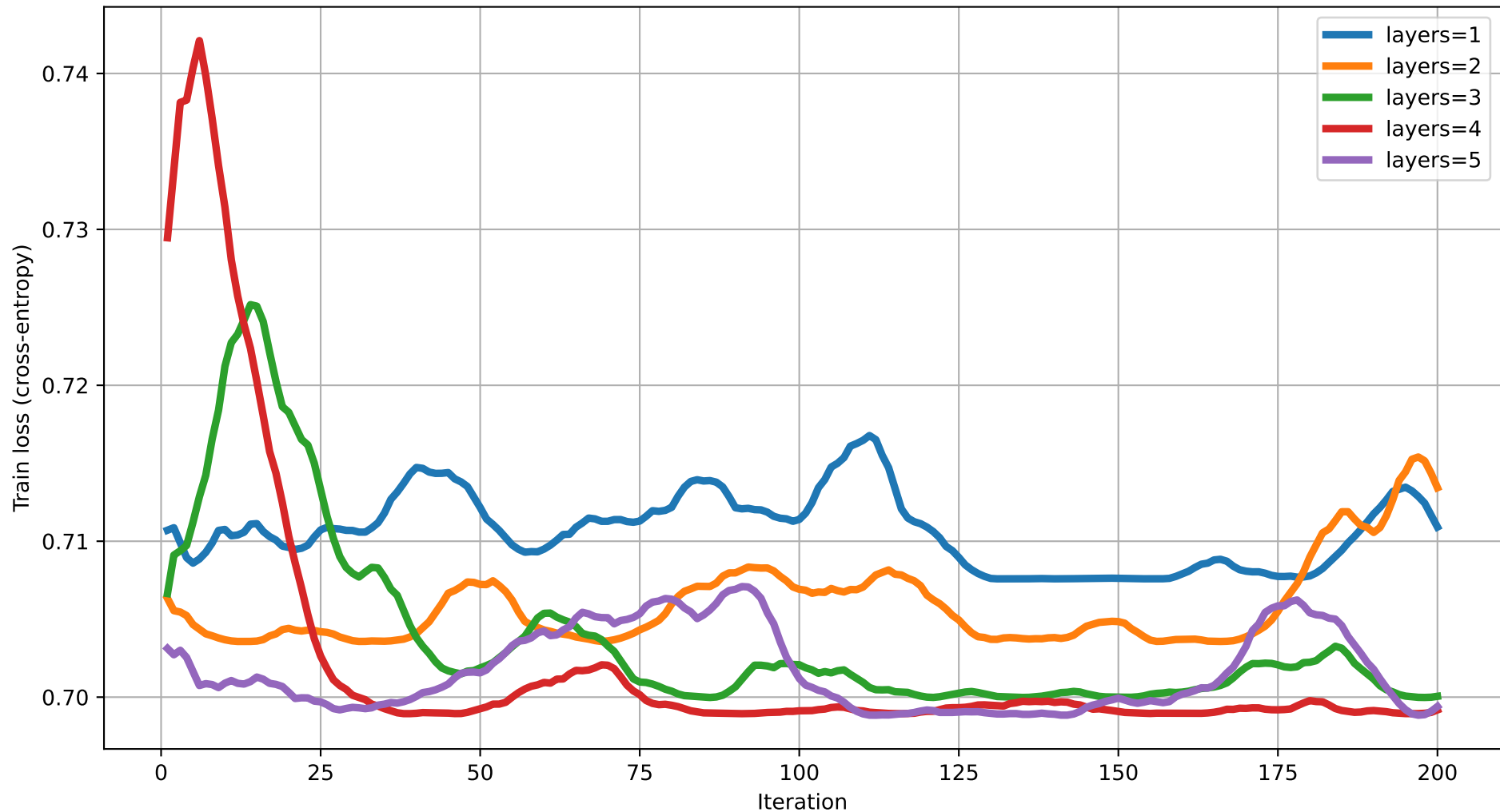
Train loss vs Iteration (dim=12) rot=RZ, ent=ring, gate=CNOT
