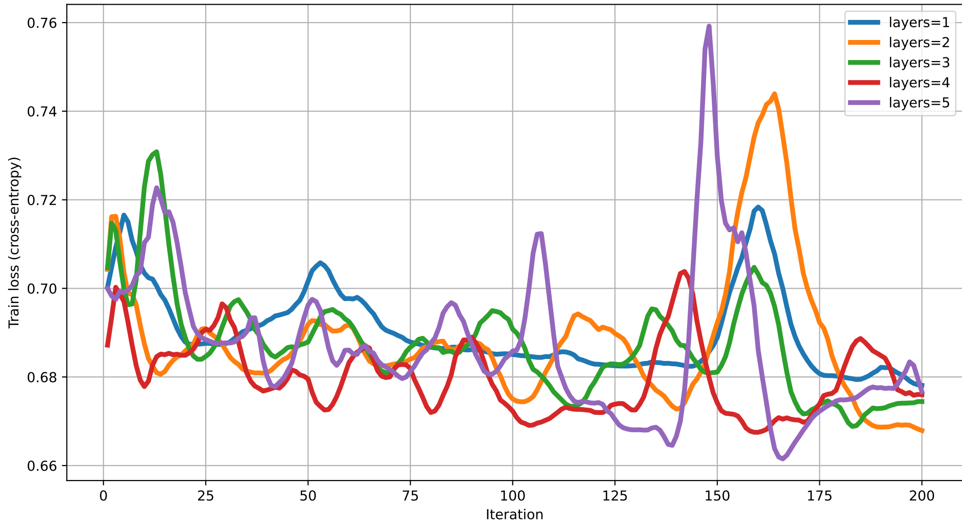
Train loss vs Iteration (dim=13) rot=RYZ, ent=ring, gate=IsingXX
