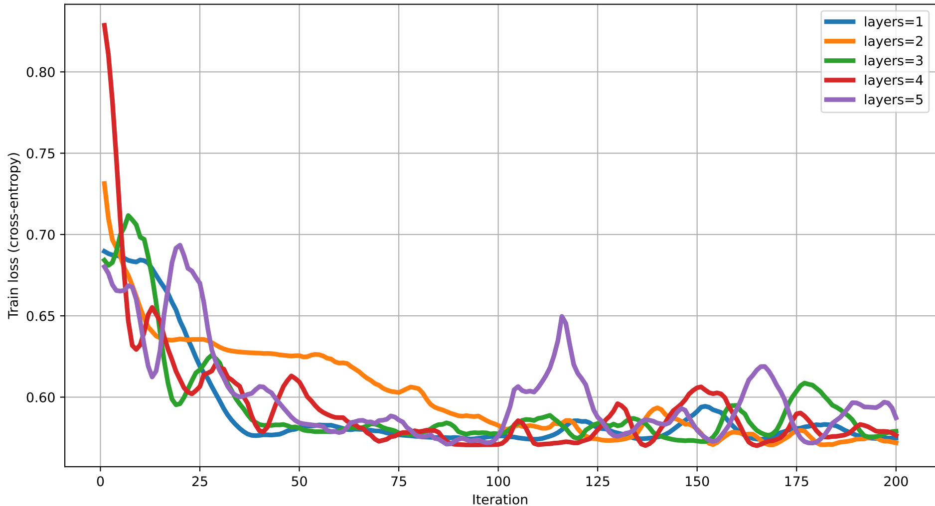
Train loss vs Iteration (dim=2) rot=RYZ, ent=full, gate=IsingXX
