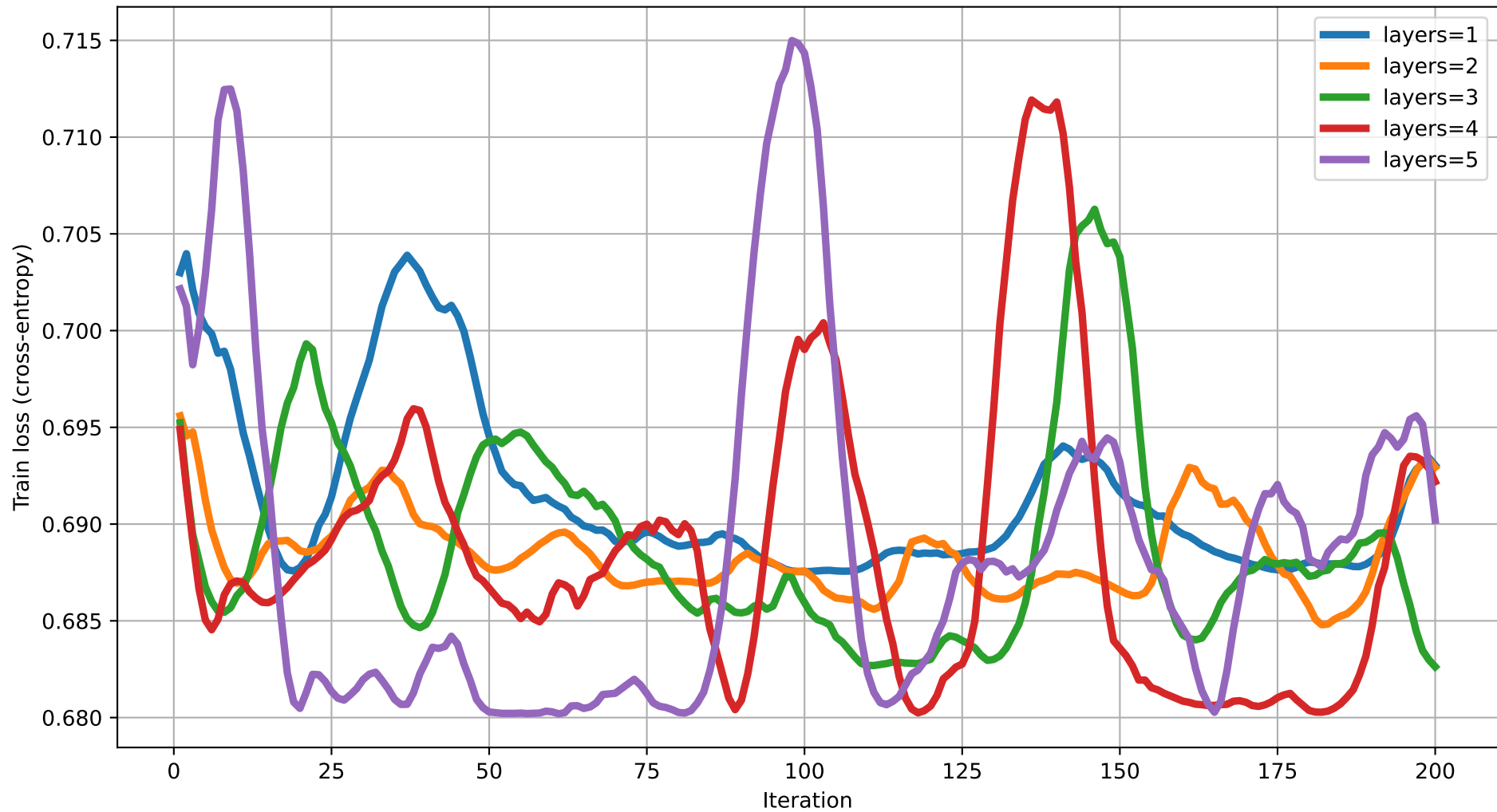
Train loss vs Iteration (dim=13) rot=RX, ent=chain, gate=CNOT
