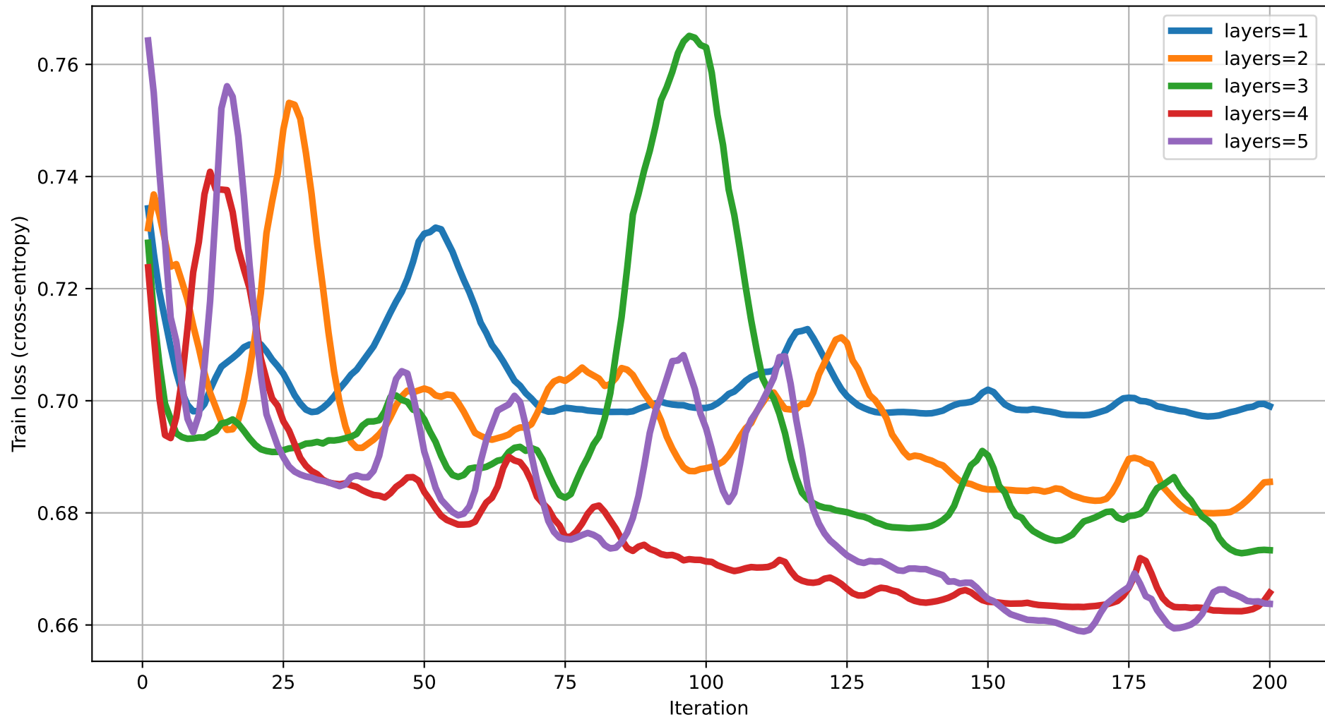
Train loss vs Iteration (dim=19) rot=RY, ent=chain, gate=CNOT
