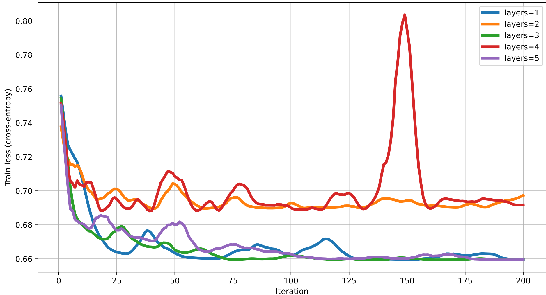
Train loss vs Iteration (dim=16) rot=RX, ent=ring, gate=IsingXX
