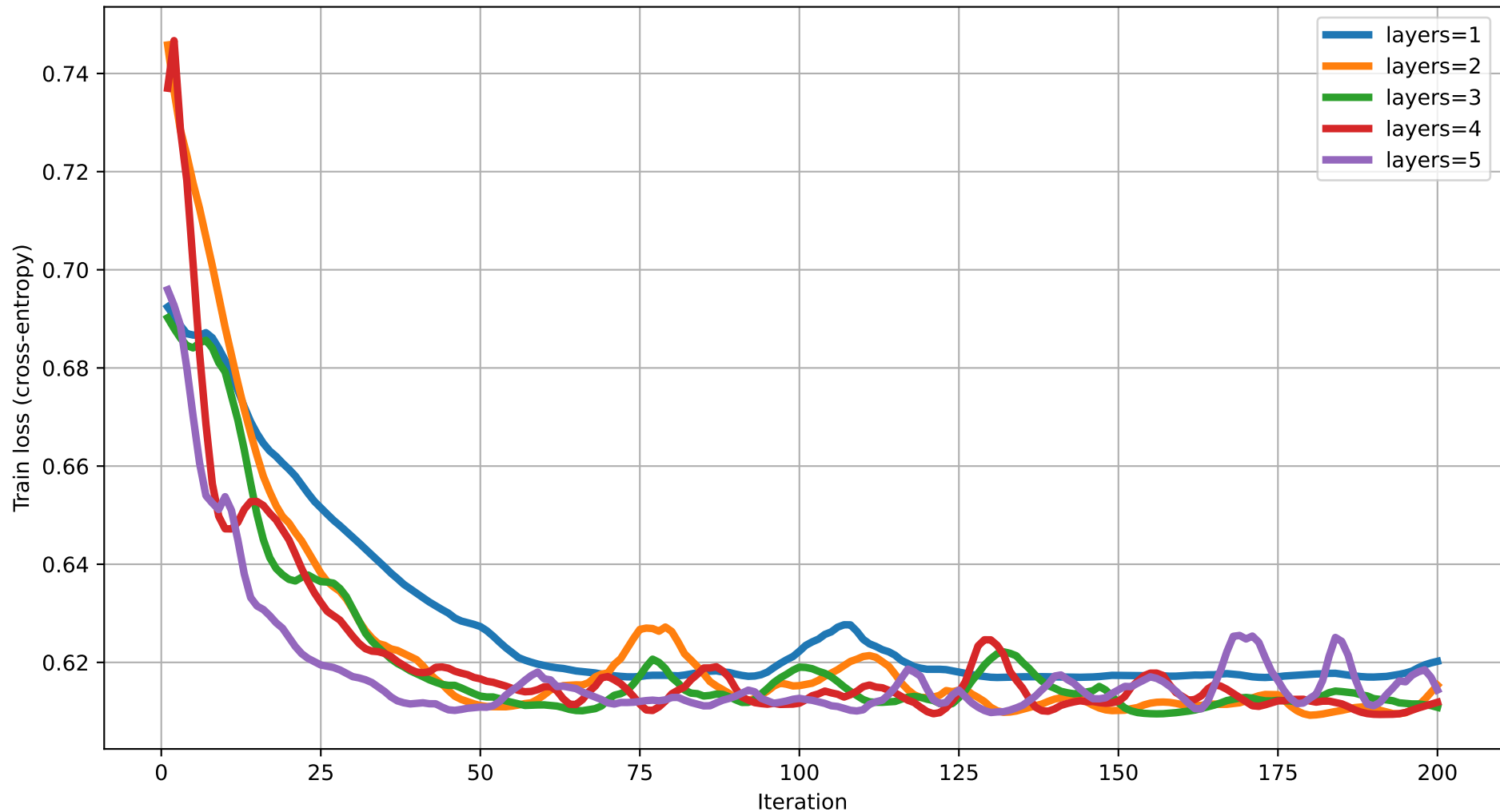
Train loss vs Iteration (degree=4) rot=RYZ, ent=pairwise, gate=IsingXX
