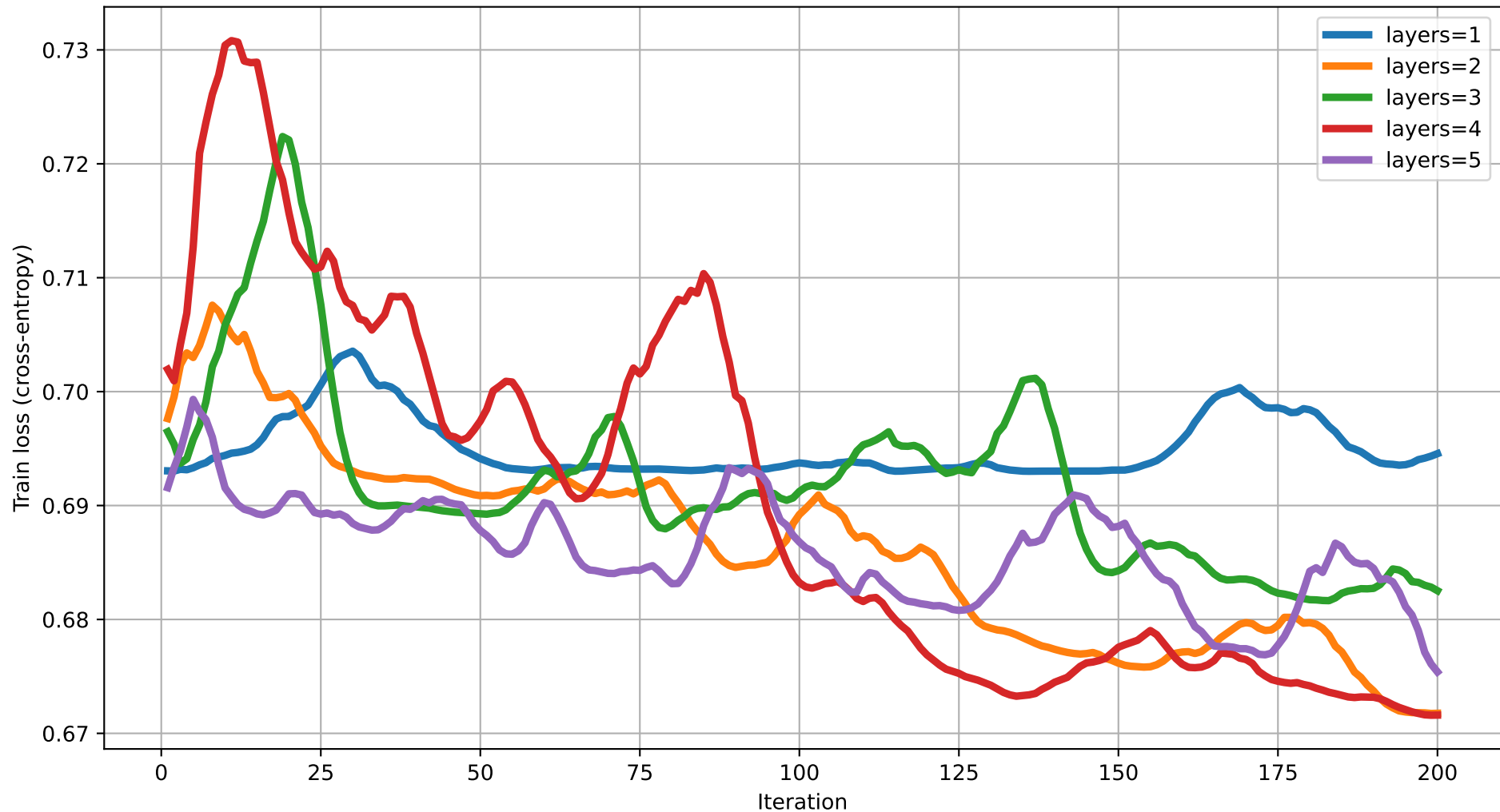
Train loss vs Iteration (dim=14) rot=RY, ent=chain, gate=IsingXX
