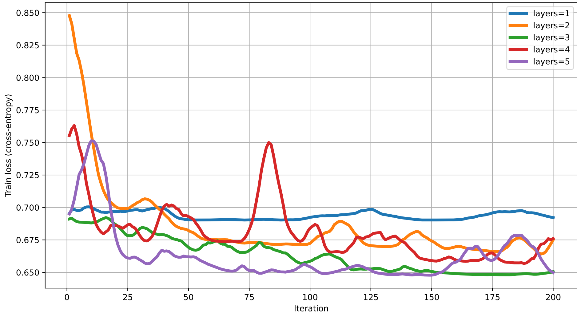
Train loss vs Iteration (dim=8) rot=RY, ent=full, gate=IsingXX
