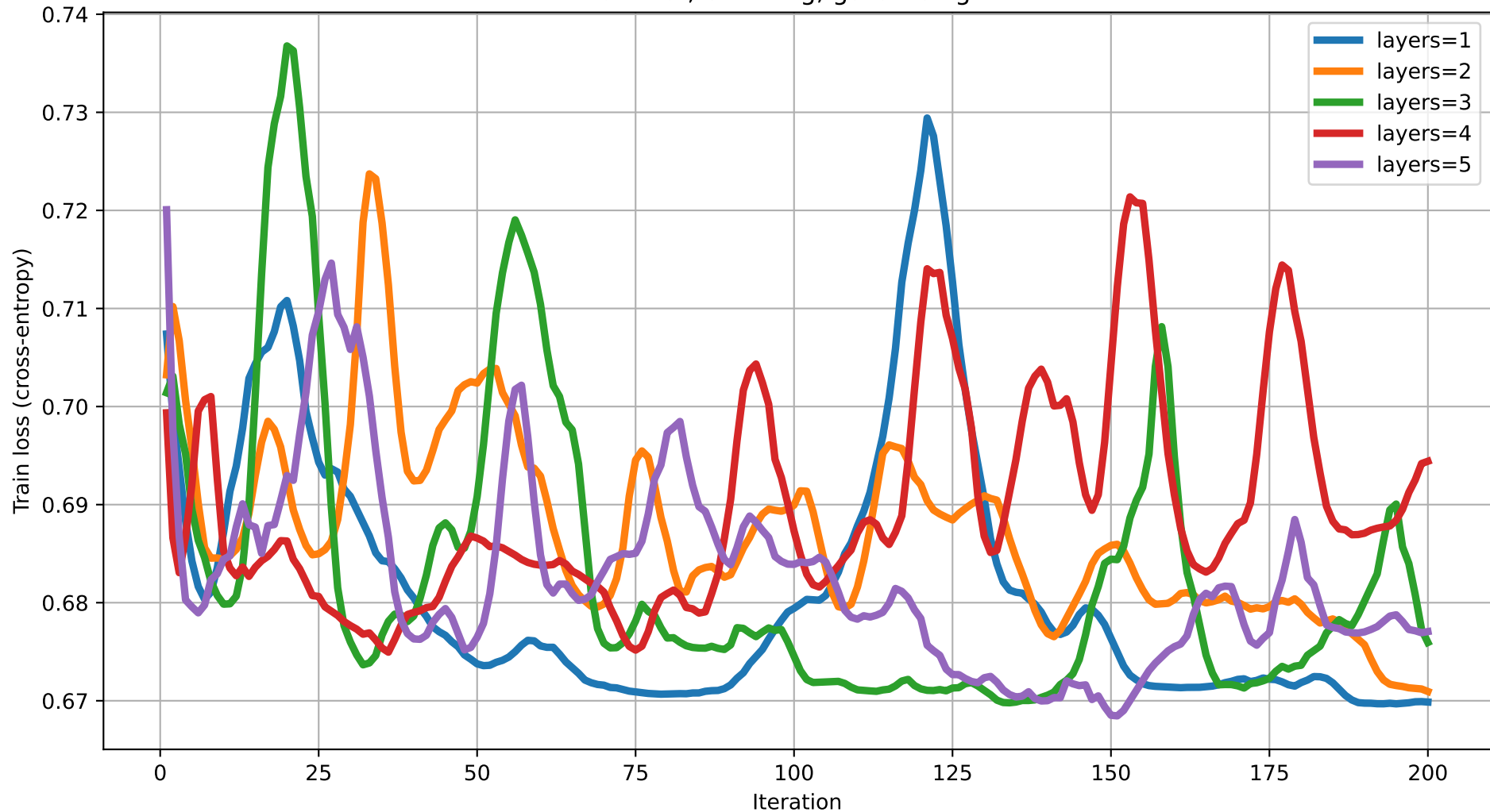
Train loss vs Iteration (dim=20) rot=Rot, ent=ring, gate=IsingXX
