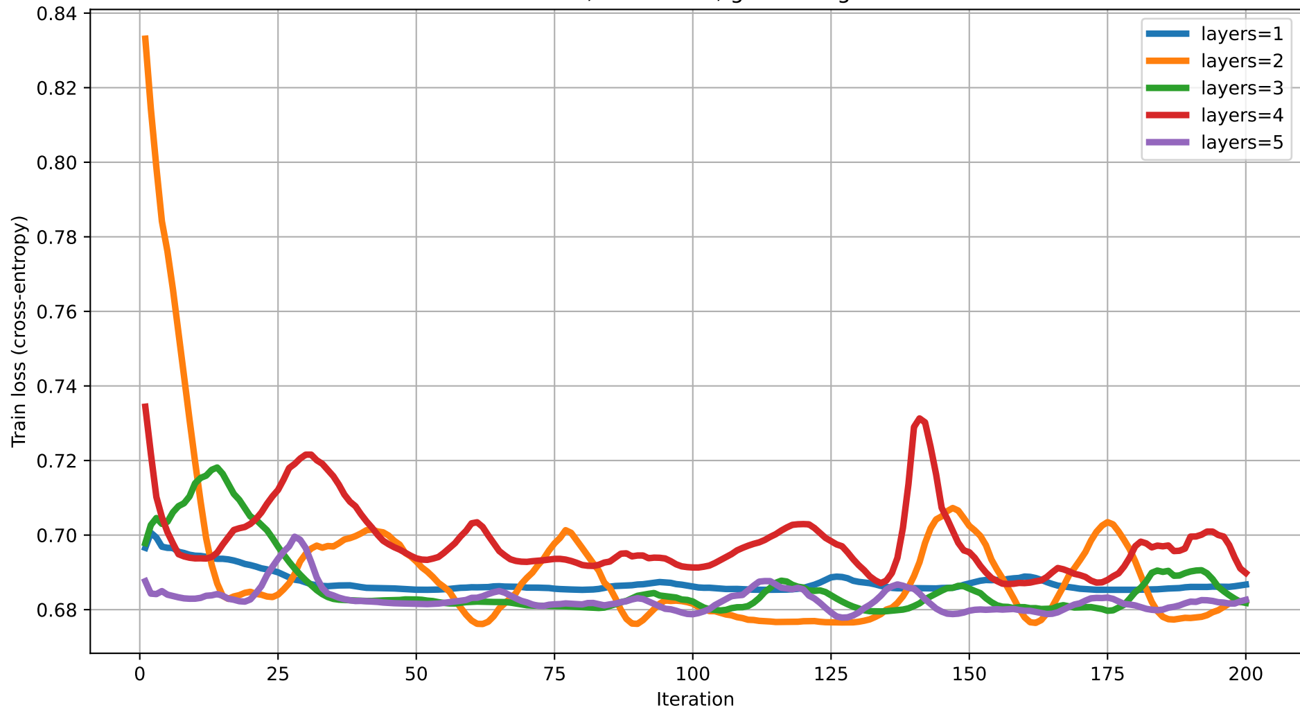
Train loss vs Iteration (dim=16) rot=RY, ent=chain, gate=IsingXX
