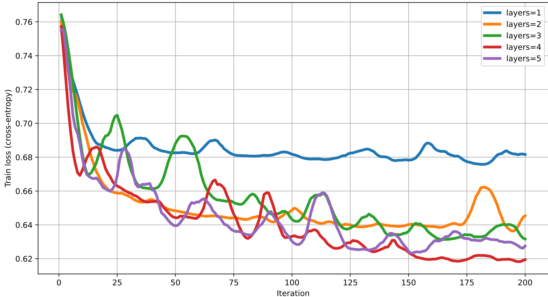
Train loss vs Iteration (dim=8) rot=RY, ent=chain, gate=CZ
