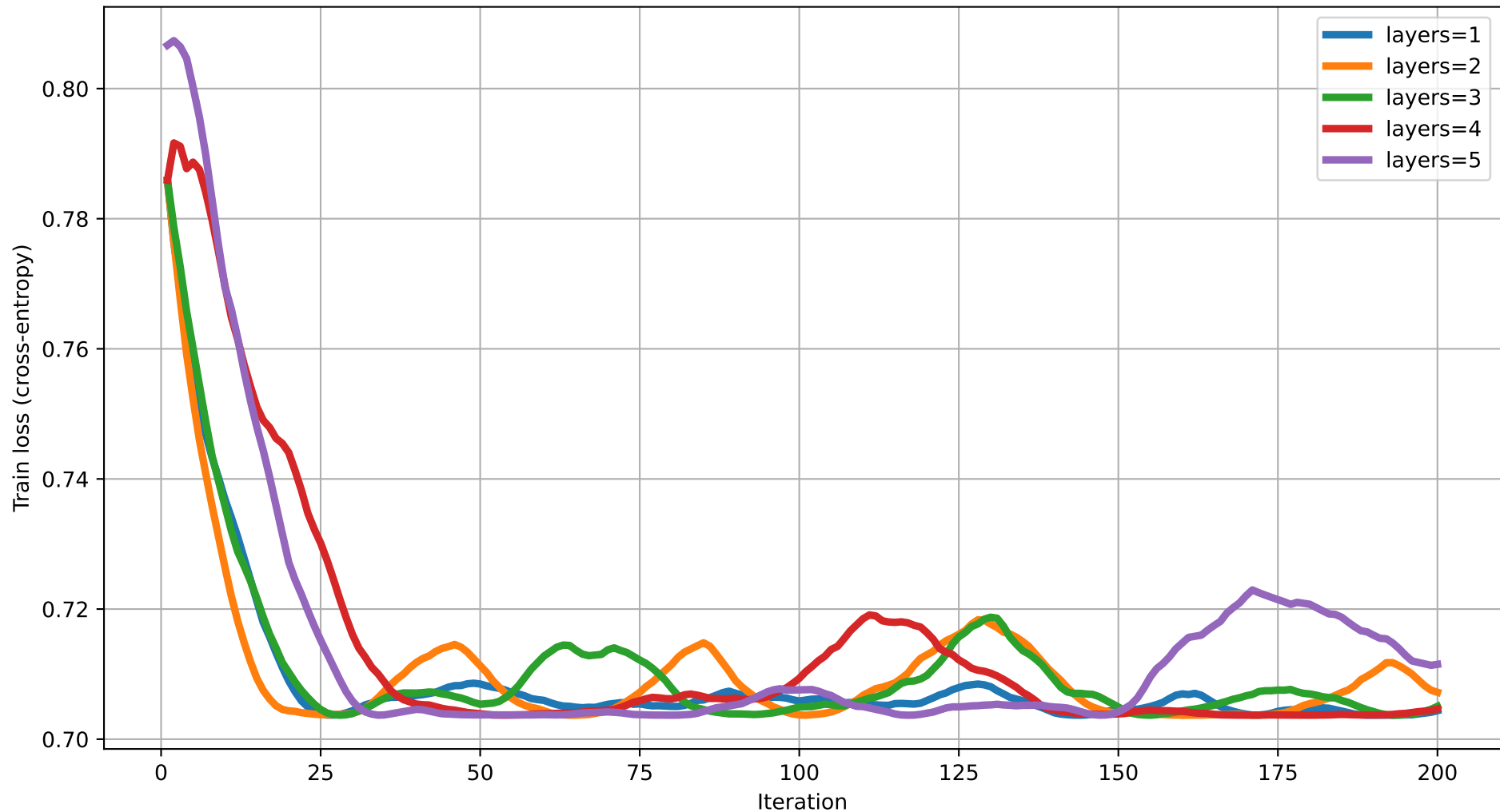
Train loss vs Iteration (dim=9) rot=RZ, ent=chain, gate=CZ
