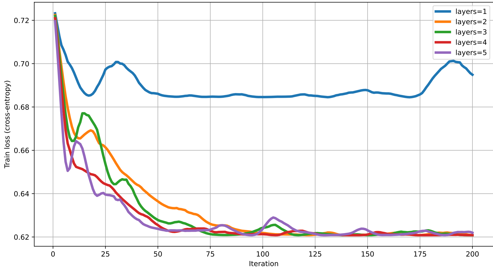
Train loss vs Iteration (degree=3) rot=RX, ent=pairwise, gate=CNOT
