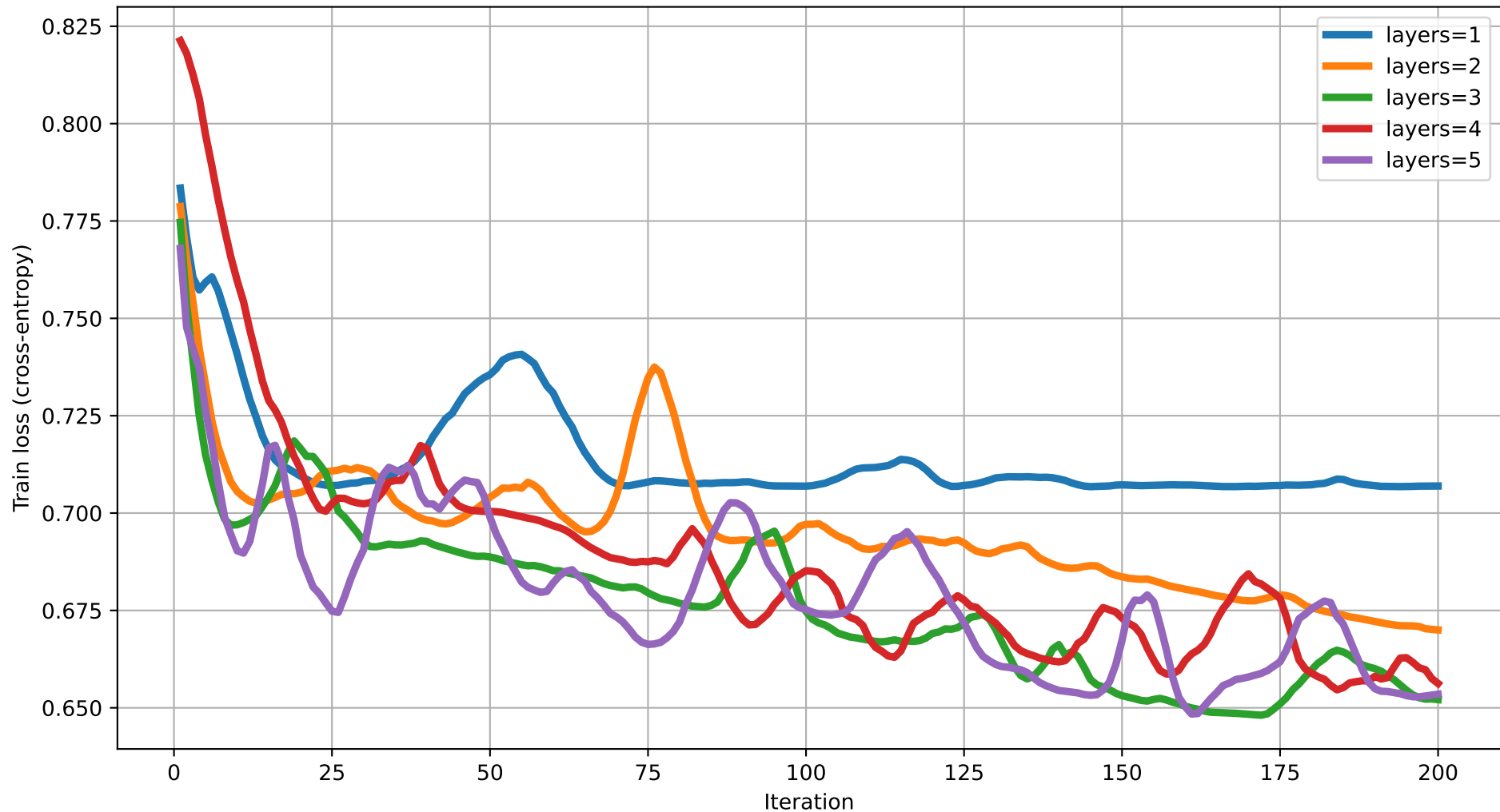
Train loss vs Iteration (dim=9) rot=RYZ, ent=chain, gate=CNOT
