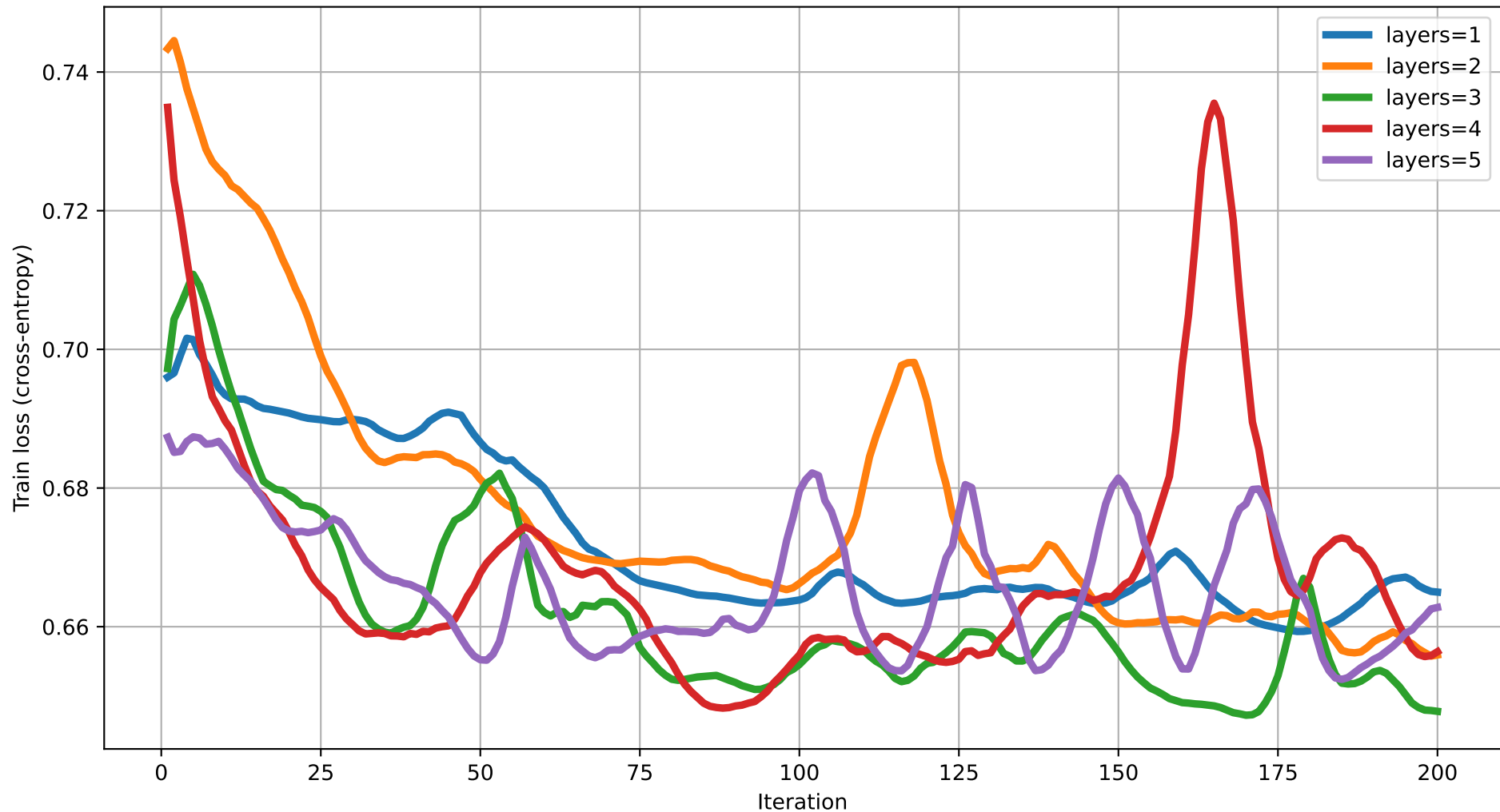
Train loss vs Iteration (dim=5) rot=RYZ, ent=pairwise, gate=IsingXX
