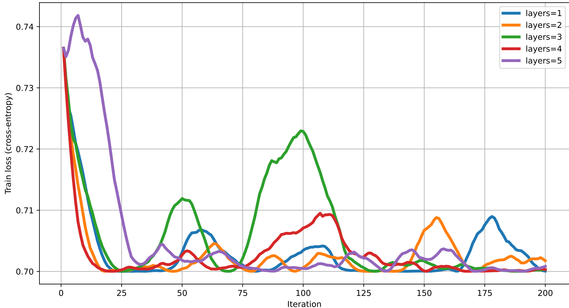
Train loss vs Iteration (dim=19) rot=RZ, ent=full, gate=CZ
