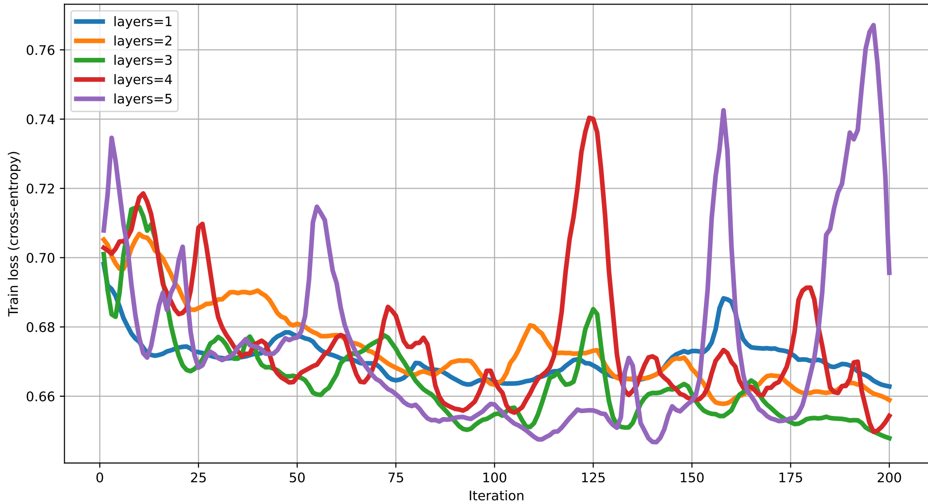
Train loss vs Iteration (dim=6) rot=Rot, ent=ring, gate=IsingXX
