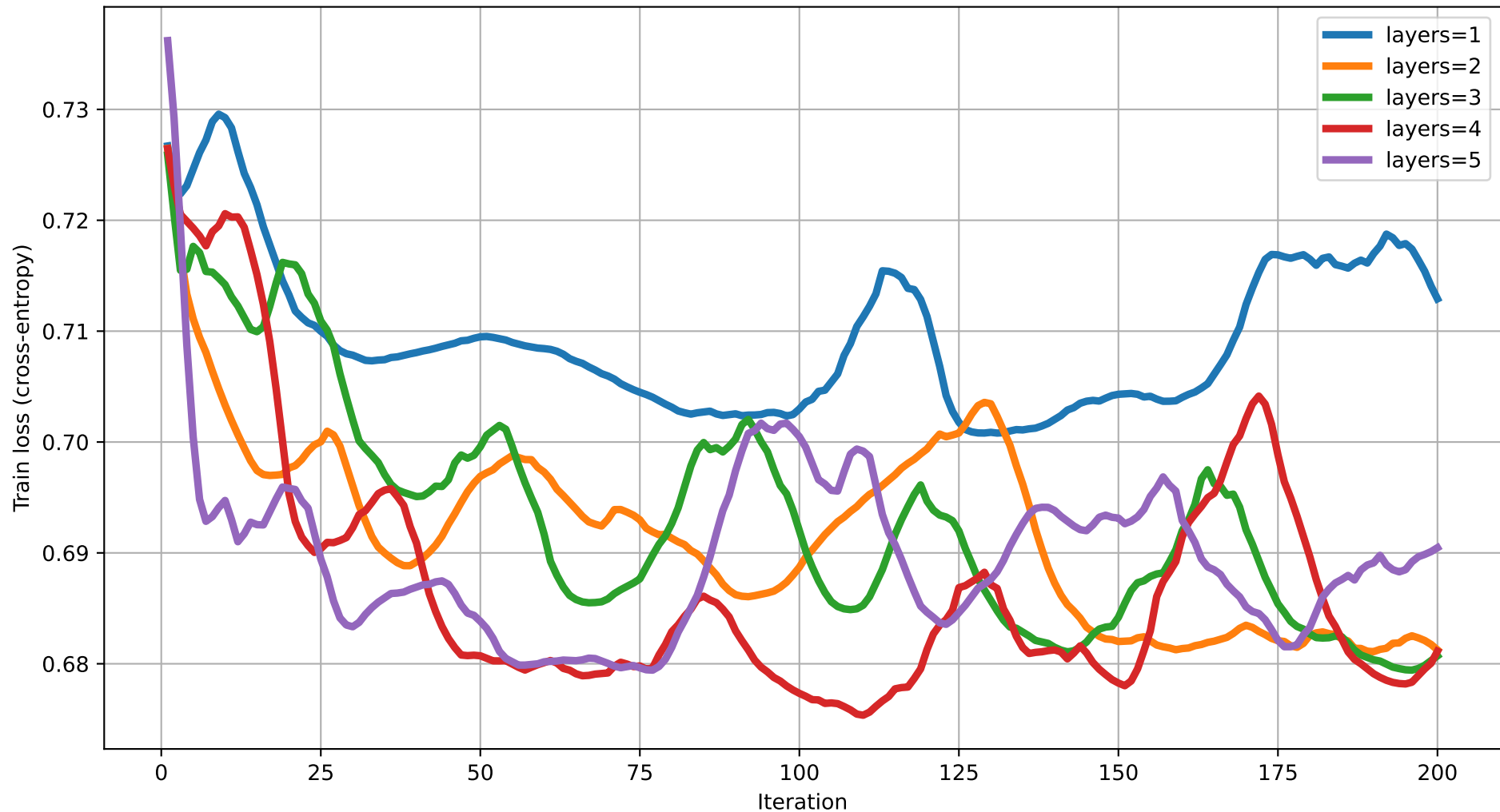
Train loss vs Iteration (dim=5) rot=RX, ent=chain, gate=CZ
