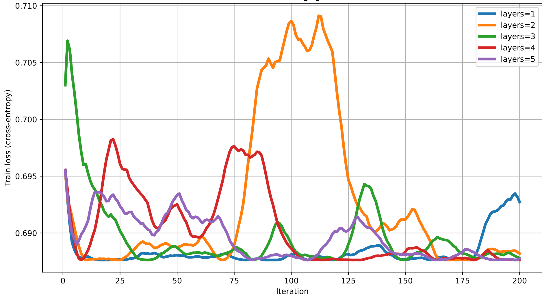
Train loss vs Iteration (dim=13) rot=RZ, ent=ring, gate=CZ
