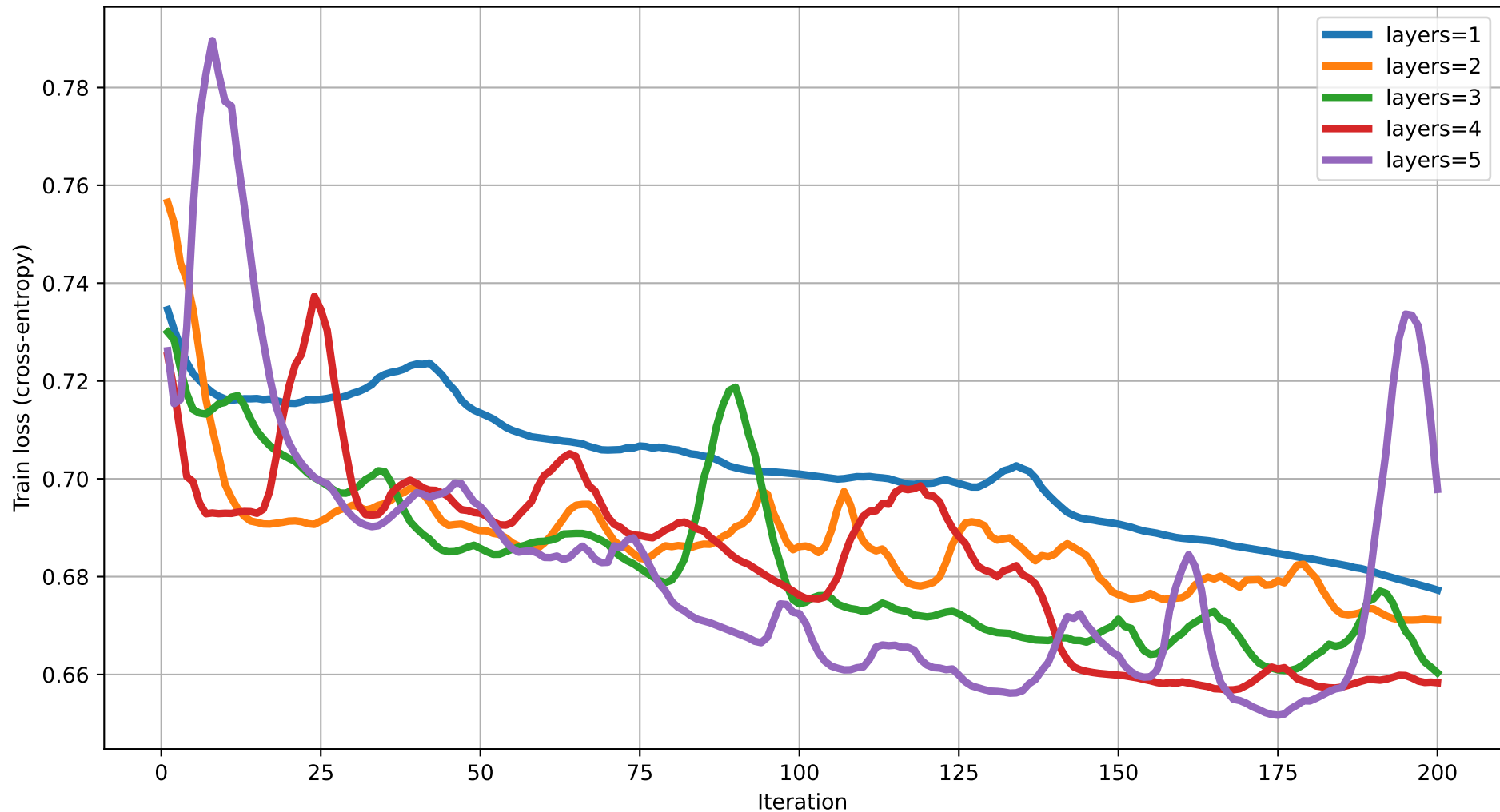
Train loss vs Iteration (dim=16) rot=RY, ent=full, gate=IsingXX
