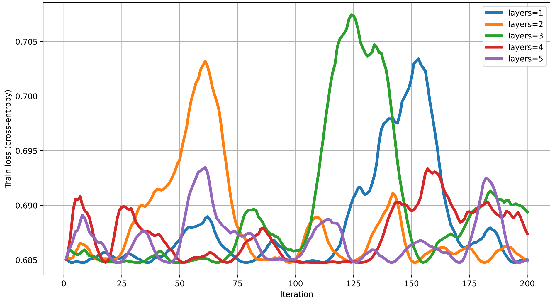
Train loss vs Iteration (dim=15) rot=RZ, ent=pairwise, gate=CZ
