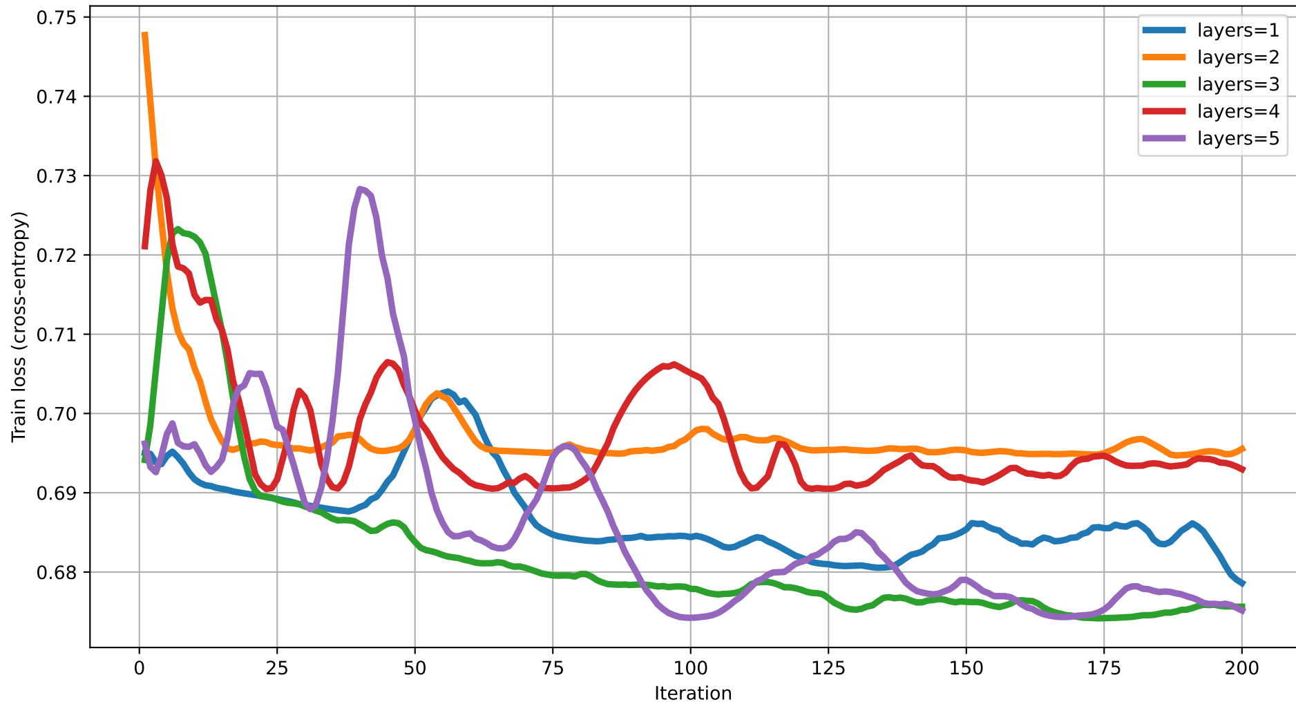
Train loss vs Iteration (dim=20) rot=RX, ent=chain, gate=IsingXX
