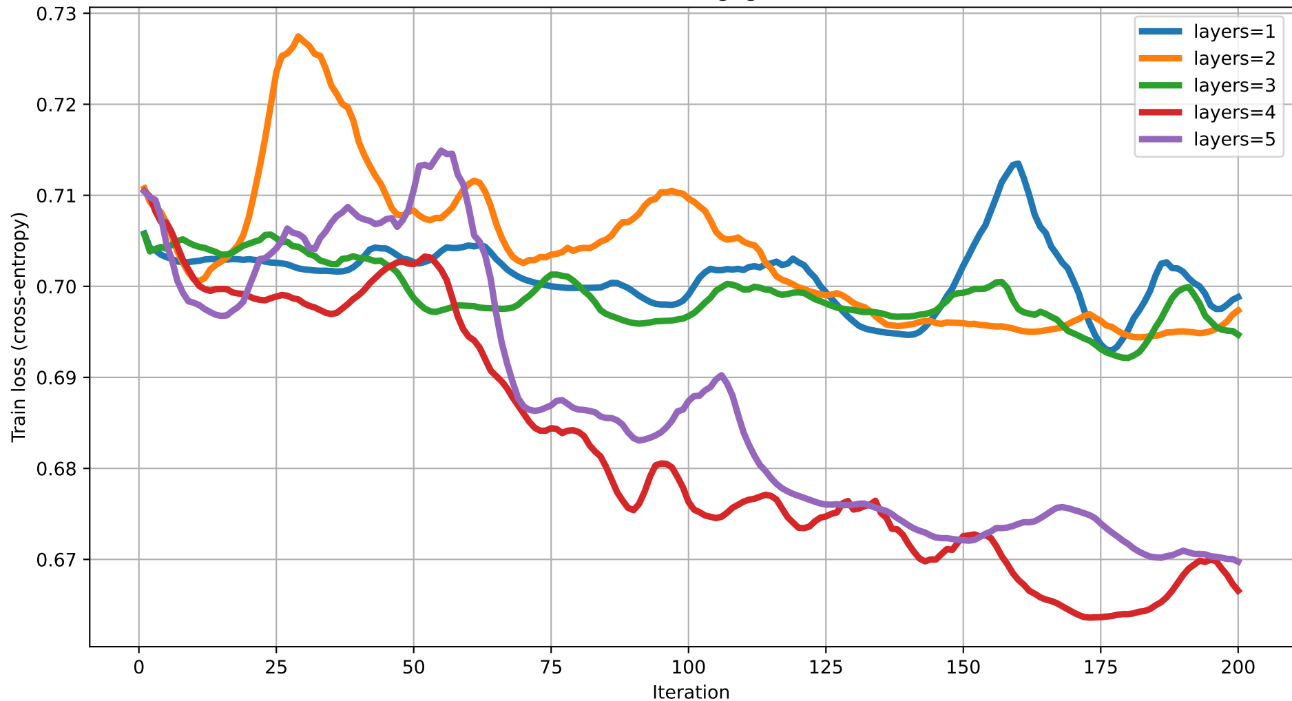
Train loss vs Iteration (dim=12) rot=RX, ent=ring, gate=CZ
