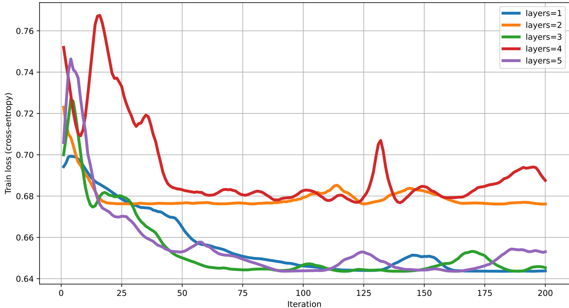
Train loss vs Iteration (dim=5) rot=RX, ent=pairwise, gate=IsingXX
