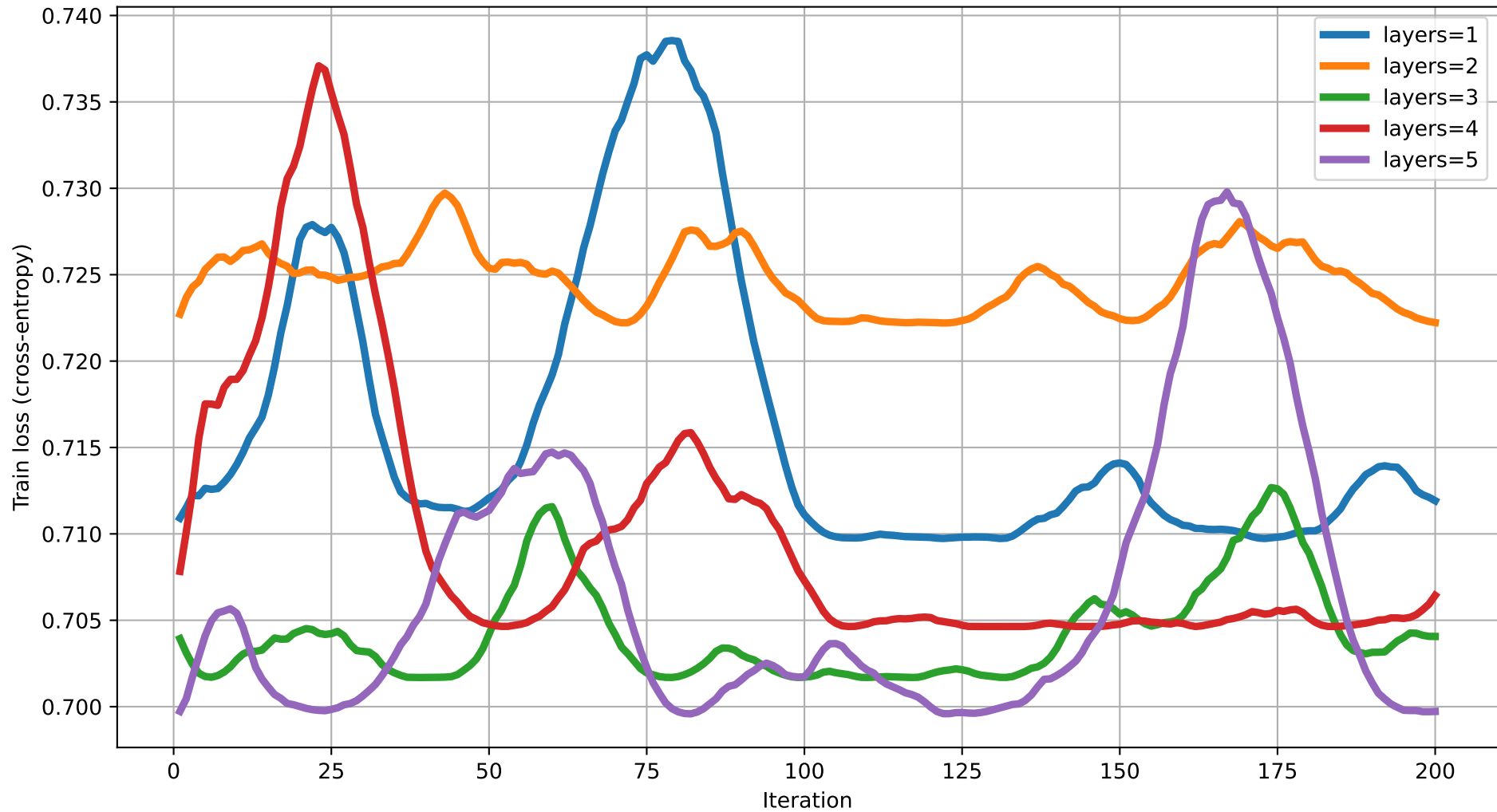
Train loss vs Iteration (dim=14) rot=RZ, ent=ring, gate=CNOT
