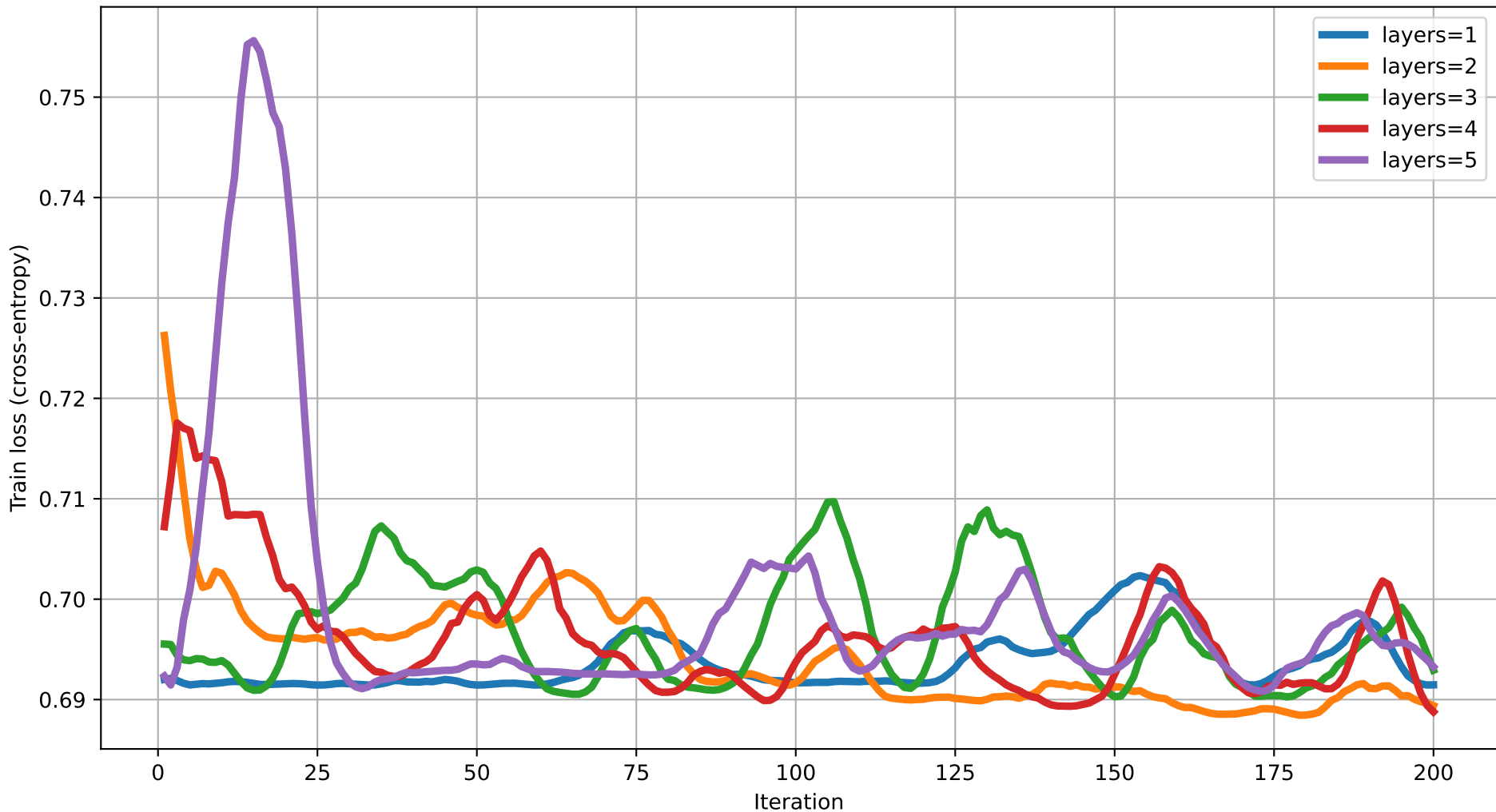
Train loss vs Iteration (dim=12) rot=RY, ent=pairwise, gate=IsingXX
