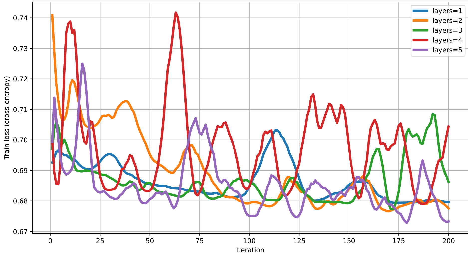
Train loss vs Iteration (dim=20) rot=RYZ, ent=pairwise, gate=IsingXX
