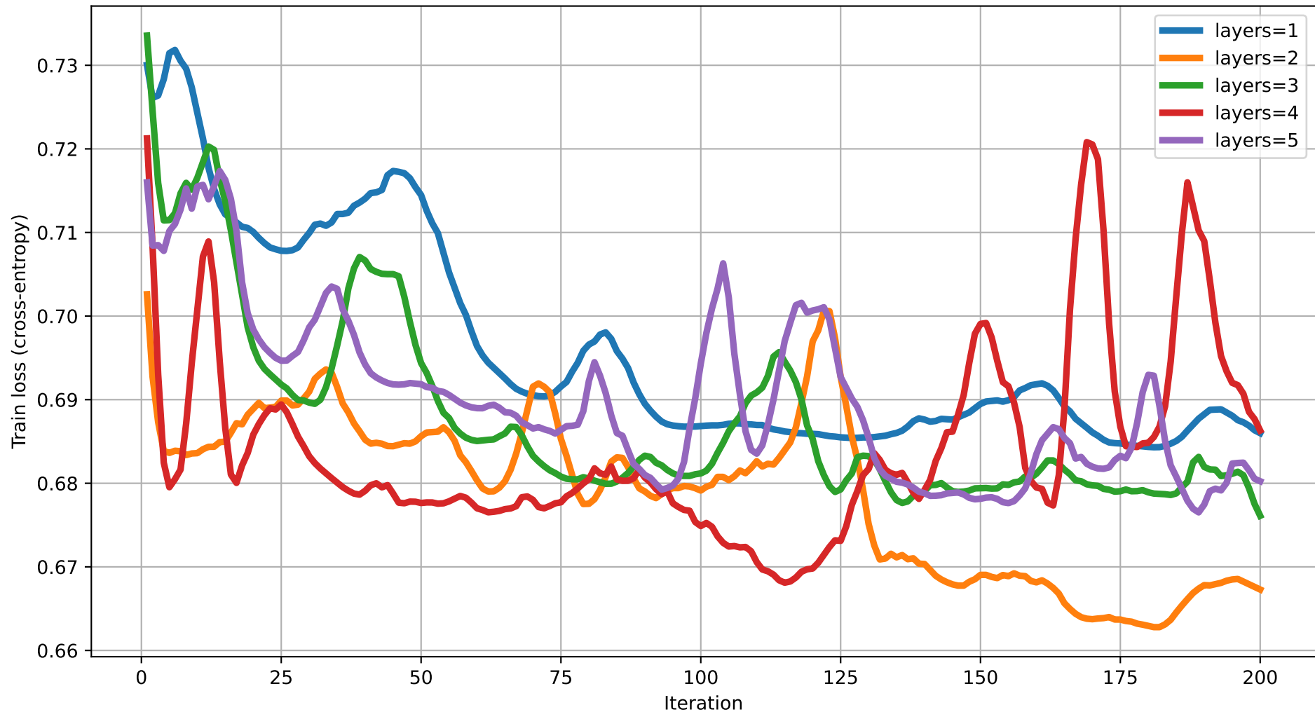
Train loss vs Iteration (dim=20) rot=RYZ, ent=full, gate=IsingXX
