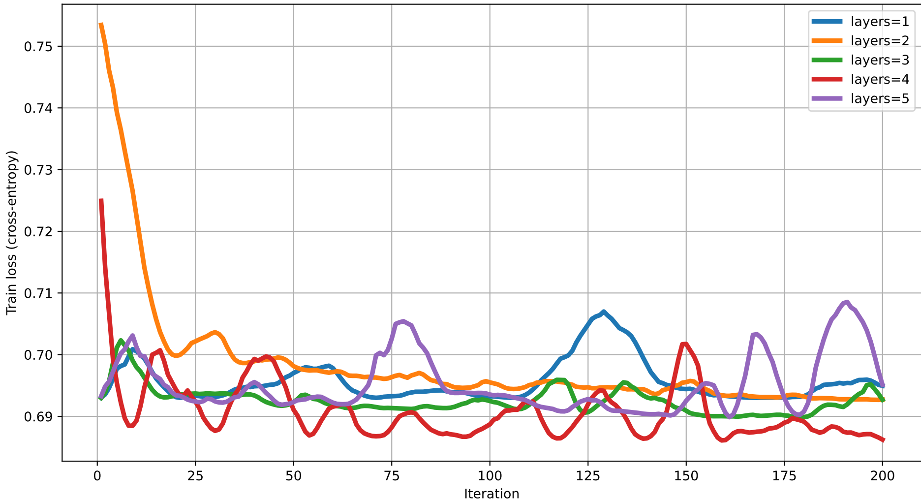
Train loss vs Iteration (degree=2) rot=RY, ent=pairwise, gate=IsingXX
