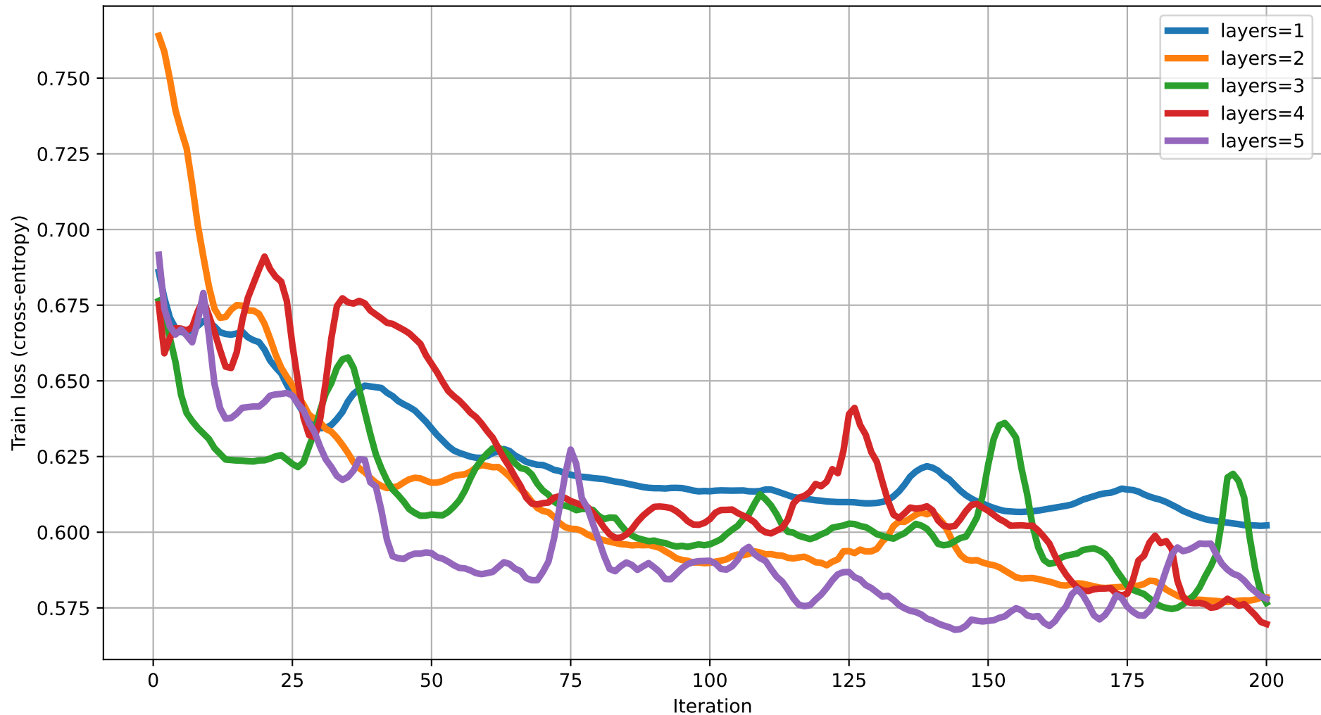
Train loss vs Iteration (dim=10) rot=Rot, ent=full, gate=lsingXX
