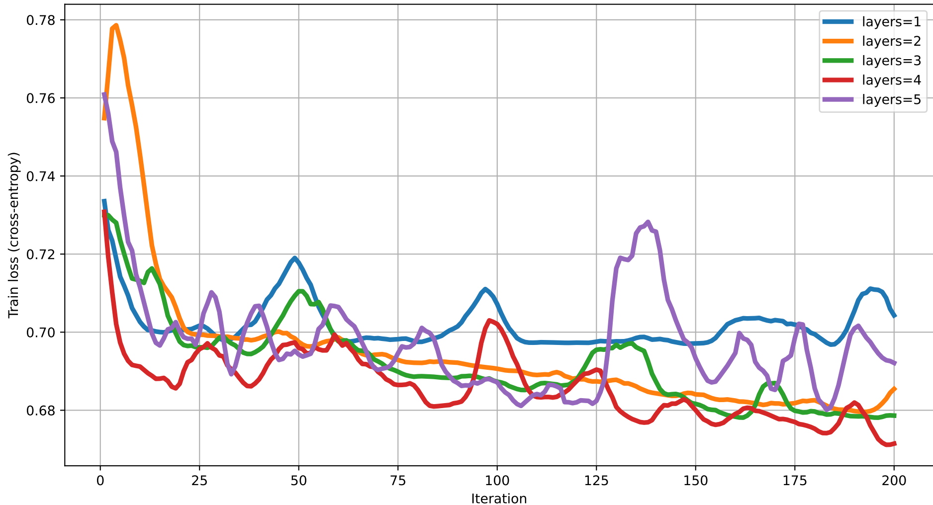
Train loss vs Iteration (dim=19) rot=Rot, ent=ring, gate=CZ
