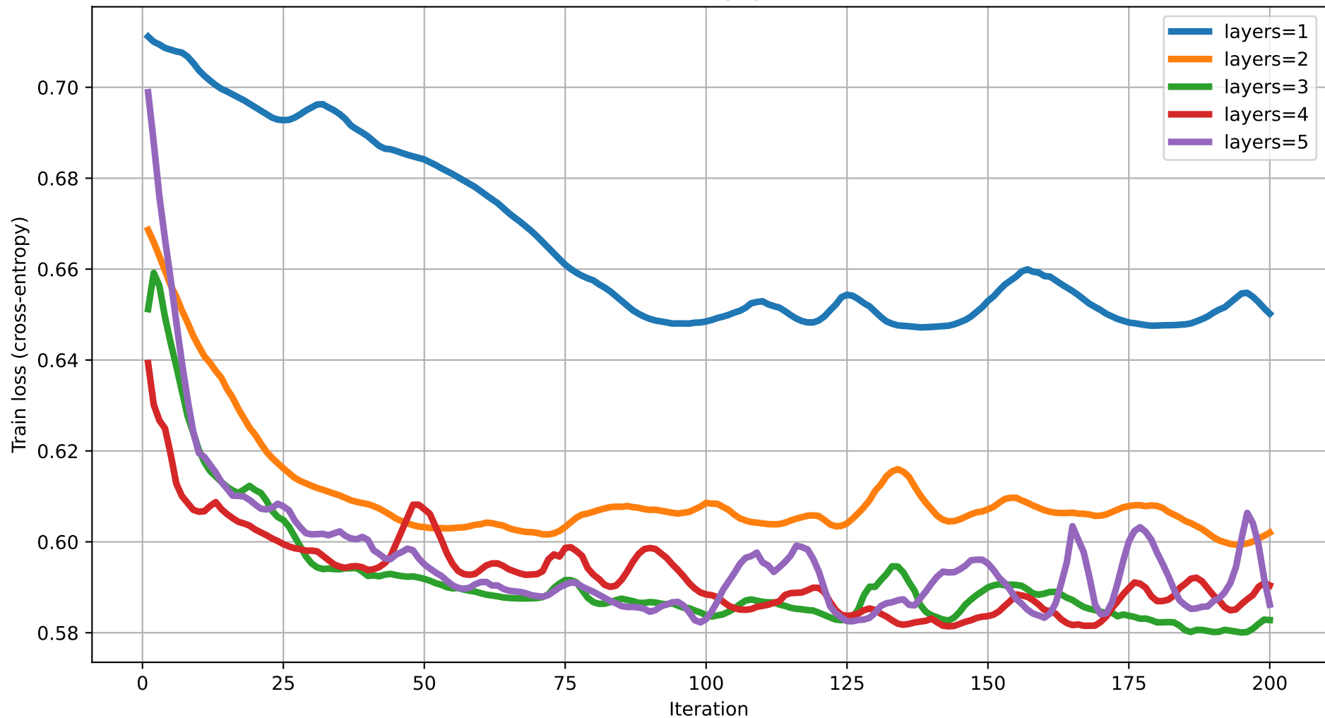
Train loss vs Iteration (degree=5) rot=Rot, ent=ring, gate=CNOT
