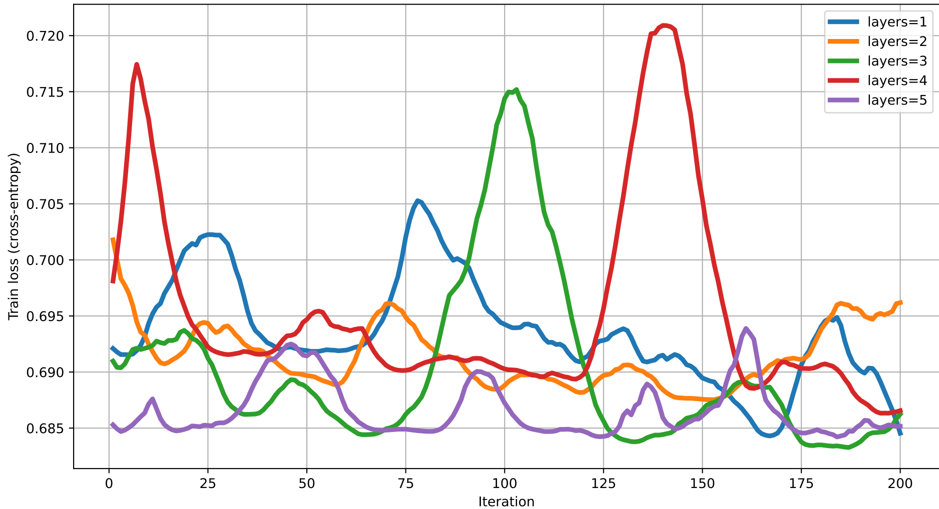
Train loss vs Iteration (dim=18) rot=RX, ent=ring, gate=CNOT
