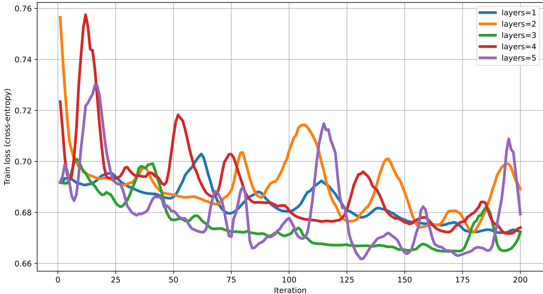
Train loss vs Iteration (dim=18) rot=RYZ, ent=chain, gate=IsingXX
