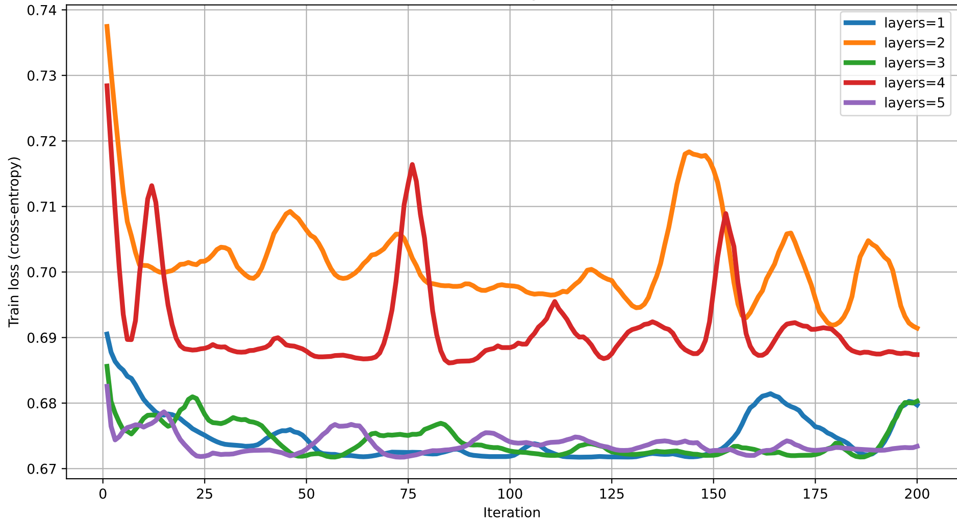
Train loss vs Iteration (degree=2) rot=RX, ent=full, gate=IsingXX
