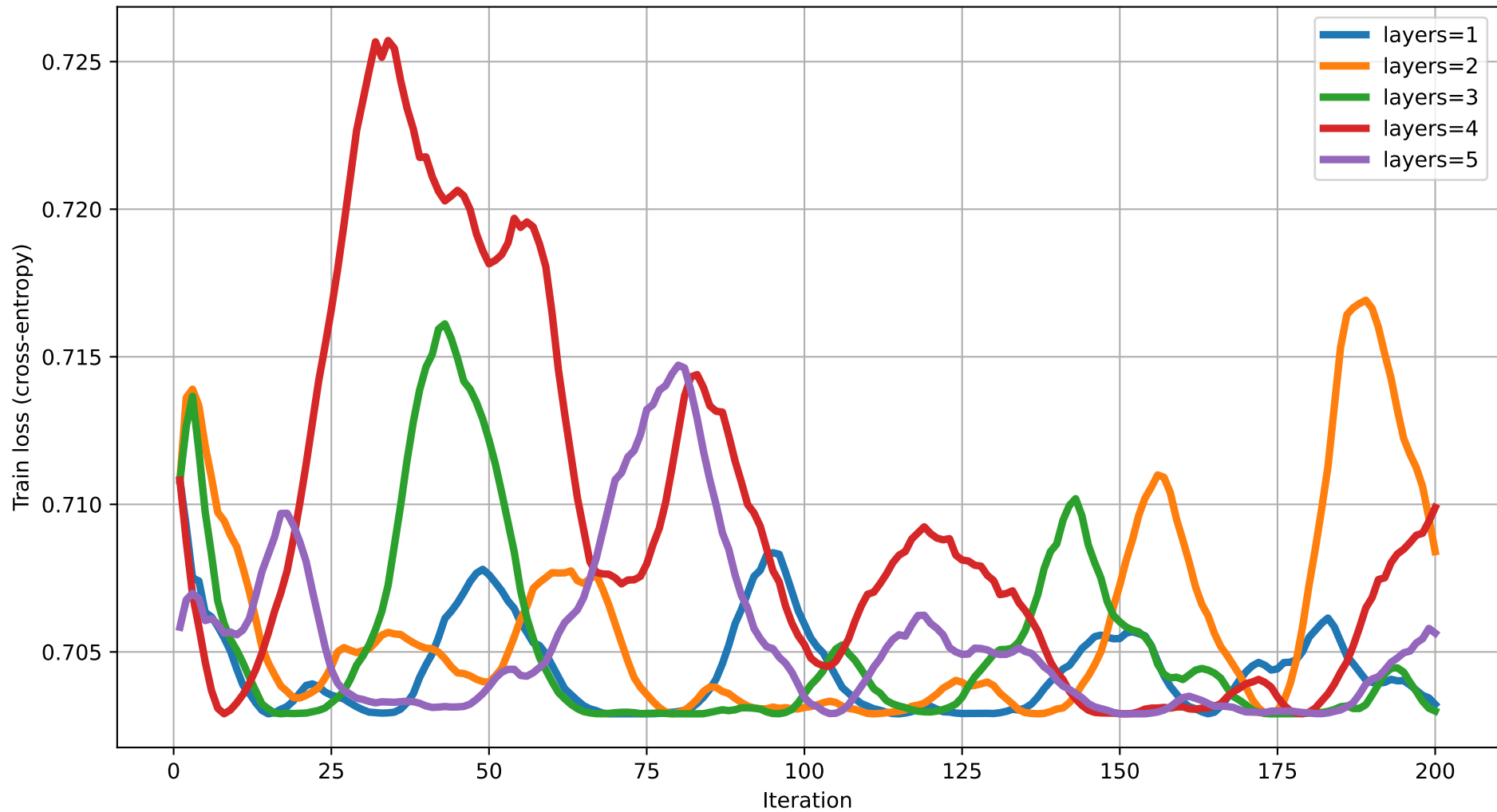
Train loss vs Iteration (dim=12) rot=RZ, ent=ring, gate=CZ
