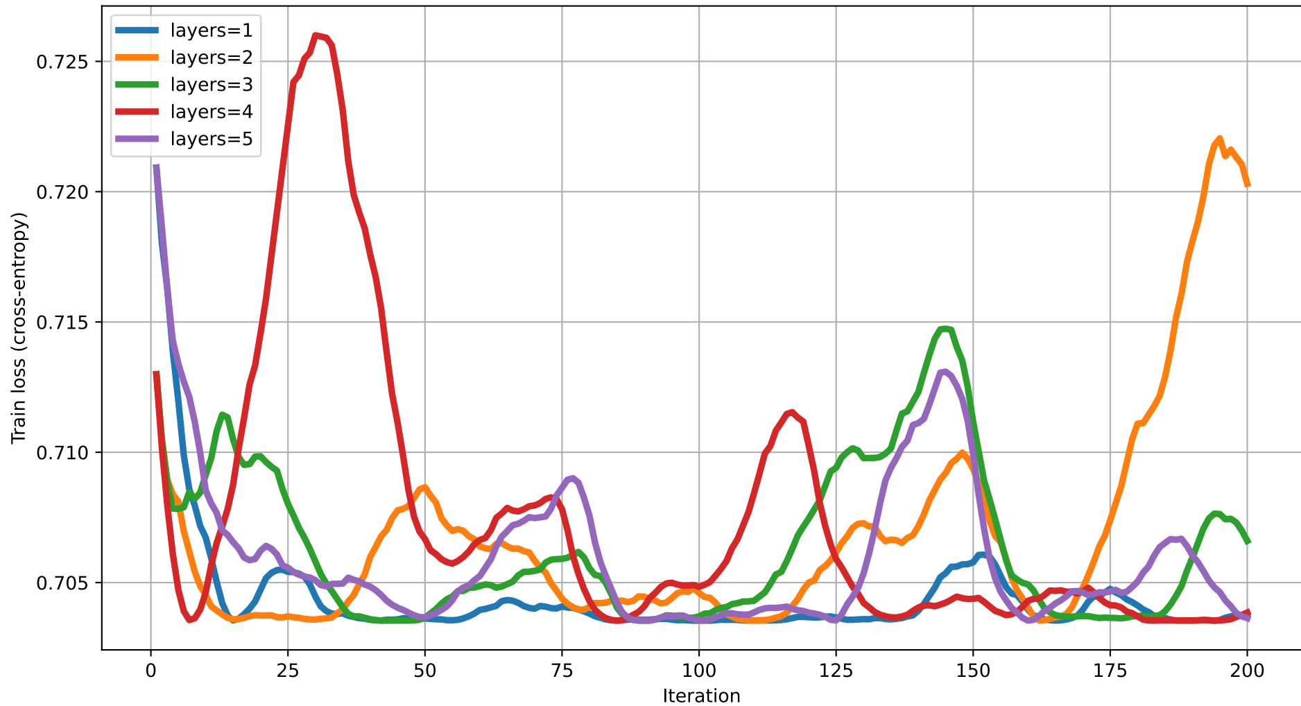
Train loss vs Iteration (dim=11) rot=RZ, ent=full, gate=CNOT
