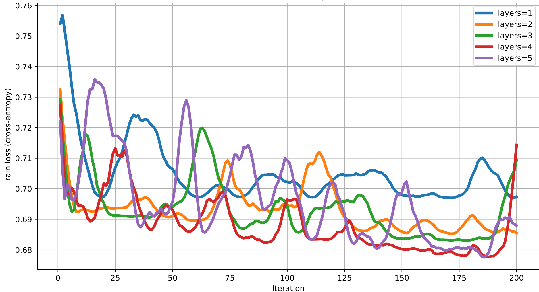
Train loss vs Iteration (dim=18) rot=RYZ, ent=chain, gate=CZ
