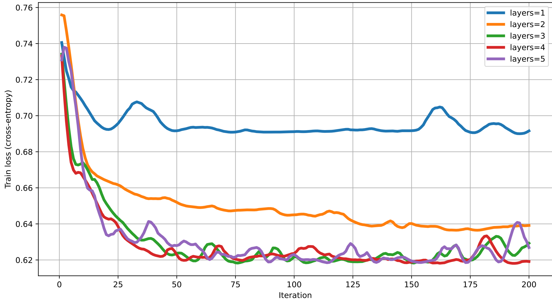
Train loss vs Iteration (degree=5) rot=Rot, ent=pairwise, gate=CNOT
