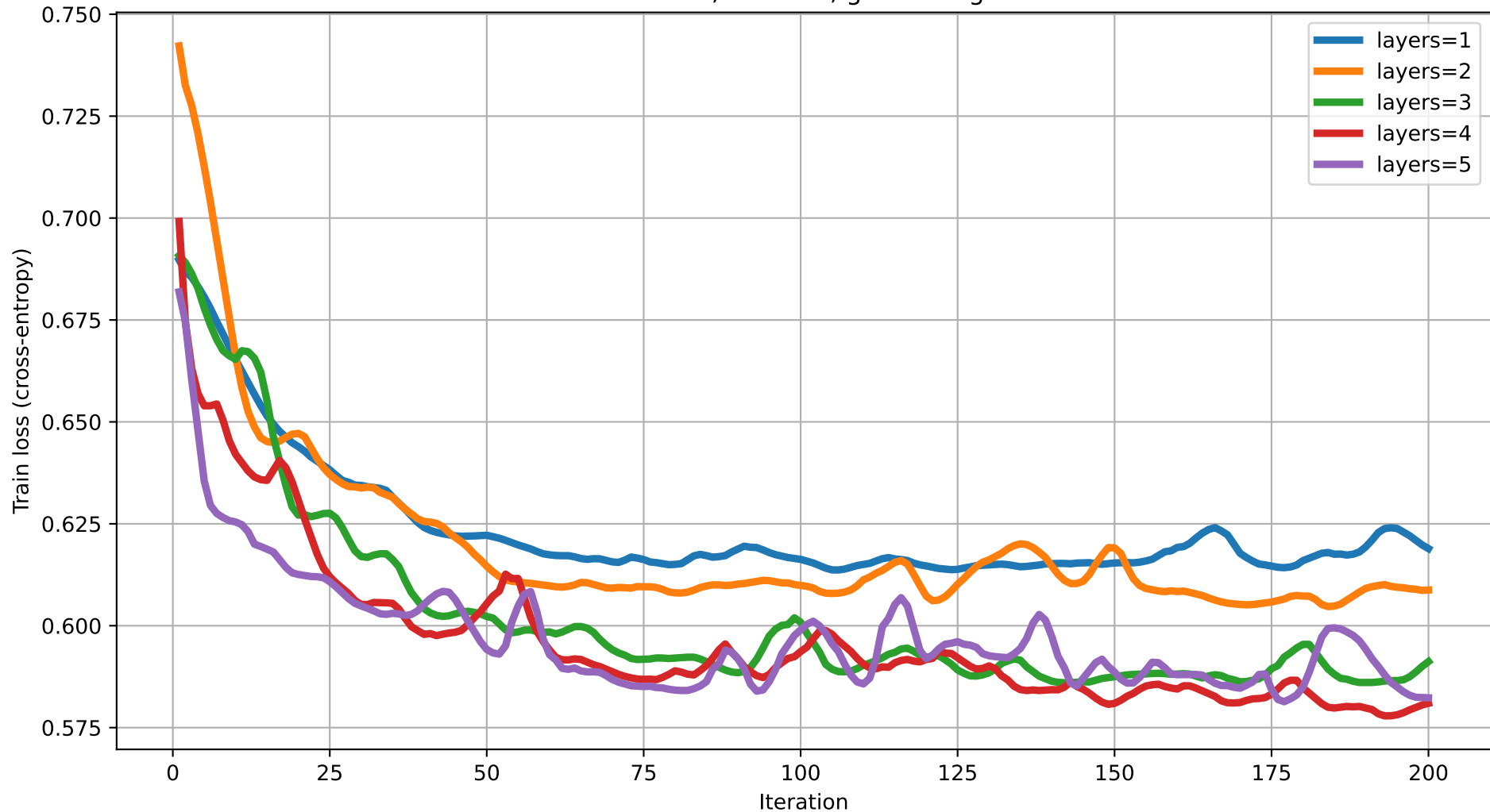
Train loss vs Iteration (degree=3) rot=RYZ, ent=full, gate=IsingXX
