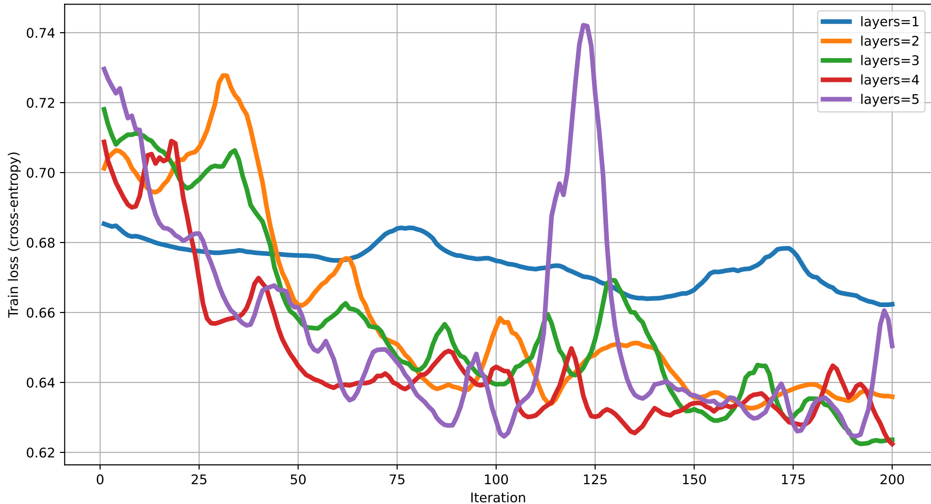
Train loss vs Iteration (dim=12) rot=Rot, ent=ring, gate=CNOT
