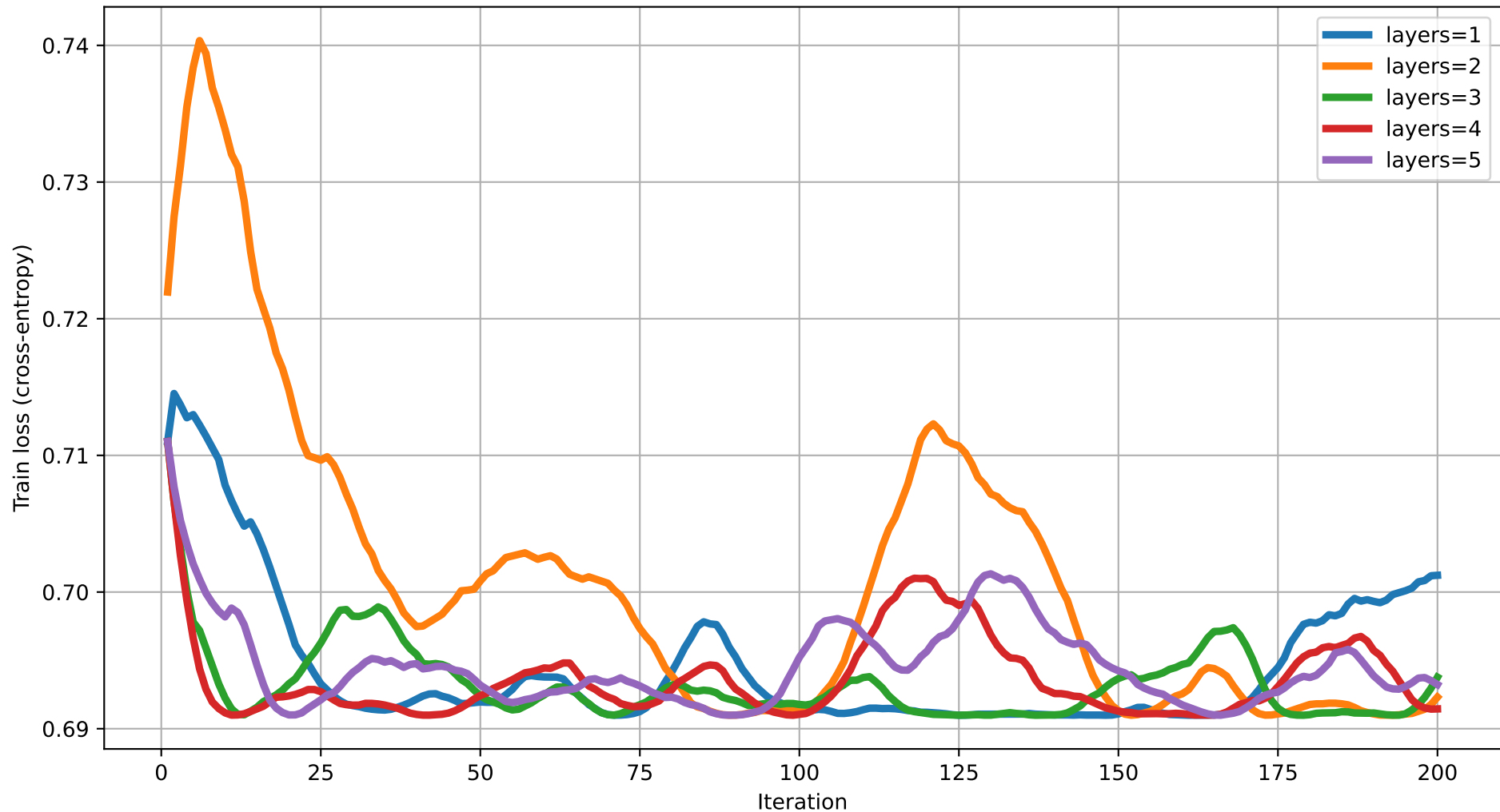
Train loss vs Iteration (dim=20) rot=RZ, ent=full, gate=CZ
