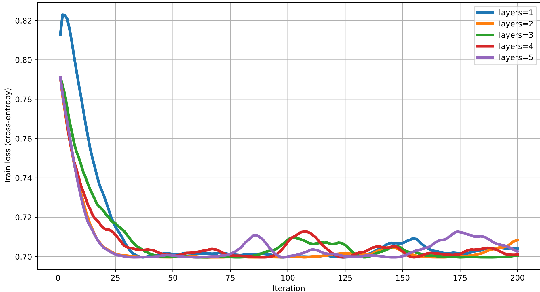
Train loss vs Iteration (dim=4) rot=RZ, ent=pairwise, gate=CZ
