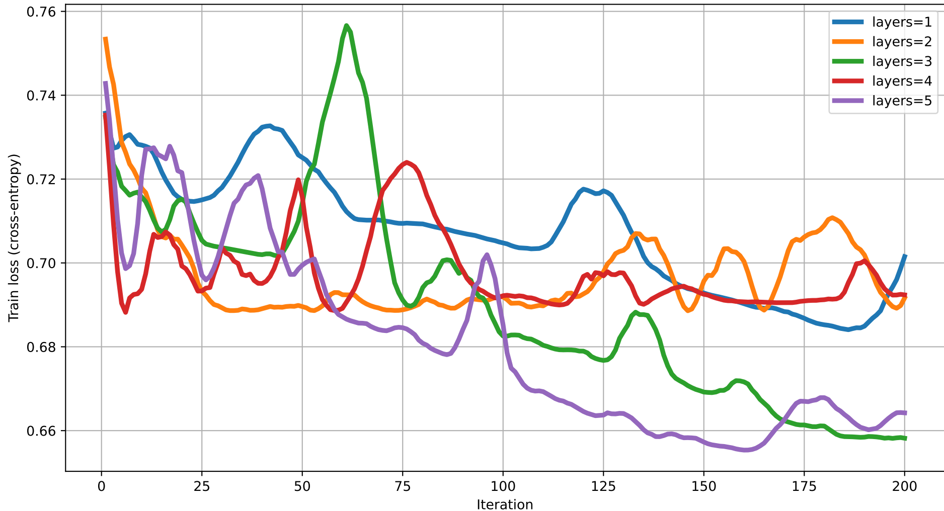
Train loss vs Iteration (dim=16) rot=RX, ent=full, gate=IsingXX
