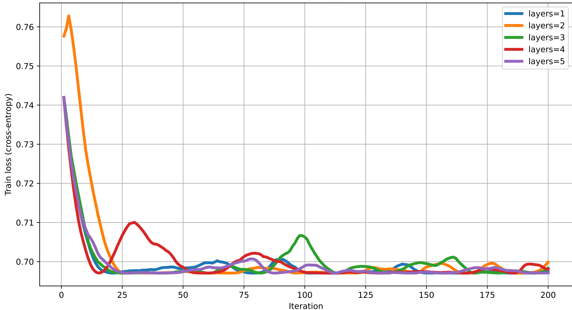
Train loss vs Iteration (degree=5) rot=RZ, ent=chain, gate=CZ
