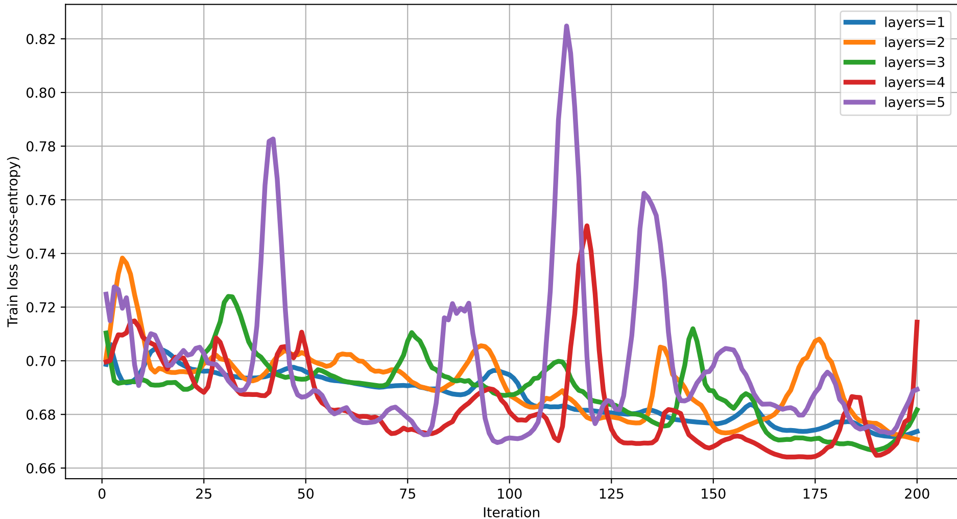
Train loss vs Iteration (dim=14) rot=Rot, ent=pairwise, gate=IsingXX
