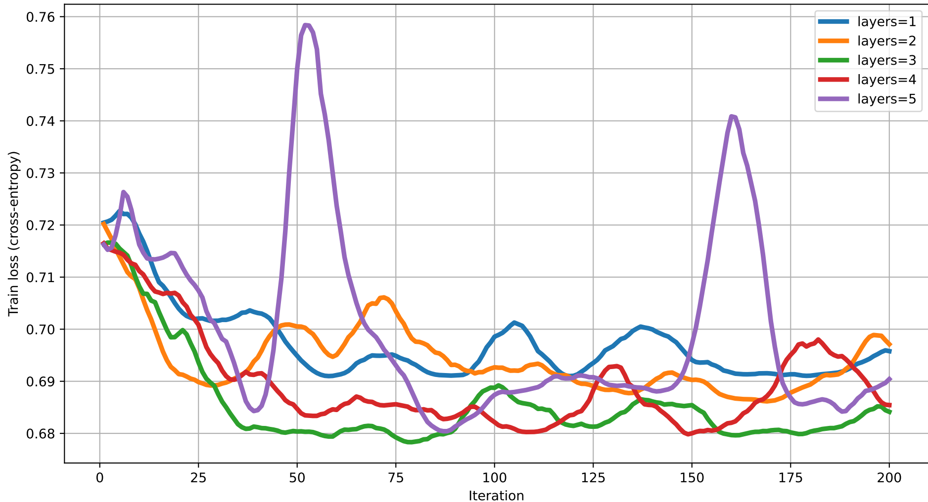
Train loss vs Iteration (dim=3) rot=RX, ent=full, gate=CZ
