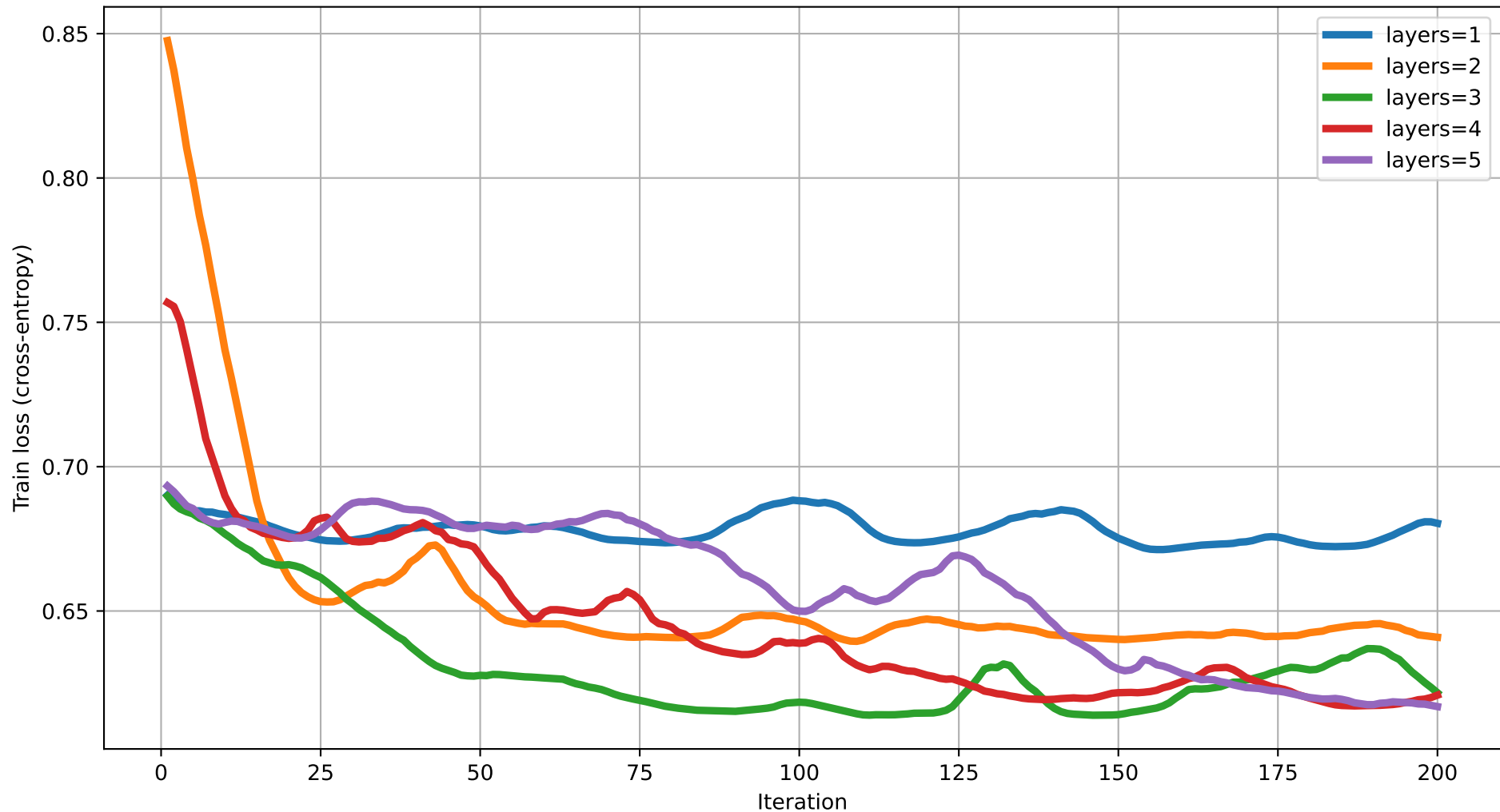
Train loss vs Iteration (dim=8) rot=RZ, ent=chain, gate=IsingXX
