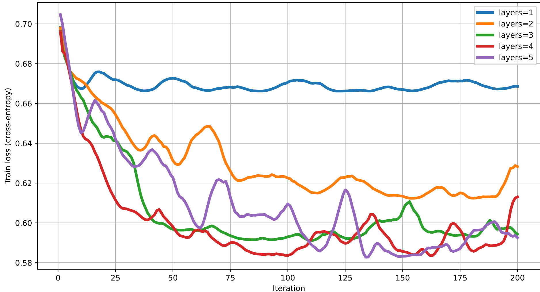
Train loss vs Iteration (dim=10) rot=RY, ent=ring, gate=CZ
