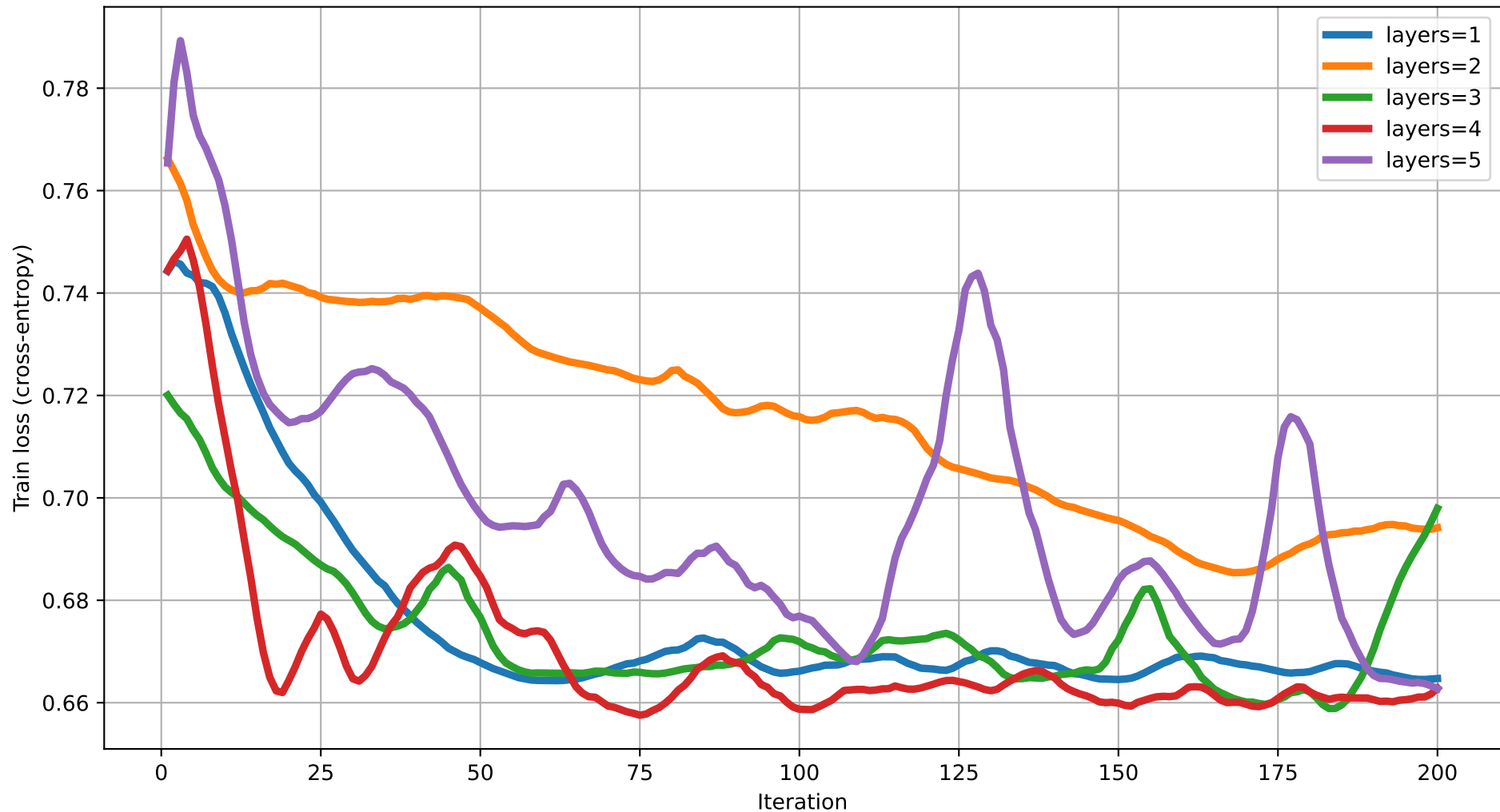
Train loss vs Iteration (dim=3) rot=RY, ent=ring, gate=CNOT
