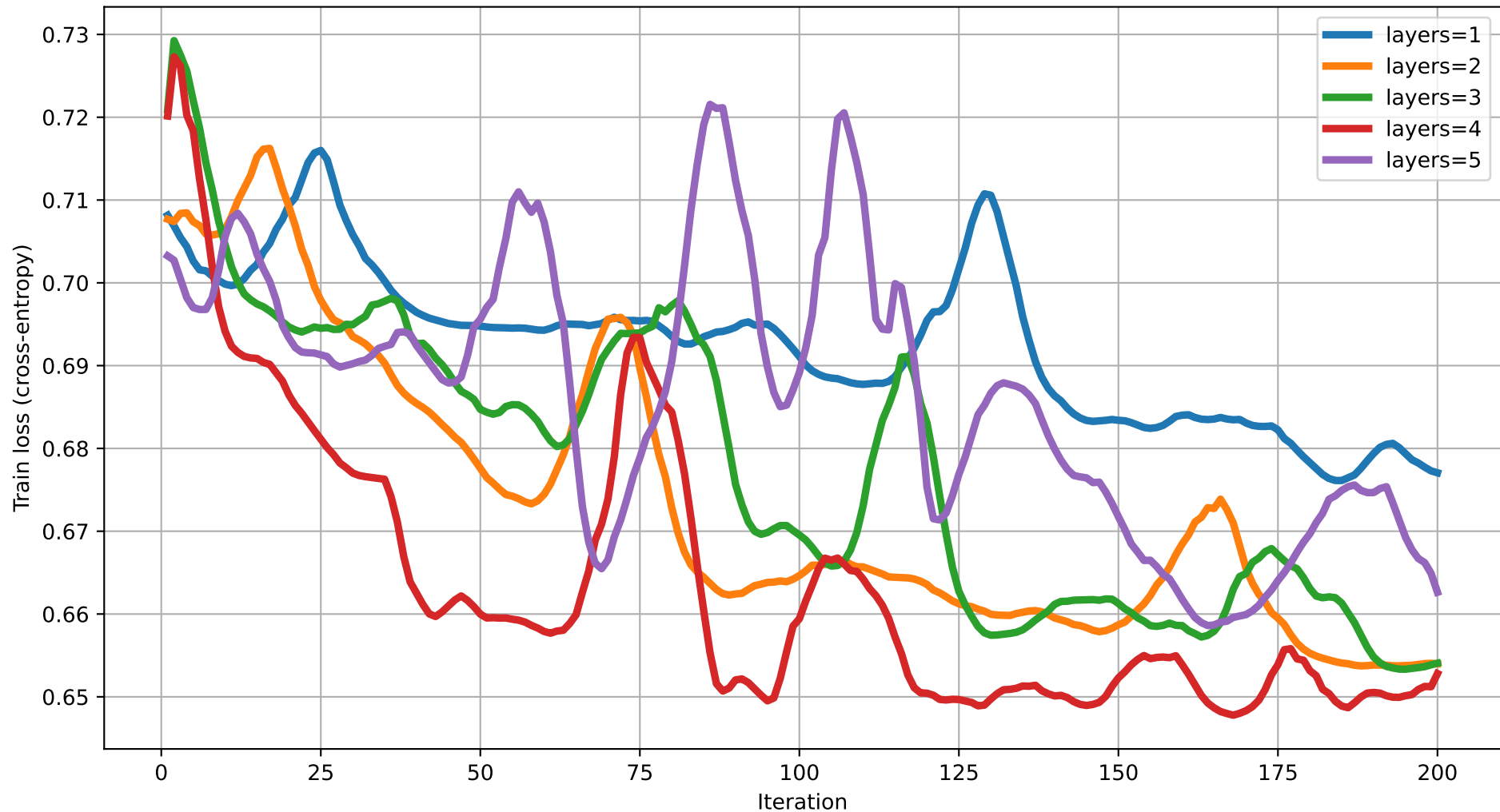
Train loss vs Iteration (dim=6) rot=RY, ent=full, gate=CZ
