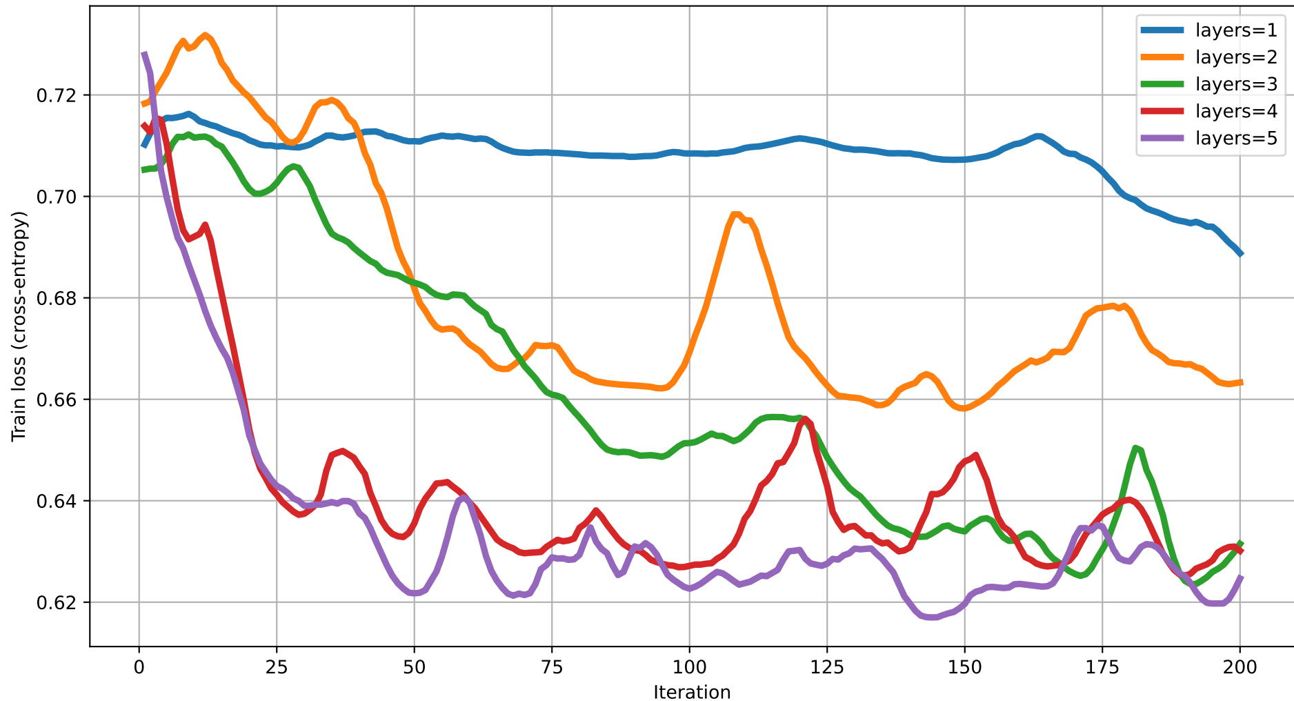
Train loss vs Iteration (dim=4) rot=RY, ent=ring, gate=CNOT
