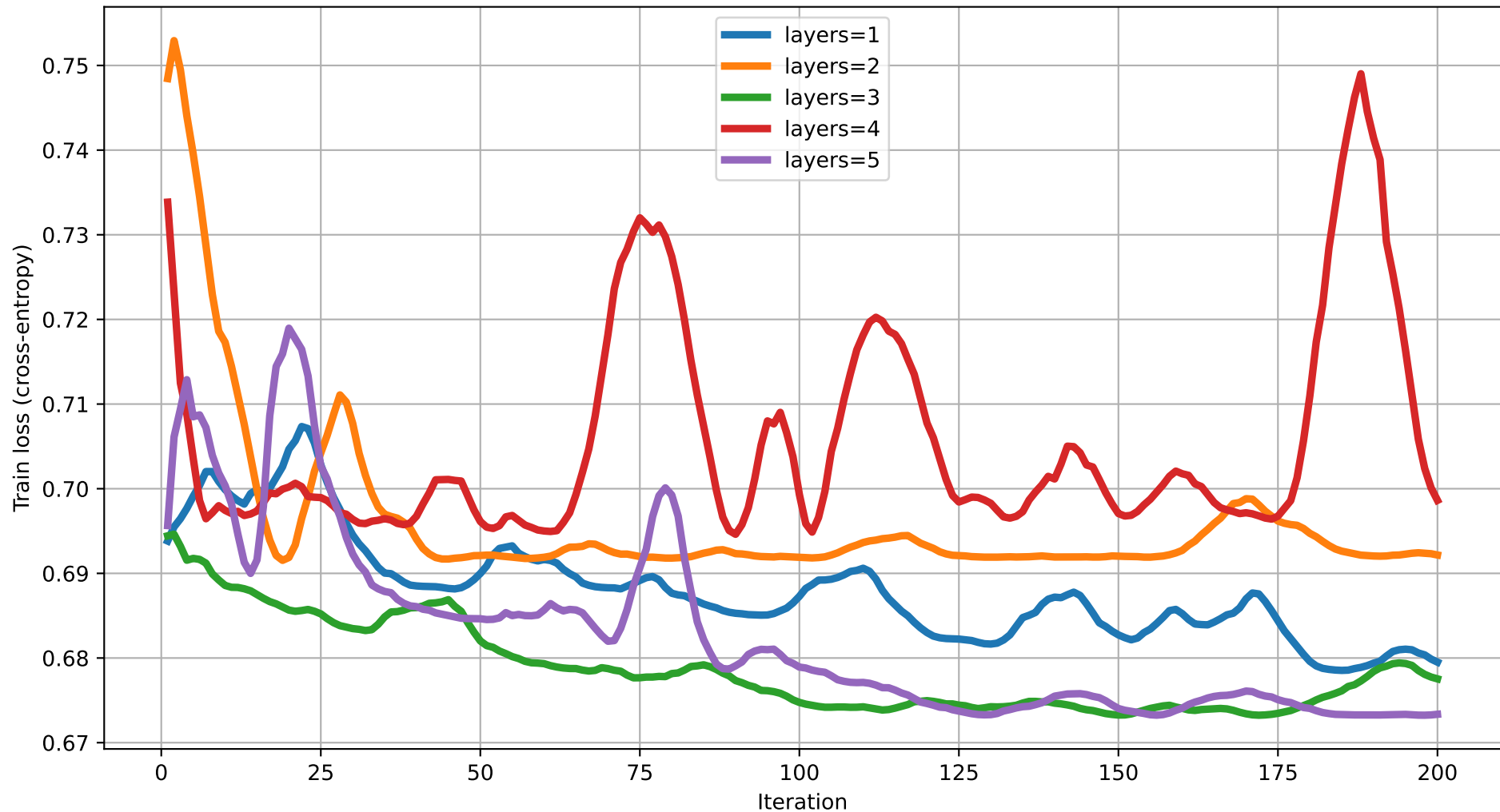
Train loss vs Iteration (dim=19) rot=RX, ent=pairwise, gate=IsingXX
