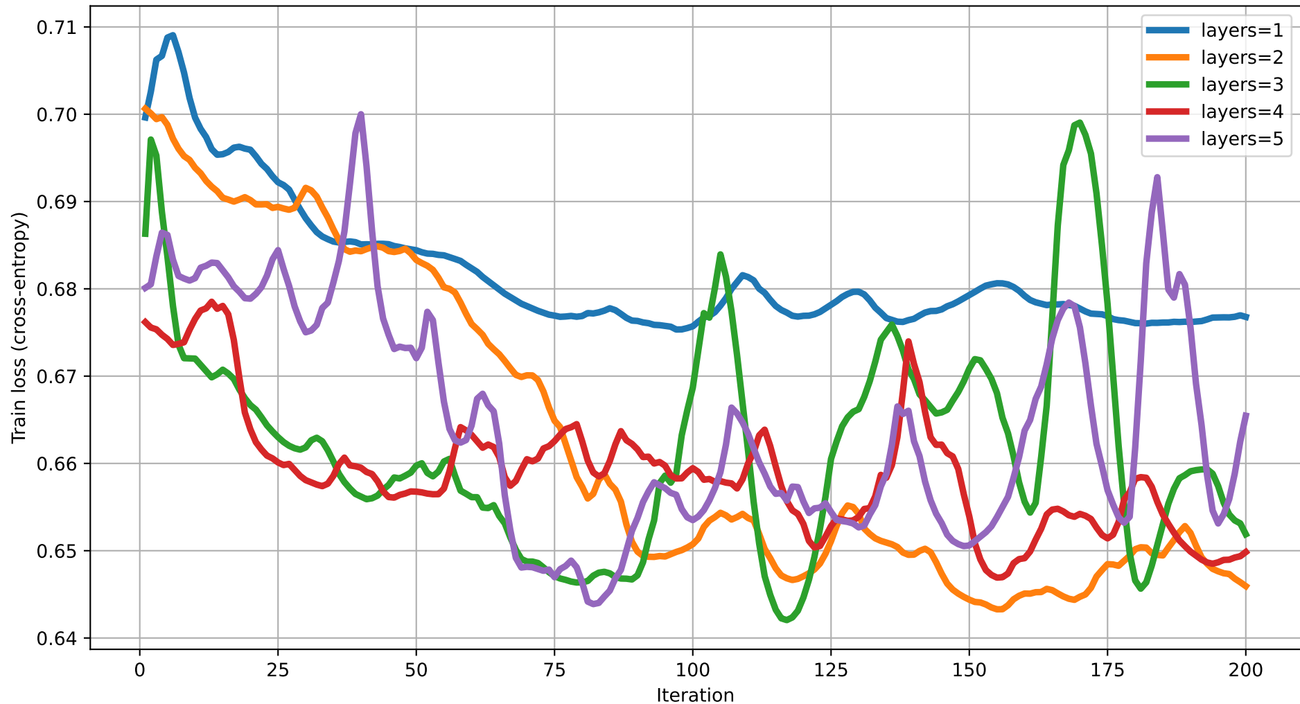
Train loss vs Iteration (dim=9) rot=Rot, ent=ring, gate=CNOT
