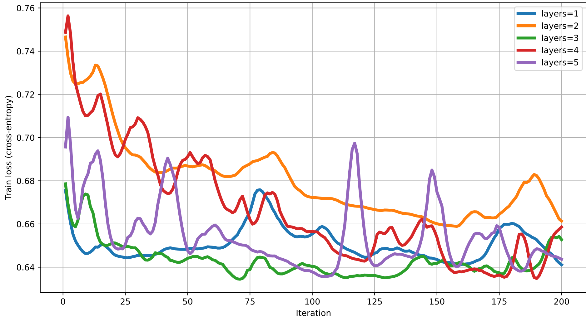
Train loss vs Iteration (dim=5) rot=RYZ, ent=ring, gate=IsingXX
