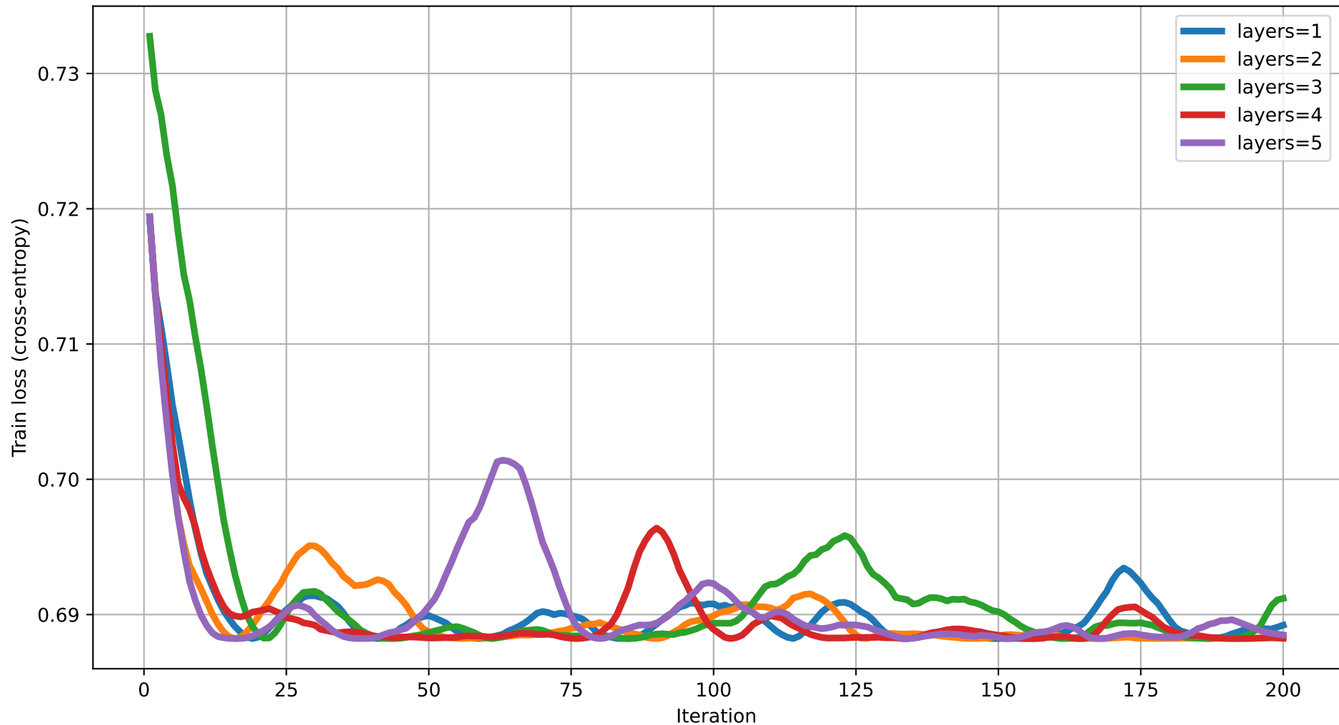
Train loss vs Iteration (degree=4) rot=RZ, ent=pairwise, gate=CNOT
