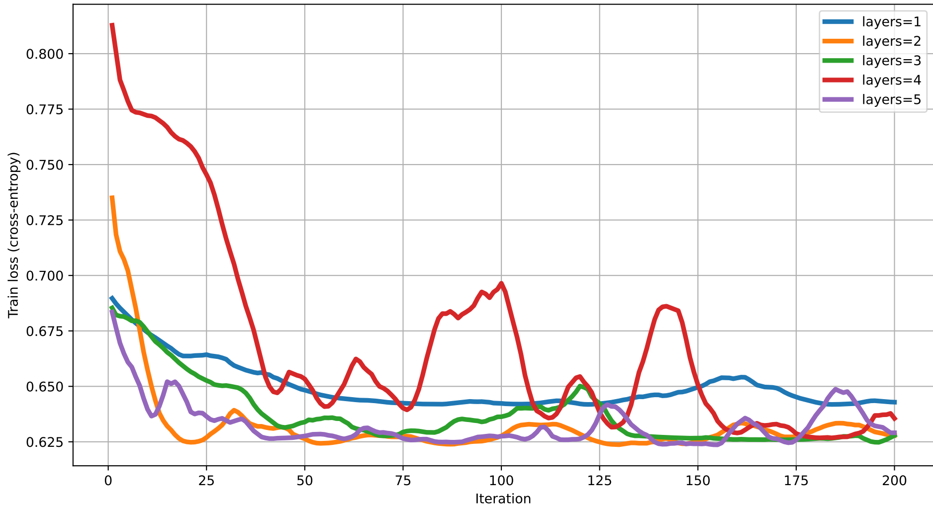
Train loss vs Iteration (dim=2) rot=RZ, ent=chain, gate=IsingXX
