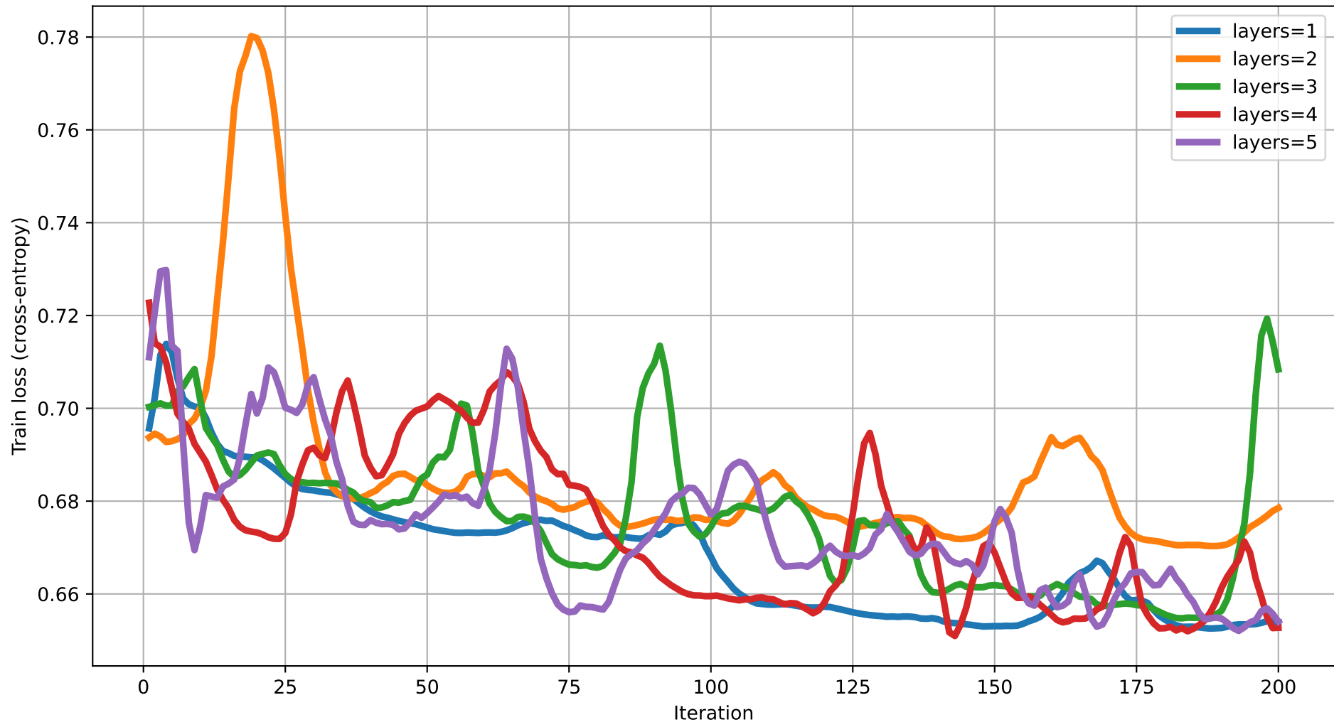
Train loss vs Iteration (dim=7) rot=Rot, ent=chain, gate=IsingXX
