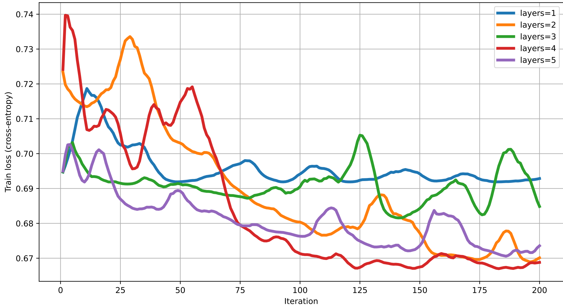
Train loss vs Iteration (dim=6) rot=RY, ent=chain, gate=IsingXX
