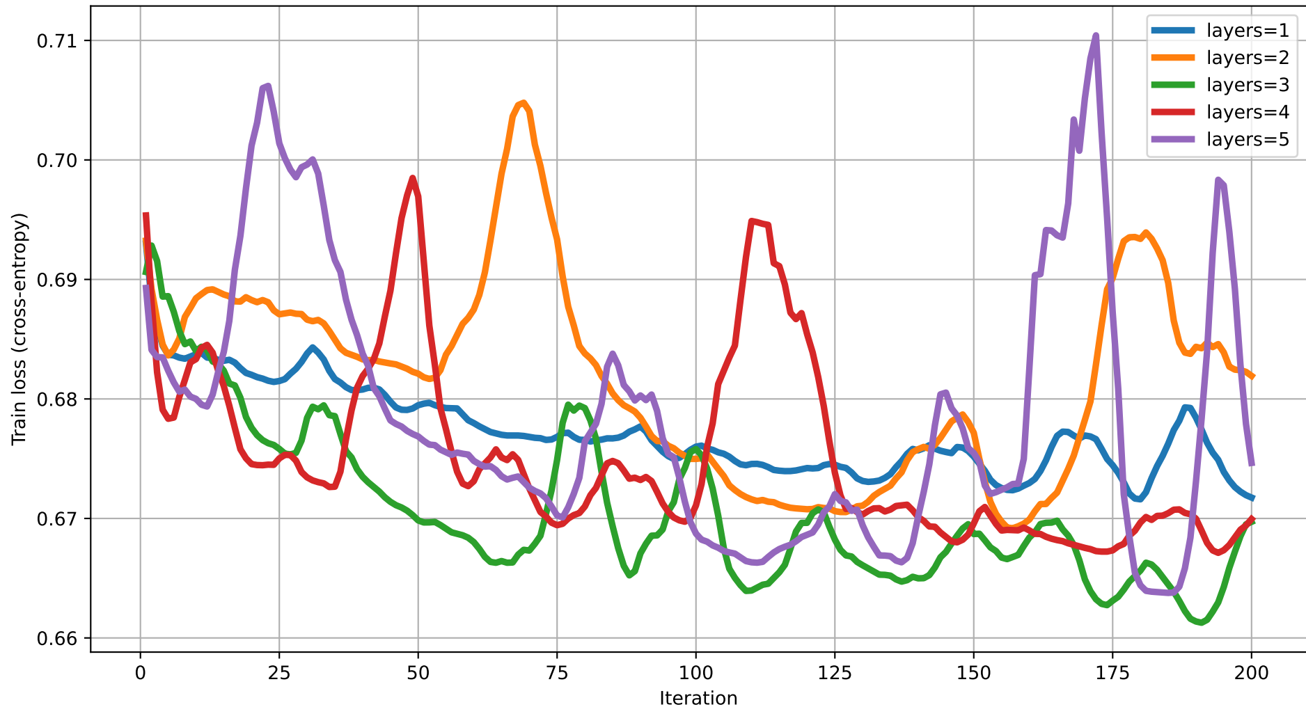
Train loss vs Iteration (dim=13) rot=RYZ, ent=full, gate=CZ
