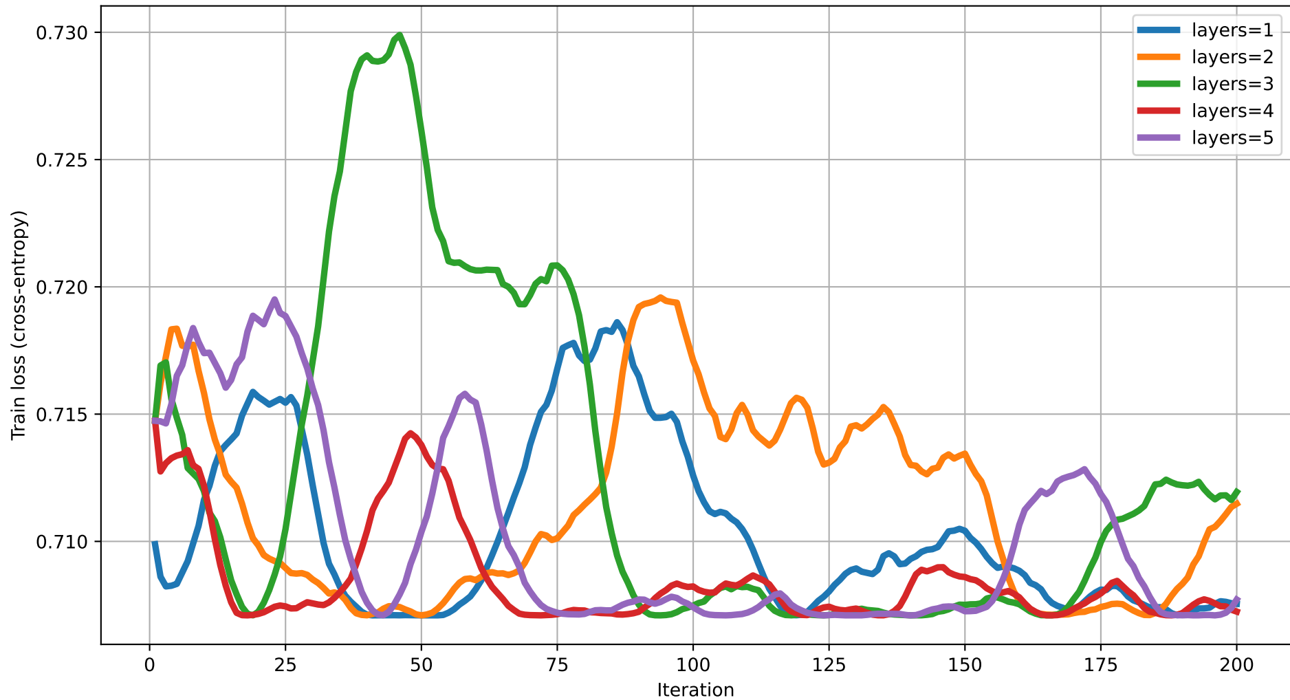
Train loss vs Iteration (dim=6) rot=RZ, ent=chain, gate=CNOT
