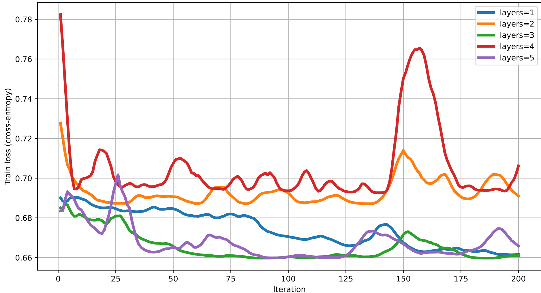
Train loss vs Iteration (dim=9) rot=RX, ent=chain, gate=IsingXX
