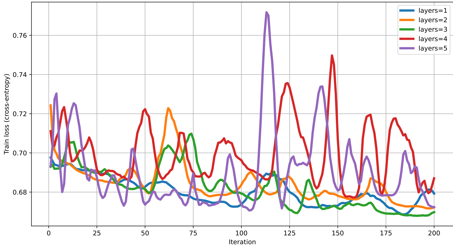
Train loss vs Iteration (dim=10) rot=Rot, ent=pairwise, gate=IsingXX
