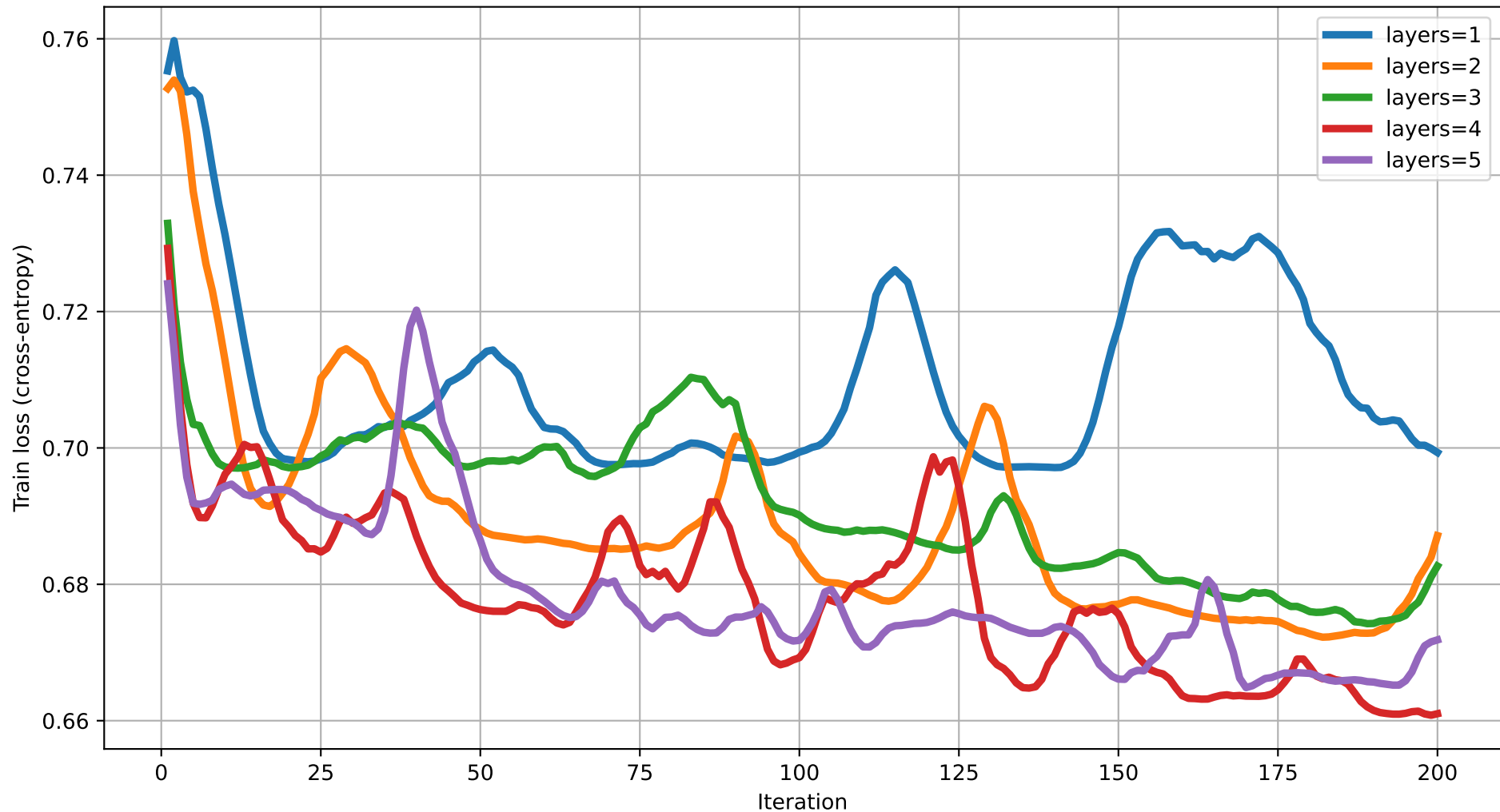
Train loss vs Iteration (dim=19) rot=RYZ, ent=ring, gate=CZ
