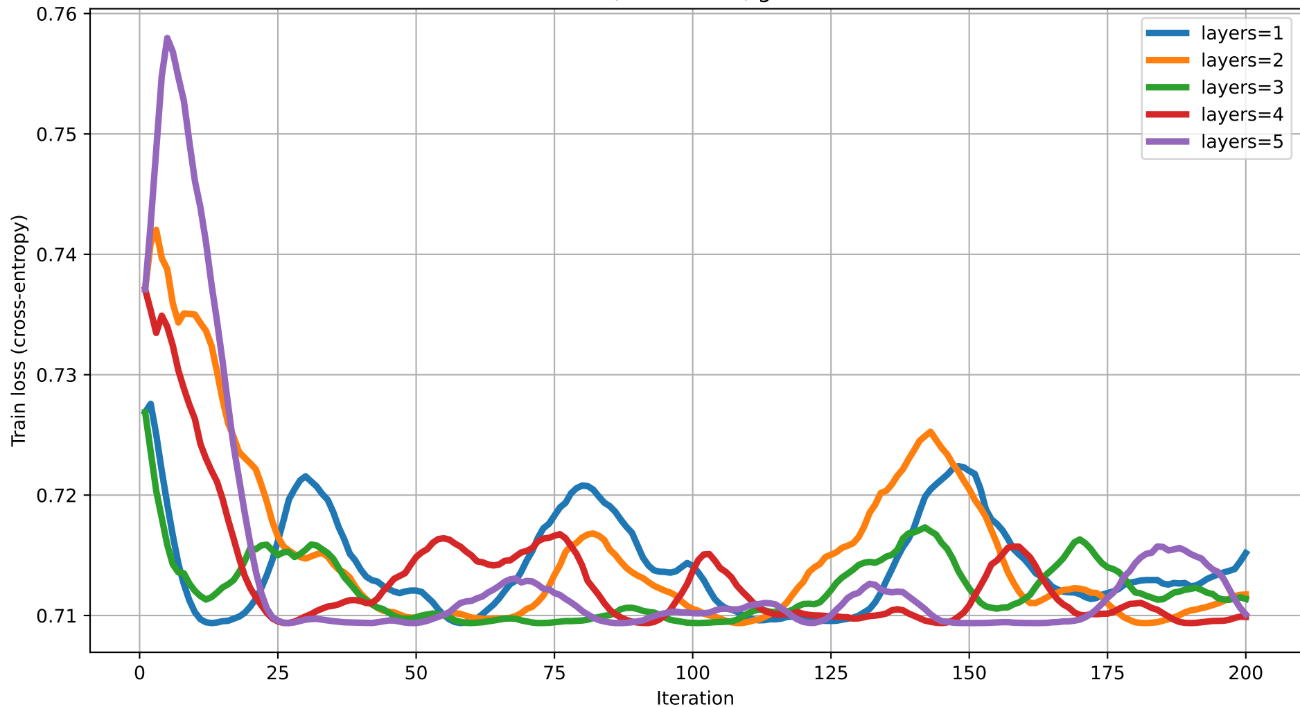
Train loss vs Iteration (dim=5) rot=RZ, ent=chain, gate=CZ
