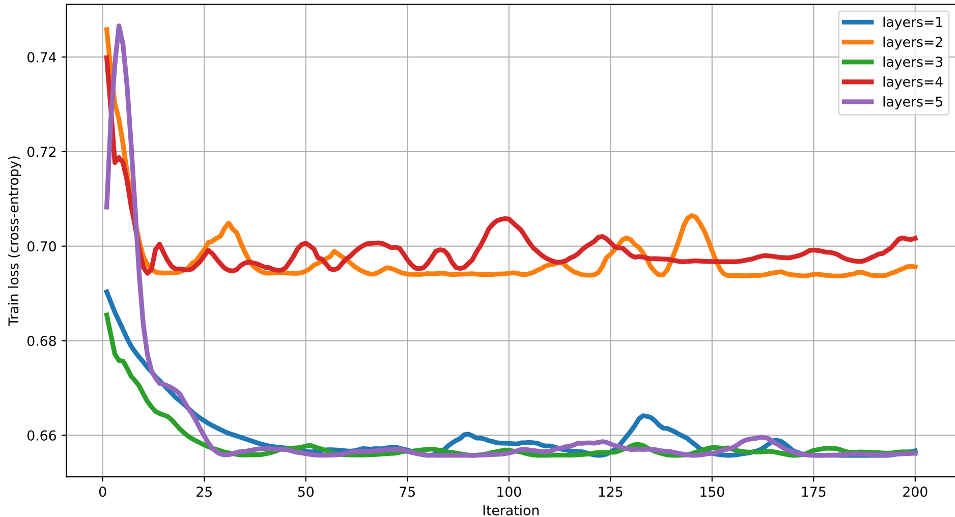
Train loss vs Iteration (degree=5) rot=RX, ent=chain, gate=IsingXX
