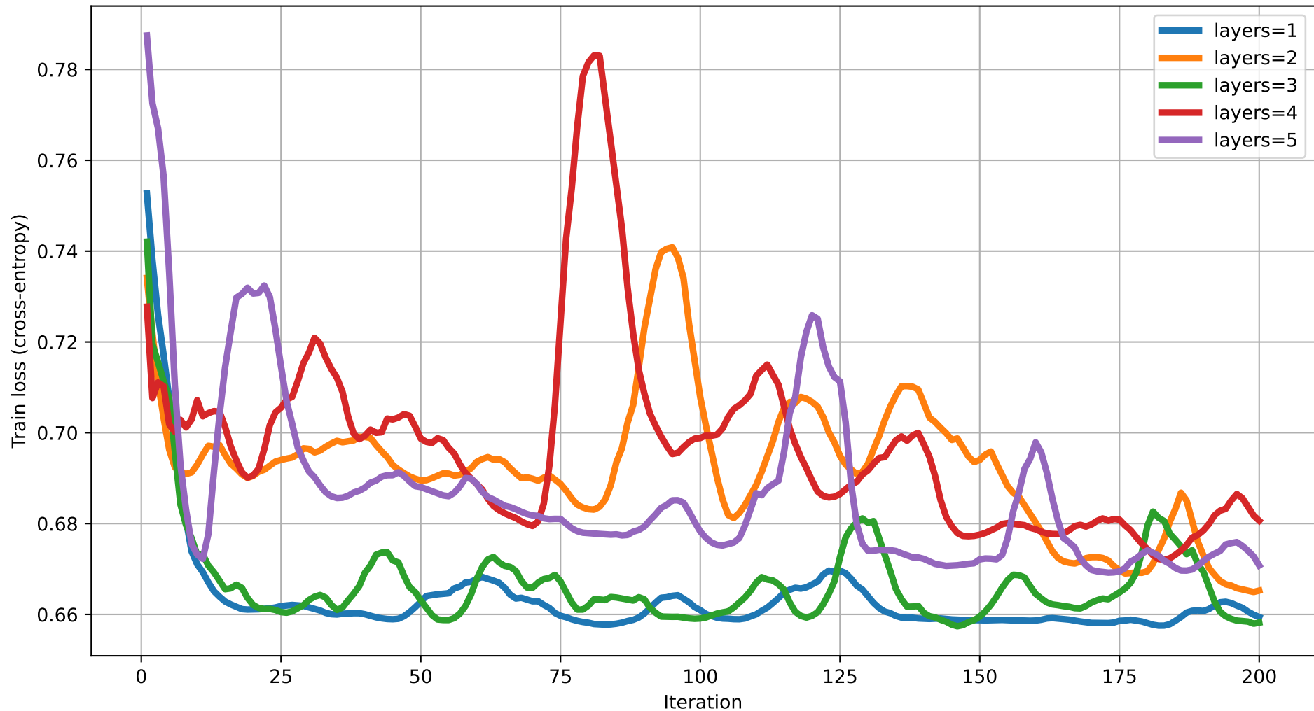
Train loss vs Iteration (dim=16) rot=RYZ, ent=ring, gate=IsingXX
