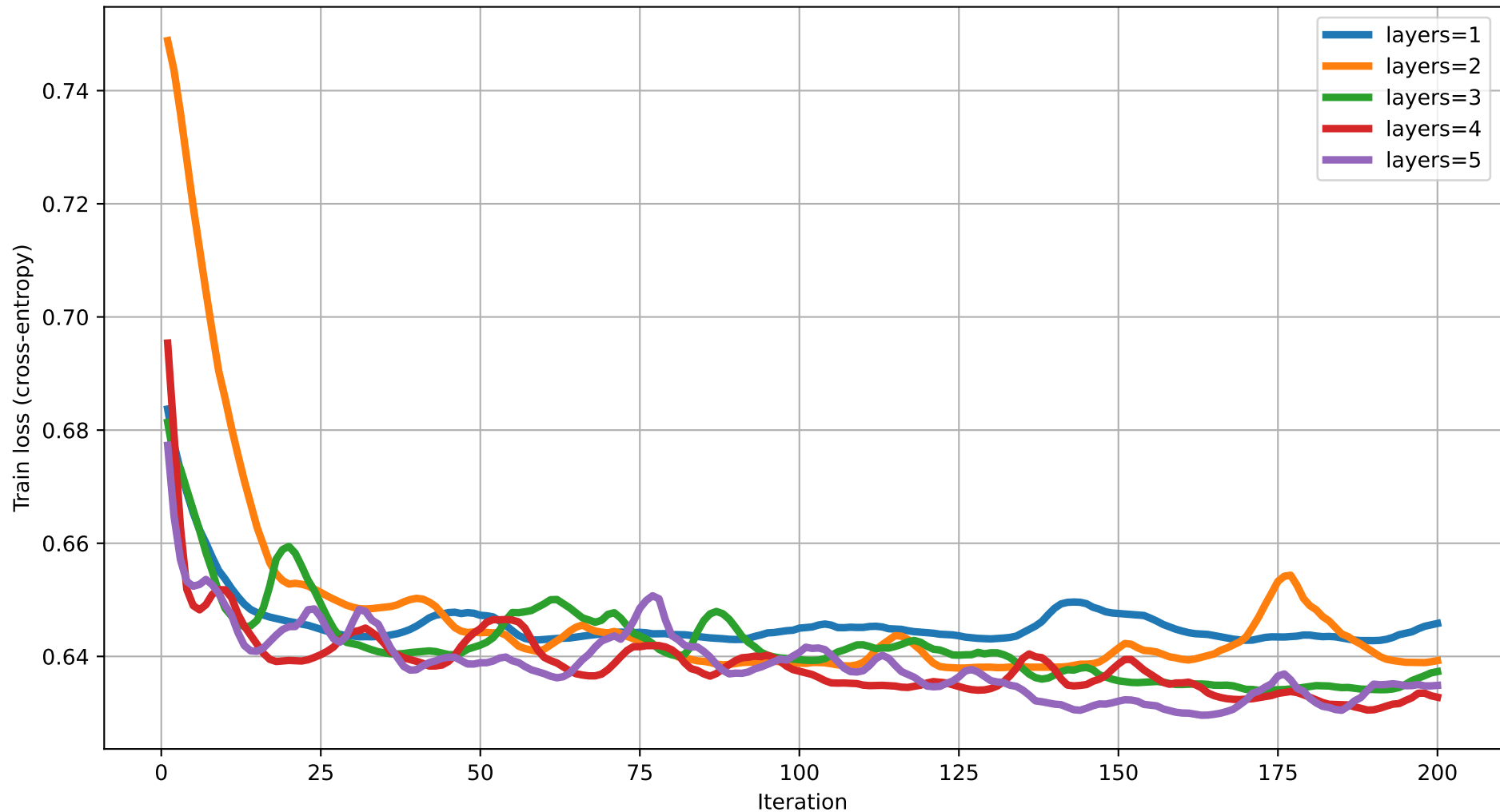
Train loss vs Iteration (degree=4) rot=RZ, ent=full, gate=IsingXX
