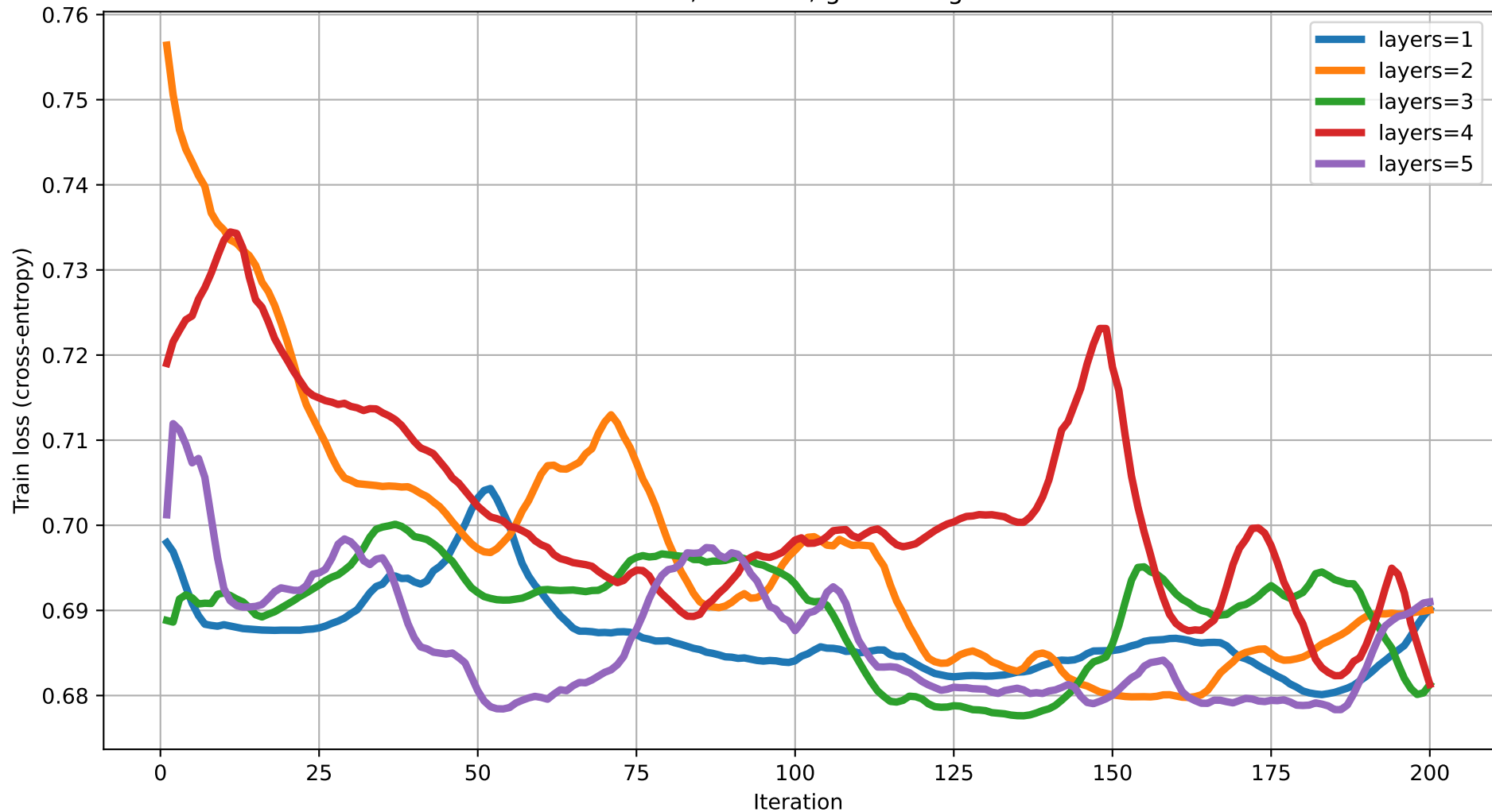
Train loss vs Iteration (dim=3) rot=RZ, ent=full, gate=IsingXX
