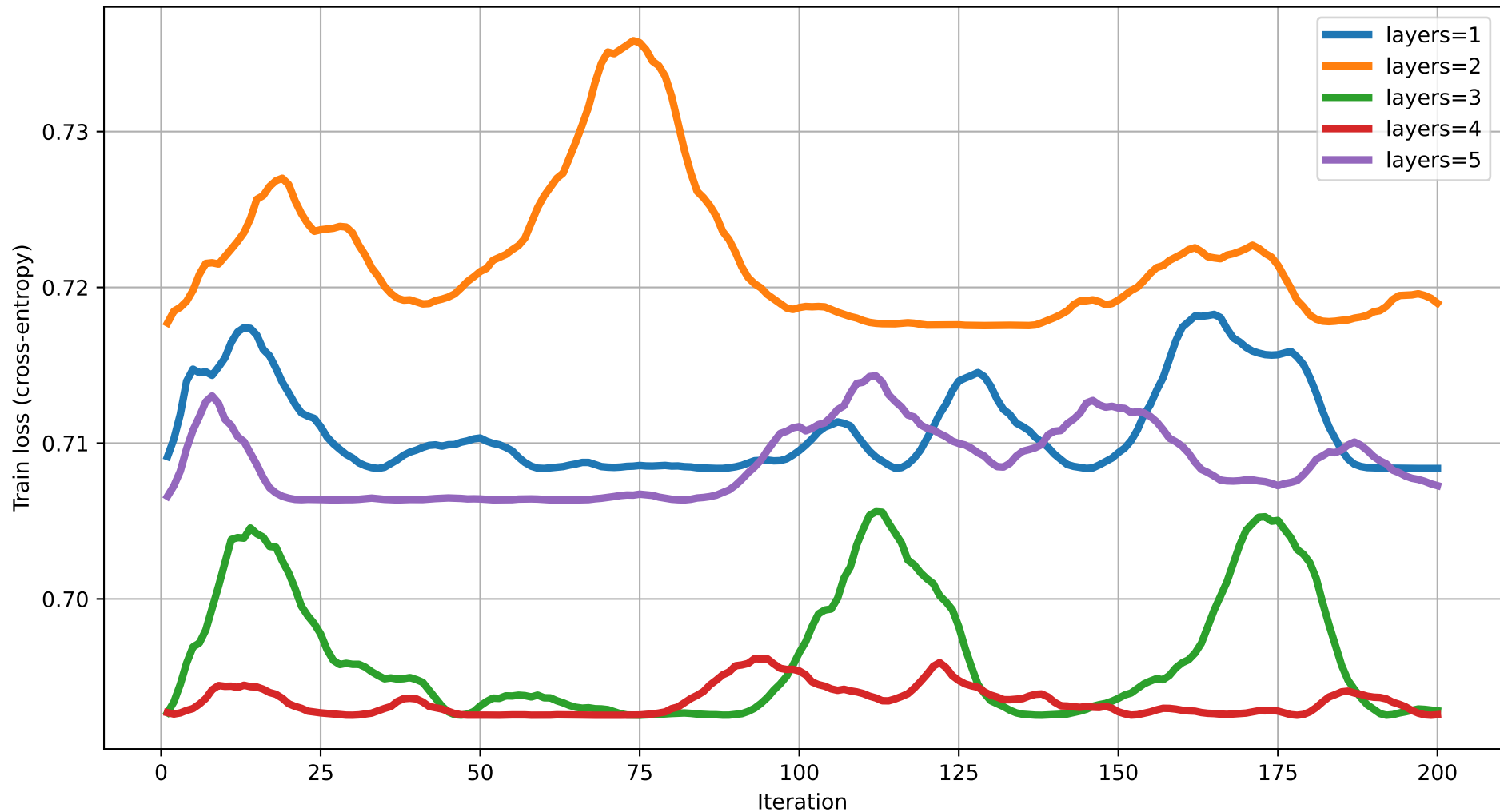
Train loss vs Iteration (dim=8) rot=RZ, ent=ring, gate=CNOT
