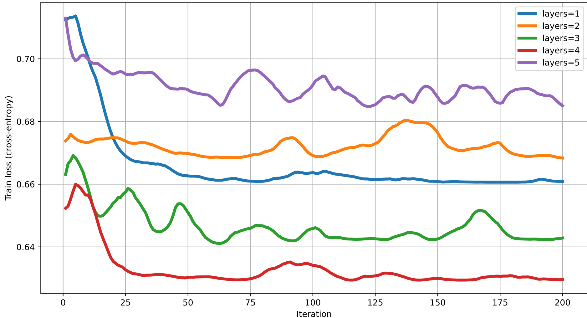
Train loss vs Iteration (degree=5) rot=RX, ent=ring, gate=CNOT
