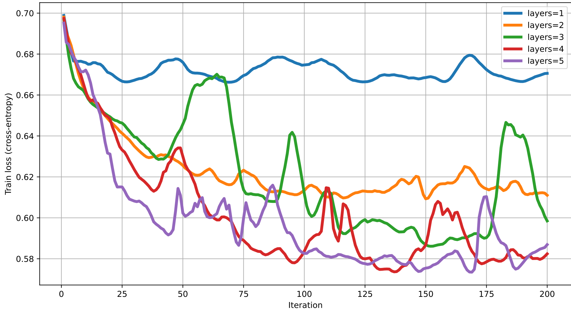
Train loss vs Iteration (dim=10) rot=Rot, ent=full, gate=CZ
