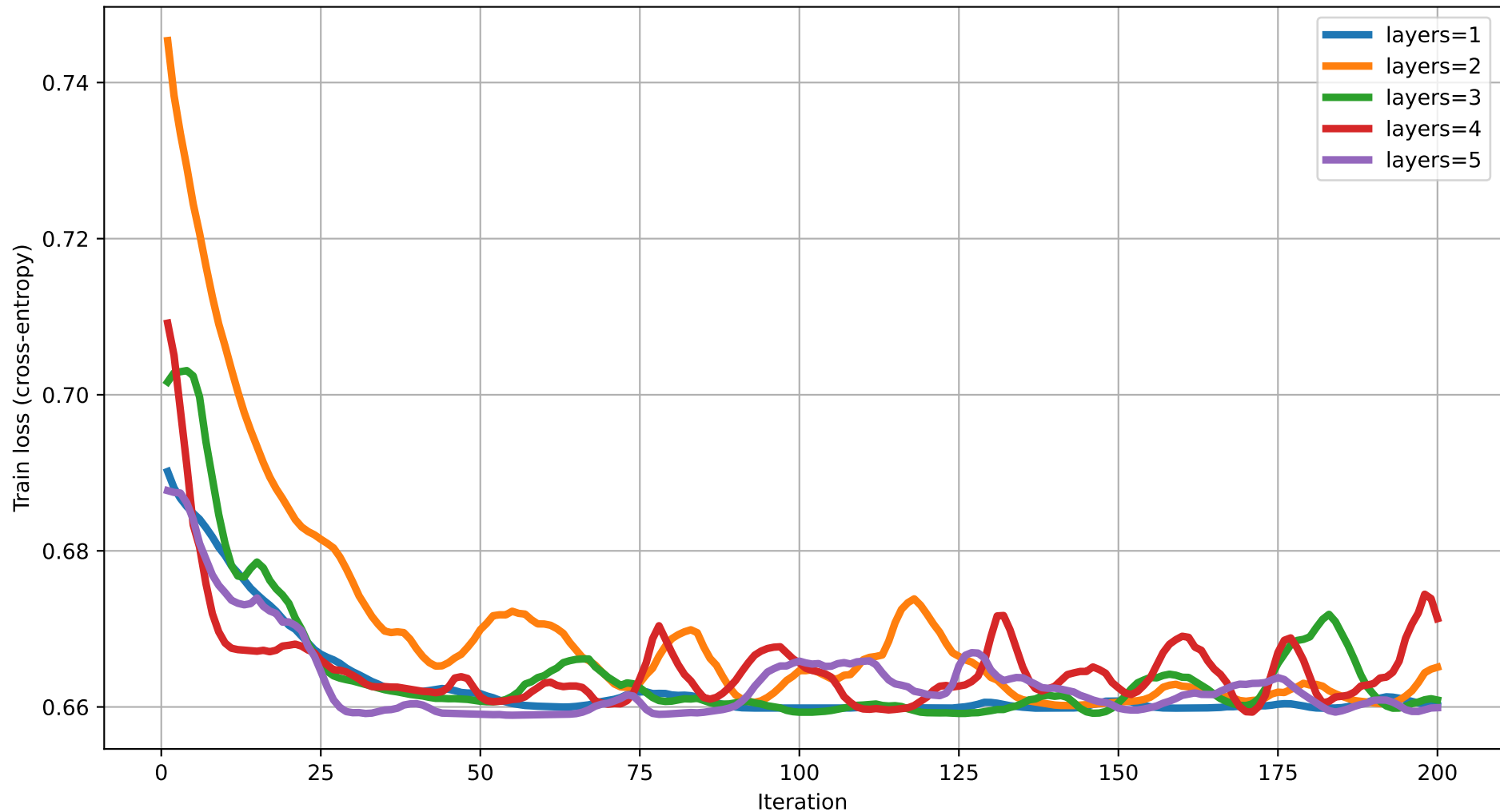
Train loss vs Iteration (degree=3) rot=RZ, ent=pairwise, gate=IsingXX
