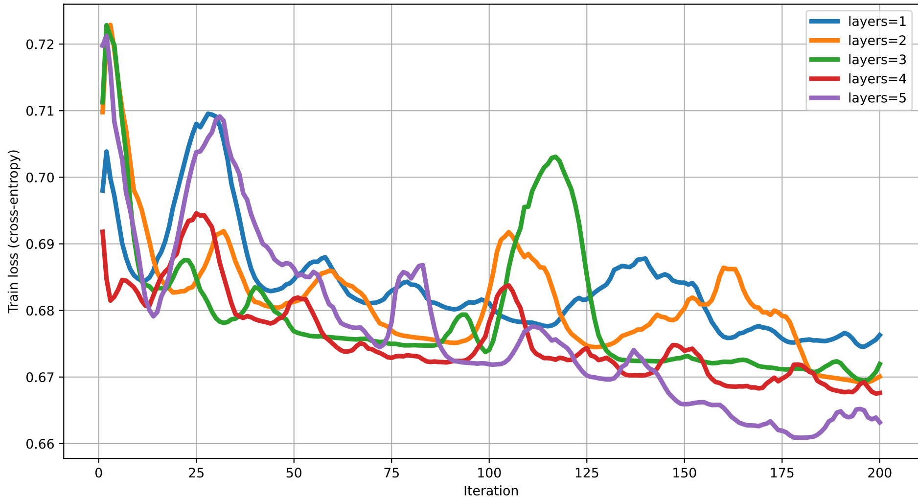
Train loss vs Iteration (dim=13) rot=RYZ, ent=chain, gate=CZ
