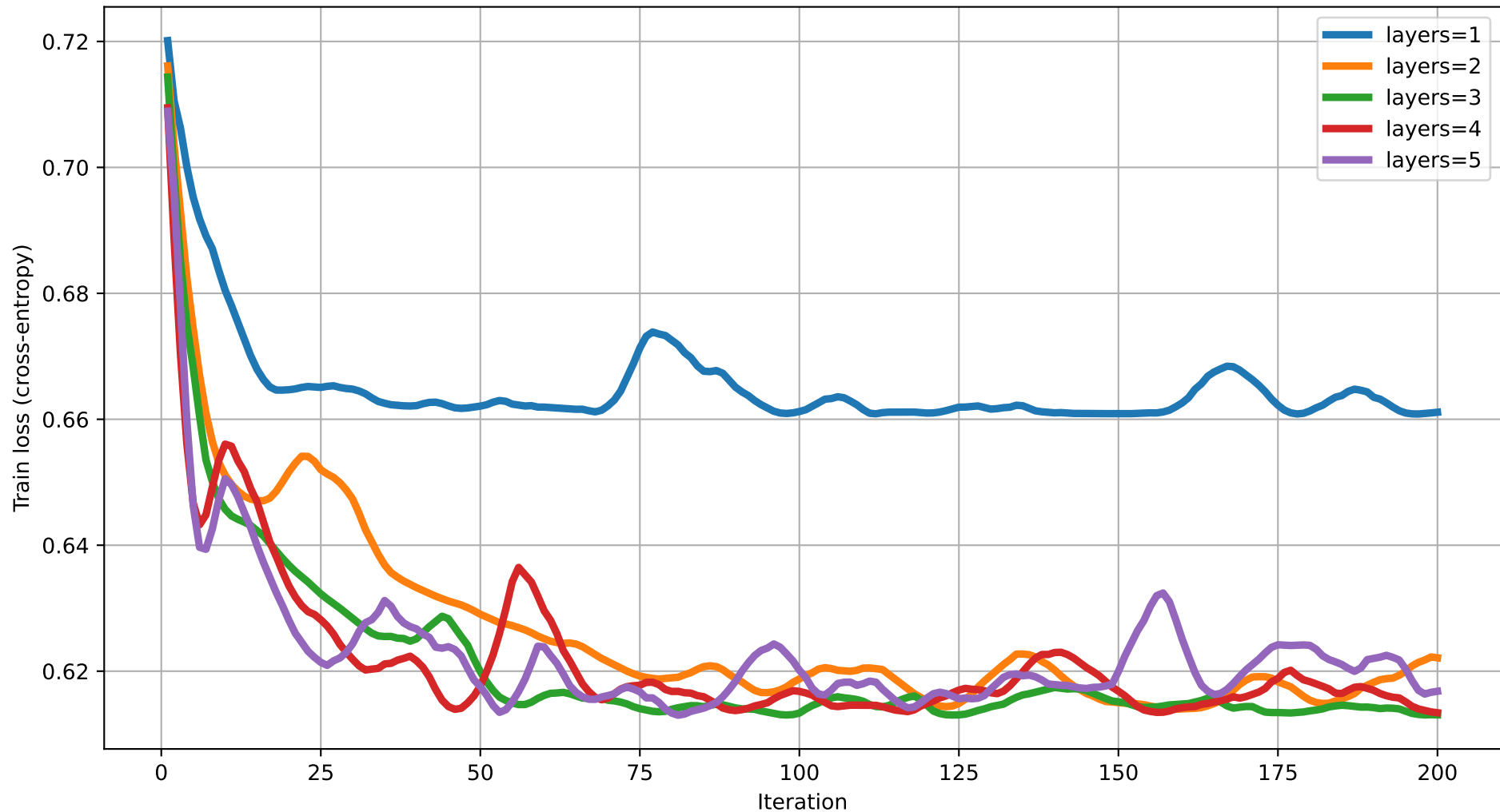
Train loss vs Iteration (degree=3) rot=RY, ent=pairwise, gate=CNOT
