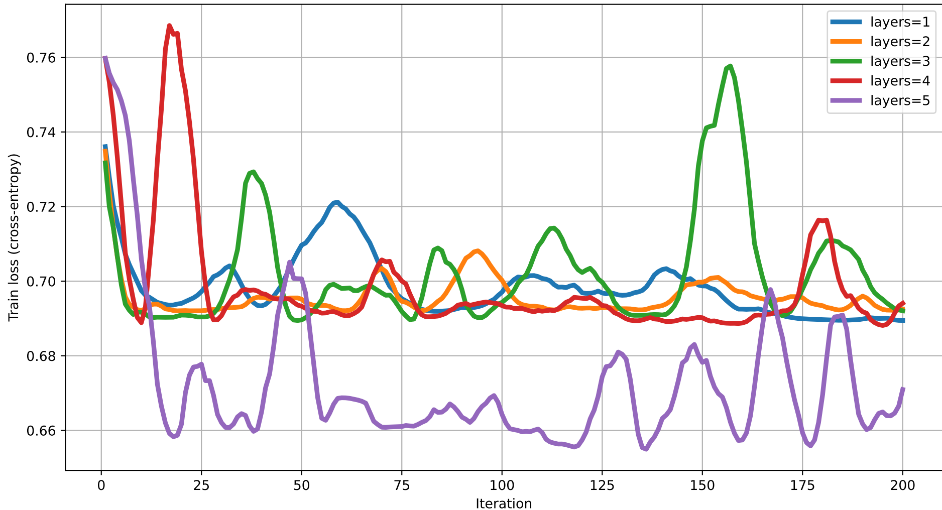
Train loss vs Iteration (dim=16) rot=RYZ, ent=chain, gate=CNOT
