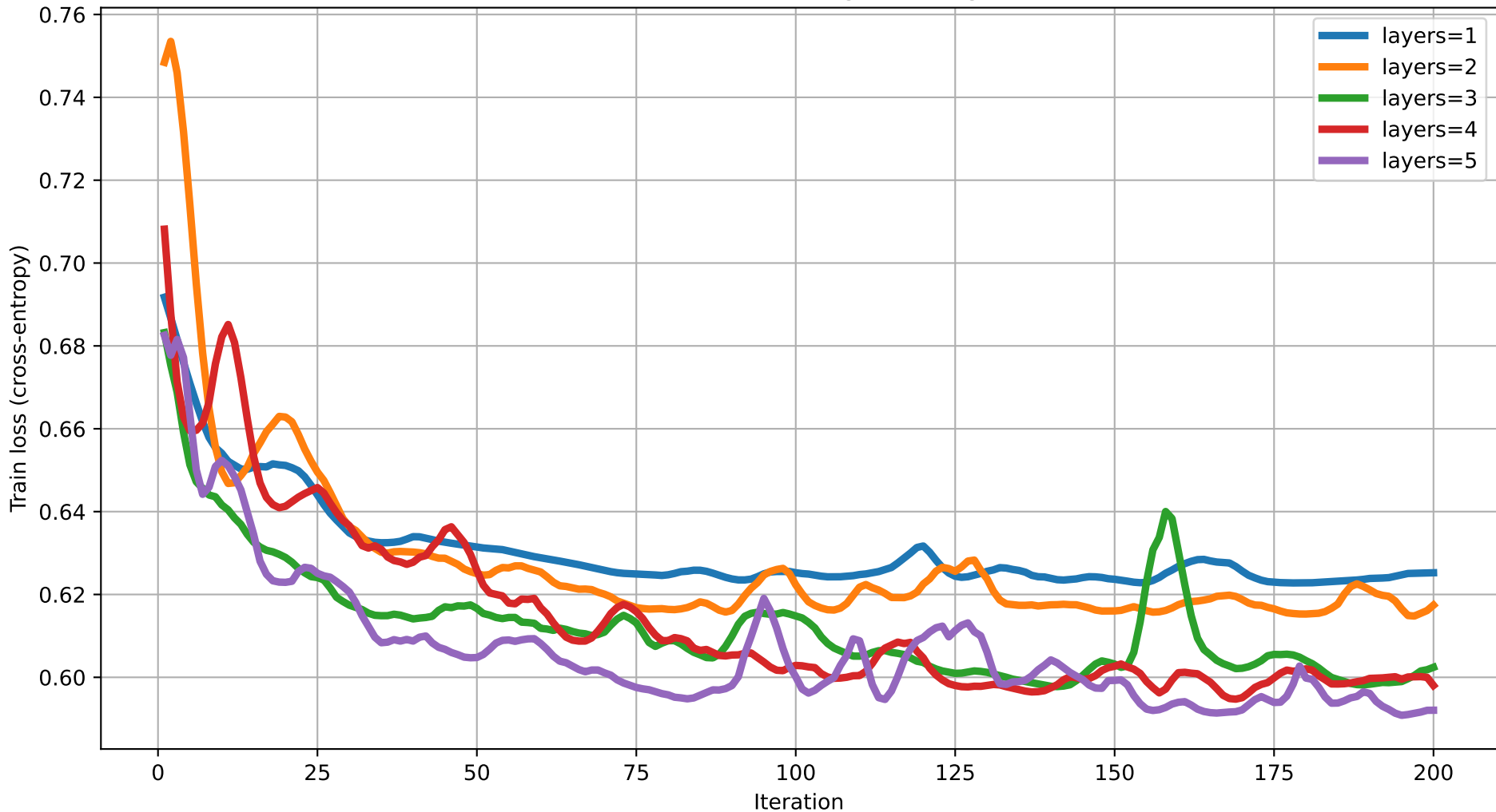
Train loss vs Iteration (degree=2) rot=RYZ, ent=full, gate=IsingXX
