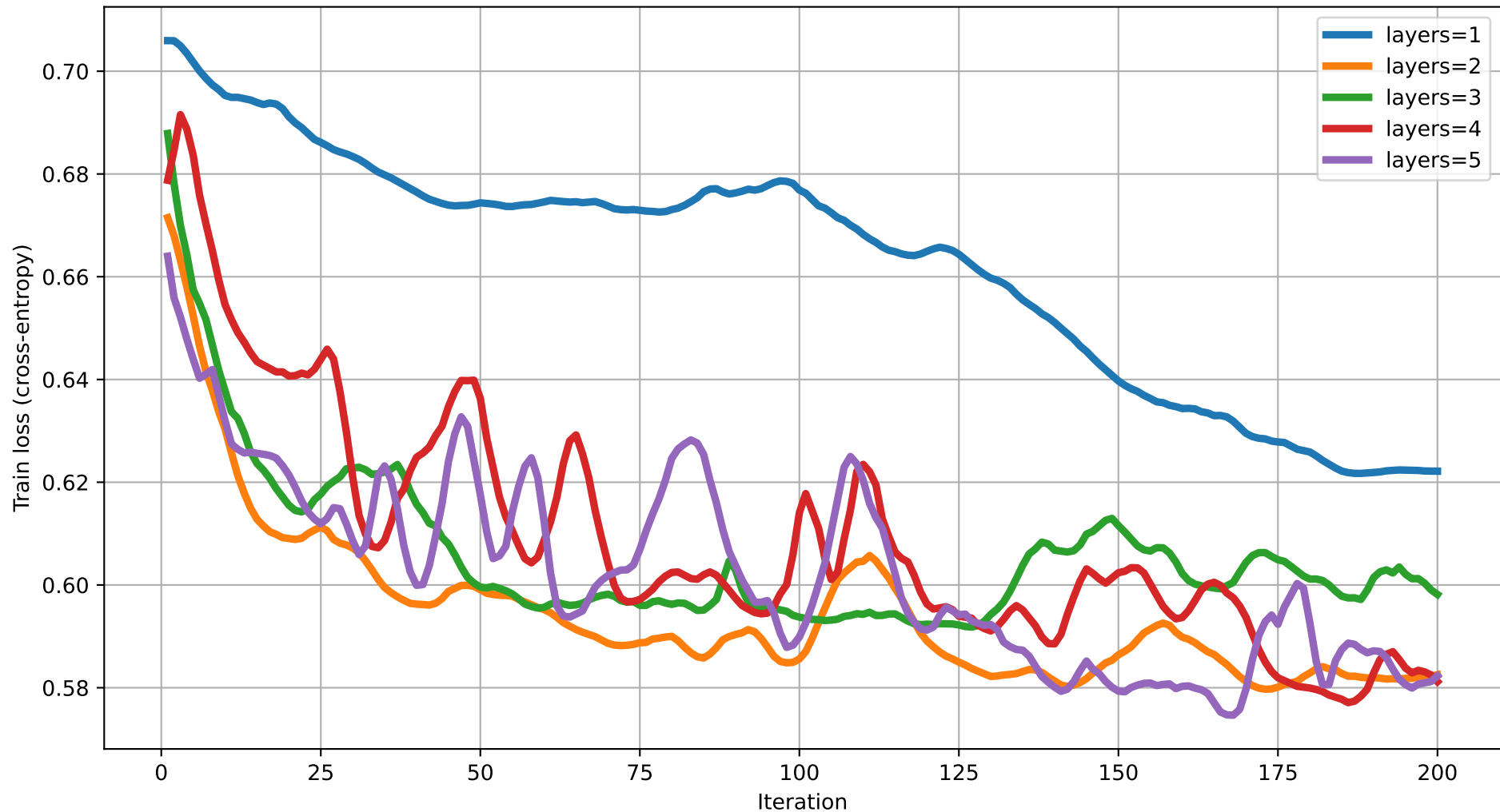
Train loss vs Iteration (dim=11) rot=Rot, ent=ring, gate=CNOT
