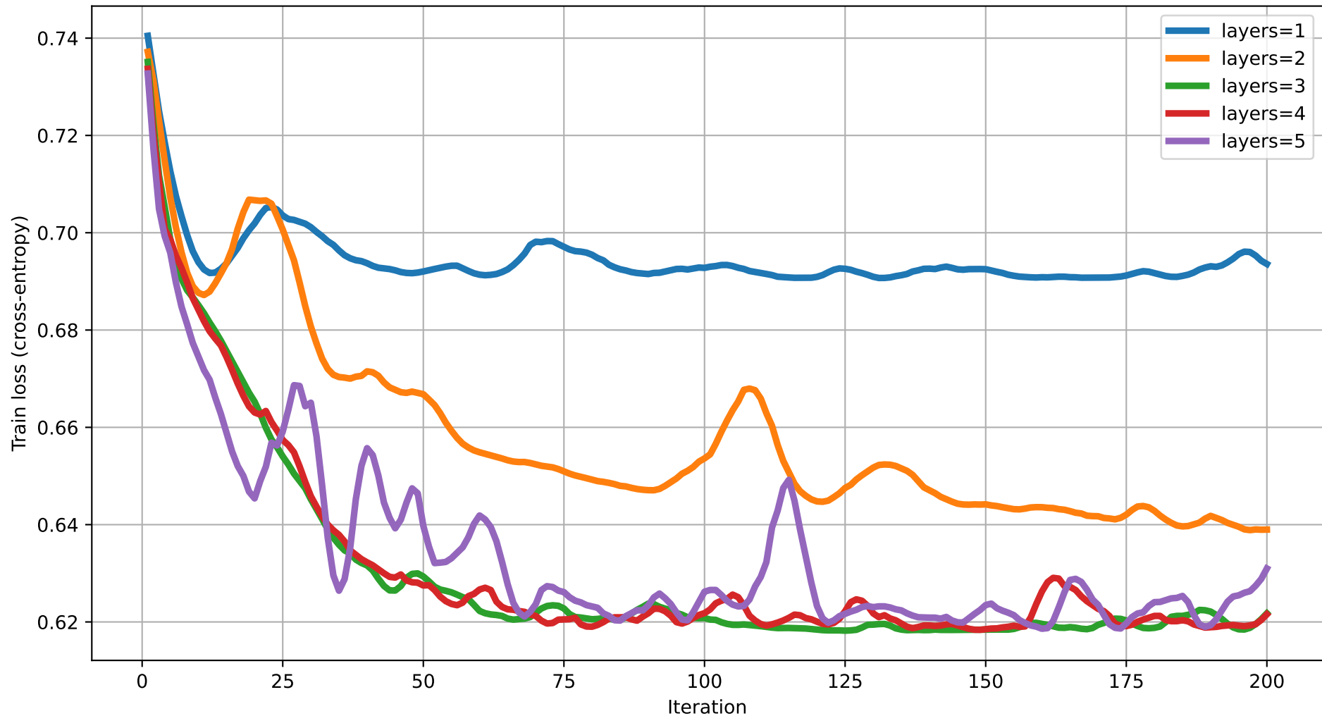
Train loss vs Iteration (degree=5) rot=Rot, ent=pairwise, gate=CZ
