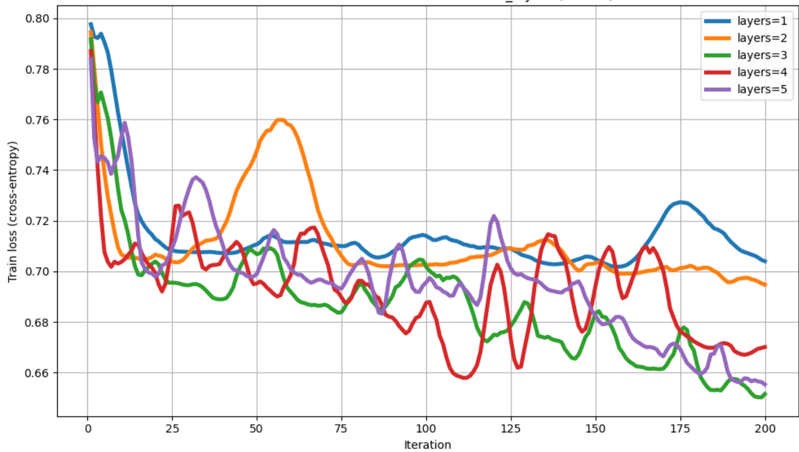
Train loss vs Iteration for different num_layers (dim=8)
