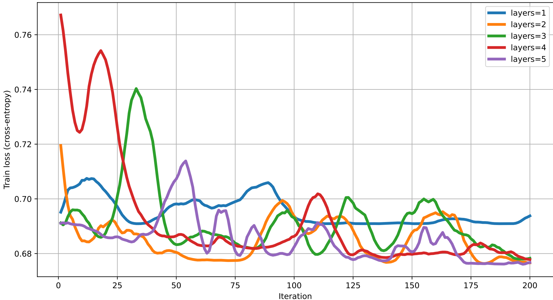
Train loss vs Iteration (dim=5) rot=RY, ent=pairwise, gate=IsingXX
