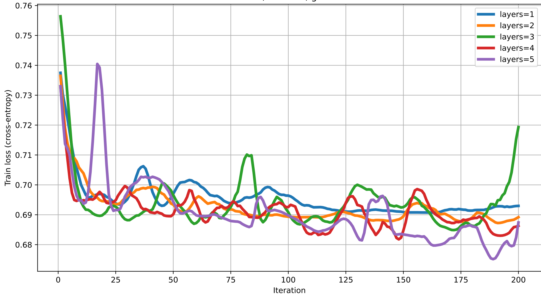
Train loss vs Iteration (dim=16) rot=Rot, ent=full, gate=CZ
