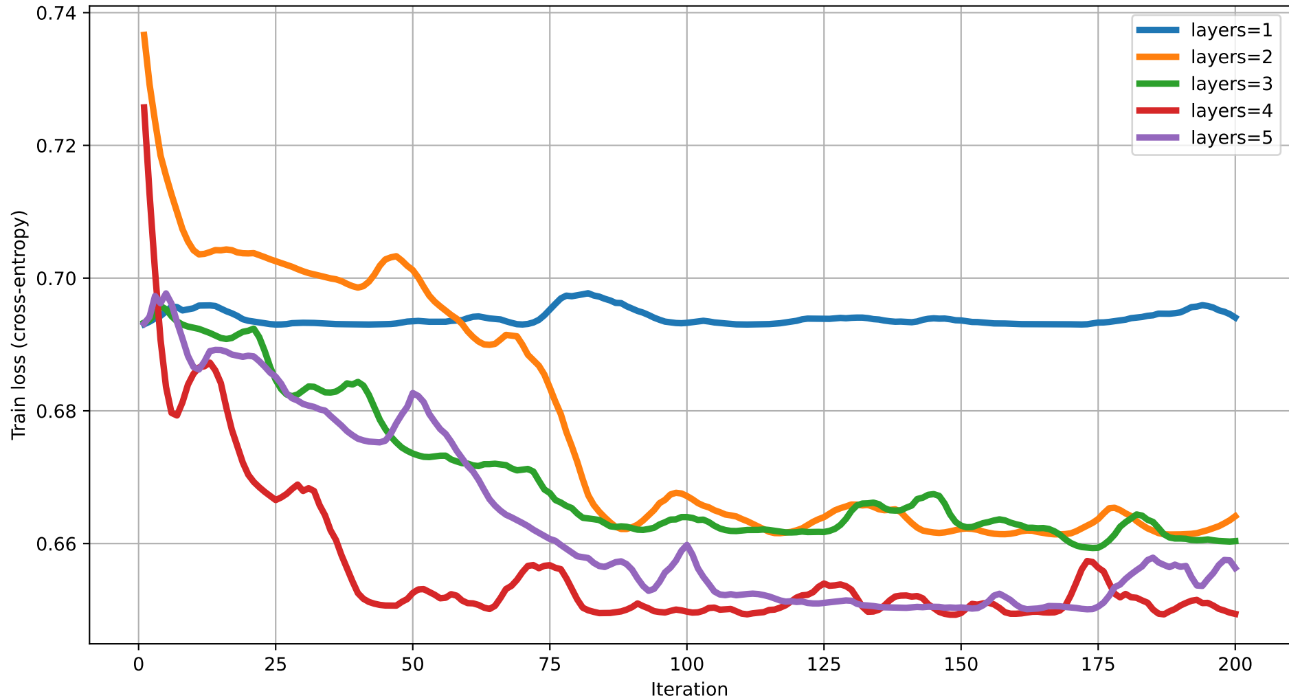
Train loss vs Iteration (degree=2) rot=RY, ent=full, gate=IsingXX
