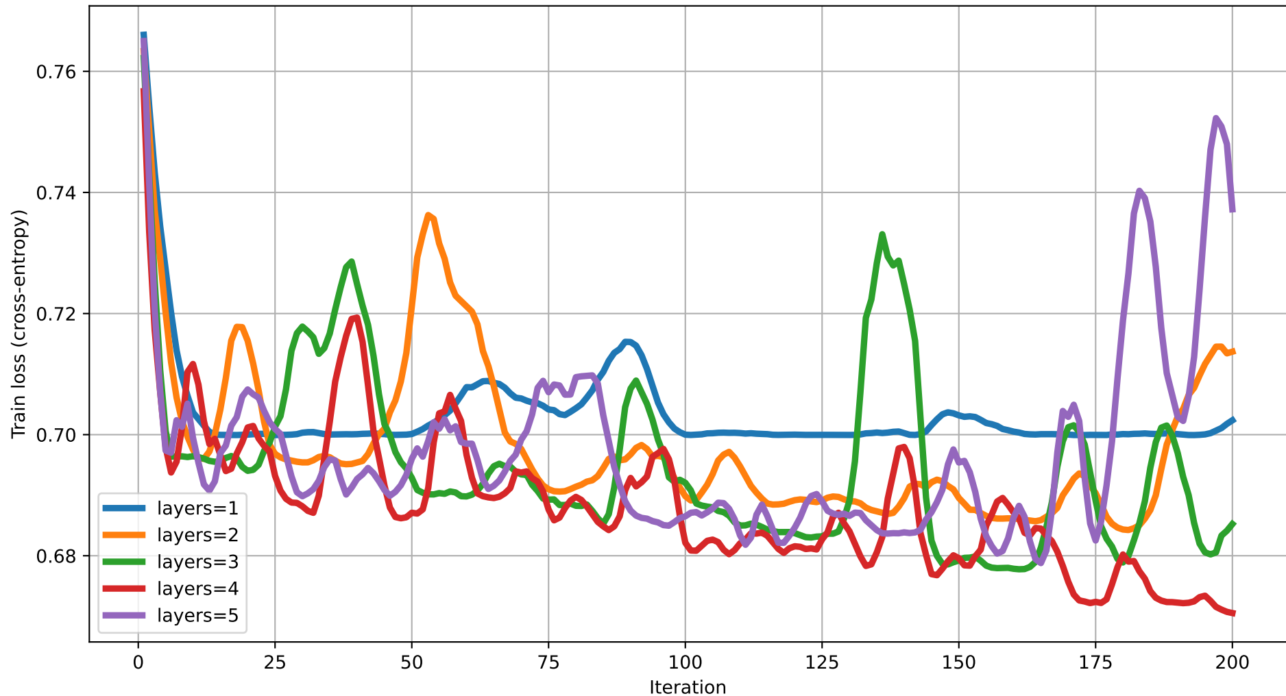
Train loss vs Iteration (dim=17) rot=Rot, ent=pairwise, gate=CNOT
