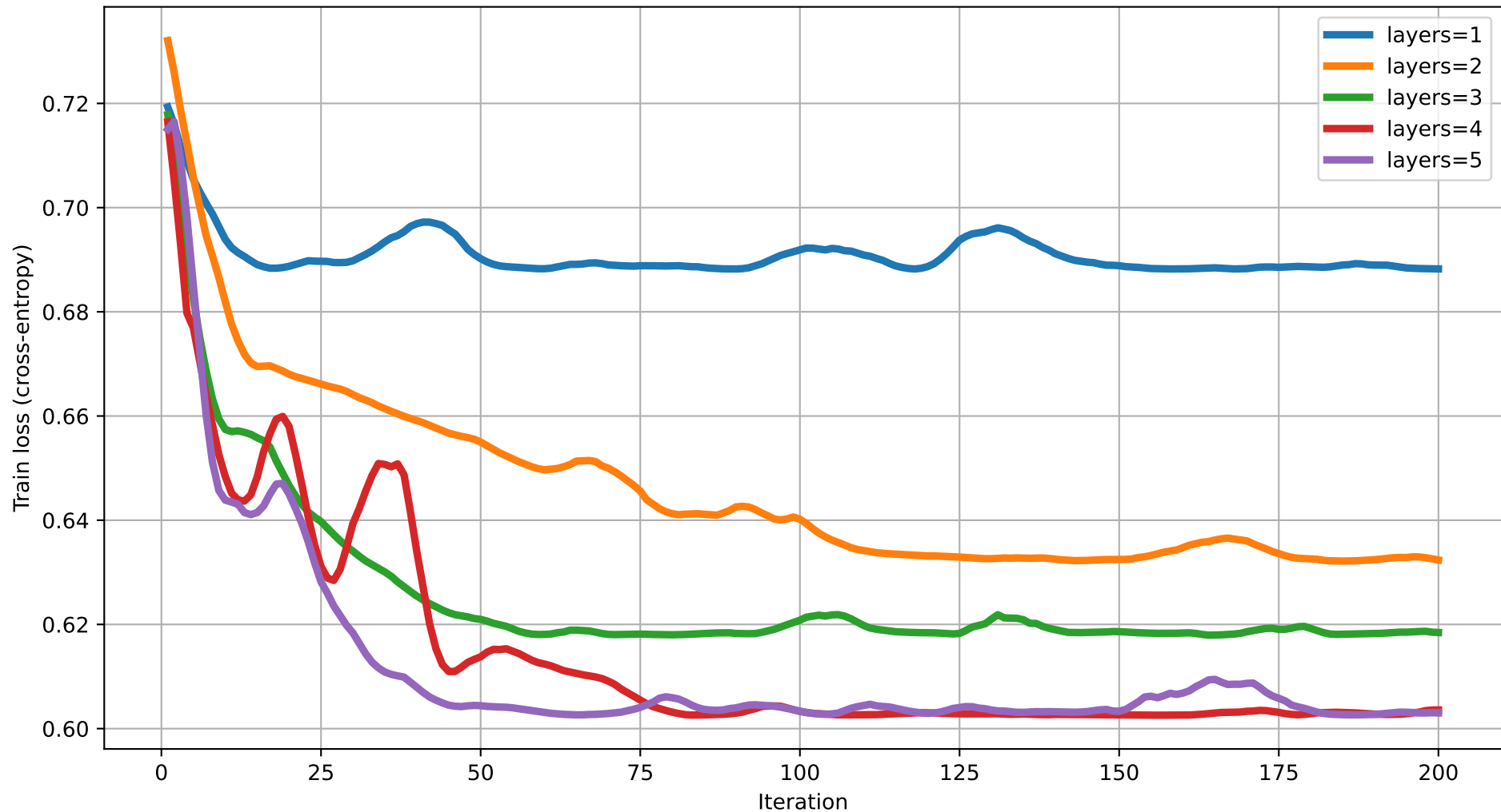
Train loss vs Iteration (degree=4) rot=RX, ent=full, gate=CNOT
