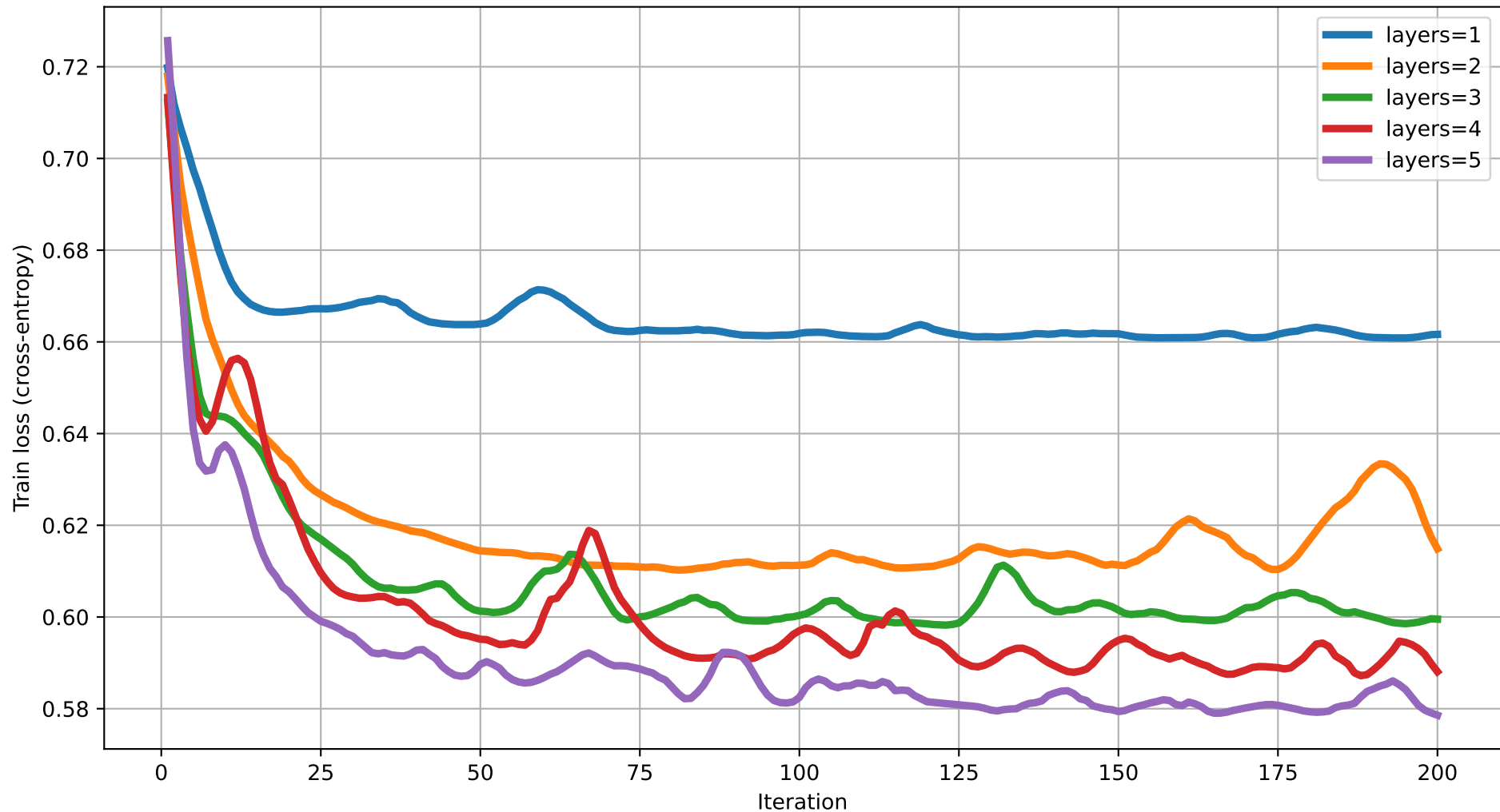
Train loss vs Iteration (degree=3) rot=RYZ, ent=full, gate=CNOT
