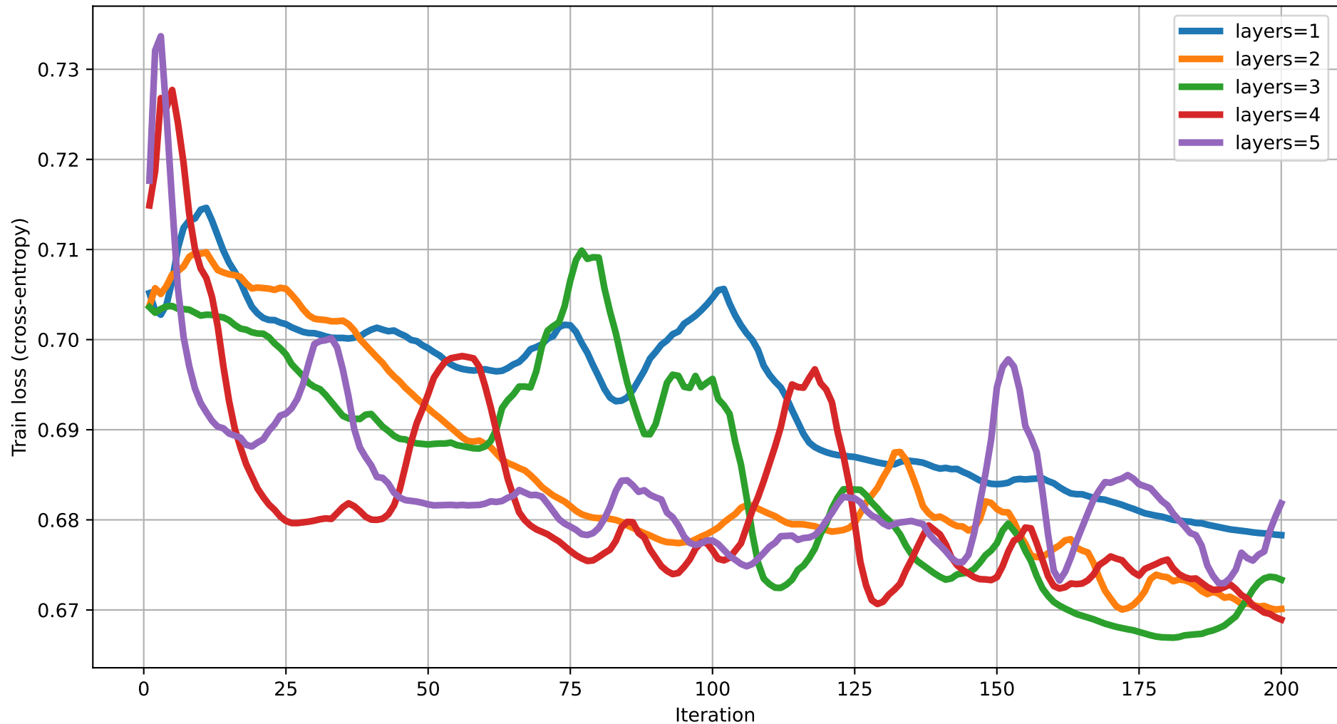
Train loss vs Iteration (dim=14) rot=RY, ent=full, gate=CZ
