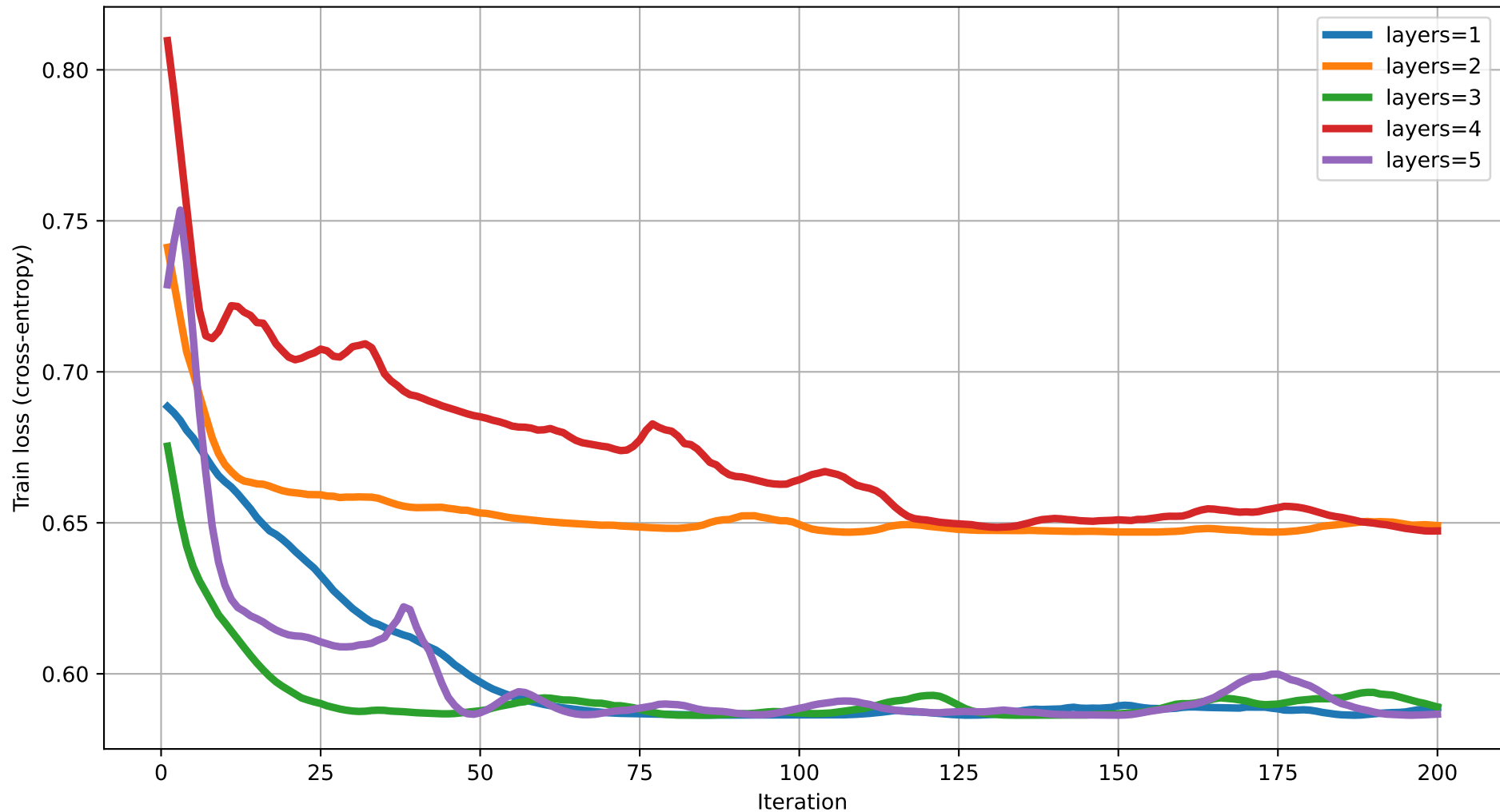
Train loss vs Iteration (dim=2) rot=RX, ent=chain, gate=IsingXX
