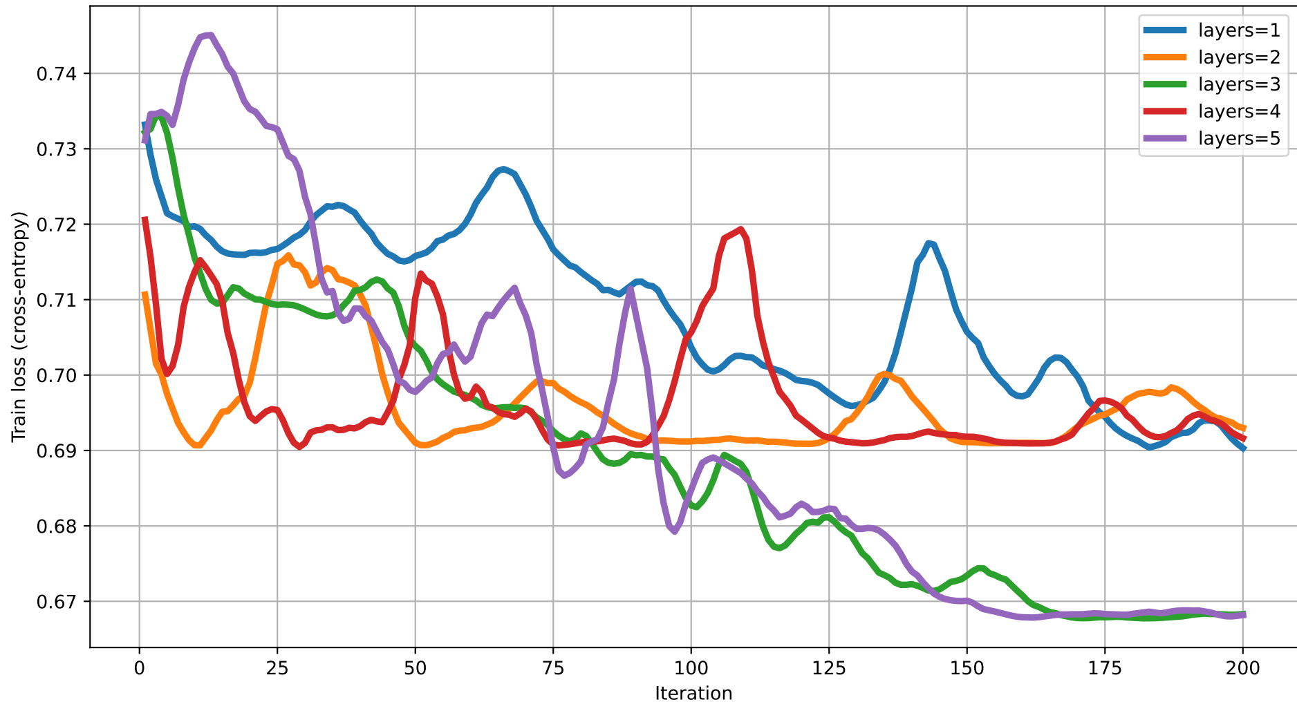
Train loss vs Iteration (dim=20) rot=RX, ent=full, gate=IsingXX
