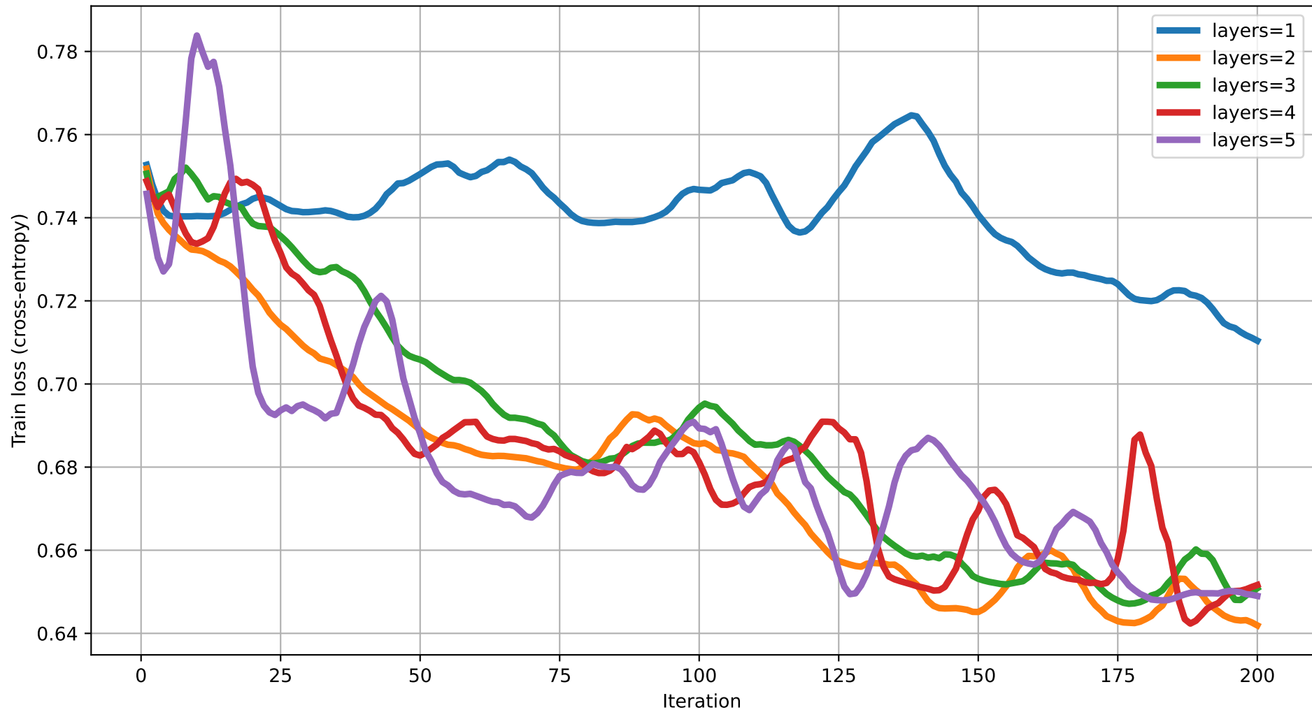
Train loss vs Iteration (dim=5) rot=RYZ, ent=full, gate=CZ
