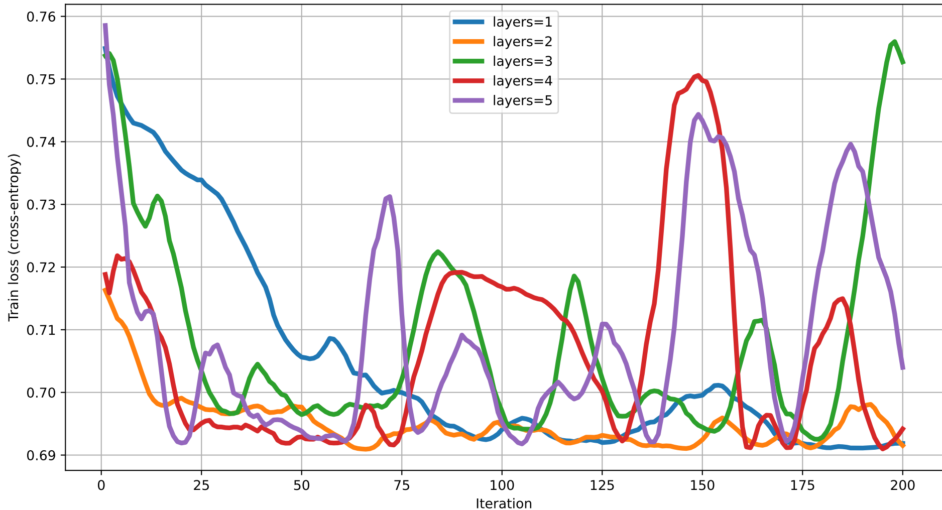
Train loss vs Iteration (dim=3) rot=RX, ent=ring, gate=IsingXX
