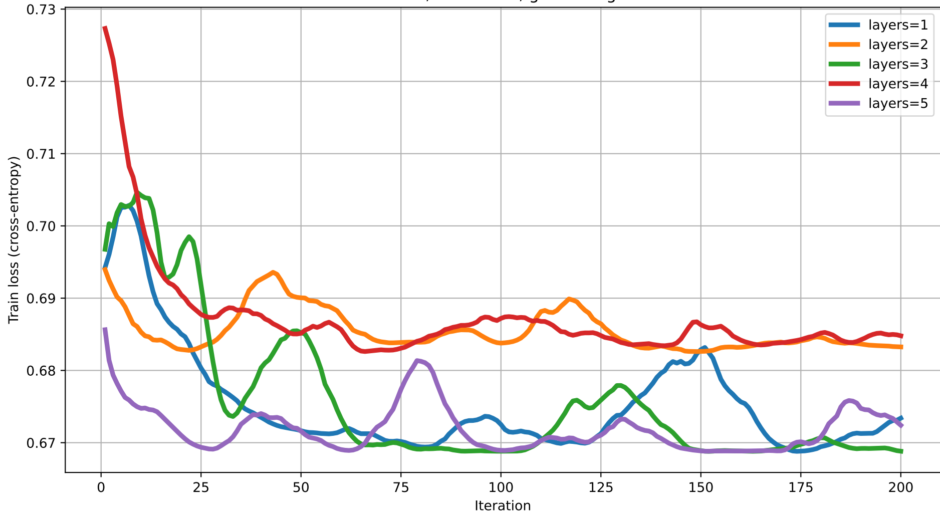
Train loss vs Iteration (dim=7) rot=RX, ent=chain, gate=IsingXX
