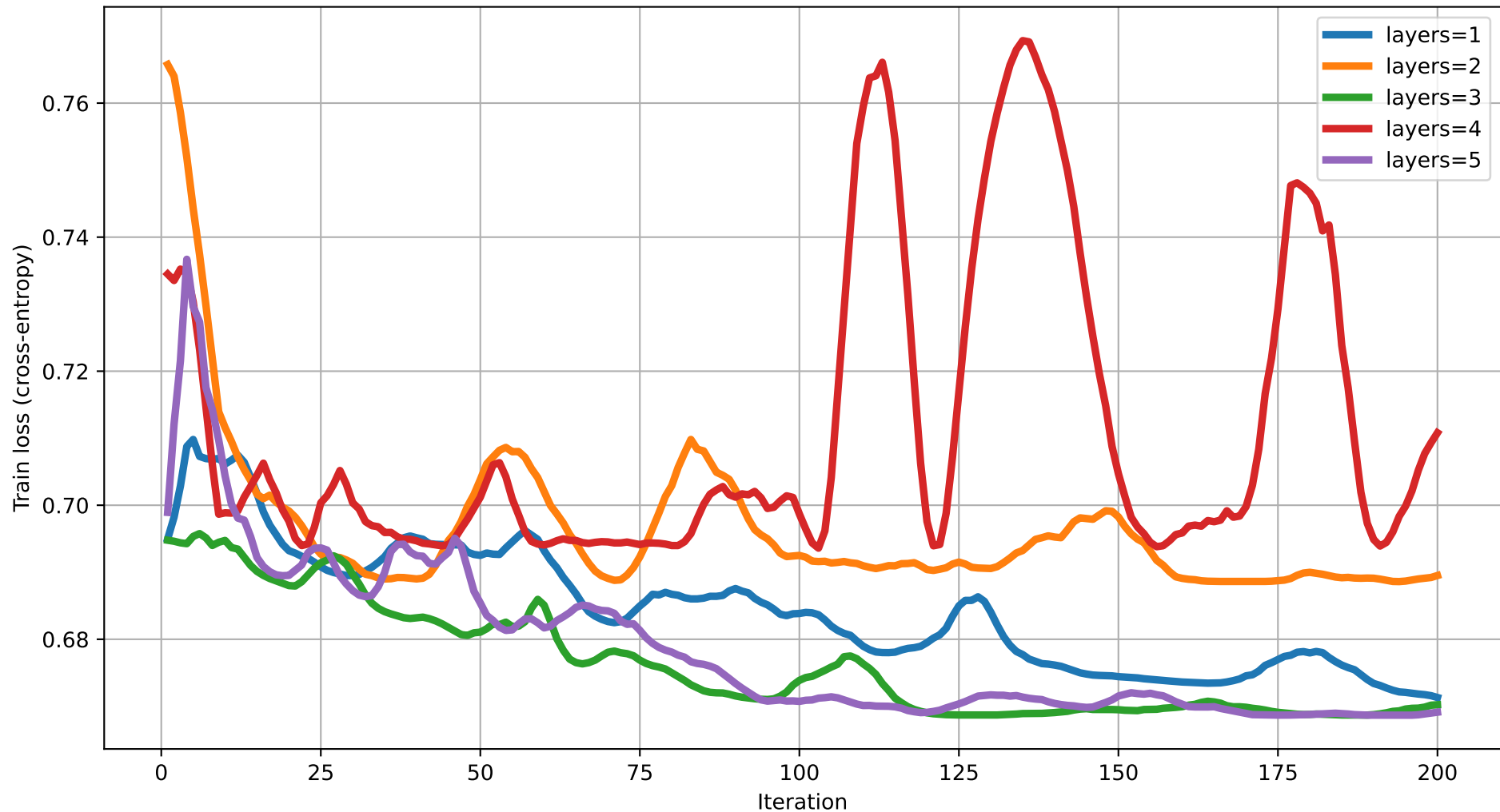
Train loss vs Iteration (dim=18) rot=RX, ent=pairwise, gate=IsingXX
