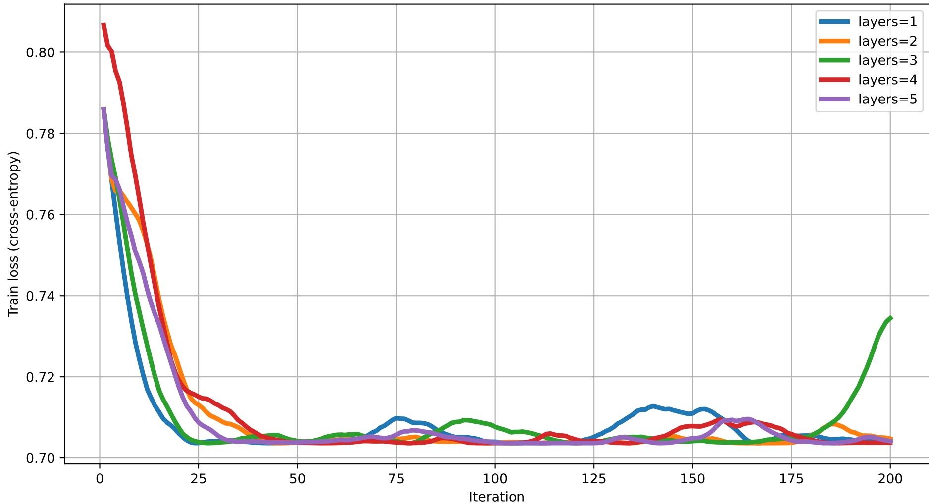
Train loss vs Iteration (dim=9) rot=RZ, ent=full, gate=CZ
