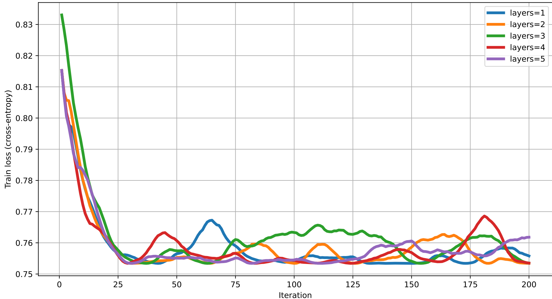
Train loss vs Iteration (dim=2) rot=RZ, ent=chain, gate=CNOT
