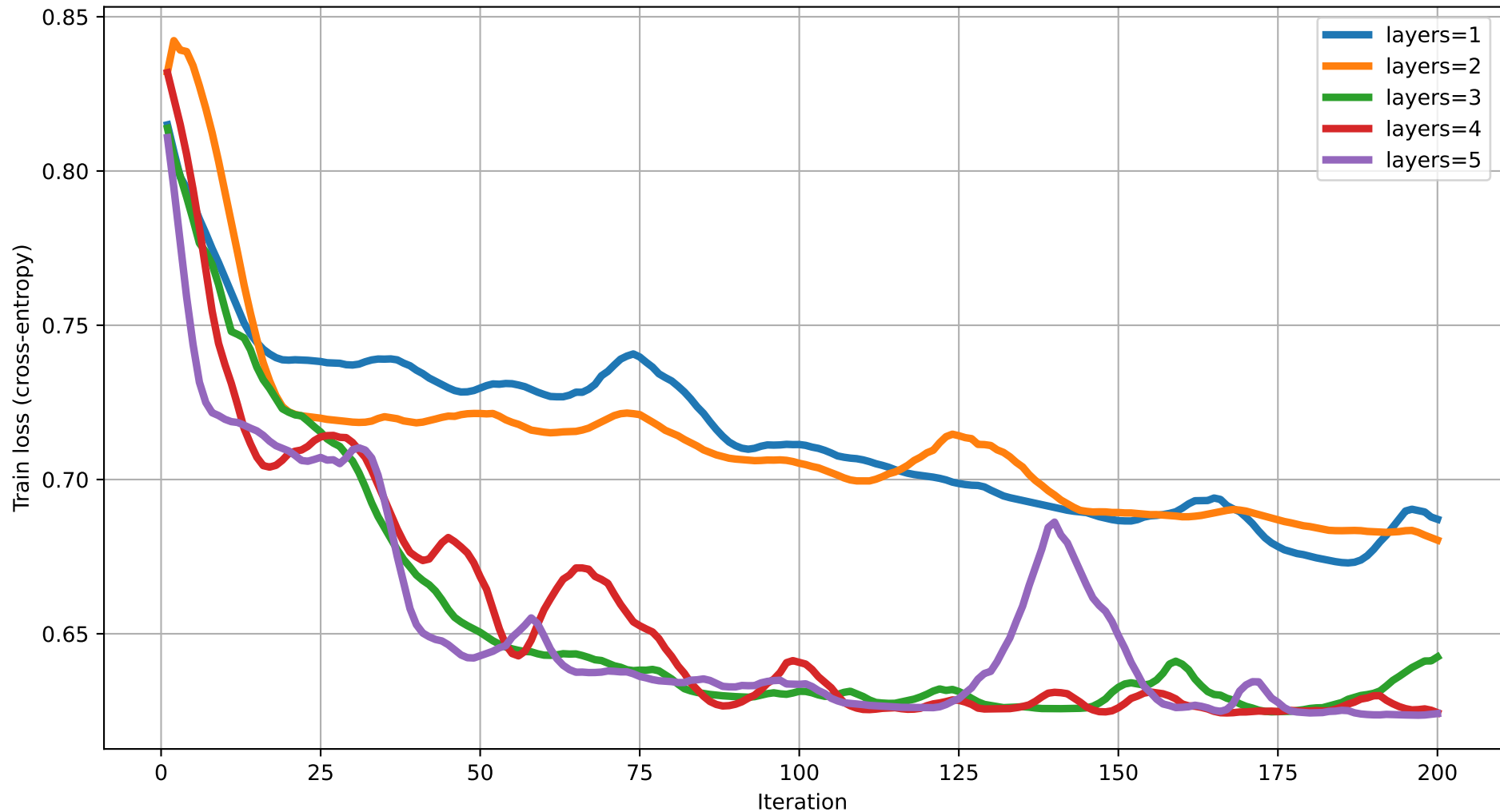
Train loss vs Iteration (dim=2) rot=RX, ent=pairwise, gate=CZ
