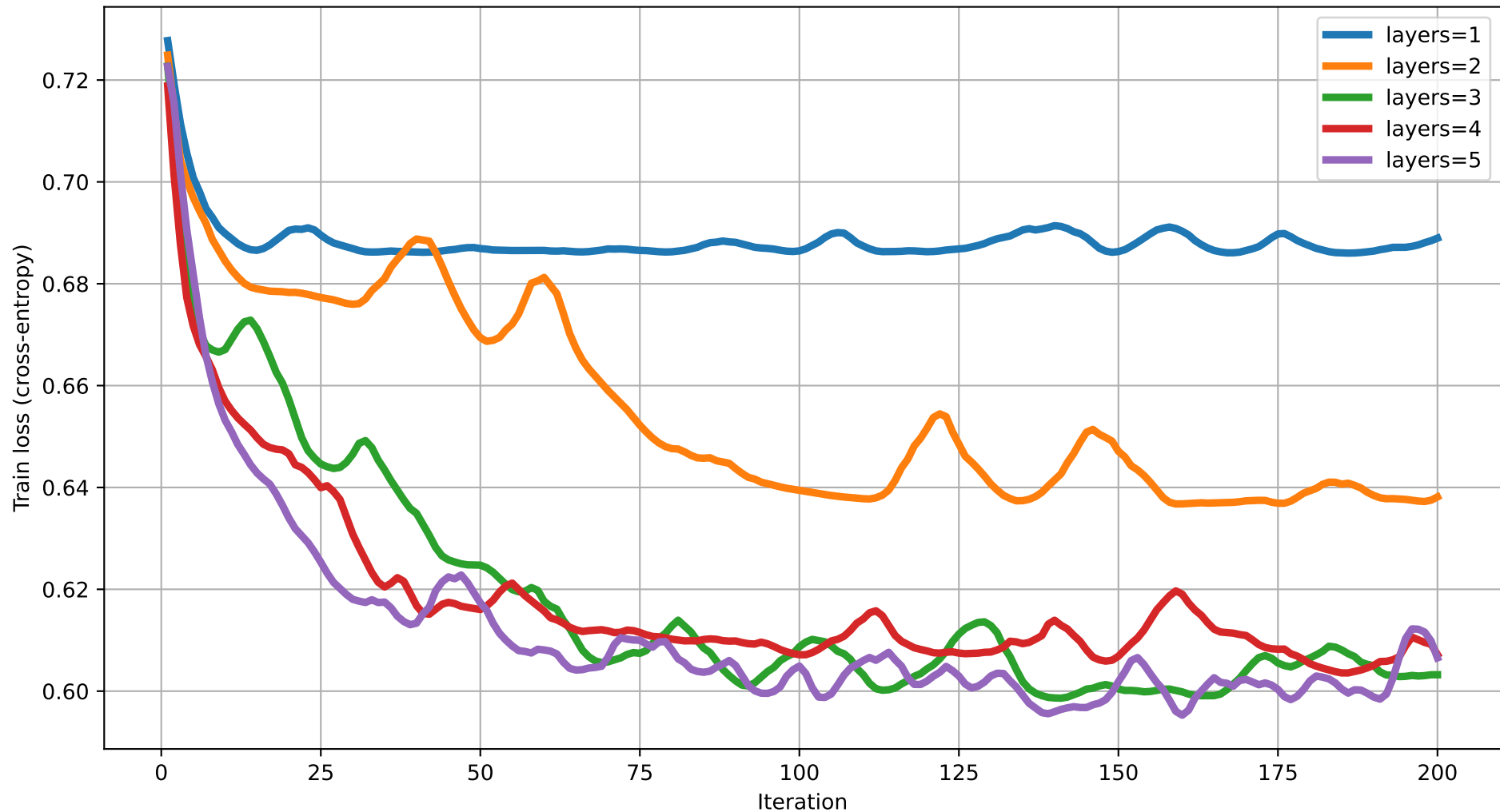
Train loss vs Iteration (degree=2) rot=RYZ, ent=full, gate=CNOT
