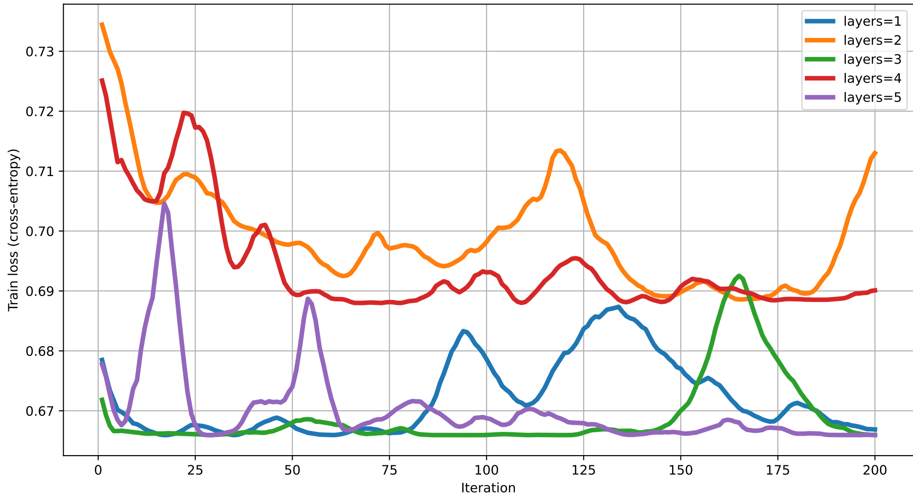
Train loss vs Iteration (dim=6) rot=RX, ent=full, gate=IsingXX
