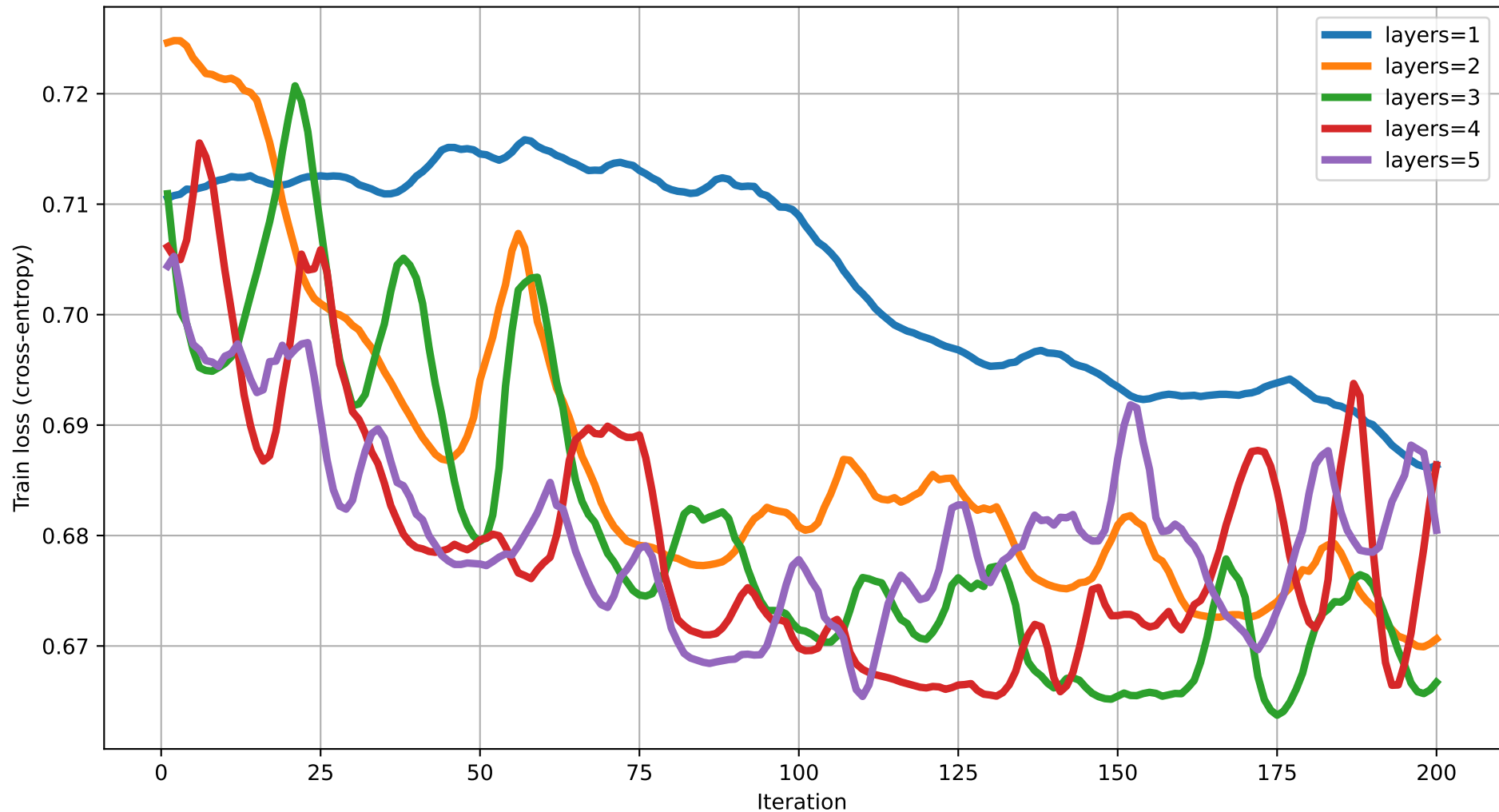
Train loss vs Iteration (dim=14) rot=RYZ, ent=ring, gate=CNOT
