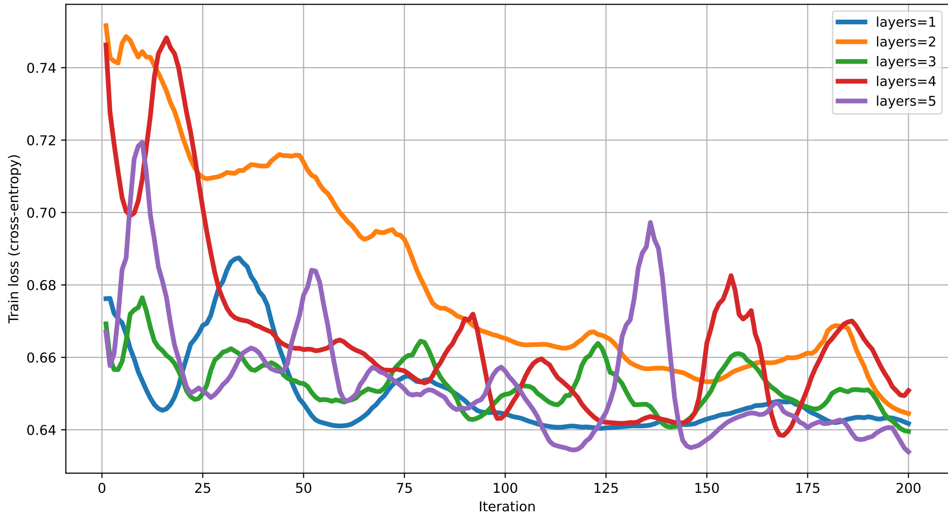
Train loss vs Iteration (dim=5) rot=RY, ent=ring, gate=IsingXX
