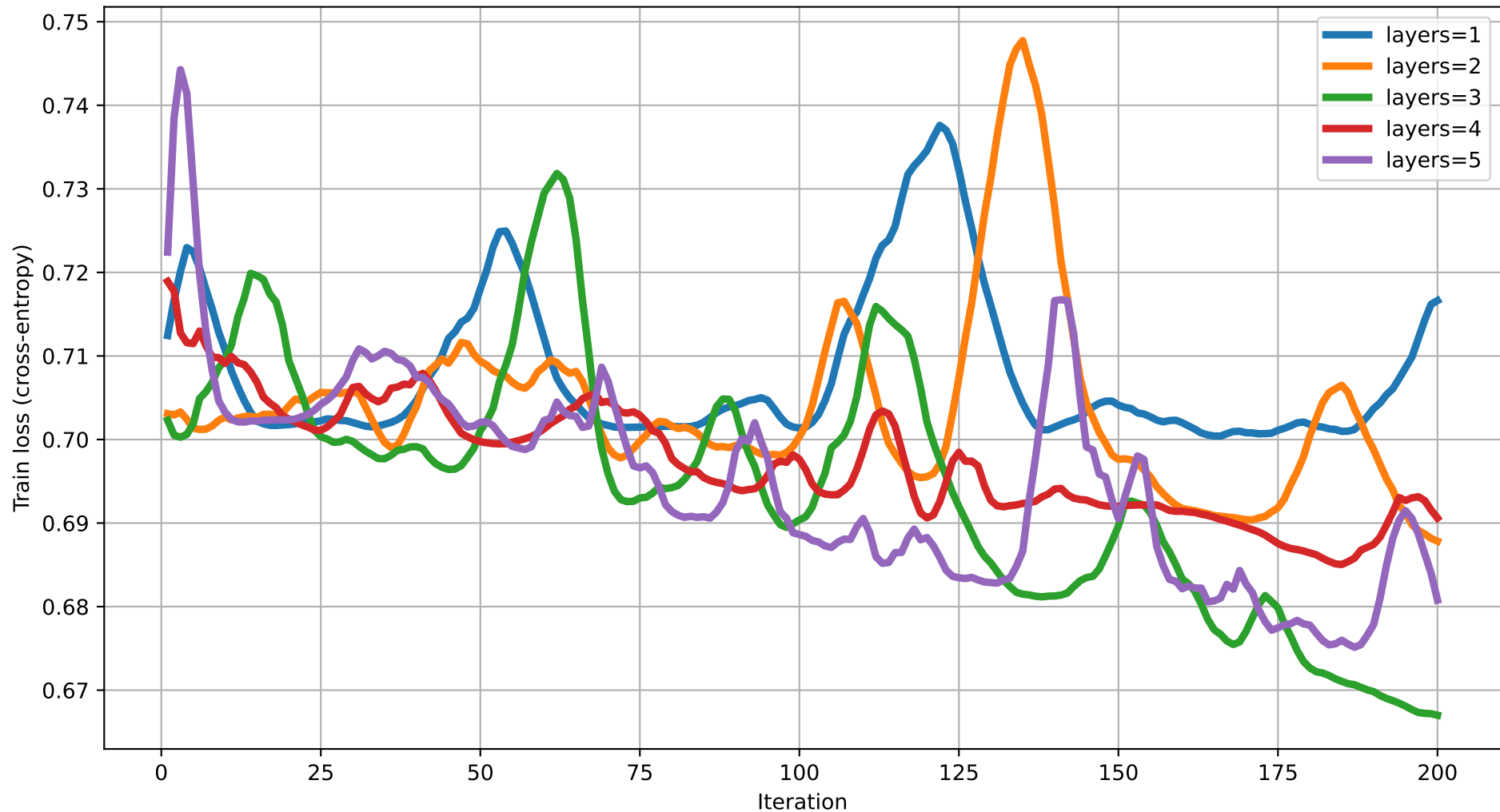
Train loss vs Iteration (dim=12) rot=RYZ, ent=pairwise, gate=CZ
