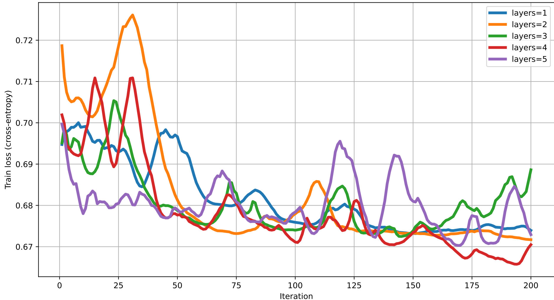
Train loss vs Iteration (dim=11) rot=RYZ, ent=pairwise, gate=IsingXX
