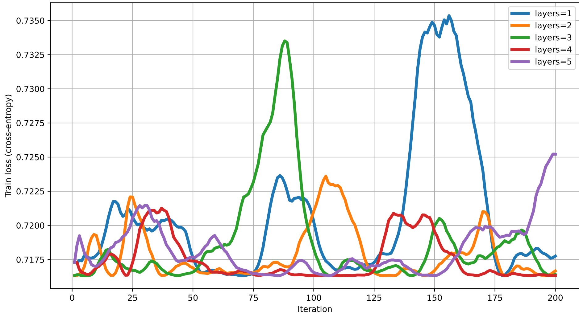
Train loss vs Iteration (dim=7) rot=RZ, ent=ring, gate=CZ
