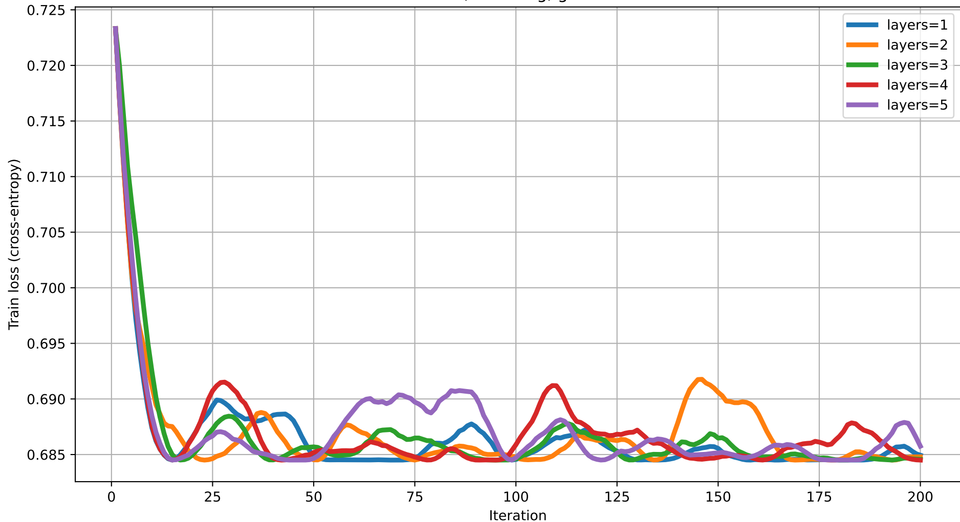
Train loss vs Iteration (degree=3) rot=RZ, ent=ring, gate=CZ
