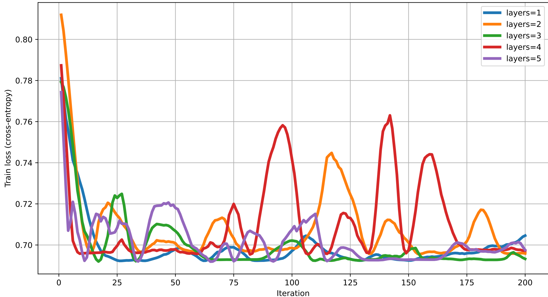
Train loss vs Iteration (dim=2) rot=RX, ent=ring, gate=IsingXX
