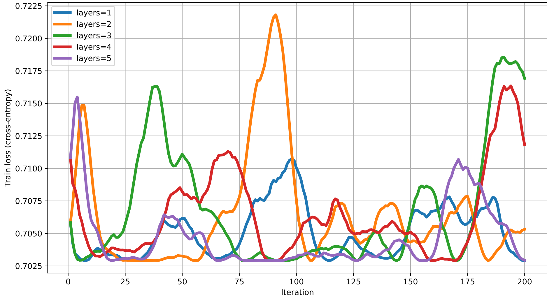
Train loss vs Iteration (dim=12) rot=RZ, ent=full, gate=CZ
