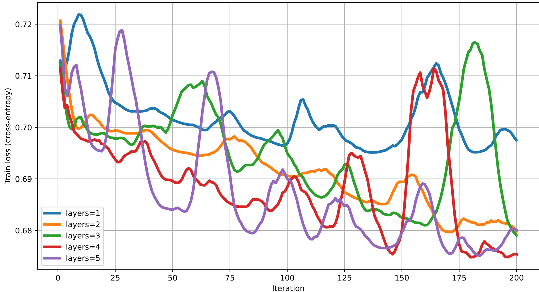
Train loss vs Iteration (dim=11) rot=RX, ent=pairwise, gate=CZ
