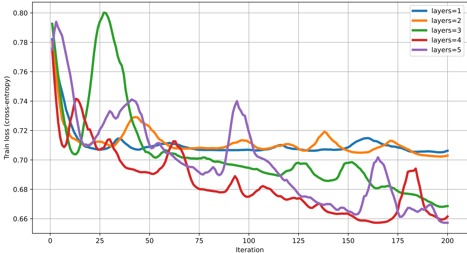
Train loss vs Iteration (dim=9) rot=RY, ent=pairwise, gate=CZ
