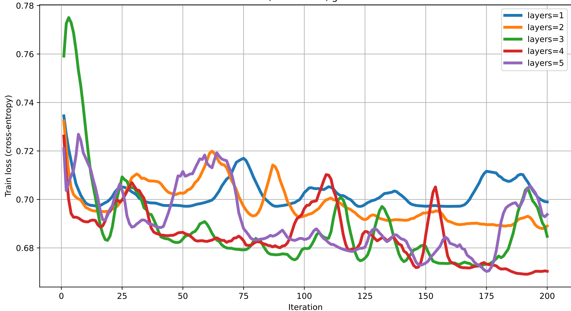
Train loss vs Iteration (dim=18) rot=RYZ, ent=chain, gate=CNOT
