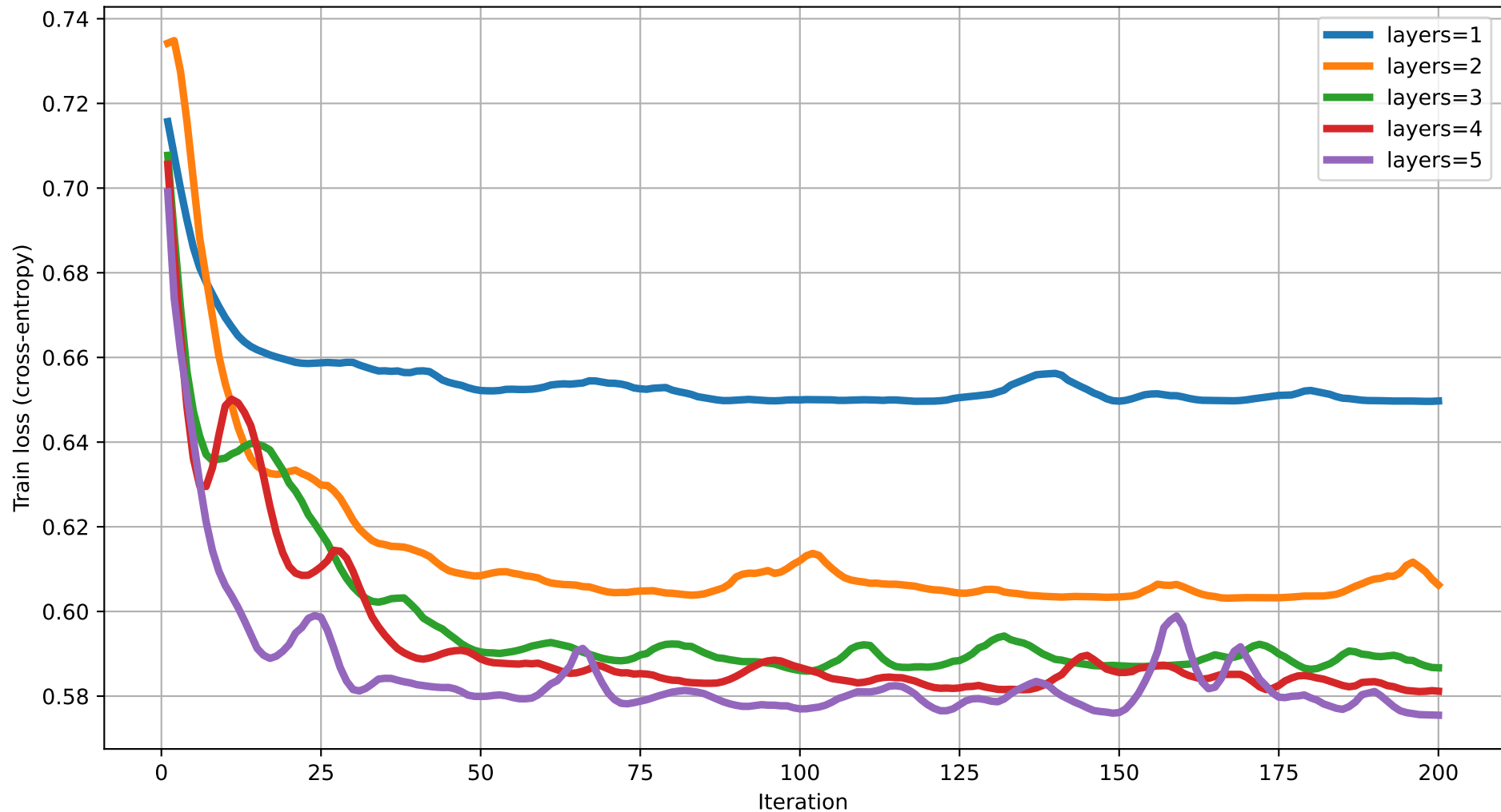
Train loss vs Iteration (degree=4) rot=RY, ent=full, gate=CNOT
