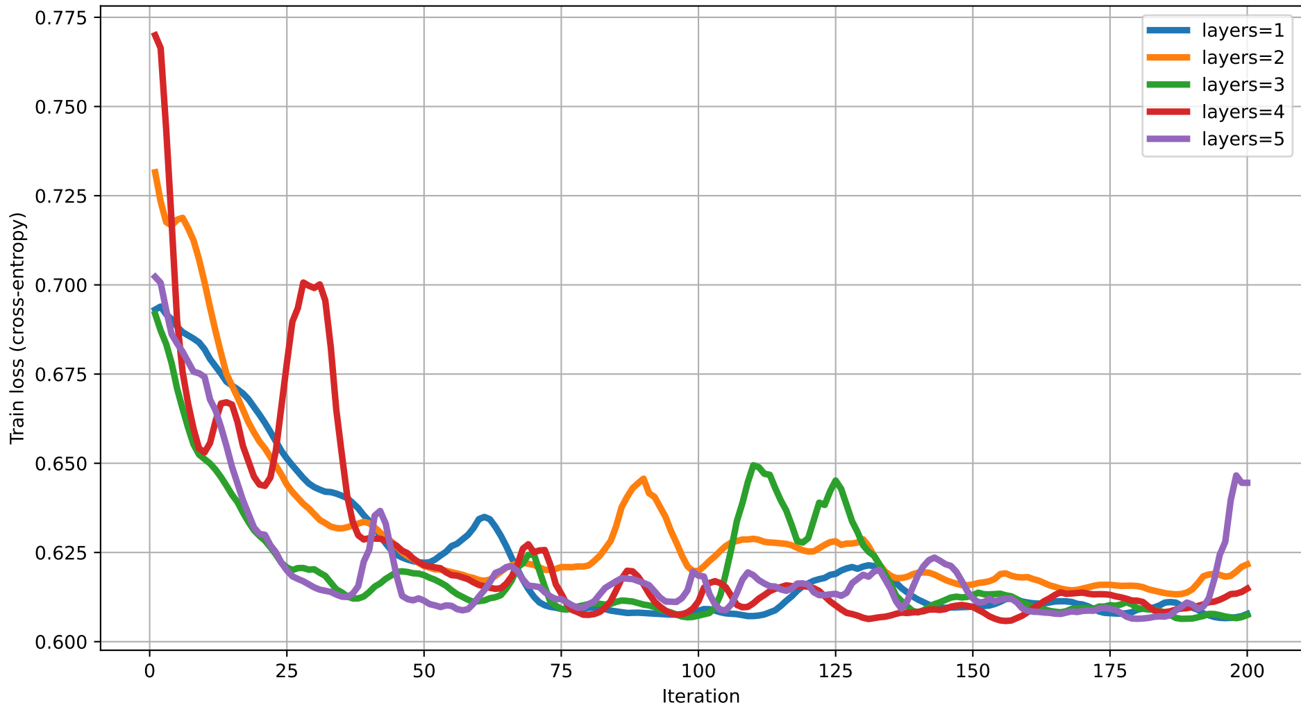
Train loss vs Iteration (dim=9) rot=Rot, ent=pairwise, gate=IsingXX
