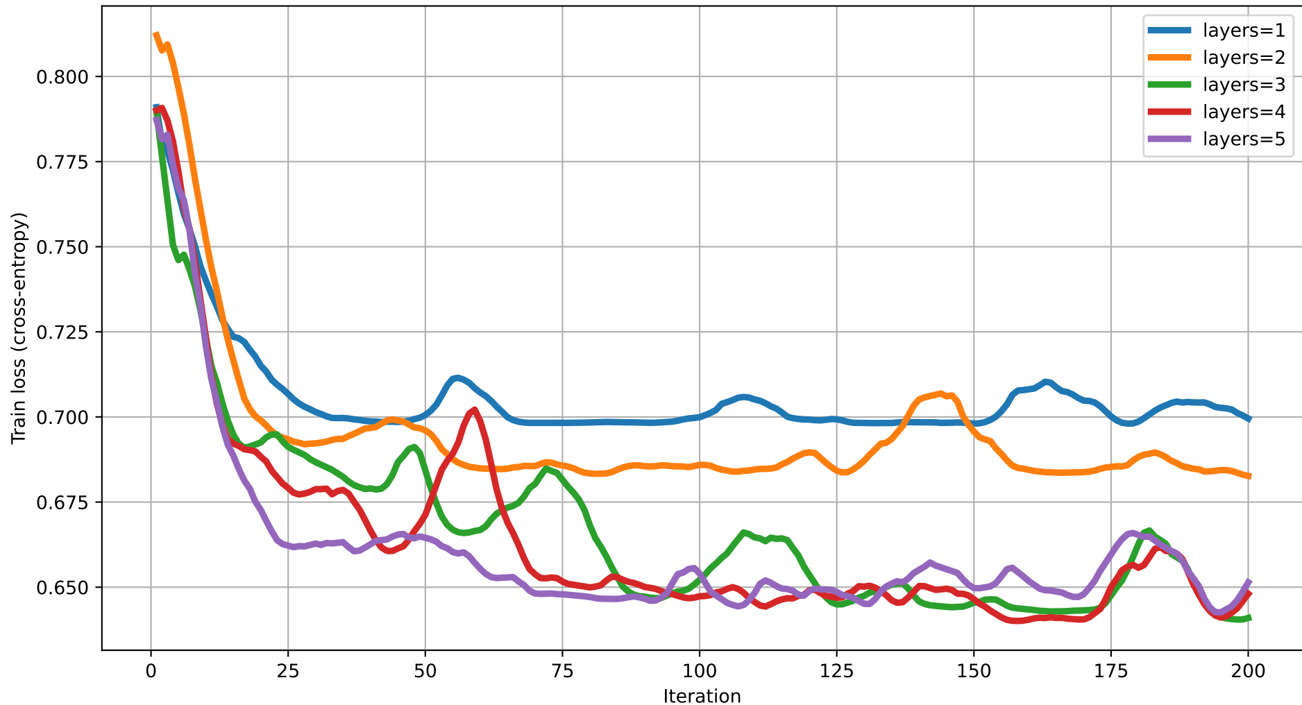
Train loss vs Iteration (dim=4) rot=RX, ent=full, gate=CZ
