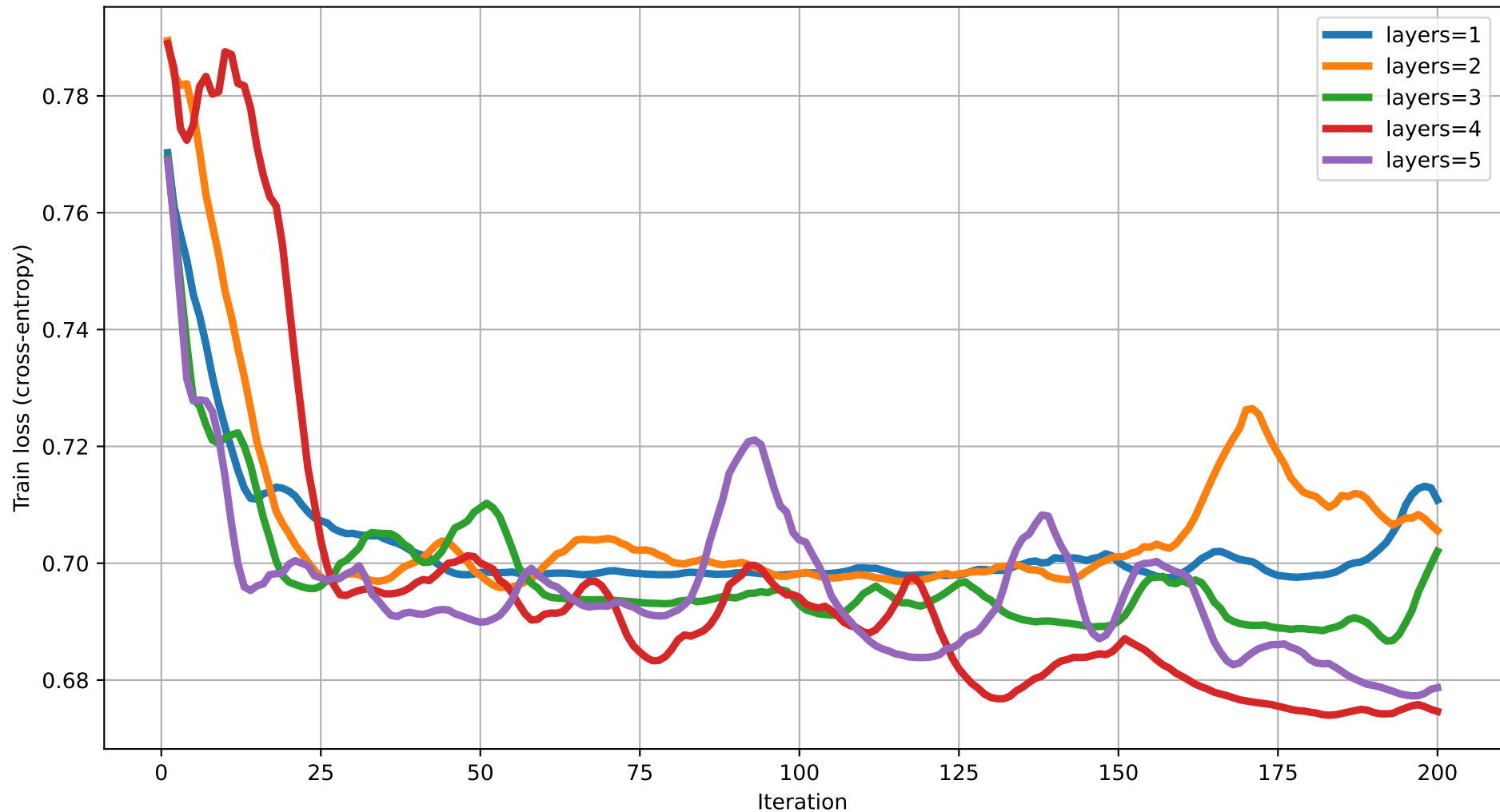
Train loss vs Iteration (dim=17) rot=RX, ent=full, gate=CZ
