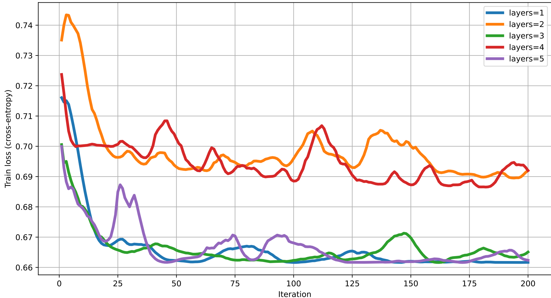
Train loss vs Iteration (dim=10) rot=RX, ent=ring, gate=lsingXX
