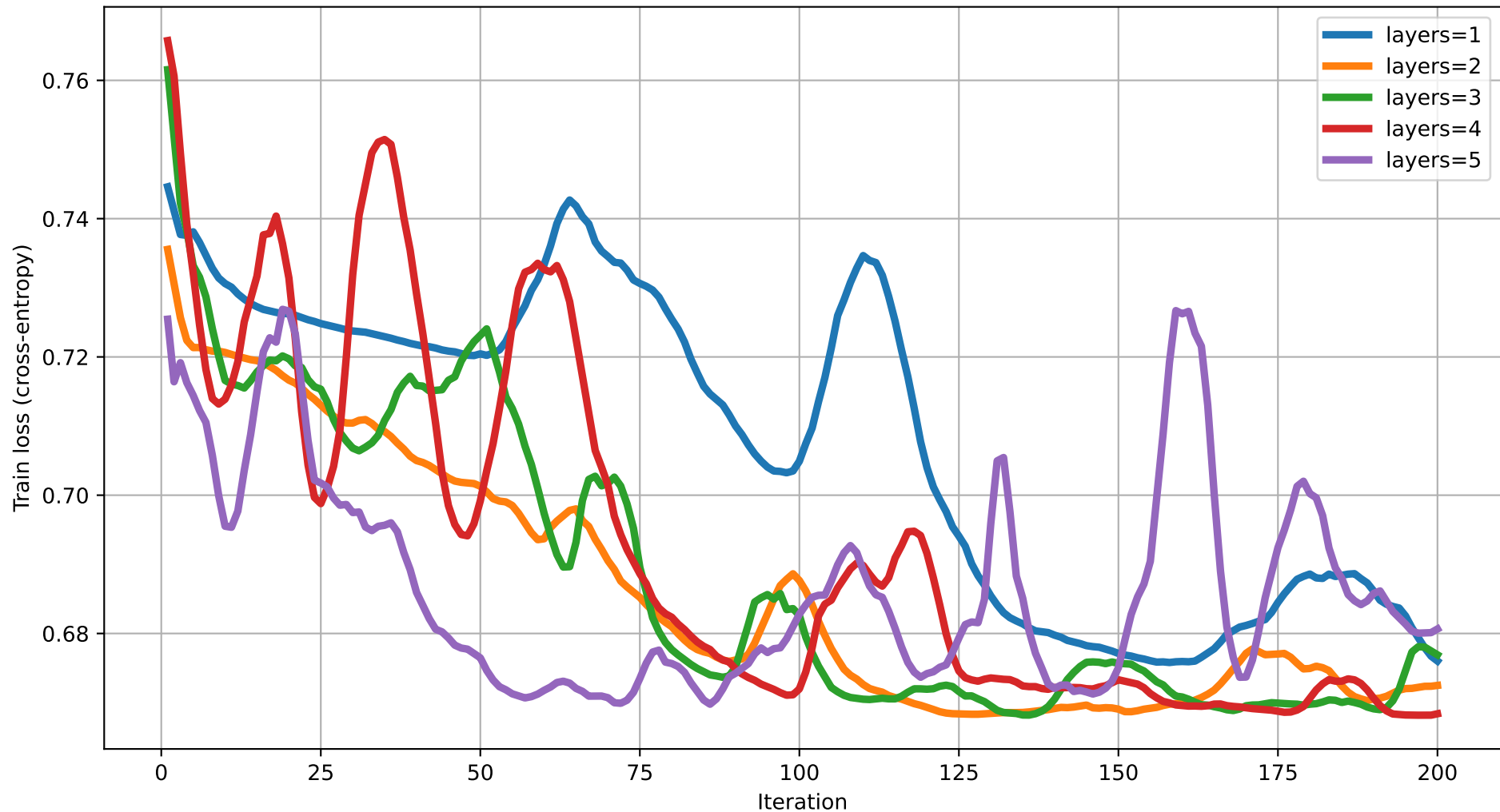
Train loss vs Iteration (dim=3) rot=Rot, ent=ring, gate=CZ
