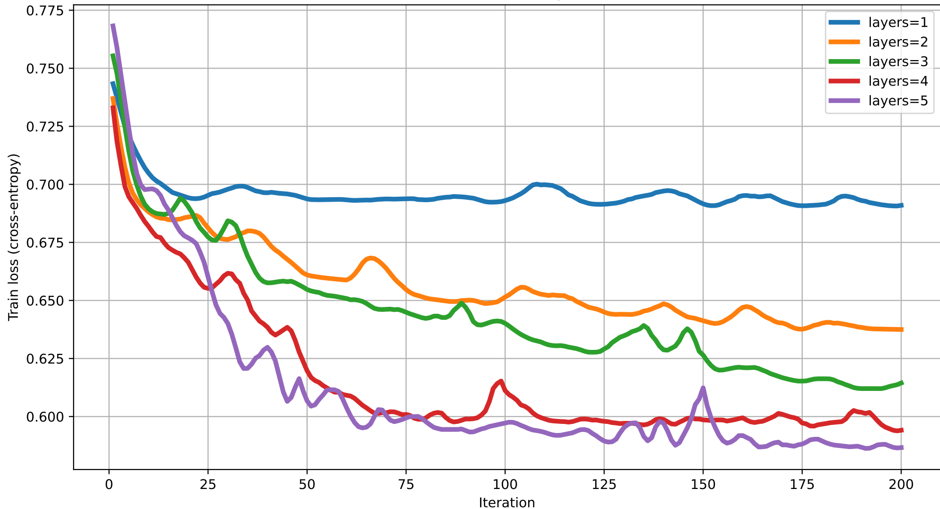
Train loss vs Iteration (degree=5) rot=Rot, ent=chain, gate=CZ
