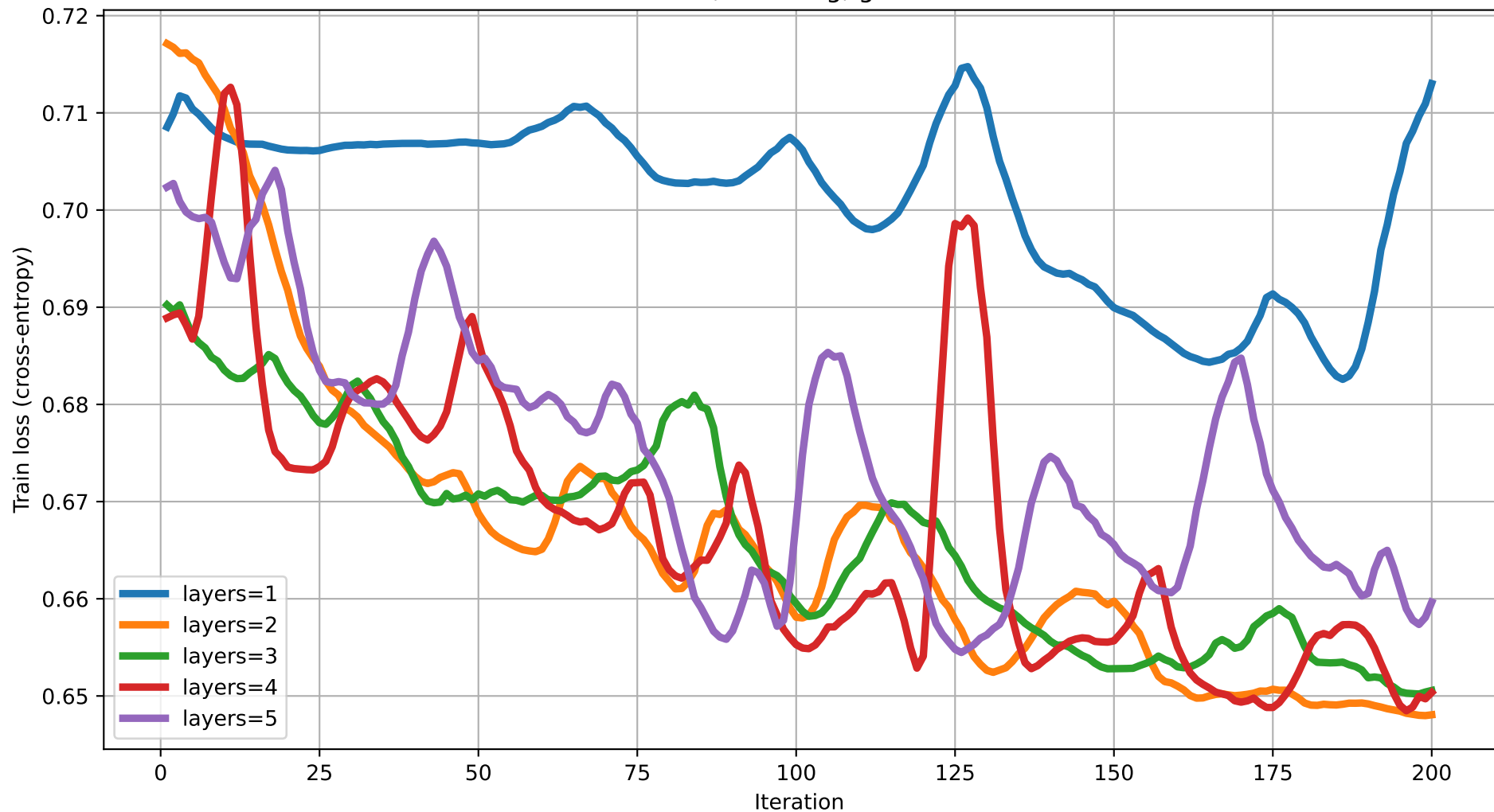
Train loss vs Iteration (dim=8) rot=RYZ, ent=ring, gate=CNOT
