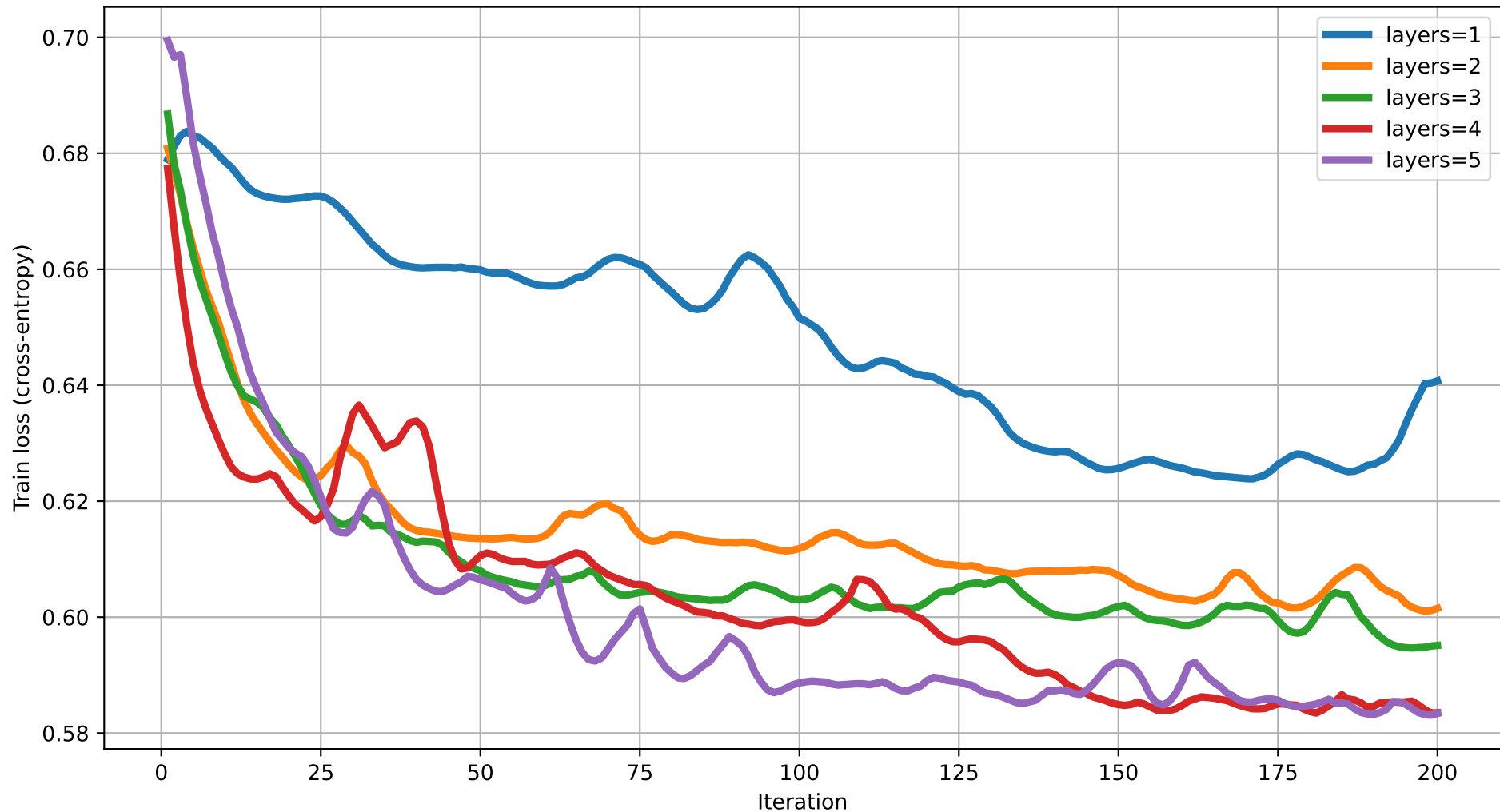
Train loss vs Iteration (degree=4) rot=RYZ, ent=ring, gate=CNOT
