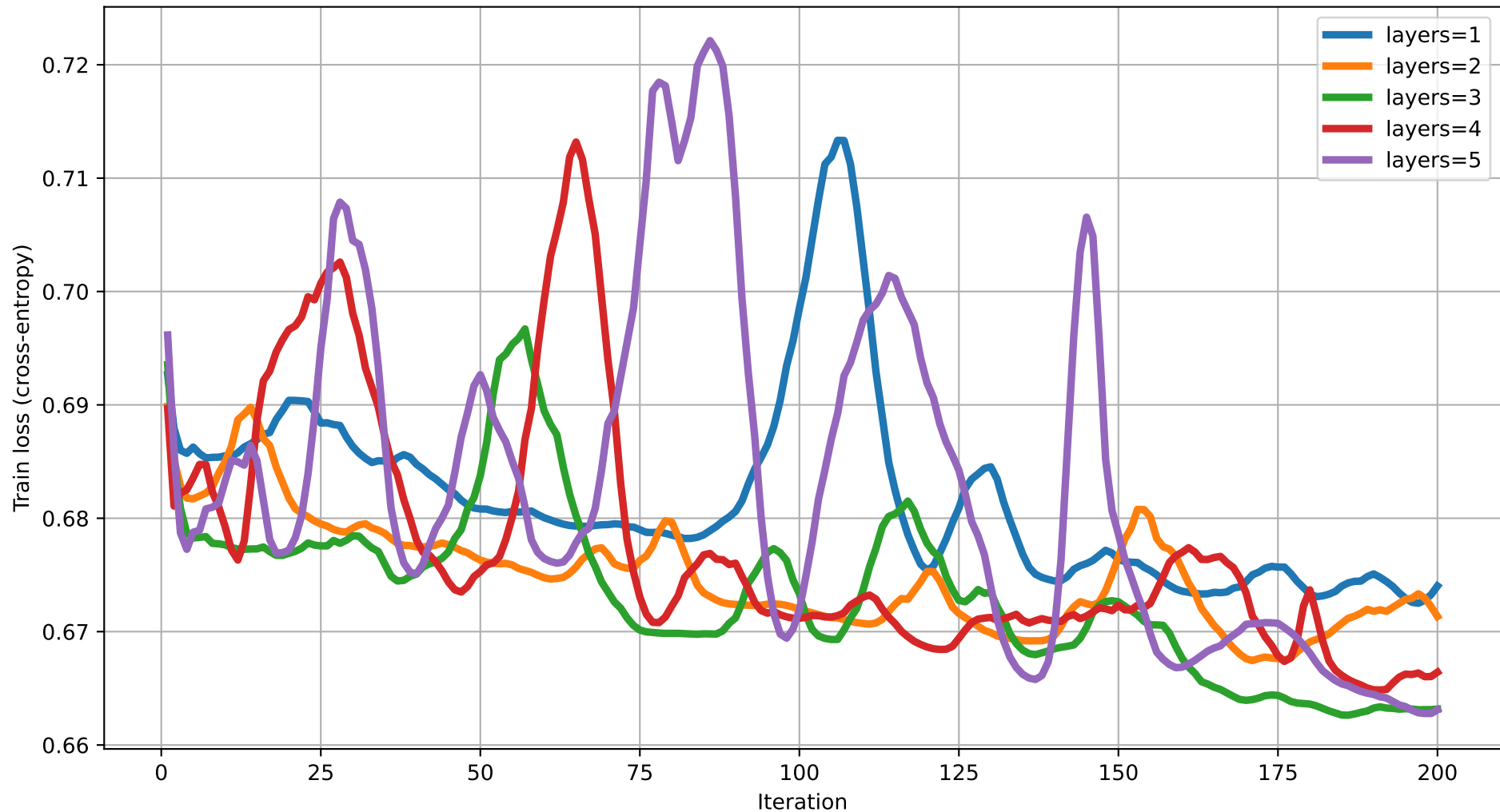
Train loss vs Iteration (dim=13) rot=RY, ent=pairwise, gate=CNOT
