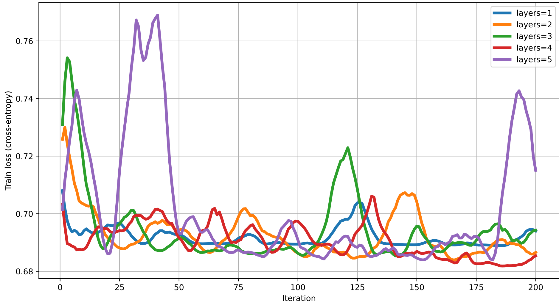
Train loss vs Iteration (dim=20) rot=RYZ, ent=pairwise, gate=CZ
