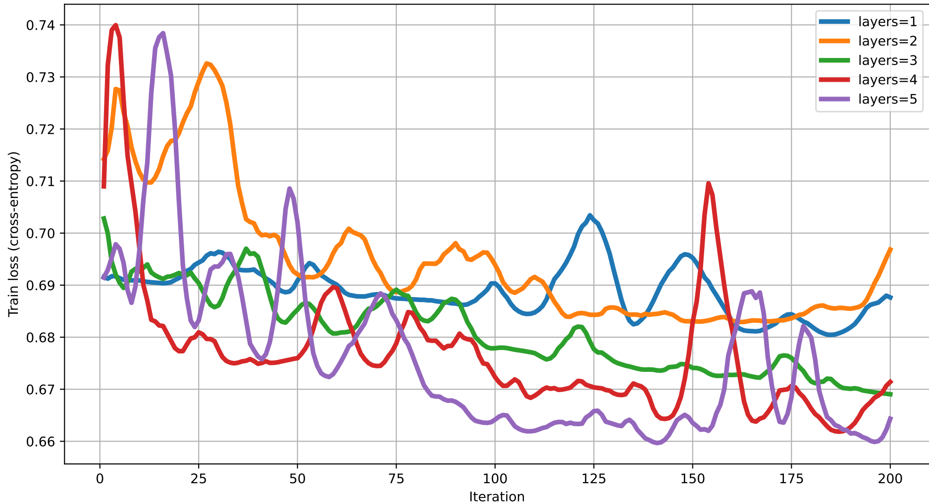
Train loss vs Iteration (dim=13) rot=RYZ, ent=pairwise, gate=IsingXX
