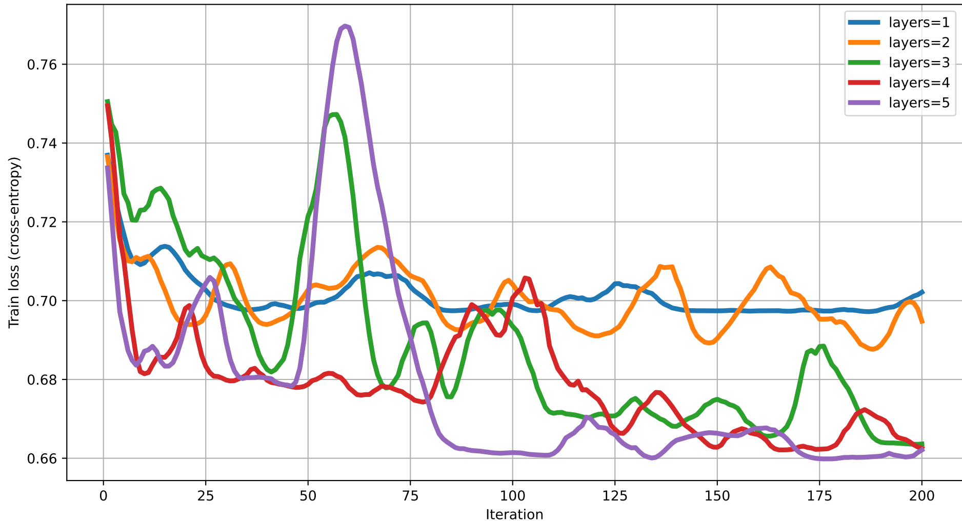
Train loss vs Iteration (dim=18) rot=RX, ent=full, gate=CNOT
