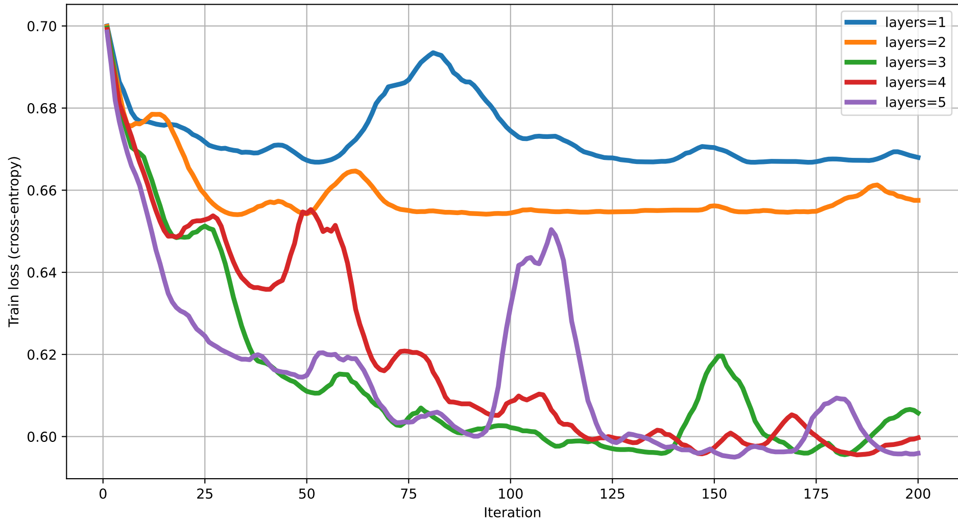
Train loss vs Iteration (dim=10) rot=RX, ent=ring, gate=CZ
