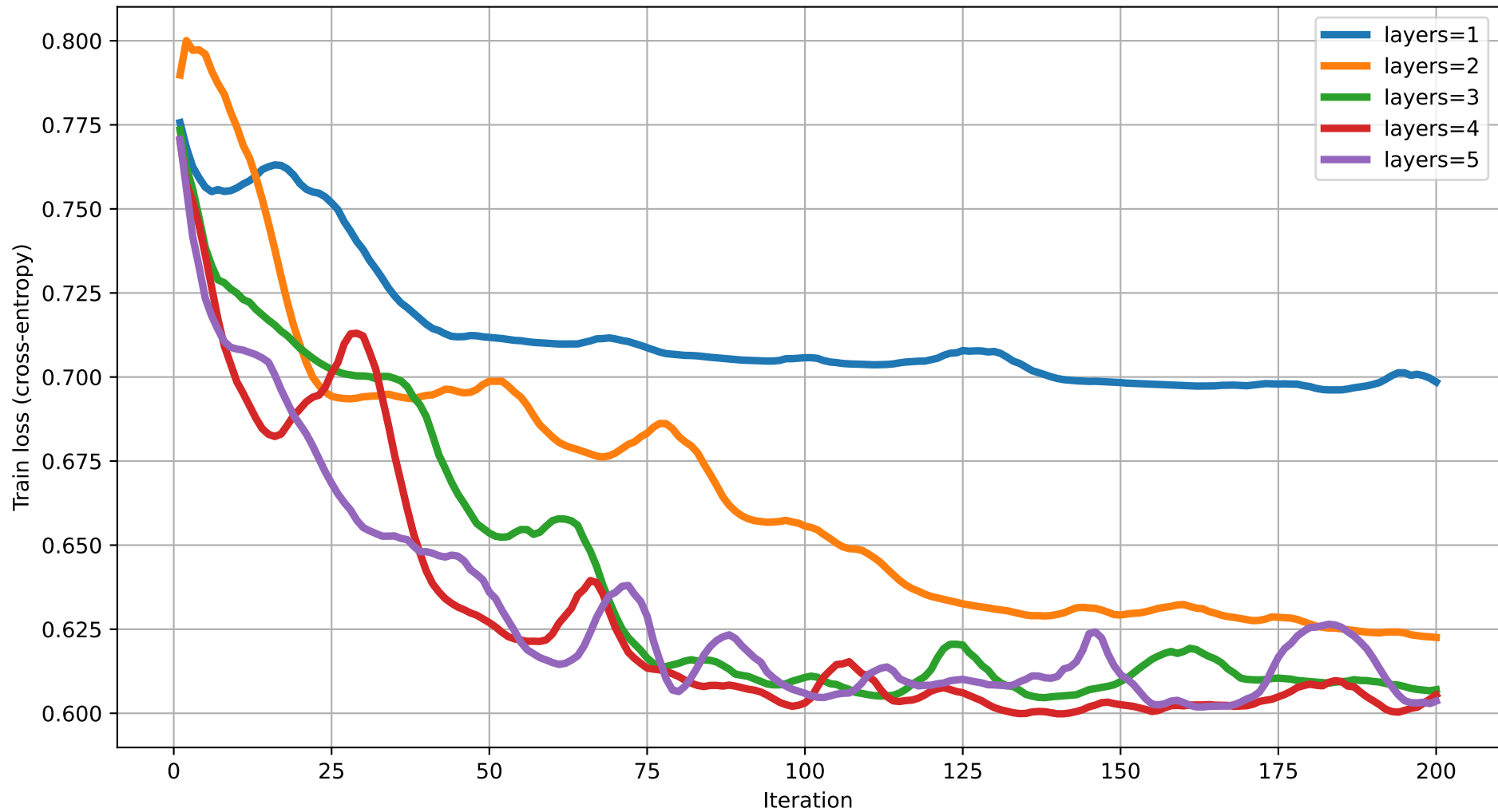
Train loss vs Iteration (dim=9) rot=RYZ, ent=ring, gate=CZ
