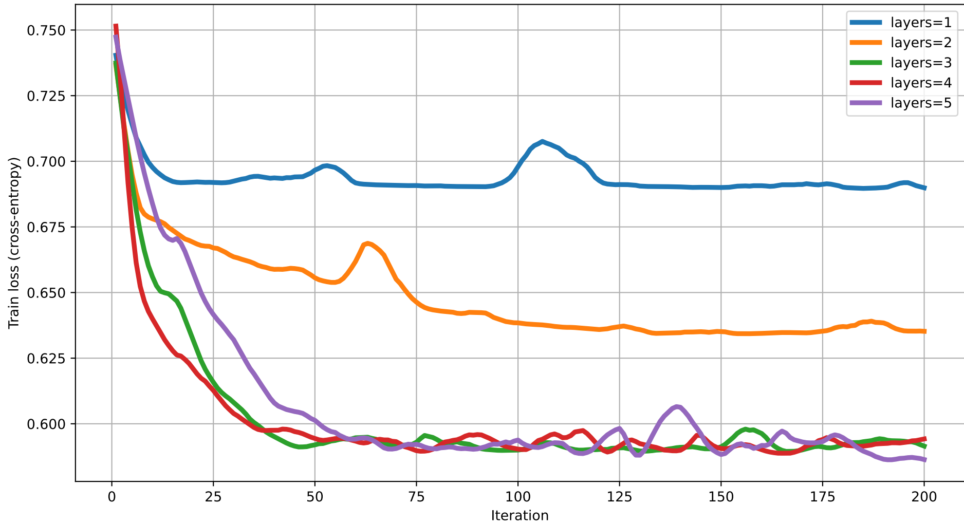
Train loss vs Iteration (degree=5) rot=RY, ent=chain, gate=CNOT
