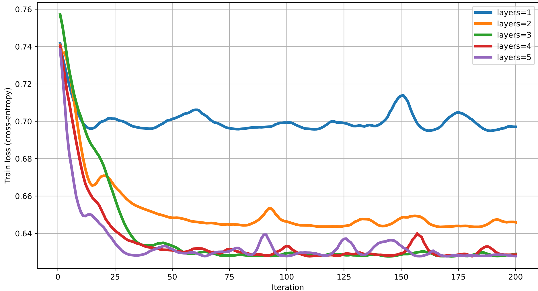
Train loss vs Iteration (degree=5) rot=RX, ent=pairwise, gate=CZ
