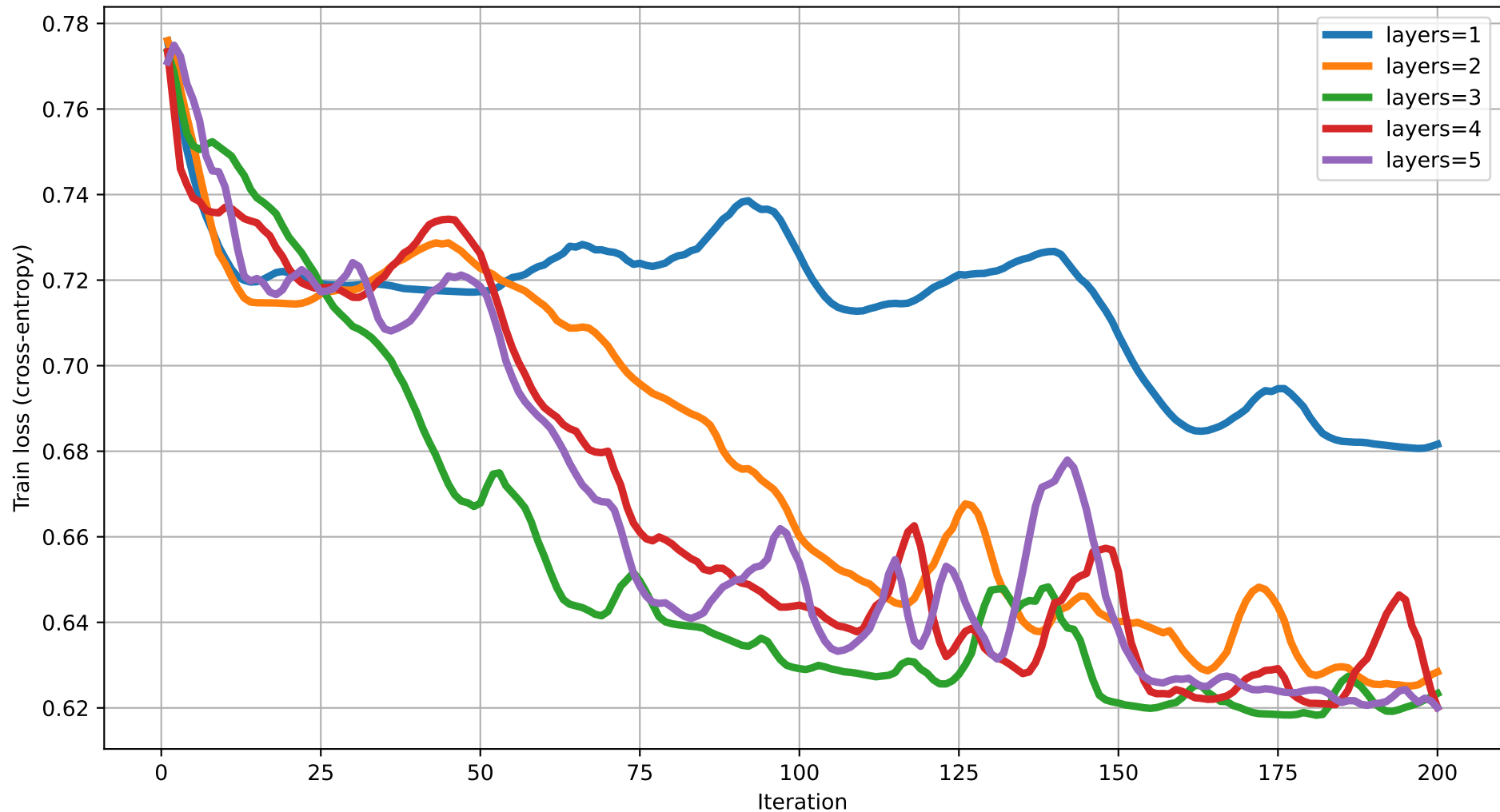
Train loss vs Iteration (dim=4) rot=RYZ, ent=chain, gate=CZ
