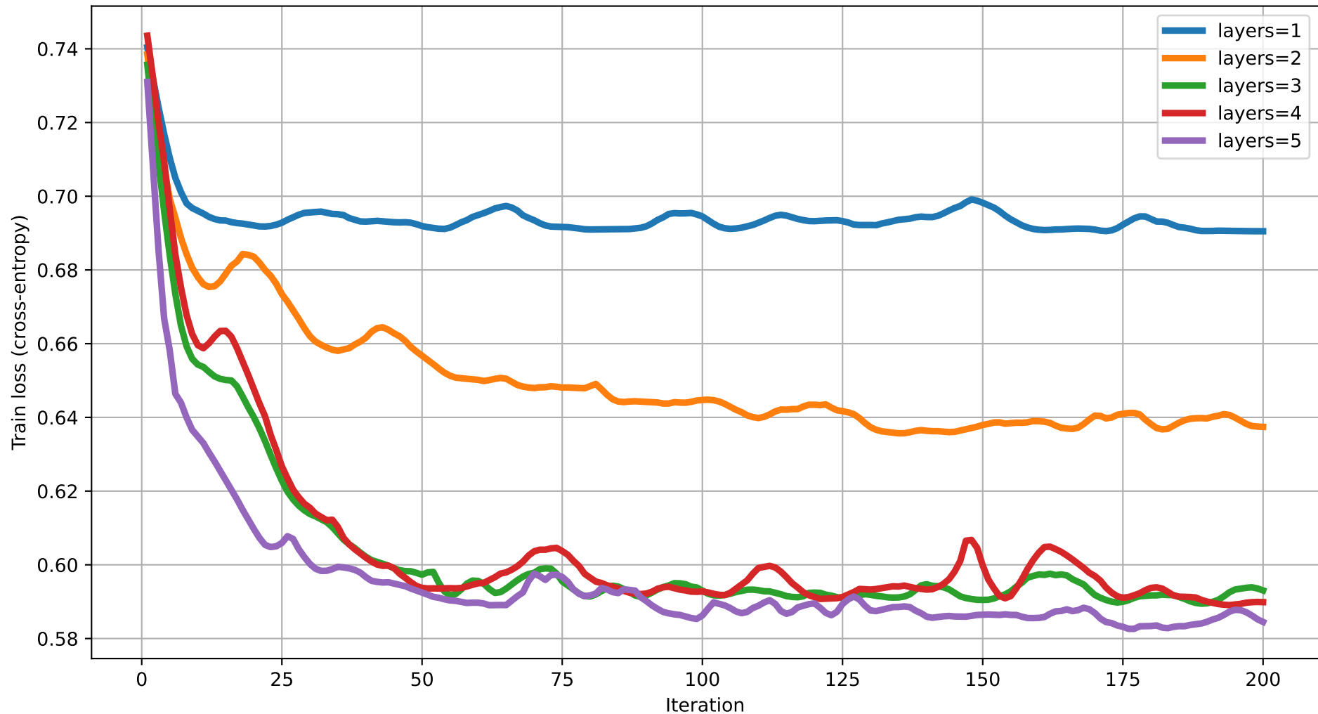
Train loss vs Iteration (degree=5) rot=Rot, ent=chain, gate=CNOT
