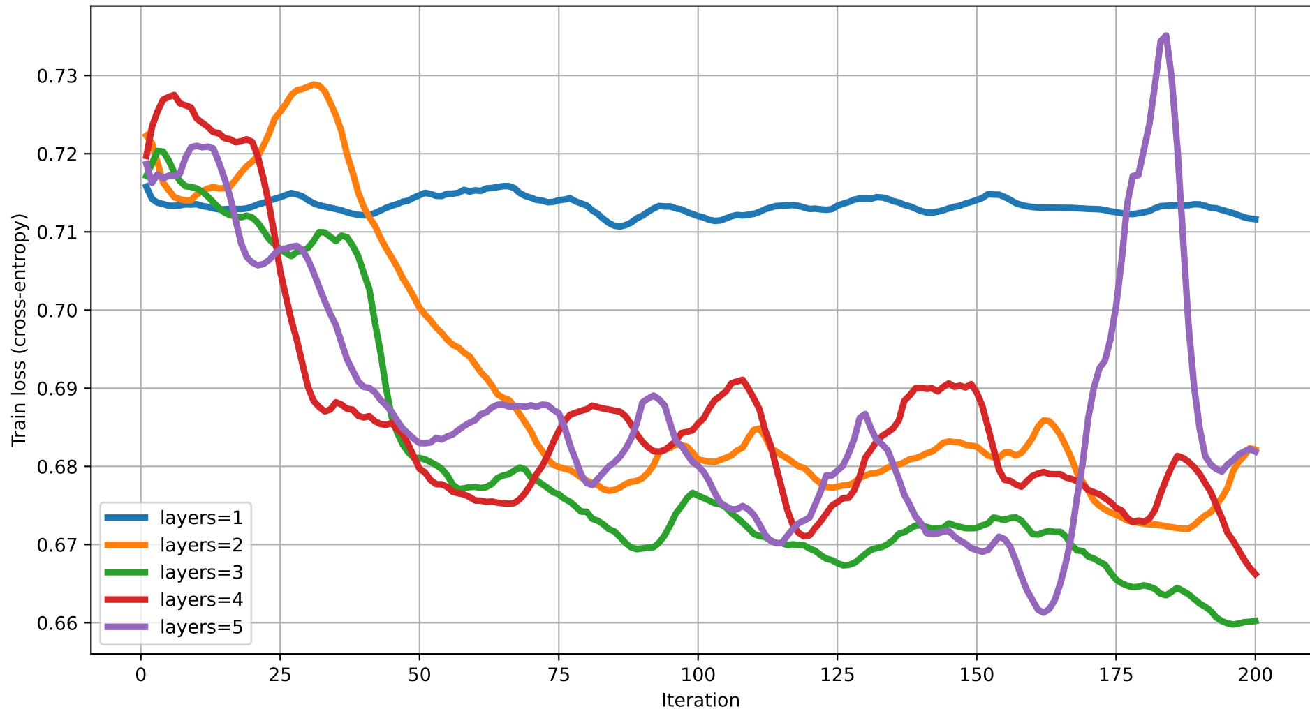
Train loss vs Iteration (dim=3) rot=RYZ, ent=full, gate=CZ
