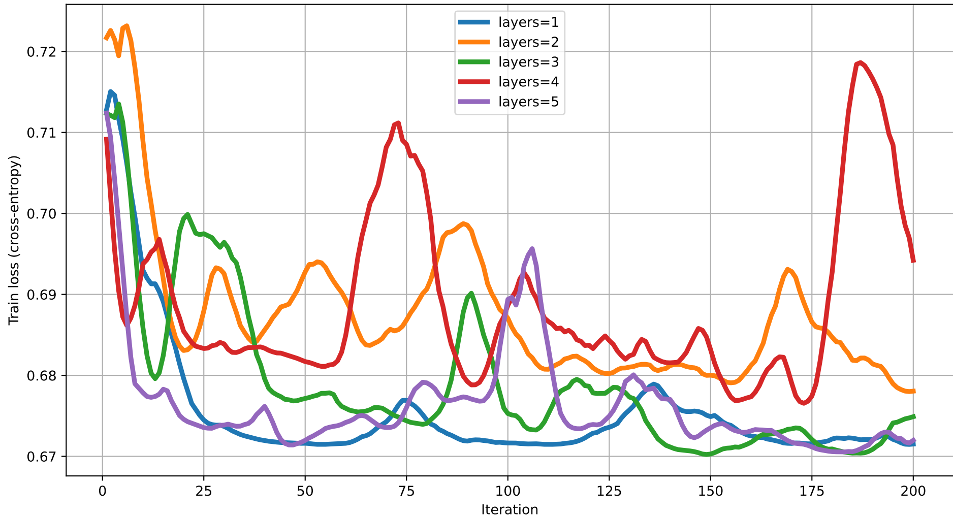
Train loss vs Iteration (dim=20) rot=RZ, ent=ring, gate=IsingXX
