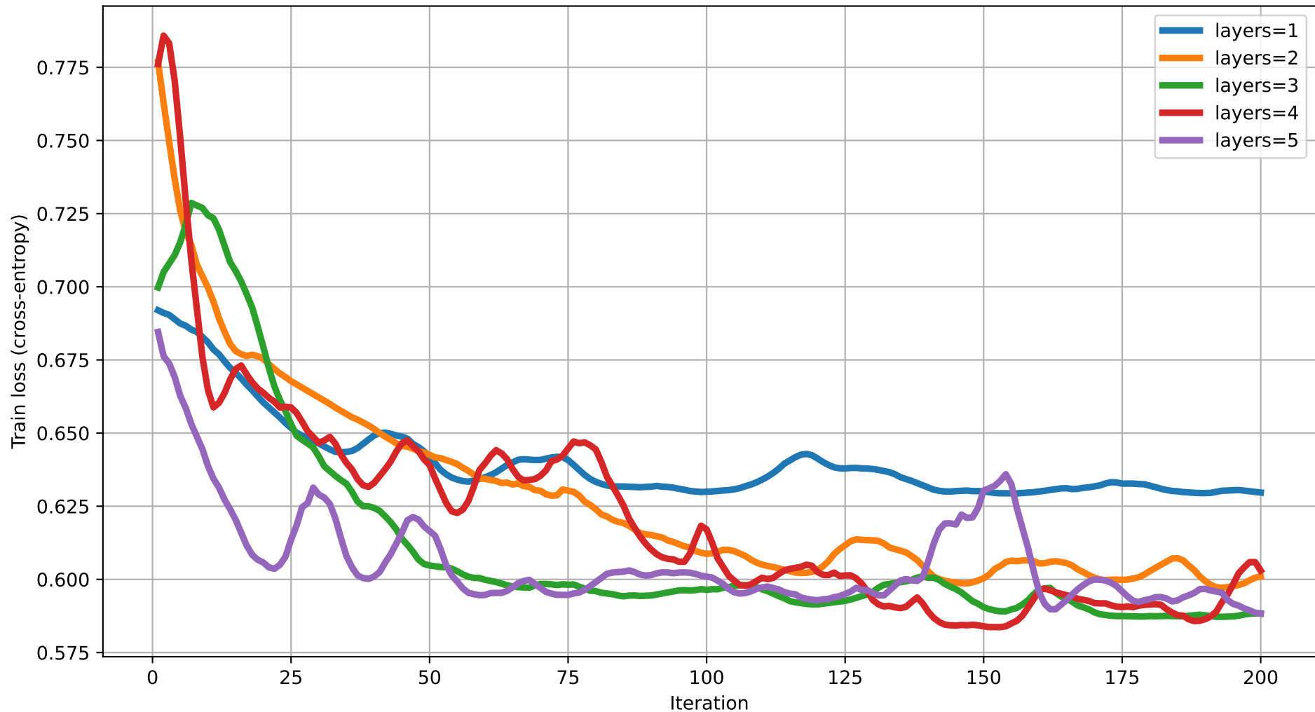
Train loss vs Iteration (dim=4) rot=RYZ, ent=chain, gate=IsingXX
