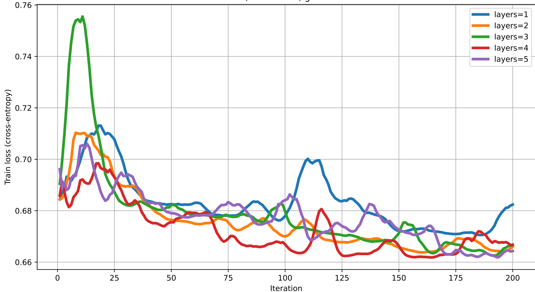
Train loss vs Iteration (dim=15) rot=RY, ent=chain, gate=CNOT
