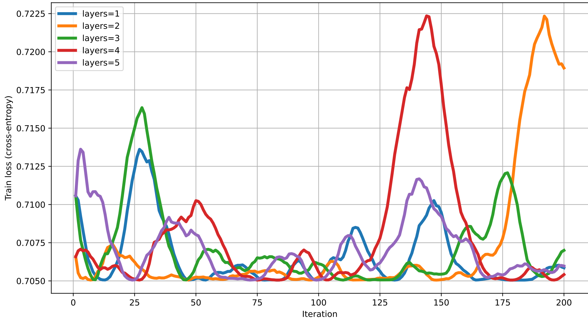
Train loss vs Iteration (dim=14) rot=RZ, ent=ring, gate=CZ
