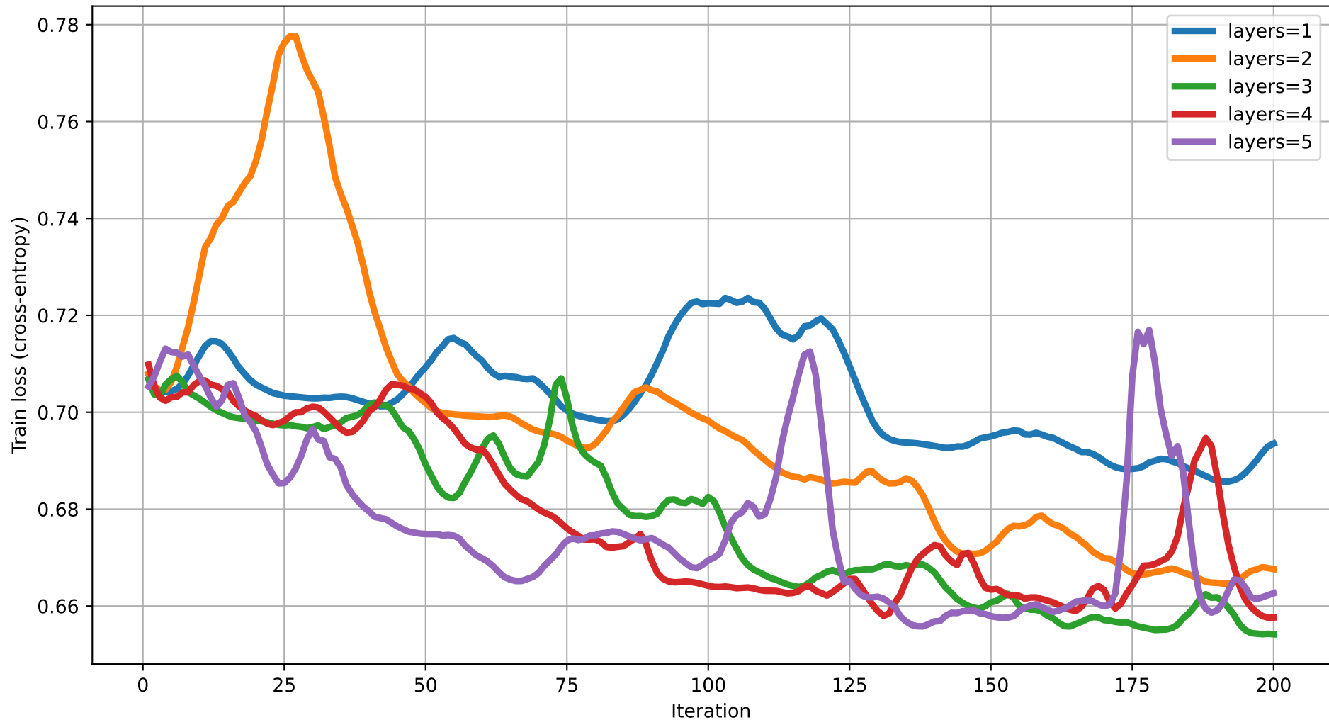
Train loss vs Iteration (dim=6) rot=Rot, ent=full, gate=CZ
