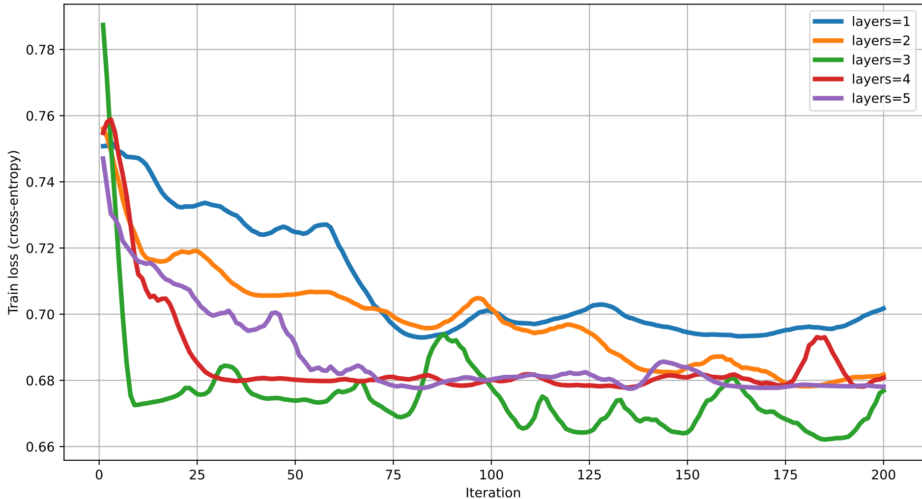
Train loss vs Iteration (dim=2) rot=RX, ent=ring, gate=CNOT
