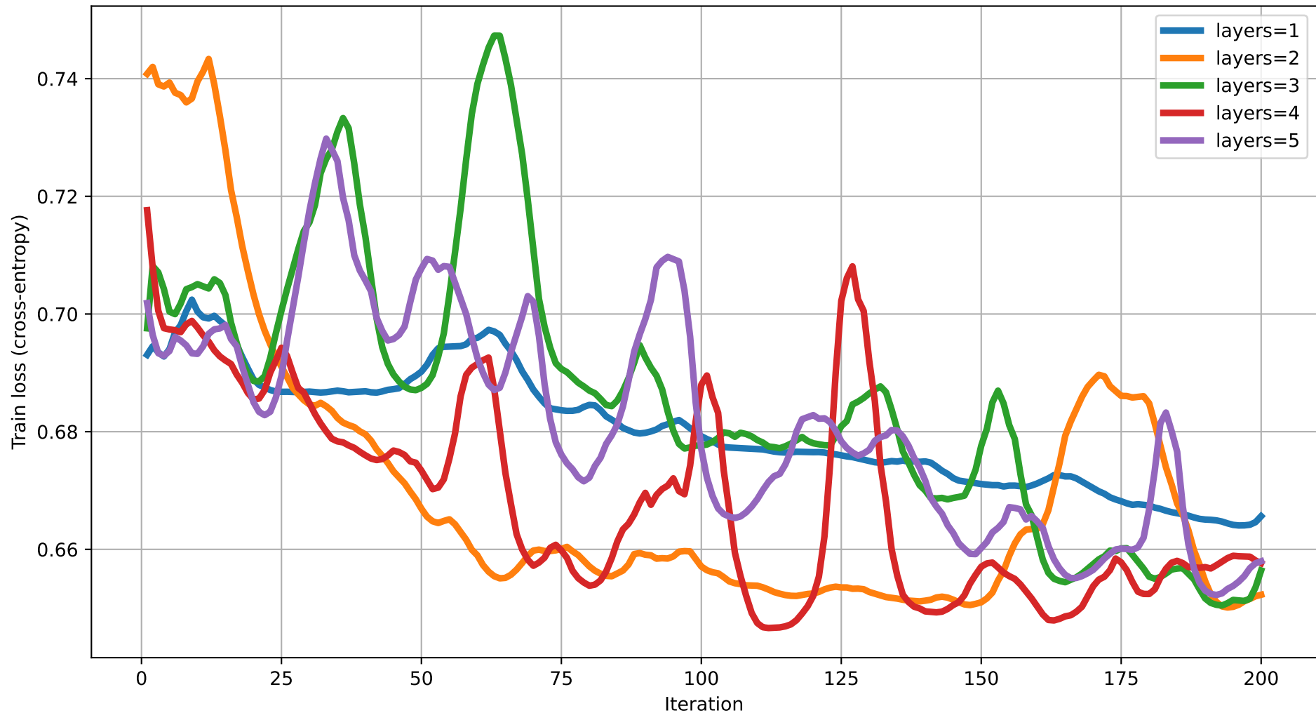
Train loss vs Iteration (dim=6) rot=RYZ, ent=chain, gate=IsingXX
