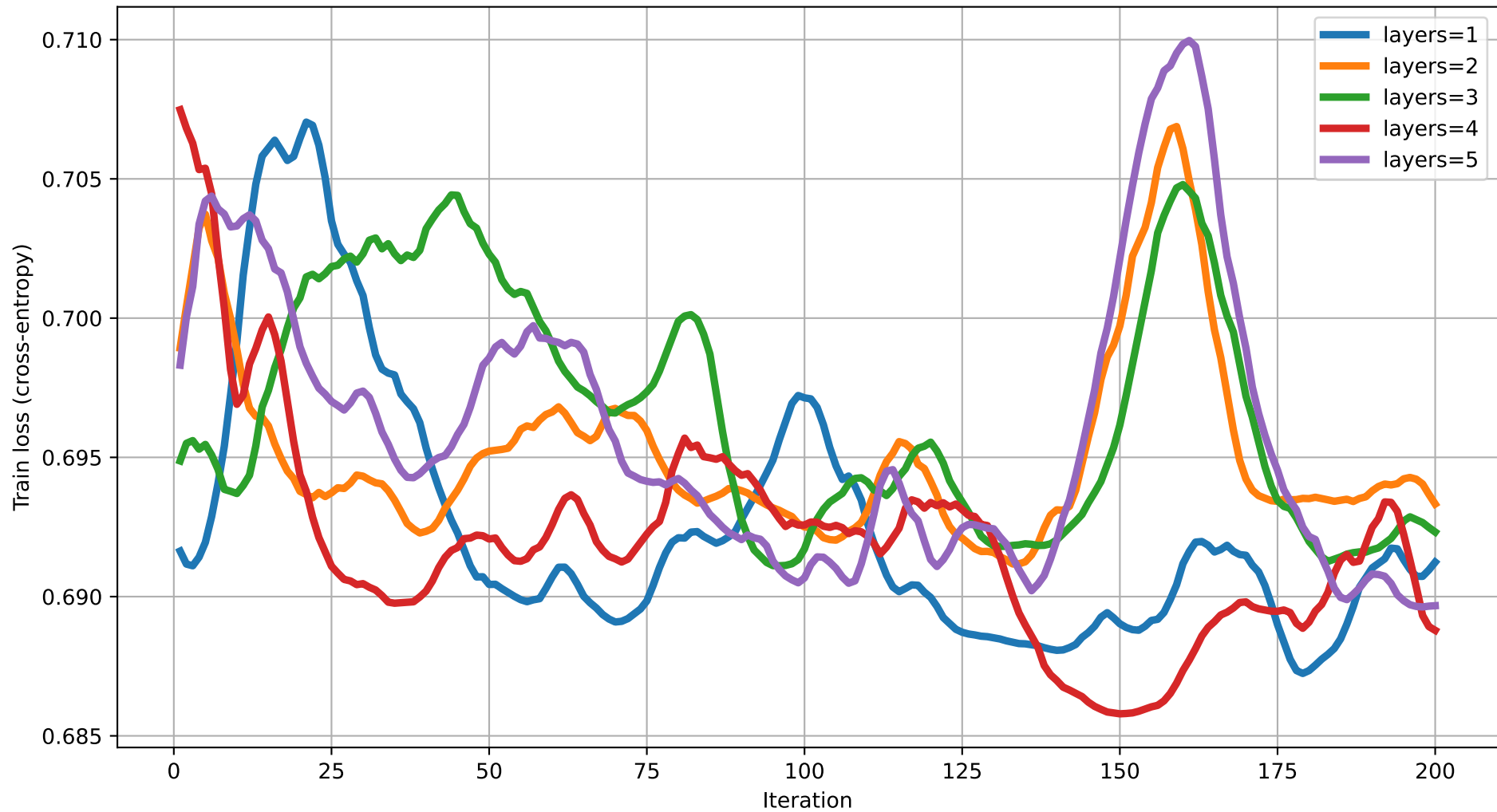
Train loss vs Iteration (dim=20) rot=RX, ent=ring, gate=CNOT
