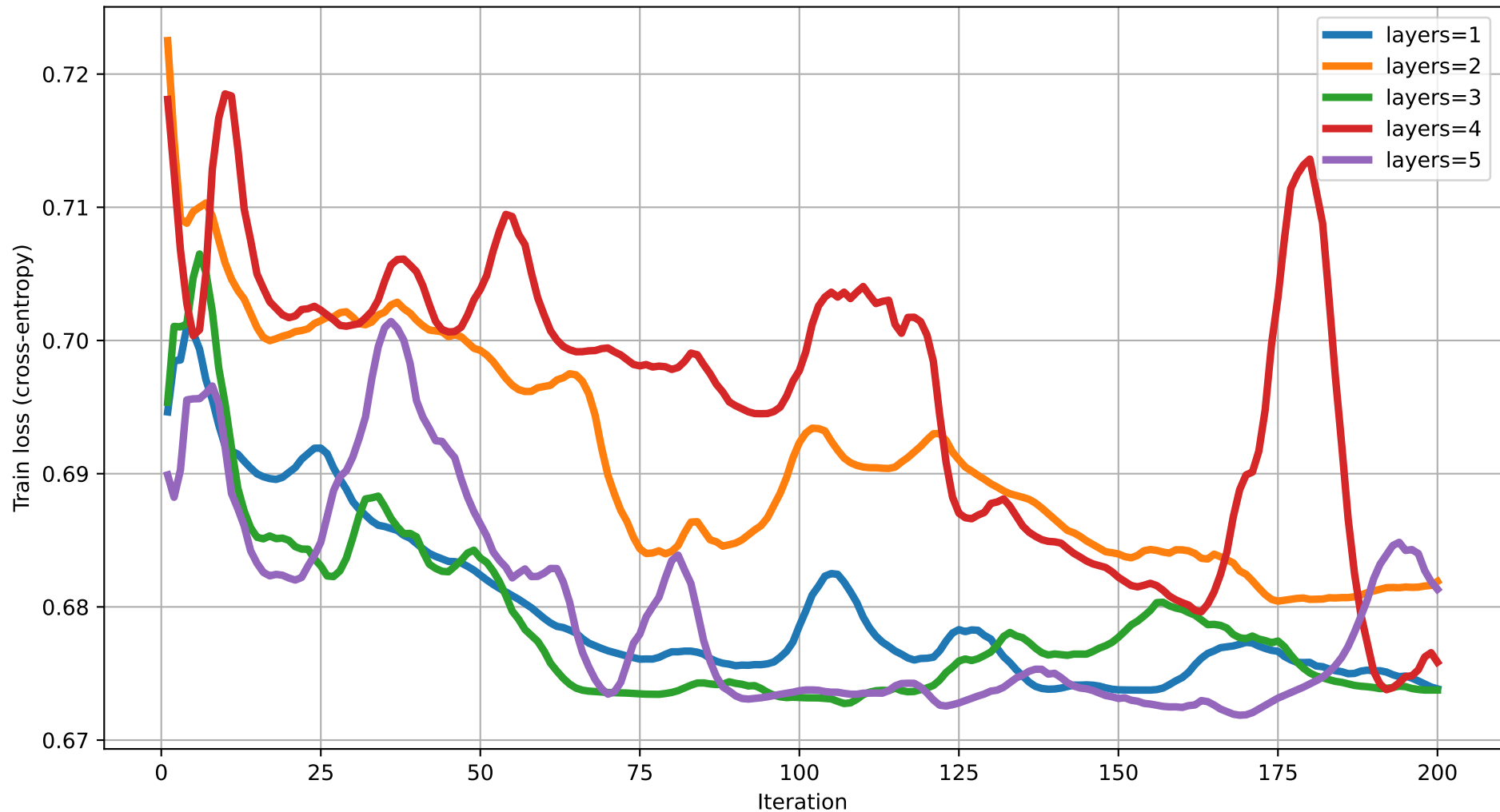
Train loss vs Iteration (dim=11) rot=RZ, ent=chain, gate=IsingXX
