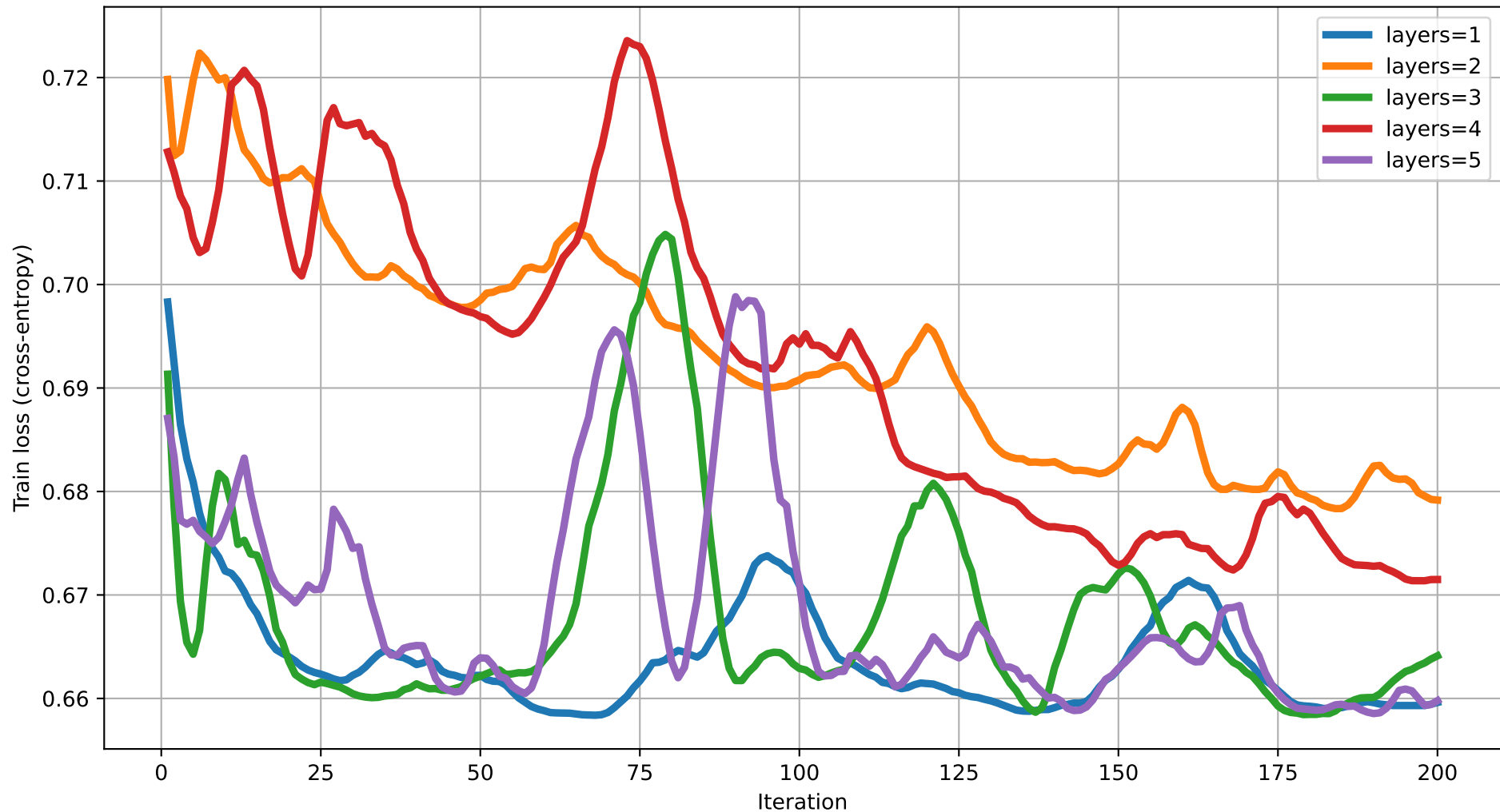
Train loss vs Iteration (dim=10) rot=RY, ent=ring, gate=IsingXX
