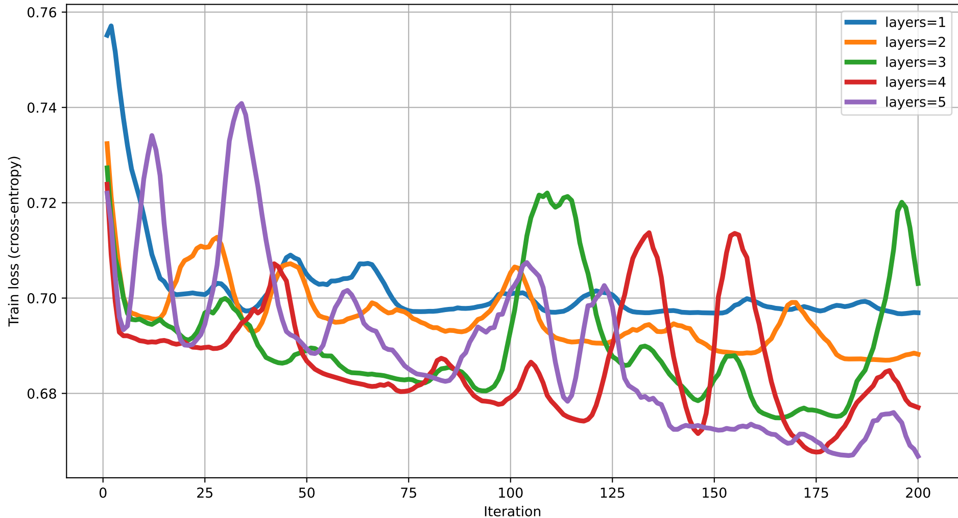
Train loss vs Iteration (dim=18) rot=RY, ent=chain, gate=CNOT
