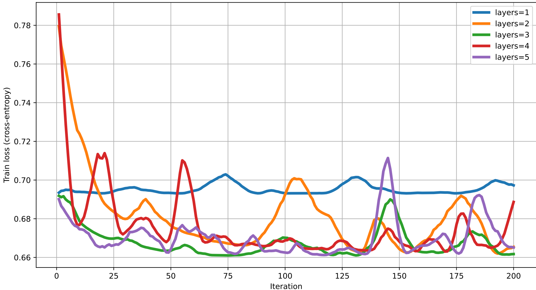
Train loss vs Iteration (dim=4) rot=RY, ent=pairwise, gate=IsingXX
