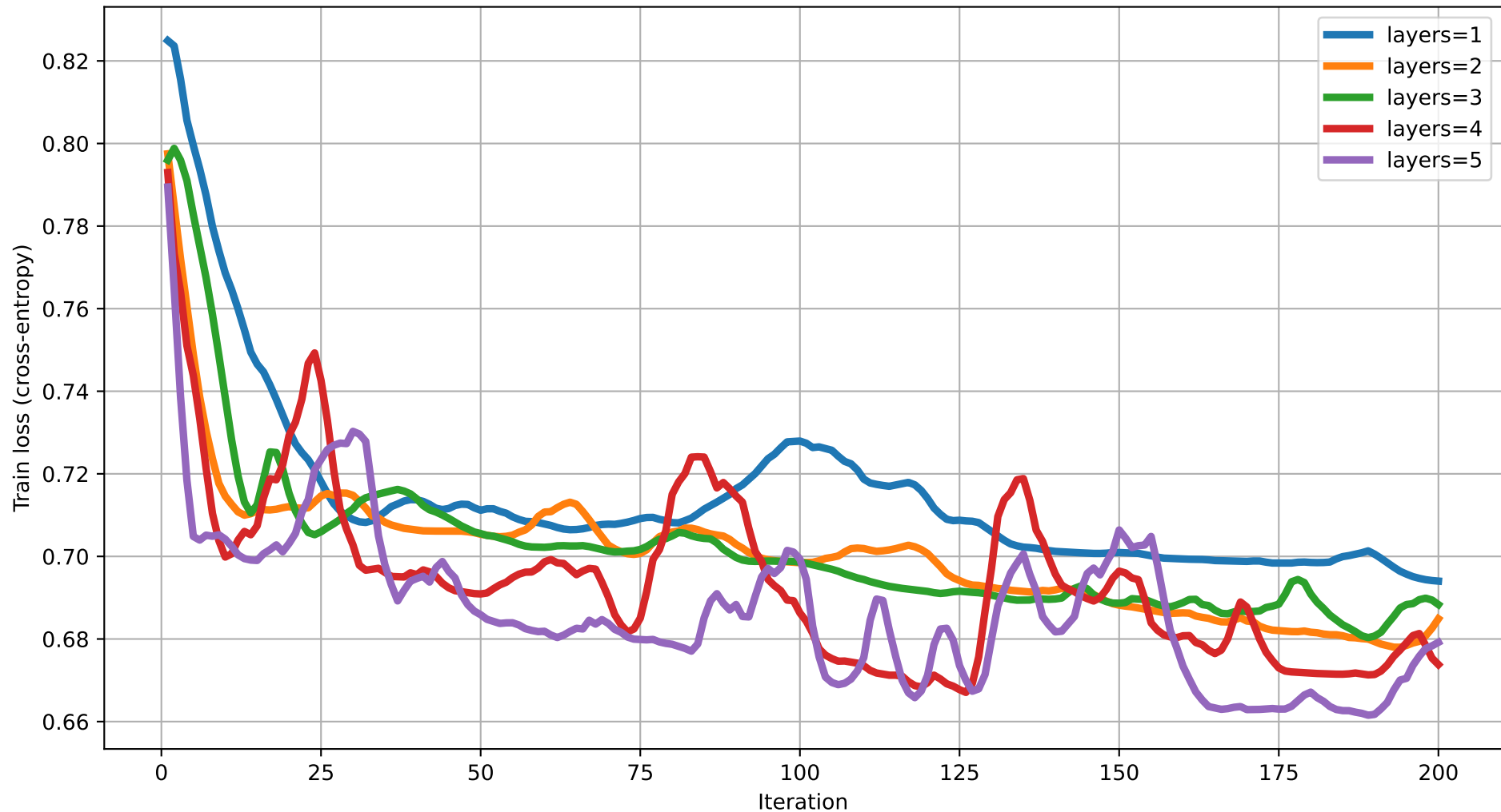
Train loss vs Iteration (dim=8) rot=Rot, ent=pairwise, gate=CZ
