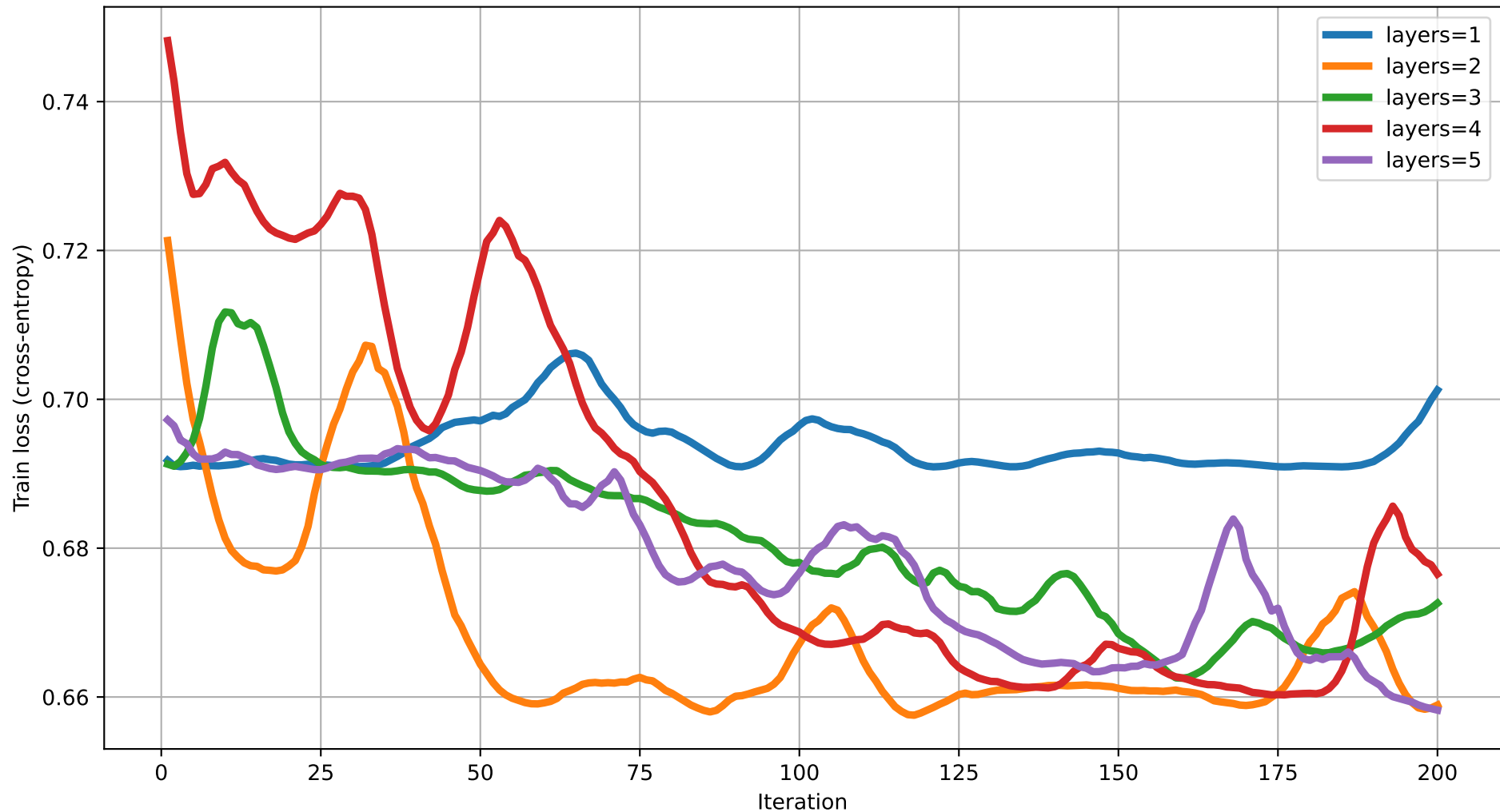
Train loss vs Iteration (dim=5) rot=RY, ent=chain, gate=IsingXX
