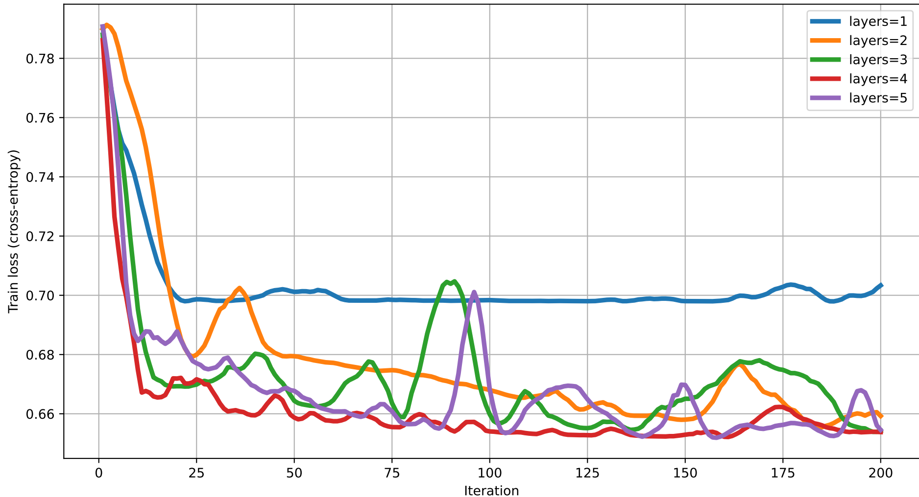
Train loss vs Iteration (dim=4) rot=RX, ent=pairwise, gate=CNOT
