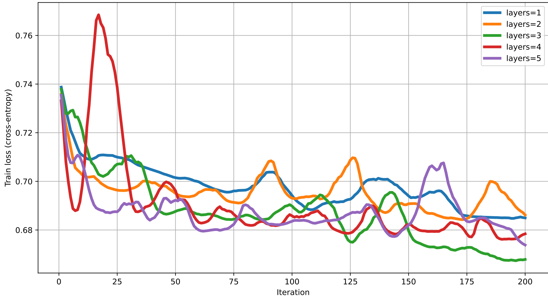
Train loss vs Iteration (dim=19) rot=RZ, ent=full, gate=IsingXX
