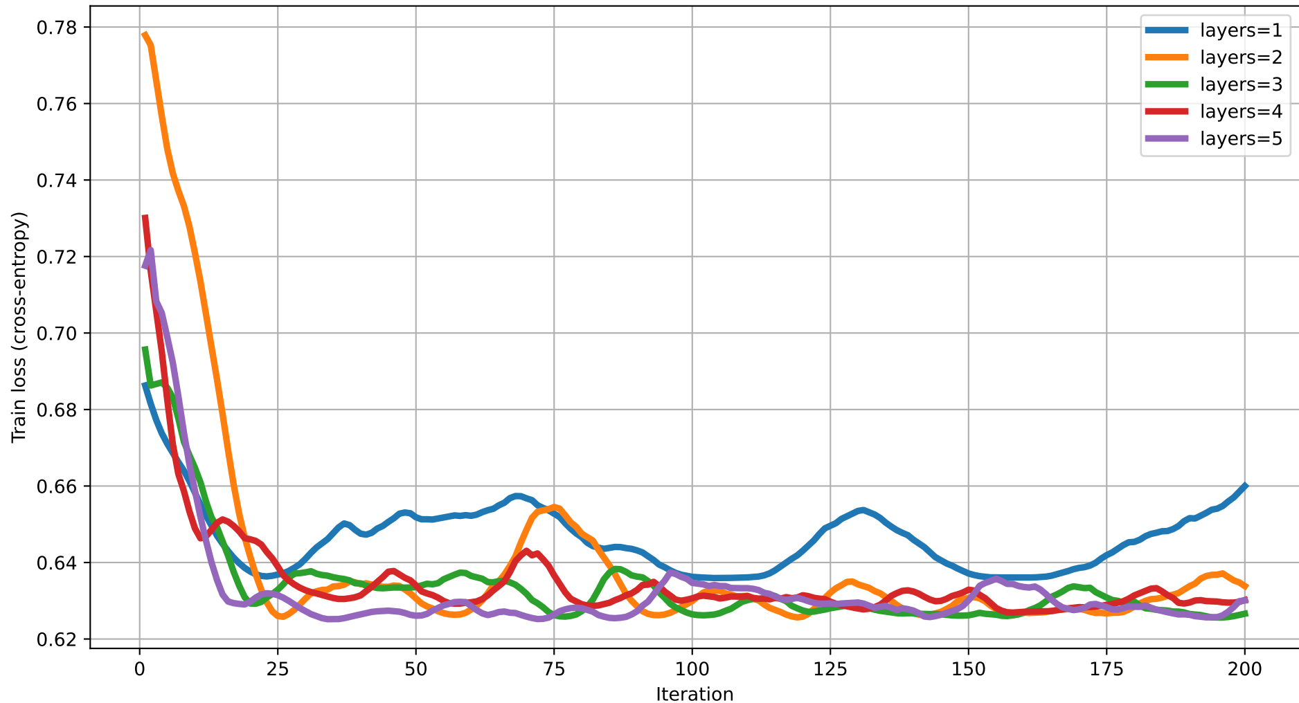
Train loss vs Iteration (dim=10) rot=RZ, ent=pairwise, gate=IsingXX
