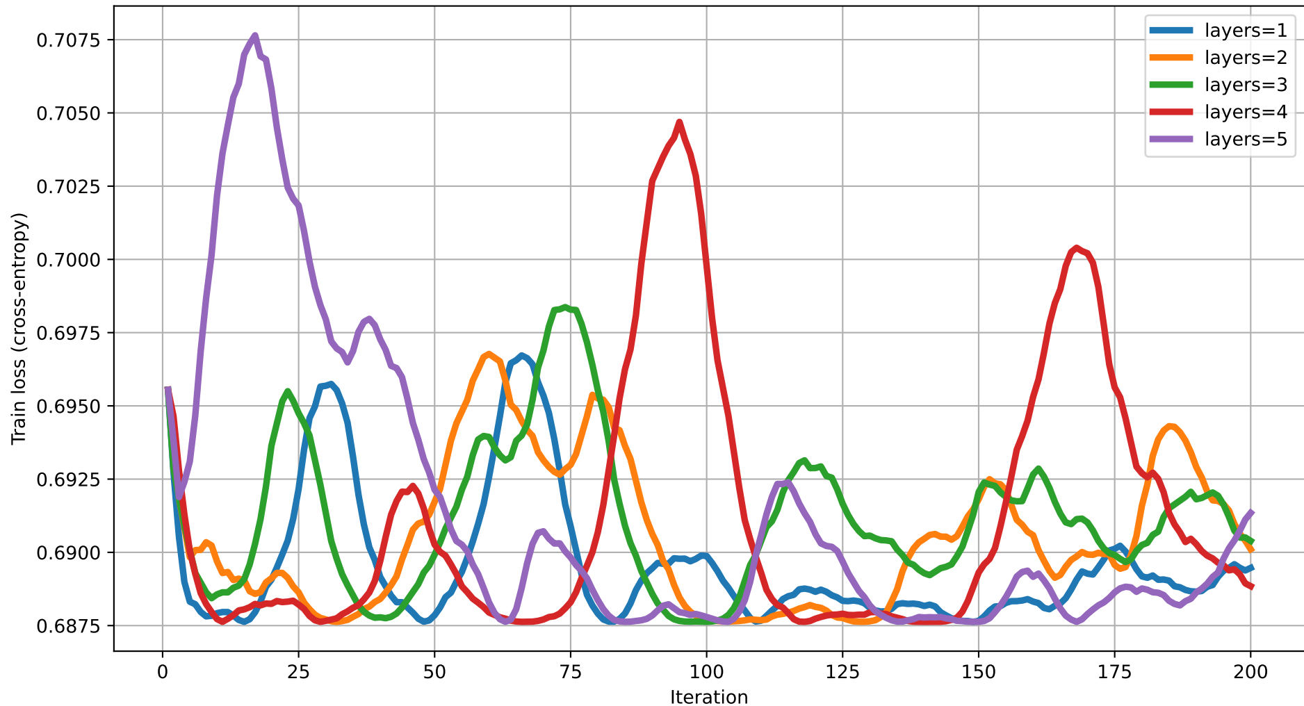
Train loss vs Iteration (dim=13) rot=RZ, ent=chain, gate=CNOT
