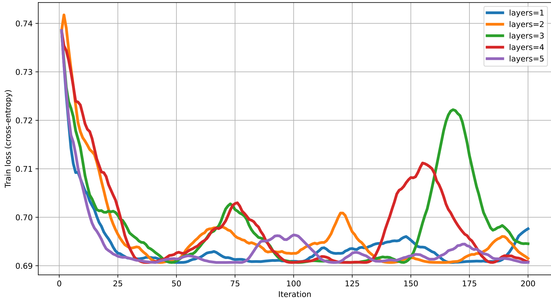
Train loss vs Iteration (dim=16) rot=RZ, ent=chain, gate=CZ
