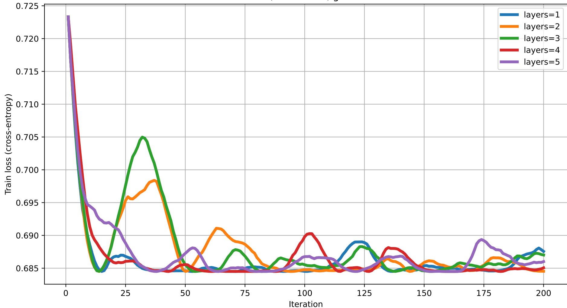
Train loss vs Iteration (degree=3) rot=RZ, ent=chain, gate=CZ
