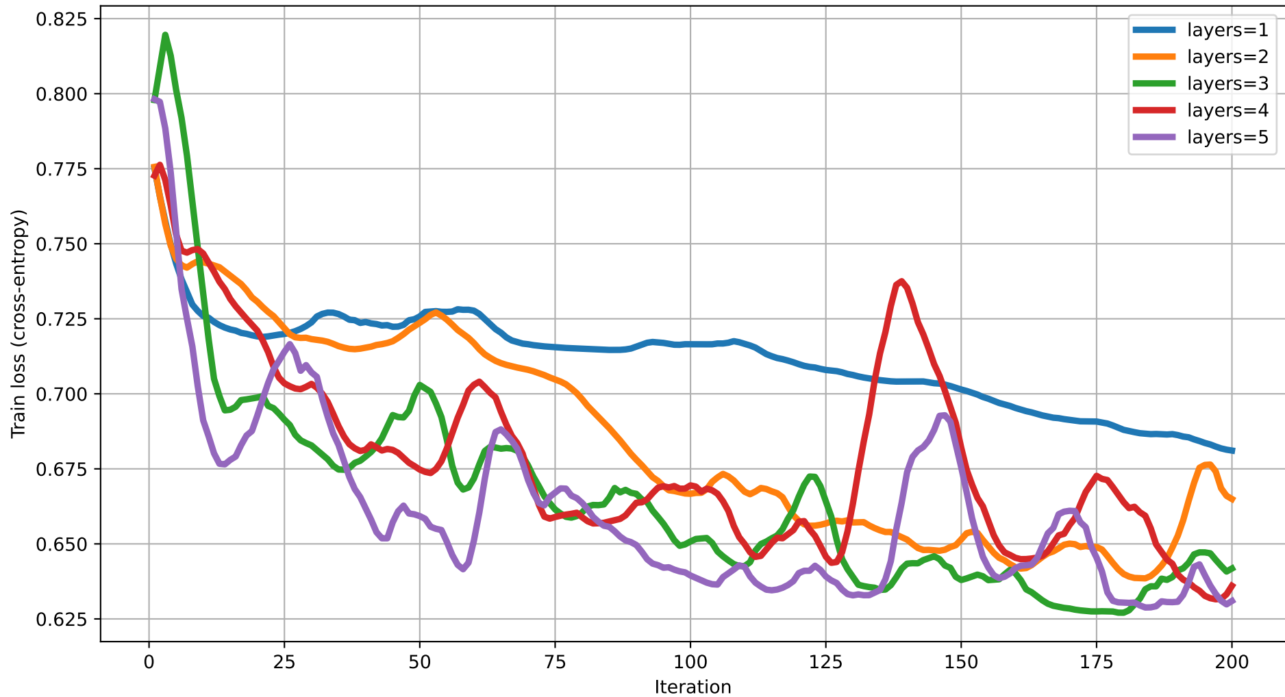
Train loss vs Iteration (dim=4) rot=RYZ, ent=full, gate=CZ
