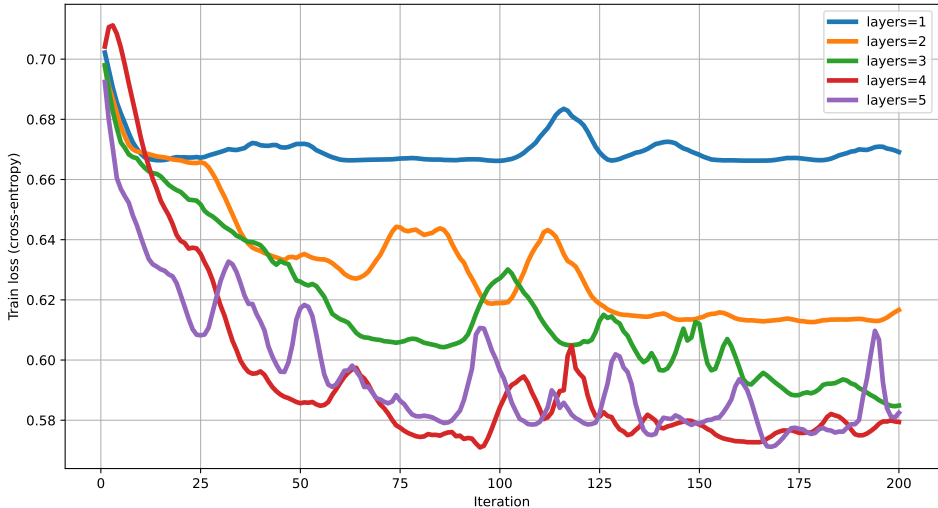
Train loss vs Iteration (dim=10) rot=Rot, ent=ring, gate=CZ
