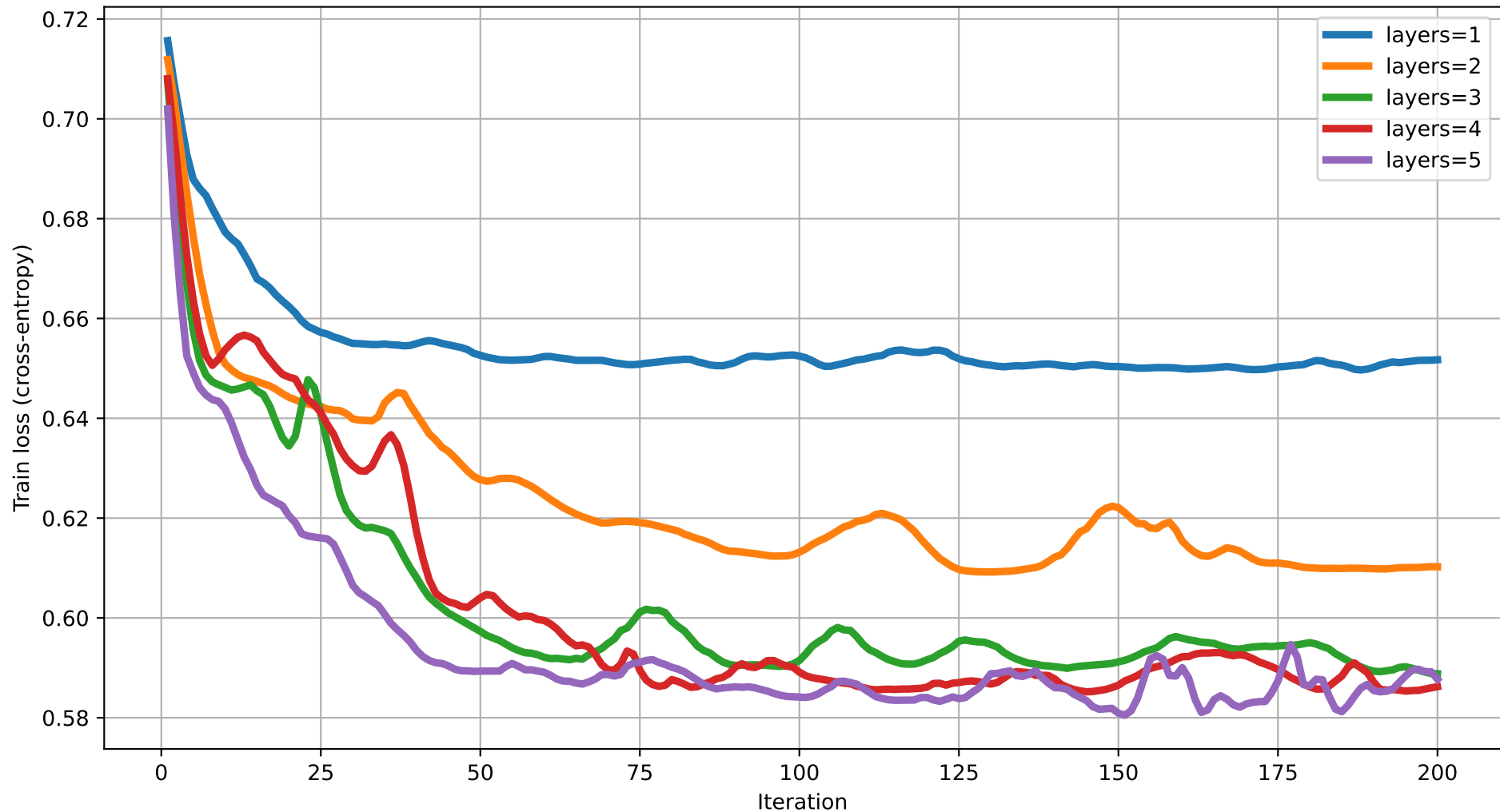
Train loss vs Iteration (degree=4) rot=Rot, ent=chain, gate=CZ
