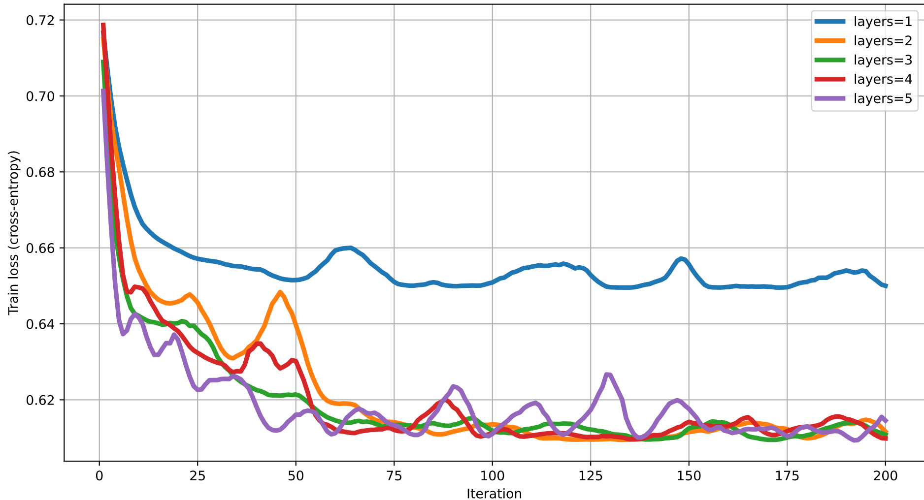
Train loss vs Iteration (degree=4) rot=RY, ent=pairwise, gate=CNOT
