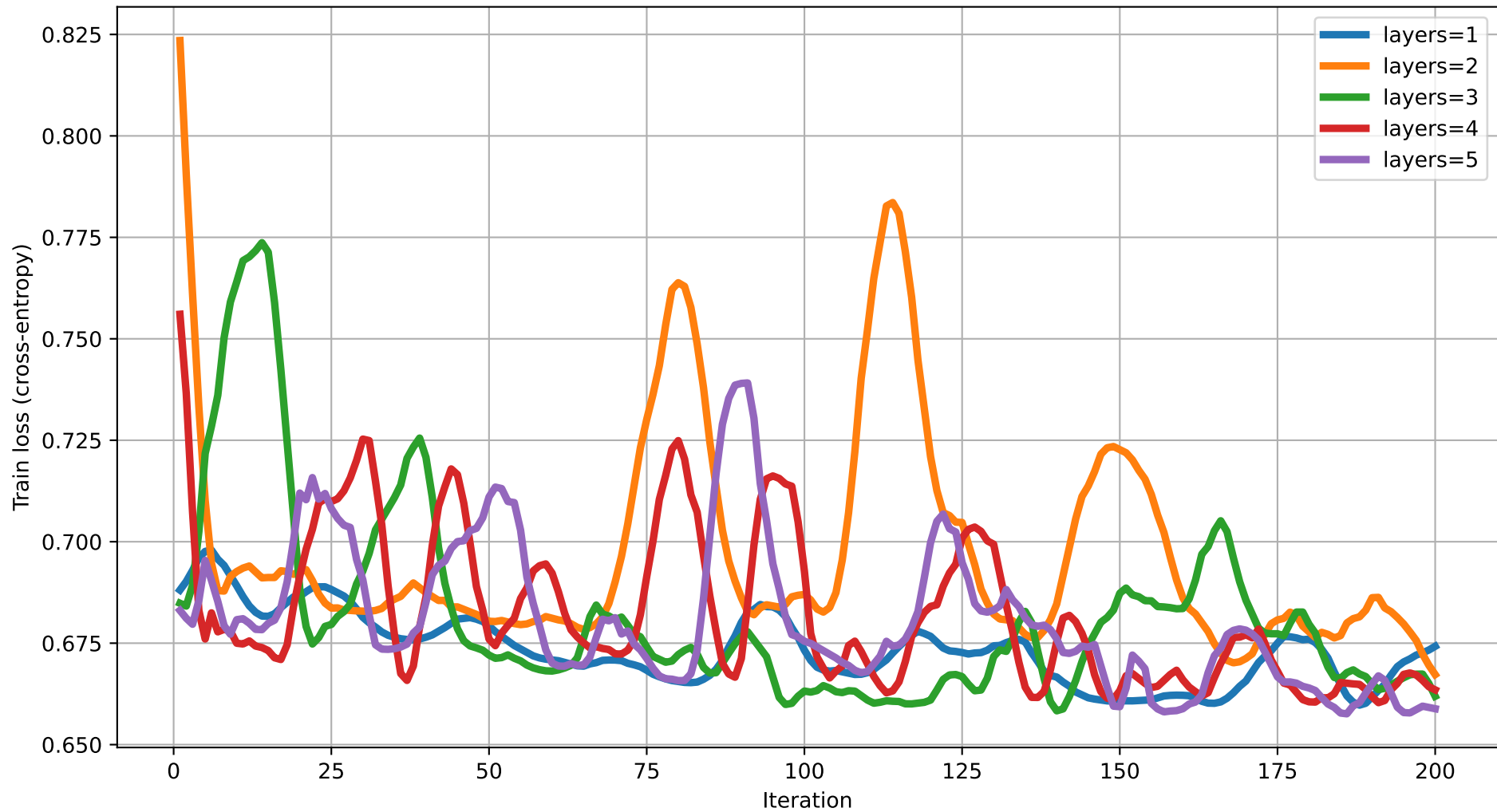
Train loss vs Iteration (dim=16) rot=Rot, ent=pairwise, gate=IsingXX
