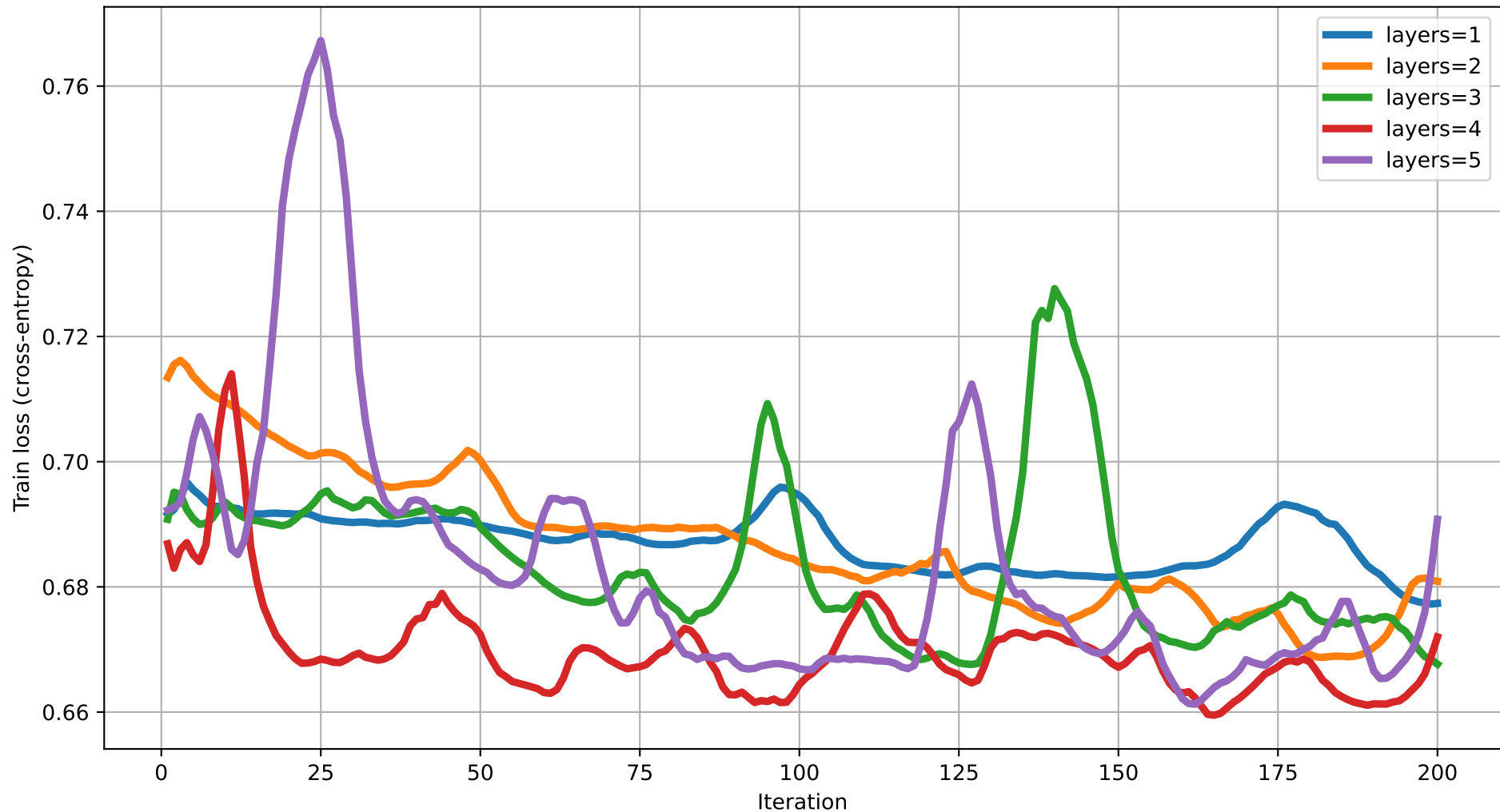
Train loss vs Iteration (dim=13) rot=RYZ, ent=full, gate=IsingXX
