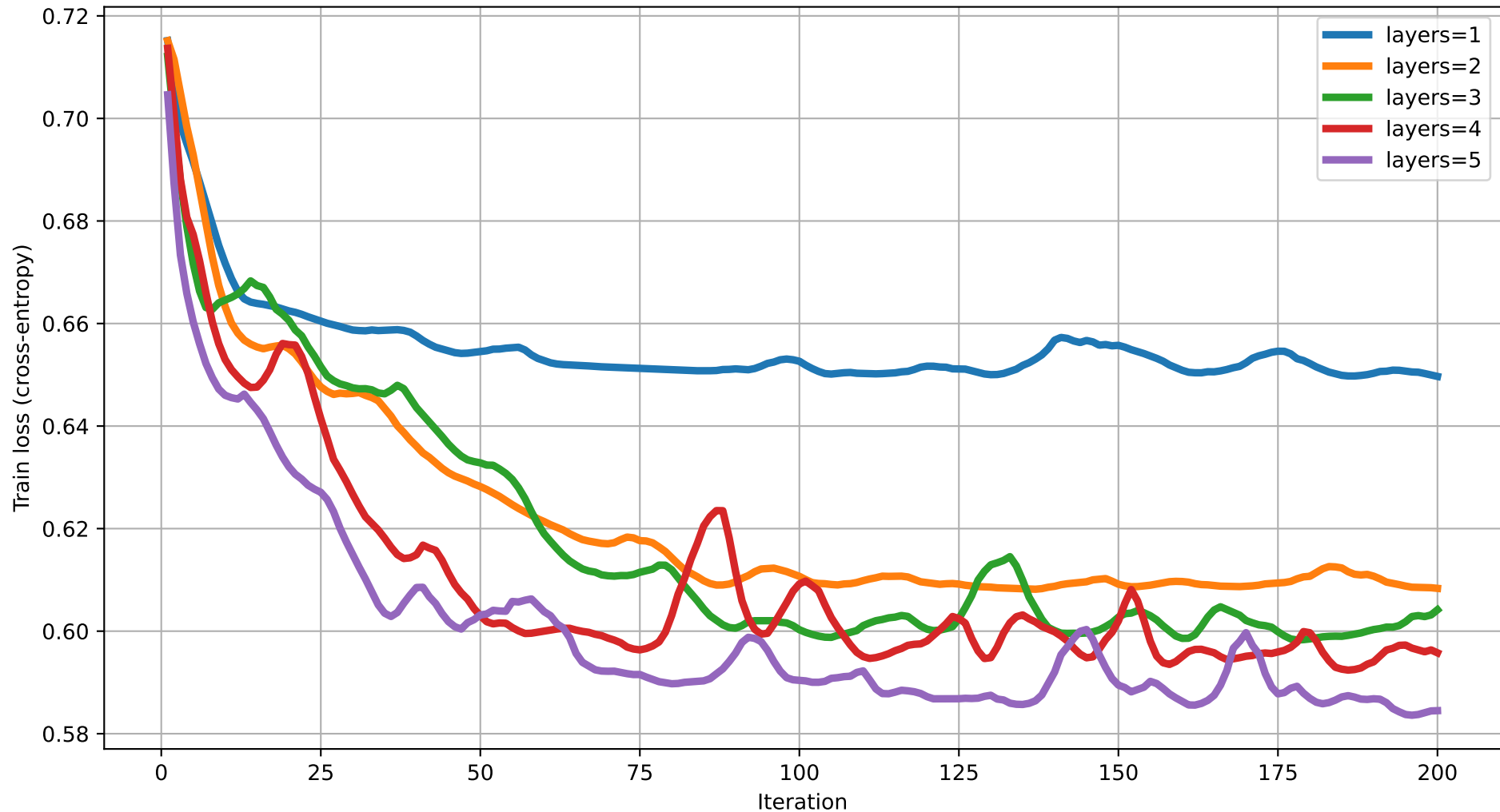
Train loss vs Iteration (degree=4) rot=RYZ, ent=ring, gate=CZ
