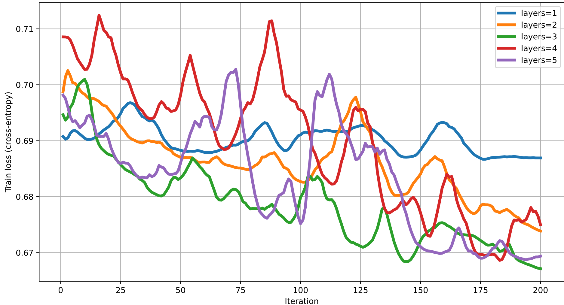
Train loss vs Iteration (dim=20) rot=RY, ent=ring, gate=CNOT
