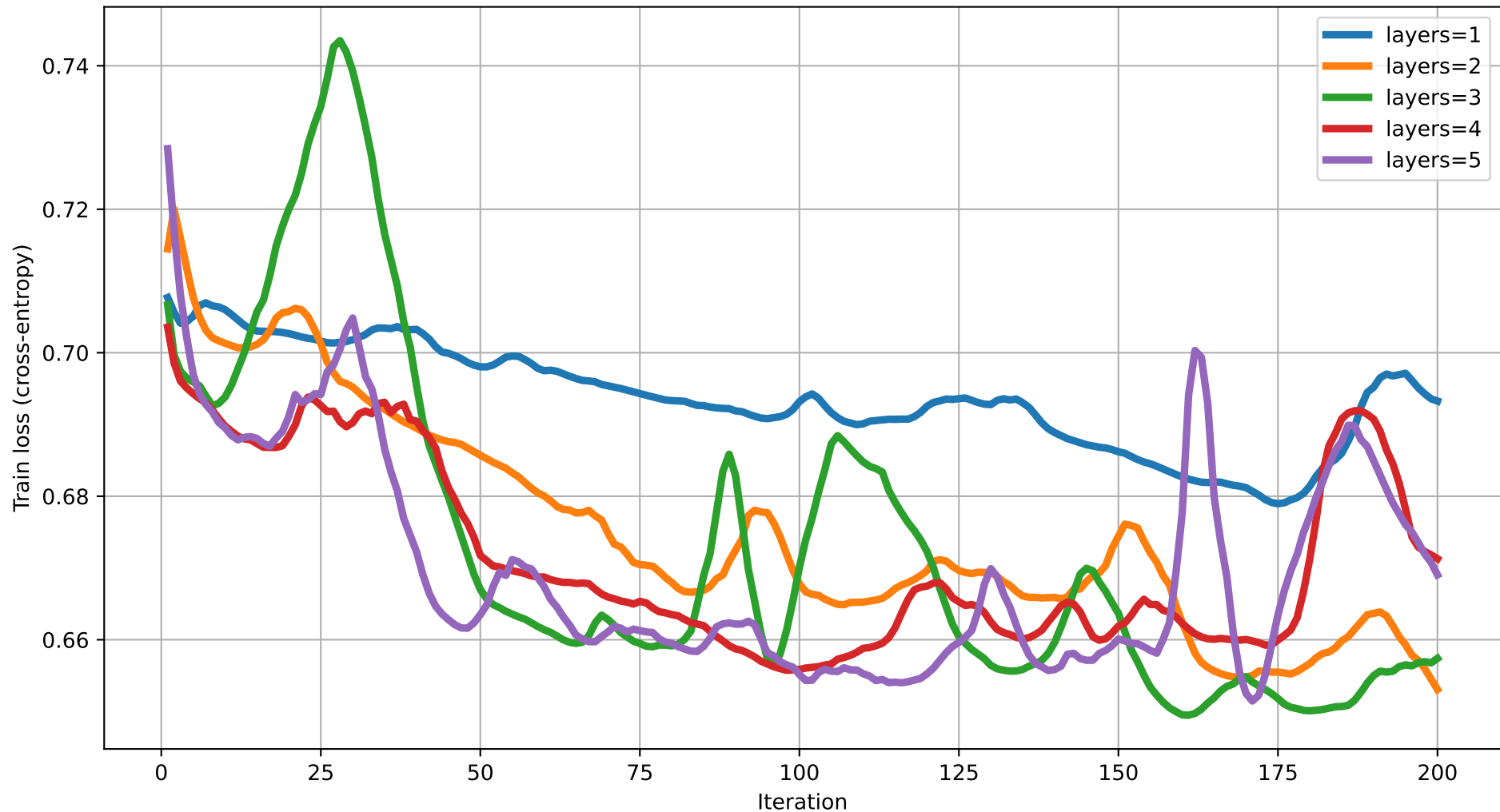
Train loss vs Iteration (dim=6) rot=RYZ, ent=pairwise, gate=CZ
