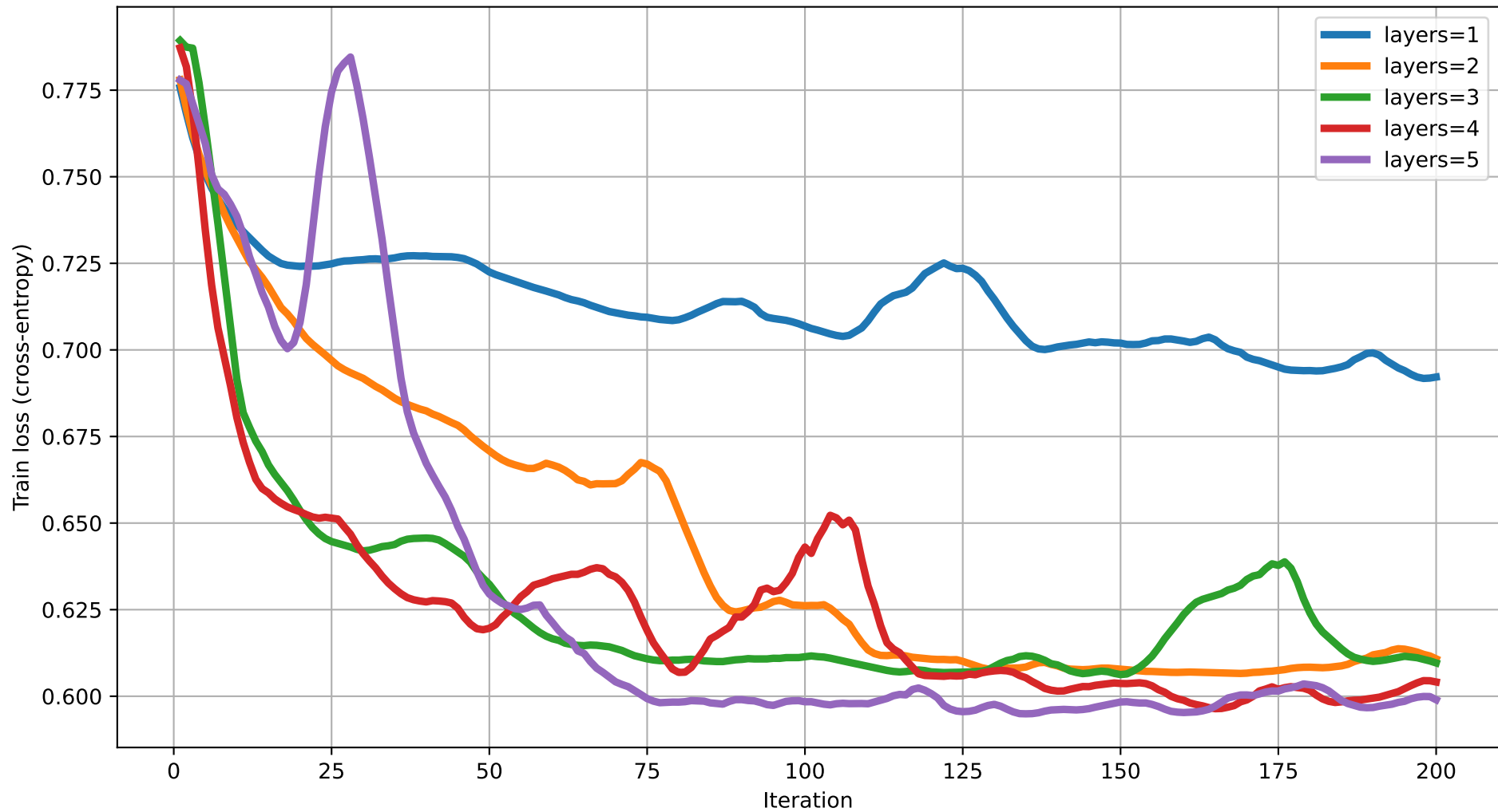
Train loss vs Iteration (dim=9) rot=RY, ent=chain, gate=CZ
