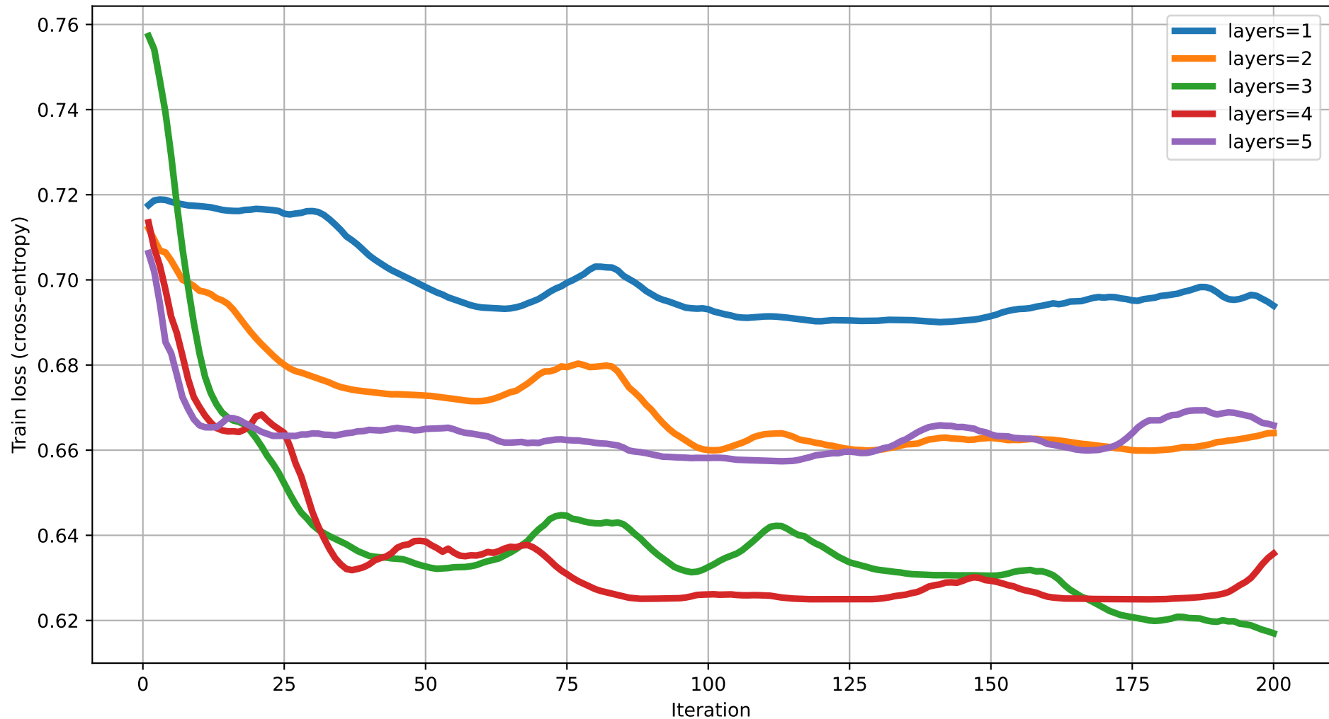
Train loss vs Iteration (dim=10) rot=RX, ent=ring, gate=CNOT
