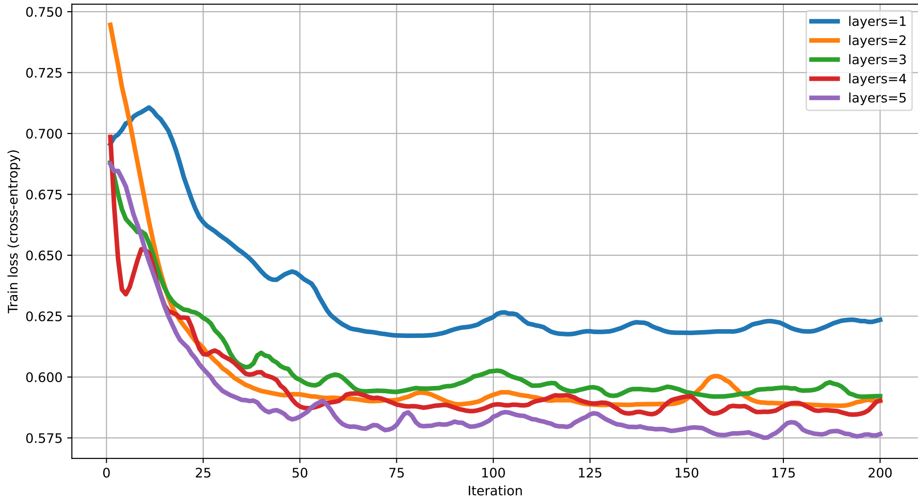
Train loss vs Iteration (degree=4) rot=RYZ, ent=chain, gate=IsingXX
