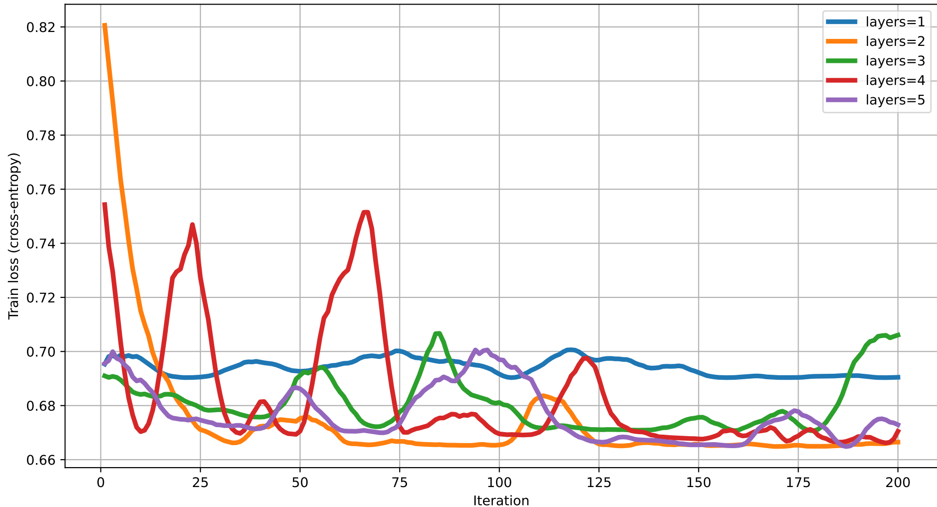
Train loss vs Iteration (dim=8) rot=RY, ent=chain, gate=IsingXX
