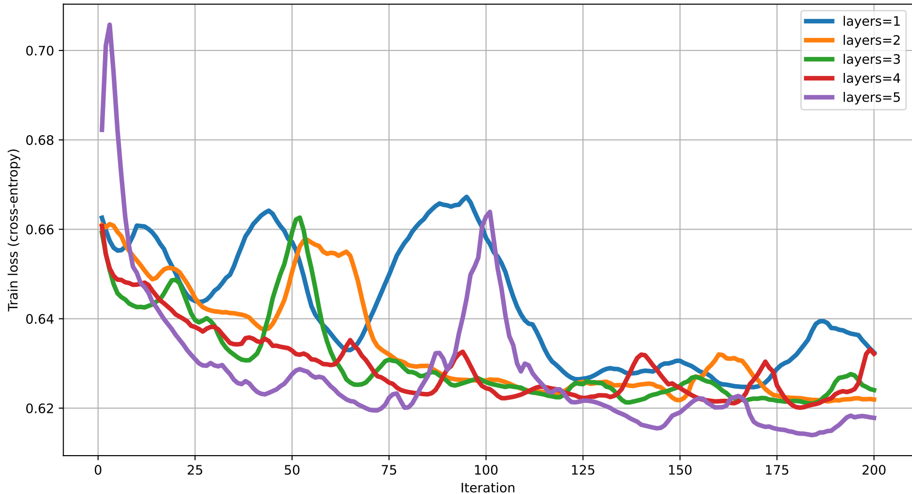
Train loss vs Iteration (dim=15) rot=Rot, ent=chain, gate=CZ
