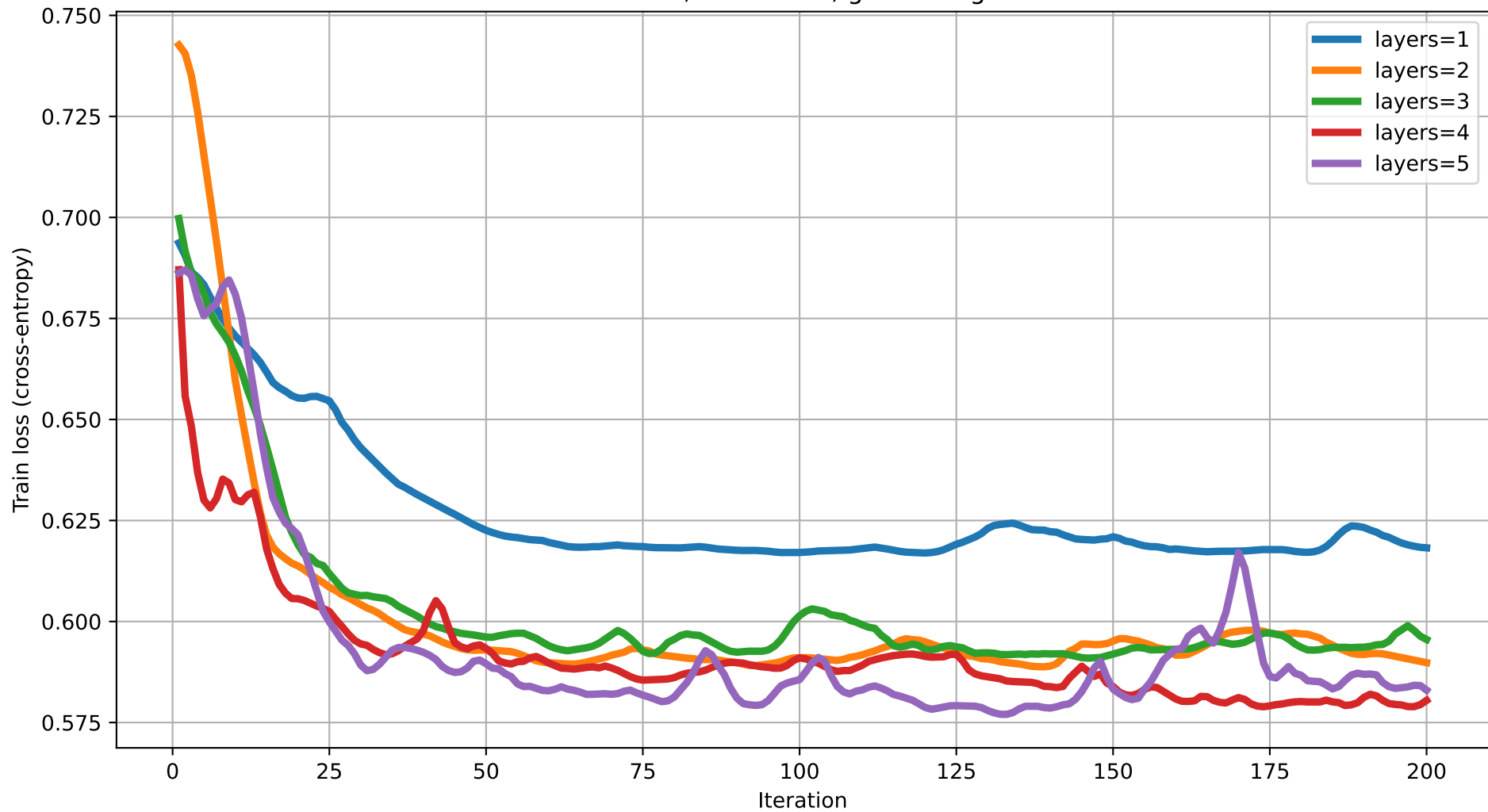
Train loss vs Iteration (degree=4) rot=Rot, ent=chain, gate=IsingXX
