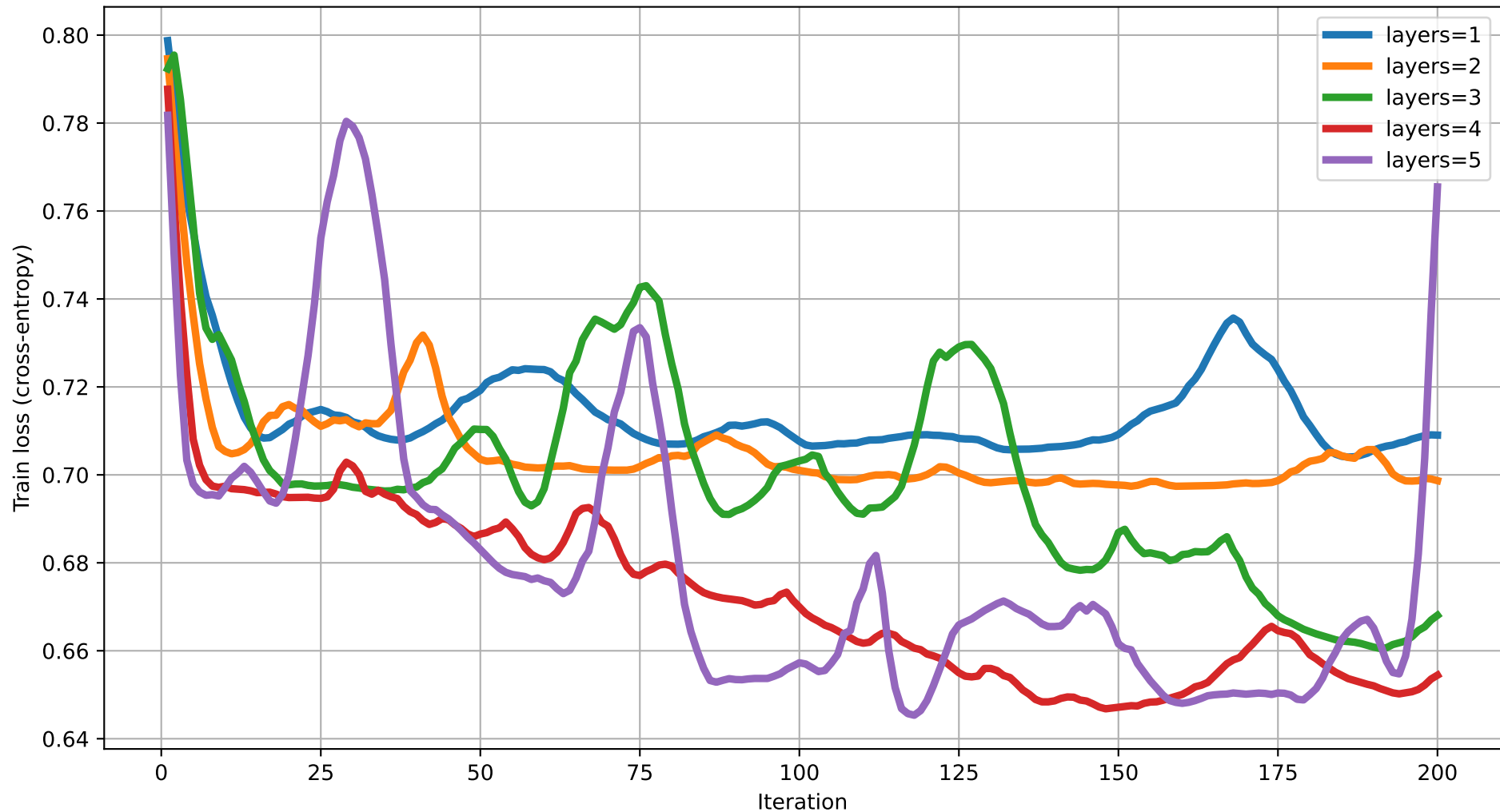
Train loss vs Iteration (dim=8) rot=RYZ, ent=chain, gate=CNOT
