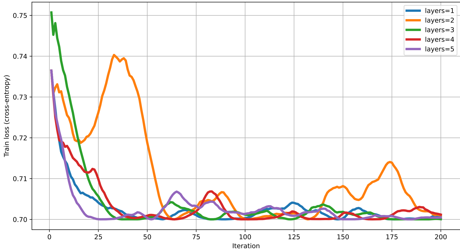
Train loss vs Iteration (dim=19) rot=RZ, ent=pairwise, gate=CNOT
