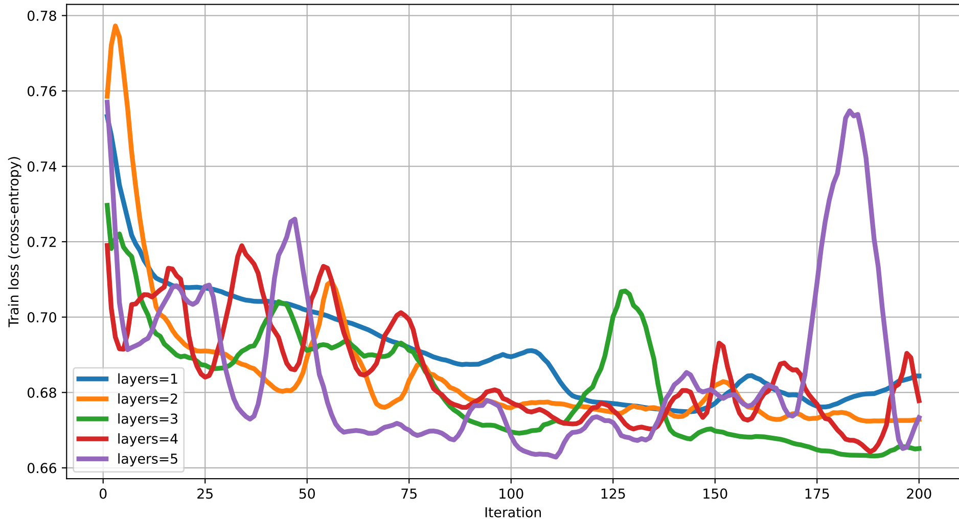
Train loss vs Iteration (dim=19) rot=RY, ent=full, gate=IsingXX
