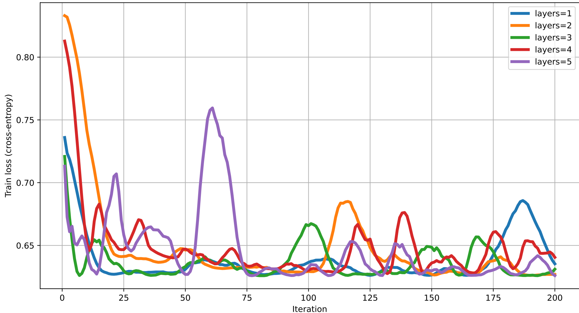
Train loss vs Iteration (dim=2) rot=Rot, ent=ring, gate=IsingXX
