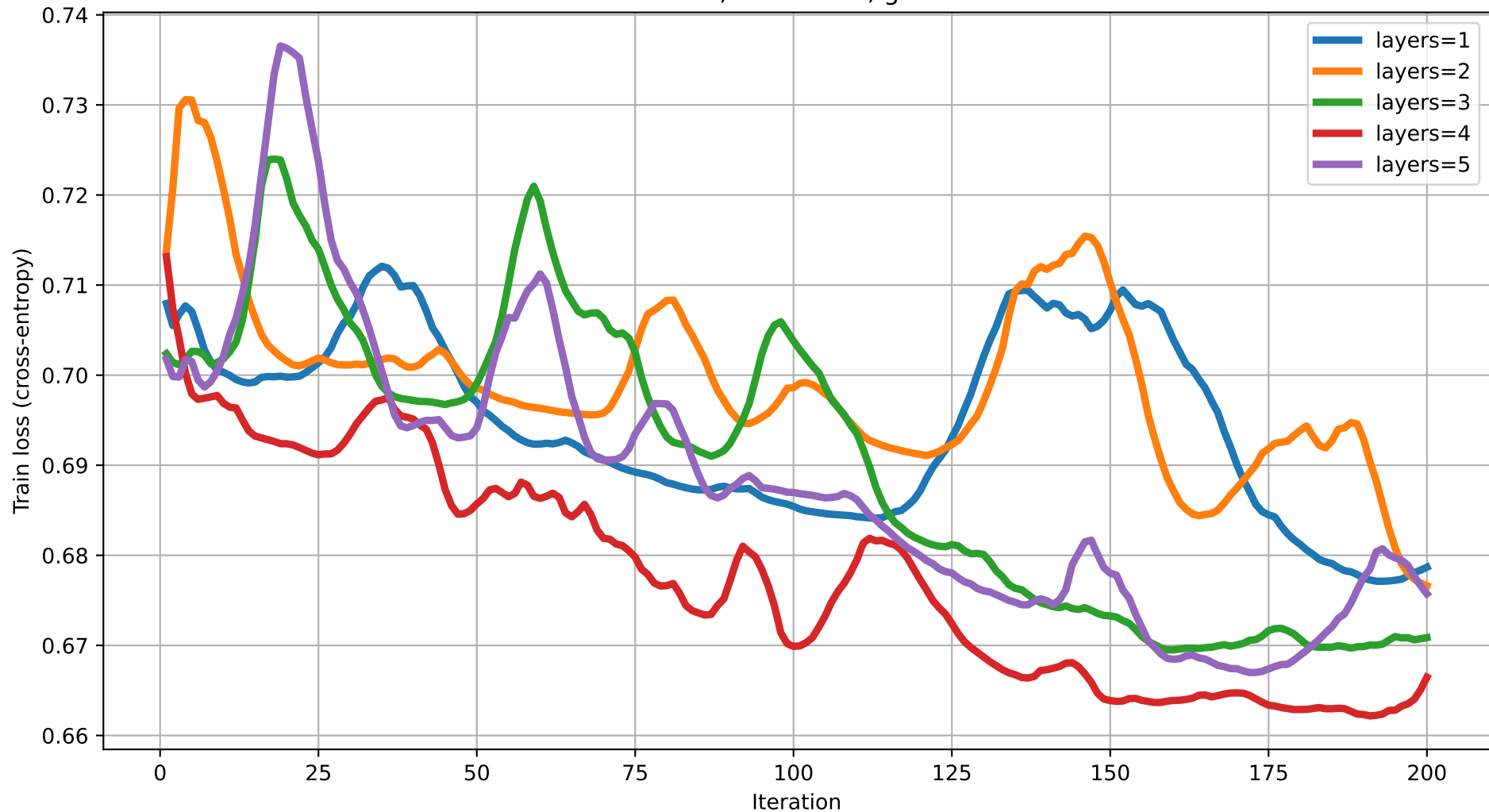
Train loss vs Iteration (dim=14) rot=RYZ, ent=chain, gate=CZ
