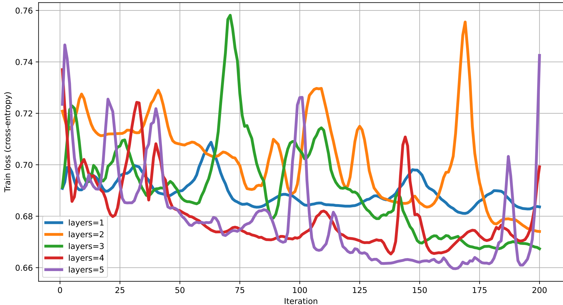
Train loss vs Iteration (dim=13) rot=Rot, ent=pairwise, gate=IsingXX
