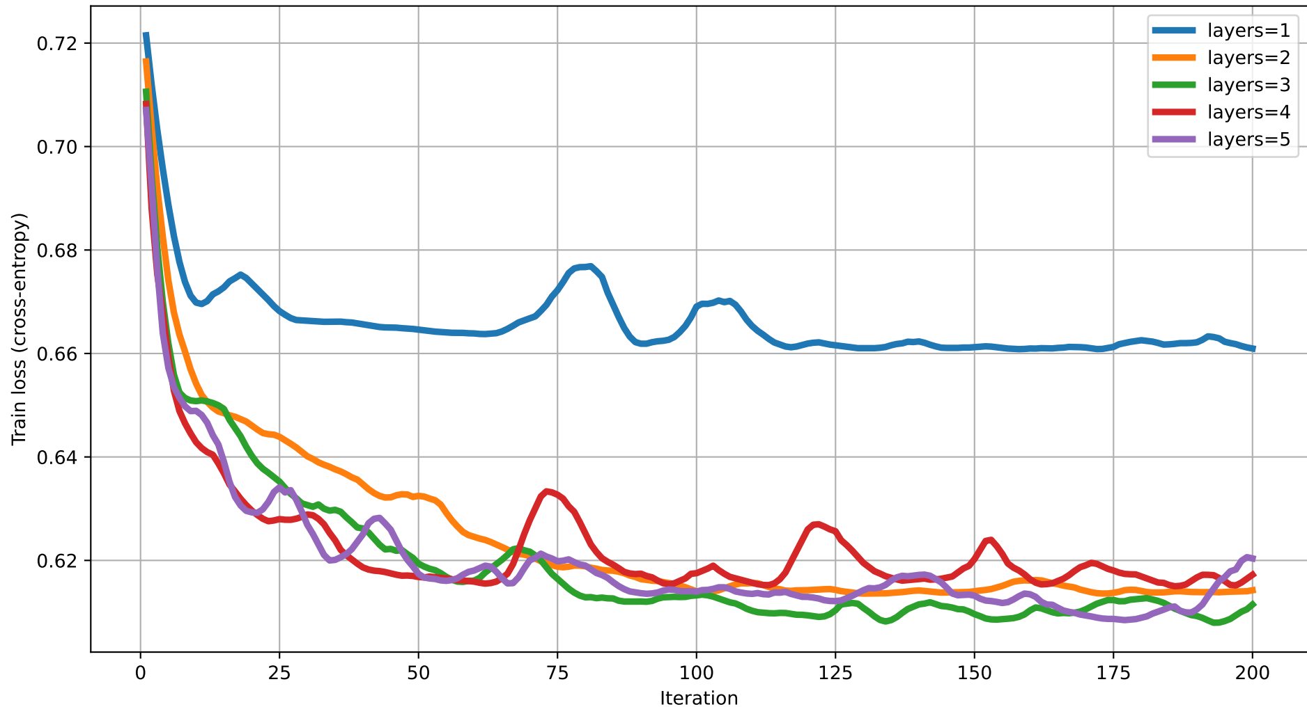
Train loss vs Iteration (degree=3) rot=RY, ent=chain, gate=CZ
