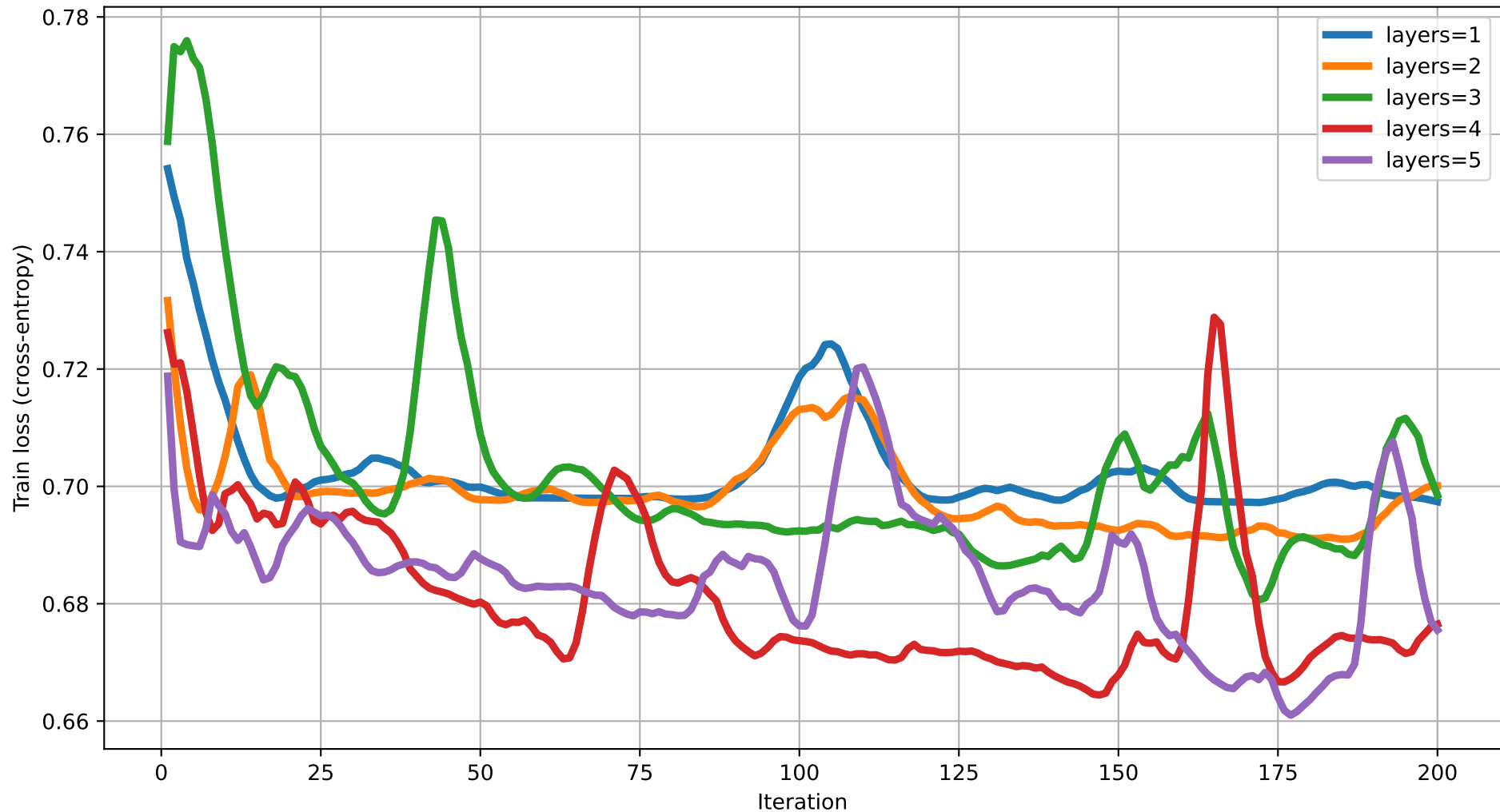
Train loss vs Iteration (dim=19) rot=Rot, ent=full, gate=CNOT
