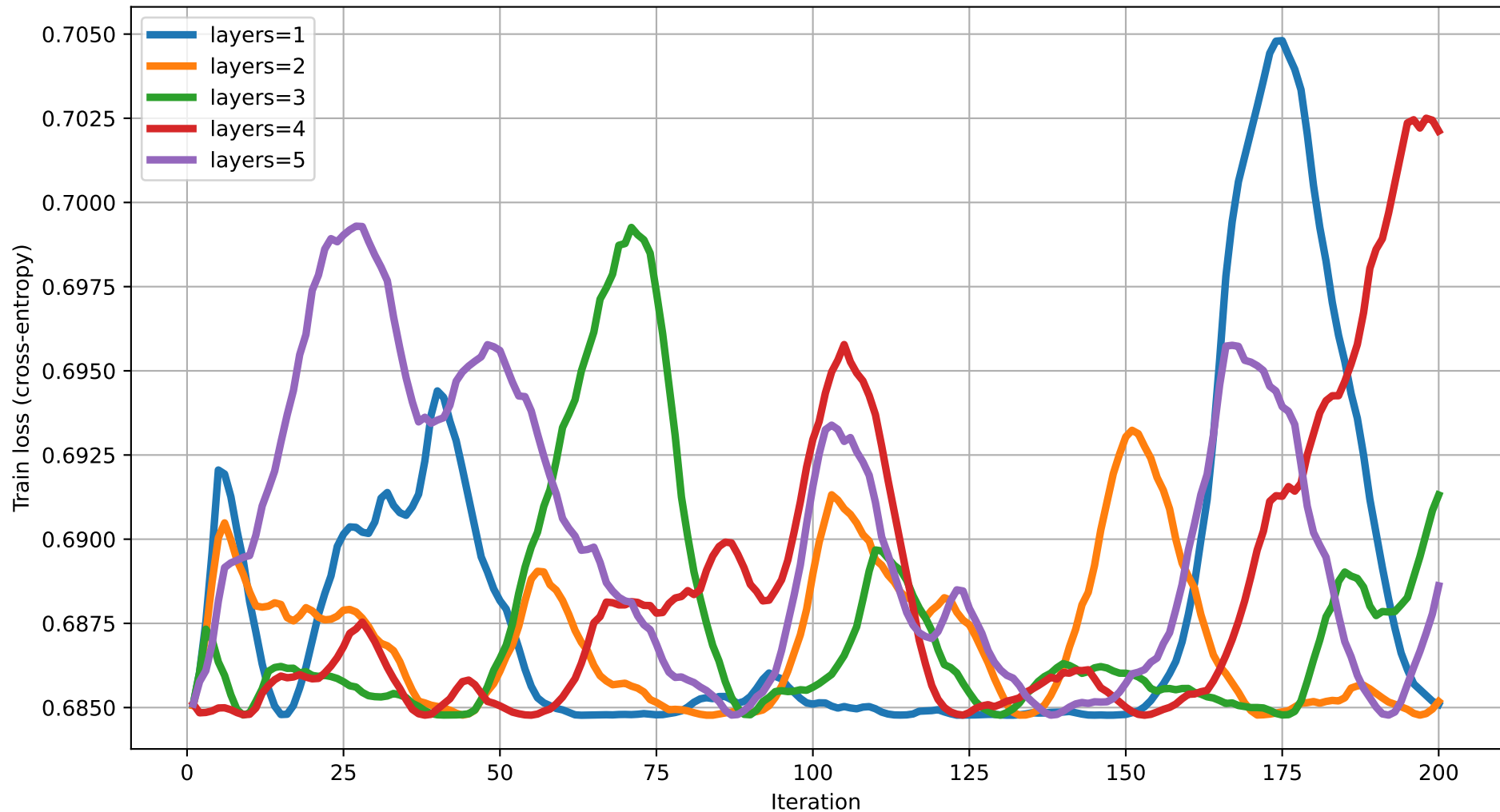
Train loss vs Iteration (dim=15) rot=RZ, ent=chain, gate=CNOT
