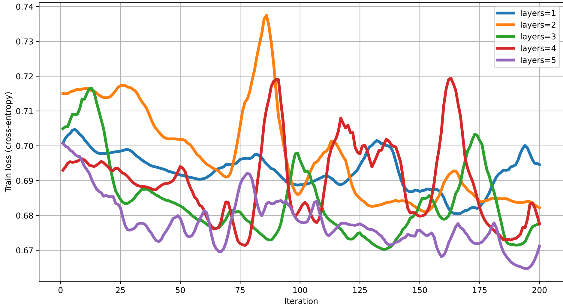
Train loss vs Iteration (dim=17) rot=RYZ, ent=ring, gate=CNOT
