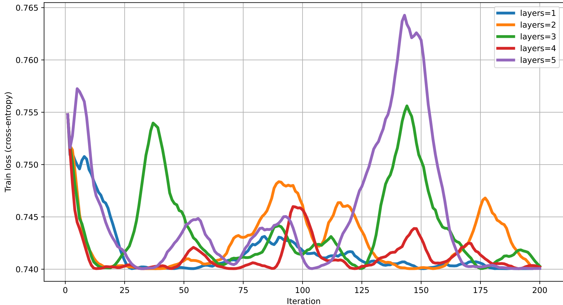
Train loss vs Iteration (dim=5) rot=RZ, ent=full, gate=CZ
