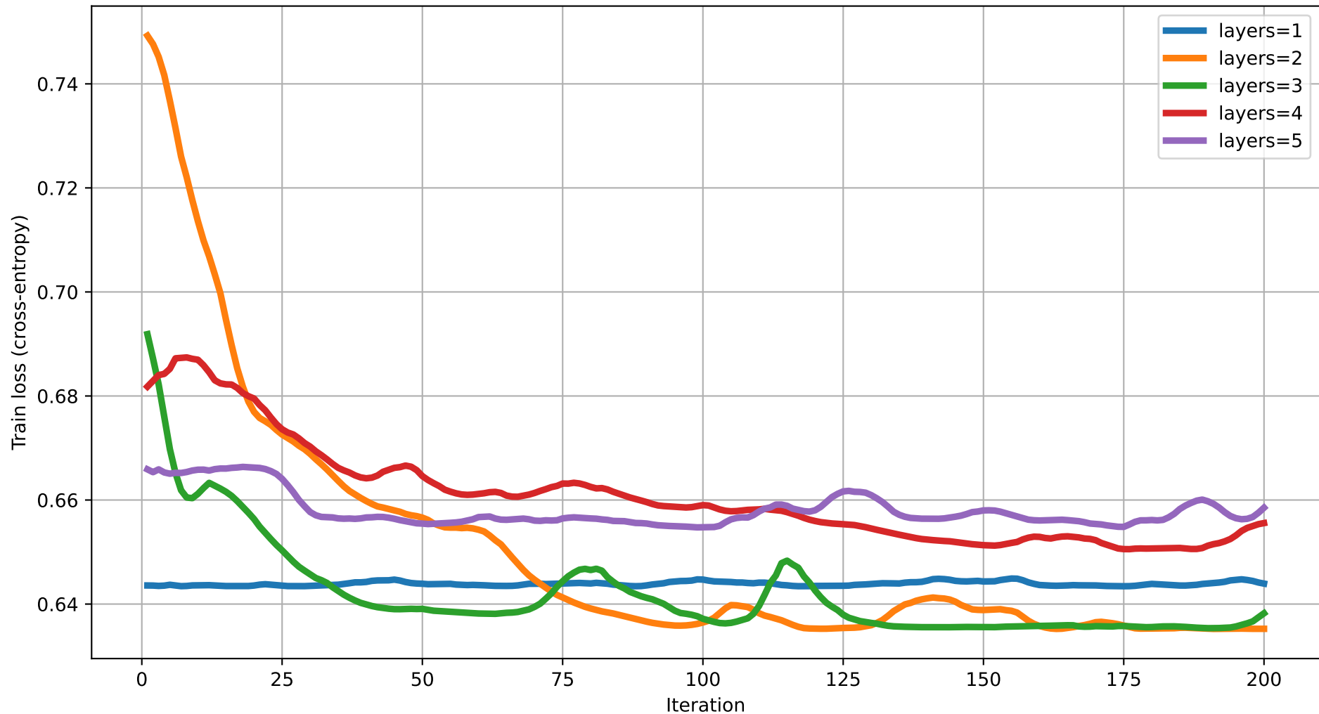
Train loss vs Iteration (degree=3) rot=RX, ent=ring, gate=CNOT
