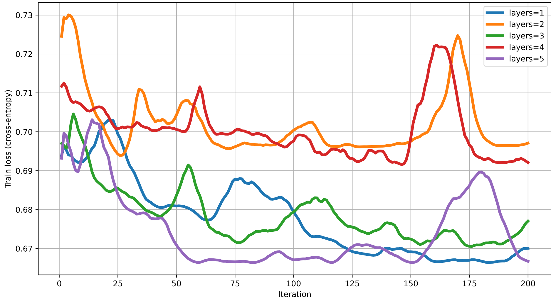
Train loss vs Iteration (dim=11) rot=RX, ent=full, gate=IsingXX
