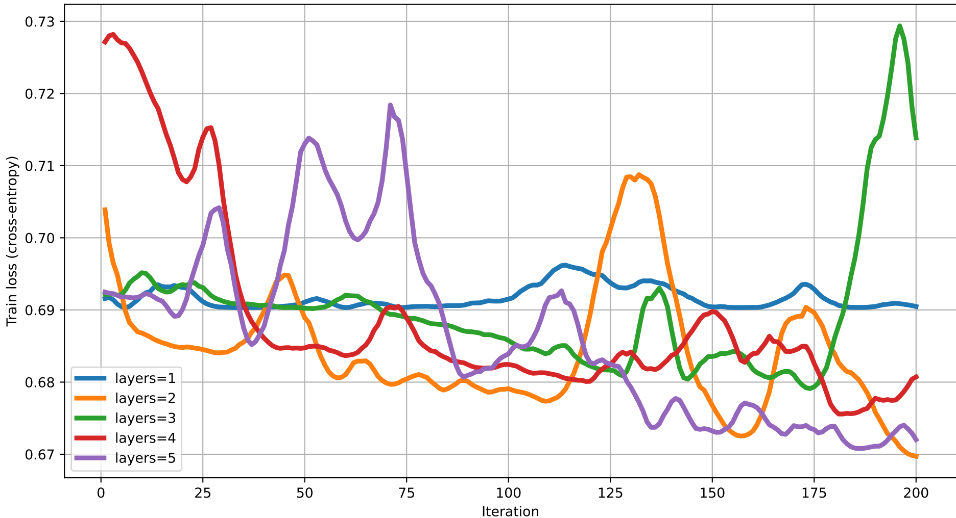
Train loss vs Iteration (dim=7) rot=RY, ent=pairwise, gate=IsingXX
