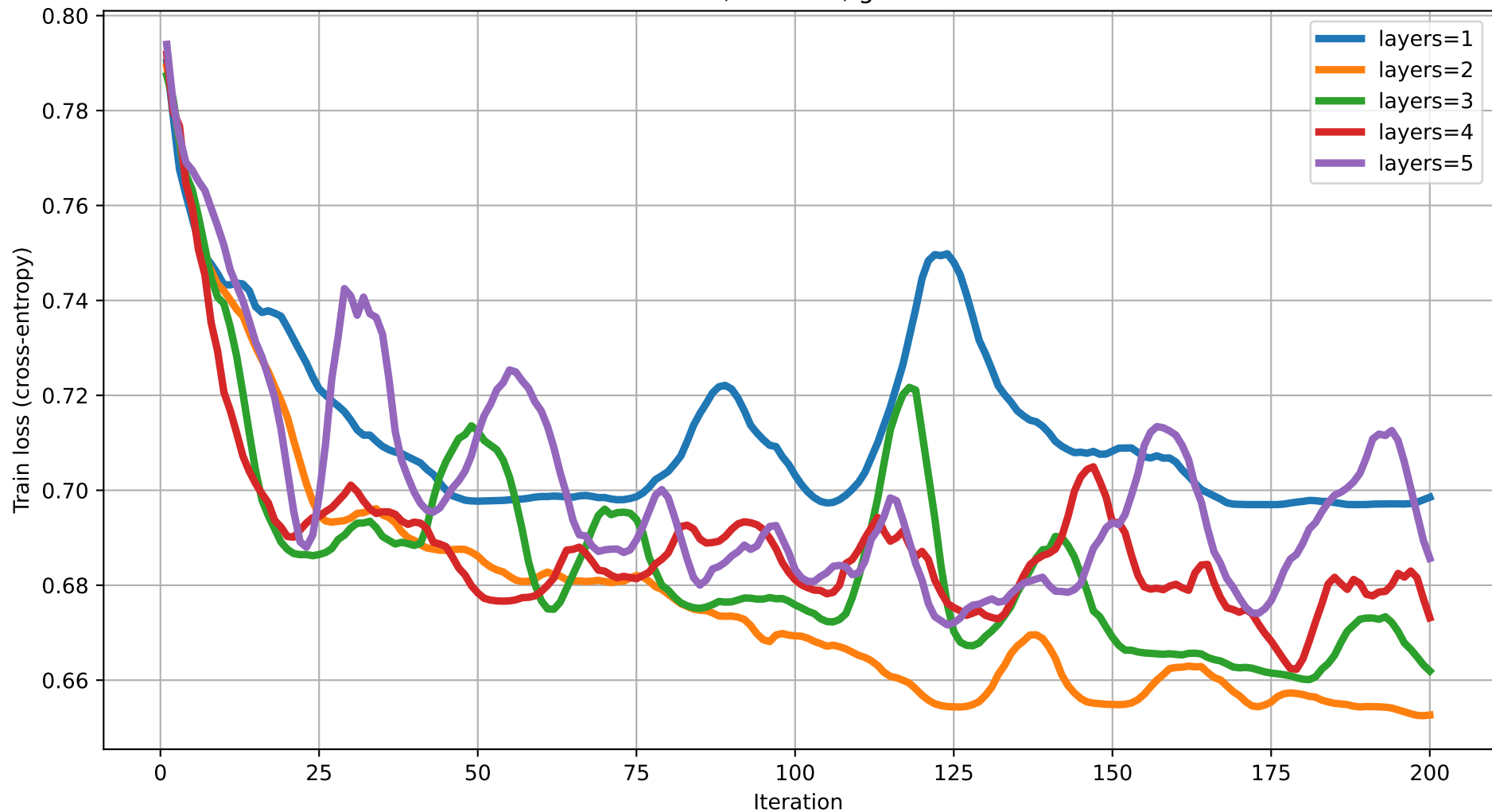
Train loss vs Iteration (dim=2) rot=Rot, ent=full, gate=CZ
