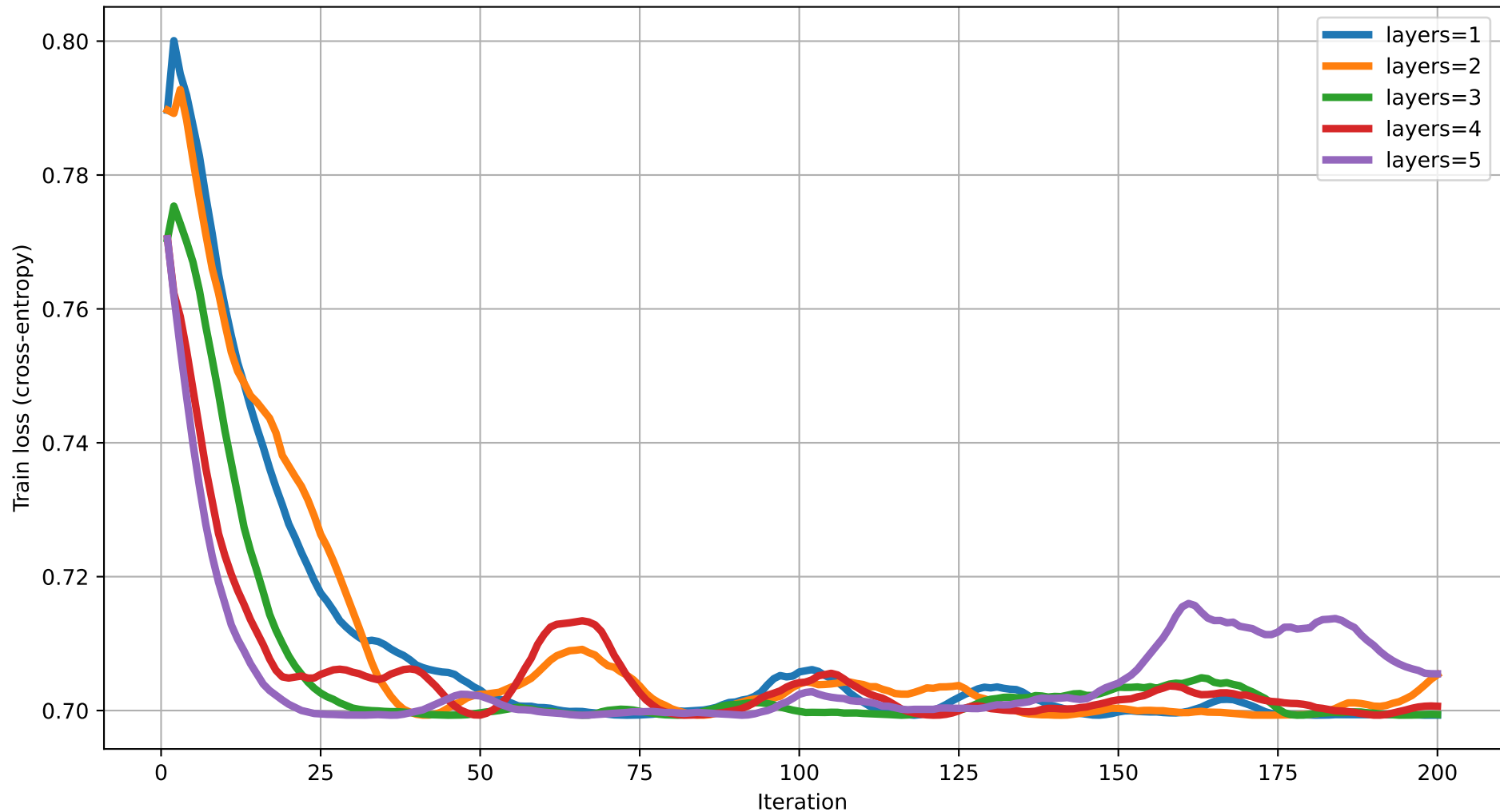
Train loss vs Iteration (dim=17) rot=RZ, ent=ring, gate=CZ
