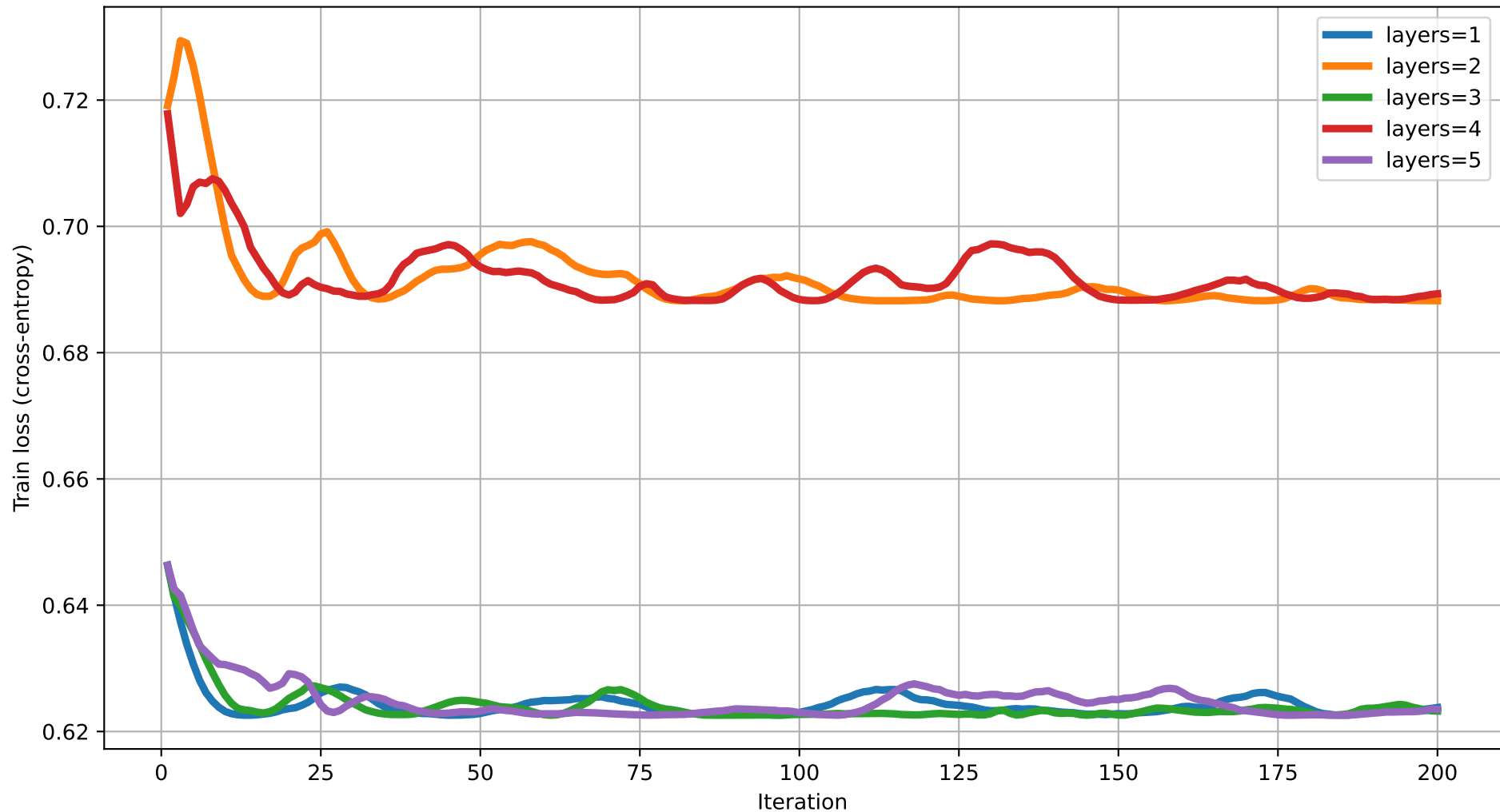
Train loss vs Iteration (degree=4) rot=RX, ent=ring, gate=IsingXX
