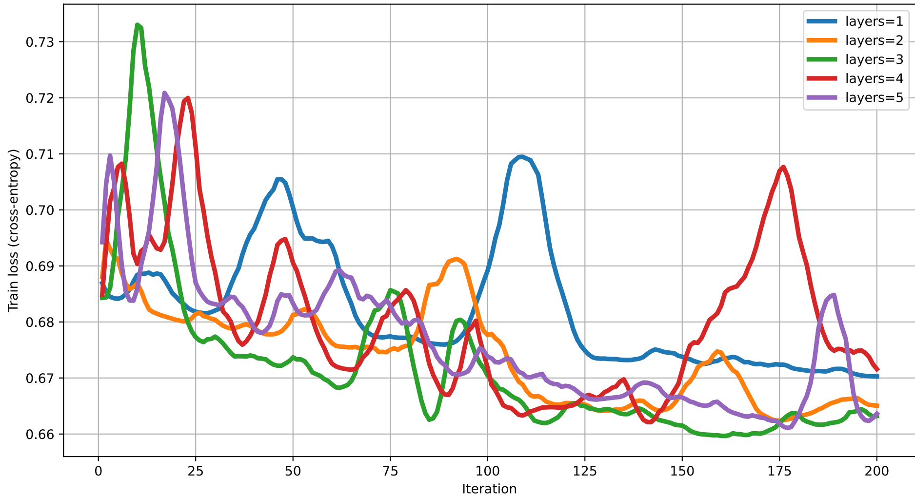
Train loss vs Iteration (dim=15) rot=RYZ, ent=full, gate=CNOT
