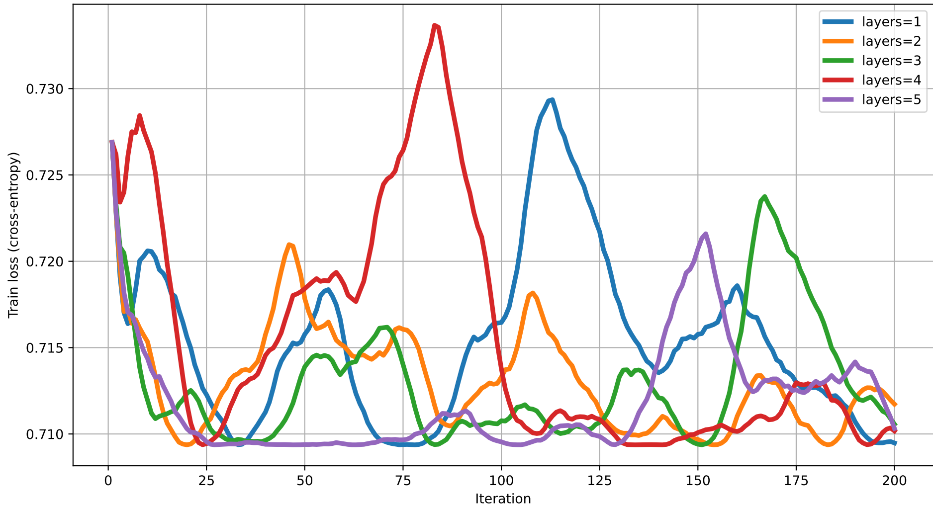
Train loss vs Iteration (dim=5) rot=RZ, ent=pairwise, gate=CNOT
