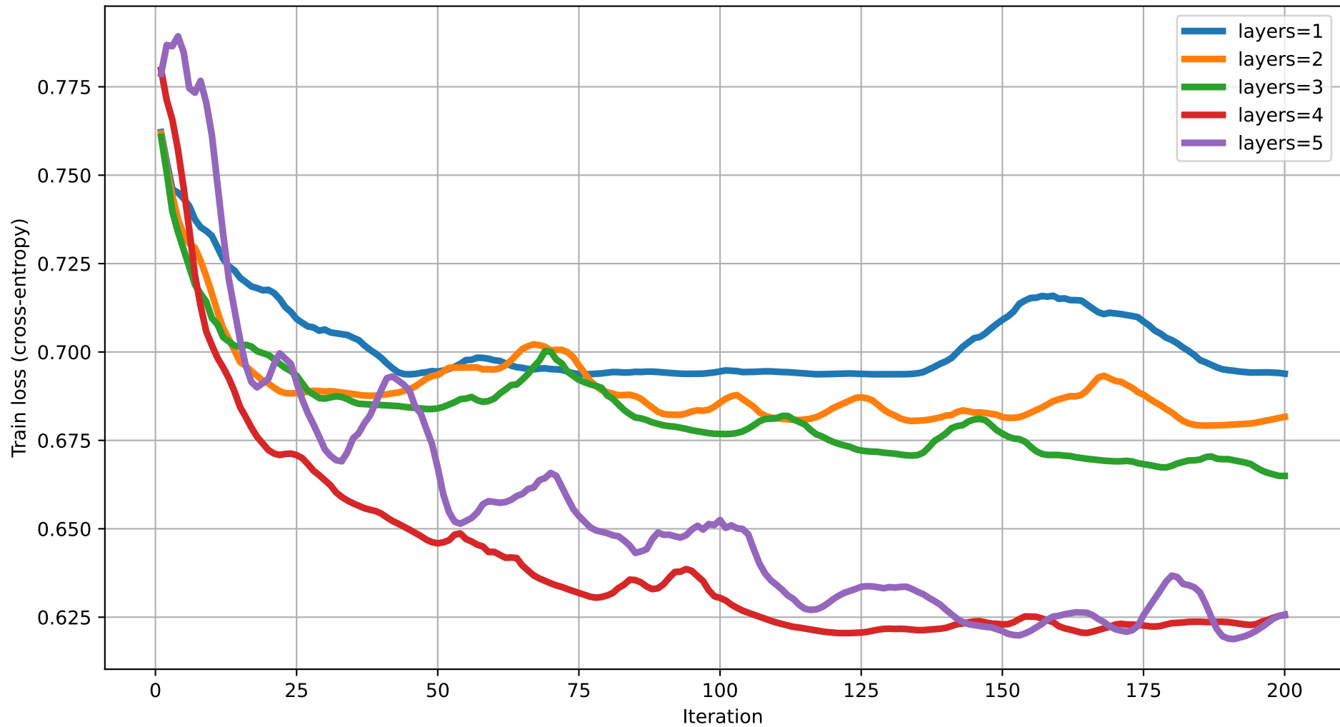
Train loss vs Iteration (dim=8) rot=RX, ent=ring, gate=CZ
