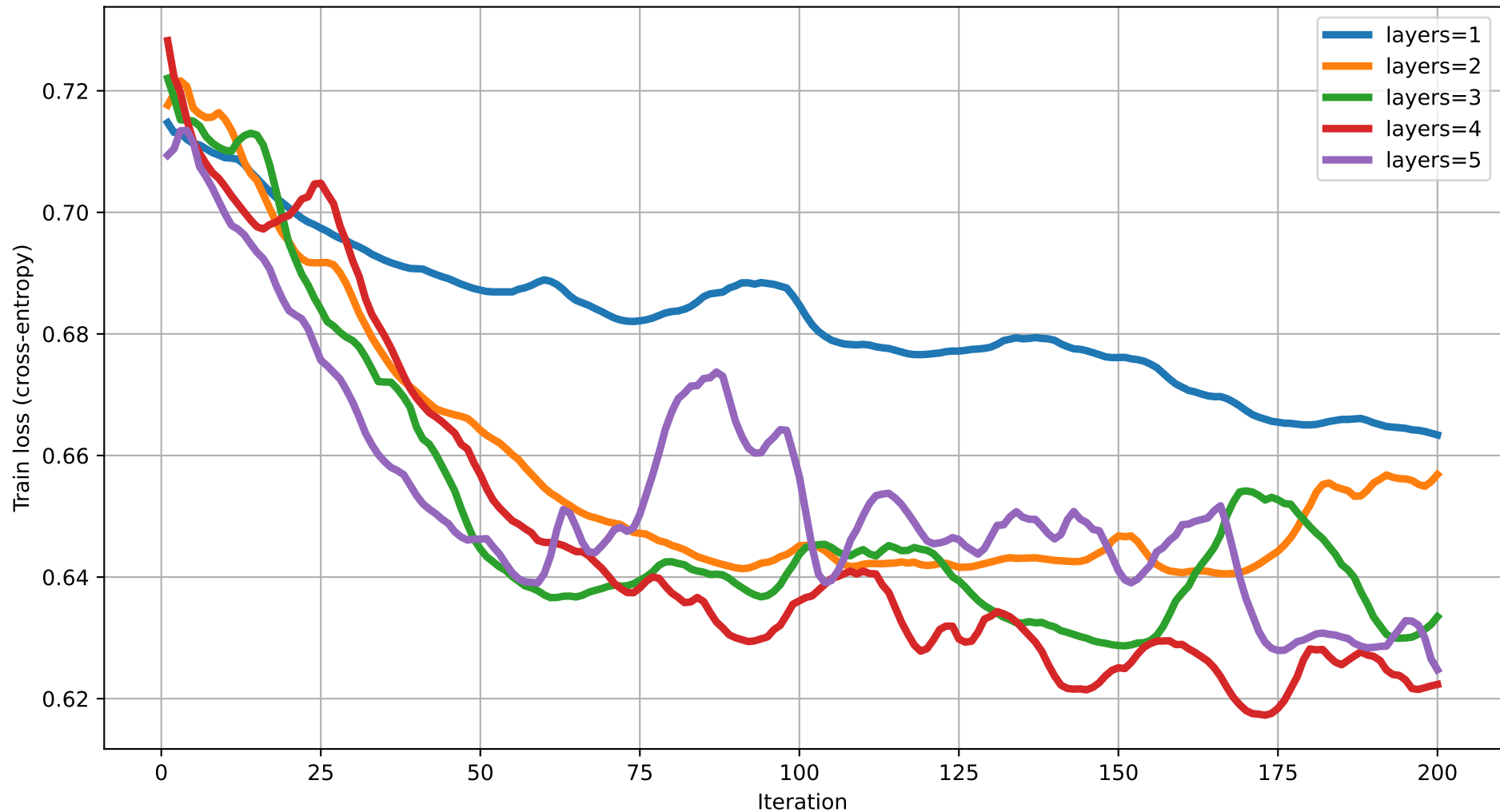
Train loss vs Iteration (dim=7) rot=RYZ, ent=full, gate=CNOT
