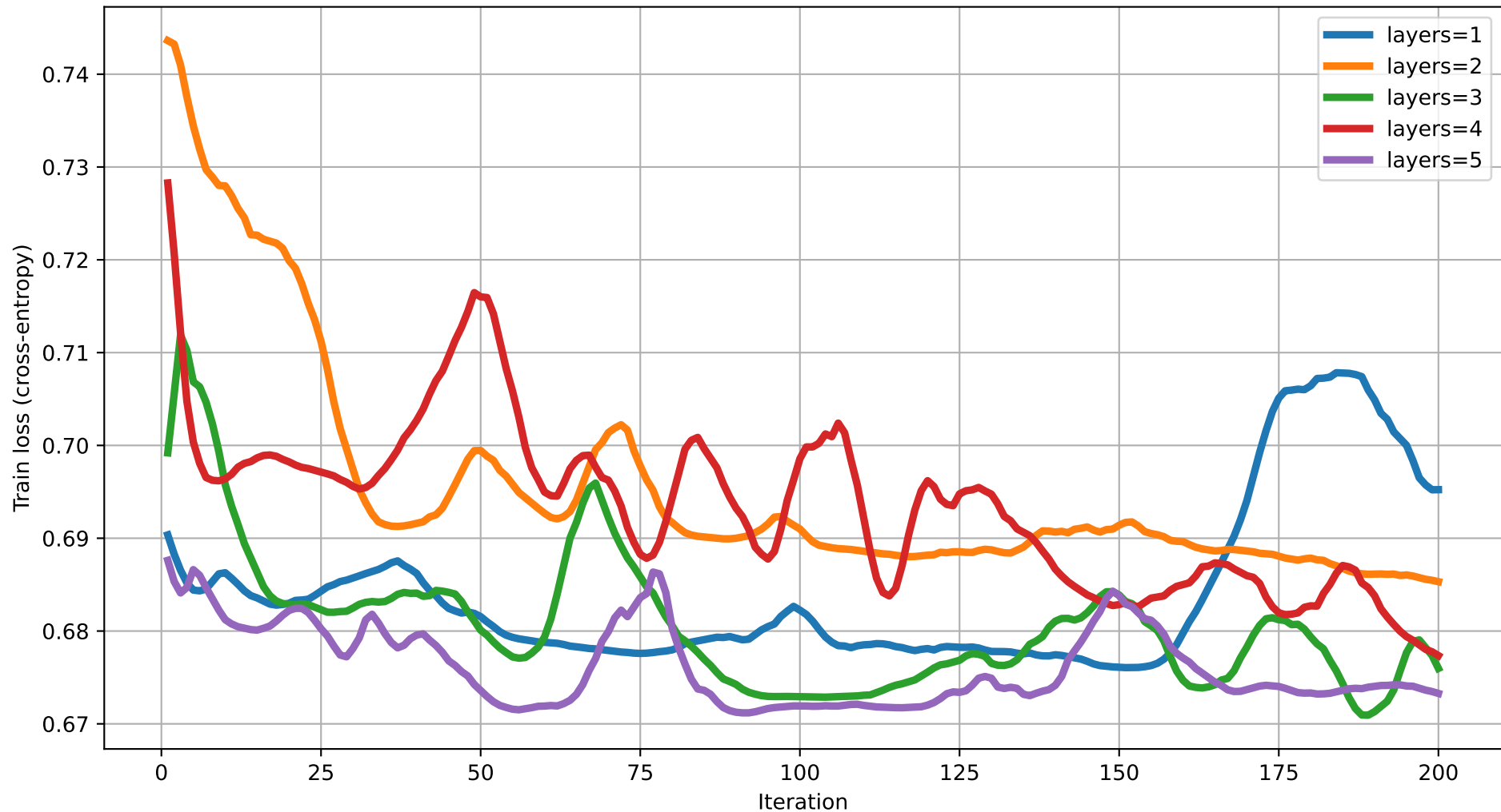
Train loss vs Iteration (dim=5) rot=RZ, ent=chain, gate=IsingXX
