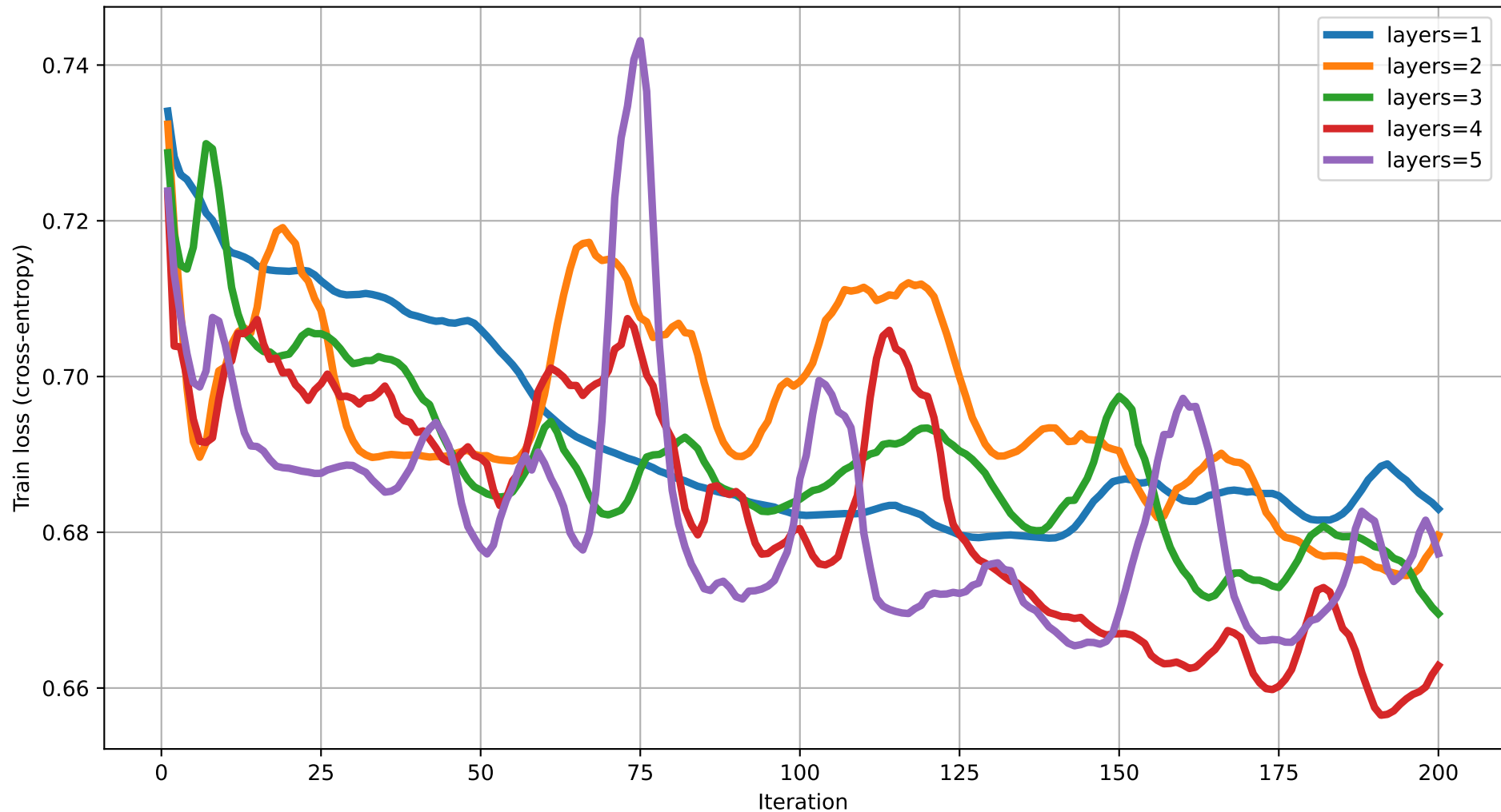
Train loss vs Iteration (dim=16) rot=RYZ, ent=full, gate=IsingXX
