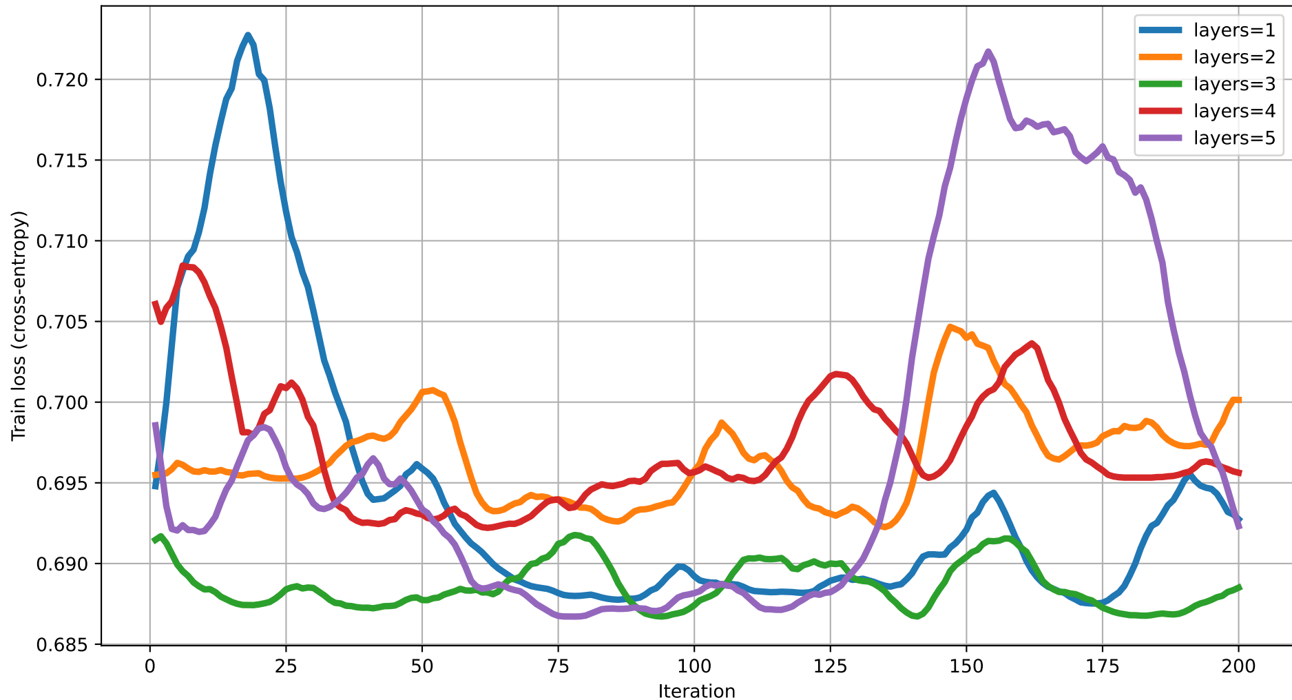
Train loss vs Iteration (dim=14) rot=RX, ent=full, gate=IsingXX
