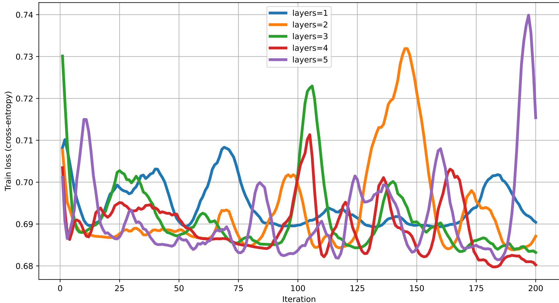
Train loss vs Iteration (dim=20) rot=RY, ent=chain, gate=CZ
