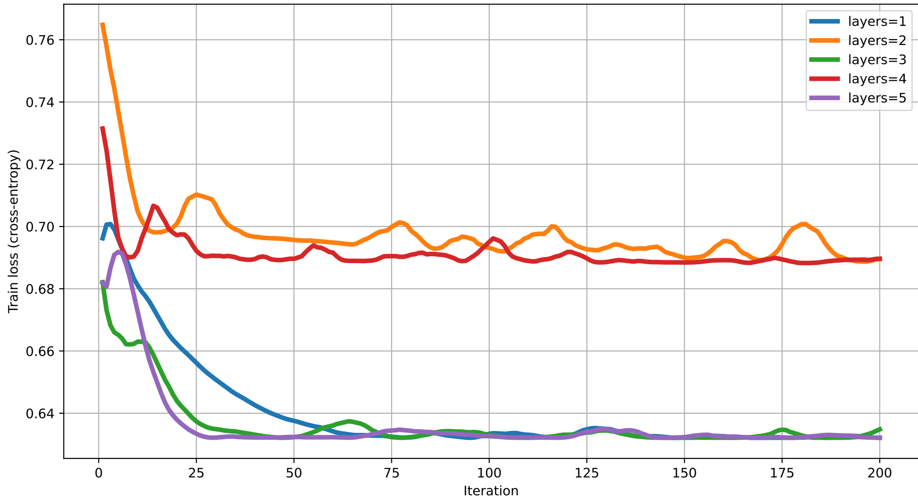
Train loss vs Iteration (degree=4) rot=RX, ent=full, gate=IsingXX
