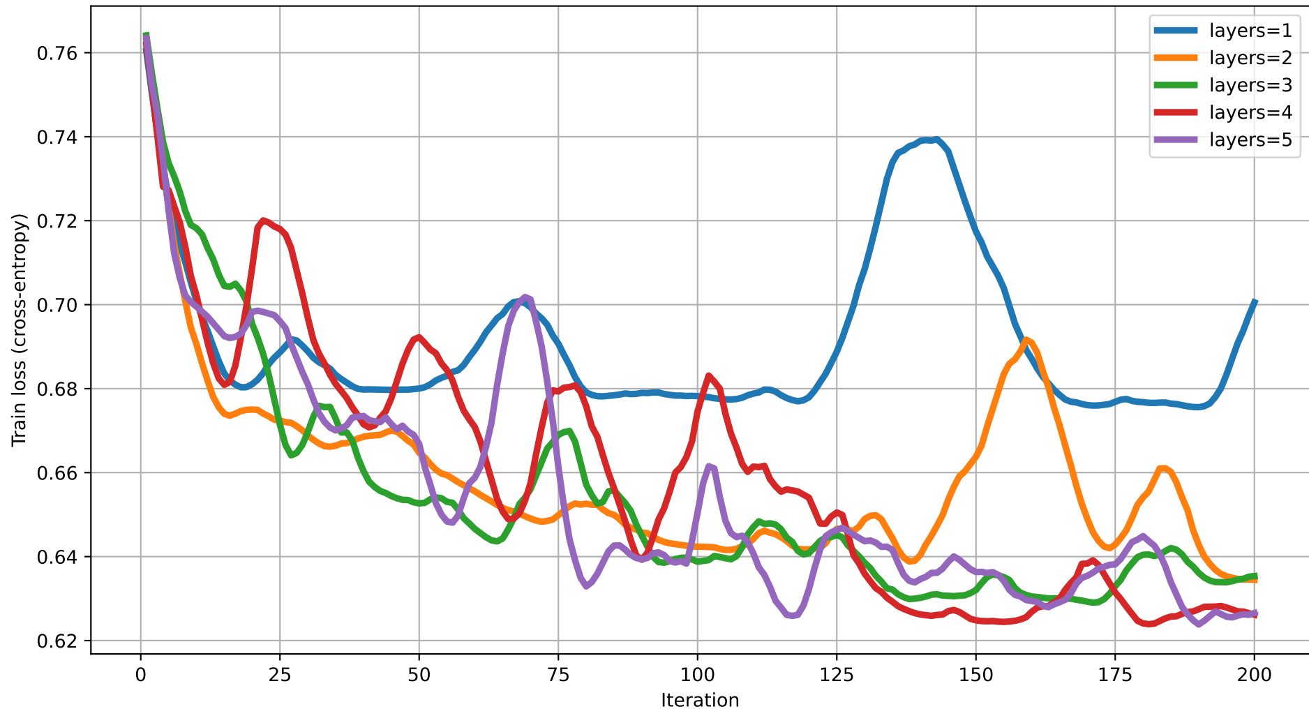
Train loss vs Iteration (dim=8) rot=RYZ, ent=chain, gate=CZ
