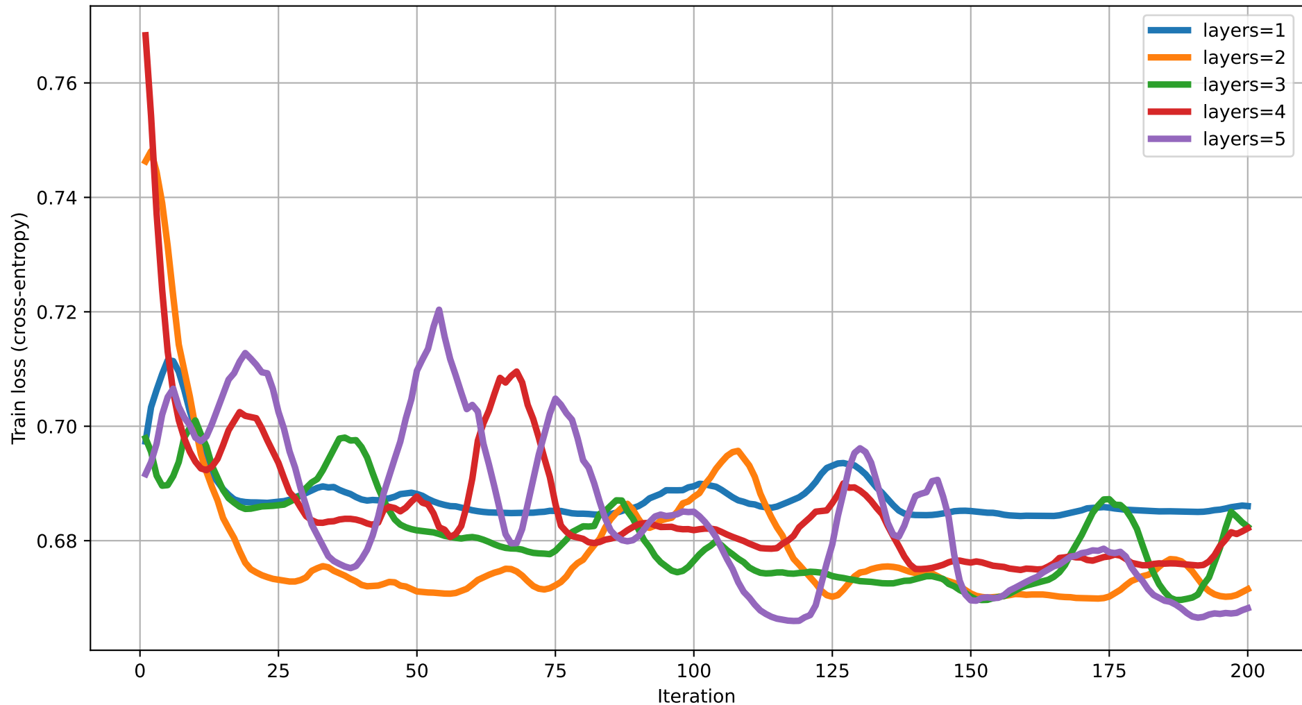
Train loss vs Iteration (dim=9) rot=RZ, ent=full, gate=IsingXX
