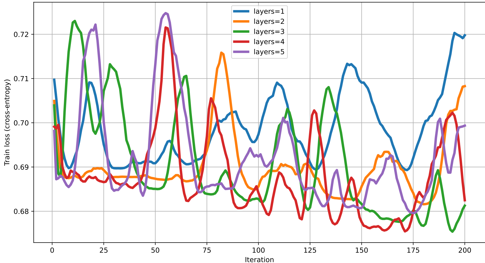
Train loss vs Iteration (dim=20) rot=RY, ent=pairwise, gate=CNOT
