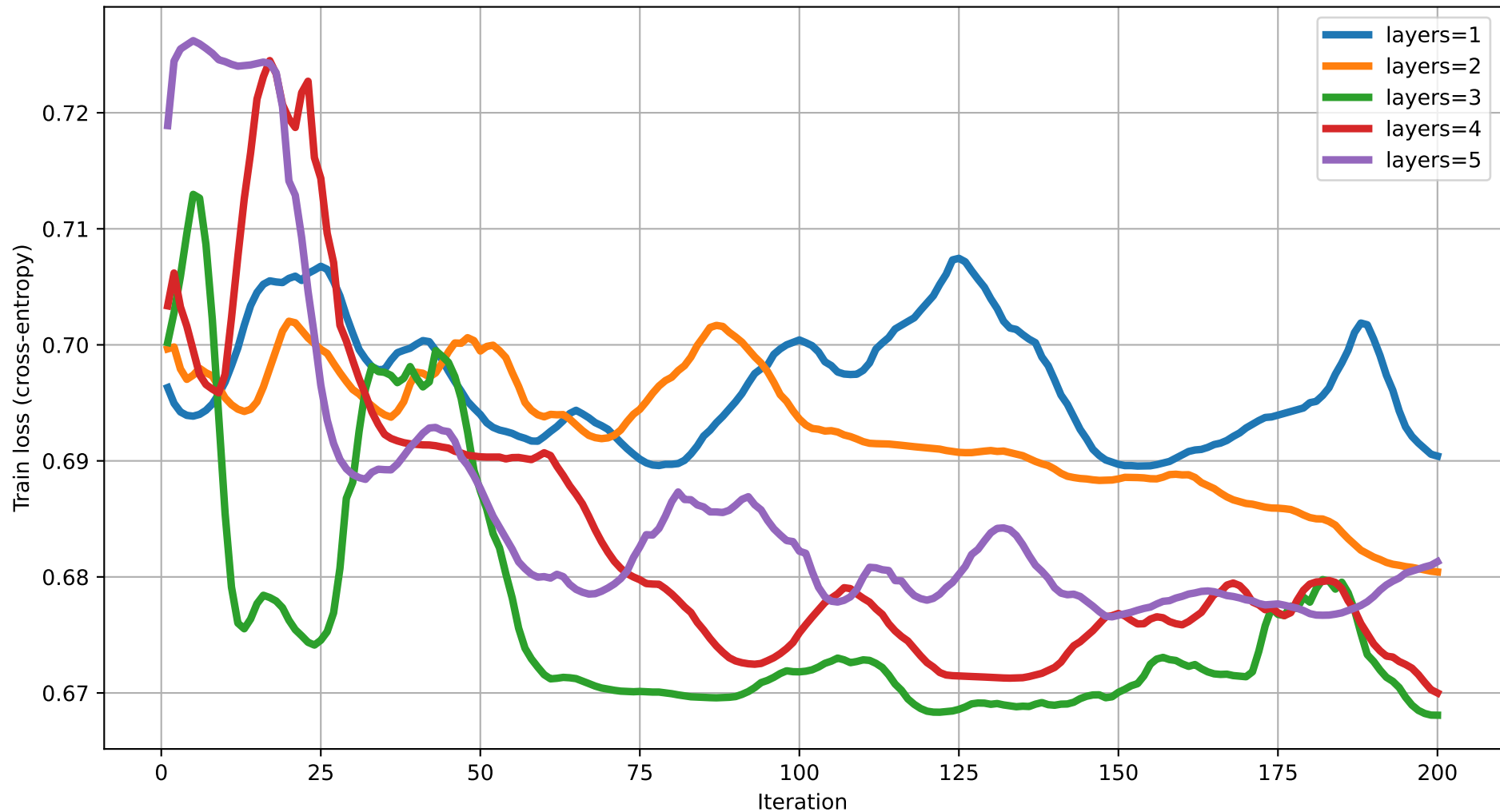
Train loss vs Iteration (dim=11) rot=RX, ent=ring, gate=CNOT
