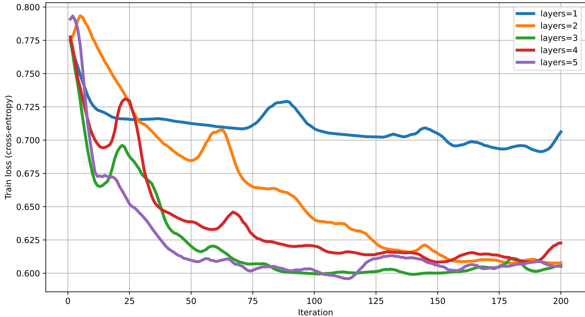
Train loss vs Iteration (dim=9) rot=RY, ent=chain, gate=CNOT
