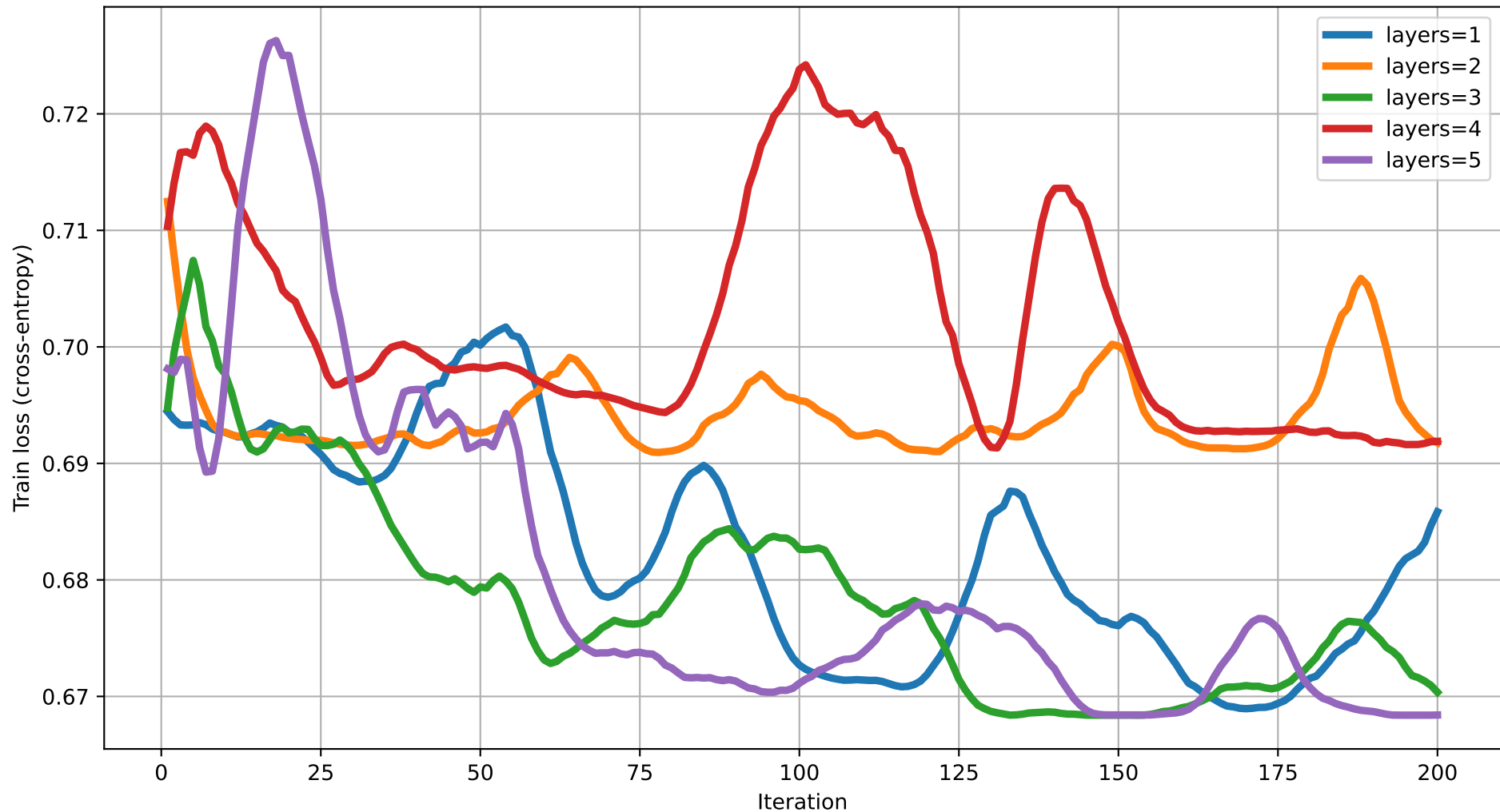
Train loss vs Iteration (dim=12) rot=RX, ent=pairwise, gate=IsingXX
