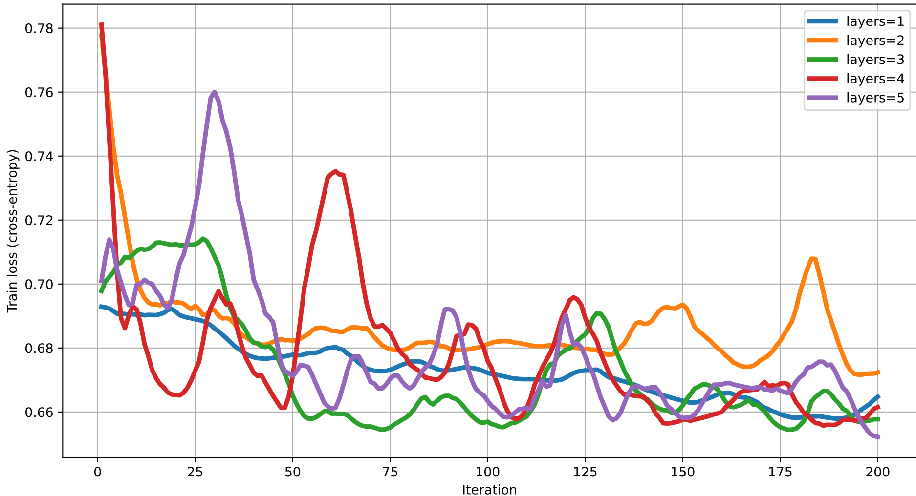
Train loss vs Iteration (dim=2) rot=RYZ, ent=chain, gate=IsingXX
