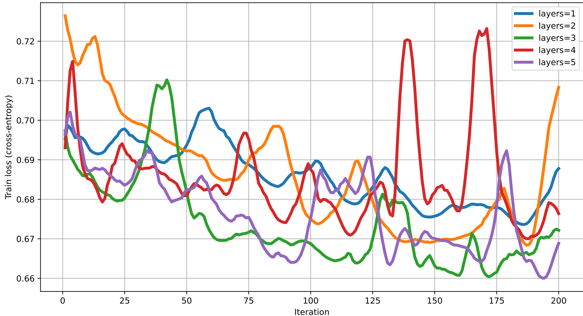
Train loss vs Iteration (dim=15) rot=RYZ, ent=full, gate=IsingXX
