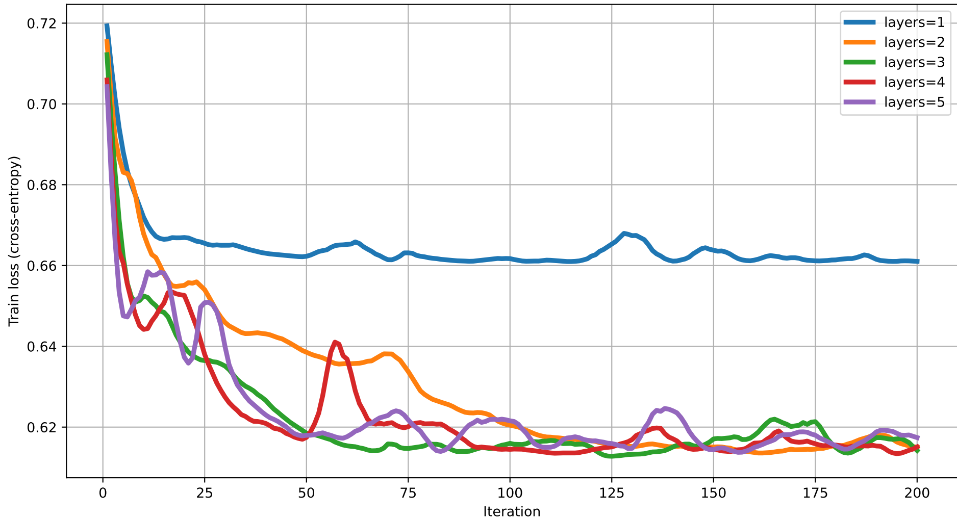
Train loss vs Iteration (degree=3) rot=RYZ, ent=pairwise, gate=CZ
