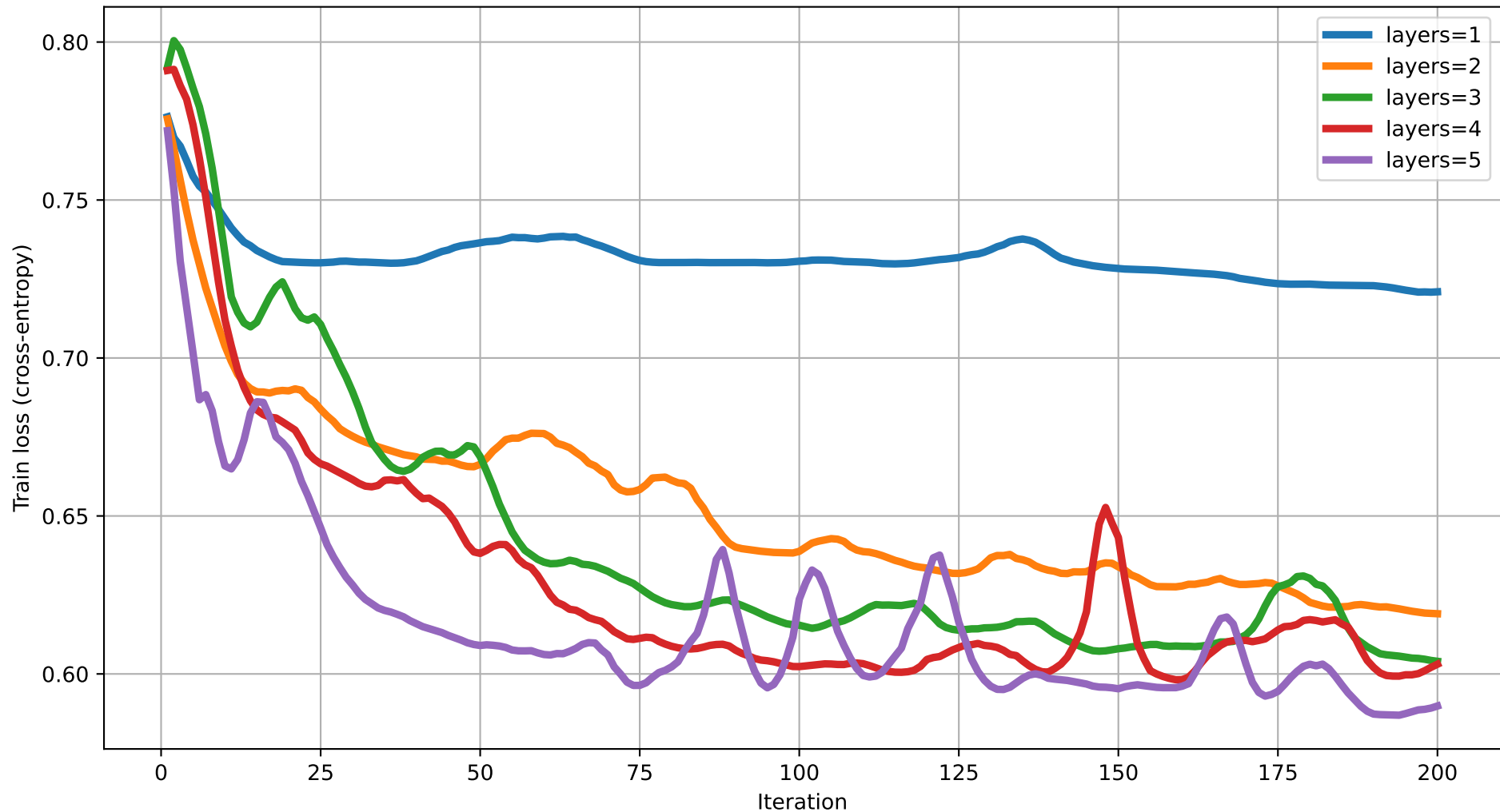
Train loss vs Iteration (dim=9) rot=RYZ, ent=full, gate=CNOT
