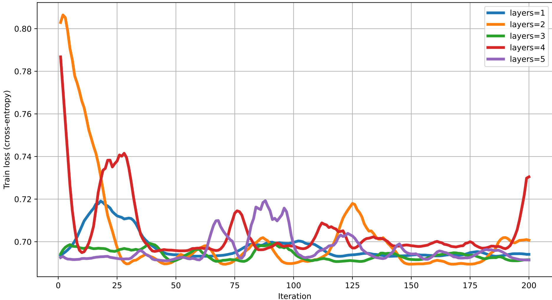
Train loss vs Iteration (dim=2) rot=RY, ent=pairwise, gate=IsingXX
