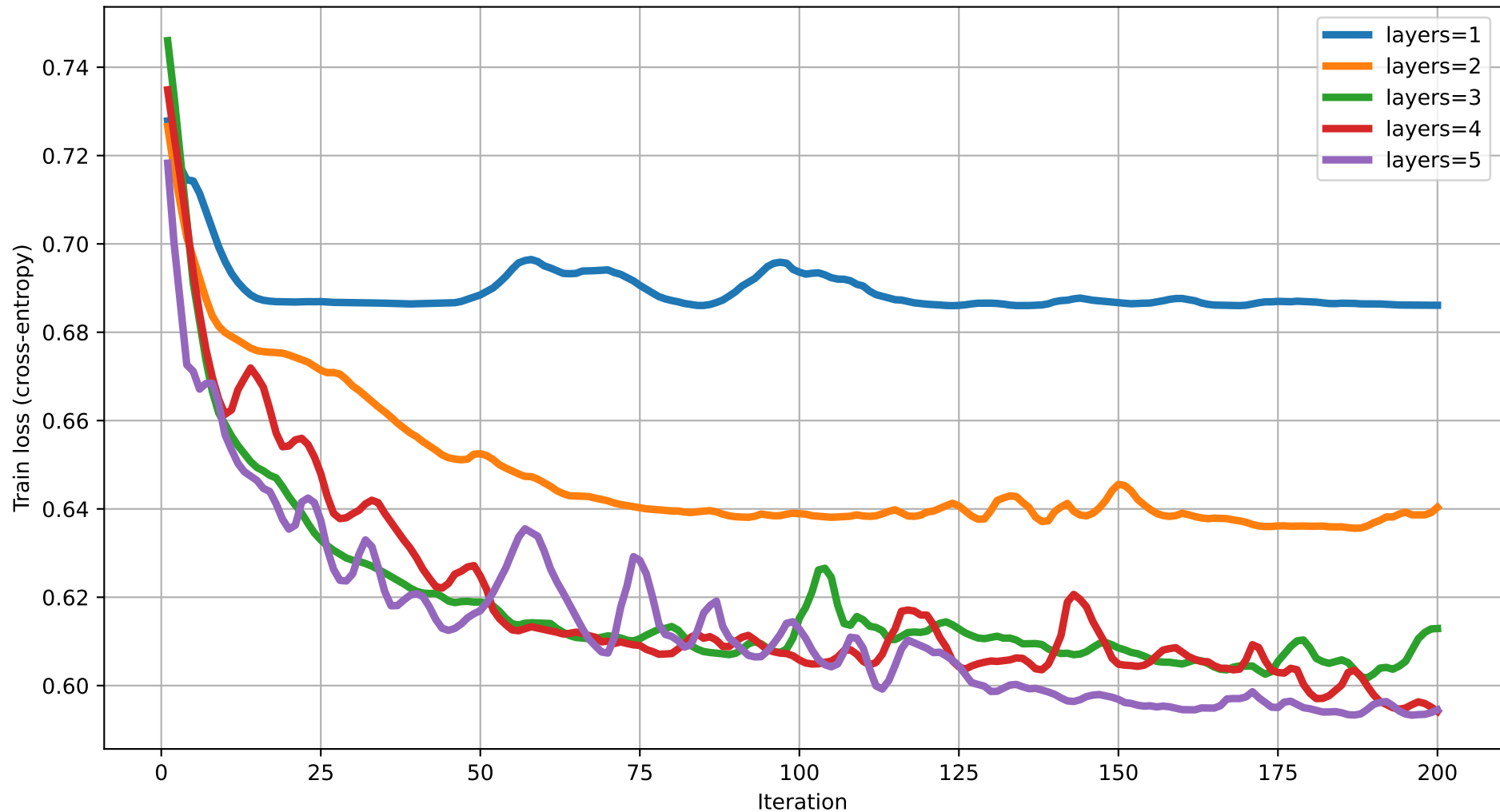
Train loss vs Iteration (degree=2) rot=Rot, ent=full, gate=CNOT
