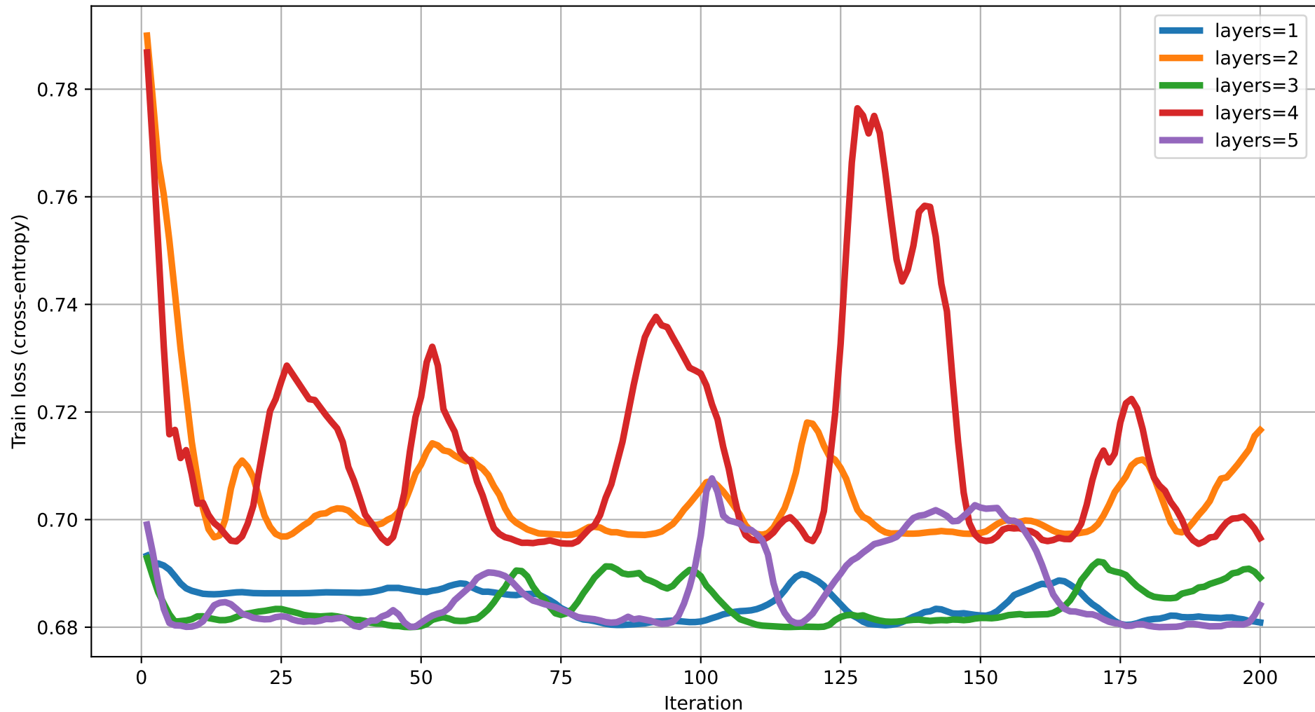
Train loss vs Iteration (dim=4) rot=RX, ent=full, gate=IsingXX
