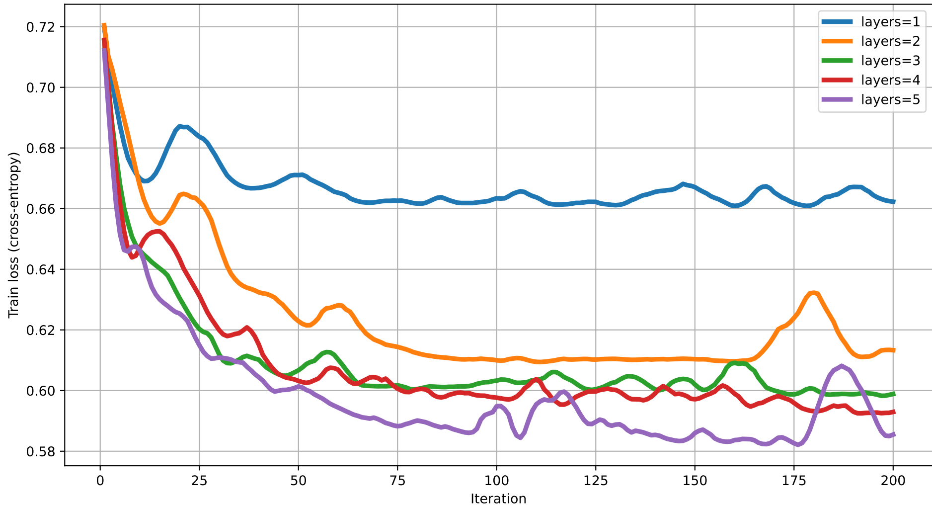
Train loss vs Iteration (degree=3) rot=RY, ent=full, gate=CZ
