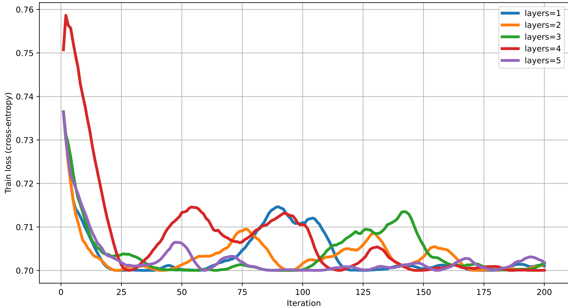
Train loss vs Iteration (dim=19) rot=RZ, ent=ring, gate=CZ
