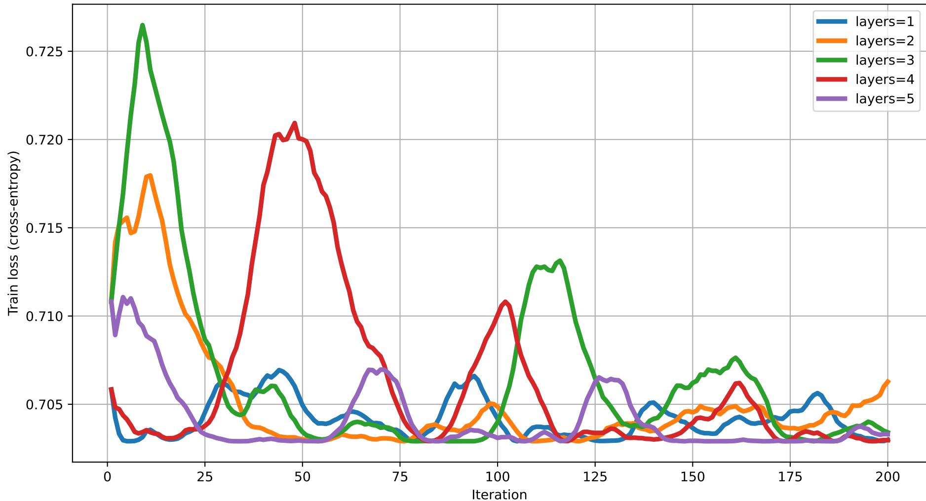
Train loss vs Iteration (dim=12) rot=RZ, ent=pairwise, gate=CZ
