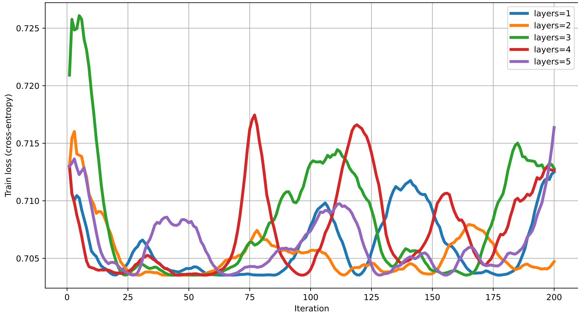
Train loss vs Iteration (dim=11) rot=RZ, ent=ring, gate=CZ
