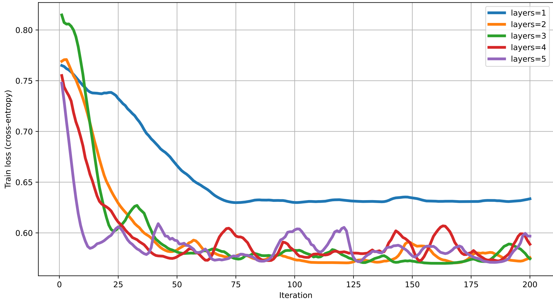
Train loss vs Iteration (dim=2) rot=RYZ, ent=ring, gate=CNOT
