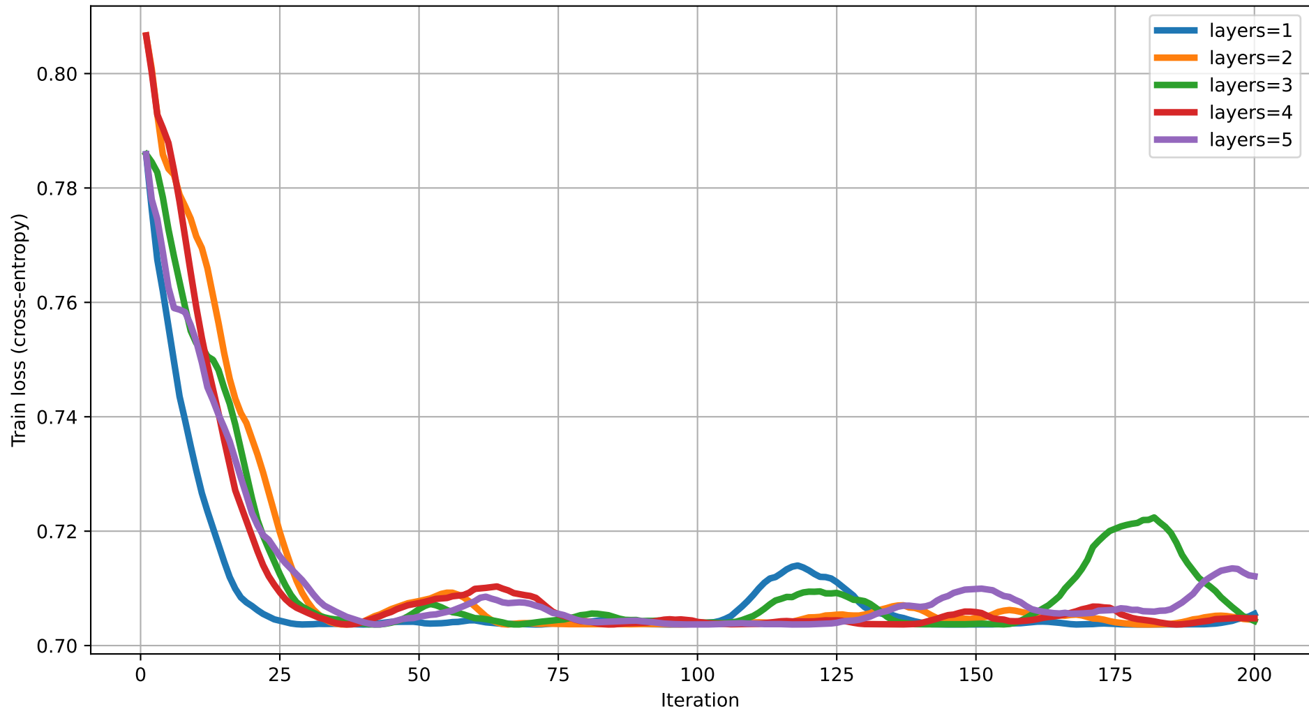
Train loss vs Iteration (dim=9) rot=RZ, ent=chain, gate=CNOT
