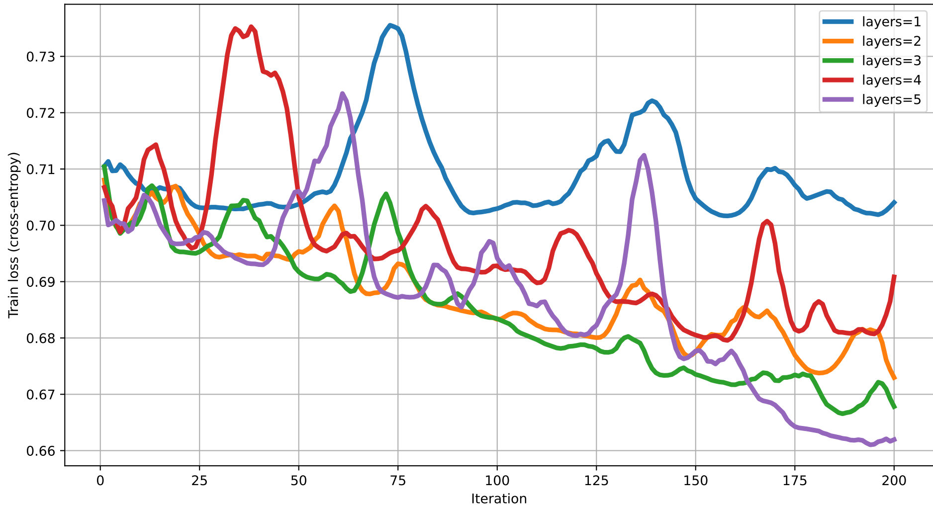
Train loss vs Iteration (dim=11) rot=RY, ent=full, gate=CNOT
