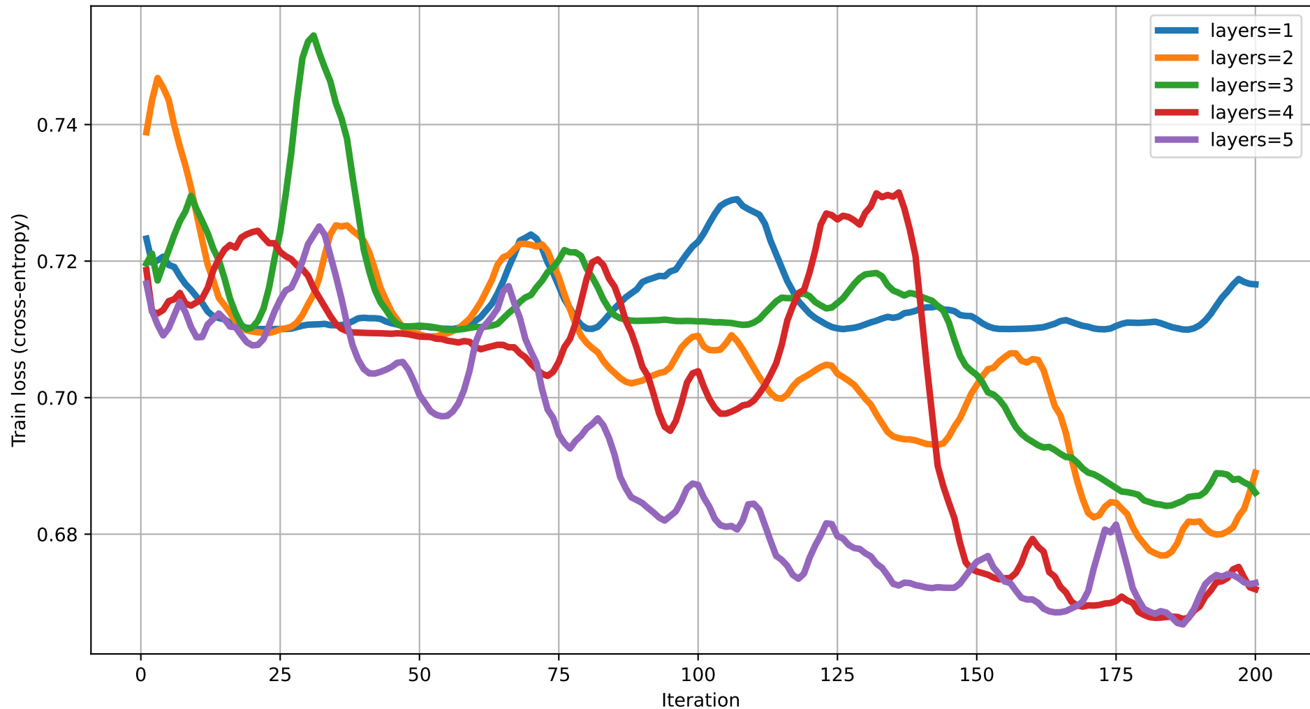
Train loss vs Iteration (dim=10) rot=RY, ent=chain, gate=CZ
