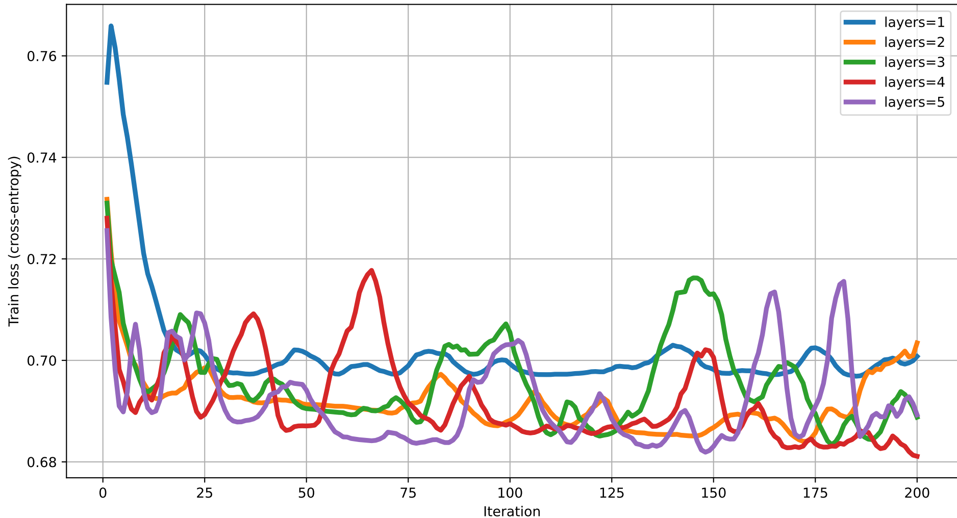
Train loss vs Iteration (dim=18) rot=Rot, ent=pairwise, gate=CZ
