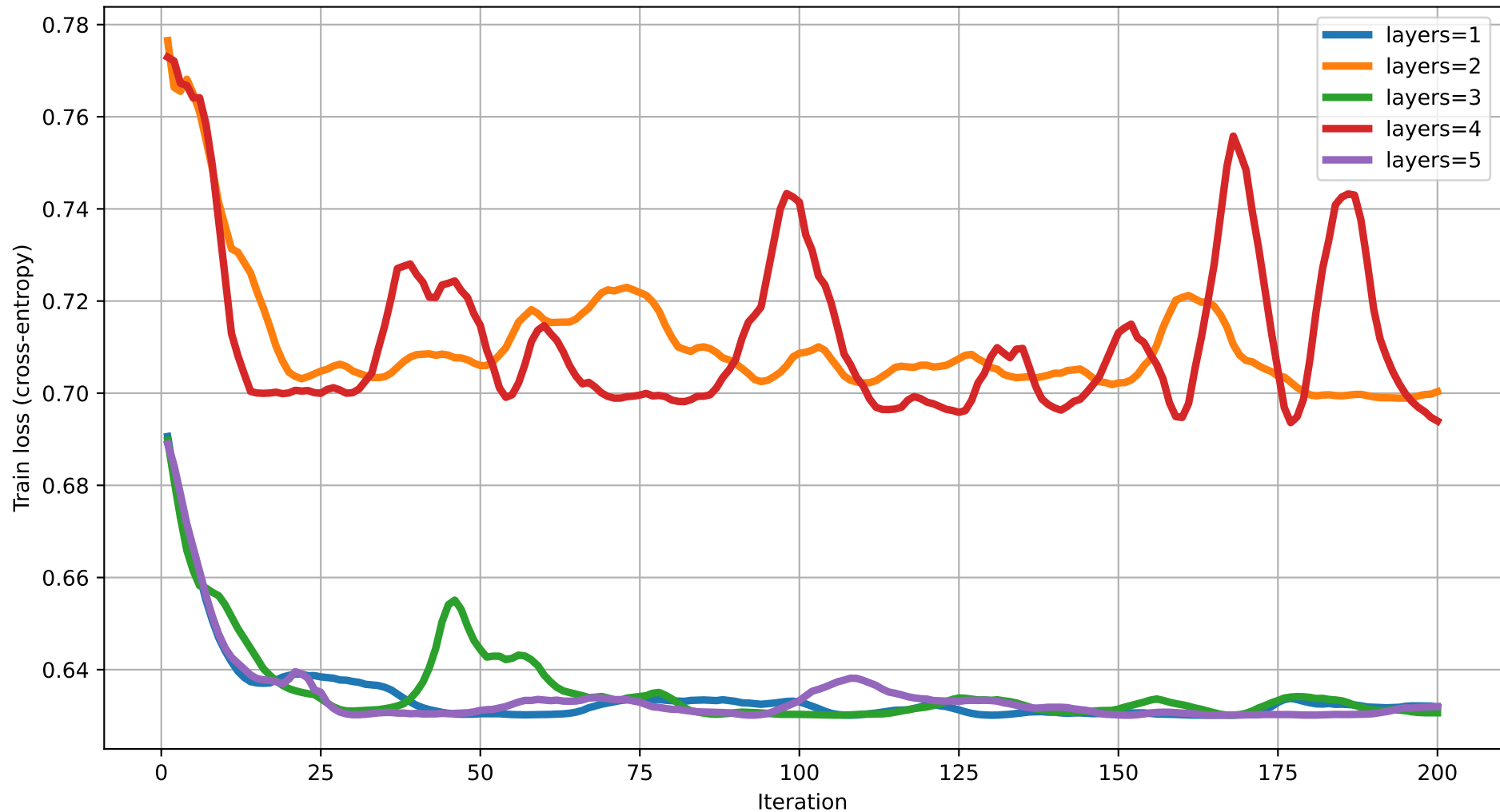
Train loss vs Iteration (dim=4) rot=RX, ent=ring, gate=IsingXX
