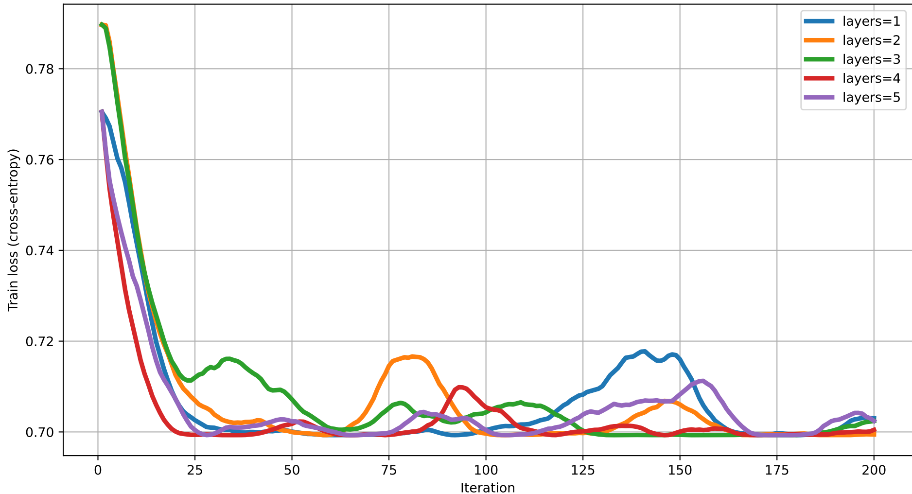
Train loss vs Iteration (dim=17) rot=RZ, ent=full, gate=CZ
