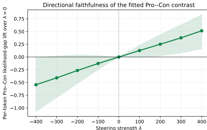
Figure 6: Directional faithfulness of the fitted Pro-minus-Con contrast. The line is the mean likelihood-gap lift across ten topics fixed in advance; the band spans the 10th to 90th percentiles across topics. Every topic-specific curve is centered at \lambda = 0 , which is the direction-specific ablation.
