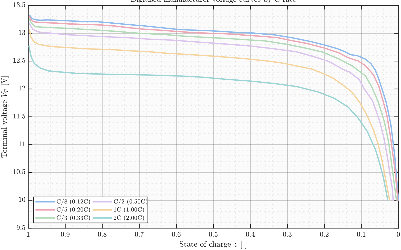
Digitised manufacturer voltage curves by C-rate
