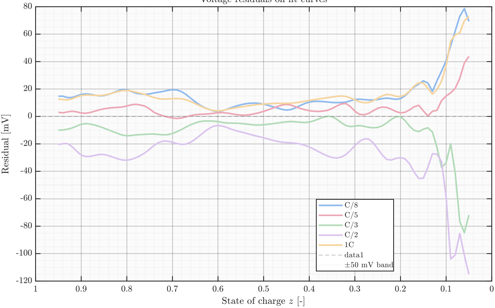
Voltage residuals on fit curves
