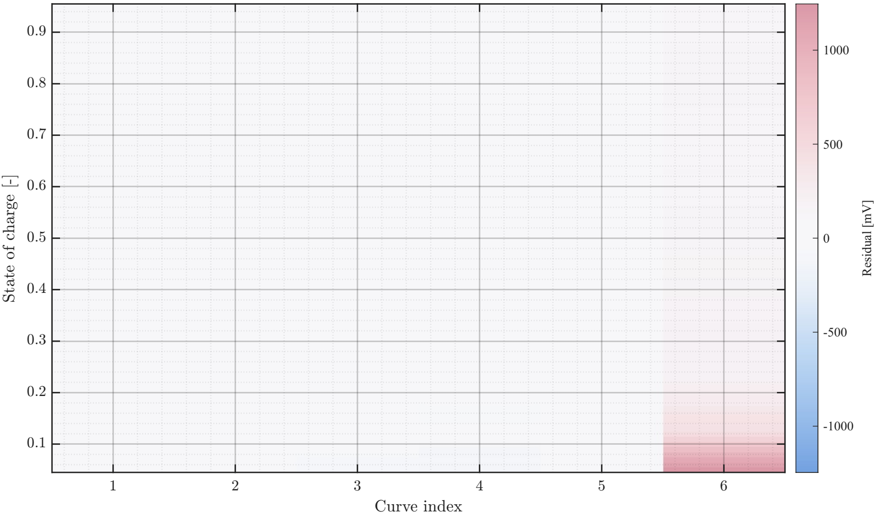
Residual heatmap [mV] across SoC and curve index
