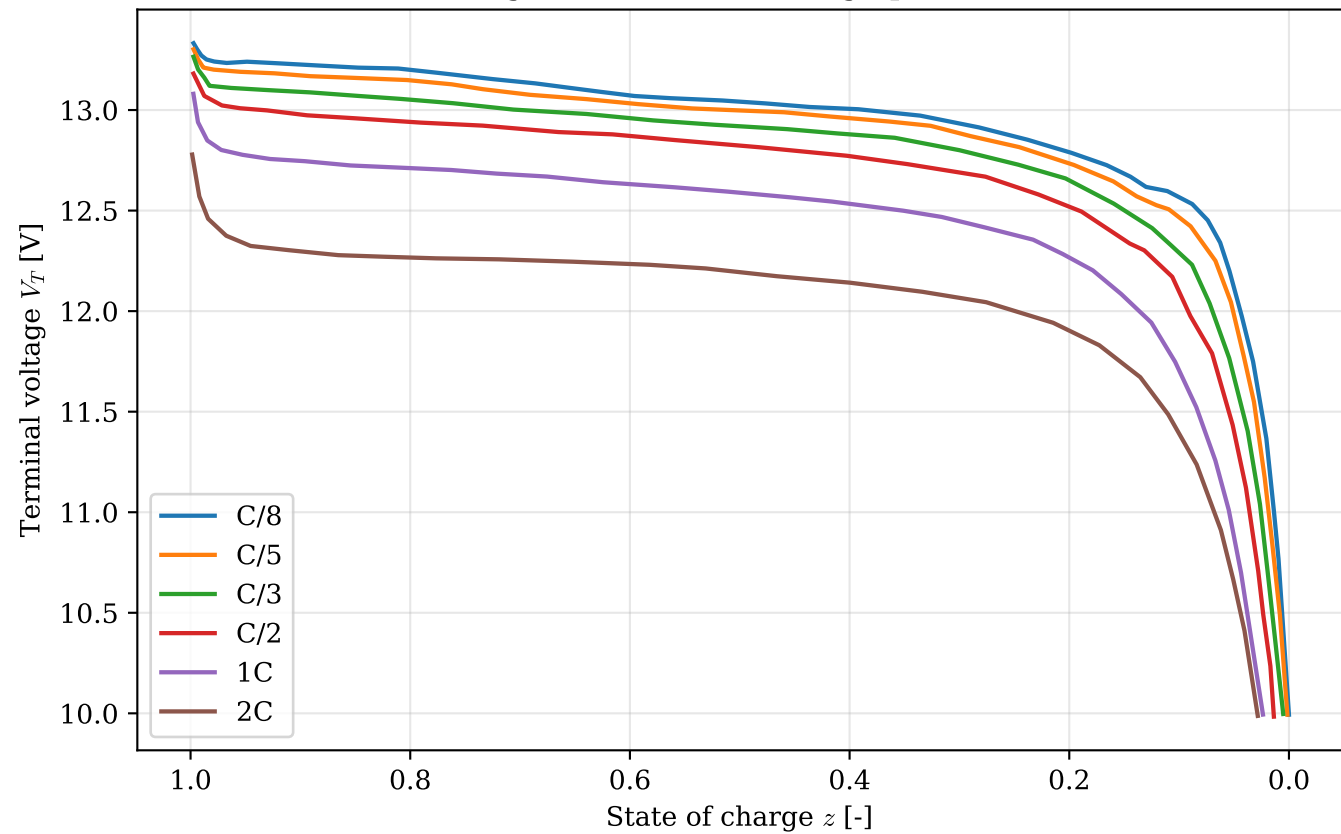
Digitised Valence voltage profiles
