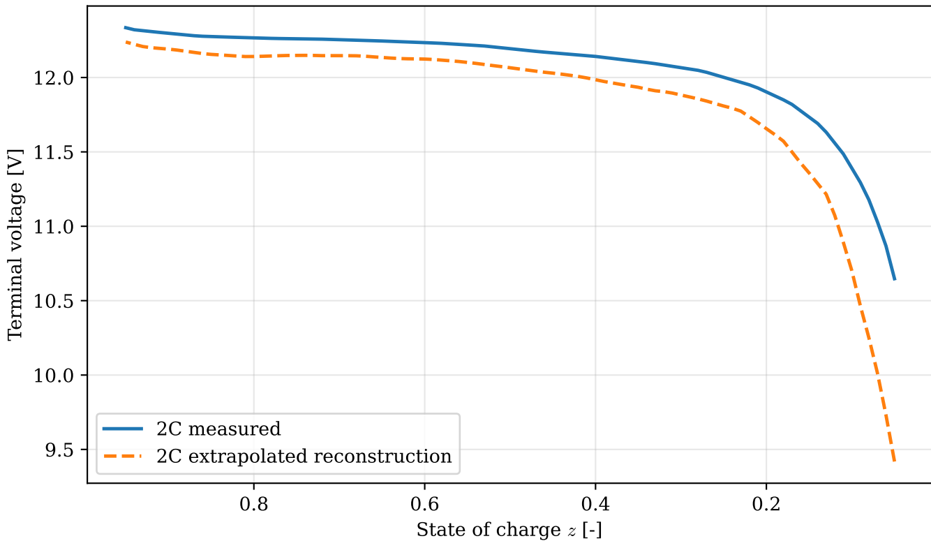
2C high-current validation: extrapolation outside continuous fit
