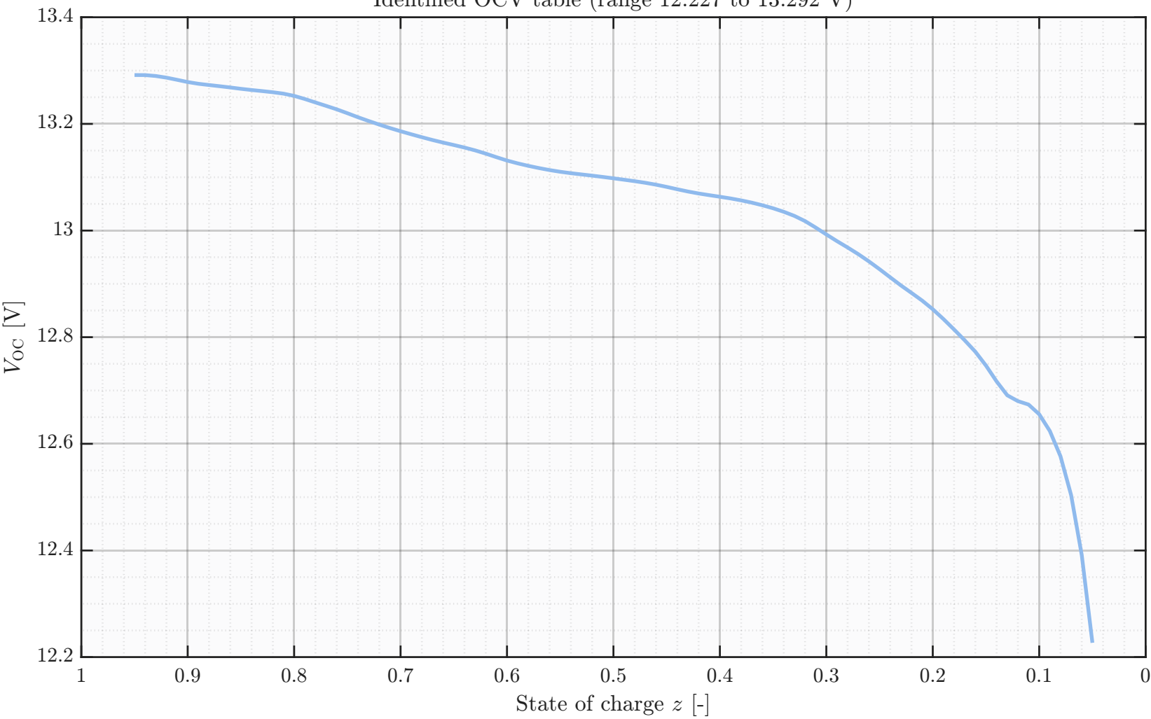
Identified OCV table (range 12.227 to 13.292 V)
