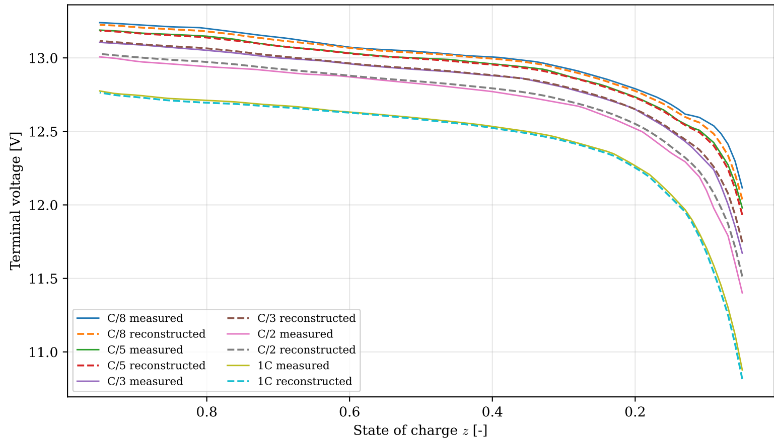
Static ECM validation on fitted C-rate curves
