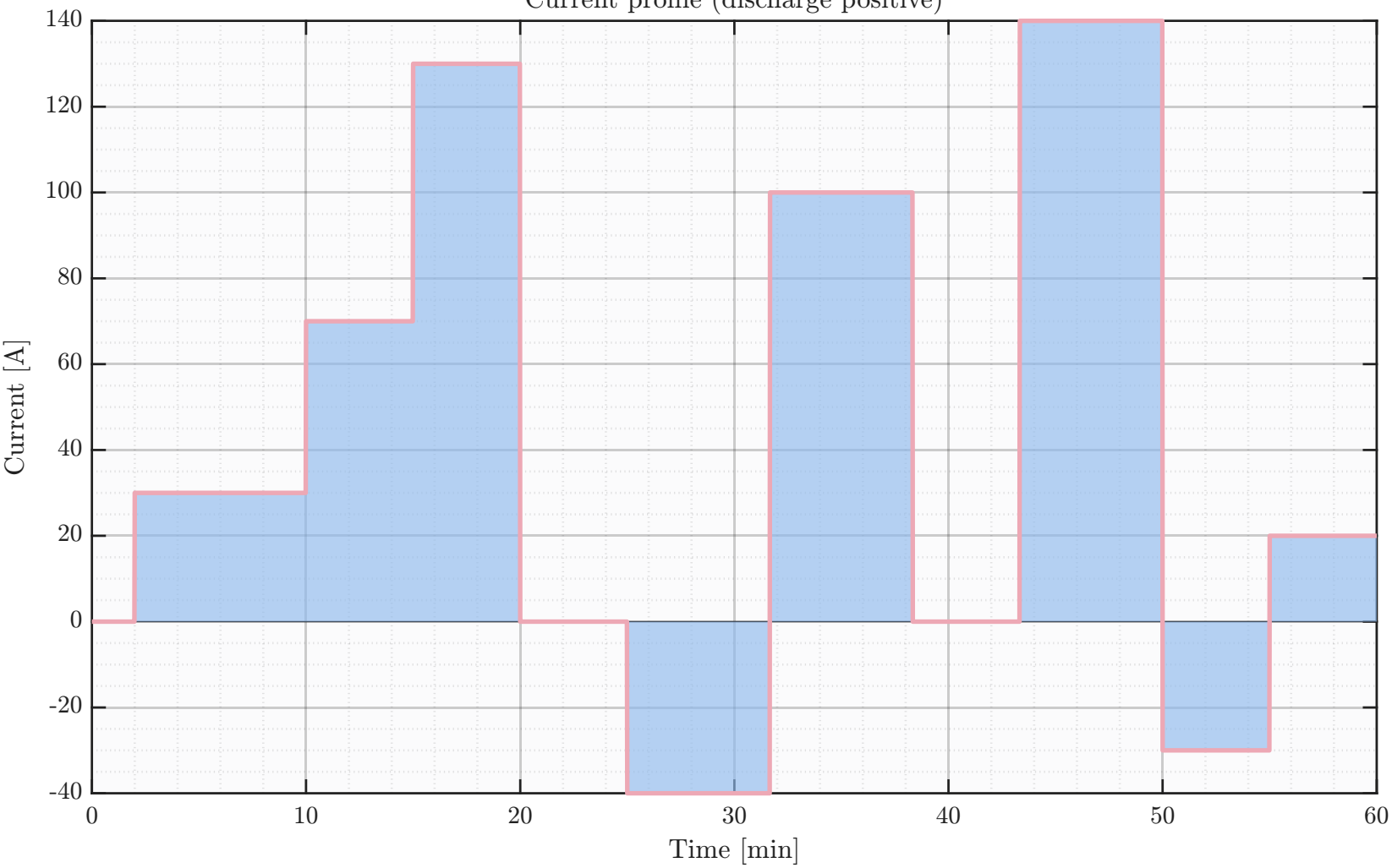
Current profile (discharge positive)
