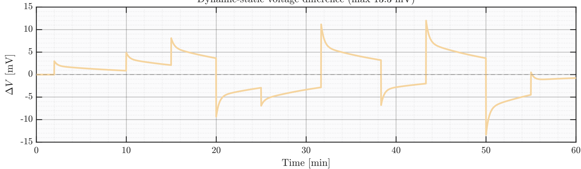
Dynamic-static voltage difference (max 13.3 mV)
