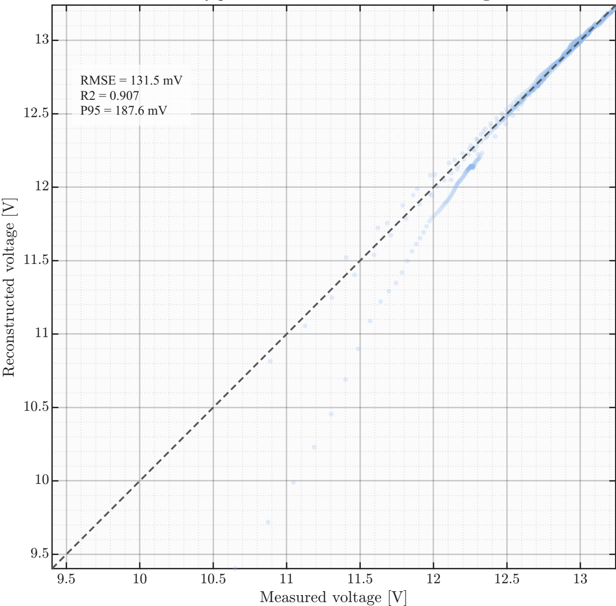
Parity plot: measured vs reconstructed voltage
