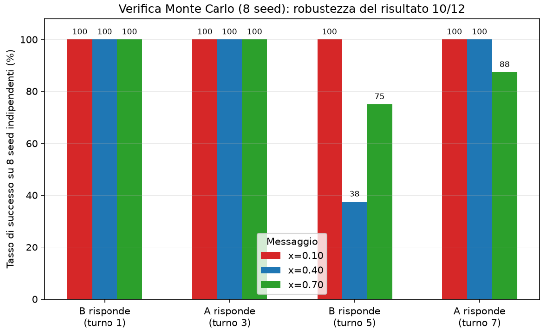
Fig. 30 — Success rate per message and exchange, aggregated over 8 independent seeds: B(t_1) and A(t_3) perfect at 100%, B(t_5) and A(t_7) variable and non-monotonic with respect to position in the round-robin.
