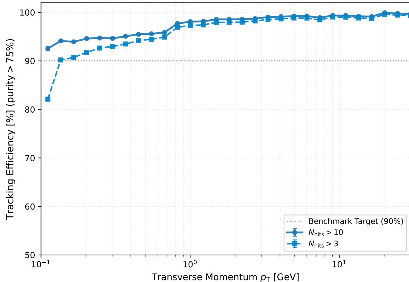
(a) Tracking Efficiency vs p_T ( 15^\circ < \theta < 165^\circ )
