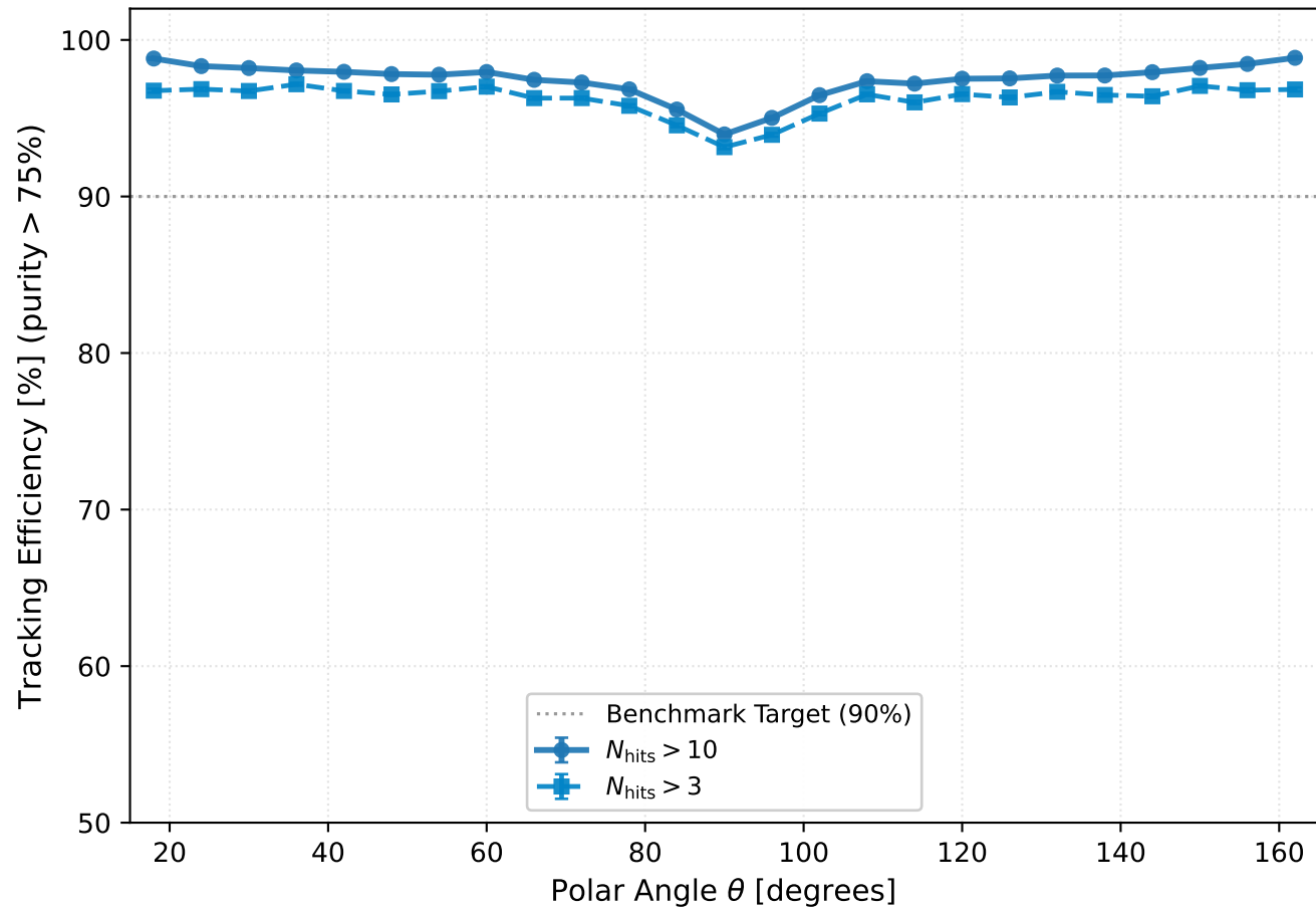
(b) Tracking Efficiency vs Polar Angle Across Acceptance
