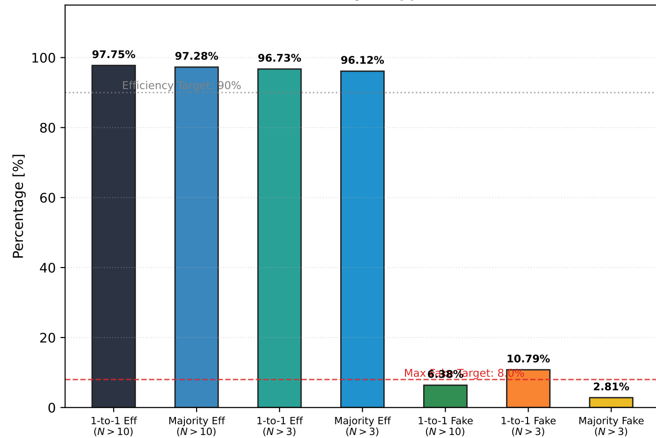
(d) Performance Summary (Mapped Across Hit Cuts)
