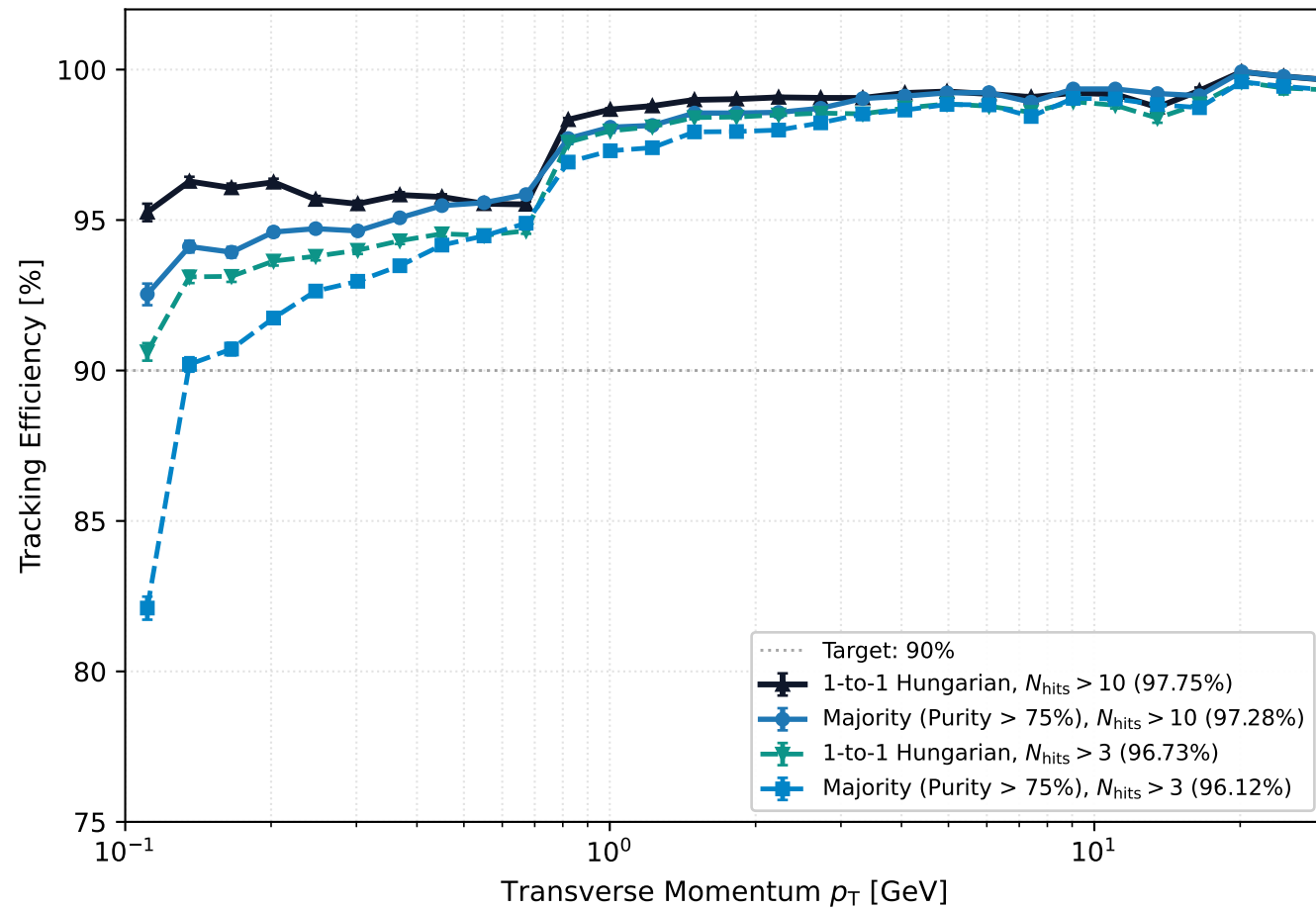
(a) Efficiency vs p_T ( 15^\circ < \theta < 165^\circ )
