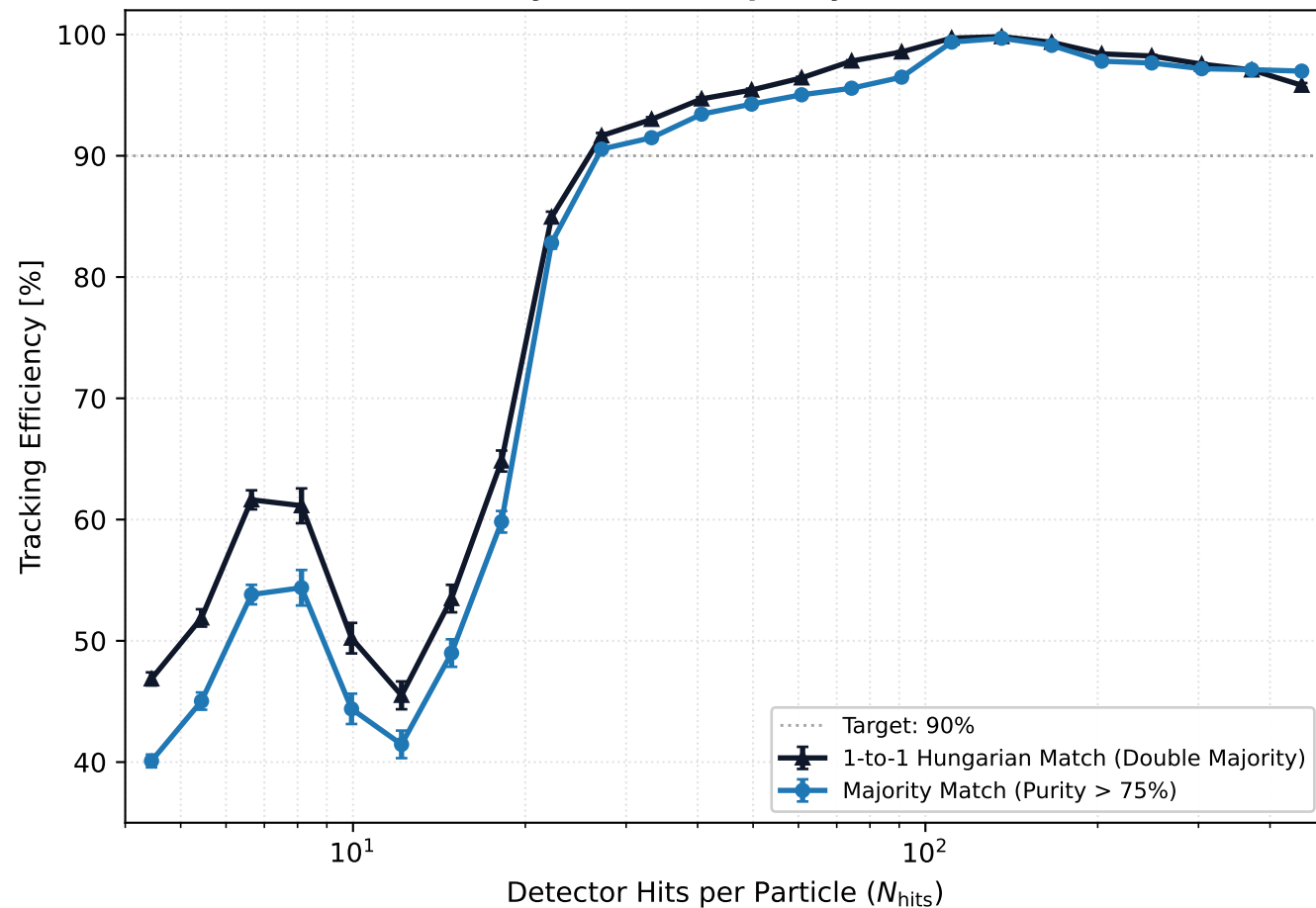
(c) Efficiency vs Hit Multiplicity (Turn-on Curve)
