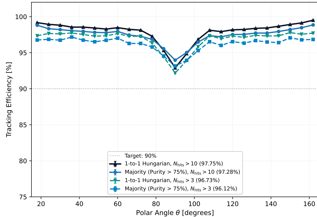
(b) Efficiency vs Polar Angle \theta Across Acceptance
