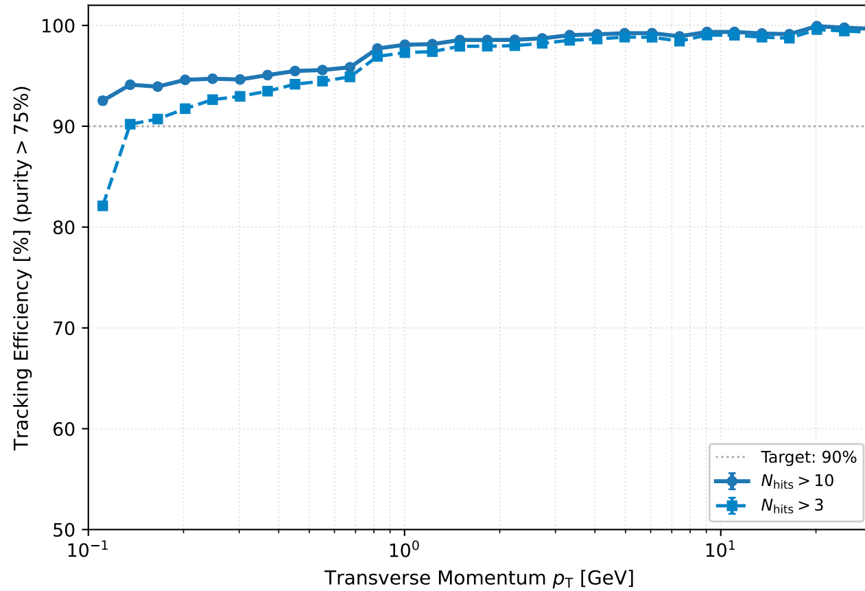
(a) Efficiency vs p_T ( 15^\circ < \theta < 165^\circ )
