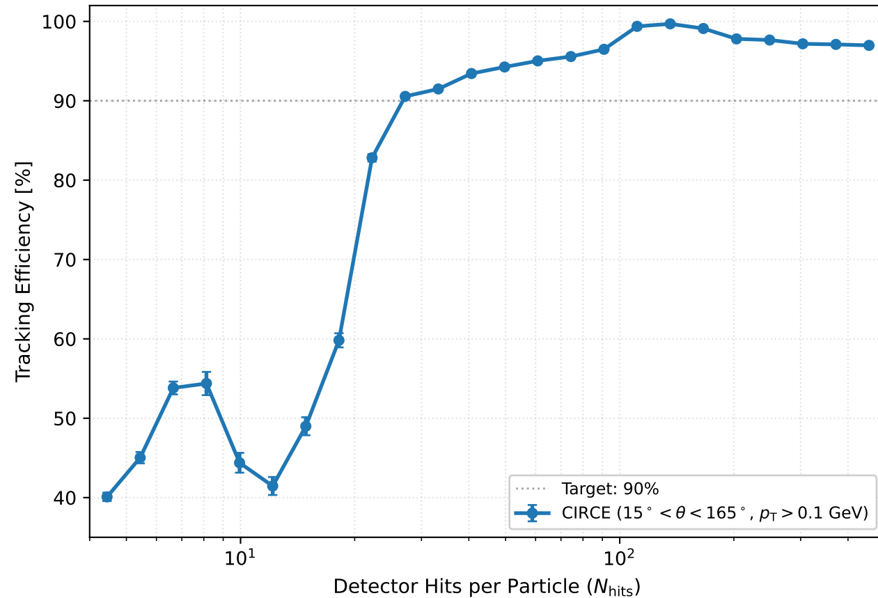
(c) Efficiency vs Hit Multiplicity (Turn-on Curve)
