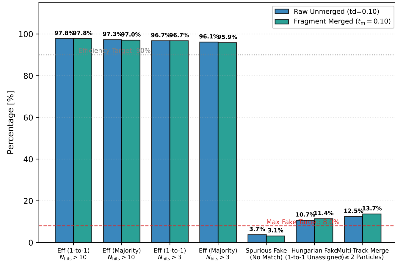
(d) Performance Breakdown: Raw Unmerged vs. Fragment Merged
