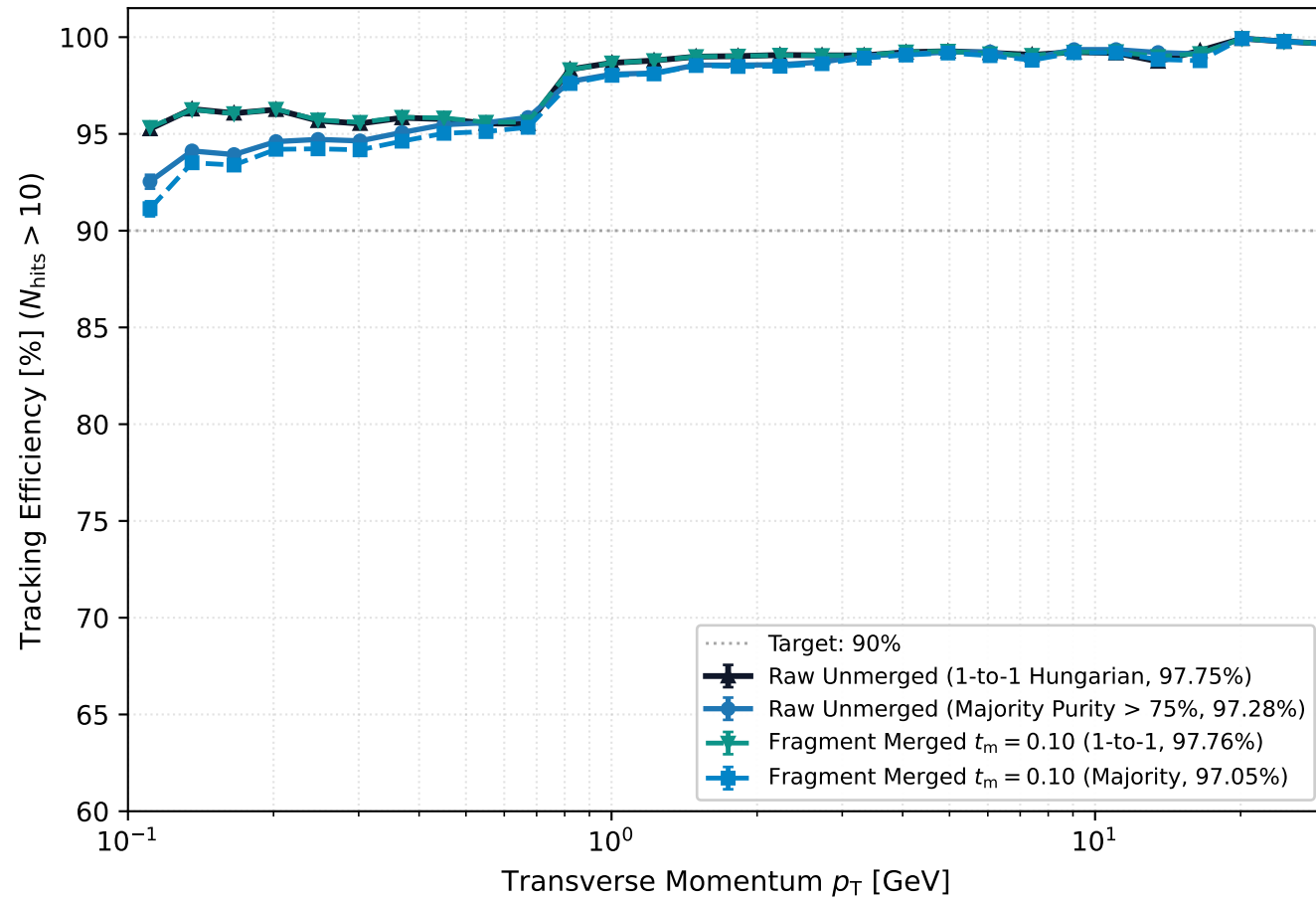
(a) Efficiency vs p_T ( 15^\circ < \theta < 165^\circ )
