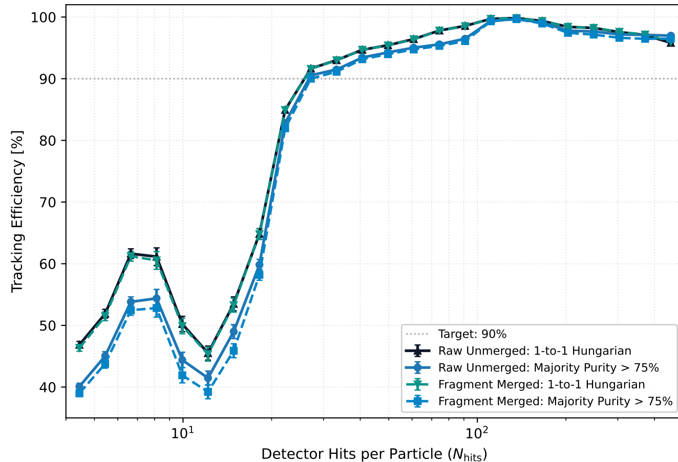
(c) Efficiency vs Hit Multiplicity (Turn-on Curve)
