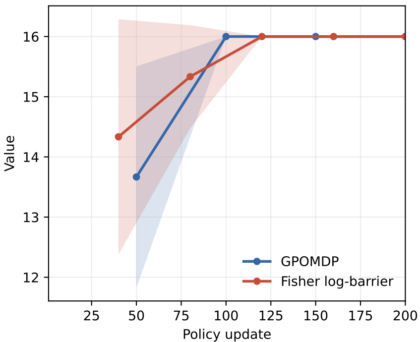
Numerical rank
