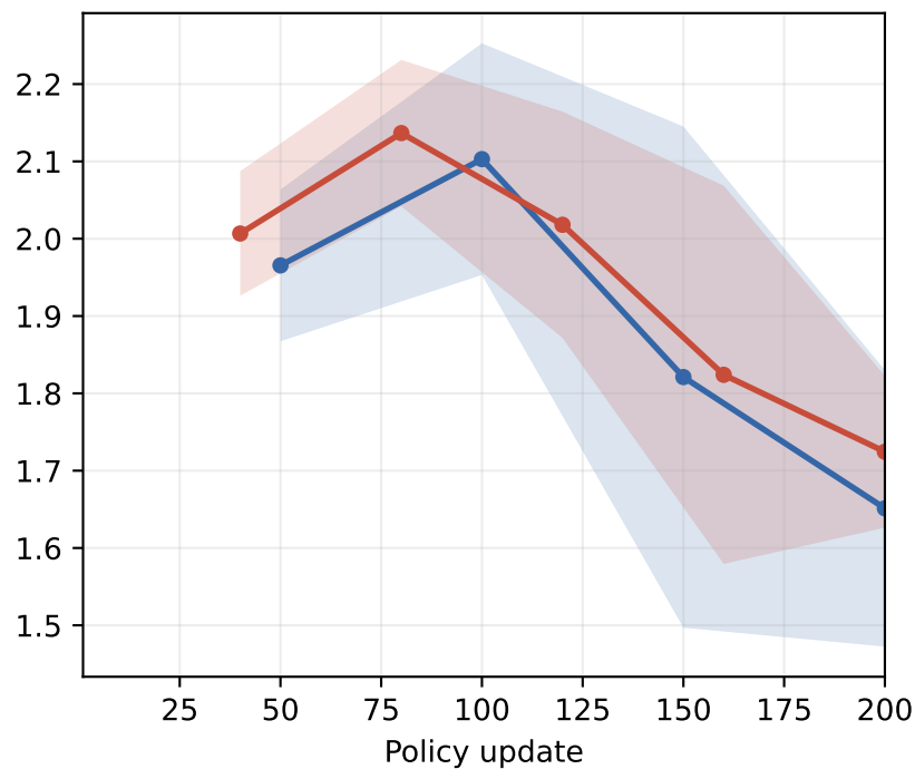
Effective rank
