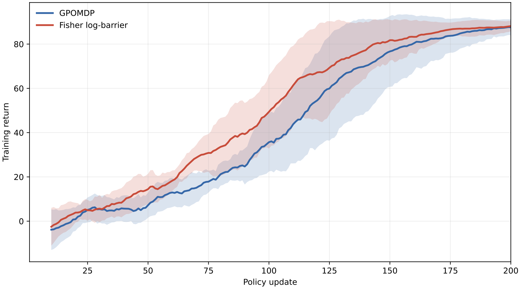
MountainCarContinuous-v0 performance (6 seeds, 200 updates)
