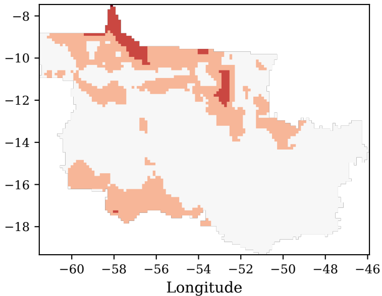
Predicted
