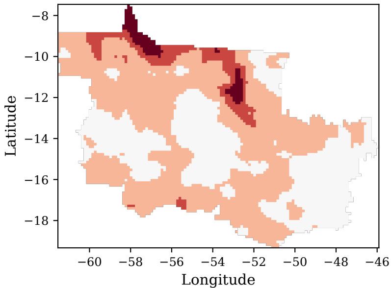
Observed
