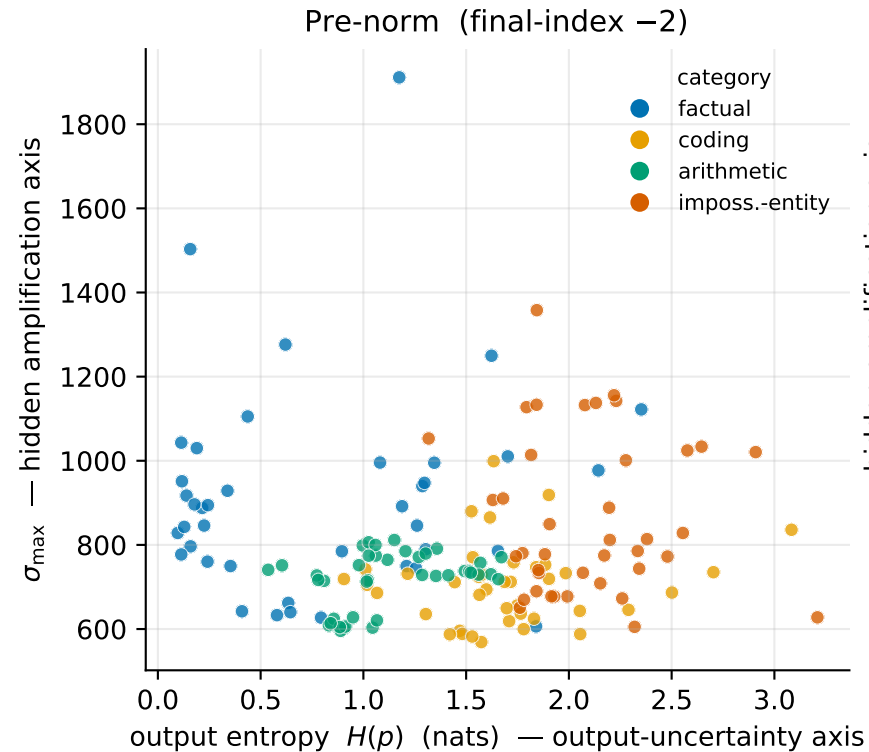
Two-axis dissociation: output uncertainty vs. hidden amplification (Qwen2.5-0.5B, n=40/cat)
