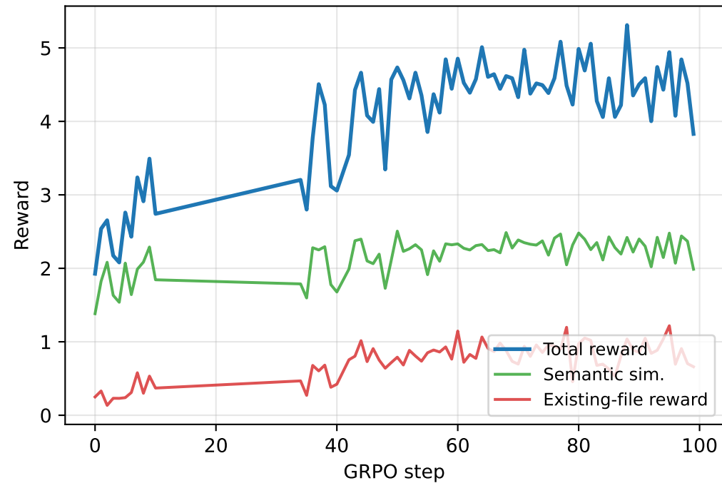
(a) Reward components vs. step
