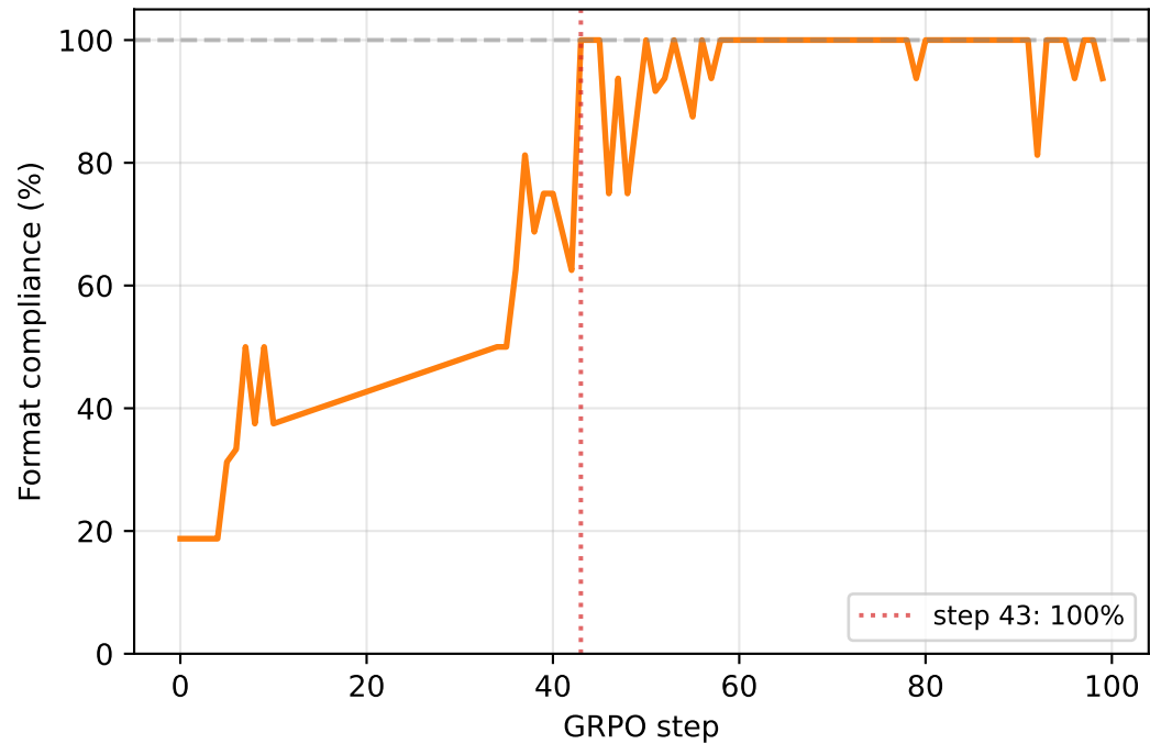
(b) Format compliance rate
