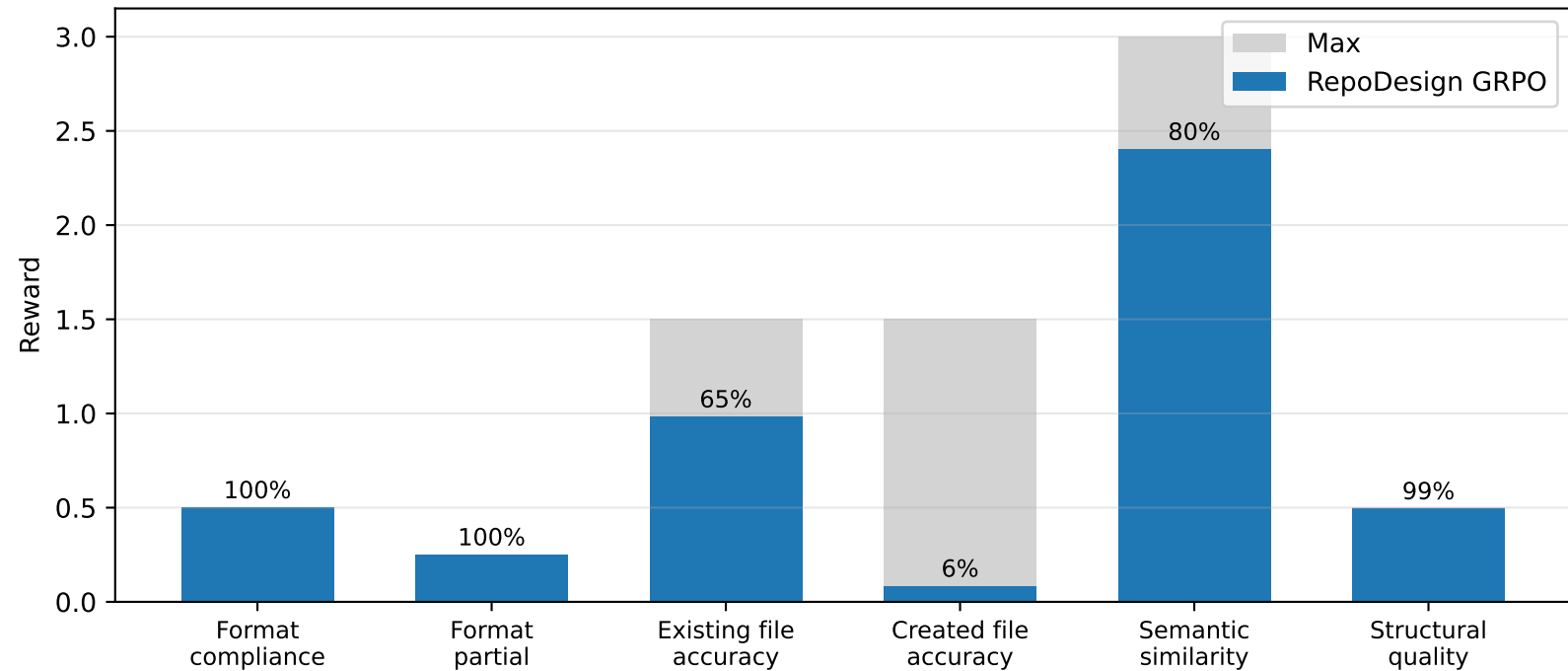
Per-component reward on 12 unseen-repo examples (total 4.71/7.25)
