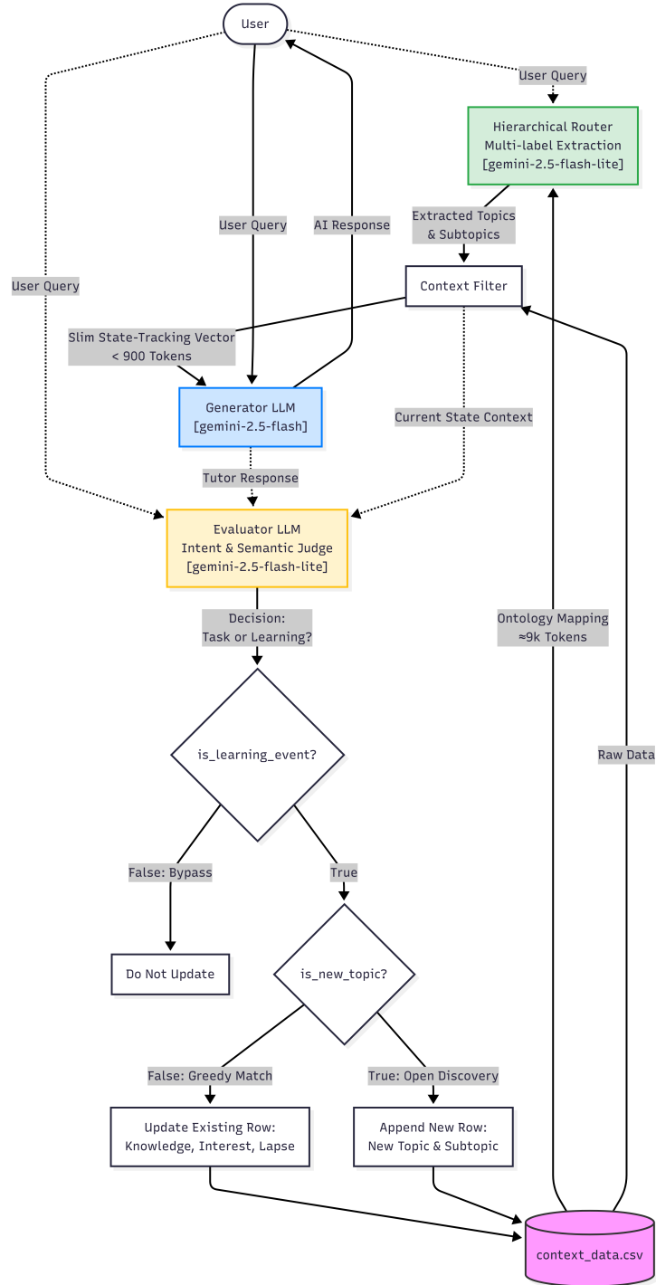
Figure 5.3: The definitive Closed-Loop Hierarchical Router-Based (HRB) Architecture. The system dynamically filters the context via the Router and continuously updates the user profile through the asynchronous Evaluator LLM.
