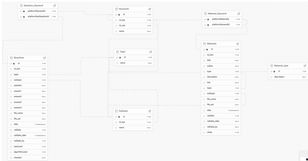
Figure 1 – ERD MathE Use Case (Supabase example)
