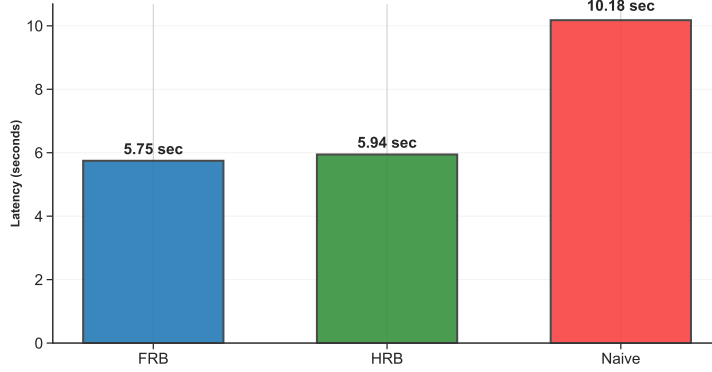
Figure 6.2: Comparison of execution times at the text-generation layer. The chart visually highlights the severe operational bottleneck of the unroute Naive model (exceeding 10 seconds per turn). The introduction of an upstream semantic routing mechanism successfully halves the generation latency, stabilizing the user-facing response time around the 6-second threshold regardless of the specific extraction methodology (FRB or HRB).
