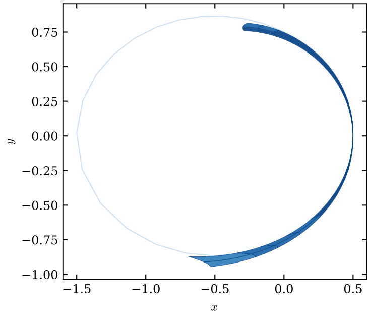
(c) flow-aligned tiling at t = T
