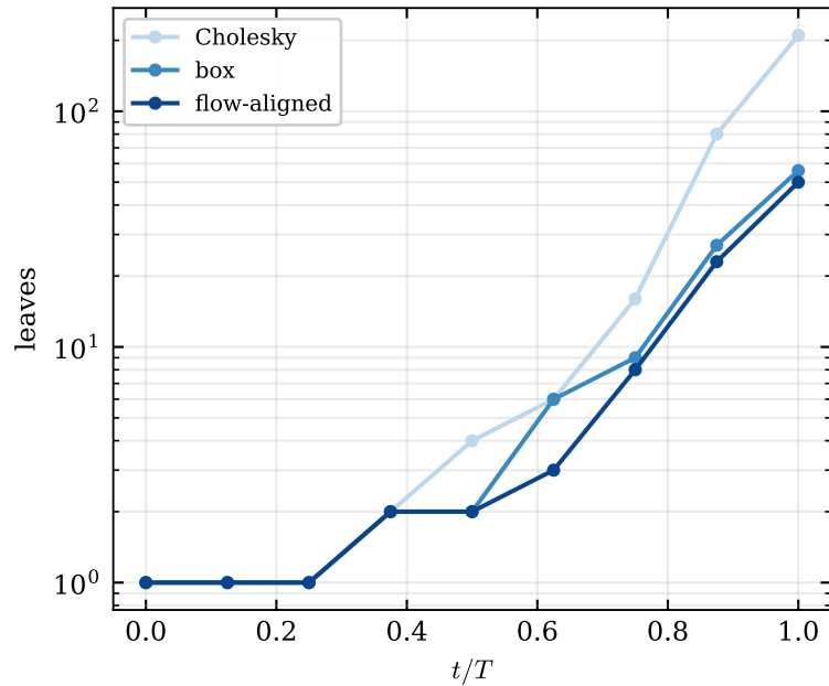
(b) leaves over a full period
