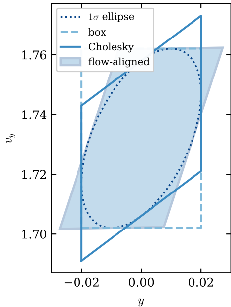
(a) one ellipsoid, three coverings
