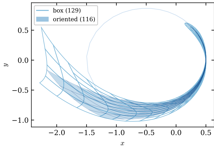
(c) leaf tiling at t_f
