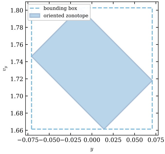
(a) initial set, (y, v_y)
