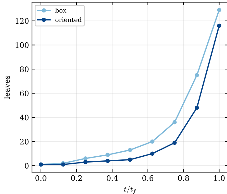
(b) leaves vs time
