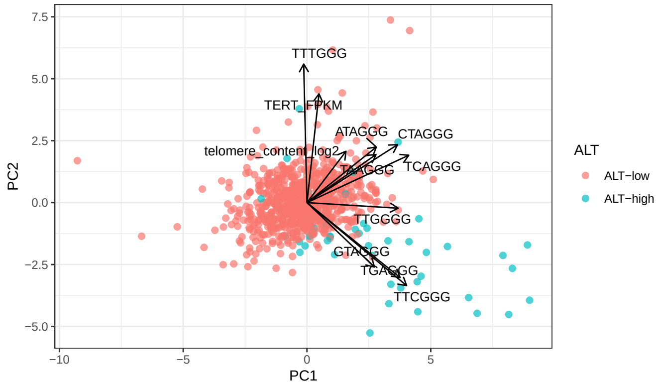
PCA biplot without TF rate and telomere insertion rate
