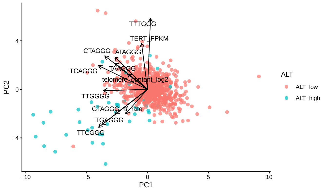
PCA biplot without tel. insertion
