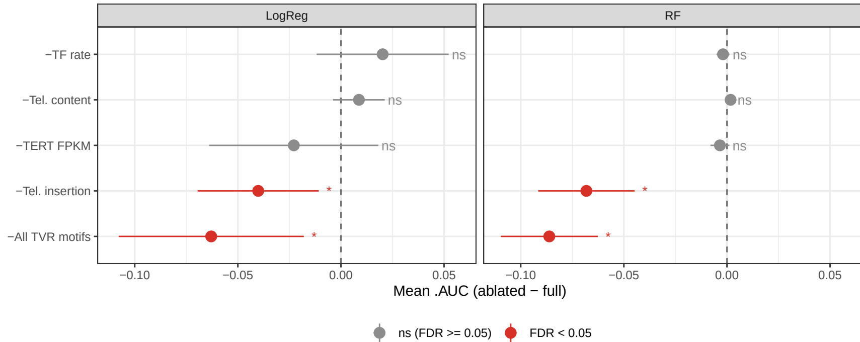
Mean .AUC with 95% CI (paired Wilcoxon, FDR-adjusted)
