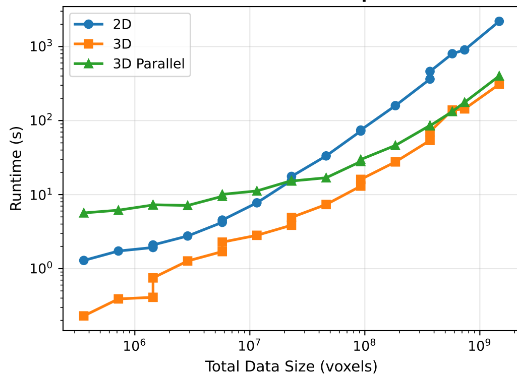
Absolute Runtime Comparison
