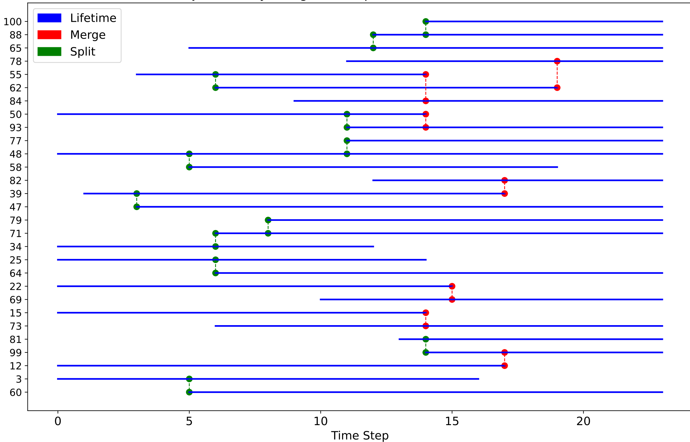
Watershed Object History: Merges and Splits (Filtered to Event-Involved Labels)
