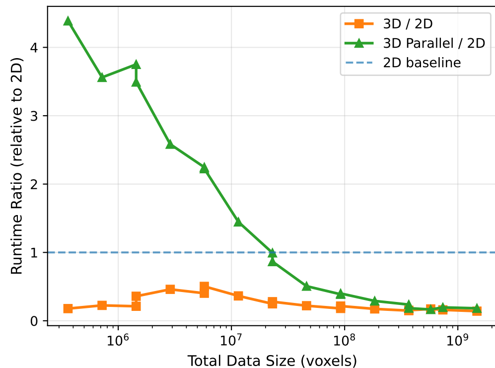
Relative Runtime Performance
