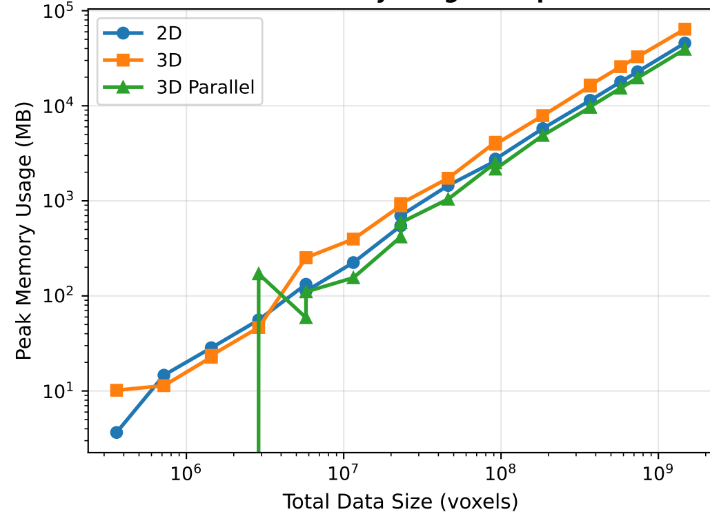
Absolute Memory Usage Comparison
