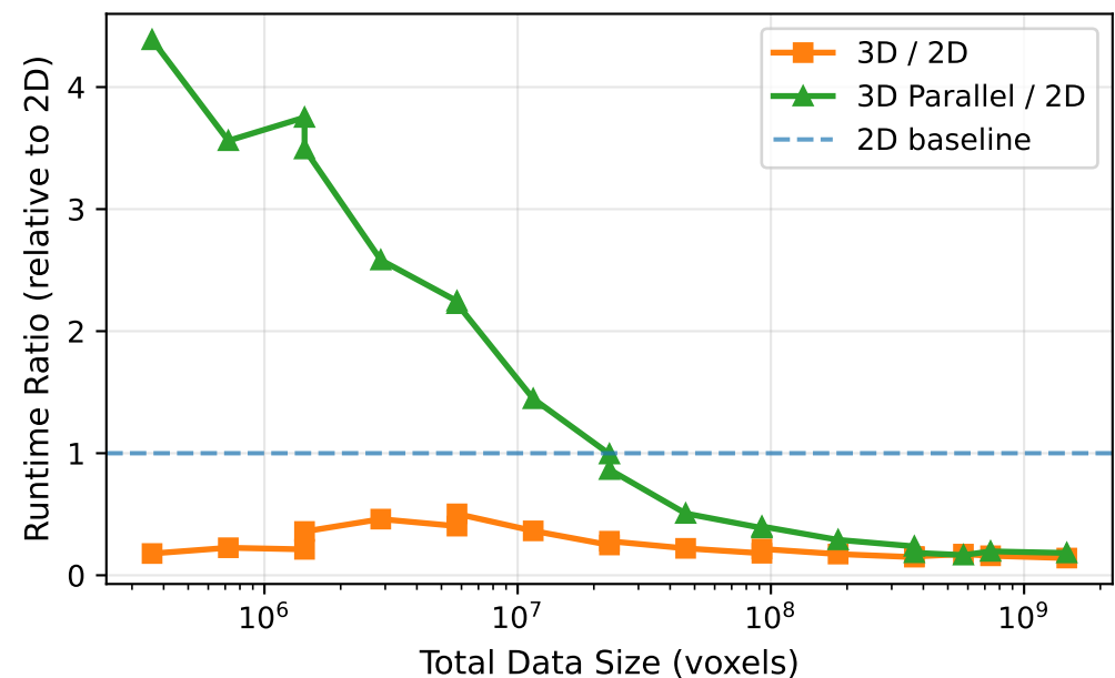
Relative Runtime Performance
