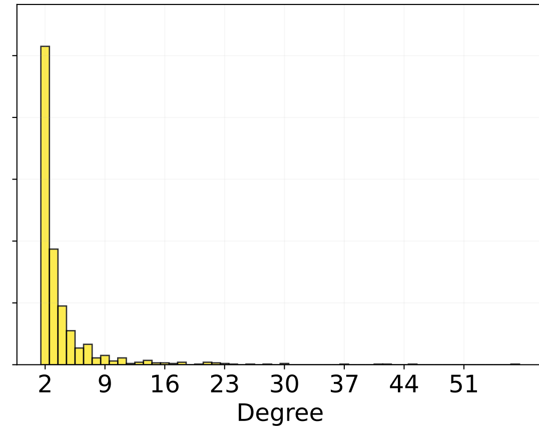
Scale-free
