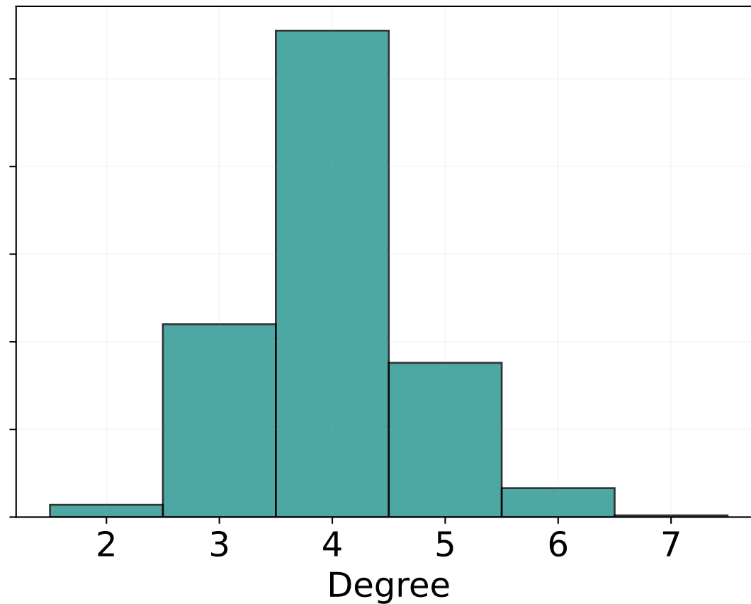
Small-world
