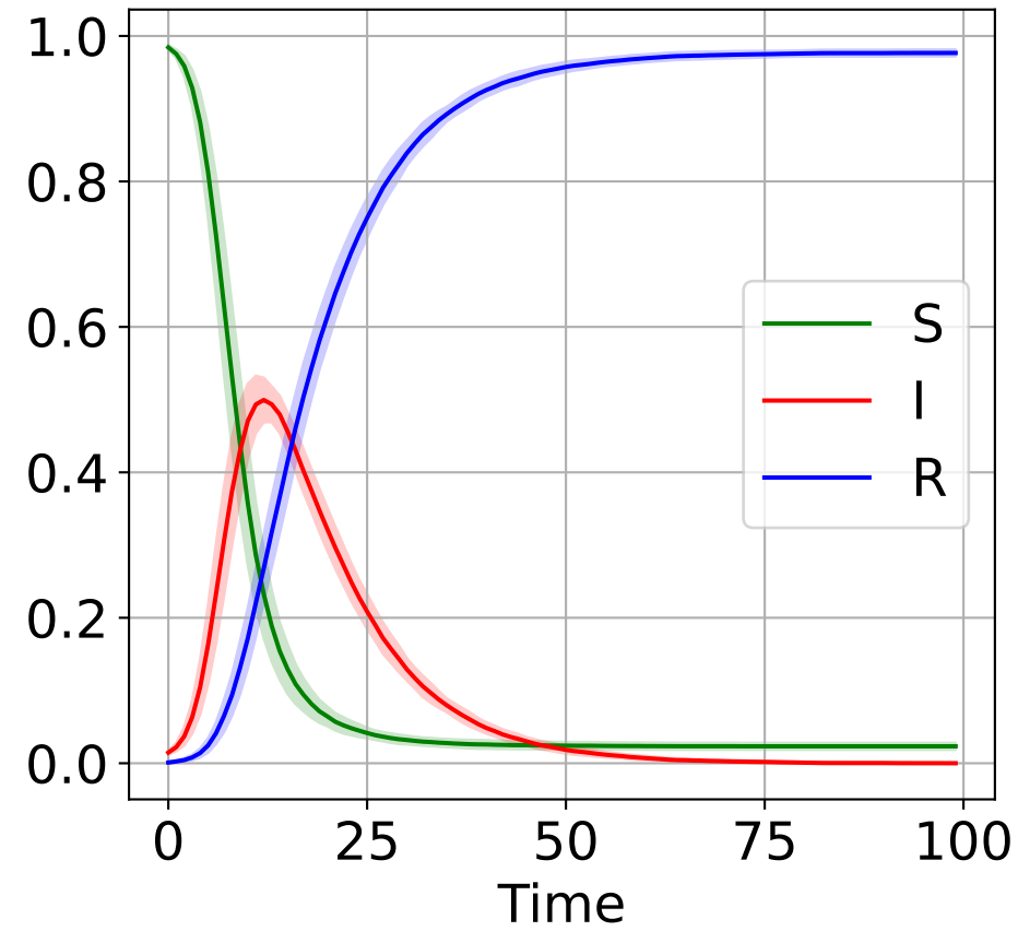
SIR model
