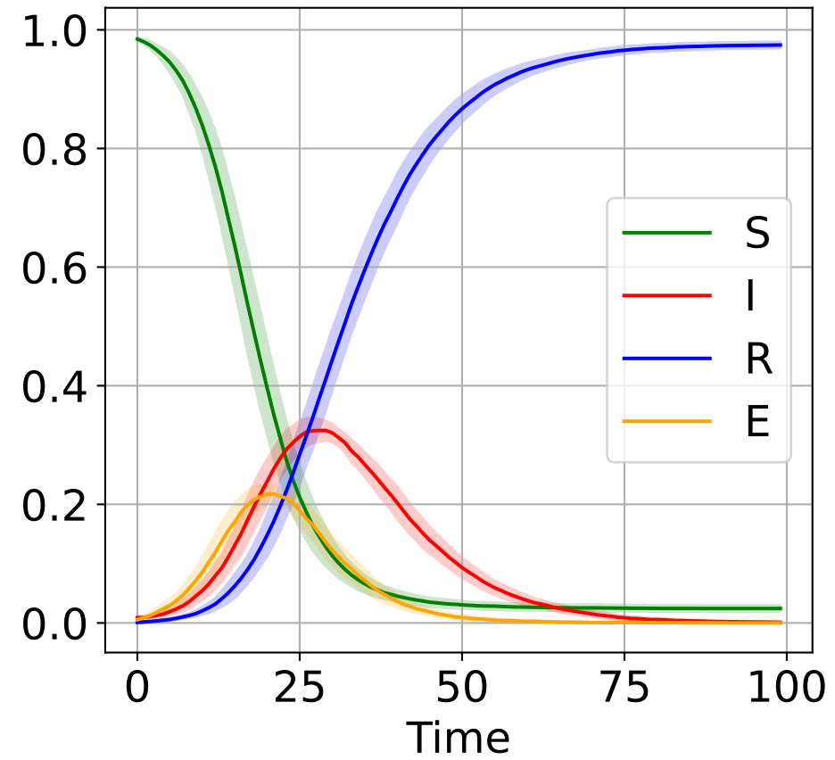
SEIR model
