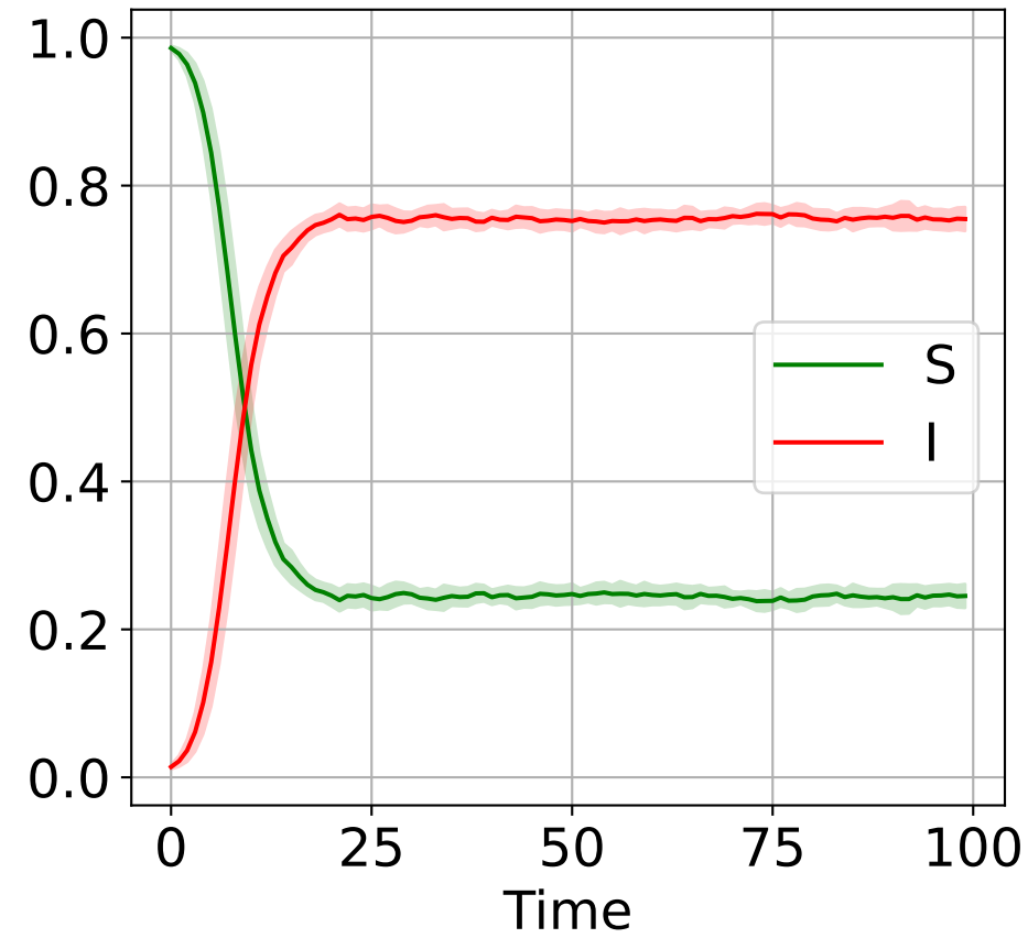
SIS model
