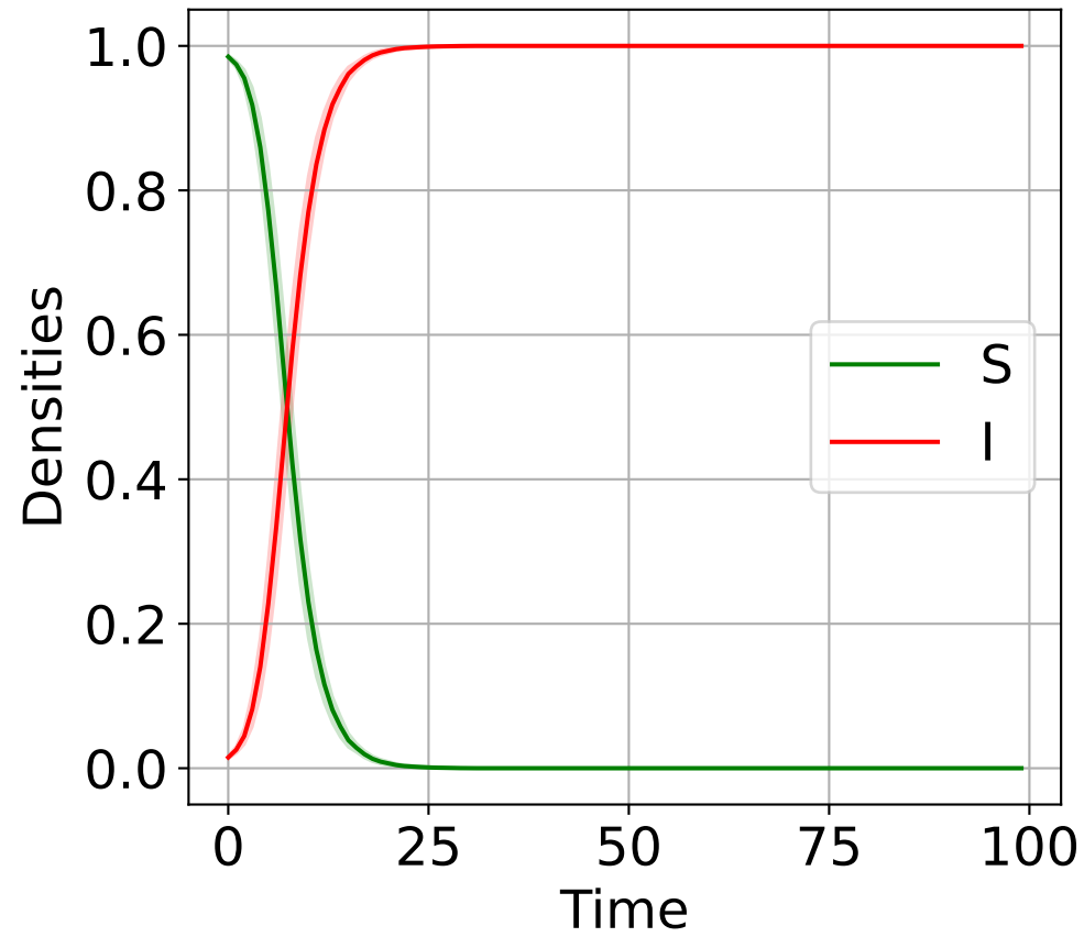
SI model
