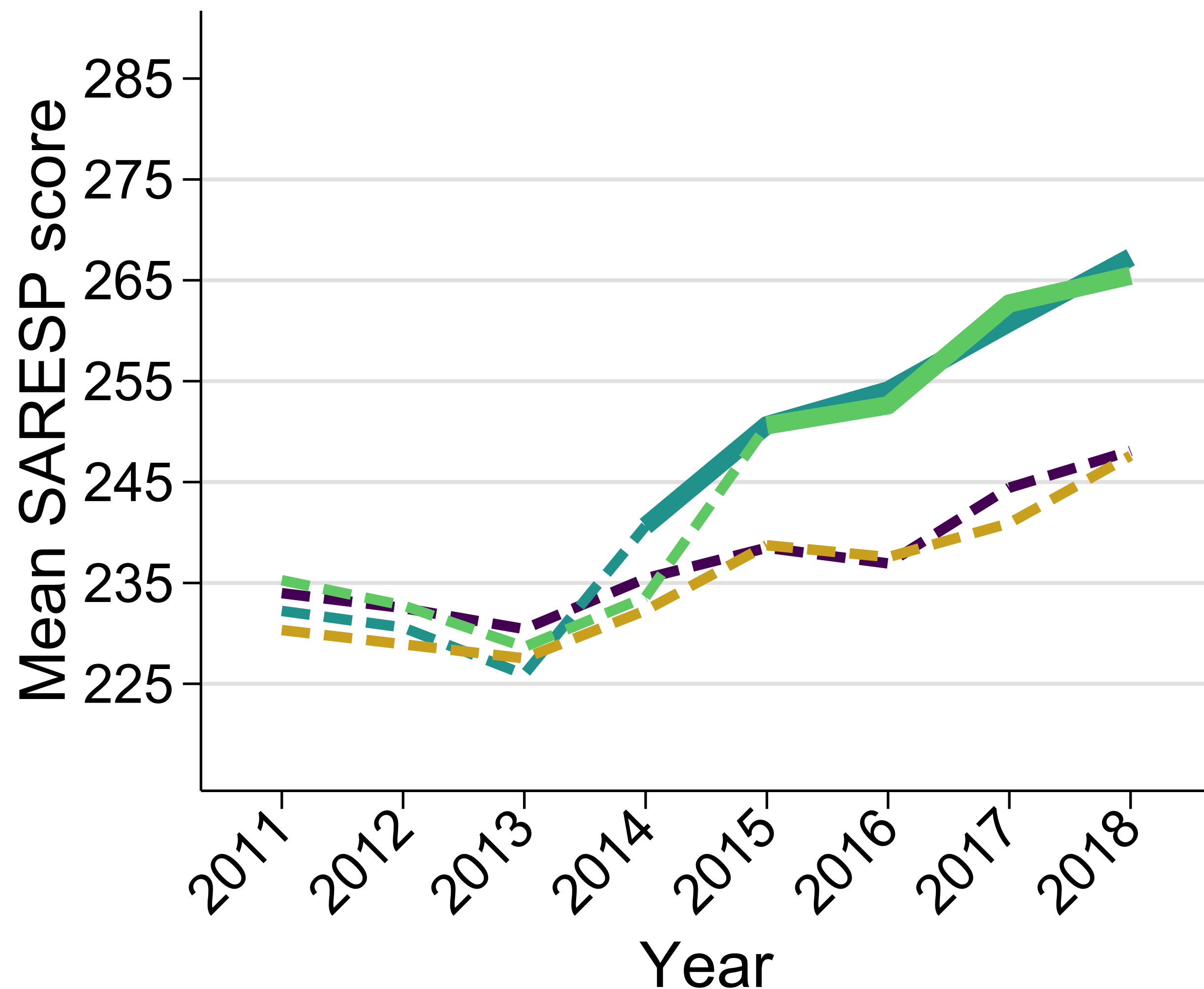
Portuguese Language
