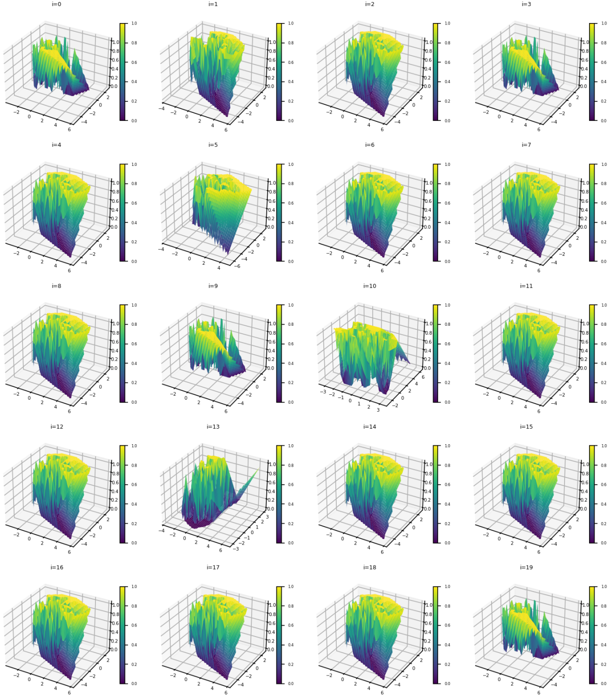
Figure 4 Distribution of data generated based on G2c (SM+SH+SR).
