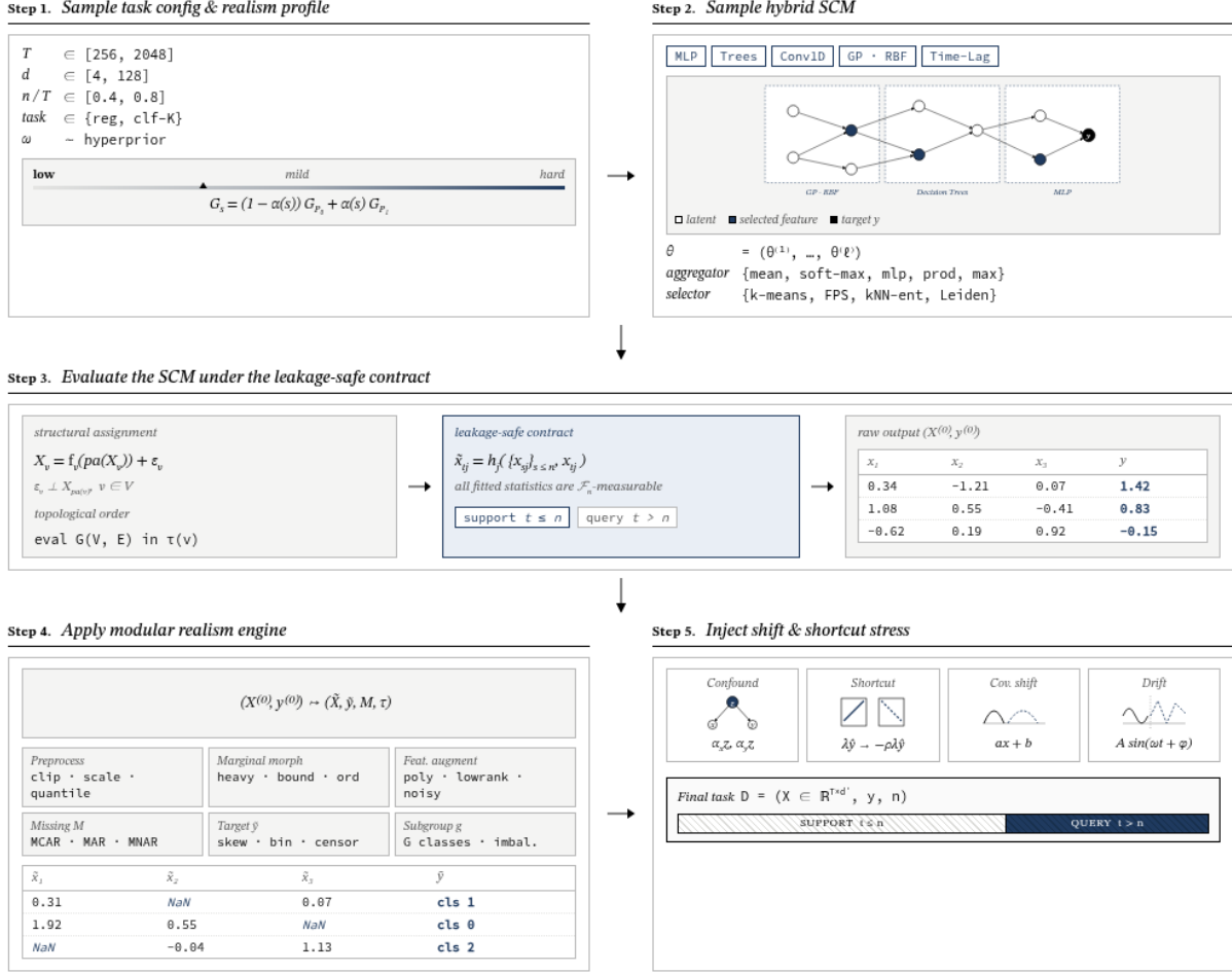
Figure 1 Schematic overview of the O’PRIOR compositional realism prior. (i) Task-level hyperparameters and a curriculum-controlled realism profile P \in \{\text{LOW}, \text{MILD}, \text{HARD}\} are sampled jointly, with curriculum mixing G_s = (1 - \alpha(s))G_{P_0} + \alpha(s)G_{P_1} ; (ii) A Hybrid SCM is sampled by composing base mechanisms from five families—MLPs, decision trees, one-dimensional convolutions, RBF Gaussian processes, and time-lagged VARs—into a single random DAG, with per-node aggregation rules and a diversity-aware feature/target selector drawn jointly; (iii) The DAG is evaluated in topological order under the leakage-safe contract \tilde{x}_{tj} = h_j(\{x_{sj}, s \leq n, x_{tj}\}) , so every fitted statistic is \mathcal{F}_n -measurable; (iv) A modular realism engine maps (X^{(0)}, y^{(0)}) to (\tilde{X}, \tilde{y}, M, \tau) through marginal morphing, feature augmentation, MCAR/MAR/MNAR missingness, target reshaping, and optional subgroup structure; (v) A shift-and-shortcut stress module injects latent confounding, in-support shortcuts that weaken or invert on query rows, affine covariate shift, and seasonal or regime drift, each controlled by independent Bernoulli gates and task-level parameters \omega . The surviving episode is emitted as the final in-context task.
