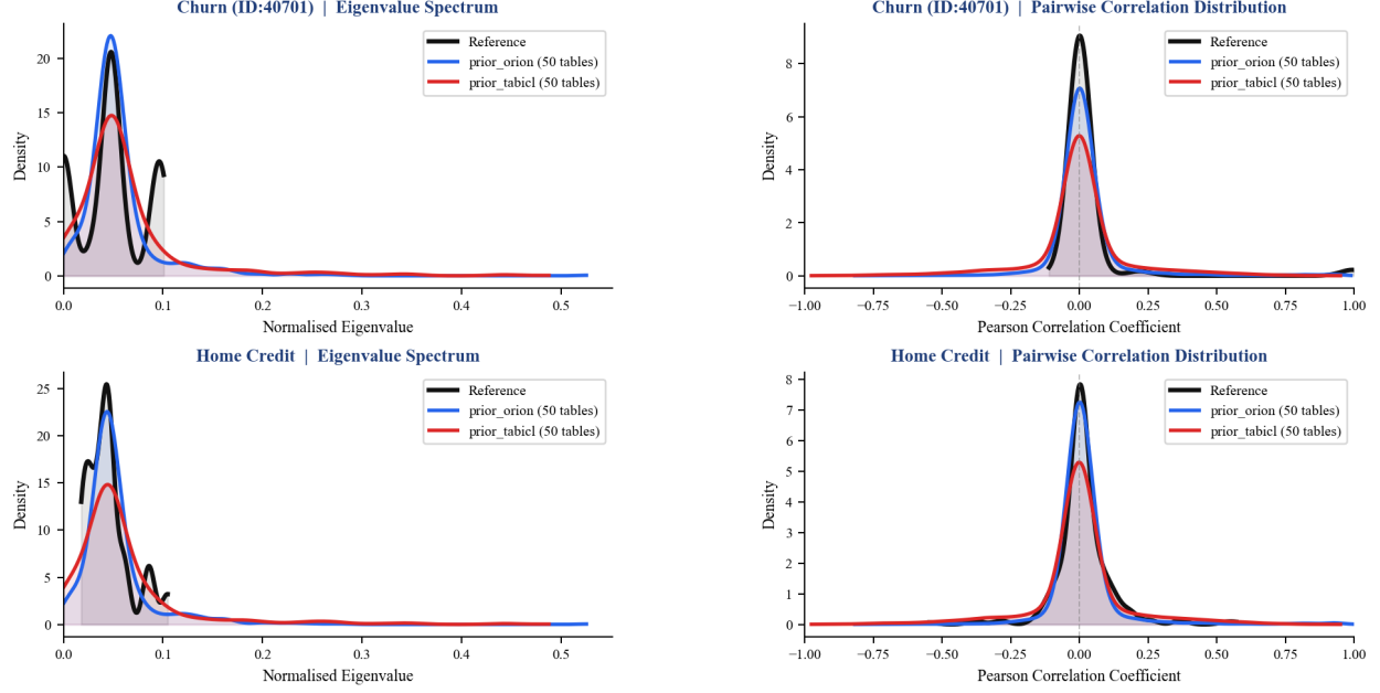
Figure 2 Structural alignment between real reference datasets and synthetic priors. Eigenvalue spectra and pairwise-correlation distributions are aggregated over 50 sampled tables per synthetic source. O’PRIOR better matches the eigenvalue decay and correlation spread of high-dimensional real datasets, while TABICL-v2 produces weaker inter-feature dependence.
