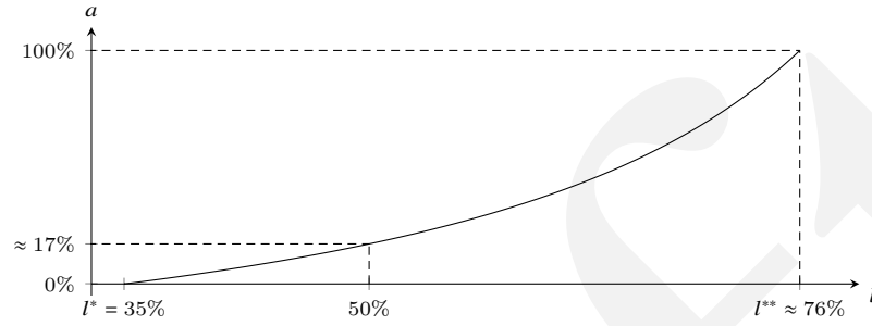
Fig. 6.4: Share a in Prob. 2.11.
