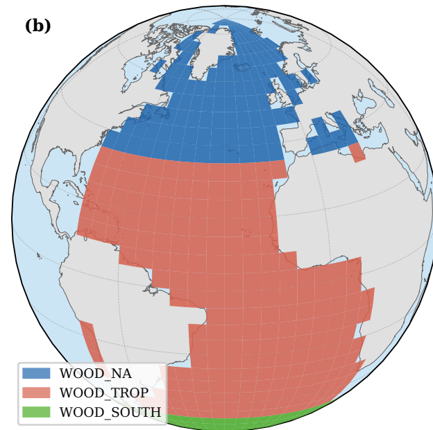
Boussinesq | geographic box areas
