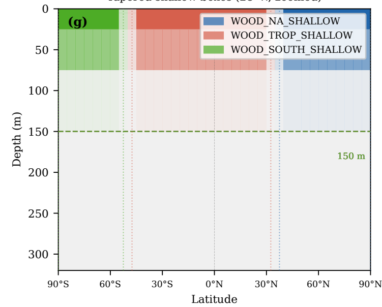
Tapered shallow boxes (28°W, zoomed)
