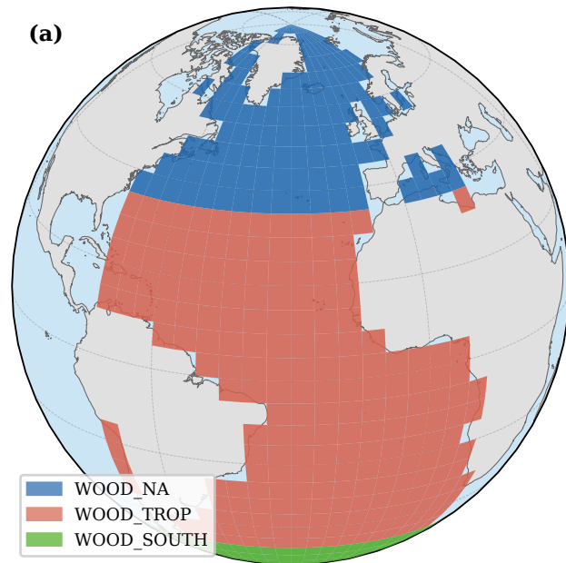
CLIMBER-X | non-tapered boxes
