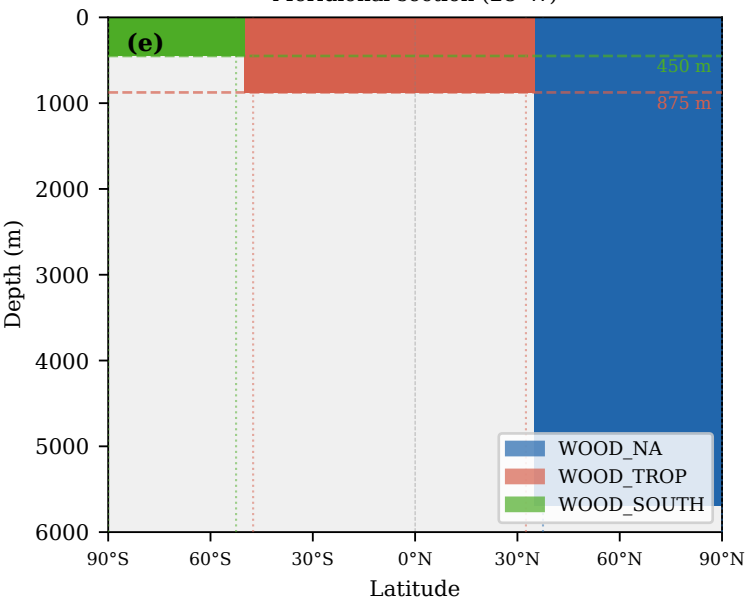
Meridional section (28°W)
