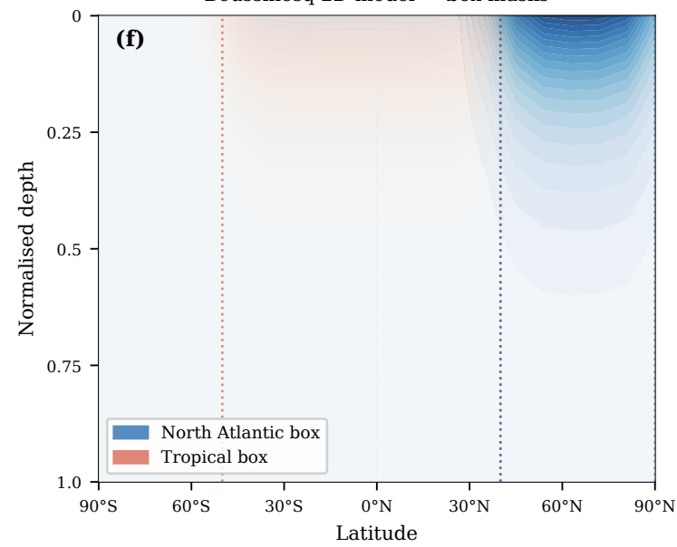
Boussinesq 2D model — box masks
