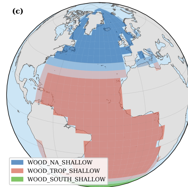
CLIMBER-X | tapered perturbation (5° cells)
