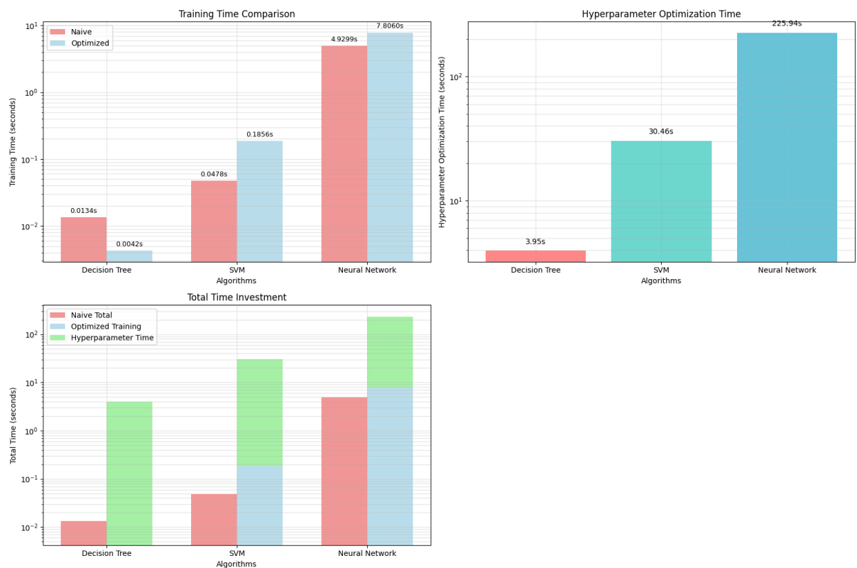
ML Algorithms Timing Performance Analysis - Actual Results (Log Scale)
