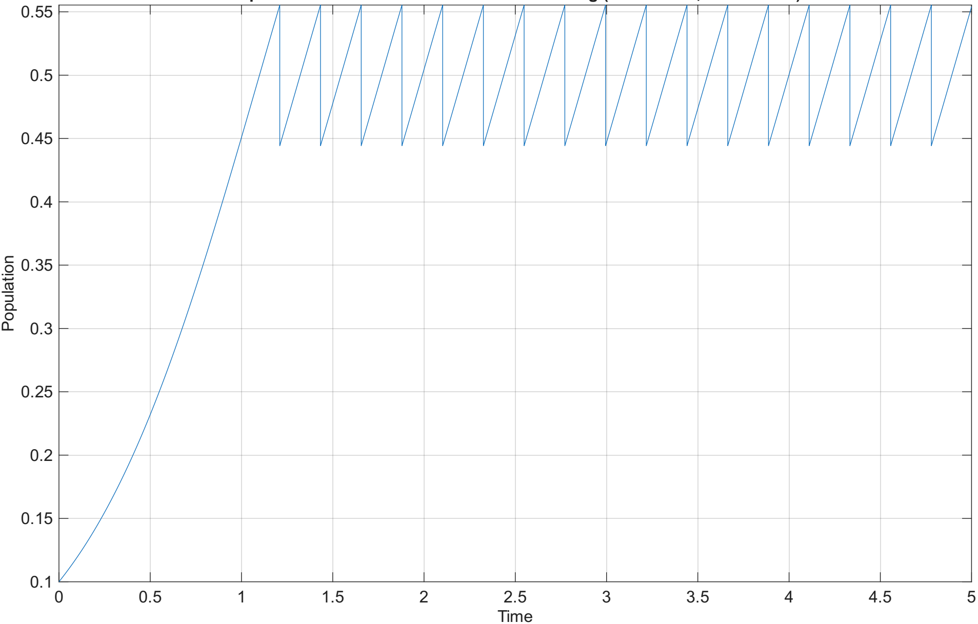
Population over time with threshold harvesting ( T=0.555376 , \alpha=0.200043 )
