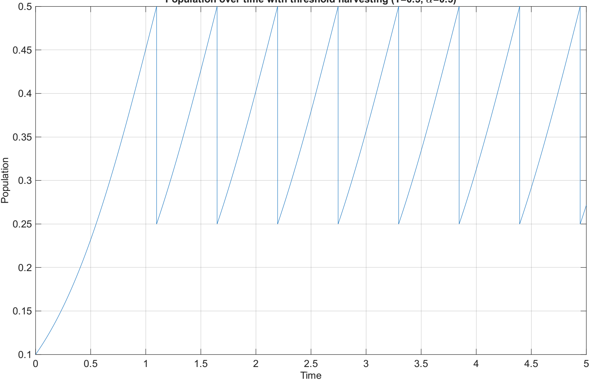
Population over time with threshold harvesting ( T=0.5 , \alpha=0.5 )
