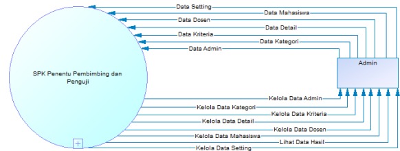
Gambar 1. Context Diagram
