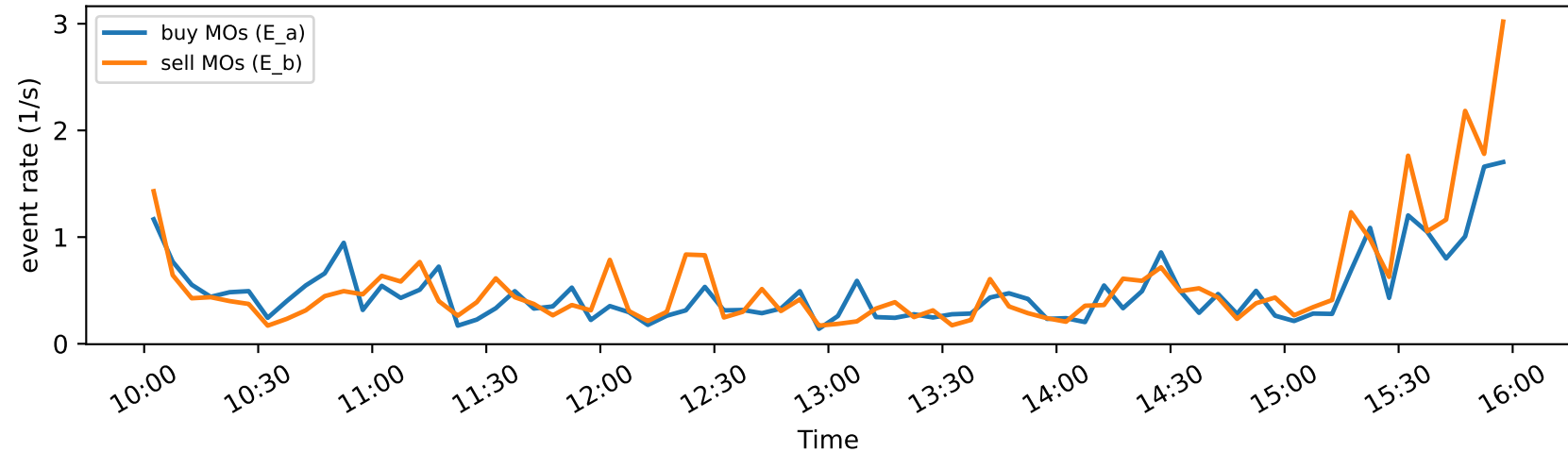
Intraday seasonality: binned event rates (bin=300s)
