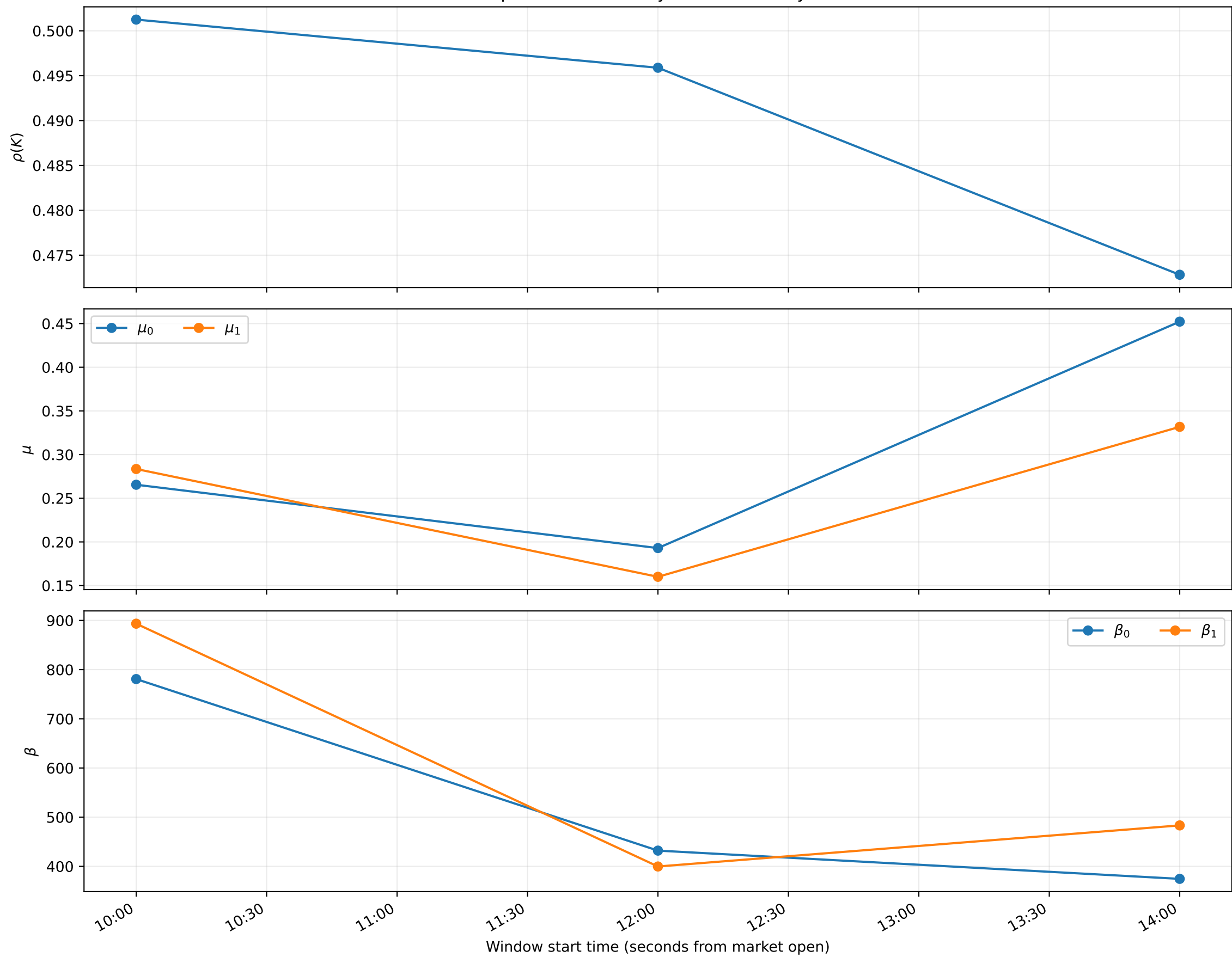
Hawkes parameter stability across intraday windows
