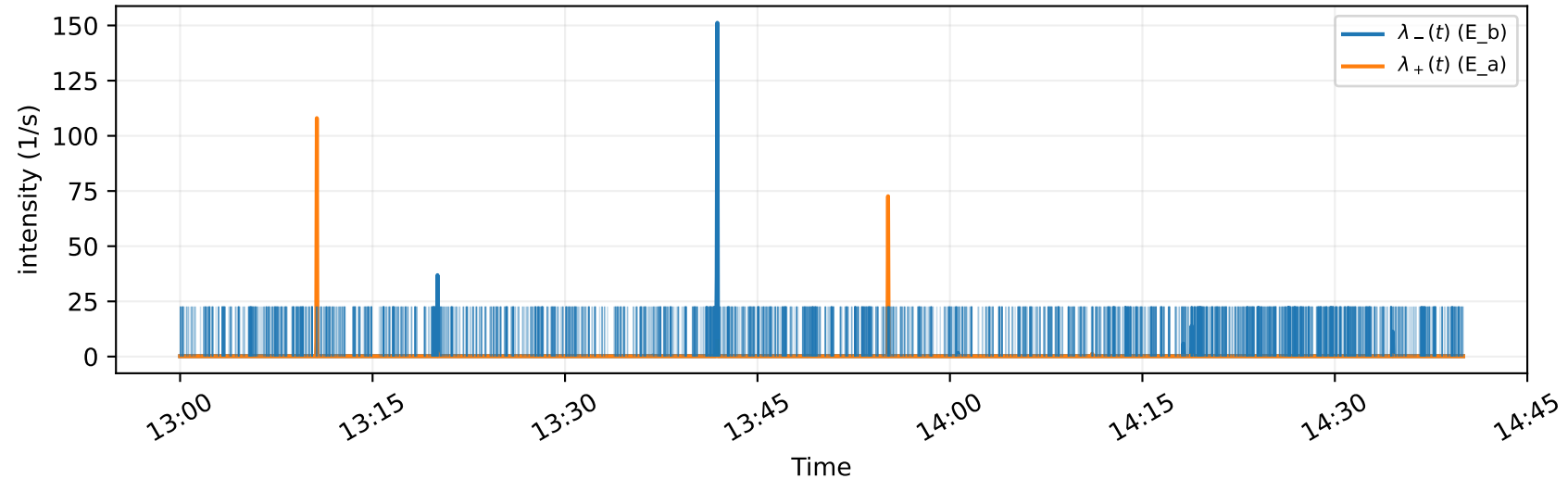
Hawkes intensities on the real episode (with event times)
